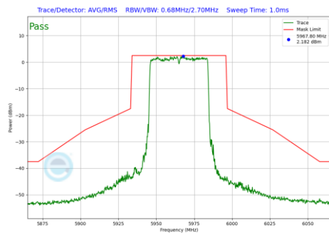
Plot 7-870 In-Band Emission Plot Antenna WF2a (40MHz BW 802.11be(RU) RU484 Index65 (UNII Band 5) - Ch.3)
