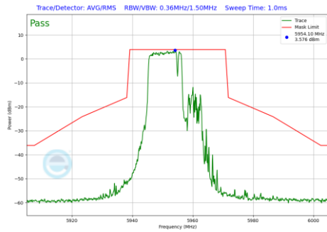
Plot 7-860 In-Band Emission Plot Antenna WF2a (20MHz BW 802.11be(RU) RU106+26 Index82 (UNII Band 5) - Ch.1)
