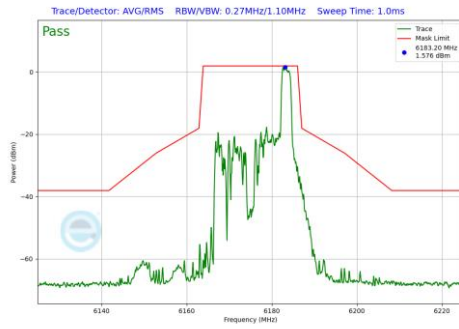
Plot 7-925 In-Band Emission Plot Antenna WF7b (20MHz BW 802.11be(RU) RU26 Index8 (UNII Band 5) - Ch.45)
