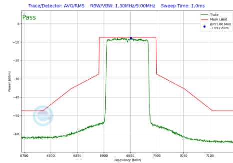
Plot 7-923 In-Band Emission Plot Antenna WF2a (80MHz BW 802.11be(RU) RU996 Index67 (UNII Band 8) - Ch.199)
