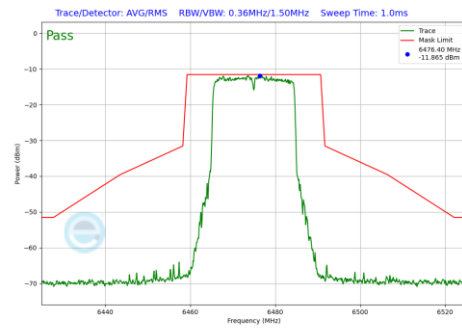
Plot 7-913 In-Band Emission Plot Antenna WF2a (20MHz BW 802.11be(RU) RU242 Index61 (UNII Band 6) - Ch.105)
