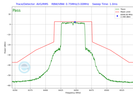
Plot 7-797 In-Band Emission Plot Antenna WF7a (40MHz BW 802.11be(RU) RU484 Index65 (UNII Band 6) - Ch.99)
