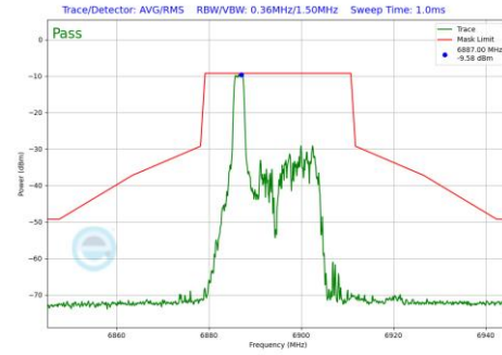
Plot 7-816 In-Band Emission Plot Antenna WF7a (20MHz BW 802.11be(RU) RU26 Index0 (UNII Band 8) - Ch.189)
