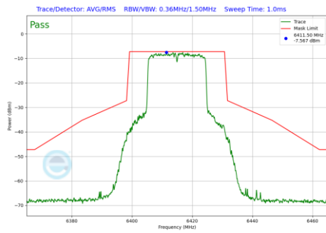
Plot 7-832 In-Band Emission Plot Antenna WF7a (20MHz BW 802.11be(RU) RU242 Index61 (UNII Band 5) - Ch.93)
