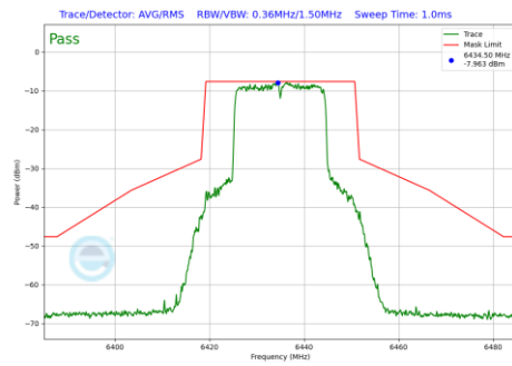
Plot 7-836 In-Band Emission Plot Antenna WF7a (20MHz BW 802.11be(RU) RU242 Index61 (UNII Band 6) - Ch.97)
