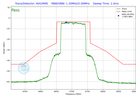
Plot 7-842 In-Band Emission Plot Antenna WF7a (80MHz BW 802.11be(RU) RU996 Index67 (UNII Band 7) - Ch.151)
