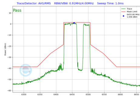
Plot 7-941 In-Band Emission Plot Antenna WF7b (80MHz BW 802.11be(RU) RU484+242 Index92 (UNII Band 6) - Ch.103)
