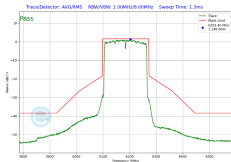
Plot 7-795 In-Band Emission Plot Antenna WF7a (160MHz BW 802.11be(RU) RU996X2 Index68 (UNII Band 5) - Ch.47)
