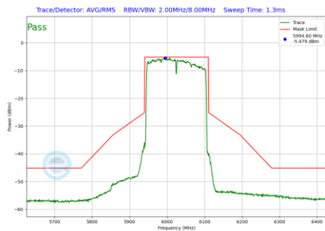
Plot 7-912 In-Band Emission Plot Antenna WF2a (160MHz BW 802.11be(RU) RU996X2 Index68 (UNII Band 5) - Ch.15)
