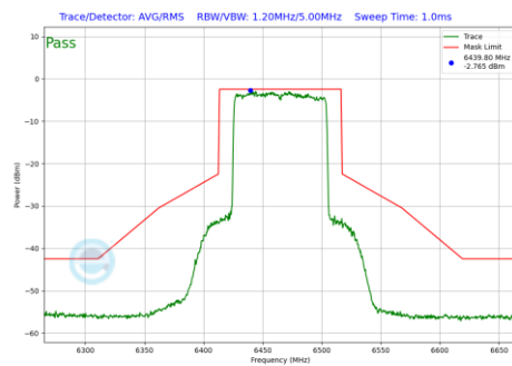
Plot 7-838 In-Band Emission Plot Antenna WF7a (80MHz BW 802.11be(RU) RU996 Index67 (UNII Band 6) - Ch.103)
