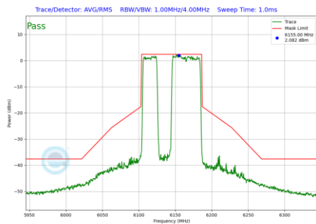
Plot 7-938 In-Band Emission Plot Antenna WF7b (80MHz BW 802.11be(RU) RU484+242 Index91 (UNII Band 5) - Ch.39)
