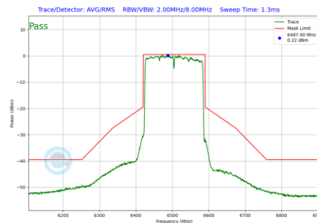
Plot 7-799 In-Band Emission Plot Antenna WF7a (160MHz BW 802.11be(RU) RU996X2 Index68 (UNII Band 6) - Ch.111)
