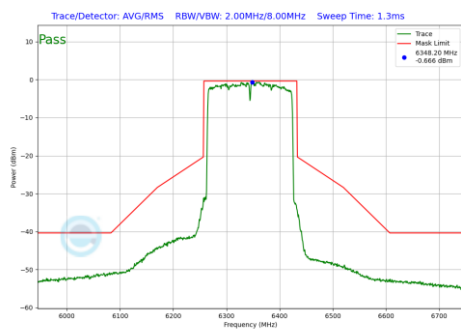
Plot 7-835 In-Band Emission Plot Antenna WF7a (160MHz BW 802.11be(RU) RU996X2 Index68 (UNII Band 5) - Ch.79)
