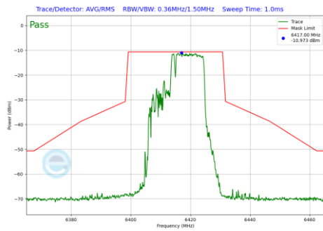
Plot 7-897 In-Band Emission Plot Antenna WF2a (20MHz BW 802.11be(RU) RU106+26 Index83 (UNII Band 5) - Ch.93)
