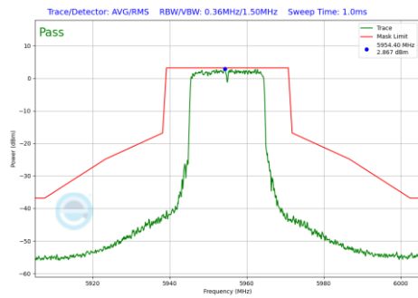
Plot 7-869 In-Band Emission Plot Antenna WF2a (20MHz BW 802.11be(RU) RU242 Index61 (UNII Band 5) - Ch.1)
