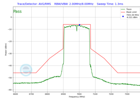
Plot 7-924 In-Band Emission Plot Antenna WF2a (160MHz BW 802.11be(RU) RU996X2 Index68 (UNII Band 8) - Ch.207)
