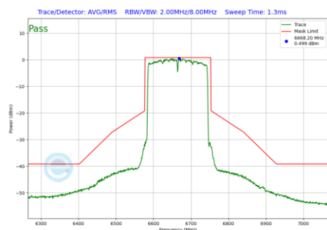
Plot 7-803 In-Band Emission Plot Antenna WF7a (160MHz BW 802.11be(RU) RU996X2 Index68 (UNII Band 7) - Ch.143)
