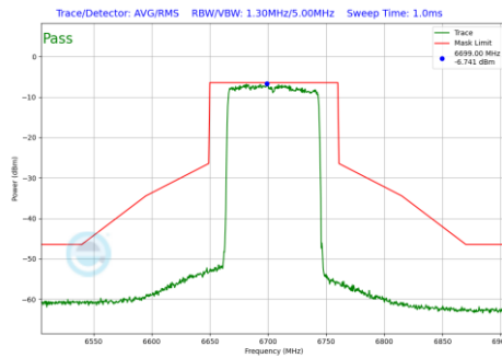
Plot 7-919 In-Band Emission Plot Antenna WF2a (80MHz BW 802.11be(RU) RU996 Index67 (UNII Band 7) - Ch.151)
