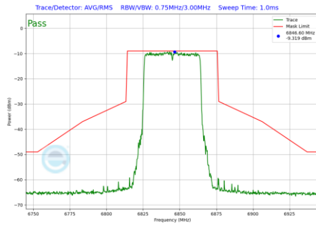
Plot 7-918 In-Band Emission Plot Antenna WF2a (40MHz BW 802.11be(RU) RU484 Index65 (UNII Band 7) - Ch.179)
