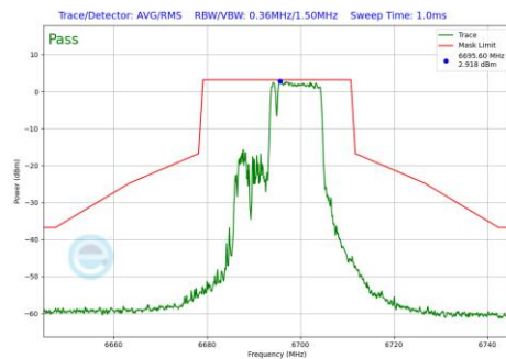
Plot 7-866 In-Band Emission Plot Antenna WF2a (20MHz BW 802.11be(RU) RU106+26 Index83 (UNII Band 7) - Ch.149)
