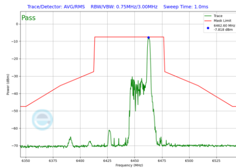
Plot 7-886 In-Band Emission Plot Antenna WF2a (40MHz BW 802.11be(RU) RU26 Index17 (UNII Band 6) - Ch.99)
