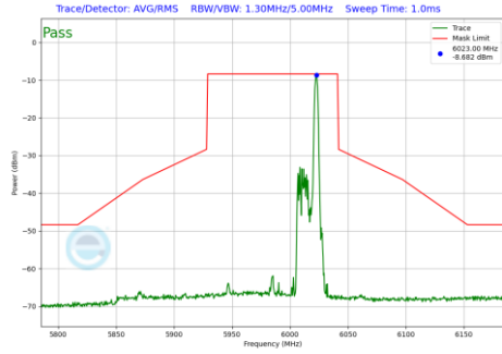
Plot 7-883 In-Band Emission Plot Antenna WF2a (80MHz BW 802.11be(RU) RU26 Index36 (UNII Band 5) - Ch.7)
