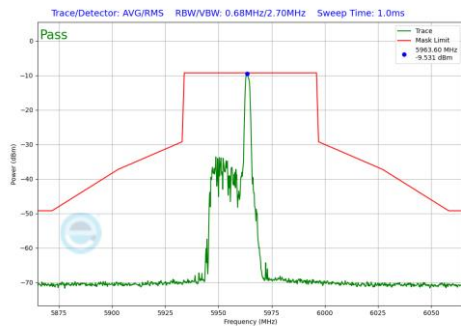
Plot 7-882 In-Band Emission Plot Antenna WF2a (40MHz BW 802.11be(RU) RU26 Index8 (UNII Band 5) - Ch.3)
