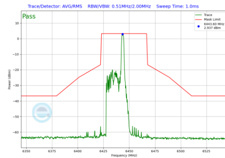
Plot 7-930 In-Band Emission Plot Antenna WF7b (40MHz BW 802.11be(RU) RU26 Index8 (UNII Band 6) - Ch.99)
