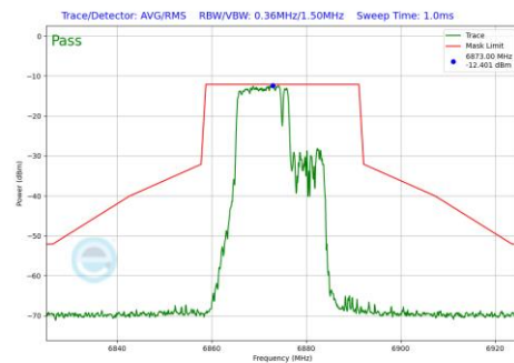
Plot 7-903 In-Band Emission Plot Antenna WF2a (20MHz BW 802.11be(RU) RU106+26 Index82 (UNII Band 7) - Ch.185)
