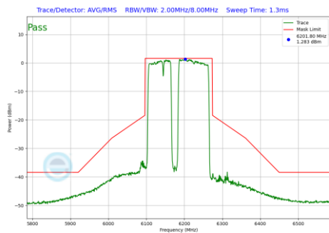
Plot 7-939 In-Band Emission Plot Antenna WF7b (160MHz BW 802.11be(RU) RU996+484+242 Index99 (UNII Band 5) - Ch.47)
