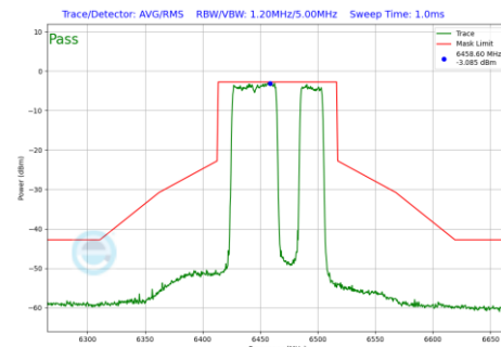
Plot 7-824 In-Band Emission Plot Antenna WF7a (80MHz BW 802.11be(RU) RU484+242 Index92 (UNII Band 6) - Ch.103)
