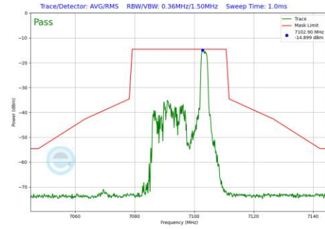
Plot 7-893 In-Band Emission Plot Antenna WF2a (20MHz BW 802.11be(RU) RU26 Index8 (UNII Band 8) - Ch.229)
