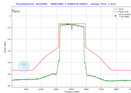
Plot 7-916 In-Band Emission Plot Antenna WF2a (160MHz BW 802.11be(RU) RU996X2 Index68 (UNII Band 6) - Ch.111)
