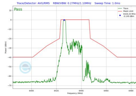
Plot 7-929 In-Band Emission Plot Antenna WF7b (20MHz BW 802.11be(RU) RU26 Index0 (UNII Band 6) - Ch.97)
