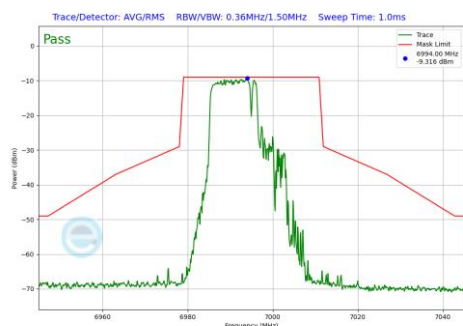
Plot 7-829 In-Band Emission Plot Antenna WF7a (20MHz BW 802.11be(RU) RU106+26 Index82 (UNII Band 8) - Ch.209)
