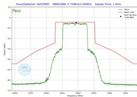
Plot 7-837 In-Band Emission Plot Antenna WF7a (40MHz BW 802.11be(RU) RU484 Index65 (UNII Band 6) - Ch.99)
