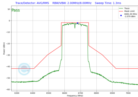
Plot 7-843 In-Band Emission Plot Antenna WF7a (160MHz BW 802.11be(RU) RU996X2 Index68 (UNII Band 7) - Ch.143)
