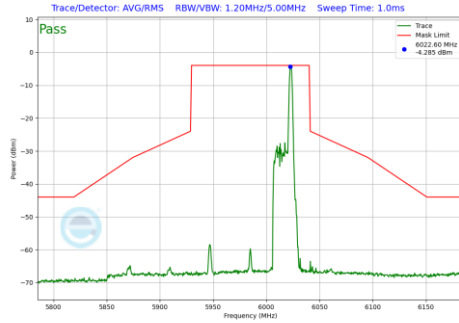
Plot 7-806 In-Band Emission Plot Antenna WF7a (80MHz BW 802.11be(RU) RU26 Index36 (UNII Band 5) - Ch.7)
