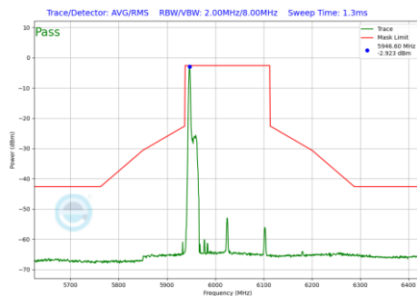
Plot 7-807 In-Band Emission Plot Antenna WF7a (160MHz BW 802.11be(RU) RU26 Index0 (UNII Band 5) - Ch.15)
