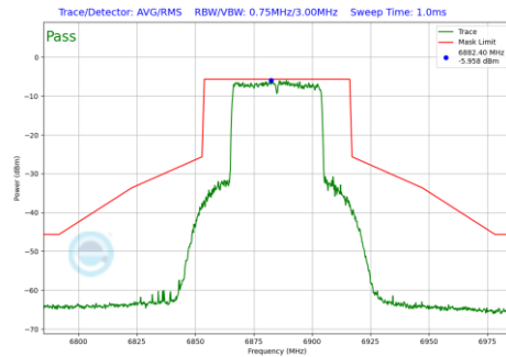
Plot 7-845 In-Band Emission Plot Antenna WF7a (40MHz BW 802.11be(RU) RU484 Index65 (UNII Band 8) - Ch.187)
