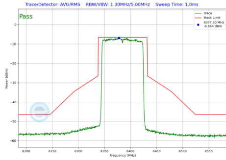
Plot 7-911 In-Band Emission Plot Antenna WF2a (80MHz BW 802.11be(RU) RU996 Index67 (UNII Band 5) - Ch.87)
