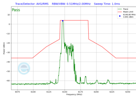
Plot 7-926 In-Band Emission Plot Antenna WF7b (40MHz BW 802.11be(RU) RU26 Index0 (UNII Band 5) - Ch.43)
