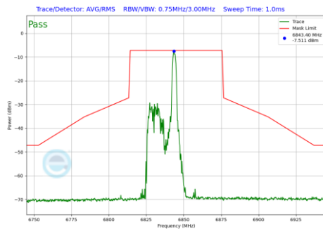
Plot 7-890 In-Band Emission Plot Antenna WF2a (40MHz BW 802.11be(RU) RU26 Index8 (UNII Band 7) - Ch.179)
