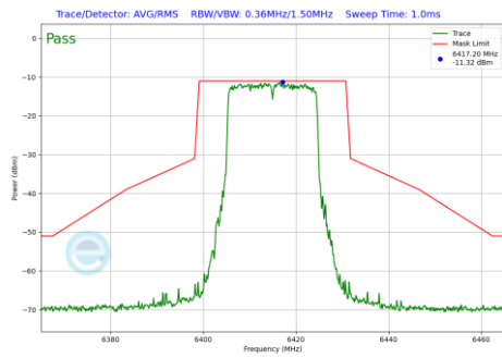
Plot 7-909 In-Band Emission Plot Antenna WF2a (20MHz BW 802.11be(RU) RU242 Index61 (UNII Band 5) - Ch.93)
