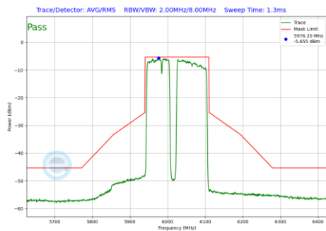
Plot 7-899 In-Band Emission Plot Antenna WF2a (160MHz BW 802.11be(RU) RU996+484+242 Index99 (UNII Band 5) - Ch.15)
