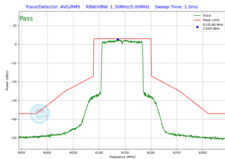
Plot 7-794 In-Band Emission Plot Antenna WF7a (80MHz BW 802.11be(RU) RU996 Index67 (UNII Band 5) - Ch.39)
