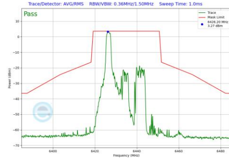
Plot 7-852 In-Band Emission Plot Antenna WF2a (20MHz BW 802.11be(RU) RU26 Index0 (UNII Band 6) - Ch.97)
