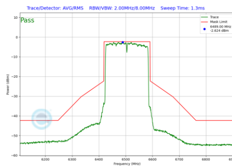
Plot 7-839 In-Band Emission Plot Antenna WF7a (160MHz BW 802.11be(RU) RU996X2 Index68 (UNII Band 6) - Ch.111)
