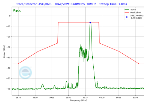
Plot 7-805 In-Band Emission Plot Antenna WF7a (40MHz BW 802.11be(RU) RU26 Index17 (UNII Band 5) - Ch.3)
