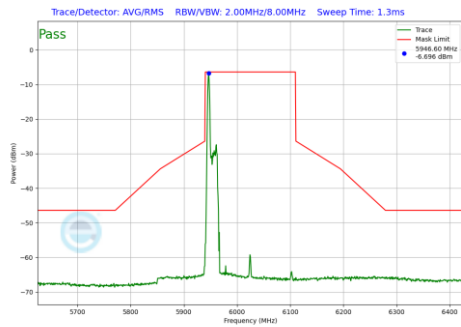
Plot 7-884 In-Band Emission Plot Antenna WF2a (160MHz BW 802.11be(RU) RU26 Index0 (UNII Band 5) - Ch.15)
