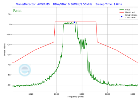
Plot 7-789 In-Band Emission Plot Antenna WF7a (20MHz BW 802.11be(RU) RU106+26 Index82 (UNII Band 7) - Ch.181)
