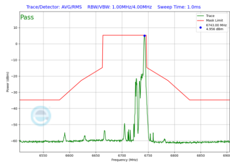
Plot 7-935 In-Band Emission Plot Antenna WF7b (80MHz BW 802.11be(RU) RU26 Index36 (UNII Band 7) - Ch.151)
