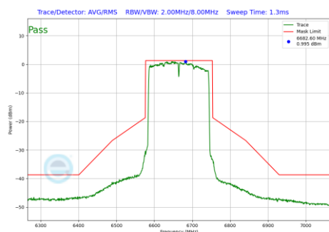
Plot 7-880 In-Band Emission Plot Antenna WF2a (160MHz BW 802.11be(RU) RU996X2 Index68 (UNII Band 7) - Ch.143)
