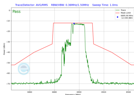
Plot 7-906 In-Band Emission Plot Antenna WF2a (20MHz BW 802.11be(RU) RU106+26 Index83 (UNII Band 8) - Ch.189)
