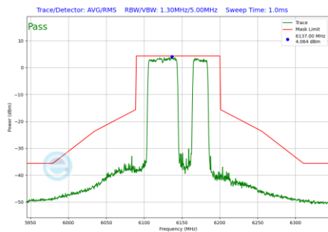
Plot 7-784 In-Band Emission Plot Antenna WF7a (80MHz BW 802.11be(RU) RU484+242 Index92 (UNII Band 5) - Ch.39)
