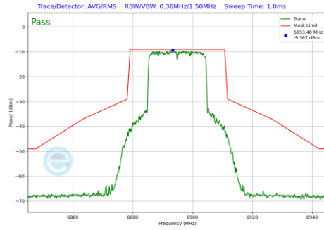
Plot 7-844 In-Band Emission Plot Antenna WF7a (20MHz BW 802.11be(RU) RU242 Index61 (UNII Band 8) - Ch.189)
