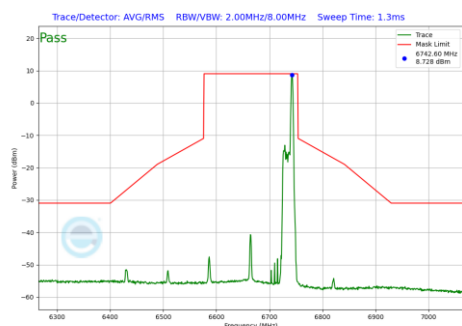
Plot 7-859 In-Band Emission Plot Antenna WF2a (160MHz BW 802.11be(RU) RU26 Index36 (UNII Band 7) - Ch.143)
