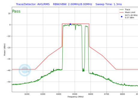
Plot 7-788 In-Band Emission Plot Antenna WF7a (160MHz BW 802.11be(RU) RU996+484+242 Index98 (UNII Band 6) - Ch.111)
