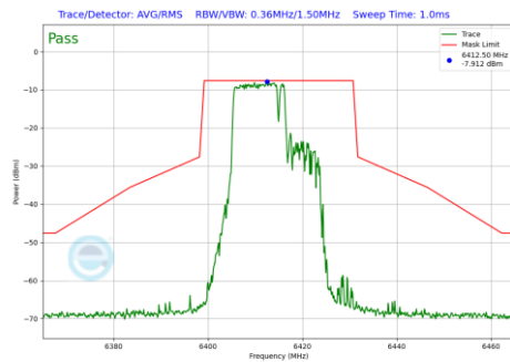
Plot 7-820 In-Band Emission Plot Antenna WF7a (20MHz BW 802.11be(RU) RU106+26 Index82 (UNII Band 5) - Ch.93)
