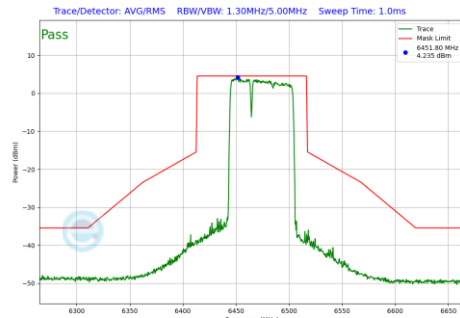
Plot 7-864 In-Band Emission Plot Antenna WF2a (80MHz BW 802.11be(RU) RU484+242 Index90 (UNII Band 6) - Ch.103)
