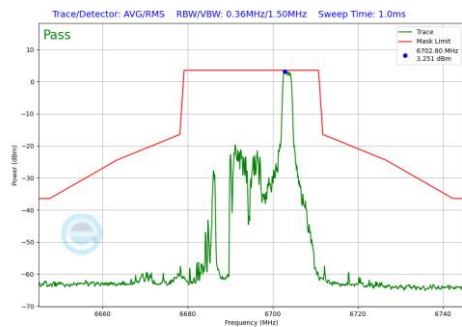
Plot 7-856 In-Band Emission Plot Antenna WF2a (20MHz BW 802.11be(RU) RU26 Index8 (UNII Band 7) - Ch.149)
