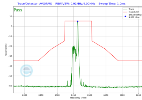
Plot 7-931 In-Band Emission Plot Antenna WF7b (80MHz BW 802.11be(RU) RU26 Index17 (UNII Band 6) - Ch.103)
