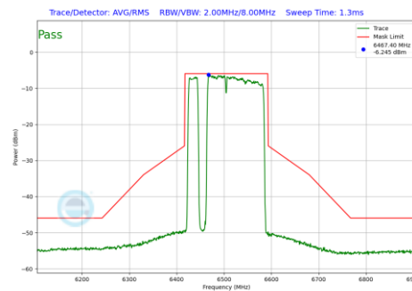
Plot 7-902 In-Band Emission Plot Antenna WF2a (160MHz BW 802.11be(RU) RU996+484+242 Index97 (UNII Band 6) - Ch.111)
