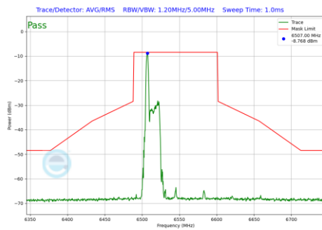
Plot 7-891 In-Band Emission Plot Antenna WF2a (80MHz BW 802.11be(RU) RU26 Index0 (UNII Band 7) - Ch.119)
