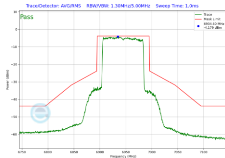
Plot 7-846 In-Band Emission Plot Antenna WF7a (80MHz BW 802.11be(RU) RU996 Index67 (UNII Band 8) - Ch.199)
