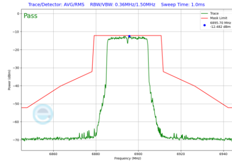
Plot 7-921 In-Band Emission Plot Antenna WF2a (20MHz BW 802.11be(RU) RU242 Index61 (UNII Band 8) - Ch.189)
