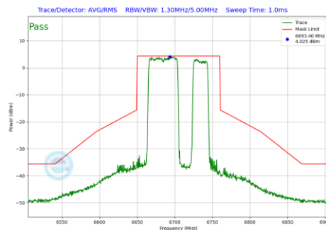
Plot 7-867 In-Band Emission Plot Antenna WF2a (80MHz BW 802.11be(RU) RU484+242 Index92 (UNII Band 7) - Ch.151)
