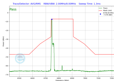
Plot 7-892 In-Band Emission Plot Antenna WF2a (160MHz BW 802.11be(RU) RU26 Index0 (UNII Band 7) - Ch.175)
