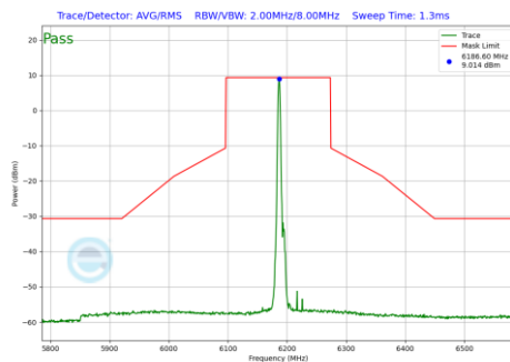
Plot 7-928 In-Band Emission Plot Antenna WF7b (160MHz BW 802.11be(RU) RU26 Index0 (UNII Band 5) - Ch.47)
