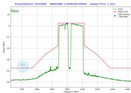
Plot 7-862 In-Band Emission Plot Antenna WF2a (160MHz BW 802.11be(RU) RU996+484+242 Index99 (UNII Band 5) - Ch.15)
