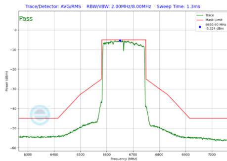
Plot 7-920 In-Band Emission Plot Antenna WF2a (160MHz BW 802.11be(RU) RU996X2 Index68 (UNII Band 7) - Ch.143)
