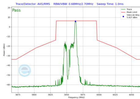
Plot 7-849 In-Band Emission Plot Antenna WF2a (40MHz BW 802.11be(RU) RU26 Index8 (UNII Band 5) - Ch.3)
