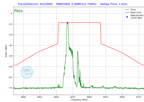
Plot 7-894 In-Band Emission Plot Antenna WF2a (40MHz BW 802.11be(RU) RU26 Index0 (UNII Band 8) - Ch.187)
