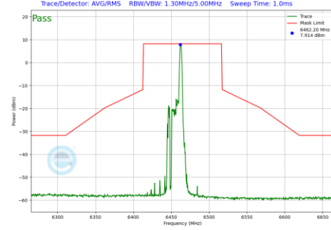
Plot 7-854 In-Band Emission Plot Antenna WF2a (80MHz BW 802.11be(RU) RU26 Index17 (UNII Band 6) - Ch.103)
