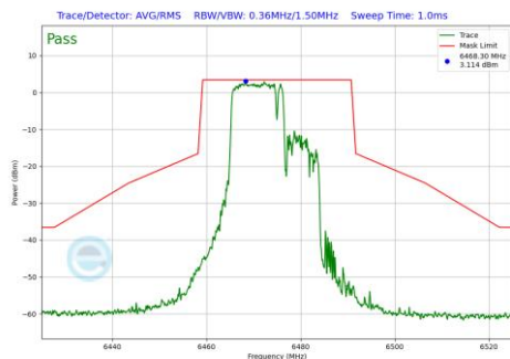
Plot 7-863 In-Band Emission Plot Antenna WF2a (20MHz BW 802.11be(RU) RU106+26 Index82 (UNII Band 6) - Ch.105)
