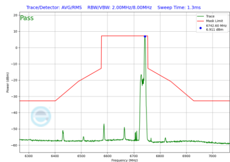
Plot 7-936 In-Band Emission Plot Antenna WF7b (160MHz BW 802.11be(RU) RU26 Index36 (UNII Band 7) - Ch.143)
