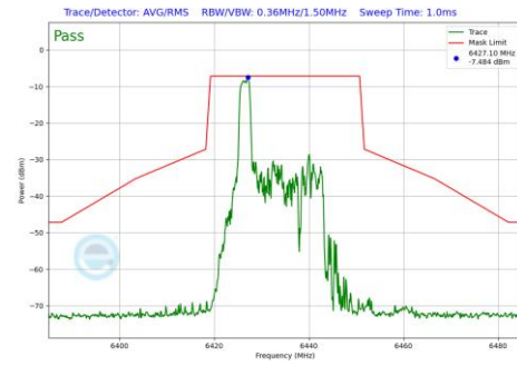
Plot 7-808 In-Band Emission Plot Antenna WF7a (20MHz BW 802.11be(RU) RU26 Index0 (UNII Band 6) - Ch.97)
