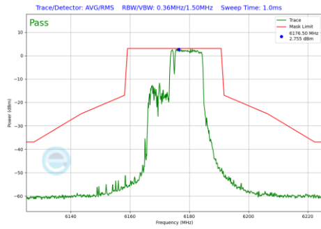
Plot 7-783 In-Band Emission Plot Antenna WF7a (20MHz BW 802.11be(RU) RU106+26 Index83 (UNII Band 5) - Ch.45)
