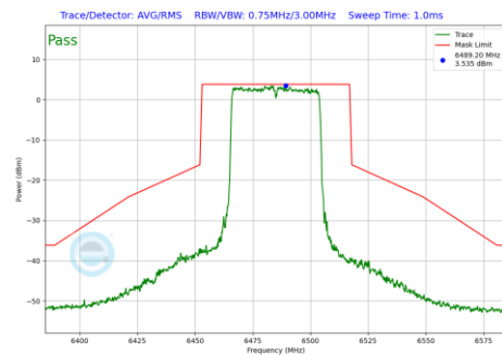
Plot 7-874 In-Band Emission Plot Antenna WF2a (40MHz BW 802.11be(RU) RU484 Index65 (UNII Band 6) - Ch.107)
