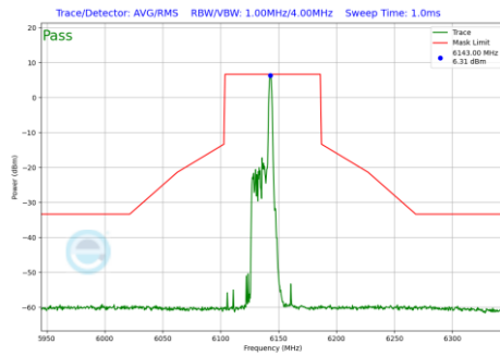
Plot 7-927 In-Band Emission Plot Antenna WF7b (80MHz BW 802.11be(RU) RU26 Index17 (UNII Band 5) - Ch.39)
