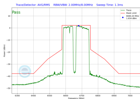
Plot 7-868 In-Band Emission Plot Antenna WF2a (160MHz BW 802.11be(RU) RU996+484+242 Index99 (UNII Band 7) - Ch.143)
