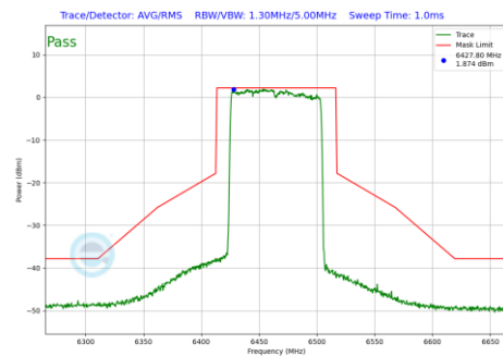
Plot 7-875 In-Band Emission Plot Antenna WF2a (80MHz BW 802.11be(RU) RU996 Index67 (UNII Band 6) - Ch.103)
