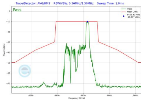
Plot 7-881 In-Band Emission Plot Antenna WF2a (20MHz BW 802.11be(RU) RU26 Index8 (UNII Band 5) - Ch.93)
