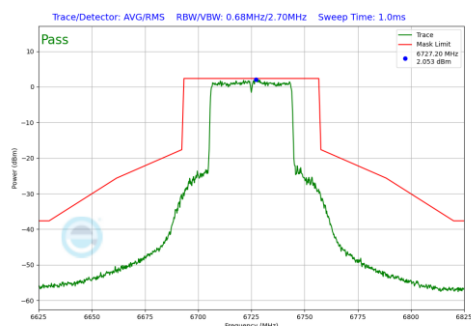
Plot 7-801 In-Band Emission Plot Antenna WF7a (40MHz BW 802.11be(RU) RU484 Index65 (UNII Band 7) - Ch.155)
