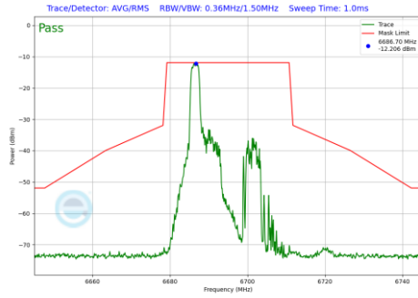
Plot 7-889 In-Band Emission Plot Antenna WF2a (20MHz BW 802.11be(RU) RU26 Index0 (UNII Band 7) - Ch.149)
