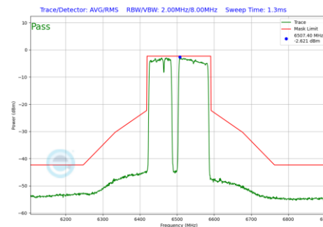
Plot 7-825 In-Band Emission Plot Antenna WF7a (160MHz BW 802.11be(RU) RU996+484+242 Index99 (UNII Band 6) - Ch.111)
