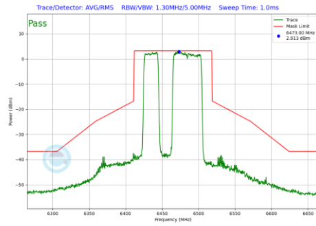
Plot 7-787 In-Band Emission Plot Antenna WF7a (80MHz BW 802.11be(RU) RU484+242 Index91 (UNII Band 6) - Ch.103)
