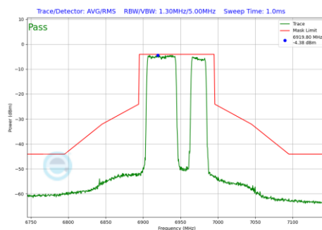
Plot 7-830 In-Band Emission Plot Antenna WF7a (80MHz BW 802.11be(RU) RU484+242 Index92 (UNII Band 8) - Ch.199)
