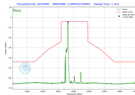
Plot 7-811 In-Band Emission Plot Antenna WF7a (160MHz BW 802.11be(RU) RU26 Index17 (UNII Band 6) - Ch.111)
