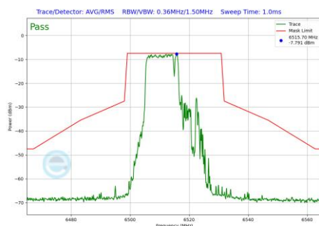
Plot 7-823 In-Band Emission Plot Antenna WF7a (20MHz BW 802.11be(RU) RU106+26 Index82 (UNII Band 6) - Ch.113)
