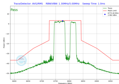
Plot 7-790 In-Band Emission Plot Antenna WF7a (80MHz BW 802.11be(RU) RU484+242 Index92 (UNII Band 7) - Ch.167)
