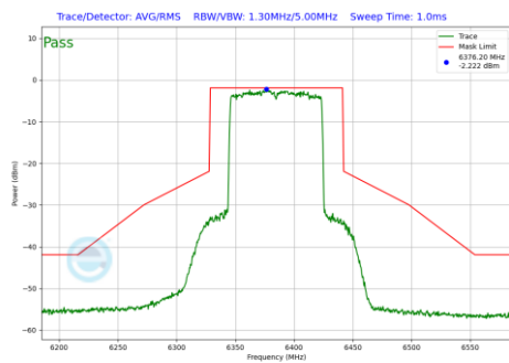
Plot 7-834 In-Band Emission Plot Antenna WF7a (80MHz BW 802.11be(RU) RU996 Index67 (UNII Band 5) - Ch.87)
