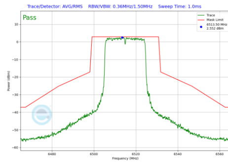
Plot 7-873 In-Band Emission Plot Antenna WF2a (20MHz BW 802.11be(RU) RU242 Index61 (UNII Band 6) - Ch.113)
