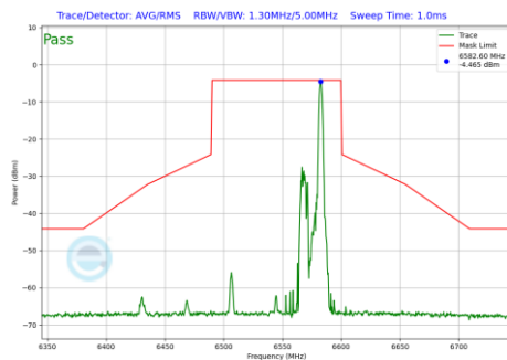
Plot 7-814 In-Band Emission Plot Antenna WF7a (80MHz BW 802.11be(RU) RU26 Index36 (UNII Band 7) - Ch.119)
