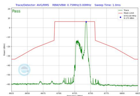
Plot 7-857 In-Band Emission Plot Antenna WF2a (40MHz BW 802.11be(RU) RU26 Index17 (UNII Band 7) - Ch.155)
