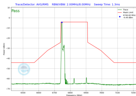
Plot 7-815 In-Band Emission Plot Antenna WF7a (160MHz BW 802.11be(RU) RU26 Index0 (UNII Band 7) - Ch.175)
