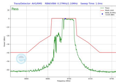
Plot 7-943 In-Band Emission Plot Antenna WF7b (20MHz BW 802.11be(RU) RU106+26 Index83 (UNII Band 7) - Ch.149)
