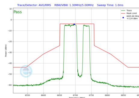
Plot 7-827 In-Band Emission Plot Antenna WF7a (80MHz BW 802.11be(RU) RU484+242 Index92 (UNII Band 7) - Ch.151)
