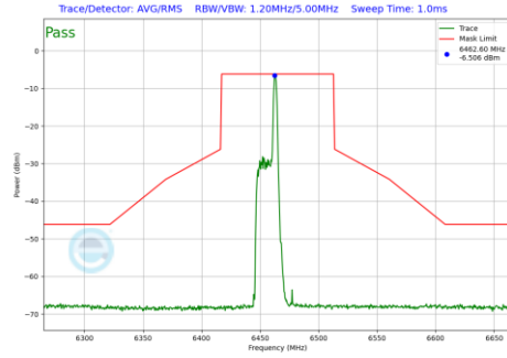
Plot 7-887 In-Band Emission Plot Antenna WF2a (80MHz BW 802.11be(RU) RU26 Index17 (UNII Band 6) - Ch.103)
