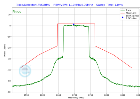
Plot 7-802 In-Band Emission Plot Antenna WF7a (80MHz BW 802.11be(RU) RU996 Index67 (UNII Band 7) - Ch.151)
