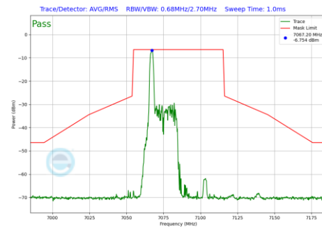
Plot 7-817 In-Band Emission Plot Antenna WF7a (40MHz BW 802.11be(RU) RU26 Index0 (UNII Band 8) - Ch.227)
