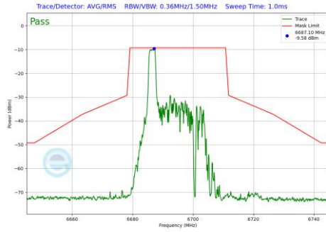
Plot 7-812 In-Band Emission Plot Antenna WF7a (20MHz BW 802.11be(RU) RU26 Index0 (UNII Band 7) - Ch.149)
