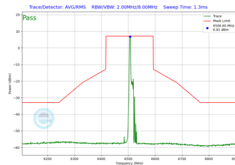
Plot 7-932 In-Band Emission Plot Antenna WF7b (160MHz BW 802.11be(RU) RU26 Index0 (UNII Band 6) - Ch.111)
