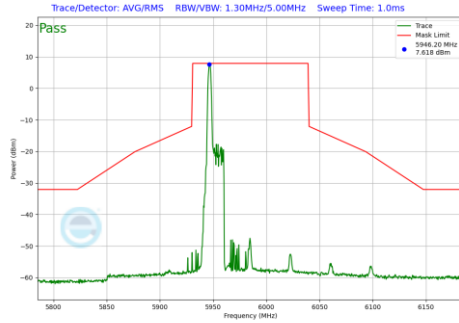
Plot 7-850 In-Band Emission Plot Antenna WF2a (80MHz BW 802.11be(RU) RU26 Index0 (UNII Band 5) - Ch.7)
