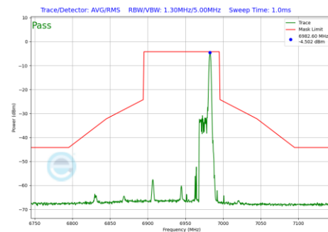
Plot 7-818 In-Band Emission Plot Antenna WF7a (80MHz BW 802.11be(RU) RU26 Index36 (UNII Band 8) - Ch.199)
