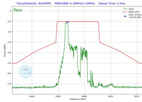
Plot 7-885 In-Band Emission Plot Antenna WF2a (20MHz BW 802.11be(RU) RU26 Index0 (UNII Band 6) - Ch.105)
