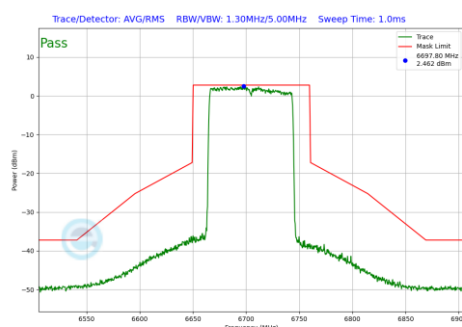
Plot 7-879 In-Band Emission Plot Antenna WF2a (80MHz BW 802.11be(RU) RU996 Index67 (UNII Band 7) - Ch.151)
