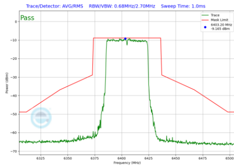
Plot 7-910 In-Band Emission Plot Antenna WF2a (40MHz BW 802.11be(RU) RU484 Index65 (UNII Band 5) - Ch.91)
