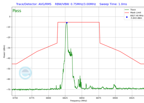
Plot 7-813 In-Band Emission Plot Antenna WF7a (40MHz BW 802.11be(RU) RU26 Index0 (UNII Band 7) - Ch.179)
