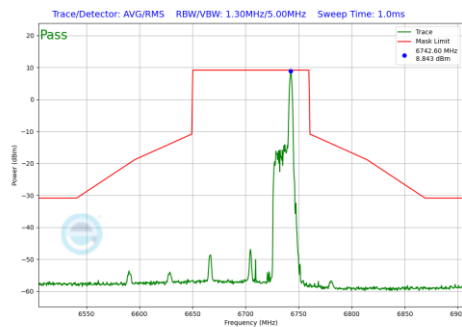
Plot 7-858 In-Band Emission Plot Antenna WF2a (80MHz BW 802.11be(RU) RU26 Index36 (UNII Band 7) - Ch.151)
