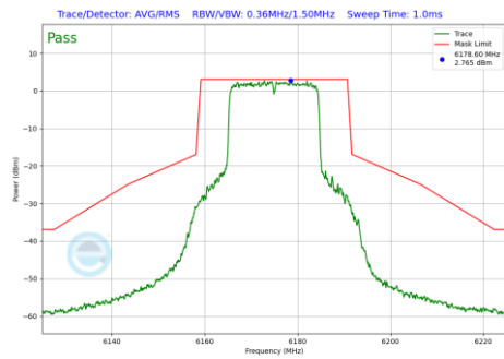
Plot 7-792 In-Band Emission Plot Antenna WF7a (20MHz BW 802.11be(RU) RU242 Index61 (UNII Band 5) - Ch.45)
