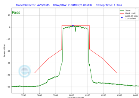
Plot 7-872 In-Band Emission Plot Antenna WF2a (160MHz BW 802.11be(RU) RU996X2 Index68 (UNII Band 5) - Ch.15)
