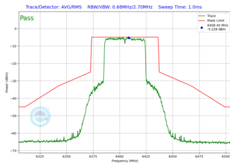
Plot 7-833 In-Band Emission Plot Antenna WF7a (40MHz BW 802.11be(RU) RU484 Index65 (UNII Band 5) - Ch.91)
