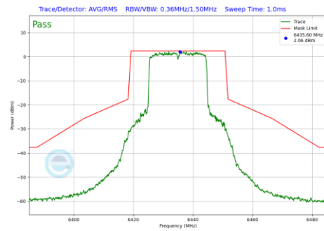
Plot 7-796 In-Band Emission Plot Antenna WF7a (20MHz BW 802.11be(RU) RU242 Index61 (UNII Band 6) - Ch.97)
