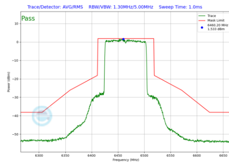
Plot 7-798 In-Band Emission Plot Antenna WF7a (80MHz BW 802.11be(RU) RU996 Index67 (UNII Band 6) - Ch.103)
