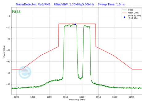
Plot 7-898 In-Band Emission Plot Antenna WF2a (80MHz BW 802.11be(RU) RU484+242 Index92 (UNII Band 5) - Ch.7)
