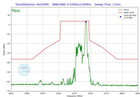
Plot 7-934 In-Band Emission Plot Antenna WF7b (40MHz BW 802.11be(RU) RU26 Index17 (UNII Band 7) - Ch.155)
