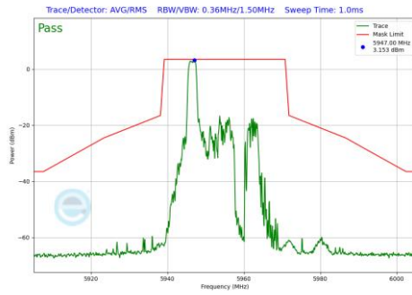
Plot 7-848 In-Band Emission Plot Antenna WF2a (20MHz BW 802.11be(RU) RU26 Index0 (UNII Band 5) - Ch.1)
