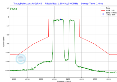
Plot 7-821 In-Band Emission Plot Antenna WF7a (80MHz BW 802.11be(RU) RU484+242 Index92 (UNII Band 5) - Ch.87)
