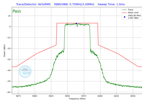
Plot 7-793 In-Band Emission Plot Antenna WF7a (40MHz BW 802.11be(RU) RU484 Index65 (UNII Band 5) - Ch.3)
