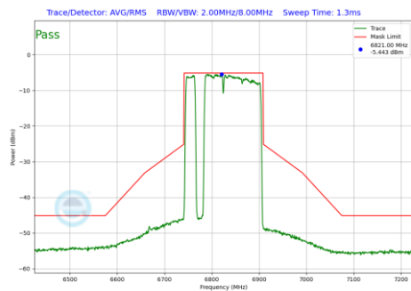
Plot 7-905 In-Band Emission Plot Antenna WF2a (160MHz BW 802.11be(RU) RU996+484+242 Index97 (UNII Band 7) - Ch.175)
