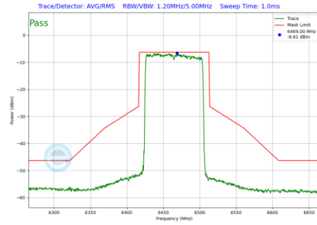
Plot 7-915 In-Band Emission Plot Antenna WF2a (80MHz BW 802.11be(RU) RU996 Index67 (UNII Band 6) - Ch.103)
