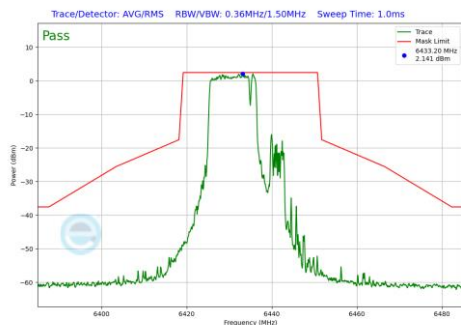
Plot 7-786 In-Band Emission Plot Antenna WF7a (20MHz BW 802.11be(RU) RU106+26 Index82 (UNII Band 6) - Ch.97)
