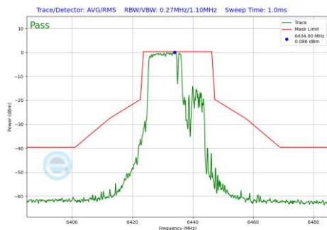
Plot 7-940 In-Band Emission Plot Antenna WF7b (20MHz BW 802.11be(RU) RU106+26 Index82 (UNII Band 6) - Ch.97)
