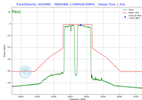
Plot 7-822 In-Band Emission Plot Antenna WF7a (160MHz BW 802.11be(RU) RU996+484+242 Index99 (UNII Band 5) - Ch.79)
