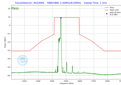
Plot 7-855 In-Band Emission Plot Antenna WF2a (160MHz BW 802.11be(RU) RU26 Index17 (UNII Band 6) - Ch.111)
