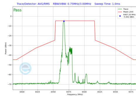
Plot 7-809 In-Band Emission Plot Antenna WF7a (40MHz BW 802.11be(RU) RU26 Index0 (UNII Band 6) - Ch.107)
