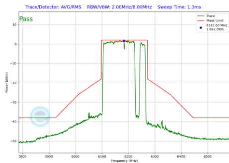
Plot 7-785 In-Band Emission Plot Antenna WF7a (160MHz BW 802.11be(RU) RU996+484+242 Index98 (UNII Band 5) - Ch.47)
