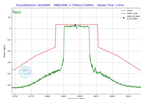
Plot 7-878 In-Band Emission Plot Antenna WF2a (40MHz BW 802.11be(RU) RU484 Index65 (UNII Band 7) - Ch.179)
