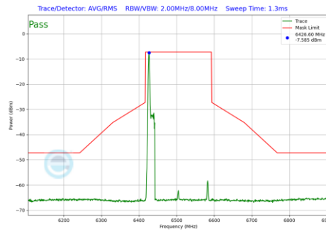
Plot 7-888 In-Band Emission Plot Antenna WF2a (160MHz BW 802.11be(RU) RU26 Index0 (UNII Band 6) - Ch.111)
