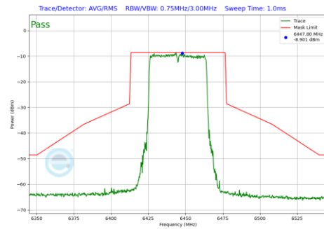
Plot 7-914 In-Band Emission Plot Antenna WF2a (40MHz BW 802.11be(RU) RU484 Index65 (UNII Band 6) - Ch.99)
