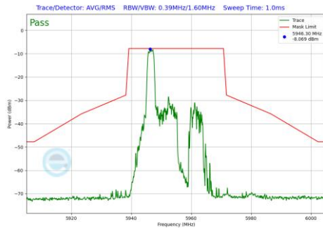
Plot 7-804 In-Band Emission Plot Antenna WF7a (20MHz BW 802.11be(RU) RU26 Index0 (UNII Band 5) - Ch.1)
