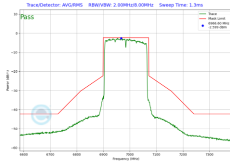
Plot 7-847 In-Band Emission Plot Antenna WF7a (160MHz BW 802.11be(RU) RU996X2 Index68 (UNII Band 8) - Ch.207)
