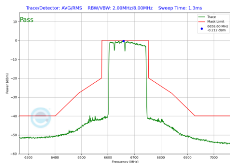
Plot 7-945 In-Band Emission Plot Antenna WF7b (160MHz BW 802.11be(RU) RU996+484+242 Index96 (UNII Band 7) - Ch.143)
