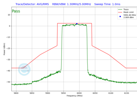
Plot 7-871 In-Band Emission Plot Antenna WF2a (80MHz BW 802.11be(RU) RU996 Index67 (UNII Band 5) - Ch.7)
