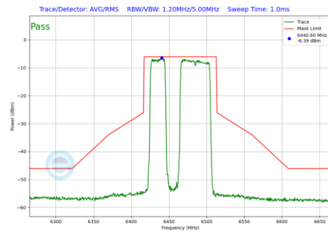
Plot 7-901 In-Band Emission Plot Antenna WF2a (80MHz BW 802.11be(RU) RU484+242 Index91 (UNII Band 6) - Ch.103)
