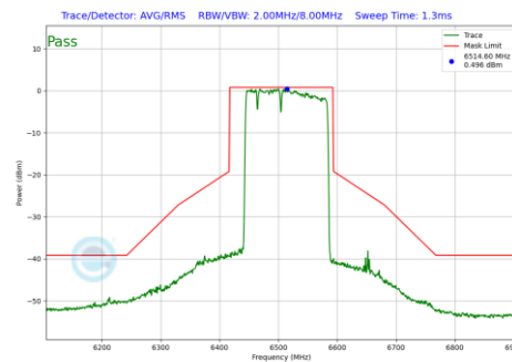
Plot 7-942 In-Band Emission Plot Antenna WF7b (160MHz BW 802.11be(RU) RU996+484+242 Index96 (UNII Band 6) - Ch.111)
