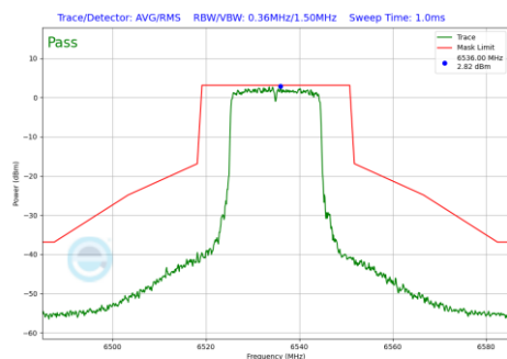
Plot 7-877 In-Band Emission Plot Antenna WF2a (20MHz BW 802.11be(RU) RU242 Index61 (UNII Band 7) - Ch.117)
