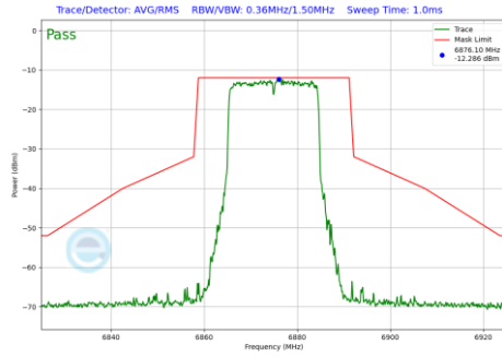
Plot 7-917 In-Band Emission Plot Antenna WF2a (20MHz BW 802.11be(RU) RU242 Index61 (UNII Band 7) - Ch.185)
