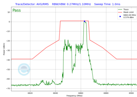
Plot 7-933 In-Band Emission Plot Antenna WF7b (20MHz BW 802.11be(RU) RU26 Index8 (UNII Band 7) - Ch.181)
