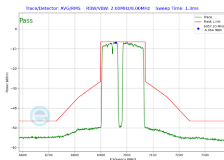
Plot 7-908 In-Band Emission Plot Antenna WF2a (160MHz BW 802.11be(RU) RU996+484+242 Index99 (UNII Band 8) - Ch.207)
