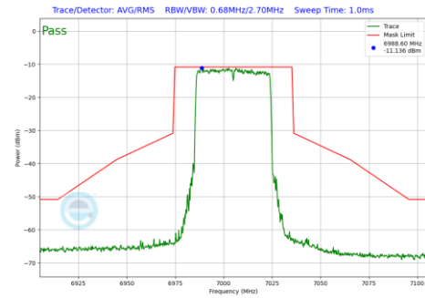
Plot 7-922 In-Band Emission Plot Antenna WF2a (40MHz BW 802.11be(RU) RU484 Index65 (UNII Band 8) - Ch.211)
