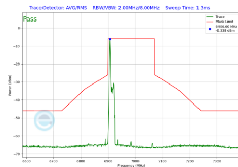
Plot 7-896 In-Band Emission Plot Antenna WF2a (160MHz BW 802.11be(RU) RU26 Index0 (UNII Band 8) - Ch.207)
