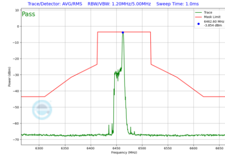
Plot 7-810 In-Band Emission Plot Antenna WF7a (80MHz BW 802.11be(RU) RU26 Index17 (UNII Band 6) - Ch.103)
