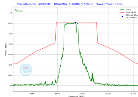
Plot 7-826 In-Band Emission Plot Antenna WF7a (20MHz BW 802.11be(RU) RU106+26 Index82 (UNII Band 7) - Ch.149)
