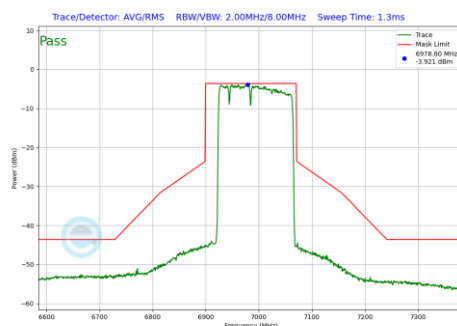
Plot 7-831 In-Band Emission Plot Antenna WF7a (160MHz BW 802.11be(RU) RU996+484+242 Index96 (UNII Band 8) - Ch.207)
