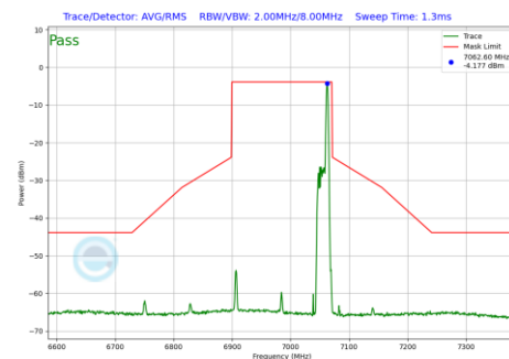
Plot 7-819 In-Band Emission Plot Antenna WF7a (160MHz BW 802.11be(RU) RU26 Index36 (UNII Band 8) - Ch.207)
