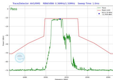
Plot 7-900 In-Band Emission Plot Antenna WF2a (20MHz BW 802.11be(RU) RU106+26 Index82 (UNII Band 6) - Ch.113)
