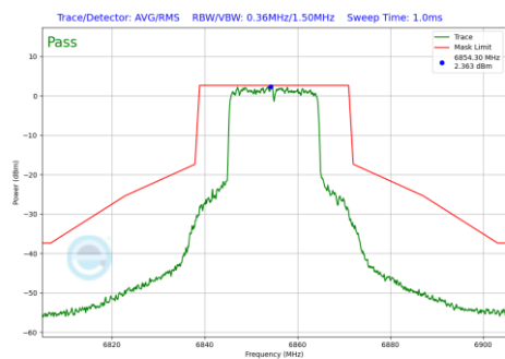
Plot 7-800 In-Band Emission Plot Antenna WF7a (20MHz BW 802.11be(RU) RU242 Index61 (UNII Band 7) - Ch.181)
