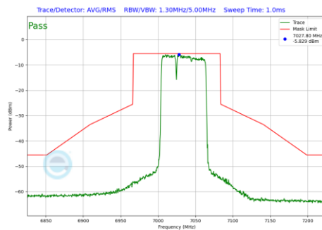
Plot 7-907 In-Band Emission Plot Antenna WF2a (80MHz BW 802.11be(RU) RU484+242 Index90 (UNII Band 8) - Ch.215)
