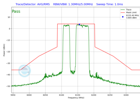
Plot 7-861 In-Band Emission Plot Antenna WF2a (80MHz BW 802.11be(RU) RU484+242 Index91 (UNII Band 5) - Ch.39)
