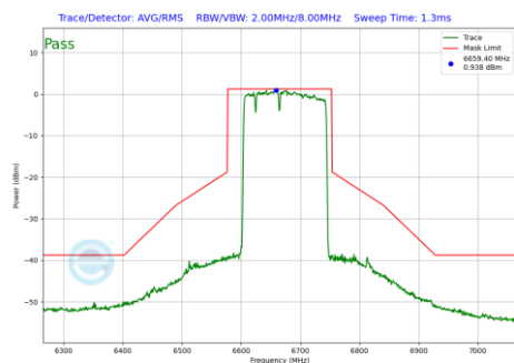
Plot 7-791 In-Band Emission Plot Antenna WF7a (160MHz BW 802.11be(RU) RU996+484+242 Index96 (UNII Band 7) - Ch.143)
