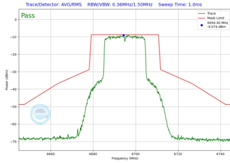
Plot 7-840 In-Band Emission Plot Antenna WF7a (20MHz BW 802.11be(RU) RU242 Index61 (UNII Band 7) - Ch.149)
