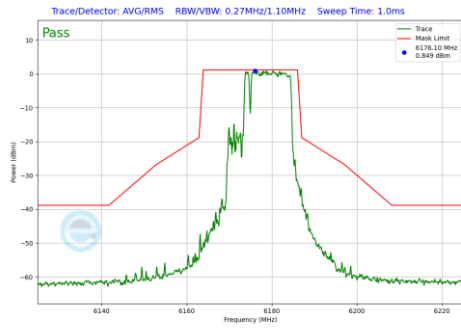
Plot 7-937 In-Band Emission Plot Antenna WF7b (20MHz BW 802.11be(RU) RU106+26 Index83 (UNII Band 5) - Ch.45)
