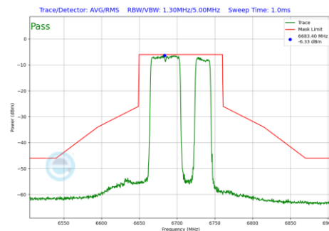
Plot 7-904 In-Band Emission Plot Antenna WF2a (80MHz BW 802.11be(RU) RU484+242 Index92 (UNII Band 7) - Ch.151)
