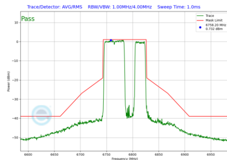
Plot 7-944 In-Band Emission Plot Antenna WF7b (80MHz BW 802.11be(RU) RU484+242 Index92 (UNII Band 7) - Ch.167)
