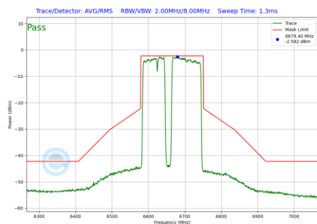
Plot 7-828 In-Band Emission Plot Antenna WF7a (160MHz BW 802.11be(RU) RU996+484+242 Index99 (UNII Band 7) - Ch.143)
