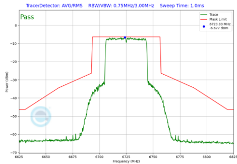
Plot 7-841 In-Band Emission Plot Antenna WF7a (40MHz BW 802.11be(RU) RU484 Index65 (UNII Band 7) - Ch.155)
