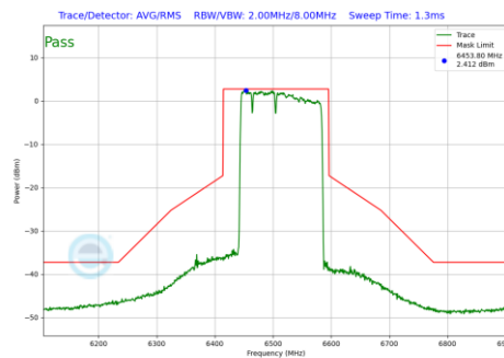
Plot 7-865 In-Band Emission Plot Antenna WF2a (160MHz BW 802.11be(RU) RU996+484+242 Index96 (UNII Band 6) - Ch.111)
