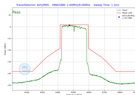
Plot 7-876 In-Band Emission Plot Antenna WF2a (160MHz BW 802.11be(RU) RU996X2 Index68 (UNII Band 6) - Ch.111)
