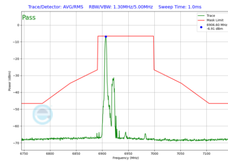
Plot 7-895 In-Band Emission Plot Antenna WF2a (80MHz BW 802.11be(RU) RU26 Index0 (UNII Band 8) - Ch.199)
