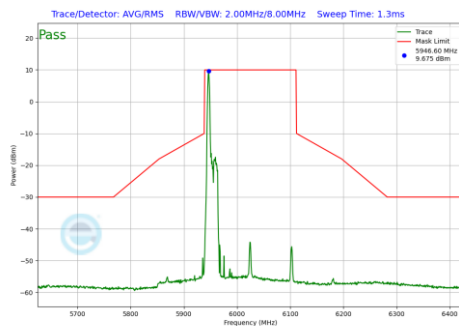
Plot 7-851 In-Band Emission Plot Antenna WF2a (160MHz BW 802.11be(RU) RU26 Index0 (UNII Band 5) - Ch.15)
