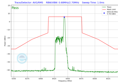
Plot 7-853 In-Band Emission Plot Antenna WF2a (40MHz BW 802.11be(RU) RU26 Index8 (UNII Band 6) - Ch.99)
