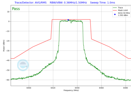
Plot 7-1059 In-Band Emission Plot CDD Primary Antenna WF2a (20MHz BW 802.11be(RU) RU242 Index61 (UNII Band 6) - Ch.97)
