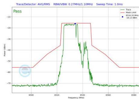
Plot 7-980 In-Band Emission Plot Antenna WF7b (20MHz BW 802.11be(RU) RU106+26 Index82 (UNII Band 7) - Ch.117)
