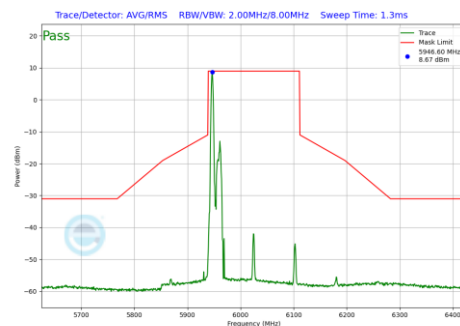
Plot 7-1016 In-Band Emission Plot CDD Primary Antenna WF2a (160MHz BW 802.11be(RU) RU26 Index0 (UNII Band 5) - Ch.15)
