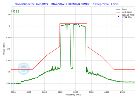
Plot 7-1027 In-Band Emission Plot CDD Primary Antenna WF7a (160MHz BW 802.11be(RU) RU996+484+242 Index99 (UNII Band 5) - Ch.47)
