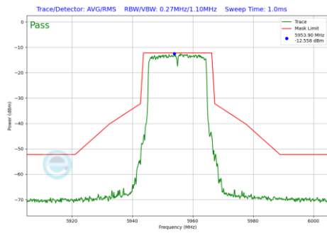
Plot 7-985 In-Band Emission Plot Antenna WF7b (20MHz BW 802.11be(RU) RU242 Index61 (UNII Band 5) - Ch.1)
