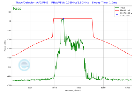
Plot 7-1013 In-Band Emission Plot CDD Primary Antenna WF2a (20MHz BW 802.11be(RU) RU26 Index0 (UNII Band 5) - Ch.1)
