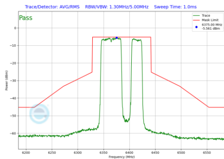
Plot 7-1100 In-Band Emission Plot SDM Primary Antenna WF7a (80MHz BW 802.11be(RU) RU484+242 Index92 (UNII Band 5) - Ch.87)
