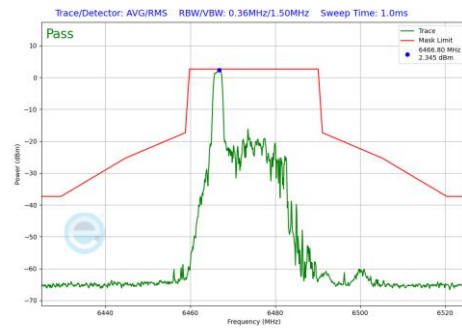
Plot 7-1005 In-Band Emission Plot CDD Primary Antenna WF7a (20MHz BW 802.11be(RU) RU26 Index0 (UNII Band 6) - Ch.105)
