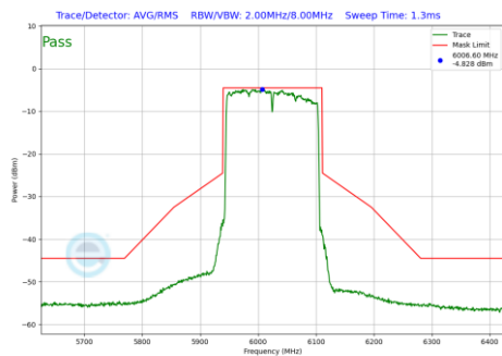
Plot 7-988 In-Band Emission Plot Antenna WF7b (160MHz BW 802.11be(RU) RU996X2 Index68 (UNII Band 5) - Ch.15)
