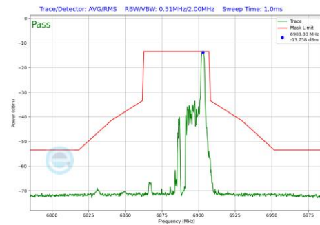
Plot 7-971 In-Band Emission Plot Antenna WF7b (40MHz BW 802.11be(RU) RU26 Index17 (UNII Band 8) - Ch.187)
