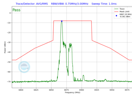
Plot 7-1080 In-Band Emission Plot SDM Primary Antenna WF7a (40MHz BW 802.11be(RU) RU26 Index0 (UNII Band 8) - Ch.187)
