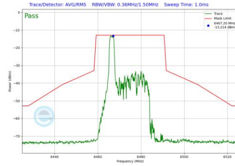
Plot 7-1087 In-Band Emission Plot SDM Primary Antenna WF2a (20MHz BW 802.11be(RU) RU26 Index0 (UNII Band 6) - Ch.105)
