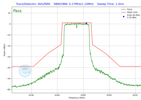
Plot 7-946 In-Band Emission Plot Antenna WF7b (20MHz BW 802.11be(RU) RU242 Index61 (UNII Band 5) - Ch.45)
