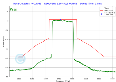
Plot 7-1061 In-Band Emission Plot CDD Primary Antenna WF2a (80MHz BW 802.11be(RU) RU996 Index67 (UNII Band 6) - Ch.103)
