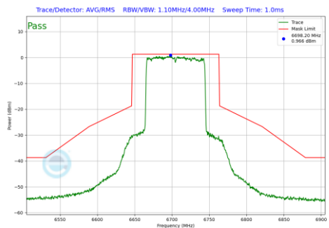
Plot 7-1053 In-Band Emission Plot CDD Primary Antenna WF7a (80MHz BW 802.11be(RU) RU996 Index67 (UNII Band 7) - Ch.151)
