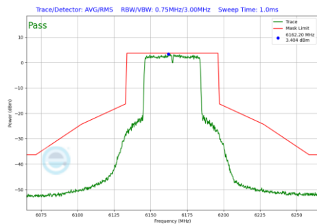
Plot 7-1044 In-Band Emission Plot CDD Primary Antenna WF7a (40MHz BW 802.11be(RU) RU484 Index65 (UNII Band 5) - Ch.43)
