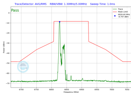
Plot 7-1093 In-Band Emission Plot SDM Primary Antenna WF2a (80MHz BW 802.11be(RU) RU26 Index0 (UNII Band 7) - Ch.183)
