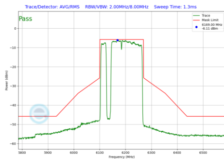
Plot 7-976 In-Band Emission Plot Antenna WF7b (160MHz BW 802.11be(RU) RU996+484+242 Index97 (UNII Band 5) - Ch.47)
