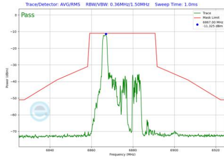
Plot 7-1075 In-Band Emission Plot SDM Primary Antenna WF7a (20MHz BW 802.11be(RU) RU26 Index0 (UNII Band 7) - Ch.185)
