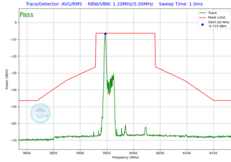
Plot 7-1069 In-Band Emission Plot SDM Primary Antenna WF7a (80MHz BW 802.11be(RU) RU26 Index0 (UNII Band 5) - Ch.7)
