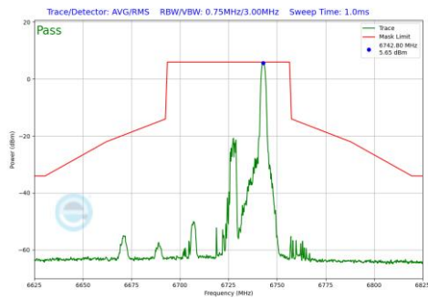
Plot 7-1010 In-Band Emission Plot CDD Primary Antenna WF7a (40MHz BW 802.11be(RU) RU26 Index17 (UNII Band 7) - Ch.155)
