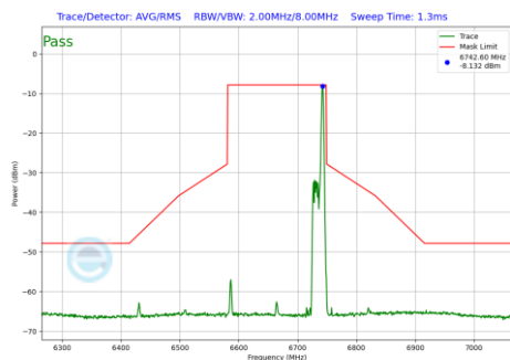
Plot 7-1094 In-Band Emission Plot SDM Primary Antenna WF2a (160MHz BW 802.11be(RU) RU26 Index36 (UNII Band 7) - Ch.143)
