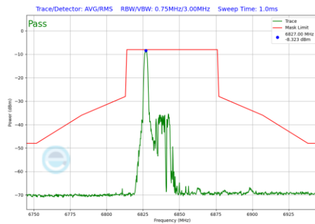
Plot 7-1076 In-Band Emission Plot SDM Primary Antenna WF7a (40MHz BW 802.11be(RU) RU26 Index0 (UNII Band 7) - Ch.179)
