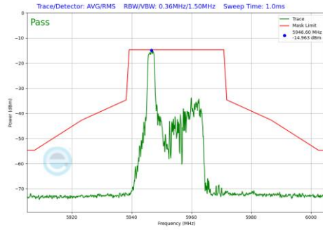
Plot 7-1083 In-Band Emission Plot SDM Primary Antenna WF2a (20MHz BW 802.11be(RU) RU26 Index0 (UNII Band 5) - Ch.1)
