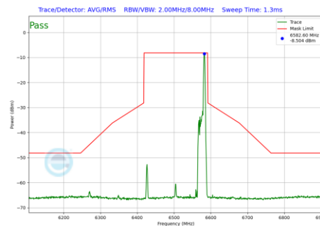
Plot 7-965 In-Band Emission Plot Antenna WF7b (160MHz BW 802.11be(RU) RU26 Index36 (UNII Band 6) - Ch.111)
