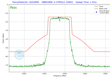
Plot 7-993 In-Band Emission Plot Antenna WF7b (20MHz BW 802.11be(RU) RU242 Index61 (UNII Band 7) - Ch.117)
