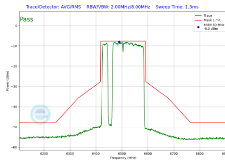
Plot 7-979 In-Band Emission Plot Antenna WF7b (160MHz BW 802.11be(RU) RU996+484+242 Index97 (UNII Band 6) - Ch.111)
