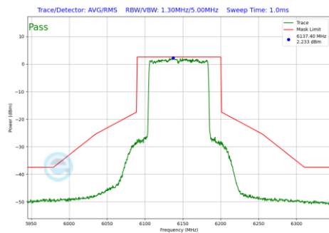
Plot 7-1045 In-Band Emission Plot CDD Primary Antenna WF7a (80MHz BW 802.11be(RU) RU996 Index67 (UNII Band 5) - Ch.39)
