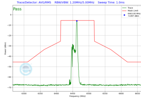
Plot 7-1073 In-Band Emission Plot SDM Primary Antenna WF7a (80MHz BW 802.11be(RU) RU26 Index17 (UNII Band 6) - Ch.103)
