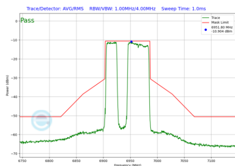
Plot 7-983 In-Band Emission Plot Antenna WF7b (80MHz BW 802.11be(RU) RU484+242 Index91 (UNII Band 8) - Ch.199)
