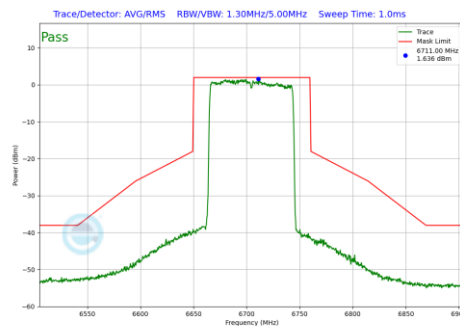
Plot 7-1065 In-Band Emission Plot CDD Primary Antenna WF2a (80MHz BW 802.11be(RU) RU996 Index67 (UNII Band 7) - Ch.151)
