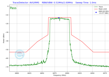
Plot 7-998 In-Band Emission Plot Antenna WF7b (40MHz BW 802.11be(RU) RU484 Index65 (UNII Band 8) - Ch.187)
