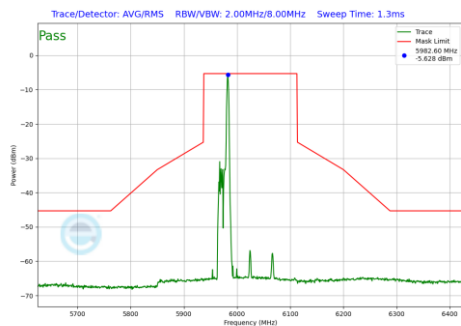
Plot 7-1070 In-Band Emission Plot SDM Primary Antenna WF7a (160MHz BW 802.11be(RU) RU26 Index17 (UNII Band 5) - Ch.15)
