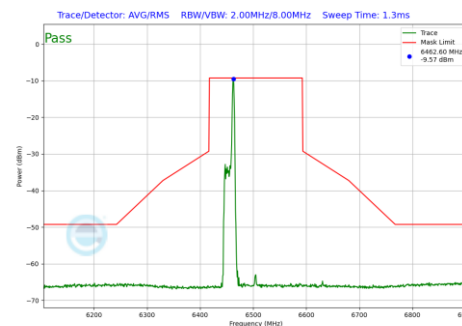
Plot 7-1090 In-Band Emission Plot SDM Primary Antenna WF2a (160MHz BW 802.11be(RU) RU26 Index17 (UNII Band 6) - Ch.111)
