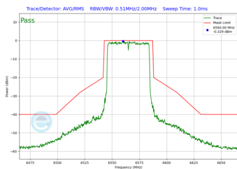
Plot 7-955 In-Band Emission Plot Antenna WF7b (40MHz BW 802.11be(RU) RU484 Index65 (UNII Band 7) - Ch.123)
