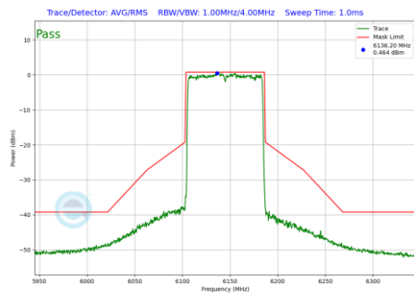
Plot 7-948 In-Band Emission Plot Antenna WF7b (80MHz BW 802.11be(RU) RU996 Index67 (UNII Band 5) - Ch.39)
