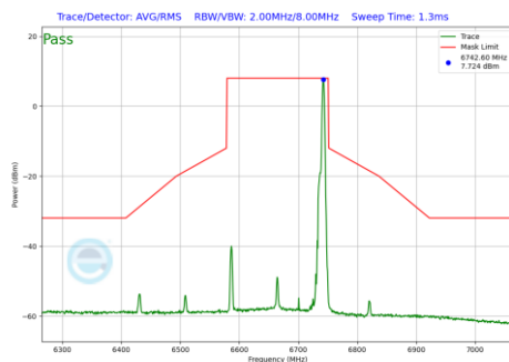
Plot 7-1012 In-Band Emission Plot CDD Primary Antenna WF7a (160MHz BW 802.11be(RU) RU26 Index36 (UNII Band 7) - Ch.143)
