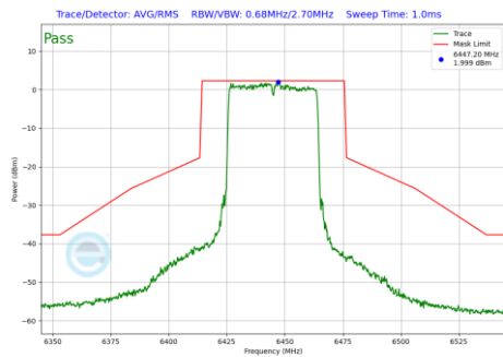
Plot 7-1060 In-Band Emission Plot CDD Primary Antenna WF2a (40MHz BW 802.11be(RU) RU484 Index65 (UNII Band 6) - Ch.99)
