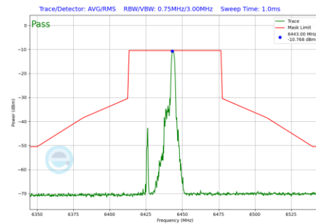
Plot 7-1088 In-Band Emission Plot SDM Primary Antenna WF2a (40MHz BW 802.11be(RU) RU26 Index8 (UNII Band 6) - Ch.99)
