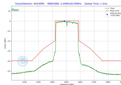
Plot 7-1050 In-Band Emission Plot CDD Primary Antenna WF7a (160MHz BW 802.11be(RU) RU996X2 Index68 (UNII Band 6) - Ch.111)
