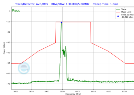
Plot 7-1085 In-Band Emission Plot SDM Primary Antenna WF2a (80MHz BW 802.11be(RU) RU26 Index0 (UNII Band 5) - Ch.7)
