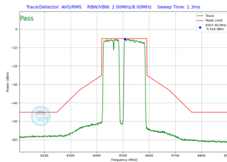
Plot 7-1104 In-Band Emission Plot SDM Primary Antenna WF7a (160MHz BW 802.11be(RU) RU996+484+242 Index99 (UNII Band 6) - Ch.111)
