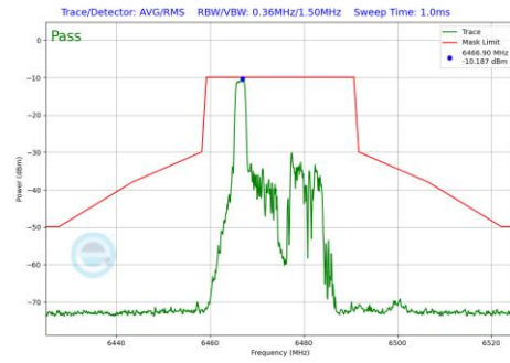
Plot 7-1071 In-Band Emission Plot SDM Primary Antenna WF7a (20MHz BW 802.11be(RU) RU26 Index0 (UNII Band 6) - Ch.105)
