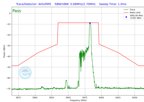
Plot 7-1068 In-Band Emission Plot SDM Primary Antenna WF7a (40MHz BW 802.11be(RU) RU26 Index17 (UNII Band 5) - Ch.3)
