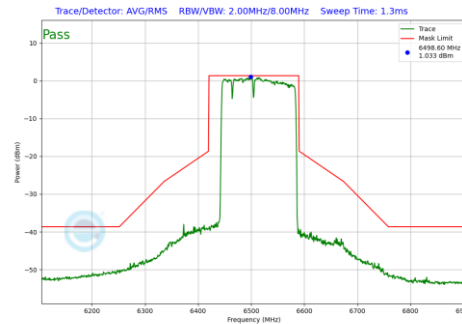
Plot 7-1030 In-Band Emission Plot CDD Primary Antenna WF7a (160MHz BW 802.11be(RU) RU996+484+242 Index96 (UNII Band 6) - Ch.111)
