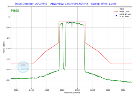
Plot 7-1107 In-Band Emission Plot SDM Primary Antenna WF7a (160MHz BW 802.11be(RU) RU996+484+242 Index97 (UNII Band 7) - Ch.143)
