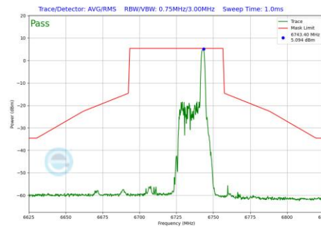
Plot 7-1022 In-Band Emission Plot CDD Primary Antenna WF2a (40MHz BW 802.11be(RU) RU26 Index17 (UNII Band 7) - Ch.155)
