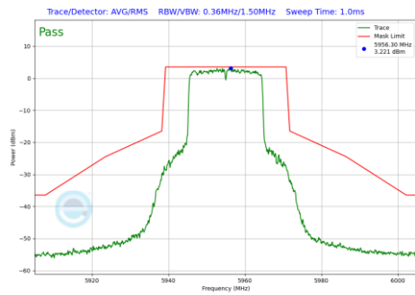
Plot 7-1043 In-Band Emission Plot CDD Primary Antenna WF7a (20MHz BW 802.11be(RU) RU242 Index61 (UNII Band 5) - Ch.1)
