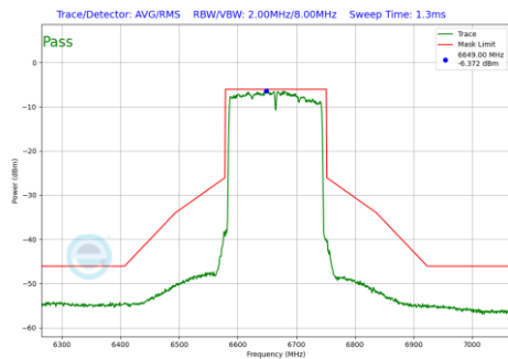
Plot 7-996 In-Band Emission Plot Antenna WF7b (160MHz BW 802.11be(RU) RU996X2 Index68 (UNII Band 7) - Ch.143)
