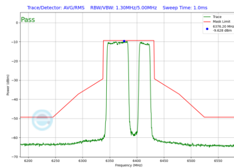
Plot 7-1112 In-Band Emission Plot SDM Primary Antenna WF2a (80MHz BW 802.11be(RU) RU484+242 Index92 (UNII Band 5) - Ch.87)
