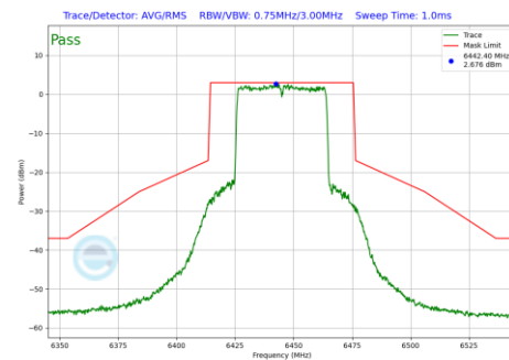
Plot 7-1048 In-Band Emission Plot CDD Primary Antenna WF7a (40MHz BW 802.11be(RU) RU484 Index65 (UNII Band 6) - Ch.99)
