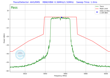
Plot 7-1055 In-Band Emission Plot CDD Primary Antenna WF2a (20MHz BW 802.11be(RU) RU242 Index61 (UNII Band 5) - Ch.1)
