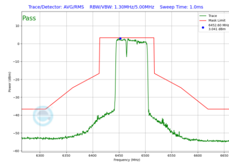
Plot 7-1038 In-Band Emission Plot CDD Primary Antenna WF2a (80MHz BW 802.11be(RU) RU484+242 Index90 (UNII Band 6) - Ch.103)
