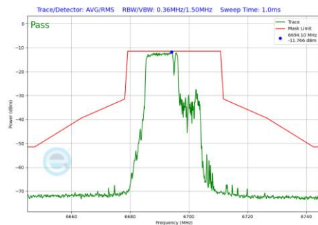
Plot 7-1105 In-Band Emission Plot SDM Primary Antenna WF7a (20MHz BW 802.11be(RU) RU106+26 Index82 (UNII Band 7) - Ch.149)
