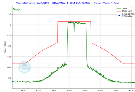
Plot 7-1029 In-Band Emission Plot CDD Primary Antenna WF7a (80MHz BW 802.11be(RU) RU484+242 Index90 (UNII Band 6) - Ch.103)
