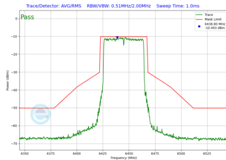
Plot 7-990 In-Band Emission Plot Antenna WF7b (40MHz BW 802.11be(RU) RU484 Index65 (UNII Band 6) - Ch.99)
