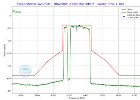
Plot 7-1113 In-Band Emission Plot SDM Primary Antenna WF2a (160MHz BW 802.11be(RU) RU996+484+242 Index97 (UNII Band 5) - Ch.79)
