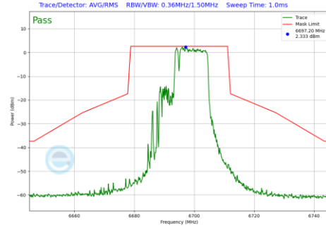
Plot 7-1031 In-Band Emission Plot CDD Primary Antenna WF7a (20MHz BW 802.11be(RU) RU106+26 Index83 (UNII Band 7) - Ch.149)
