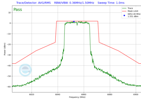
Plot 7-1063 In-Band Emission Plot CDD Primary Antenna WF2a (20MHz BW 802.11be(RU) RU242 Index61 (UNII Band 7) - Ch.181)
