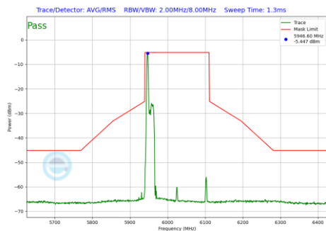
Plot 7-961 In-Band Emission Plot Antenna WF7b (160MHz BW 802.11be(RU) RU26 Index0 (UNII Band 5) - Ch.15)
