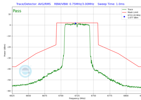
Plot 7-1064 In-Band Emission Plot CDD Primary Antenna WF2a (40MHz BW 802.11be(RU) RU484 Index65 (UNII Band 7) - Ch.155)
