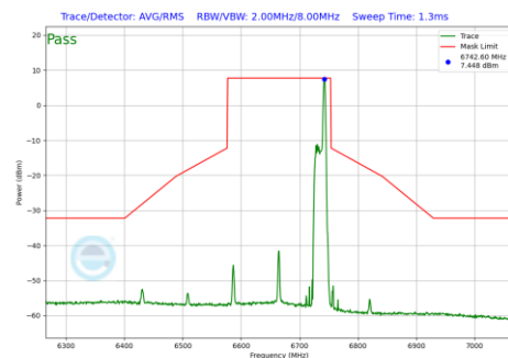
Plot 7-1024 In-Band Emission Plot CDD Primary Antenna WF2a (160MHz BW 802.11be(RU) RU26 Index36 (UNII Band 7) - Ch.143)
