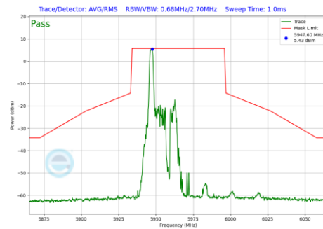
Plot 7-1014 In-Band Emission Plot CDD Primary Antenna WF2a (40MHz BW 802.11be(RU) RU26 Index0 (UNII Band 5) - Ch.3)
