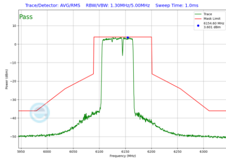
Plot 7-1026 In-Band Emission Plot CDD Primary Antenna WF7a (80MHz BW 802.11be(RU) RU484+242 Index93 (UNII Band 5) - Ch.39)
