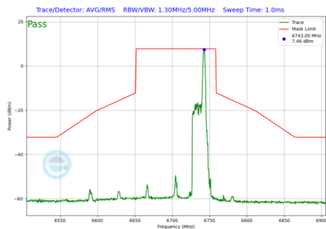
Plot 7-1011 In-Band Emission Plot CDD Primary Antenna WF7a (80MHz BW 802.11be(RU) RU26 Index36 (UNII Band 7) - Ch.151)
