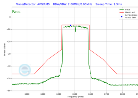
Plot 7-992 In-Band Emission Plot Antenna WF7b (160MHz BW 802.11be(RU) RU996X2 Index68 (UNII Band 6) - Ch.111)
