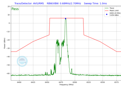
Plot 7-1006 In-Band Emission Plot CDD Primary Antenna WF7a (40MHz BW 802.11be(RU) RU26 Index8 (UNII Band 6) - Ch.107)
