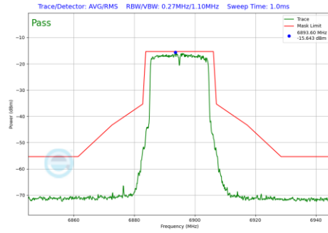
Plot 7-997 In-Band Emission Plot Antenna WF7b (20MHz BW 802.11be(RU) RU242 Index61 (UNII Band 8) - Ch.189)
