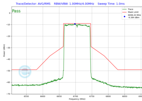
Plot 7-995 In-Band Emission Plot Antenna WF7b (80MHz BW 802.11be(RU) RU996 Index67 (UNII Band 7) - Ch.151)
