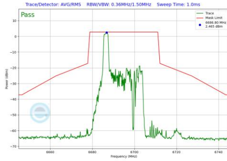
Plot 7-1009 In-Band Emission Plot CDD Primary Antenna WF7a (20MHz BW 802.11be(RU) RU26 Index0 (UNII Band 7) - Ch.149)
