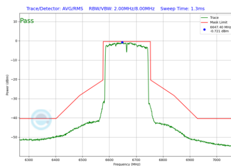
Plot 7-957 In-Band Emission Plot Antenna WF7b (160MHz BW 802.11be(RU) RU996X2 Index68 (UNII Band 7) - Ch.143)
