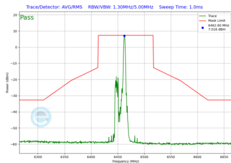
Plot 7-1019 In-Band Emission Plot CDD Primary Antenna WF2a (80MHz BW 802.11be(RU) RU26 Index17 (UNII Band 6) - Ch.103)
