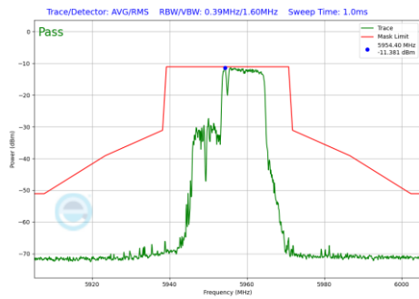
Plot 7-1099 In-Band Emission Plot SDM Primary Antenna WF7a (20MHz BW 802.11be(RU) RU106+26 Index83 (UNII Band 5) - Ch.1)
