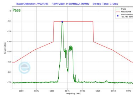
Plot 7-1096 In-Band Emission Plot SDM Primary Antenna WF2a (40MHz BW 802.11be(RU) RU26 Index0 (UNII Band 8) - Ch.187)
