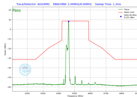
Plot 7-1008 In-Band Emission Plot CDD Primary Antenna WF7a (160MHz BW 802.11be(RU) RU26 Index17 (UNII Band 6) - Ch.111)
