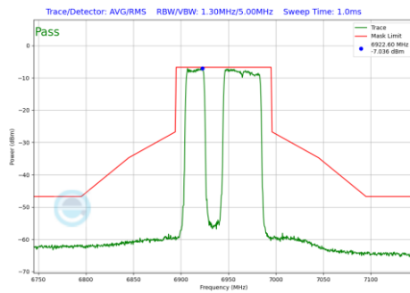
Plot 7-1109 In-Band Emission Plot SDM Primary Antenna WF7a (80MHz BW 802.11be(RU) RU484+242 Index91 (UNII Band 8) - Ch.199)
