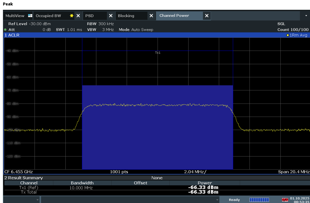
Plot 7-1326. Channel Power – UNII 6 – 20MHz
