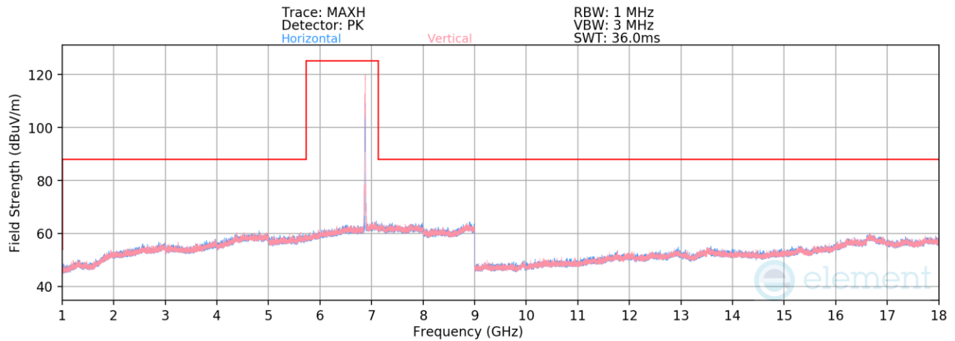
Plot 7-1368. Radiated Spurious Emissions above 1GHz SDM Primary (802.11be – Ch. 185 – RU26)
