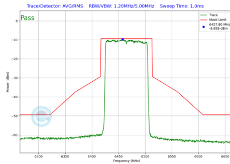
Plot 7-1296 In-Band Emission Plot SDM Diversity Antenna WF2a (80MHz BW 802.11be(RU) RU996 Index67 (UNII Band 6) - Ch.103)
