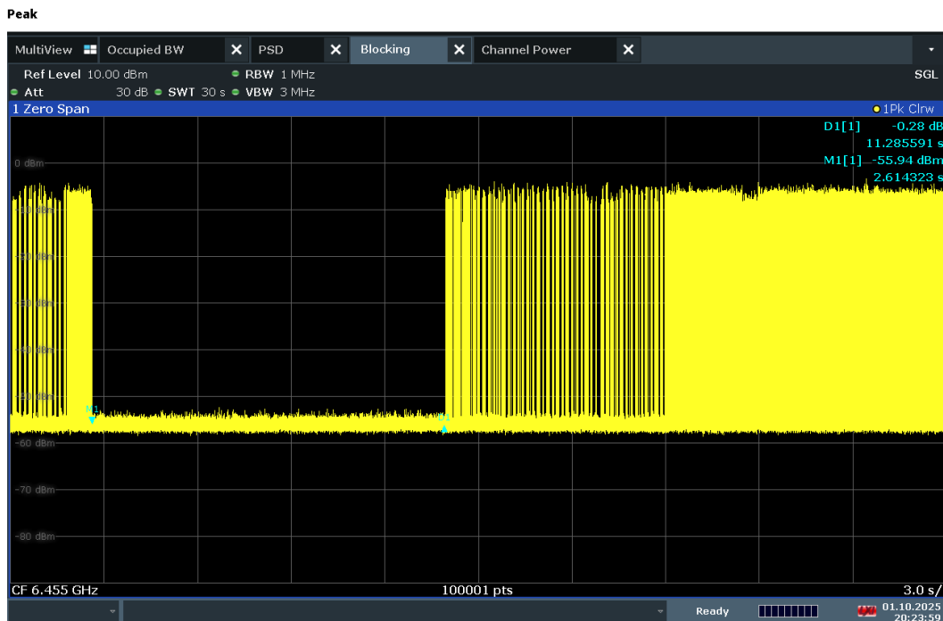
Plot 7-1342. Contention Based Protocol Timing Plot – UNII 6 – 20MHz Channel 101
