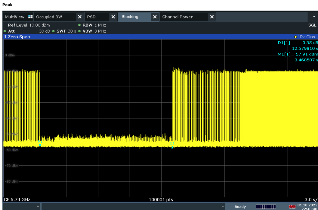
Plot 7-1348. Contention Based Protocol Timing Plot – UNII 7 – 160MHz Channel 143 – Mid
