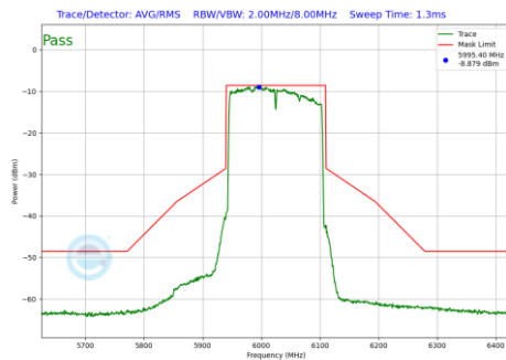
Plot 7-1293 In-Band Emission Plot SDM Diversity Antenna WF2a (160MHz BW 802.11be(RU) RU996X2 Index68 (UNII Band 5) - Ch.15)
