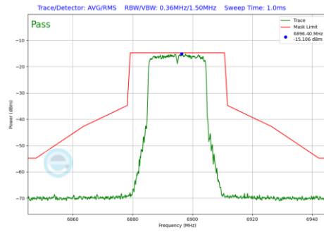
Plot 7-1302 In-Band Emission Plot SDM Diversity Antenna WF2a (20MHz BW 802.11be(RU) RU242 Index61 (UNII Band 8) - Ch.189)
