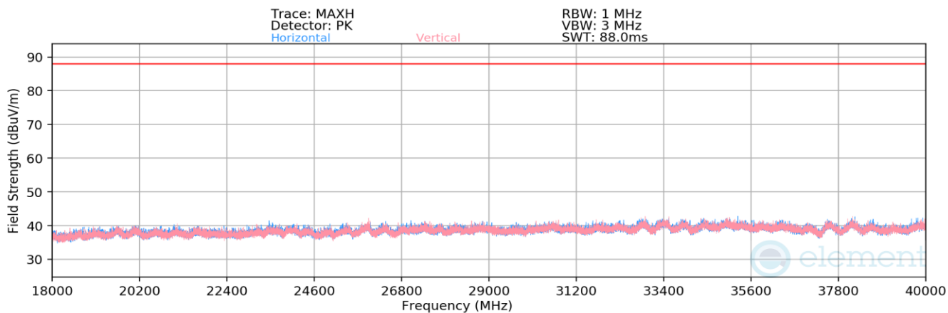
Plot 7-1379. Radiated Spurious Emissions 18-40GHz CDD Primary (802.11be – Ch. 105 – RU242)
