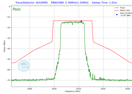
Plot 7-1294 In-Band Emission Plot SDM Diversity Antenna WF2a (20MHz BW 802.11be(RU) RU242 Index61 (UNII Band 6) - Ch.113)
