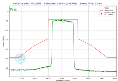
Plot 7-1300 In-Band Emission Plot SDM Diversity Antenna WF2a (80MHz BW 802.11be(RU) RU996 Index67 (UNII Band 7) - Ch.151)
