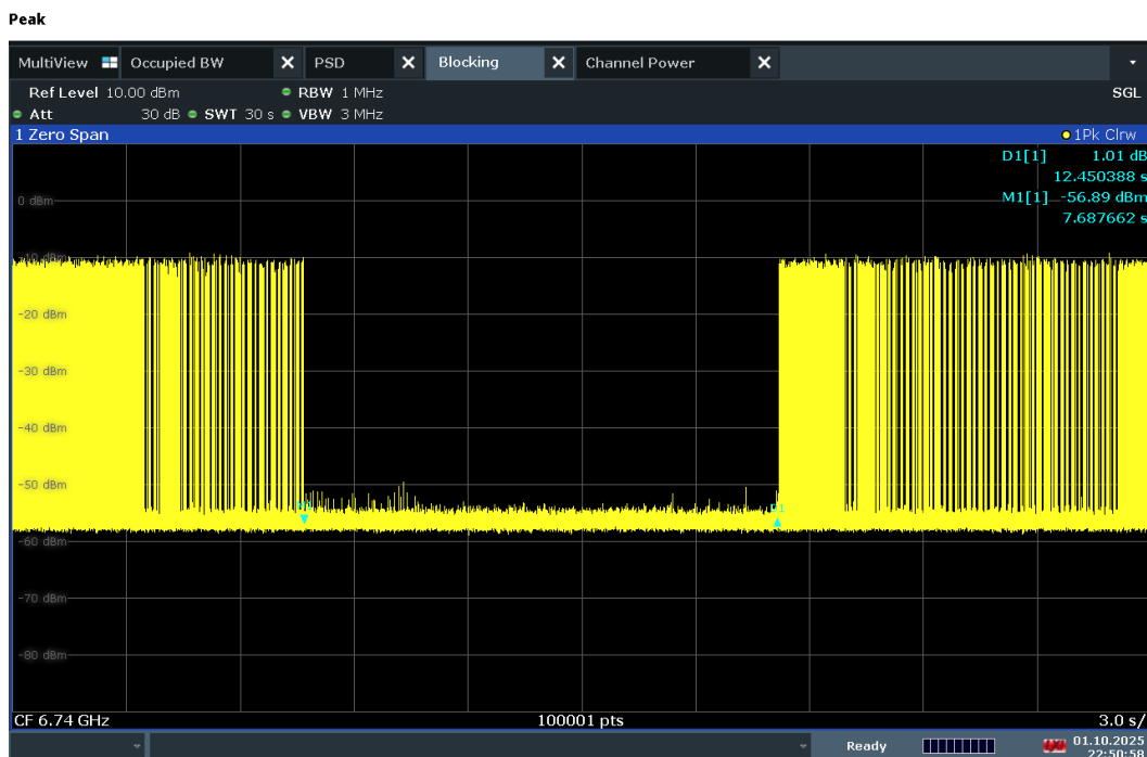
Plot 7-1349. Contention Based Protocol Timing Plot – UNII 7 – 160MHz Channel 143 – High
