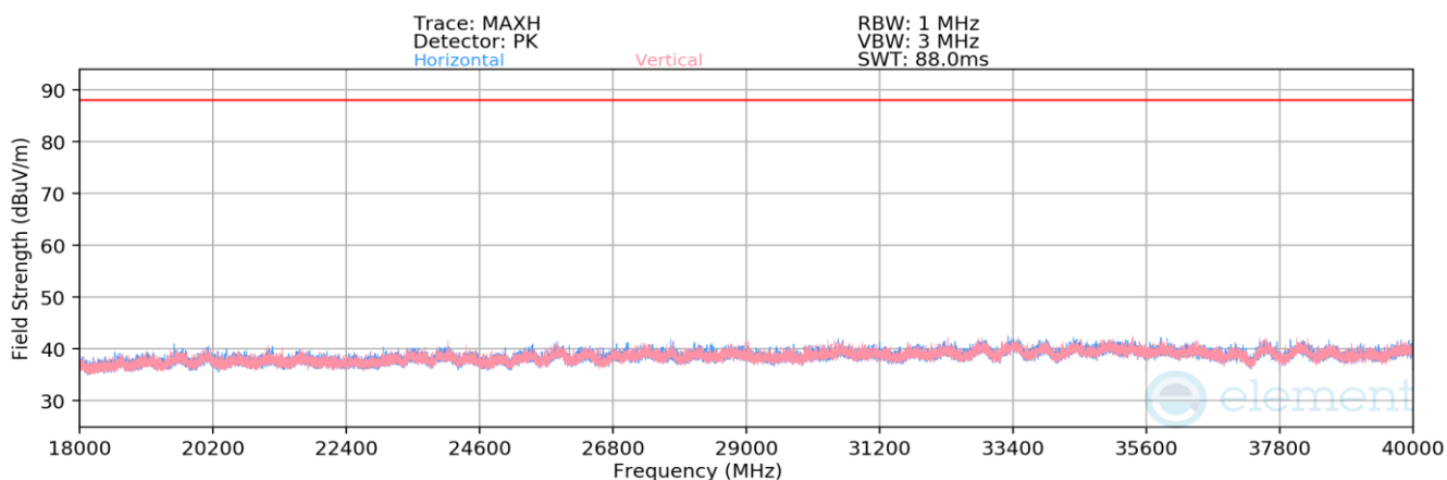
Plot 7-1383. Radiated Spurious Emissions 18-40GHz CDD Primary (802.11be – Ch. 149 – RU242)
