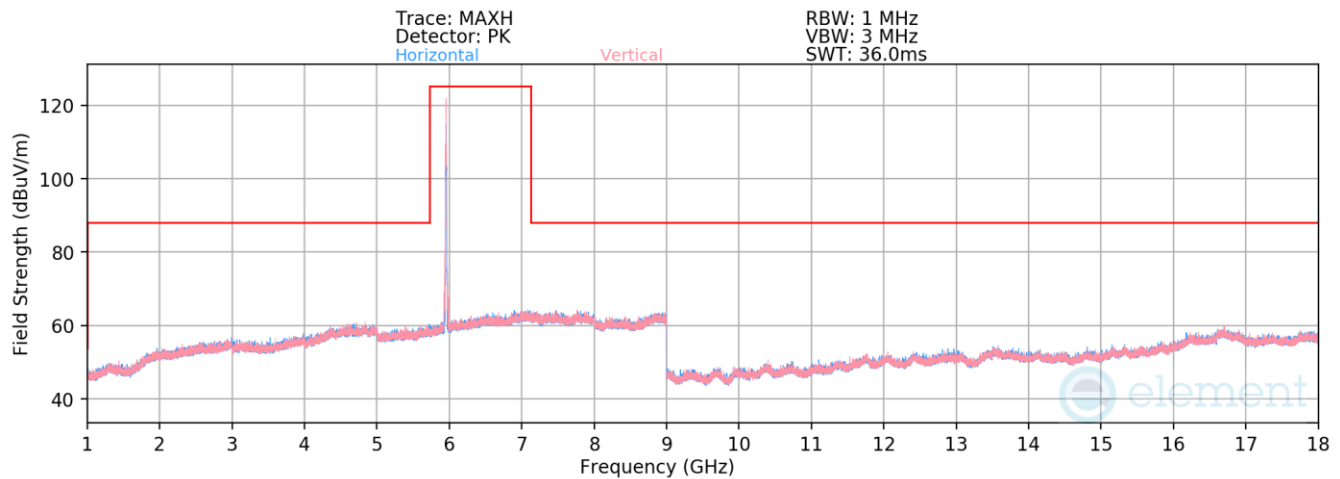
Plot 7-1357. Radiated Spurious Emissions above 1GHz CDD Primary (802.11be – Ch. 1 – RU26)
