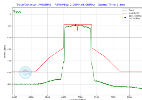
Plot 7-1305 In-Band Emission Plot SDM Diversity Antenna WF2a (160MHz BW 802.11be(RU) RU996X2 Index68 (UNII Band 8) - Ch.207)
