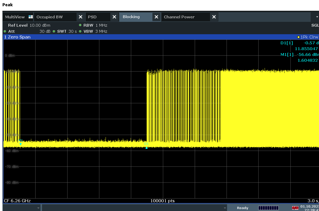
Plot 7-1341. Contention Based Protocol Timing Plot – UNII 5 – 160MHz Channel 47 – High
