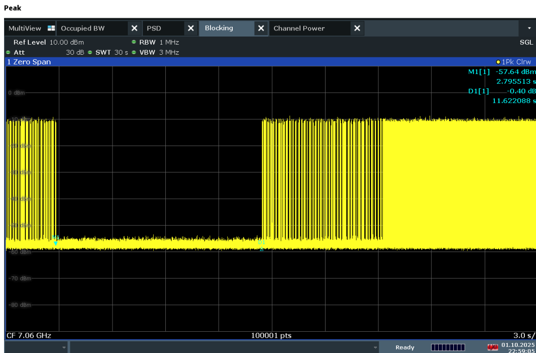
Plot 7-1352. Contention Based Protocol Timing Plot – UNII 8 – 160MHz Channel 207 – Mid
