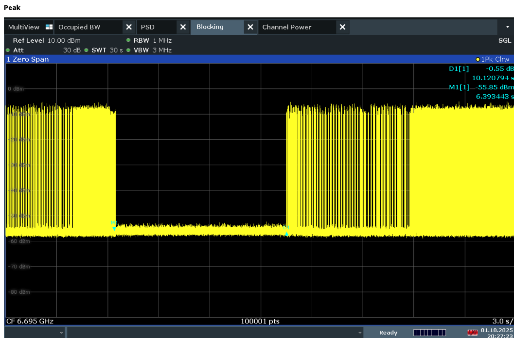
Plot 7-1346. Contention Based Protocol Timing Plot – UNII 7 – 20MHz Channel 149
