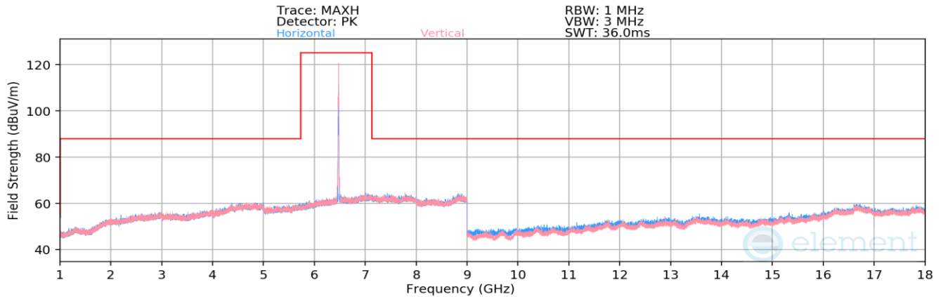
Plot 7-1362. Radiated Spurious Emissions above 1GHz CDD Primary (802.11be – Ch. 105 – RU26)
