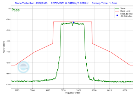
Plot 7-1291 In-Band Emission Plot SDM Diversity Antenna WF2a (40MHz BW 802.11be(RU) RU484 Index65 (UNII Band 5) - Ch.3)
