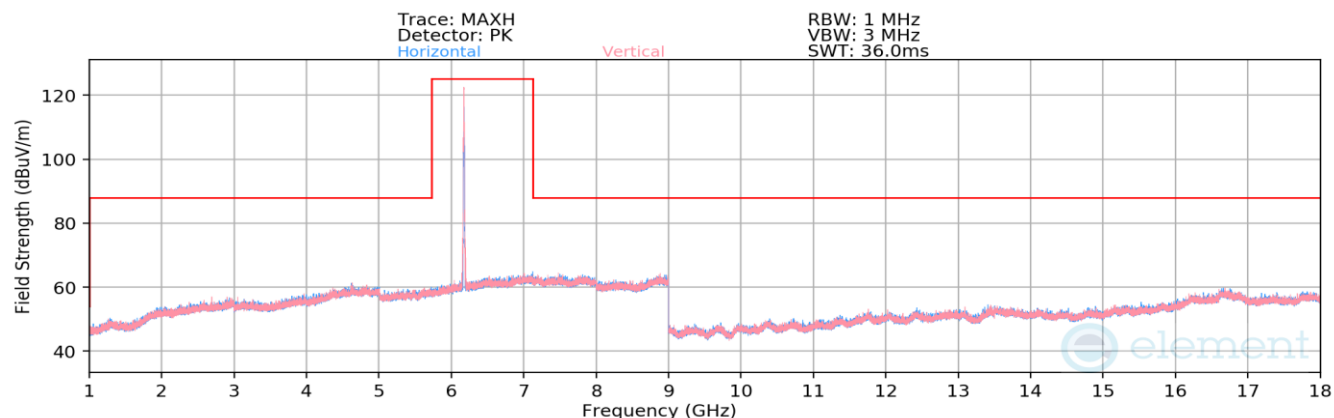
Plot 7-1358. Radiated Spurious Emissions above 1GHz CDD Primary (802.11be – Ch. 45 – RU26)
