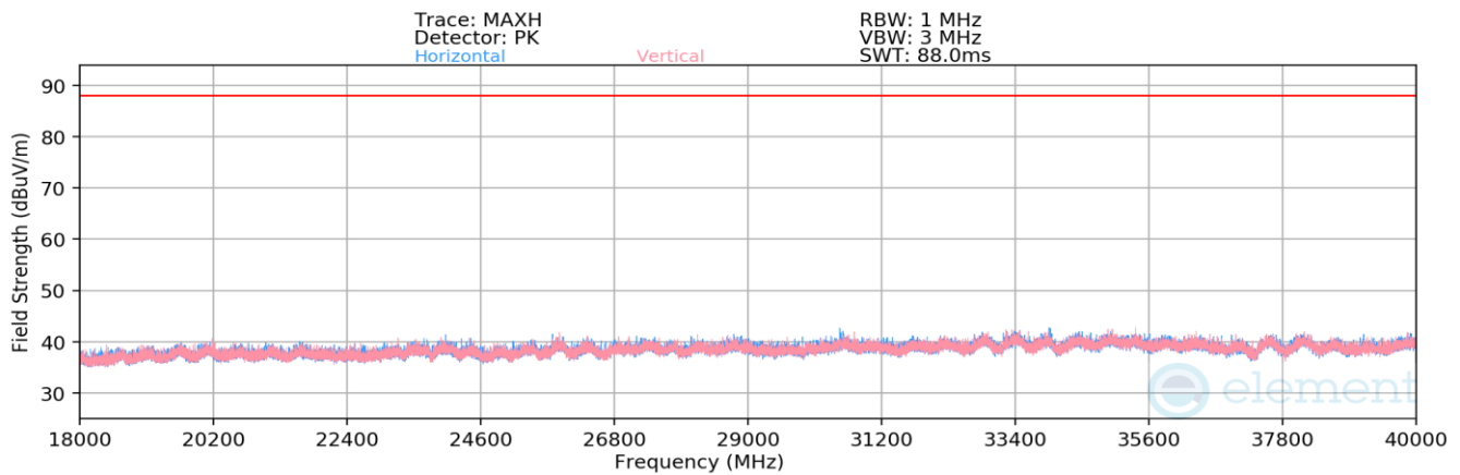
Plot 7-1363. Radiated Spurious Emissions 18-40GHz CDD Primary (802.11be – Ch. 105 – RU26)
