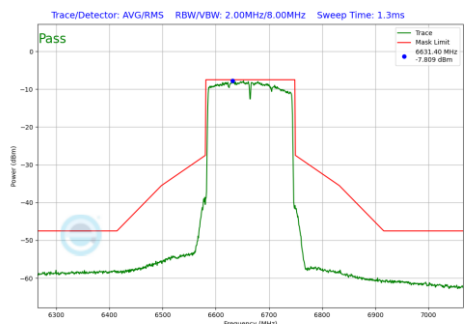
Plot 7-1301 In-Band Emission Plot SDM Diversity Antenna WF2a (160MHz BW 802.11be(RU) RU996X2 Index68 (UNII Band 7) - Ch.143)
