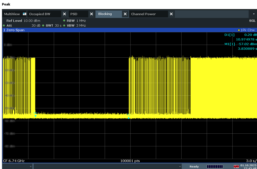
Plot 7-1347. Contention Based Protocol Timing Plot – UNII 7 – 160MHz Channel 143 – Low
