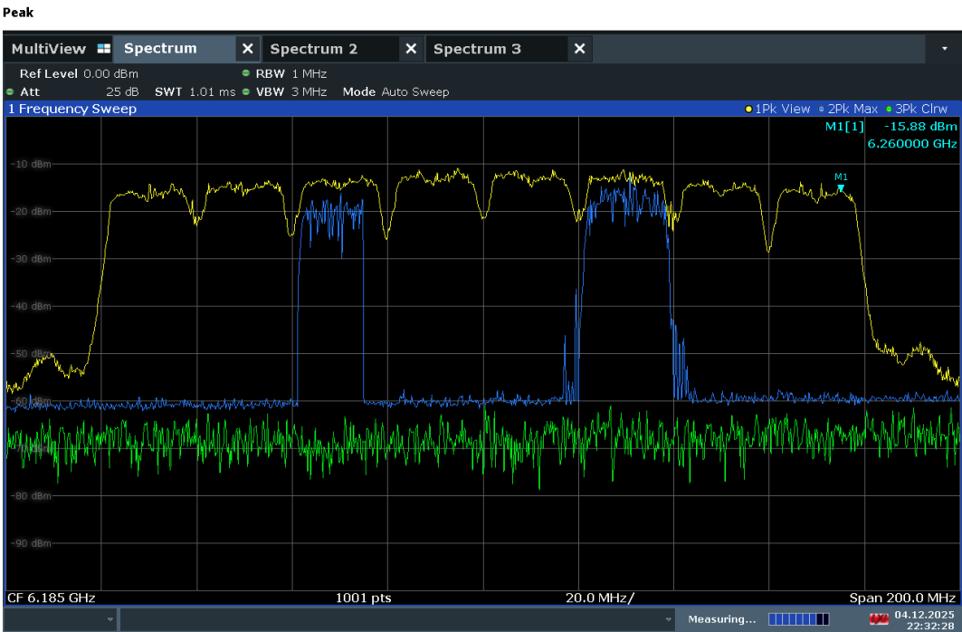
Plot 7-1356. 160MHz Bandwidth, AWGN Signal Injected – 6260MHz
