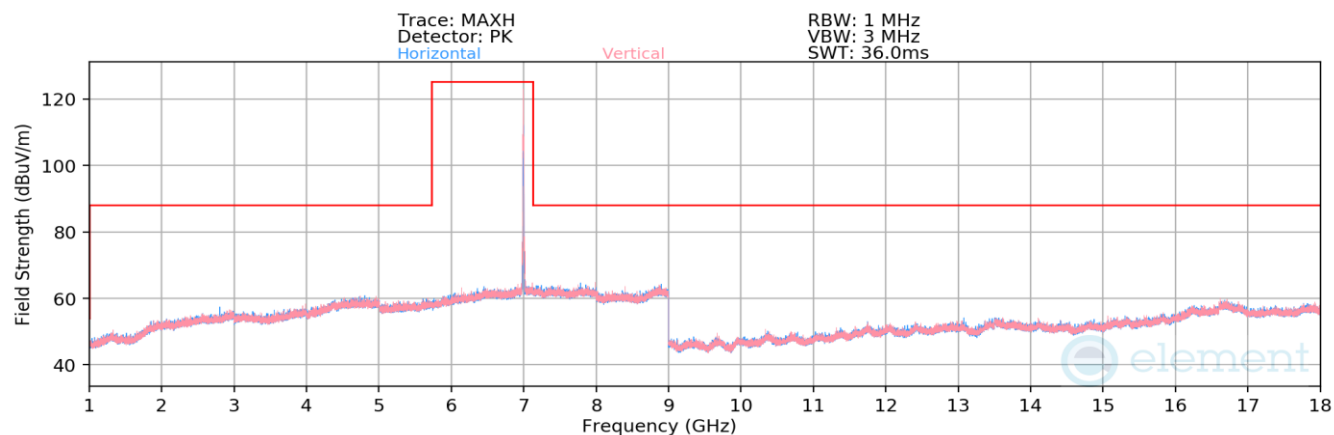
Plot 7-1370. Radiated Spurious Emissions above 1GHz SDM Primary (802.11be – Ch. 209 – RU26)
