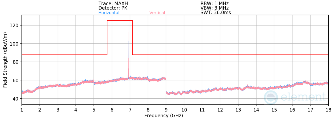
Plot 7-1369. Radiated Spurious Emissions above 1GHz SDM Primary (802.11be – Ch. 189 – RU26)
