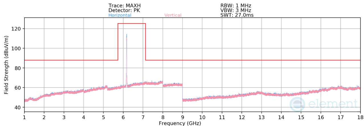
Plot 7-1374. Radiated Spurious Emissions above 1GHz CDD Primary (802.11be – Ch. 45 – RU242)
