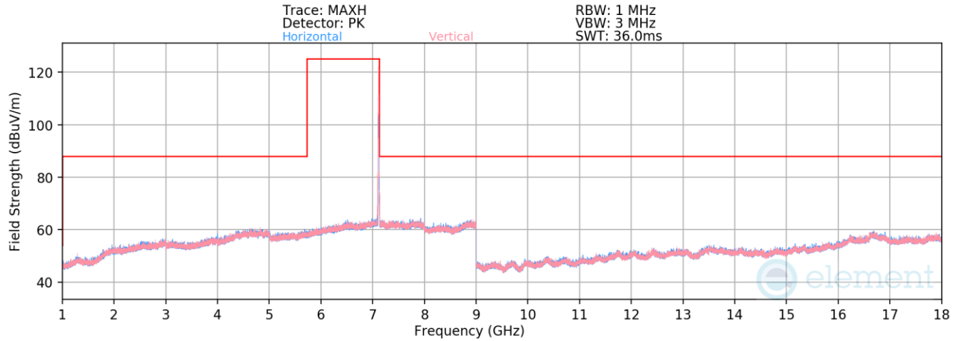
Plot 7-1372. Radiated Spurious Emissions above 1GHz SDM Primary (802.11be – Ch. 229 – RU26)
