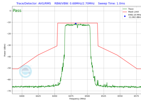
Plot 7-1295 In-Band Emission Plot SDM Diversity Antenna WF2a (40MHz BW 802.11be(RU) RU484 Index65 (UNII Band 6) - Ch.107)
