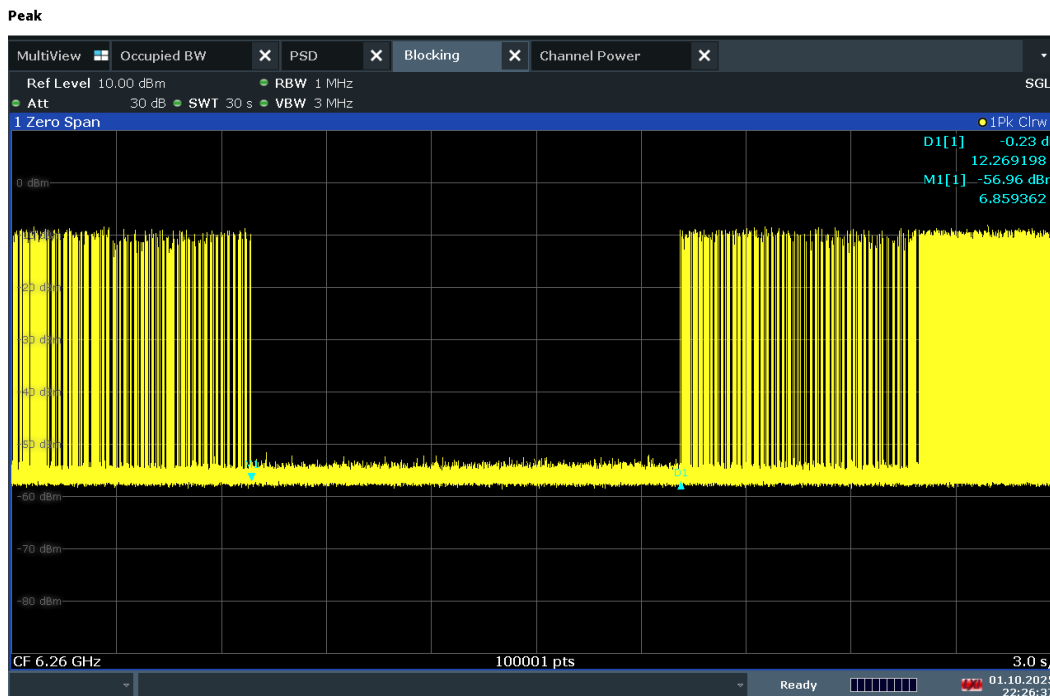
Plot 7-1340. Contention Based Protocol Timing Plot –UNII 5 – 160MHz Channel 47 – Mid
