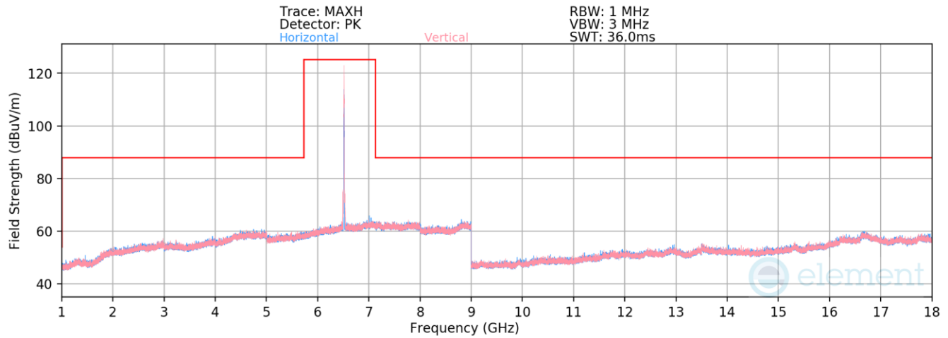
Plot 7-1364. Radiated Spurious Emissions above 1GHz CDD Primary (802.11be – Ch. 113 – RU26)
