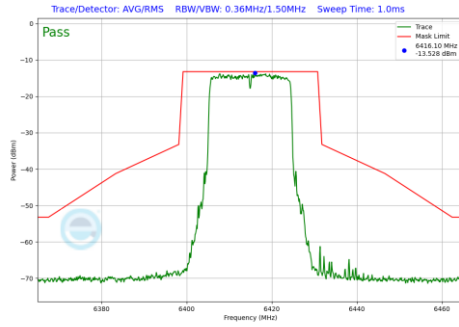
Plot 7-1290 In-Band Emission Plot SDM Diversity Antenna WF2a (20MHz BW 802.11be(RU) RU242 Index61 (UNII Band 5) - Ch.93)
