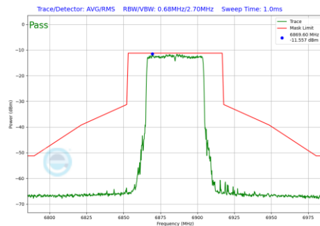
Plot 7-1303 In-Band Emission Plot SDM Diversity Antenna WF2a (40MHz BW 802.11be(RU) RU484 Index65 (UNII Band 8) - Ch.187)
