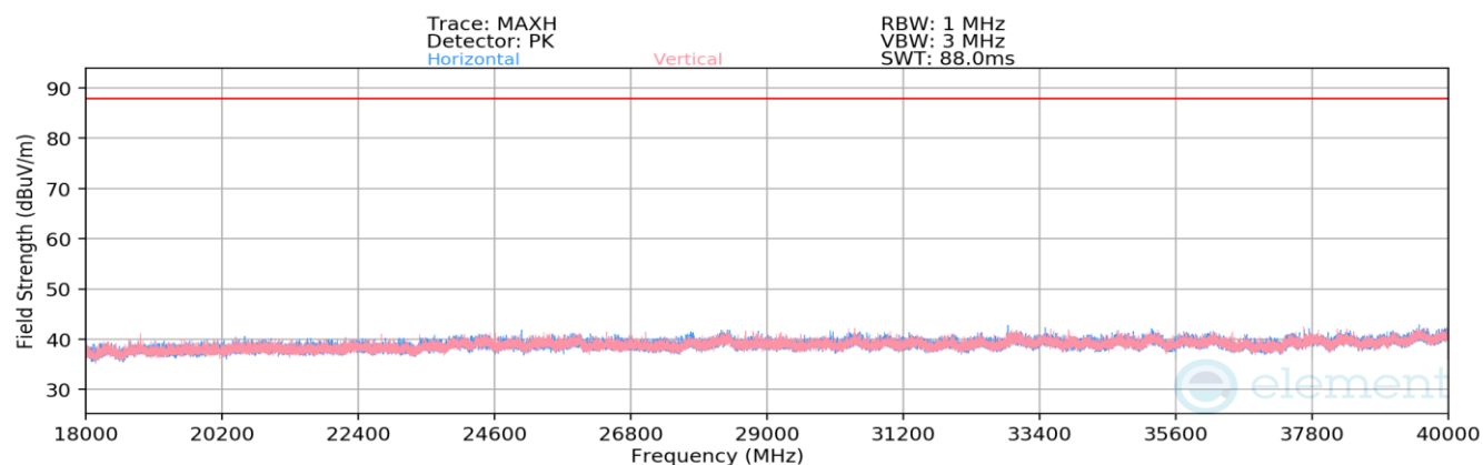
Plot 7-1367. Radiated Spurious Emissions 18-40GHz CDD Primary (802.11be – Ch. 149 – RU26)
