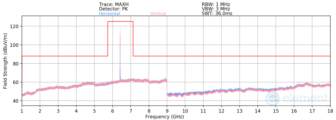
Plot 7-1360. Radiated Spurious Emissions above 1GHz CDD Primary (802.11be – Ch. 93 – RU26)
