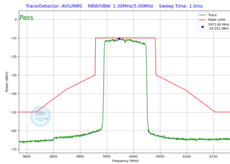
Plot 7-1292 In-Band Emission Plot SDM Diversity Antenna WF2a (80MHz BW 802.11be(RU) RU996 Index67 (UNII Band 5) - Ch.7)
