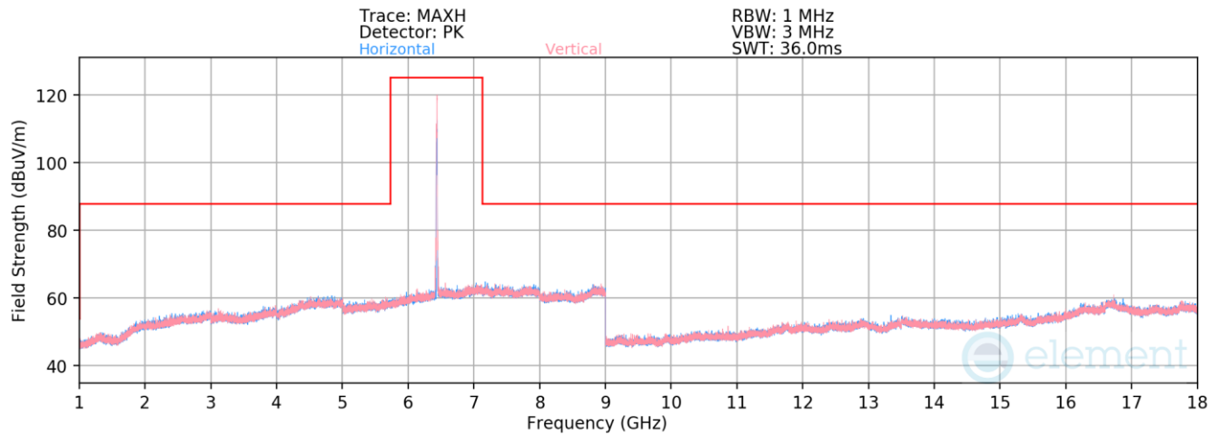
Plot 7-1361. Radiated Spurious Emissions above 1GHz CDD Primary (802.11be – Ch. 97 – RU26)
