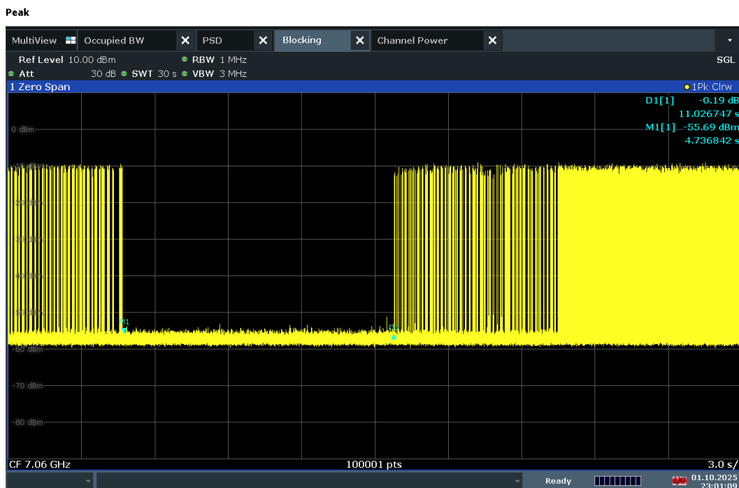
Plot 7-1353. Contention Based Protocol Timing Plot – UNII 8 – 160MHz Channel 207 – High
