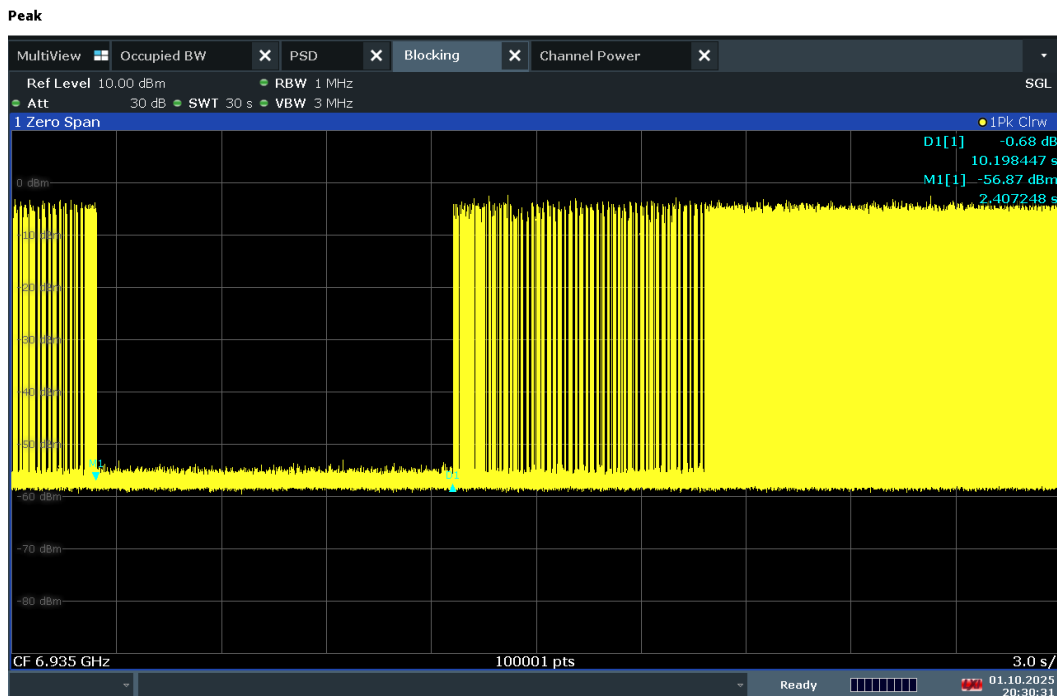
Plot 7-1350. Contention Based Protocol Timing Plot – UNII 8 – 20MHz Channel 197
