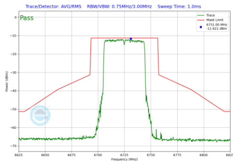
Plot 7-1299 In-Band Emission Plot SDM Diversity Antenna WF2a (40MHz BW 802.11be(RU) RU484 Index65 (UNII Band 7) - Ch.155)
