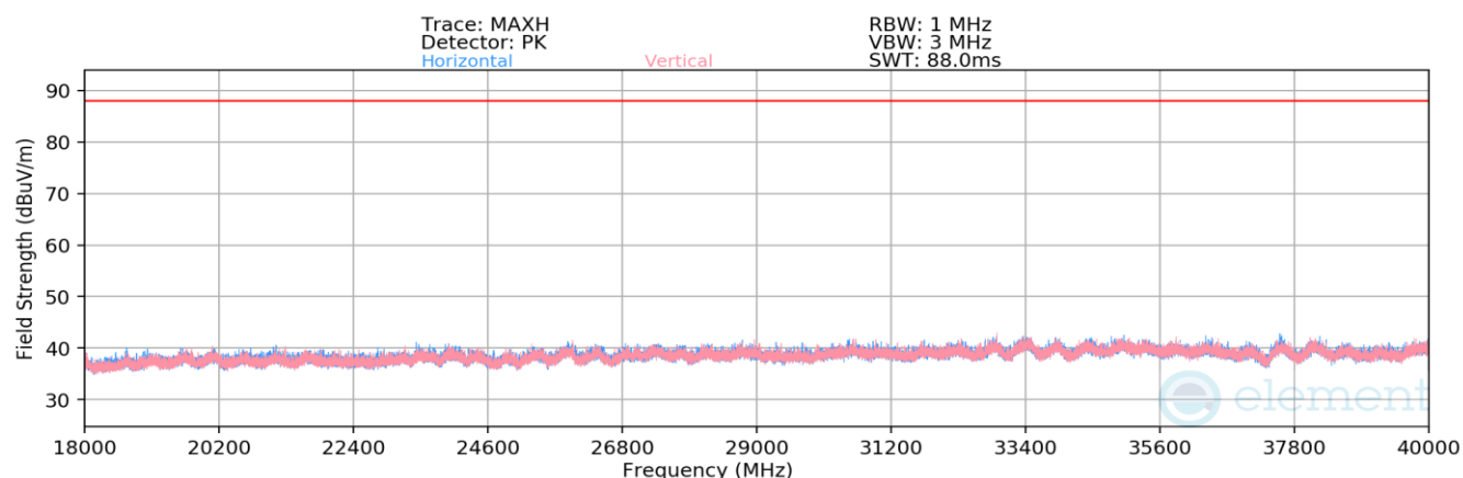
Plot 7-1359. Radiated Spurious Emissions 18-40GHz CDD Primary (802.11be – Ch. 45 – RU26)
