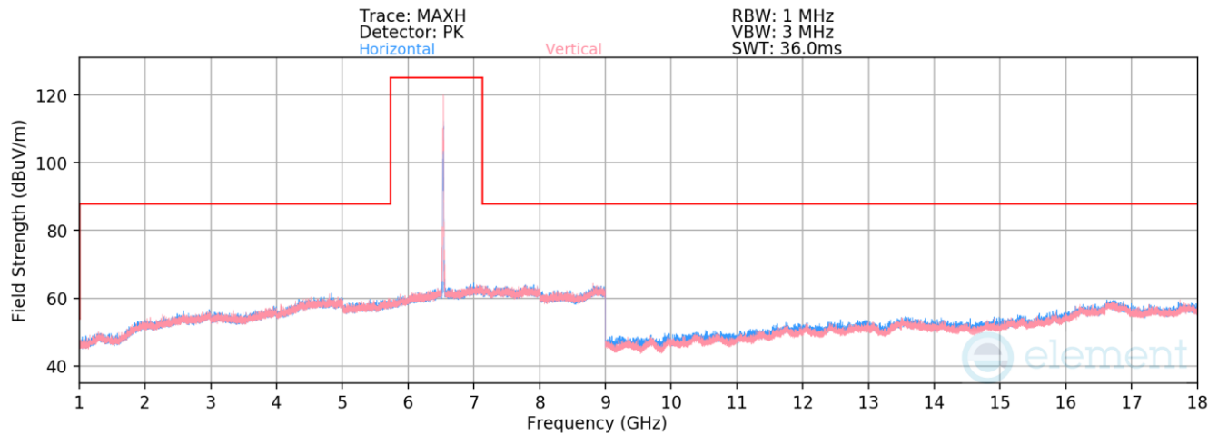
Plot 7-1365. Radiated Spurious Emissions above 1GHz CDD Primary (802.11be – Ch. 117 – RU26)
