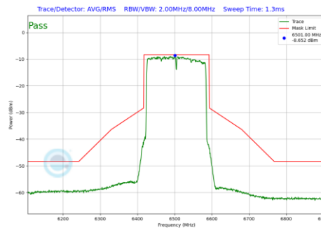
Plot 7-1297 In-Band Emission Plot SDM Diversity Antenna WF2a (160MHz BW 802.11be(RU) RU996X2 Index68 (UNII Band 6) - Ch.111)
