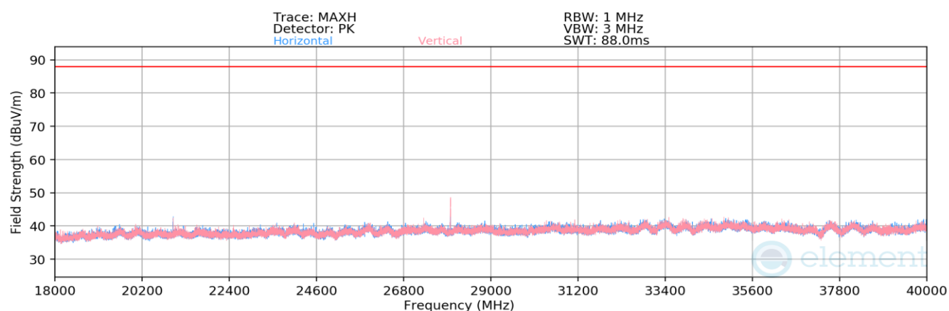
Plot 7-1371. Radiated Spurious Emissions 18-40GHz SDM Primary (802.11be – Ch. 209 – RU26)
