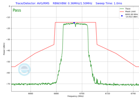
Plot 7-1298 In-Band Emission Plot SDM Diversity Antenna WF2a (20MHz BW 802.11be(RU) RU242 Index61 (UNII Band 7) - Ch.149)
