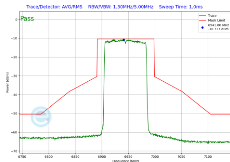
Plot 7-1304 In-Band Emission Plot SDM Diversity Antenna WF2a (80MHz BW 802.11be(RU) RU996 Index67 (UNII Band 8) - Ch.199)
