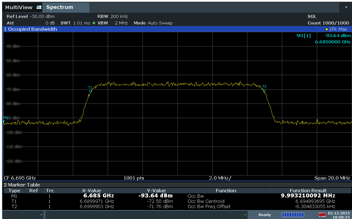
Plot 7-1314. AWGN Signal – UNII 7 – 20MHz
