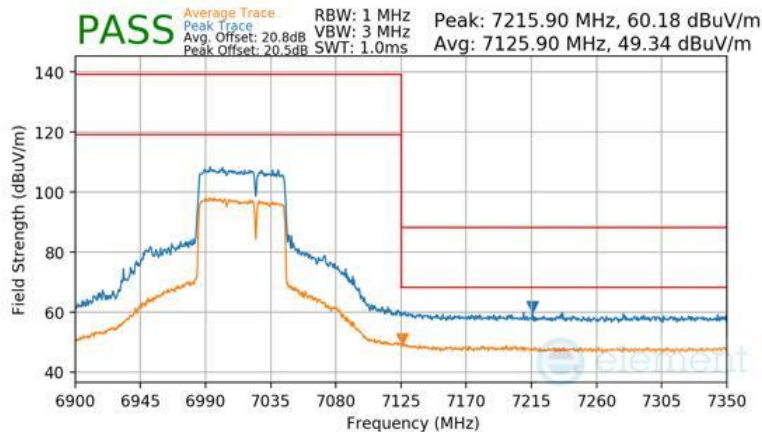
Plot 7-1574 Antenna WF7b Radiated Upper Band Edge (Peak & Average – UNII Band 8) - RU484+242
