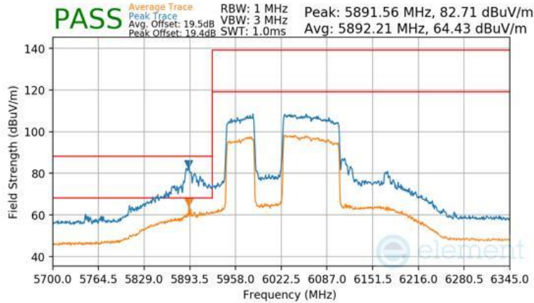
Plot 7-1521 Antenna WF2a Radiated Lower Band Edge (Peak & Average – UNII Band 5) - RU996+484 (L)
