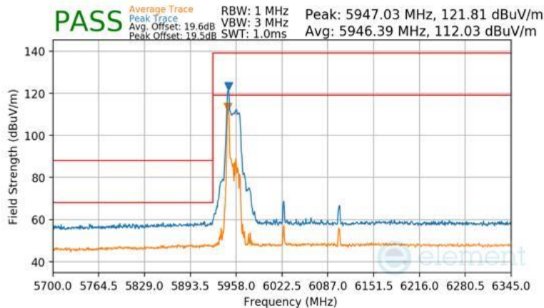
Plot 7-1515 Antenna WF2a Radiated Lower Band Edge (Peak & Average – UNII Band 5) - RU26 (L)
