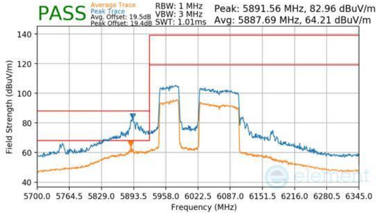
Plot 7-1583 Antenna WF7b Radiated Lower Band Edge (Peak & Average – UNII Band 5) - RU996+484 (L)
