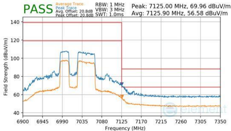
Plot 7-1572 Antenna WF7b Radiated Upper Band Edge (Peak & Average – UNII Band 8) - RU484+242
