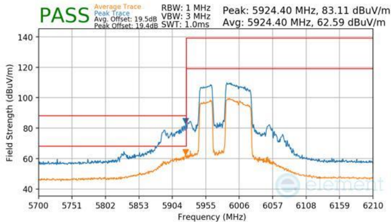
Plot 7-1568 Antenna WF7b Radiated Lower Band Edge (Peak & Average – UNII Band 5) - RU484+242
