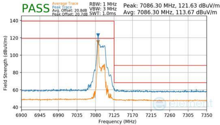
Plot 7-1485 Antenna WF2a Radiated Upper Band Edge (Peak & Average – UNII Band 8) - RU26
