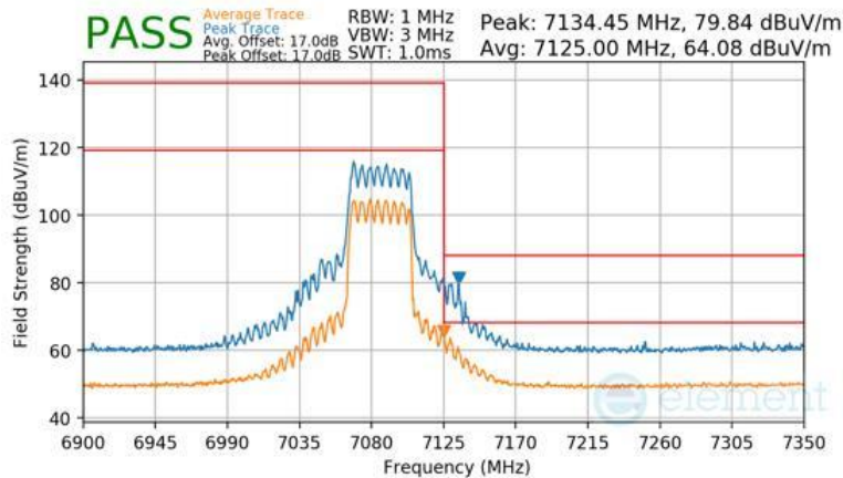
Plot 7-1624 CDD Primary Radiated Upper Band Edge (Peak & Average – UNII Band 8) - RU484
