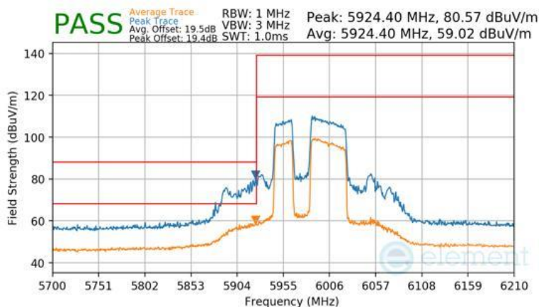
Plot 7-1506 Antenna WF2a Radiated Lower Band Edge (Peak & Average – UNII Band 5) - RU484+242
