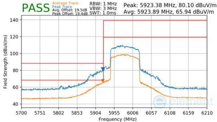
Plot 7-1575 Antenna WF7b Radiated Lower Band Edge (Peak & Average – UNII Band 5) - RU996
