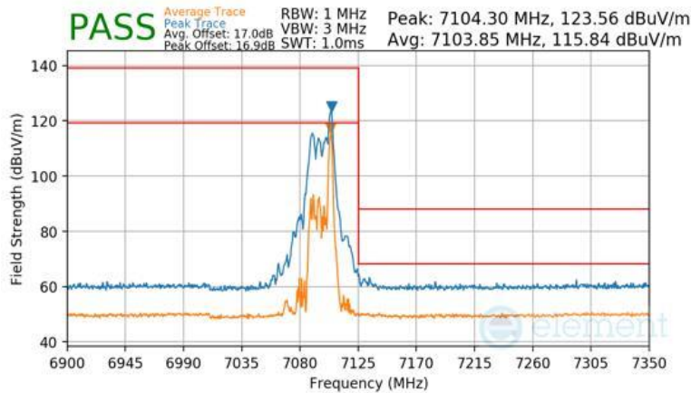
Plot 7-1610 CDD Primary Radiated Upper Band Edge (Peak & Average – UNII Band 8) - RU26
