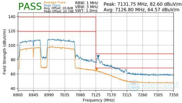
Plot 7-1541 Antenna WF2a Radiated Upper Band Edge (Peak & Average – UNII Band 8) - RU996+484+242 (L)
