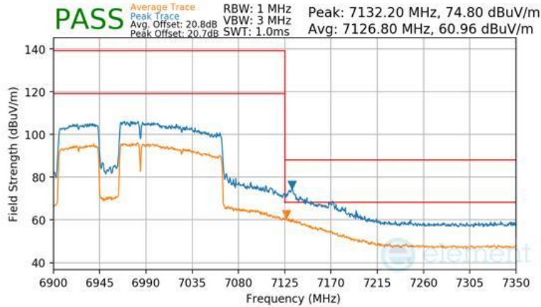
Plot 7-1601 Antenna WF7b Radiated Upper Band Edge (Peak & Average – UNII Band 8) - RU996+484+242 (L)
