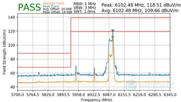
Plot 7-1578 Antenna WF7b Radiated Lower Band Edge (Peak & Average – UNII Band 5) - RU26 (H)
