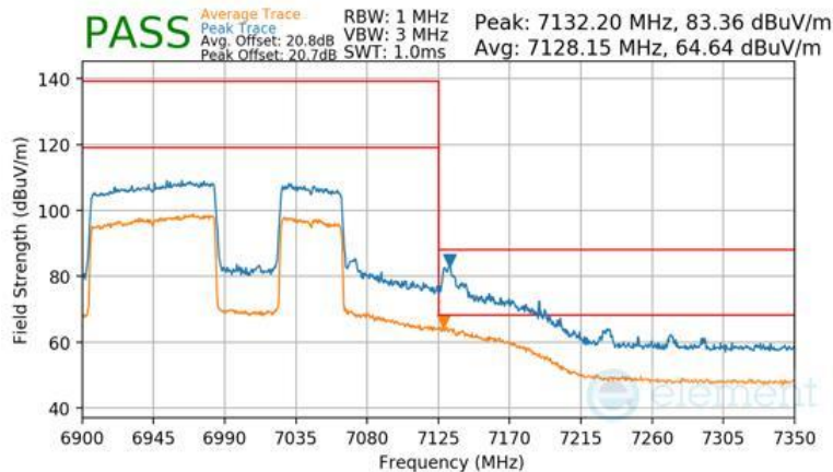
Plot 7-1524 Antenna WF2a Radiated Upper Band Edge (Peak & Average – UNII Band 8) - RU996+484 (H)
