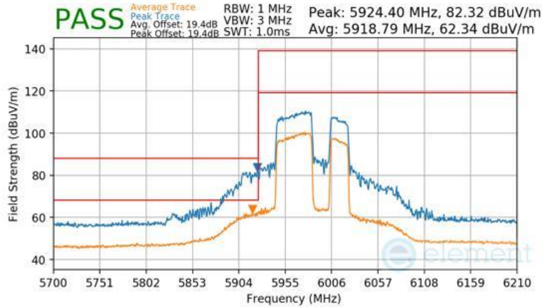
Plot 7-1507 Antenna WF2a Radiated Lower Band Edge (Peak & Average – UNII Band 5) - RU484+242
