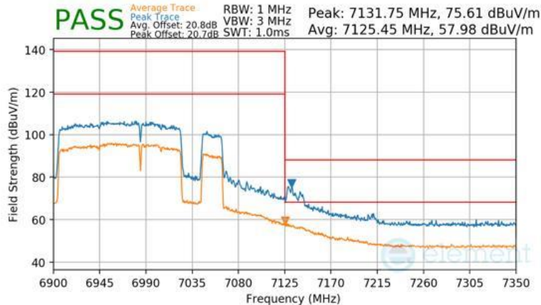
Plot 7-1602 Antenna WF7b Radiated Upper Band Edge (Peak & Average – UNII Band 8) - RU996+484+242 (H)
