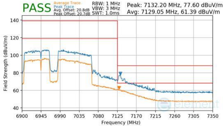
Plot 7-1603 Antenna WF7b Radiated Upper Band Edge (Peak & Average – UNII Band 8) - RU996+484+242 (L)
