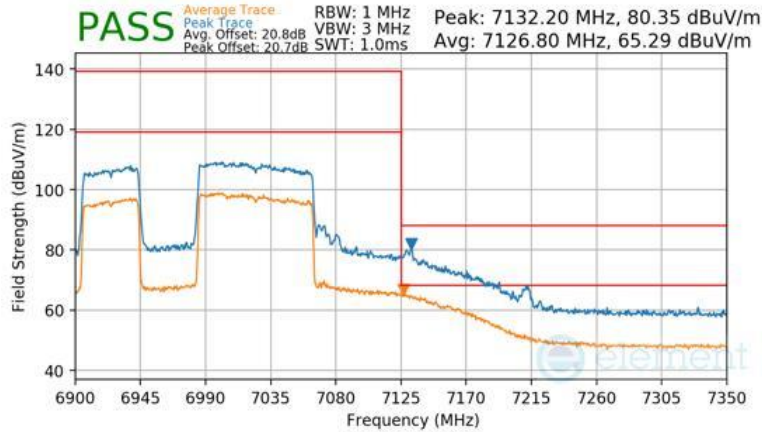
Plot 7-1525 Antenna WF2a Radiated Upper Band Edge (Peak & Average – UNII Band 8) - RU996+484 (L)
