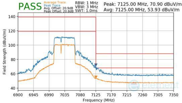
Plot 7-1509 Antenna WF2a Radiated Upper Band Edge (Peak & Average – UNII Band 8) - RU484+242
