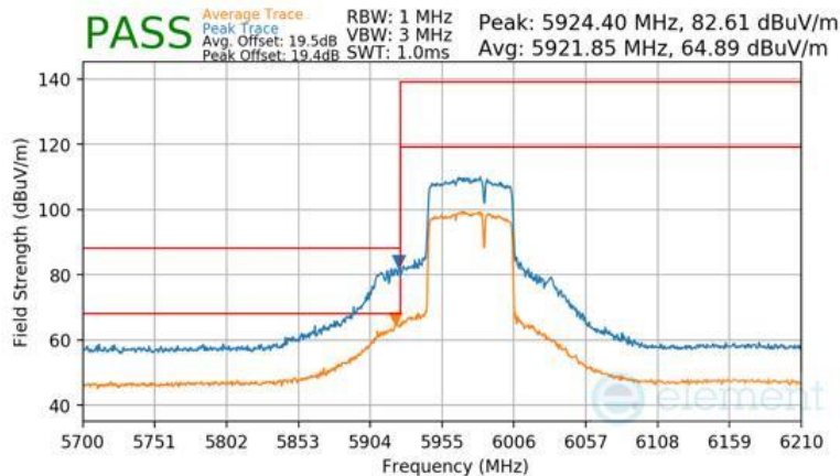
Plot 7-1570 Antenna WF7b Radiated Lower Band Edge (Peak & Average – UNII Band 5) - RU484+242
