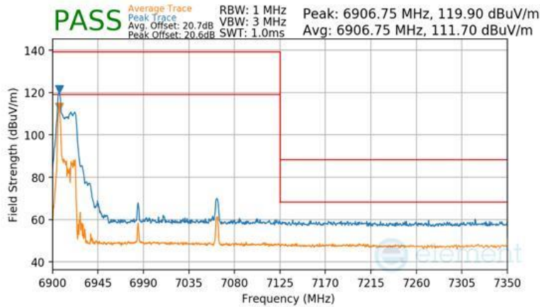
Plot 7-1579 Antenna WF7b Radiated Upper Band Edge (Peak & Average – UNII Band 8) - RU26 (L)
