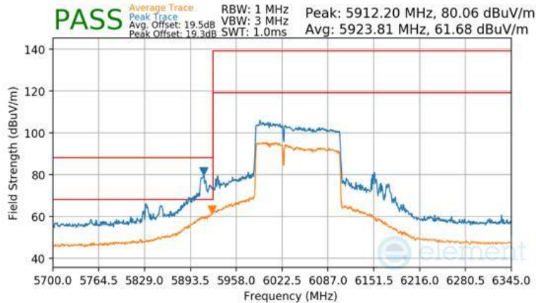
Plot 7-1581 Antenna WF7b Radiated Lower Band Edge (Peak & Average – UNII Band 5) - RU996+484 (L)
