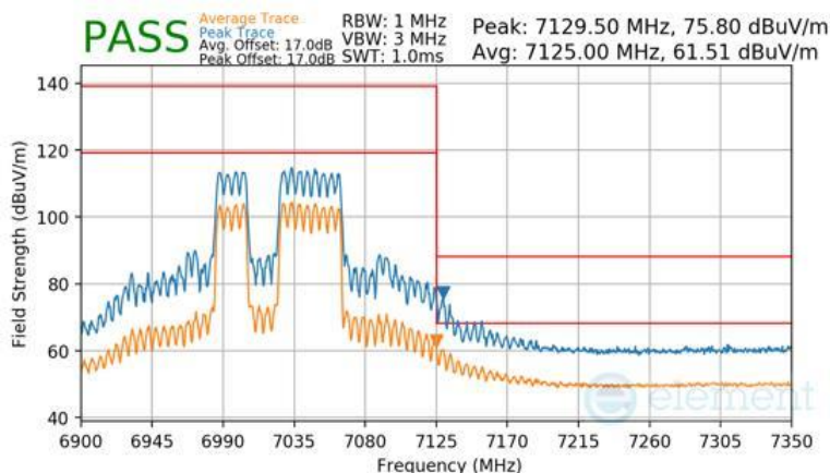
Plot 7-1634 CDD Primary Radiated Upper Band Edge (Peak & Average – UNII Band 8) - RU484+242
