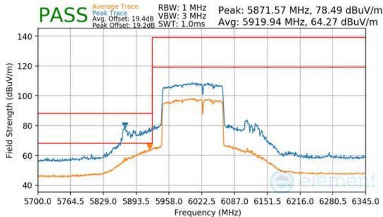
Plot 7-1522 Antenna WF2a Radiated Lower Band Edge (Peak & Average – UNII Band 5) - RU996+484 (H)
