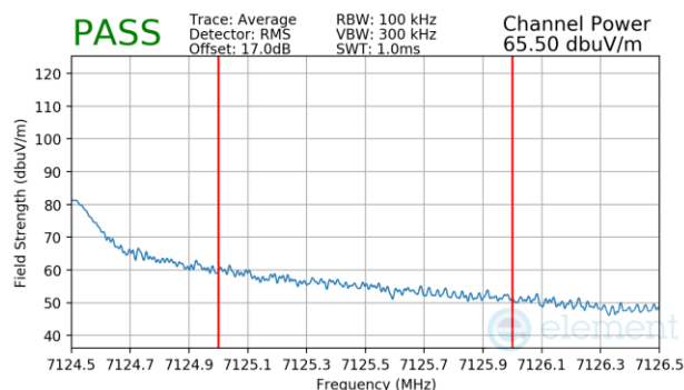
Plot 7-1618 CDD Primary Radiated Upper Band Edge (Average – UNII Band 8) – RU242
