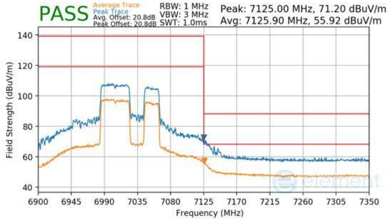
Plot 7-1573 Antenna WF7b Radiated Upper Band Edge (Peak & Average – UNII Band 8) - RU484+242
