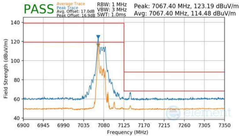
Plot 7-1621 CDD Primary Radiated Upper Band Edge (Peak & Average – UNII Band 8) - RU26
