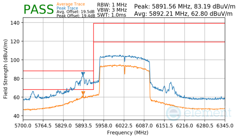
Plot 7-1605 Antenna WF7b Radiated Lower Band Edge (Peak & Average – UNII Band 5) - RU996X2
