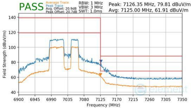
Plot 7-1511 Antenna WF2a Radiated Upper Band Edge (Peak & Average – UNII Band 8) - RU484+242
