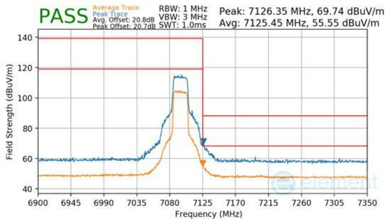
Plot 7-1492 Antenna WF2a Radiated Upper Band Edge (Peak & Average – UNII Band 8) - RU242
