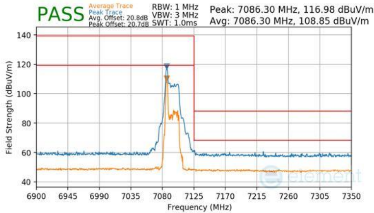
Plot 7-1547 Antenna WF7b Radiated Upper Band Edge (Peak & Average – UNII Band 8) - RU26
