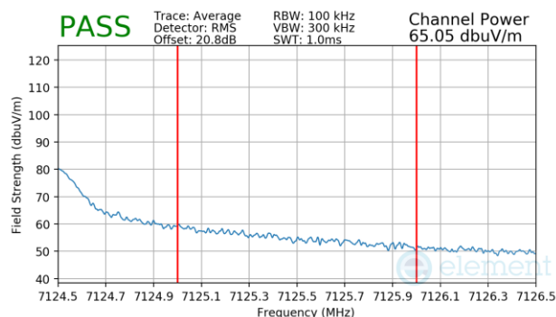
Plot 7-1556 Antenna WF7b Radiated Upper Band Edge (Average – UNII Band 8) – RU242
