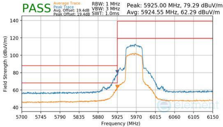
Plot 7-1499 Antenna WF2a Radiated Lower Band Edge (Peak & Average – UNII Band 5) - RU484
