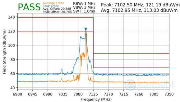
Plot 7-1498 Antenna WF2a Radiated Upper Band Edge (Peak & Average – UNII Band 8) - RU26
