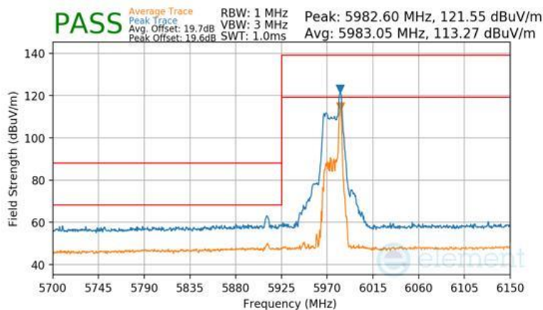
Plot 7-1496 Antenna WF2a Radiated Lower Band Edge (Peak & Average – UNII Band 5) - RU26
