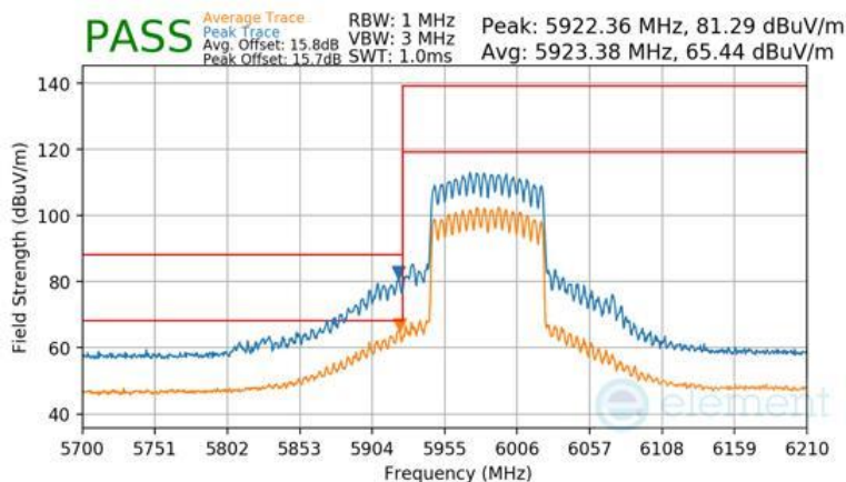
Plot 7-1637 CDD Primary Radiated Lower Band Edge (Peak & Average – UNII Band 5) - RU996
