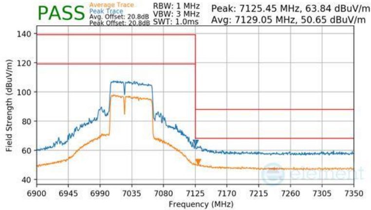
Plot 7-1571 Antenna WF7b Radiated Upper Band Edge (Peak & Average – UNII Band 8) - RU484+242
