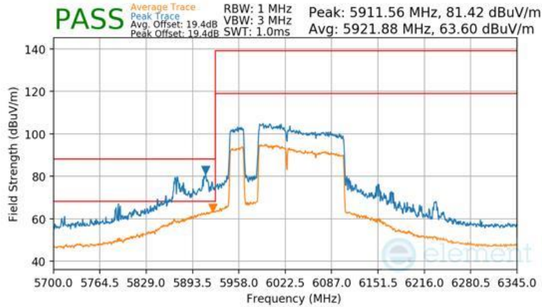
Plot 7-1591 Antenna WF7b Radiated Lower Band Edge (Peak & Average – UNII Band 5) - RU996+484+242 (L)
