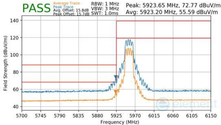
Plot 7-1615 CDD Primary Radiated Lower Band Edge (Peak & Average – UNII Band 5) - RU242
