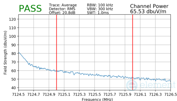
Plot 7-1494 Antenna WF2a Radiated Upper Band Edge (Average – UNII Band 8) – RU242
