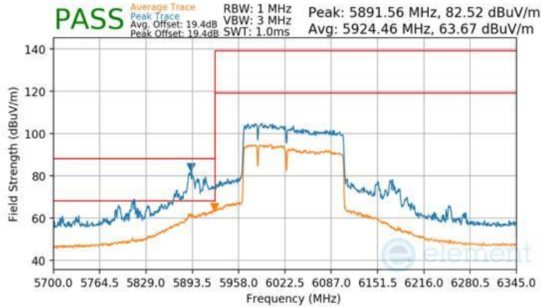
Plot 7-1589 Antenna WF7b Radiated Lower Band Edge (Peak & Average – UNII Band 5) - RU996+484+242 (L)
