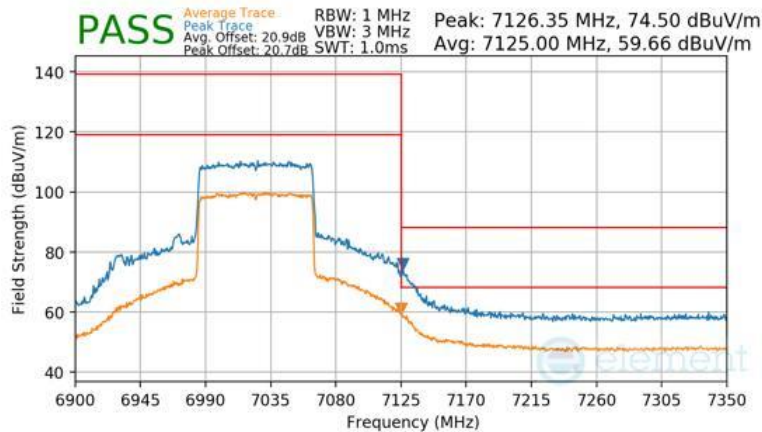
Plot 7-1514 Antenna WF2a Radiated Upper Band Edge (Peak & Average – UNII Band 8) - RU996
