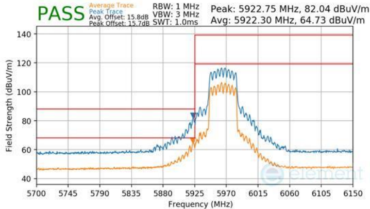
Plot 7-1623 CDD Primary Radiated Lower Band Edge (Peak & Average – UNII Band 5) - RU484
