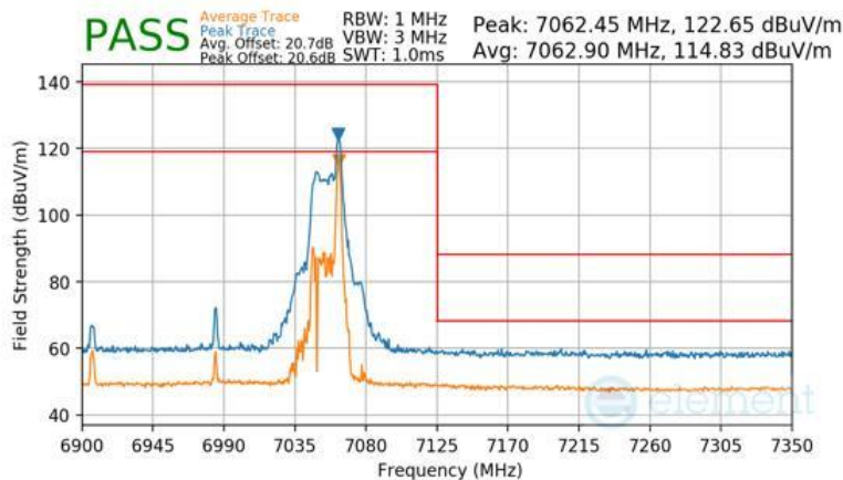
Plot 7-1518 Antenna WF2a Radiated Upper Band Edge (Peak & Average – UNII Band 8) - RU26 (H)
