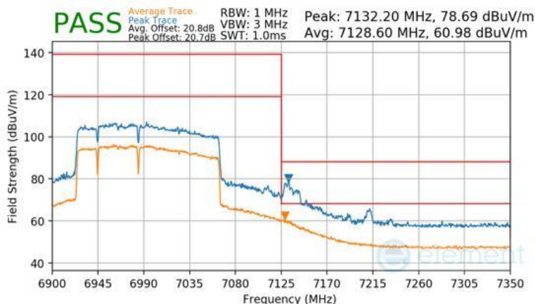
Plot 7-1597 Antenna WF7b Radiated Upper Band Edge (Peak & Average – UNII Band 8) - RU996+484+242 (L)
