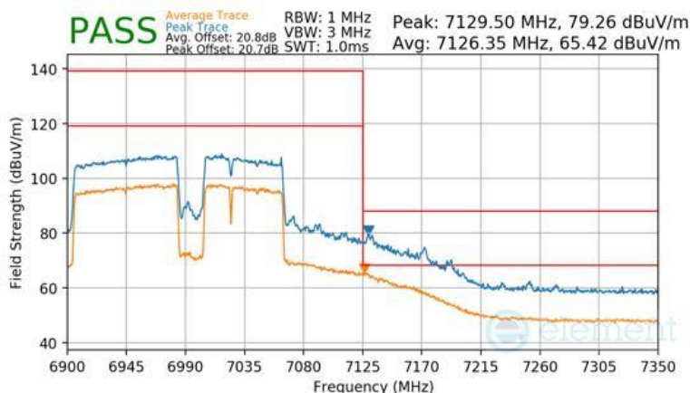
Plot 7-1536 Antenna WF2a Radiated Upper Band Edge (Peak & Average – UNII Band 8) - RU996+484+242 (H)
