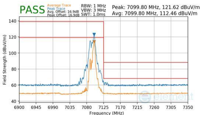
Plot 7-1614 CDD Primary Radiated Upper Band Edge (Peak & Average – UNII Band 8) - RU52+26
