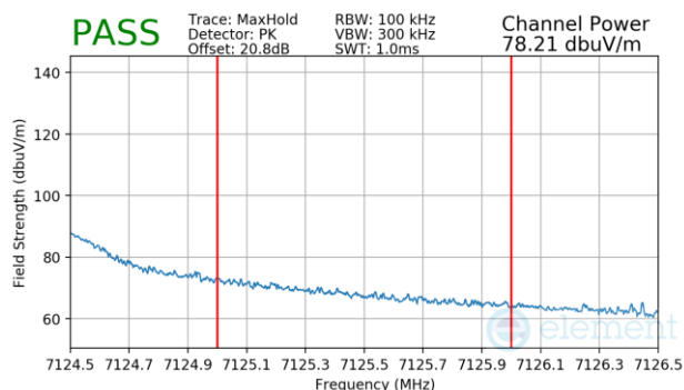
Plot 7-1555 Antenna WF7b Radiated Upper Band Edge (Peak – UNII Band 8) – RU242
