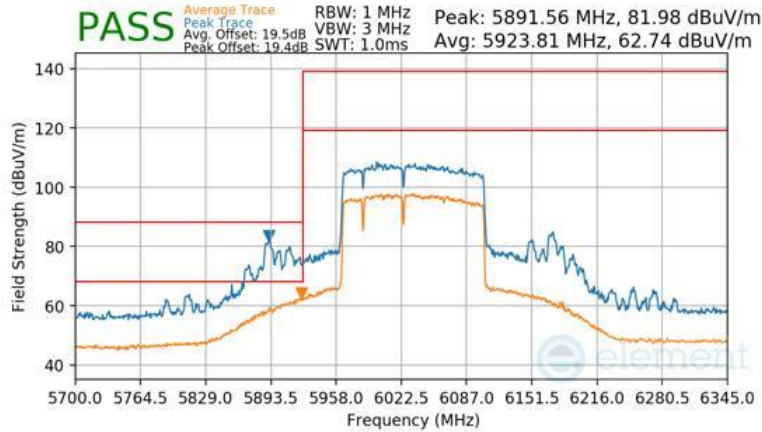
Plot 7-1527 Antenna WF2a Radiated Lower Band Edge (Peak & Average – UNII Band 5) - RU996+484+242 (L)
