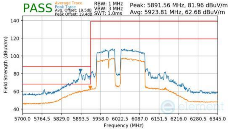
Plot 7-1533 Antenna WF2a Radiated Lower Band Edge (Peak & Average – UNII Band 5) - RU996+484+242 (L)
