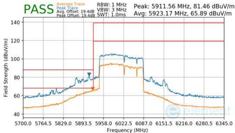
Plot 7-1596 Antenna WF7b Radiated Lower Band Edge (Peak & Average – UNII Band 5) - RU996+484+242 (H)
