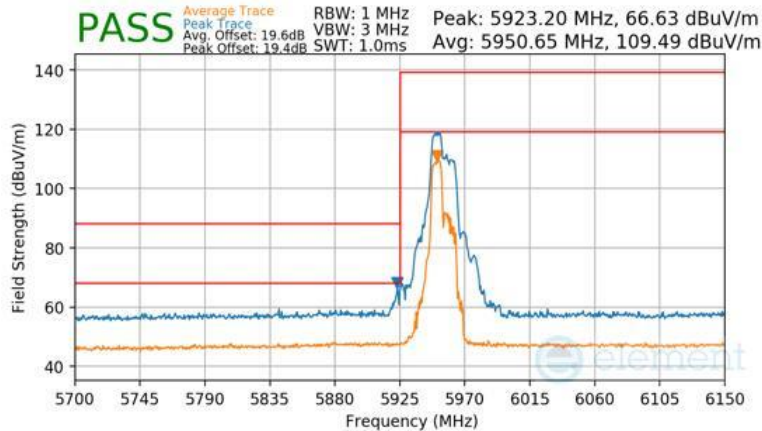
Plot 7-1549 Antenna WF7b Radiated Lower Band Edge (Peak & Average – UNII Band 5) - RU52+26
