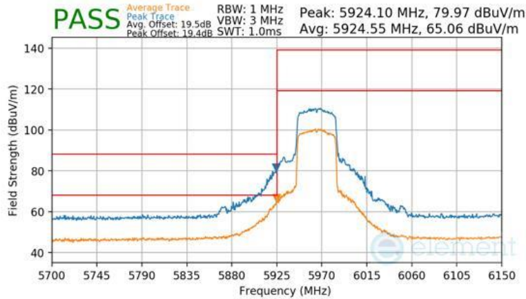
Plot 7-1561 Antenna WF7b Radiated Lower Band Edge (Peak & Average – UNII Band 5) - RU484
