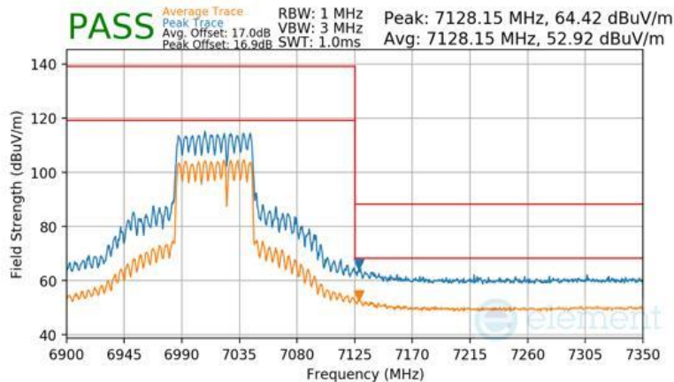
Plot 7-1636 CDD Primary Radiated Upper Band Edge (Peak & Average – UNII Band 8) - RU484+242
