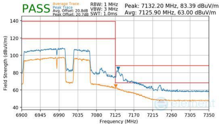
Plot 7-1538 Antenna WF2a Radiated Upper Band Edge (Peak & Average – UNII Band 8) - RU996+484+242 (H)
