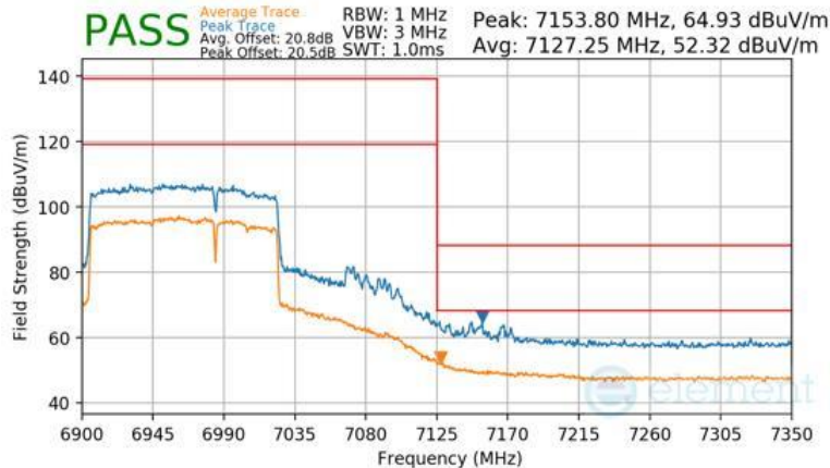
Plot 7-1588 Antenna WF7b Radiated Upper Band Edge (Peak & Average – UNII Band 8) - RU996+484 (H)
