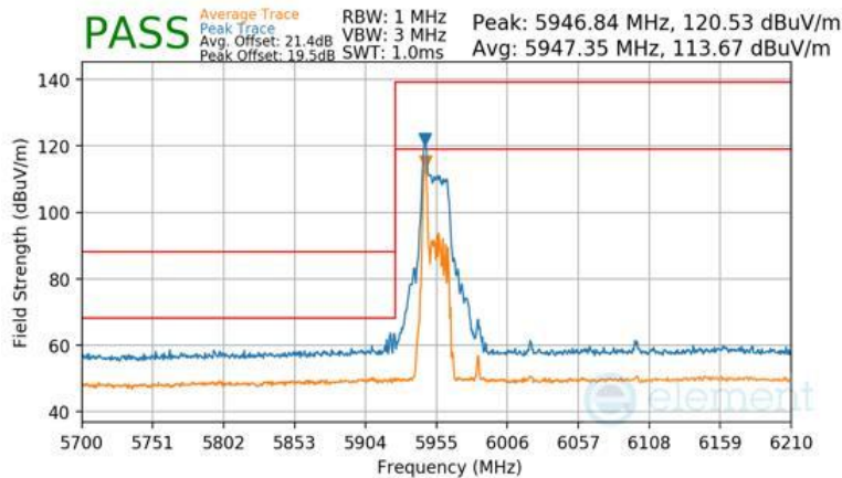
Plot 7-1501 Antenna WF2a Radiated Lower Band Edge (Peak & Average – UNII Band 5) - RU26
