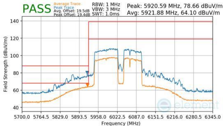
Plot 7-1528 Antenna WF2a Radiated Lower Band Edge (Peak & Average – UNII Band 5) - RU996+484+242 (H)
