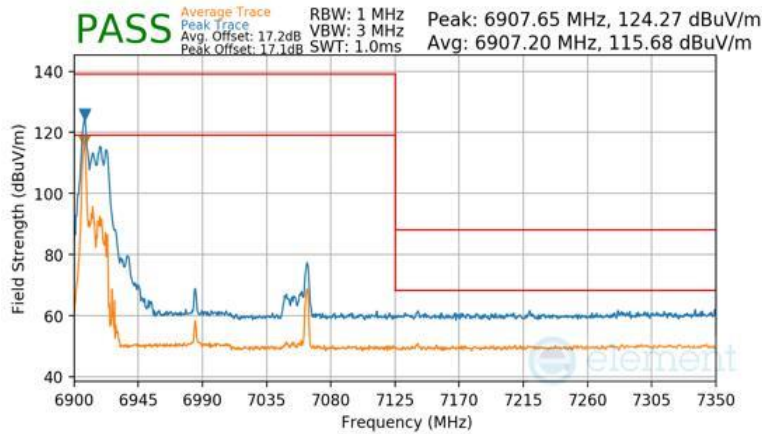
Plot 7-1641 CDD Primary Radiated Upper Band Edge (Peak & Average – UNII Band 8) - RU26 (L)
