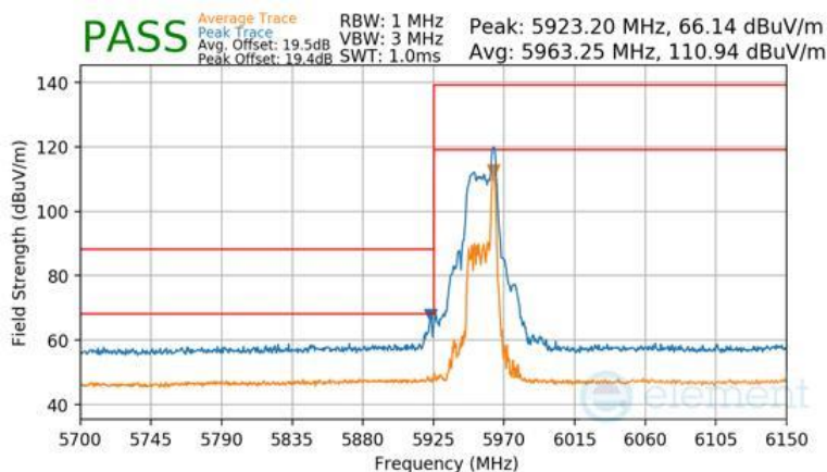
Plot 7-1546 Antenna WF7b Radiated Lower Band Edge (Peak & Average – UNII Band 5) - RU26
