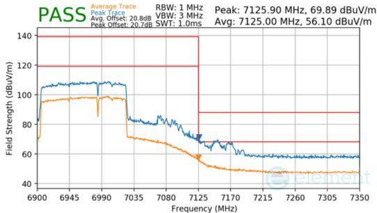
Plot 7-1526 Antenna WF2a Radiated Upper Band Edge (Peak & Average – UNII Band 8) - RU996+484 (H)
