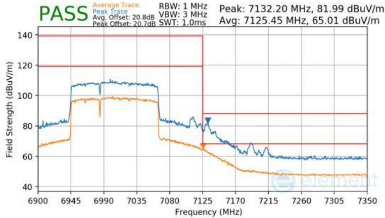
Plot 7-1523 Antenna WF2a Radiated Upper Band Edge (Peak & Average – UNII Band 8) - RU996+484 (L)
