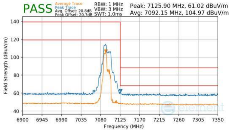
Plot 7-1551 Antenna WF7b Radiated Upper Band Edge (Peak & Average – UNII Band 8) - RU52+26
