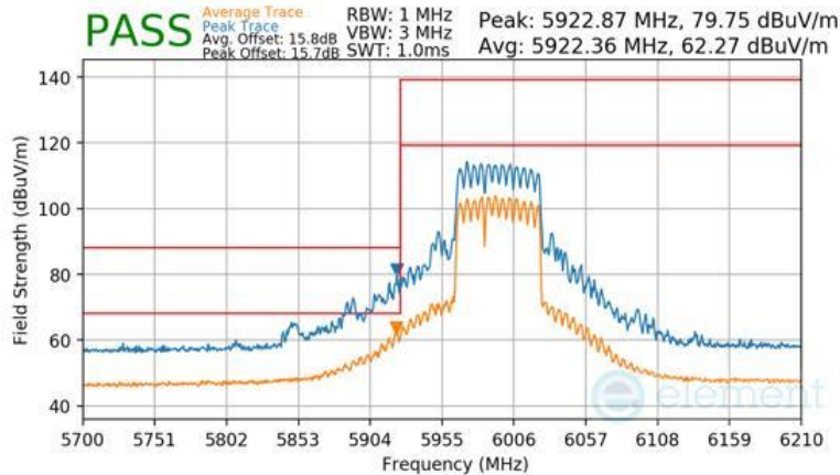
Plot 7-1629 CDD Primary Radiated Lower Band Edge (Peak & Average – UNII Band 5) - RU484+242
