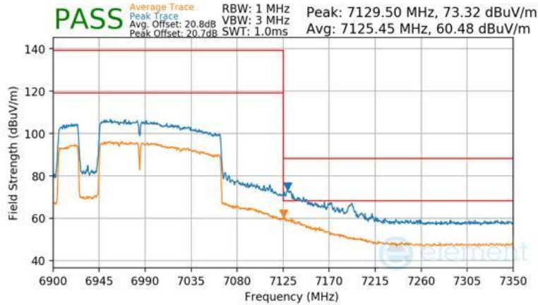
Plot 7-1599 Antenna WF7b Radiated Upper Band Edge (Peak & Average – UNII Band 8) - RU996+484+242 (L)
