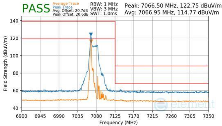
Plot 7-1497 Antenna WF2a Radiated Upper Band Edge (Peak & Average – UNII Band 8) - RU26
