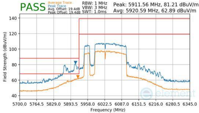
Plot 7-1529 Antenna WF2a Radiated Lower Band Edge (Peak & Average – UNII Band 5) - RU996+484+242 (L)
