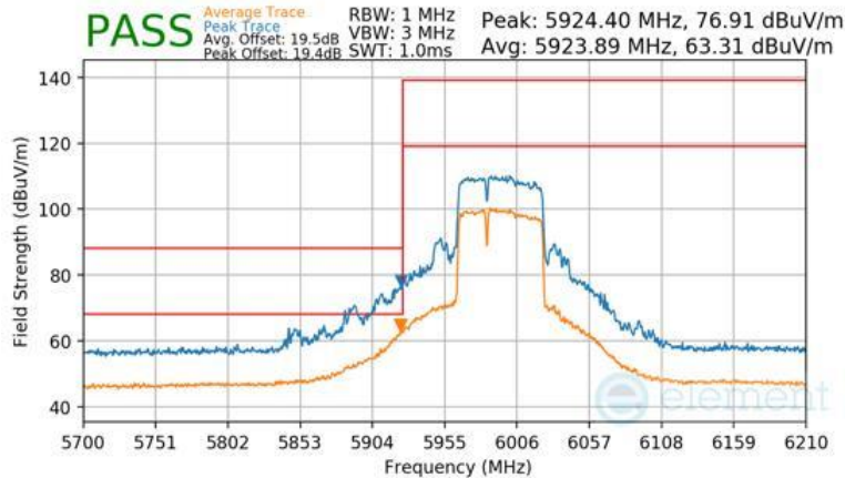
Plot 7-1567 Antenna WF7b Radiated Lower Band Edge (Peak & Average – UNII Band 5) - RU484+242
