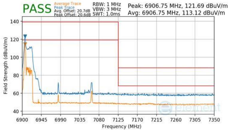
Plot 7-1517 Antenna WF2a Radiated Upper Band Edge (Peak & Average – UNII Band 8) - RU26 (L)
