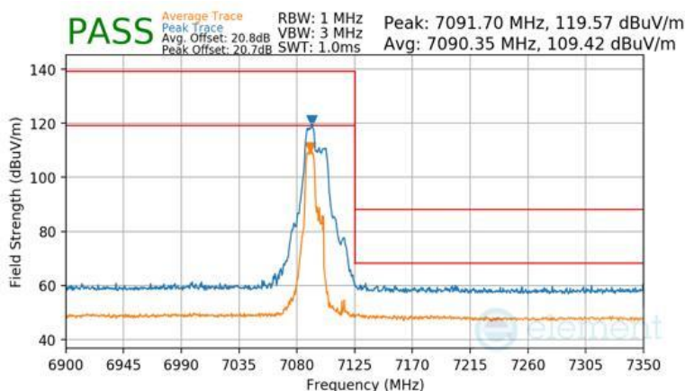
Plot 7-1489 Antenna WF2a Radiated Upper Band Edge (Peak & Average – UNII Band 8) - RU52+26
