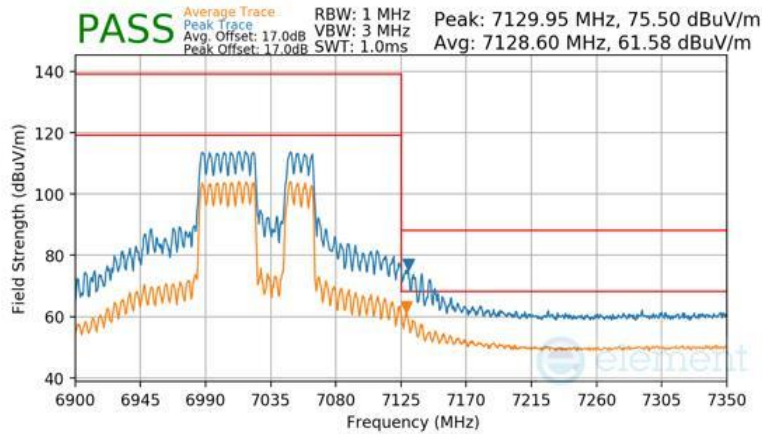
Plot 7-1635 CDD Primary Radiated Upper Band Edge (Peak & Average – UNII Band 8) - RU484+242
