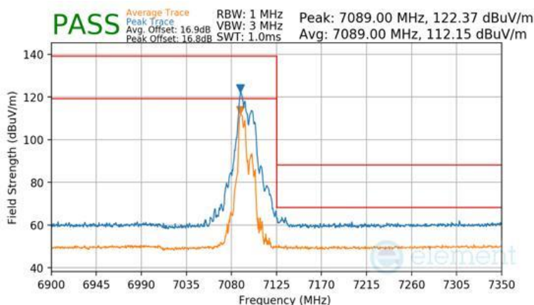
Plot 7-1613 CDD Primary Radiated Upper Band Edge (Peak & Average – UNII Band 8) - RU52+26
