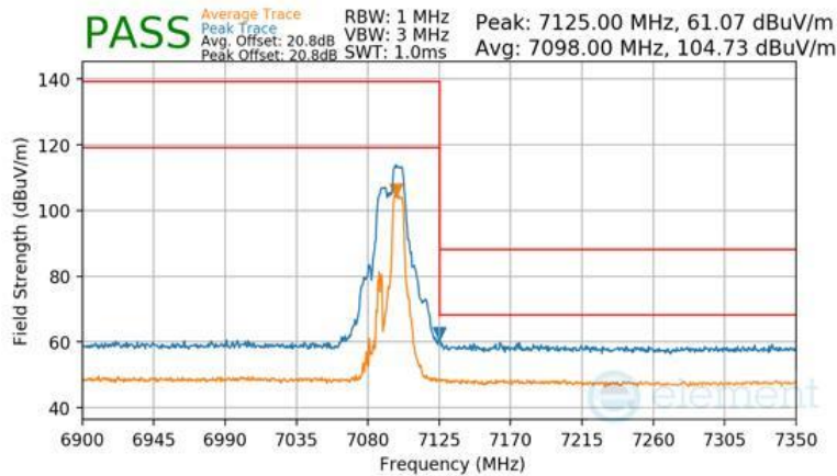
Plot 7-1552 Antenna WF7b Radiated Upper Band Edge (Peak & Average – UNII Band 8) - RU52+26
