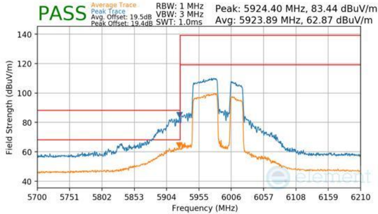
Plot 7-1569 Antenna WF7b Radiated Lower Band Edge (Peak & Average – UNII Band 5) - RU484+242
