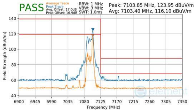
Plot 7-1622 CDD Primary Radiated Upper Band Edge (Peak & Average – UNII Band 8) - RU26
