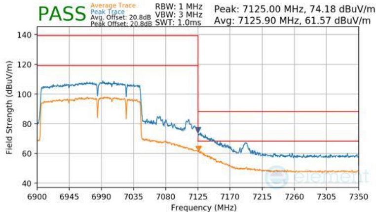
Plot 7-1542 Antenna WF2a Radiated Upper Band Edge (Peak & Average – UNII Band 8) - RU996+484+242 (H)
