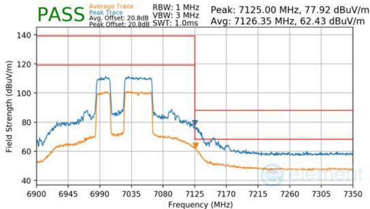
Plot 7-1510 Antenna WF2a Radiated Upper Band Edge (Peak & Average – UNII Band 8) - RU484+242
