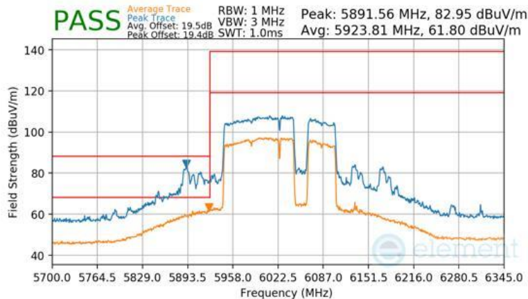
Plot 7-1530 Antenna WF2a Radiated Lower Band Edge (Peak & Average – UNII Band 5) - RU996+484+242 (H)
