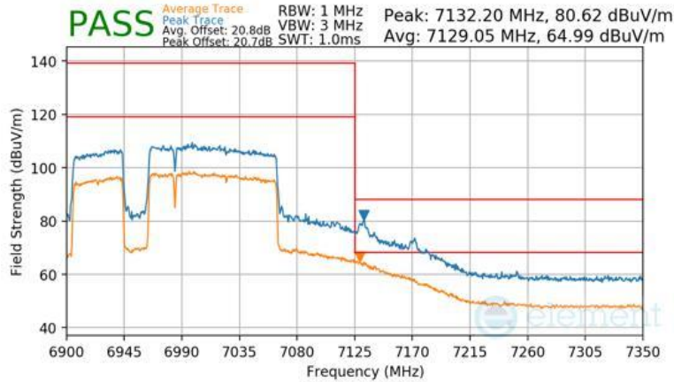
Plot 7-1539 Antenna WF2a Radiated Upper Band Edge (Peak & Average – UNII Band 8) - RU996+484+242 (L)
