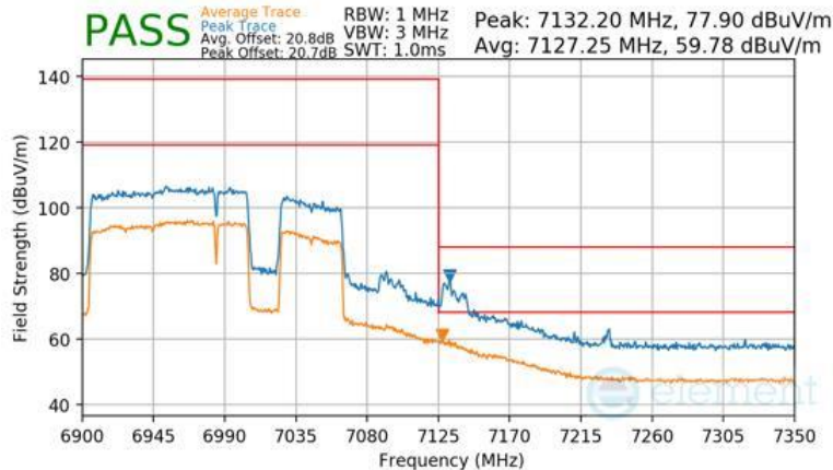
Plot 7-1600 Antenna WF7b Radiated Upper Band Edge (Peak & Average – UNII Band 8) - RU996+484+242 (H)
