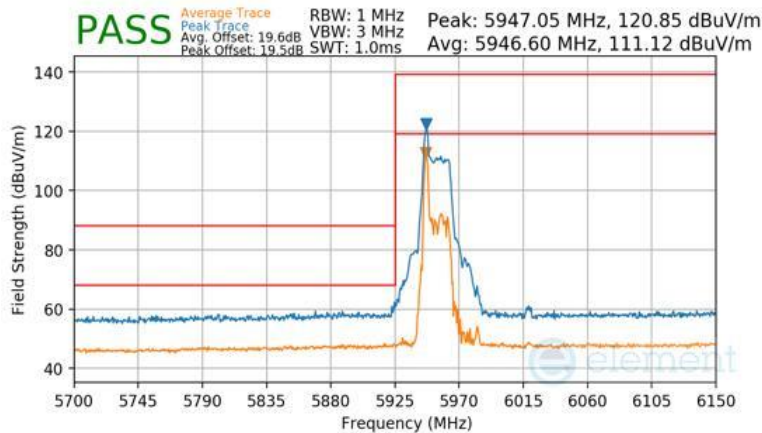
Plot 7-1495 Antenna WF2a Radiated Lower Band Edge (Peak & Average – UNII Band 5) - RU26
