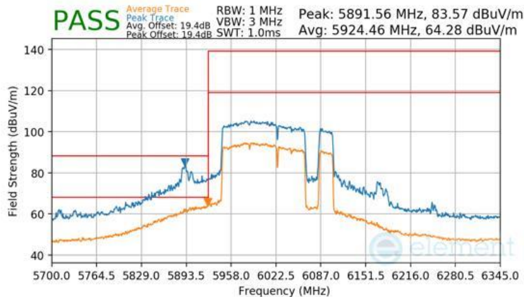
Plot 7-1594 Antenna WF7b Radiated Lower Band Edge (Peak & Average – UNII Band 5) - RU996+484+242 (H)
