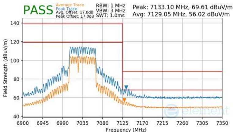
Plot 7-1633 CDD Primary Radiated Upper Band Edge (Peak & Average – UNII Band 8) - RU484+242
