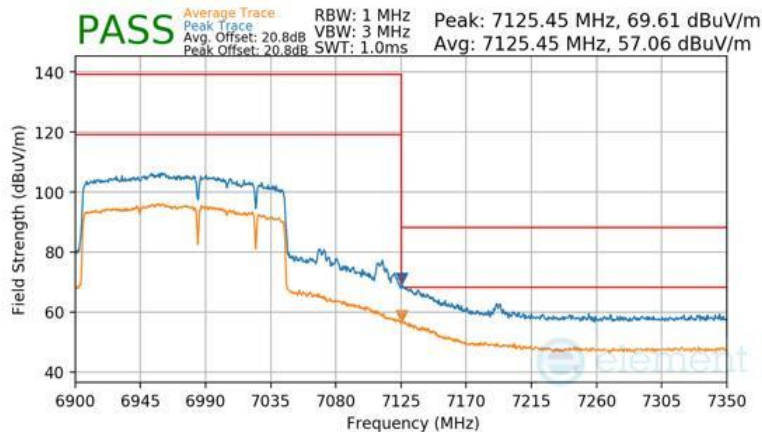
Plot 7-1604 Antenna WF7b Radiated Upper Band Edge (Peak & Average – UNII Band 8) - RU996+484+242 (H)
