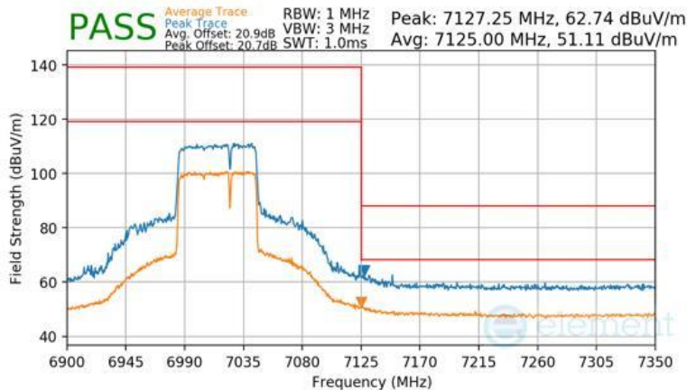
Plot 7-1512 Antenna WF2a Radiated Upper Band Edge (Peak & Average – UNII Band 8) - RU484+242
