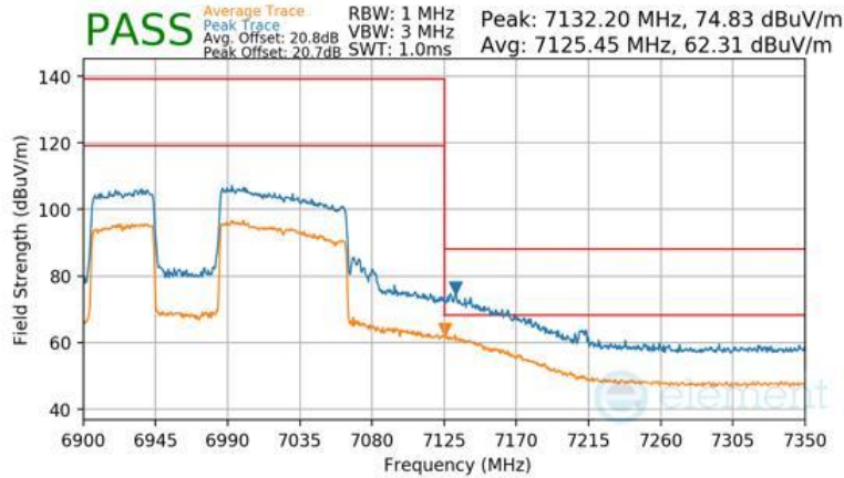
Plot 7-1587 Antenna WF7b Radiated Upper Band Edge (Peak & Average – UNII Band 8) - RU996+484 (L)
