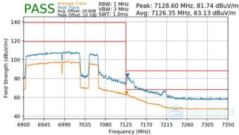
Plot 7-1540 Antenna WF2a Radiated Upper Band Edge (Peak & Average – UNII Band 8) - RU996+484+242 (H)
