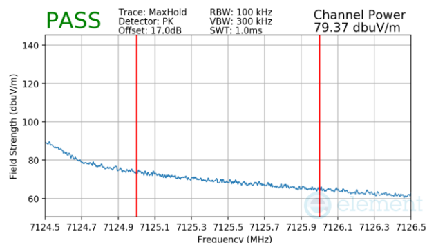
Plot 7-1617 CDD Primary Radiated Upper Band Edge (Peak – UNII Band 8) – RU242
