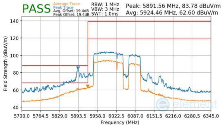
Plot 7-1592 Antenna WF7b Radiated Lower Band Edge (Peak & Average – UNII Band 5) - RU996+484+242 (H)
