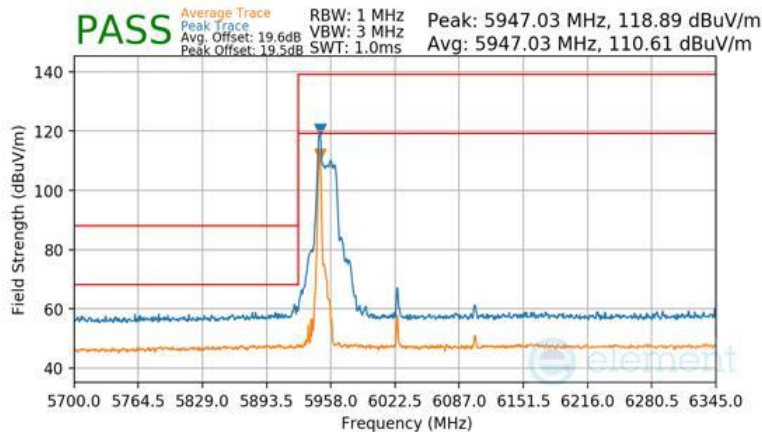
Plot 7-1577 Antenna WF7b Radiated Lower Band Edge (Peak & Average – UNII Band 5) - RU26 (L)
