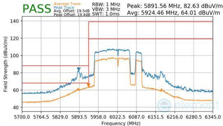
Plot 7-1532 Antenna WF2a Radiated Lower Band Edge (Peak & Average – UNII Band 5) - RU996+484+242 (H)
