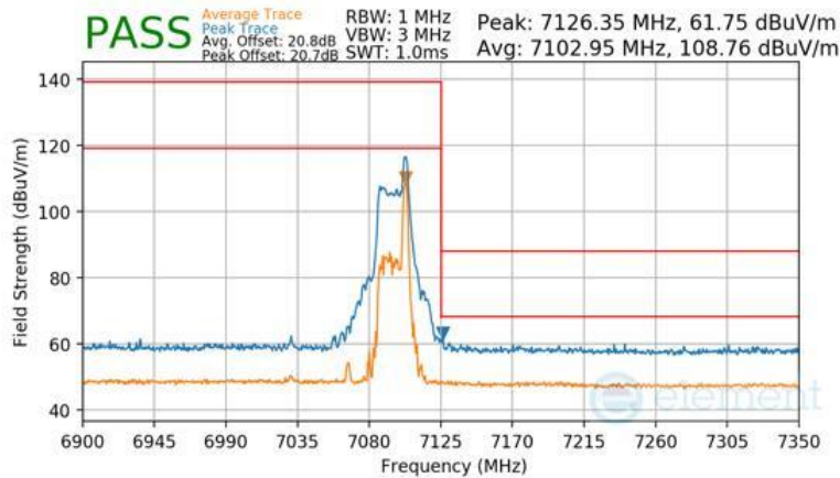
Plot 7-1560 Antenna WF7b Radiated Upper Band Edge (Peak & Average – UNII Band 8) - RU26
