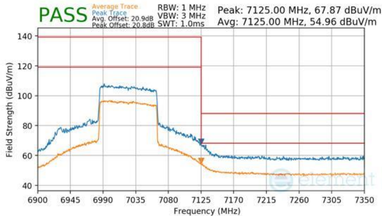
Plot 7-1576 Antenna WF7b Radiated Upper Band Edge (Peak & Average – UNII Band 8) - RU996
