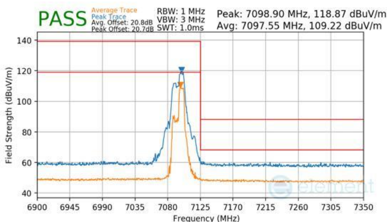
Plot 7-1490 Antenna WF2a Radiated Upper Band Edge (Peak & Average – UNII Band 8) - RU52+26
