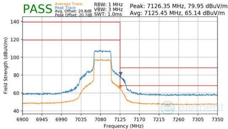
Plot 7-1562 Antenna WF7b Radiated Upper Band Edge (Peak & Average – UNII Band 8) - RU484
