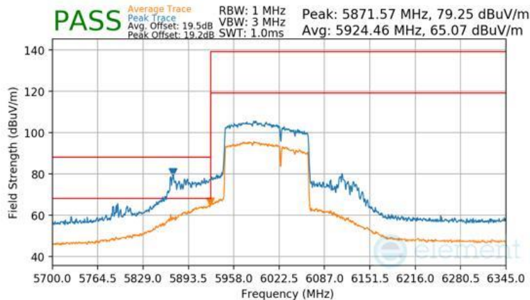
Plot 7-1584 Antenna WF7b Radiated Lower Band Edge (Peak & Average – UNII Band 5) - RU996+484 (H)
