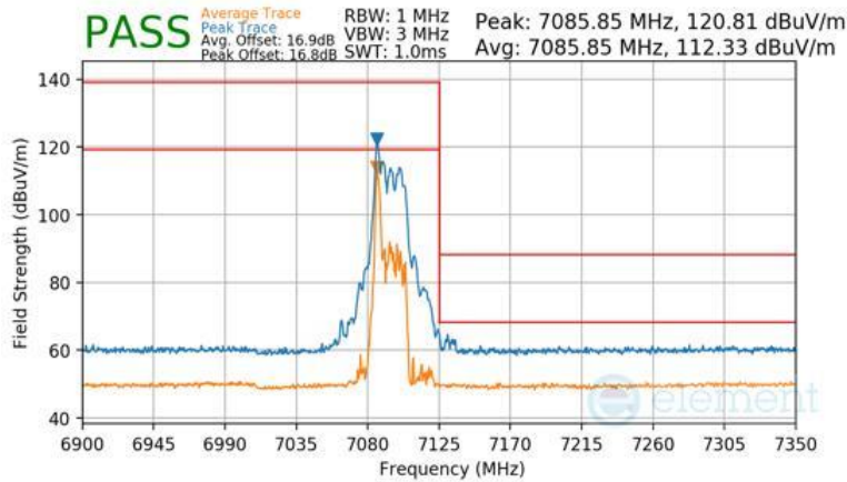
Plot 7-1609 CDD Primary Radiated Upper Band Edge (Peak & Average – UNII Band 8) - RU26
