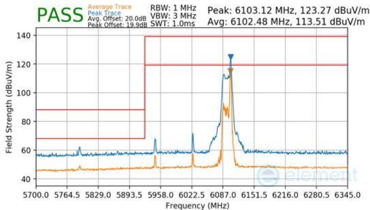
Plot 7-1516 Antenna WF2a Radiated Lower Band Edge (Peak & Average – UNII Band 5) - RU26 (H)
