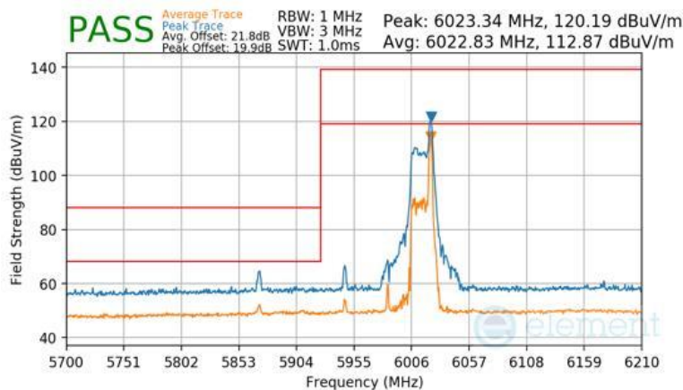
Plot 7-1502 Antenna WF2a Radiated Lower Band Edge (Peak & Average – UNII Band 5) - RU26
