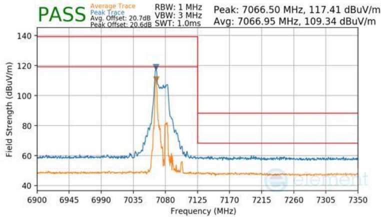
Plot 7-1559 Antenna WF7b Radiated Upper Band Edge (Peak & Average – UNII Band 8) - RU26
