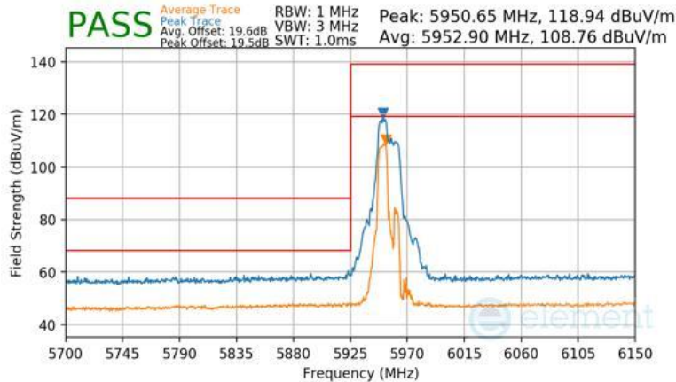
Plot 7-1487 Antenna WF2a Radiated Lower Band Edge (Peak & Average – UNII Band 5) - RU52+26
