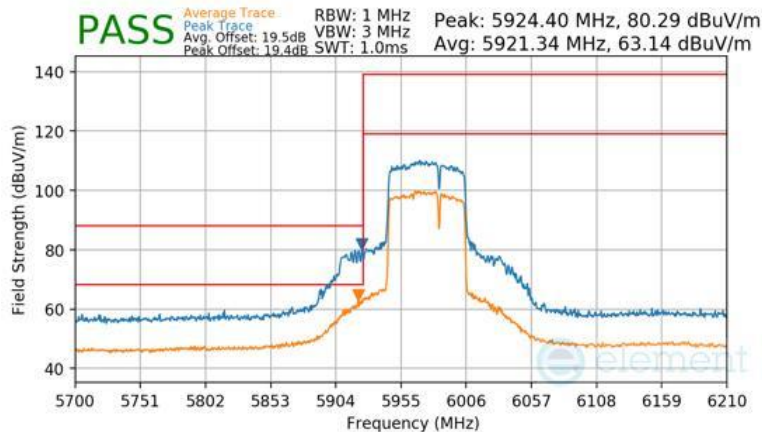
Plot 7-1508 Antenna WF2a Radiated Lower Band Edge (Peak & Average – UNII Band 5) - RU484+242
