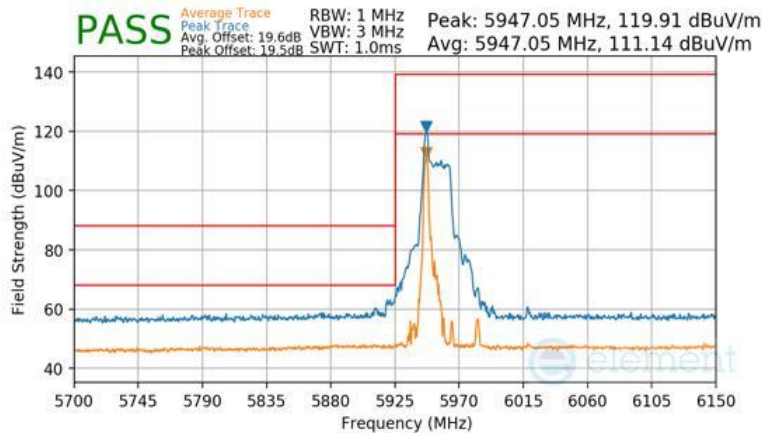
Plot 7-1557 Antenna WF7b Radiated Lower Band Edge (Peak & Average – UNII Band 5) - RU26
