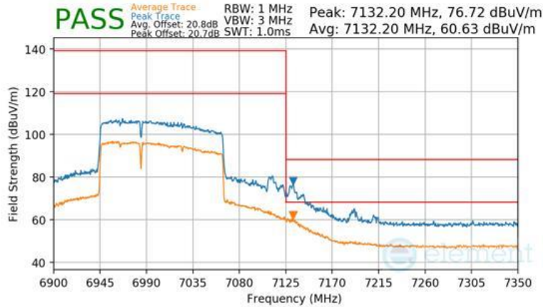
Plot 7-1585 Antenna WF7b Radiated Upper Band Edge (Peak & Average – UNII Band 8) - RU996+484 (L)
