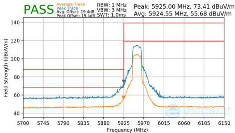
Plot 7-1553 Antenna WF7b Radiated Lower Band Edge (Peak & Average – UNII Band 5) - RU242
