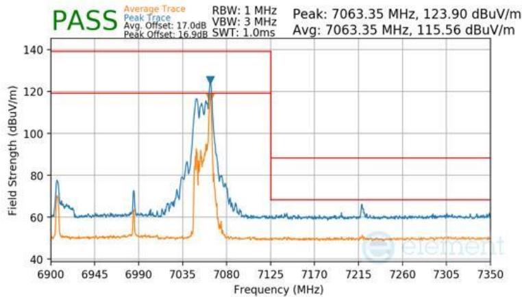
Plot 7-1642 CDD Primary Radiated Upper Band Edge (Peak & Average – UNII Band 8) - RU26 (H)
