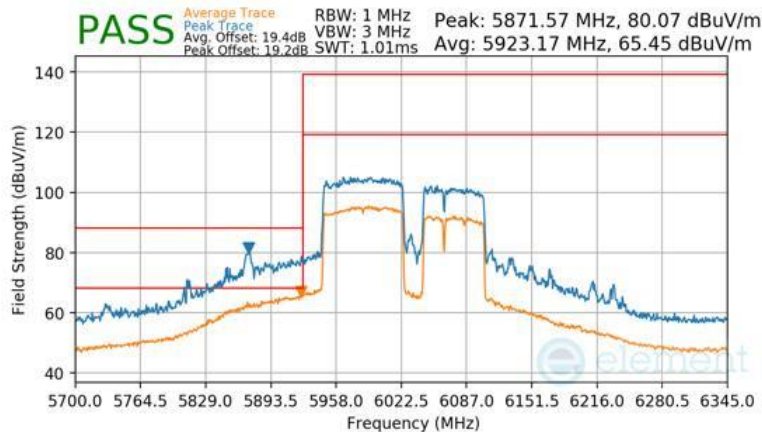
Plot 7-1590 Antenna WF7b Radiated Lower Band Edge (Peak & Average – UNII Band 5) - RU996+484+242 (H)
