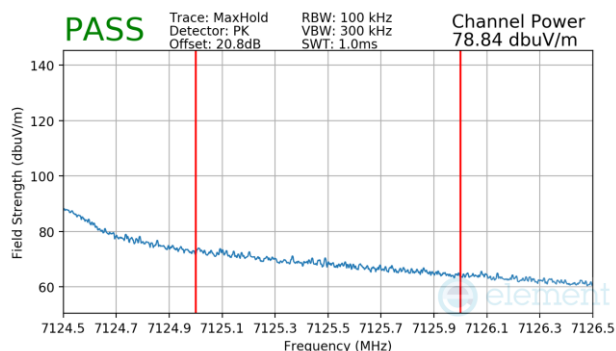
Plot 7-1493 Antenna WF2a Radiated Upper Band Edge (Peak – UNII Band 8) – RU242
