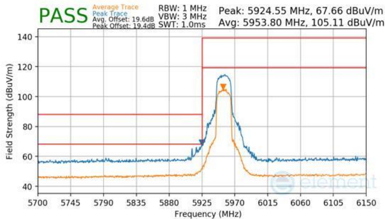
Plot 7-1491 Antenna WF2a Radiated Lower Band Edge (Peak & Average – UNII Band 5) - RU242
