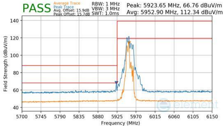
Plot 7-1611 CDD Primary Radiated Lower Band Edge (Peak & Average – UNII Band 5) - RU52+26
