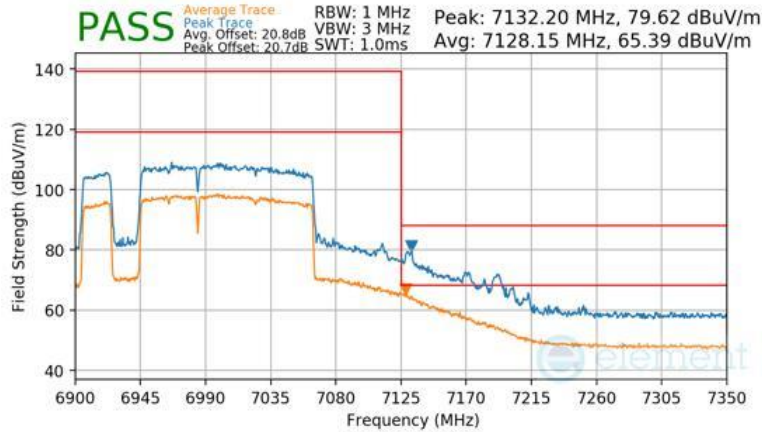
Plot 7-1537 Antenna WF2a Radiated Upper Band Edge (Peak & Average – UNII Band 8) - RU996+484+242 (L)
