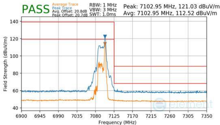
Plot 7-1486 Antenna WF2a Radiated Upper Band Edge (Peak & Average – UNII Band 8) - RU26
