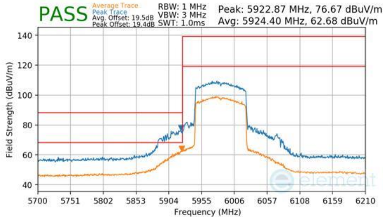
Plot 7-1513 Antenna WF2a Radiated Lower Band Edge (Peak & Average – UNII Band 5) - RU996
