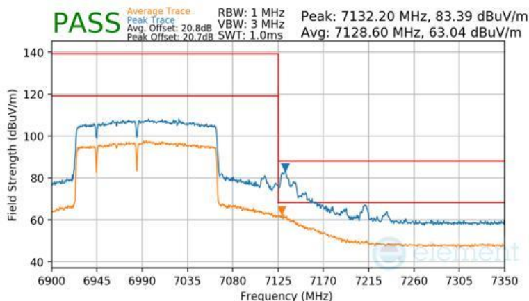
Plot 7-1535 Antenna WF2a Radiated Upper Band Edge (Peak & Average – UNII Band 8) - RU996+484+242 (L)
