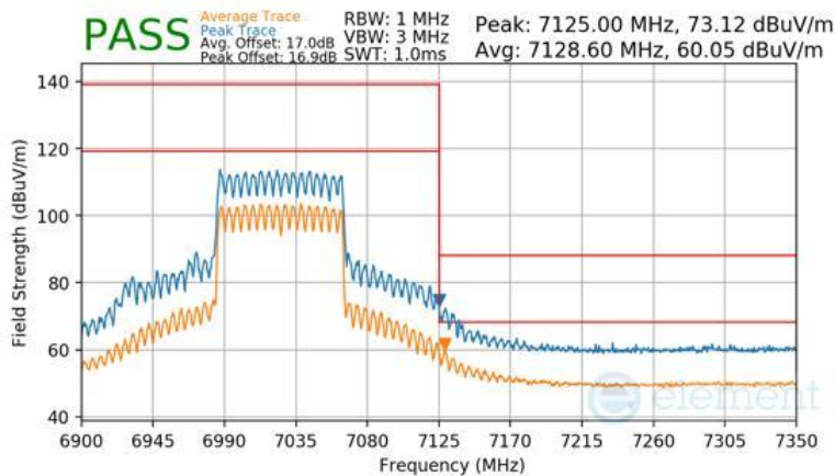
Plot 7-1638 CDD Primary Radiated Upper Band Edge (Peak & Average – UNII Band 8) - RU996
