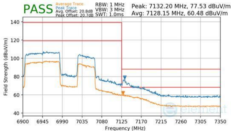
Plot 7-1586 Antenna WF7b Radiated Upper Band Edge (Peak & Average – UNII Band 8) - RU996+484 (H)
