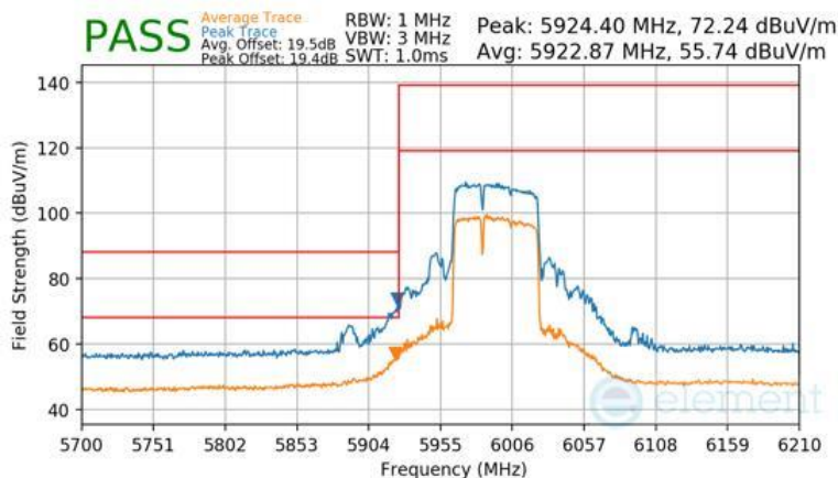
Plot 7-1505 Antenna WF2a Radiated Lower Band Edge (Peak & Average – UNII Band 5) - RU484+242
