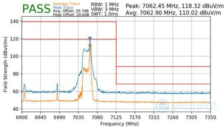
Plot 7-1580 Antenna WF7b Radiated Upper Band Edge (Peak & Average – UNII Band 8) - RU26 (H)
