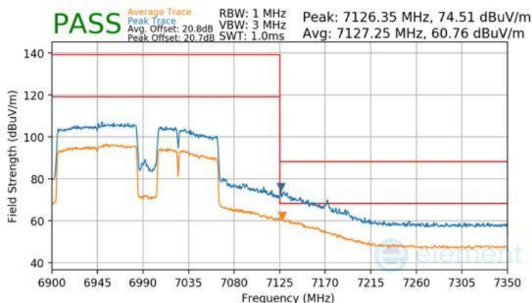
Plot 7-1598 Antenna WF7b Radiated Upper Band Edge (Peak & Average – UNII Band 8) - RU996+484+242 (H)
