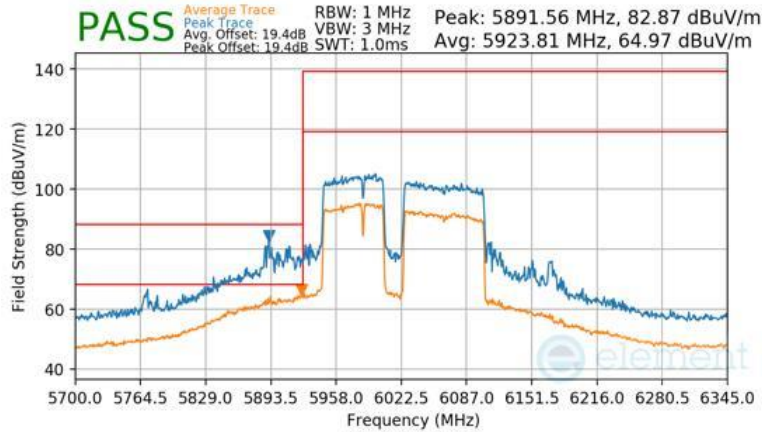
Plot 7-1595 Antenna WF7b Radiated Lower Band Edge (Peak & Average – UNII Band 5) - RU996+484+242 (L)
