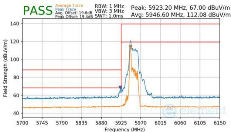
Plot 7-1545 Antenna WF7b Radiated Lower Band Edge (Peak & Average – UNII Band 5) - RU26
