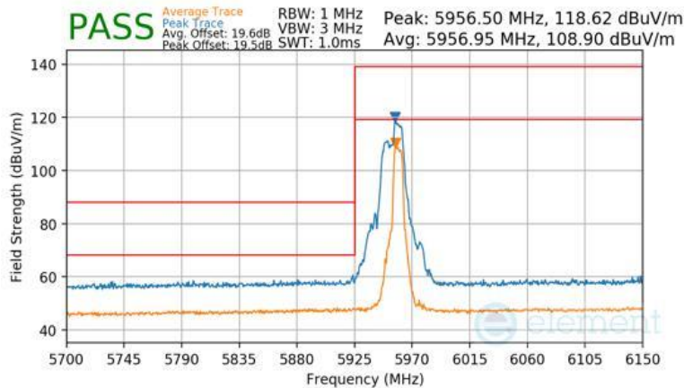
Plot 7-1488 Antenna WF2a Radiated Lower Band Edge (Peak & Average – UNII Band 5) - RU52+26
