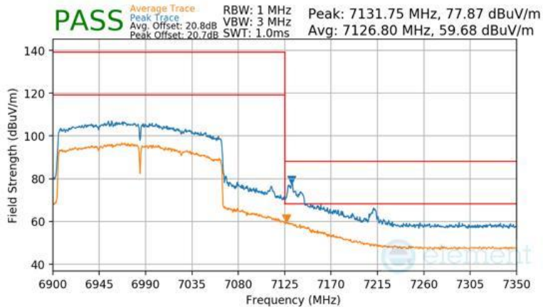
Plot 7-1606 Antenna WF7b Radiated Upper Band Edge (Peak & Average – UNII Band 8) - RU996X2
