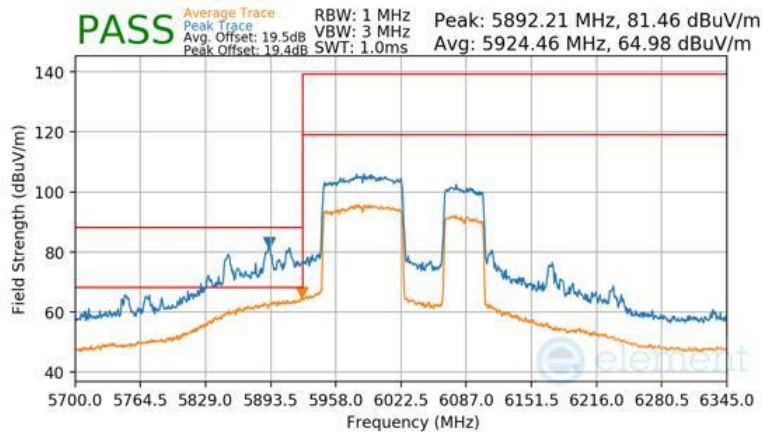
Plot 7-1582 Antenna WF7b Radiated Lower Band Edge (Peak & Average – UNII Band 5) - RU996+484 (H)
