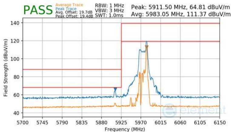
Plot 7-1558 Antenna WF7b Radiated Lower Band Edge (Peak & Average – UNII Band 5) - RU26
