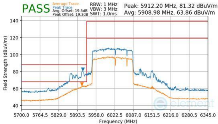
Plot 7-1534 Antenna WF2a Radiated Lower Band Edge (Peak & Average – UNII Band 5) - RU996+484+242 (H)
