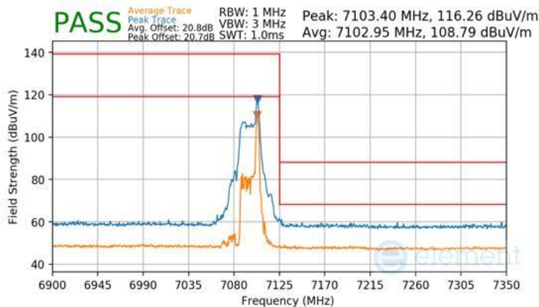
Plot 7-1548 Antenna WF7b Radiated Upper Band Edge (Peak & Average – UNII Band 8) - RU26
