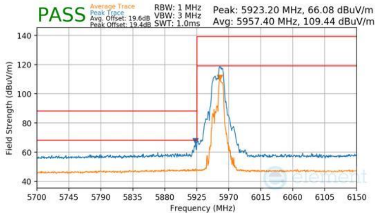
Plot 7-1550 Antenna WF7b Radiated Lower Band Edge (Peak & Average – UNII Band 5) - RU52+26
