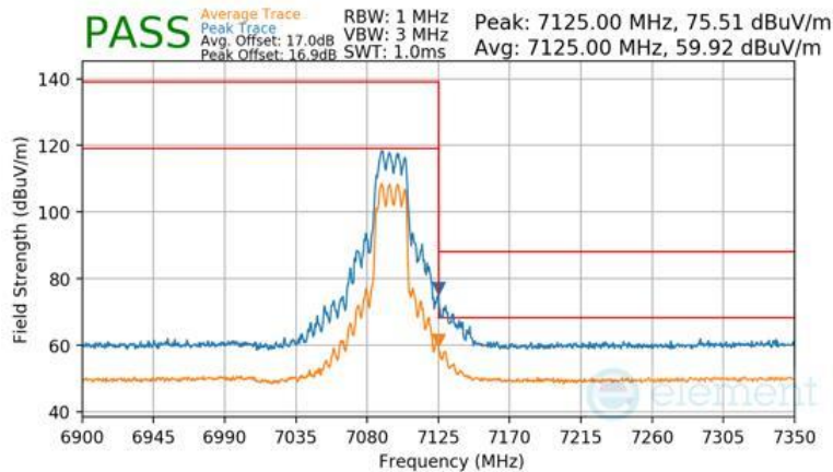
Plot 7-1616 CDD Primary Radiated Upper Band Edge (Peak & Average – UNII Band 8) - RU242
