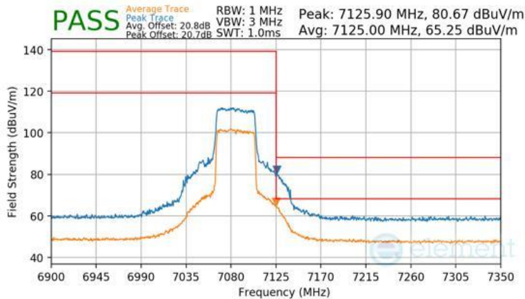
Plot 7-1500 Antenna WF2a Radiated Upper Band Edge (Peak & Average – UNII Band 8) - RU484
