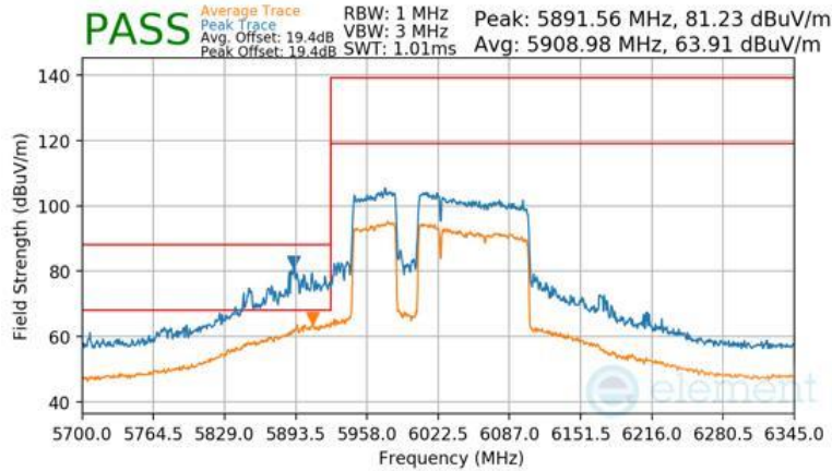
Plot 7-1593 Antenna WF7b Radiated Lower Band Edge (Peak & Average – UNII Band 5) - RU996+484+242 (L)
