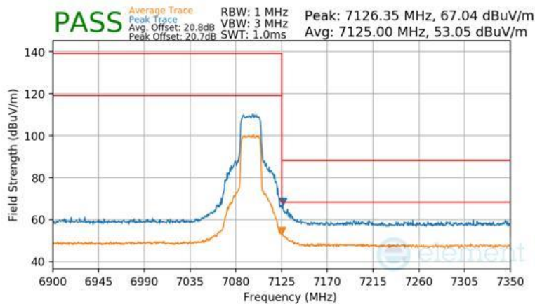
Plot 7-1554 Antenna WF7b Radiated Upper Band Edge (Peak & Average – UNII Band 8) - RU242
