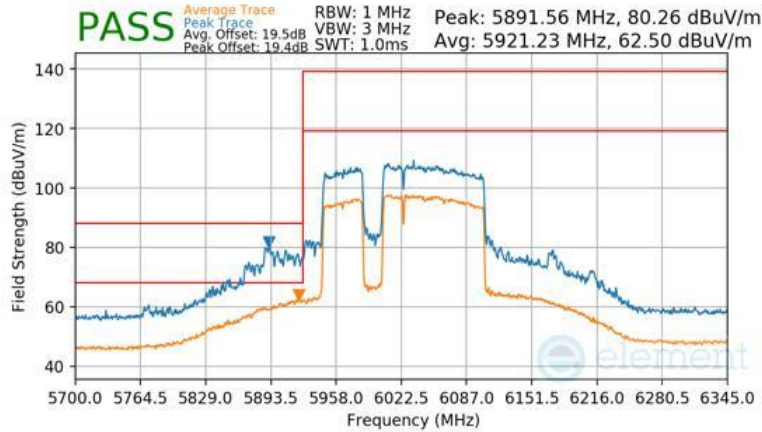
Plot 7-1531 Antenna WF2a Radiated Lower Band Edge (Peak & Average – UNII Band 5) - RU996+484+242 (L)
