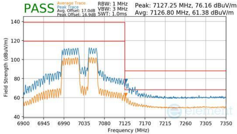
Plot 7-1697 CDD Diversity Radiated Upper Band Edge (Peak & Average – UNII Band 8) - RU484+242
