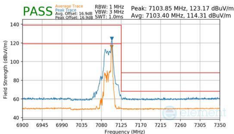
Plot 7-1672 CDD Diversity Radiated Upper Band Edge (Peak & Average – UNII Band 8) - RU26
