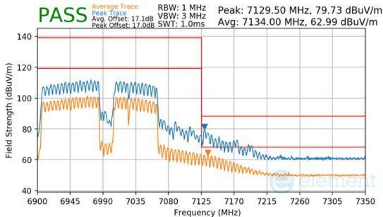
Plot 7-1660 CDD Primary Radiated Upper Band Edge (Peak & Average – UNII Band 8) - RU996+484+242 (H)
