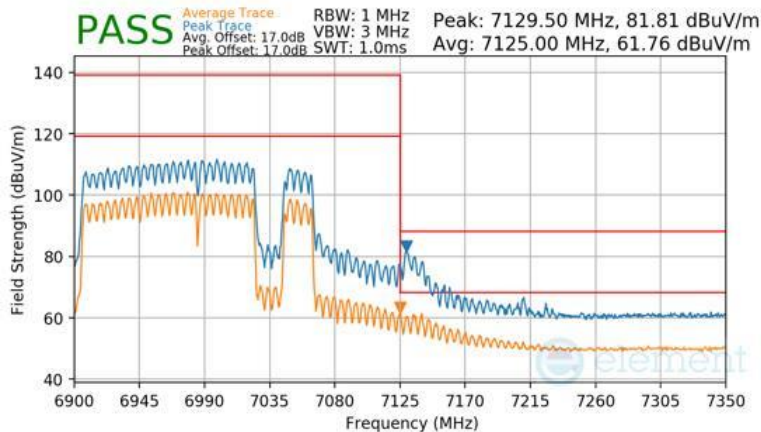
Plot 7-1664 CDD Primary Radiated Upper Band Edge (Peak & Average – UNII Band 8) - RU996+484+242 (H)
