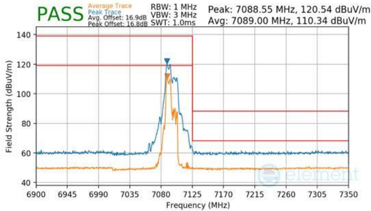
Plot 7-1675 CDD Diversity Radiated Upper Band Edge (Peak & Average – UNII Band 8) - RU52+26
