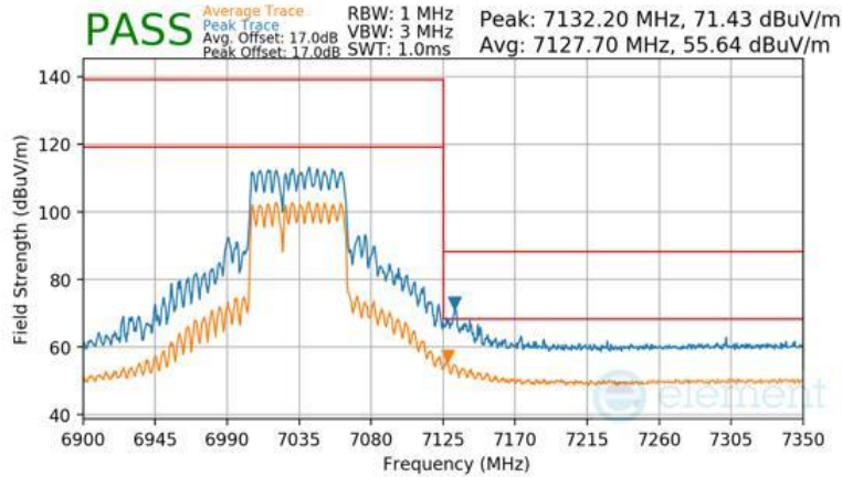
Plot 7-1695 CDD Diversity Radiated Upper Band Edge (Peak & Average – UNII Band 8) - RU484+242
