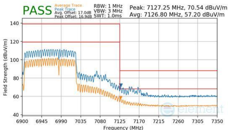
Plot 7-1712 CDD Diversity Radiated Upper Band Edge (Peak & Average – UNII Band 8) - RU996+484 (H)
