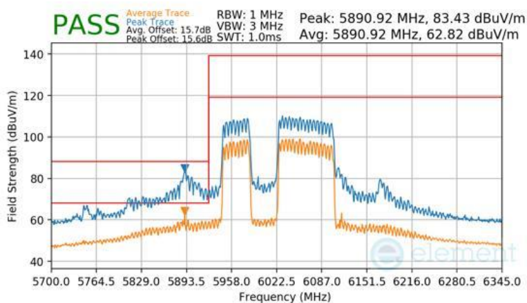
Plot 7-1707 CDD Diversity Radiated Lower Band Edge (Peak & Average – UNII Band 5) - RU996+484 (L)
