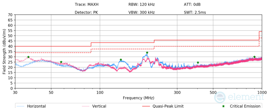
Plot 7-1734. Radiated Spurious Emissions below 1GHz CDD Diversity (802.11be – Ch.45 – RU242) with AC/DC Adapter
