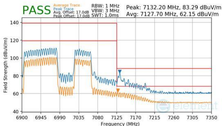
Plot 7-1710 CDD Diversity Radiated Upper Band Edge (Peak & Average – UNII Band 8) - RU996+484 (H)
