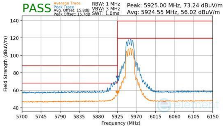
Plot 7-1677 CDD Diversity Radiated Lower Band Edge (Peak & Average – UNII Band 5) - RU242
