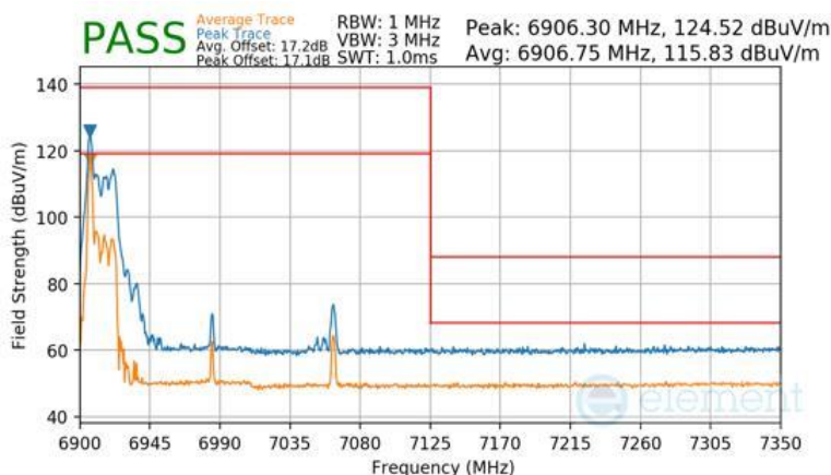
Plot 7-1703 CDD Diversity Radiated Upper Band Edge (Peak & Average – UNII Band 8) - RU26 (L)
