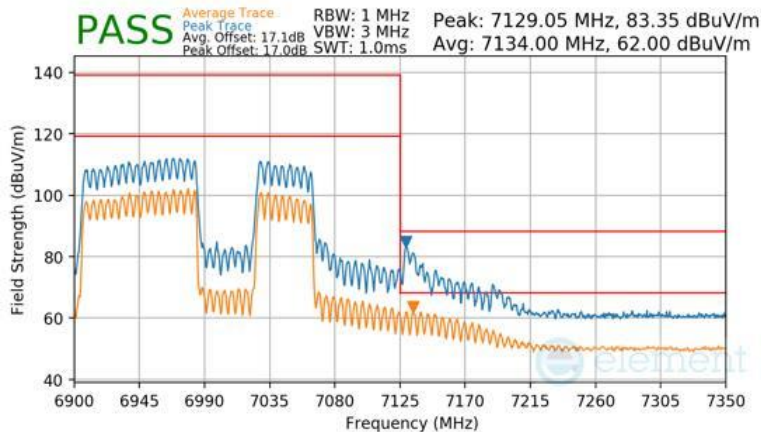
Plot 7-1648 CDD Primary Radiated Upper Band Edge (Peak & Average – UNII Band 8) - RU996+484 (H)
