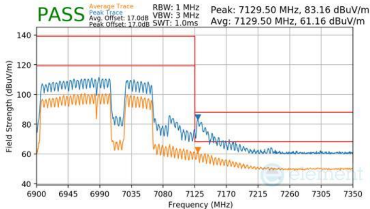
Plot 7-1662 CDD Primary Radiated Upper Band Edge (Peak & Average – UNII Band 8) - RU996+484+242 (H)
