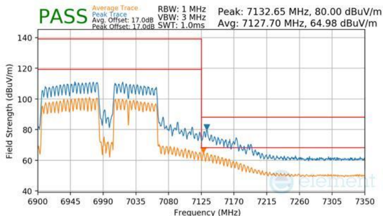
Plot 7-1722 CDD Diversity Radiated Upper Band Edge (Peak & Average – UNII Band 8) - RU996+484+242 (H)
