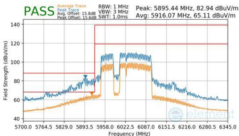
Plot 7-1717 CDD Diversity Radiated Lower Band Edge (Peak & Average – UNII Band 5) - RU996+484+242 (L)
