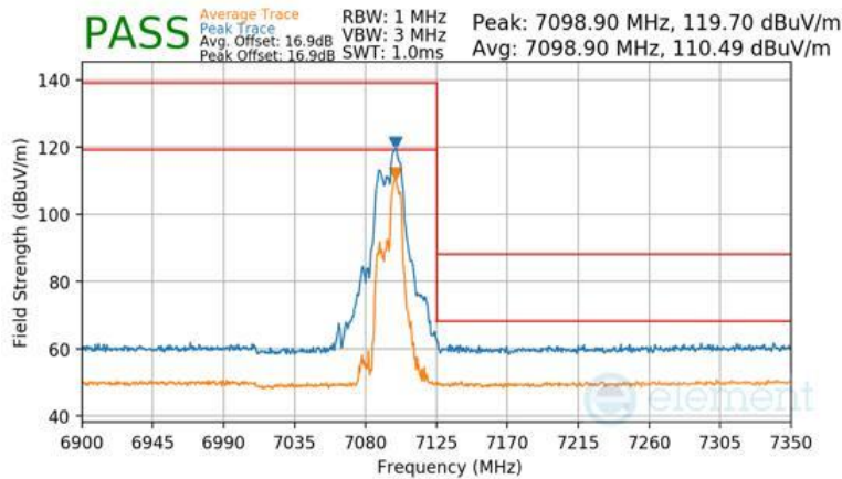
Plot 7-1676 CDD Diversity Radiated Upper Band Edge (Peak & Average – UNII Band 8) - RU52+26
