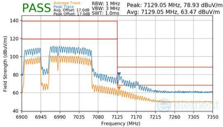
Plot 7-1663 CDD Primary Radiated Upper Band Edge (Peak & Average – UNII Band 8) - RU996+484+242 (L)
