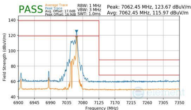
Plot 7-1704 CDD Diversity Radiated Upper Band Edge (Peak & Average – UNII Band 8) - RU26 (H)
