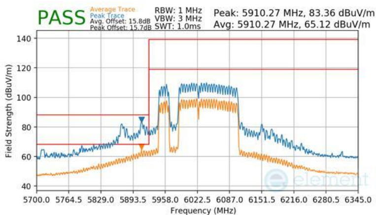
Plot 7-1715 CDD Diversity Radiated Lower Band Edge (Peak & Average – UNII Band 5) - RU996+484+242 (L)
