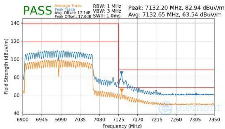
Plot 7-1730 CDD Diversity Radiated Upper Band Edge (Peak & Average – UNII Band 8) - RU996X2
