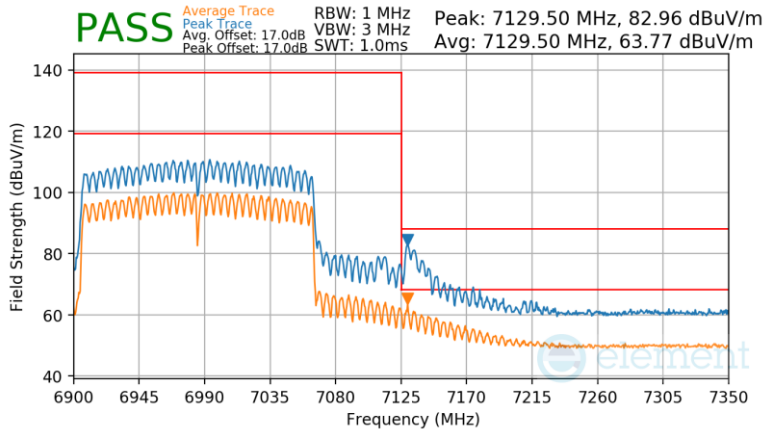
Plot 7-1668 CDD Primary Radiated Upper Band Edge (Peak & Average – UNII Band 8) - RU996X2
