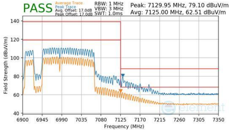
Plot 7-1661 CDD Primary Radiated Upper Band Edge (Peak & Average – UNII Band 8) - RU996+484+242 (L)
