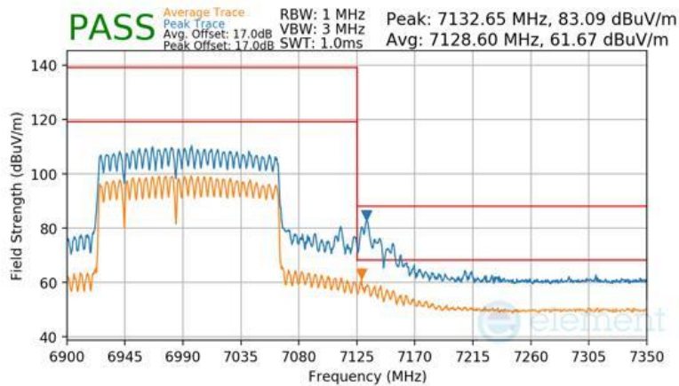
Plot 7-1721 CDD Diversity Radiated Upper Band Edge (Peak & Average – UNII Band 8) - RU996+484+242 (L)
