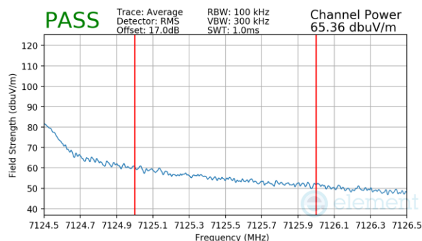
Plot 7-1680 CDD Diversity Radiated Upper Band Edge (Average – UNII Band 8) – RU242
