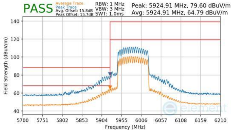
Plot 7-1699 CDD Diversity Radiated Lower Band Edge (Peak & Average – UNII Band 5) - RU996
