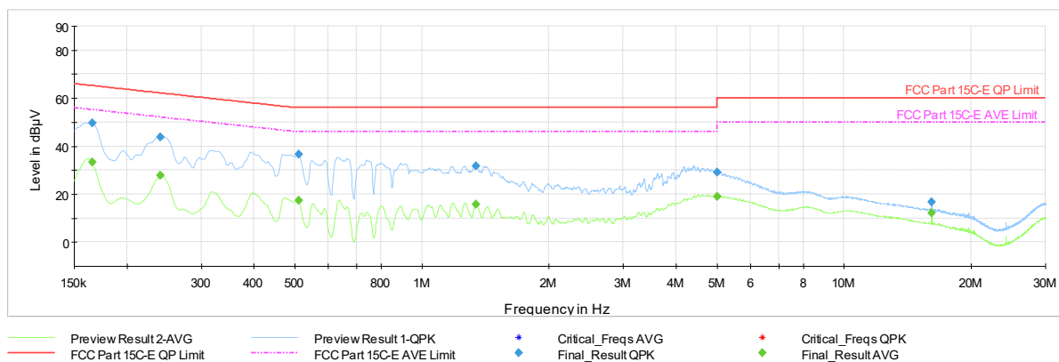
Plot 7-1739. AC Line Conducted Plot with 11be CDD Diversity UNII Band 5 – RU26 – Ch.45 (L1) with AC/DC Adapter
