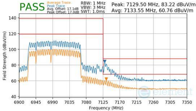
Plot 7-1659 CDD Primary Radiated Upper Band Edge (Peak & Average – UNII Band 8) - RU996+484+242 (L)
