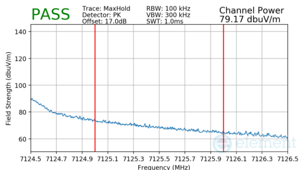
Plot 7-1679 CDD Diversity Radiated Upper Band Edge (Peak – UNII Band 8) – RU242
