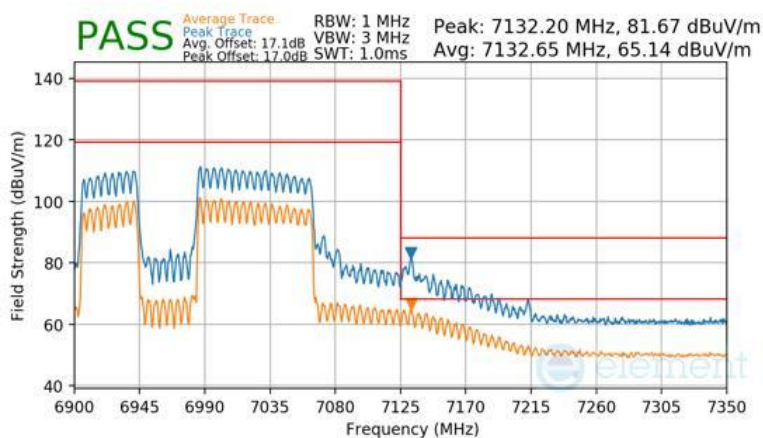
Plot 7-1711 CDD Diversity Radiated Upper Band Edge (Peak & Average – UNII Band 8) - RU996+484 (L)
