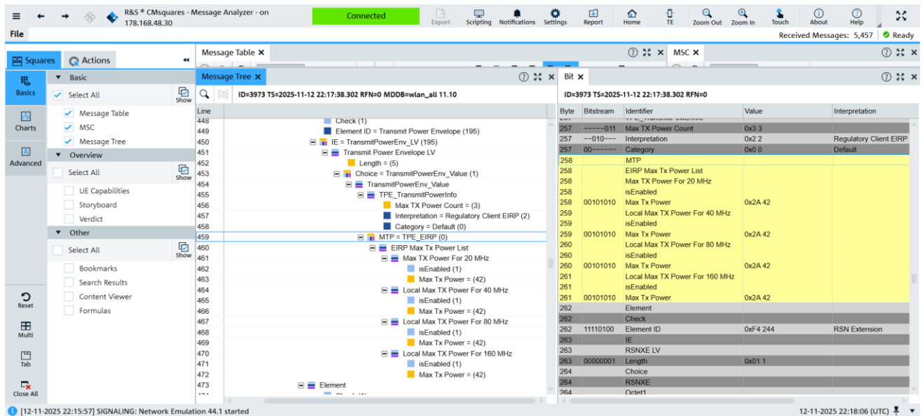
Plot 7-1745. AFC EIRP/PSD Auhorization by channel – 21dBm
