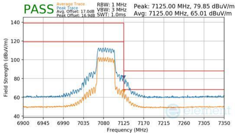
Plot 7-1686 CDD Diversity Radiated Upper Band Edge (Peak & Average – UNII Band 8) - RU484
