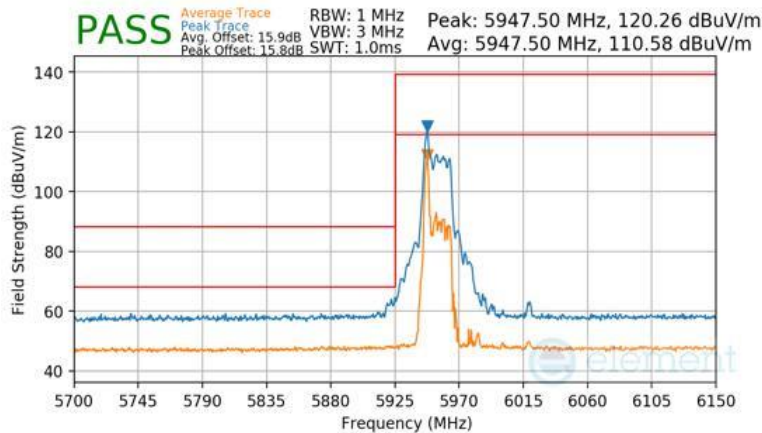
Plot 7-1681 CDD Diversity Radiated Lower Band Edge (Peak & Average – UNII Band 5) - RU26
