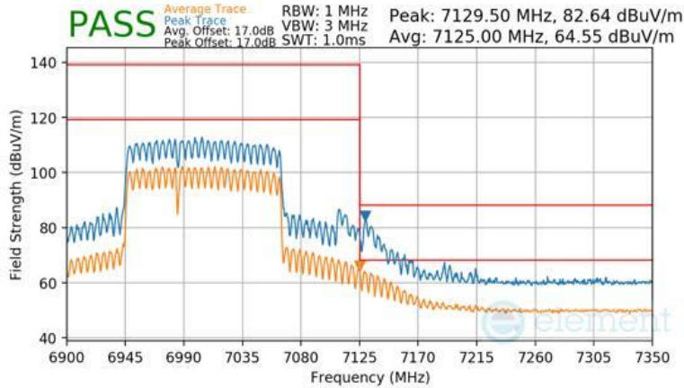
Plot 7-1647 CDD Primary Radiated Upper Band Edge (Peak & Average – UNII Band 8) - RU996+484 (L)
