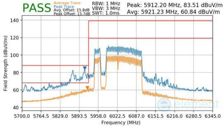
Plot 7-1653 CDD Primary Radiated Lower Band Edge (Peak & Average – UNII Band 5) - RU996+484+242 (L)
