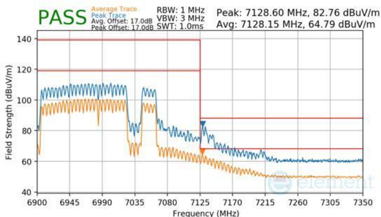
Plot 7-1726 CDD Diversity Radiated Upper Band Edge (Peak & Average – UNII Band 8) - RU996+484+242 (H)
