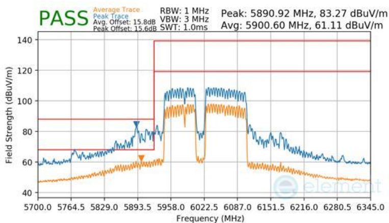
Plot 7-1719 CDD Diversity Radiated Lower Band Edge (Peak & Average – UNII Band 5) - RU996+484+242 (L)
