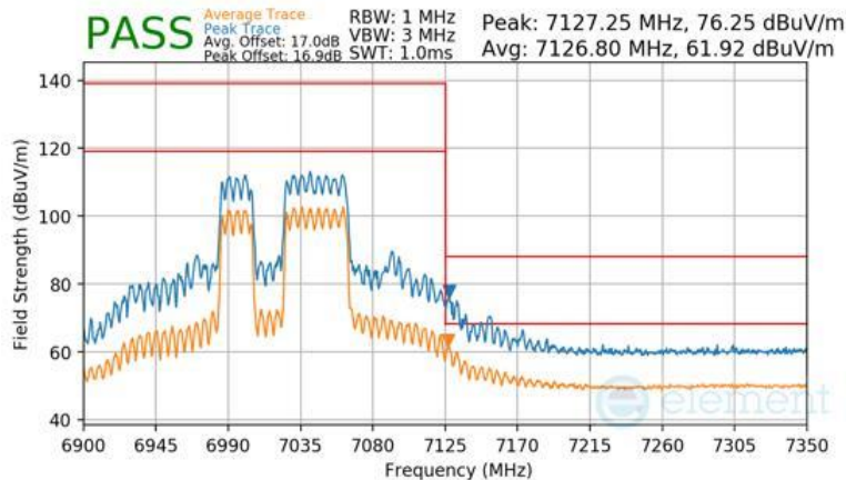
Plot 7-1696 CDD Diversity Radiated Upper Band Edge (Peak & Average – UNII Band 8) - RU484+242
