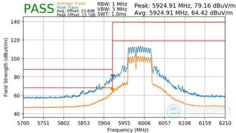
Plot 7-1691 CDD Diversity Radiated Lower Band Edge (Peak & Average – UNII Band 5) - RU484+242
