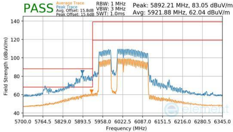
Plot 7-1655 CDD Primary Radiated Lower Band Edge (Peak & Average – UNII Band 5) - RU996+484+242 (L)
