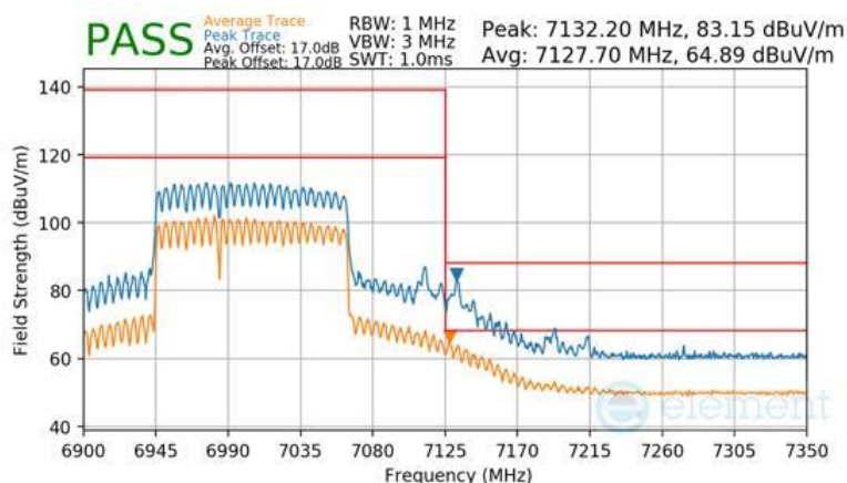
Plot 7-1709 CDD Diversity Radiated Upper Band Edge (Peak & Average – UNII Band 8) - RU996+484 (L)
