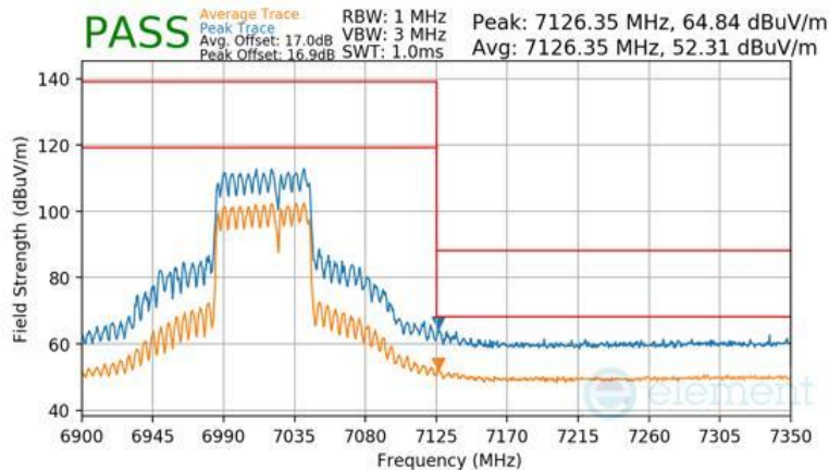
Plot 7-1698 CDD Diversity Radiated Upper Band Edge (Peak & Average – UNII Band 8) - RU484+242
