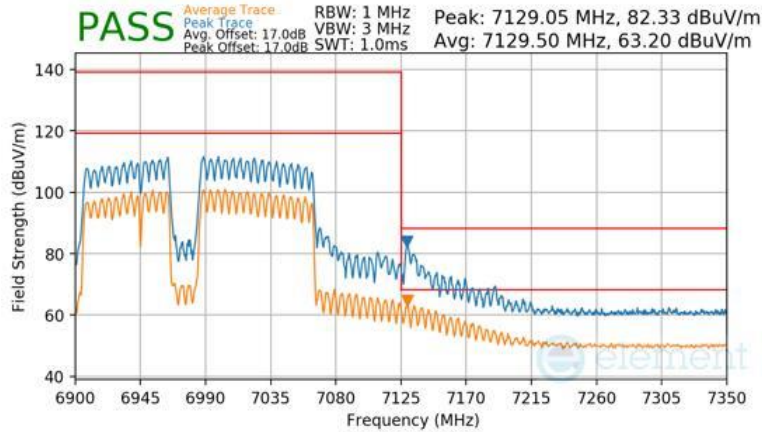
Plot 7-1665 CDD Primary Radiated Upper Band Edge (Peak & Average – UNII Band 8) - RU996+484+242 (L)
