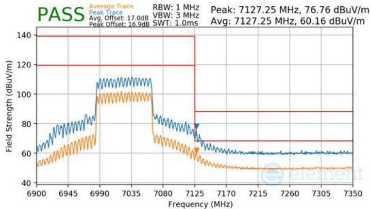
Plot 7-1700 CDD Diversity Radiated Upper Band Edge (Peak & Average – UNII Band 8) - RU996
