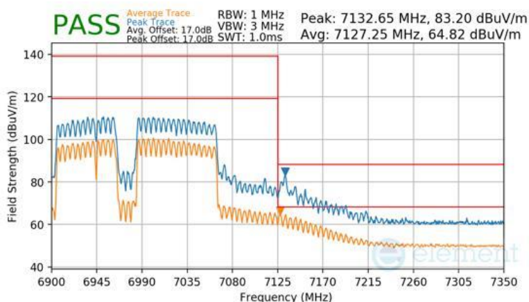
Plot 7-1727 CDD Diversity Radiated Upper Band Edge (Peak & Average – UNII Band 8) - RU996+484+242 (L)
