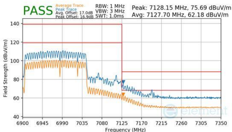
Plot 7-1728 CDD Diversity Radiated Upper Band Edge (Peak & Average – UNII Band 8) - RU996+484+242 (H)
