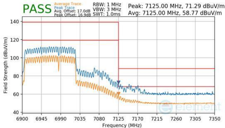
Plot 7-1650 CDD Primary Radiated Upper Band Edge (Peak & Average – UNII Band 8) - RU996+484 (H)
