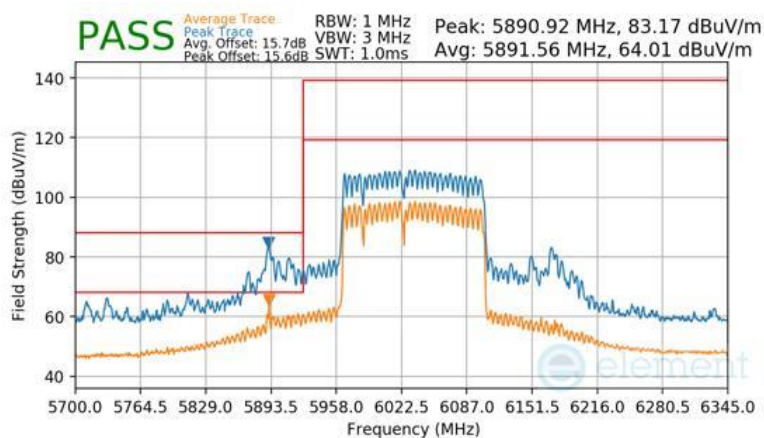
Plot 7-1713 CDD Diversity Radiated Lower Band Edge (Peak & Average – UNII Band 5) - RU996+484+242 (L)
