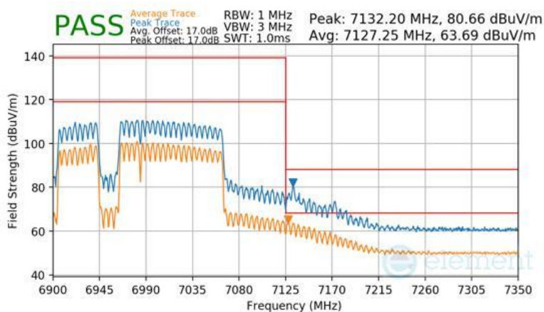
Plot 7-1725 CDD Diversity Radiated Upper Band Edge (Peak & Average – UNII Band 8) - RU996+484+242 (L)
