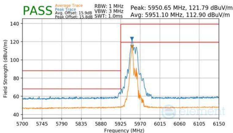
Plot 7-1673 CDD Diversity Radiated Lower Band Edge (Peak & Average – UNII Band 5) - RU52+26
