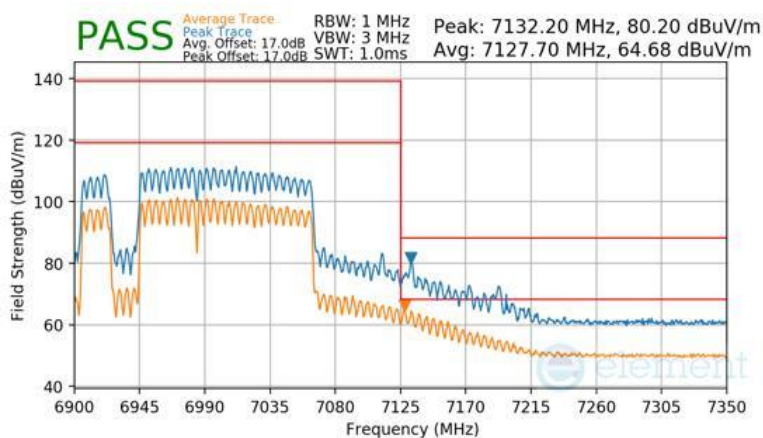
Plot 7-1723 CDD Diversity Radiated Upper Band Edge (Peak & Average – UNII Band 8) - RU996+484+242 (L)
