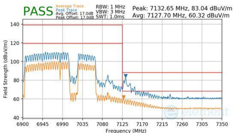
Plot 7-1724 CDD Diversity Radiated Upper Band Edge (Peak & Average – UNII Band 8) - RU996+484+242 (H)
