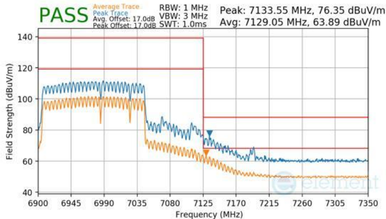
Plot 7-1666 CDD Primary Radiated Upper Band Edge (Peak & Average – UNII Band 8) - RU996+484+242 (H)
