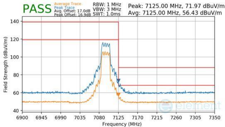
Plot 7-1678 CDD Diversity Radiated Upper Band Edge (Peak & Average – UNII Band 8) - RU242
