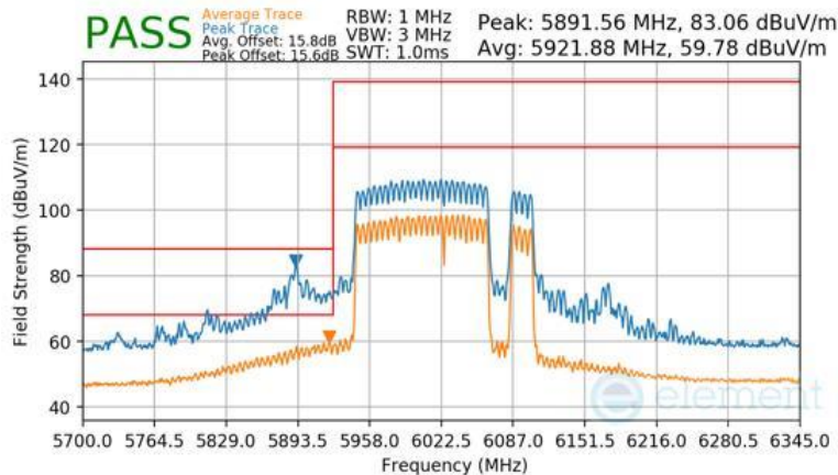
Plot 7-1656 CDD Primary Radiated Lower Band Edge (Peak & Average – UNII Band 5) - RU996+484+242 (H)
