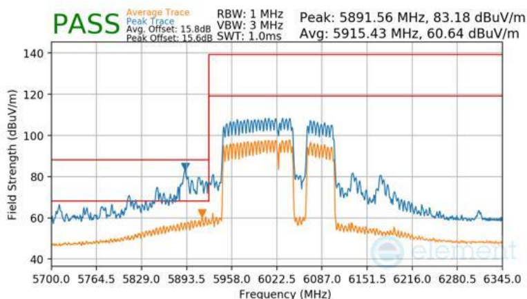
Plot 7-1716 CDD Diversity Radiated Lower Band Edge (Peak & Average – UNII Band 5) - RU996+484+242 (H)
