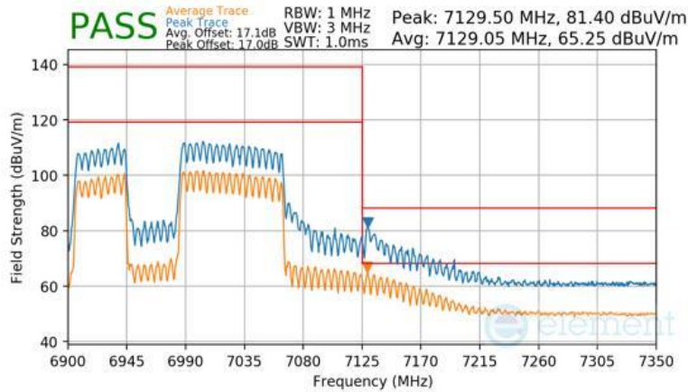
Plot 7-1649 CDD Primary Radiated Upper Band Edge (Peak & Average – UNII Band 8) - RU996+484 (L)
