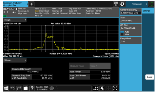
Plot 7-102 26dB BW & 99% OBW Antenna WF7b (80Mhz BW 802.11be(RU) RU26 Index0 - Ch.103)
