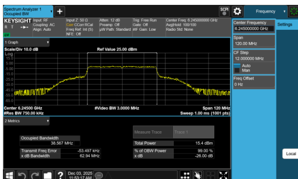
Plot 7-97 26dB BW & 99% OBW Antenna WF7b (40MHz BW 802.11be(RU) RU484 Index65 - Ch.59)
