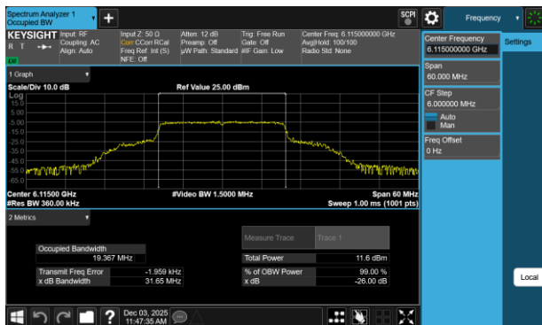
Plot 7-96 26dB BW & 99% OBW Antenna WF7b (20MHz BW 802.11be(RU) RU242 Index61 - Ch.33)
