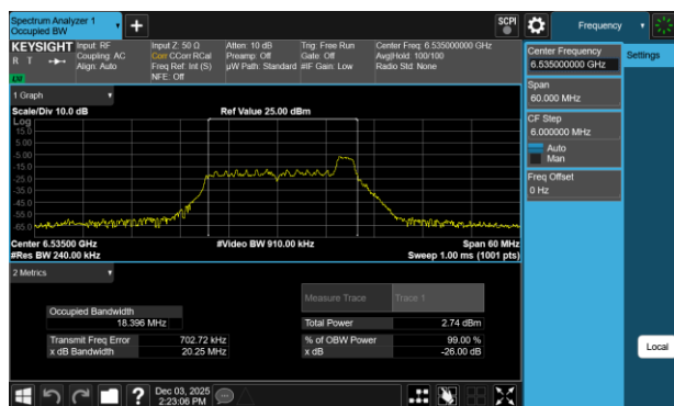
Plot 7-111 26dB BW & 99% OBW Antenna WF7b (20MHz BW 802.11be(RU) RU26 Index8 - Ch.117)
