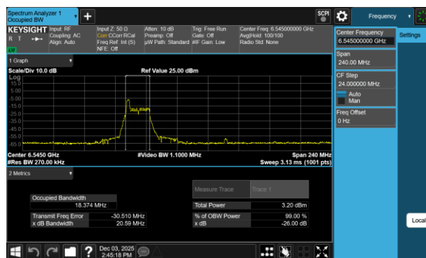
Plot 7-113 26dB BW & 99% OBW Antenna WF7b (80MHz BW 802.11be(RU) RU26 Index0 - Ch.119)
