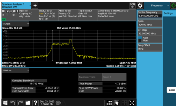
Plot 7-101 26dB BW & 99% OBW Antenna WF7b (40MHz BW 802.11be(RU) RU26 Index8 - Ch.99)
