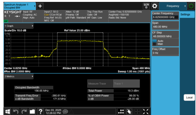
Plot 7-121 26dB BW & 99% OBW Antenna WF7b (160MHz BW 802.11be(RU) RU996X2 Index68 - Ch.175)
