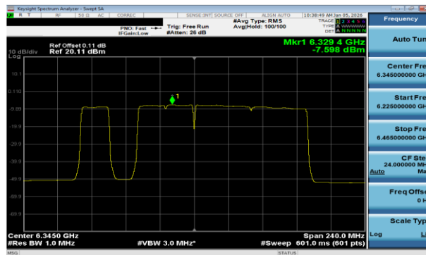
Plot 7-139 PSD Antenna WF7a (160MHz BW 802.11be(RU) RU996+484+242 Index97 - Ch.79)
