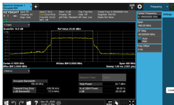
Plot 7-99 26dB BW & 99% OBW Antenna WF7b (160MHz BW 802.11be(RU) RU996X2 Index68 - Ch.47)
