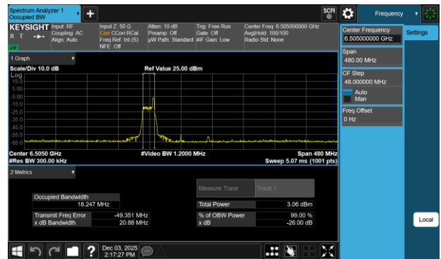
Plot 7-103 26dB BW & 99% OBW Antenna WF7b (160MHz BW 802.11be(RU) RU26 Index17 - Ch.111)
