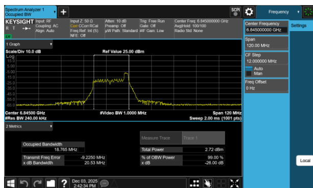
Plot 7-112 26dB BW & 99% OBW Antenna WF7b (40MHz BW 802.11be(RU) RU26 Index8 - Ch.179)
