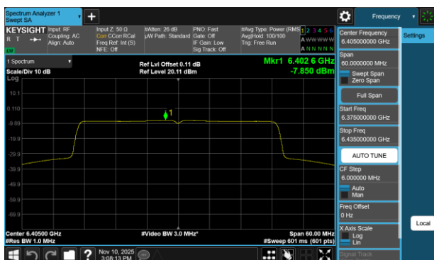
Plot 7-141 PSD Antenna WF7a (40MHz BW 802.11be(RU) RU484 Index65 - Ch.91)
