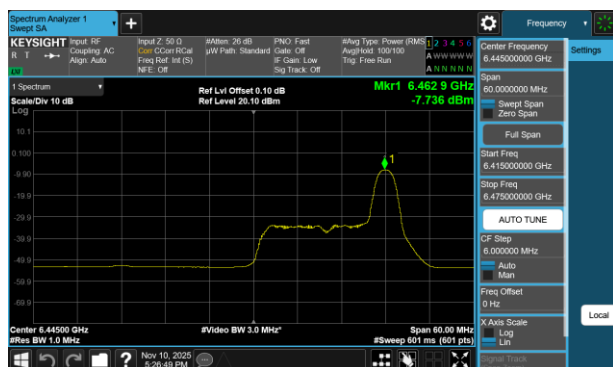
Plot 7-145 PSD Antenna WF7a (40MHz BW 802.11be(RU) RU26 Index17 - Ch.99)
