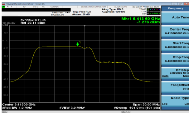
Plot 7-137 PSD Antenna WF7a (20MHz BW 802.11be(RU) RU106+26 Index82 - Ch.93)
