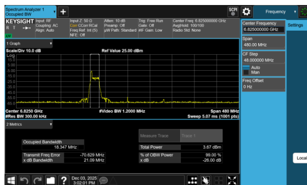
Plot 7-114 26dB BW & 99% OBW Antenna WF7b (160MHz BW 802.11be(RU) RU26 Index0 - Ch.175)
