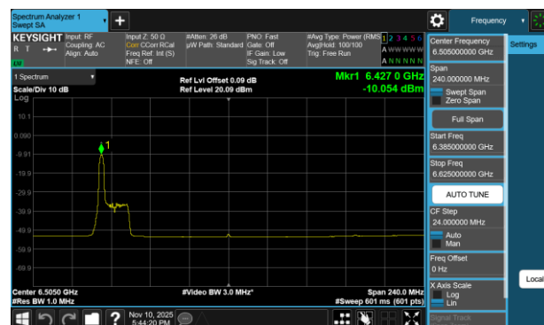
Plot 7-147 PSD Antenna WF7a (160MHz BW 802.11be(RU) RU26 Index0 - Ch.111)
