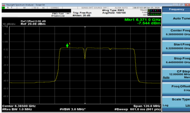
Plot 7-138 PSD Antenna WF7a (80MHz BW 802.11be(RU) RU484+242 Index90 - Ch.87)
