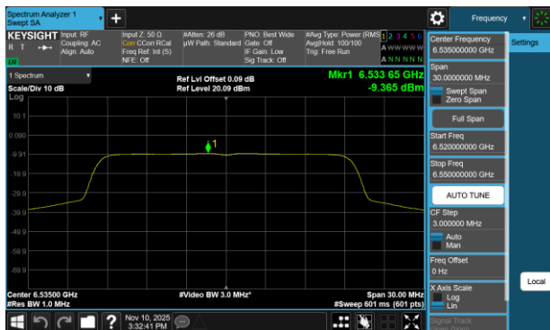
Plot 7-162 PSD Antenna WF7a (20MHz BW 802.11be(RU) RU242 Index61 - Ch.117)
