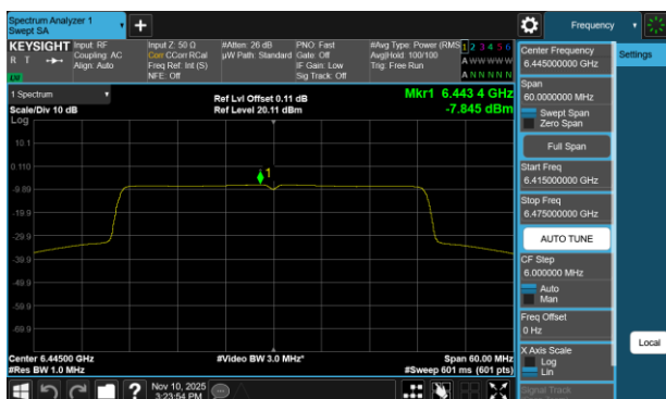
Plot 7-152 PSD Antenna WF7a (40MHz BW 802.11be(RU) RU484 Index65 - Ch.99)
