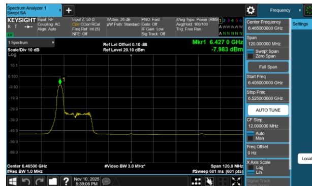
Plot 7-146 PSD Antenna WF7a (80MHz BW 802.11be(RU) RU26 Index0 - Ch.103)
