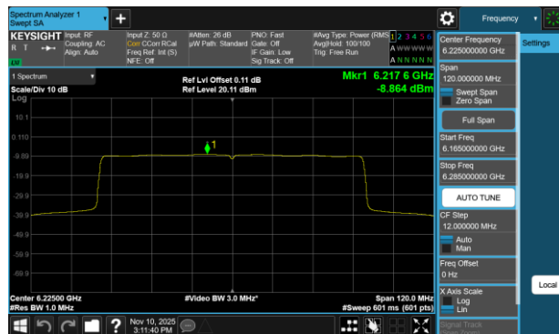
Plot 7-142 PSD Antenna WF7a (80MHz BW 802.11be(RU) RU996 Index67 - Ch.55)
