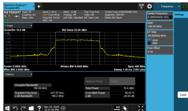
Plot 7-132 26dB BW & 99% OBW Antenna WF7b (160MHz BW 802.11be(RU) RU996X2 Index68 - Ch.207)
