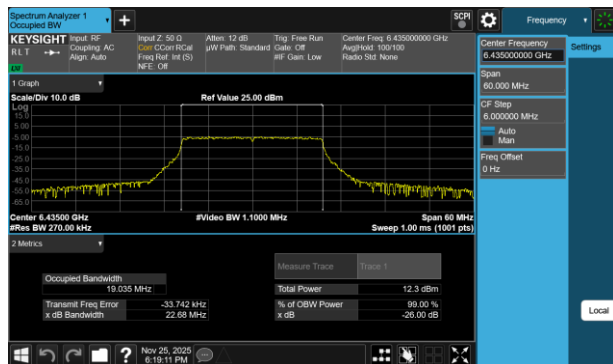
Plot 7-206 26dB BW & 99% OBW Antenna WF7b (20MHz BW 802.11be(RU) RU242 Index61 - Ch.97)
