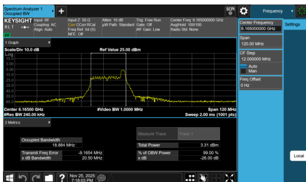
Plot 7-189 26dB BW & 99% OBW Antenna WF7b (40MHz BW 802.11be(RU) RU26 Index8 - Ch.43)
