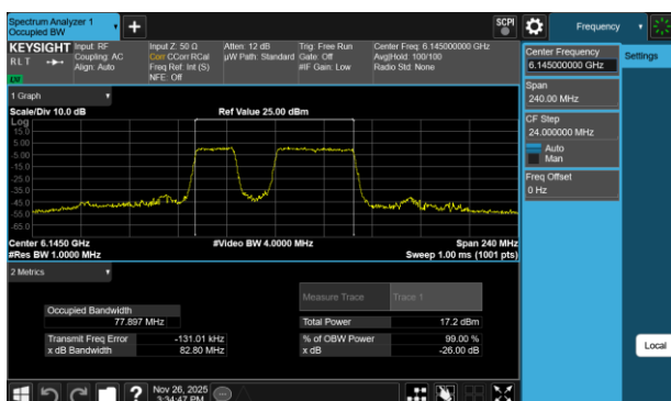
Plot 7-193 26dB BW & 99% OBW Antenna WF7b (80MHz BW 802.11be(RU) RU484+242 Index91 - Ch.39)
