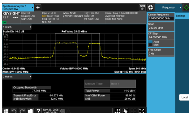
Plot 7-226 26dB BW & 99% OBW Antenna WF7b (80MHz BW 802.11be(RU) RU484+242 Index92 - Ch.199)
