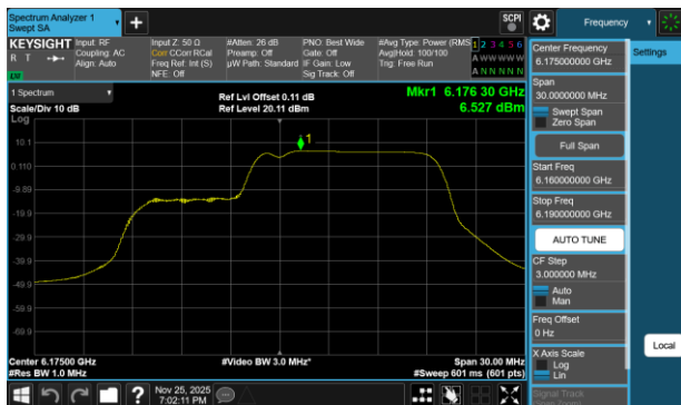
Plot 7-236 PSD Antenna WF7a (20MHz BW 802.11be(RU) RU106+26 Index83 - Ch.45)
