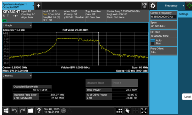
Plot 7-181 26dB BW & 99% OBW Antenna WF7b (20MHz BW 802.11be(RU) RU106+26 Index82 - Ch.181)
