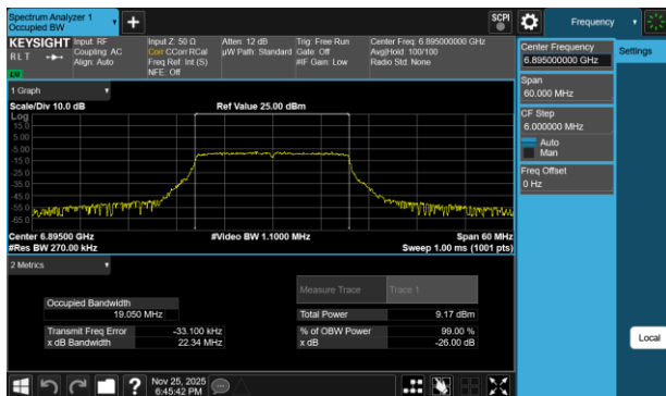
Plot 7-228 26dB BW & 99% OBW Antenna WF7b (20MHz BW 802.11be(RU) RU242 Index61 - Ch.189)
