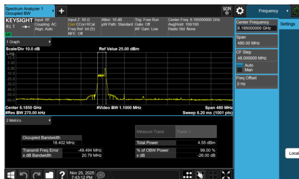
Plot 7-191 26dB BW & 99% OBW Antenna WF7b (160MHz BW 802.11be(RU) RU26 Index17 - Ch.47)
