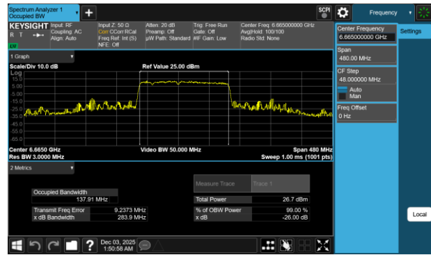
Plot 7-183 26dB BW & 99% OBW Antenna WF7b (160MHz BW 802.11be(RU) RU996+484+242 Index96 - Ch.143)
