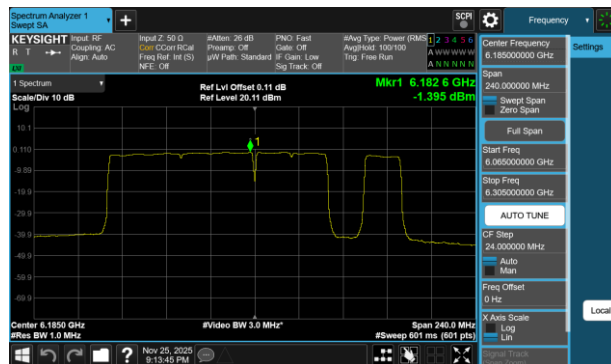
Plot 7-238 PSD Antenna WF7a (160MHz BW 802.11be(RU) RU996+484+242 Index98 - Ch.47)
