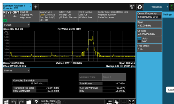
Plot 7-180 26dB BW & 99% OBW Antenna WF7b (160MHz BW 802.11be(RU) RU26 Index36 - Ch.143)
