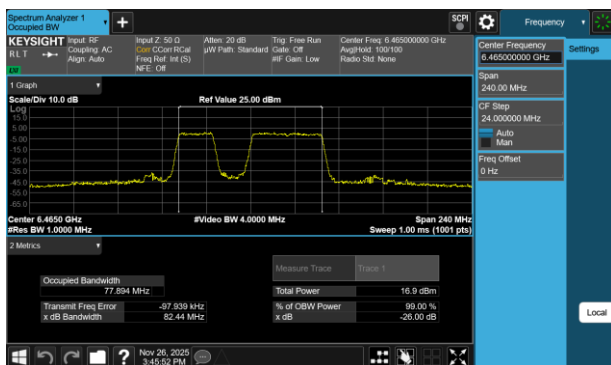
Plot 7-204 26dB BW & 99% OBW Antenna WF7b (80MHz BW 802.11be(RU) RU484+242 Index91 - Ch.103)
