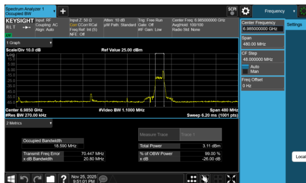
Plot 7-224 26dB BW & 99% OBW Antenna WF7b (160MHz BW 802.11be(RU) RU26 Index36 - Ch.207)
