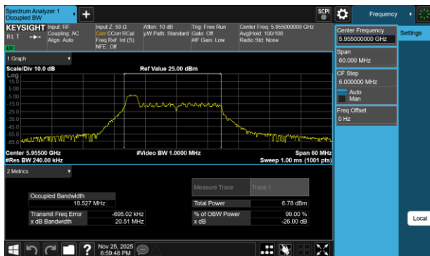
Plot 7-188 26dB BW & 99% OBW Antenna WF7b (20MHz BW 802.11be(RU) RU26 Index0 - Ch.1)
