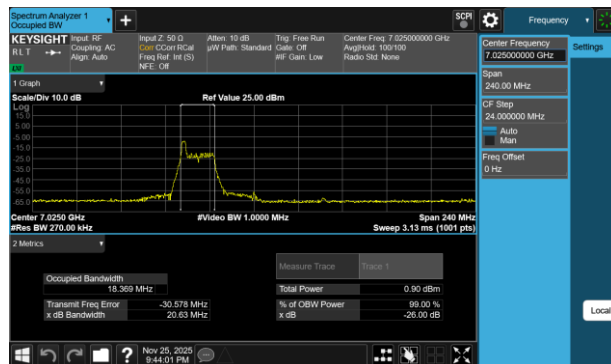
Plot 7-223 26dB BW & 99% OBW Antenna WF7b (80MHz BW 802.11be(RU) RU26 Index0 - Ch.215)
