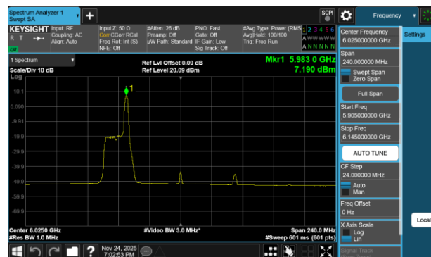
Plot 7-235 PSD Antenna WF7a (160MHz BW 802.11be(RU) RU26 Index17 - Ch.15)
