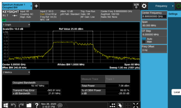
Plot 7-225 26dB BW & 99% OBW Antenna WF7b (20MHz BW 802.11be(RU) RU106+26 Index82 - Ch.189)
