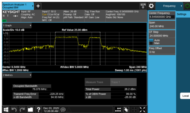
Plot 7-182 26dB BW & 99% OBW Antenna WF7b (80MHz BW 802.11be(RU) RU484+242 Index92 - Ch.119)
