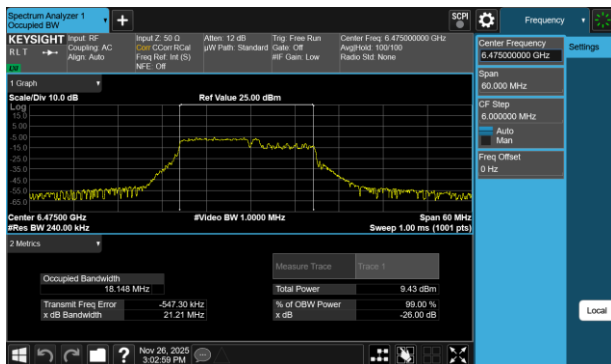
Plot 7-203 26dB BW & 99% OBW Antenna WF7b (20MHz BW 802.11be(RU) RU106+26 Index82 - Ch.105)
