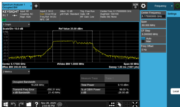
Plot 7-192 26dB BW & 99% OBW Antenna WF7b (20MHz BW 802.11be(RU) RU106+26 Index82 - Ch.45)
