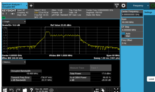
Plot 7-177 26dB BW & 99% OBW Antenna WF7b (20MHz BW 802.11be(RU) RU26 Index0 - Ch.149)
