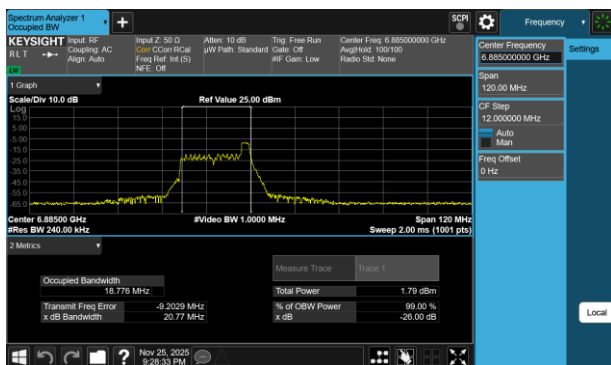
Plot 7-222 26dB BW & 99% OBW Antenna WF7b (40MHz BW 802.11be(RU) RU26 Index8 - Ch.187)
