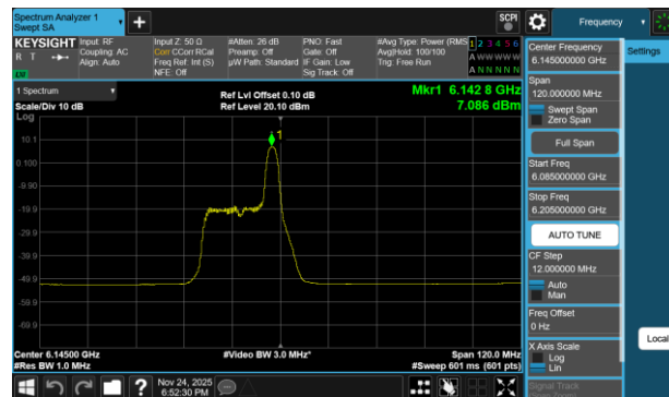
Plot 7-234 PSD Antenna WF7a (80MHz BW 802.11be(RU) RU26 Index17 - Ch.39)
