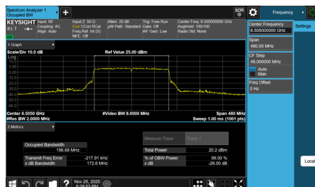
Plot 7-209 26dB BW & 99% OBW Antenna WF7b (160MHz BW 802.11be(RU) RU996X2 Index68 - Ch.111)
