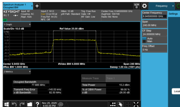
Plot 7-230 26dB BW & 99% OBW Antenna WF7b (80MHz BW 802.11be(RU) RU996 Index67 - Ch.199)
