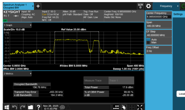
Plot 7-227 26dB BW & 99% OBW Antenna WF7b (160MHz BW 802.11be(RU) RU996+484+242 Index98 - Ch.207)
