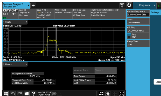
Plot 7-190 26dB BW & 99% OBW Antenna WF7b (80MHz BW 802.11be(RU) RU26 Index0 - Ch.39)
