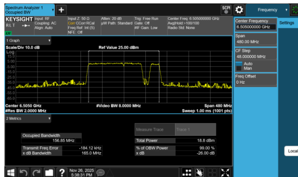
Plot 7-205 26dB BW & 99% OBW Antenna WF7b (160MHz BW 802.11be(RU) RU996+484+242 Index98 - Ch.111)
