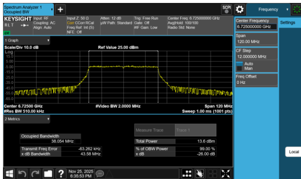
Plot 7-218 26dB BW & 99% OBW Antenna WF7b (40MHz BW 802.11be(RU) RU484 Index65 - Ch.155)
