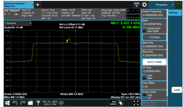
Plot 7-252 PSD Antenna WF7a (80MHz BW 802.11be(RU) RU996 Index67 - Ch.103)
