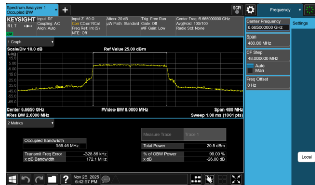
Plot 7-220 26dB BW & 99% OBW Antenna WF7b (160MHz BW 802.11be(RU) RU996X2 Index68 - Ch.143)
