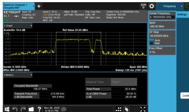
Plot 7-194 26dB BW & 99% OBW Antenna WF7b (160MHz BW 802.11be(RU) RU996+484+242 Index98 - Ch.47)
