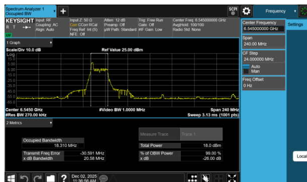
Plot 7-179 26dB BW & 99% OBW Antenna WF7b (80MHz BW 802.11be(RU) RU26 Index0 - Ch.119)
