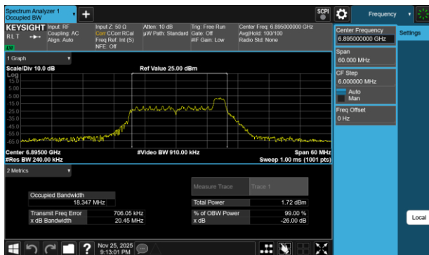
Plot 7-221 26dB BW & 99% OBW Antenna WF7b (20MHz BW 802.11be(RU) RU26 Index8 - Ch.189)
