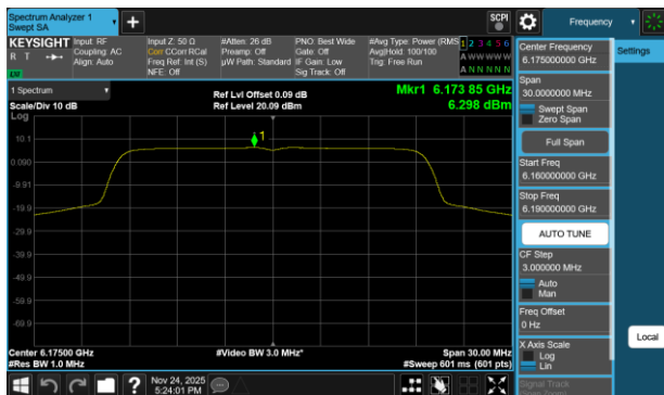
Plot 7-239 PSD Antenna WF7a (20MHz BW 802.11be(RU) RU242 Index61 - Ch.45)
