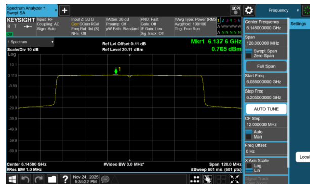
Plot 7-241 PSD Antenna WF7a (80MHz BW 802.11be(RU) RU996 Index67 - Ch.39)
