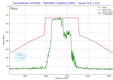
Plot 7-605 In-Band Emission Plot SDM Primary Antenna WF7a (20MHz BW 802.11be(RU) RU106+26 Index82 (UNII Band 5) - Ch.93)
