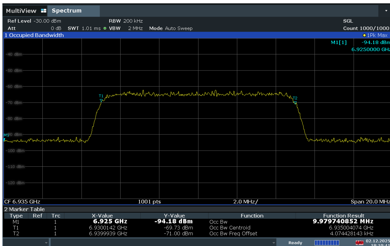
Plot 7-761. AWGN Signal – UNII 8 – 20MHz
