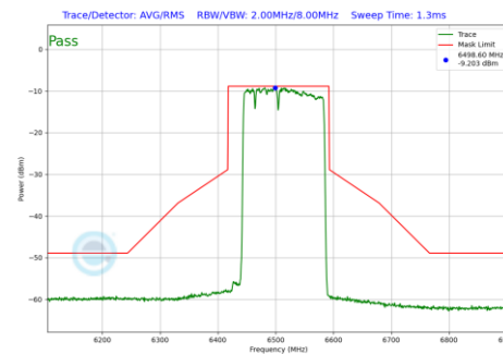
Plot 7-610 In-Band Emission Plot SDM Primary Antenna WF7a (160MHz BW 802.11be(RU) RU996+484+242 Index96 (UNII Band 6) - Ch.111)
