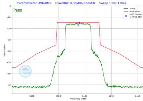
Plot 7-733 In-Band Emission Plot SDM Diversity Antenna WF2a (20MHz BW 802.11be(RU) RU242 Index61 (UNII Band 5) - Ch.33)
