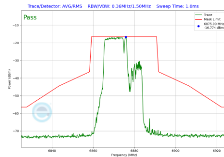
Plot 7-611 In-Band Emission Plot SDM Primary Antenna WF7a (20MHz BW 802.11be(RU) RU106+26 Index82 (UNII Band 7) - Ch.185)
