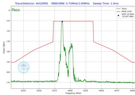
Plot 7-678 In-Band Emission Plot SDM Diversity Antenna WF2a (40MHz BW 802.11be(RU) RU26 Index0 (UNII Band 5) - Ch.91)
