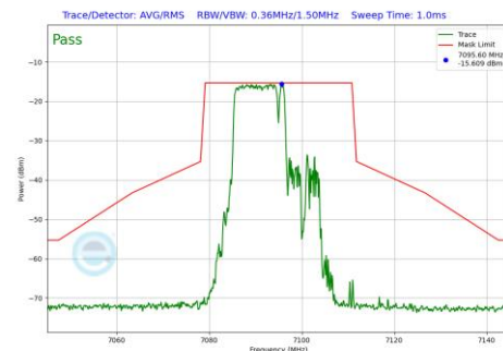
Plot 7-626 In-Band Emission Plot SDM Primary Antenna WF2a (20MHz BW 802.11be(RU) RU106+26 Index82 (UNII Band 8) - Ch.229)
