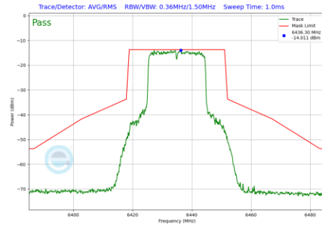
Plot 7-649 In-Band Emission Plot SDM Primary Antenna WF2a (20MHz BW 802.11be(RU) RU242 Index61 (UNII Band 6) - Ch.97)
