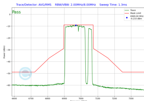
Plot 7-616 In-Band Emission Plot SDM Primary Antenna WF7a (160MHz BW 802.11be(RU) RU996+484+242 Index98 (UNII Band 8) - Ch.207)
