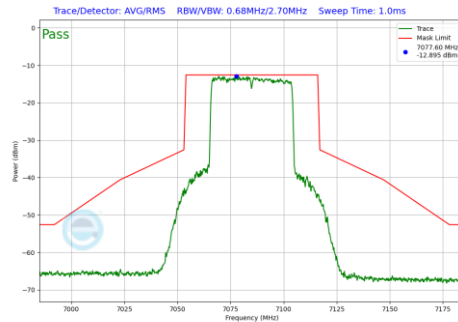
Plot 7-658 In-Band Emission Plot SDM Primary Antenna WF2a (40MHz BW 802.11be(RU) RU484 Index65 (UNII Band 8) - Ch.227)
