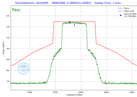
Plot 7-741 In-Band Emission Plot SDM Diversity Antenna WF2a (20MHz BW 802.11be(RU) RU242 Index61 (UNII Band 7) - Ch.117)
