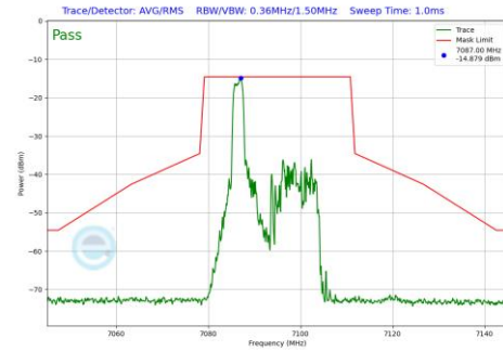
Plot 7-601 In-Band Emission Plot SDM Primary Antenna WF2a (20MHz BW 802.11be(RU) RU26 Index0 (UNII Band 8) - Ch.229)
