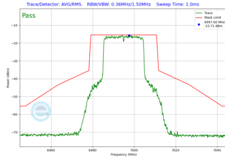
Plot 7-745 In-Band Emission Plot SDM Diversity Antenna WF2a (20MHz BW 802.11be(RU) RU242 Index61 (UNII Band 8) - Ch.209)
