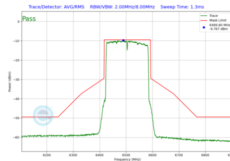
Plot 7-724 In-Band Emission Plot SDM Diversity Antenna WF7b (160MHz BW 802.11be(RU) RU996X2 Index68 (UNII Band 6) - Ch.111)
