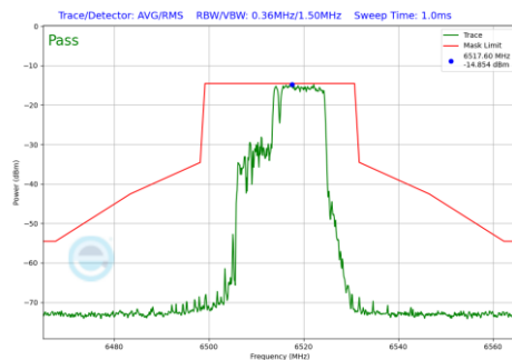
Plot 7-608 In-Band Emission Plot SDM Primary Antenna WF7a (20MHz BW 802.11be(RU) RU106+26 Index83 (UNII Band 6) - Ch.113)
