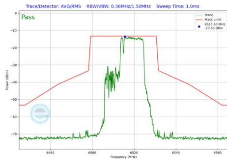
Plot 7-696 In-Band Emission Plot SDM Diversity Antenna WF7b (20MHz BW 802.11be(RU) RU106+26 Index83 (UNII Band 6) - Ch.113)
