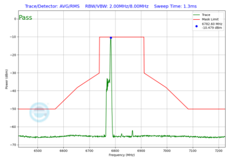
Plot 7-672 In-Band Emission Plot SDM Diversity Antenna WF7b (160MHz BW 802.11be(RU) RU26 Index17 (UNII Band 7) - Ch.175)
