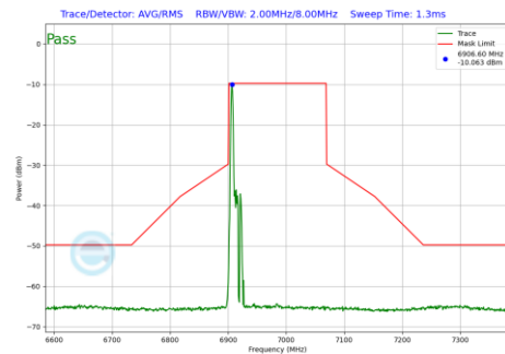
Plot 7-692 In-Band Emission Plot SDM Diversity Antenna WF2a (160MHz BW 802.11be(RU) RU26 Index0 (UNII Band 8) - Ch.207)
