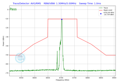
Plot 7-671 In-Band Emission Plot SDM Diversity Antenna WF7b (80MHz BW 802.11be(RU) RU26 Index17 (UNII Band 7) - Ch.151)
