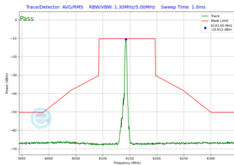
Plot 7-679 In-Band Emission Plot SDM Diversity Antenna WF2a (80MHz BW 802.11be(RU) RU26 Index17 (UNII Band 5) - Ch.39)
