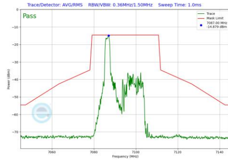
Plot 7-689 In-Band Emission Plot SDM Diversity Antenna WF2a (20MHz BW 802.11be(RU) RU26 Index0 (UNII Band 8) - Ch.229)
