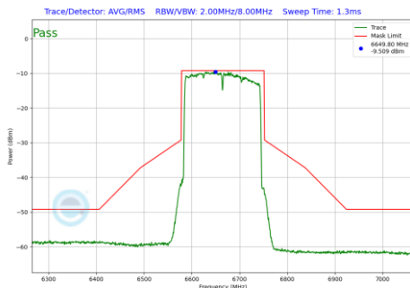
Plot 7-656 In-Band Emission Plot SDM Primary Antenna WF2a (160MHz BW 802.11be(RU) RU996X2 Index68 (UNII Band 7) - Ch.143)
