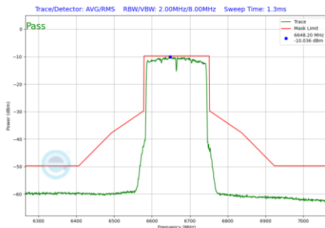
Plot 7-640 In-Band Emission Plot SDM Primary Antenna WF7a (160MHz BW 802.11be(RU) RU996X2 Index68 (UNII Band 7) - Ch.143)
