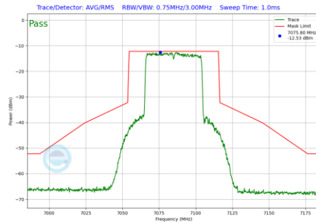
Plot 7-642 In-Band Emission Plot SDM Primary Antenna WF7a (40MHz BW 802.11be(RU) RU484 Index65 (UNII Band 8) - Ch.227)
