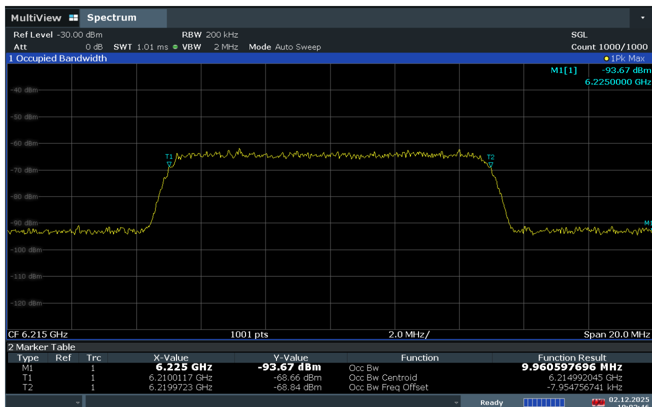
Plot 7-749. AWGN Signal – UNII 5 – 20MHz
