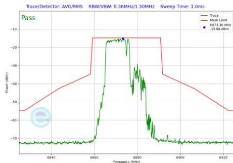
Plot 7-711 In-Band Emission Plot SDM Diversity Antenna WF2a (20MHz BW 802.11be(RU) RU106+26 Index82 (UNII Band 7) - Ch.185)
