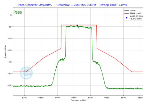
Plot 7-739 In-Band Emission Plot SDM Diversity Antenna WF2a (80MHz BW 802.11be(RU) RU996 Index67 (UNII Band 6) - Ch.103)
