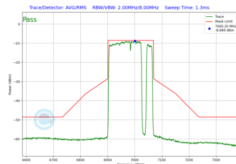
Plot 7-628 In-Band Emission Plot SDM Primary Antenna WF2a (160MHz BW 802.11be(RU) RU996+484+242 Index98 (UNII Band 8) - Ch.207)
