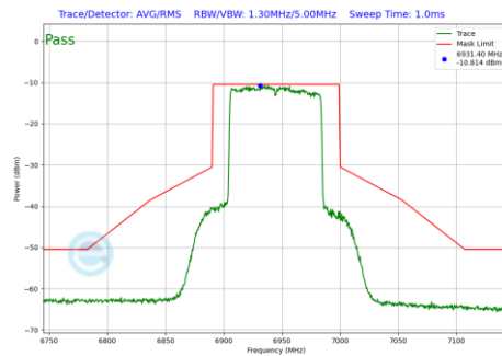
Plot 7-643 In-Band Emission Plot SDM Primary Antenna WF7a (80MHz BW 802.11be(RU) RU996 Index67 (UNII Band 8) - Ch.199)
