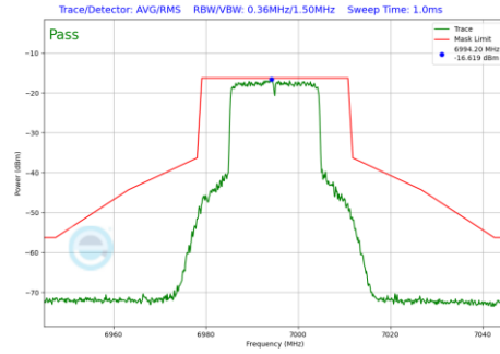
Plot 7-641 In-Band Emission Plot SDM Primary Antenna WF7a (20MHz BW 802.11be(RU) RU242 Index61 (UNII Band 8) - Ch.209)
