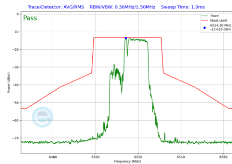
Plot 7-708 In-Band Emission Plot SDM Diversity Antenna WF2a (20MHz BW 802.11be(RU) RU106+26 Index83 (UNII Band 6) - Ch.113)
