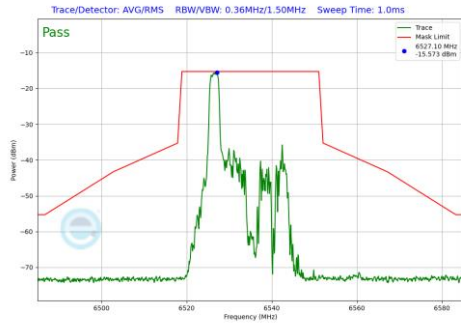
Plot 7-685 In-Band Emission Plot SDM Diversity Antenna WF2a (20MHz BW 802.11be(RU) RU26 Index0 (UNII Band 7) - Ch.117)
