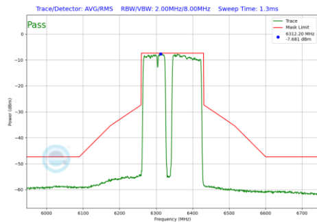
Plot 7-695 In-Band Emission Plot SDM Diversity Antenna WF7b (160MHz BW 802.11be(RU) RU996+484+242 Index99 (UNII Band 5) - Ch.79)
