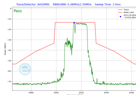
Plot 7-620 In-Band Emission Plot SDM Primary Antenna WF2a (20MHz BW 802.11be(RU) RU106+26 Index83 (UNII Band 6) - Ch.113)
