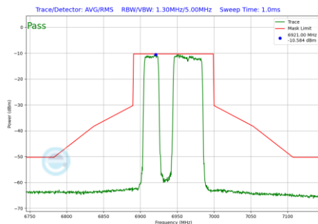
Plot 7-615 In-Band Emission Plot SDM Primary Antenna WF7a (80MHz BW 802.11be(RU) RU484+242 Index91 (UNII Band 8) - Ch.199)
