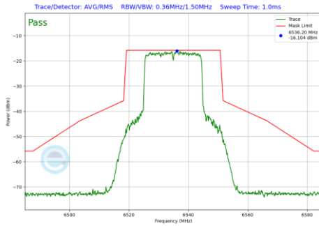
Plot 7-637 In-Band Emission Plot SDM Primary Antenna WF7a (20MHz BW 802.11be(RU) RU242 Index61 (UNII Band 7) - Ch.117)
