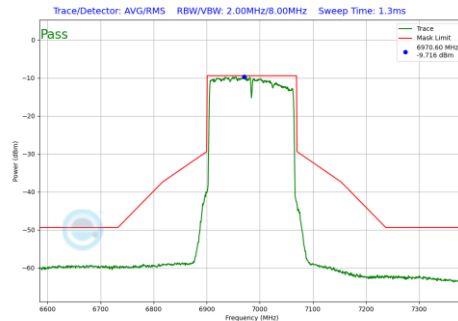
Plot 7-732 In-Band Emission Plot SDM Diversity Antenna WF7b (160MHz BW 802.11be(RU) RU996X2 Index68 (UNII Band 8) - Ch.207)
