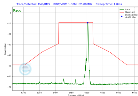
Plot 7-667 In-Band Emission Plot SDM Diversity Antenna WF7b (80MHz BW 802.11be(RU) RU26 Index36 (UNII Band 6) - Ch.103)
