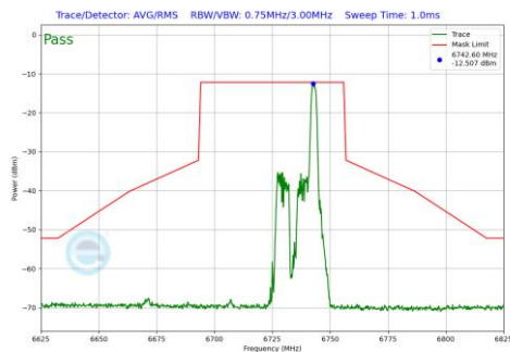
Plot 7-686 In-Band Emission Plot SDM Diversity Antenna WF2a (40MHz BW 802.11be(RU) RU26 Index17 (UNII Band 7) - Ch.155)
