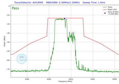
Plot 7-705 In-Band Emission Plot SDM Diversity Antenna WF2a (20MHz BW 802.11be(RU) RU106+26 Index82 (UNII Band 5) - Ch.93)
