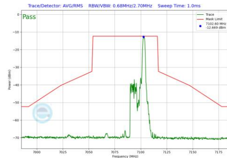
Plot 7-602 In-Band Emission Plot SDM Primary Antenna WF2a (40MHz BW 802.11be(RU) RU26 Index17 (UNII Band 8) - Ch.227)
