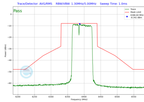
Plot 7-706 In-Band Emission Plot SDM Diversity Antenna WF2a (80MHz BW 802.11be(RU) RU484+242 Index90 (UNII Band 5) - Ch.87)
