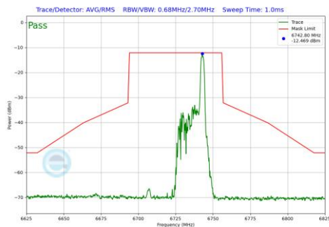
Plot 7-670 In-Band Emission Plot SDM Diversity Antenna WF7b (40MHz BW 802.11be(RU) RU26 Index17 (UNII Band 7) - Ch.155)
