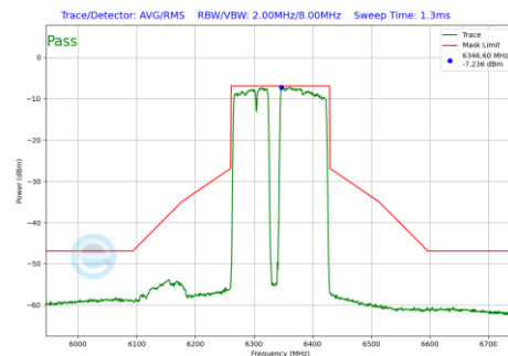
Plot 7-619 In-Band Emission Plot SDM Primary Antenna WF2a (160MHz BW 802.11be(RU) RU996+484+242 Index99 (UNII Band 5) - Ch.79)
