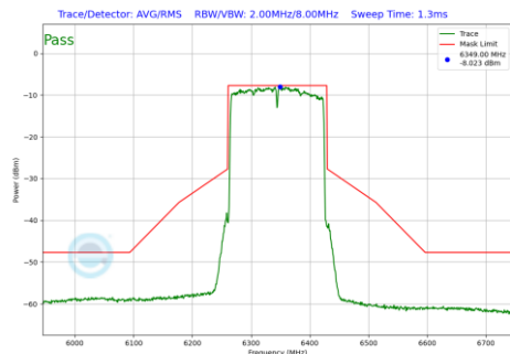
Plot 7-648 In-Band Emission Plot SDM Primary Antenna WF2a (160MHz BW 802.11be(RU) RU996X2 Index68 (UNII Band 5) - Ch.79)
