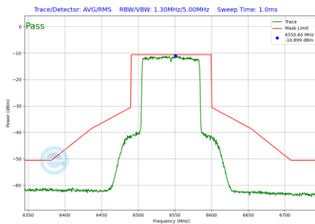
Plot 7-639 In-Band Emission Plot SDM Primary Antenna WF7a (80MHz BW 802.11be(RU) RU996 Index67 (UNII Band 7) - Ch.119)
