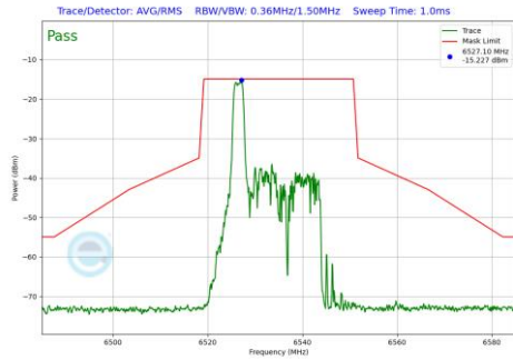
Plot 7-669 In-Band Emission Plot SDM Diversity Antenna WF7b (20MHz BW 802.11be(RU) RU26 Index0 (UNII Band 7) - Ch.117)
