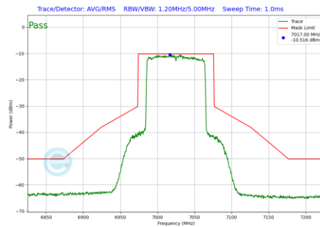
Plot 7-747 In-Band Emission Plot SDM Diversity Antenna WF2a (80MHz BW 802.11be(RU) RU996 Index67 (UNII Band 8) - Ch.215)
