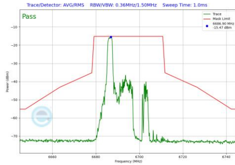
Plot 7-597 In-Band Emission Plot SDM Primary Antenna WF2a (20MHz BW 802.11be(RU) RU26 Index0 (UNII Band 7) - Ch.149)
