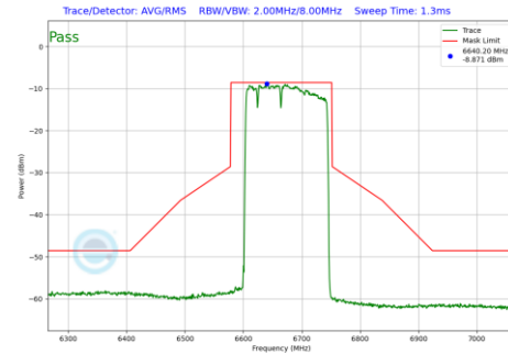
Plot 7-625 In-Band Emission Plot SDM Primary Antenna WF2a (160MHz BW 802.11be(RU) RU996+484+242 Index96 (UNII Band 7) - Ch.143)
