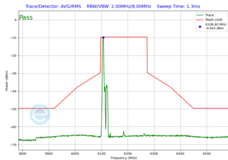
Plot 7-680 In-Band Emission Plot SDM Diversity Antenna WF2a (160MHz BW 802.11be(RU) RU26 Index0 (UNII Band 5) - Ch.47)
