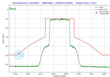
Plot 7-631 In-Band Emission Plot SDM Primary Antenna WF7a (80MHz BW 802.11be(RU) RU996 Index67 (UNII Band 5) - Ch.55)
