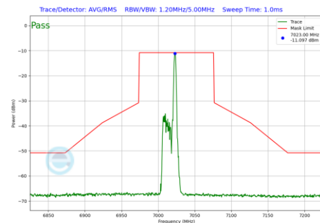
Plot 7-603 In-Band Emission Plot SDM Primary Antenna WF2a (80MHz BW 802.11be(RU) RU26 Index17 (UNII Band 8) - Ch.215)
