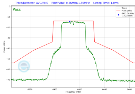
Plot 7-645 In-Band Emission Plot SDM Primary Antenna WF2a (20MHz BW 802.11be(RU) RU242 Index61 (UNII Band 5) - Ch.93)
