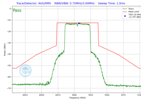
Plot 7-730 In-Band Emission Plot SDM Diversity Antenna WF7b (40MHz BW 802.11be(RU) RU484 Index65 (UNII Band 8) - Ch.211)
