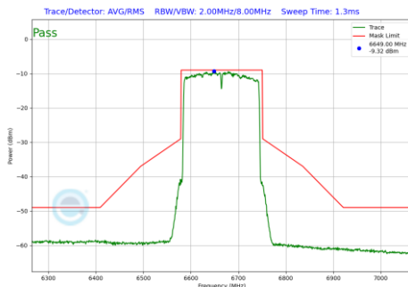
Plot 7-728 In-Band Emission Plot SDM Diversity Antenna WF7b (160MHz BW 802.11be(RU) RU996X2 Index68 (UNII Band 7) - Ch.143)
