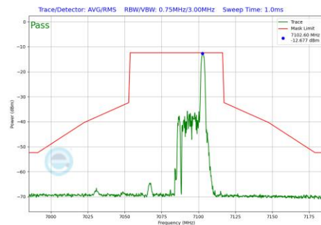
Plot 7-674 In-Band Emission Plot SDM Diversity Antenna WF7b (40MHz BW 802.11be(RU) RU26 Index17 (UNII Band 8) - Ch.227)
