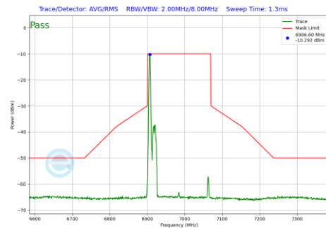
Plot 7-676 In-Band Emission Plot SDM Diversity Antenna WF7b (160MHz BW 802.11be(RU) RU26 Index0 (UNII Band 8) - Ch.207)
