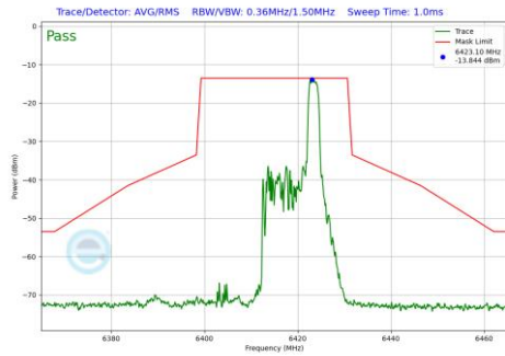
Plot 7-661 In-Band Emission Plot SDM Diversity Antenna WF7b (20MHz BW 802.11be(RU) RU26 Index8 (UNII Band 5) - Ch.93)
