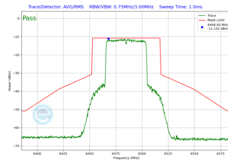
Plot 7-722 In-Band Emission Plot SDM Diversity Antenna WF7b (40MHz BW 802.11be(RU) RU484 Index65 (UNII Band 6) - Ch.107)
