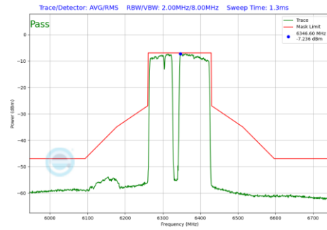
Plot 7-707 In-Band Emission Plot SDM Diversity Antenna WF2a (160MHz BW 802.11be(RU) RU996+484+242 Index99 (UNII Band 5) - Ch.79)
