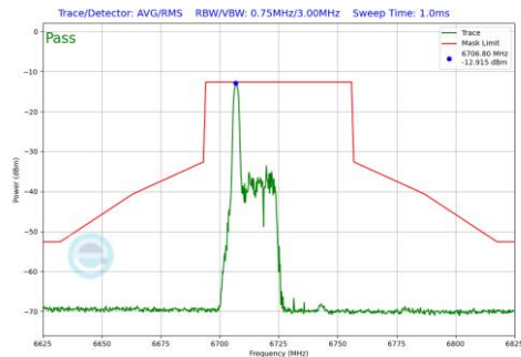
Plot 7-598 In-Band Emission Plot SDM Primary Antenna WF2a (40MHz BW 802.11be(RU) RU26 Index0 (UNII Band 7) - Ch.155)
