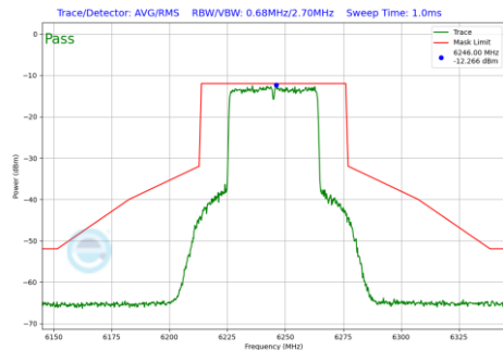
Plot 7-646 In-Band Emission Plot SDM Primary Antenna WF2a (40MHz BW 802.11be(RU) RU484 Index65 (UNII Band 5) - Ch.59)
