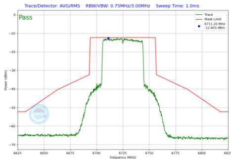
Plot 7-742 In-Band Emission Plot SDM Diversity Antenna WF2a (40MHz BW 802.11be(RU) RU484 Index65 (UNII Band 7) - Ch.155)
