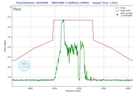
Plot 7-681 In-Band Emission Plot SDM Diversity Antenna WF2a (20MHz BW 802.11be(RU) RU26 Index0 (UNII Band 6) - Ch.113)
