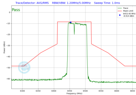
Plot 7-621 In-Band Emission Plot SDM Primary Antenna WF2a (80MHz BW 802.11be(RU) RU484+242 Index90 (UNII Band 6) - Ch.103)
