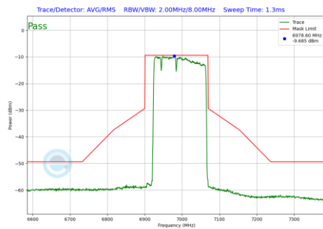
Plot 7-704 In-Band Emission Plot SDM Diversity Antenna WF7b (160MHz BW 802.11be(RU) RU996+484+242 Index96 (UNII Band 8) - Ch.207)
