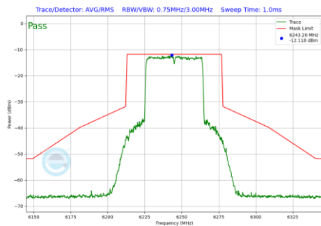
Plot 7-630 In-Band Emission Plot SDM Primary Antenna WF7a (40MHz BW 802.11be(RU) RU484 Index65 (UNII Band 5) - Ch.59)
