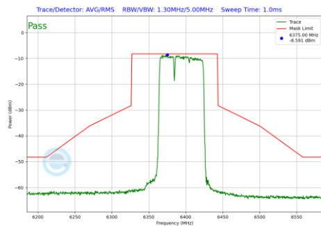
Plot 7-694 In-Band Emission Plot SDM Diversity Antenna WF7b (80MHz BW 802.11be(RU) RU484+242 Index90 (UNII Band 5) - Ch.87)
