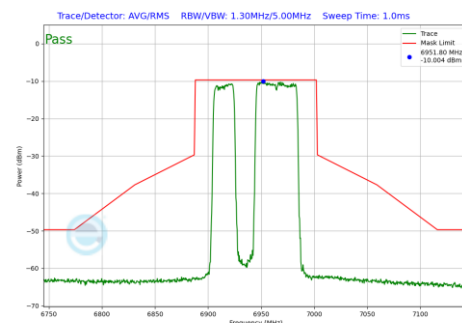
Plot 7-627 In-Band Emission Plot SDM Primary Antenna WF2a (80MHz BW 802.11be(RU) RU484+242 Index91 (UNII Band 8) - Ch.199)
