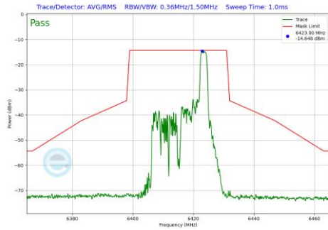
Plot 7-677 In-Band Emission Plot SDM Diversity Antenna WF2a (20MHz BW 802.11be(RU) RU26 Index8 (UNII Band 5) - Ch.93)
