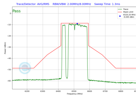
Plot 7-698 In-Band Emission Plot SDM Diversity Antenna WF7b (160MHz BW 802.11be(RU) RU996+484+242 Index97 (UNII Band 6) - Ch.111)
