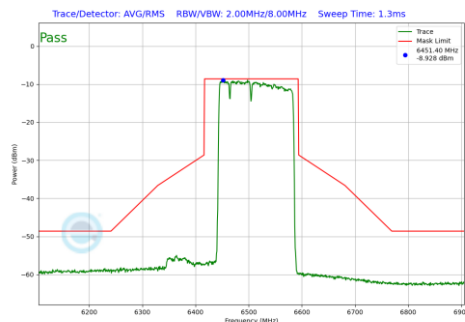
Plot 7-622 In-Band Emission Plot SDM Primary Antenna WF2a (160MHz BW 802.11be(RU) RU996+484+242 Index96 (UNII Band 6) - Ch.111)
