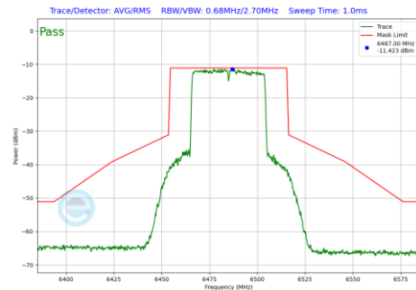
Plot 7-650 In-Band Emission Plot SDM Primary Antenna WF2a (40MHz BW 802.11be(RU) RU484 Index65 (UNII Band 6) - Ch.107)
