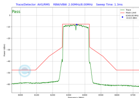
Plot 7-736 In-Band Emission Plot SDM Diversity Antenna WF2a (160MHz BW 802.11be(RU) RU996X2 Index68 (UNII Band 5) - Ch.79)
