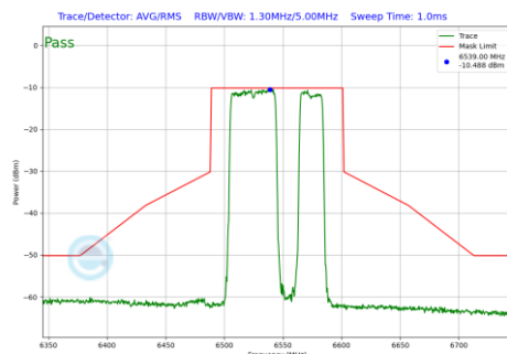
Plot 7-624 In-Band Emission Plot SDM Primary Antenna WF2a (80MHz BW 802.11be(RU) RU484+242 Index92 (UNII Band 7) - Ch.119)
