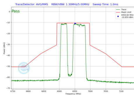
Plot 7-703 In-Band Emission Plot SDM Diversity Antenna WF7b (80MHz BW 802.11be(RU) RU484+242 Index91 (UNII Band 8) - Ch.199)
