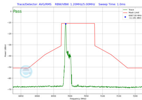
Plot 7-691 In-Band Emission Plot SDM Diversity Antenna WF2a (80MHz BW 802.11be(RU) RU26 Index0 (UNII Band 8) - Ch.215)
