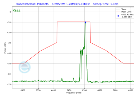
Plot 7-683 In-Band Emission Plot SDM Diversity Antenna WF2a (80MHz BW 802.11be(RU) RU26 Index36 (UNII Band 6) - Ch.103)
