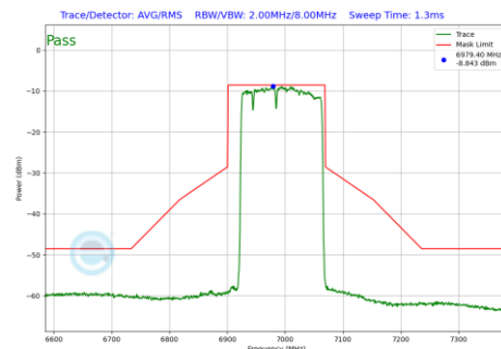
Plot 7-716 In-Band Emission Plot SDM Diversity Antenna WF2a (160MHz BW 802.11be(RU) RU996+484+242 Index96 (UNII Band 8) - Ch.207)
