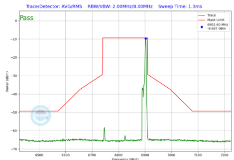
Plot 7-600 In-Band Emission Plot SDM Primary Antenna WF2a (160MHz BW 802.11be(RU) RU26 Index36 (UNII Band 7) - Ch.175)
