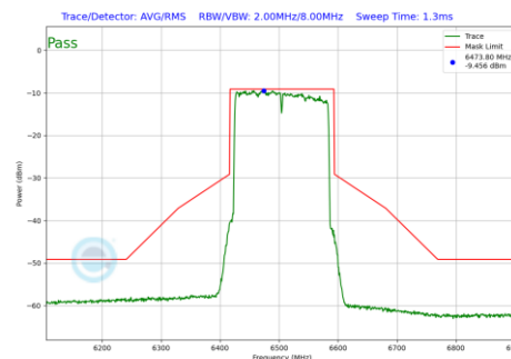
Plot 7-740 In-Band Emission Plot SDM Diversity Antenna WF2a (160MHz BW 802.11be(RU) RU996X2 Index68 (UNII Band 6) - Ch.111)
