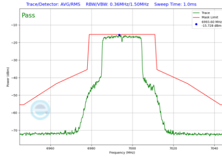
Plot 7-729 In-Band Emission Plot SDM Diversity Antenna WF7b (20MHz BW 802.11be(RU) RU242 Index61 (UNII Band 8) - Ch.209)
