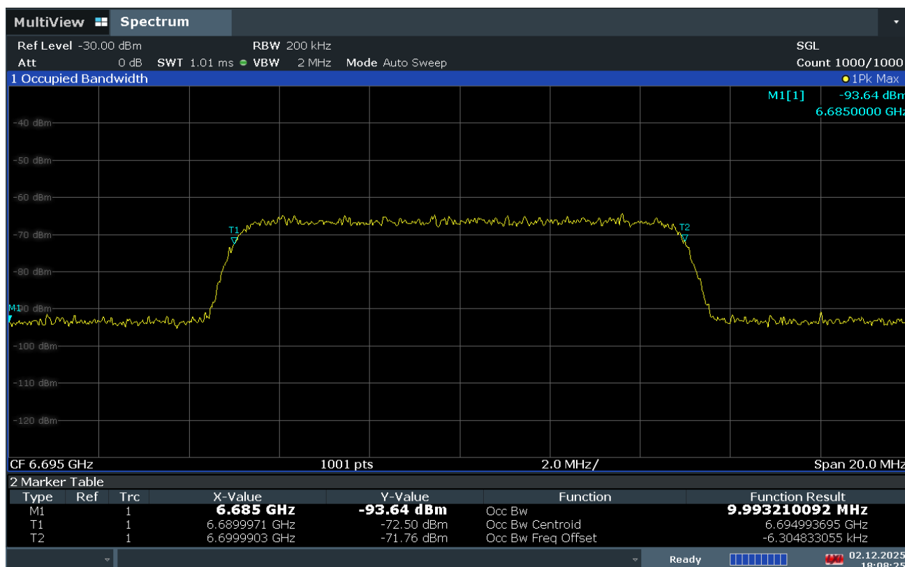
Plot 7-757. AWGN Signal – UNII 7 – 20MHz
