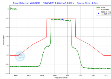
Plot 7-731 In-Band Emission Plot SDM Diversity Antenna WF7b (80MHz BW 802.11be(RU) RU996 Index67 (UNII Band 8) - Ch.215)
