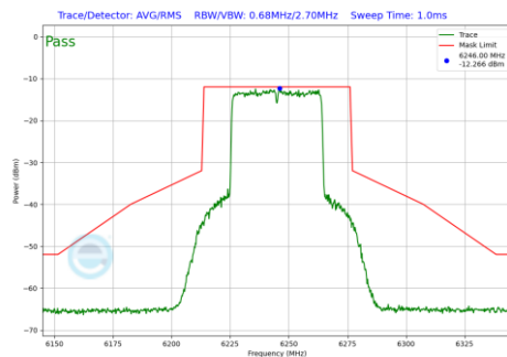
Plot 7-734 In-Band Emission Plot SDM Diversity Antenna WF2a (40MHz BW 802.11be(RU) RU484 Index65 (UNII Band 5) - Ch.59)
