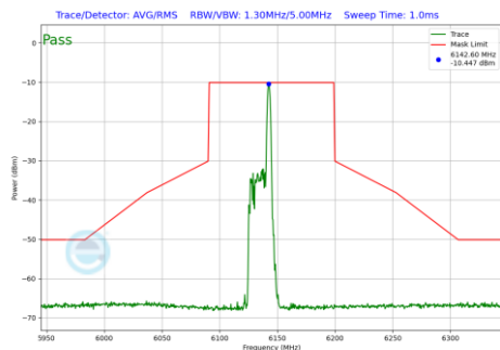
Plot 7-663 In-Band Emission Plot SDM Diversity Antenna WF7b (80MHz BW 802.11be(RU) RU26 Index17 (UNII Band 5) - Ch.39)
