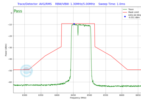
Plot 7-609 In-Band Emission Plot SDM Primary Antenna WF7a (80MHz BW 802.11be(RU) RU484+242 Index90 (UNII Band 6) - Ch.103)
