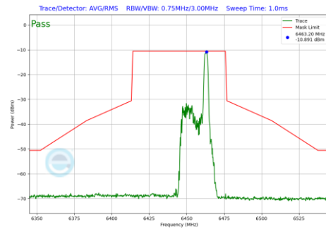
Plot 7-682 In-Band Emission Plot SDM Diversity Antenna WF2a (40MHz BW 802.11be(RU) RU26 Index17 (UNII Band 6) - Ch.99)
