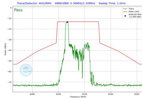
Plot 7-665 In-Band Emission Plot SDM Diversity Antenna WF7b (20MHz BW 802.11be(RU) RU26 Index0 (UNII Band 6) - Ch.113)
