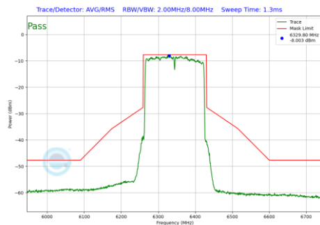
Plot 7-720 In-Band Emission Plot SDM Diversity Antenna WF7b (160MHz BW 802.11be(RU) RU996X2 Index68 (UNII Band 5) - Ch.79)
