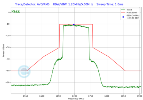
Plot 7-743 In-Band Emission Plot SDM Diversity Antenna WF2a (80MHz BW 802.11be(RU) RU996 Index67 (UNII Band 7) - Ch.151)
