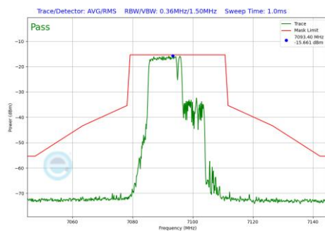
Plot 7-702 In-Band Emission Plot SDM Diversity Antenna WF7b (20MHz BW 802.11be(RU) RU106+26 Index82 (UNII Band 8) - Ch.229)
