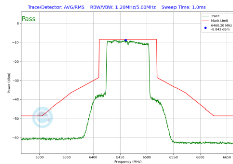
Plot 7-651 In-Band Emission Plot SDM Primary Antenna WF2a (80MHz BW 802.11be(RU) RU996 Index67 (UNII Band 6) - Ch.103)
