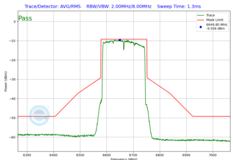
Plot 7-744 In-Band Emission Plot SDM Diversity Antenna WF2a (160MHz BW 802.11be(RU) RU996X2 Index68 (UNII Band 7) - Ch.143)
