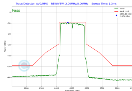
Plot 7-652 In-Band Emission Plot SDM Primary Antenna WF2a (160MHz BW 802.11be(RU) RU996X2 Index68 (UNII Band 6) - Ch.111)
