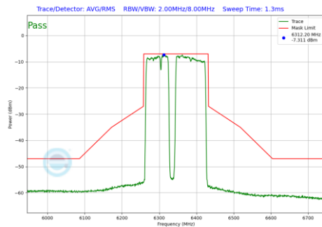
Plot 7-607 In-Band Emission Plot SDM Primary Antenna WF7a (160MHz BW 802.11be(RU) RU996+484+242 Index99 (UNII Band 5) - Ch.79)
