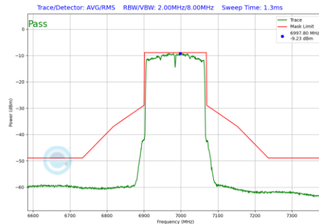
Plot 7-660 In-Band Emission Plot SDM Primary Antenna WF2a (160MHz BW 802.11be(RU) RU996X2 Index68 (UNII Band 8) - Ch.207)
