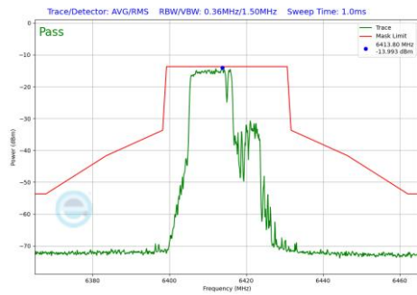
Plot 7-693 In-Band Emission Plot SDM Diversity Antenna WF7b (20MHz BW 802.11be(RU) RU106+26 Index82 (UNII Band 5) - Ch.93)
