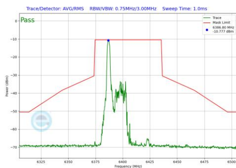
Plot 7-662 In-Band Emission Plot SDM Diversity Antenna WF7b (40MHz BW 802.11be(RU) RU26 Index0 (UNII Band 5) - Ch.91)
