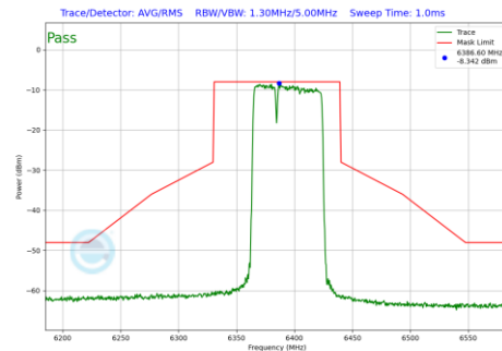
Plot 7-618 In-Band Emission Plot SDM Primary Antenna WF2a (80MHz BW 802.11be(RU) RU484+242 Index90 (UNII Band 5) - Ch.87)
