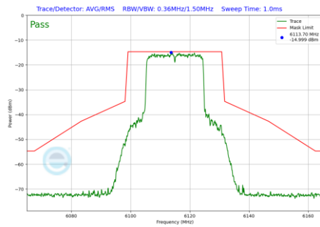
Plot 7-717 In-Band Emission Plot SDM Diversity Antenna WF7b (20MHz BW 802.11be(RU) RU242 Index61 (UNII Band 5) - Ch.33)
