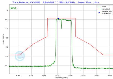
Plot 7-709 In-Band Emission Plot SDM Diversity Antenna WF2a (80MHz BW 802.11be(RU) RU484+242 Index90 (UNII Band 6) - Ch.103)
