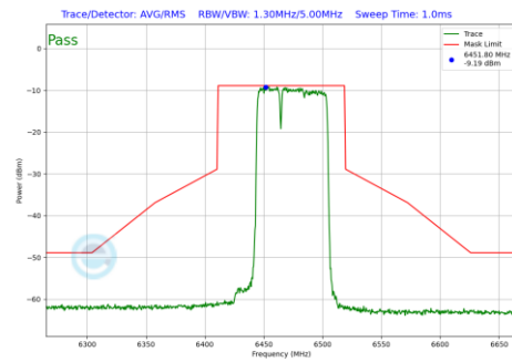
Plot 7-697 In-Band Emission Plot SDM Diversity Antenna WF7b (80MHz BW 802.11be(RU) RU484+242 Index90 (UNII Band 6) - Ch.103)
