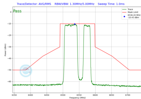
Plot 7-700 In-Band Emission Plot SDM Diversity Antenna WF7b (80MHz BW 802.11be(RU) RU484+242 Index92 (UNII Band 7) - Ch.119)
