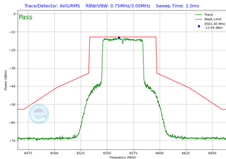
Plot 7-638 In-Band Emission Plot SDM Primary Antenna WF7a (40MHz BW 802.11be(RU) RU484 Index65 (UNII Band 7) - Ch.123)
