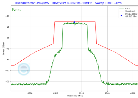
Plot 7-725 In-Band Emission Plot SDM Diversity Antenna WF7b (20MHz BW 802.11be(RU) RU242 Index61 (UNII Band 7) - Ch.117)
