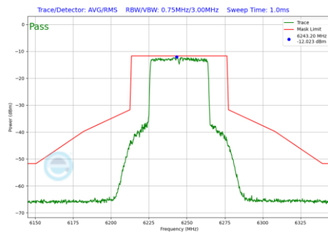
Plot 7-718 In-Band Emission Plot SDM Diversity Antenna WF7b (40MHz BW 802.11be(RU) RU484 Index65 (UNII Band 5) - Ch.59)
