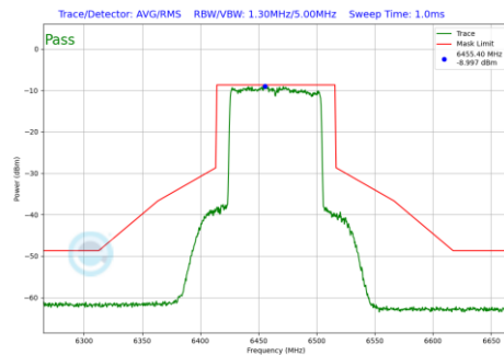
Plot 7-635 In-Band Emission Plot SDM Primary Antenna WF7a (80MHz BW 802.11be(RU) RU996 Index67 (UNII Band 6) - Ch.103)
