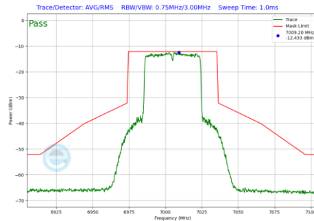
Plot 7-746 In-Band Emission Plot SDM Diversity Antenna WF2a (40MHz BW 802.11be(RU) RU484 Index65 (UNII Band 8) - Ch.211)
