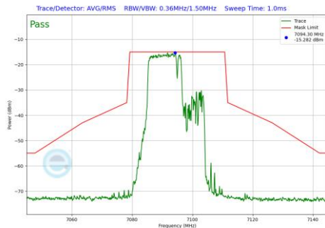
Plot 7-614 In-Band Emission Plot SDM Primary Antenna WF7a (20MHz BW 802.11be(RU) RU106+26 Index82 (UNII Band 8) - Ch.229)
