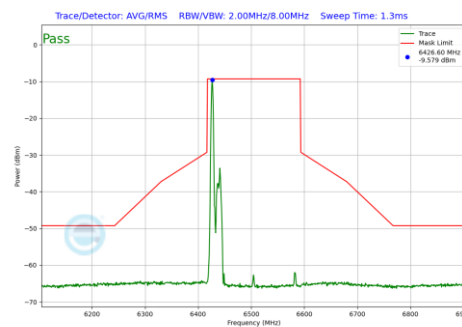
Plot 7-668 In-Band Emission Plot SDM Diversity Antenna WF7b (160MHz BW 802.11be(RU) RU26 Index0 (UNII Band 6) - Ch.111)
