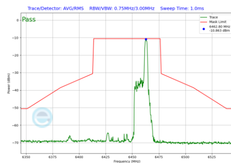
Plot 7-666 In-Band Emission Plot SDM Diversity Antenna WF7b (40MHz BW 802.11be(RU) RU26 Index17 (UNII Band 6) - Ch.99)
