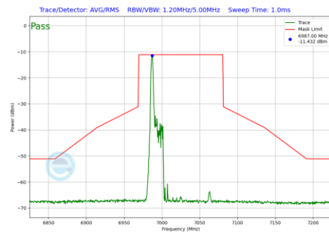
Plot 7-675 In-Band Emission Plot SDM Diversity Antenna WF7b (80MHz BW 802.11be(RU) RU26 Index0 (UNII Band 8) - Ch.215)
