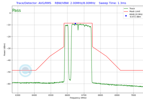
Plot 7-701 In-Band Emission Plot SDM Diversity Antenna WF7b (160MHz BW 802.11be(RU) RU996+484+242 Index97 (UNII Band 7) - Ch.143)
