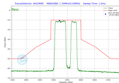
Plot 7-612 In-Band Emission Plot SDM Primary Antenna WF7a (80MHz BW 802.11be(RU) RU484+242 Index92 (UNII Band 7) - Ch.119)
