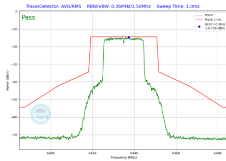
Plot 7-633 In-Band Emission Plot SDM Primary Antenna WF7a (20MHz BW 802.11be(RU) RU242 Index61 (UNII Band 6) - Ch.97)
