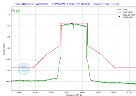
Plot 7-632 In-Band Emission Plot SDM Primary Antenna WF7a (160MHz BW 802.11be(RU) RU996X2 Index68 (UNII Band 5) - Ch.79)
