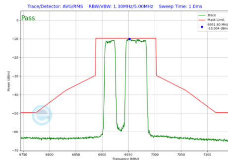
Plot 7-715 In-Band Emission Plot SDM Diversity Antenna WF2a (80MHz BW 802.11be(RU) RU484+242 Index91 (UNII Band 8) - Ch.199)
