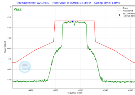
Plot 7-737 In-Band Emission Plot SDM Diversity Antenna WF2a (20MHz BW 802.11be(RU) RU242 Index61 (UNII Band 6) - Ch.113)
