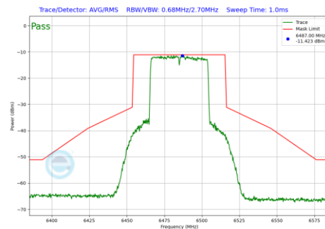
Plot 7-738 In-Band Emission Plot SDM Diversity Antenna WF2a (40MHz BW 802.11be(RU) RU484 Index65 (UNII Band 6) - Ch.107)
