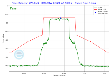
Plot 7-629 In-Band Emission Plot SDM Primary Antenna WF7a (20MHz BW 802.11be(RU) RU242 Index61 (UNII Band 5) - Ch.93)
