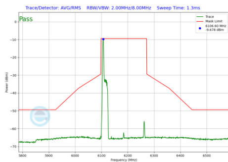
Plot 7-664 In-Band Emission Plot SDM Diversity Antenna WF7b (160MHz BW 802.11be(RU) RU26 Index0 (UNII Band 5) - Ch.47)
