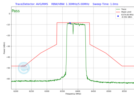
Plot 7-606 In-Band Emission Plot SDM Primary Antenna WF7a (80MHz BW 802.11be(RU) RU484+242 Index90 (UNII Band 5) - Ch.87)
