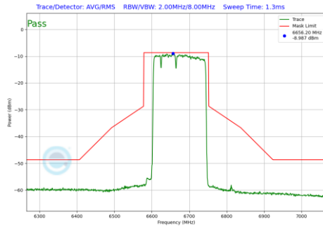
Plot 7-613 In-Band Emission Plot SDM Primary Antenna WF7a (160MHz BW 802.11be(RU) RU996+484+242 Index96 (UNII Band 7) - Ch.143)
