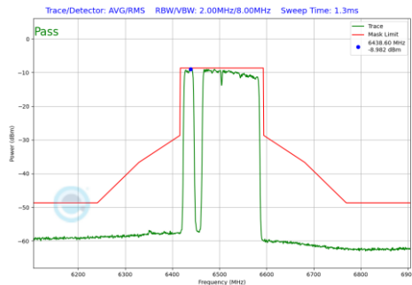
Plot 7-710 In-Band Emission Plot SDM Diversity Antenna WF2a (160MHz BW 802.11be(RU) RU996+484+242 Index97 (UNII Band 6) - Ch.111)
