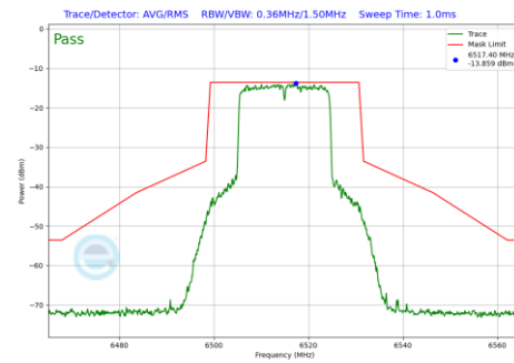
Plot 7-721 In-Band Emission Plot SDM Diversity Antenna WF7b (20MHz BW 802.11be(RU) RU242 Index61 (UNII Band 6) - Ch.113)
