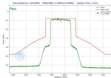
Plot 7-719 In-Band Emission Plot SDM Diversity Antenna WF7b (80MHz BW 802.11be(RU) RU996 Index67 (UNII Band 5) - Ch.87)
