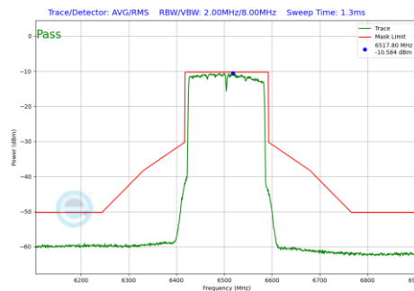
Plot 7-636 In-Band Emission Plot SDM Primary Antenna WF7a (160MHz BW 802.11be(RU) RU996X2 Index68 (UNII Band 6) - Ch.111)
