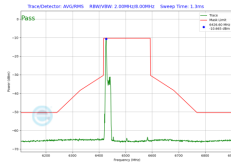
Plot 7-684 In-Band Emission Plot SDM Diversity Antenna WF2a (160MHz BW 802.11be(RU) RU26 Index0 (UNII Band 6) - Ch.111)
