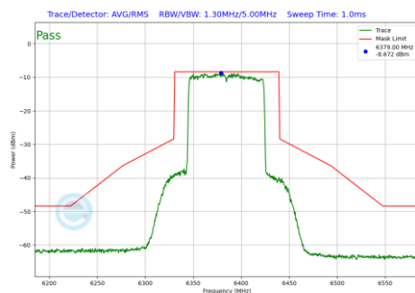
Plot 7-735 In-Band Emission Plot SDM Diversity Antenna WF2a (80MHz BW 802.11be(RU) RU996 Index67 (UNII Band 5) - Ch.87)
