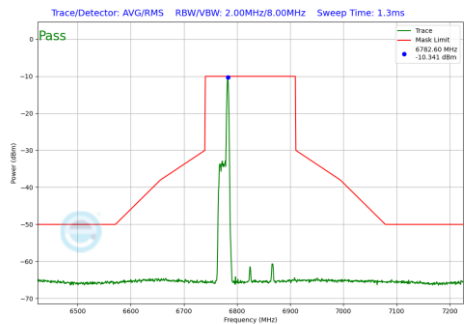
Plot 7-688 In-Band Emission Plot SDM Diversity Antenna WF2a (160MHz BW 802.11be(RU) RU26 Index17 (UNII Band 7) - Ch.175)
