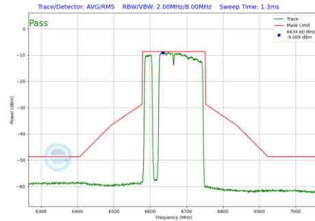
Plot 7-713 In-Band Emission Plot SDM Diversity Antenna WF2a (160MHz BW 802.11be(RU) RU996+484+242 Index97 (UNII Band 7) - Ch.143)
