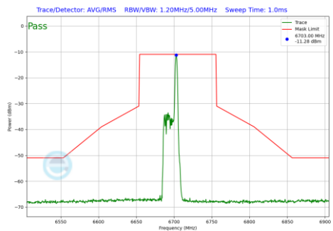
Plot 7-687 In-Band Emission Plot SDM Diversity Antenna WF2a (80MHz BW 802.11be(RU) RU26 Index17 (UNII Band 7) - Ch.151)
