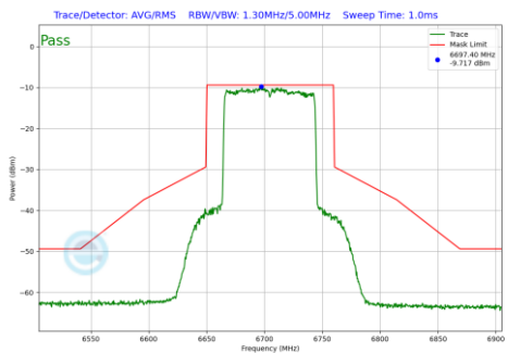
Plot 7-727 In-Band Emission Plot SDM Diversity Antenna WF7b (80MHz BW 802.11be(RU) RU996 Index67 (UNII Band 7) - Ch.151)
