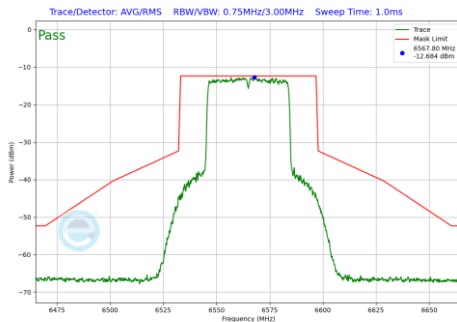
Plot 7-654 In-Band Emission Plot SDM Primary Antenna WF2a (40MHz BW 802.11be(RU) RU484 Index65 (UNII Band 7) - Ch.123)
