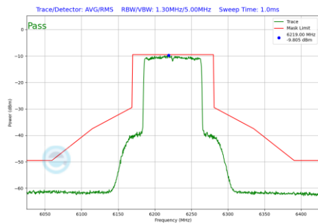
Plot 7-647 In-Band Emission Plot SDM Primary Antenna WF2a (80MHz BW 802.11be(RU) RU996 Index67 (UNII Band 5) - Ch.55)
