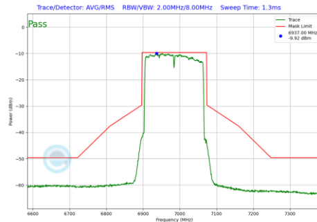
Plot 7-644 In-Band Emission Plot SDM Primary Antenna WF7a (160MHz BW 802.11be(RU) RU996X2 Index68 (UNII Band 8) - Ch.207)
