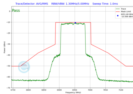
Plot 7-659 In-Band Emission Plot SDM Primary Antenna WF2a (80MHz BW 802.11be(RU) RU996 Index67 (UNII Band 8) - Ch.199)
