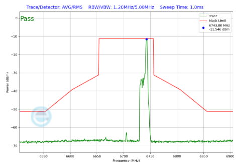
Plot 7-599 In-Band Emission Plot SDM Primary Antenna WF2a (80MHz BW 802.11be(RU) RU26 Index36 (UNII Band 7) - Ch.151)
