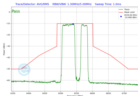
Plot 7-712 In-Band Emission Plot SDM Diversity Antenna WF2a (80MHz BW 802.11be(RU) RU484+242 Index92 (UNII Band 7) - Ch.119)
