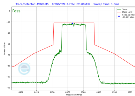
Plot 7-634 In-Band Emission Plot SDM Primary Antenna WF7a (40MHz BW 802.11be(RU) RU484 Index65 (UNII Band 6) - Ch.107)
