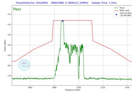
Plot 7-673 In-Band Emission Plot SDM Diversity Antenna WF7b (20MHz BW 802.11be(RU) RU26 Index0 (UNII Band 8) - Ch.229)
