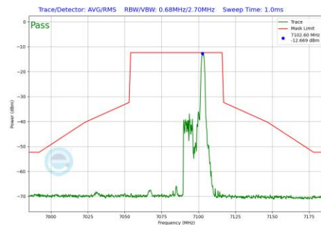
Plot 7-690 In-Band Emission Plot SDM Diversity Antenna WF2a (40MHz BW 802.11be(RU) RU26 Index17 (UNII Band 8) - Ch.227)
