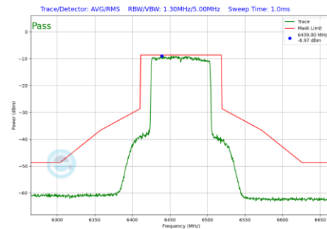
Plot 7-723 In-Band Emission Plot SDM Diversity Antenna WF7b (80MHz BW 802.11be(RU) RU996 Index67 (UNII Band 6) - Ch.103)
