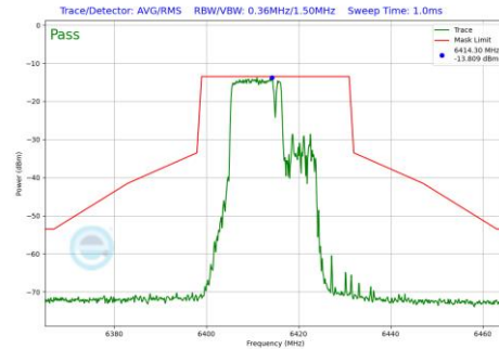
Plot 7-617 In-Band Emission Plot SDM Primary Antenna WF2a (20MHz BW 802.11be(RU) RU106+26 Index82 (UNII Band 5) - Ch.93)
