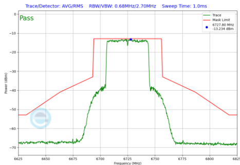
Plot 7-726 In-Band Emission Plot SDM Diversity Antenna WF7b (40MHz BW 802.11be(RU) RU484 Index65 (UNII Band 7) - Ch.155)
