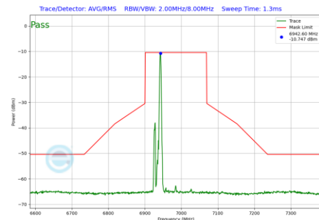
Plot 7-604 In-Band Emission Plot SDM Primary Antenna WF2a (160MHz BW 802.11be(RU) RU26 Index17 (UNII Band 8) - Ch.207)
