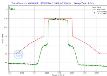
Plot 7-655 In-Band Emission Plot SDM Primary Antenna WF2a (80MHz BW 802.11be(RU) RU996 Index67 (UNII Band 7) - Ch.119)
