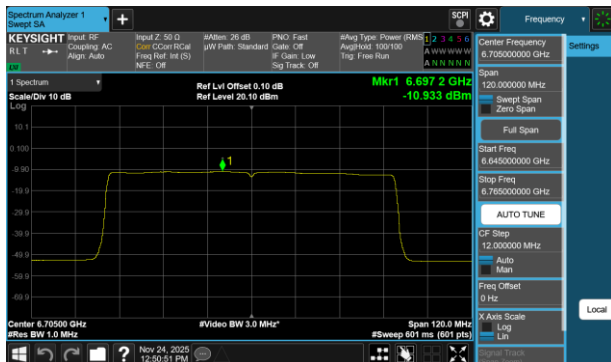
Plot 7-743 PSD SDM Diversity Antenna WF2a (80MHz BW 802.11be(RU) RU996 Index67 - Ch.151)
