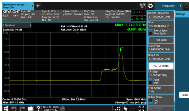
Plot 7-729 PSD SDM Diversity Antenna WF2a (80MHz BW 802.11be(RU) RU26 Index36 - Ch.151)
