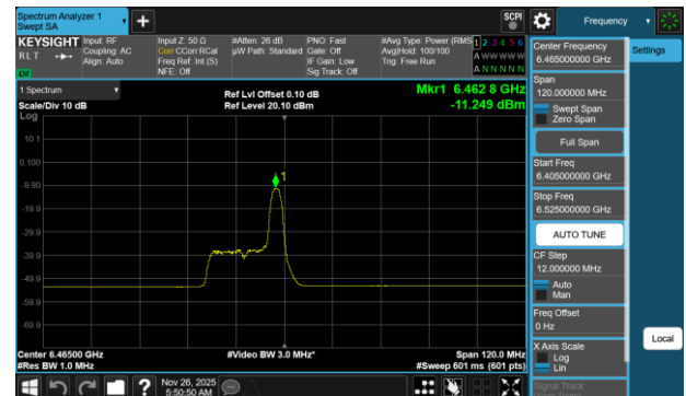
Plot 7-711 PSD SDM Diversity Antenna WF7b (80MHz BW 802.11be(RU) RU26 Index17 - Ch.103)
