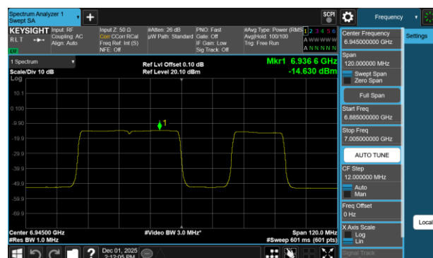
Plot 7-761 PSD SDM Diversity Antenna WF7b (80MHz BW 802.11be(RU) RU484+242 Index92 - Ch.199)
