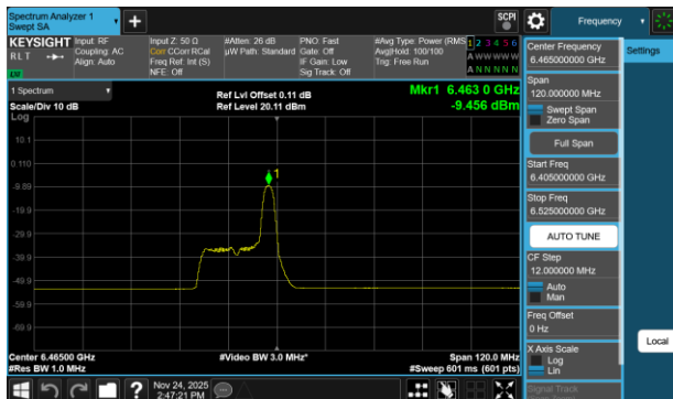
Plot 7-707 PSD SDM Diversity Antenna WF2a (80MHz BW 802.11be(RU) RU26 Index17 - Ch.103)
