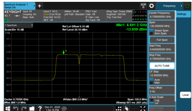
Plot 7-739 PSD SDM Diversity Antenna WF7b (80MHz BW 802.11be(RU) RU484+242 Index90 - Ch.151)
