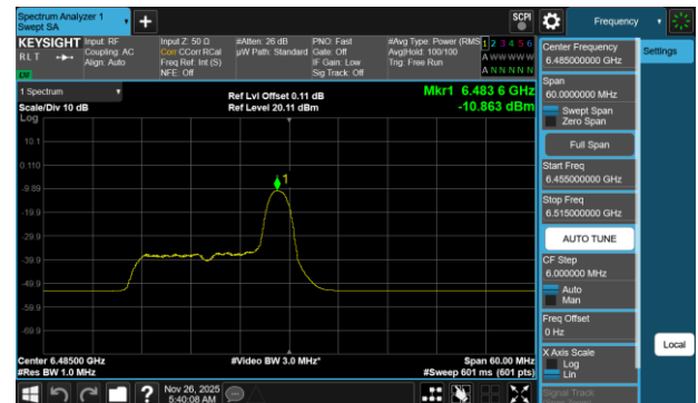
Plot 7-710 PSD SDM Diversity Antenna WF7b (40MHz BW 802.11be(RU) RU26 Index8 - Ch.107)
