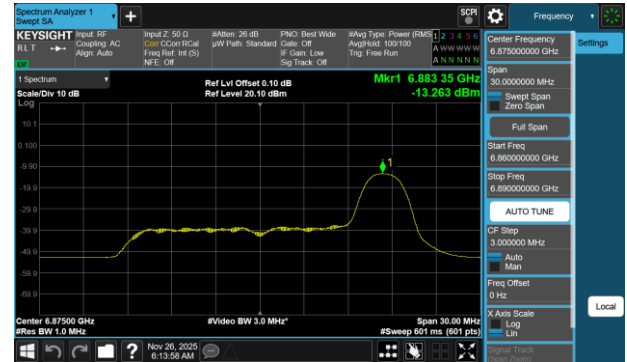
Plot 7-731 PSD SDM Diversity Antenna WF7b (20MHz BW 802.11be(RU) RU26 Index8 - Ch.185)
