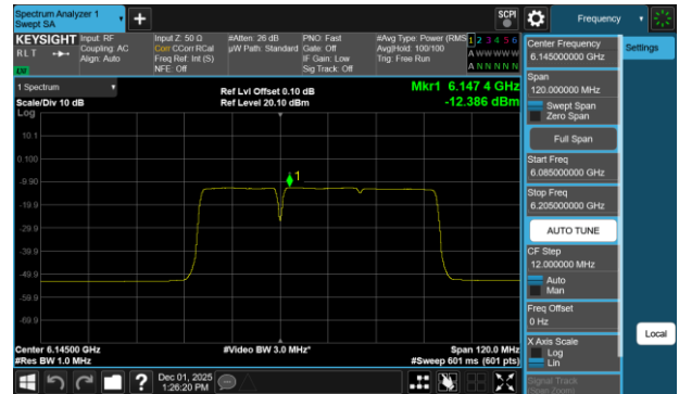
Plot 7-695 PSD SDM Diversity Antenna WF7b (80MHz BW 802.11be(RU) RU484+242 Index90 - Ch.39)
