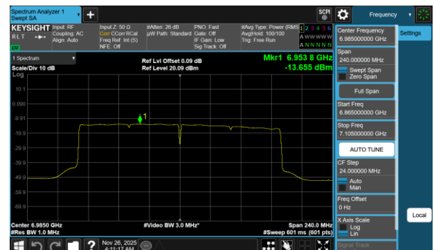
Plot 7-770 PSD SDM Diversity Antenna WF7b (160MHz BW 802.11be(RU) RU996X2 Index68 - Ch.207)
