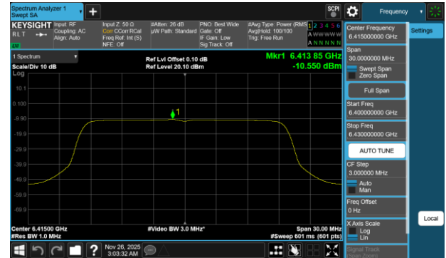
Plot 7-701 PSD SDM Diversity Antenna WF7b (20MHz BW 802.11be(RU) RU242 Index61 - Ch.93)
