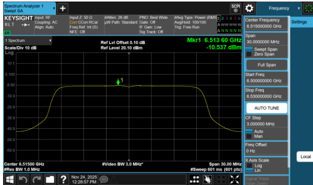
Plot 7-719 PSD SDM Diversity Antenna WF2a (20MHz BW 802.11be(RU) RU242 Index61 - Ch.113)
