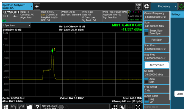
Plot 7-708 PSD SDM Diversity Antenna WF2a (160MHz BW 802.11be(RU) RU26 Index17 - Ch.111)
