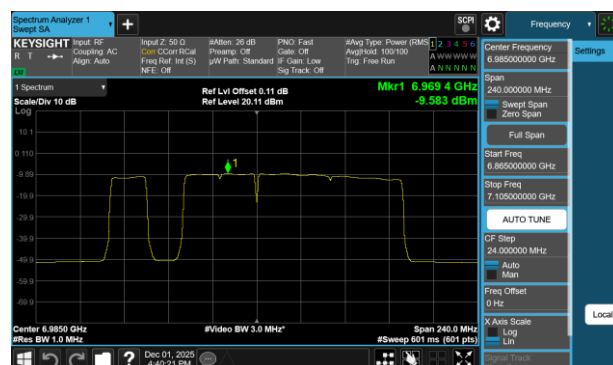
Plot 7-762 PSD SDM Diversity Antenna WF7b (160MHz BW 802.11be(RU) RU996+484+242 Index97 - Ch.207)
