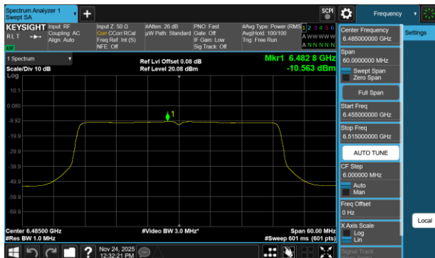
Plot 7-720 PSD SDM Diversity Antenna WF2a (40MHz BW 802.11be(RU) RU484 Index65 - Ch.107)
