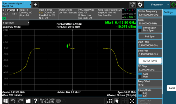
Plot 7-697 PSD SDM Diversity Antenna WF2a (20MHz BW 802.11be(RU) RU242 Index61 - Ch.93)
