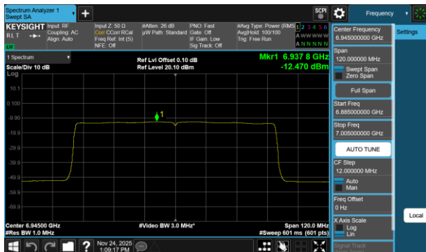
Plot 7-765 PSD SDM Diversity Antenna WF2a (80MHz BW 802.11be(RU) RU996 Index67 - Ch.199)
