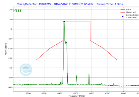
Plot 7-778 In-Band Emission Plot Antenna WF7a (160MHz BW 802.11be(RU) RU26 Index0 (UNII Band 6) - Ch.111)
