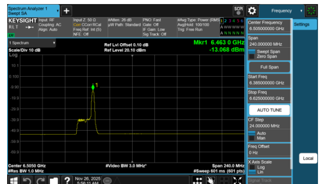
Plot 7-712 PSD SDM Diversity Antenna WF7b (160MHz BW 802.11be(RU) RU26 Index17 - Ch.111)
