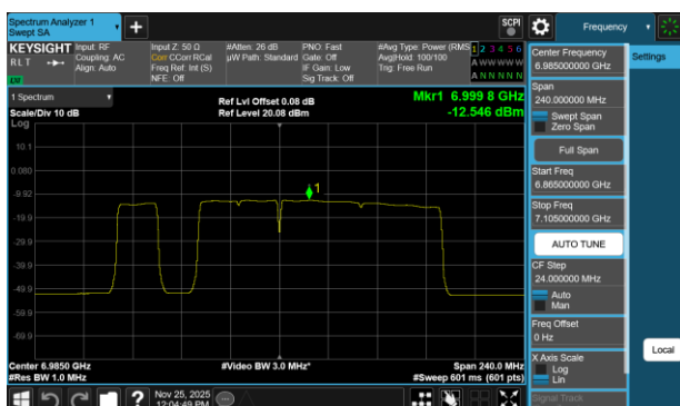
Plot 7-759 PSD SDM Diversity Antenna WF2a (160MHz BW 802.11be(RU) RU996+484+242 Index97 - Ch.207)
