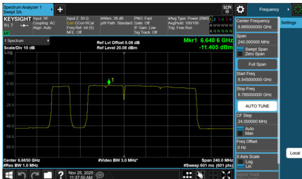
Plot 7-737 PSD SDM Diversity Antenna WF2a (160MHz BW 802.11be(RU) RU996+484+242 Index97 - Ch.143)
