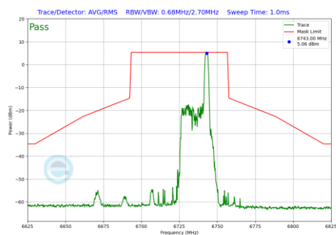
Plot 7-780 In-Band Emission Plot Antenna WF7a (40MHz BW 802.11be(RU) RU26 Index17 (UNII Band 7) - Ch.155)
