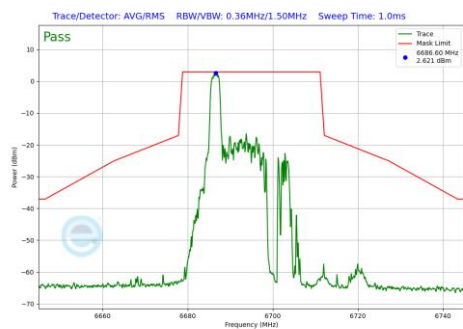
Plot 7-779 In-Band Emission Plot Antenna WF7a (20MHz BW 802.11be(RU) RU26 Index0 (UNII Band 7) - Ch.149)
