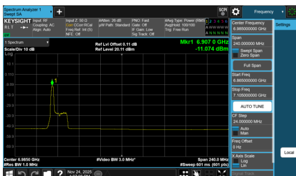
Plot 7-752 PSD SDM Diversity Antenna WF2a (160MHz BW 802.11be(RU) RU26 Index0 - Ch.207)
