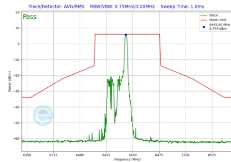
Plot 7-776 In-Band Emission Plot Antenna WF7a (40MHz BW 802.11be(RU) RU26 Index8 (UNII Band 6) - Ch.99)
