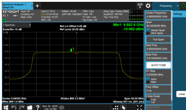
Plot 7-764 PSD SDM Diversity Antenna WF2a (40MHz BW 802.11be(RU) RU484 Index65 - Ch.187)
