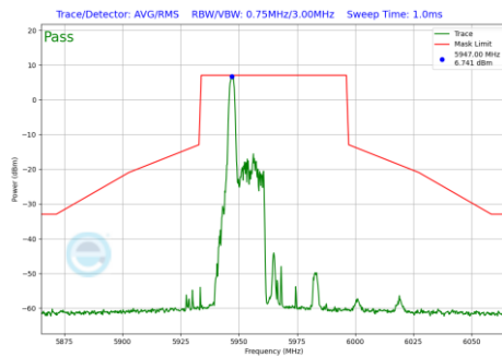
Plot 7-772 In-Band Emission Plot Antenna WF7a (40MHz BW 802.11be(RU) RU26 Index0 (UNII Band 5) - Ch.3)
