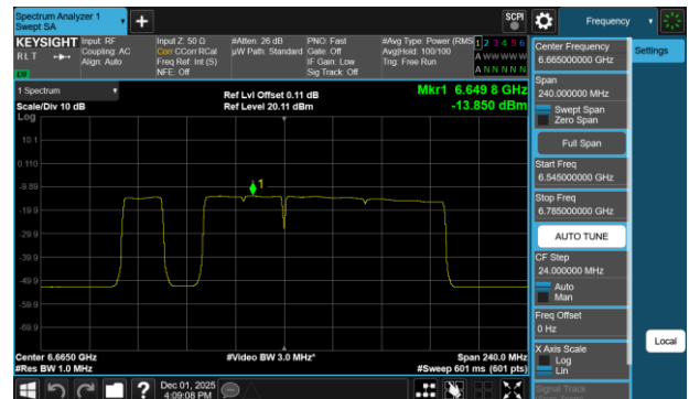
Plot 7-740 PSD SDM Diversity Antenna WF7b (160MHz BW 802.11be(RU) RU996+484+242 Index97 - Ch.143)
