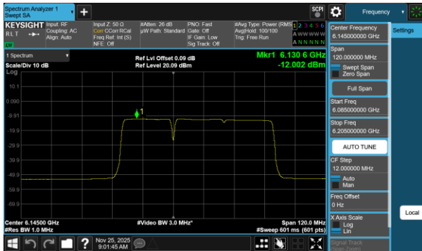
Plot 7-692 PSD SDM Diversity Antenna WF2a (80MHz BW 802.11be(RU) RU484+242 Index90 - Ch.39)
