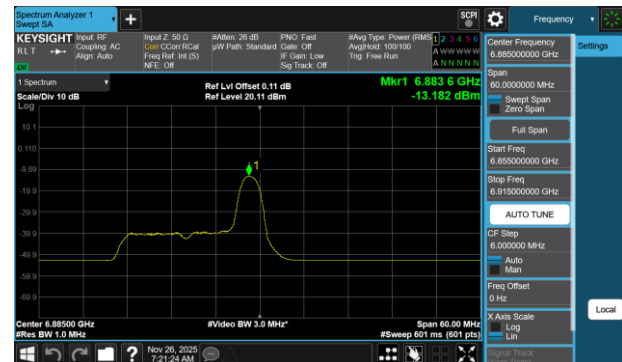
Plot 7-754 PSD SDM Diversity Antenna WF7b (40MHz BW 802.11be(RU) RU26 Index8 - Ch.187)
