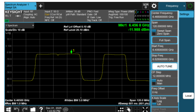
Plot 7-717 PSD SDM Diversity Antenna WF7b (80MHz BW 802.11be(RU) RU484+242 Index92 - Ch.103)
