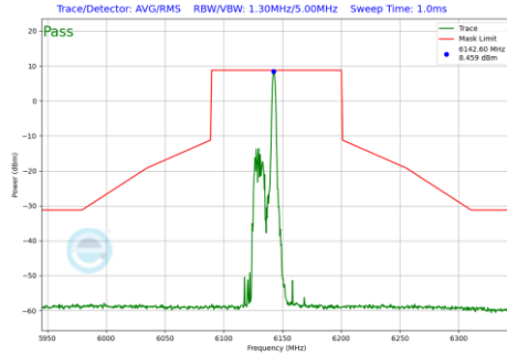
Plot 7-773 In-Band Emission Plot Antenna WF7a (80MHz BW 802.11be(RU) RU26 Index17 (UNII Band 5) - Ch.39)
