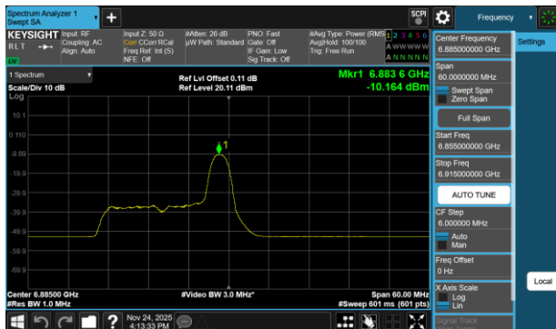
Plot 7-750 PSD SDM Diversity Antenna WF2a (40MHz BW 802.11be(RU) RU26 Index8 - Ch.187)
