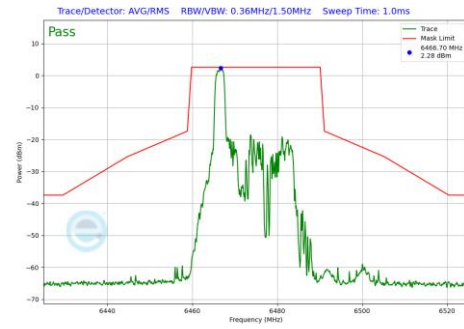
Plot 7-775 In-Band Emission Plot Antenna WF7a (20MHz BW 802.11be(RU) RU26 Index0 (UNII Band 6) - Ch.105)
