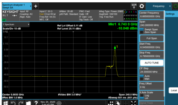
Plot 7-730 PSD SDM Diversity Antenna WF2a (160MHz BW 802.11be(RU) RU26 Index36 - Ch.143)
