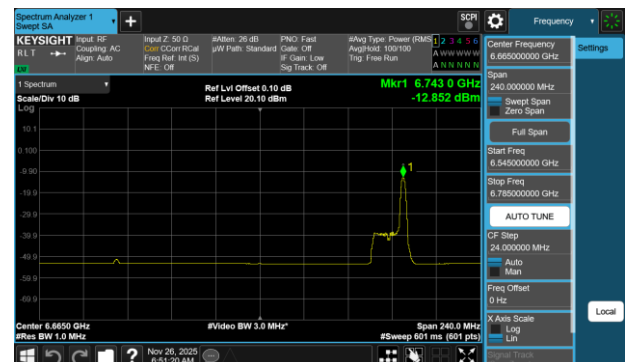
Plot 7-734 PSD SDM Diversity Antenna WF7b (160MHz BW 802.11be(RU) RU26 Index36 - Ch.143)
