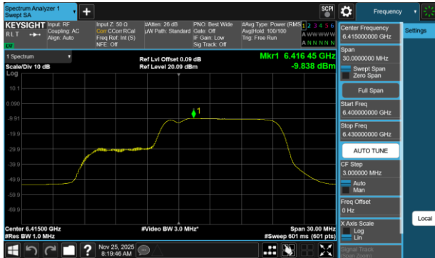
Plot 7-691 PSD SDM Diversity Antenna WF2a (20MHz BW 802.11be(RU) RU106+26 Index83 - Ch.93)
