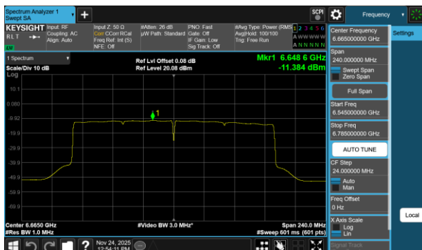
Plot 7-744 PSD SDM Diversity Antenna WF2a (160MHz BW 802.11be(RU) RU996X2 Index68 - Ch.143)
