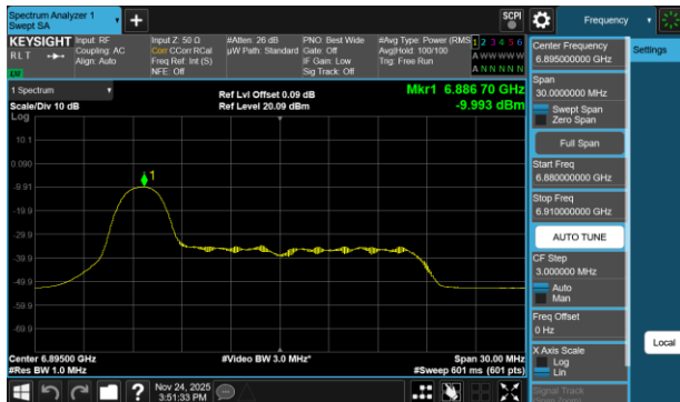
Plot 7-749 PSD SDM Diversity Antenna WF2a (20MHz BW 802.11be(RU) RU26 Index0 - Ch.189)
