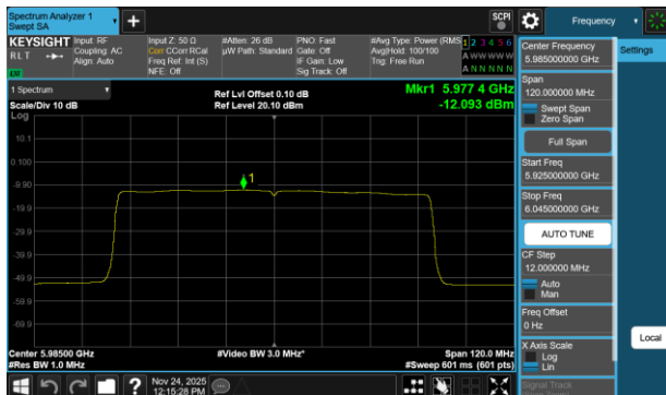
Plot 7-699 PSD SDM Diversity Antenna WF2a (80MHz BW 802.11be(RU) RU996 Index67 - Ch.7)
