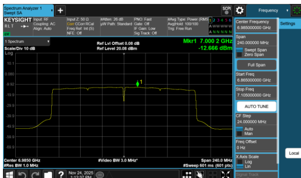
Plot 7-766 PSD SDM Diversity Antenna WF2a (160MHz BW 802.11be(RU) RU996X2 Index68 - Ch.207)
