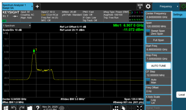
Plot 7-751 PSD SDM Diversity Antenna WF2a (80MHz BW 802.11be(RU) RU26 Index0 - Ch.199)
