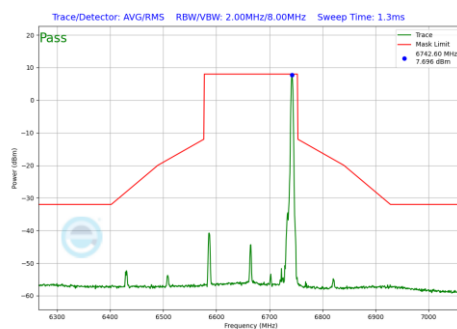
Plot 7-782 In-Band Emission Plot Antenna WF7a (160MHz BW 802.11be(RU) RU26 Index36 (UNII Band 7) - Ch.143)
