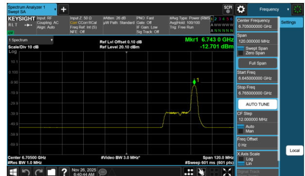
Plot 7-733 PSD SDM Diversity Antenna WF7b (80MHz BW 802.11be(RU) RU26 Index36 - Ch.151)
