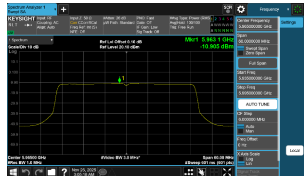
Plot 7-702 PSD SDM Diversity Antenna WF7b (40MHz BW 802.11be(RU) RU484 Index65 - Ch.3)
