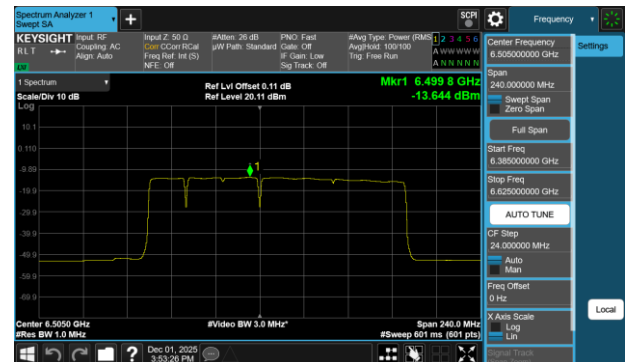
Plot 7-718 PSD SDM Diversity Antenna WF7b (160MHz BW 802.11be(RU) RU996+484+242 Index96 - Ch.111)
