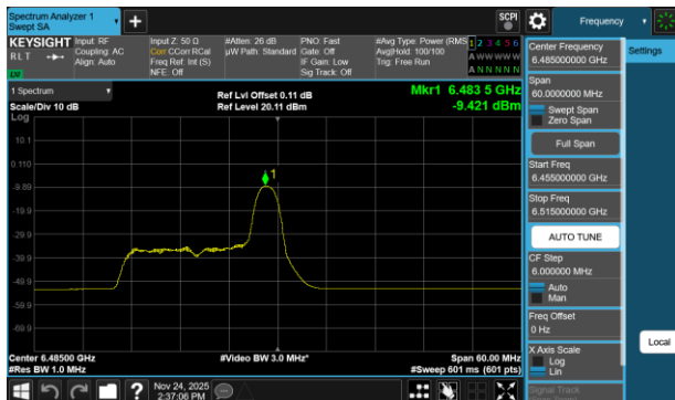
Plot 7-706 PSD SDM Diversity Antenna WF2a (40MHz BW 802.11be(RU) RU26 Index8 - Ch.107)
