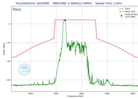
Plot 7-771 In-Band Emission Plot Antenna WF7a (20MHz BW 802.11be(RU) RU26 Index0 (UNII Band 5) - Ch.1)
