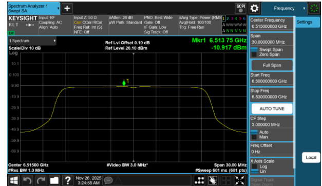
Plot 7-723 PSD SDM Diversity Antenna WF7b (20MHz BW 802.11be(RU) RU242 Index61 - Ch.113)
