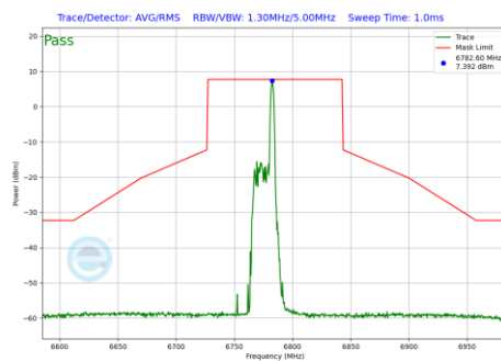
Plot 7-781 In-Band Emission Plot Antenna WF7a (80MHz BW 802.11be(RU) RU26 Index17 (UNII Band 7) - Ch.167)
