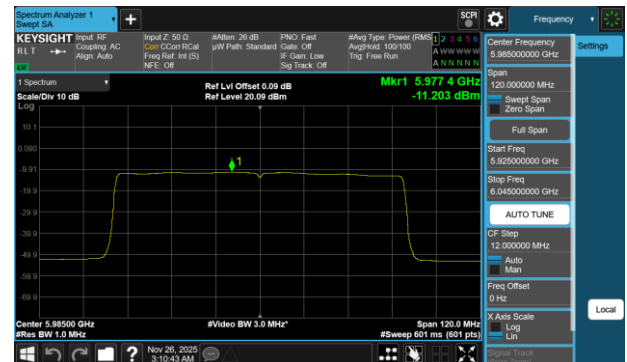
Plot 7-703 PSD SDM Diversity Antenna WF7b (80MHz BW 802.11be(RU) RU996 Index67 - Ch.7)
