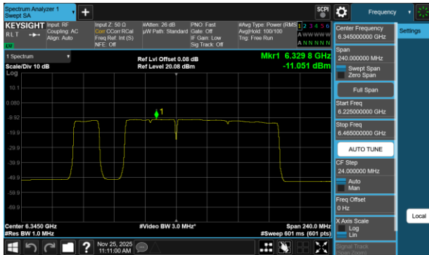
Plot 7-693 PSD SDM Diversity Antenna WF2a (160MHz BW 802.11be(RU) RU996+484+242 Index97 - Ch.79)
