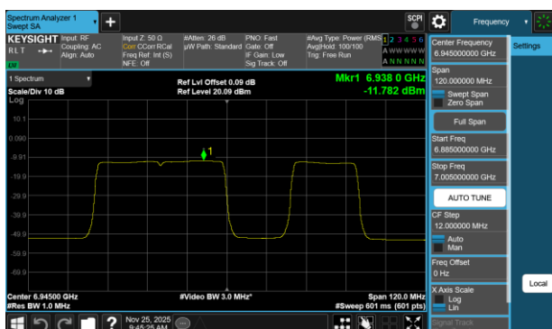
Plot 7-758 PSD SDM Diversity Antenna WF2a (80MHz BW 802.11be(RU) RU484+242 Index92 - Ch.199)
