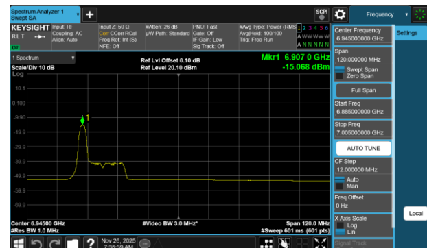
Plot 7-755 PSD SDM Diversity Antenna WF7b (80MHz BW 802.11be(RU) RU26 Index0 - Ch.199)
