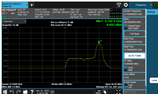
Plot 7-728 PSD SDM Diversity Antenna WF2a (40MHz BW 802.11be(RU) RU26 Index17 - Ch.155)
