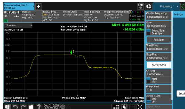
Plot 7-760 PSD SDM Diversity Antenna WF7b (20MHz BW 802.11be(RU) RU106+26 Index82 - Ch.189)
