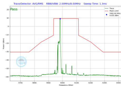
Plot 7-774 In-Band Emission Plot Antenna WF7a (160MHz BW 802.11be(RU) RU26 Index17 (UNII Band 5) - Ch.15)
