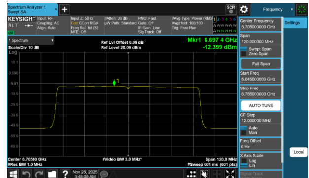
Plot 7-747 PSD SDM Diversity Antenna WF7b (80MHz BW 802.11be(RU) RU996 Index67 - Ch.151)
