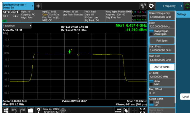
Plot 7-721 PSD SDM Diversity Antenna WF2a (80MHz BW 802.11be(RU) RU996 Index67 - Ch.103)
