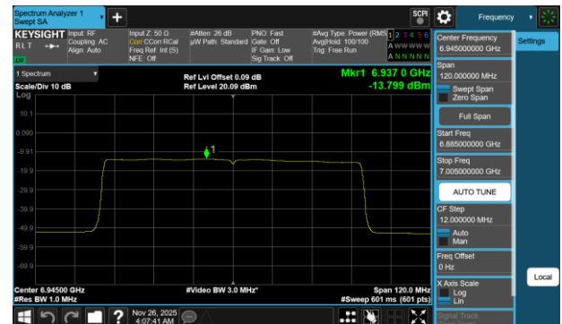
Plot 7-769 PSD SDM Diversity Antenna WF7b (80MHz BW 802.11be(RU) RU996 Index67 - Ch.199)
