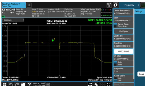
Plot 7-722 PSD SDM Diversity Antenna WF2a (160MHz BW 802.11be(RU) RU996X2 Index68 - Ch.111)
