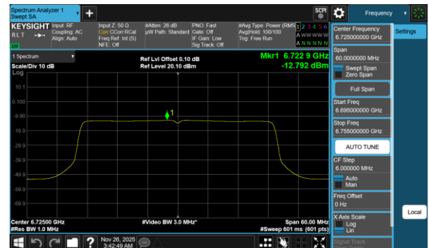
Plot 7-746 PSD SDM Diversity Antenna WF7b (40MHz BW 802.11be(RU) RU484 Index65 - Ch.155)
