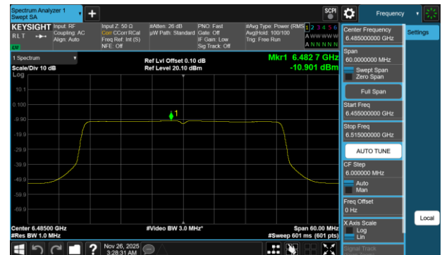
Plot 7-724 PSD SDM Diversity Antenna WF7b (40MHz BW 802.11be(RU) RU484 Index65 - Ch.107)
