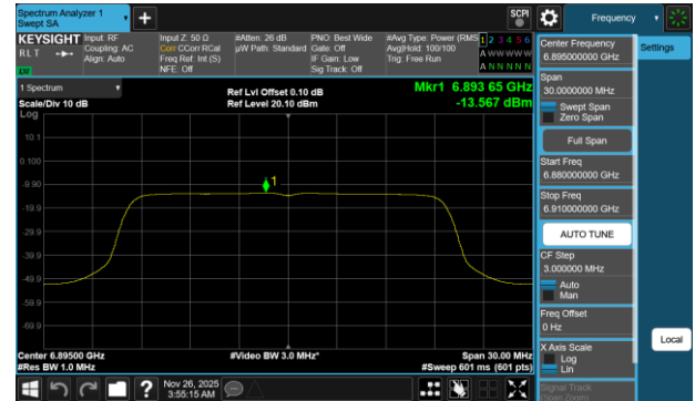
Plot 7-767 PSD SDM Diversity Antenna WF7b (20MHz BW 802.11be(RU) RU242 Index61 - Ch.189)
