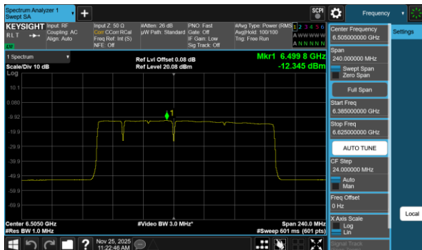
Plot 7-715 PSD SDM Diversity Antenna WF2a (160MHz BW 802.11be(RU) RU996+484+242 Index96 - Ch.111)
