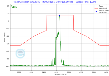
Plot 7-777 In-Band Emission Plot Antenna WF7a (80MHz BW 802.11be(RU) RU26 Index17 (UNII Band 6) - Ch.103)
