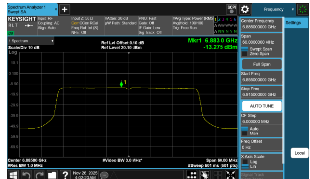
Plot 7-768 PSD SDM Diversity Antenna WF7b (40MHz BW 802.11be(RU) RU484 Index65 - Ch.187)
