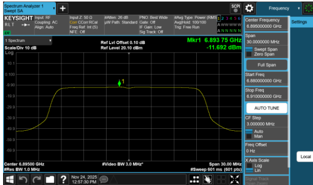
Plot 7-763 PSD SDM Diversity Antenna WF2a (20MHz BW 802.11be(RU) RU242 Index61 - Ch.189)
