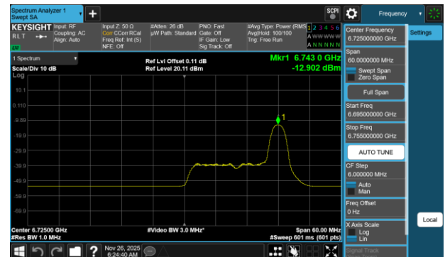
Plot 7-732 PSD SDM Diversity Antenna WF7b (40MHz BW 802.11be(RU) RU26 Index17 - Ch.155)
