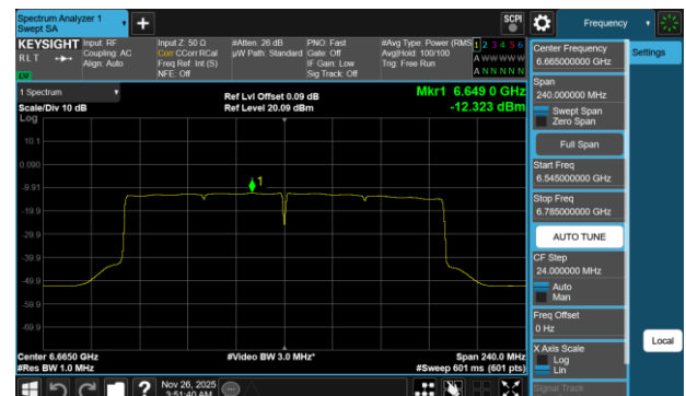
Plot 7-748 PSD SDM Diversity Antenna WF7b (160MHz BW 802.11be(RU) RU996X2 Index68 - Ch.143)
