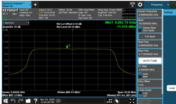
Plot 7-741 PSD SDM Diversity Antenna WF2a (20MHz BW 802.11be(RU) RU242 Index61 - Ch.149)
