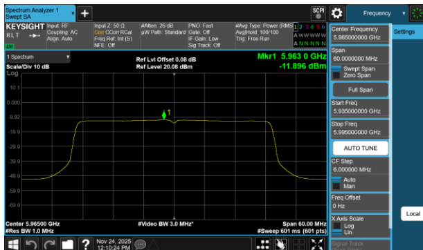
Plot 7-698 PSD SDM Diversity Antenna WF2a (40MHz BW 802.11be(RU) RU484 Index65 - Ch.3)
