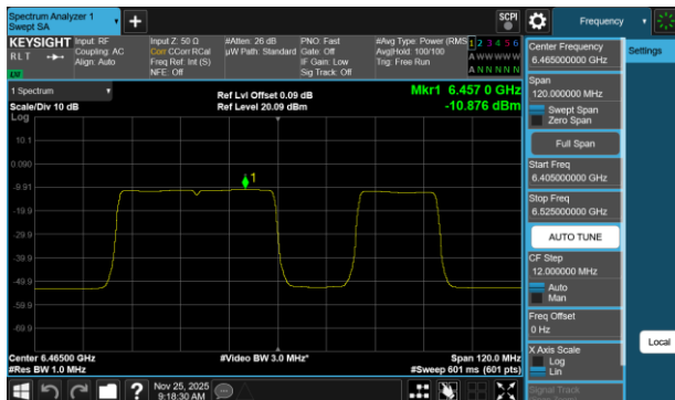
Plot 7-714 PSD SDM Diversity Antenna WF2a (80MHz BW 802.11be(RU) RU484+242 Index92 - Ch.103)
