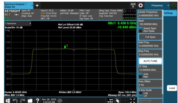
Plot 7-725 PSD SDM Diversity Antenna WF7b (80MHz BW 802.11be(RU) RU996 Index67 - Ch.103)
