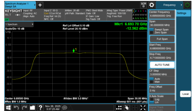
Plot 7-745 PSD SDM Diversity Antenna WF7b (20MHz BW 802.11be(RU) RU242 Index61 - Ch.149)
