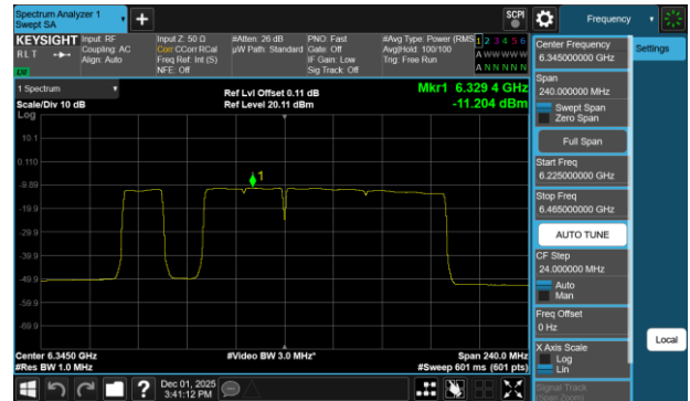
Plot 7-696 PSD SDM Diversity Antenna WF7b (160MHz BW 802.11be(RU) RU996+484+242 Index97 - Ch.79)
