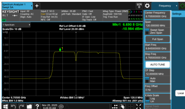
Plot 7-736 PSD SDM Diversity Antenna WF2a (80MHz BW 802.11be(RU) RU484+242 Index90 - Ch.151)
