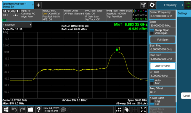
Plot 7-727 PSD SDM Diversity Antenna WF2a (20MHz BW 802.11be(RU) RU26 Index8 - Ch.185)
