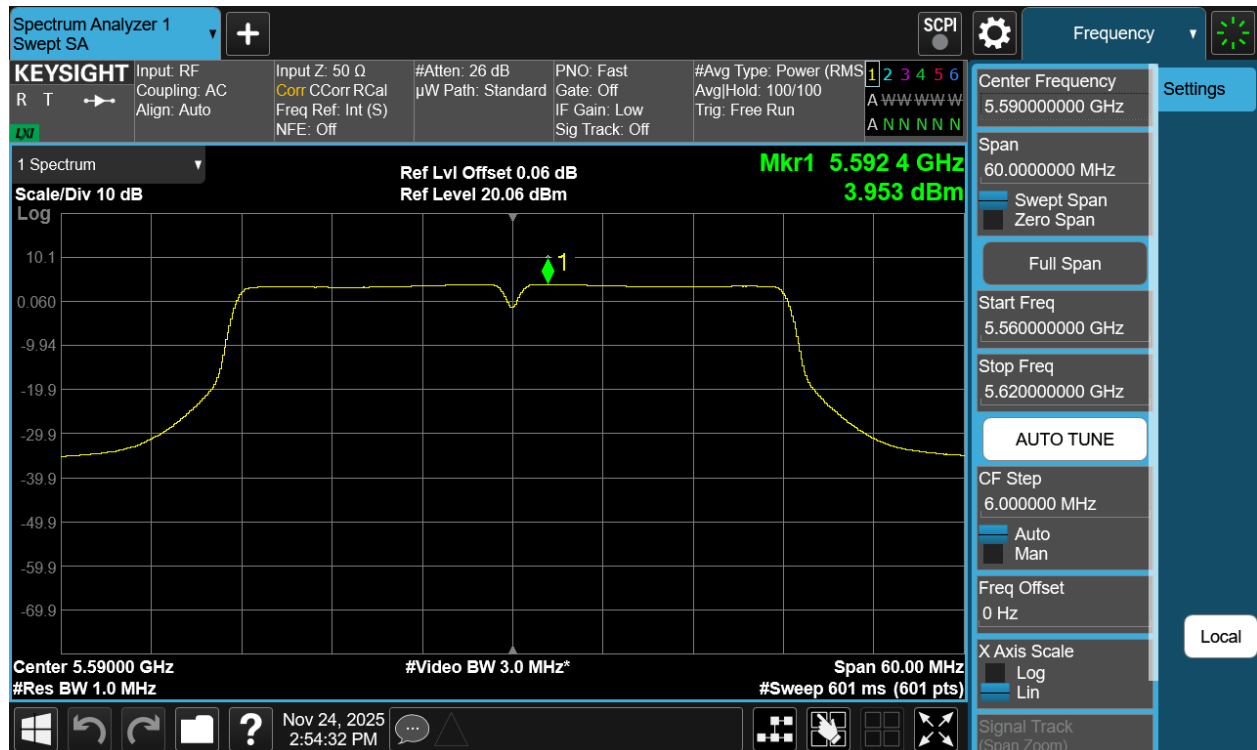
Plot 7-23 PSD Antenna WF7a (40MHz BW 802.11n - Ch.118)
