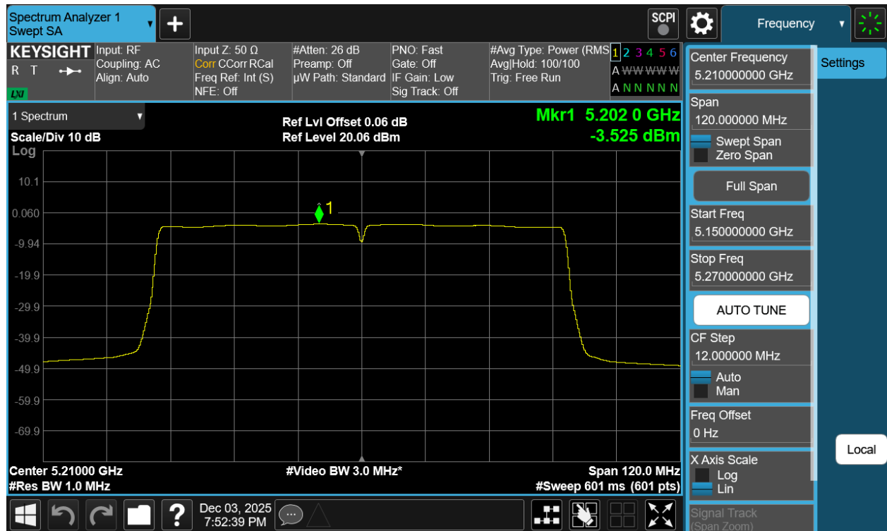
Plot 7-53 PSD Antenna WF7b (80MHz BW 802.11ac - Ch.42)
