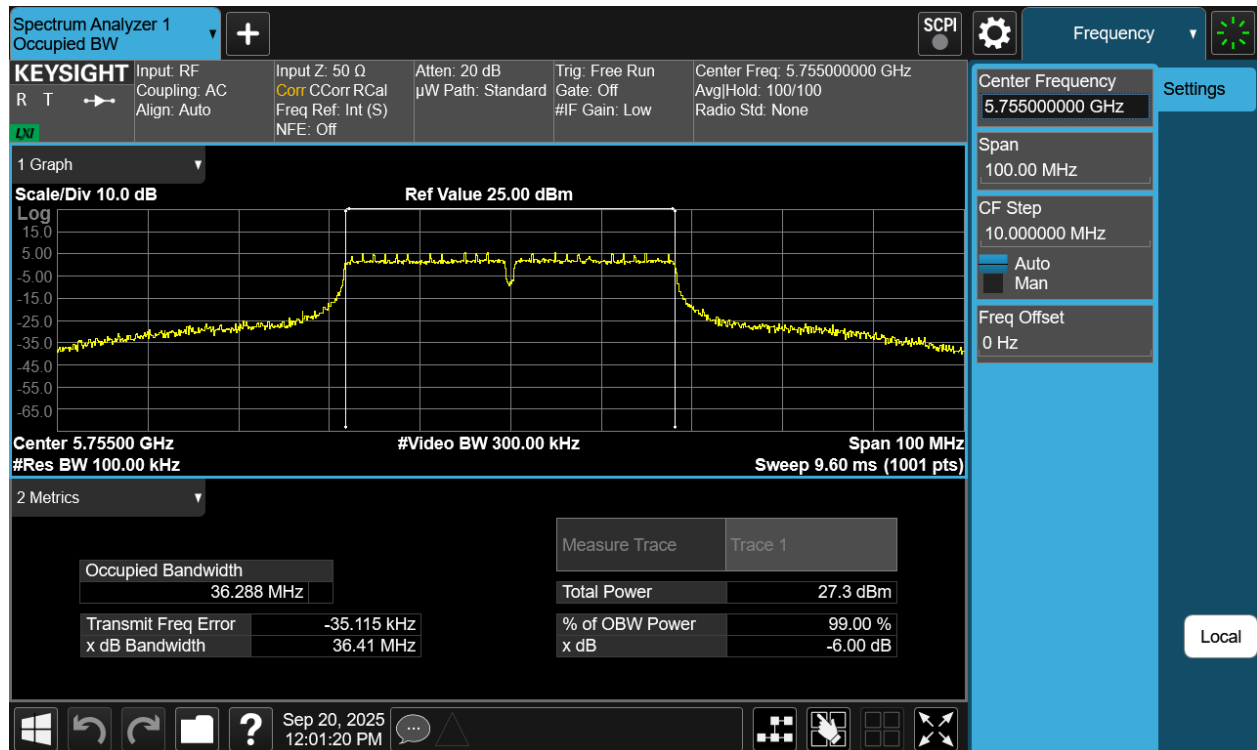
Plot 7-20 6dB OBW Antenna WF7b (40MHz BW 802.11n - Ch.151)
