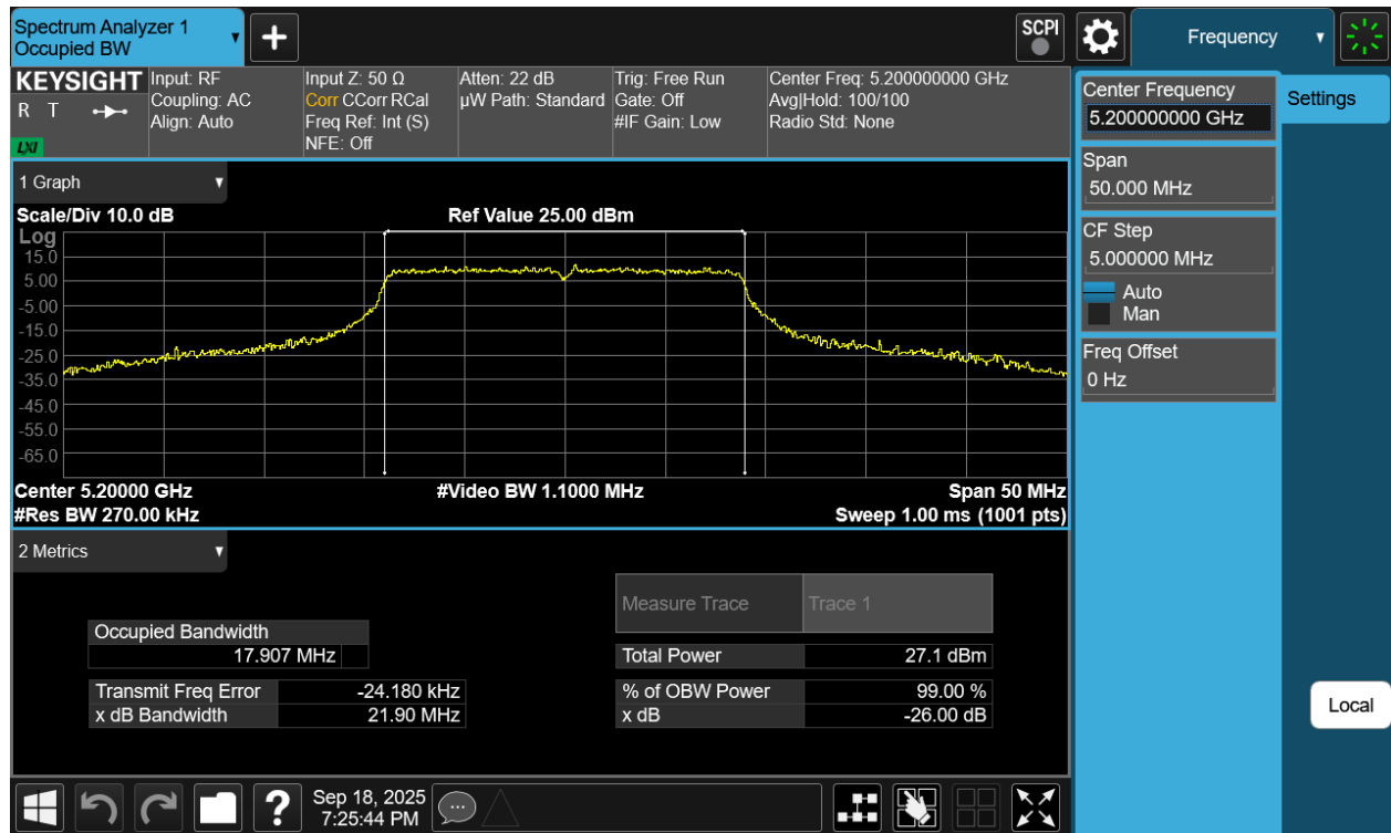
Plot 7-1 26dB BW & 99% OBW Antenna WF7a (20MHz BW 802.11n - Ch.40)
