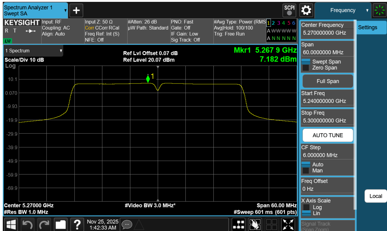
Plot 7-34 PSD Antenna WF2a (40MHz BW 802.11n - Ch.54)
