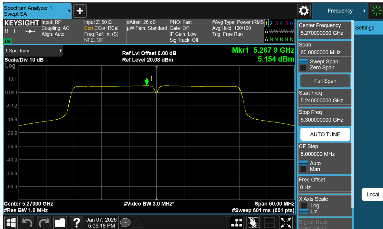
Plot 7-56 PSD CDD Primary Antenna WF7a (40MHz BW 802.11n - Ch.54)
