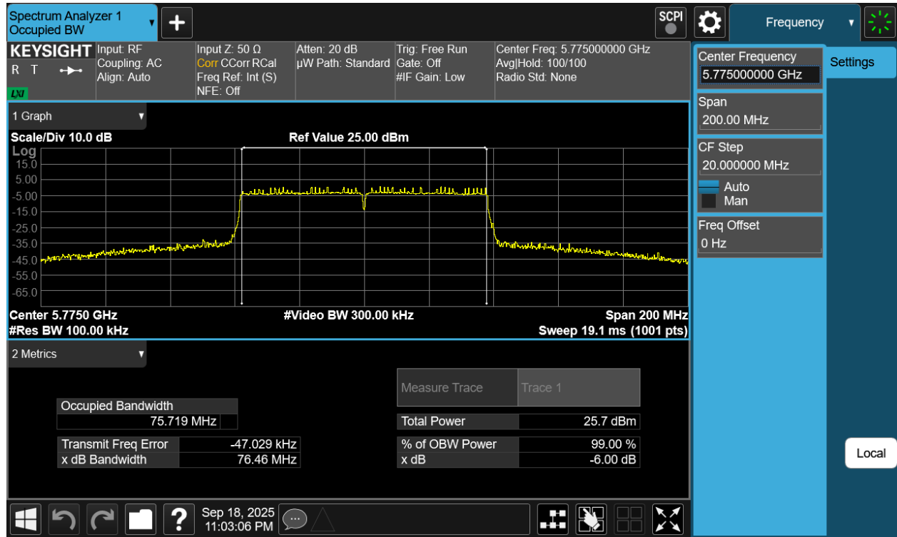
Plot 7-15 6dB OBW Antenna WF7a (80MHz BW 802.11ac - Ch.155)
