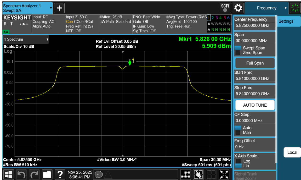
Plot 7-48 PSD Antenna WF7b (20MHz BW 802.11a - Ch.165)
