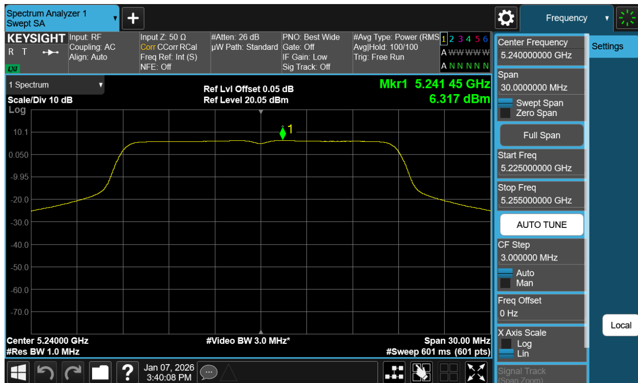
Plot 7-55 PSD CDD Primary Antenna WF7a (20MHz BW 802.11n - Ch.48)
