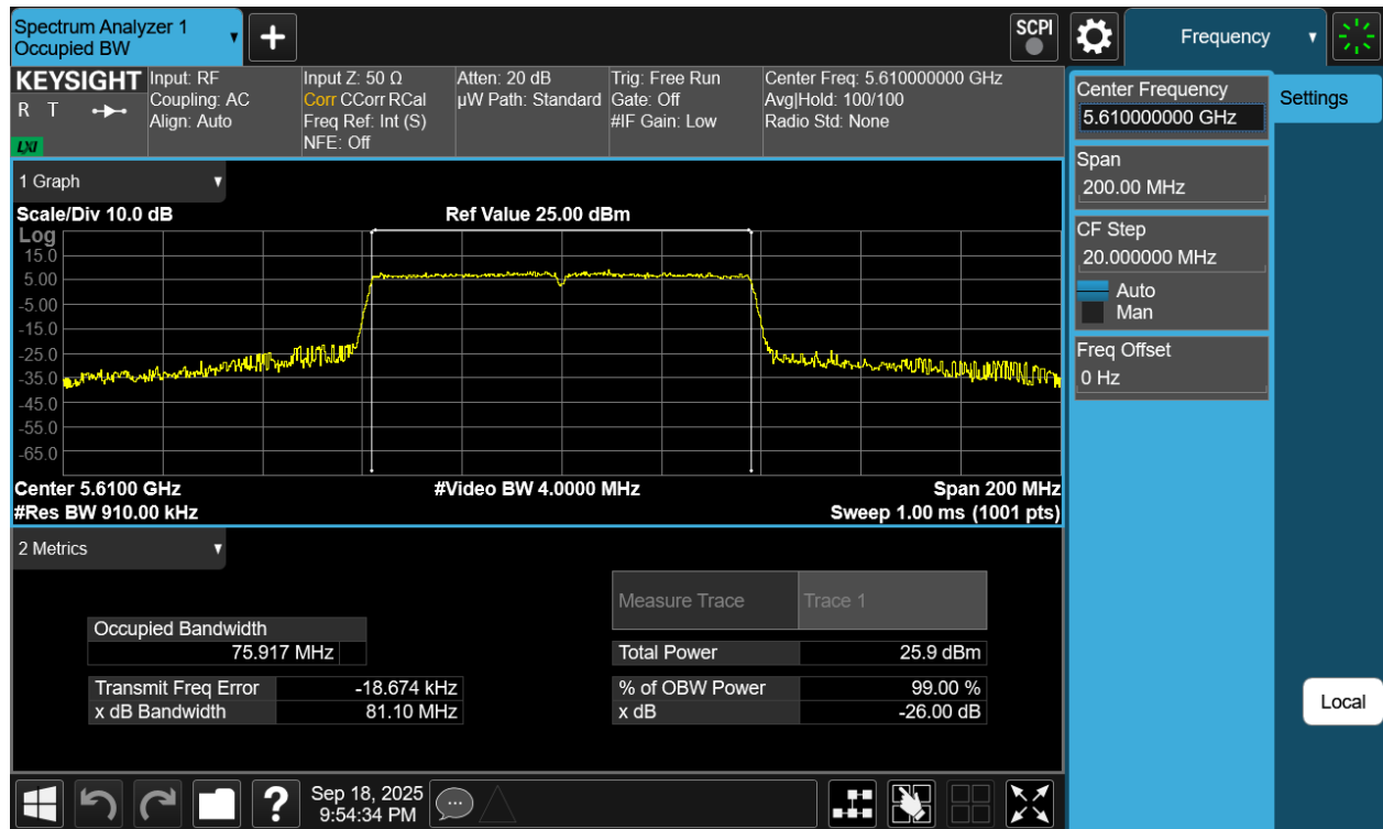
Plot 7-3 26dB BW & 99% OBW Antenna WF7a (80MHz BW 802.11ac - Ch.122)
