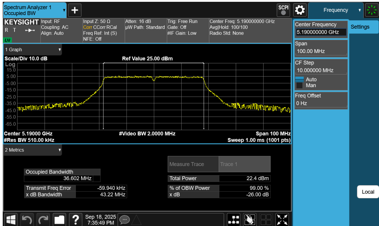
Plot 7-2 26dB BW & 99% OBW Antenna WF7a (40MHz BW 802.11n - Ch.38)
