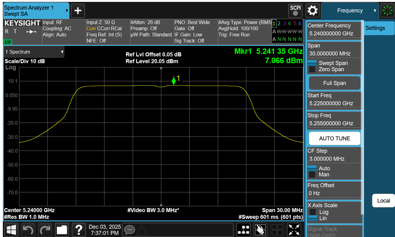
Plot 7-51 PSD Antenna WF7b (20MHz BW 802.11n - Ch.48)
