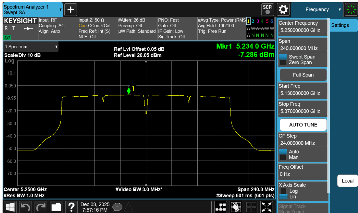
Plot 7-54 PSD Antenna WF7b (160MHz BW 802.11ac - Ch.50)
