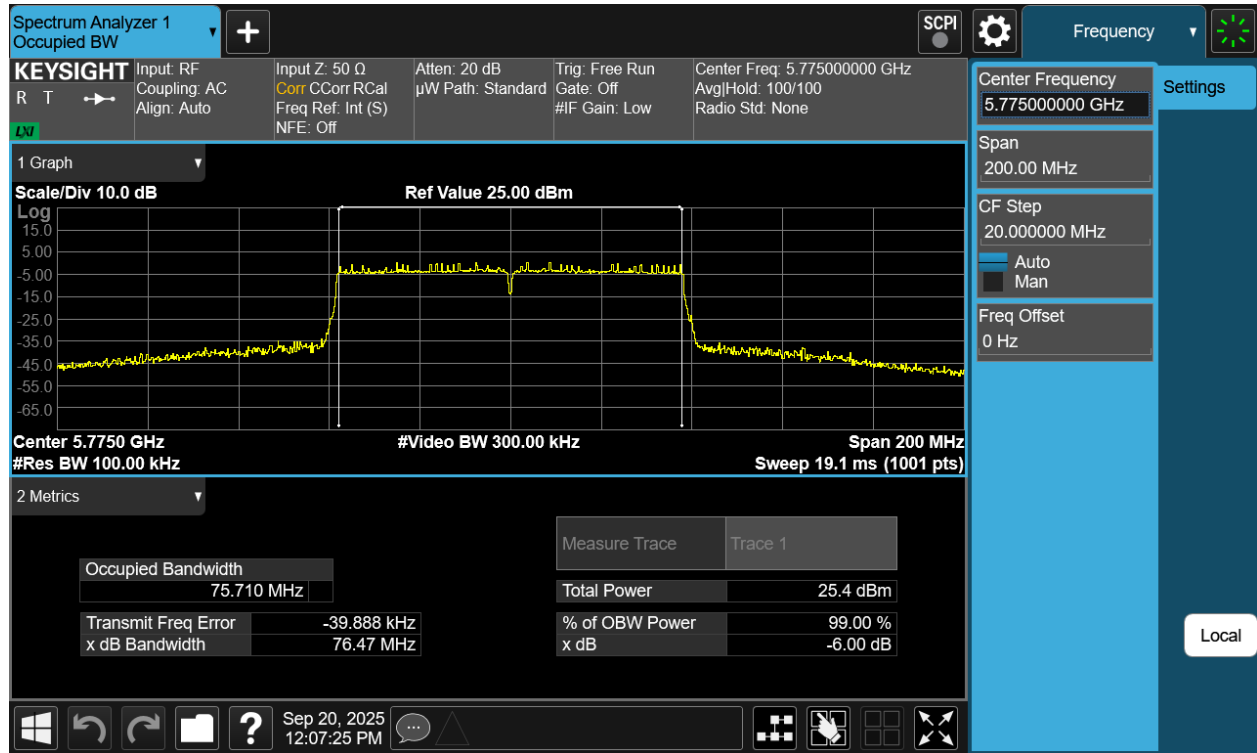
Plot 7-21 6dB OBW Antenna WF7b (80MHz BW 802.11ac - Ch.155)
