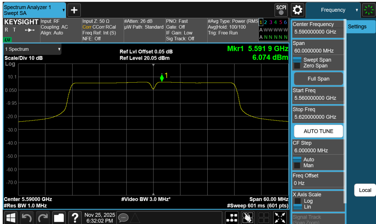
Plot 7-45 PSD Antenna WF7b (40MHz BW 802.11n - Ch.118)
