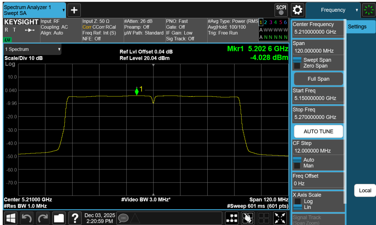
Plot 7-31 PSD Antenna WF7a (80MHz BW 802.11ac - Ch.42)
