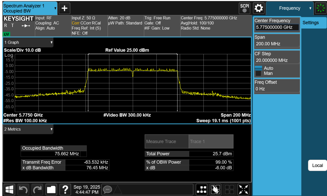
Plot 7-18 6dB OBW Antenna WF2a (80MHz BW 802.11ac - Ch.155)
