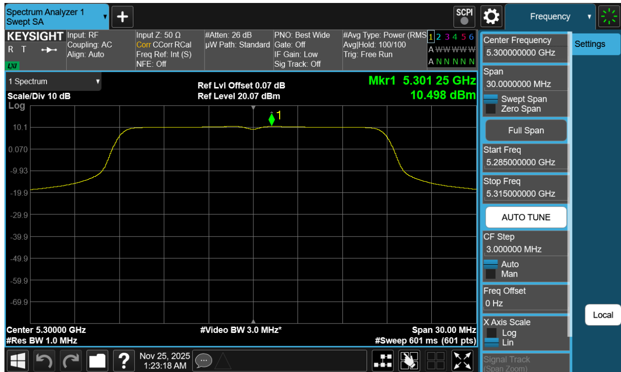
Plot 7-33 PSD Antenna WF2a (20MHz BW 802.11a - Ch.60)
