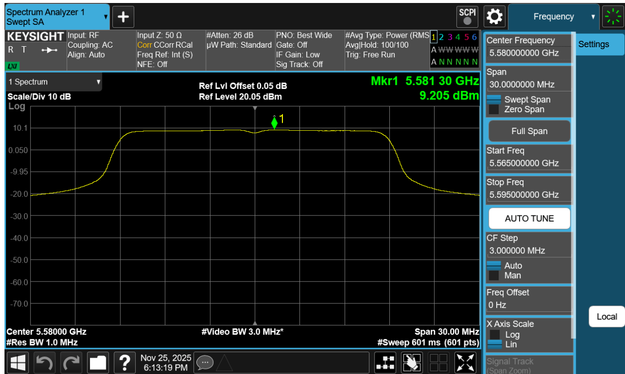
Plot 7-44 PSD Antenna WF7b (20MHz BW 802.11n - Ch.116)
