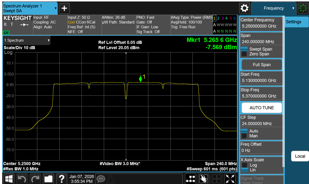
Plot 7-58 PSD CDD Primary Antenna WF7a (160MHz BW 802.11ac - Ch.50)
