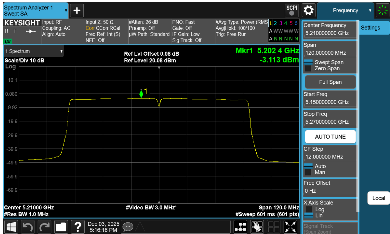
Plot 7-42 PSD Antenna WF2a (80MHz BW 802.11ac - Ch.42)
