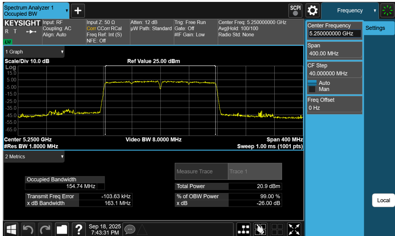
Plot 7-4 26dB BW & 99% OBW Antenna WF7a (160MHz BW 802.11ac - Ch.50)
