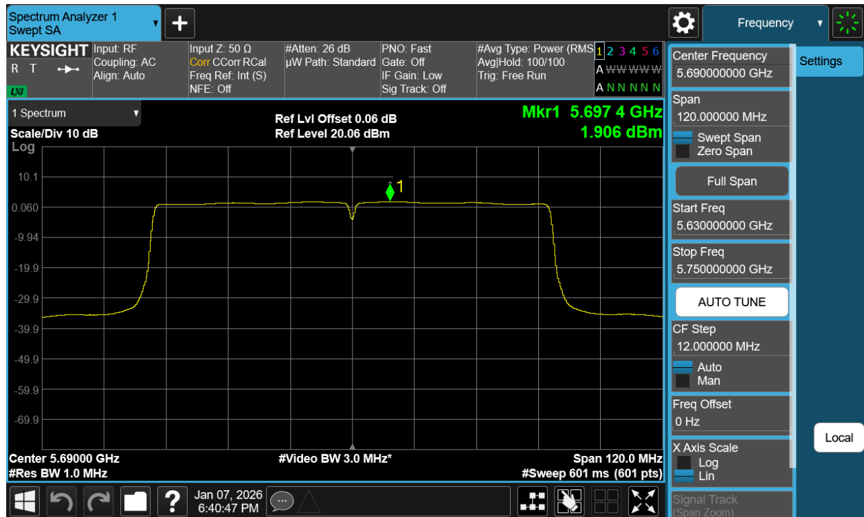
Plot 7-57 PSD CDD Primary Antenna WF7a (80MHz BW 802.11ac - Ch.138)
