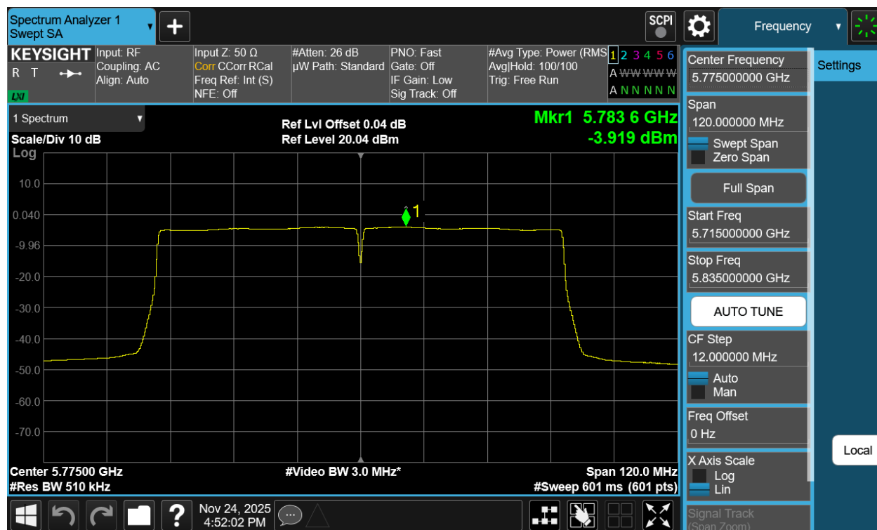
Plot 7-28 PSD Antenna WF7a (80MHz BW 802.11ac - Ch.155)
