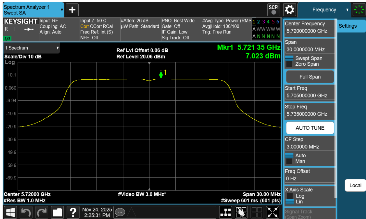
Plot 7-22 PSD Antenna WF7a (20MHz BW 802.11a - Ch.144)
