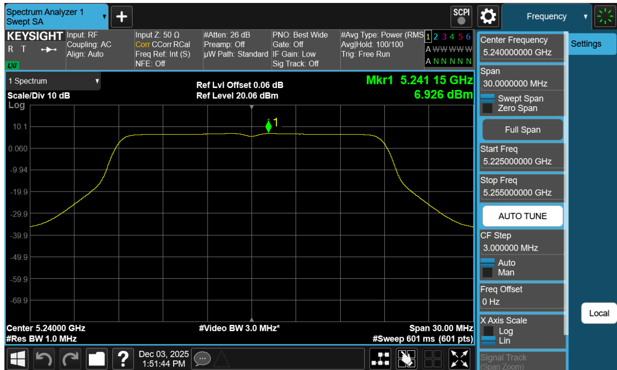
Plot 7-29 PSD Antenna WF7a (20MHz BW 802.11a - Ch.48)
