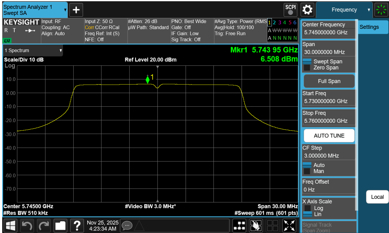
Plot 7-37 PSD Antenna WF2a (20MHz BW 802.11a - Ch.149)
