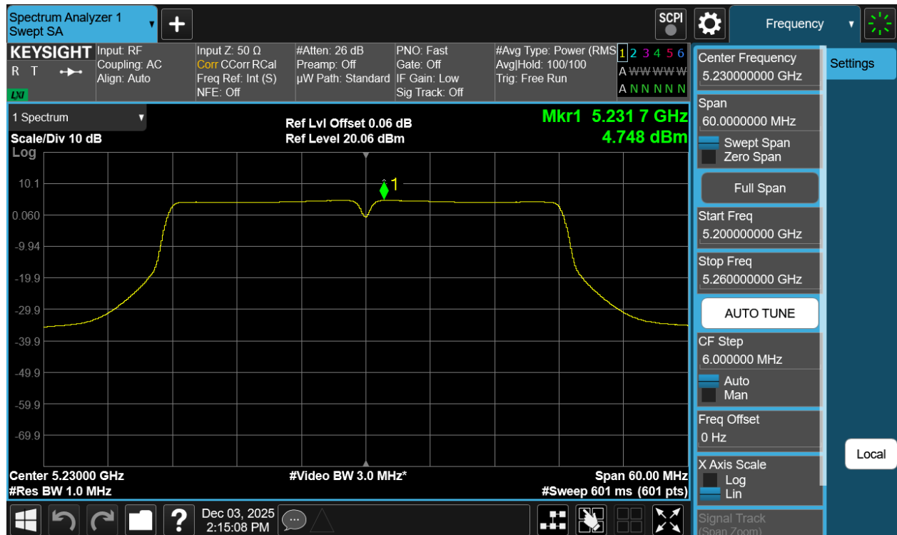
Plot 7-30 PSD Antenna WF7a (40MHz BW 802.11n - Ch.46)
