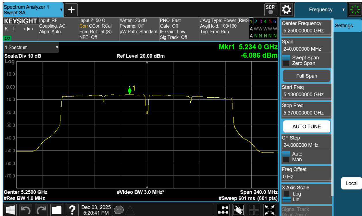
Plot 7-43 PSD Antenna WF2a (160MHz BW 802.11ac - Ch.50)
