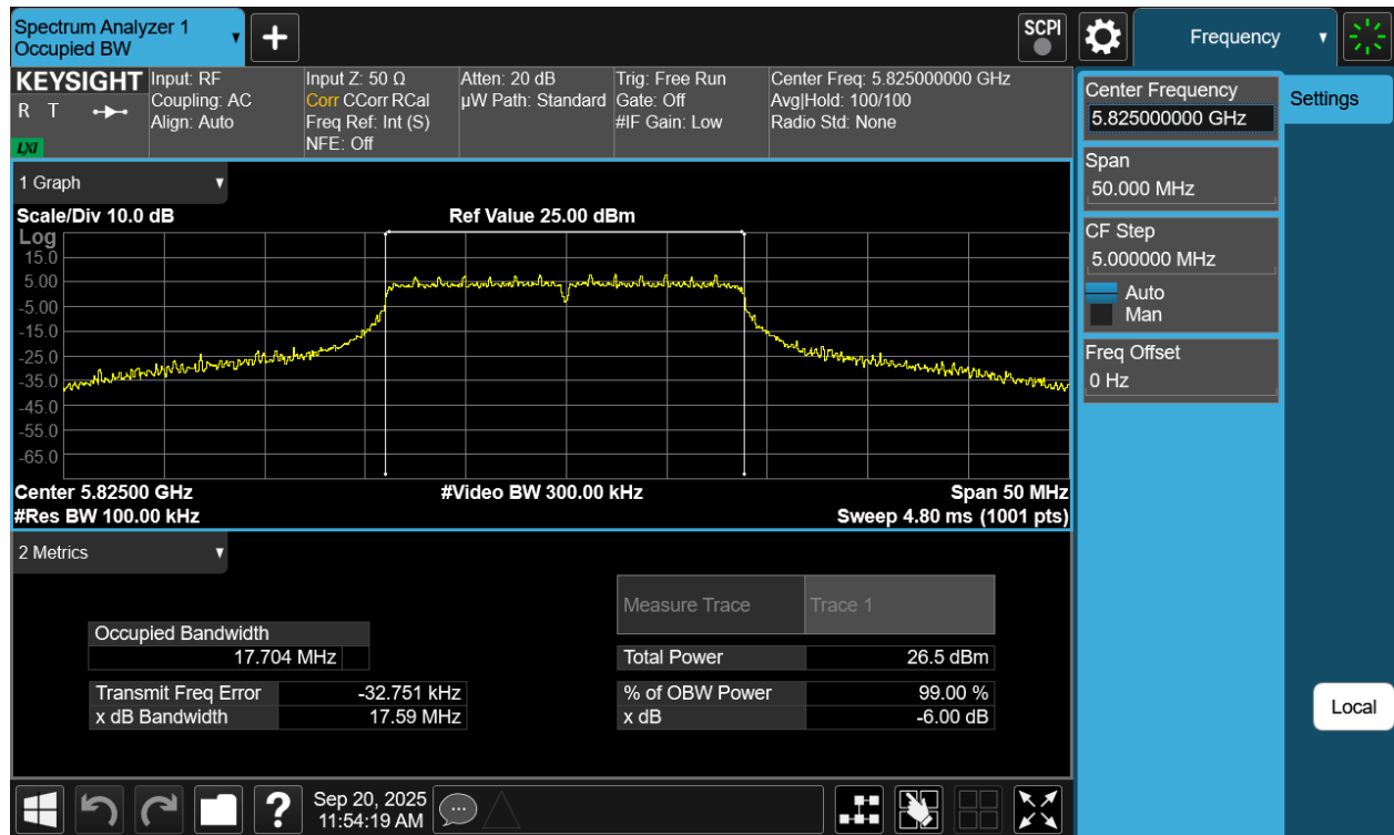
Plot 7-19 6dB OBW Antenna WF7b (20MHz BW 802.11n - Ch.165)
