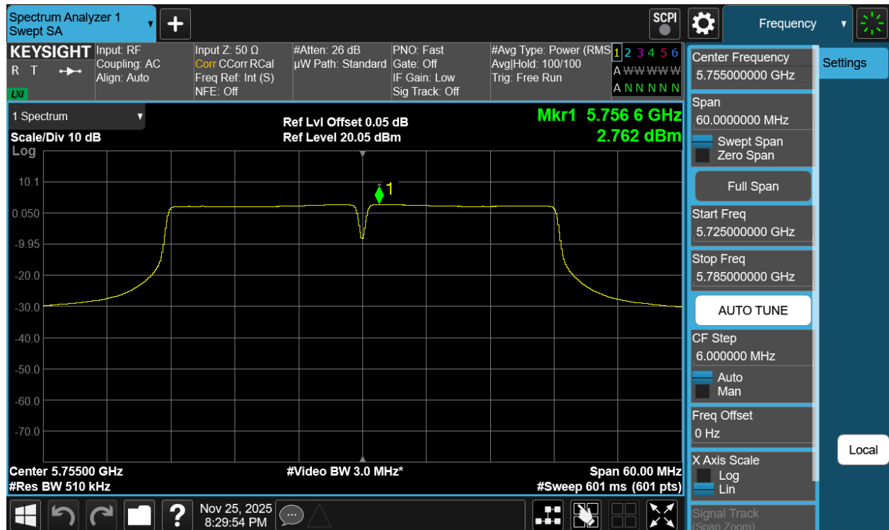
Plot 7-49 PSD Antenna WF7b (40MHz BW 802.11n - Ch.151)
