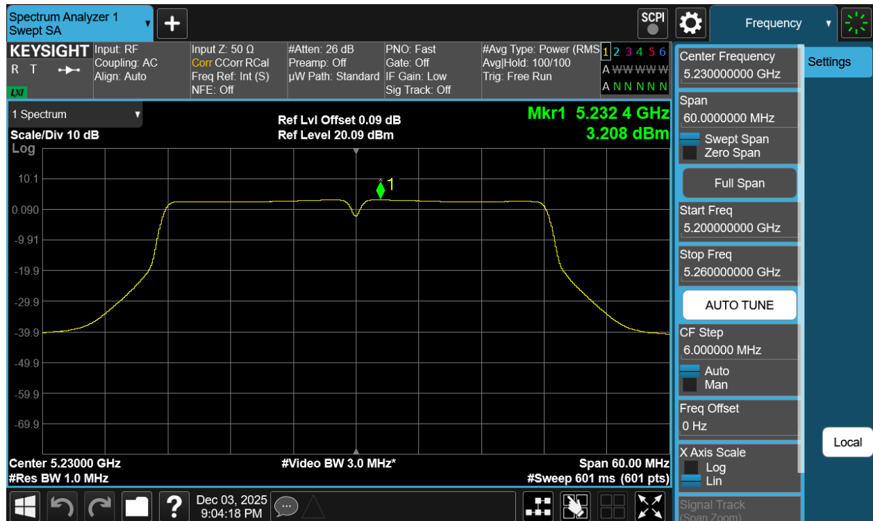
Plot 7-96 PSD CDD Diversity Antenna WF7b (40MHz BW 802.11n - Ch.46)
