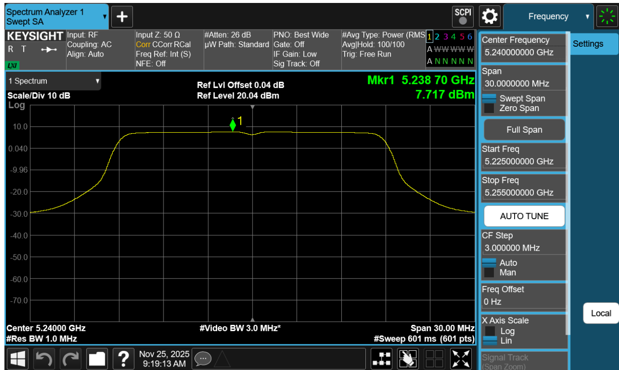
Plot 7-77 PSD CDD Diversity Antenna WF2a (20MHz BW 802.11n - Ch.48)
