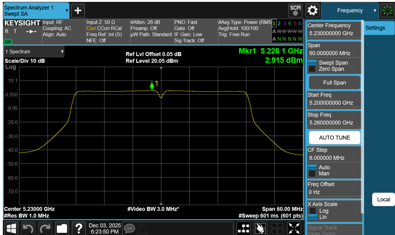
Plot 7-92 PSD CDD Diversity Antenna WF2a (40MHz BW 802.11n - Ch.46)
