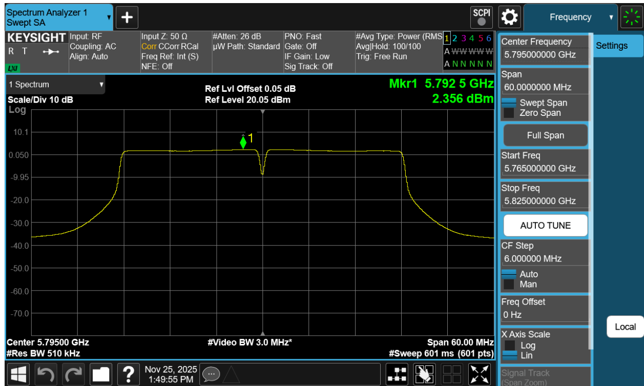
Plot 7-67 PSD CDD Primary Antenna WF2a (40MHz BW 802.11n - Ch.159)
