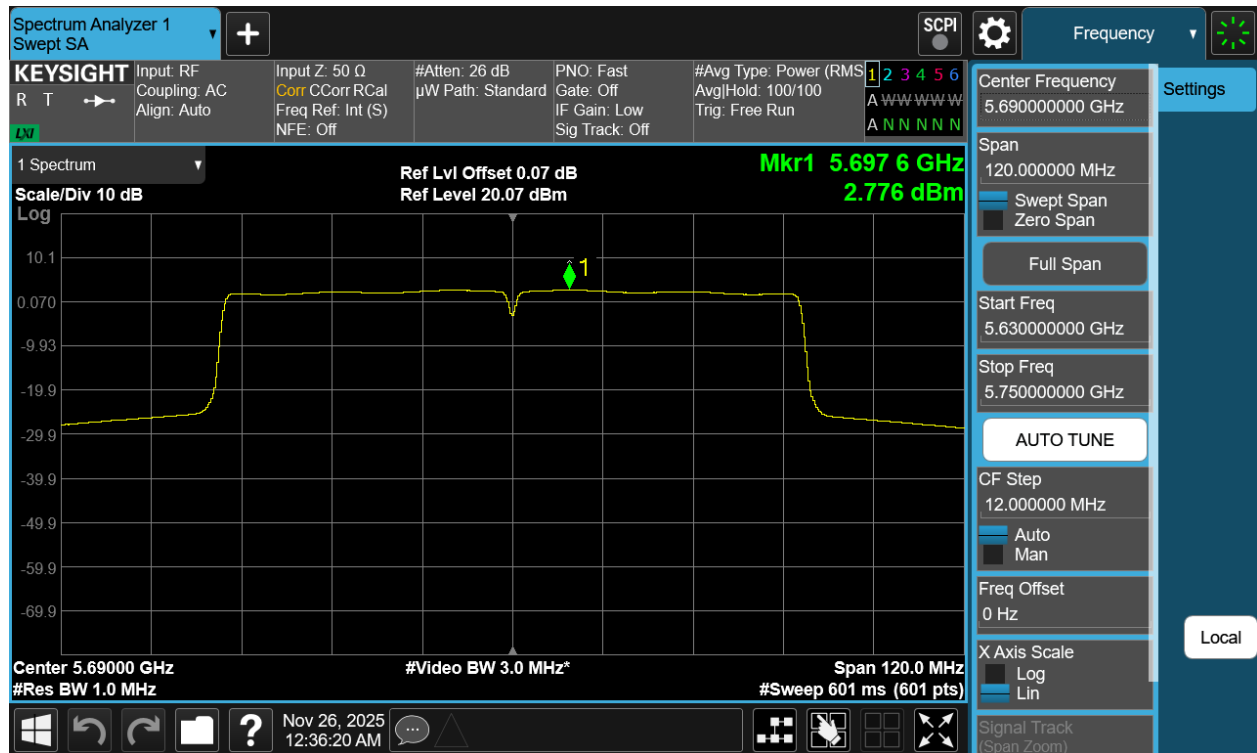
Plot 7-83 PSD CDD Diversity Antenna WF7b (80MHz BW 802.11ac - Ch.138)
