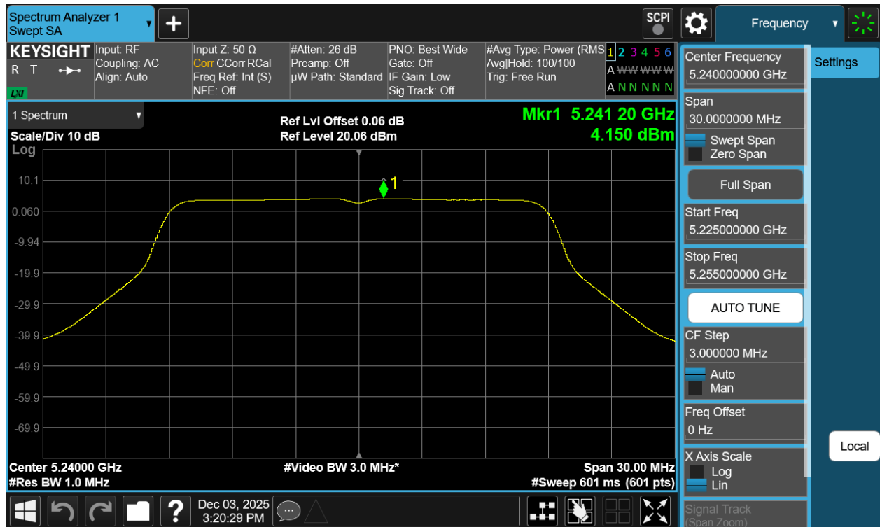
Plot 7-69 PSD CDD Primary Antenna WF7a (20MHz BW 802.11n - Ch.48)
