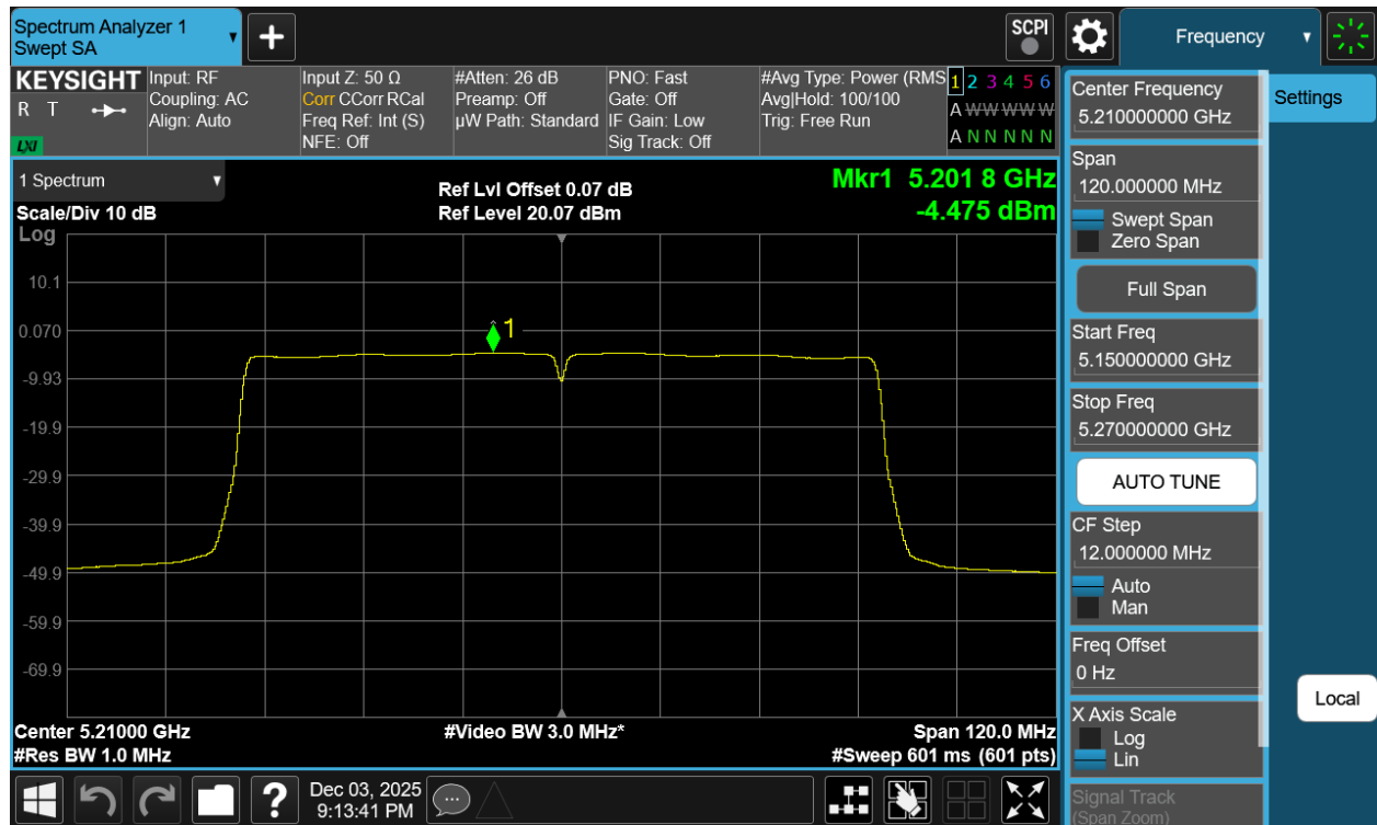
Plot 7-97 PSD CDD Diversity Antenna WF7b (80MHz BW 802.11ac - Ch.42)
