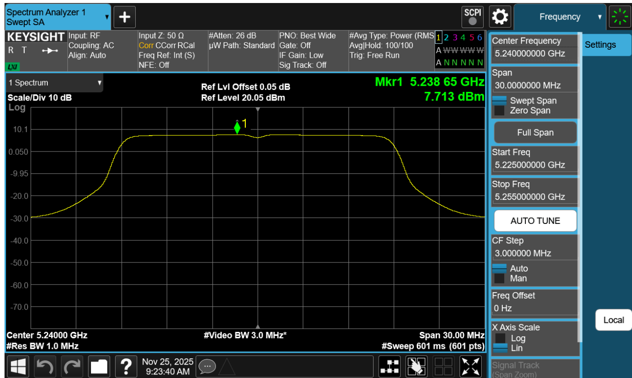
Plot 7-59 PSD CDD Primary Antenna WF2a (20MHz BW 802.11n - Ch.48)
