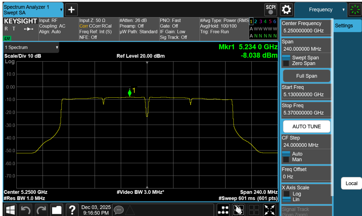
Plot 7-98 PSD CDD Diversity Antenna WF7b (160MHz BW 802.11ac - Ch.50)
