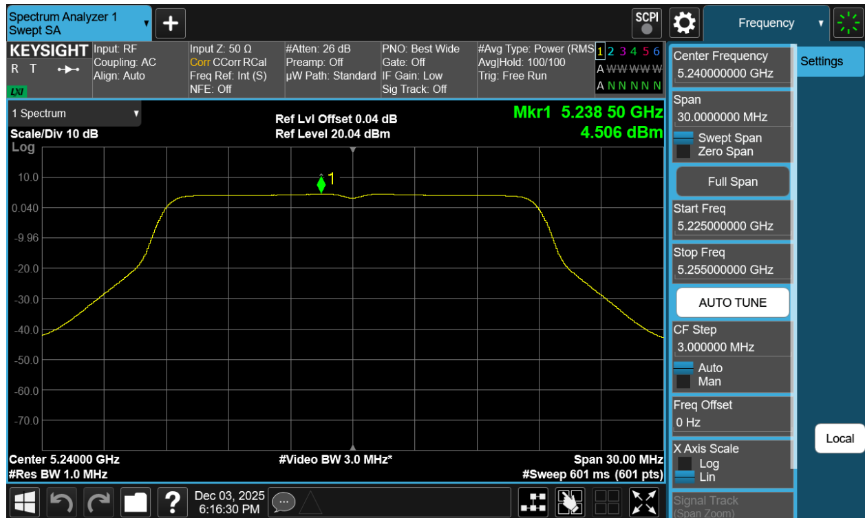
Plot 7-73 PSD CDD Primary Antenna WF2a (20MHz BW 802.11n - Ch.48)
