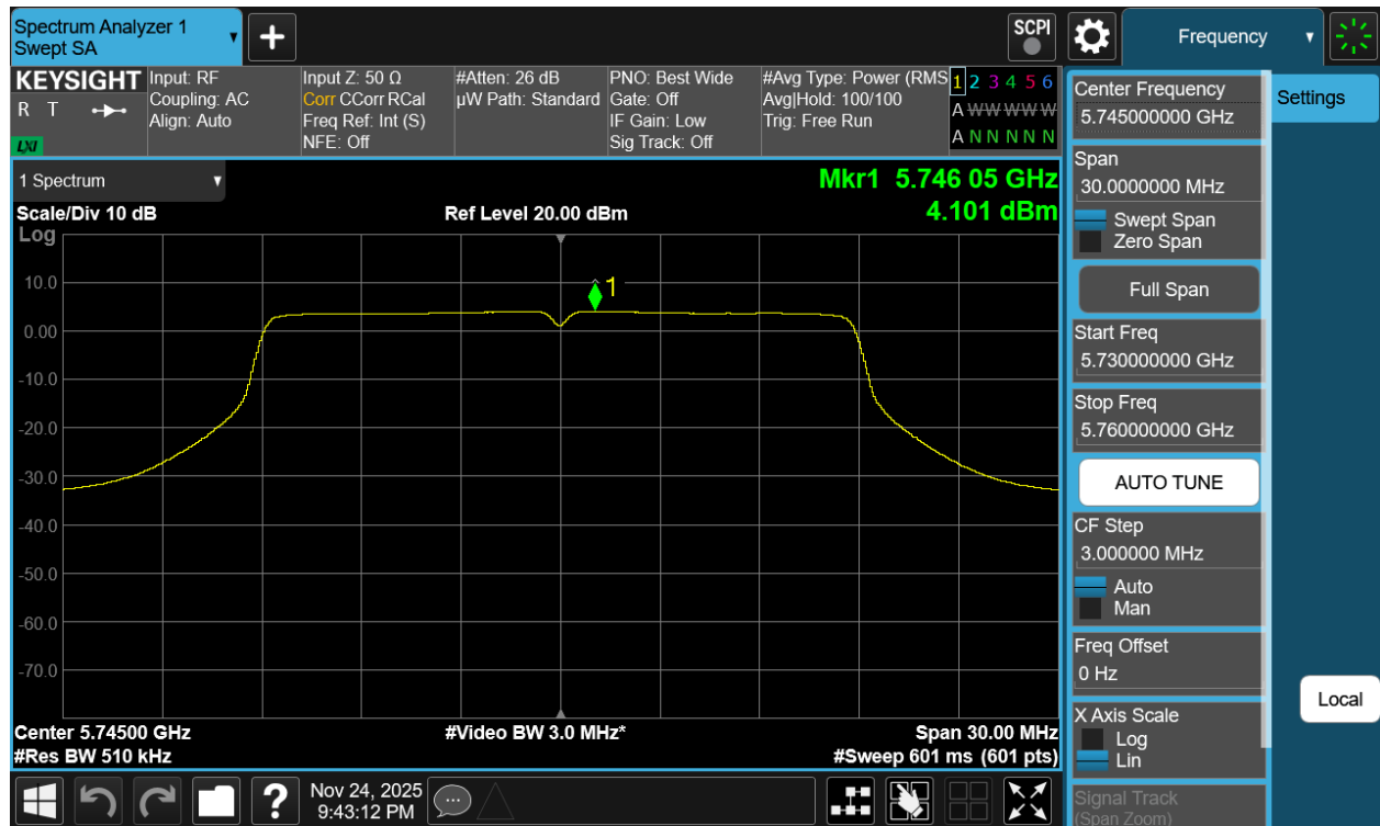
Plot 7-63 PSD CDD Primary Antenna WF7a (20MHz BW 802.11a - Ch.149)
