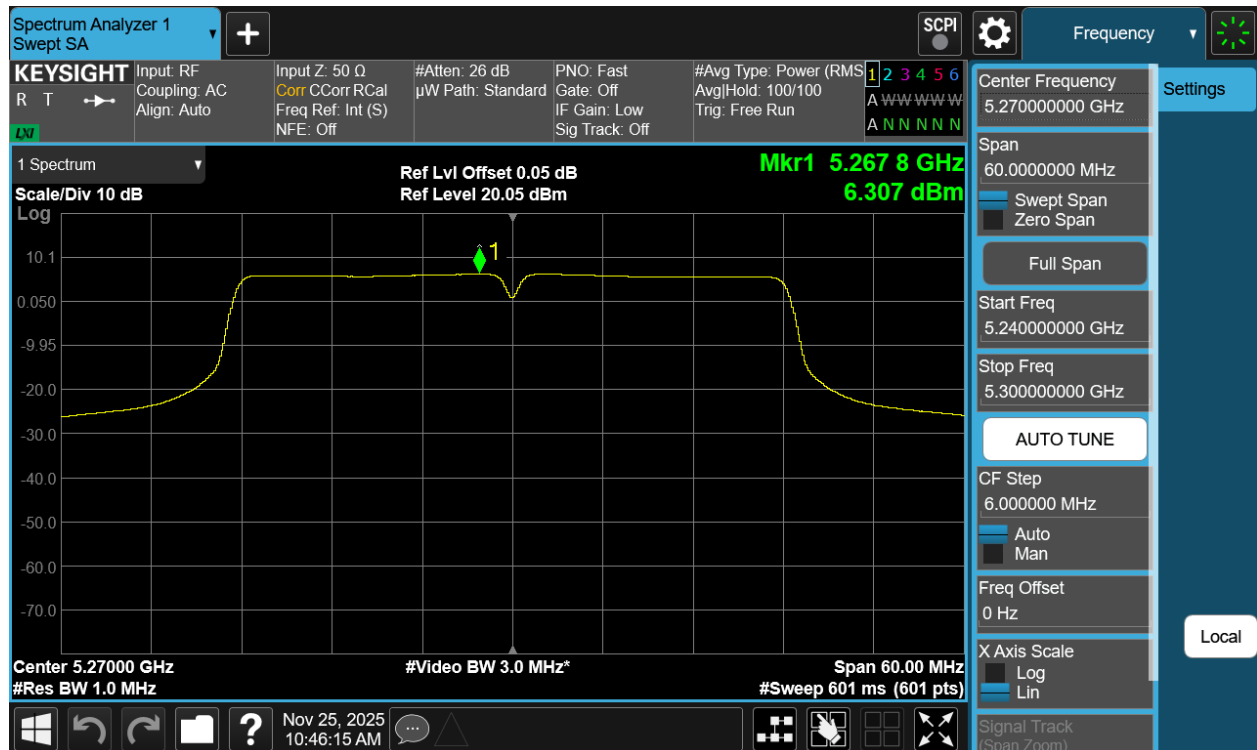
Plot 7-60 PSD CDD Primary Antenna WF2a (40MHz BW 802.11n - Ch.54)
