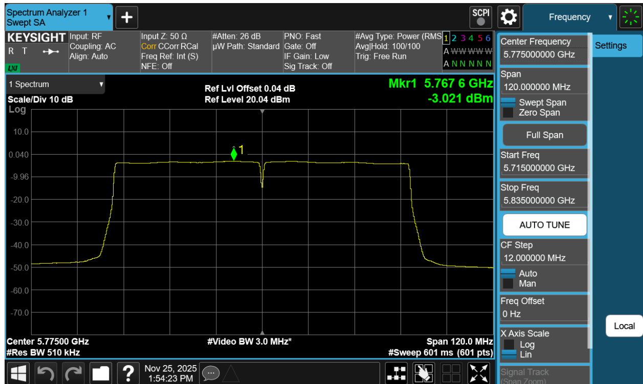
Plot 7-68 PSD CDD Primary Antenna WF2a (80MHz BW 802.11ac - Ch.155)
