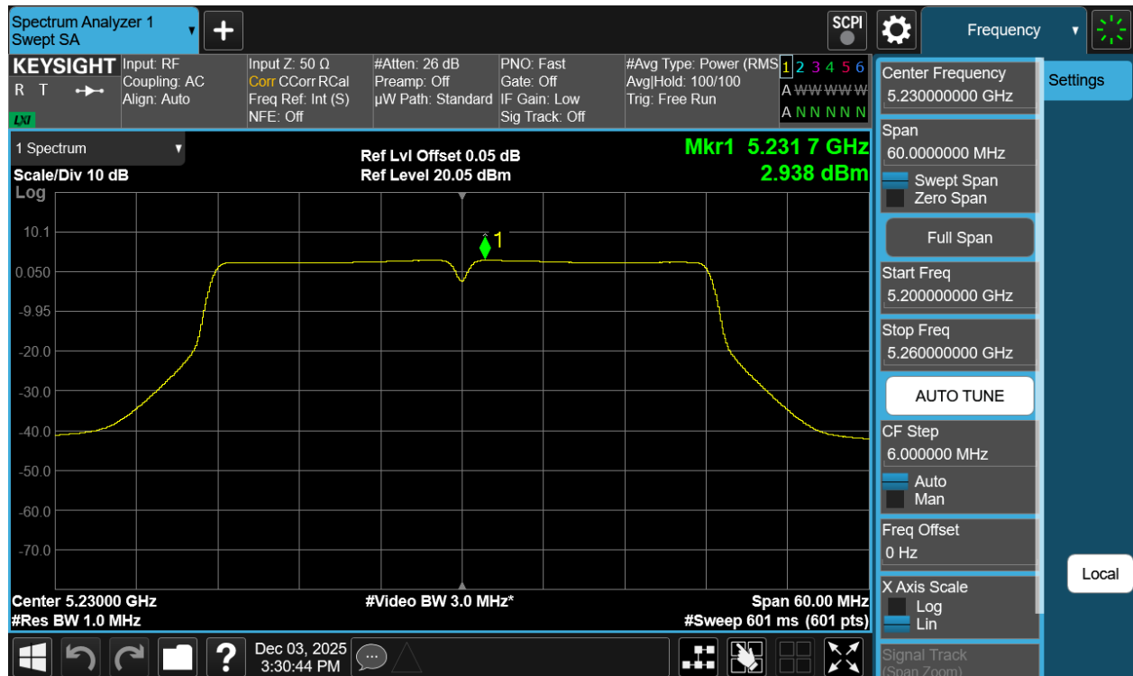
Plot 7-70 PSD CDD Primary Antenna WF7a (40MHz BW 802.11n - Ch.46)
