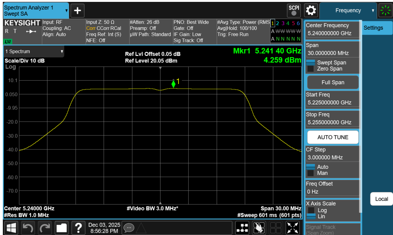
Plot 7-95 PSD CDD Diversity Antenna WF7b (20MHz BW 802.11n - Ch.48)
