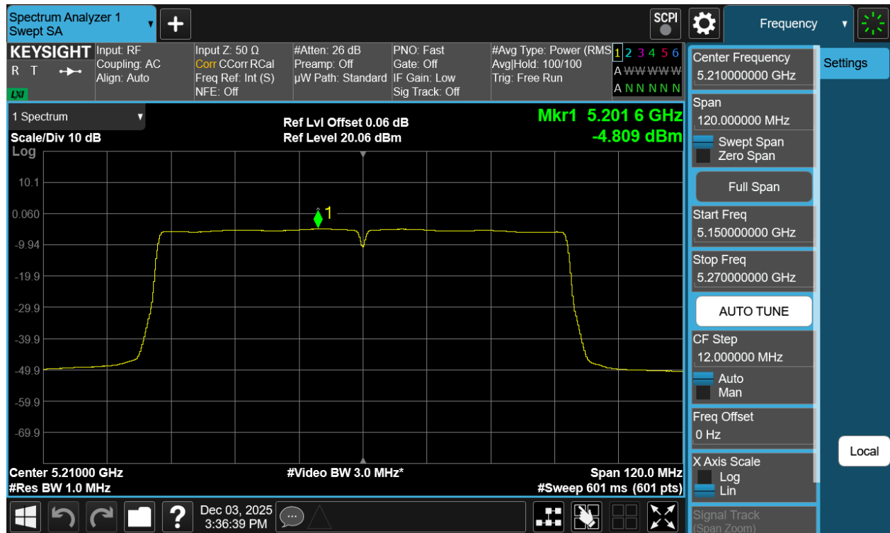
Plot 7-71 PSD CDD Primary Antenna WF7a (80MHz BW 802.11ac - Ch.42)
