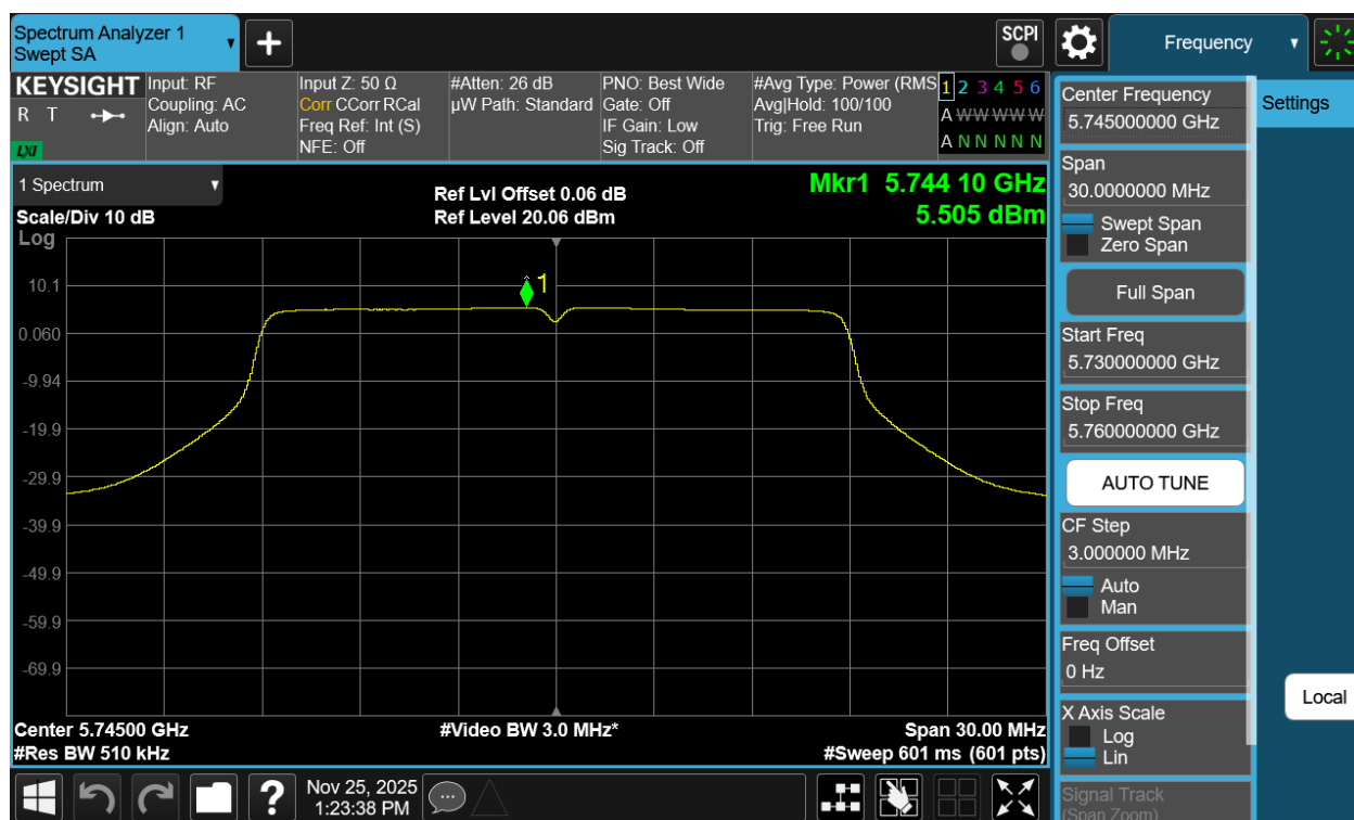
Plot 7-66 PSD CDD Primary Antenna WF2a (20MHz BW 802.11a - Ch.149)
