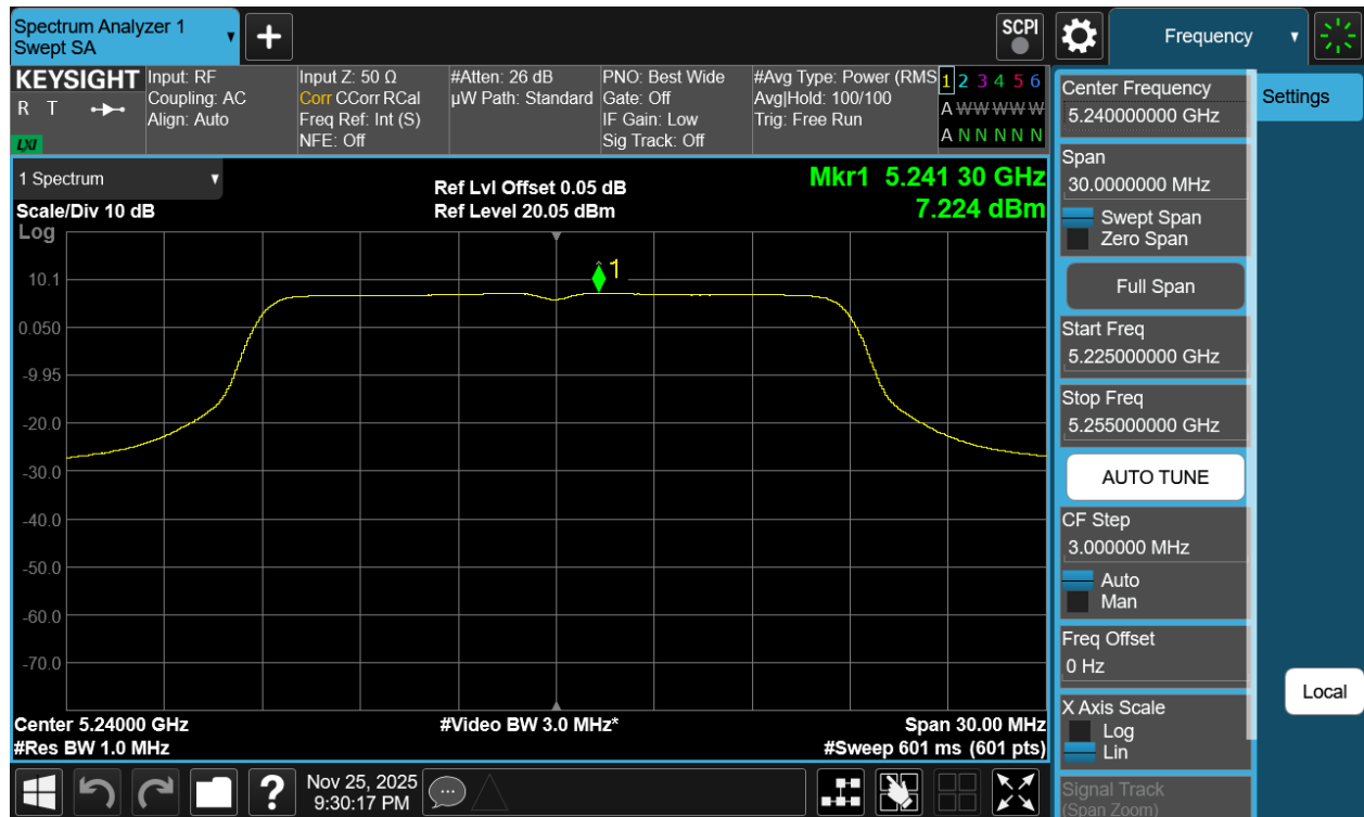
Plot 7-81 PSD CDD Diversity Antenna WF7b (20MHz BW 802.11n - Ch.48)
