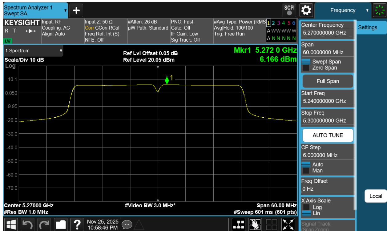
Plot 7-82 PSD CDD Diversity Antenna WF7b (40MHz BW 802.11n - Ch.54)
