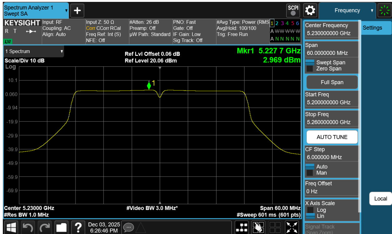
Plot 7-74 PSD CDD Primary Antenna WF2a (40MHz BW 802.11n - Ch.46)
