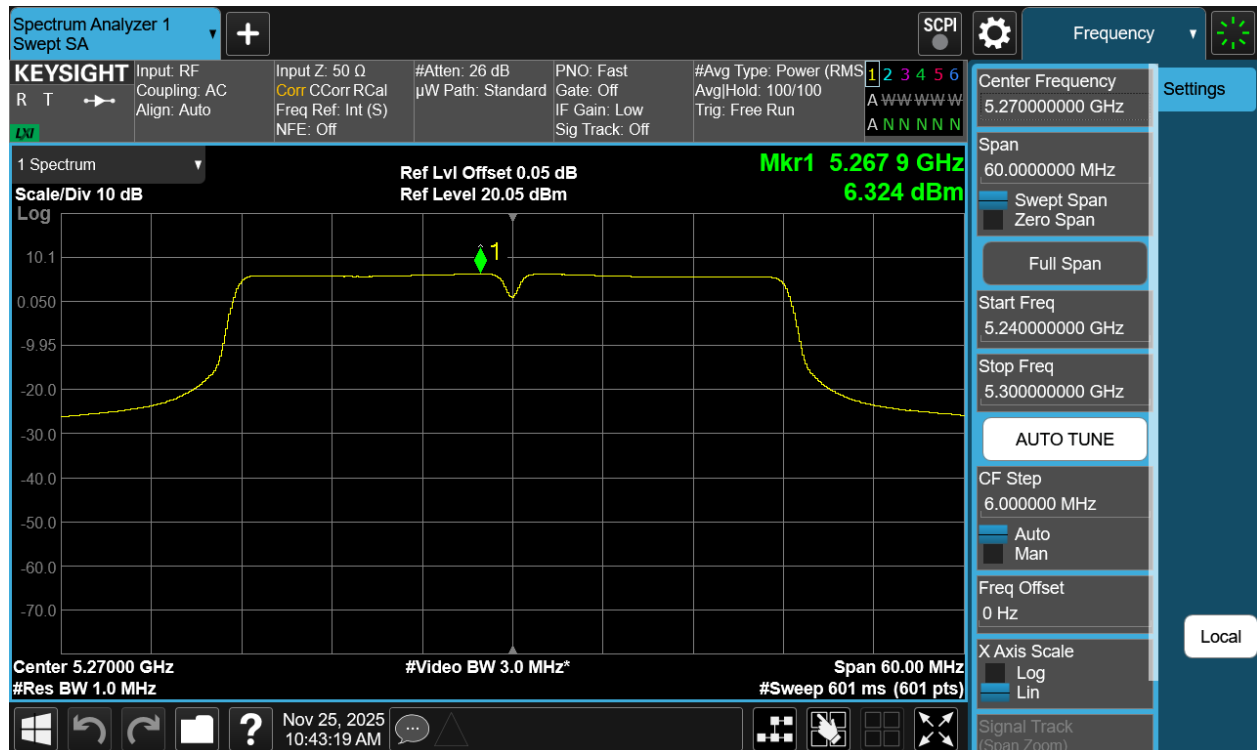
Plot 7-78 PSD CDD Diversity Antenna WF2a (40MHz BW 802.11n - Ch.54)
