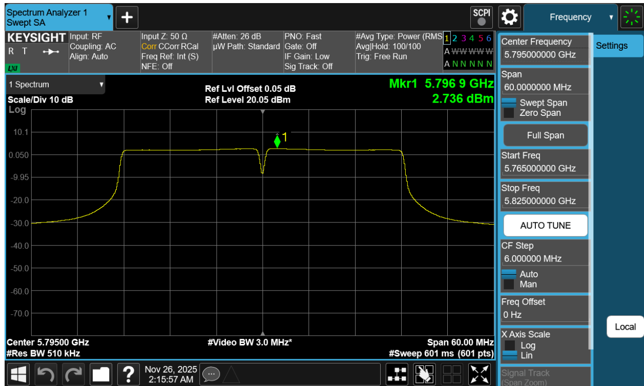
Plot 7-89 PSD CDD Diversity Antenna WF7b (40MHz BW 802.11n - Ch.159)
