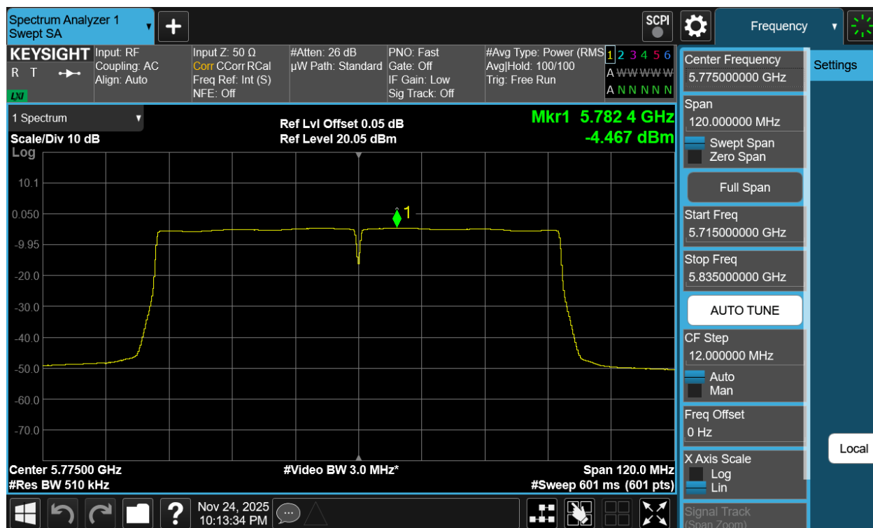
Plot 7-65 PSD CDD Primary Antenna WF7a (80MHz BW 802.11ac - Ch.155)
