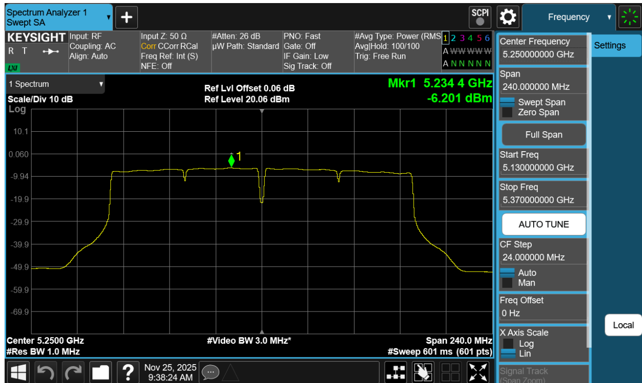
Plot 7-62 PSD CDD Primary Antenna WF2a (160MHz BW 802.11ac - Ch.50)
