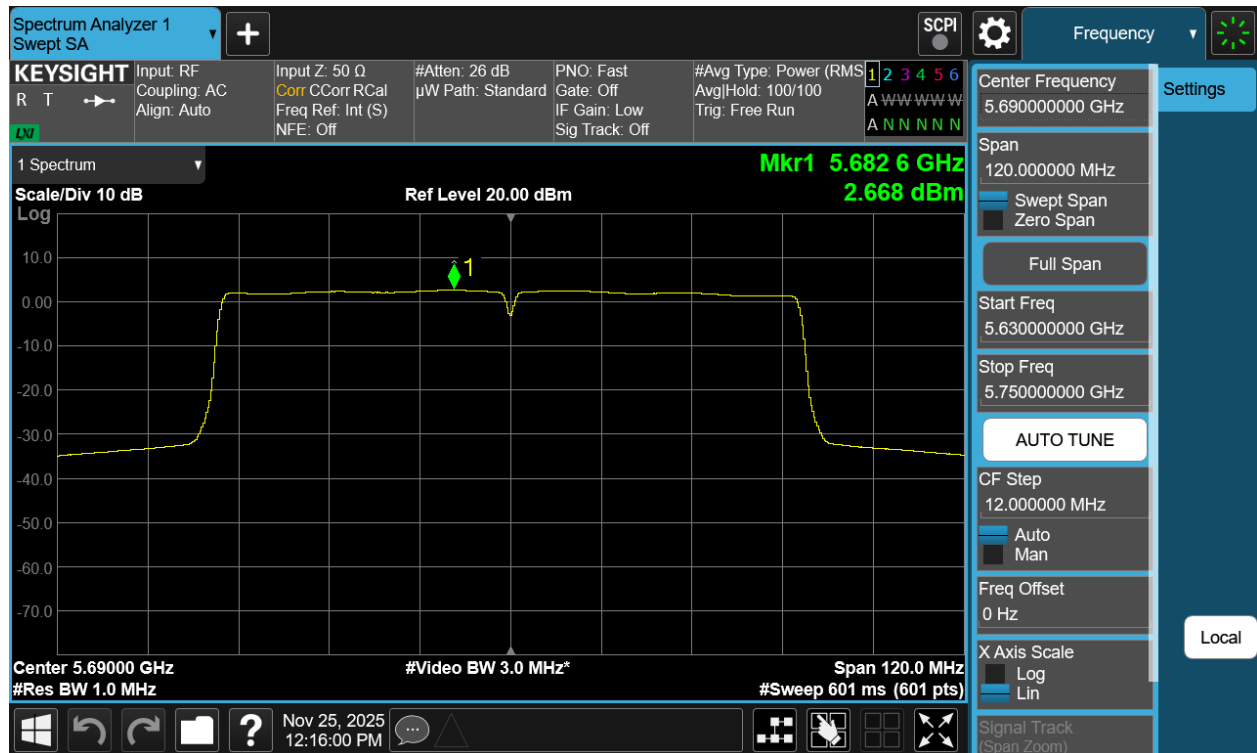
Plot 7-61 PSD CDD Primary Antenna WF2a (80MHz BW 802.11ac - Ch.138)
