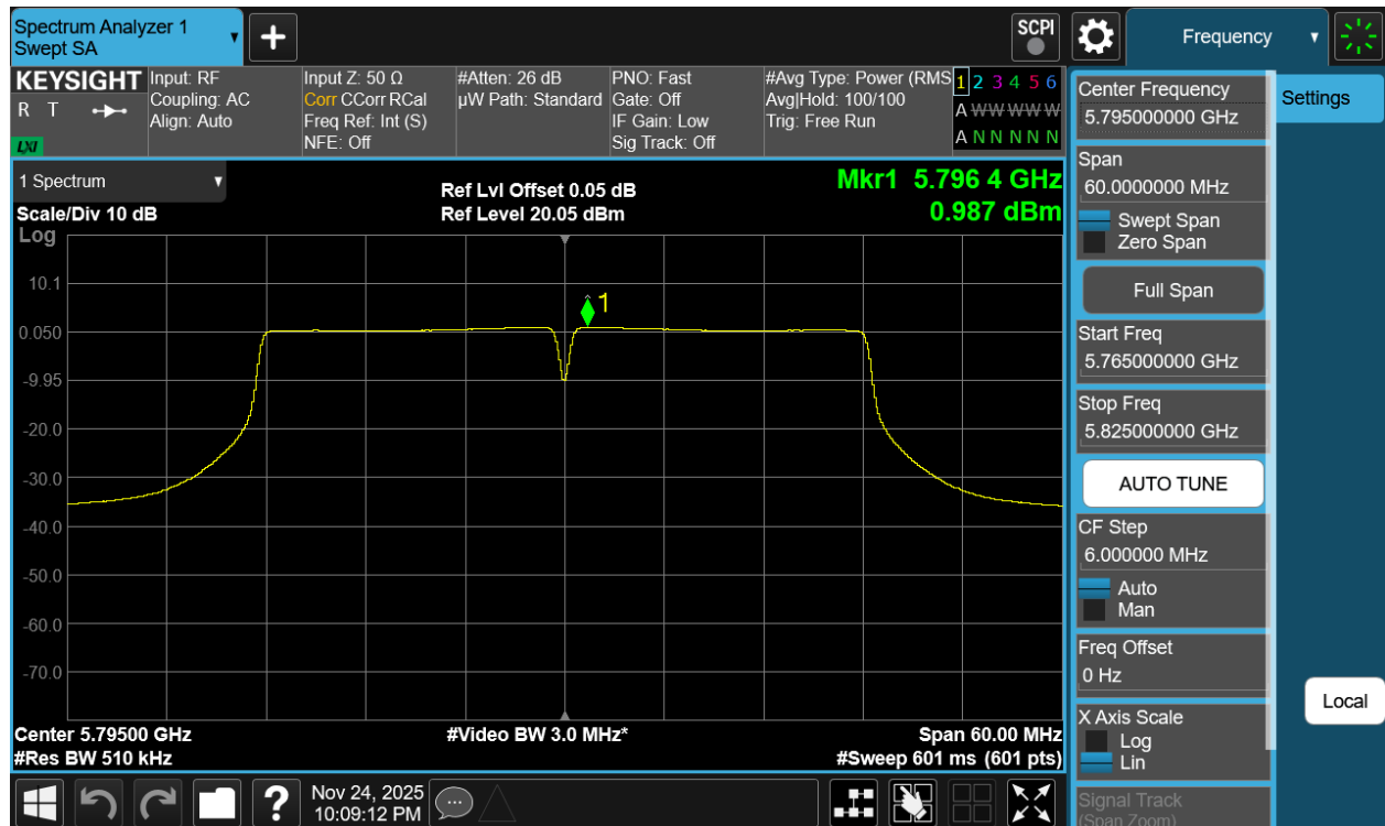
Plot 7-64 PSD CDD Primary Antenna WF7a (40MHz BW 802.11n - Ch.159)
