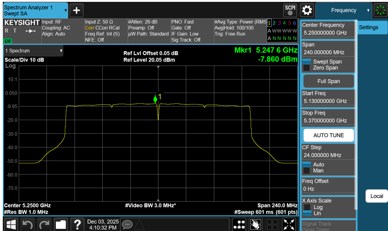
Plot 7-72 PSD CDD Primary Antenna WF7a (160MHz BW 802.11be(SU) - Ch.50)
