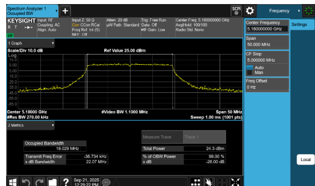
Plot 7-8 26dB BW & 99% OBW Antenna WF7a (20MHz BW 802.11be(RU) RU242 Index61 - Ch.36)
