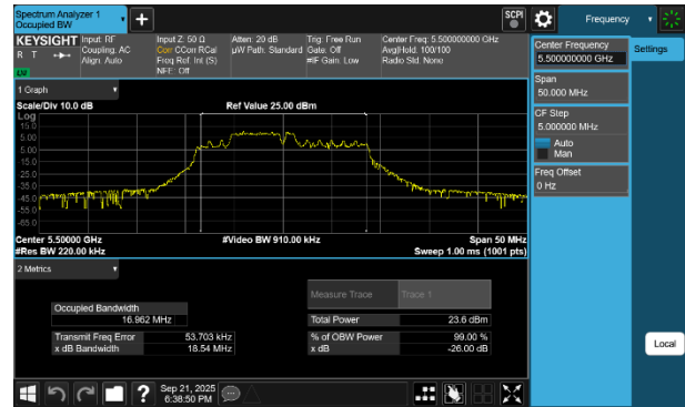
Plot 7-5 26dB BW & 99% OBW Antenna WF7a (20MHz BW 802.11be(RU) RU52+26 Index71 - Ch.100)
