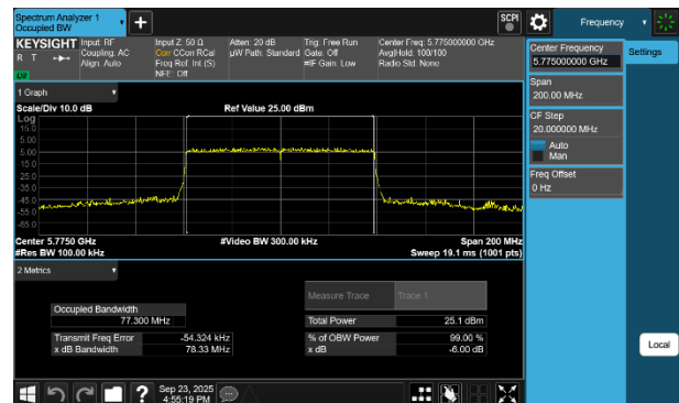
Plot 7-57 6dB OBW Antenna WF7b (80MHz BW 802.11be(RU) RU996 Index67 - Ch.155)
