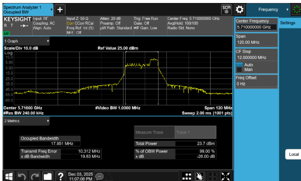
Plot 7-2 26dB BW & 99% OBW Antenna WF7a (40MHz BW 802.11be(RU) RU52 Index44 - Ch.142)
