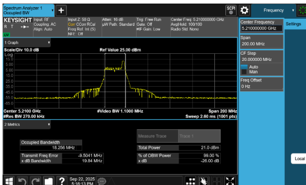
Plot 7-14 26dB BW & 99% OBW Antenna WF2a (80MHz BW 802.11be(RU) RU26 Index17 - Ch.42)
