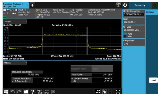
Plot 7-49 6dB OBW Antenna WF2a (80MHz BW 802.11be(RU) RU996 Index67 - Ch.155)
