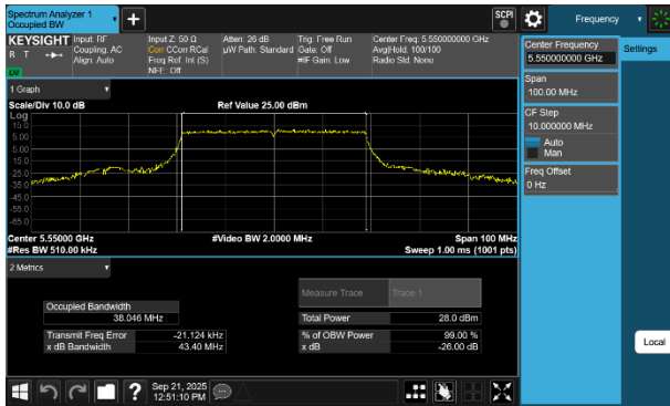
Plot 7-9 26dB BW & 99% OBW Antenna WF7a (40MHz BW 802.11be(RU) RU484 Index65 - Ch.110)
