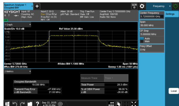
Plot 7-19 26dB BW & 99% OBW Antenna WF2a (20MHz BW 802.11be(RU) RU242 Index61 - Ch.144)
