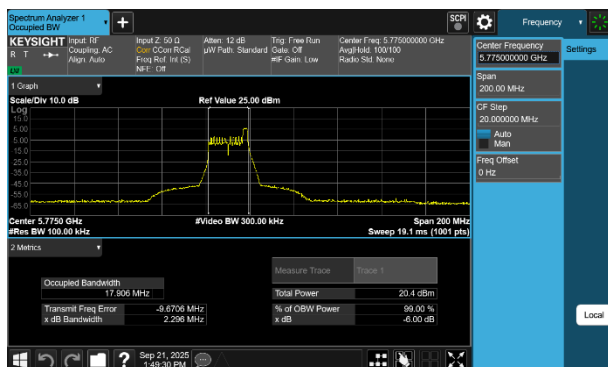
Plot 7-36 6dB OBW Antenna WF7a (80MHz BW 802.11be(RU) RU26 Index17 - Ch.155)
