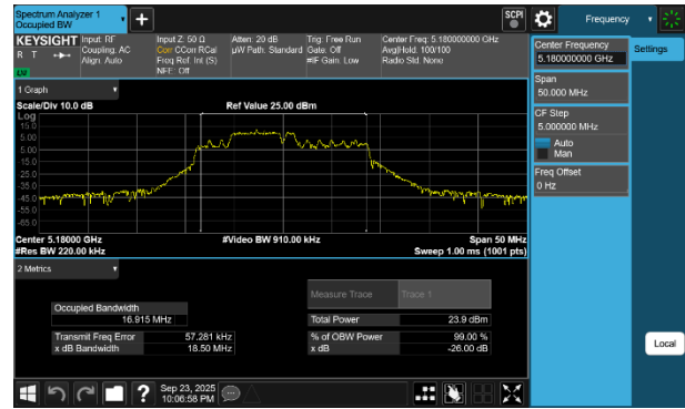
Plot 7-27 26dB BW & 99% OBW Antenna WF7b (20MHz BW 802.11be(RU) RU52+26 Index71 - Ch.36)
