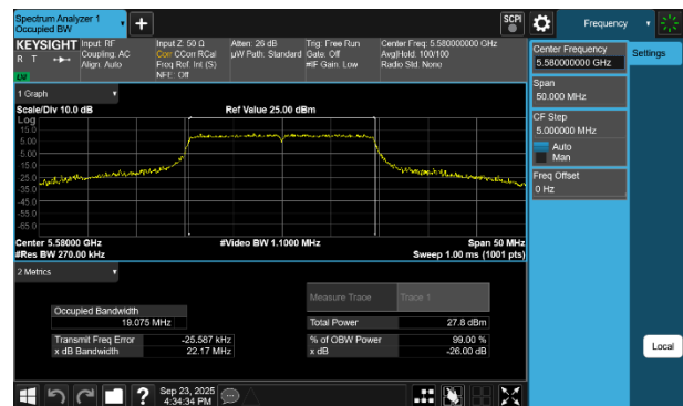
Plot 7-30 26dB BW & 99% OBW Antenna WF7b (20MHz BW 802.11be(RU) RU242 Index61 - Ch.116)
