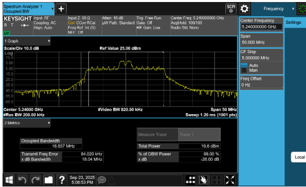
Plot 7-23 26dB BW & 99% OBW Antenna WF7b (20MHz BW 802.11be(RU) RU26 Index4 - Ch.48)
