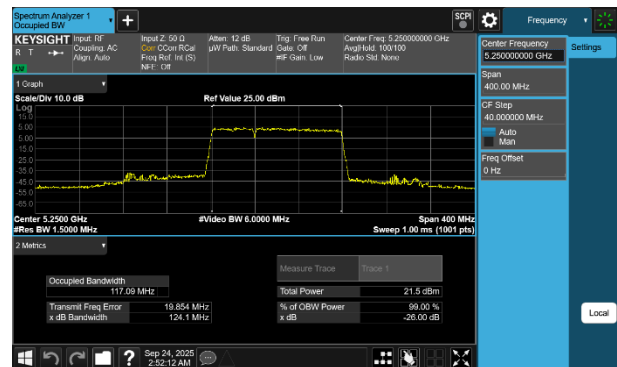
Plot 7-29 26dB BW & 99% OBW Antenna WF7b (160MHz BW 802.11be(RU) RU996+484 Index94 - Ch.50)
