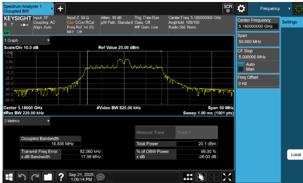
Plot 7-1 26dB BW & 99% OBW Antenna WF7a (20MHz BW 802.11be(RU) RU26 Index4 - Ch.36)
