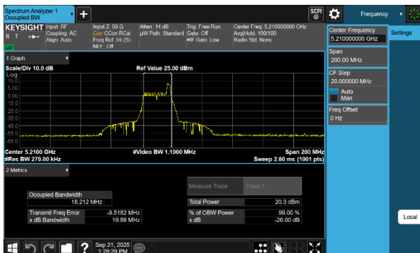
Plot 7-3 26dB BW & 99% OBW Antenna WF7a (80MHz BW 802.11be(RU) RU26 Index17 - Ch.42)
