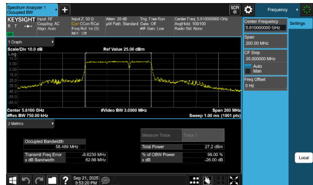
Plot 7-6 26dB BW & 99% OBW Antenna WF7a (80MHz BW 802.11be(RU) RU484+242 Index93 - Ch.122)
