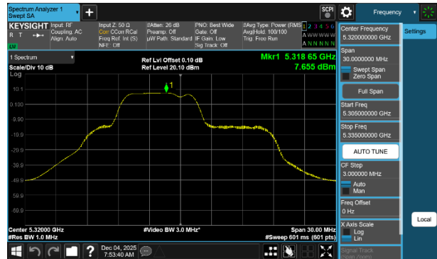
Plot 7-62 PSD Antenna WF7a (20MHz BW 802.11be(RU) RU52+26 Index71 - Ch.64)
