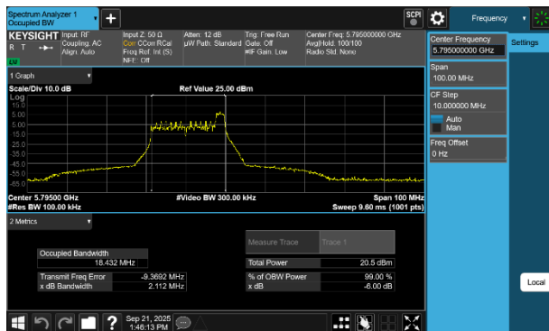
Plot 7-35 6dB OBW Antenna WF7a (40MHz BW 802.11be(RU) RU26 Index8 - Ch.159)
