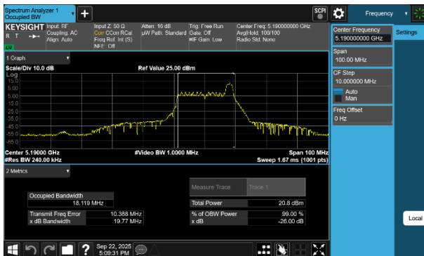
Plot 7-13 26dB BW & 99% OBW Antenna WF2a (40MHz BW 802.11be(RU) RU26 Index17 - Ch.38)
