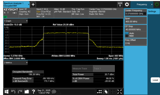
Plot 7-11 26dB BW & 99% OBW Antenna WF7a (160MHz BW 802.11be(RU) RU996X2 Index68 - Ch.114)
