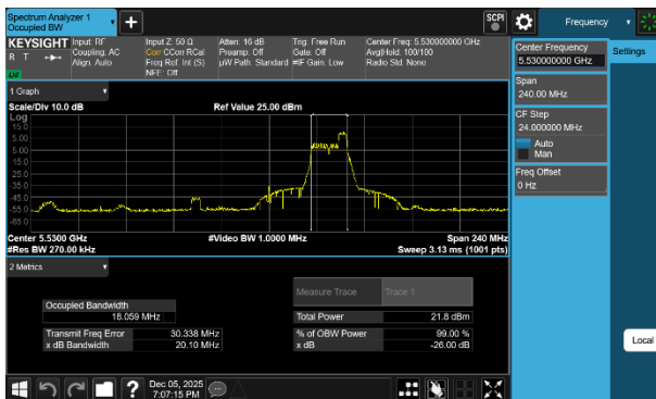
Plot 7-25 26dB BW & 99% OBW Antenna WF7b (80MHz BW 802.11be(RU) RU52 Index52 - Ch.106)
