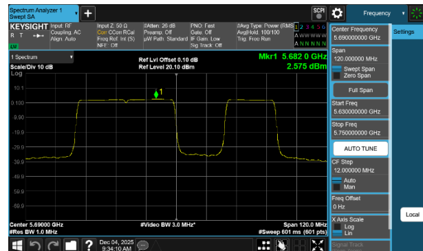
Plot 7-63 PSD Antenna WF7a (80MHz BW 802.11be(RU) RU484+242 Index92 - Ch.138)
