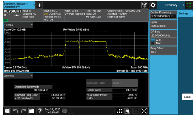
Plot 7-46 26dB BW & 99% OBW Antenna WF2a (80MHz BW 802.11be(RU) RU484+242 Index90 - Ch.155)
