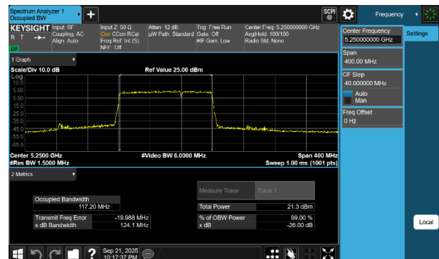
Plot 7-7 26dB BW & 99% OBW Antenna WF7a (160MHz BW 802.11be(RU) RU996+484 Index95 - Ch.50)
