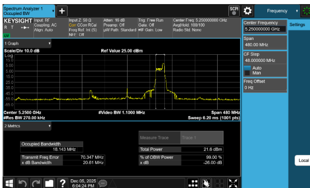
Plot 7-26 26dB BW & 99% OBW Antenna WF7b (160MHz BW 802.11be(RU) RU52 Index52 - Ch.50)
