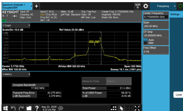
Plot 7-44 6dB OBW Antenna WF2a (80MHz BW 802.11be(RU) RU26 Index36 - Ch.155)
