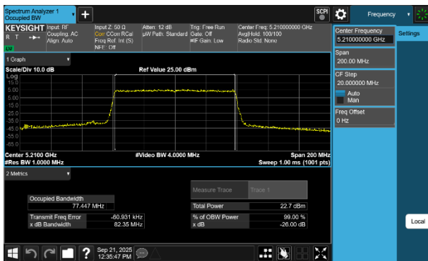
Plot 7-10 26dB BW & 99% OBW Antenna WF7a (80MHz BW 802.11be(RU) RU996 Index67 - Ch.42)
