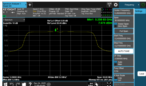
Plot 7-65 PSD Antenna WF7a (20MHz BW 802.11be(RU) RU242 Index61 - Ch.52)
