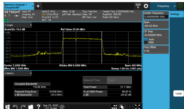
Plot 7-18 26dB BW & 99% OBW Antenna WF2a (160MHz BW 802.11be(RU) RU996+484 Index94 - Ch.50)
