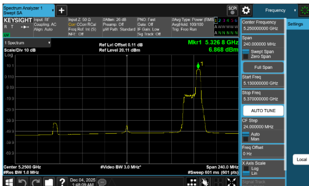
Plot 7-61 PSD Antenna WF7a (160MHz BW 802.11be(RU) RU52 Index52 - Ch.50)
