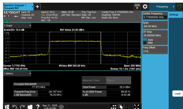
Plot 7-41 6dB OBW Antenna WF7a (80MHz BW 802.11be(RU) RU996 Index67 - Ch.155)
