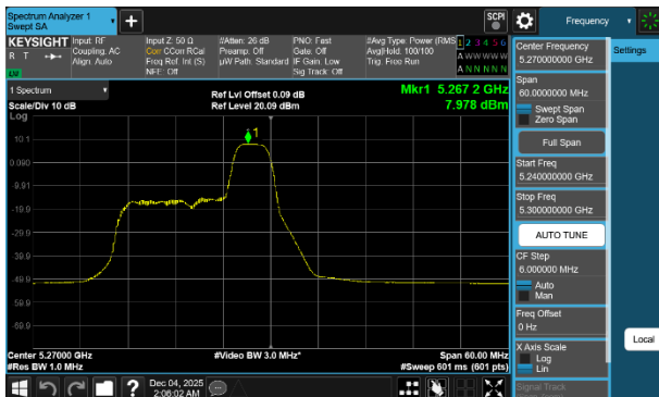
Plot 7-59 PSD Antenna WF7a (40MHz BW 802.11be(RU) RU52 Index40 - Ch.54)
