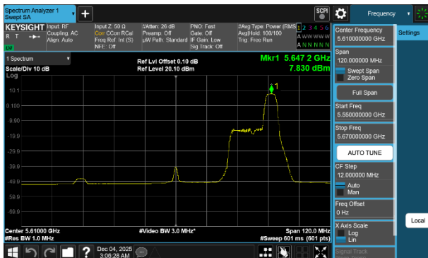
Plot 7-60 PSD Antenna WF7a (80MHz BW 802.11be(RU) RU52 Index52 - Ch.122)
