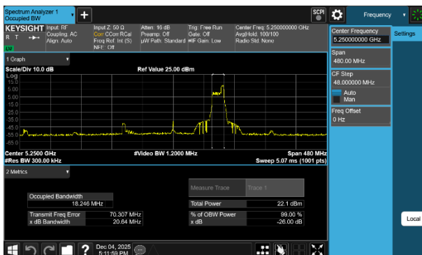
Plot 7-15 26dB BW & 99% OBW Antenna WF2a (160MHz BW 802.11be(RU) RU52 Index52 - Ch.50)
