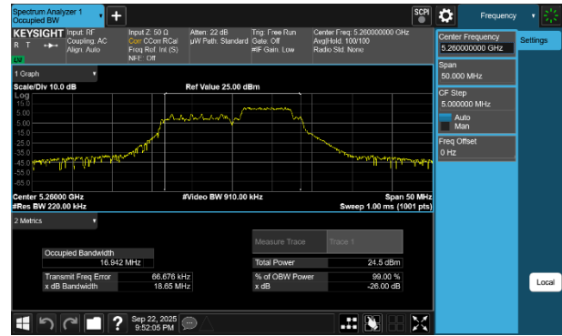
Plot 7-16 26dB BW & 99% OBW Antenna WF2a (20MHz BW 802.11be(RU) RU52+26 Index72 - Ch.52)
