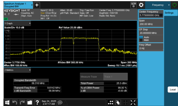
Plot 7-54 6dB OBW Antenna WF7b (80MHz BW 802.11be(RU) RU484+242 Index90 - Ch.155)
