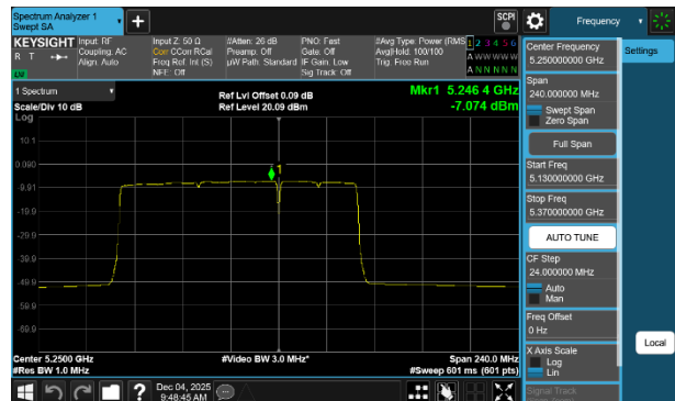
Plot 7-64 PSD Antenna WF7a (160MHz BW 802.11be(RU) RU996+484 Index95 - Ch.50)
