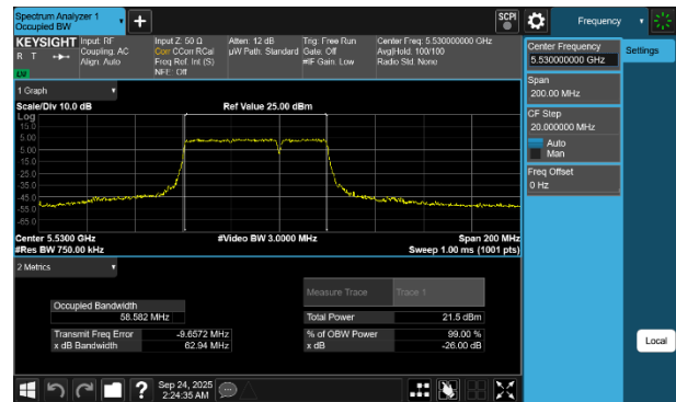
Plot 7-28 26dB BW & 99% OBW Antenna WF7b (80MHz BW 802.11be(RU) RU484+242 Index93 - Ch.106)
