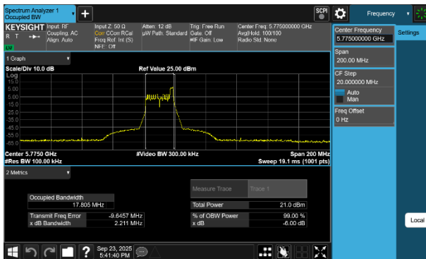
Plot 7-52 6dB OBW Antenna WF7b (80MHz BW 802.11be(RU) RU26 Index17 - Ch.155)
