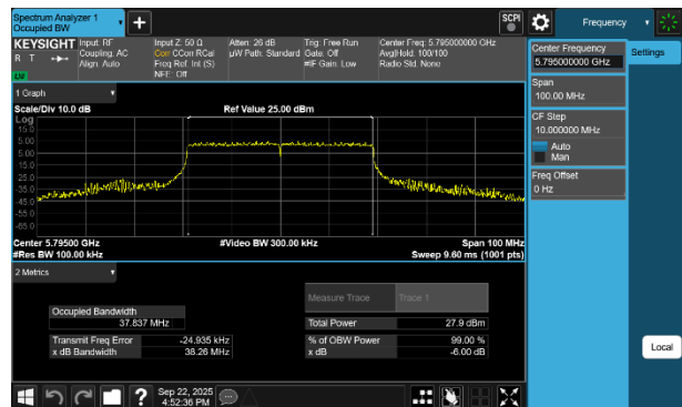
Plot 7-48 6dB OBW Antenna WF2a (40MHz BW 802.11be(RU) RU484 Index65 - Ch.159)
