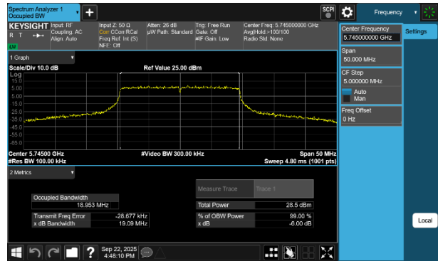
Plot 7-47 6dB OBW Antenna WF2a (20MHz BW 802.11be(RU) RU242 Index61 - Ch.149)
