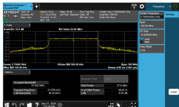
Plot 7-40 6dB OBW Antenna WF7a (40MHz BW 802.11be(RU) RU484 Index65 - Ch.159)
