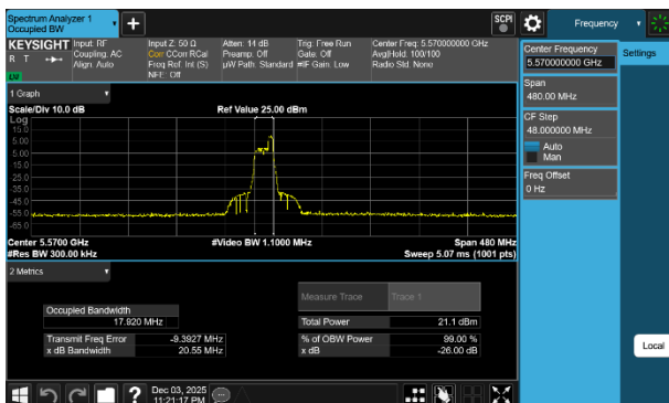
Plot 7-4 26dB BW & 99% OBW Antenna WF7a (160MHz BW 802.11be(RU) RU52 Index52 - Ch.114)
