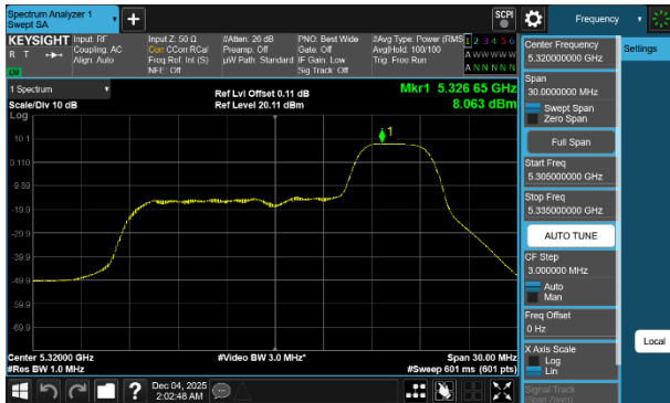
Plot 7-58 PSD Antenna WF7a (20MHz BW 802.11be(RU) RU52 Index40 - Ch.64)
