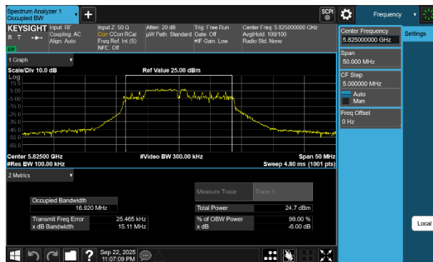
Plot 7-45 26dB BW & 99% OBW Antenna WF2a (20MHz BW 802.11be(RU) RU52+26 Index71 - Ch.165)
