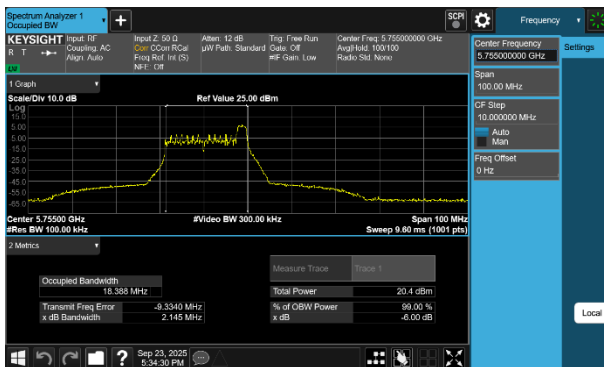
Plot 7-51 6dB OBW Antenna WF7b (40MHz BW 802.11be(RU) RU26 Index8 - Ch.151)
