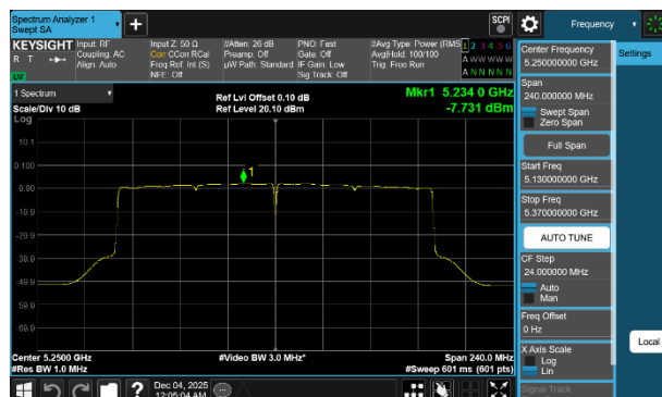
Plot 7-68 PSD Antenna WF7a (160MHz BW 802.11be(RU) RU996X2 Index68 - Ch.50)
