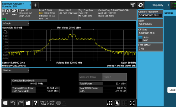
Plot 7-12 26dB BW & 99% OBW Antenna WF2a (20MHz BW 802.11be(RU) RU26 Index4 - Ch.48)
