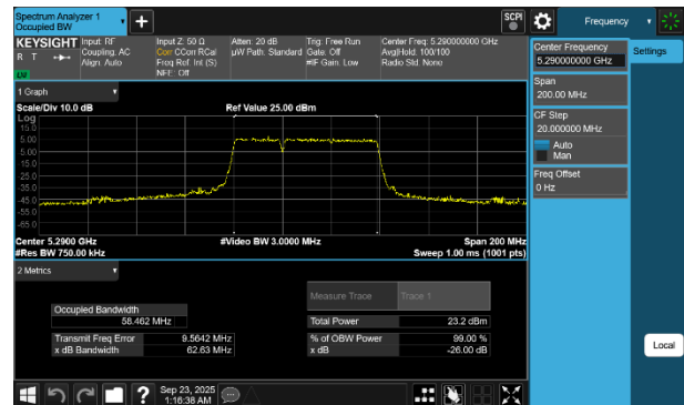
Plot 7-17 26dB BW & 99% OBW Antenna WF2a (80MHz BW 802.11be(RU) RU48+242 Index90 - Ch.58)
