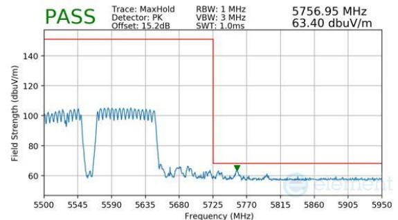
Plot 7-1176. CDD Diversity (Peak, RU996+484+242, Index 99 (L), Ch.114, MCS11)
