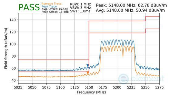
Plot 7-1085. CDD Diversity (Peak & Average, RU484+242, Index 93, Ch.42, MCS11)
