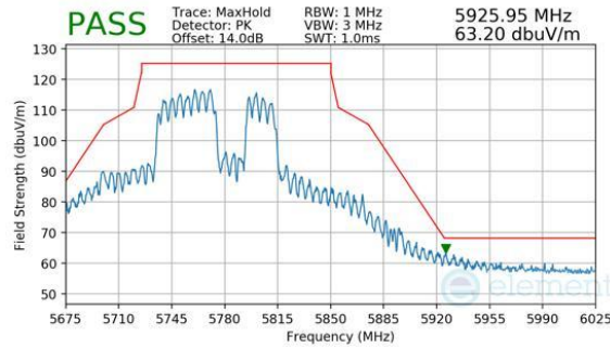
Plot 7-1112. CDD Diversity (Peak, RU484+242, Index 92, Ch.155, MCS11)
