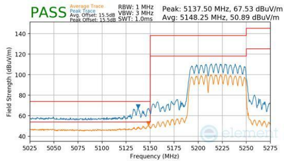
Plot 7-1082. CDD Diversity (Peak & Average, RU484+242, Index 90, Ch.42, MCS11)
