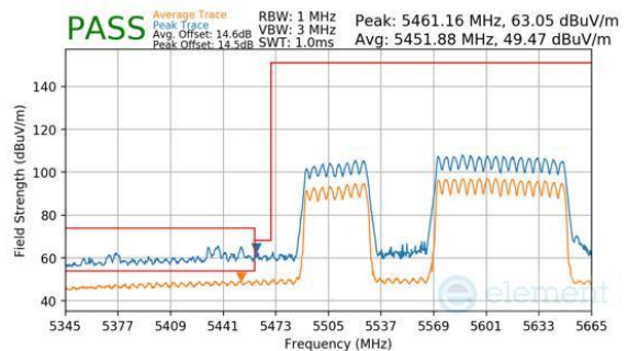
Plot 7-1139. CDD Diversity (Peak & Average, RU996+484, Index 95 (L), Ch.114, MCS11)
