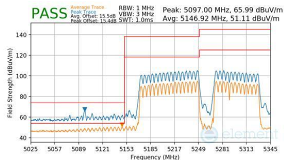
Plot 7-1146. CDD Diversity (Peak & Average, RU996+484+242, Index 96 (H), Ch.50, MCS11)
