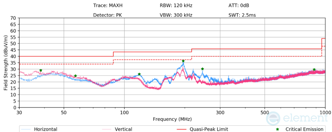
Plot 7-1185. RSE below 1GHz CDD Diversity (RU78 – Ch.40), with AC/DC Adapter
