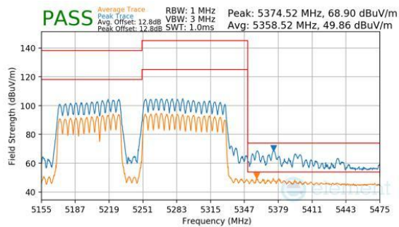
Plot 7-1160. CDD Diversity (Peak & Average, RU996+484+242, Index 99 (L), Ch.50, MCS11)
