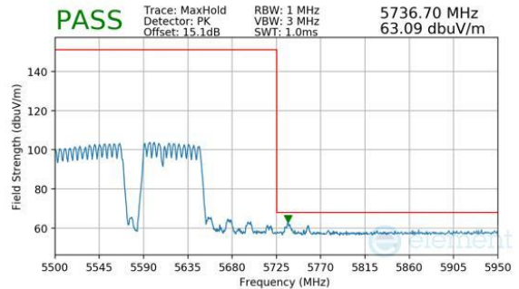
Plot 7-1170. CDD Diversity (Peak, RU996+484+242, Index 96 (H), Ch.114, MCS11)
