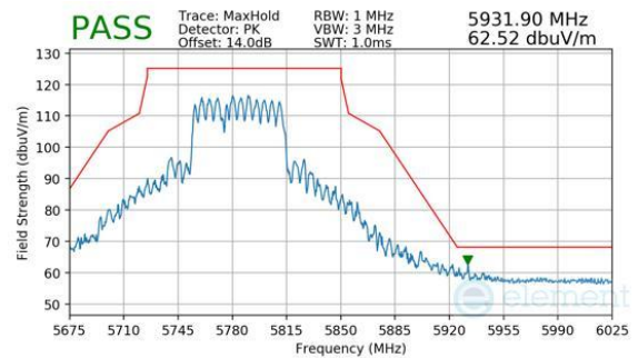
Plot 7-1110. CDD Diversity (Peak, RU484+242, Index 90, Ch.155, MCS11)
