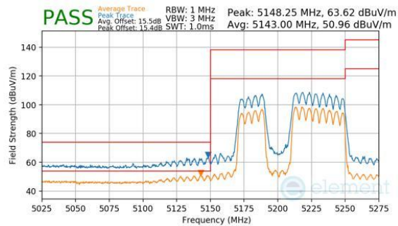
Plot 7-1083. CDD Diversity (Peak & Average, RU484+242, Index 91, Ch.42, MCS11)
