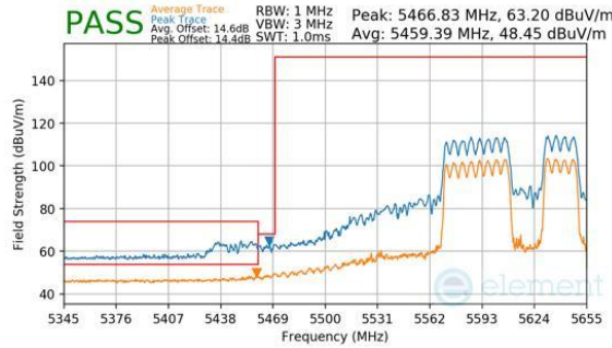
Plot 7-1100. CDD Diversity (Peak & Average, RU484+242, Index 92, Ch.122, MCS11)
