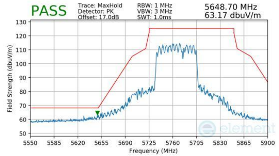
Plot 7-1109. CDD Diversity (Peak, RU484+242, Index 93, Ch.155, MCS11)
