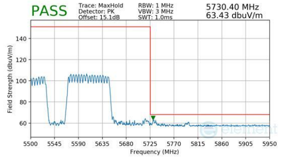
Plot 7-1144. CDD Diversity (Peak, RU996+484, Index 95 (L), Ch.114, MCS11)
