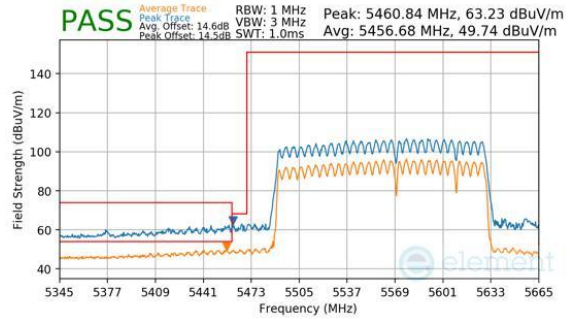
Plot 7-1168. CDD Diversity (Peak & Average, RU996+484+242, Index 99 (H), Ch.114, MCS11)
