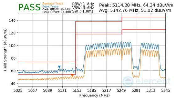
Plot 7-1148. CDD Diversity (Peak & Average, RU996+484+242, Index 97 (H), Ch.50, MCS11)
