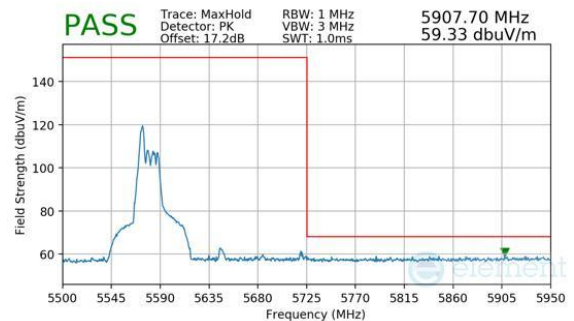
Plot 7-1080. CDD Diversity (Peak, RU52, Index 37, Ch.122, MCS11)
