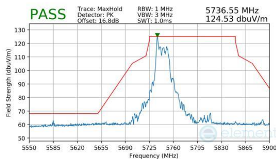
Plot 7-1072. CDD Diversity (Peak, RU26, Index 0, Ch.155, MCS11)
