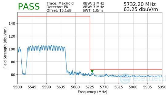
Plot 7-1171. CDD Diversity (Peak, RU996+484+242, Index 97 (L), Ch.114, MCS11)
