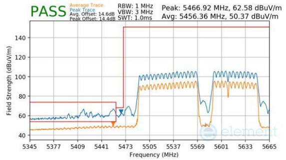
Plot 7-1162. CDD Diversity (Peak & Average, RU996+484+242, Index 96 (H), Ch.114, MCS11)
