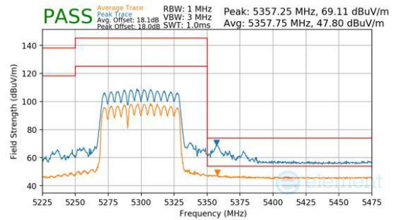
Plot 7-1087. CDD Diversity (Peak & Average, RU484+242, Index 90, Ch.58, MCS11)
