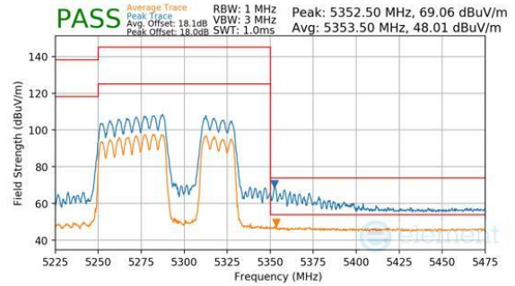
Plot 7-1091. CDD Diversity (Peak & Average, RU484+242, Index 92, Ch.58, MCS11)
