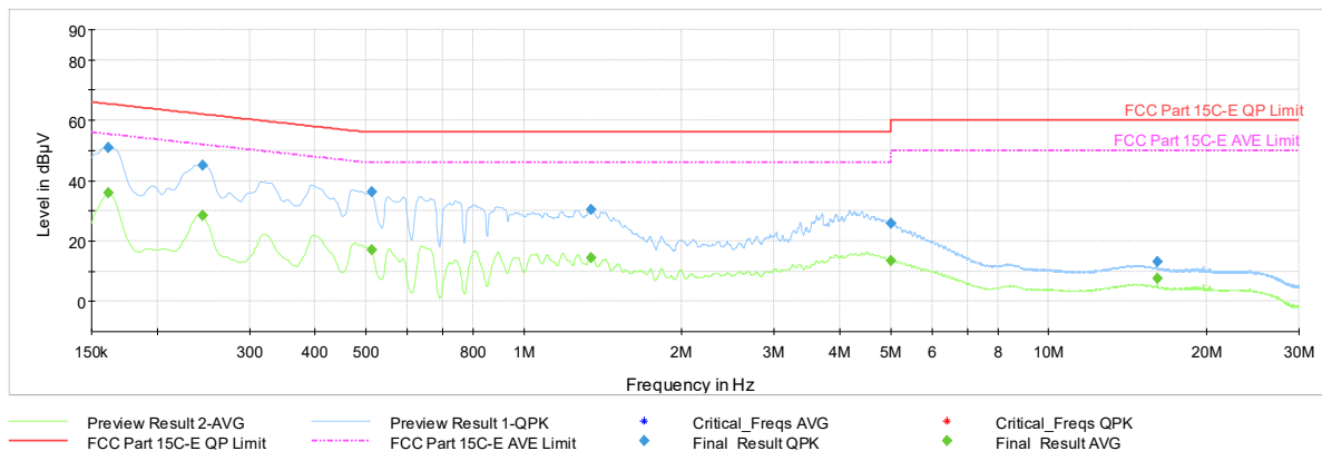
Plot 7-1196. AC Line Conducted Plot with 11be CDD Diversity – RU78 – Ch.40 (N) with AC/DC Adapter
