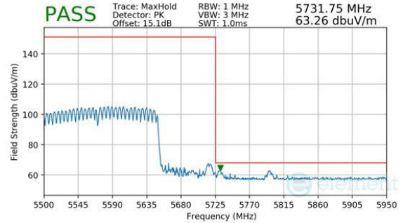
Plot 7-1180. CDD Diversity (Peak, RU996X2, Index 68, Ch.114, MCS11)
