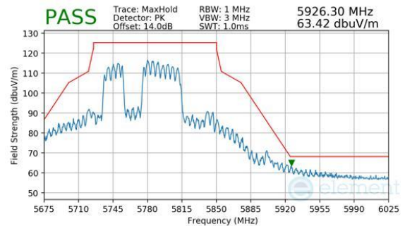
Plot 7-1111. CDD Diversity (Peak, RU484+242, Index 91, Ch.155, MCS11)
