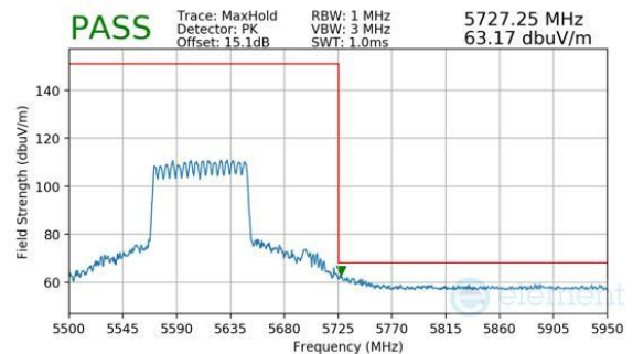
Plot 7-1118. CDD Diversity (Peak, RU996, Index 67, Ch.122, MCS11)
