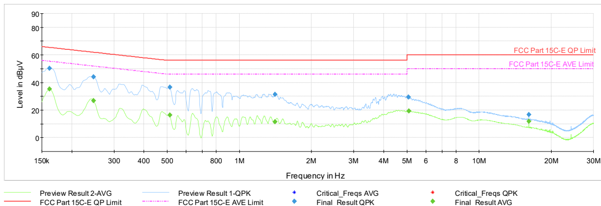
Plot 7-1197. AC Line Conducted Plot with 11be CDD Diversity – RU242 – Ch.40 (L1) with AC/DC Adapter
