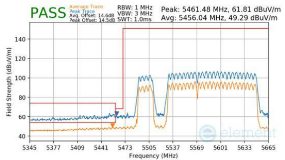
Plot 7-1163. CDD Diversity (Peak & Average, RU996+484+242, Index 97 (L), Ch.114, MCS11)
