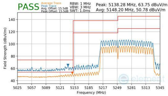
Plot 7-1129. CDD Diversity (Peak & Average, RU996+484, Index 94 (L), Ch.50, MCS11)
