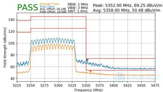
Plot 7-1115. CDD Diversity (Peak & Average, RU996, Index 67, Ch.58, MCS11)
