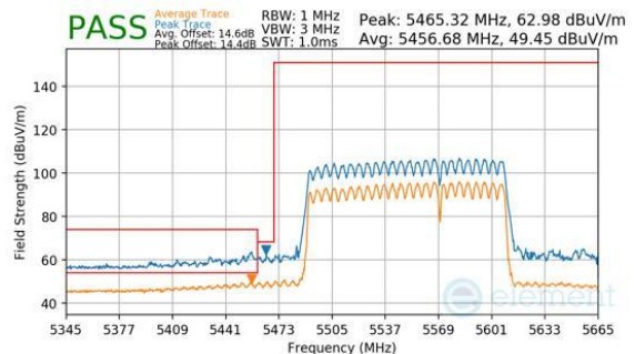
Plot 7-1140. CDD Diversity (Peak & Average, RU996+484, Index 95 (H), Ch.114, MCS11)
