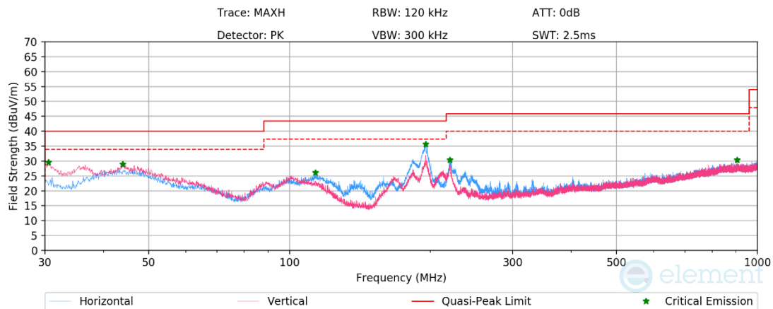
Plot 7-1186. RSE below 1GHz CDD Diversity (RU242 – Ch.40), with AC/DC Adapter
