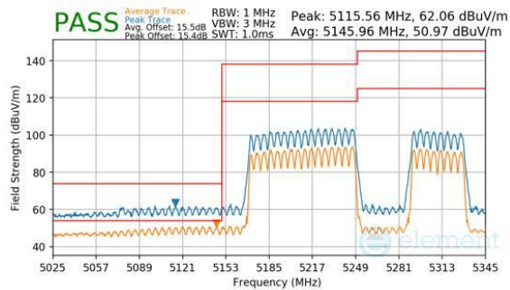
Plot 7-1130. CDD Diversity (Peak & Average, RU996+484, Index 94 (H), Ch.50, MCS11)
