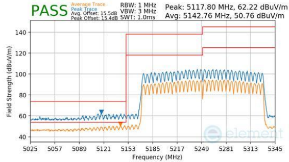
Plot 7-1177. CDD Diversity (Peak & Average, RU996X2, Index 68, Ch.50, MCS11)
