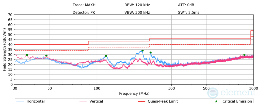
Plot 7-1181. RSE below 1GHz CDD Primary (RU26 – Ch.40), with AC/DC Adapter
