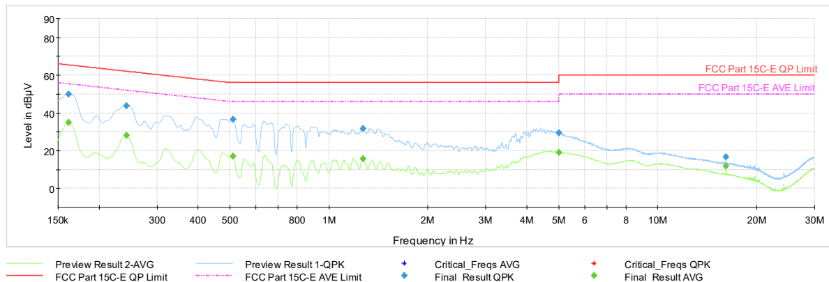
Plot 7-1195. AC Line Conducted Plot with 11be CDD Diversity – RU78 – Ch.40 (L1) with AC/DC Adapter
