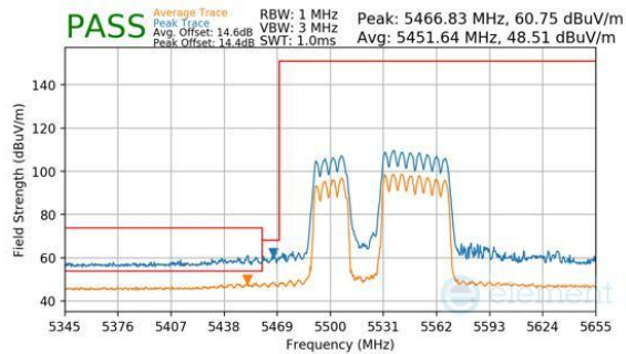
Plot 7-1095. CDD Diversity (Peak & Average, RU484+242, Index 91, Ch.106, MCS11)
