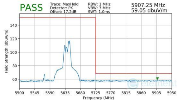
Plot 7-1081. CDD Diversity (Peak, RU52, Index 52, Ch.122, MCS11)
