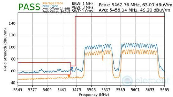
Plot 7-1167. CDD Diversity (Peak & Average, RU996+484+242, Index 99 (L), Ch.114, MCS11)
