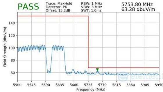
Plot 7-1172. CDD Diversity (Peak, RU996+484+242, Index 97 (H), Ch.114, MCS11)
