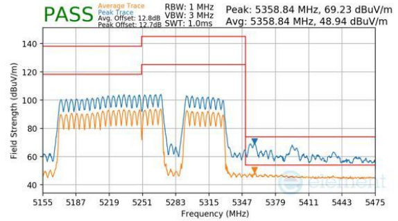
Plot 7-1156. CDD Diversity (Peak & Average, RU996+484+242, Index 97 (H), Ch.50, MCS11)
