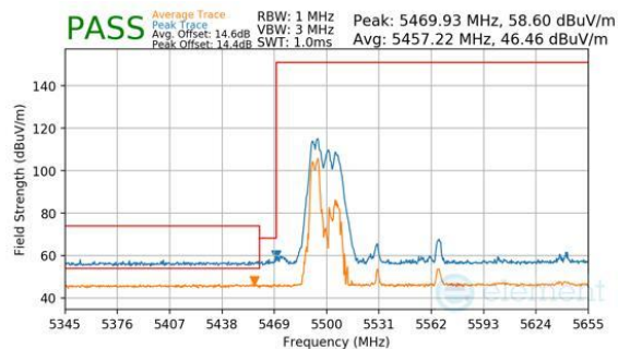
Plot 7-1078. CDD Diversity (Peak & Average, RU52, Index 37, Ch.106, MCS11)
