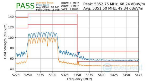
Plot 7-1093. CDD Diversity (Peak & Average, RU484+242, Index 93, Ch.58, MCS11)
