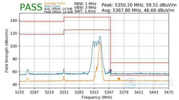
Plot 7-1124. CDD Diversity (Peak & Average, RU52, Index 52 (H), Ch.50, MCS11)
