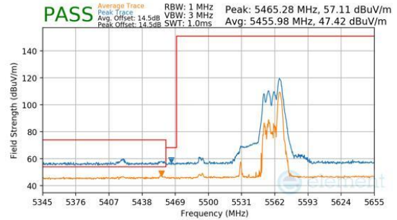
Plot 7-1079. CDD Diversity (Peak & Average, RU52, Index 52, Ch.106, MCS11)
