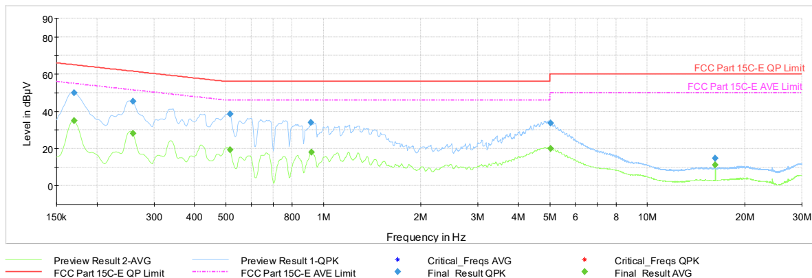
Plot 7-1191. AC Line Conducted Plot with 11be CDD Primary – RU242 – Ch.40 (L1) with AC/DC Adapter
