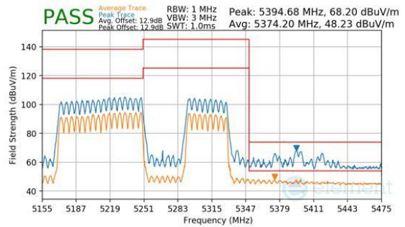
Plot 7-1134. CDD Diversity (Peak & Average, RU996+484, Index 94 (H), Ch.50, MCS11)
