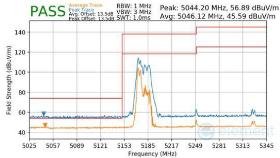
Plot 7-1121. CDD Diversity (Peak & Average, RU52, Index 37 (L), Ch.50, MCS11)
