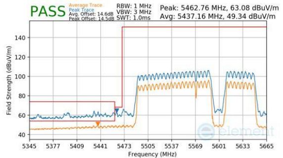
Plot 7-1164. CDD Diversity (Peak & Average, RU996+484+242, Index 97 (H), Ch.114, MCS11)
