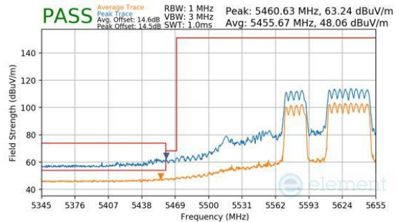
Plot 7-1099. CDD Diversity (Peak & Average, RU484+242, Index 91, Ch.122, MCS11)
