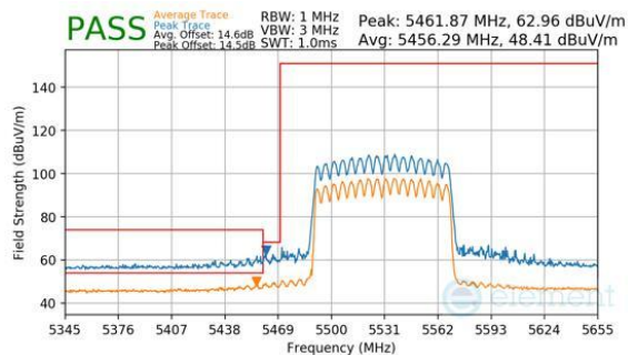
Plot 7-1116. CDD Diversity (Peak & Average, RU996, Index 67, Ch.106, MCS11)
