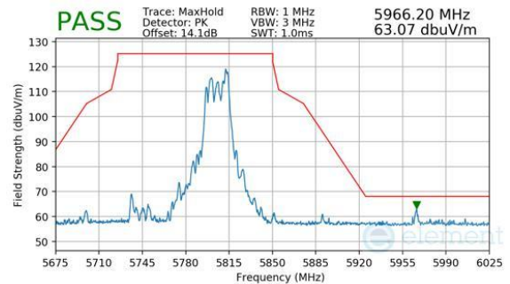
Plot 7-1075. CDD Diversity (Peak, RU26, Index 36, Ch.155, MCS11)
