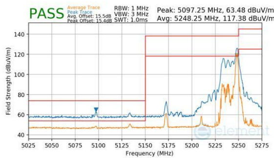
Plot 7-1071. CDD Diversity (Peak & Average, RU26, Index 36, Ch.42, MCS11)
