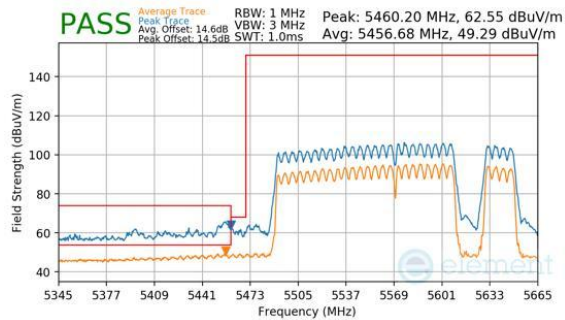
Plot 7-1166. CDD Diversity (Peak & Average, RU996+484+242, Index 98 (H), Ch.114, MCS11)
