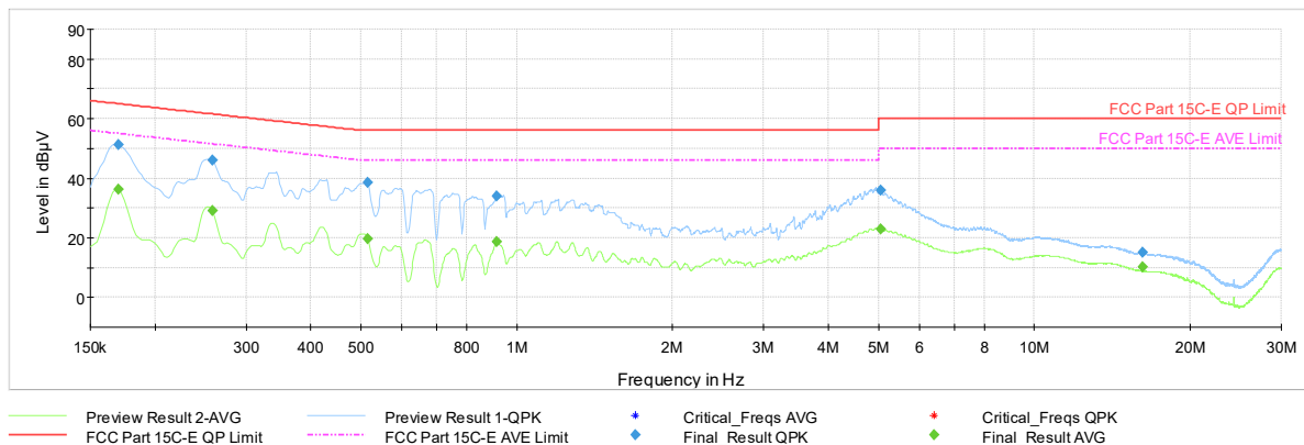
Plot 7-1190. AC Line Conducted Plot with 11be CDD Primary – RU78 – Ch.40 (N) with AC/DC Adapter
