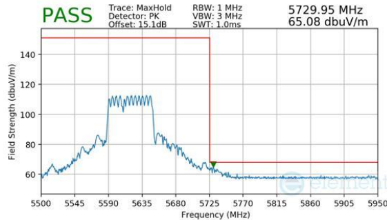
Plot 7-1102. CDD Diversity (Peak, RU484+242, Index 90, Ch.122, MCS11)
