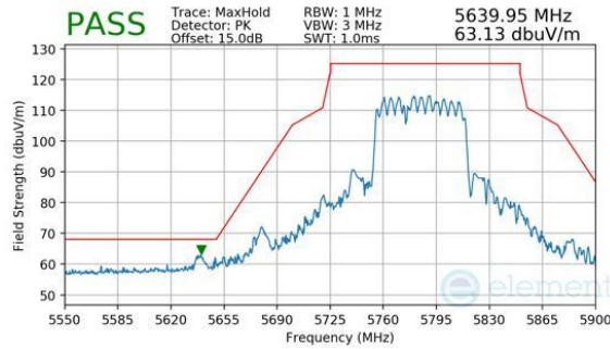
Plot 7-1106. CDD Diversity (Peak, RU484+242, Index 90, Ch.155, MCS11)
