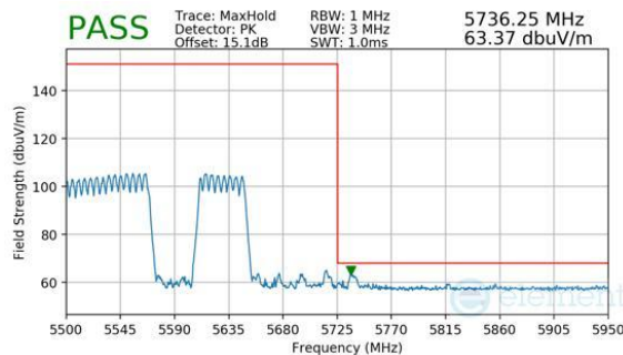
Plot 7-1142. CDD Diversity (Peak, RU996+484, Index 94 (H), Ch.114, MCS11)
