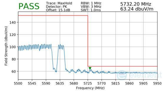
Plot 7-1174. CDD Diversity (Peak, RU996+484+242, Index 98 (H), Ch.114, MCS11)
