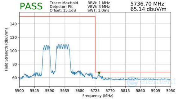
Plot 7-1103. CDD Diversity (Peak, RU484+242, Index 91, Ch.122, MCS11)
