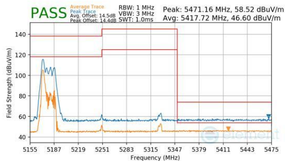
Plot 7-1123. CDD Diversity (Peak & Average, RU52, Index 37 (L), Ch.50, MCS11)
