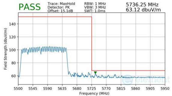
Plot 7-1169. CDD Diversity (Peak, RU996+484+242, Index 96 (L), Ch.114, MCS11)
