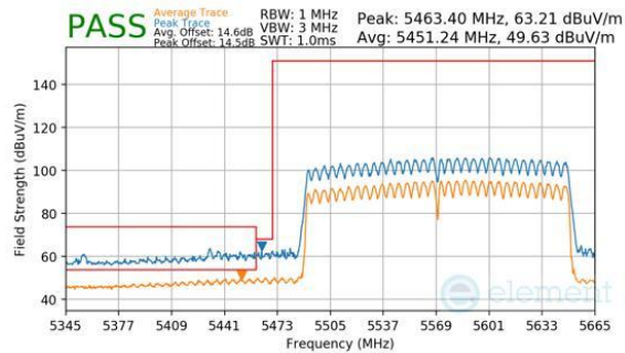
Plot 7-1179. CDD Diversity (Peak & Average, RU996X2, Index 68, Ch.114, MCS11)
