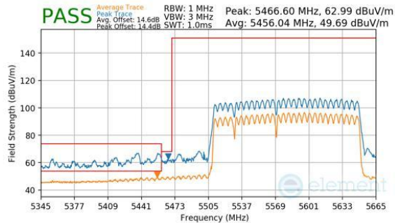
Plot 7-1161. CDD Diversity (Peak & Average, RU996+484+242, Index 96 (L), Ch.114, MCS11)
