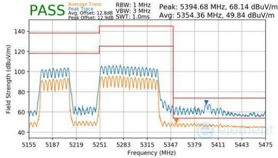
Plot 7-1135. CDD Diversity (Peak & Average, RU996+484, Index 95 (L), Ch.50, MCS11)
