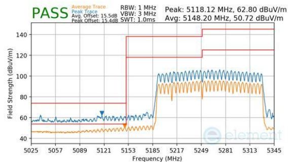
Plot 7-1145. CDD Diversity (Peak & Average, RU996+484+242, Index 96 (L), Ch.50, MCS11)
