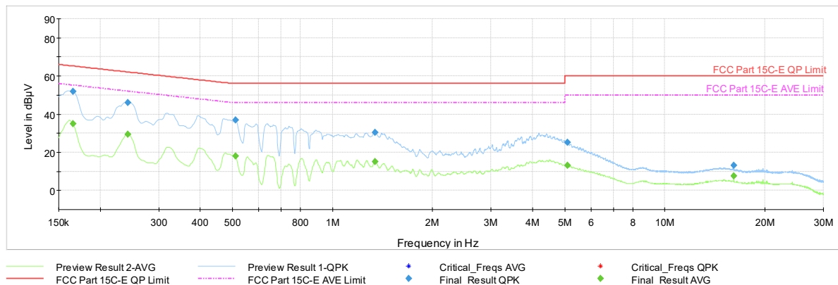
Plot 7-1198. AC Line Conducted Plot with 11be CDD Diversity – RU242 – Ch.40 (N) with AC/DC Adapter
