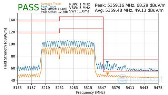
Plot 7-1133. CDD Diversity (Peak & Average, RU996+484, Index 94 (L), Ch.50, MCS11)
