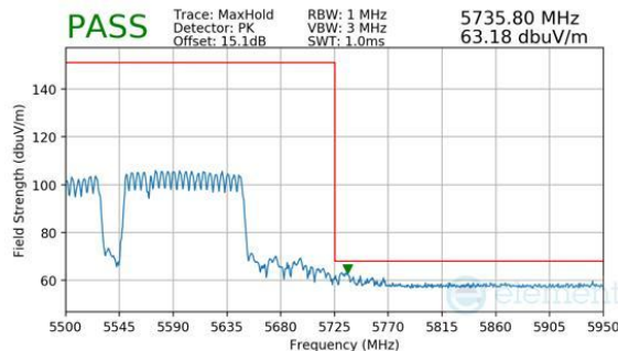
Plot 7-1173. CDD Diversity (Peak, RU996+484+242, Index 98 (L), Ch.114, MCS11)
