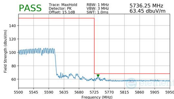
Plot 7-1143. CDD Diversity (Peak, RU996+484, Index 95 (H), Ch.114, MCS11)
