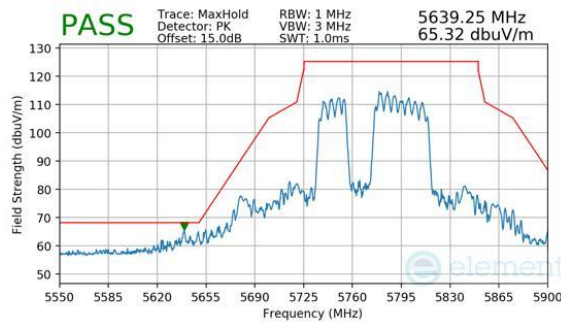
Plot 7-1107. CDD Diversity (Peak, RU484+242, Index 91, Ch.155, MCS11)
