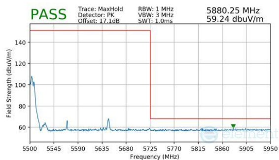
Plot 7-1127. CDD Diversity (Peak, RU52, Index 37 (L), Ch.114, MCS11)
