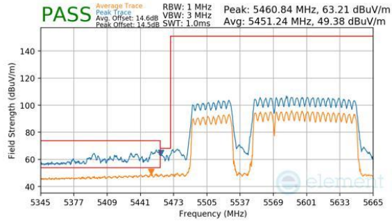
Plot 7-1165. CDD Diversity (Peak & Average, RU996+484+242, Index 98 (L), Ch.114, MCS11)
