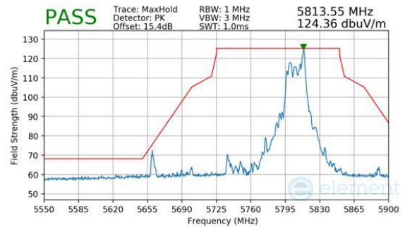
Plot 7-1073. CDD Diversity (Peak, RU26, Index 36, Ch.155, MCS11)
