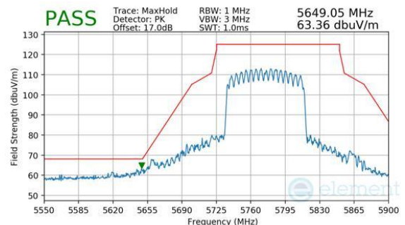
Plot 7-1119. CDD Diversity (Peak, RU996, Index 67, Ch.155, MCS11)
