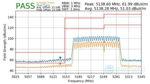
Plot 7-1132. CDD Diversity (Peak & Average, RU996+484, Index 95 (H), Ch.50, MCS11)
