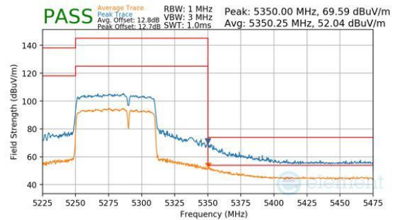
Plot 7-1092. CDD Diversity (Peak & Average, RU484+242, Index 93, Ch.58, MCS11)
