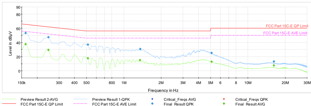
Plot 7-1194. AC Line Conducted Plot with 11be CDD Diversity – RU26 – Ch.40 (N) with AC/DC Adapter
