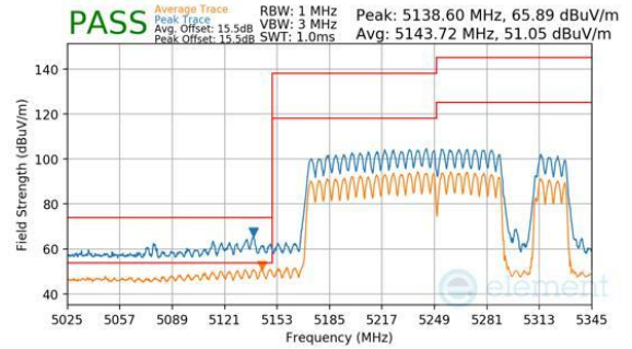
Plot 7-1150. CDD Diversity (Peak & Average, RU996+484+242, Index 98 (H), Ch.50, MCS11)
