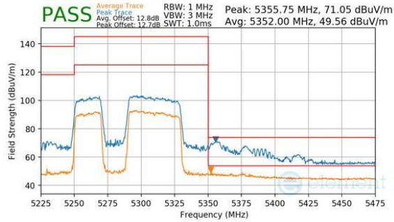
Plot 7-1088. CDD Diversity (Peak & Average, RU484+242, Index 91, Ch.58, MCS11)
