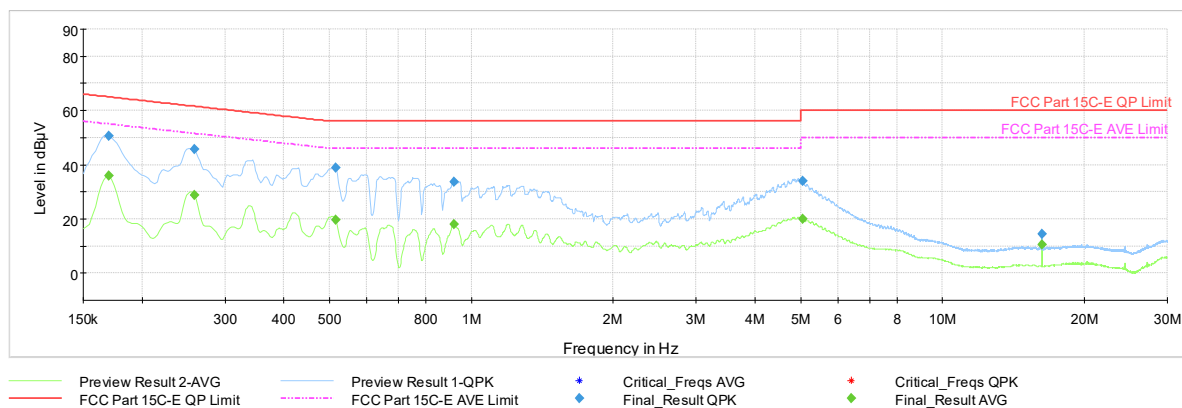
Plot 7-1187. AC Line Conducted Plot with 11be CDD Primary – RU26 – Ch.40 (L1) with AC/DC Adapter
