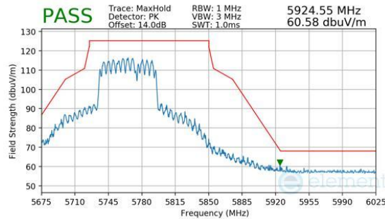
Plot 7-1113. CDD Diversity (Peak, RU484+242, Index 93, Ch.155, MCS11)
