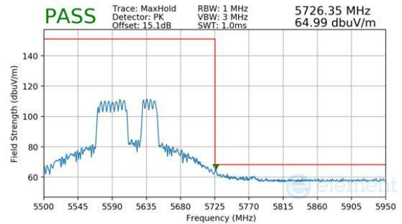
Plot 7-1104. CDD Diversity (Peak, RU484+242, Index 92, Ch.122, MCS11)
