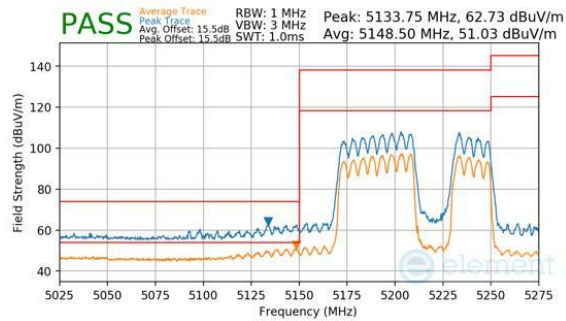
Plot 7-1084. CDD Diversity (Peak & Average, RU484+242, Index 92, Ch.42, MCS11)
