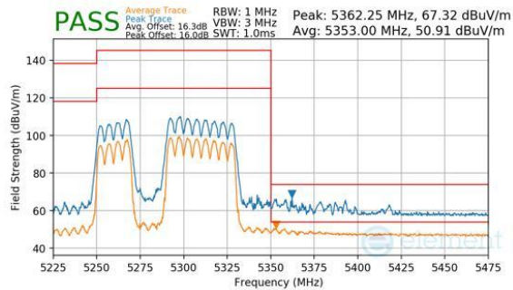
Plot 7-1089. CDD Diversity (Peak & Average, RU484+242, Index 91, Ch.58, MCS11)
