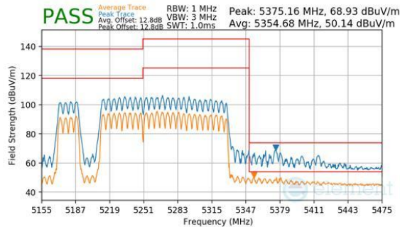
Plot 7-1155. CDD Diversity (Peak & Average, RU996+484+242, Index 97 (L), Ch.50, MCS11)
