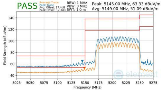
Plot 7-1114. CDD Diversity (Peak & Average, RU996, Index 67, Ch.42, MCS11)
