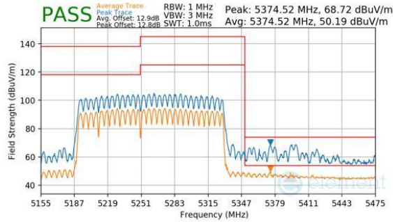
Plot 7-1153. CDD Diversity (Peak & Average, RU996+484+242, Index 96 (L), Ch.50, MCS11)
