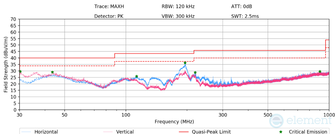
Plot 7-1184. RSE below 1GHz CDD Diversity (RU26 – Ch.40), with AC/DC Adapter
