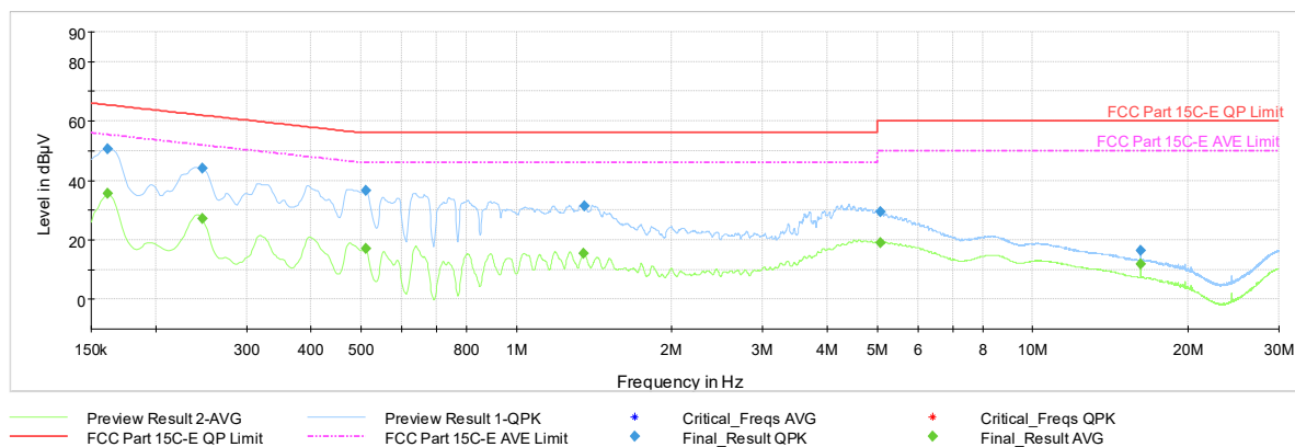
Plot 7-1193. AC Line Conducted Plot with 11be CDD Diversity – RU26 – Ch.40 (L1) with AC/DC Adapter
