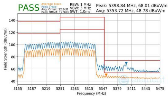
Plot 7-1178. CDD Diversity (Peak & Average, RU996X2, Index 68, Ch.50, MCS11)
