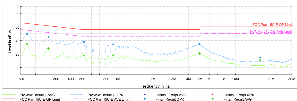
Plot 7-1189. AC Line Conducted Plot with 11be CDD Primary – RU78 – Ch.40 (L1) with AC/DC Adapter
