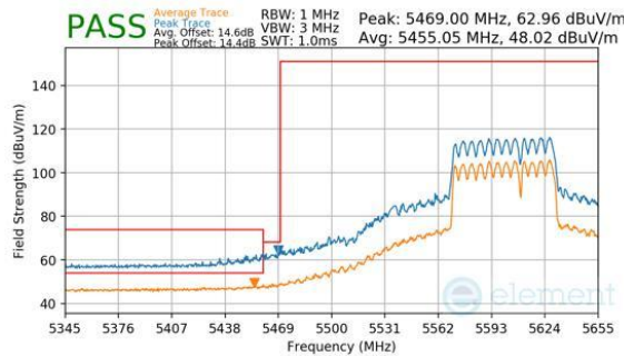
Plot 7-1101. CDD Diversity (Peak & Average, RU484+242, Index 93, Ch.122, MCS11)
