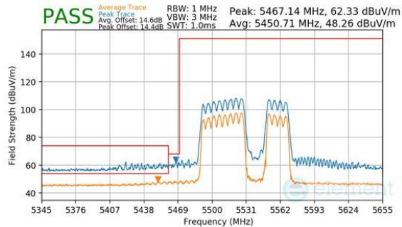
Plot 7-1096. CDD Diversity (Peak & Average, RU484+242, Index 92, Ch.106, MCS11)
