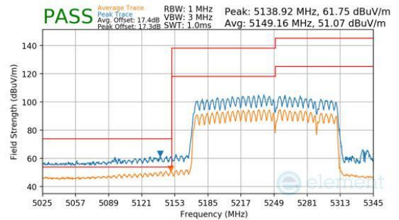
Plot 7-1151. CDD Diversity (Peak & Average, RU996+484+242, Index 99 (H), Ch.50, MCS11)
