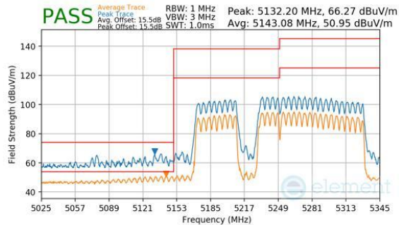
Plot 7-1149. CDD Diversity (Peak & Average, RU996+484+242, Index 98 (L), Ch.50, MCS11)
