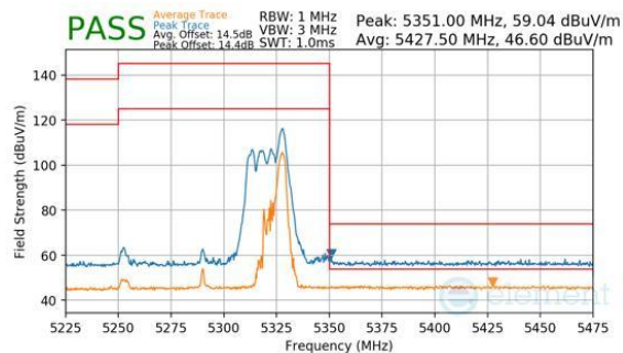
Plot 7-1077. CDD Diversity (Peak & Average, RU52, Index 52, Ch.58, MCS11)
