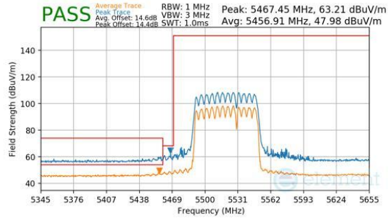
Plot 7-1097. CDD Diversity (Peak & Average, RU484+242, Index 93, Ch.106, MCS11)
