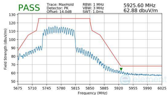
Plot 7-1120. CDD Diversity (Peak, RU996, Index 67, Ch.155, MCS11)
