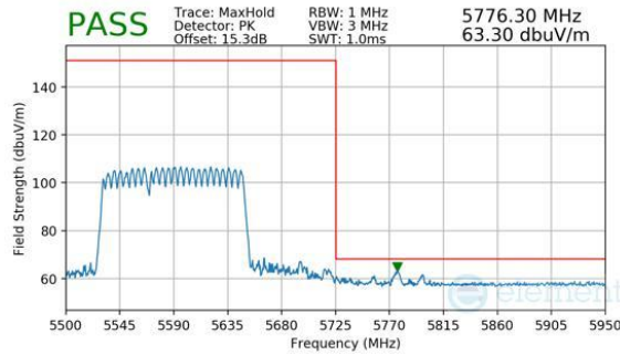
Plot 7-1141. CDD Diversity (Peak, RU996+484, Index 94 (L), Ch.114, MCS11)
