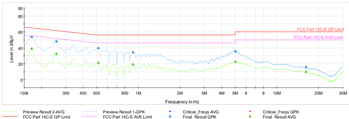
Plot 7-1188. AC Line Conducted Plot with 11be CDD Primary – RU26 – Ch.40 (N) with AC/DC Adapter
