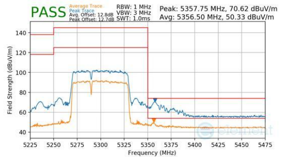
Plot 7-1086. CDD Diversity (Peak & Average, RU484+242, Index 90, Ch.58, MCS11)
