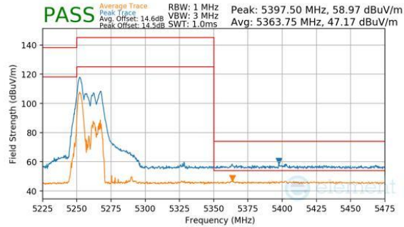
Plot 7-1076. CDD Diversity (Peak & Average, RU52, Index 37, Ch.58, MCS11)
