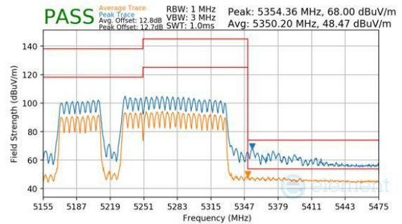
Plot 7-1157. CDD Diversity (Peak & Average, RU996+484+242, Index 98 (L), Ch.50, MCS11)
