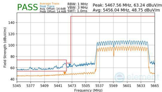
Plot 7-1137. CDD Diversity (Peak & Average, RU996+484, Index 94 (L), Ch.114, MCS11)
