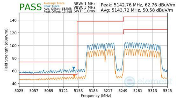
Plot 7-1152. CDD Diversity (Peak & Average, RU996+484+242, Index 99 (L), Ch.50, MCS11)
