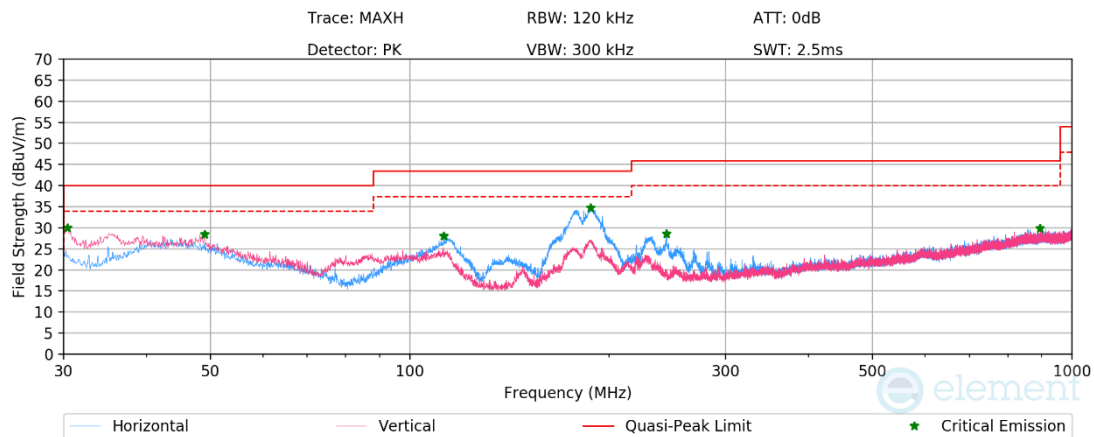
Plot 7-1182. RSE below 1GHz CDD Primary (RU78 – Ch.40), with AC/DC Adapter
