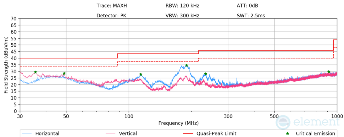
Plot 7-1183. RSE below 1GHz CDD Primary (RU242 – Ch.40), with AC/DC Adapter
