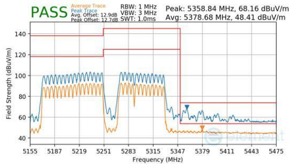
Plot 7-1154. CDD Diversity (Peak & Average, RU996+484+242, Index 96 (H), Ch.50, MCS11)
