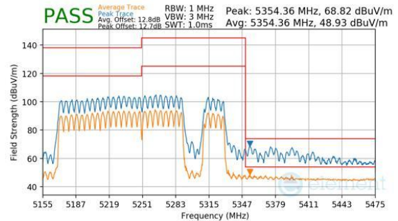
Plot 7-1158. CDD Diversity (Peak & Average, RU996+484+242, Index 98 (H), Ch.50, MCS11)
