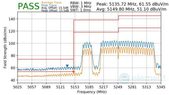
Plot 7-1147. CDD Diversity (Peak & Average, RU996+484+242, Index 97 (L), Ch.50, MCS11)
