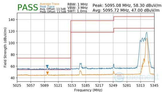
Plot 7-1122. CDD Diversity (Peak & Average, RU52, Index 52 (H), Ch.50, MCS11)
