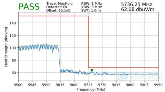
Plot 7-1175. CDD Diversity (Peak, RU996+484+242, Index 99 (H), Ch.114, MCS11)
