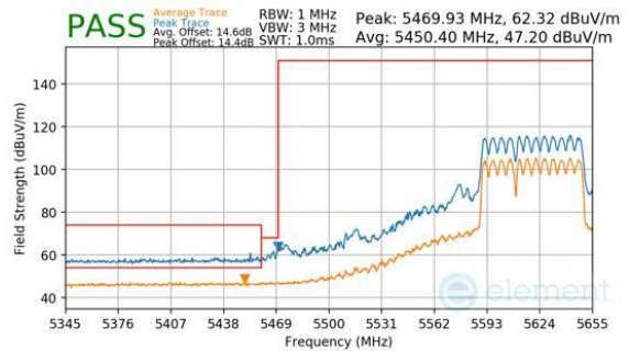
Plot 7-1098. CDD Diversity (Peak & Average, RU484+242, Index 90, Ch.122, MCS11)
