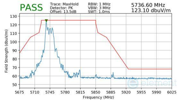
Plot 7-1074. CDD Diversity (Peak, RU26, Index 0, Ch.155, MCS11)
