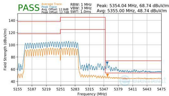
Plot 7-1136. CDD Diversity (Peak & Average, RU996+484, Index 95 (H), Ch.50, MCS11)
