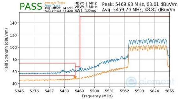
Plot 7-1117. CDD Diversity (Peak & Average, RU996, Index 67, Ch.122, MCS11)
