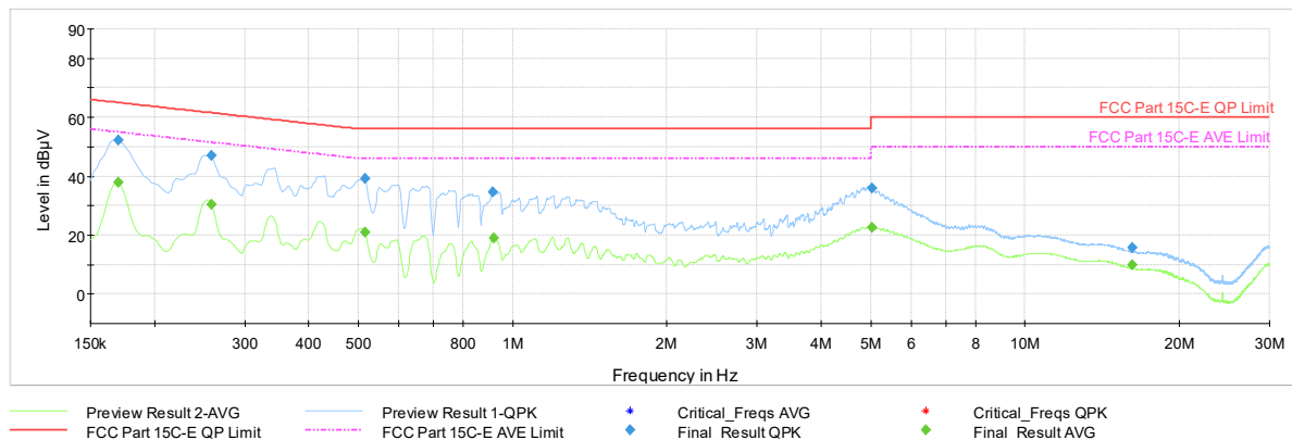
Plot 7-1192. AC Line Conducted Plot with 11be CDD Primary – RU242 – Ch.40 (N) with AC/DC Adapter
