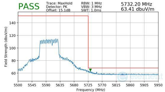
Plot 7-1105. CDD Diversity (Peak, RU484+242, Index 93, Ch.122, MCS11)
