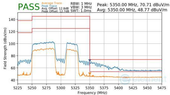
Plot 7-1090. CDD Diversity (Peak & Average, RU484+242, Index 92, Ch.58, MCS11)
