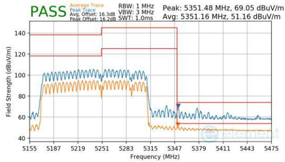
Plot 7-1159. CDD Diversity (Peak & Average, RU996+484+242, Index 99 (H), Ch.50, MCS11)
