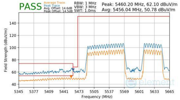
Plot 7-1138. CDD Diversity (Peak & Average, RU996+484, Index 94 (H), Ch.114, MCS11)
