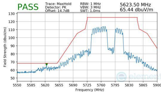
Plot 7-1108. CDD Diversity (Peak, RU484+242, Index 92, Ch.155, MCS11)
