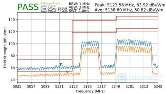
Plot 7-1131. CDD Diversity (Peak & Average, RU996+484, Index 95 (L), Ch.50, MCS11)
