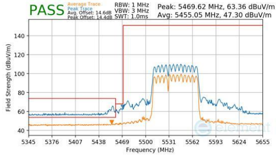
Plot 7-1094. CDD Diversity (Peak & Average, RU484+242, Index 90, Ch.106, MCS11)
