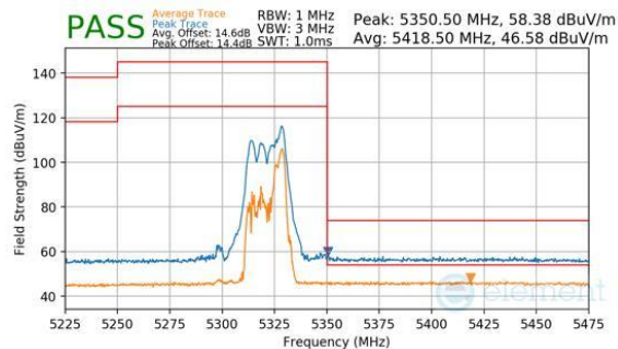
Plot 7-844. CDD Primary (Peak & Average, RU52, Index 40, Ch.64, MCS11)
