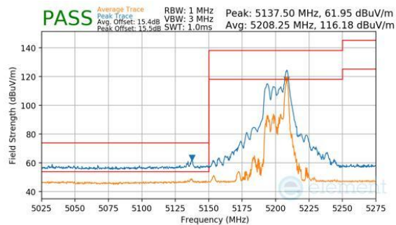
Plot 7-878. CDD Primary (Peak & Average, RU26, Index 17, Ch.38, MCS11)
