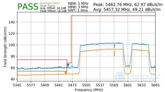
Plot 7-820. Antenna WF7b (Peak & Average, RU996+484+242, Index 97 (H), Ch.114, MCS11)
