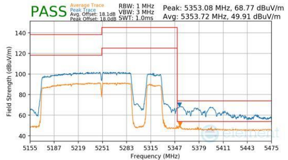
Plot 7-814. Antenna WF7b (Peak & Average, RU996+484+242, Index 98 (H), Ch.50, MCS11)
