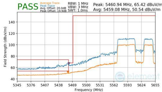
Plot 7-756. Antenna WF7b (Peak & Average, RU484+242, Index 92, Ch.122, MCS11)
