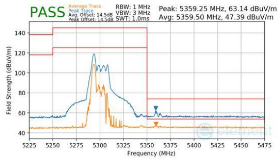
Plot 7-883. CDD Primary (Peak & Average, RU52, Index 37, Ch.62, MCS11)
