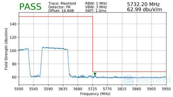
Plot 7-800. Antenna WF7b (Peak, RU996+484, Index 95 (L), Ch.114, MCS11)
