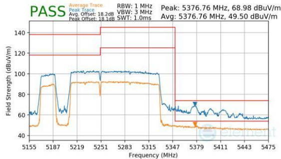
Plot 7-811. Antenna WF7b (Peak & Average, RU996+484+242, Index 97 (L), Ch.50, MCS11)
