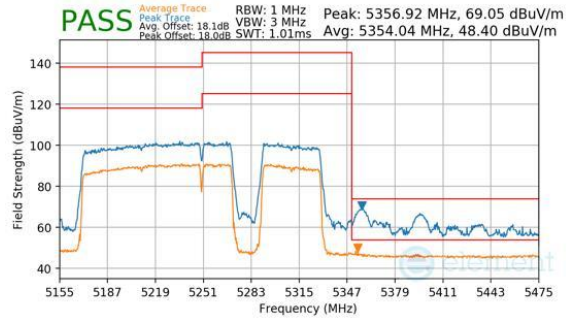
Plot 7-812. Antenna WF7b (Peak & Average, RU996+484+242, Index 97 (H), Ch.50, MCS11)
