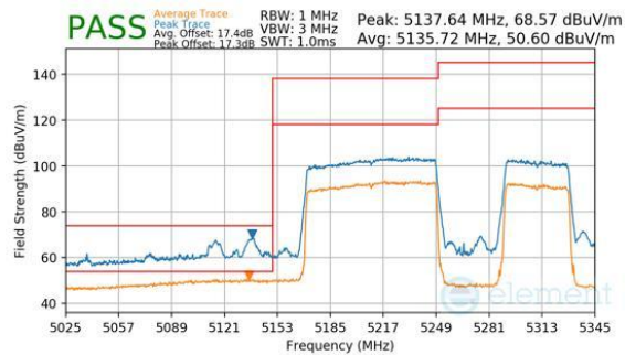
Plot 7-786. Antenna WF7b (Peak & Average, RU996+484, Index 94 (H), Ch.50, MCS11)
