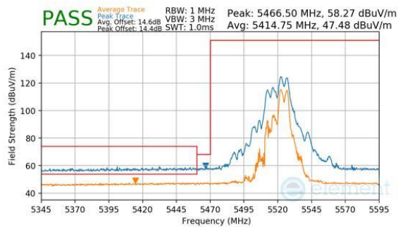
Plot 7-856. CDD Primary (Peak & Average, RU52+26, Index 72, Ch.104, MCS11)
