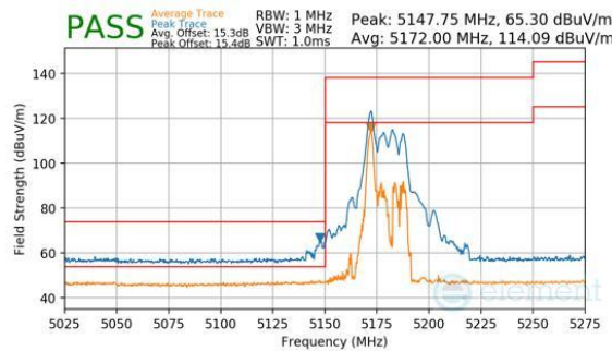
Plot 7-837. CDD Primary (Peak & Average, RU26, Index 0, Ch.36, MCS11)
