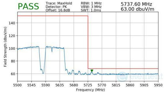
Plot 7-826. Antenna WF7b (Peak, RU996+484+242, Index 96 (H), Ch.114, MCS11)
