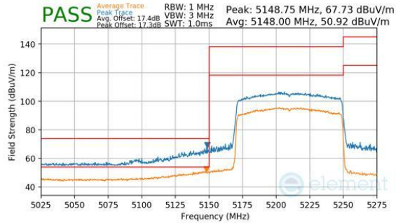
Plot 7-770. Antenna WF7b (Peak & Average, RU996, Index 67, Ch.42, MCS11)
