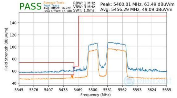
Plot 7-751. Antenna WF7b (Peak & Average, RU484+242, Index 91, Ch.106, MCS11)
