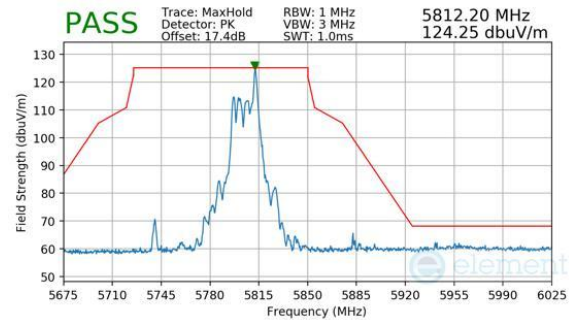
Plot 7-882. CDD Primary (Peak, RU26, Index 17, Ch.159, MCS11)
