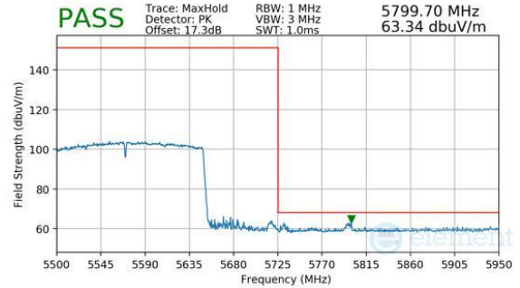
Plot 7-836. Antenna WF7b (Peak, RU996X2, Index 68, Ch.114, MCS11)
