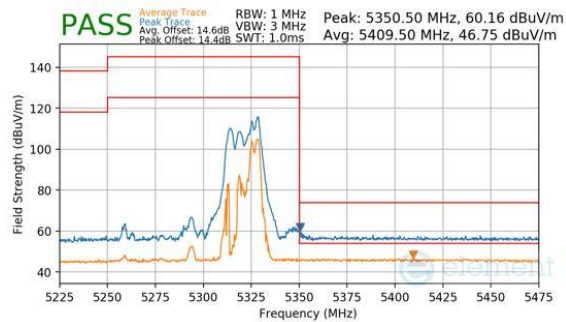
Plot 7-884. CDD Primary (Peak & Average, RU52, Index 44, Ch.62, MCS11)
