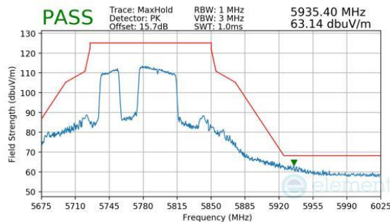
Plot 7-767. Antenna WF7b (Peak, RU484+242, Index 91, Ch.155, MCS11)
