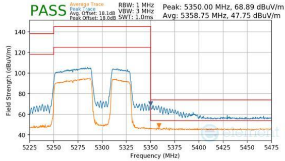
Plot 7-748. Antenna WF7b (Peak & Average, RU484+242, Index 92, Ch.58, MCS11)
