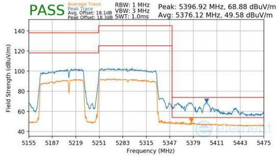
Plot 7-815. Antenna WF7b (Peak & Average, RU996+484+242, Index 99 (L), Ch.50, MCS11)
