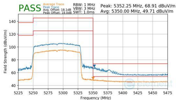
Plot 7-771. Antenna WF7b (Peak & Average, RU996, Index 67, Ch.58, MCS11)
