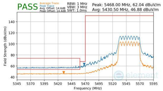
Plot 7-895. CDD Primary (Peak & Average, RU484, Index 65, Ch.110, MCS11)
