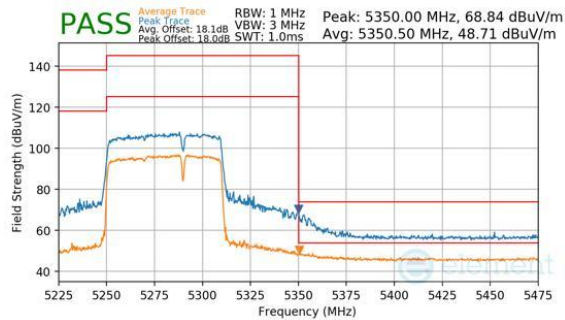
Plot 7-749. Antenna WF7b (Peak & Average, RU484+242, Index 93, Ch.58, MCS11)
