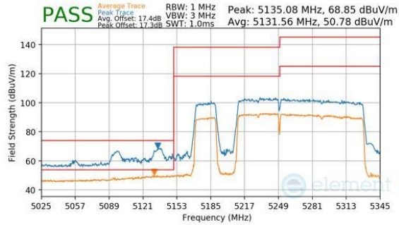
Plot 7-803. Antenna WF7b (Peak & Average, RU996+484+242, Index 97 (L), Ch.50, MCS11)
