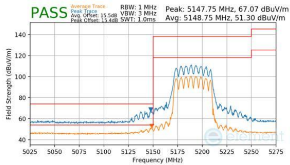
Plot 7-890. CDD Primary (Peak & Average, RU484, Index 65, Ch.38, MCS11)
