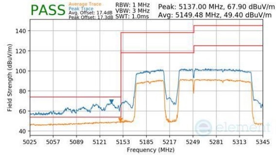
Plot 7-806. Antenna WF7b (Peak & Average, RU996+484+242, Index 98 (L), Ch.50, MCS11)
