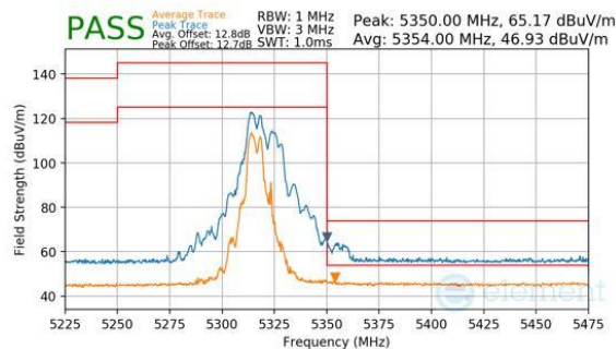
Plot 7-851. CDD Primary (Peak & Average, RU52+26, Index 70, Ch.64, MCS11)
