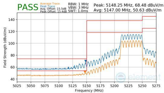
Plot 7-891. CDD Primary (Peak & Average, RU484, Index 65, Ch.46, MCS11)
