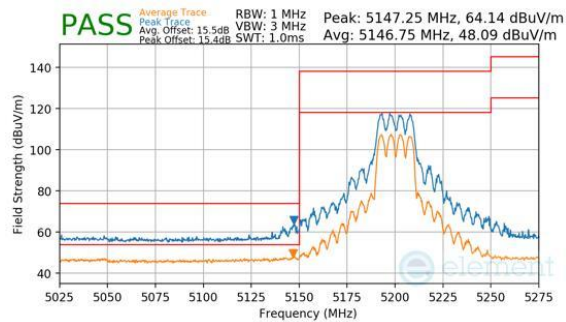
Plot 7-866. CDD Primary (Peak & Average, RU242, Index 61, Ch.40, MCS11)
