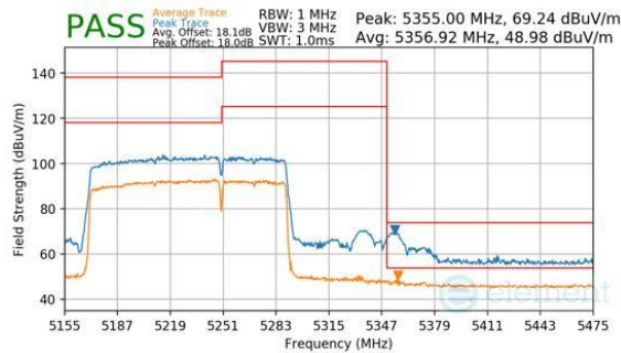
Plot 7-792. Antenna WF7b (Peak & Average, RU996+484, Index 95 (H), Ch.50, MCS11)
