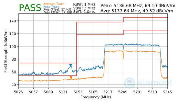
Plot 7-785. Antenna WF7b (Peak & Average, RU996+484, Index 94 (L), Ch.50, MCS11)
