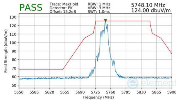
Plot 7-862. CDD Primary (Peak, RU52+26, Index 72, Ch.149, MCS11)
