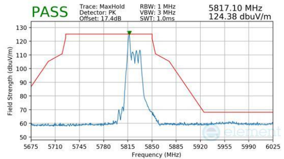
Plot 7-841. CDD Primary (Peak, RU26, Index 0, Ch.165, MCS11)
