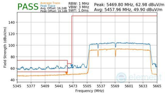
Plot 7-817. Antenna WF7b (Peak & Average, RU996+484+242, Index 96 (L), Ch.114, MCS11)
