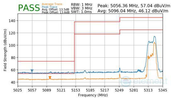
Plot 7-778. Antenna WF7b (Peak & Average, RU52, Index 52 (H), Ch.50, MCS11)
