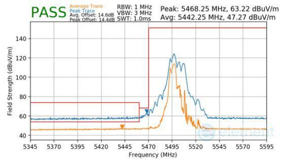
Plot 7-853. CDD Primary (Peak & Average, RU52+26, Index 70, Ch.100, MCS11)
