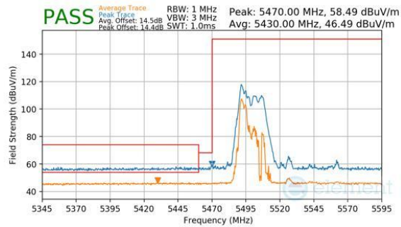
Plot 7-885. CDD Primary (Peak & Average, RU52, Index 37, Ch.102, MCS11)
