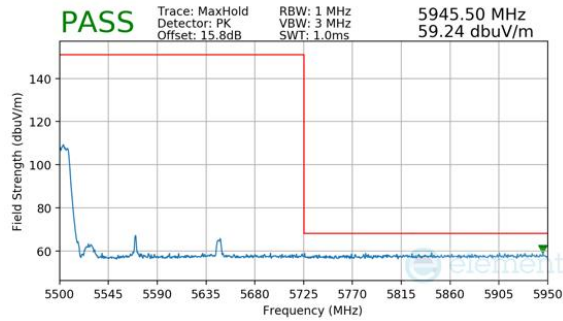
Plot 7-783. Antenna WF7b (Peak, RU52, Index 37 (L), Ch.114, MCS11)
