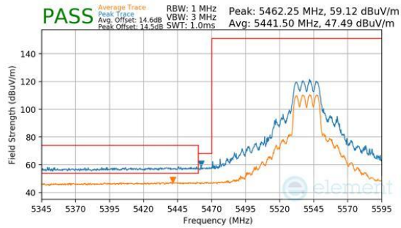
Plot 7-871. CDD Primary (Peak & Average, RU242, Index 61, Ch.108, MCS11)
