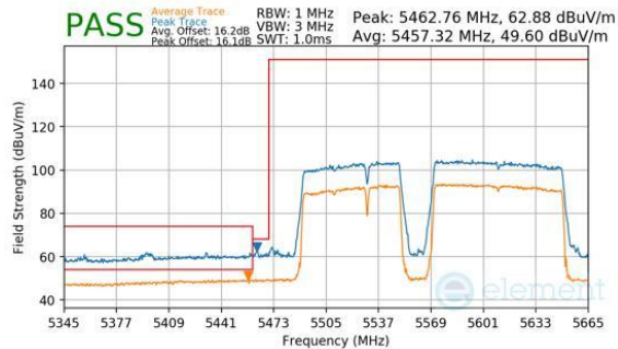
Plot 7-823. Antenna WF7b (Peak & Average, RU996+484+242, Index 99 (L), Ch.114, MCS11)
