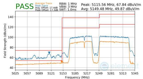
Plot 7-807. Antenna WF7b (Peak & Average, RU996+484+242, Index 99 (L), Ch.50, MCS11)
