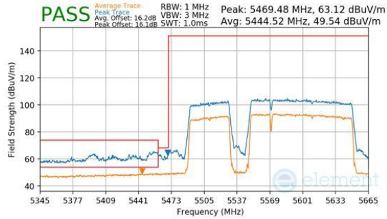
Plot 7-821. Antenna WF7b (Peak & Average, RU996+484+242, Index 98 (L), Ch.114, MCS11)
