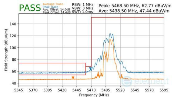
Plot 7-854. CDD Primary (Peak & Average, RU52+26, Index 72, Ch.100, MCS11)
