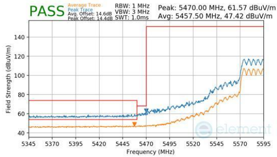
Plot 7-896. CDD Primary (Peak & Average, RU484, Index 65, Ch.118, MCS11)
