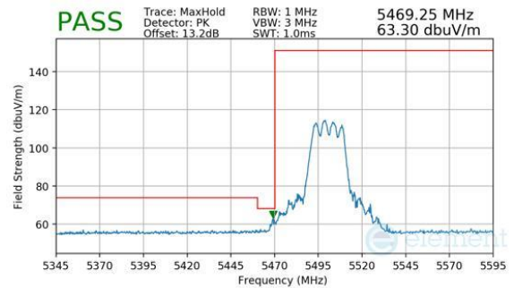
Plot 7-869. CDD Primary (Peak & Average, RU242, Index 61, Ch.100, MCS11)
