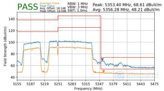
Plot 7-813. Antenna WF7b (Peak & Average, RU996+484+242, Index 98 (L), Ch.50, MCS11)
