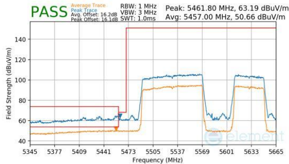
Plot 7-793. Antenna WF7b (Peak & Average, RU996+484, Index 94 (H), Ch.114, MCS11)
