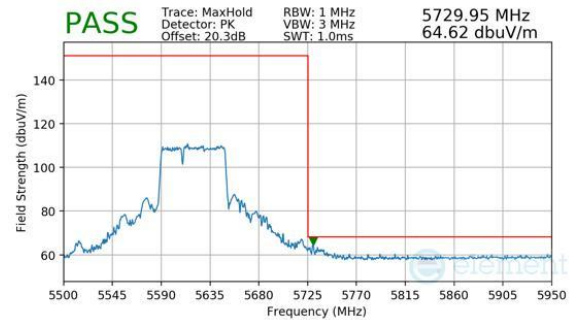
Plot 7-758. Antenna WF7b (Peak, RU484+242, Index 90, Ch.122, MCS11)
