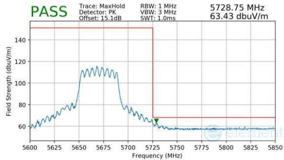
Plot 7-897. CDD Primary (Peak, RU484, Index 65, Ch.134, MCS11)
