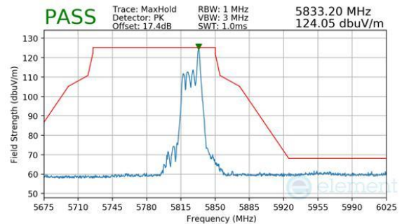
Plot 7-842. CDD Primary (Peak, RU26, Index 8, Ch.165, MCS11)
