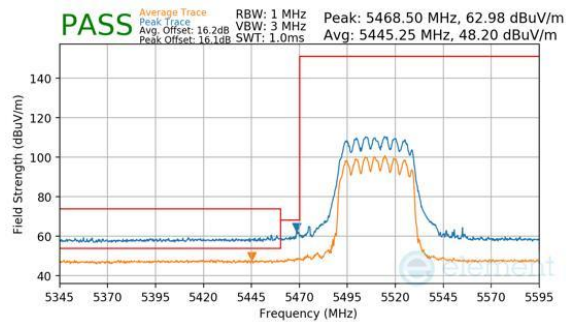
Plot 7-894. CDD Primary (Peak & Average, RU484, Index 65, Ch.102, MCS11)
