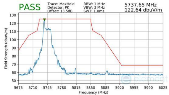
Plot 7-734. Antenna WF7b (Peak, RU26, Index 0, Ch.155, MCS11)
