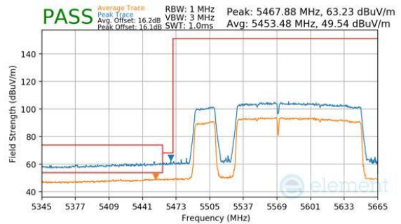
Plot 7-819. Antenna WF7b (Peak & Average, RU996+484+242, Index 97 (L), Ch.114, MCS11)
