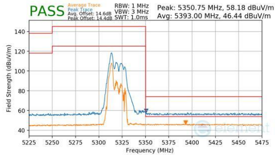
Plot 7-843. CDD Primary (Peak & Average, RU52, Index 37, Ch.64, MCS11)
