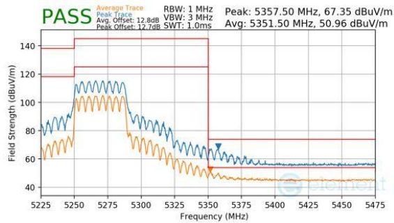
Plot 7-892. CDD Primary (Peak & Average, RU484, Index 65, Ch.54, MCS11)
