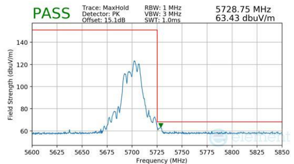
Plot 7-860. CDD Primary (Peak, RU52+26, Index 72, Ch.140, MCS11)
