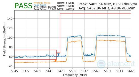
Plot 7-795. Antenna WF7b (Peak & Average, RU996+484, Index 95 (L), Ch.114, MCS11)
