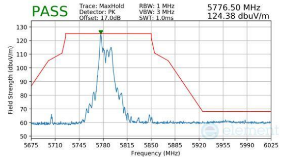
Plot 7-881. CDD Primary (Peak, RU26, Index 0, Ch.159, MCS11)
