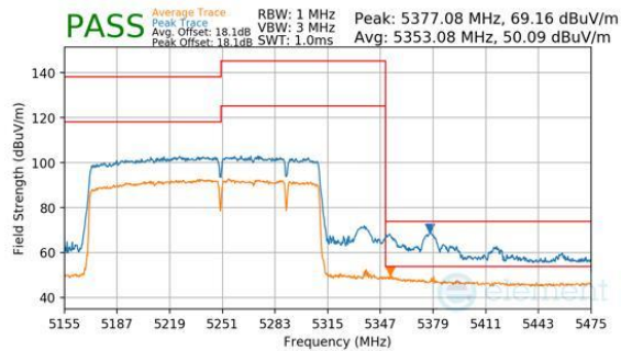
Plot 7-816. Antenna WF7b (Peak & Average, RU996+484+242, Index 99 (H), Ch.50, MCS11)
