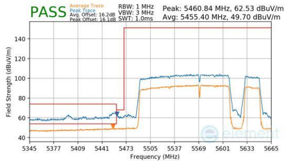
Plot 7-822. Antenna WF7b (Peak & Average, RU996+484+242, Index 98 (H), Ch.114, MCS11)
