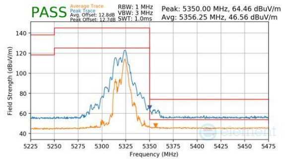
Plot 7-852. CDD Primary (Peak & Average, RU52+26, Index 72, Ch.64, MCS11)
