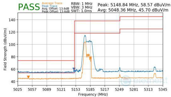
Plot 7-777. Antenna WF7b (Peak & Average, RU52, Index 37 (L), Ch.50, MCS11)
