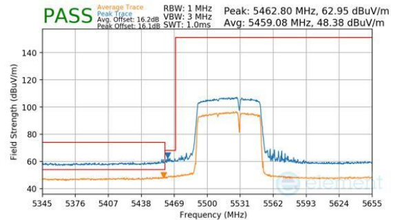
Plot 7-753. Antenna WF7b (Peak & Average, RU484+242, Index 93, Ch.106, MCS11)
