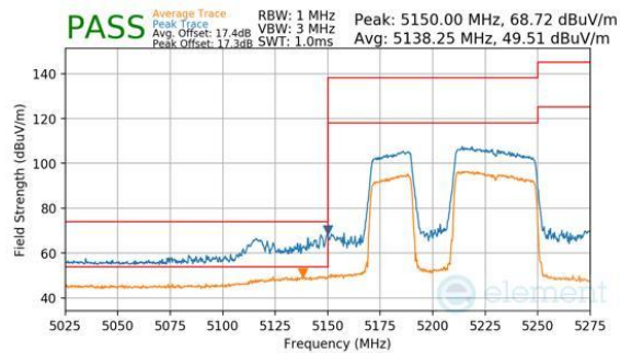
Plot 7-743. Antenna WF7b (Peak & Average, RU484+242, Index 91, Ch.42, MCS11)
