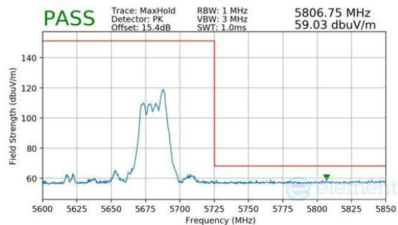
Plot 7-889. CDD Primary (Peak, RU52, Index 44, Ch.134, MCS11)
