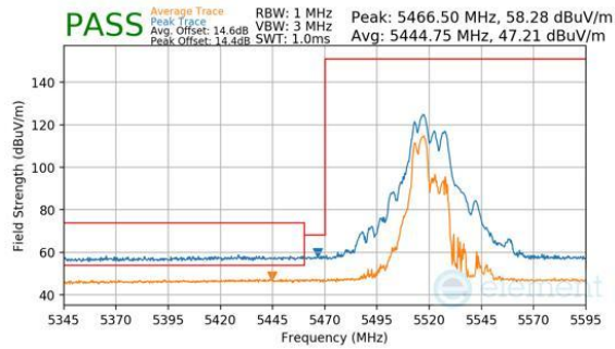
Plot 7-855. CDD Primary (Peak & Average, RU52+26, Index 70, Ch.104, MCS11)
