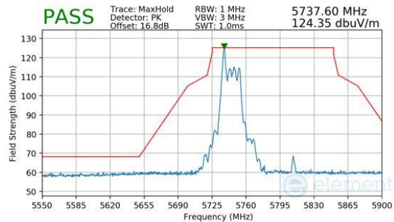
Plot 7-879. CDD Primary (Peak, RU26, Index 0, Ch.151, MCS11)
