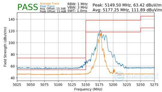
Plot 7-849. CDD Primary (Peak & Average, RU52+26, Index 70, Ch.36, MCS11)
