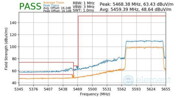
Plot 7-773. Antenna WF7b (Peak & Average, RU996, Index 67, Ch.122, MCS11)
