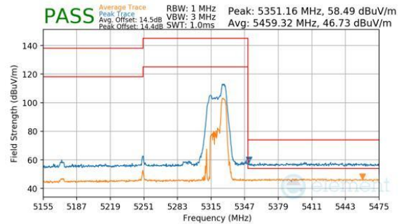
Plot 7-780. Antenna WF7b (Peak & Average, RU52, Index 52 (H), Ch.50, MCS11)
