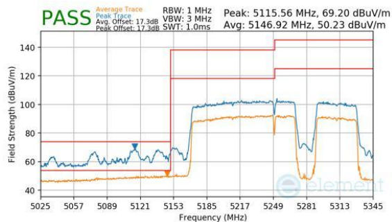
Plot 7-804. Antenna WF7b (Peak & Average, RU996+484+242, Index 97 (H), Ch.50, MCS11)
