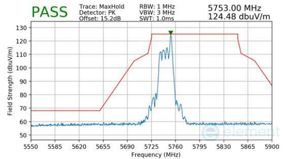
Plot 7-840. CDD Primary (Peak, RU26, Index 8, Ch.149, MCS11)
