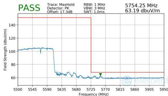
Plot 7-799. Antenna WF7b (Peak, RU996+484, Index 95 (H), Ch.114, MCS11)
