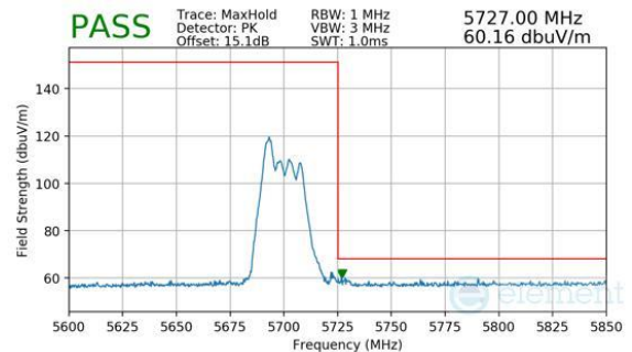
Plot 7-847. CDD Primary (Peak, RU52, Index 37, Ch.140, MCS11)
