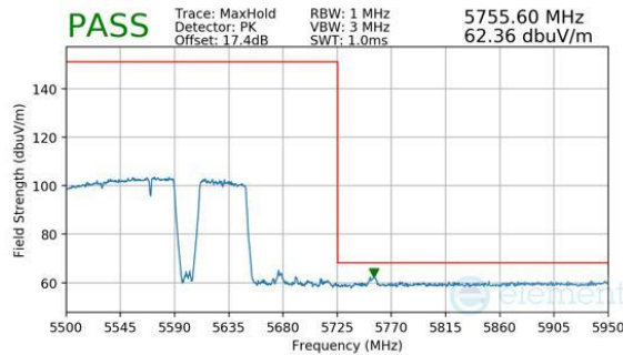
Plot 7-828. Antenna WF7b (Peak, RU996+484+242, Index 97 (H), Ch.114, MCS11)
