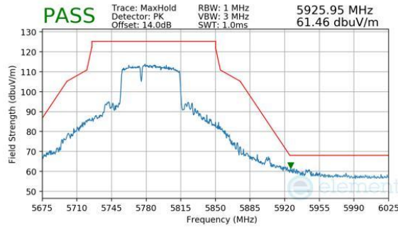
Plot 7-766. Antenna WF7b (Peak, RU484+242, Index 90, Ch.155, MCS11)
