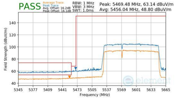
Plot 7-794. Antenna WF7b (Peak & Average, RU996+484, Index 94 (L), Ch.114, MCS11)
