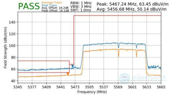
Plot 7-824. Antenna WF7b (Peak & Average, RU996+484+242, Index 99 (H), Ch.114, MCS11)
