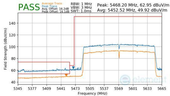
Plot 7-835. Antenna WF7b (Peak & Average, RU996X2, Index 68, Ch.114, MCS11)
