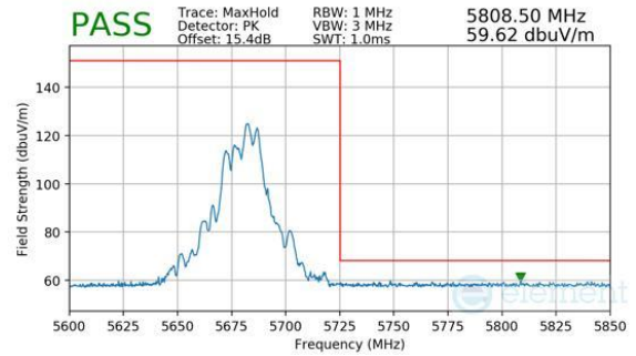
Plot 7-858. CDD Primary (Peak, RU52+26, Index 72, Ch.136, MCS11)
