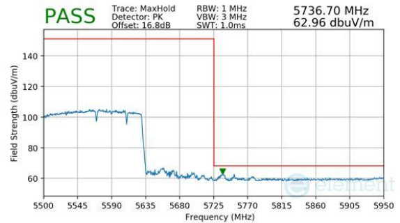
Plot 7-831. Antenna WF7b (Peak, RU996+484+242, Index 99 (H), Ch.114, MCS11)
