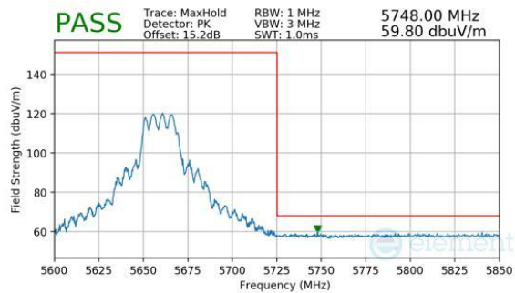
Plot 7-872. CDD Primary (Peak, RU242, Index 61, Ch.132, MCS11)
