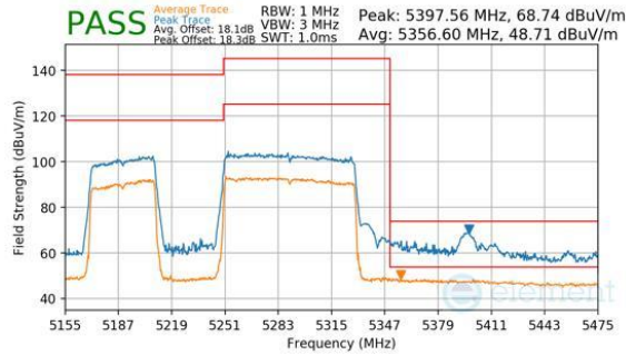
Plot 7-791. Antenna WF7b (Peak & Average, RU996+484, Index 95 (L), Ch.50, MCS11)
