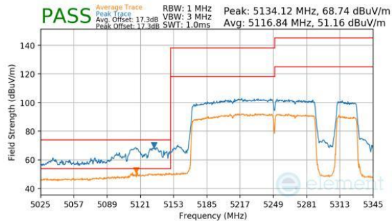
Plot 7-805. Antenna WF7b (Peak & Average, RU996+484+242, Index 98 (H), Ch.50, MCS11)
