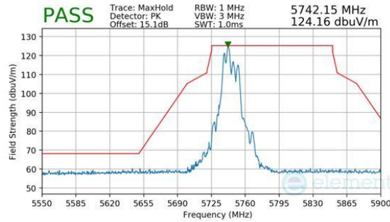
Plot 7-861. CDD Primary (Peak, RU52+26, Index 70, Ch.149, MCS11)
