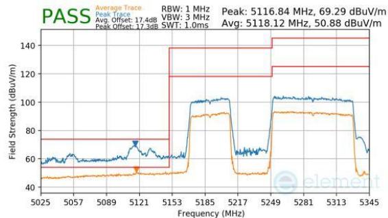
Plot 7-787. Antenna WF7b (Peak & Average, RU996+484, Index 95 (L), Ch.50, MCS11)
