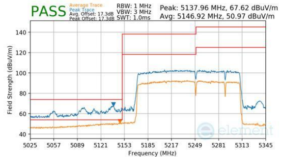
Plot 7-808. Antenna WF7b (Peak & Average, RU996+484+242, Index 99 (H), Ch.50, MCS11)
