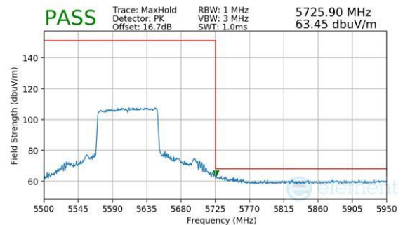
Plot 7-774. Antenna WF7b (Peak, RU996, Index 67, Ch.122, MCS11)
