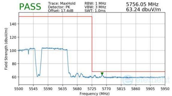
Plot 7-832. Antenna WF7b (Peak, RU996+484+242, Index 99 (L), Ch.114, MCS11)
