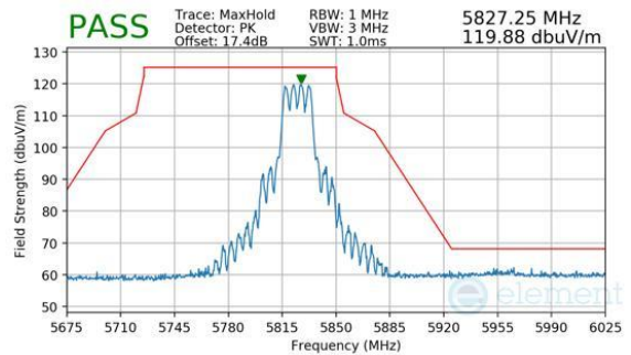
Plot 7-876. CDD Primary (Peak, RU242, Index 61, Ch.165, MCS11)
