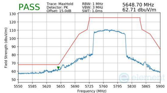
Plot 7-775. Antenna WF7b (Peak, RU996, Index 67, Ch.155, MCS11)
