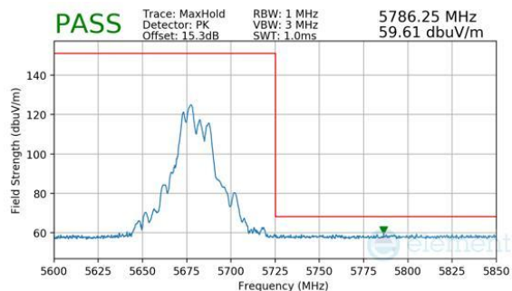
Plot 7-857. CDD Primary (Peak, RU52+26, Index 70, Ch.136, MCS11)
