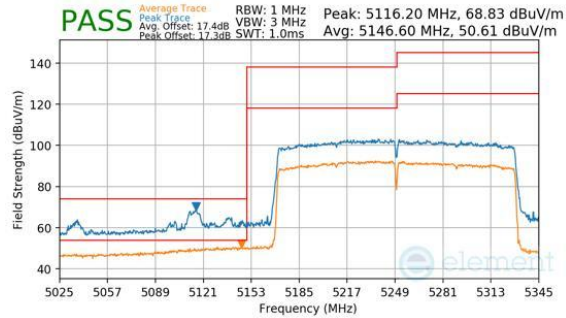
Plot 7-833. Antenna WF7b (Peak & Average, RU996X2, Index 68, Ch.50, MCS11)
