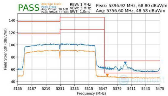
Plot 7-834. Antenna WF7b (Peak & Average, RU996X2, Index 68, Ch.50, MCS11)
