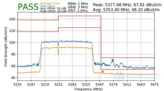
Plot 7-790. Antenna WF7b (Peak & Average, RU996+484, Index 94 (L), Ch.50, MCS11)
