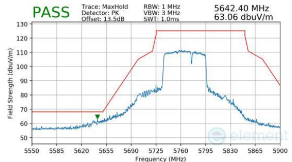
Plot 7-765. Antenna WF7b (Peak, RU484+242, Index 93, Ch.155, MCS11)
