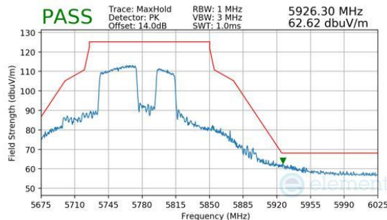
Plot 7-768. Antenna WF7b (Peak, RU484+242, Index 92, Ch.155, MCS11)
