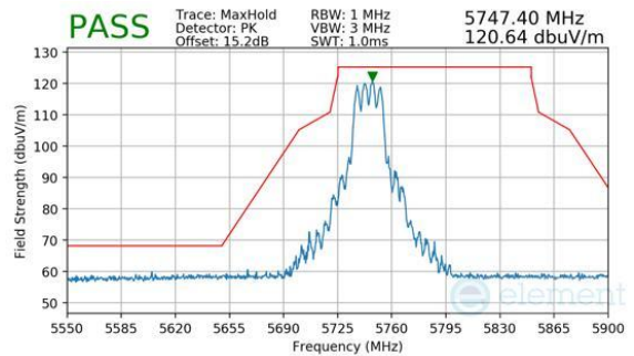
Plot 7-875. CDD Primary (Peak, RU242, Index 61, Ch.149, MCS11)
