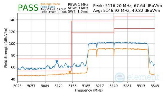
Plot 7-802. Antenna WF7b (Peak & Average, RU996+484+242, Index 96 (L), Ch.50, MCS11)
