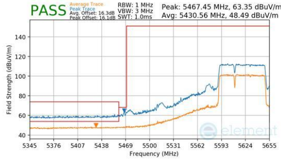
Plot 7-754. Antenna WF7b (Peak & Average, RU484+242, Index 90, Ch.122, MCS11)
