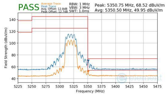
Plot 7-868. CDD Primary (Peak & Average, RU242, Index 61, Ch.64, MCS11)
