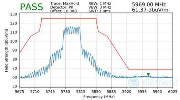
Plot 7-899. CDD Primary (Peak, RU484, Index 65, Ch.159, MCS11)
