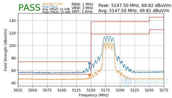
Plot 7-865. CDD Primary (Peak & Average, RU242, Index 61, Ch.36, MCS11)
