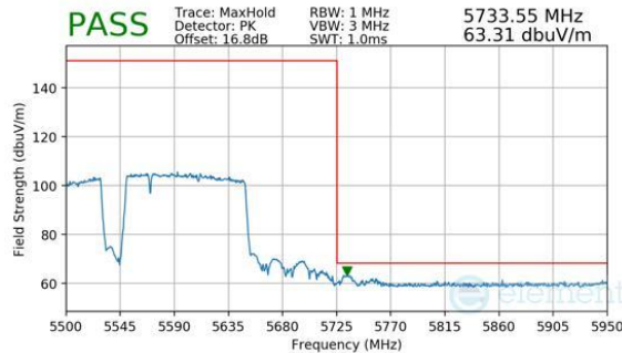
Plot 7-829. Antenna WF7b (Peak, RU996+484+242, Index 98 (L), Ch.114, MCS11)
