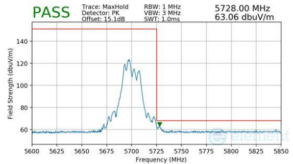
Plot 7-859. CDD Primary (Peak, RU52+26, Index 70, Ch.140, MCS11)
