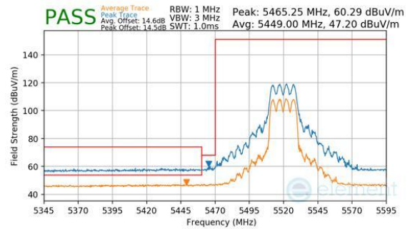
Plot 7-870. CDD Primary (Peak & Average, RU242, Index 61, Ch.104, MCS11)
