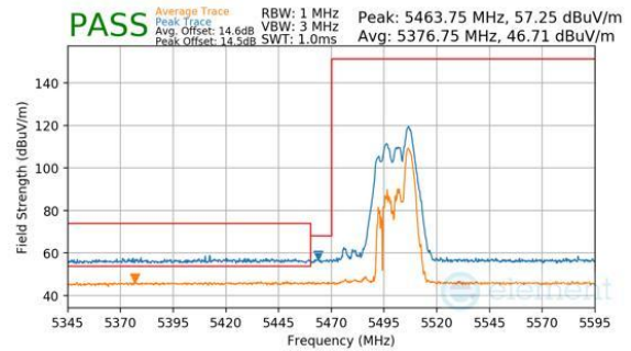
Plot 7-846. CDD Primary (Peak & Average, RU52, Index 40, Ch.100, MCS11)
