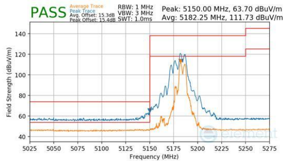
Plot 7-850. CDD Primary (Peak & Average, RU52+26, Index 72, Ch.36, MCS11)
