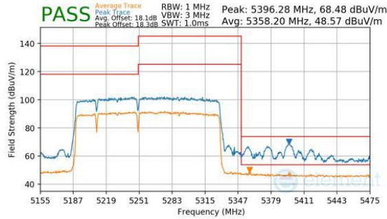
Plot 7-809. Antenna WF7b (Peak & Average, RU996+484+242, Index 96 (L), Ch.50, MCS11)
