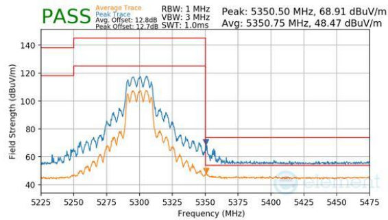
Plot 7-867. CDD Primary (Peak & Average, RU242, Index 61, Ch.60, MCS11)
