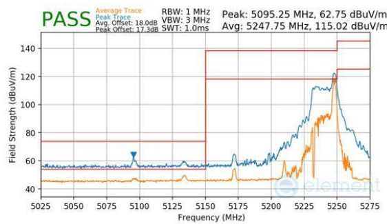
Plot 7-731. Antenna WF7b (Peak & Average, RU26, Index 36, Ch.42, MCS11)
