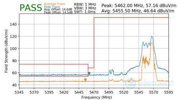
Plot 7-887. CDD Primary (Peak & Average, RU52, Index 44, Ch.110, MCS11)
