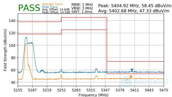
Plot 7-779. Antenna WF7b (Peak & Average, RU52, Index 37 (L), Ch.50, MCS11)
