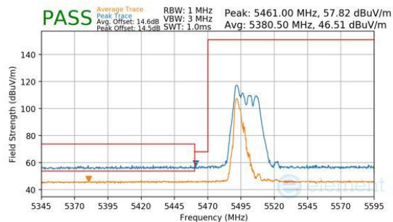
Plot 7-845. CDD Primary (Peak & Average, RU52, Index 37, Ch.100, MCS11)
