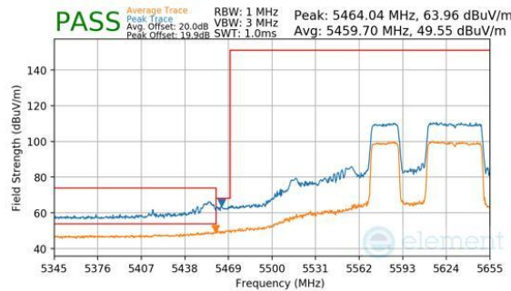
Plot 7-755. Antenna WF7b (Peak & Average, RU484+242, Index 91, Ch.122, MCS11)
