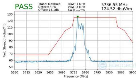
Plot 7-839. CDD Primary (Peak, RU26, Index 0, Ch.149, MCS11)
