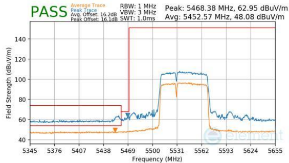
Plot 7-750. Antenna WF7b (Peak & Average, RU484+242, Index 90, Ch.106, MCS11)
