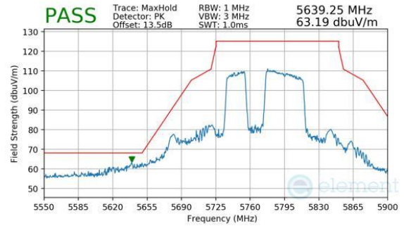
Plot 7-763. Antenna WF7b (Peak, RU484+242, Index 91, Ch.155, MCS11)
