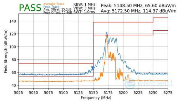
Plot 7-877. CDD Primary (Peak & Average, RU26, Index 0, Ch.38, MCS11)
