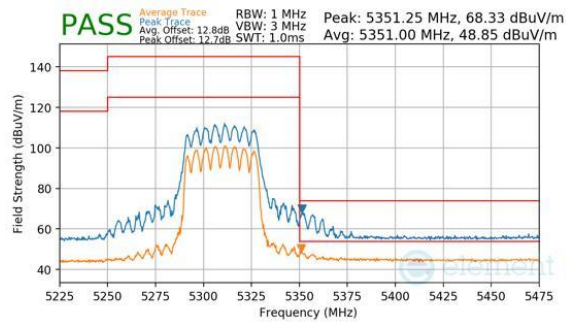
Plot 7-893. CDD Primary (Peak & Average, RU484, Index 65, Ch.62, MCS11)
