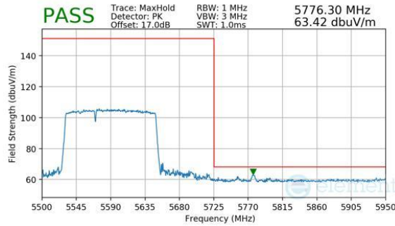
Plot 7-797. Antenna WF7b (Peak, RU996+484, Index 94 (L), Ch.114, MCS11)
