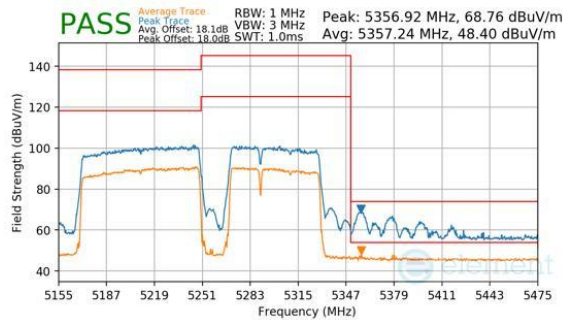
Plot 7-810. Antenna WF7b (Peak & Average, RU996+484+242, Index 96 (H), Ch.50, MCS11)
