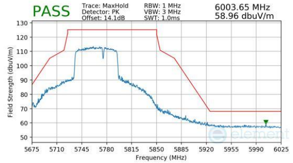
Plot 7-769. Antenna WF7b (Peak, RU484+242, Index 93, Ch.155, MCS11)
