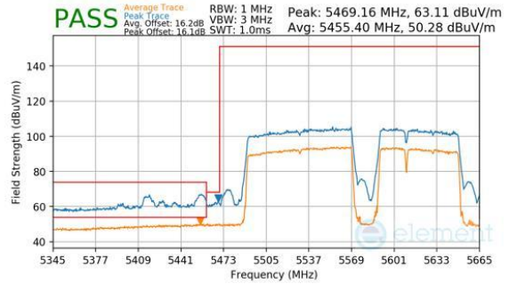
Plot 7-818. Antenna WF7b (Peak & Average, RU996+484+242, Index 96 (H), Ch.114, MCS11)
