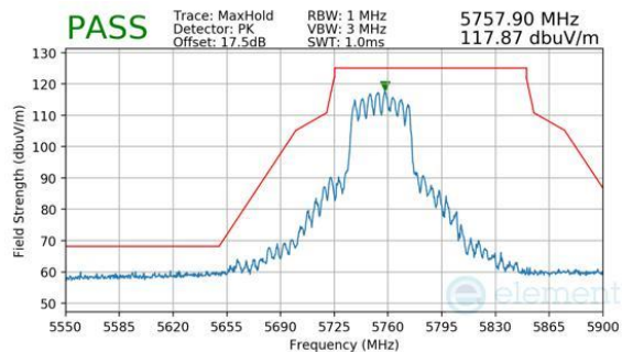
Plot 7-898. CDD Primary (Peak, RU484, Index 65, Ch.151, MCS11)
