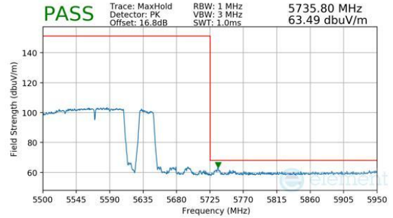
Plot 7-830. Antenna WF7b (Peak, RU996+484+242, Index 98 (H), Ch.114, MCS11)
