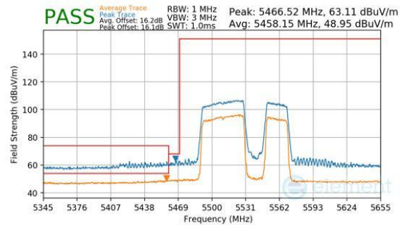
Plot 7-752. Antenna WF7b (Peak & Average, RU484+242, Index 92, Ch.106, MCS11)
