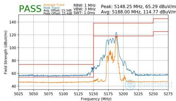
Plot 7-838. CDD Primary (Peak & Average, RU26, Index 8, Ch.36, MCS11)
