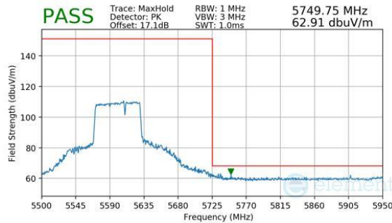
Plot 7-761. Antenna WF7b (Peak, RU484+242, Index 93, Ch.122, MCS11)
