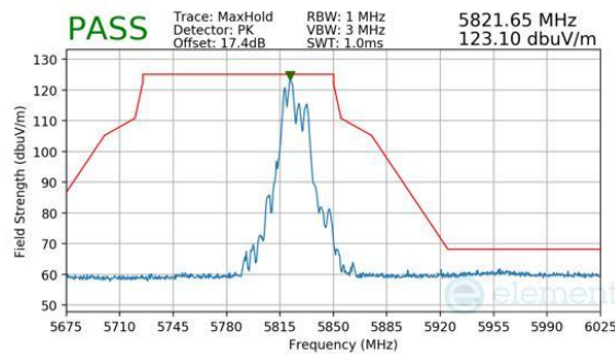
Plot 7-863. CDD Primary (Peak, RU52+26, Index 70, Ch.165, MCS11)
