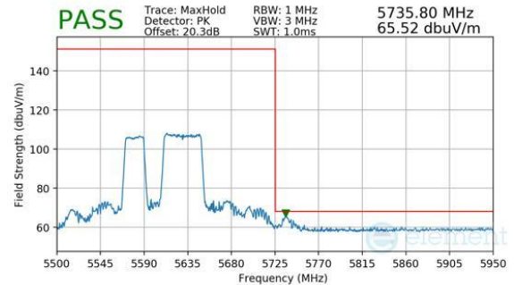
Plot 7-759. Antenna WF7b (Peak, RU484+242, Index 91, Ch.122, MCS11)
