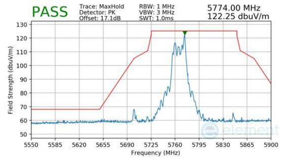
Plot 7-880. CDD Primary (Peak, RU26, Index 17, Ch.151, MCS11)
