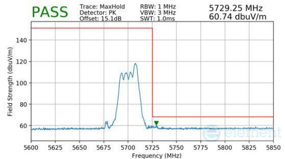
Plot 7-848. CDD Primary (Peak, RU52, Index 40, Ch.140, MCS11)
