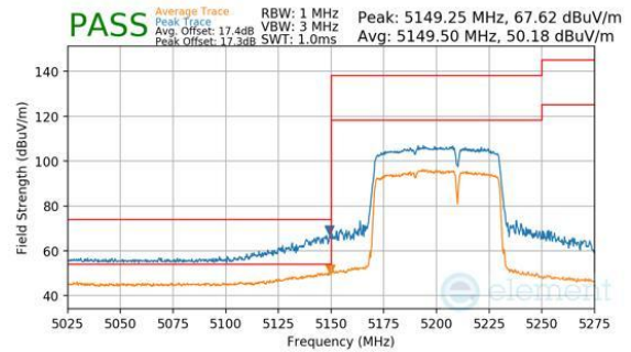
Plot 7-745. Antenna WF7b (Peak & Average, RU484+242, Index 93, Ch.42, MCS11)
