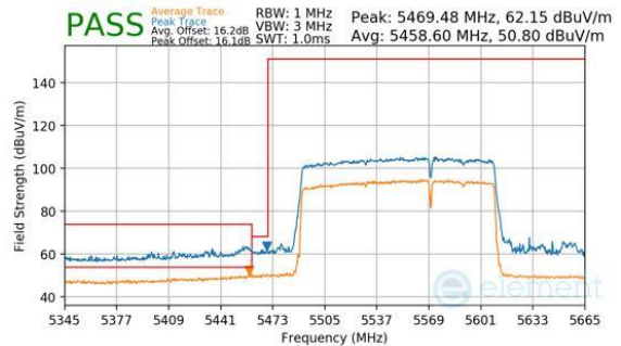
Plot 7-796. Antenna WF7b (Peak & Average, RU996+484, Index 95 (H), Ch.114, MCS11)
