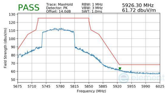
Plot 7-776. Antenna WF7b (Peak, RU996, Index 67, Ch.155, MCS11)
