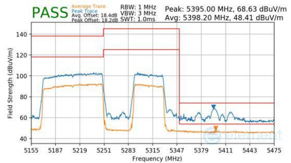
Plot 7-789. Antenna WF7b (Peak & Average, RU996+484, Index 94 (H), Ch.50, MCS11)
