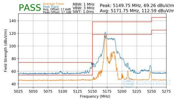
Plot 7-730. Antenna WF7b (Peak & Average, RU26, Index 0, Ch.42, MCS11)
