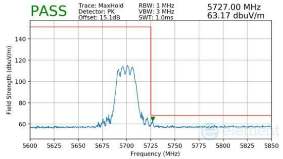
Plot 7-874. CDD Primary (Peak, RU242, Index 61, Ch.140, MCS11)
