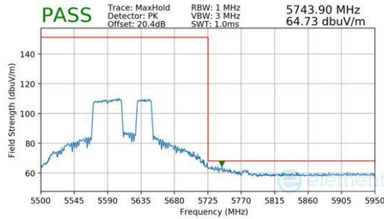
Plot 7-760. Antenna WF7b (Peak, RU484+242, Index 92, Ch.122, MCS11)
