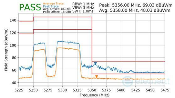
Plot 7-747. Antenna WF7b (Peak & Average, RU484+242, Index 91, Ch.58, MCS11)
