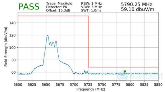
Plot 7-888. CDD Primary (Peak, RU52, Index 37, Ch.134, MCS11)
