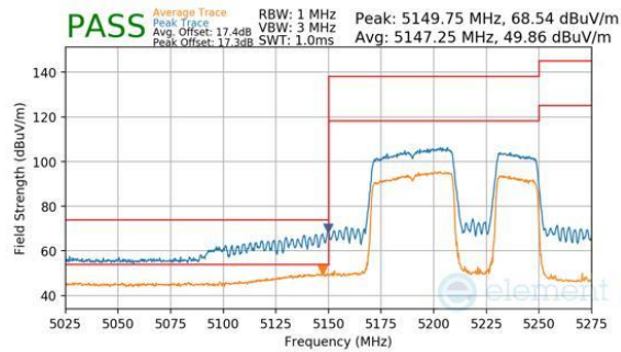
Plot 7-744. Antenna WF7b (Peak & Average, RU484+242, Index 92, Ch.42, MCS11)
