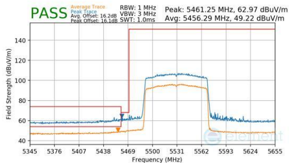
Plot 7-772. Antenna WF7b (Peak & Average, RU996, Index 67, Ch.106, MCS11)
