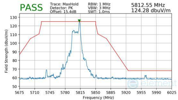
Plot 7-735. Antenna WF7b (Peak, RU26, Index 36, Ch.155, MCS11)
