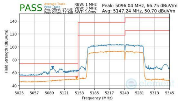
Plot 7-788. Antenna WF7b (Peak & Average, RU996+484, Index 95 (H), Ch.50, MCS11)
