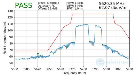
Plot 7-764. Antenna WF7b (Peak, RU484+242, Index 92, Ch.155, MCS11)
