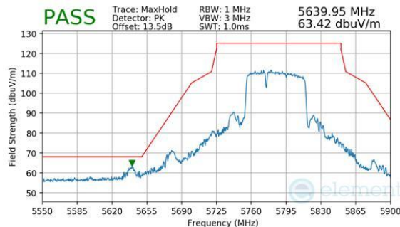
Plot 7-762. Antenna WF7b (Peak, RU484+242, Index 90, Ch.155, MCS11)
