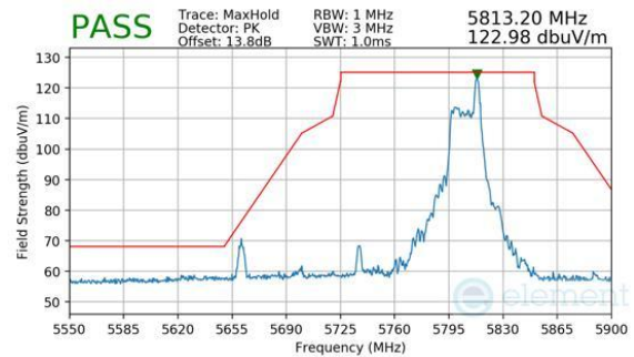
Plot 7-733. Antenna WF7b (Peak, RU26, Index 36, Ch.155, MCS11)
