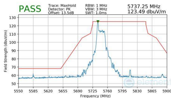
Plot 7-732. Antenna WF7b (Peak, RU26, Index 0, Ch.155, MCS11)
