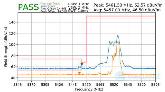
Plot 7-886. CDD Primary (Peak & Average, RU52, Index 44, Ch.102, MCS11)
