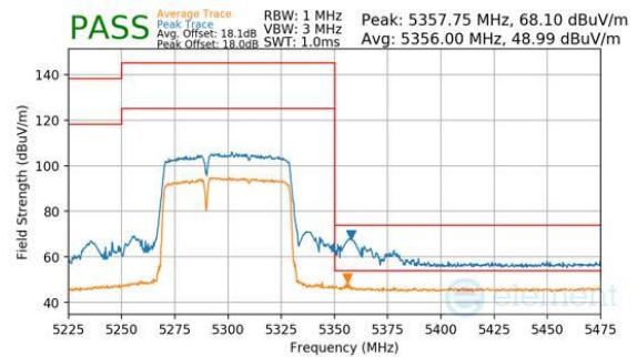
Plot 7-746. Antenna WF7b (Peak & Average, RU484+242, Index 90, Ch.58, MCS11)
