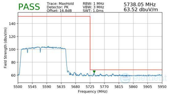
Plot 7-825. Antenna WF7b (Peak, RU996+484+242, Index 96 (L), Ch.114, MCS11)
