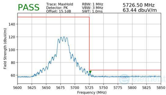
Plot 7-873. CDD Primary (Peak, RU242, Index 61, Ch.136, MCS11)
