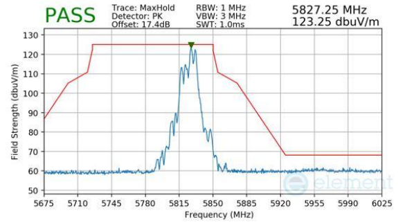
Plot 7-864. CDD Primary (Peak, RU52+26, Index 72, Ch.165, MCS11)
