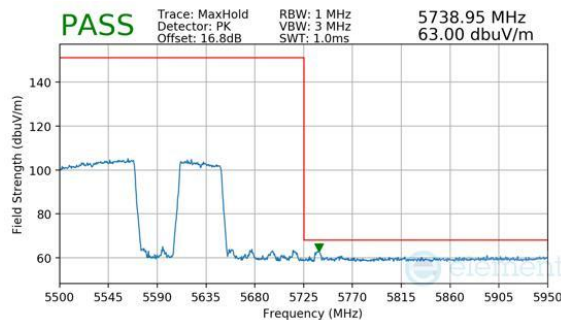
Plot 7-798. Antenna WF7b (Peak, RU996+484, Index 94 (H), Ch.114, MCS11)
