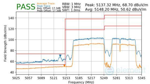
Plot 7-801. Antenna WF7b (Peak & Average, RU996+484+242, Index 96 (H), Ch.50, MCS11)
