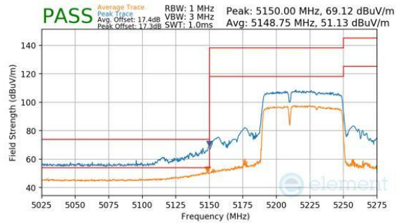
Plot 7-742. Antenna WF7b (Peak & Average, RU484+242, Index 90, Ch.42, MCS11)
