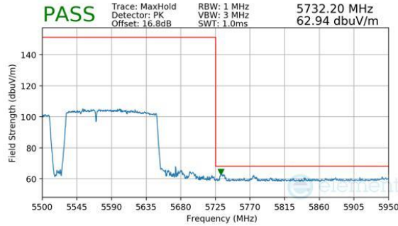
Plot 7-827. Antenna WF7b (Peak, RU996+484+242, Index 97 (L), Ch.114, MCS11)
