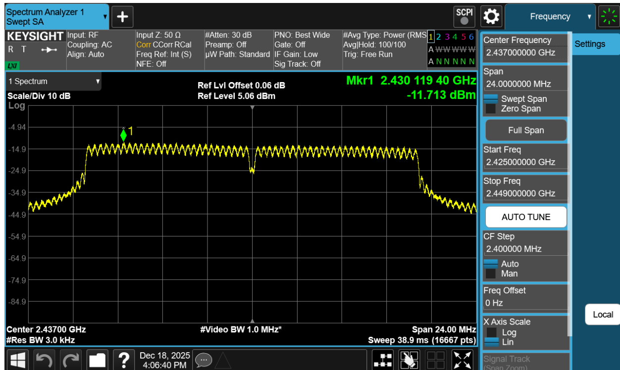
Plot 7-18 PSD Antenna WF7b (20MHz BW 802.11g - Ch.6)
