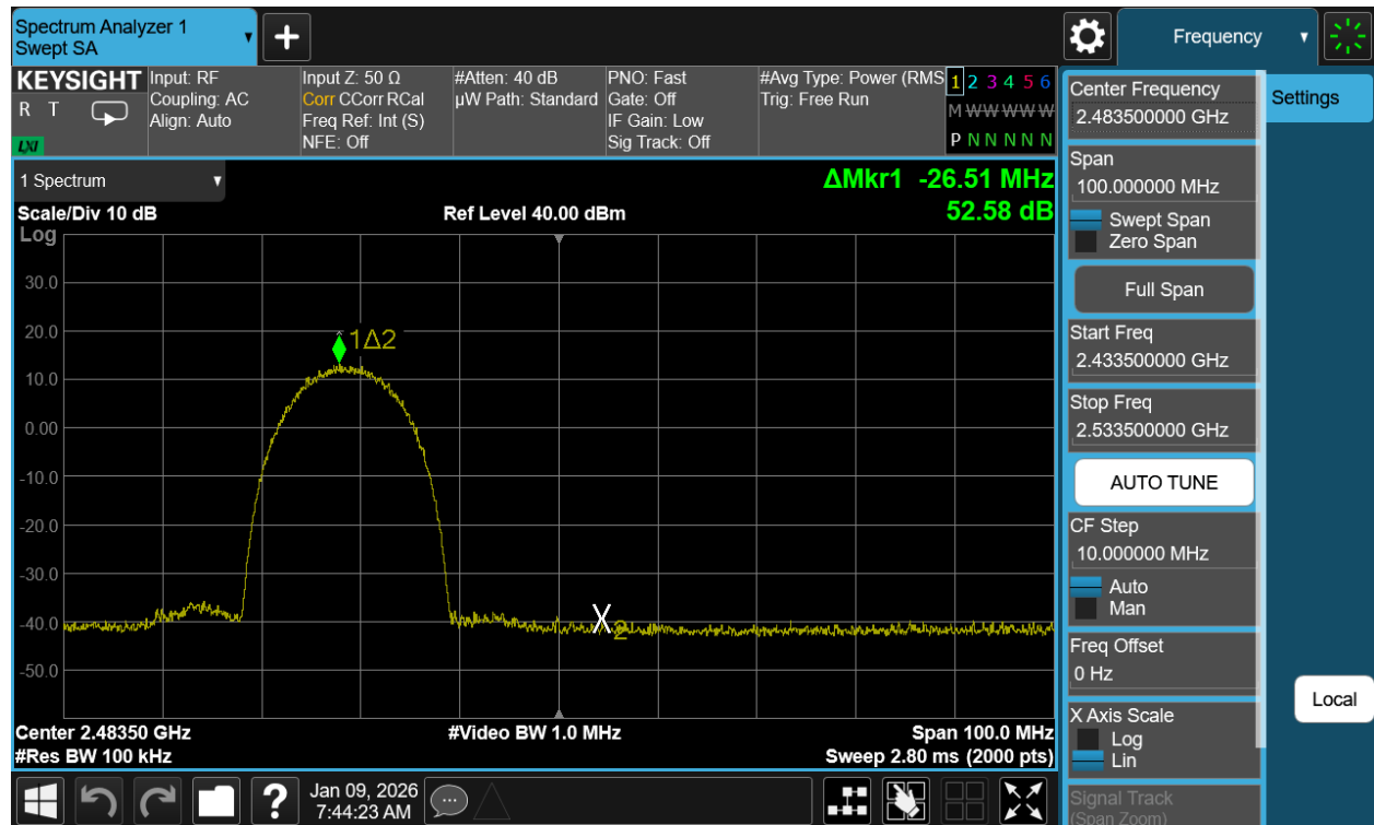
Plot 7-37. Band Edge Plot Antenna WF7b (802.11b – Ch. 11)
