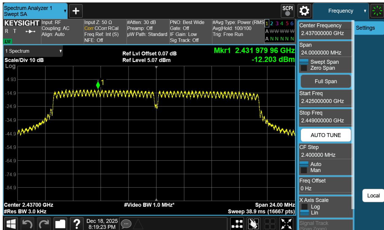
Plot 7-28 PSD CDD Antenna WF2b (20MHz BW 802.11g - Ch.6)
