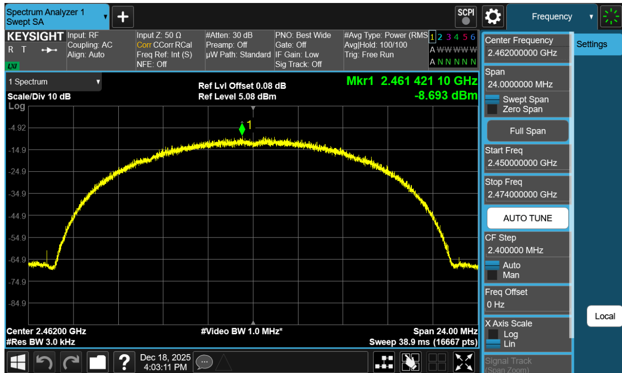
Plot 7-17 PSD Antenna WF7b (20MHz BW 802.11b - Ch.11)
