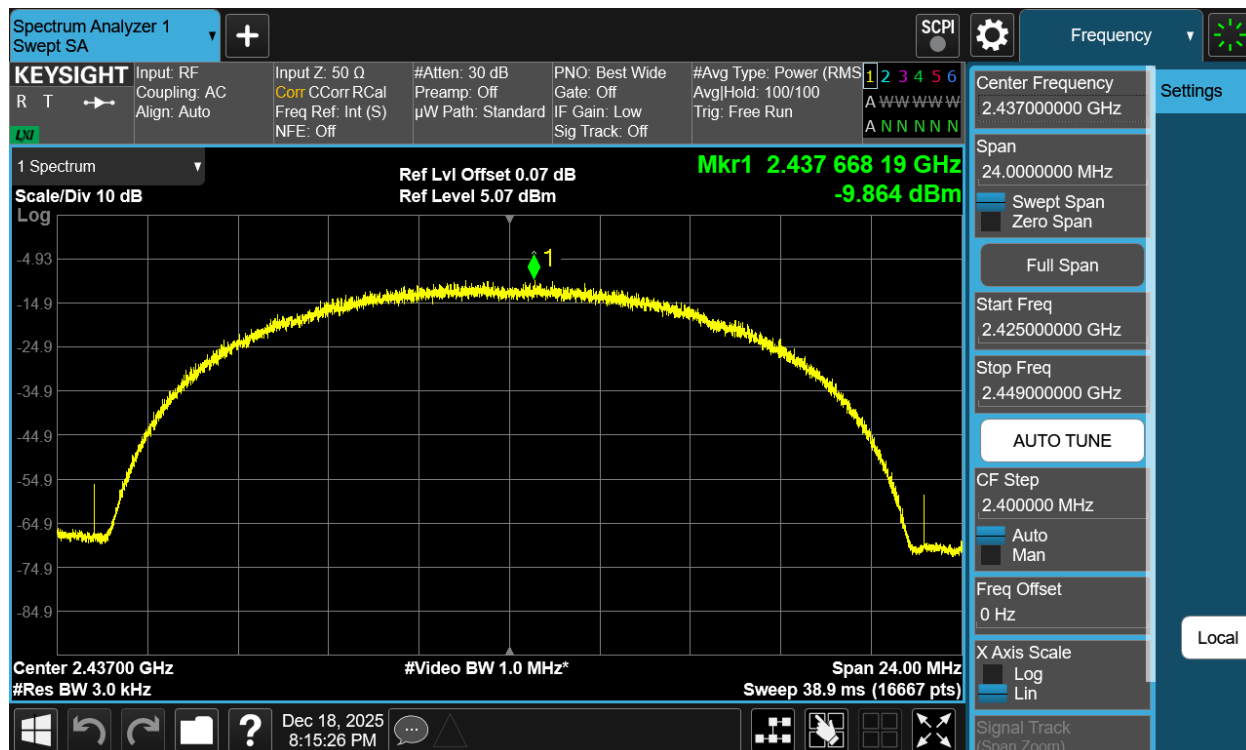
Plot 7-26 PSD CDD Antenna WF2b (20MHz BW 802.11b - Ch.6)
