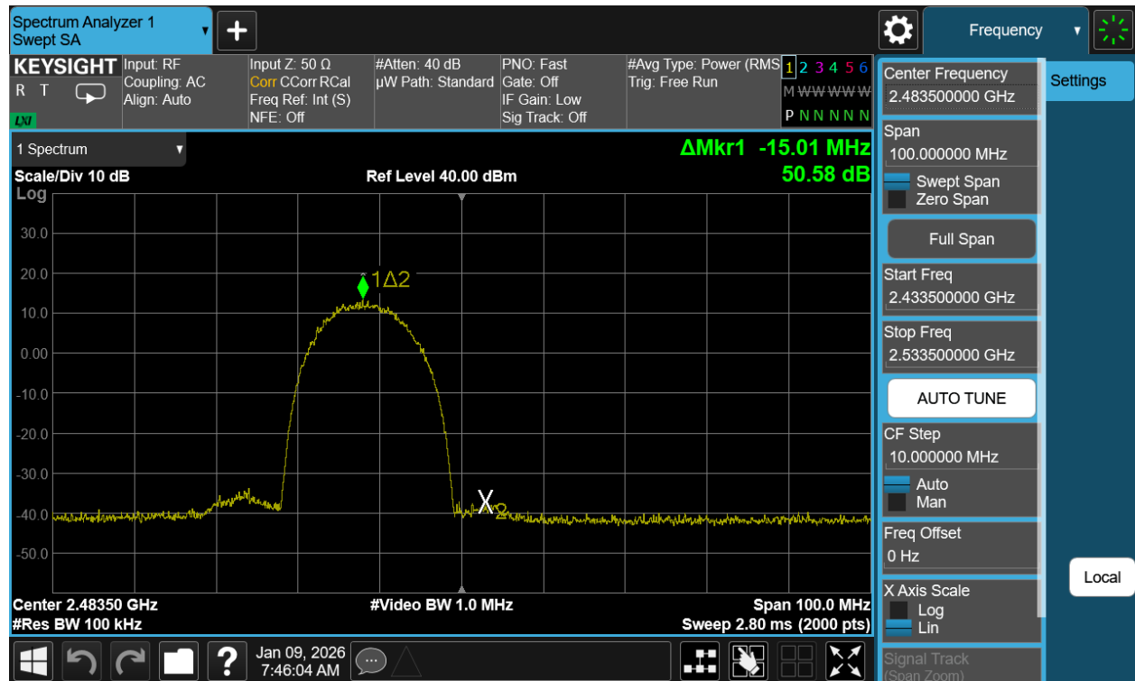
Plot 7-39. Band Edge Plot Antenna WF7b (802.11b – Ch. 13)
