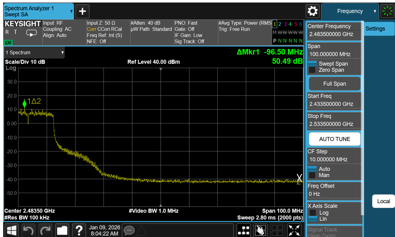
Plot 7-46. Band Edge Plot Antenna WF7b (802.11g - Ch. 6)
