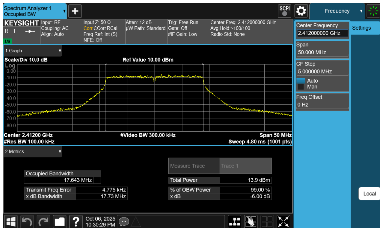
Plot 7-10 6dB OBW Antenna WF7b (20MHz BW 802.11g - Ch.1)
