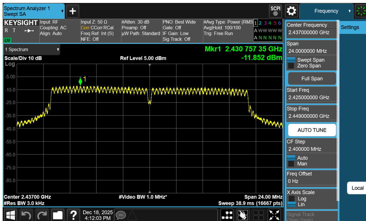
Plot 7-19 PSD Antenna WF7b (20MHz BW 802.11n - Ch.6)
