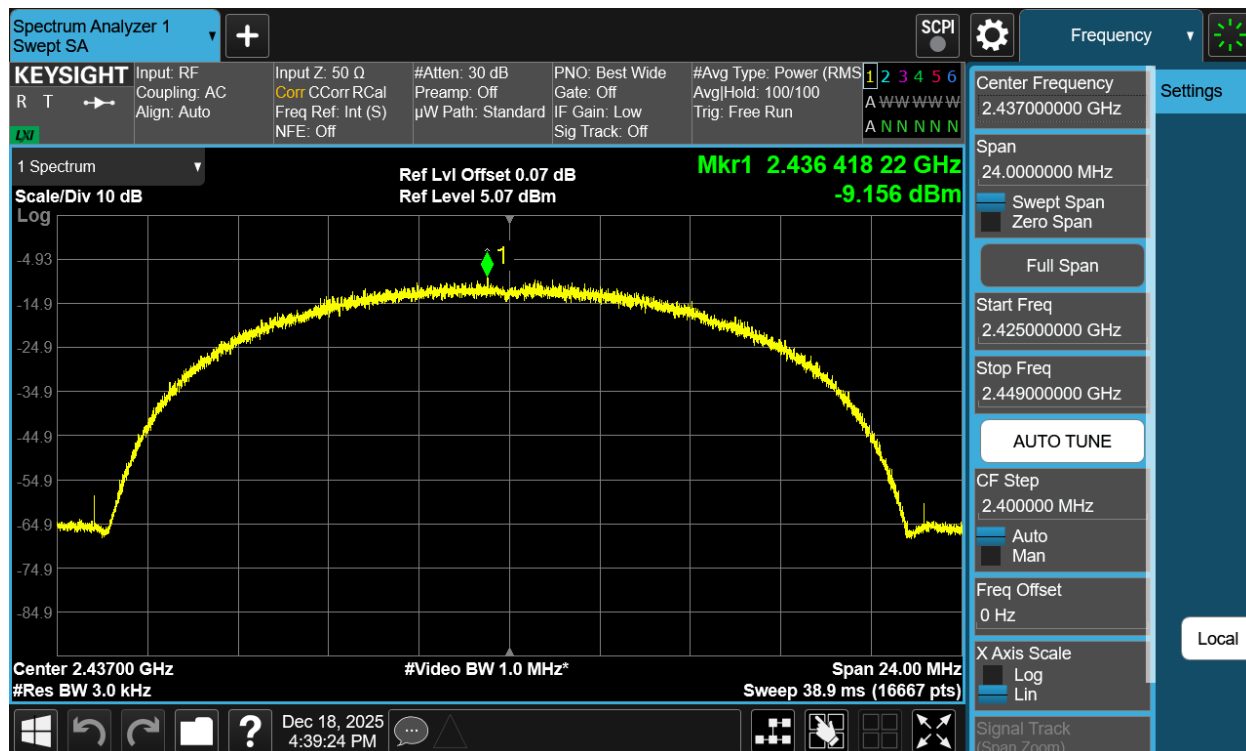
Plot 7-25 PSD CDD Antenna WF7b (20MHz BW 802.11b - Ch.6)
