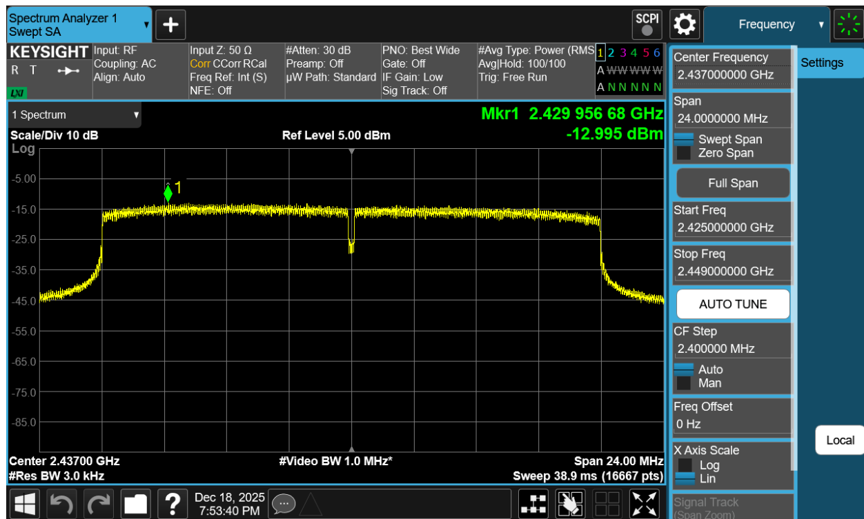
Plot 7-24 PSD Antenna WF2b (20MHz BW 802.11be(SU) - Ch.6)
