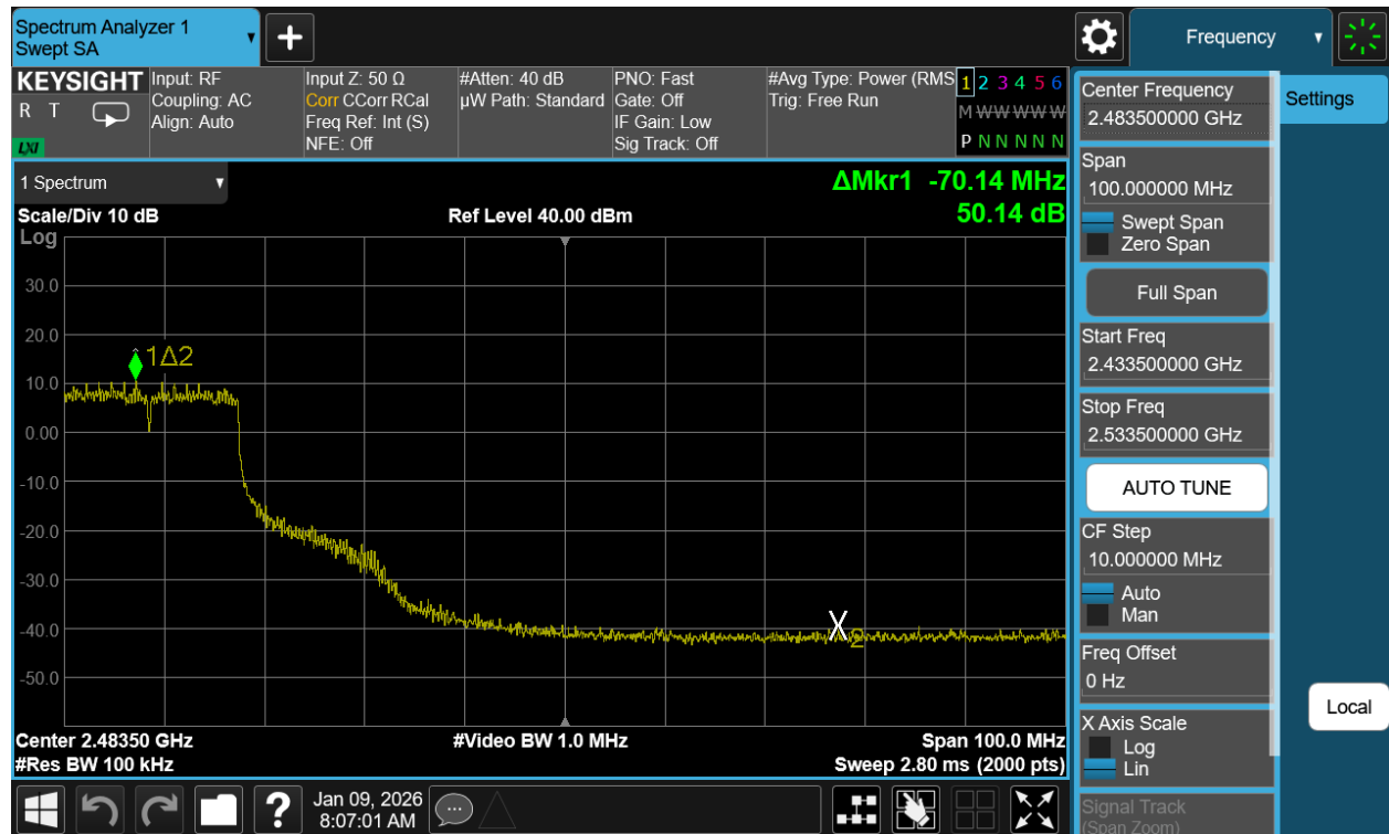
Plot 7-47. Band Edge Plot Antenna WF7b (802.11g - Ch. 7)
