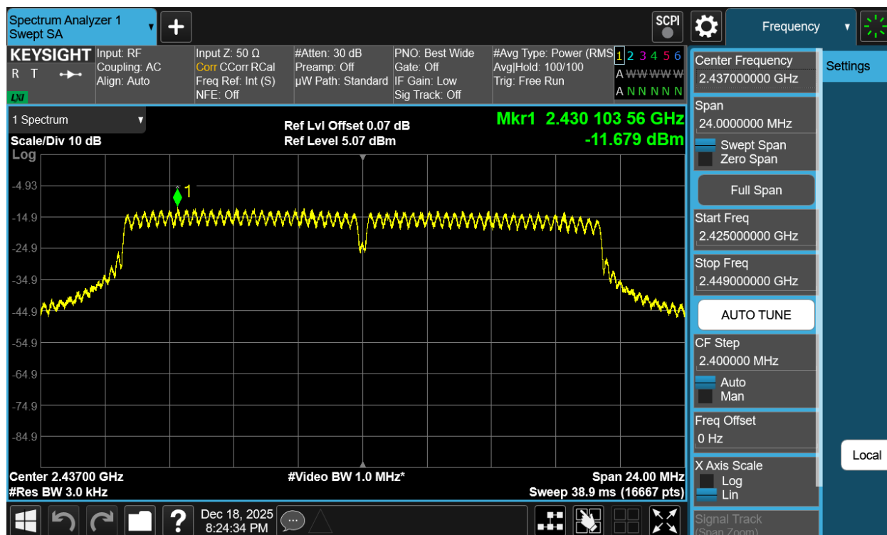
Plot 7-30 PSD CDD Antenna WF2b (20MHz BW 802.11n - Ch.6)
