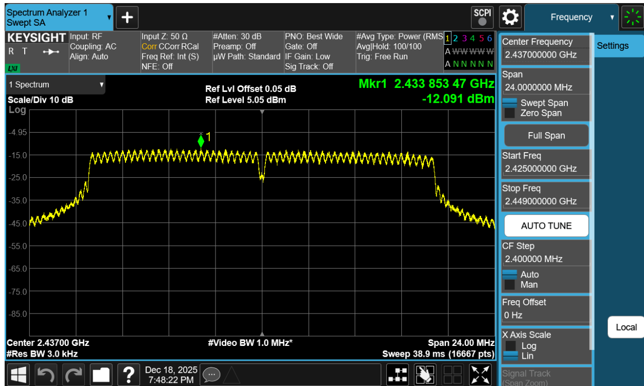
Plot 7-23 PSD Antenna WF2b (20MHz BW 802.11n - Ch.6)
