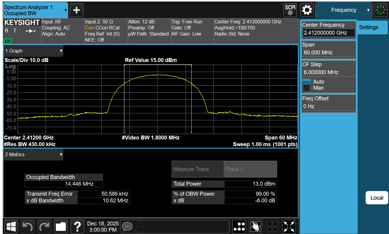
Plot 7-1 99% OBW Antenna WF7b (20MHz BW 802.11b - Ch.1)
