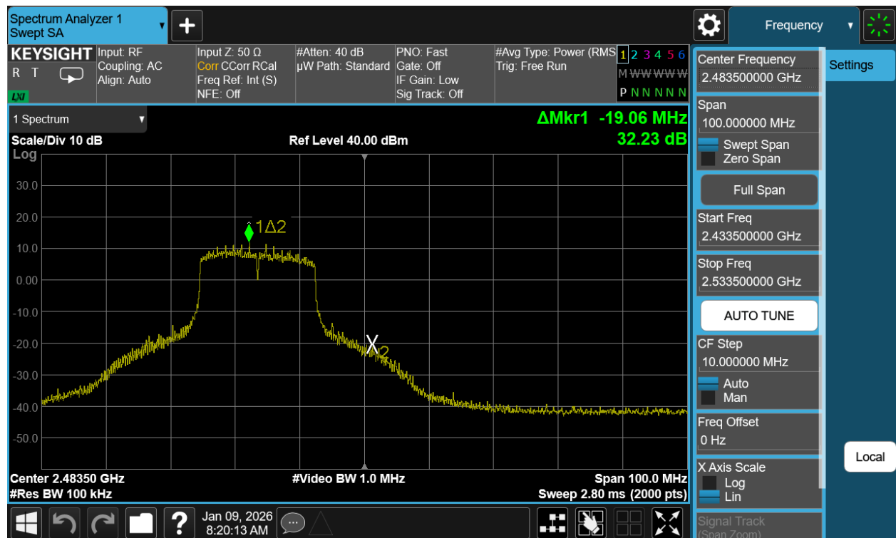
Plot 7-52. Band Edge Plot Antenna WF7b (802.11g – Ch. 12)
