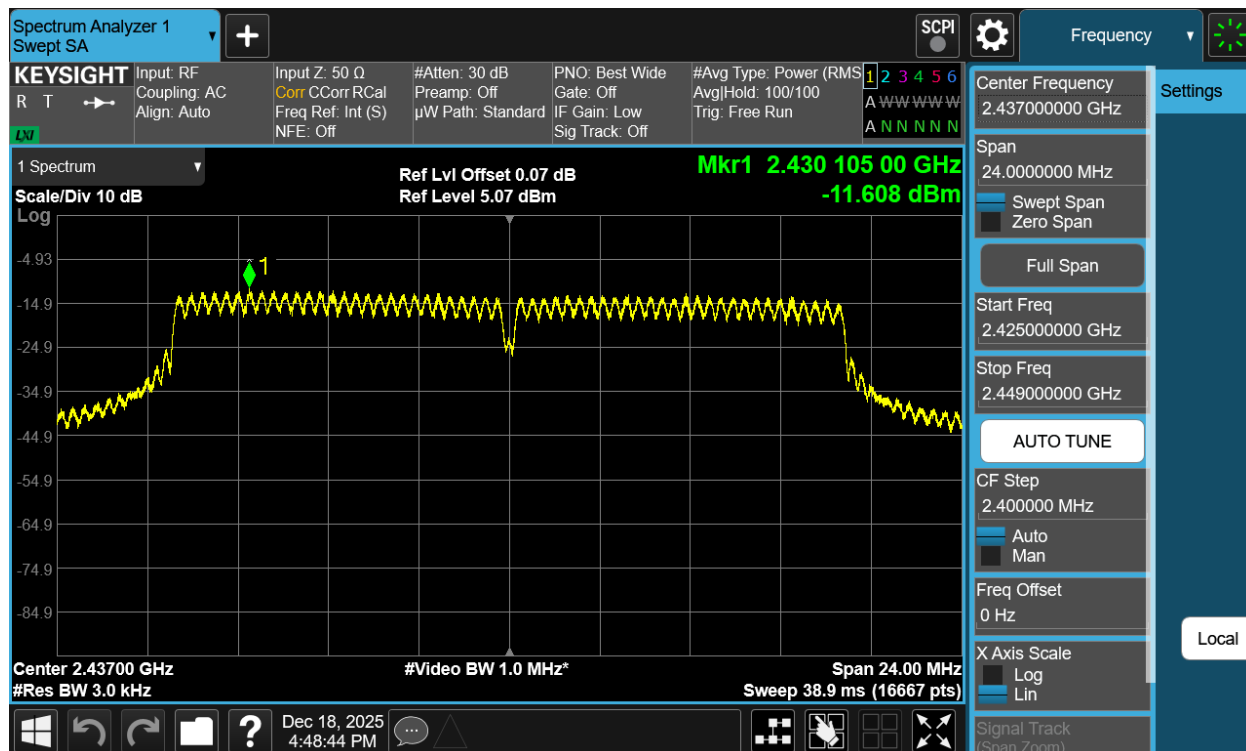
Plot 7-29 PSD CDD Antenna WF7b (20MHz BW 802.11n - Ch.6)
