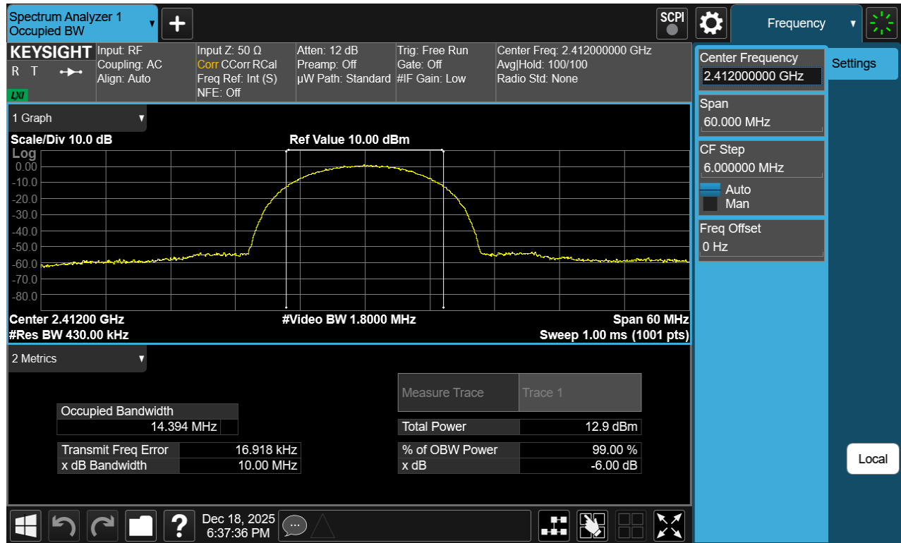
Plot 7-5 99% OBW Antenna WF2b (20MHz BW 802.11b - Ch.1)
