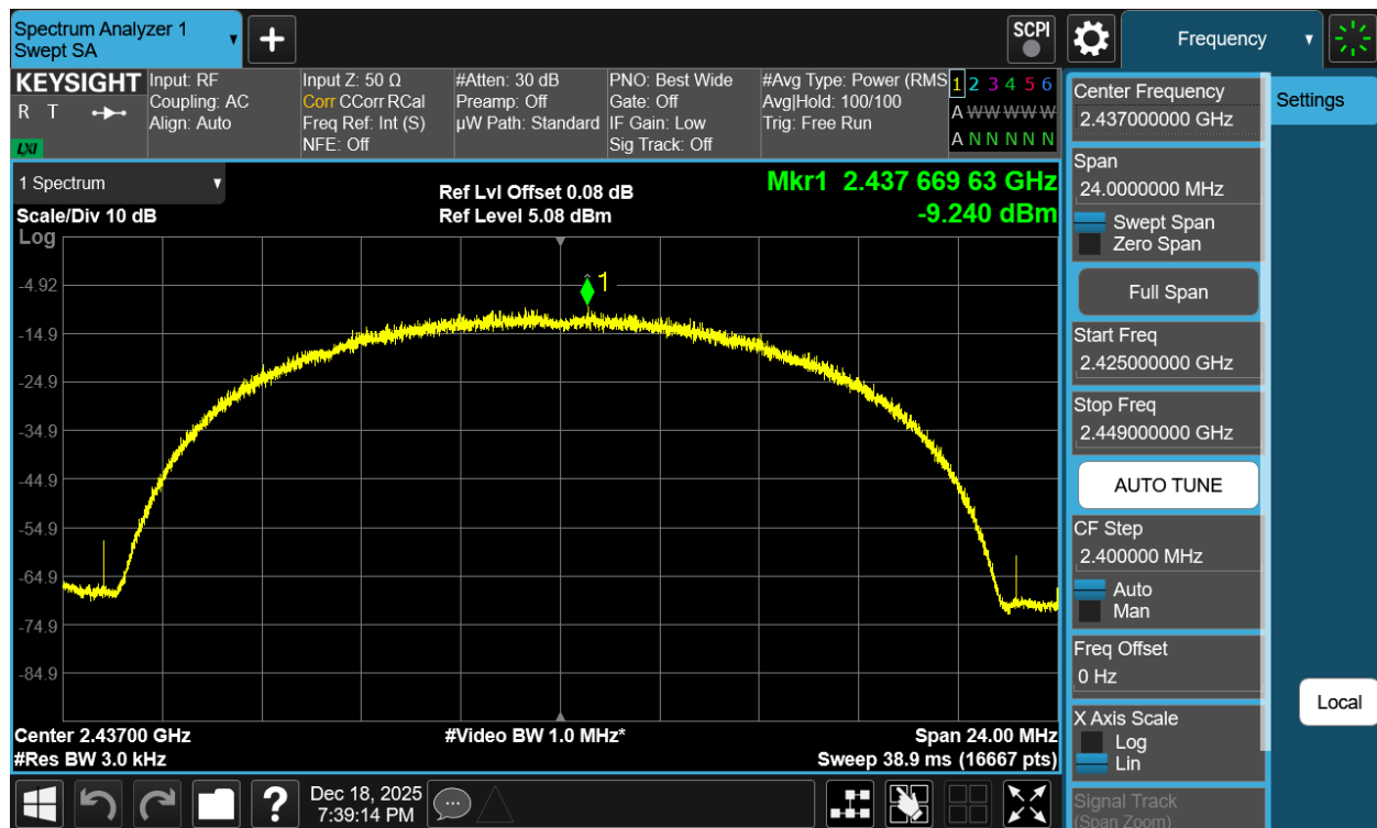
Plot 7-21 PSD Antenna WF2b (20MHz BW 802.11b - Ch.6)
