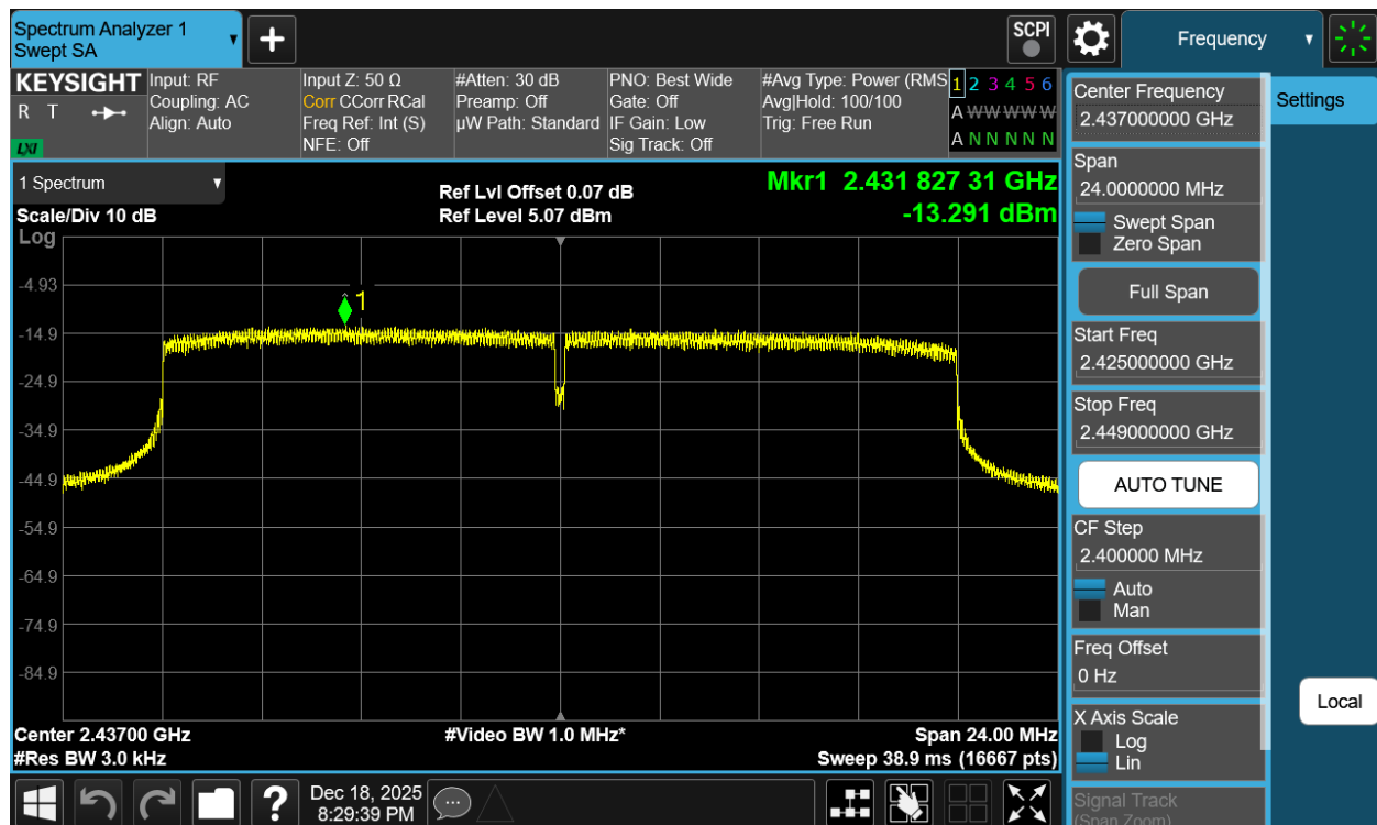
Plot 7-32 PSD CDD Antenna WF2b (20MHz BW 802.11be(SU) - Ch.6)
