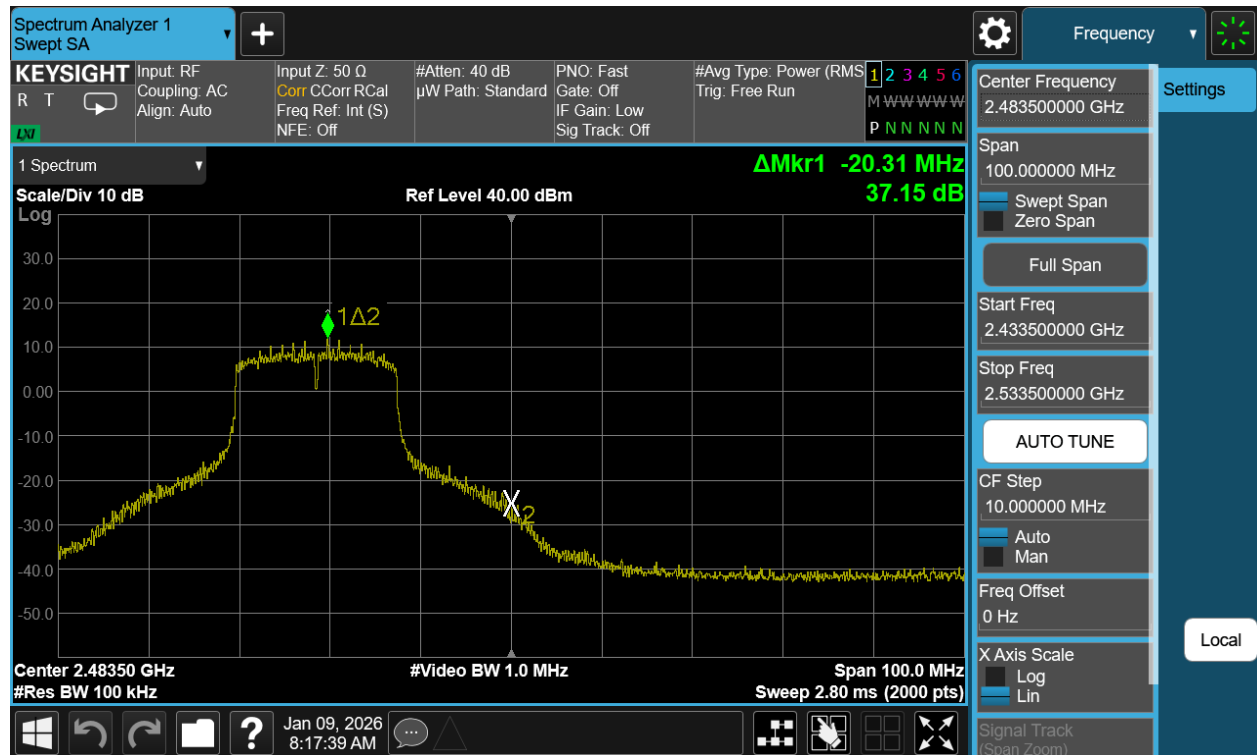
Plot 7-51. Band Edge Plot Antenna WF7b (802.11g – Ch. 11)
