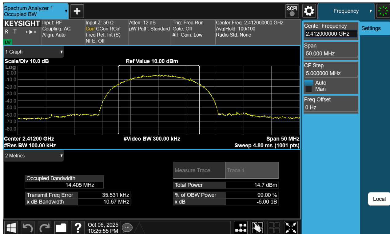
Plot 7-9 6dB OBW Antenna WF7b (20MHz BW 802.11b - Ch.1)
