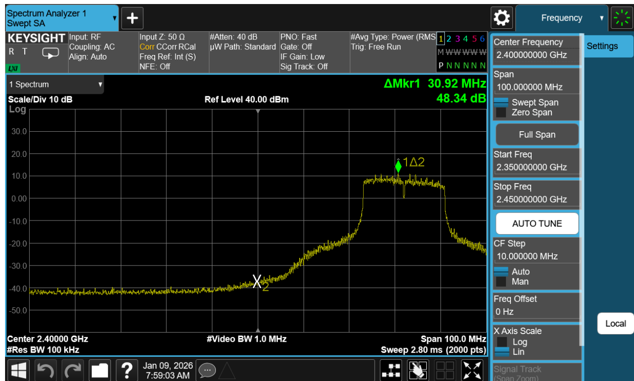
Plot 7-44. Band Edge Plot Antenna WF7b (802.11g – Ch. 5)
