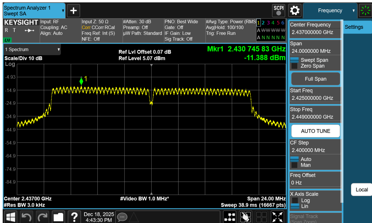
Plot 7-27 PSD CDD Antenna WF7b (20MHz BW 802.11g - Ch.6)
