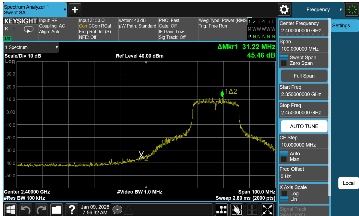
Plot 7-43. Band Edge Plot Antenna WF7b (802.11g – Ch. 4)
