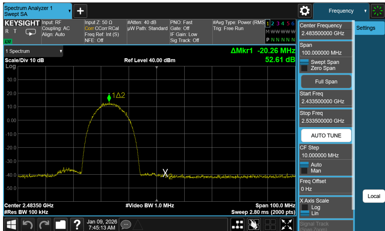
Plot 7-38. Band Edge Plot Antenna WF7b (802.11b – Ch. 12)
