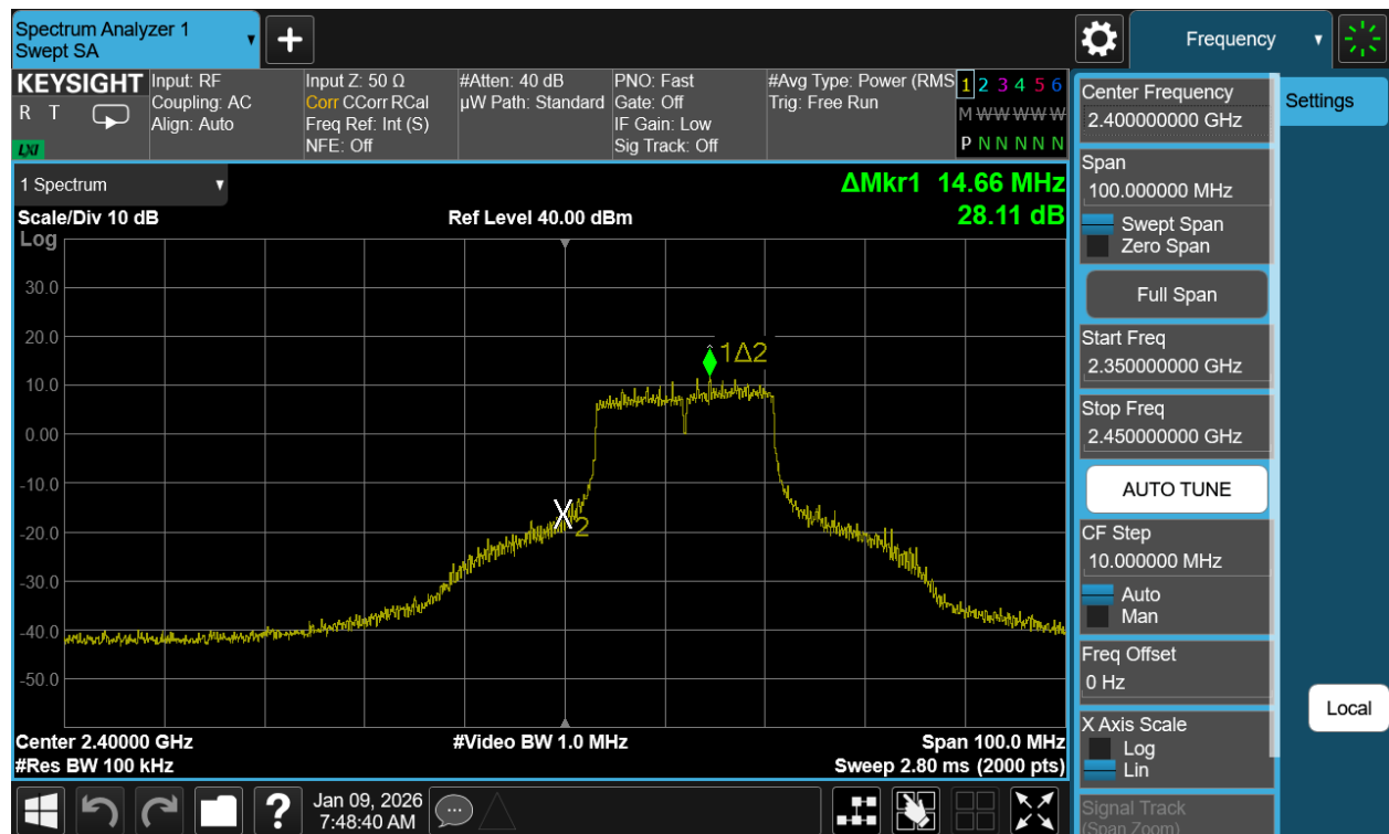
Plot 7-40. Band Edge Plot Antenna WF7b (802.11g – Ch. 1)
