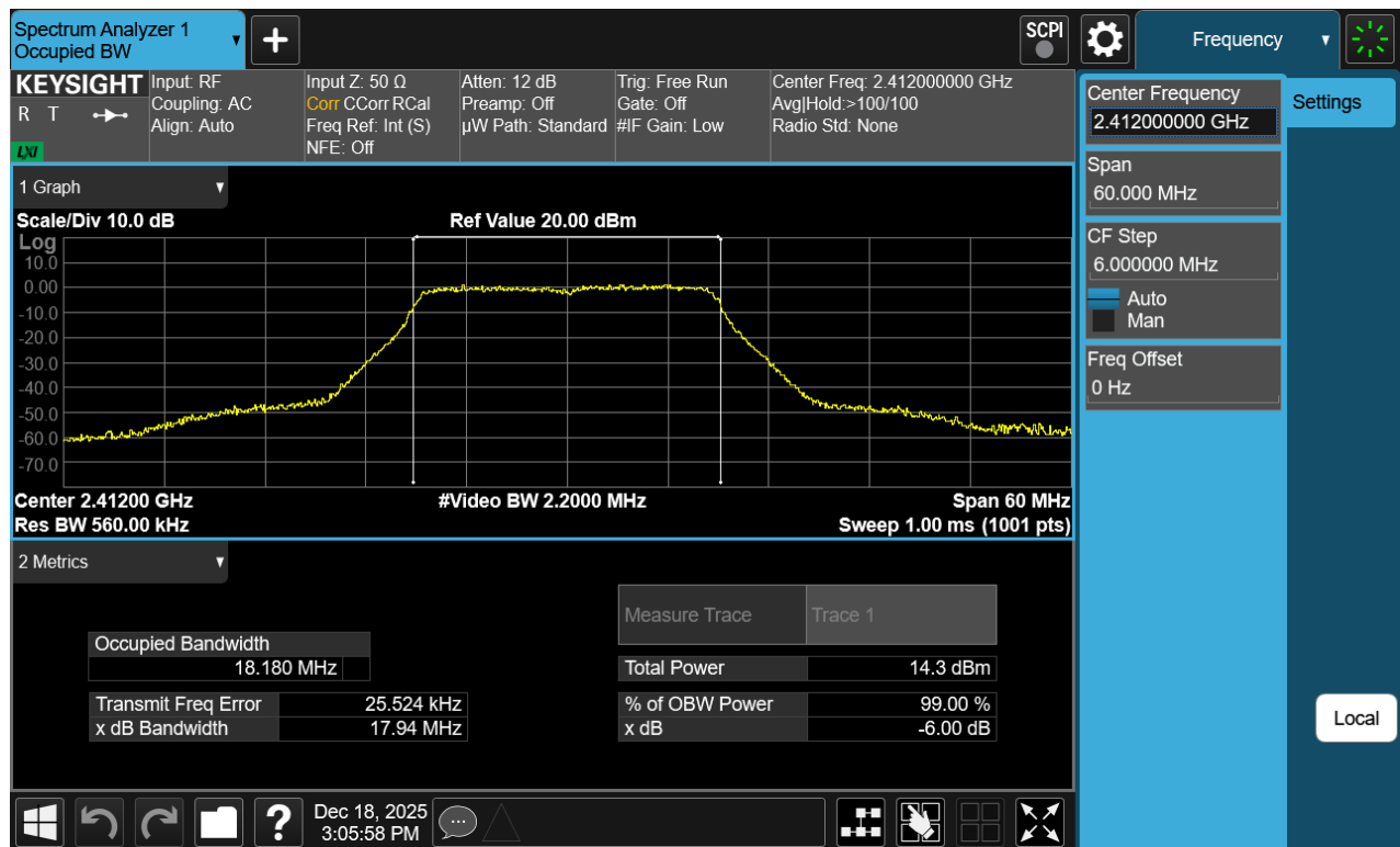
Plot 7-2 99% OBW Antenna WF7b (20MHz BW 802.11g - Ch.1)
