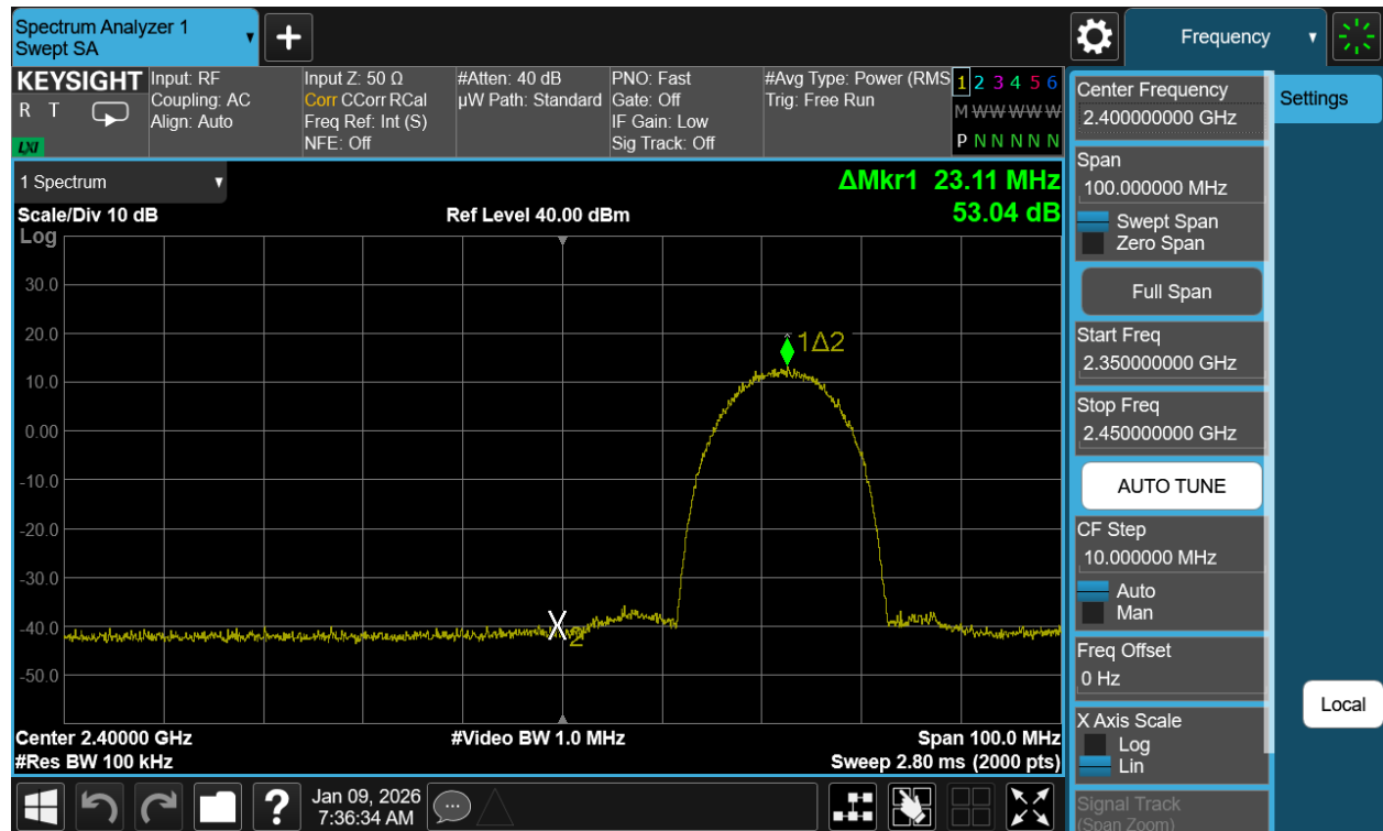
Plot 7-35. Band Edge Plot Antenna WF7b (802.11b - Ch. 3)
