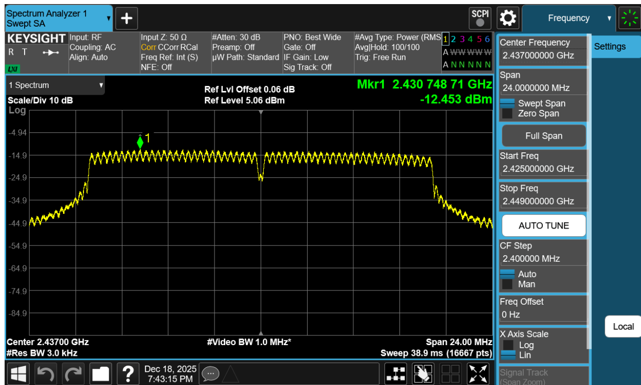
Plot 7-22 PSD Antenna WF2b (20MHz BW 802.11g - Ch.6)
