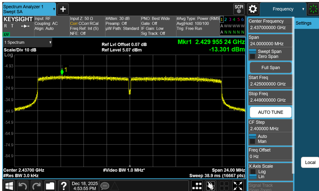
Plot 7-31 PSD CDD Antenna WF7b (20MHz BW 802.11be(SU) - Ch.6)
