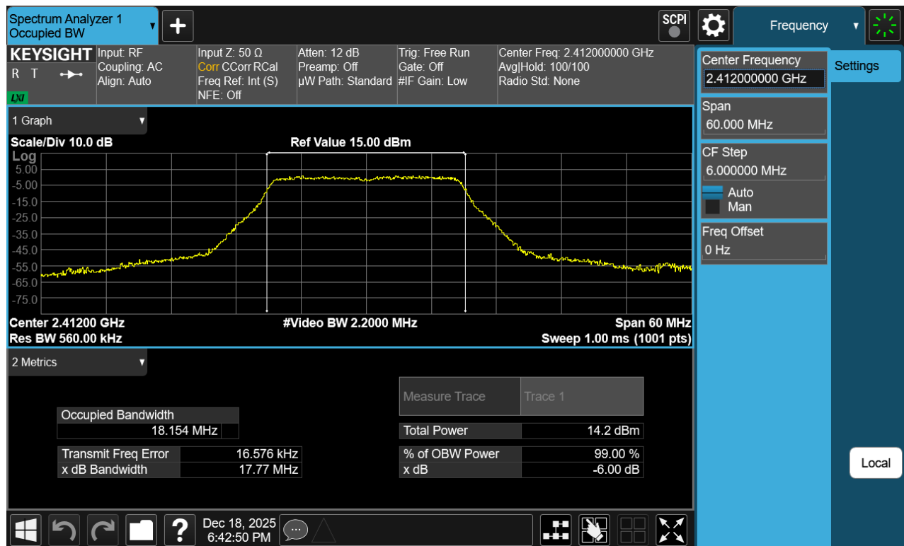
Plot 7-6 99% OBW Antenna WF2b (20MHz BW 802.11g - Ch.1)
