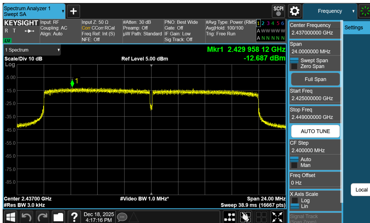
Plot 7-20 PSD Antenna WF7b (20MHz BW 802.11be(SU) - Ch.6)
