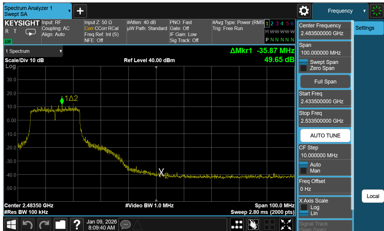
Plot 7-48. Band Edge Plot Antenna WF7b (802.11g - Ch. 8)
