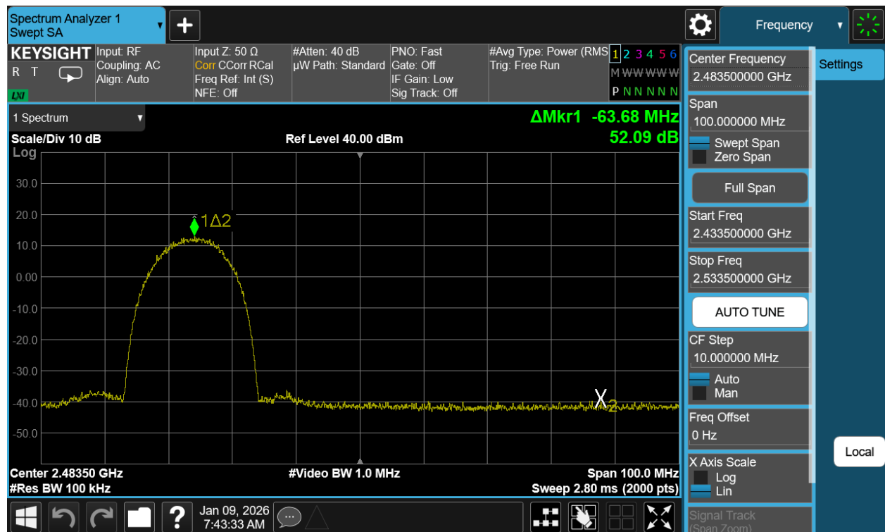
Plot 7-36. Band Edge Plot Antenna WF7b (802.11b - Ch. 10)
