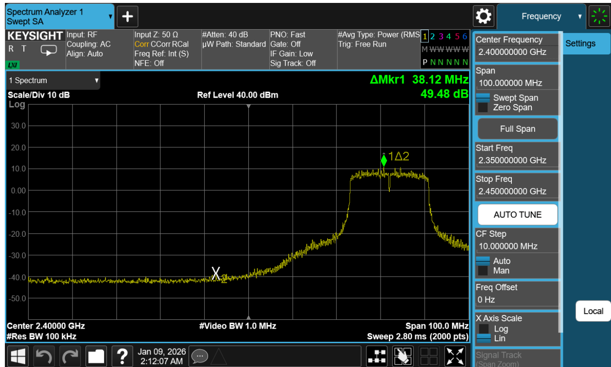
Plot 7-102. Band Edge Plot Antenna WF2b (802.11n (2.4GHz) – Ch. 5)
