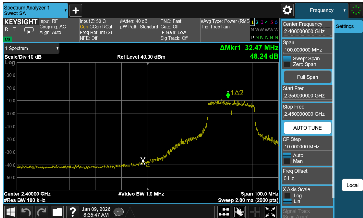
Plot 7-58. Band Edge Plot Antenna WF7b (802.11n (2.4GHz) – Ch. 5)
