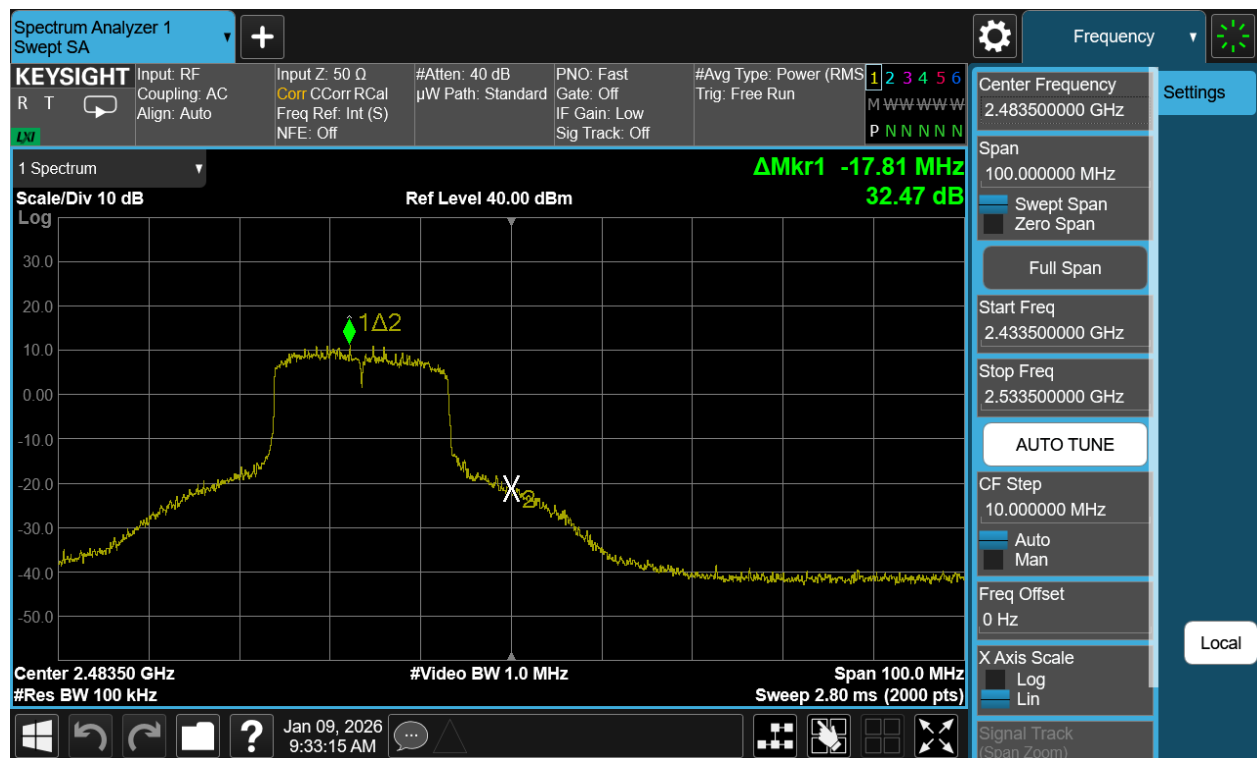
Plot 7-80. Band Edge Plot Antenna WF7b (802.11be (SU - 2.4GHz) - Ch. 12)
