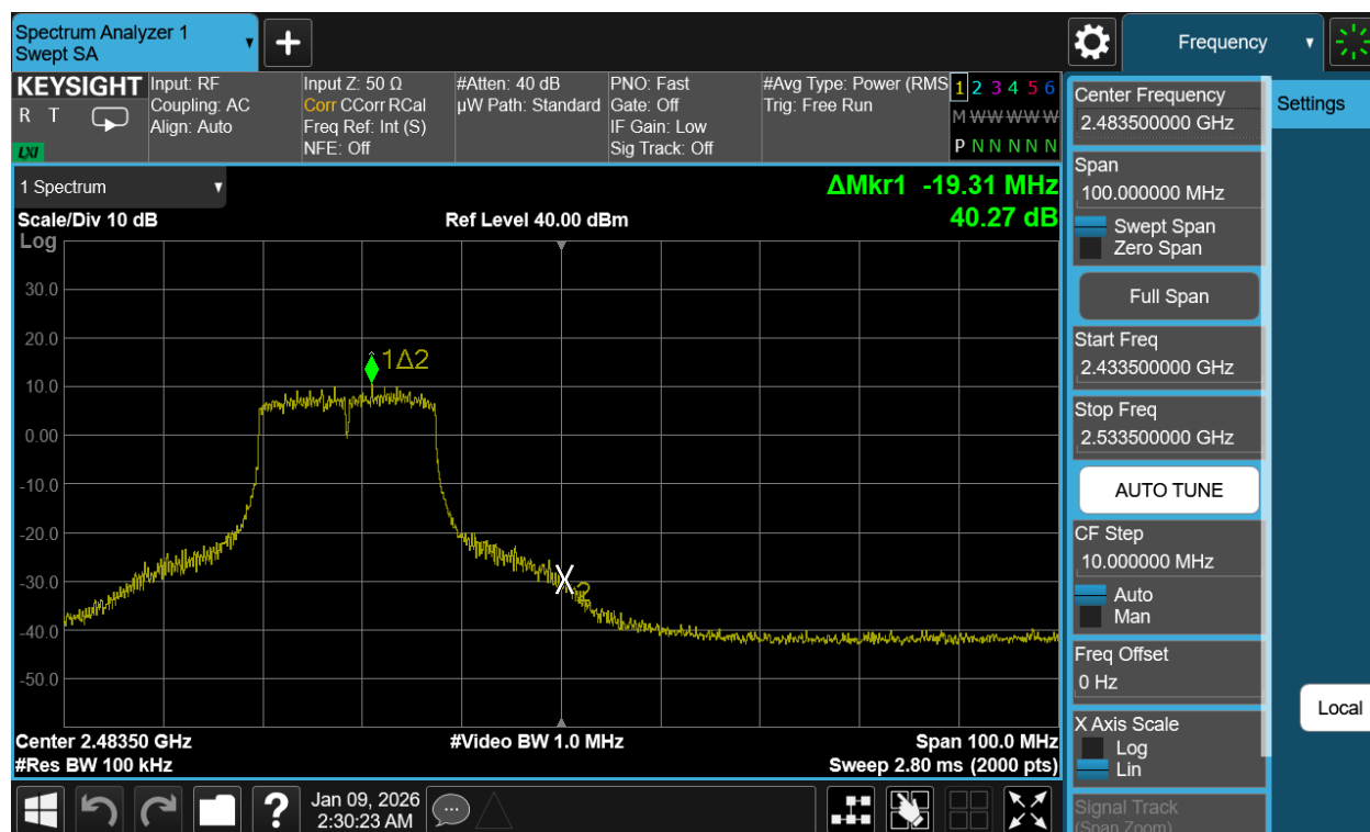
Plot 7-107. Band Edge Plot Antenna WF2b (802.11n (2.4GHz) – Ch. 11)
