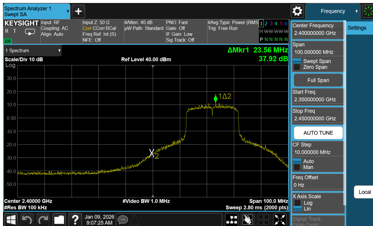
Plot 7-70. Band Edge Plot Antenna WF7b (802.11be (SU - 2.4GHz) – Ch. 3)
