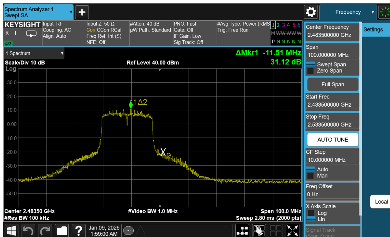
Plot 7-97. Band Edge Plot Antenna WF2b (802.11g – Ch. 13)
