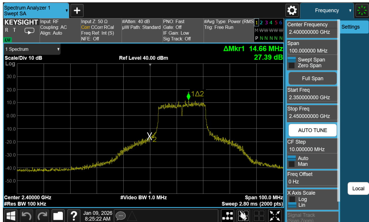
Plot 7-54. Band Edge Plot Antenna WF7b (802.11n (2.4GHz) – Ch. 1)
