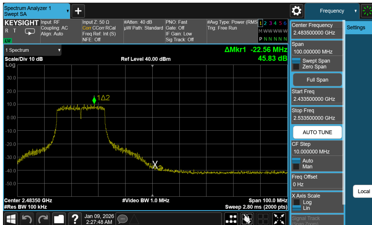
Plot 7-106. Band Edge Plot Antenna WF2b (802.11n (2.4GHz) – Ch. 10)
