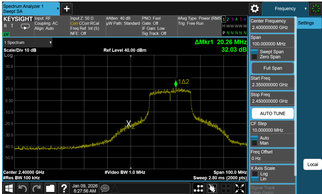
Plot 7-55. Band Edge Plot Antenna WF7b (802.11n (2.4GHz) – Ch. 2)
