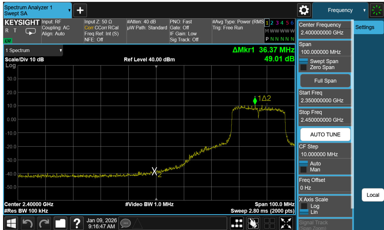
Plot 7-73. Band Edge Plot Antenna WF7b (802.11be (SU - 2.4GHz) – Ch. 6)
