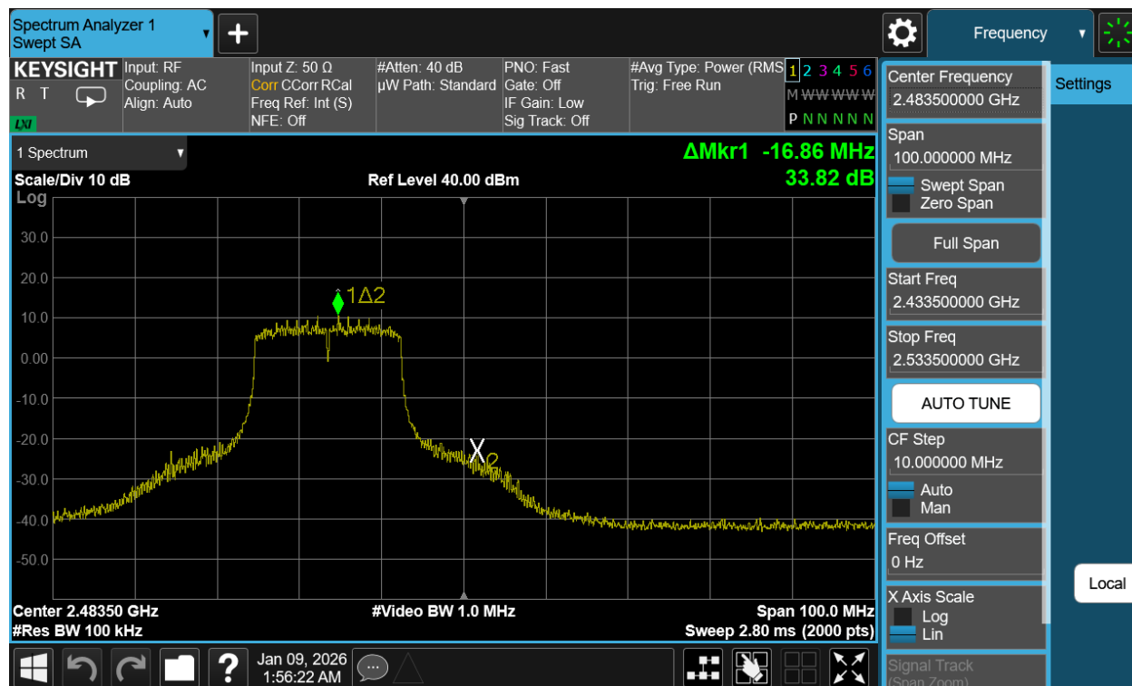
Plot 7-96. Band Edge Plot Antenna WF2b (802.11g – Ch. 12)
