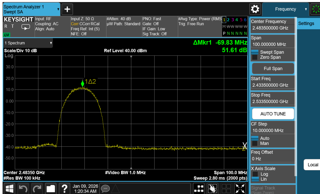
Plot 7-83. Band Edge Plot Antenna WF2b (802.11b – Ch. 11)
