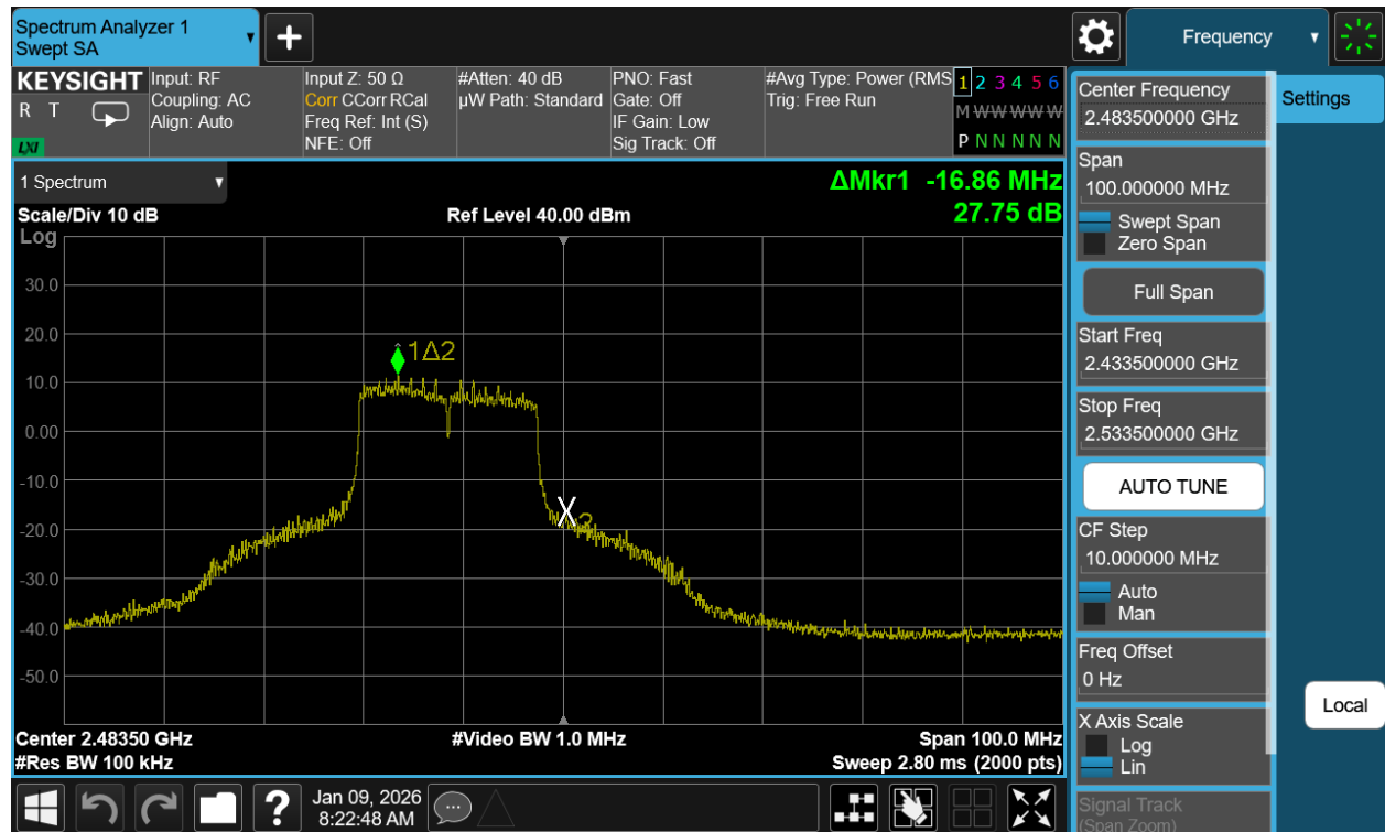
Plot 7-53. Band Edge Plot Antenna WF7b (802.11g – Ch. 13)
