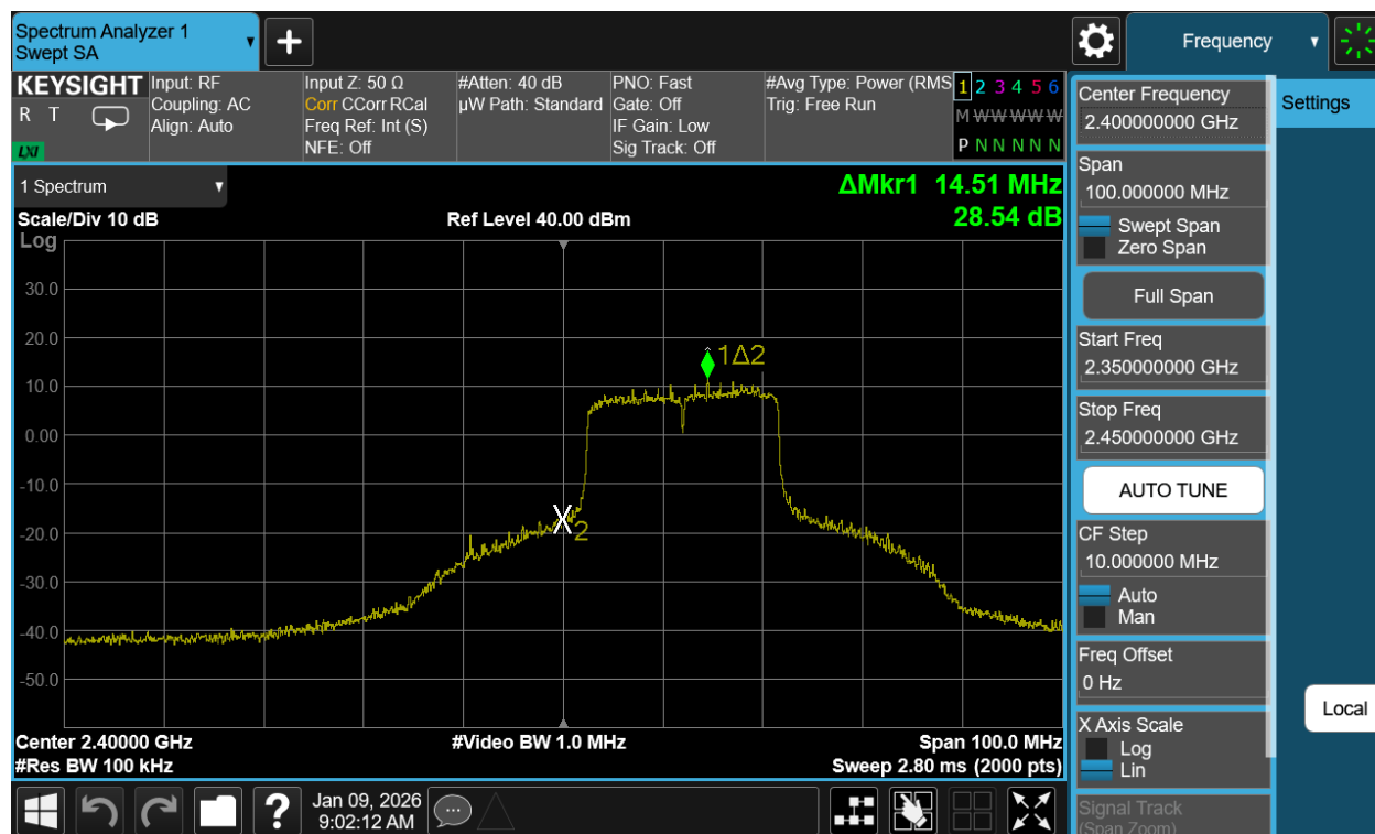
Plot 7-68. Band Edge Plot Antenna WF7b (802.11be (SU - 2.4GHz) – Ch. 1)
