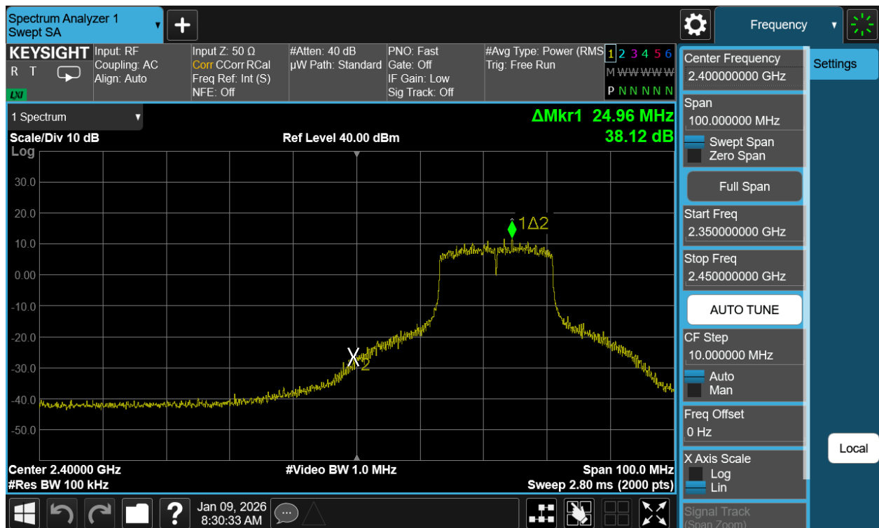
Plot 7-56. Band Edge Plot Antenna WF7b (802.11n (2.4GHz) – Ch. 3)
