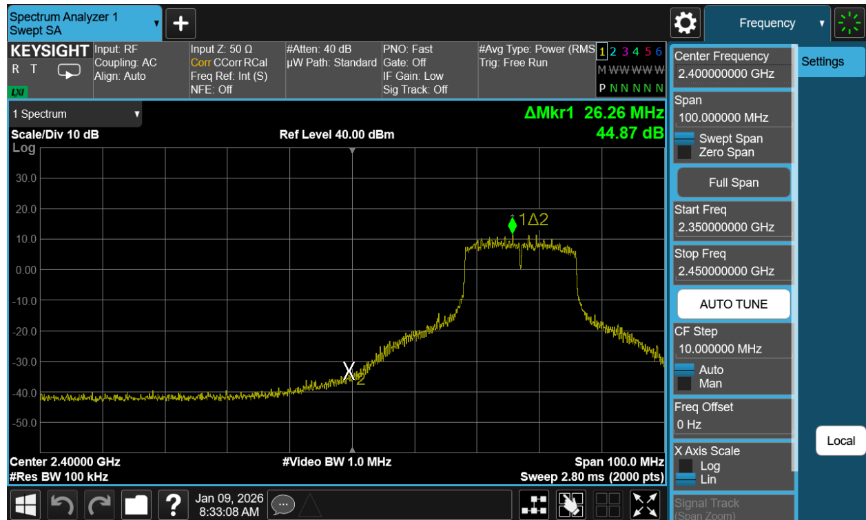
Plot 7-57. Band Edge Plot Antenna WF7b (802.11n (2.4GHz) – Ch. 4)
