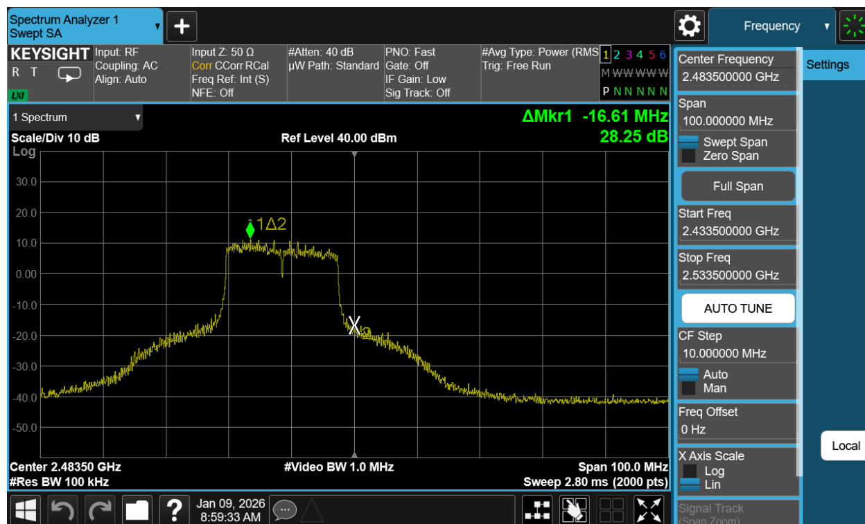
Plot 7-67. Band Edge Plot Antenna WF7b (802.11n (2.4GHz) – Ch. 13)
