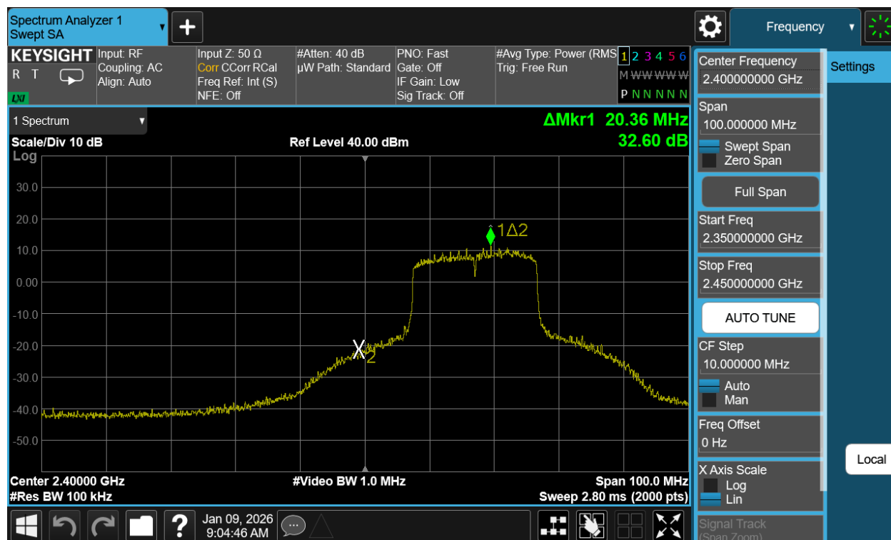
Plot 7-69. Band Edge Plot Antenna WF7b (802.11be (SU - 2.4GHz) – Ch. 2)
