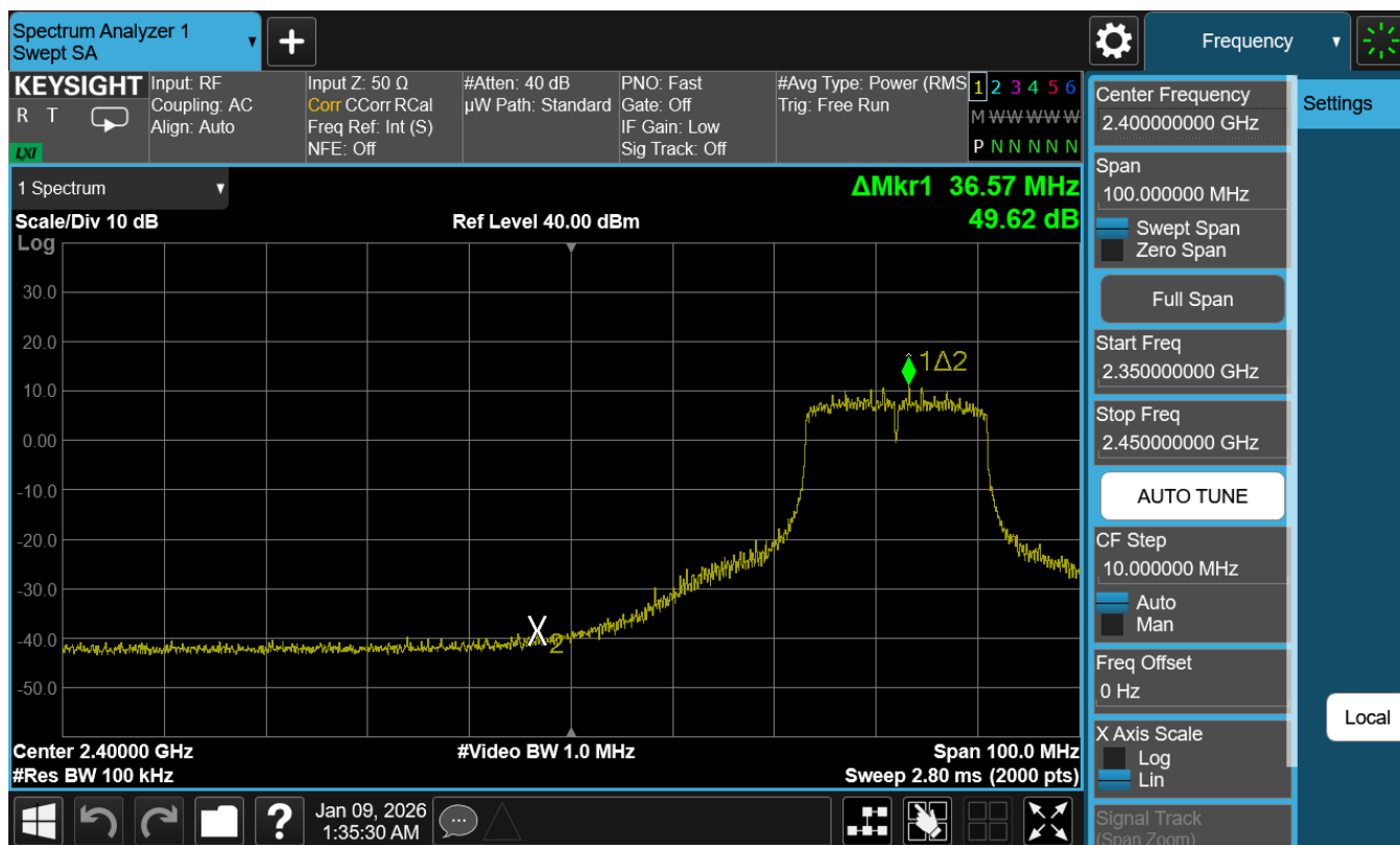
Plot 7-90. Band Edge Plot Antenna WF2b (802.11g – Ch. 5)
