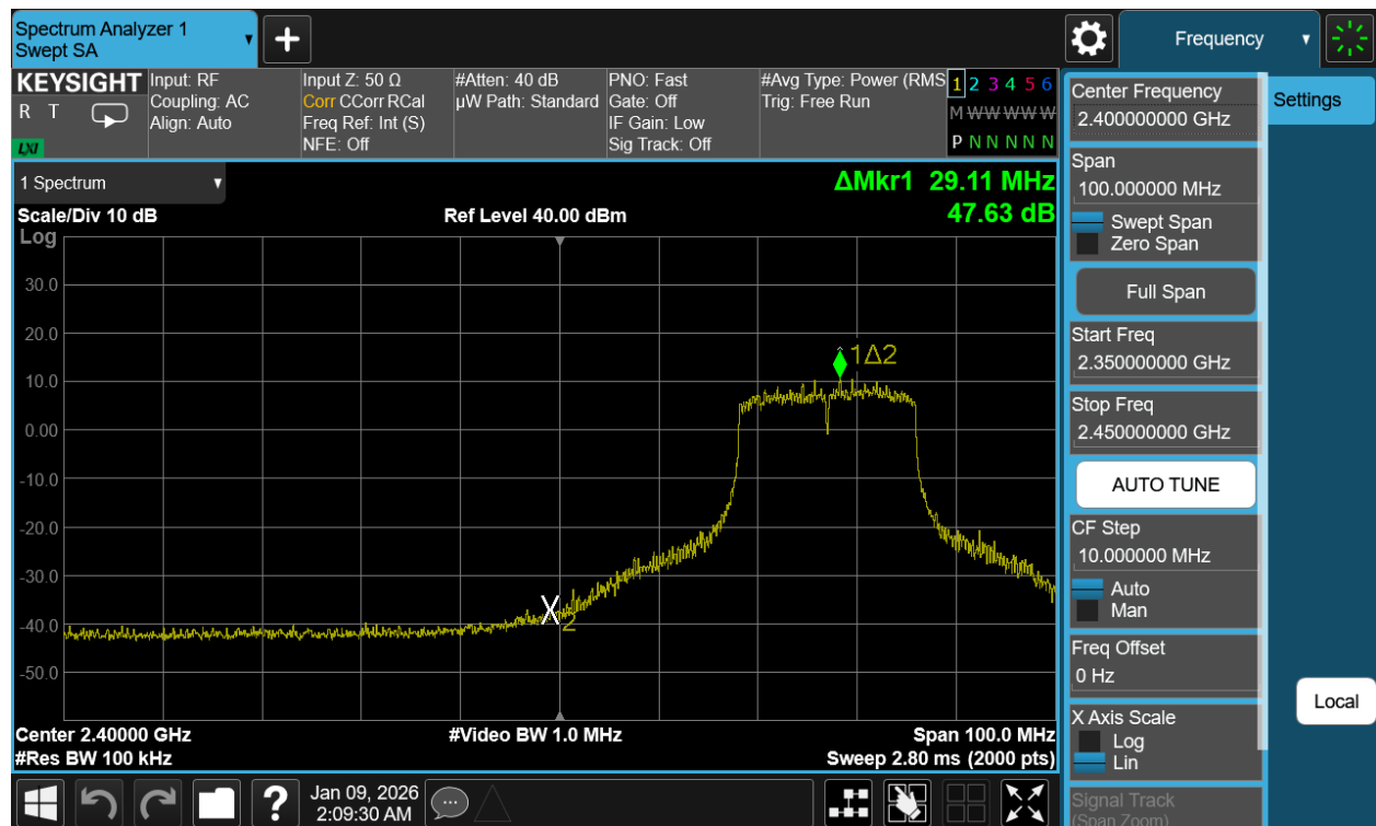
Plot 7-101. Band Edge Plot Antenna WF2b (802.11n (2.4GHz) – Ch. 4)
