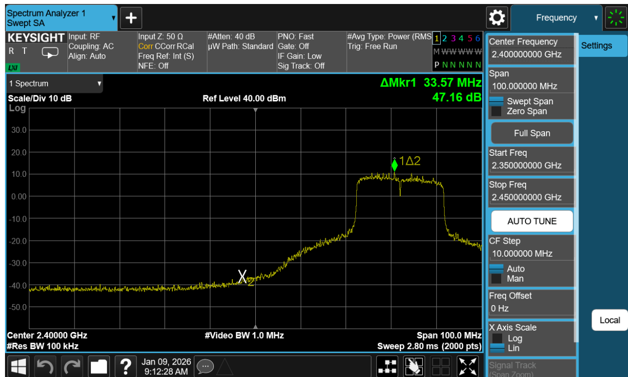
Plot 7-72. Band Edge Plot Antenna WF7b (802.11be (SU - 2.4GHz) – Ch. 5)
