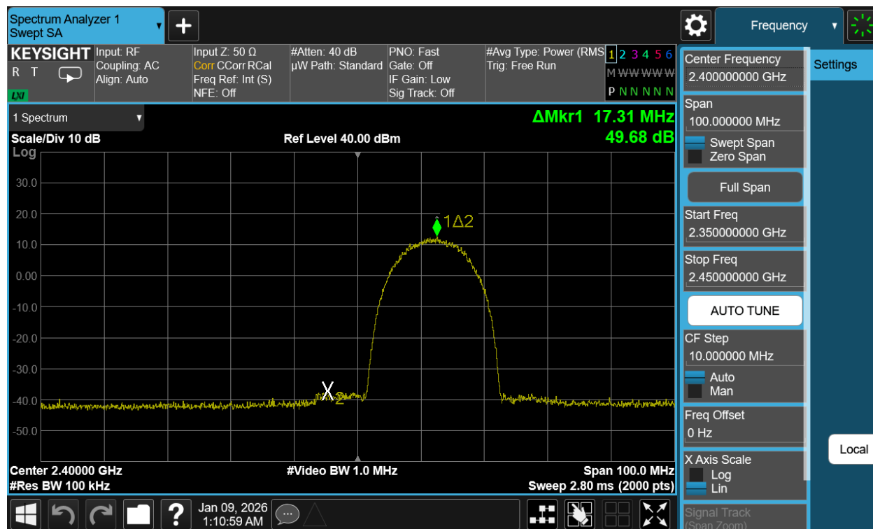
Plot 7-82. Band Edge Plot Antenna WF2b (802.11b – Ch. 1)
