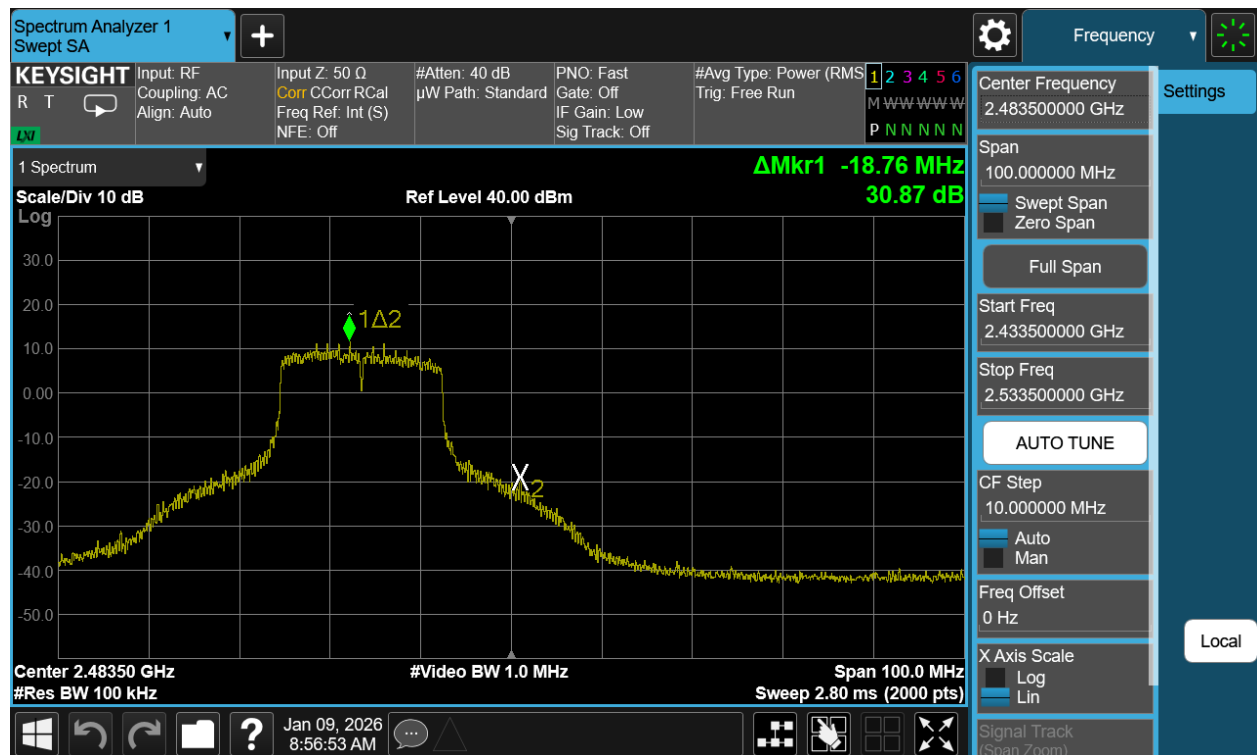
Plot 7-66. Band Edge Plot Antenna WF7b (802.11n (2.4GHz) – Ch. 12)
