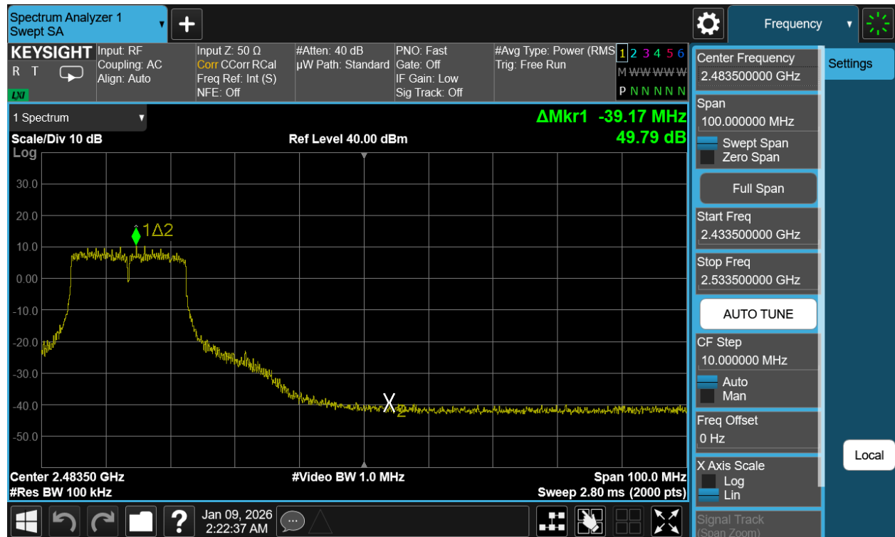
Plot 7-104. Band Edge Plot Antenna WF2b (802.11n (2.4GHz) – Ch. 8)
