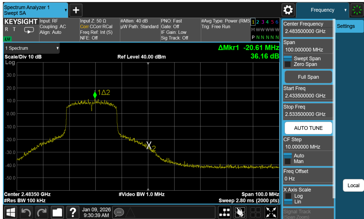
Plot 7-79. Band Edge Plot Antenna WF7b (802.11be (SU - 2.4GHz) - Ch. 11)
