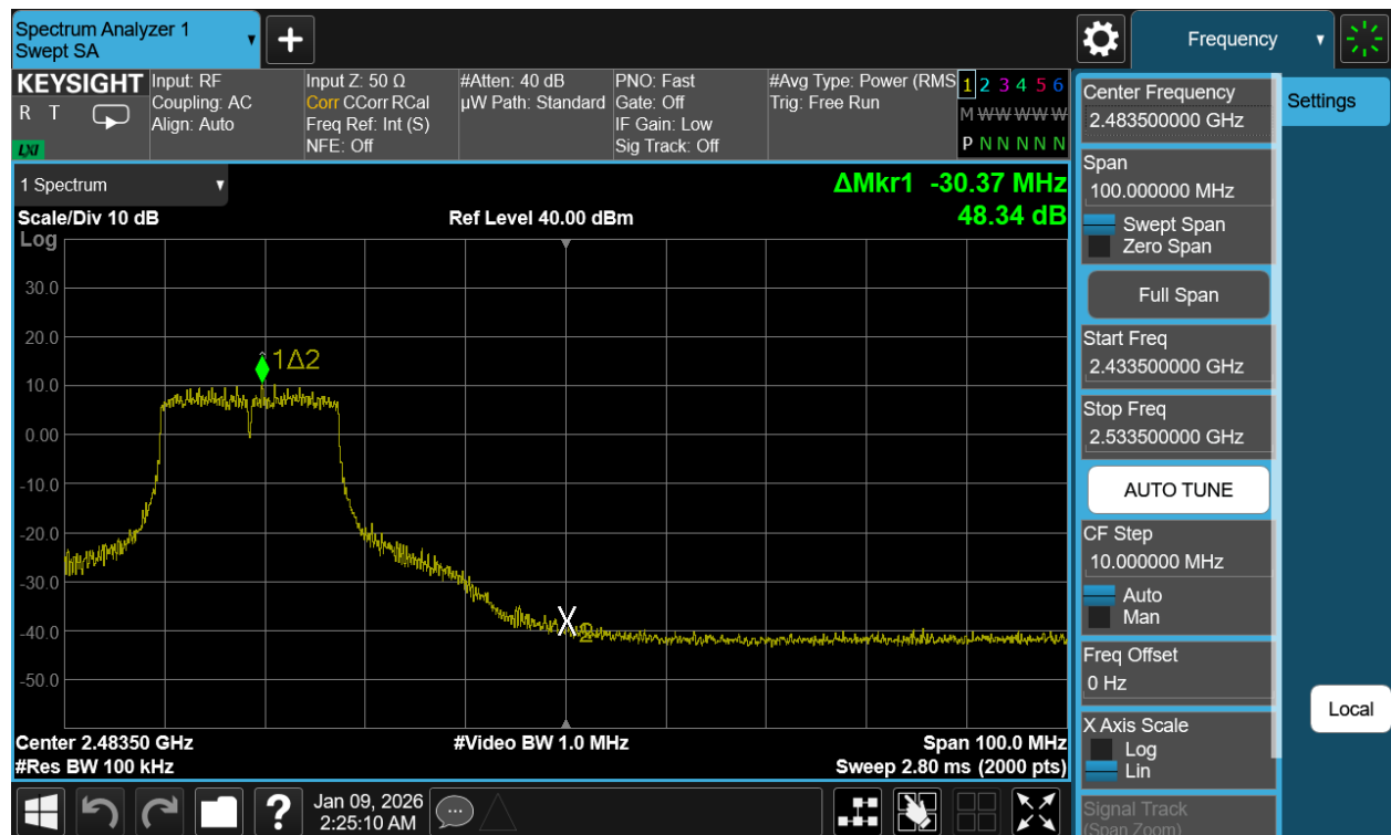
Plot 7-105. Band Edge Plot Antenna WF2b (802.11n (2.4GHz) – Ch. 9)
