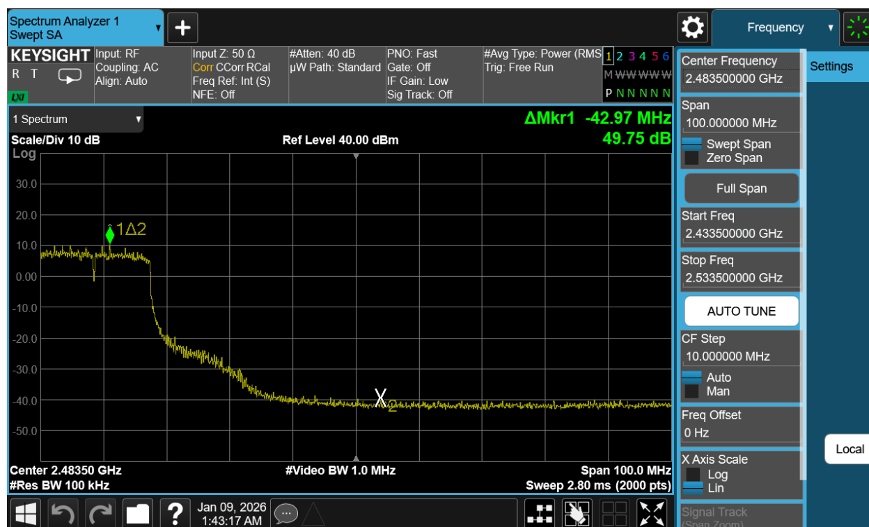
Plot 7-91. Band Edge Plot Antenna WF2b (802.11g – Ch. 7)
