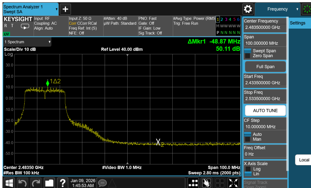
Plot 7-92. Band Edge Plot Antenna WF2b (802.11g – Ch. 8)
