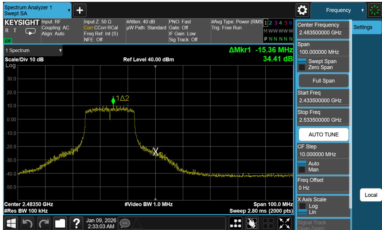
Plot 7-108. Band Edge Plot Antenna WF2b (802.11n (2.4GHz) – Ch. 12)
