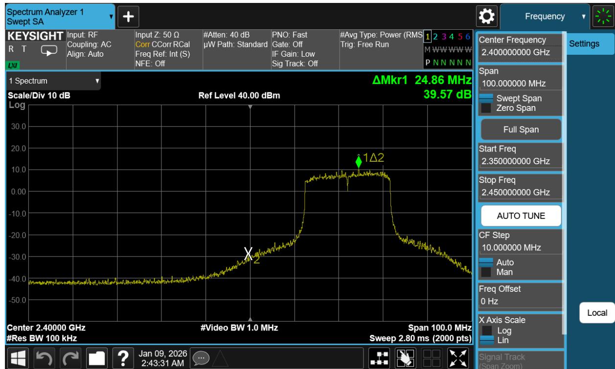
Plot 7-112. Band Edge Plot Antenna WF2b (802.11be (SU - 2.4GHz) – Ch. 3)
