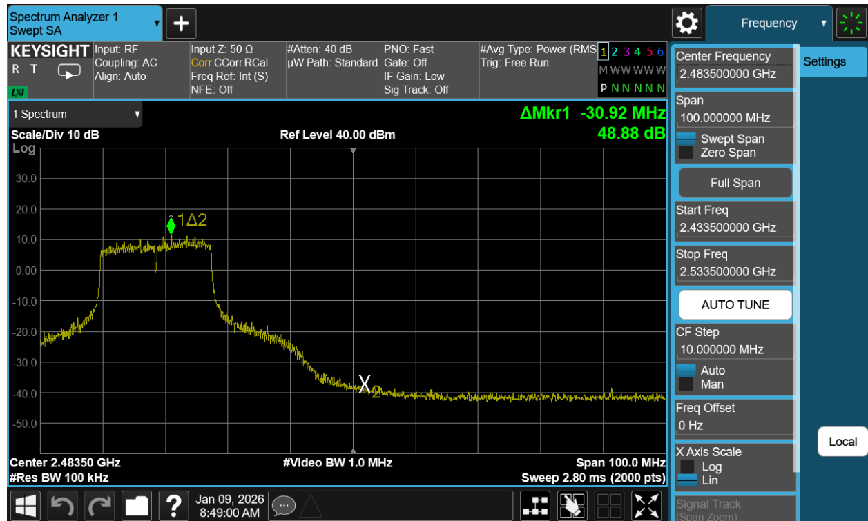
Plot 7-63. Band Edge Plot Antenna WF7b (802.11n (2.4GHz) – Ch. 9)
