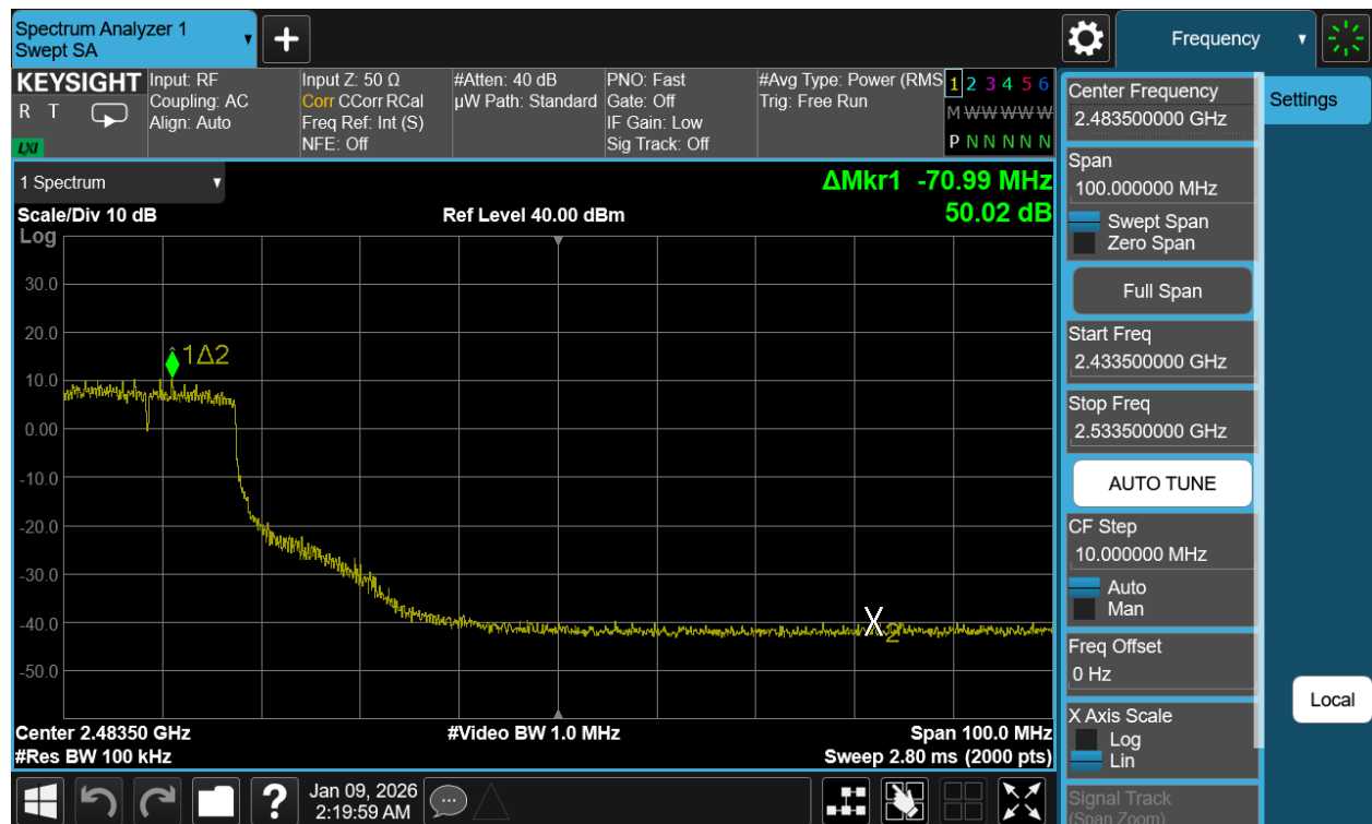
Plot 7-103. Band Edge Plot Antenna WF2b (802.11n (2.4GHz) – Ch. 7)
