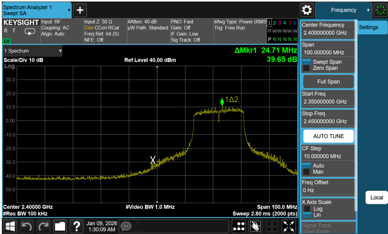
Plot 7-88. Band Edge Plot Antenna WF2b (802.11g – Ch. 3)
