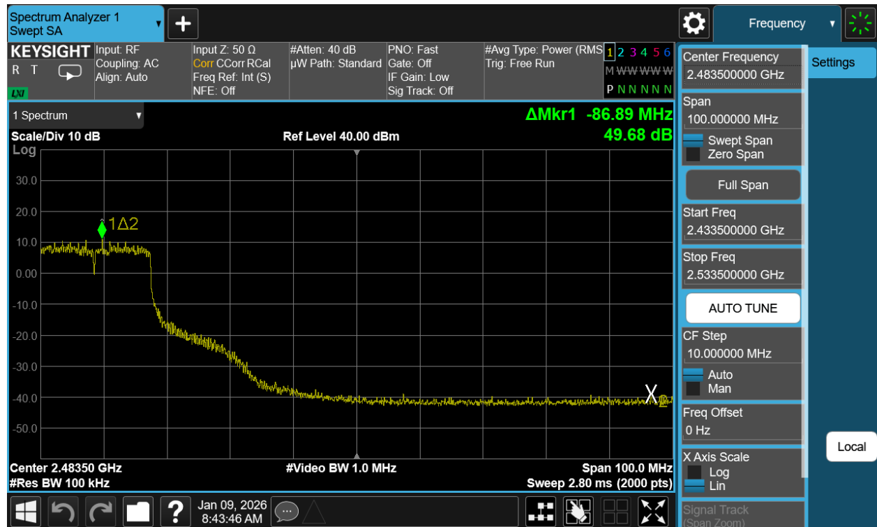
Plot 7-61. Band Edge Plot Antenna WF7b (802.11n (2.4GHz) – Ch. 7)
