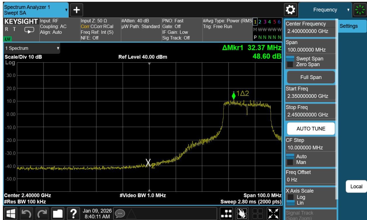
Plot 7-59. Band Edge Plot Antenna WF7b (802.11n (2.4GHz) – Ch. 6)
