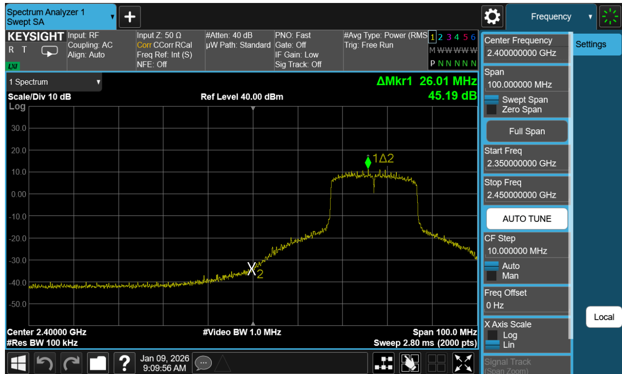
Plot 7-71. Band Edge Plot Antenna WF7b (802.11be (SU - 2.4GHz) – Ch. 4)
