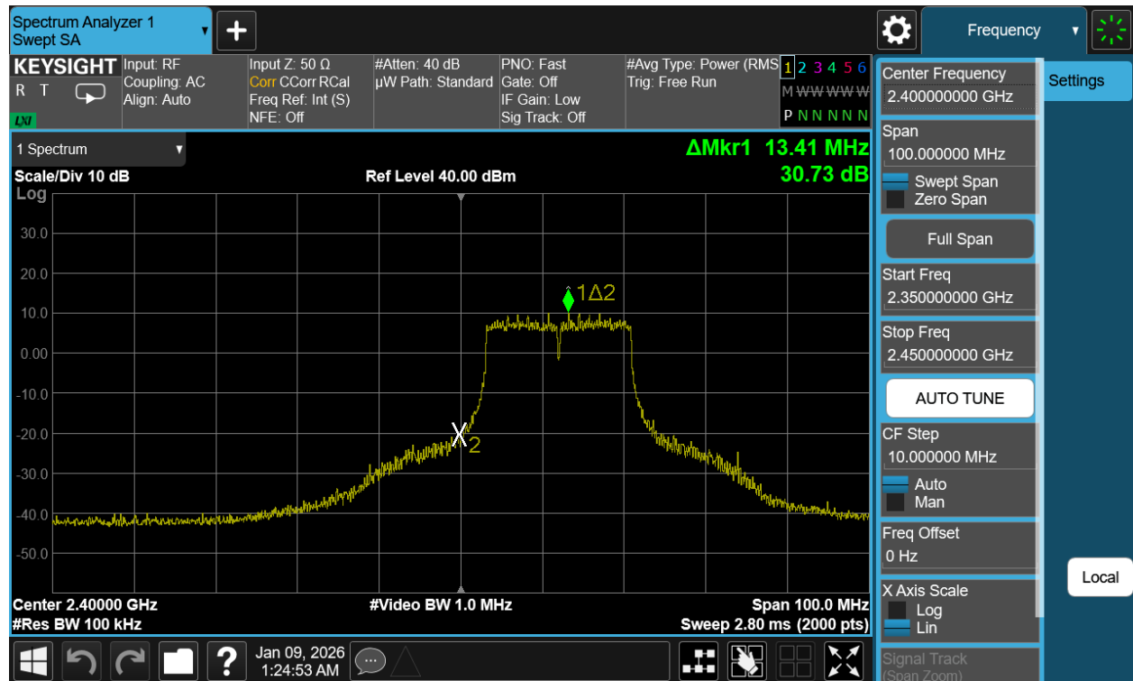
Plot 7-86. Band Edge Plot Antenna WF2b (802.11g - Ch. 1)
