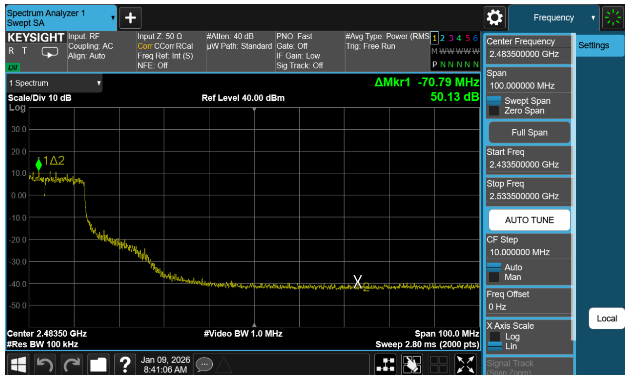
Plot 7-60. Band Edge Plot Antenna WF7b (802.11n (2.4GHz) – Ch. 6)
