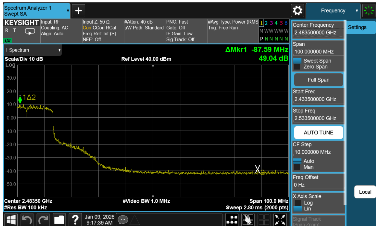
Plot 7-74. Band Edge Plot Antenna WF7b (802.11be (SU - 2.4GHz) – Ch. 6)
