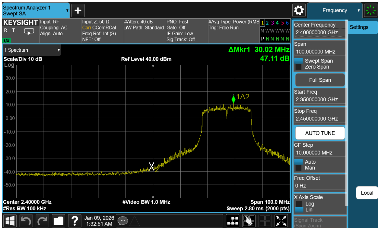
Plot 7-89. Band Edge Plot Antenna WF2b (802.11g – Ch. 4)
