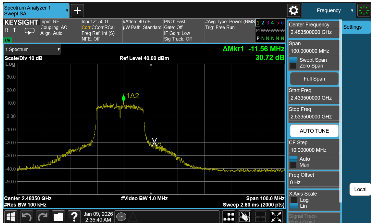
Plot 7-109. Band Edge Plot Antenna WF2b (802.11n (2.4GHz) – Ch. 13)
