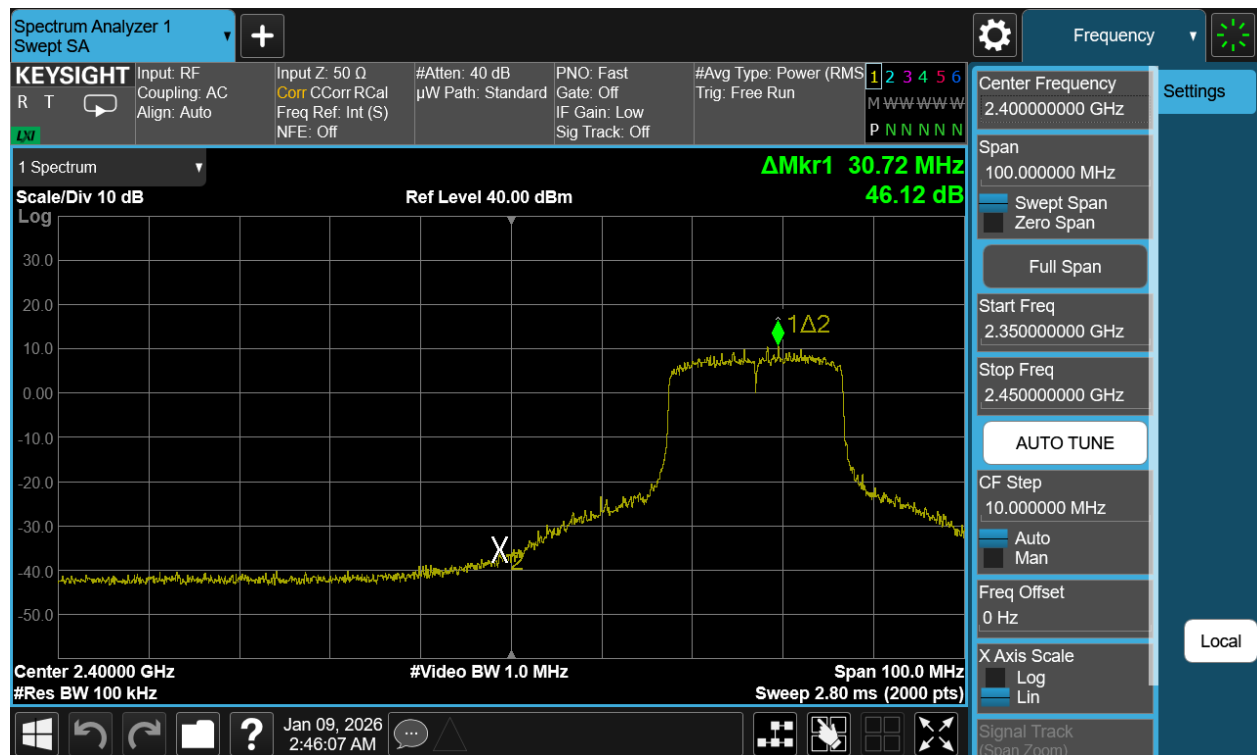
Plot 7-113. Band Edge Plot Antenna WF2b (802.11be (SU - 2.4GHz) – Ch. 4)
