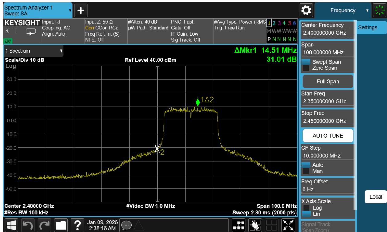
Plot 7-110. Band Edge Plot Antenna WF2b (802.11be (SU - 2.4GHz) – Ch. 1)
