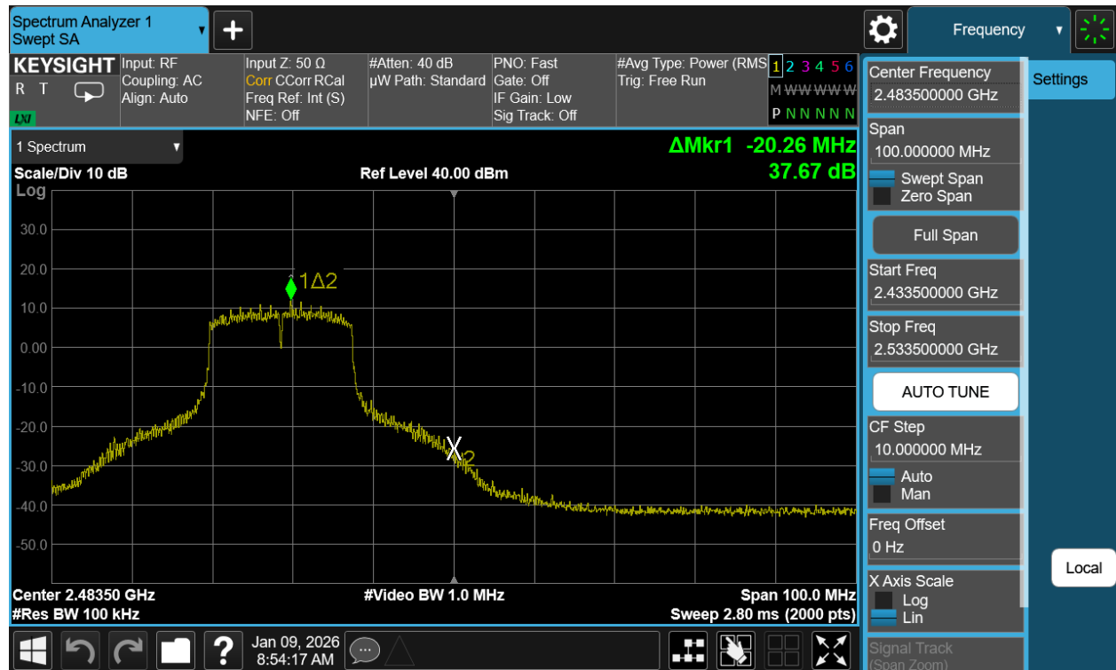
Plot 7-65. Band Edge Plot Antenna WF7b (802.11n (2.4GHz) – Ch. 11)
