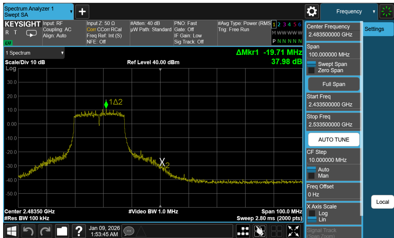
Plot 7-95. Band Edge Plot Antenna WF2b (802.11g – Ch. 11)
