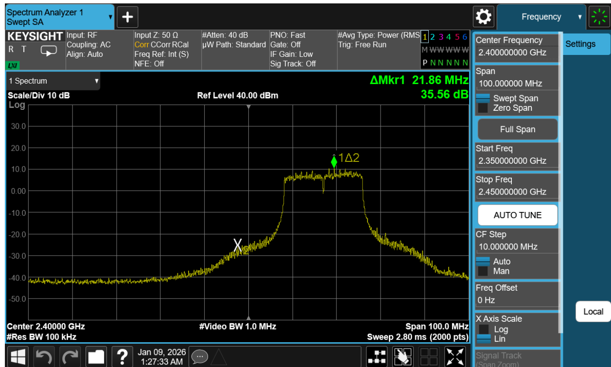
Plot 7-87. Band Edge Plot Antenna WF2b (802.11g - Ch. 2)
