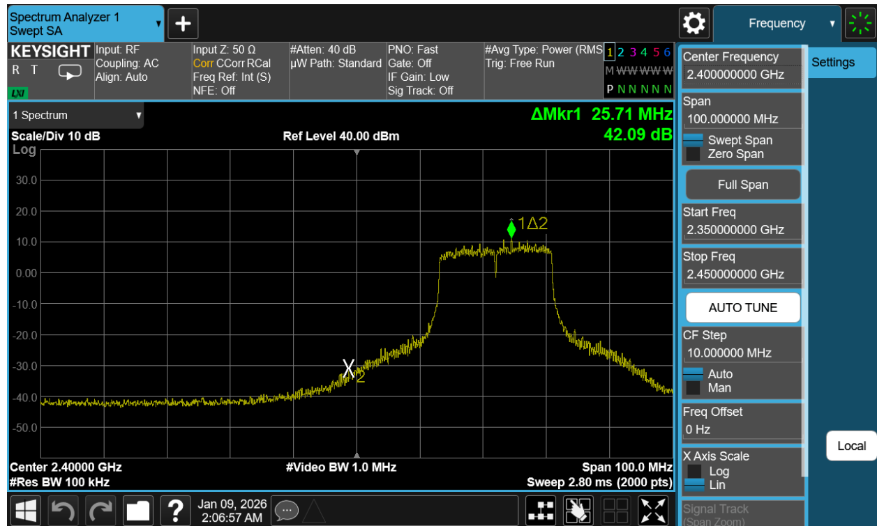
Plot 7-100. Band Edge Plot Antenna WF2b (802.11n (2.4GHz) – Ch. 3)
