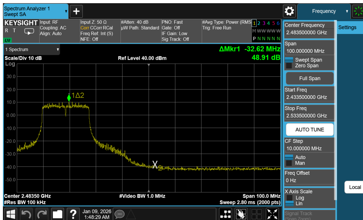
Plot 7-93. Band Edge Plot Antenna WF2b (802.11g – Ch. 9)
