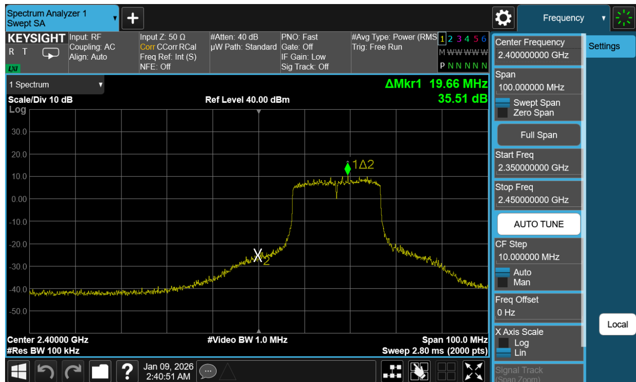
Plot 7-111. Band Edge Plot Antenna WF2b (802.11be (SU - 2.4GHz) – Ch. 2)
