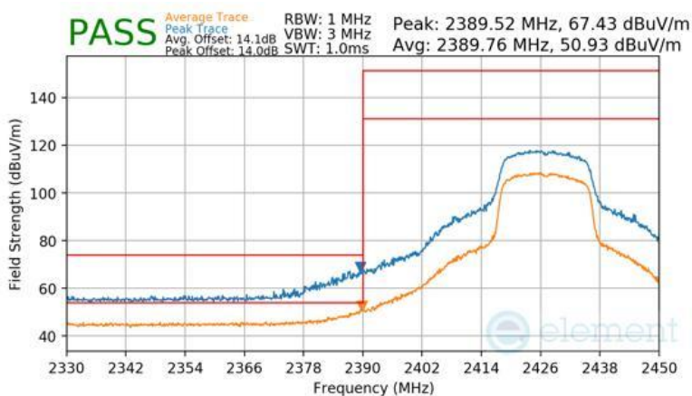
Plot 7-157 Radiated Restricted Lower Band Edge Measurement Antenna WF7b
