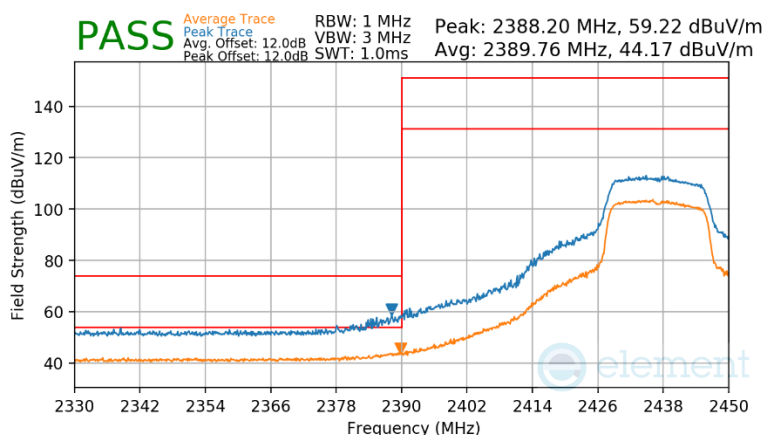
Plot 7-159 Radiated Restricted Lower Band Edge Measurement Antenna WF7b
