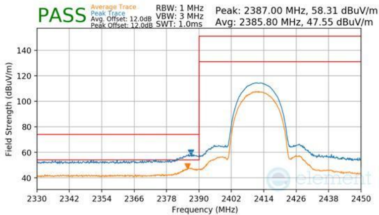
Plot 7-181 Radiated Restricted Lower Band Edge Measurement Antenna WF2b
