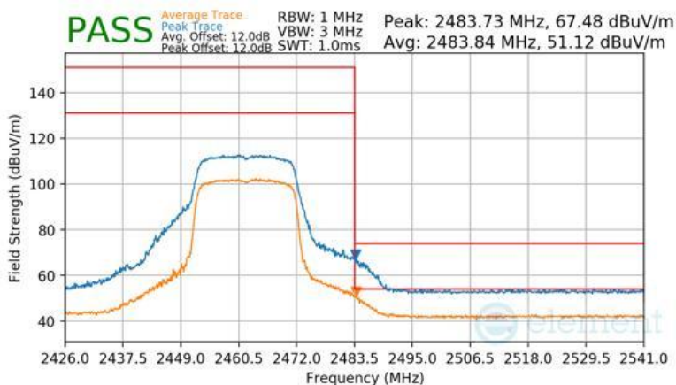
Plot 7-178 Radiated Restricted Upper Band Edge Measurement Antenna WF7b
