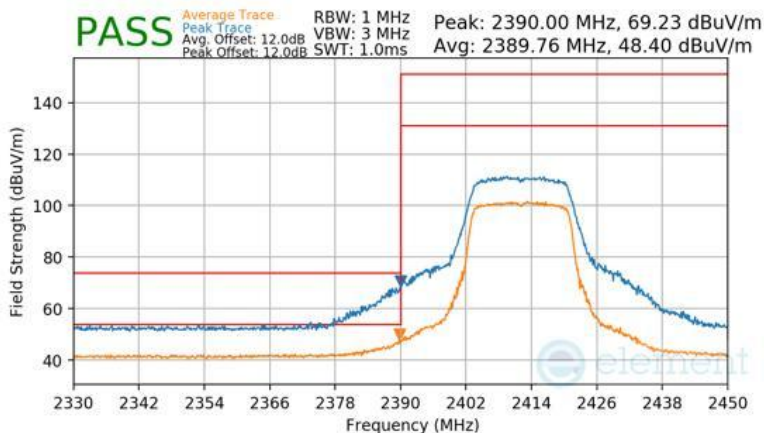
Plot 7-185 Radiated Restricted Lower Band Edge Measurement Antenna WF2b
