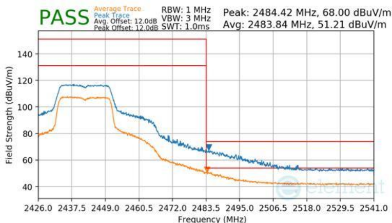
Plot 7-161 Radiated Restricted Upper Band Edge Measurement Antenna WF7b
