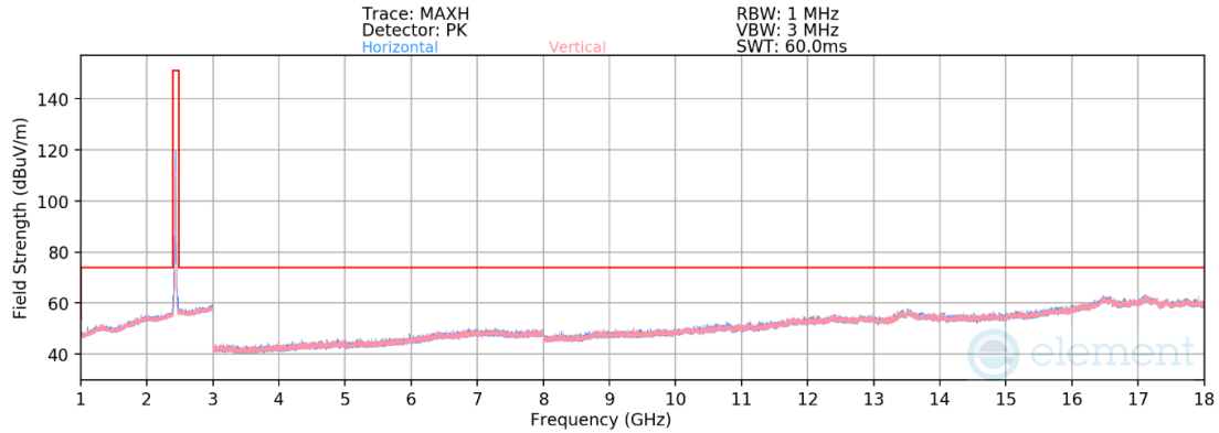
Plot 7-137. Radiated Spurious Emissions Above 1GHz CDD (802.11b – Ch. 6)
