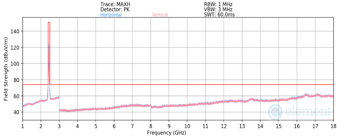
Plot 7-145. Radiated Spurious Emissions above 1GHz CDD (802.11be (SU) – Ch. 6)
