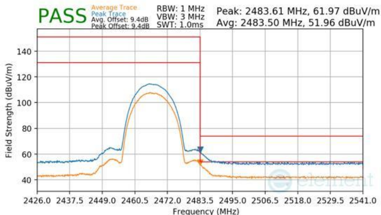
Plot 7-152 Radiated Restricted Upper Band Edge Measurement Antenna WF7b
