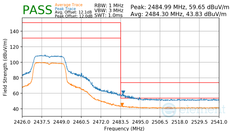
Plot 7-190 Radiated Restricted Upper Band Edge Measurement Antenna WF2b
