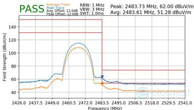
Plot 7-183 Radiated Restricted Upper Band Edge Measurement Antenna WF2b
