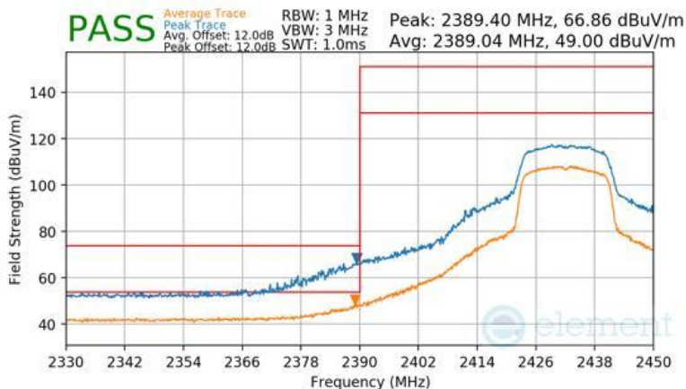
Plot 7-189 Radiated Restricted Lower Band Edge Measurement Antenna WF2b
