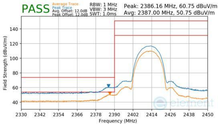
Plot 7-148 Radiated Restricted Lower Band Edge Measurement Antenna WF7b
