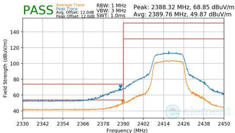
Plot 7-186 Radiated Restricted Lower Band Edge Measurement Antenna WF2b
