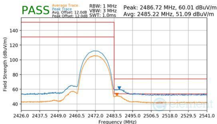
Plot 7-184 Radiated Restricted Upper Band Edge Measurement Antenna WF2b
