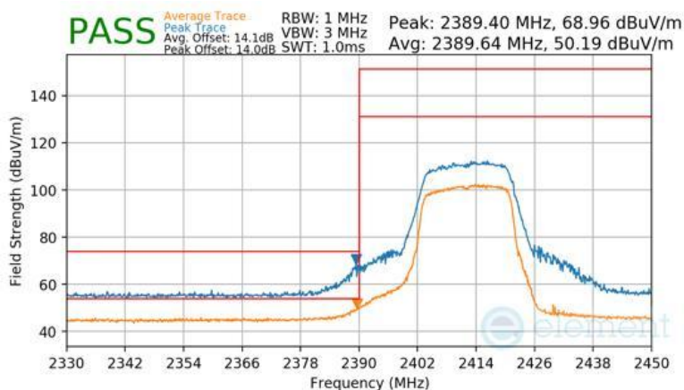
Plot 7-154 Radiated Restricted Lower Band Edge Measurement Antenna WF7b
