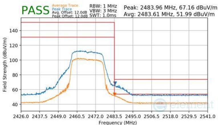
Plot 7-179 Radiated Restricted Upper Band Edge Measurement Antenna WF7b
