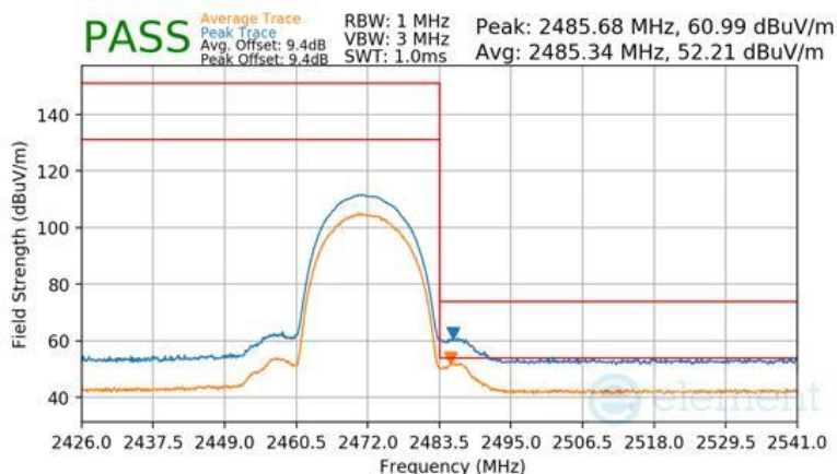
Plot 7-153 Radiated Restricted Upper Band Edge Measurement Antenna WF7b
