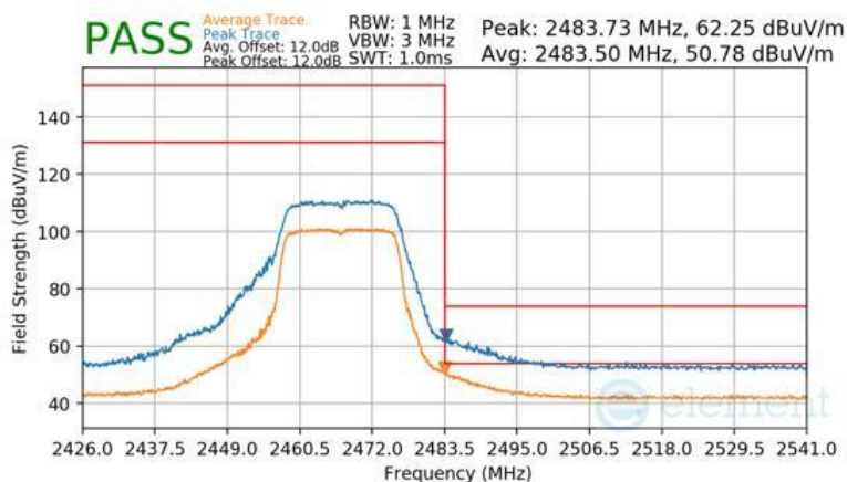
Plot 7-195 Radiated Restricted Upper Band Edge Measurement Antenna WF2b
