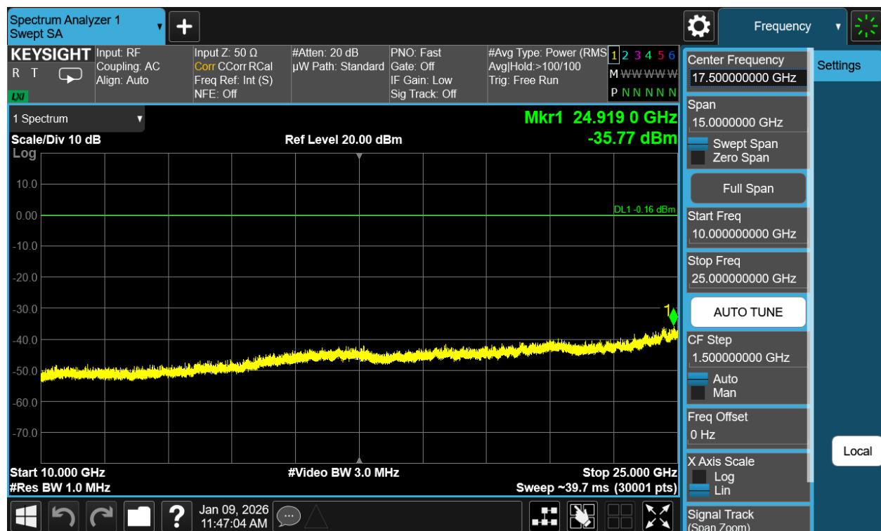
Plot 7-127. Conducted Spurious Plot Antenna WF7b (802.11b – Ch. 6)
