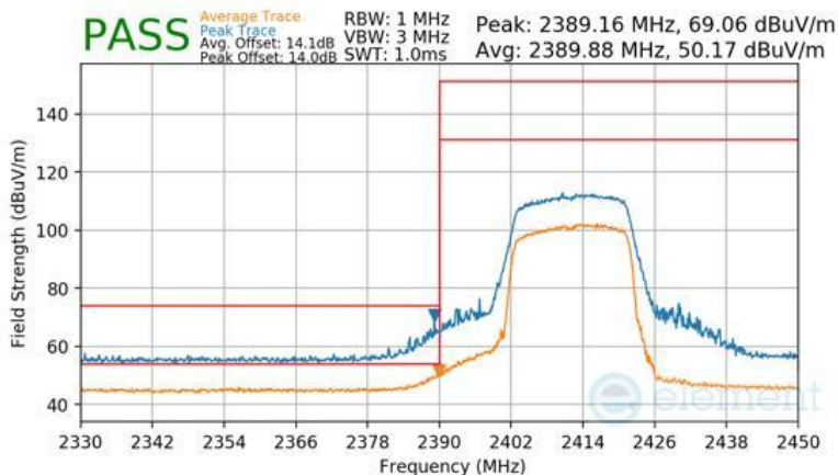
Plot 7-168 Radiated Restricted Lower Band Edge Measurement Antenna WF7b
