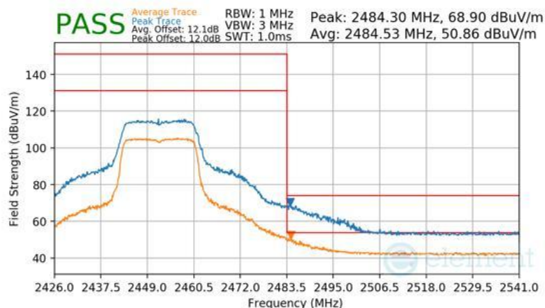
Plot 7-192 Radiated Restricted Upper Band Edge Measurement Antenna WF2b
