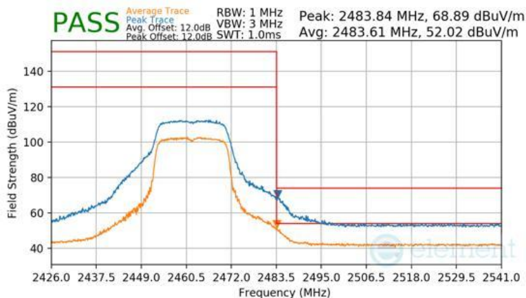
Plot 7-165 Radiated Restricted Upper Band Edge Measurement Antenna WF7b
