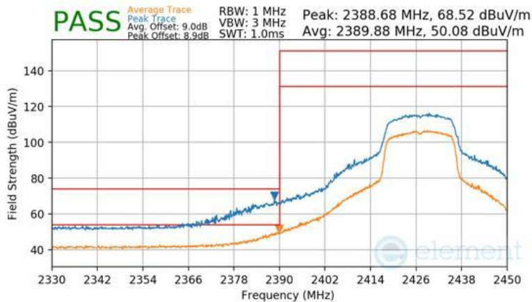
Plot 7-188 Radiated Restricted Lower Band Edge Measurement Antenna WF2b
