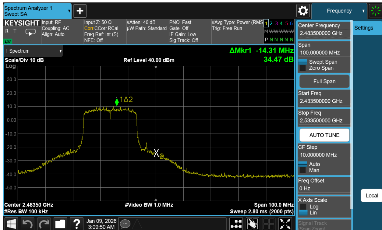
Plot 7-122. Band Edge Plot Antenna WF2b (802.11be (SU - 2.4GHz) – Ch. 12)
