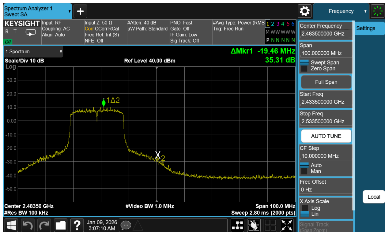
Plot 7-121. Band Edge Plot Antenna WF2b (802.11be (SU - 2.4GHz) – Ch. 11)
