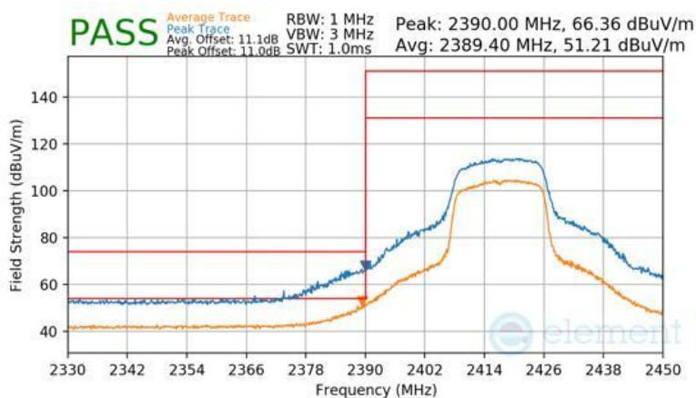
Plot 7-155 Radiated Restricted Lower Band Edge Measurement Antenna WF7b
