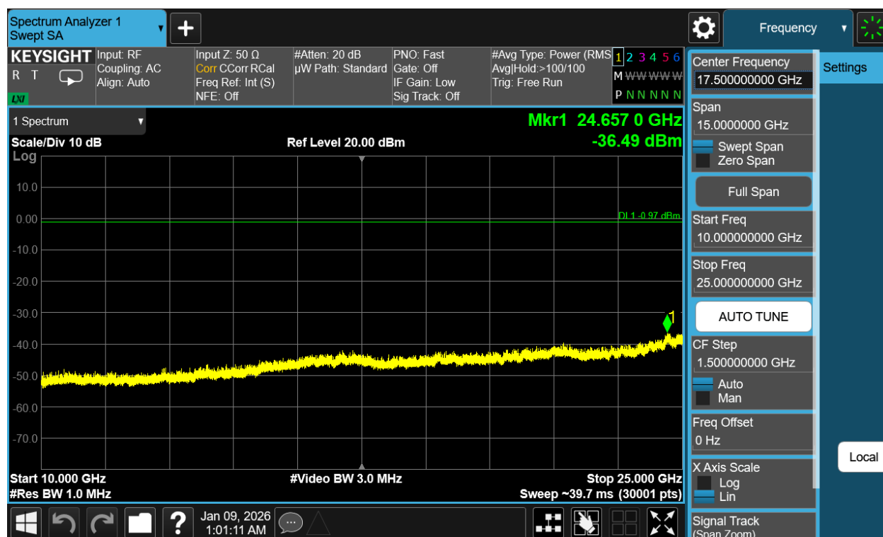
Plot 7-135. Conducted Spurious Plot Antenna WF2b (802.11b – Ch. 11)
