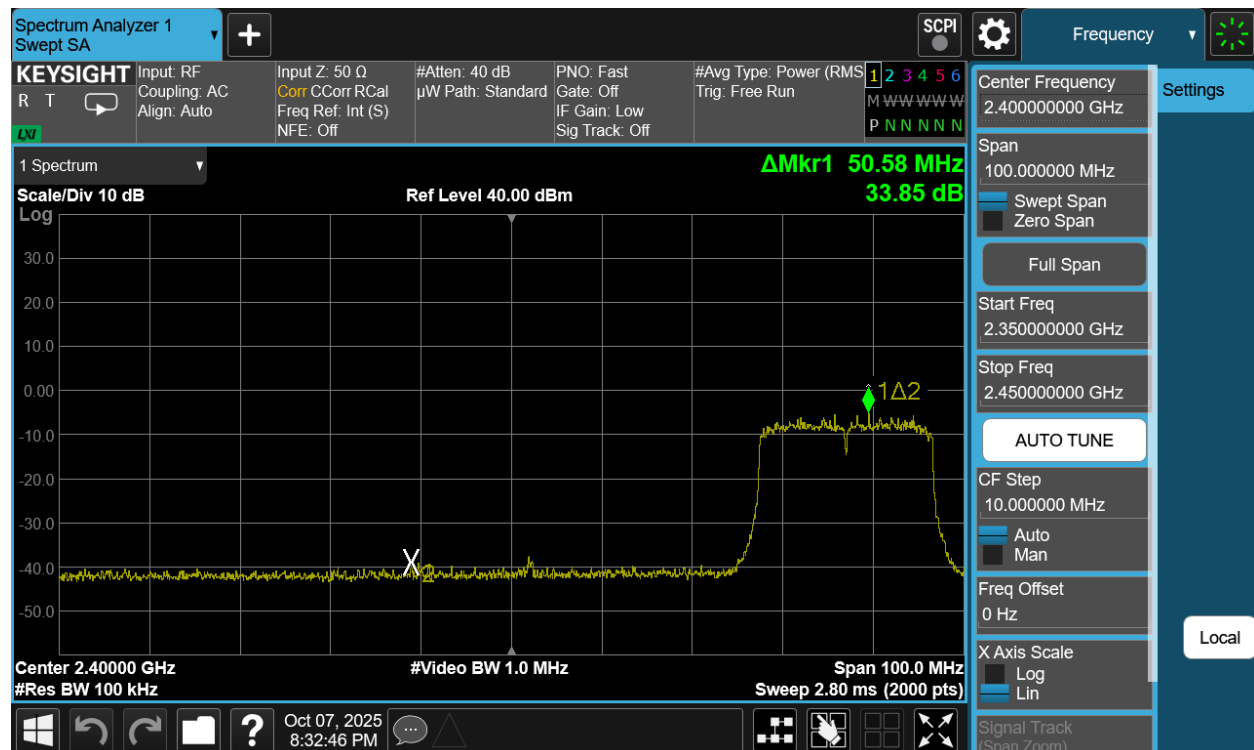
Plot 7-115. Band Edge Plot Antenna WF2b (802.11be (SU - 2.4GHz) – Ch. 6 (Low))
