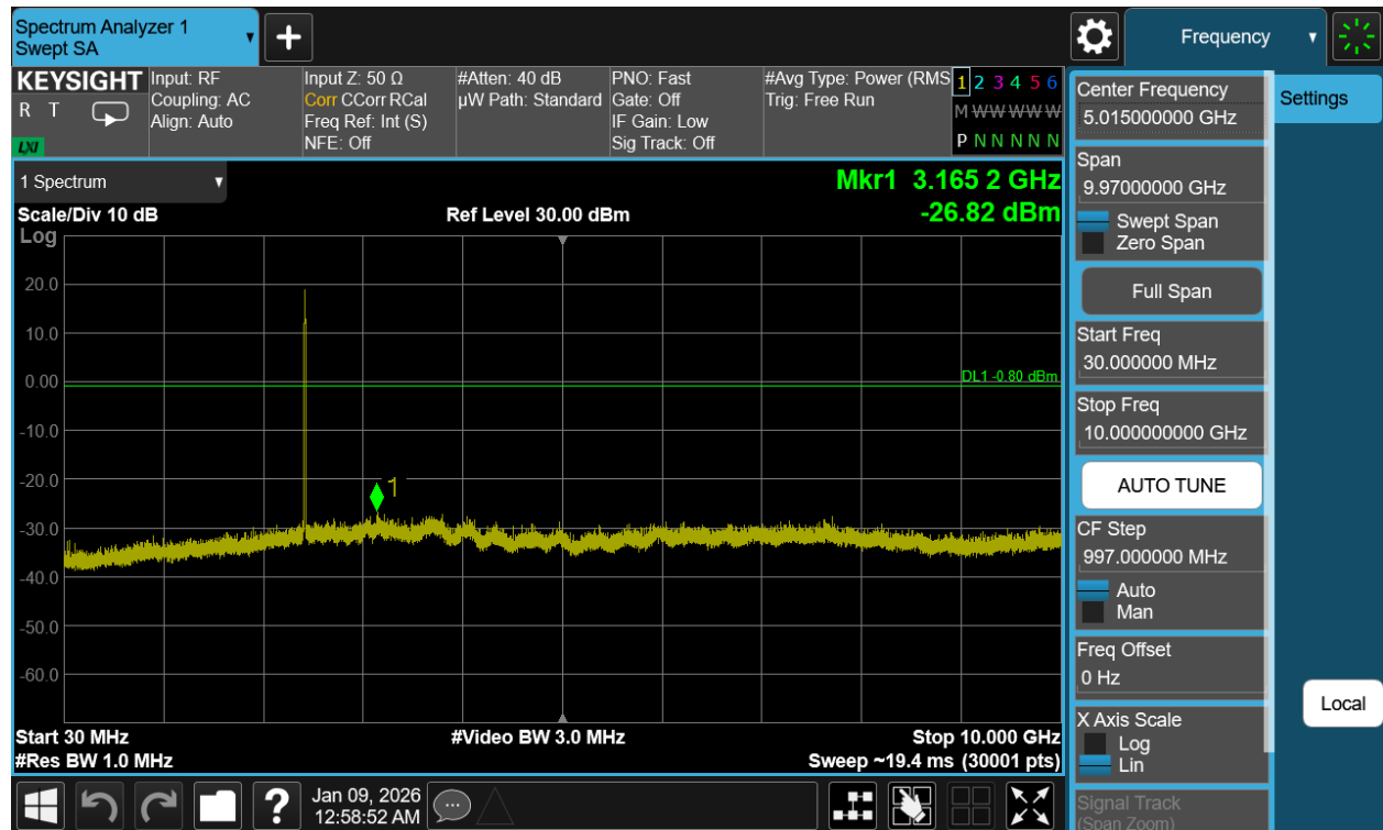
Plot 7-132. Conducted Spurious Plot Antenna WF2b (802.11b – Ch. 6)
