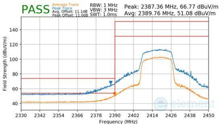
Plot 7-169 Radiated Restricted Lower Band Edge Measurement Antenna WF7b
