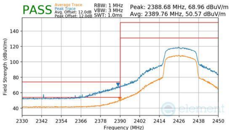
Plot 7-171 Radiated Restricted Lower Band Edge Measurement Antenna WF7b
