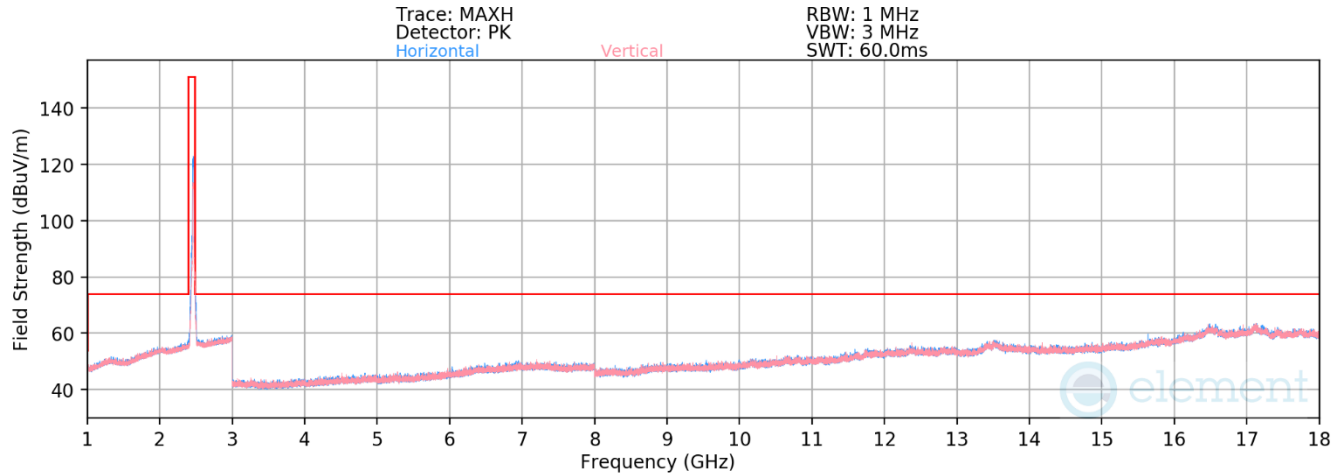
Plot 7-147. Radiated Spurious Emissions above 1GHz CDD (802.11be (SU) – Ch. 11)
