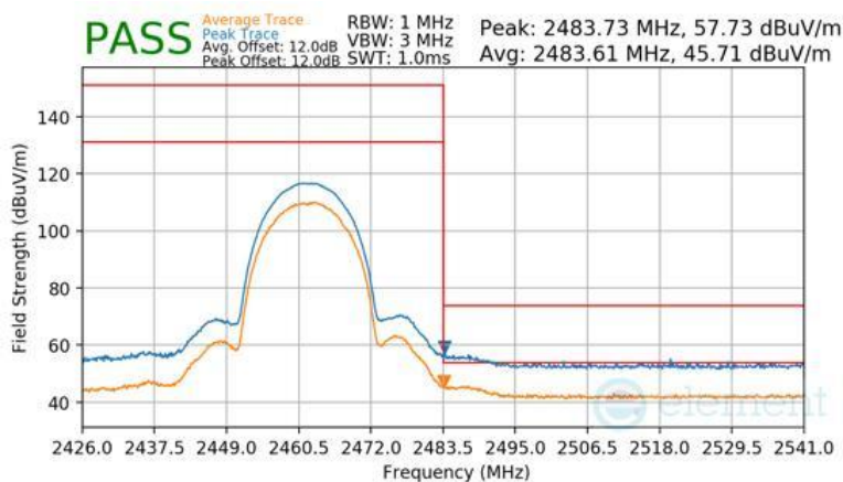
Plot 7-151 Radiated Restricted Upper Band Edge Measurement Antenna WF7b
