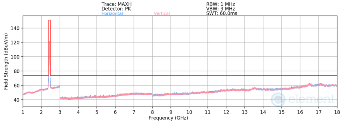
Plot 7-141. Radiated Spurious Emissions Above 1GHz CDD (802.11n – Ch. 6)
