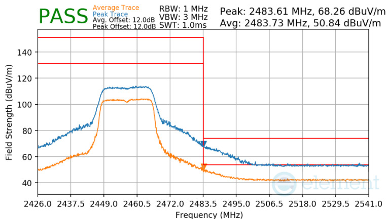
Plot 7-193 Radiated Restricted Upper Band Edge Measurement Antenna WF2b
