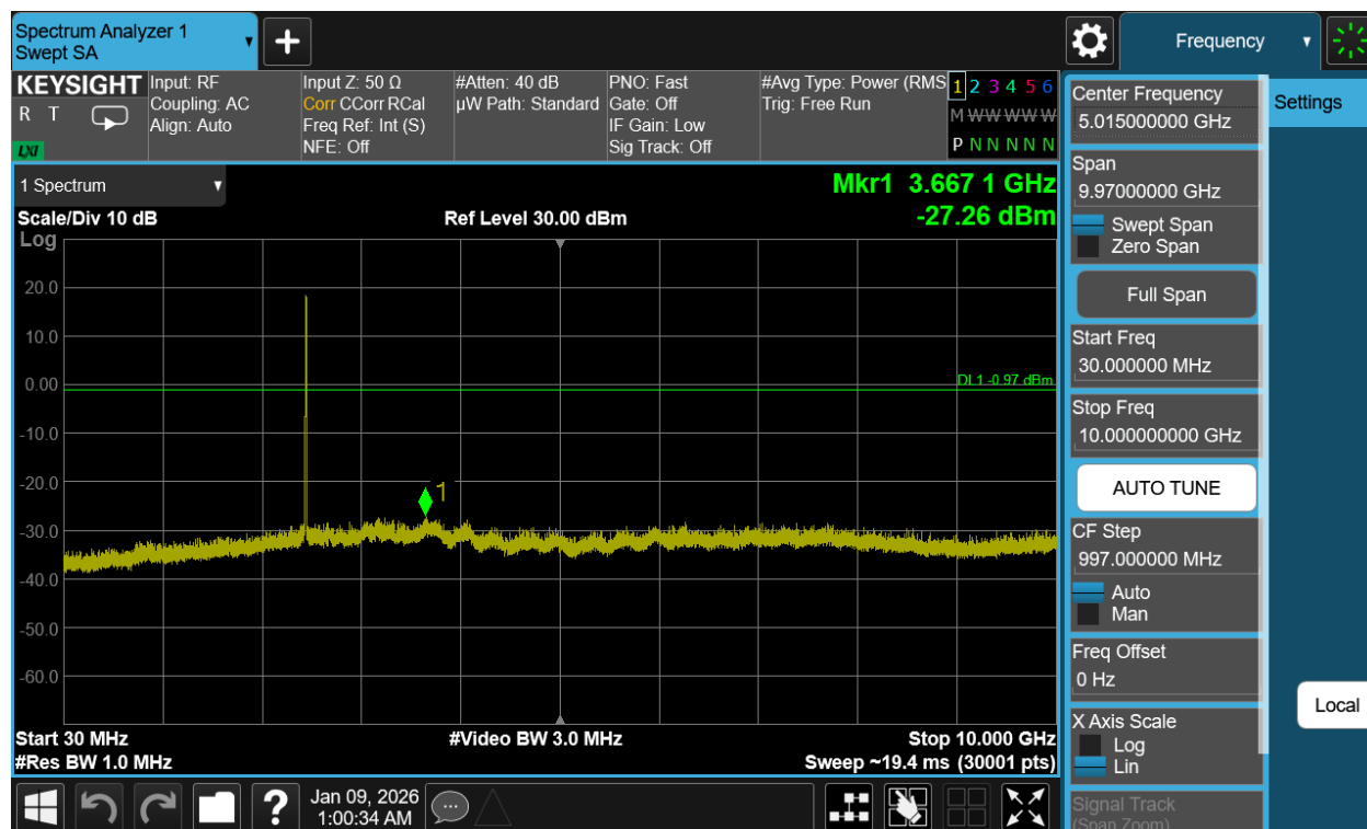
Plot 7-134. Conducted Spurious Plot Antenna WF2b (802.11b – Ch. 11)
