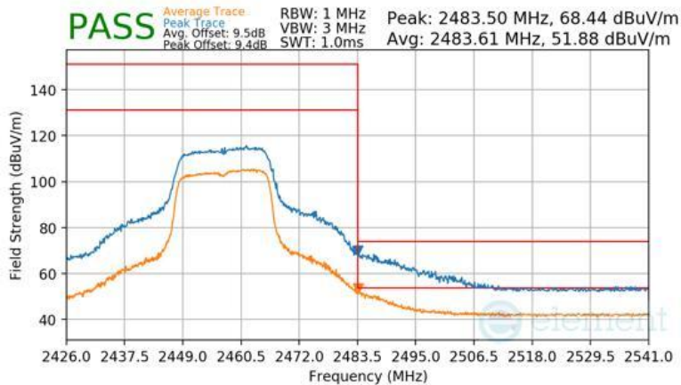
Plot 7-164 Radiated Restricted Upper Band Edge Measurement Antenna WF7b
