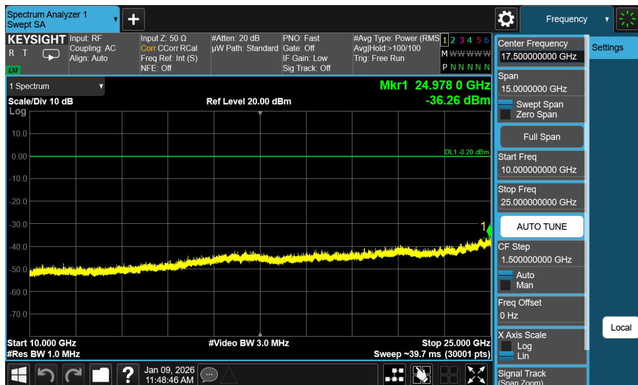
Plot 7-129. Conducted Spurious Plot Antenna WF7b (802.11b – Ch. 11)
