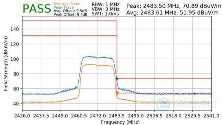
Plot 7-180 Radiated Restricted Upper Band Edge Measurement Antenna WF7b
