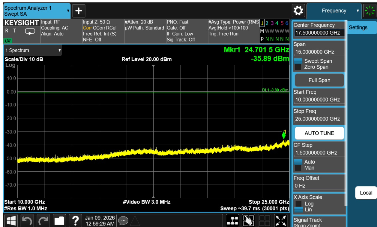
Plot 7-133. Conducted Spurious Plot Antenna WF2b (802.11b – Ch. 6)
