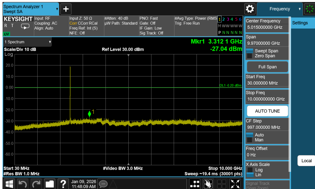
Plot 7-128. Conducted Spurious Plot Antenna WF7b (802.11b – Ch. 11)
