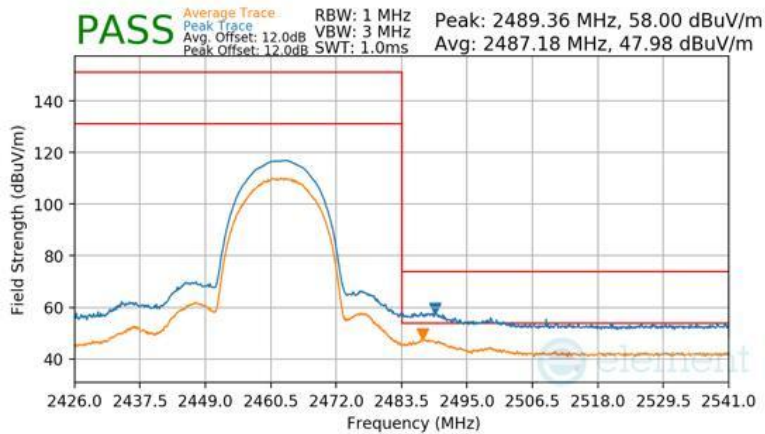
Plot 7-182 Radiated Restricted Upper Band Edge Measurement Antenna WF2b
