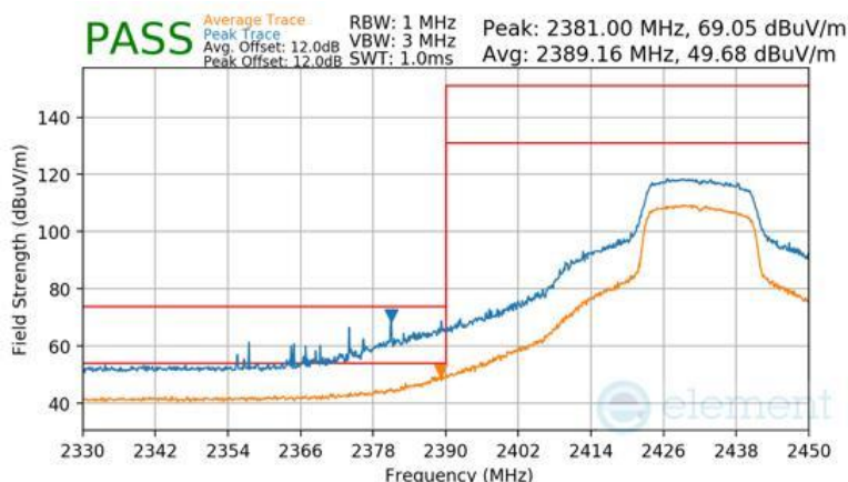
Plot 7-158 Radiated Restricted Lower Band Edge Measurement Antenna WF7b
