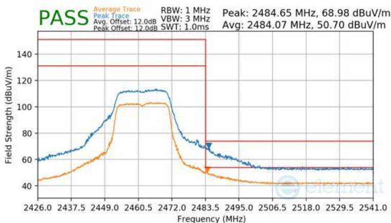
Plot 7-194 Radiated Restricted Upper Band Edge Measurement Antenna WF2b
