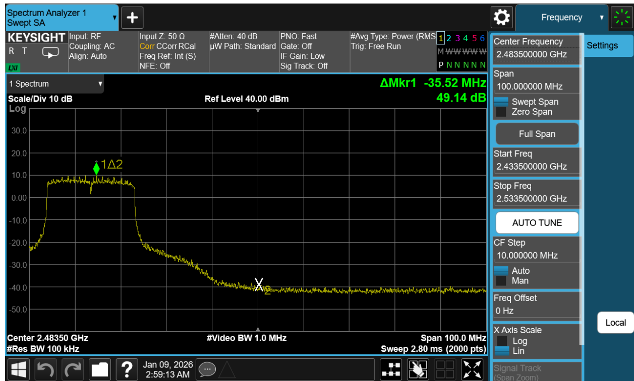
Plot 7-118. Band Edge Plot Antenna WF2b (802.11be (SU - 2.4GHz) – Ch. 8)
