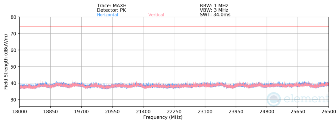
Plot 7-142. Radiated Spurious Emissions Above 18GHz CDD (802.11n – Ch.6)
