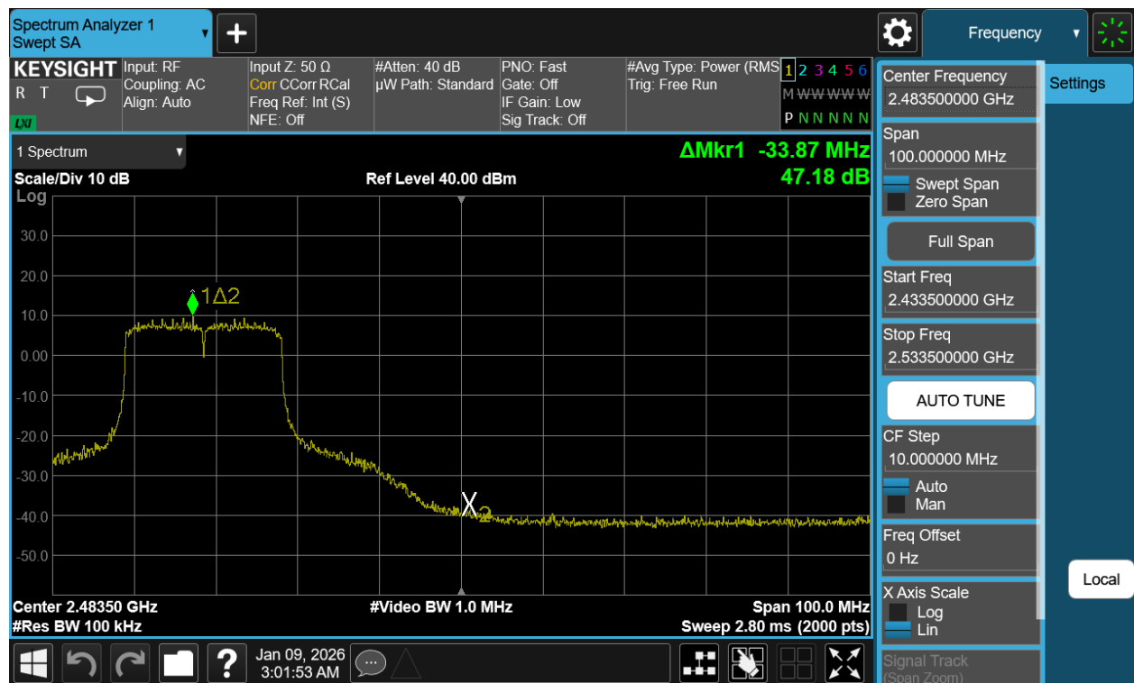
Plot 7-119. Band Edge Plot Antenna WF2b (802.11be (SU - 2.4GHz) – Ch. 9)
