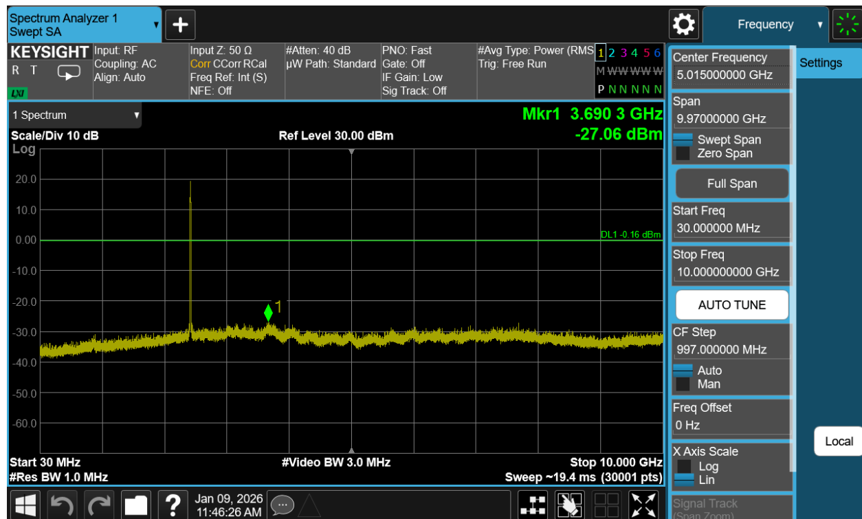
Plot 7-126. Conducted Spurious Plot Antenna WF7b (802.11b – Ch. 6)
