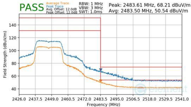
Plot 7-191 Radiated Restricted Upper Band Edge Measurement Antenna WF2b
