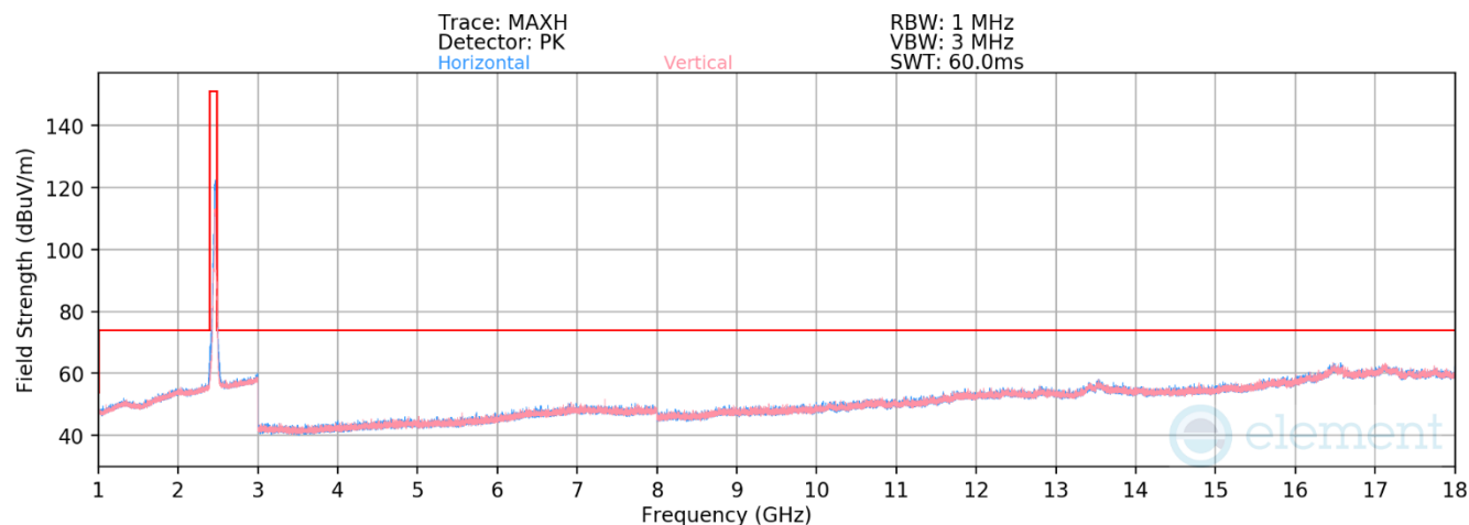
Plot 7-143. Radiated Spurious Emissions above 1GHz CDD (802.11n – Ch. 11)
