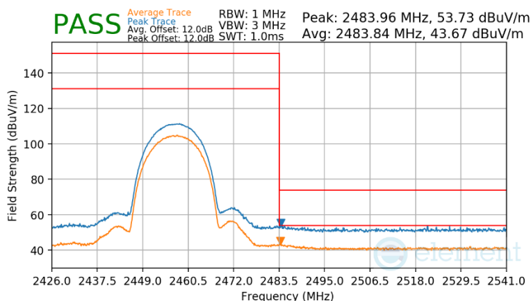
Plot 7-150 Radiated Restricted Upper Band Edge Measurement Antenna WF7b
