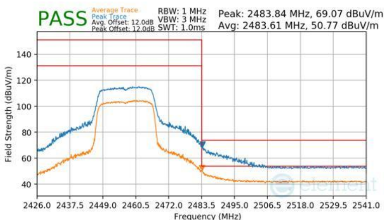
Plot 7-177 Radiated Restricted Upper Band Edge Measurement Antenna WF7b
