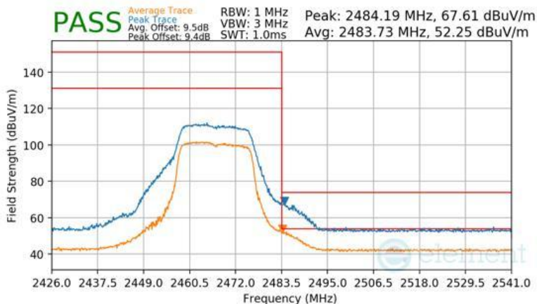
Plot 7-166 Radiated Restricted Upper Band Edge Measurement Antenna WF7b
