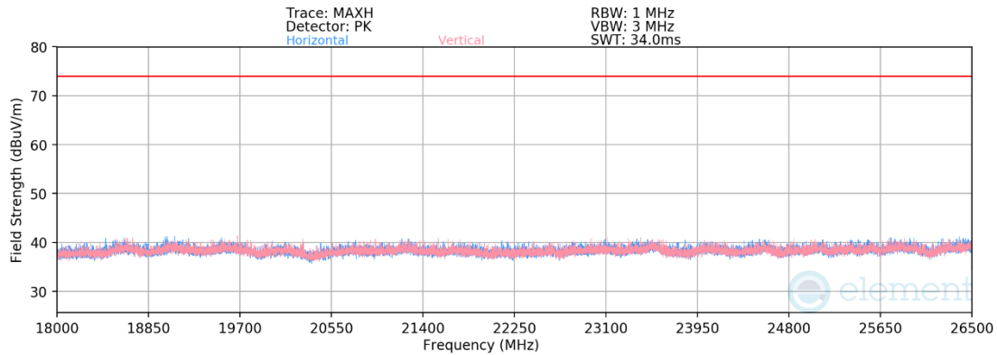
Plot 7-139. Radiated Spurious Emissions Above 18GHz CDD (802.11b – Ch.6)
