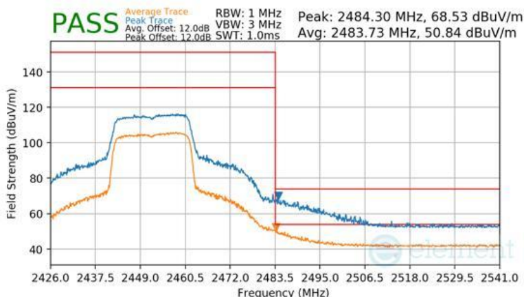
Plot 7-176 Radiated Restricted Upper Band Edge Measurement Antenna WF7b
