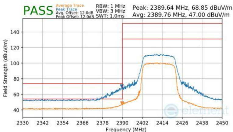
Plot 7-197 Radiated Restricted Lower Band Edge Measurement Antenna WF2b
