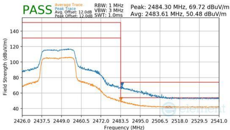
Plot 7-175 Radiated Restricted Upper Band Edge Measurement Antenna WF7b
