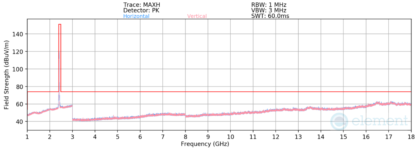
Plot 7-136. Radiated Spurious Emissions Above 1GHz CDD (802.11b – Ch. 1)
