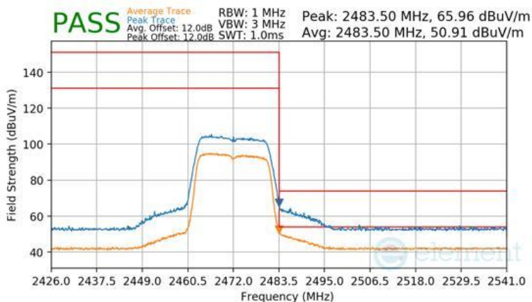
Plot 7-167 Radiated Restricted Upper Band Edge Measurement Antenna WF7b
