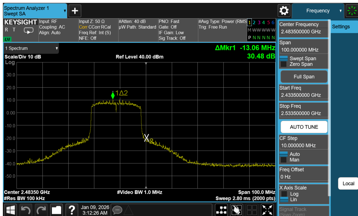
Plot 7-123. Band Edge Plot Antenna WF2b (802.11be (SU - 2.4GHz) – Ch. 13)
