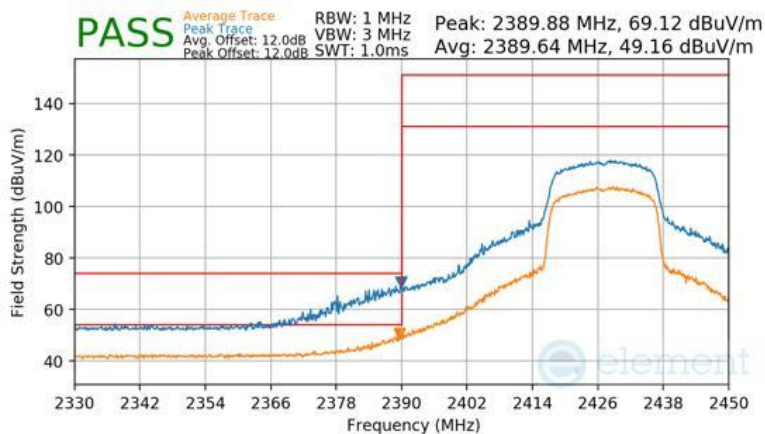
Plot 7-200 Radiated Restricted Lower Band Edge Measurement Antenna WF2b
