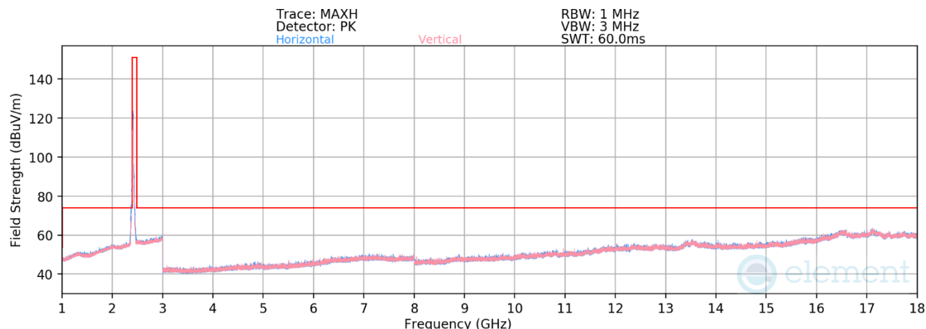
Plot 7-144. Radiated Spurious Emissions above 1GHz CDD (802.11be (SU) – Ch. 1)
