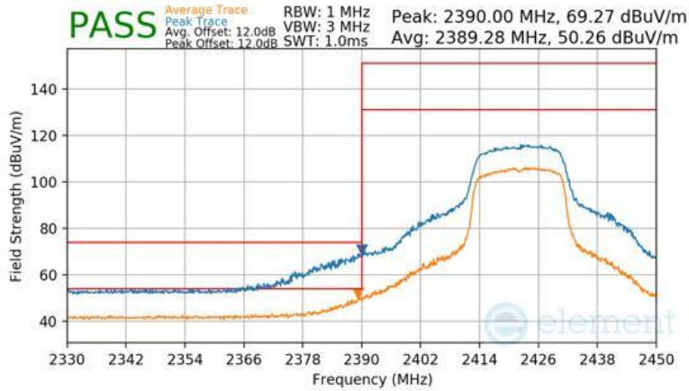
Plot 7-187 Radiated Restricted Lower Band Edge Measurement Antenna WF2b
