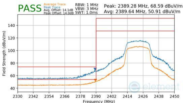
Plot 7-156 Radiated Restricted Lower Band Edge Measurement Antenna WF7b
