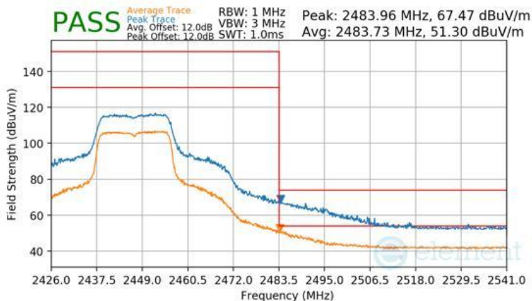
Plot 7-162 Radiated Restricted Upper Band Edge Measurement Antenna WF7b
