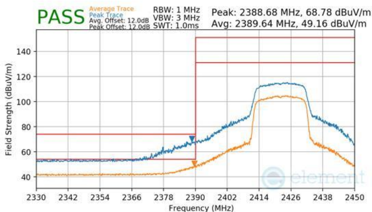
Plot 7-199 Radiated Restricted Lower Band Edge Measurement Antenna WF2b
