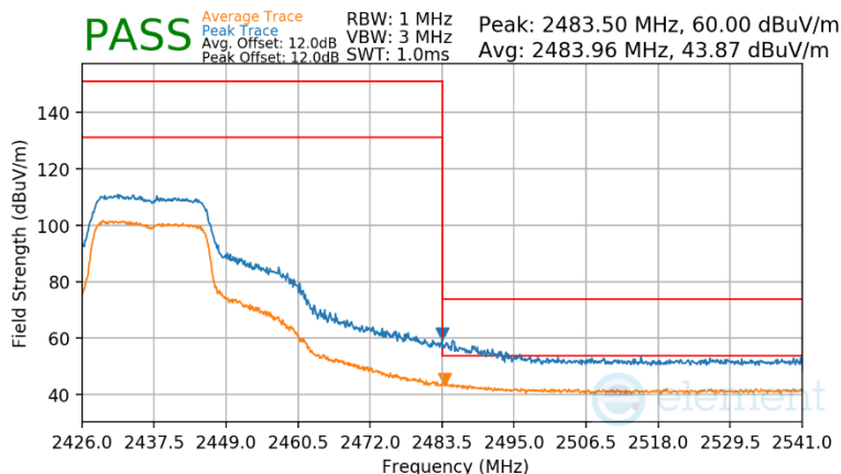
Plot 7-160 Radiated Restricted Upper Band Edge Measurement Antenna WF7b
