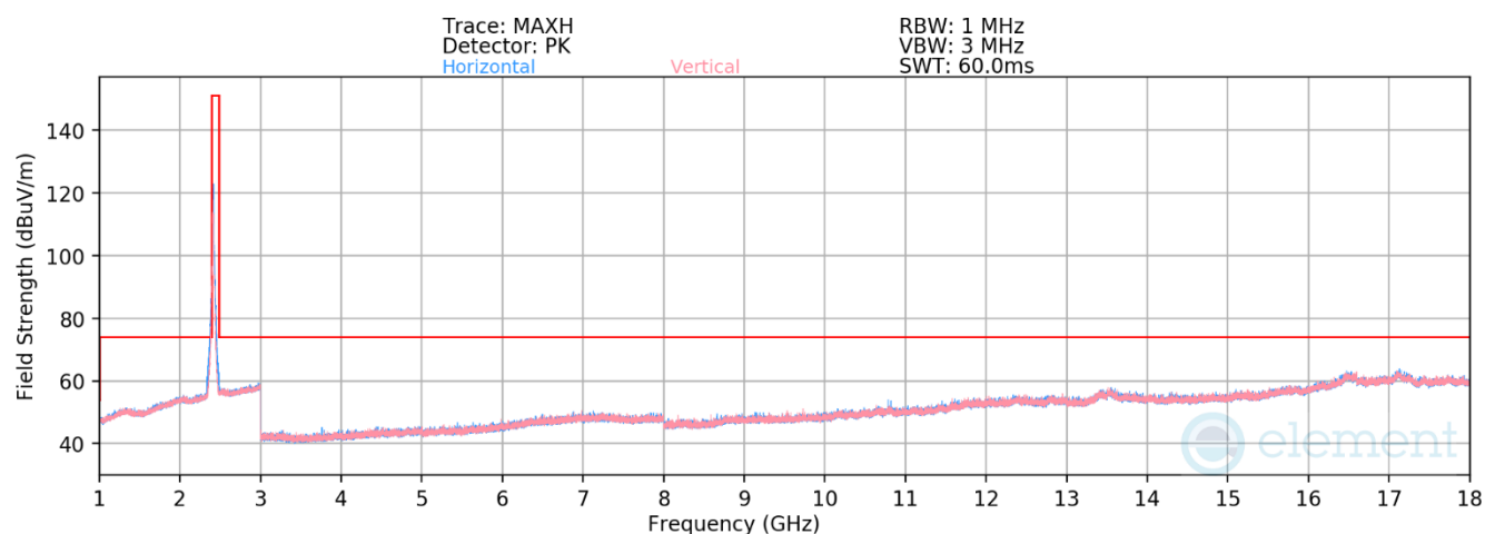
Plot 7-140. Radiated Spurious Emissions Above 1GHz CDD (802.11n – Ch. 1)
