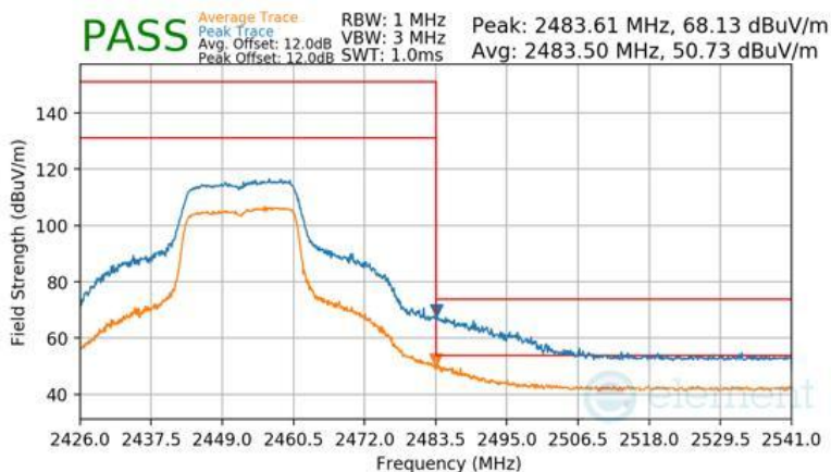
Plot 7-163 Radiated Restricted Upper Band Edge Measurement Antenna WF7b
