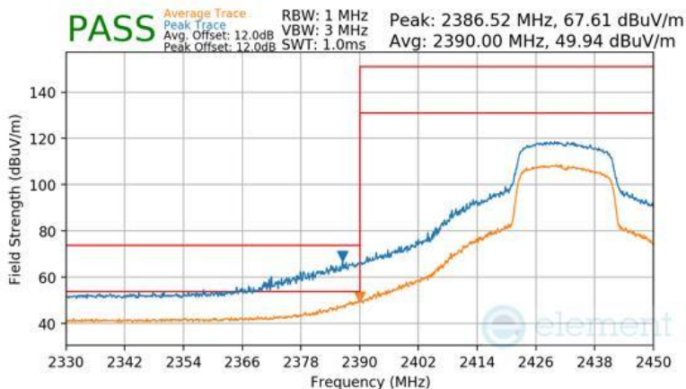
Plot 7-172 Radiated Restricted Lower Band Edge Measurement Antenna WF7b
