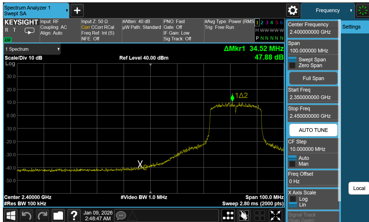
Plot 7-114. Band Edge Plot Antenna WF2b (802.11be (SU - 2.4GHz) – Ch. 5)
