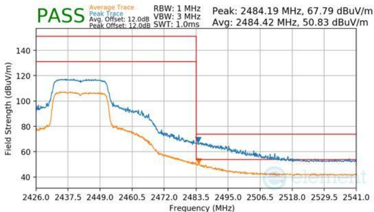
Plot 7-174 Radiated Restricted Upper Band Edge Measurement Antenna WF7b
