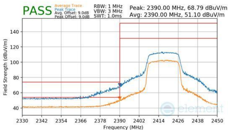
Plot 7-198 Radiated Restricted Lower Band Edge Measurement Antenna WF2b
