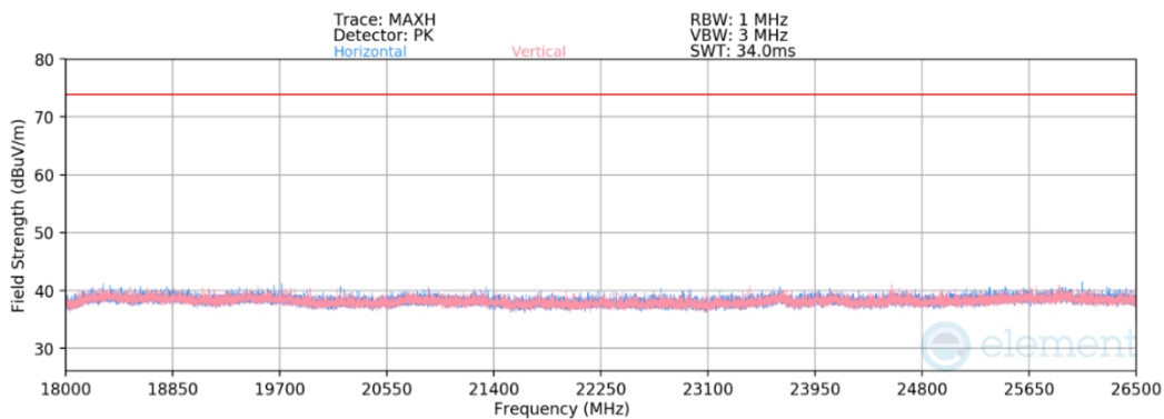
Plot 7-146. Radiated Spurious Emissions above 18GHz CDD (802.11be (SU) – Ch.6)
