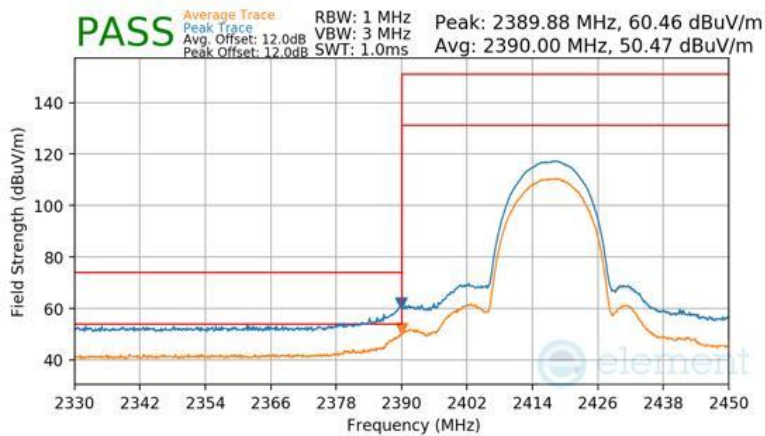
Plot 7-149 Radiated Restricted Lower Band Edge Measurement Antenna WF7b
