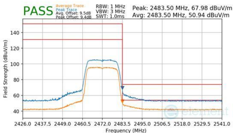
Plot 7-196 Radiated Restricted Upper Band Edge Measurement Antenna WF2b
