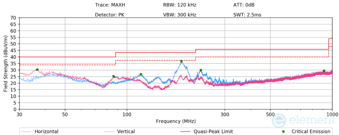
Plot 7-247. Radiated Spurious Emissions Below 1GHz CDD 11be - SU Ch.6, with AC/DC Adaptor
