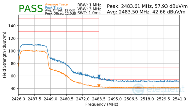
Plot 7-203 Radiated Restricted Upper Band Edge Measurement Antenna WF2b
