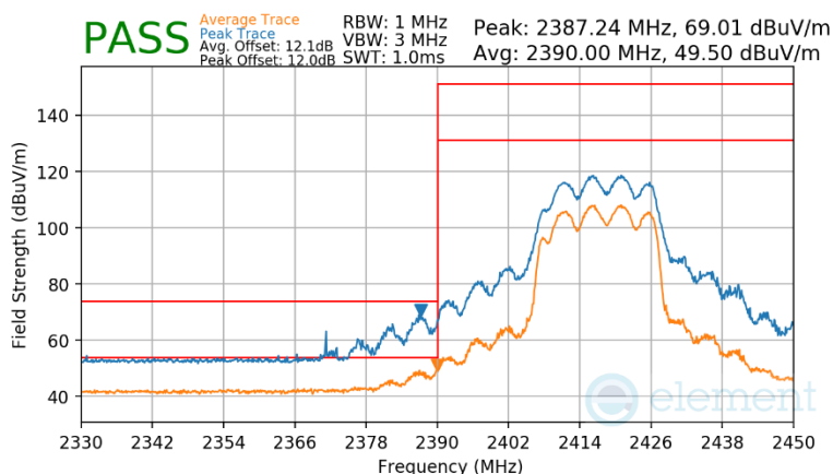
Plot 7-233 Radiated Restricted Lower Band Edge Measurement CDD
