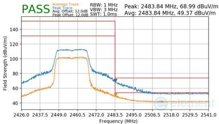
Plot 7-207 Radiated Restricted Upper Band Edge Measurement Antenna WF2b
