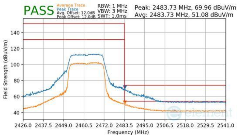
Plot 7-208 Radiated Restricted Upper Band Edge Measurement Antenna WF2b
