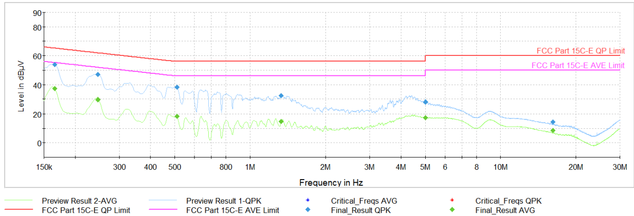
Plot 7-251. AC Line Conducted Plot with CDD 11be - SU Ch.6 (N, with AC/DC Adaptor)
