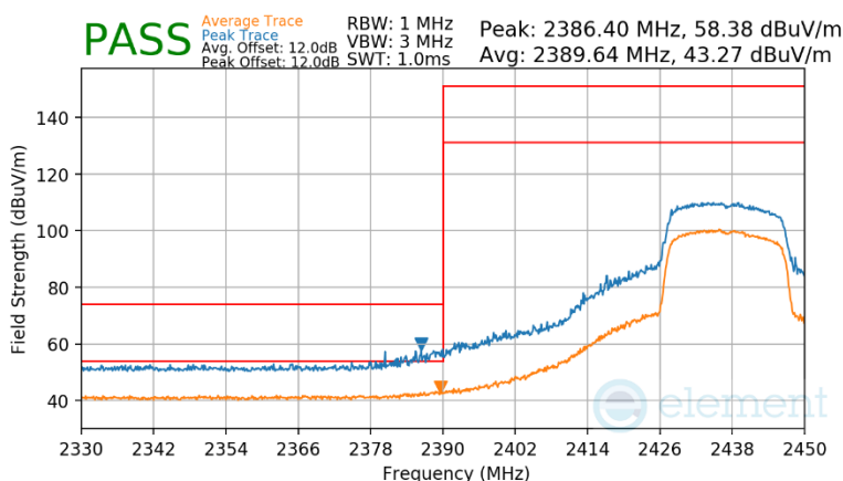
Plot 7-202 Radiated Restricted Lower Band Edge Measurement Antenna WF2b
