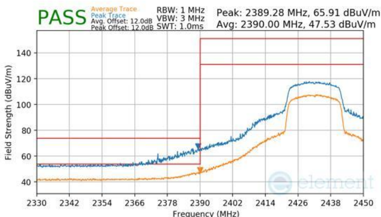
Plot 7-201 Radiated Restricted Lower Band Edge Measurement Antenna WF2b
