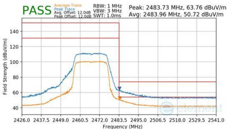
Plot 7-209 Radiated Restricted Upper Band Edge Measurement Antenna WF2b
