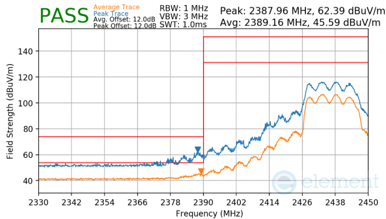
Plot 7-237 Radiated Restricted Lower Band Edge Measurement CDD
