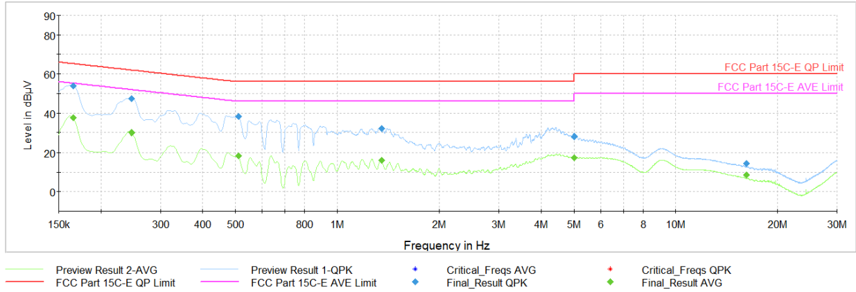
Plot 7-249. AC Line Conducted Plot with CDD 11n Ch.6 (N, with AC/DC Adaptor)
