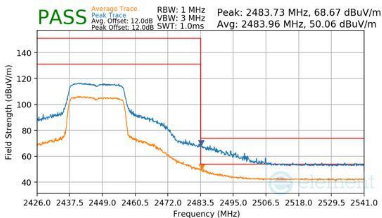
Plot 7-205 Radiated Restricted Upper Band Edge Measurement Antenna WF2b
