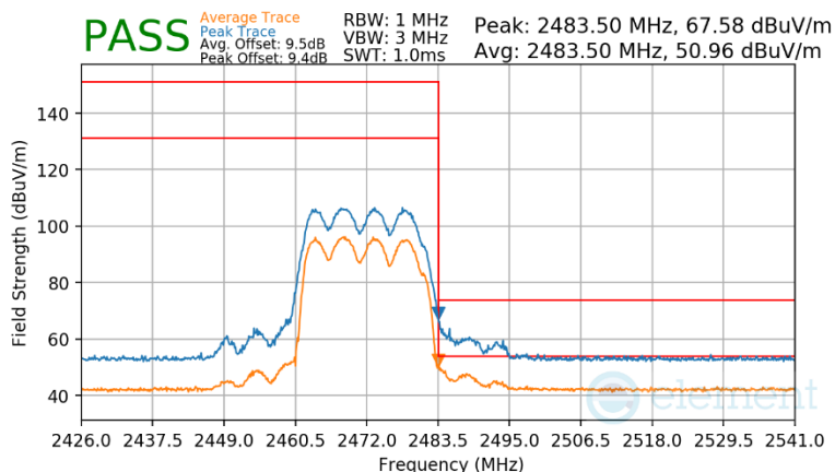
Plot 7-245 Radiated Restricted Upper Band Edge Measurement CDD
