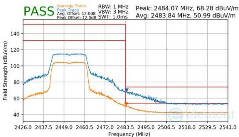
Plot 7-206 Radiated Restricted Upper Band Edge Measurement Antenna WF2b
