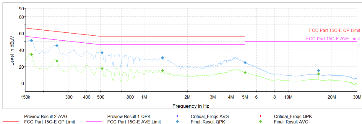
Plot 7-248. AC Line Conducted Plot with CDD 11n Ch.6 (L1, with AC/DC Adaptor)
