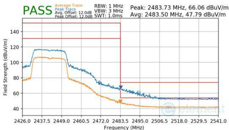
Plot 7-204 Radiated Restricted Upper Band Edge Measurement Antenna WF2b
