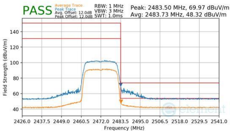
Plot 7-210 Radiated Restricted Upper Band Edge Measurement Antenna WF2b
