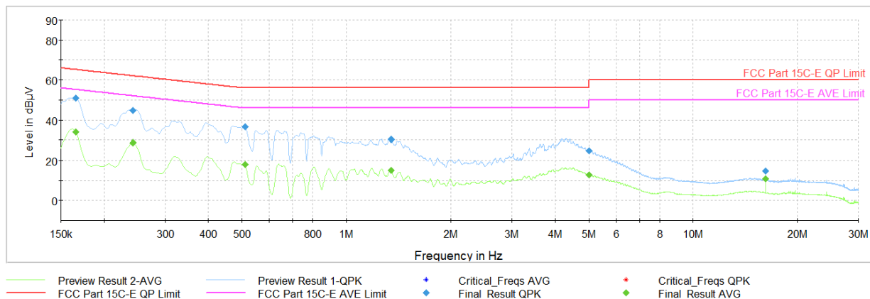
Plot 7-250. AC Line Conducted Plot with CDD 11be - SU Ch.6 (L1, with AC/DC Adaptor)
