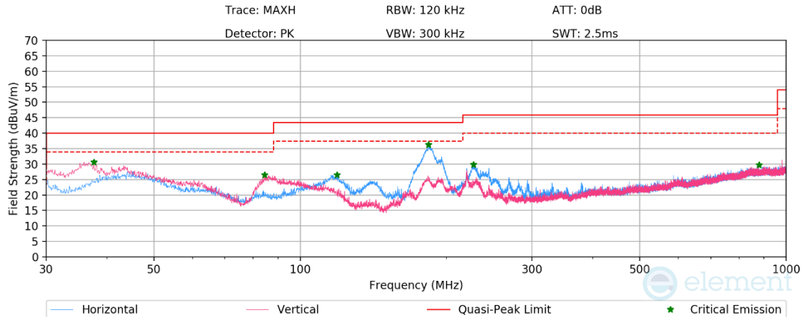
Plot 7-246. Radiated Spurious Emissions Below 1GHz CDD 11n Ch.6, with AC/DC Adaptor
