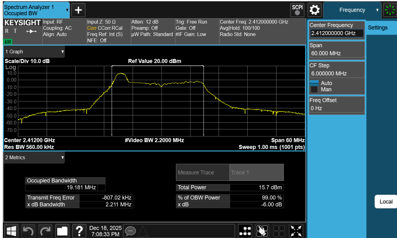
Plot 7-5 99% OBW Antenna WF2b (20MHz BW 802.11be(RU) RU26 Index0 - Ch.1)
