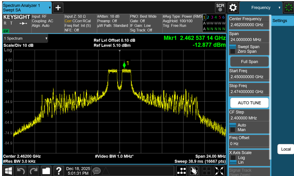
Plot 7-25 PSD CDD Antenna WF7b (20MHz BW 802.11be(RU) RU26 Index4 - Ch.11)
