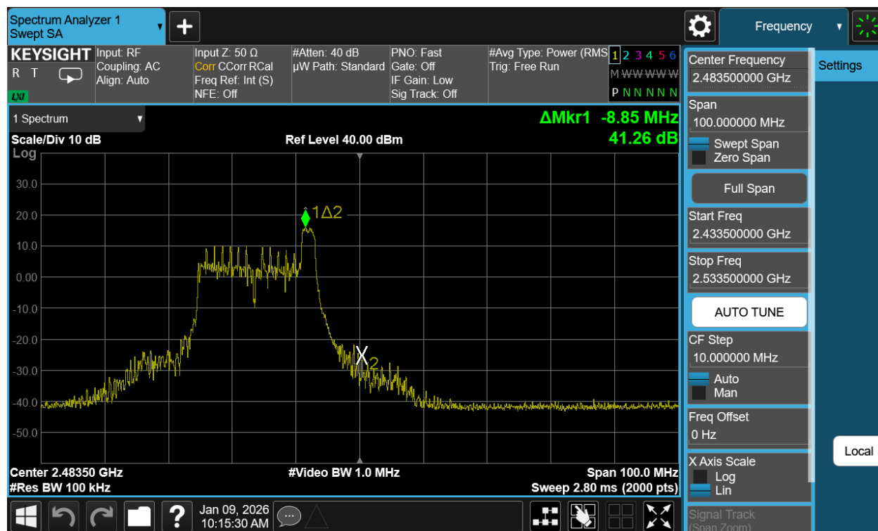
Plot 7-35. Band Edge Antenna WF7b (802.11be OFDMA – RU26 Index 8 – Ch. 12)
