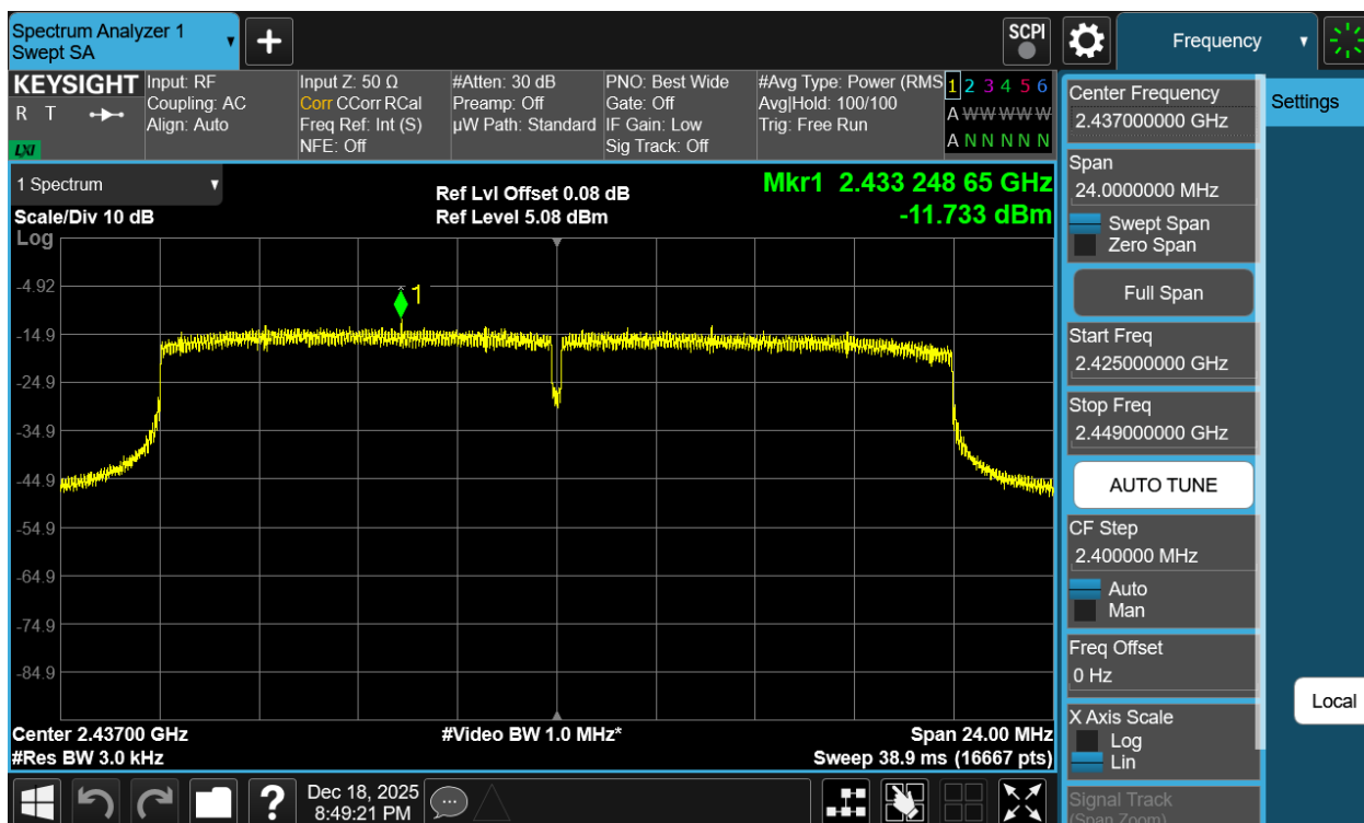
Plot 7-30 PSD CDD Antenna WF2b (20MHz BW 802.11be(RU) RU242 Index61 - Ch.6)
