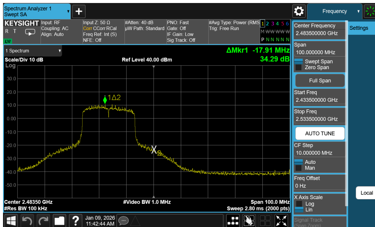
Plot 7-49. Band Edge Antenna WF7b (802.11be OFDMA – RU242 – Ch. 12)
