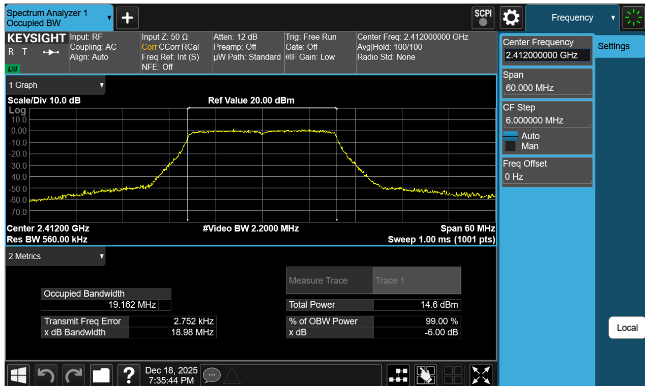
Plot 7-6 99% OBW Antenna WF2b (20MHz BW 802.11be(RU) RU242 Index61 - Ch.1)
