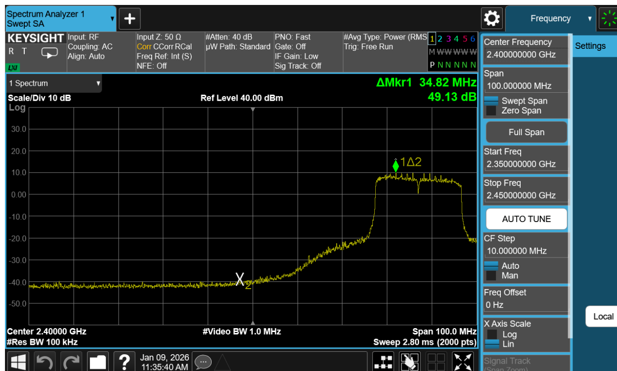
Plot 7-42. Band Edge Antenna WF7b (802.11be OFDMA – RU242 – Ch. 6(Low Channel))
