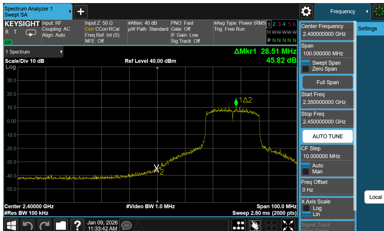
Plot 7-40. Band Edge Antenna WF7b (802.11be OFDMA – RU242 – Ch. 4)
