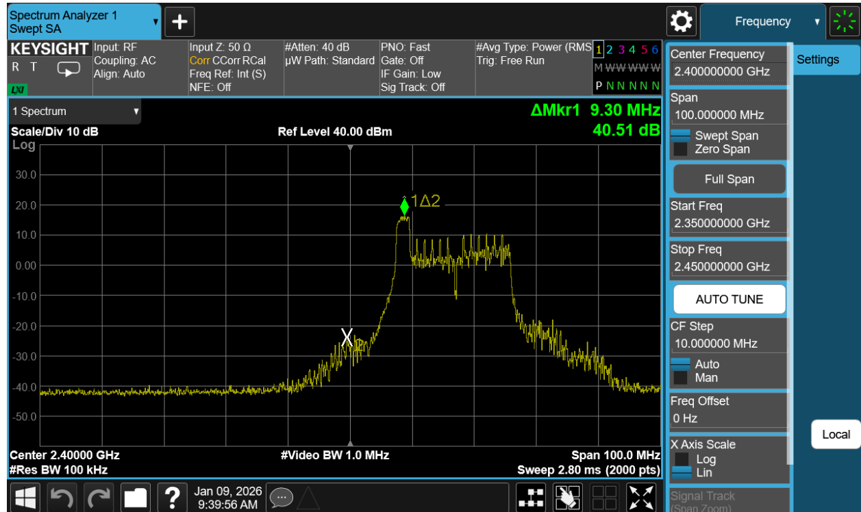
Plot 7-34. Band Edge Antenna WF7b (802.11be OFDMA – RU26 Index 0 – Ch. 2)
