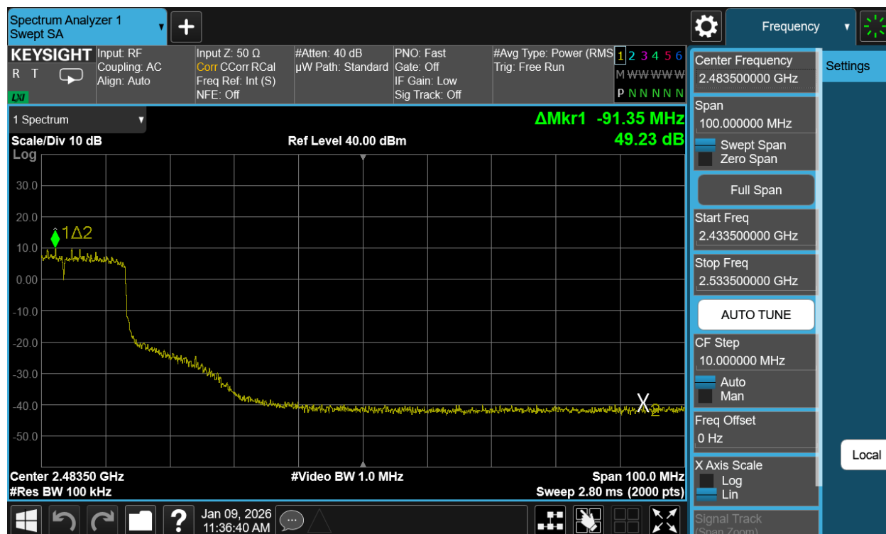
Plot 7-43. Band Edge Antenna WF7b (802.11be OFDMA – RU242 – Ch. 6(High Channel))
