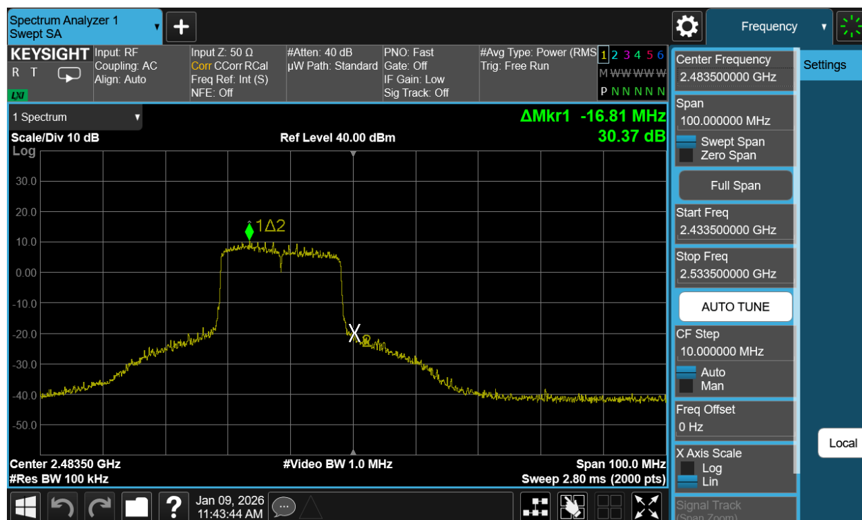
Plot 7-50. Band Edge Antenna WF7b (802.11be OFDMA – RU242 – Ch. 13)
