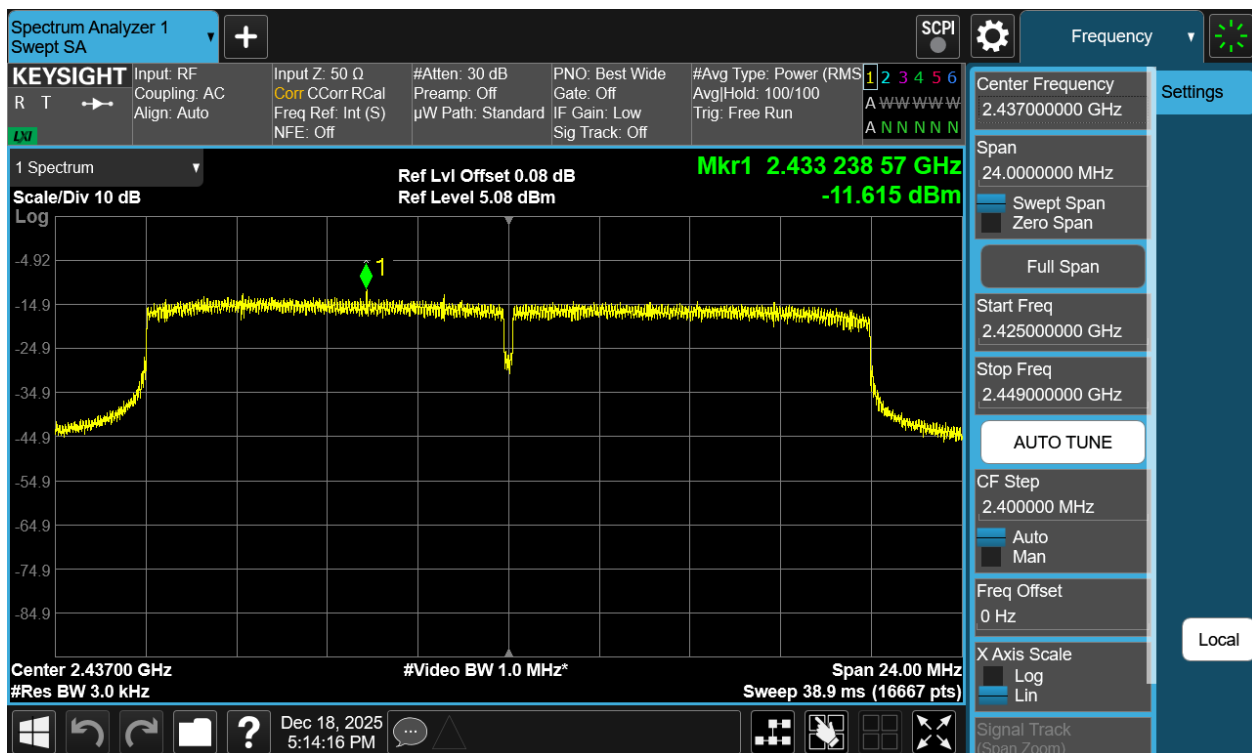
Plot 7-26 PSD CDD Antenna WF7b (20MHz BW 802.11be(RU) RU242 Index61 - Ch.6)
