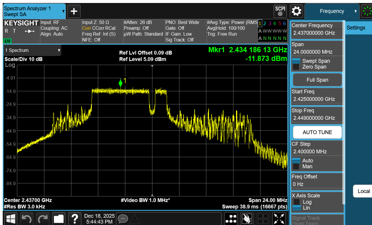
Plot 7-19 PSD Antenna WF7b (20MHz BW 802.11be(RU) RU52+26 Index71 - Ch.6)
