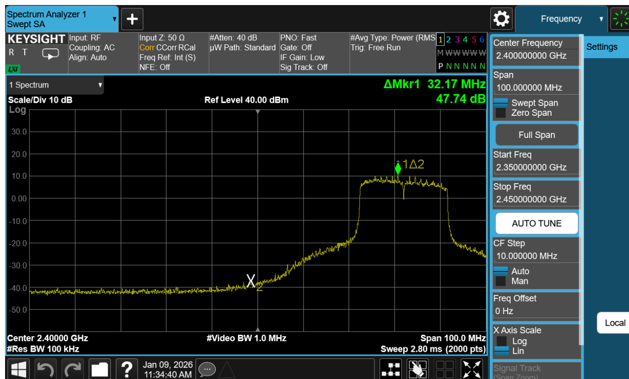
Plot 7-41. Band Edge Antenna WF7b (802.11be OFDMA – RU242 – Ch. 5)
