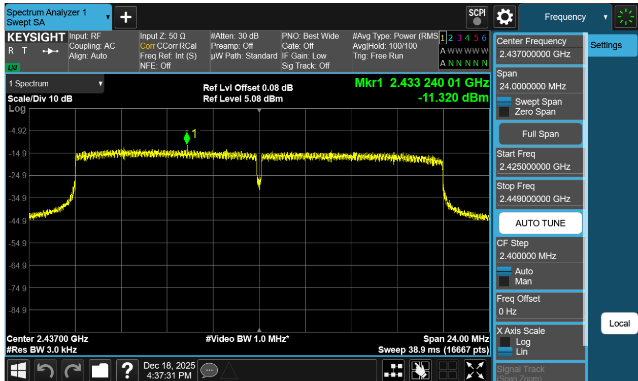
Plot 7-18 PSD Antenna WF7b (20MHz BW 802.11be(RU) RU242 Index61 - Ch.6)
