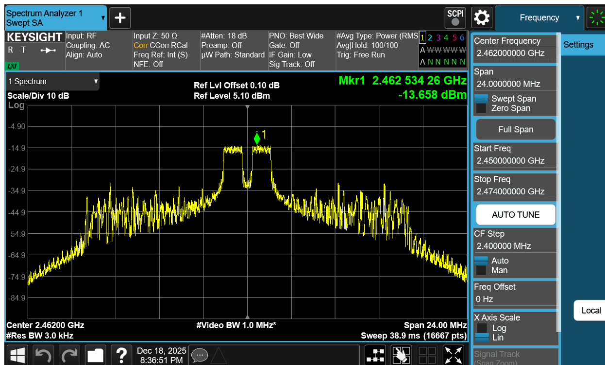
Plot 7-29 PSD CDD Antenna WF2b (20MHz BW 802.11be(RU) RU26 Index4 - Ch.11)
