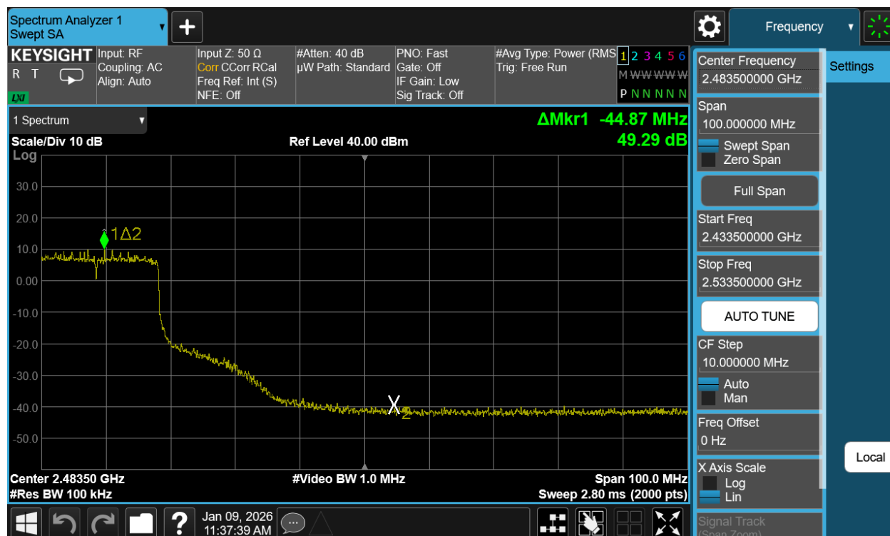
Plot 7-44. Band Edge Antenna WF7b (802.11be OFDMA – RU242 – Ch. 7)
