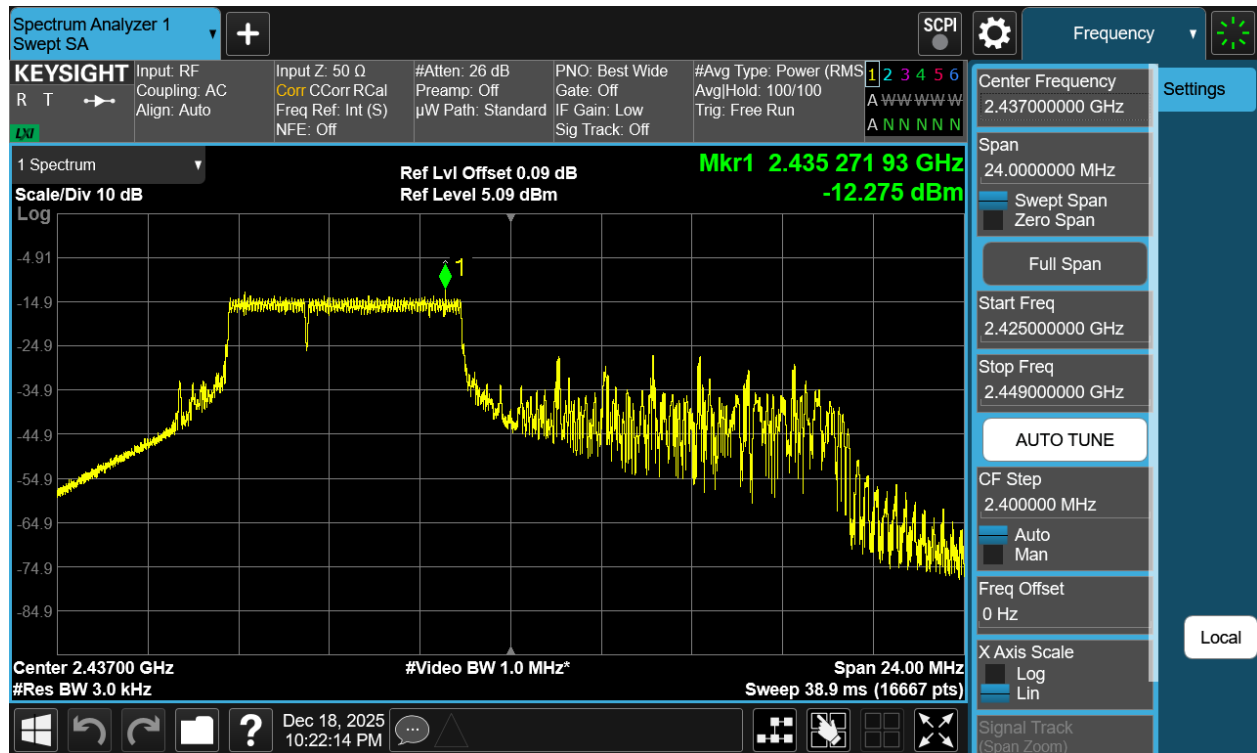
Plot 7-31 PSD CDD Antenna WF2b (20MHz BW 802.11be(RU) RU52+26 Index70 - Ch.6)
