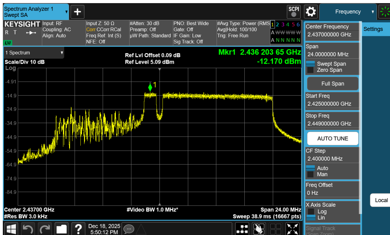
Plot 7-20 PSD Antenna WF7b (20MHz BW 802.11be(RU) RU106+26 Index83 - Ch.6)
