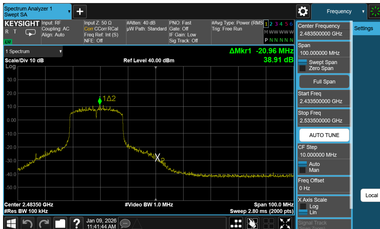
Plot 7-48. Band Edge Antenna WF7b (802.11be OFDMA – RU242 – Ch. 11)
