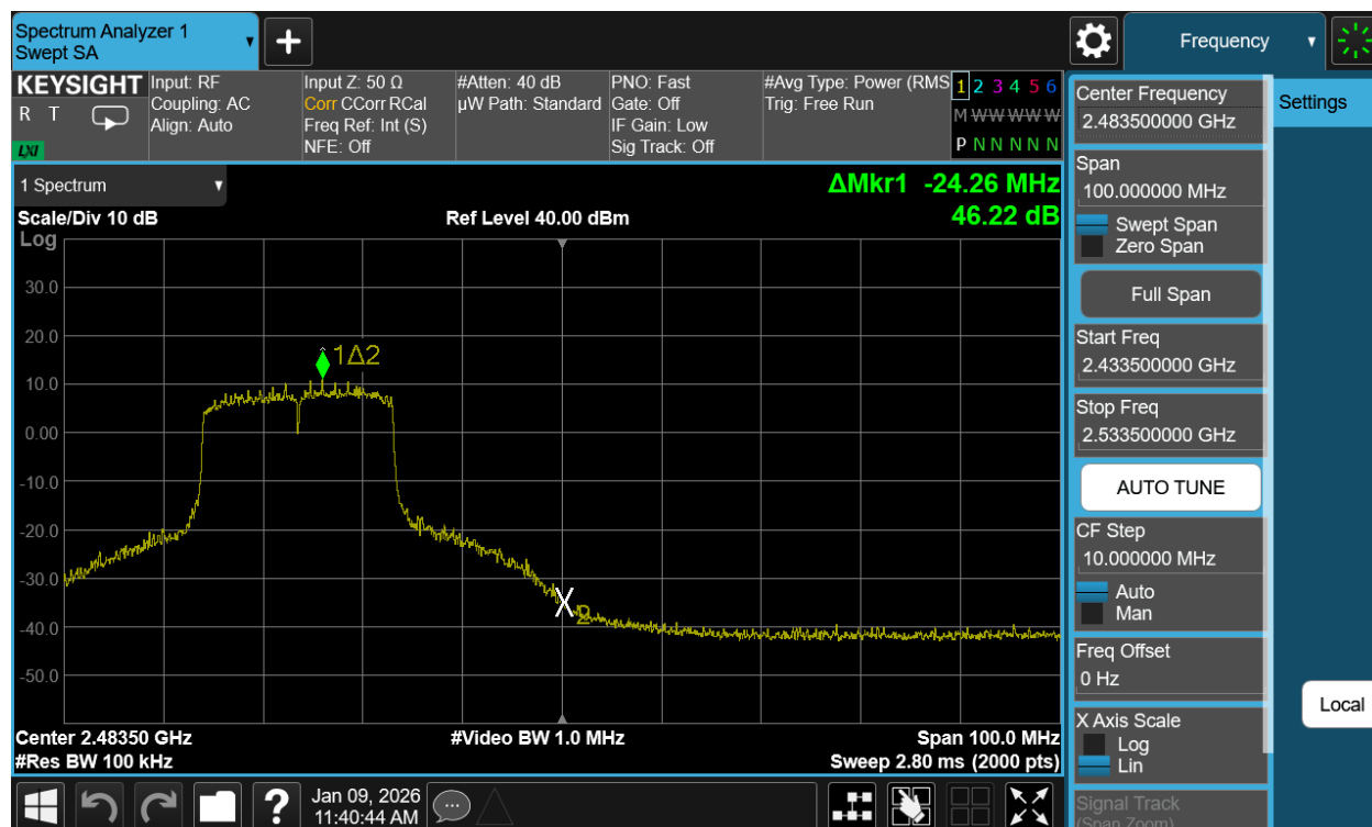
Plot 7-47. Band Edge Antenna WF7b (802.11be OFDMA – RU242 – Ch. 10)
