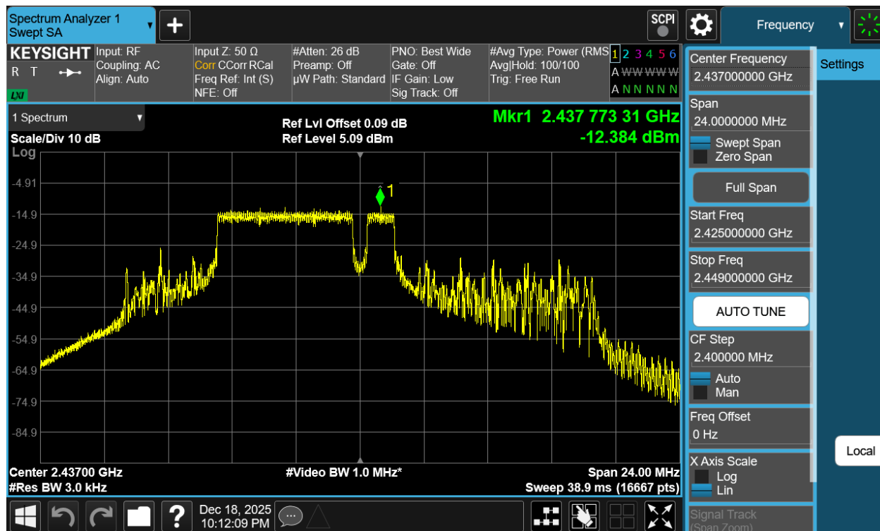
Plot 7-23 PSD Antenna WF2b (20MHz BW 802.11be(RU) RU52+26 Index71 - Ch.6)
