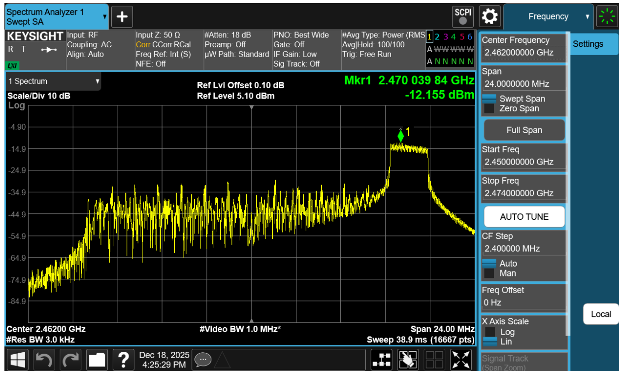
Plot 7-17 PSD Antenna WF7b (20MHz BW 802.11be(RU) RU26 Index8 - Ch.11)
