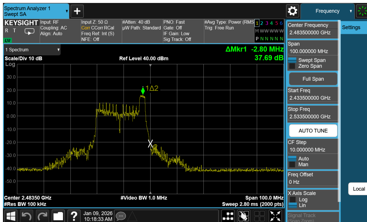
Plot 7-36. Band Edge Antenna WF7b (802.11be OFDMA – RU26 Index 8 – Ch. 13)
