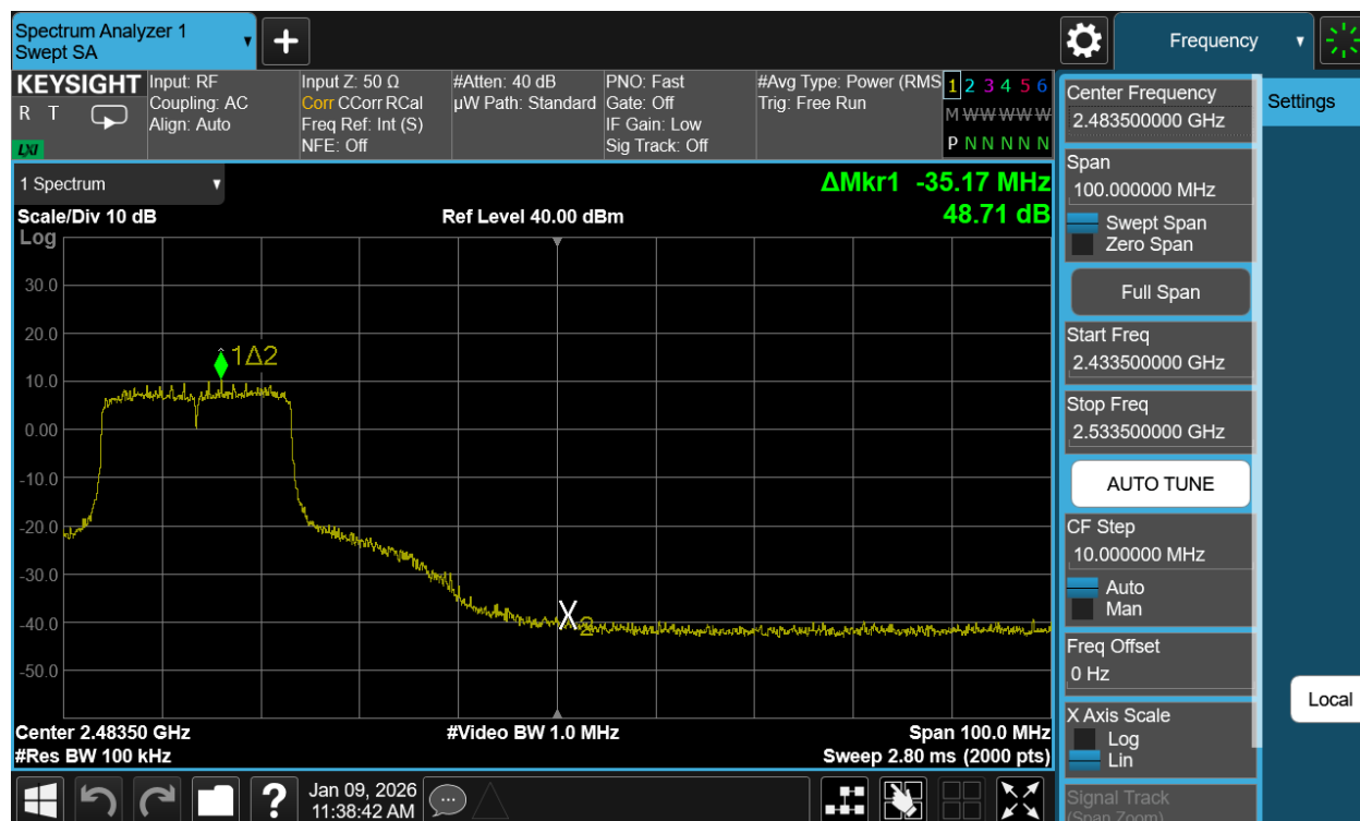
Plot 7-45. Band Edge Antenna WF7b (802.11be OFDMA – RU242 – Ch. 8)
