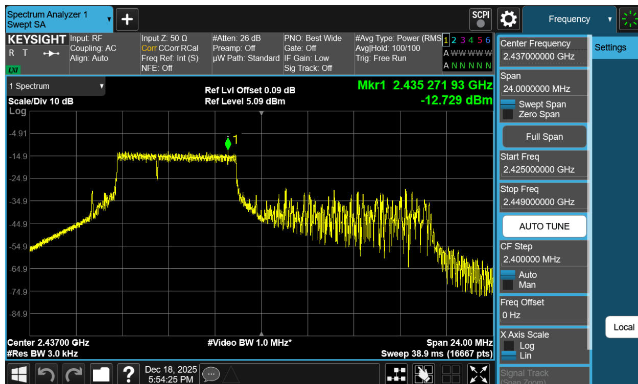
Plot 7-27 PSD CDD Antenna WF7b (20MHz BW 802.11be(RU) RU52+26 Index70 - Ch.6)
