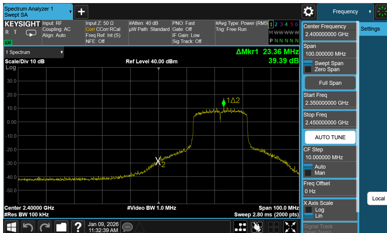
Plot 7-39. Band Edge Antenna WF7b (802.11be OFDMA – RU242 – Ch. 3)
