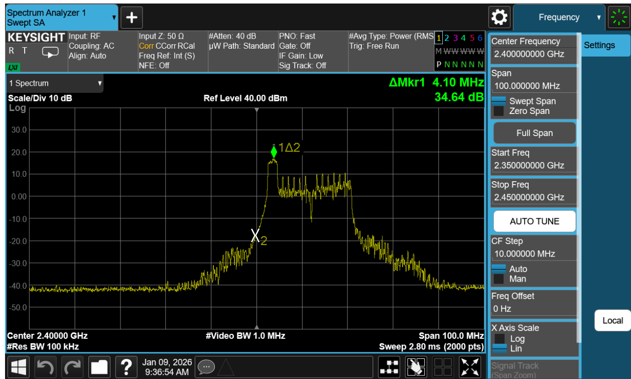
Plot 7-33. Band Edge Antenna WF7b (802.11be OFDMA – RU26 Index 0 – Ch. 1)
