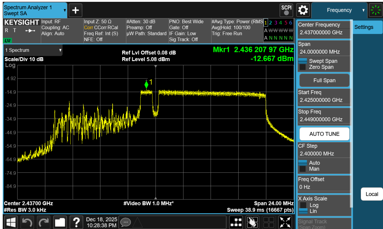
Plot 7-32 PSD CDD Antenna WF2b (20MHz BW 802.11be(RU) RU106+26 Index83 - Ch.6)
