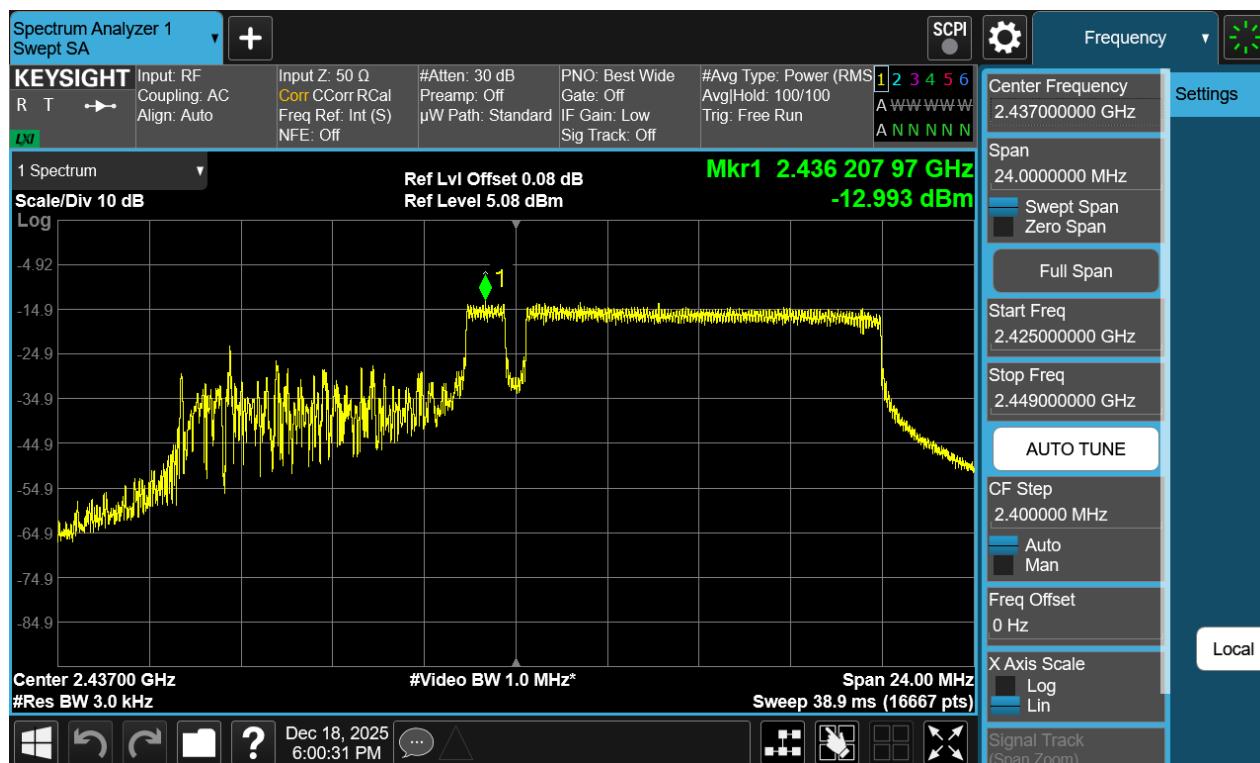
Plot 7-28 PSD CDD Antenna WF7b (20MHz BW 802.11be(RU) RU106+26 Index83 - Ch.6)
