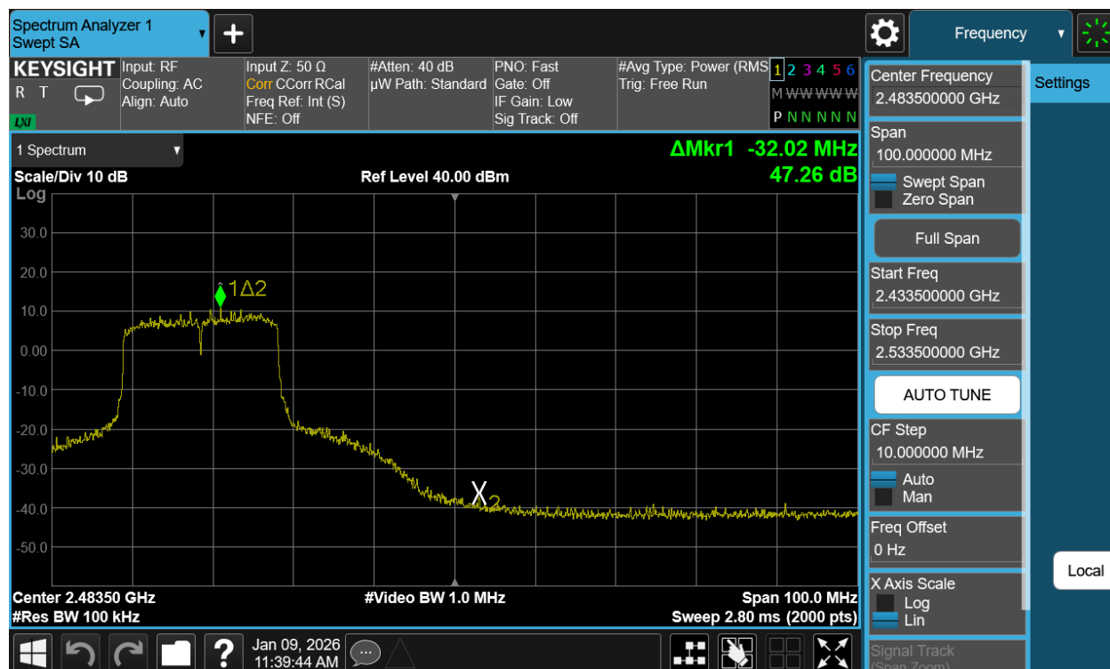
Plot 7-46. Band Edge Antenna WF7b (802.11be OFDMA – RU242 – Ch. 9)
