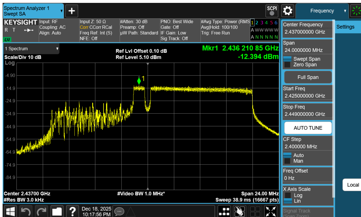
Plot 7-24 PSD Antenna WF2b (20MHz BW 802.11be(RU) RU106+26 Index83 - Ch.6)
