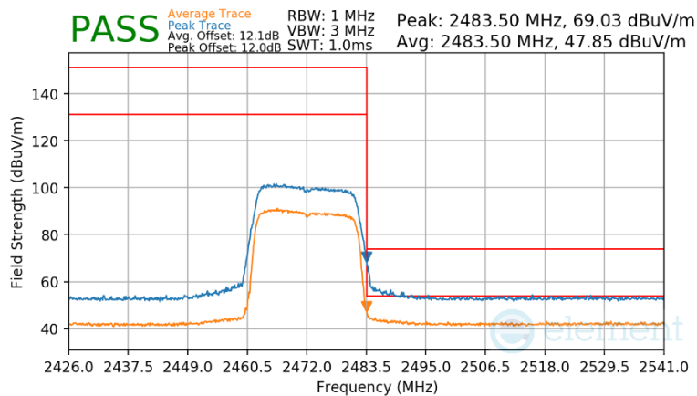
Plot 7-133 Radiated Restricted Band Edge Measurement Antenna WF7b (Peak & Average – RU242)
