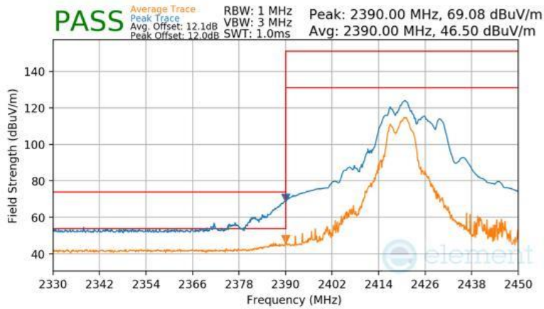
Plot 7-175 Radiated Restricted Band Edge Measurement CDD (Peak & Average – RU52+26)
