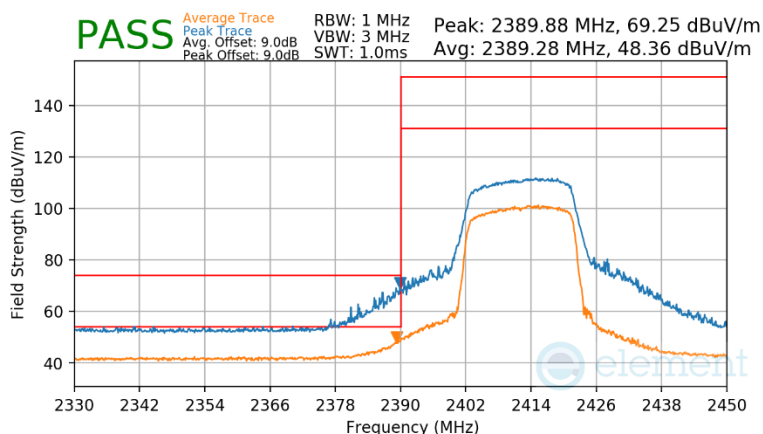
Plot 7-120 Radiated Restricted Band Edge Measurement Antenna WF7b (Peak & Average – RU242)
