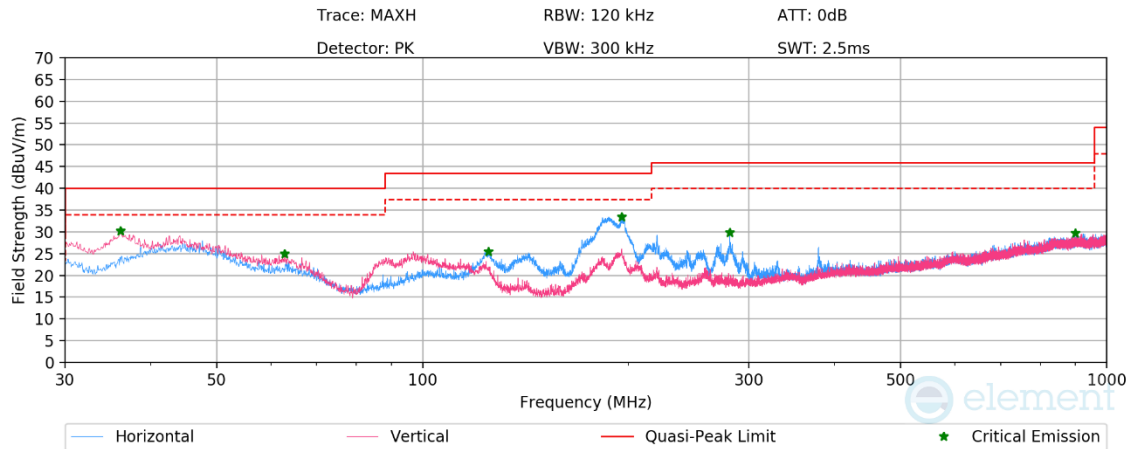
Plot 7-201. Radiated Spurious Emissions below 1GHz CDD Ch.11 (RU26), with AC/DC Adapter
