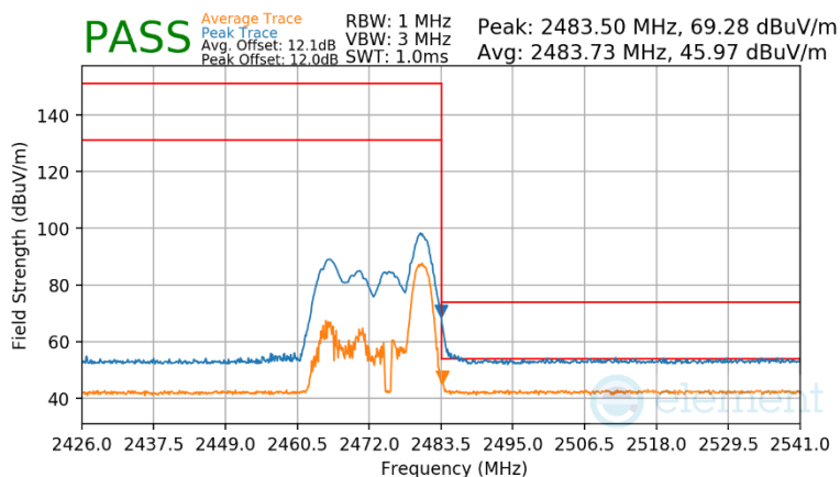
Plot 7-170 Radiated Restricted Band Edge Measurement CDD (Peak & Average – RU26)
