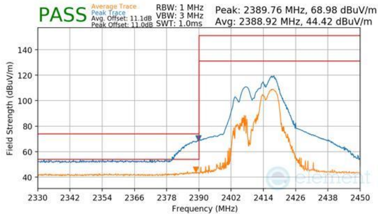
Plot 7-172 Radiated Restricted Band Edge Measurement CDD (Peak & Average – RU52+26)
