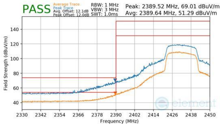
Plot 7-124 Radiated Restricted Band Edge Measurement Antenna WF7b (Peak & Average – RU242)
