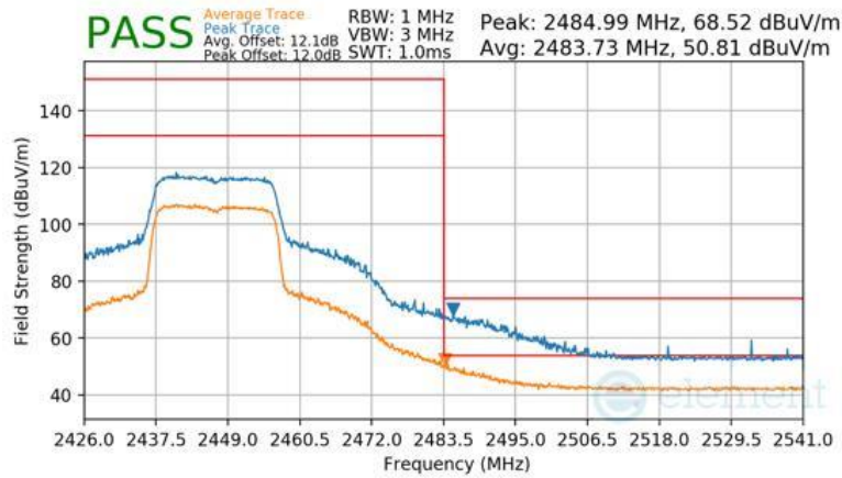
Plot 7-162 Radiated Restricted Band Edge Measurement Antenna WF2b (Peak & Average – RU242)
