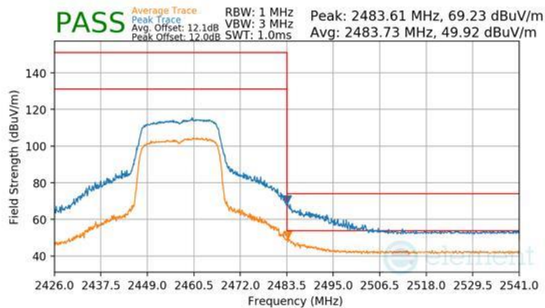
Plot 7-130 Radiated Restricted Band Edge Measurement Antenna WF7b (Peak & Average – RU242)
