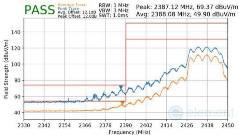
Plot 7-192 Radiated Restricted Band Edge Measurement CDD (Peak & Average – RU242)
