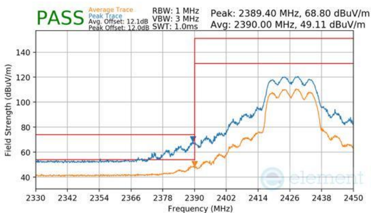
Plot 7-190 Radiated Restricted Band Edge Measurement CDD (Peak & Average – RU242)
