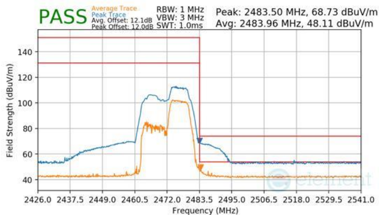
Plot 7-153 Radiated Restricted Band Edge Measurement Antenna WF2b (Peak & Average – RU52+26)
