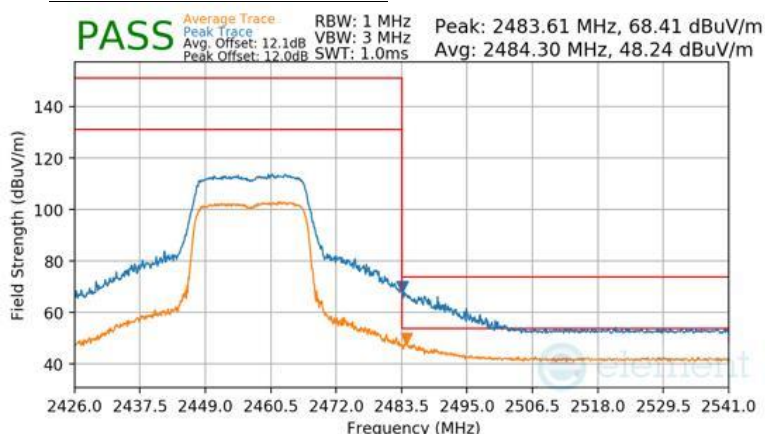
Plot 7-164 Radiated Restricted Band Edge Measurement Antenna WF2b (Peak & Average – RU242)
