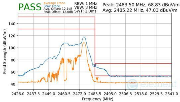
Plot 7-136 Radiated Restricted Band Edge Measurement Antenna WF2b (Peak & Average – RU26)
