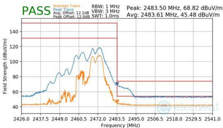
Plot 7-184 Radiated Restricted Band Edge Measurement CDD (Peak & Average – RU52+26)
