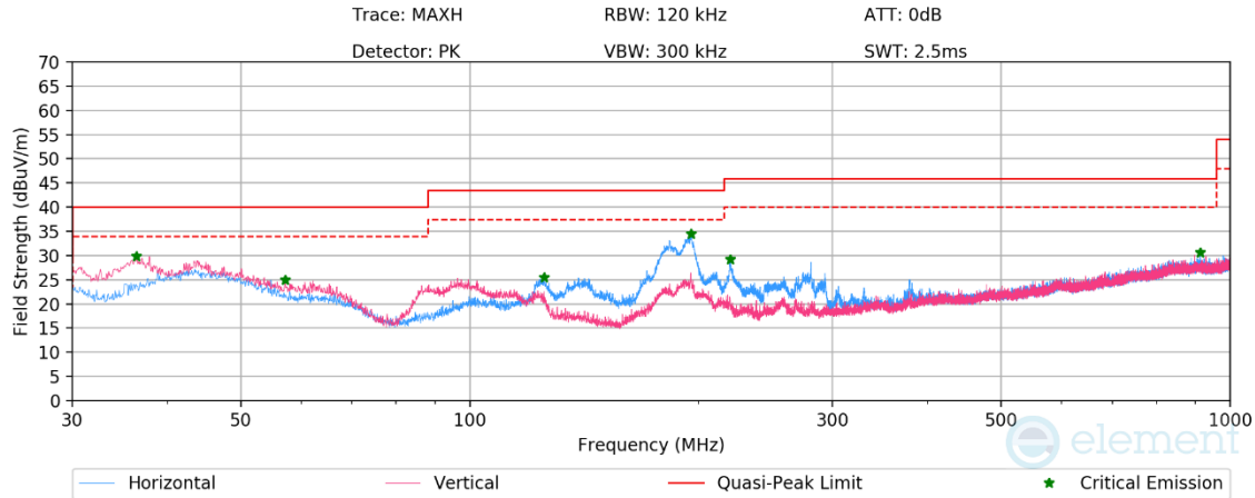
Plot 7-202. Radiated Spurious Emissions below 1GHz CDD Ch.6 (RU242), with AC/DC Adapter
