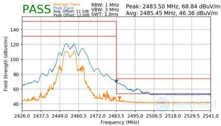
Plot 7-179 Radiated Restricted Band Edge Measurement CDD (Peak & Average – RU52+26)
