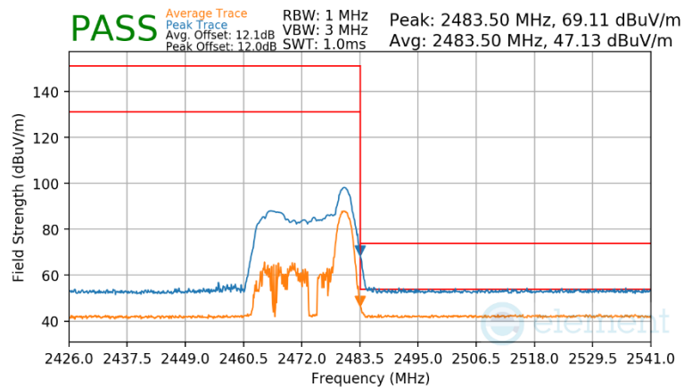
Plot 7-137 Radiated Restricted Band Edge Measurement Antenna WF2b (Peak & Average – RU26)
