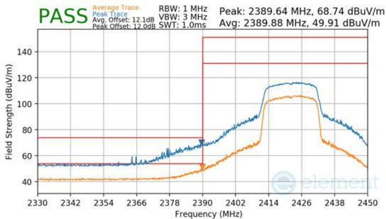
Plot 7-156 Radiated Restricted Band Edge Measurement Antenna WF2b (Peak & Average – RU242)
