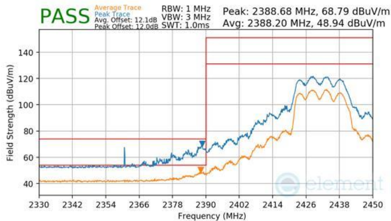
Plot 7-191 Radiated Restricted Band Edge Measurement CDD (Peak & Average – RU242)
