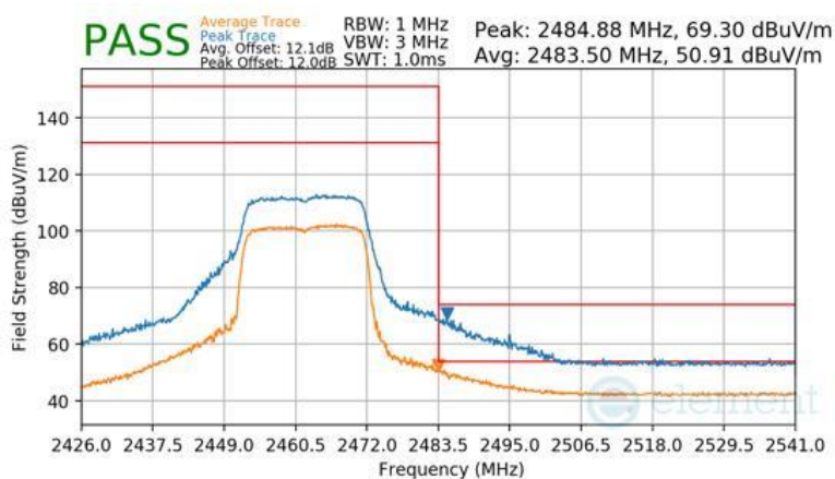
Plot 7-165 Radiated Restricted Band Edge Measurement Antenna WF2b (Peak & Average – RU242)
