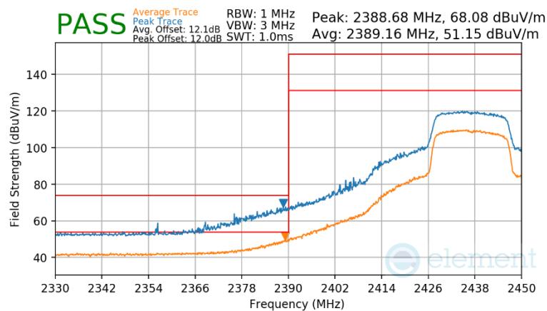
Plot 7-125 Radiated Restricted Band Edge Measurement Antenna WF7b (Peak & Average – RU242)
