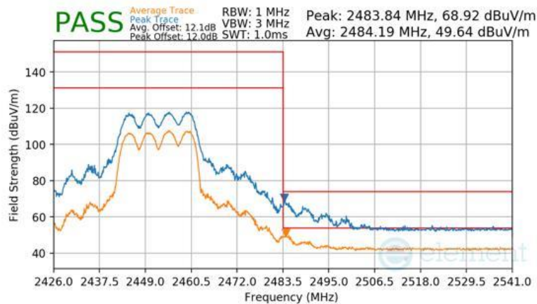
Plot 7-196 Radiated Restricted Band Edge Measurement CDD (Peak & Average – RU242)
