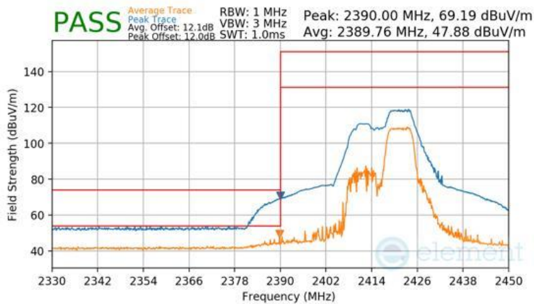
Plot 7-141 Radiated Restricted Band Edge Measurement Antenna WF2b (Peak & Average – RU52+26)
