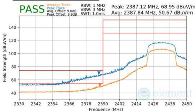
Plot 7-158 Radiated Restricted Band Edge Measurement Antenna WF2b (Peak & Average – RU242)
