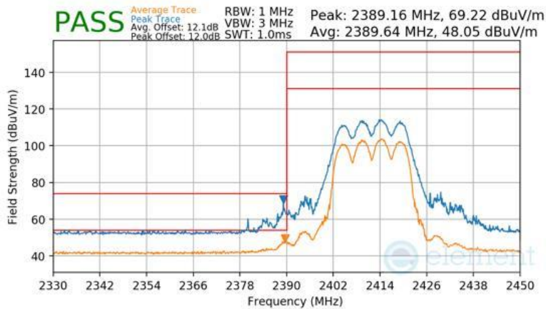
Plot 7-187 Radiated Restricted Band Edge Measurement CDD (Peak & Average – RU242)
