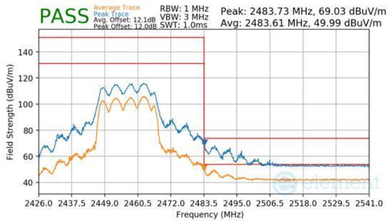
Plot 7-197 Radiated Restricted Band Edge Measurement CDD (Peak & Average – RU242)
