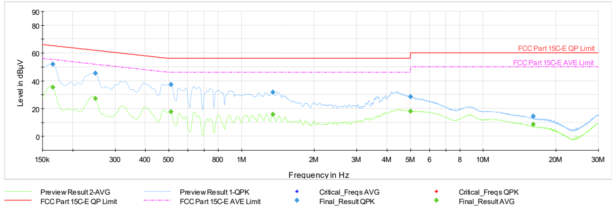
Plot 7-204. AC Line Conducted Emissions with 802.11be CDD (RU26) Ch.11 (N, with AC/DC Adapter)
