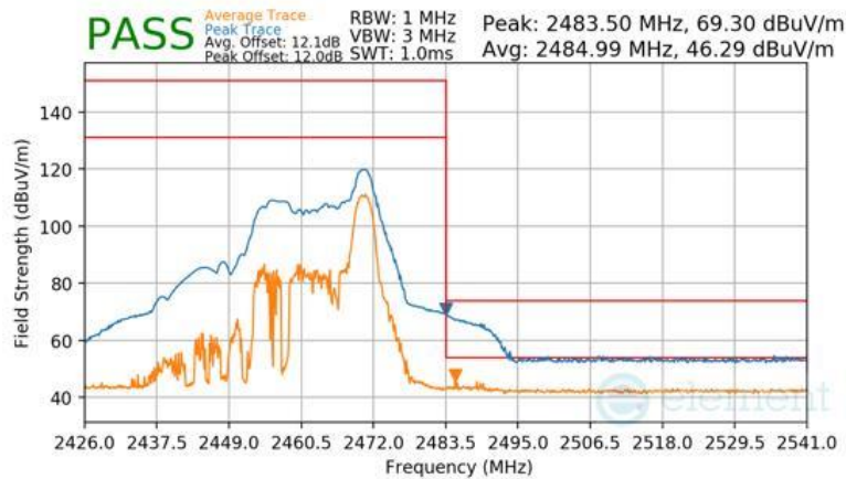
Plot 7-135 Radiated Restricted Band Edge Measurement Antenna WF2b (Peak & Average – RU26)
