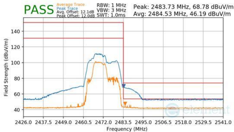
Plot 7-118 Radiated Restricted Band Edge Measurement Antenna WF7b (Peak & Average – RU52+26)
