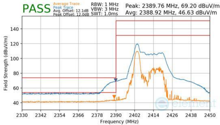
Plot 7-134 Radiated Restricted Band Edge Measurement Antenna WF2b (Peak & Average – RU26)
