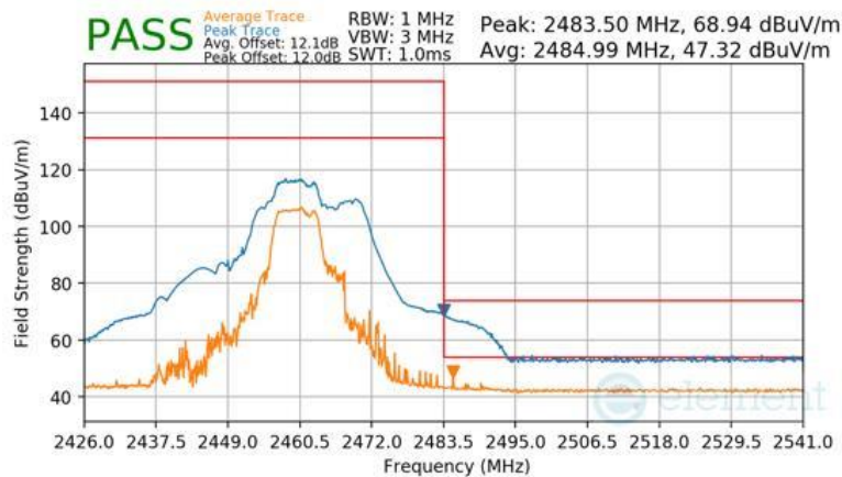
Plot 7-148 Radiated Restricted Band Edge Measurement Antenna WF2b (Peak & Average – RU52+26)
