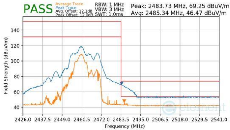
Plot 7-181 Radiated Restricted Band Edge Measurement CDD (Peak & Average – RU52+26)
