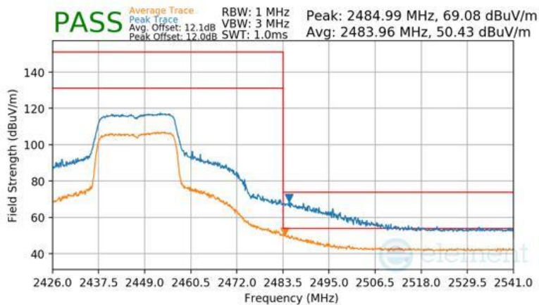
Plot 7-128 Radiated Restricted Band Edge Measurement Antenna WF7b (Peak & Average – RU242)
