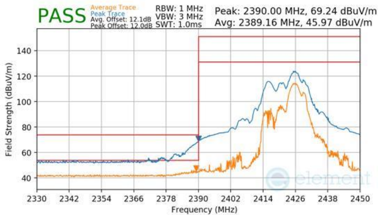
Plot 7-176 Radiated Restricted Band Edge Measurement CDD (Peak & Average – RU52+26)
