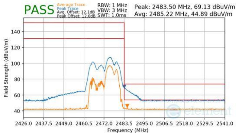
Plot 7-186 Radiated Restricted Band Edge Measurement CDD (Peak & Average – RU52+26)
