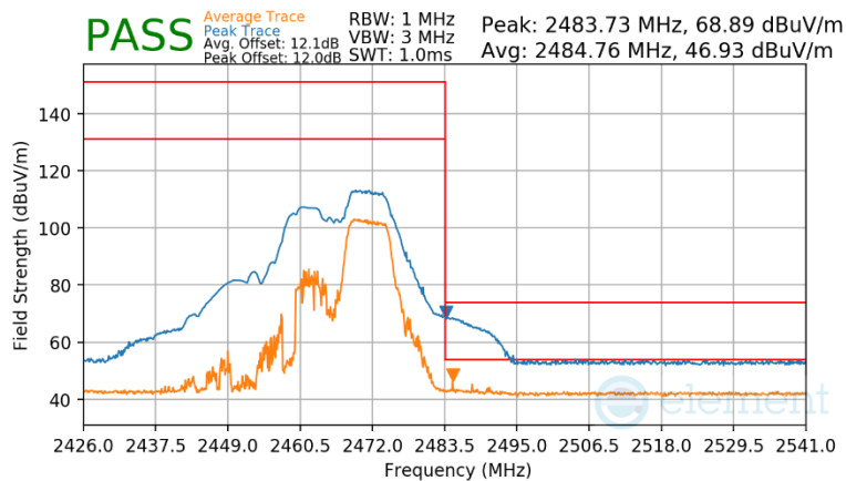
Plot 7-117 Radiated Restricted Band Edge Measurement Antenna WF7b (Peak & Average – RU52+26)
