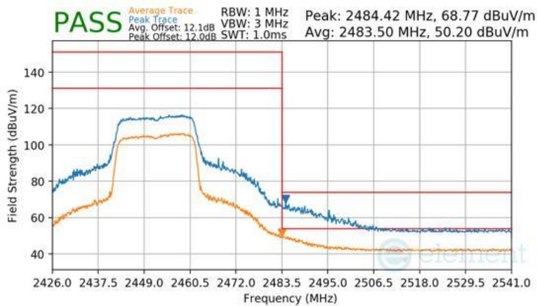
Plot 7-129 Radiated Restricted Band Edge Measurement Antenna WF7b (Peak & Average – RU242)
