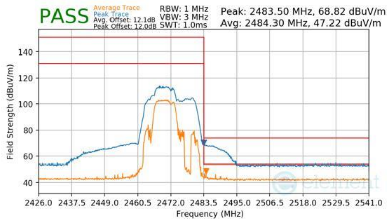
Plot 7-152 Radiated Restricted Band Edge Measurement Antenna WF2b (Peak & Average – RU52+26)
