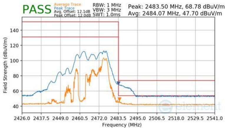
Plot 7-169 Radiated Restricted Band Edge Measurement CDD (Peak & Average – RU26)
