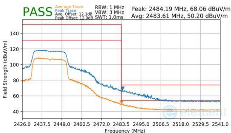
Plot 7-161 Radiated Restricted Band Edge Measurement Antenna WF2b (Peak & Average – RU242)
