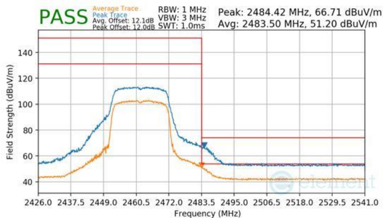
Plot 7-131 Radiated Restricted Band Edge Measurement Antenna WF7b (Peak & Average – RU242)
