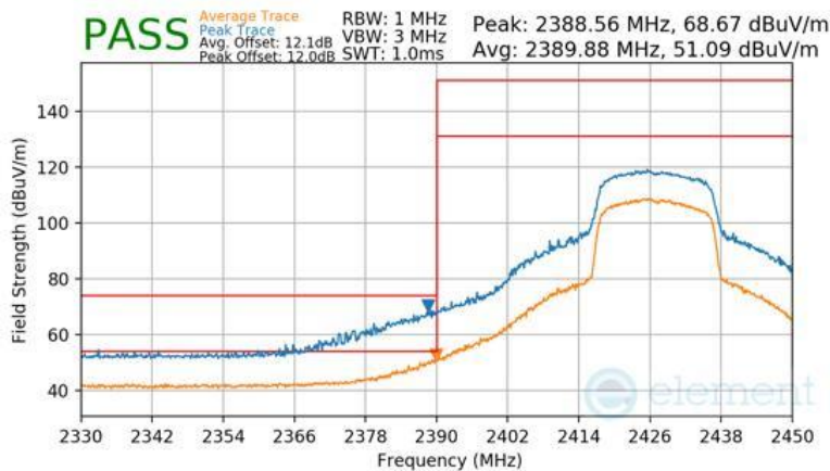
Plot 7-123 Radiated Restricted Band Edge Measurement Antenna WF7b (Peak & Average – RU242)
