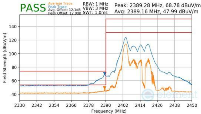
Plot 7-168 Radiated Restricted Band Edge Measurement CDD (Peak & Average – RU26)
