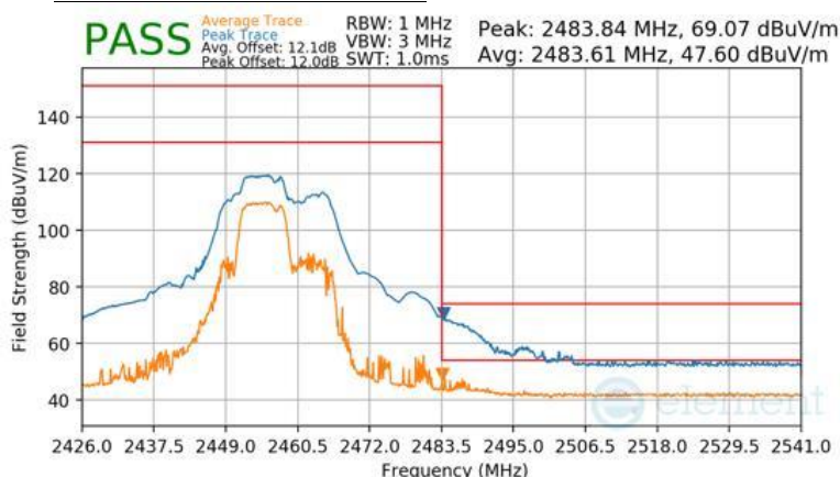
Plot 7-146 Radiated Restricted Band Edge Measurement Antenna WF2b (Peak & Average – RU52+26)
