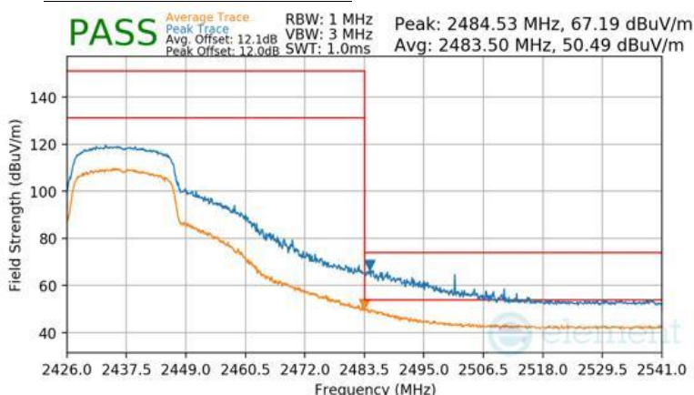
Plot 7-160 Radiated Restricted Band Edge Measurement Antenna WF2b (Peak & Average – RU242)
