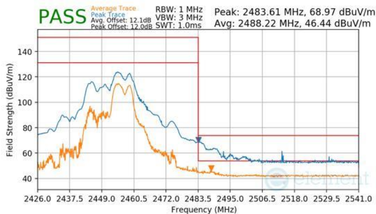
Plot 7-178 Radiated Restricted Band Edge Measurement CDD (Peak & Average – RU52+26)
