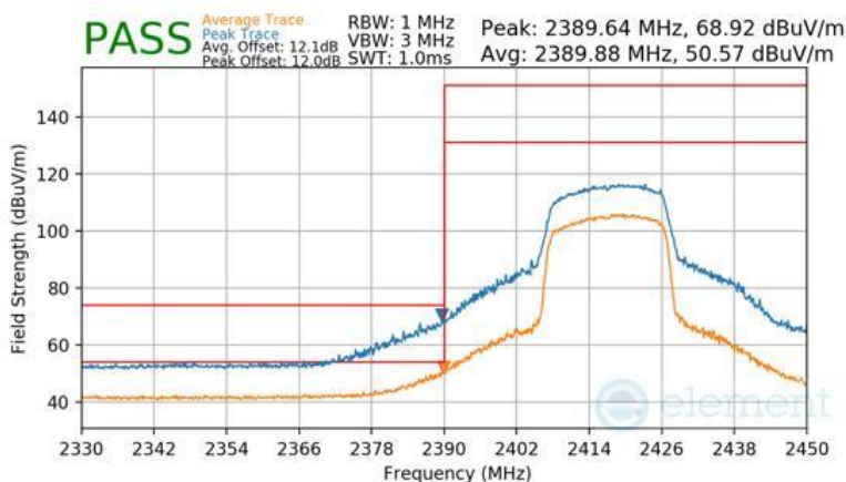
Plot 7-121 Radiated Restricted Band Edge Measurement Antenna WF7b (Peak & Average – RU242)
