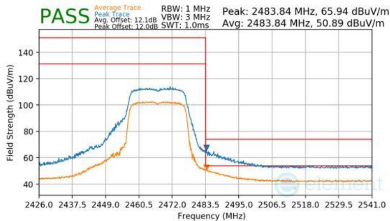
Plot 7-166 Radiated Restricted Band Edge Measurement Antenna WF2b (Peak & Average – RU242)
