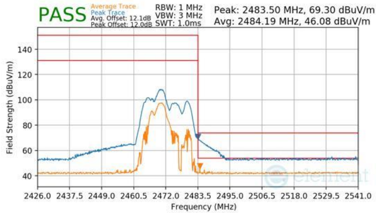
Plot 7-185 Radiated Restricted Band Edge Measurement CDD (Peak & Average – RU52+26)
