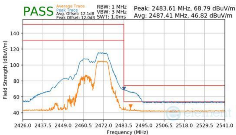
Plot 7-151 Radiated Restricted Band Edge Measurement Antenna WF2b (Peak & Average – RU52+26)
