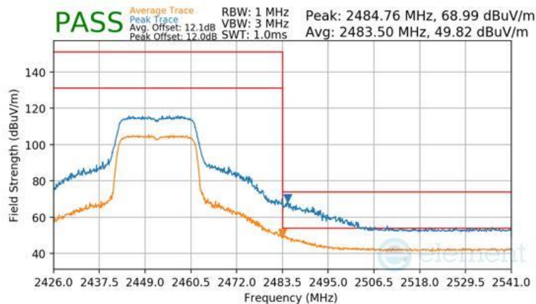
Plot 7-163 Radiated Restricted Band Edge Measurement Antenna WF2b (Peak & Average – RU242)
