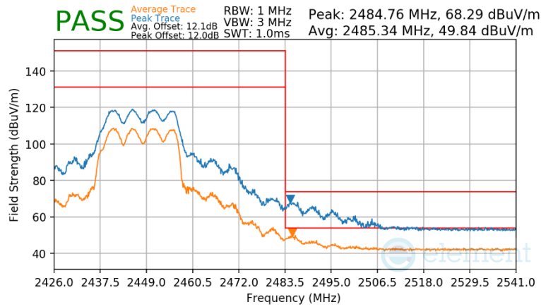
Plot 7-195 Radiated Restricted Band Edge Measurement CDD (Peak & Average – RU242)
