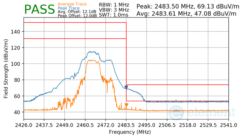
Plot 7-116 Radiated Restricted Band Edge Measurement Antenna WF7b (Peak & Average – RU52+26)
