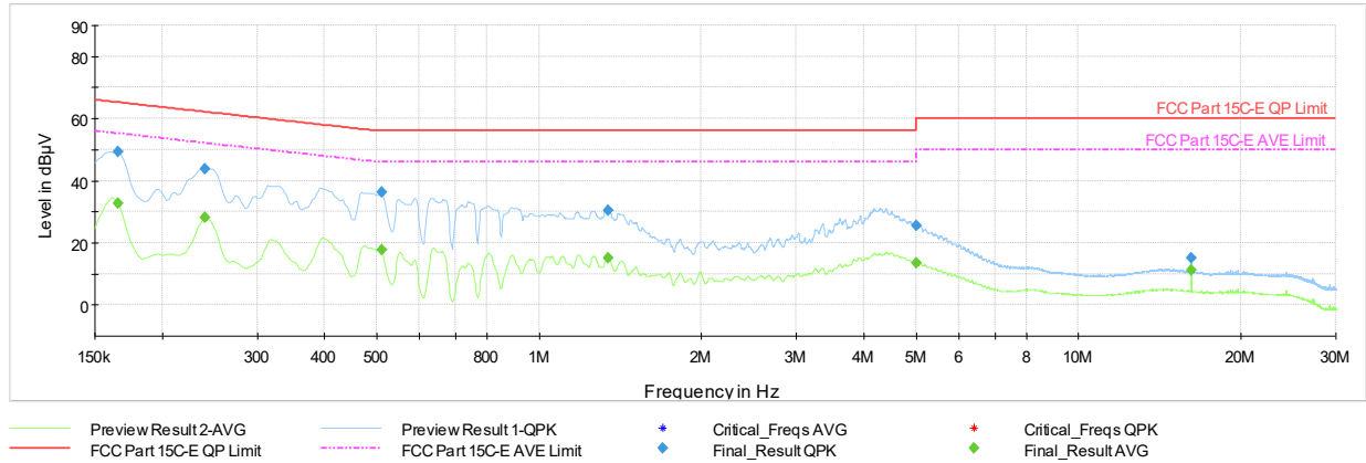
Plot 7-205. AC Line Conducted Emissions with 802.11be CDD (RU242) Ch.6 (L1, with AC/DC Adapter)
