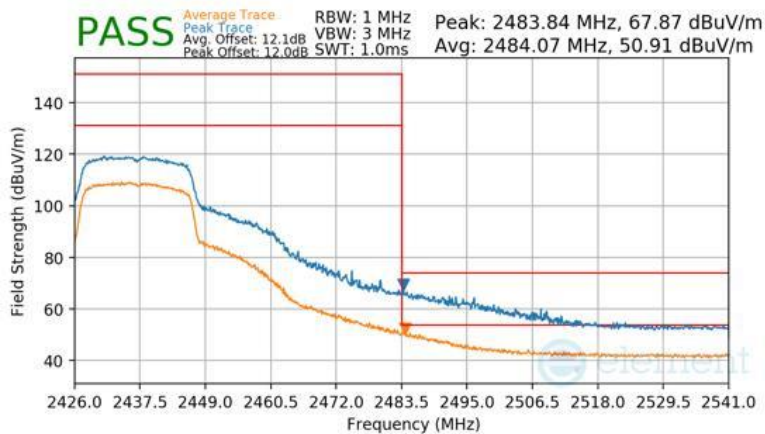
Plot 7-126 Radiated Restricted Band Edge Measurement Antenna WF7b (Peak & Average – RU242)
