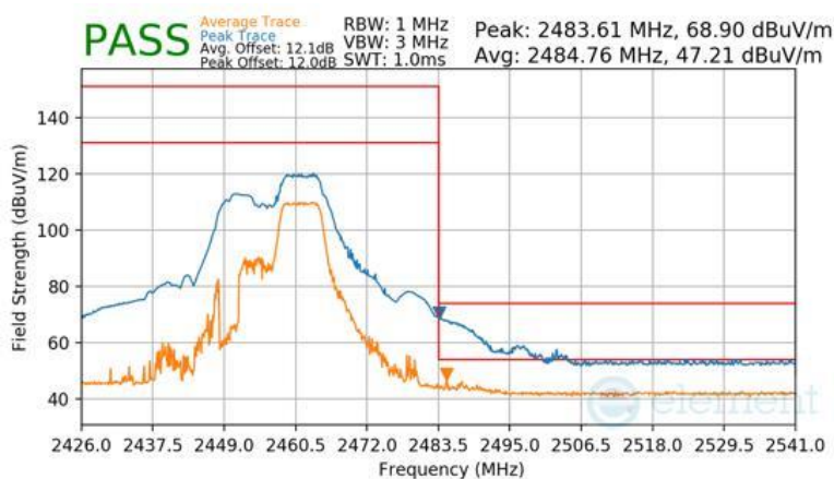
Plot 7-147 Radiated Restricted Band Edge Measurement Antenna WF2b (Peak & Average – RU52+26)
