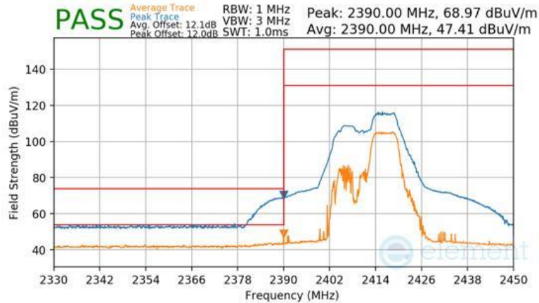
Plot 7-139 Radiated Restricted Band Edge Measurement Antenna WF2b (Peak & Average – RU52+26)
