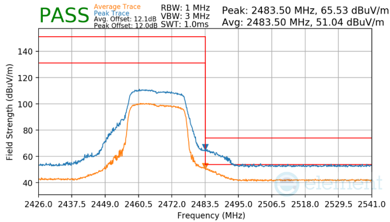
Plot 7-132 Radiated Restricted Band Edge Measurement Antenna WF7b (Peak & Average – RU242)
