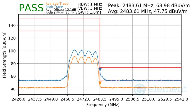
Plot 7-200 Radiated Restricted Band Edge Measurement CDD (Peak & Average – RU242)
