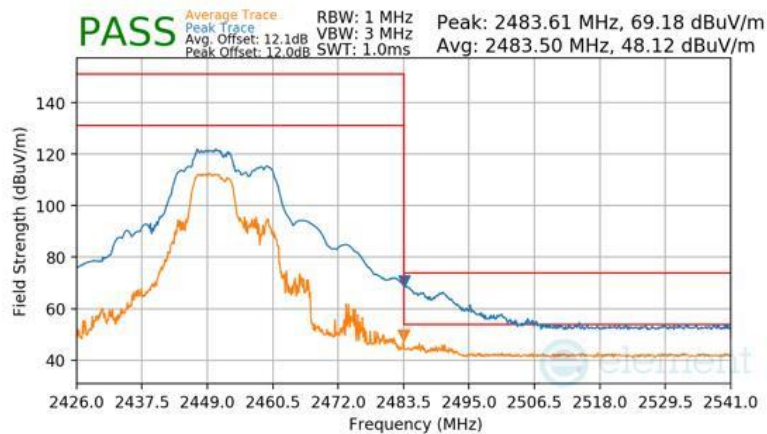
Plot 7-144 Radiated Restricted Band Edge Measurement Antenna WF2b (Peak & Average – RU52+26)
