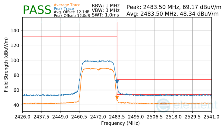
Plot 7-167 Radiated Restricted Band Edge Measurement Antenna WF2b (Peak & Average – RU242)
