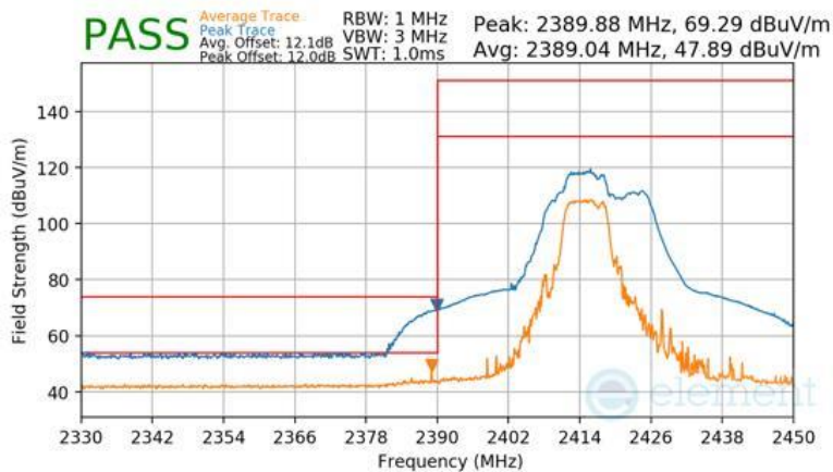
Plot 7-140 Radiated Restricted Band Edge Measurement Antenna WF2b (Peak & Average – RU52+26)
