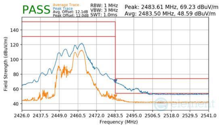
Plot 7-180 Radiated Restricted Band Edge Measurement CDD (Peak & Average – RU52+26)
