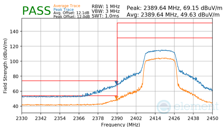
Plot 7-155 Radiated Restricted Band Edge Measurement Antenna WF2b (Peak & Average – RU242)
