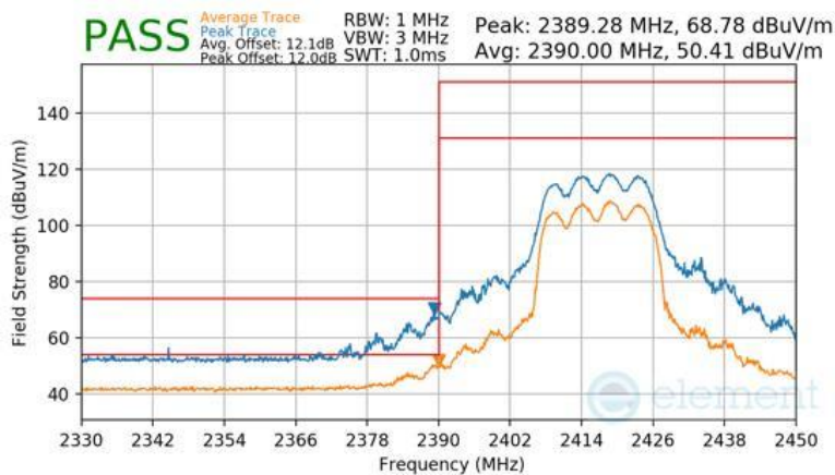
Plot 7-188 Radiated Restricted Band Edge Measurement CDD (Peak & Average – RU242)
