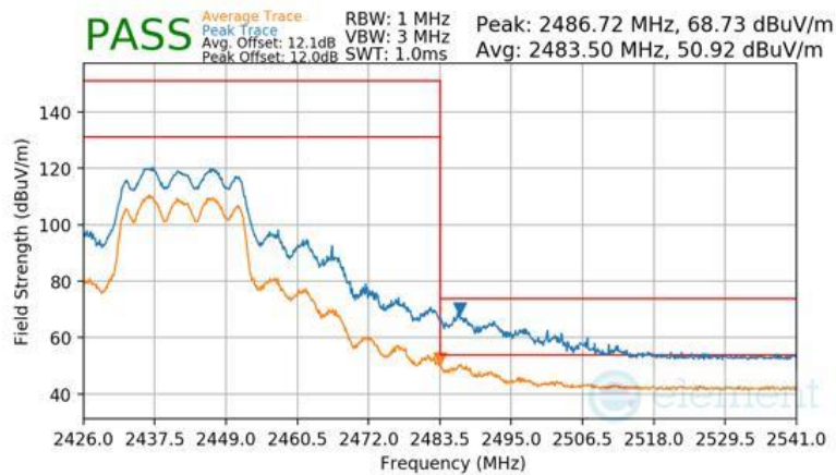
Plot 7-194 Radiated Restricted Band Edge Measurement CDD (Peak & Average – RU242)
