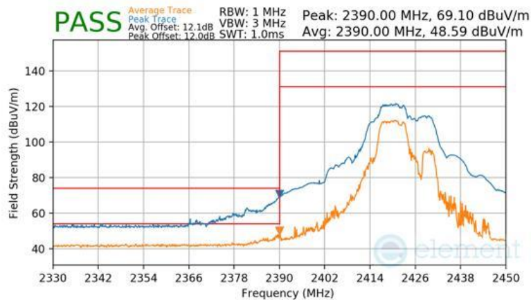
Plot 7-142 Radiated Restricted Band Edge Measurement Antenna WF2b (Peak & Average – RU52+26)
