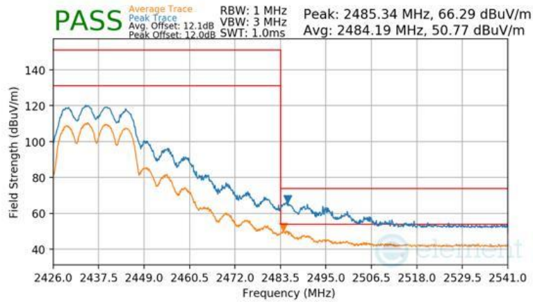
Plot 7-193 Radiated Restricted Band Edge Measurement CDD (Peak & Average – RU242)
