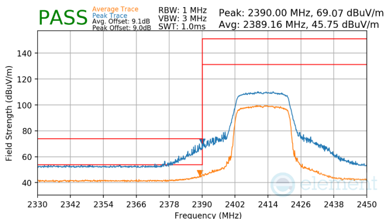
Plot 7-154 Radiated Restricted Band Edge Measurement Antenna WF2b (Peak & Average – RU242)
