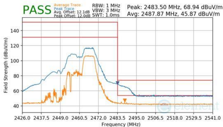
Plot 7-149 Radiated Restricted Band Edge Measurement Antenna WF2b (Peak & Average – RU52+26)
