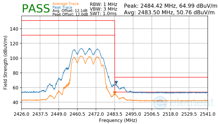
Plot 7-199 Radiated Restricted Band Edge Measurement CDD (Peak & Average – RU242)
