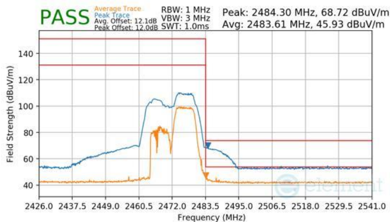
Plot 7-119 Radiated Restricted Band Edge Measurement Antenna WF7b (Peak & Average – RU52+26)
