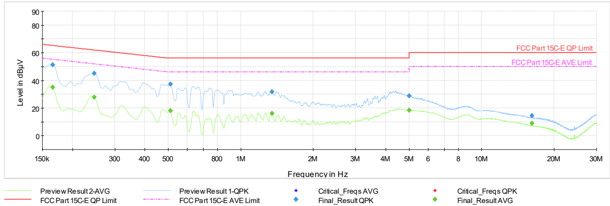
Plot 7-206. AC Line Conducted Emissions with 802.11be CDD (RU242) Ch.6 (N, with AC/DC Adapter)
