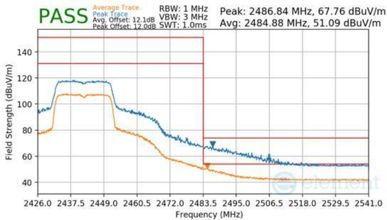
Plot 7-127 Radiated Restricted Band Edge Measurement Antenna WF7b (Peak & Average – RU242)
