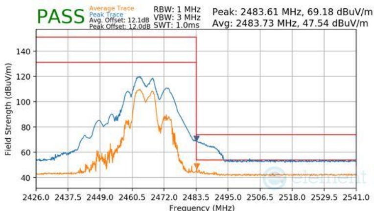
Plot 7-183 Radiated Restricted Band Edge Measurement CDD (Peak & Average – RU52+26)
