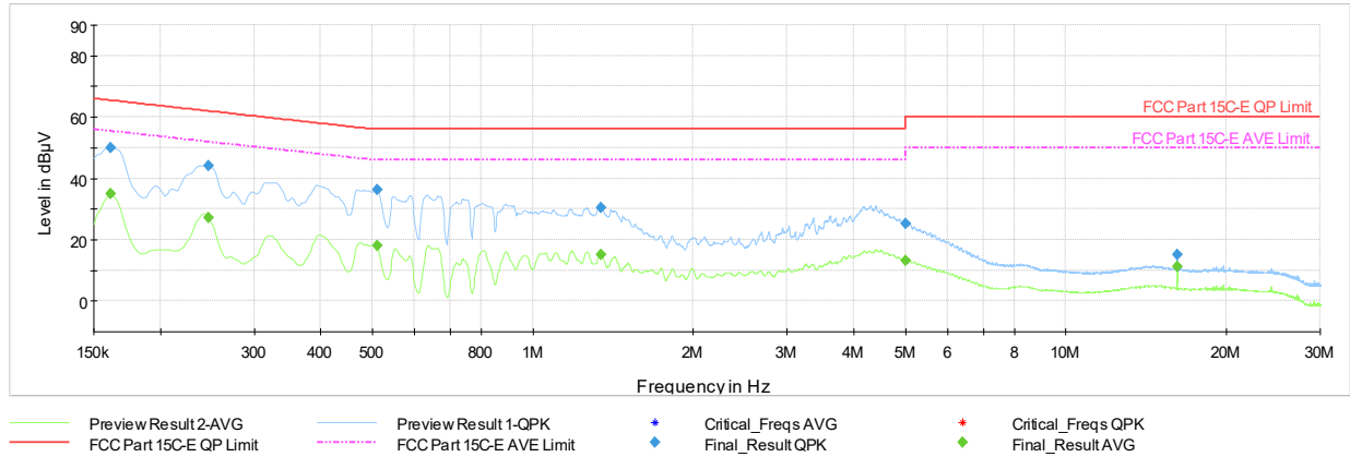
Plot 7-203. AC Line Conducted Emissions with 802.11be CDD (RU26) Ch.11 (L1, with AC/DC Adapter)
