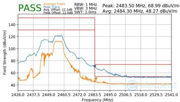
Plot 7-145 Radiated Restricted Band Edge Measurement Antenna WF2b (Peak & Average – RU52+26)
