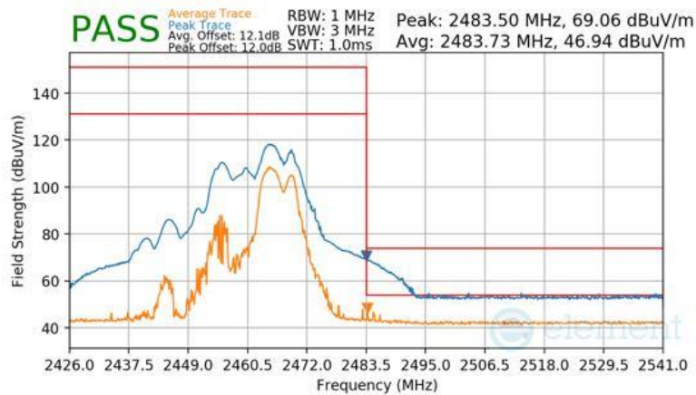
Plot 7-182 Radiated Restricted Band Edge Measurement CDD (Peak & Average – RU52+26)
