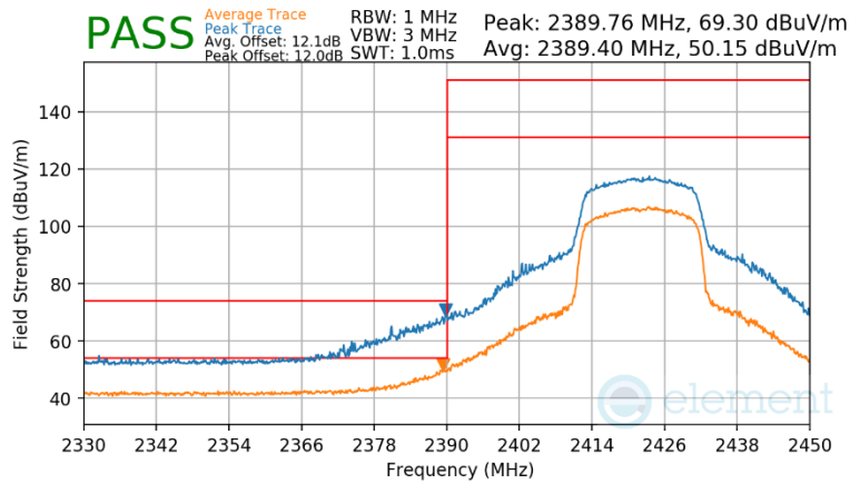
Plot 7-122 Radiated Restricted Band Edge Measurement Antenna WF7b (Peak & Average – RU242)
