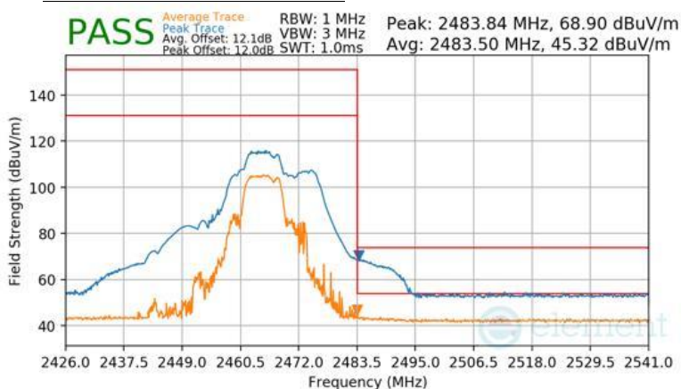
Plot 7-150 Radiated Restricted Band Edge Measurement Antenna WF2b (Peak & Average – RU52+26)
