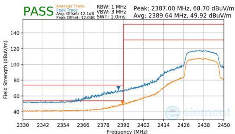
Plot 7-159 Radiated Restricted Band Edge Measurement Antenna WF2b (Peak & Average – RU242)
