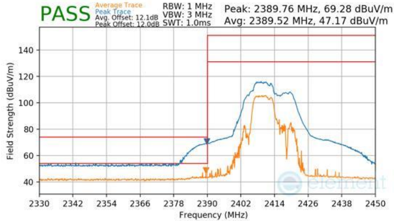
Plot 7-138 Radiated Restricted Band Edge Measurement Antenna WF2b (Peak & Average – RU52+26)
