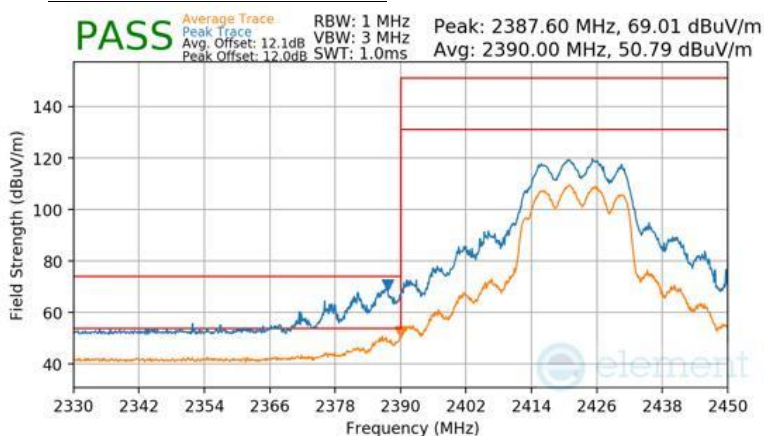
Plot 7-189 Radiated Restricted Band Edge Measurement CDD (Peak & Average – RU242)
