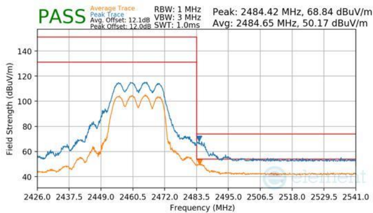
Plot 7-198 Radiated Restricted Band Edge Measurement CDD (Peak & Average – RU242)
