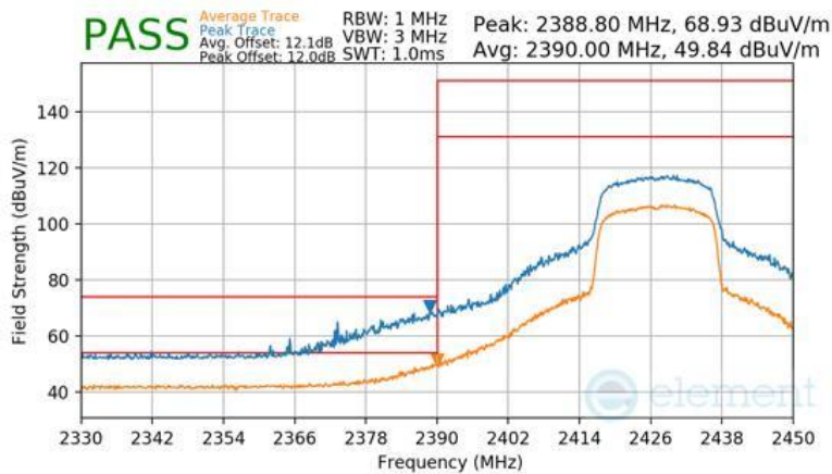
Plot 7-157 Radiated Restricted Band Edge Measurement Antenna WF2b (Peak & Average – RU242)
