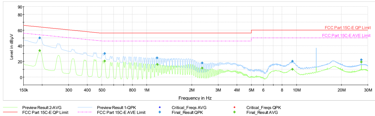
Plot 7-5. AC Line-Conducted Plot (N, Charging Rate 2.6C, with Laptop)
