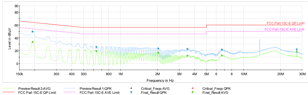
Plot 7-4. AC Line-Conducted Plot (L1, Charging Rate 2.6C, with Laptop)
