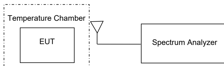
Figure 7-4. Test Instrument & Measurement Setup
