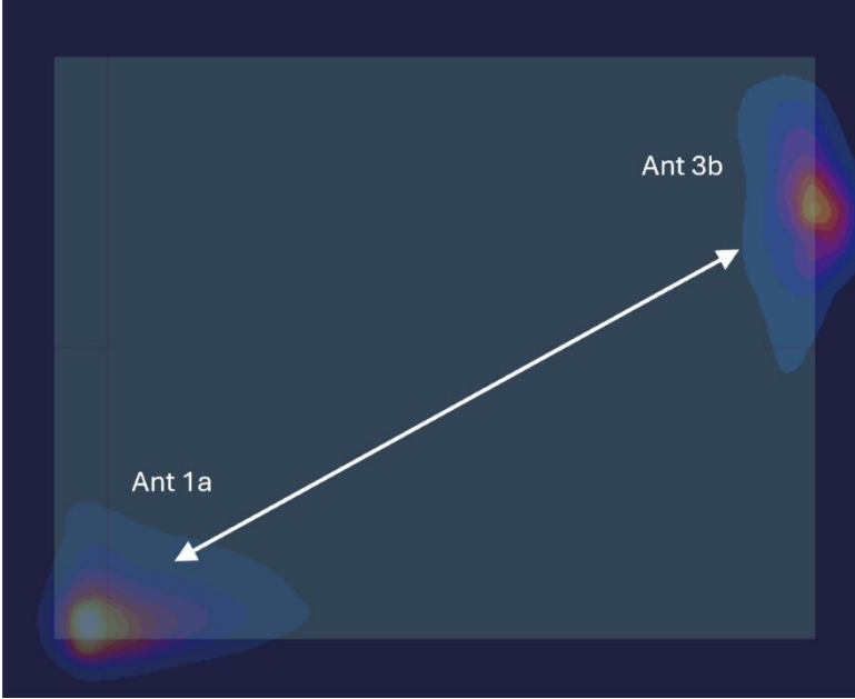
Figure F-3 Back Side Spatial Separation for Antenna 1a and Antenna 3b
