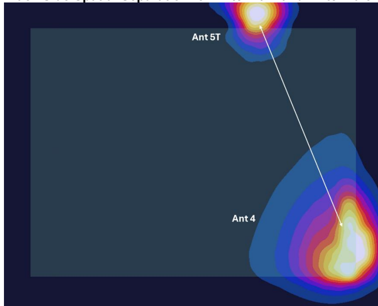
Figure F-18 Back Side Spatial Separation for Antenna 4 and Antenna 5T
