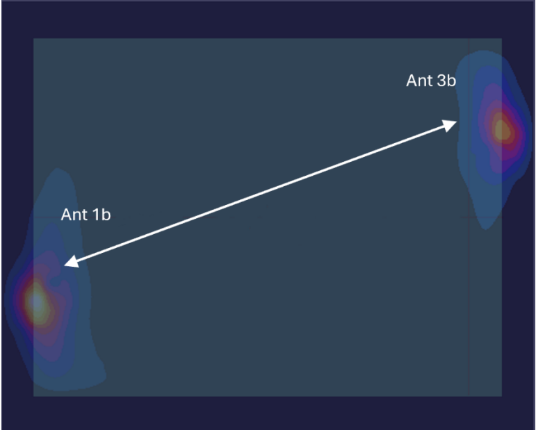
Figure F-8 Back Side Spatial Separation for Antenna 1b and Antenna 3b
