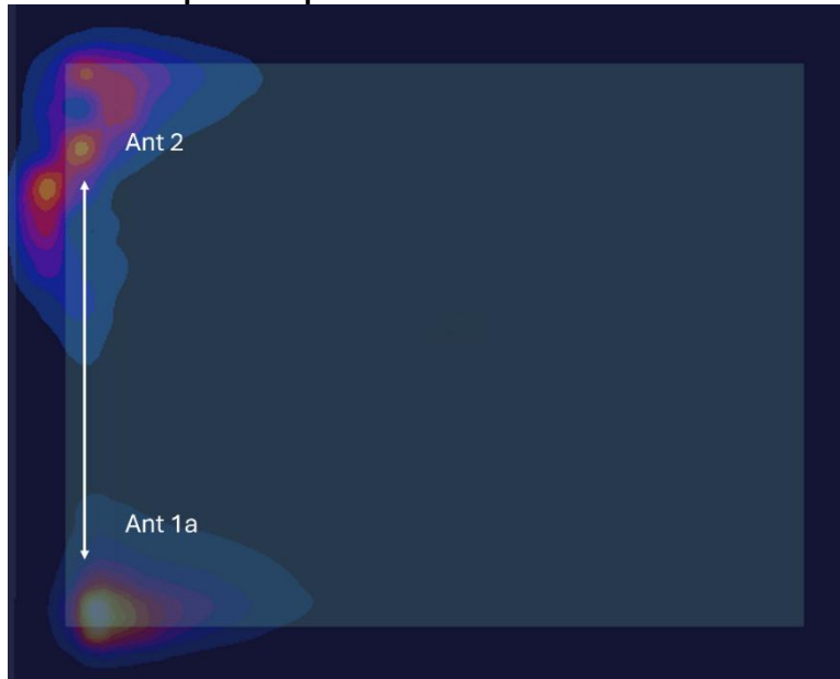
Figure F-1 Back Side Spatial Separation for Antenna 1a and Antenna 2
