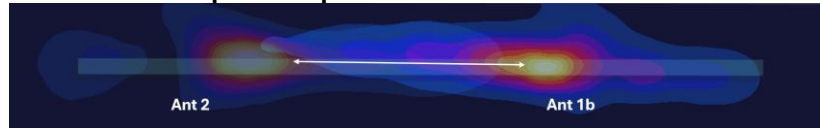
Figure F-31 Bottom Side Spatial Separation for Antenna 1b and Antenna 3a
