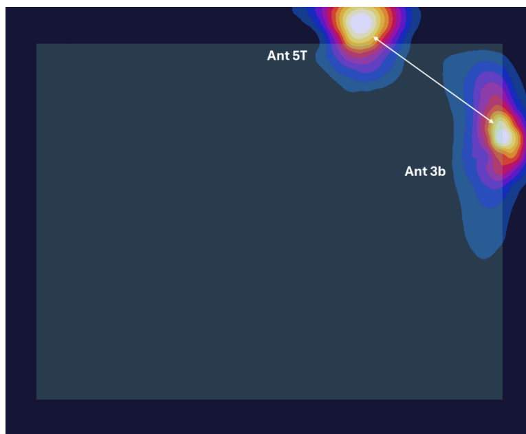
Figure F-17 Back Side Spatial Separation for Antenna 3b and Antenna 5T
