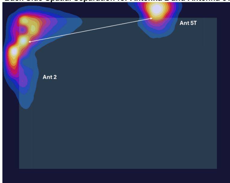
Figure F-13 Back Side Spatial Separation for Antenna 2 and Antenna 5T
