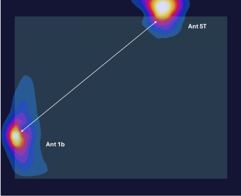
Figure F-10 Back Side Spatial Separation for Antenna 1b and Antenna 5T
