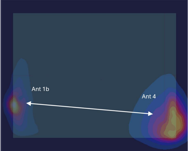
Figure F-9 Back Side Spatial Separation for Antenna 1b and Antenna 4
