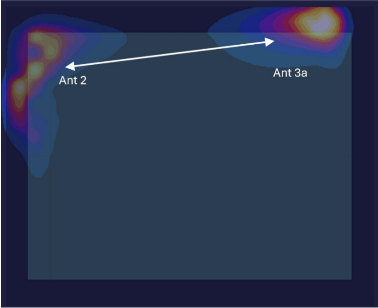
Figure F-11 Back Side Spatial Separation for Antenna 2 and Antenna 3a
