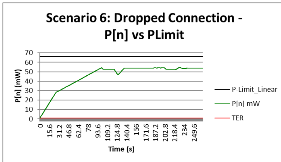
Figure 8-24: Normalized Time-averaged Power for Call Disconnection case (LTE Band 30 Ant 3b)
