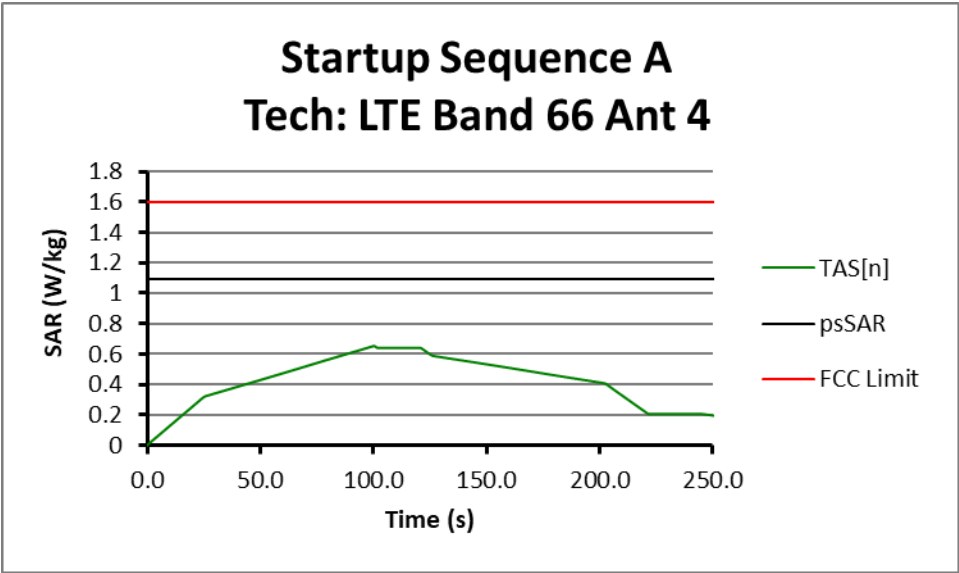
Figure 10-2: Time-averaged SAR for Change in Requested Power case (LTE Band 66 – Test Sequence A)
