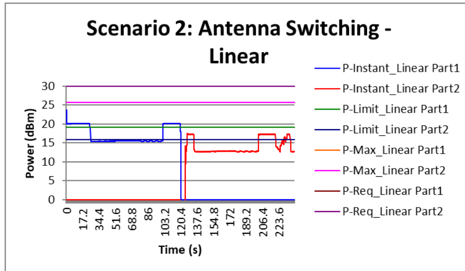
Figure 8-15: Time-averaged conducted TX power over time for Antenna Switch case (LTE Band 25 Ant 3b – Part 1 to LTE Band 66 Ant 4 – Part 2)
