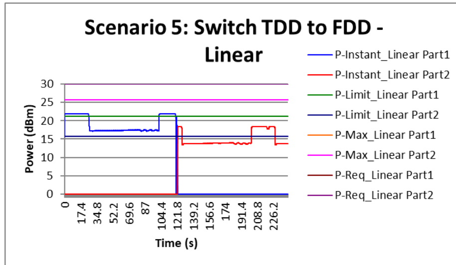
Figure 8-21: Time-averaged conducted TX power over time for TDD/FDD Switch case (LTE Band 41 PC3 Ant 4 – Part 1 to LTE Band 66 Ant 4 – Part 2)
