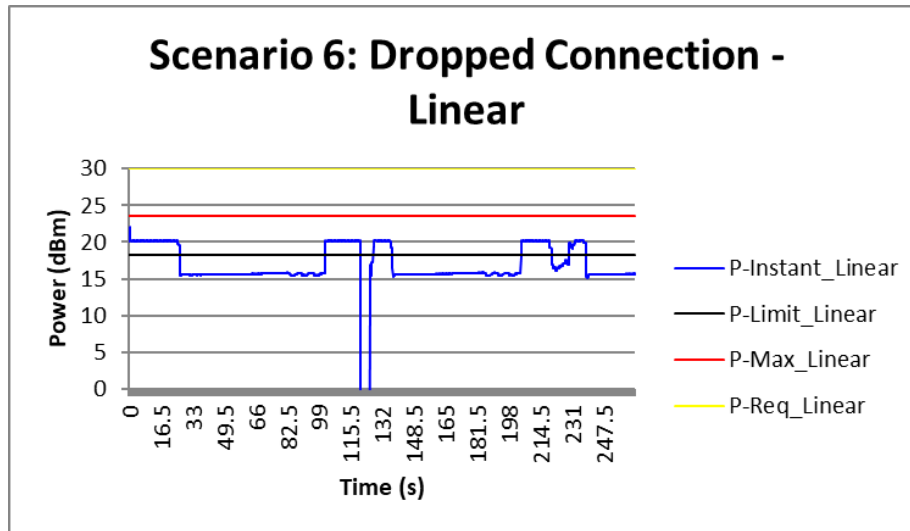
Figure 8-23: Time-averaged conducted TX power over time for Call Disconnection case (LTE Band 30 Ant 3b)
