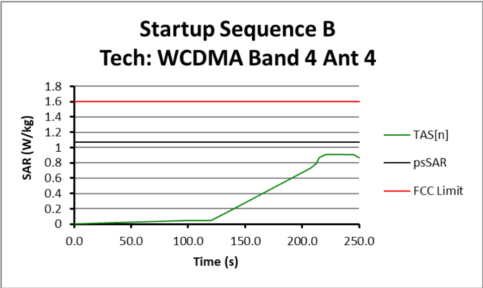
Figure 10-1: Time-averaged SAR for Change in Requested Power case (WCDMA Band 4 – Test Sequence B)
