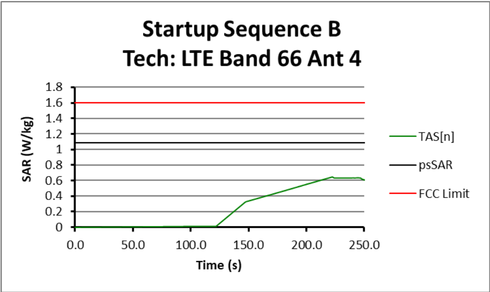
Figure 10-3: Time-averaged SAR for Change in Requested Power case (LTE Band 66 – Test Sequence B)
