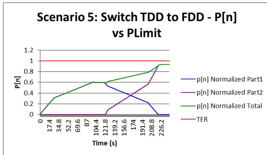
Figure 8-22: Normalized Time-averaged Power for TDD/FDD Switch case (LTE Band 41 PC3 Ant 4 – Part 1 to LTE Band 66 Ant 4 – Part 2)
