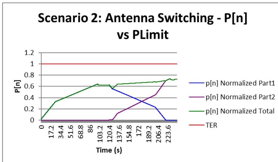
Figure 8-16: Normalized Time-averaged Power for Antenna Switch case (LTE Band 25 Ant 3b – Part 1 to LTE Band 66 Ant 4 – Part 2)
