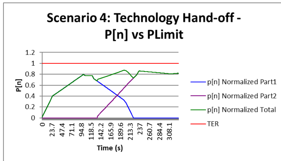
Figure 8-20: Normalized Time-averaged Power for Technology Hand-Off case (LTE Band 7 Ant 4 – Part 1 to WCDMA Band 4 Ant 4 – Part 2)
