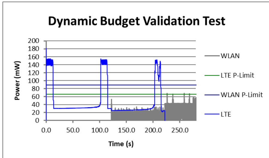
Figure 5-1(a) Dynamic Budget Validation Time-averaged conducted TX power
