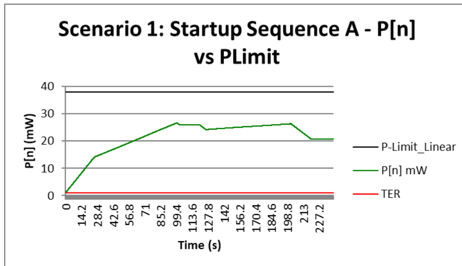
Figure 8-4: Time-averaged Power for Changes in Power case (LTE Band 66 Ant 4 – Test Sequence A)
