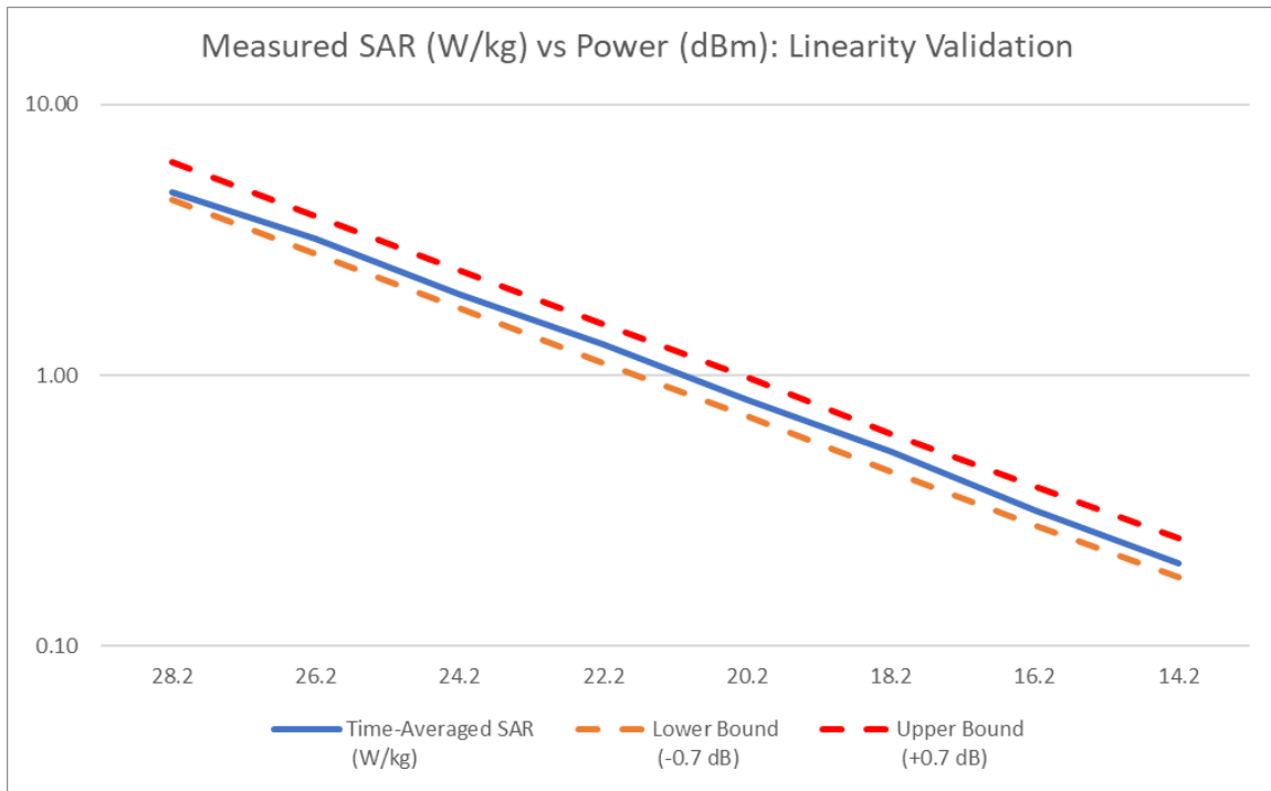
Figure 11-5 NR Band n41 Ant 3b Linearity Validation Results
