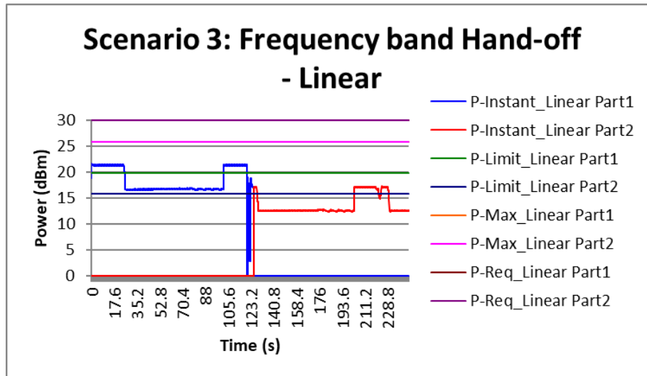
Figure 8-17: Time-averaged conducted TX power over time for Change in Band case (LTE Band 7 Ant 4 – Part 1 to LTE Band 66 Ant 4 – Part 2)
