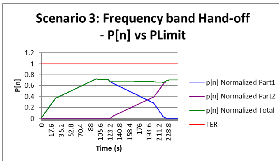
Figure 8-18: Normalized Time-averaged Power for Change in Band case (LTE Band 7 Ant 4 – Part 1 to LTE Band 66 Ant 4 – Part 2)
