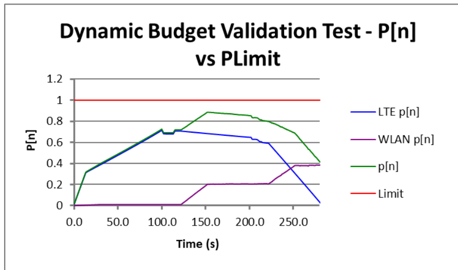
Figure 5-1(b) Dynamic Budget Validation Normalized Time-averaged conducted power
