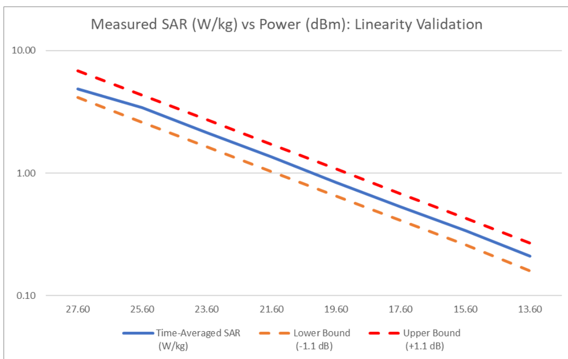
Figure 11-4 NR Band n77 Sub-band C Ant 3a Linearity Validation Results
