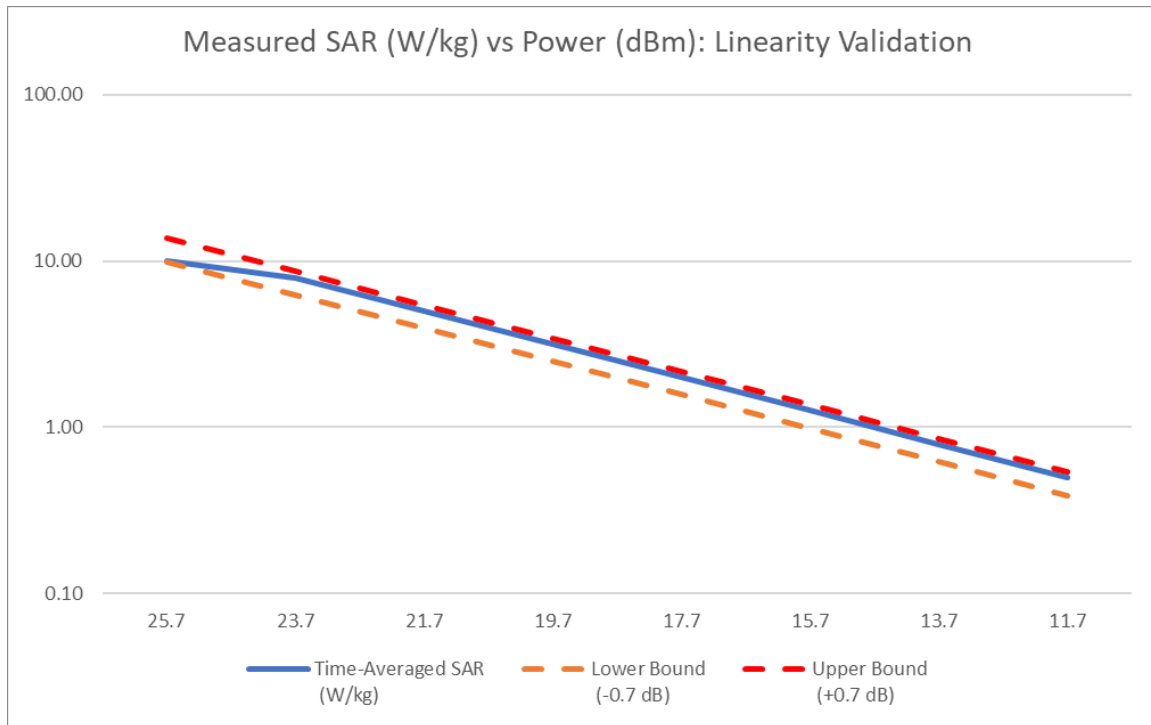
Figure 11-6 LTE Band 66 Ant 4 Linearity Validation Results
