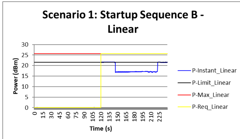
Figure 8-9: Time-averaged conducted TX power over time for Changes in Power case (LTE Band 41 Ant 3b – Test Sequence B)
