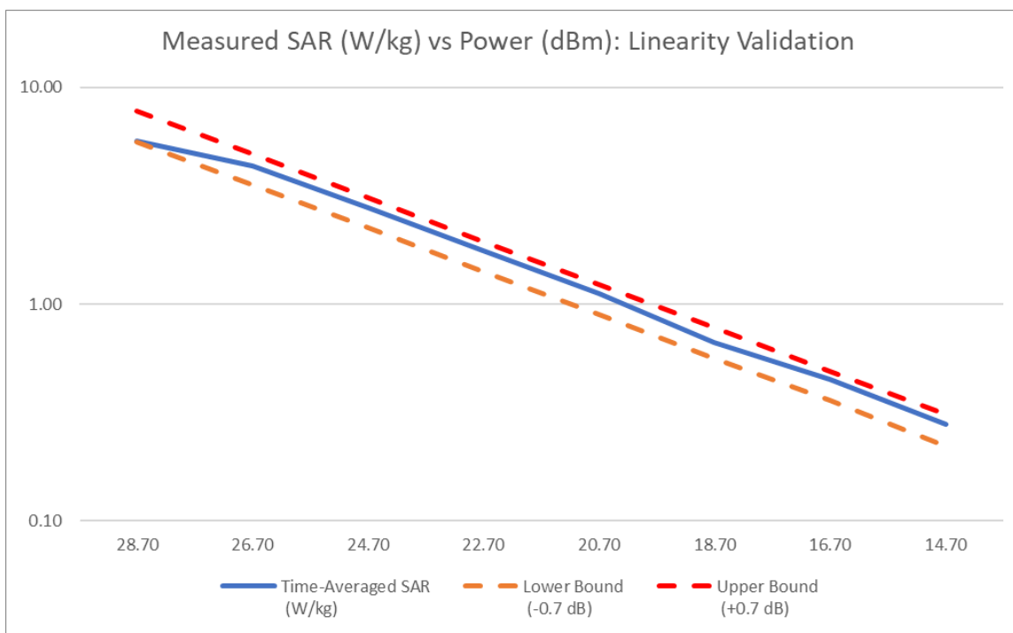
Figure 11-3 NR Band n41 Ant 2 Linearity Validation Results
