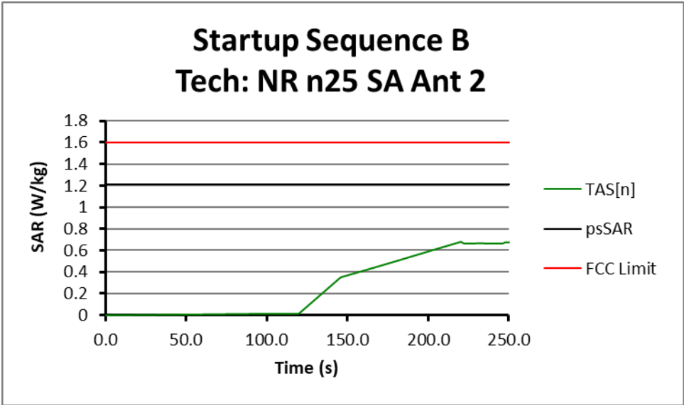
Figure 10-6: Time-averaged SAR for Change in Requested Power case (NR n25 SA – Test Sequence B)
