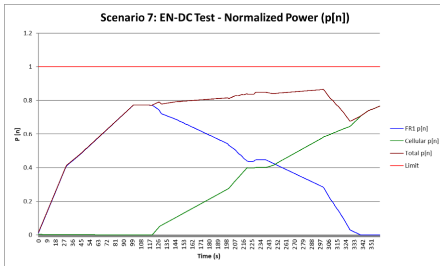
Figure 8-26: Normalized Time-averaged Power for Technology Hand-Off (ENDC) case (LTE Band 5 Ant 4 to NR n66 NSA Ant 3b)
