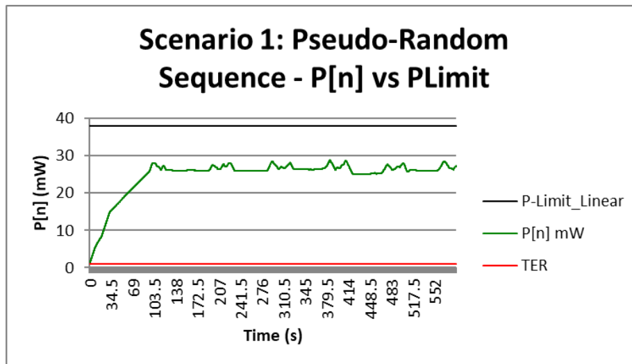
Figure 8-8: Time-averaged Power for Changes in Power case (LTE Band 66 Ant 4 – Pseudo-Random Test Sequence)
