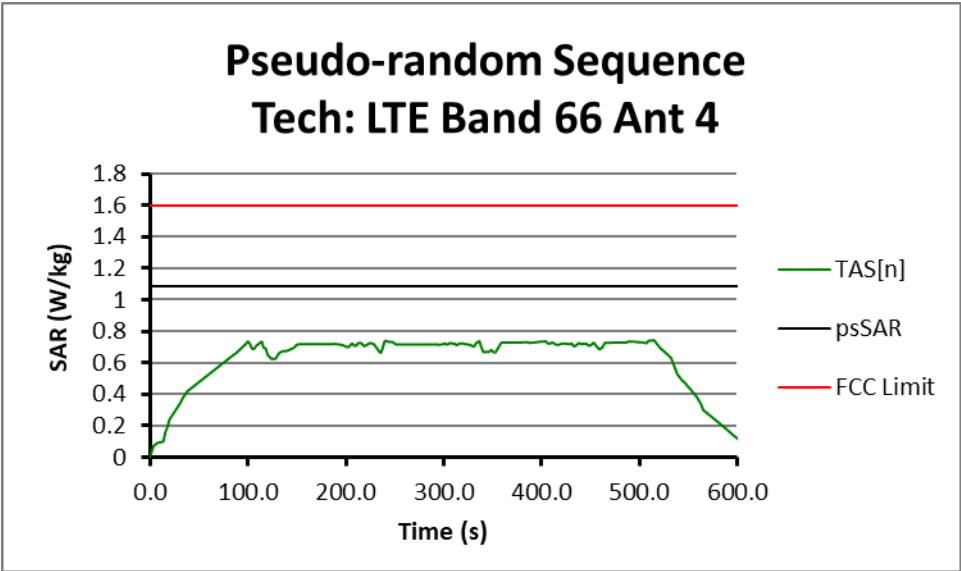
Figure 10-4: Time-averaged SAR for Change in Requested Power case (LTE Band 66 – Pseudo-Random Test Sequence)
