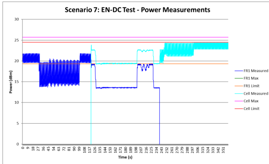
Figure 8-25: Time-averaged conducted TX power over time for Technology Hand-Off (ENDC) case LTE Band 5 Ant 4 to NR n66 NSA Ant 3b)
