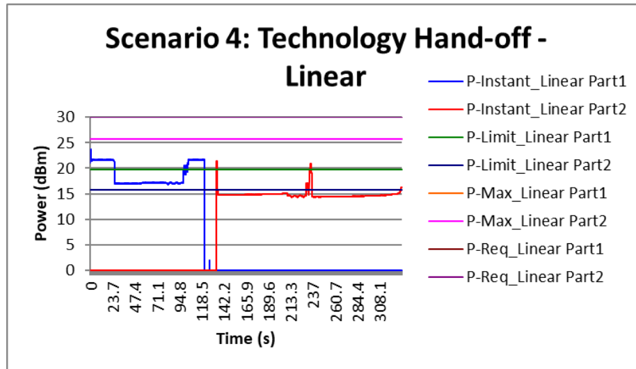
Figure 8-19: Time-averaged conducted TX power over time for Technology Hand-Off case (LTE Band 7 Ant 4 – Part 1 to WCDMA Band 4 Ant 4 – Part 2)
