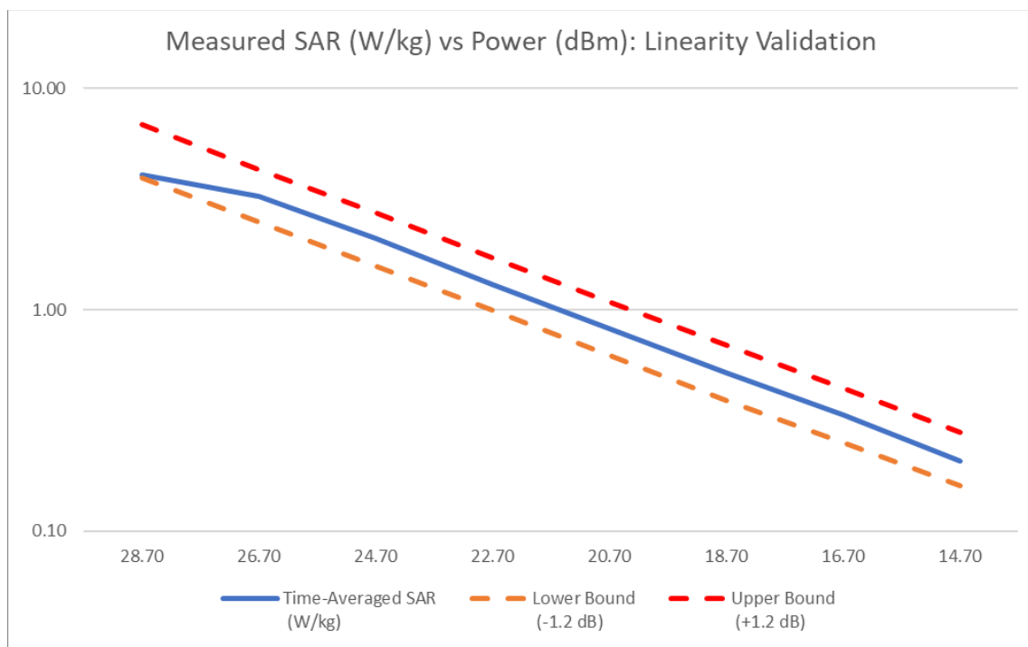
Figure 11-2 NR Band n41 Ant 1b Linearity Validation Results
