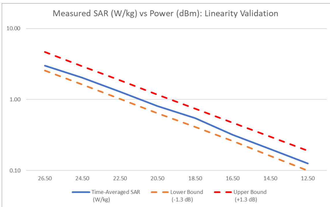
Figure 11-1 NR Band n77 Sub-band C Ant 1a Linearity Validation Results
