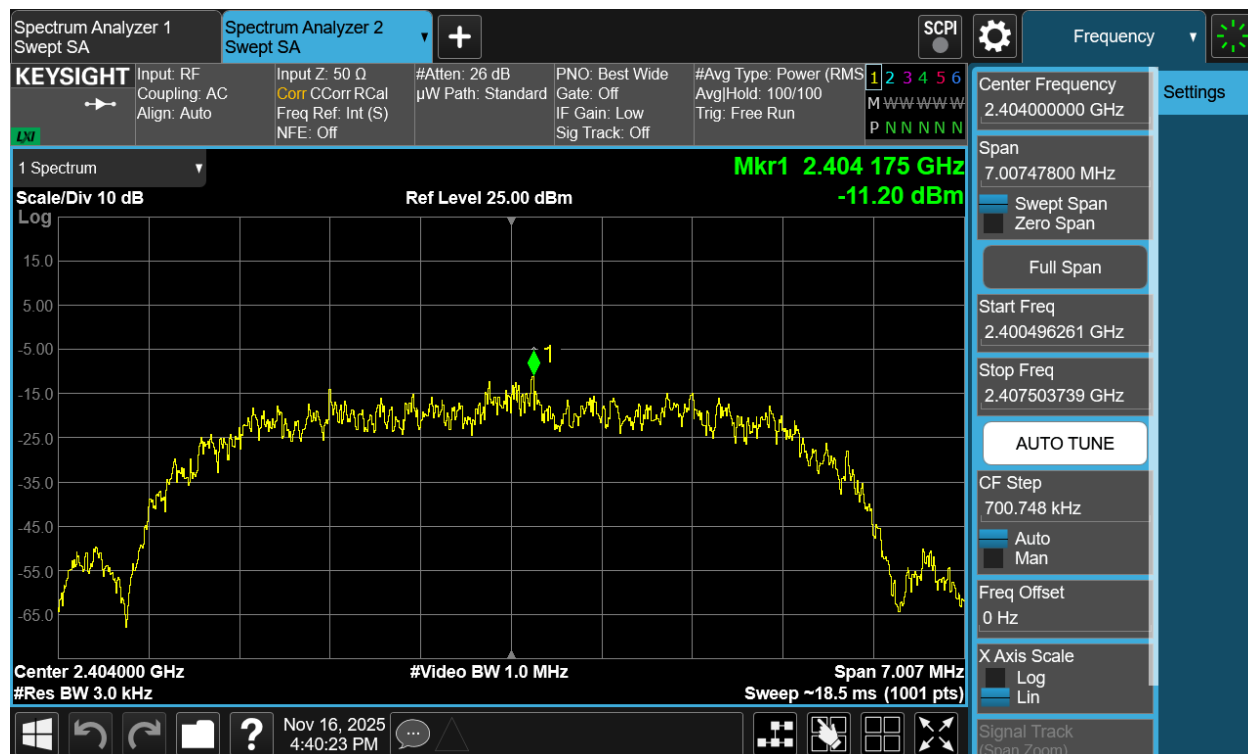
Plot 7-118. Power Spectral Density Plot Antenna 1a (Bluetooth (HDR8), 8Mbps, iPA – Ch. 1)
