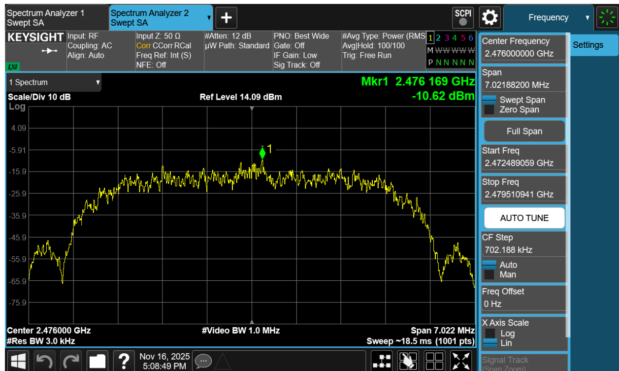
Plot 7-168. Power Spectral Density Plot TxBF Antenna 1a (Bluetooth (HDR8), 8Mbps, iPA – Ch. 73)
