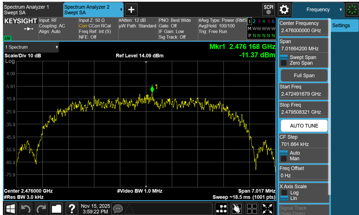
Plot 7-167. Power Spectral Density Plot TxBF Antenna 3a (Bluetooth (HDR8), 8Mbps, iPA – Ch. 73)
