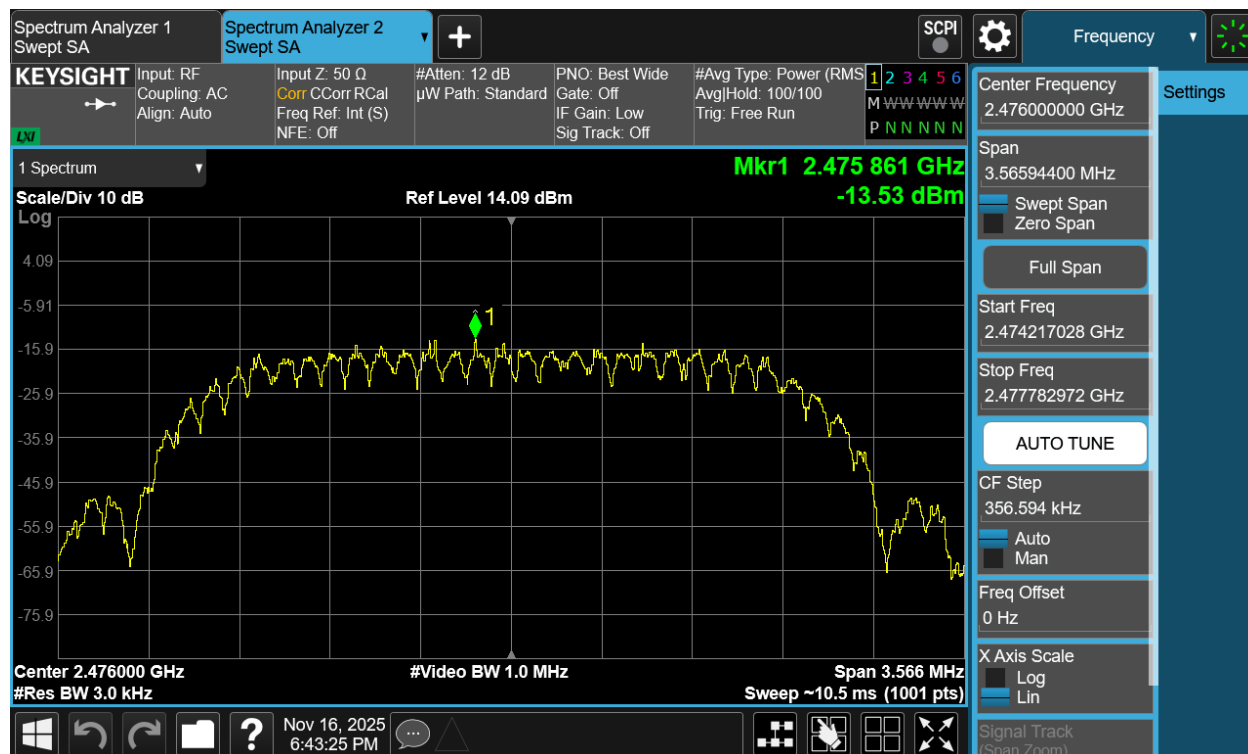
Plot 7-144. Power Spectral Density Plot Antenna 1a (Bluetooth (HDT2), 2Mbps, iPA – Ch. 73)
