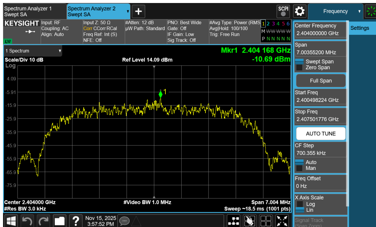
Plot 7-163. Power Spectral Density Plot TxBF Antenna 3a (Bluetooth (HDR8), 8Mbps, iPA – Ch. 1)
