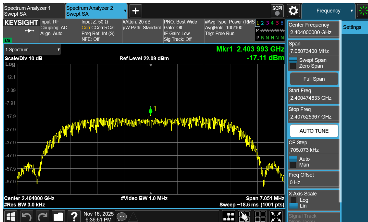
Plot 7-136. Power Spectral Density Plot Antenna 1a (Bluetooth (HDRPM16), 16Mbps, iPA – Ch. 1)
