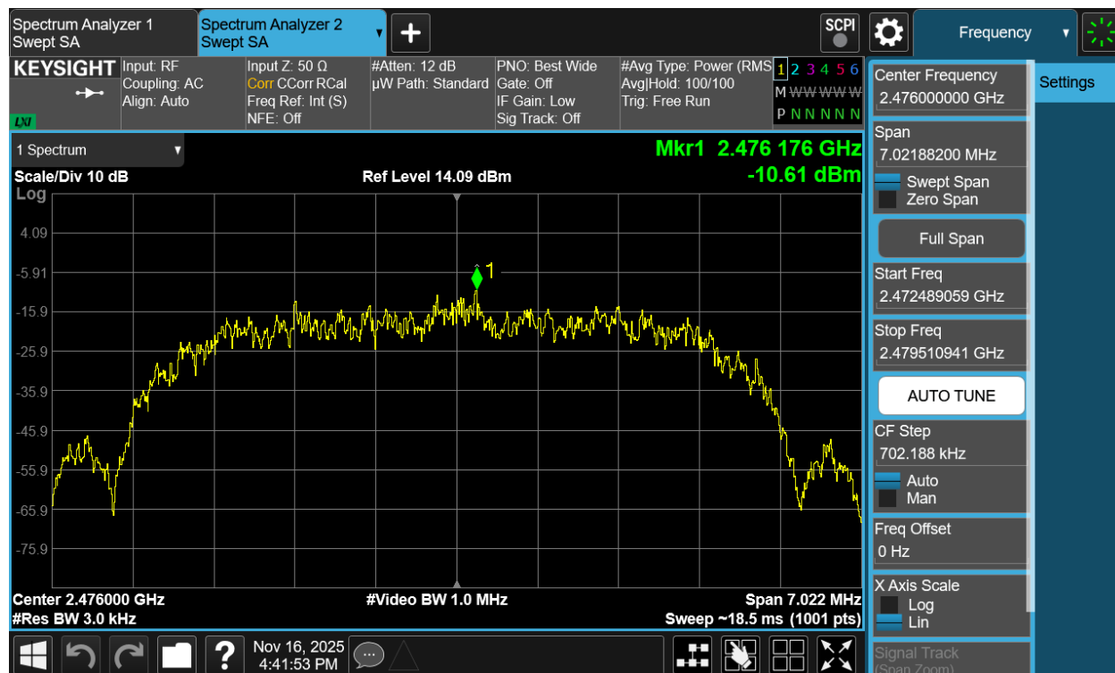
Plot 7-120. Power Spectral Density Plot Antenna 1a (Bluetooth (HDR8), 8Mbps, iPA – Ch. 73)
