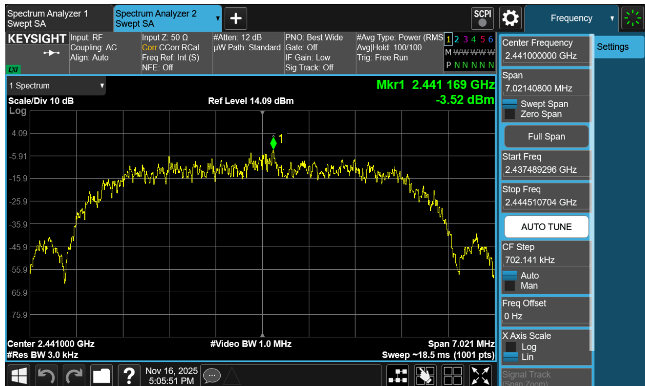
Plot 7-160. Power Spectral Density Plot TxBF Antenna 1a (Bluetooth (HDR8), 8Mbps, ePA – Ch. 38)
