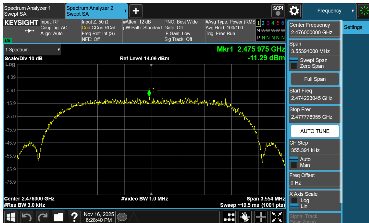
Plot 7-126. Power Spectral Density Plot Antenna 1a (Bluetooth (HDRPS2), 2Mbps, iPA – Ch. 73)
