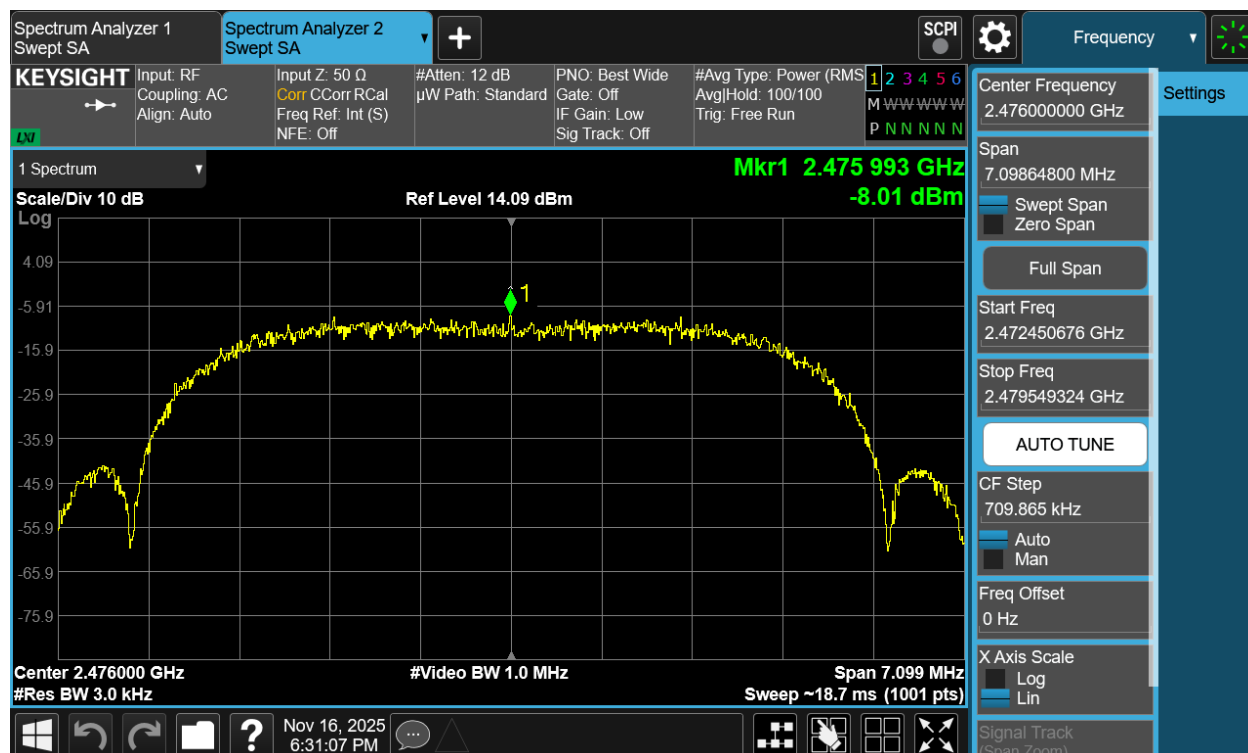
Plot 7-129. Power Spectral Density Plot Antenna 1a (Bluetooth (XHDRPM6), 6Mbps, ePA – Ch. 73)
