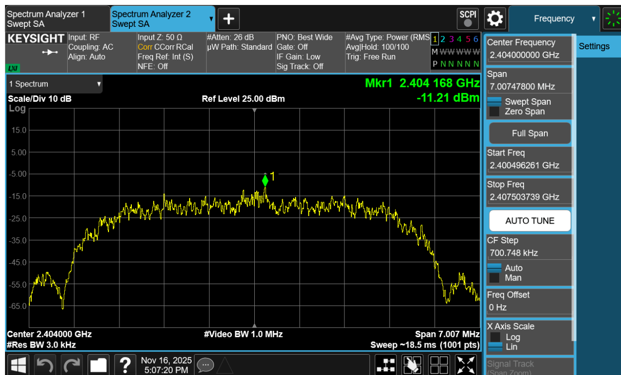
Plot 7-164. Power Spectral Density Plot TxBF Antenna 1a (Bluetooth (HDR8), 8Mbps, iPA – Ch. 1)
