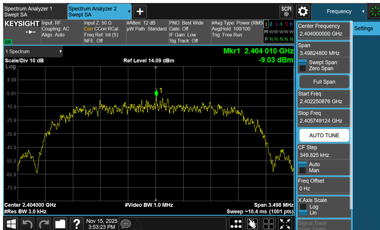
Plot 7-151. Power Spectral Density Plot TxBF Antenna 3a (Bluetooth (HDR4), 4Mbps, iPA – Ch. 1)
