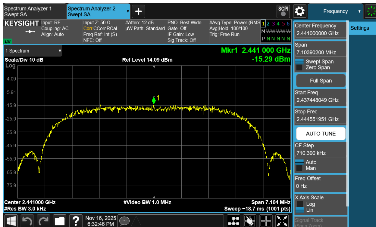
Plot 7-131. Power Spectral Density Plot Antenna 1a (Bluetooth (XHDRPM6), 6Mbps, iPA – Ch. 38)
