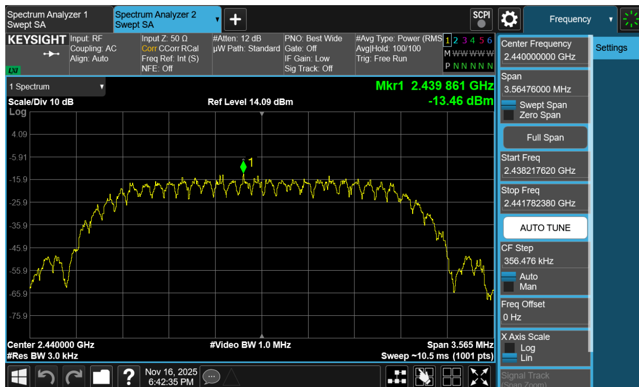
Plot 7-143. Power Spectral Density Plot Antenna 1a (Bluetooth (HDT2), 2Mbps, iPA – Ch. 37)
