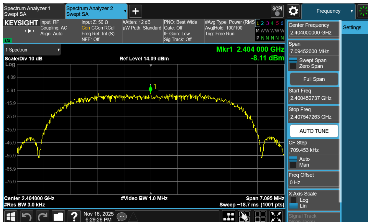
Plot 7-127. Power Spectral Density Plot Antenna 1a (Bluetooth (XHDRPM6), 6Mbps, ePA – Ch. 1)
