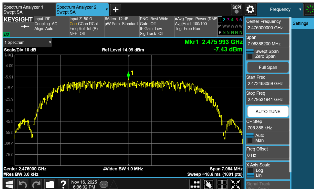
Plot 7-135. Power Spectral Density Plot Antenna 1a (Bluetooth (HDRPM16), 16Mbps, ePA – Ch. 73)
