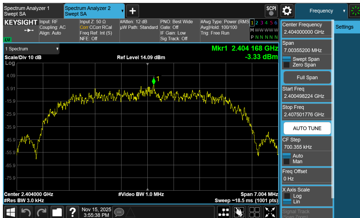
Plot 7-157. Power Spectral Density Plot TxBF Antenna 3a (Bluetooth (HDR8), 8Mbps, ePA – Ch. 1)
