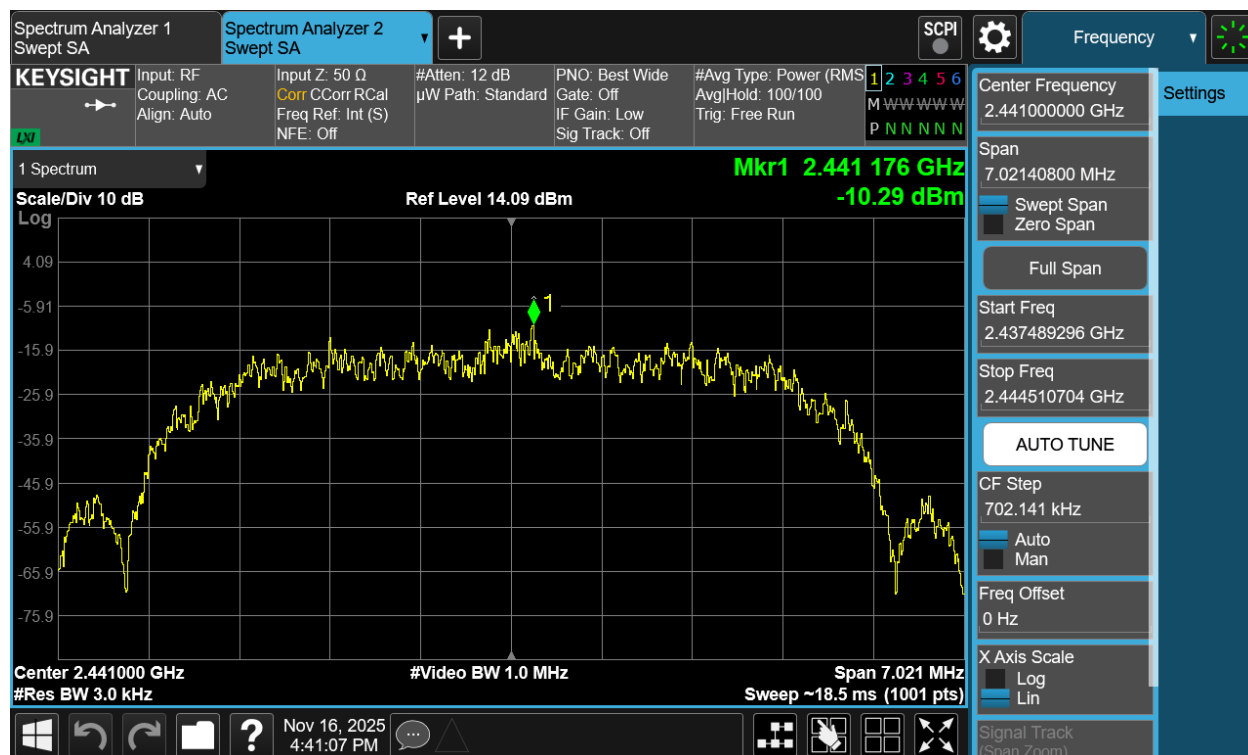
Plot 7-119. Power Spectral Density Plot Antenna 1a (Bluetooth (HDR8), 8Mbps, iPA – Ch. 38)
