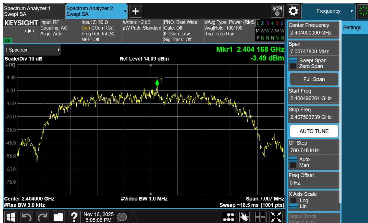
Plot 7-158. Power Spectral Density Plot TxBF Antenna 1a (Bluetooth (HDR8), 8Mbps, ePA – Ch. 1)
