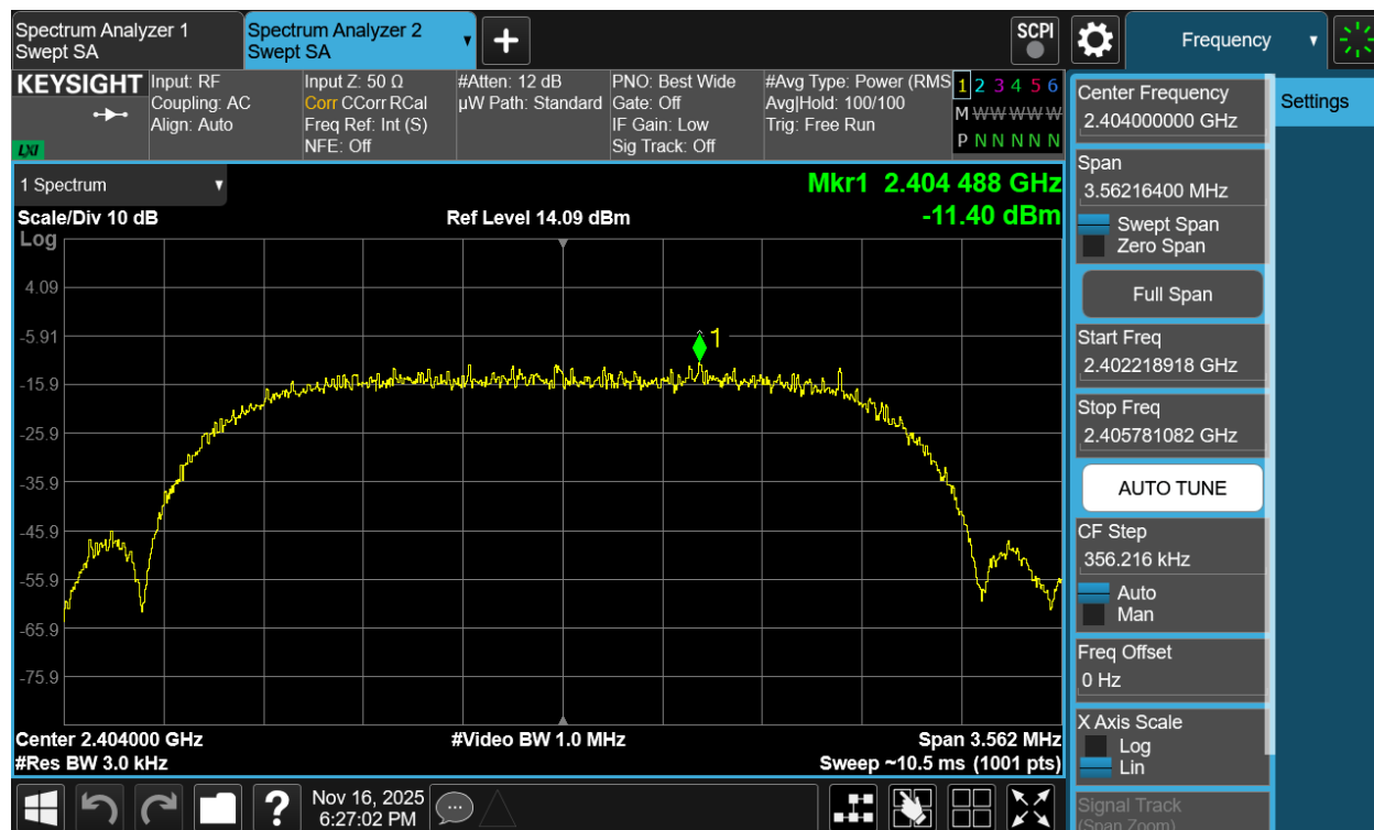
Plot 7-124. Power Spectral Density Plot Antenna 1a (Bluetooth (HDRPS2), 2Mbps, iPA – Ch. 1)
