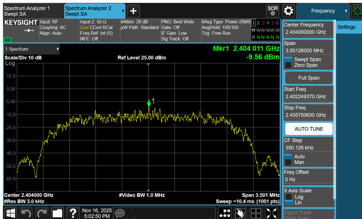
Plot 7-152. Power Spectral Density Plot TxBF Antenna 1a (Bluetooth (HDR4), 4Mbps, iPA – Ch. 1)
