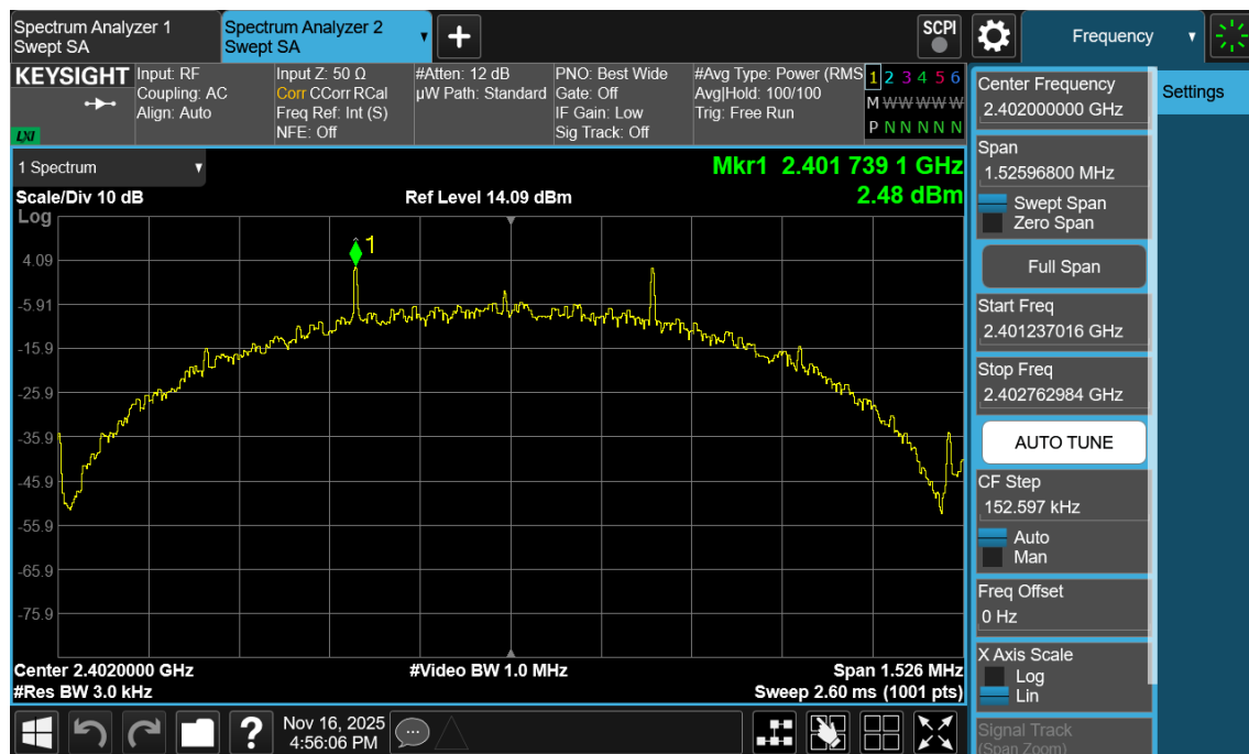
Plot 7-110. Power Spectral Density Plot Antenna 1a (Bluetooth (LE), 500kbps, ePA – Ch. 0)
