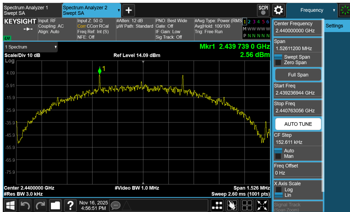
Plot 7-112. Power Spectral Density Plot Antenna 1a (Bluetooth (LE), 500kbps, ePA – Ch. 19)
