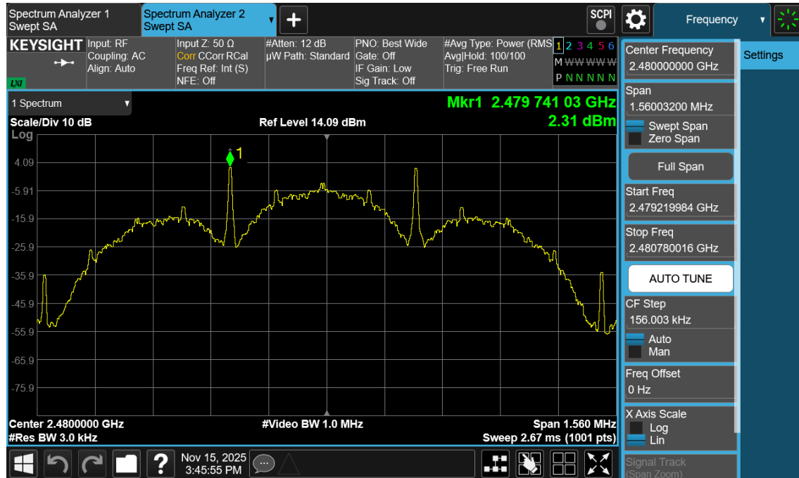
Plot 7-107. Power Spectral Density Plot Antenna 3a (Bluetooth (LE), 125kbps, iPA – Ch. 39)
