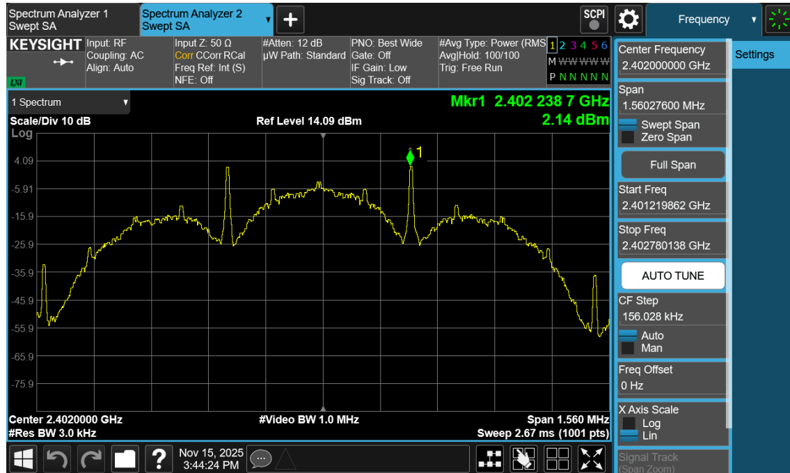
Plot 7-103. Power Spectral Density Plot Antenna 3a (Bluetooth (LE), 125kbps, iPA – Ch. 0)
