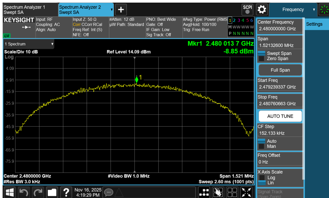
Plot 7-90. Power Spectral Density Plot Antenna 1a (Bluetooth (LE), 1Mbps, iPA – Ch. 39)
