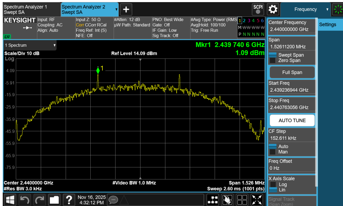
Plot 7-83. Power Spectral Density Plot Antenna 1a (Bluetooth (LE), 500kbps, iPA – Ch. 19)
