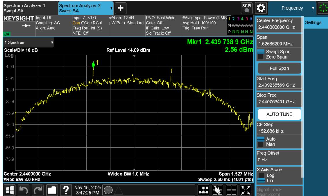
Plot 7-111. Power Spectral Density Plot Antenna 3a (Bluetooth (LE), 500kbps, ePA – Ch. 19)
