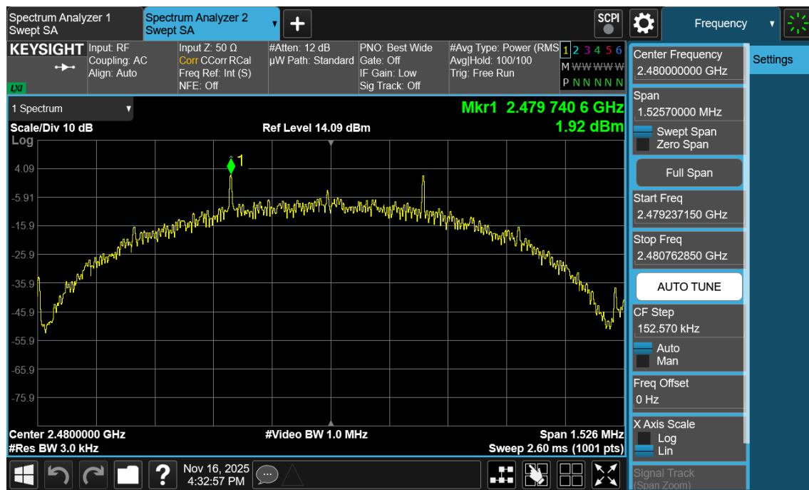
Plot 7-84. Power Spectral Density Plot Antenna 1a (Bluetooth (LE), 500kbps, iPA – Ch. 39)
