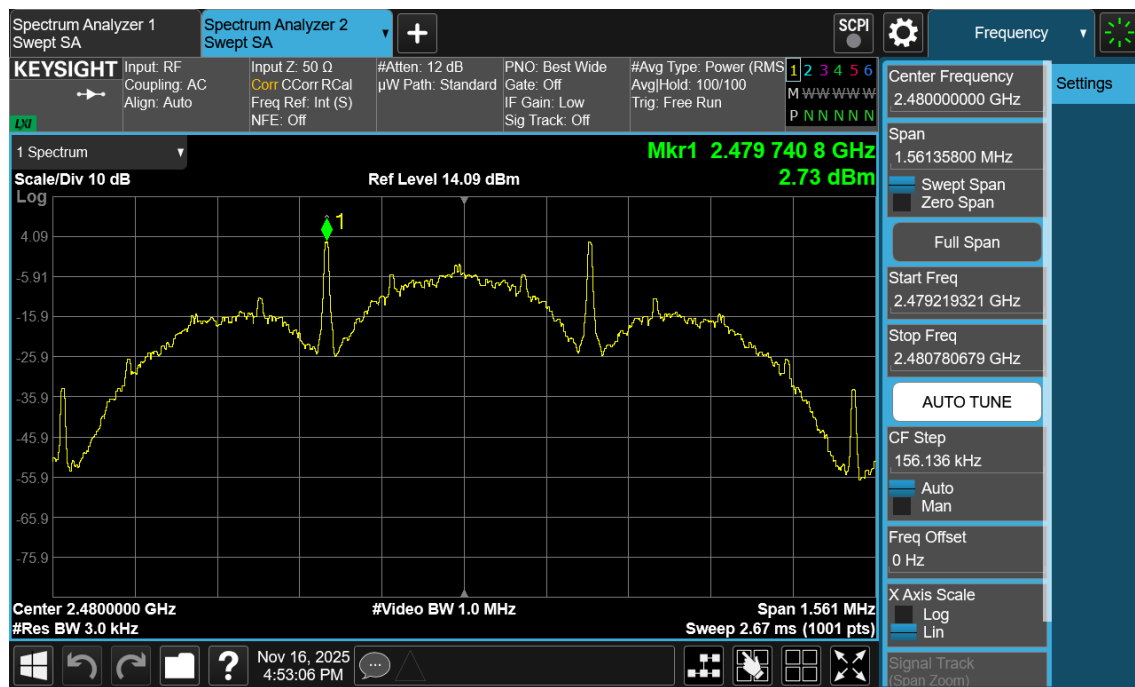
Plot 7-102. Power Spectral Density Plot Antenna 1a (Bluetooth (LE), 125kbps, ePA – Ch. 39)
