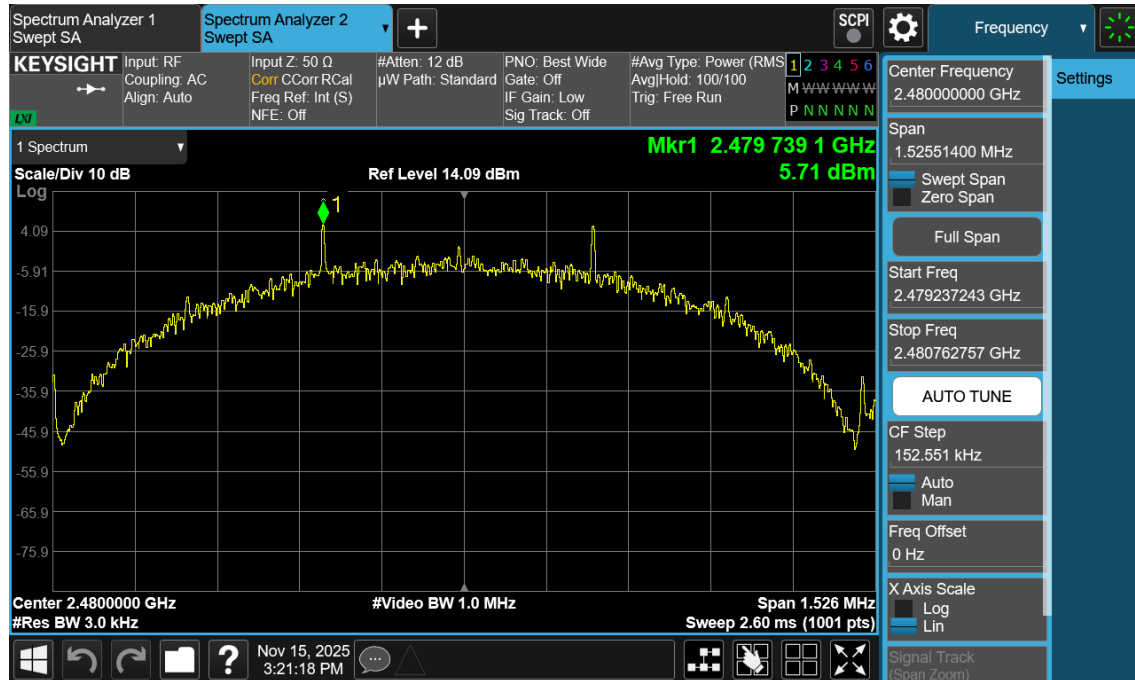
Plot 7-57. Power Spectral Density Plot Antenna 3a (Bluetooth (LE), 500kbps, ePA – Ch. 39)
