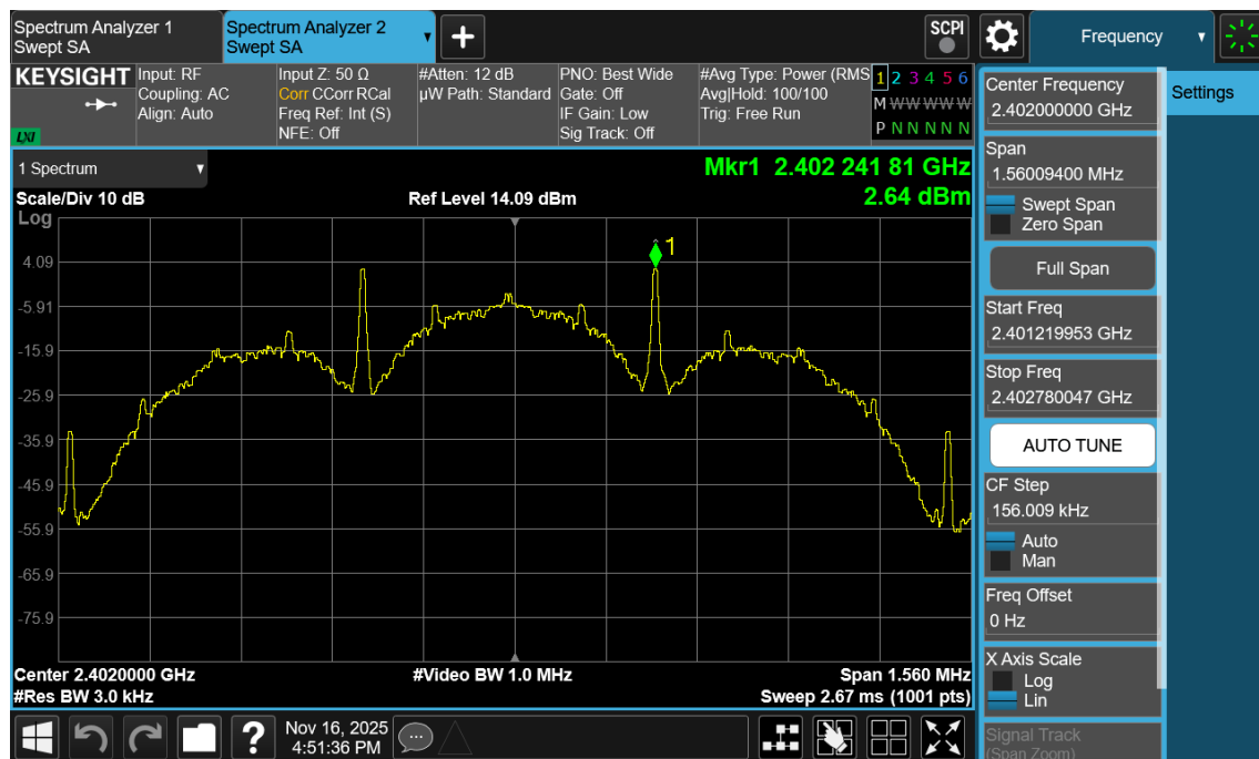
Plot 7-98. Power Spectral Density Plot Antenna 1a (Bluetooth (LE), 125kbps, ePA – Ch. 0)
