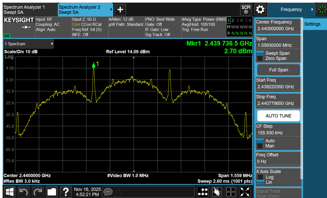
Plot 7-100. Power Spectral Density Plot Antenna 1a (Bluetooth (LE), 125kbps, ePA – Ch. 19)
