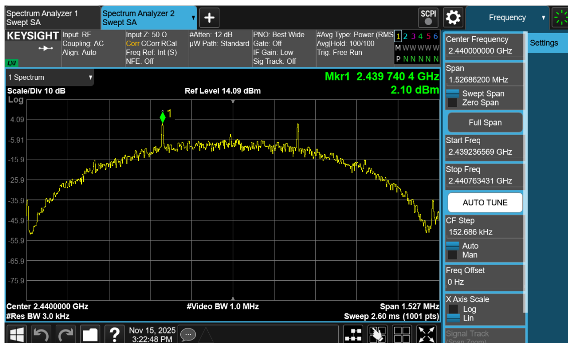
Plot 7-59. Power Spectral Density Plot Antenna 3a (Bluetooth (LE), 500kbps, iPA – Ch. 19)
