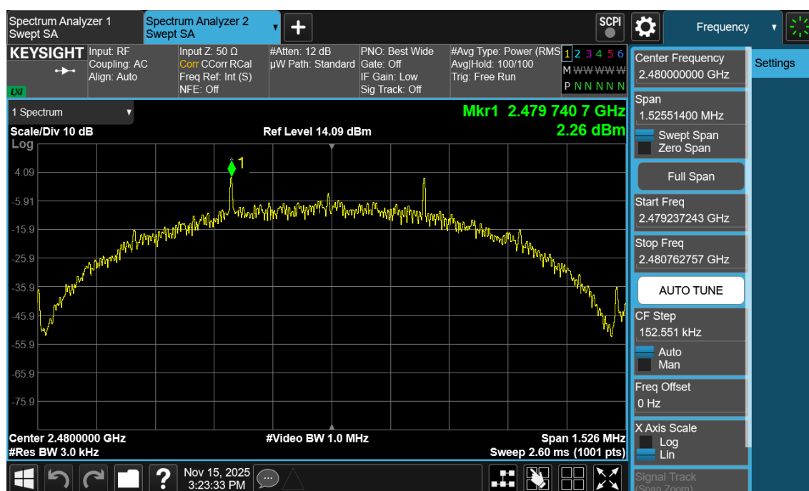
Plot 7-60. Power Spectral Density Plot Antenna 3a (Bluetooth (LE), 500kbps, iPA – Ch. 39)
