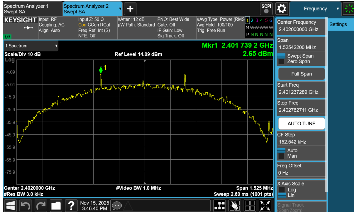
Plot 7-109. Power Spectral Density Plot Antenna 3a (Bluetooth (LE), 500kbps, ePA – Ch. 0)
