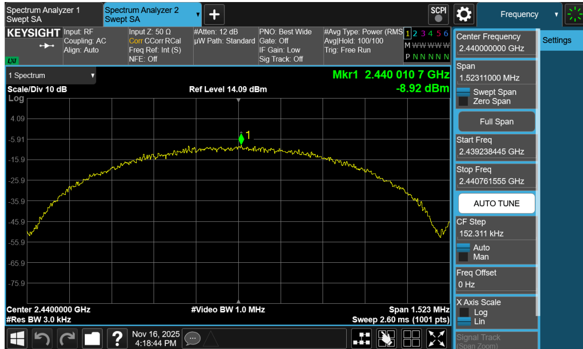
Plot 7-89. Power Spectral Density Plot Antenna 1a (Bluetooth (LE), 1Mbps, iPA – Ch. 19)
