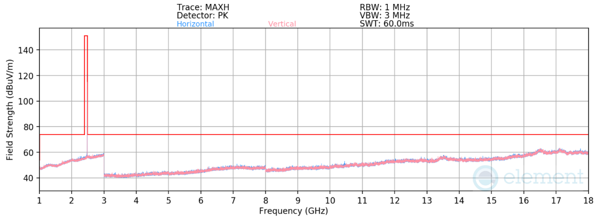
Plot 7-175. Radiated Spurious Emissions 1-18GHz TxBF (1Mbps ePA – Ch. 39)
