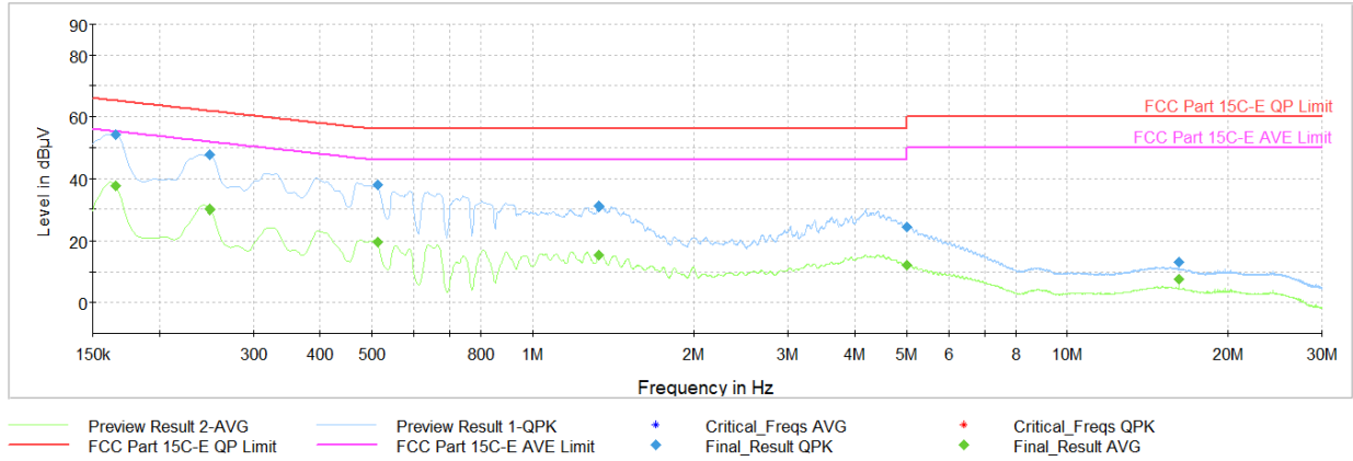
Plot 7-191. AC Line Conducted Plot with Bluetooth LE TxBF (N, 1Mbps ePA – Ch.19, with AC/DC Adapter)
