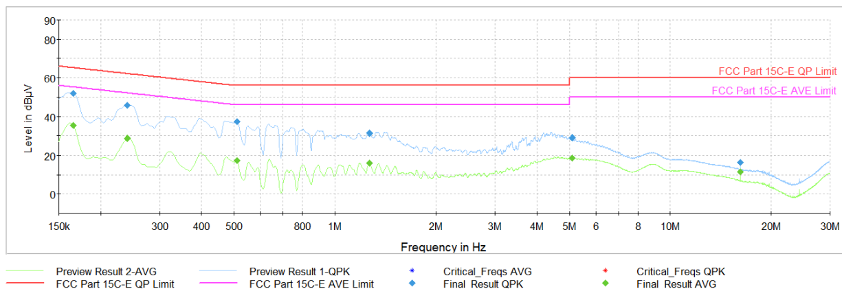
Plot 7-190. AC Line Conducted Plot with Bluetooth LE Tx BF (L1, 1Mbps ePA – Ch.19 with AC/DC Adapter)
