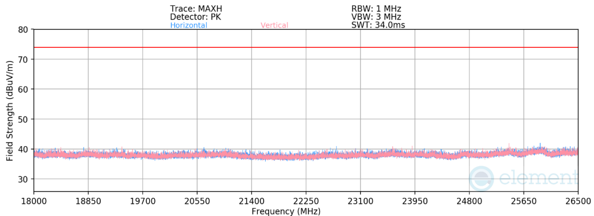
Plot 7-176. Radiated Spurious Emissions Above 18GHz TxBF (1Mbps ePA – Ch. 39)
