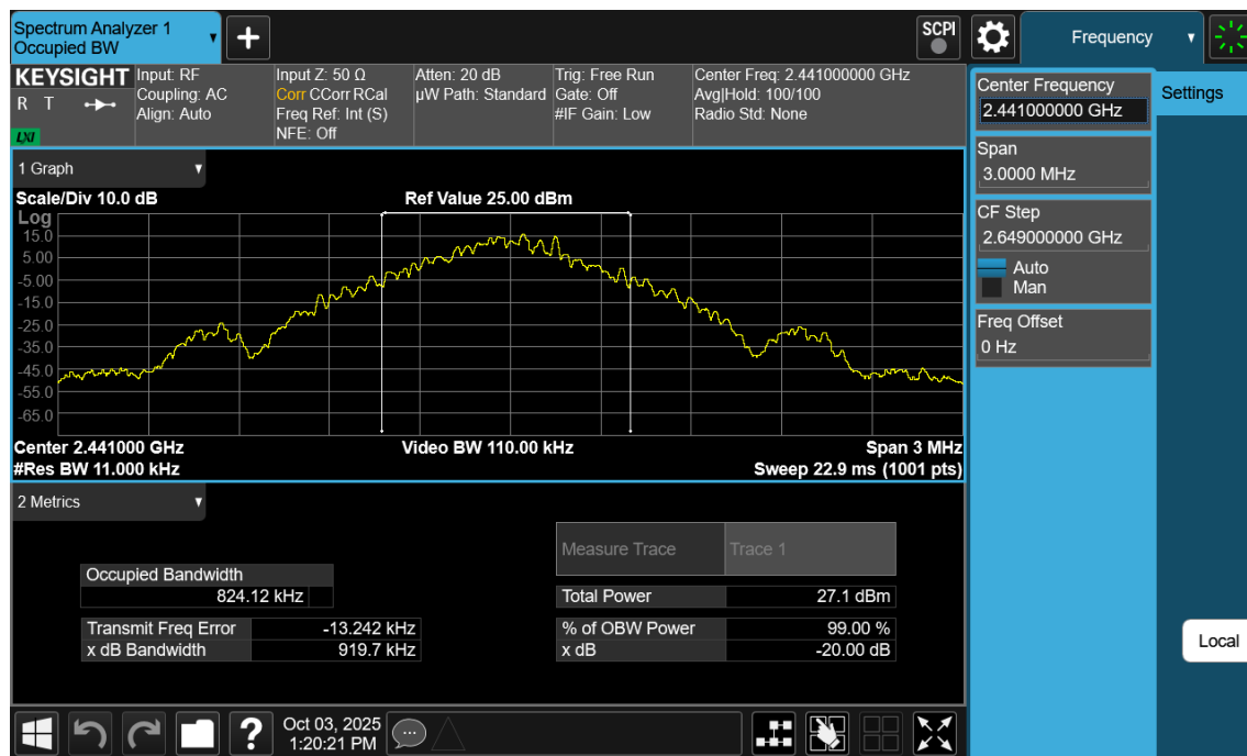
Plot 7-2. 20dB BW and 99% OBW Plot Antenna 3a (Bluetooth, GFSK, ePA – Ch. 39)
