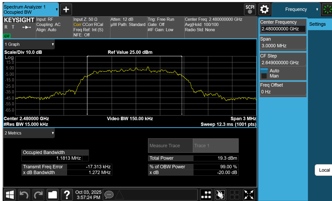
Plot 7-12. 20dB BW and 99% OBW Plot Antenna 1a (Bluetooth, 8DPSK, ePA – Ch. 78)
