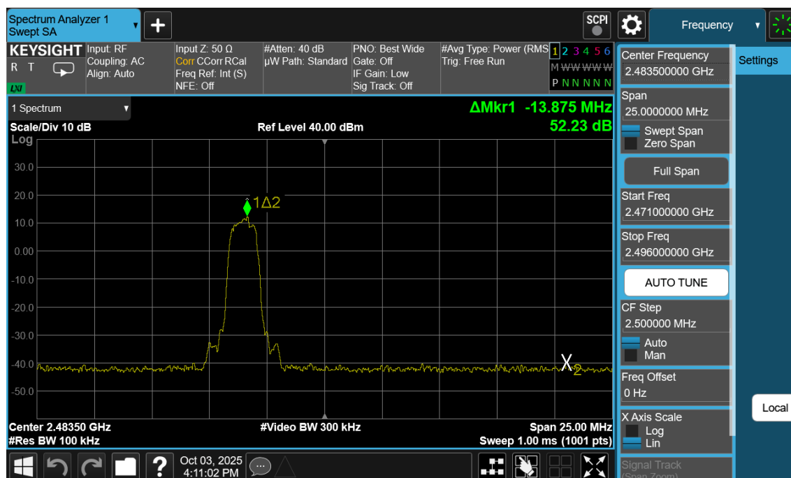
Plot 7-26. Band Edge Plot Antenna 1a (Bluetooth with Hopping Disabled, 8DPSK, ePA – Ch. 78)
