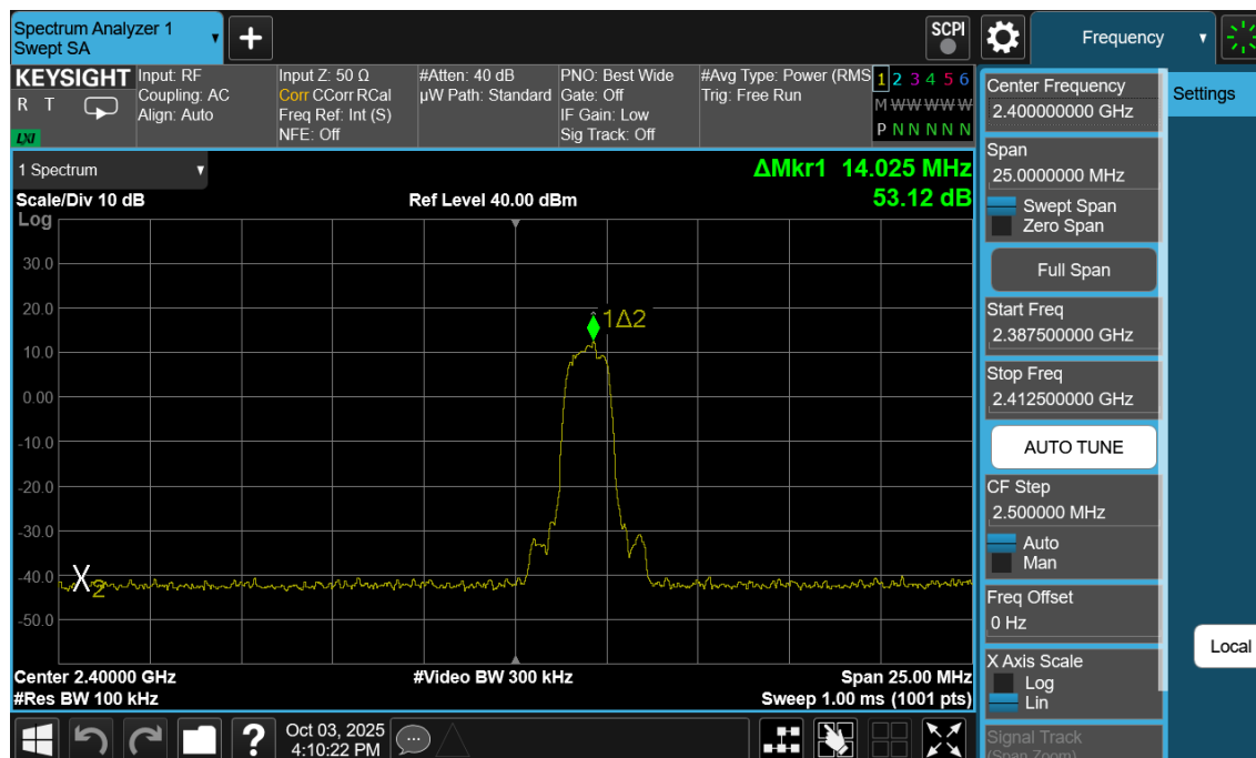
Plot 7-25. Band Edge Plot Antenna 1a (Bluetooth with Hopping Disabled, 8DPSK, ePA – Ch. 0)
