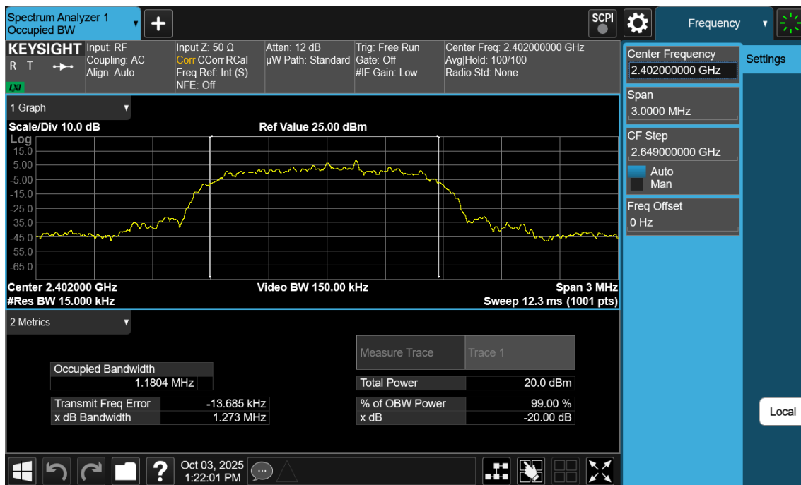
Plot 7-4. 20dB BW and 99% OBW Plot Antenna 3a (Bluetooth, 8DPSK, ePA – Ch. 0)
