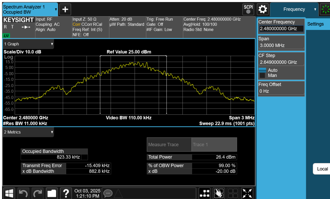
Plot 7-3. 20dB BW and 99% OBW Plot Antenna 3a (Bluetooth, GFSK, ePA – Ch. 78)
