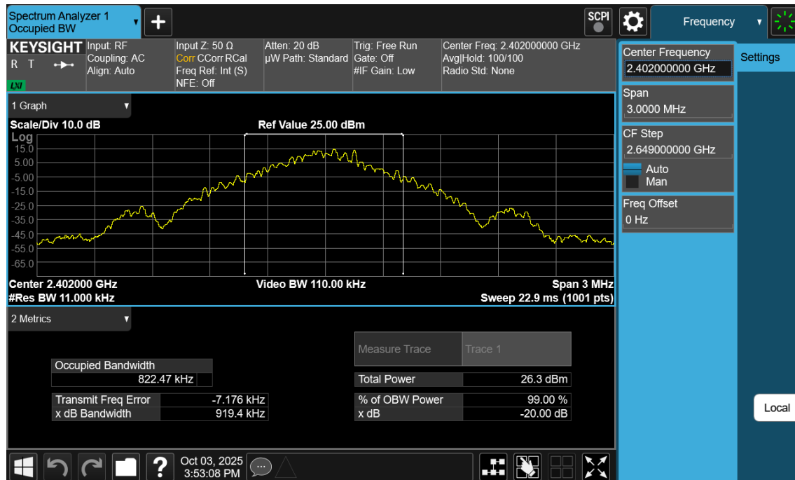
Plot 7-7. 20dB BW and 99% OBW Plot Antenna 1a (Bluetooth, GFSK, ePA – Ch. 0)
