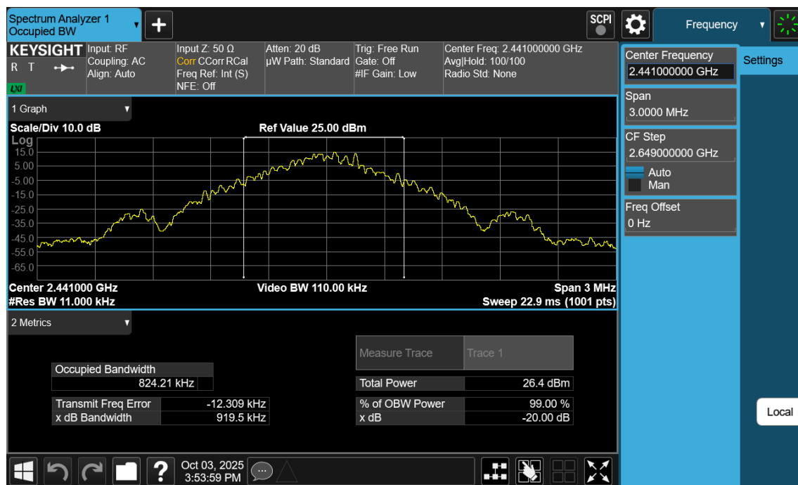
Plot 7-8. 20dB BW and 99% OBW Plot Antenna 1a (Bluetooth, GFSK, ePA – Ch. 39)
