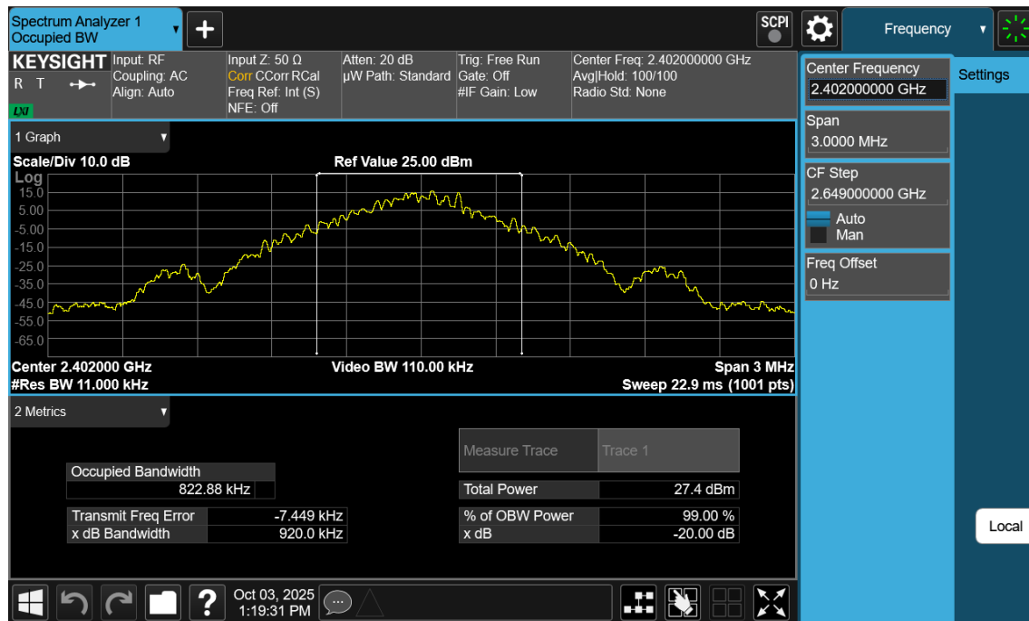
Plot 7-1. 20dB BW and 99% OBW Plot Antenna 3a (Bluetooth, GFSK, ePA – Ch. 0)
