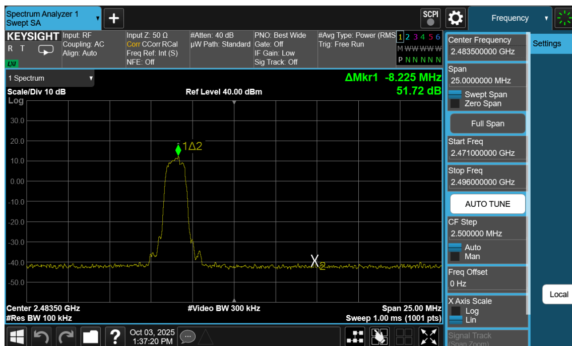
Plot 7-18. Band Edge Plot Antenna 3a (Bluetooth with Hopping Disabled, 8DPSK, ePA – Ch. 78)
