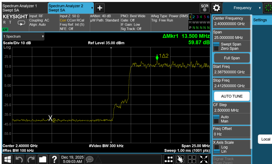
Plot 7-19. Band Edge Plot Antenna 3a (Bluetooth with Hopping Enabled, 8DPSK, ePA)
