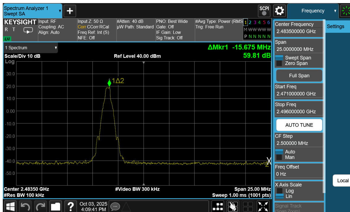
Plot 7-22. Band Edge Plot Antenna 1a (Bluetooth with Hopping Disabled, GFSK, ePA – Ch. 78)
