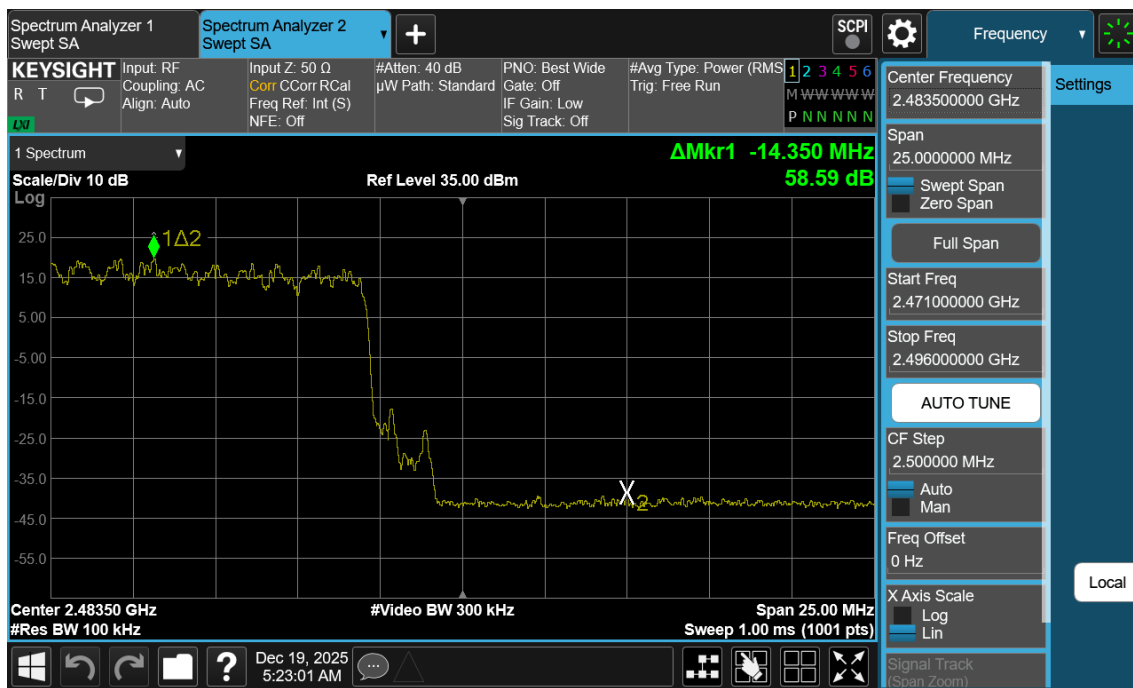
Plot 7-28. Band Edge Plot Antenna 1a (Bluetooth with Hopping Enabled, 8DPSK, ePA)
