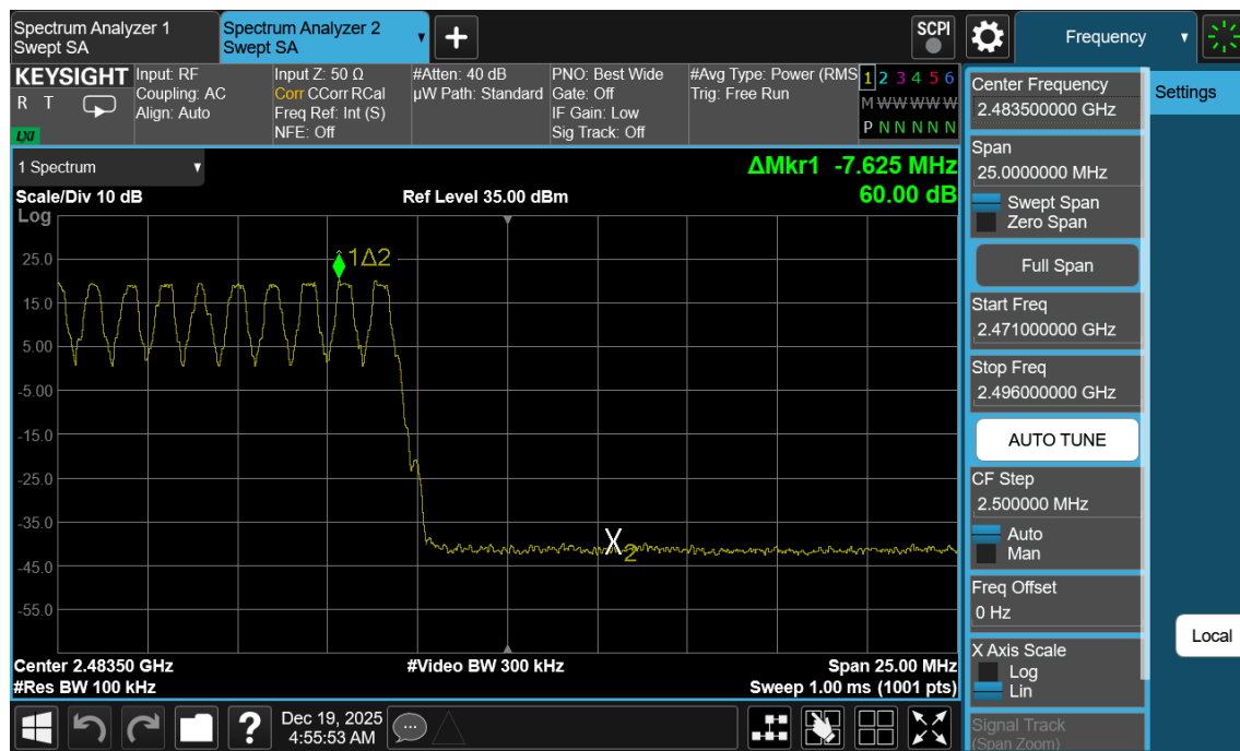
Plot 7-16. Band Edge Plot Antenna 3a (Bluetooth with Hopping Enabled, GFSK, ePA)
