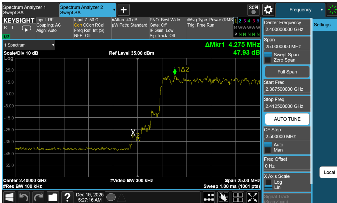
Plot 7-27. Band Edge Plot Antenna 1a (Bluetooth with Hopping Enabled, 8DPSK, ePA)
