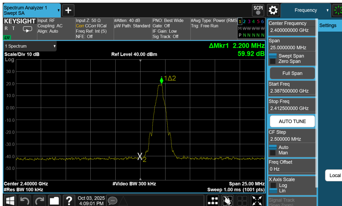
Plot 7-21. Band Edge Plot Antenna 1a (Bluetooth with Hopping Disabled, GFSK, ePA – Ch. 0)
