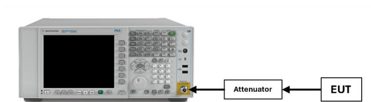
Figure 7-5. Test Instrument & Measurement Setup
