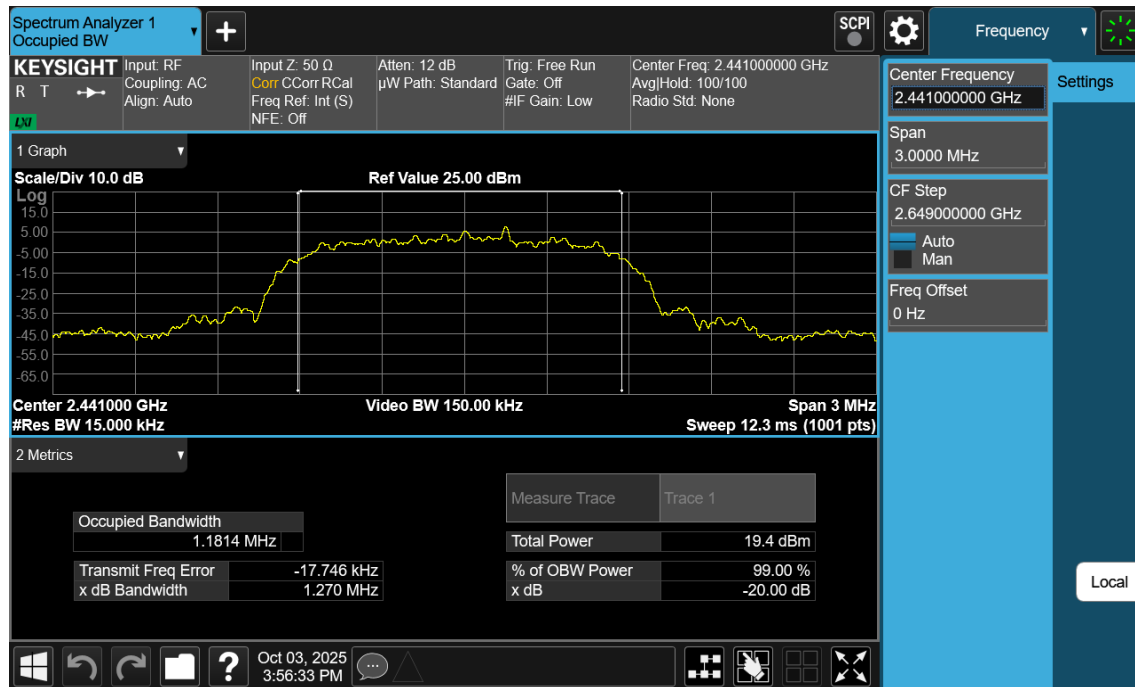
Plot 7-11. 20dB BW and 99% OBW Plot Antenna 1a (Bluetooth, 8DPSK, ePA – Ch. 39)
