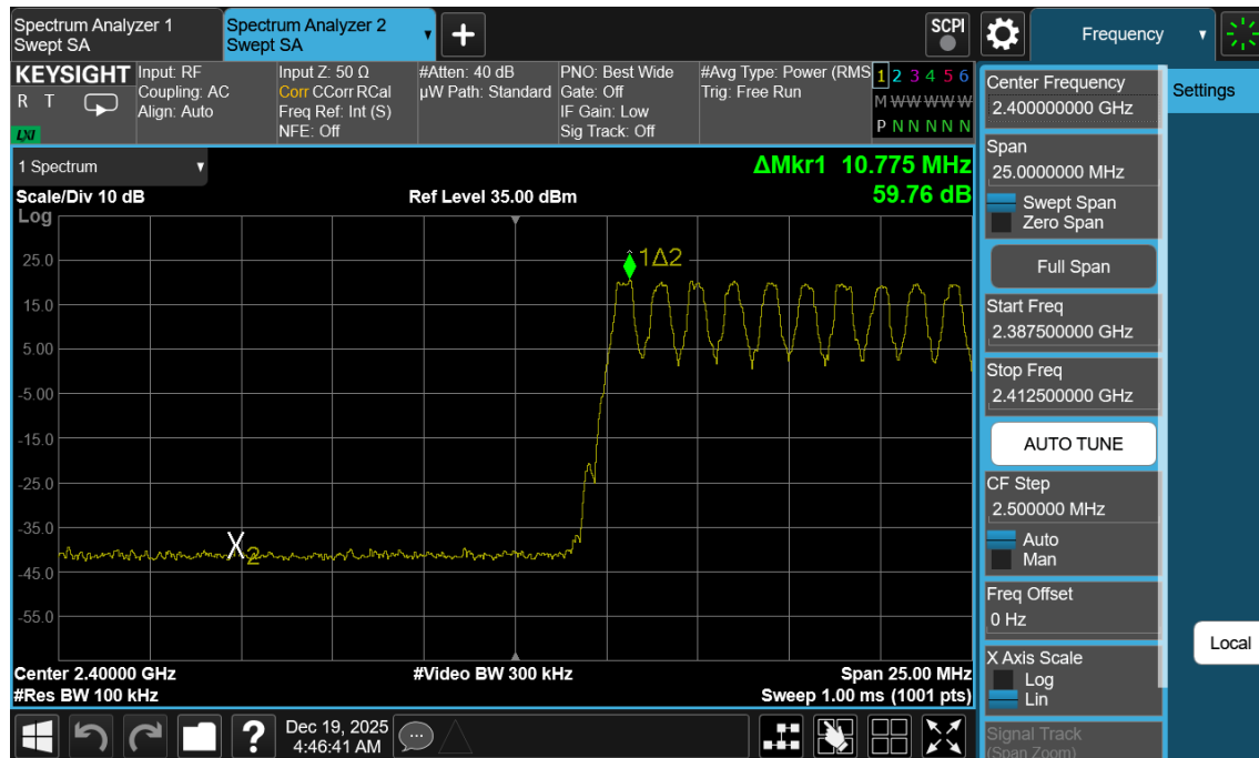
Plot 7-15. Band Edge Plot Antenna 3a (Bluetooth with Hopping Enabled, GFSK, ePA)
