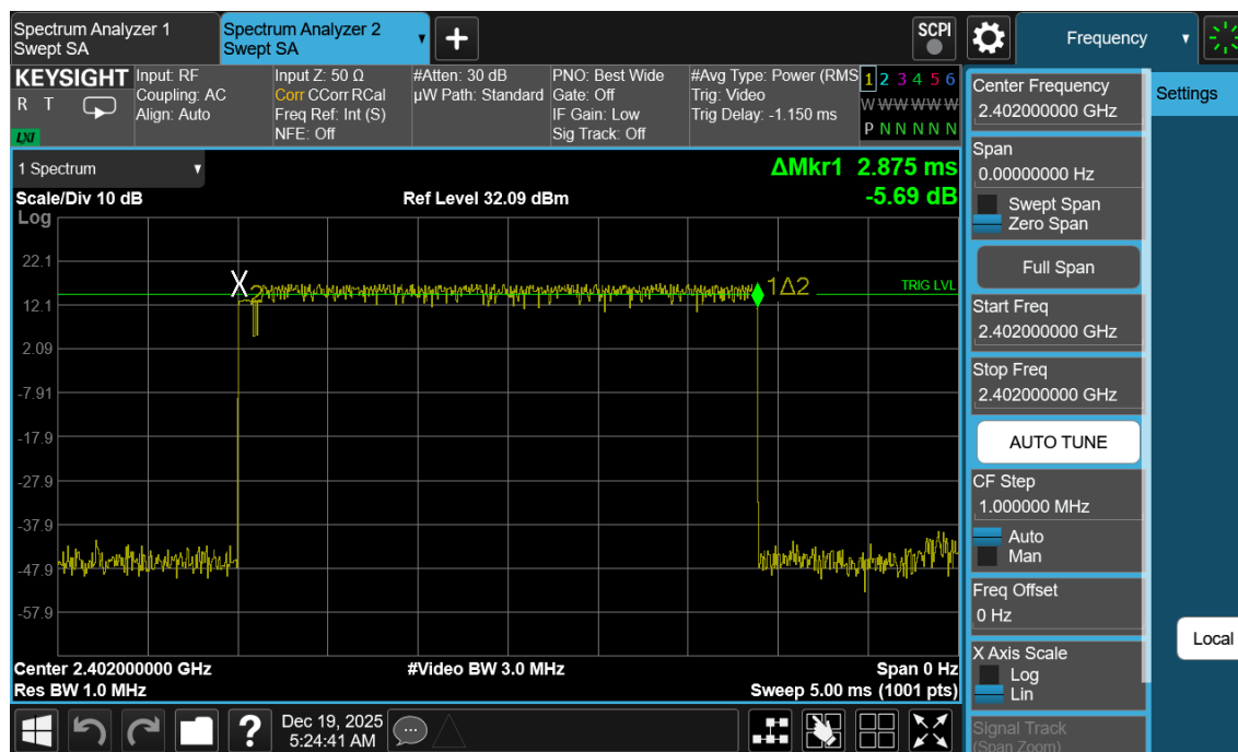
Plot 7-36. Time of Occupancy Plot Antenna 1a (Bluetooth, 8DPSK, ePA)
