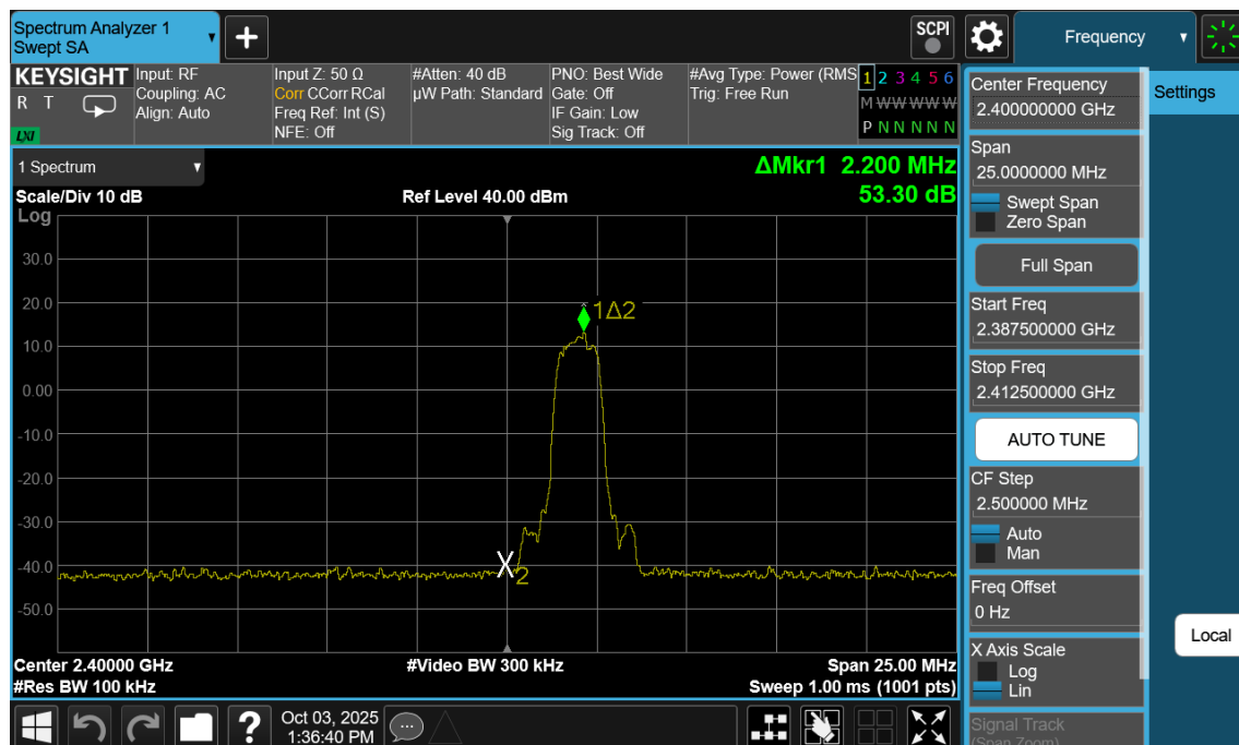
Plot 7-17. Band Edge Plot Antenna 3a (Bluetooth with Hopping Disabled, 8DPSK, ePA – Ch. 0)
