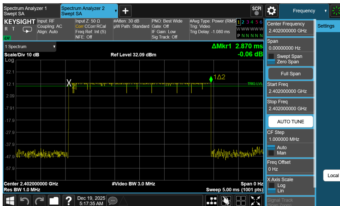
Plot 7-35. Time of Occupancy Plot Antenna 1a (Bluetooth, GFSK, ePA)
