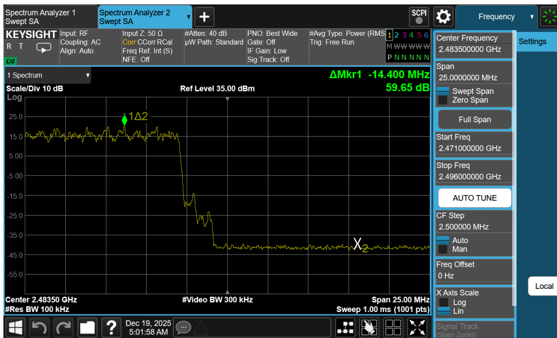
Plot 7-20. Band Edge Plot Antenna 3a (Bluetooth with Hopping Enabled, 8DPSK, ePA)
