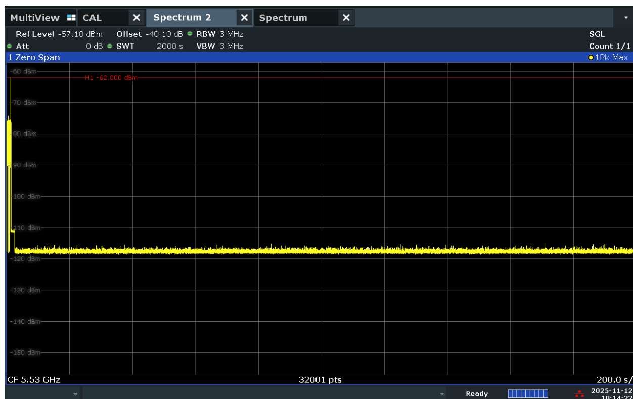
Figure 9-16. 5530MHz - Non-Occupancy Period (30 Minutes) - Mode 1 (80MHz)
