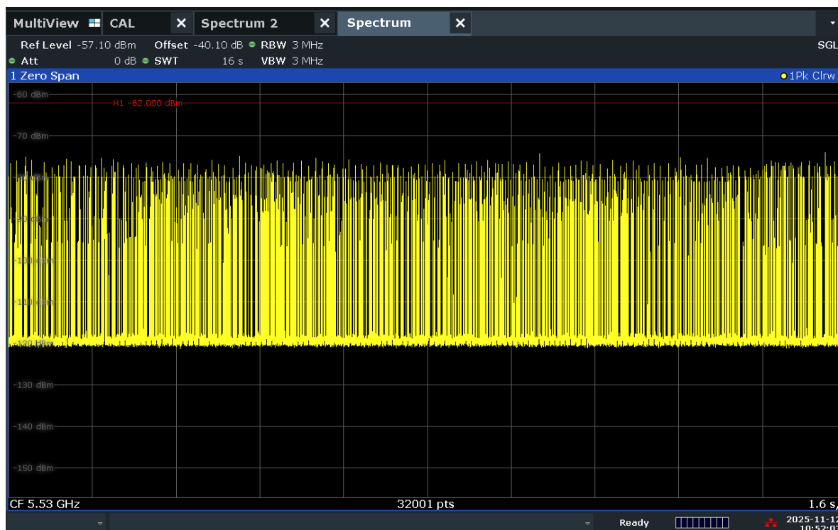
Figure 9-5. 5530MHz - Channel Loading - Mode 2 (80MHz)
