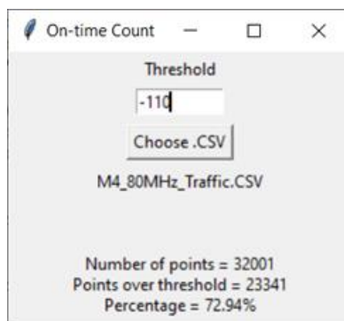
Figure 9-10. 5530MHz - Channel Loading Calculation - Mode 4 (80MHz)
