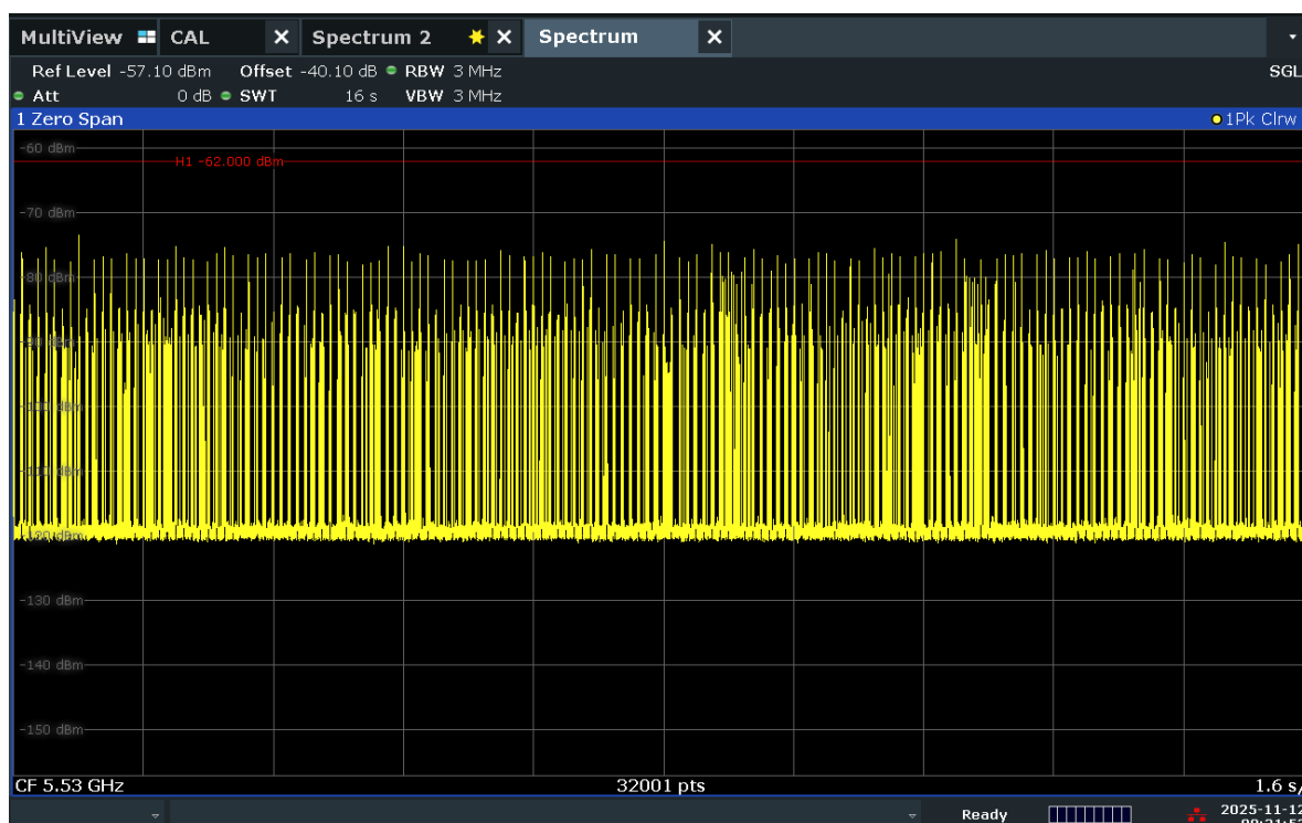
Figure 9-1. 5530MHz - Channel Loading - Mode 1 (80MHz)
