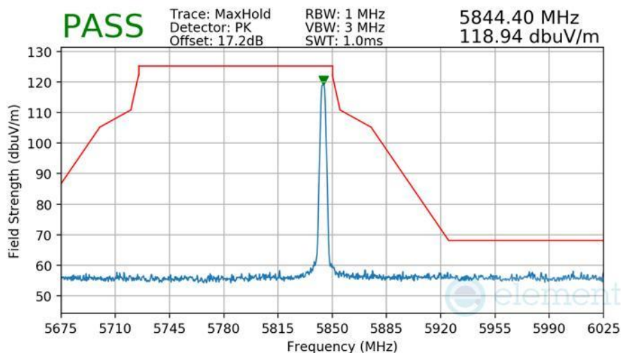
Plot 7-556 Radiated Upper Band Edge Measurement Antenna 5T
