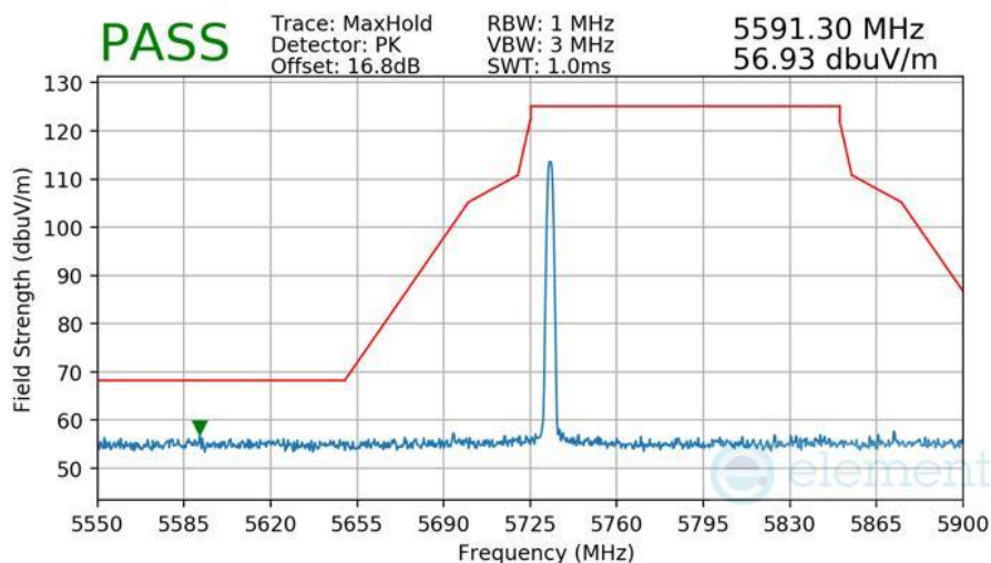
Plot 7-578 Radiated Lower Band Edge Measurement Antenna 3b
