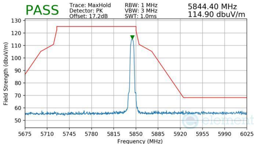
Plot 7-561 Radiated Upper Band Edge Measurement Antenna 5T
