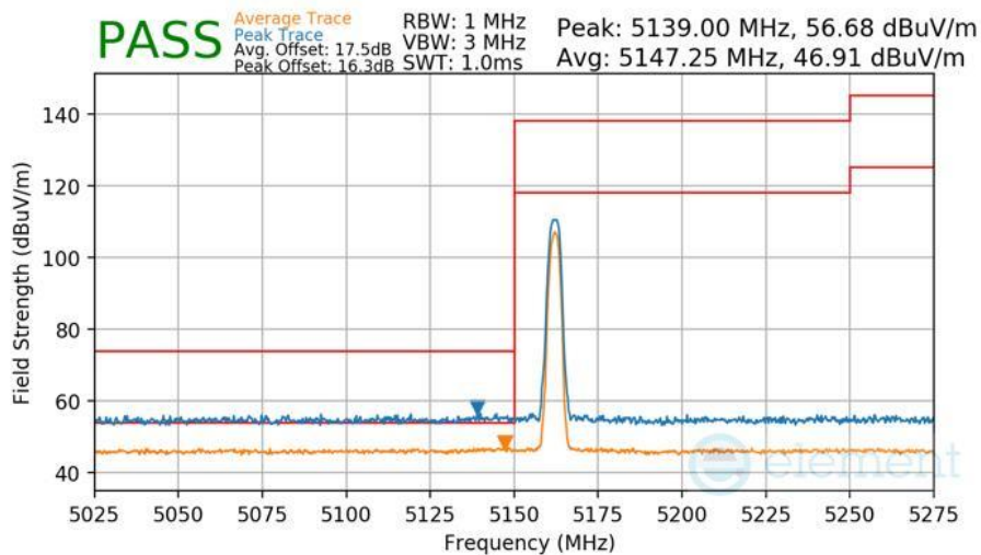
Plot 7-569 Radiated Lower Band Edge Measurement Antenna 3b
