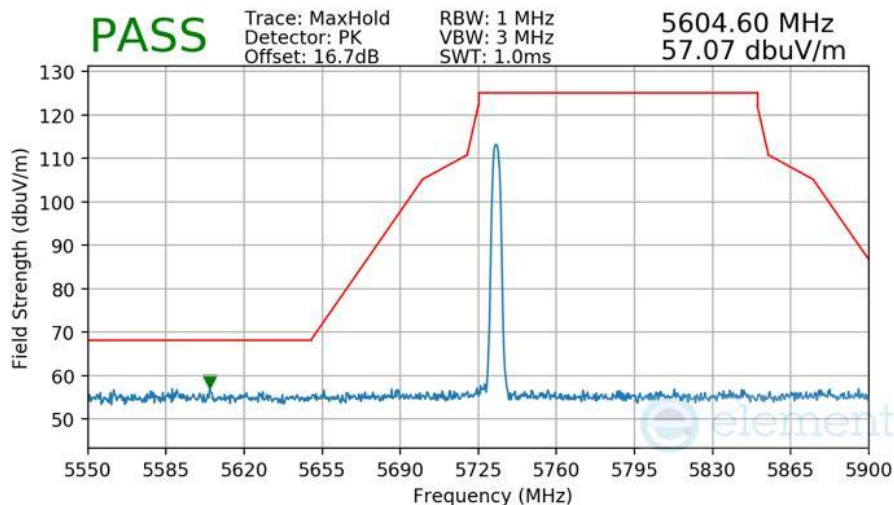
Plot 7-553 Radiated Lower Band Edge Measurement Antenna 5T
