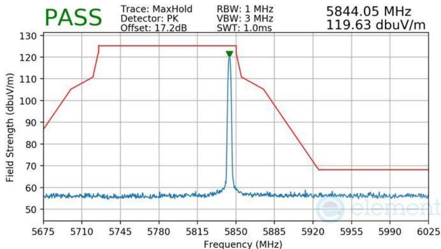
Plot 7-555 Radiated Upper Band Edge Measurement Antenna 5T
