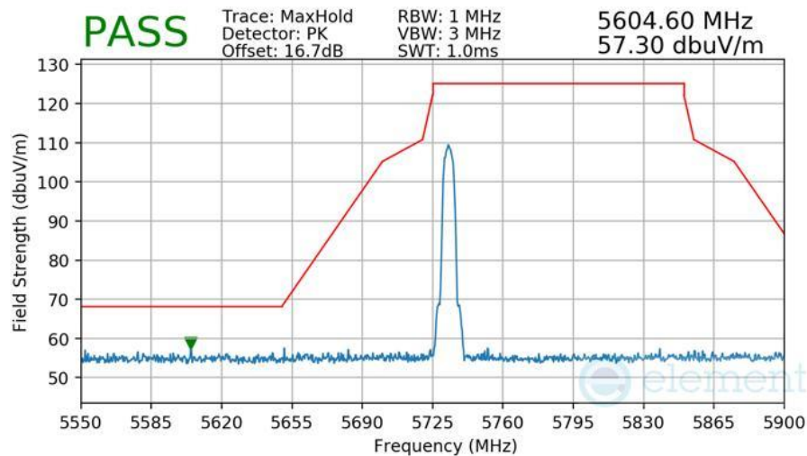
Plot 7-585 Radiated Lower Band Edge Measurement Antenna 3b
