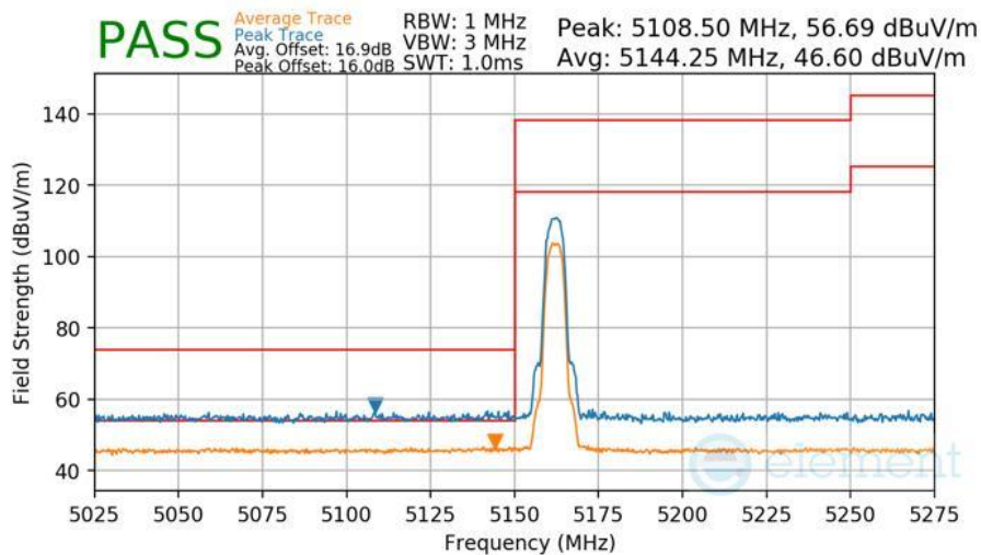
Plot 7-573 Radiated Lower Band Edge Measurement Antenna 3b
