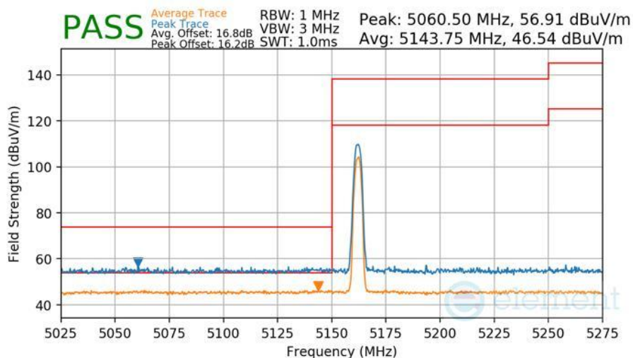
Plot 7-577 Radiated Lower Band Edge Measurement Antenna 3b
