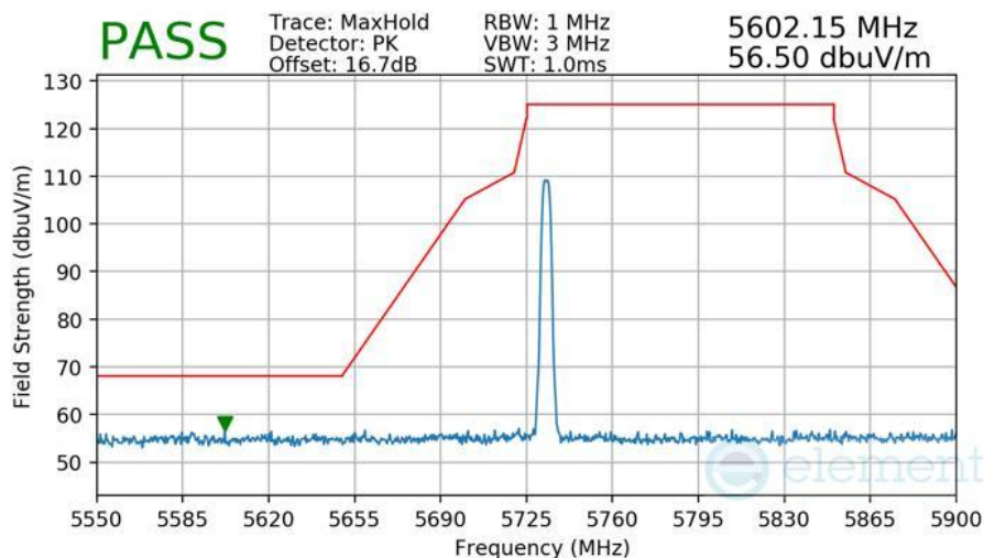
Plot 7-581 Radiated Lower Band Edge Measurement Antenna 3b
