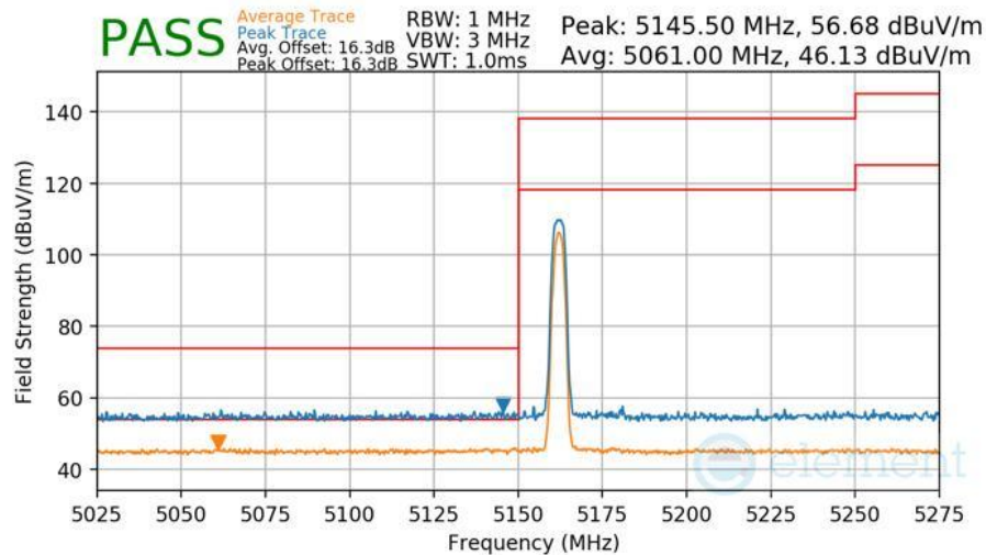
Plot 7-571 Radiated Lower Band Edge Measurement Antenna 3b
