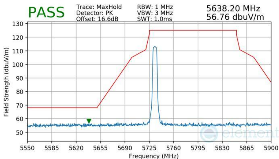
Plot 7-548 Radiated Lower Band Edge Measurement Antenna 5T
