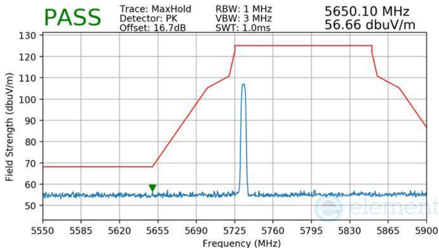
Plot 7-583 Radiated Lower Band Edge Measurement Antenna 3b
