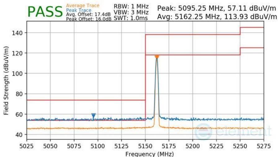
Plot 7-566 Radiated Lower Band Edge Measurement Antenna 3b
