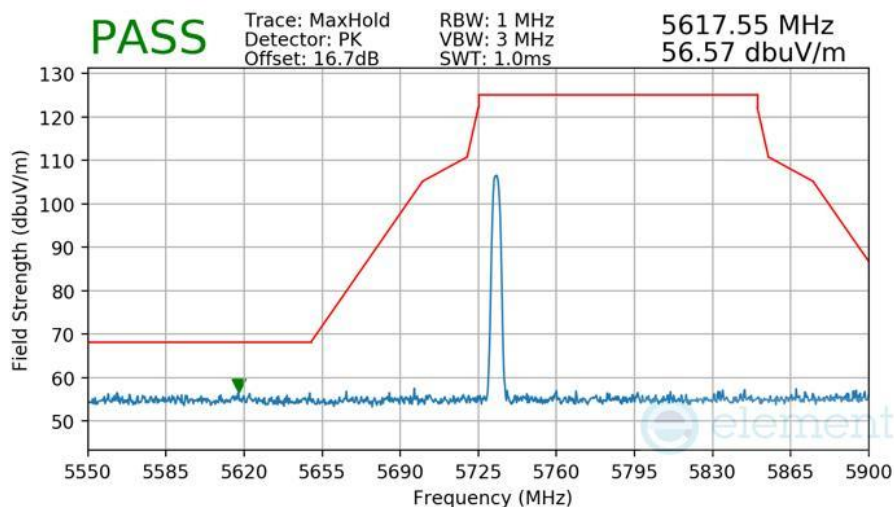
Plot 7-589 Radiated Lower Band Edge Measurement Antenna 3b
