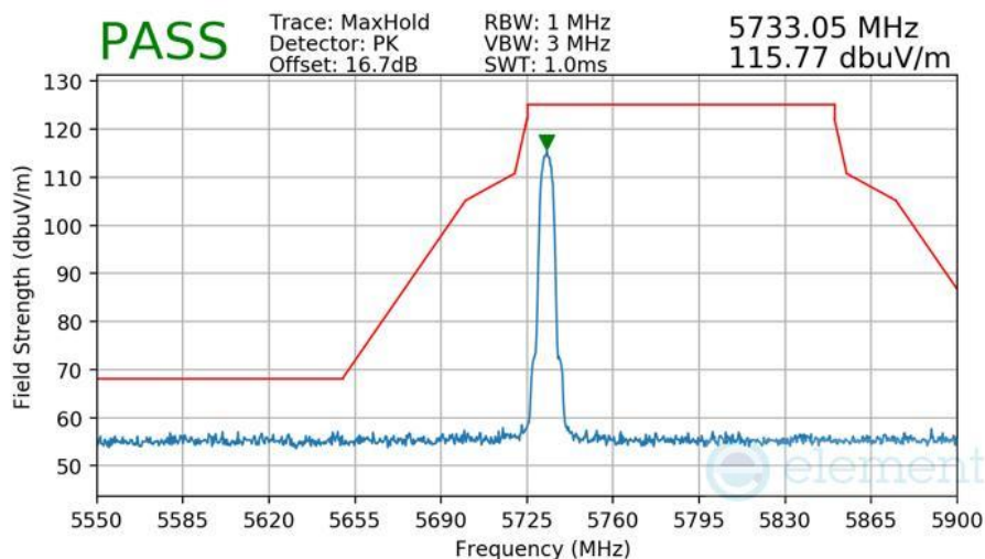
Plot 7-549 Radiated Lower Band Edge Measurement Antenna 5T
