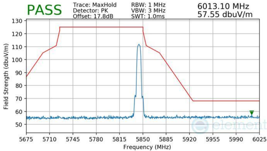
Plot 7-594 Radiated Upper Band Edge Measurement Antenna 3b
