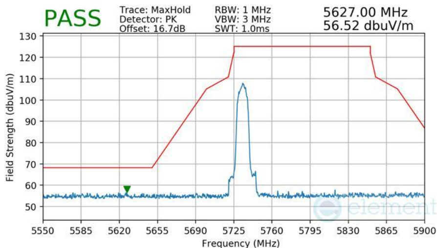
Plot 7-587 Radiated Lower Band Edge Measurement Antenna 3b
