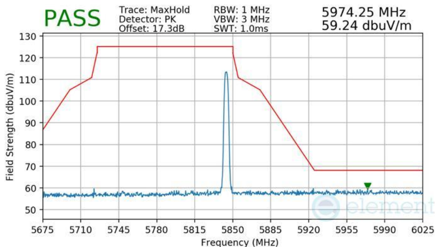
Plot 7-565 Radiated Upper Band Edge Measurement Antenna 5T
