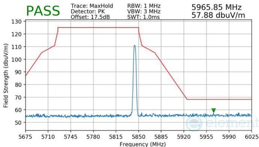
Plot 7-601 Radiated Upper Band Edge Measurement Antenna 3b
