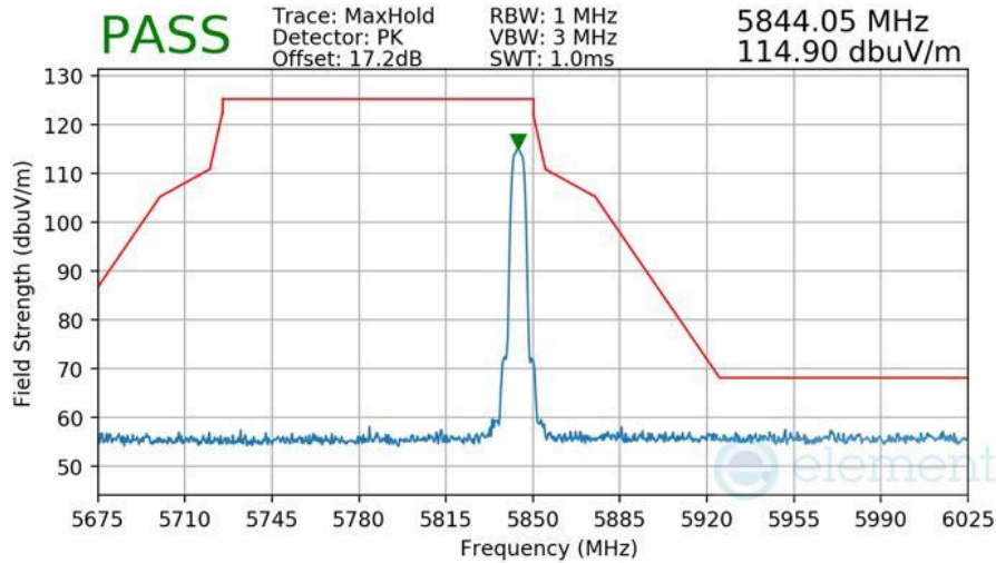
Plot 7-558 Radiated Upper Band Edge Measurement Antenna 5T
