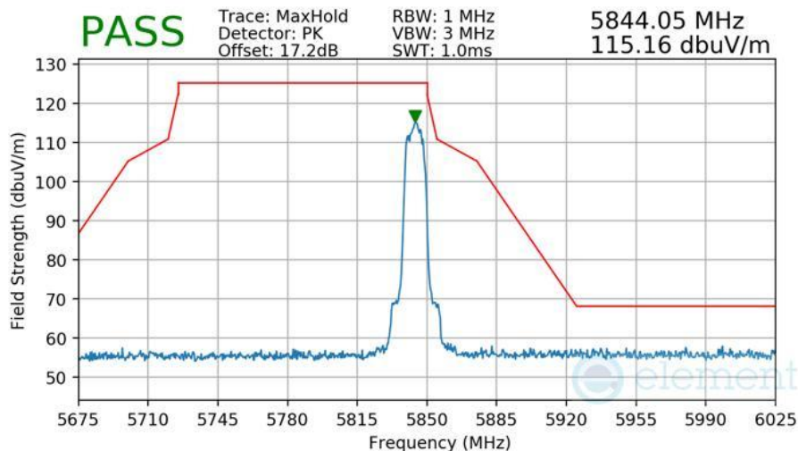
Plot 7-563 Radiated Upper Band Edge Measurement Antenna 5T
