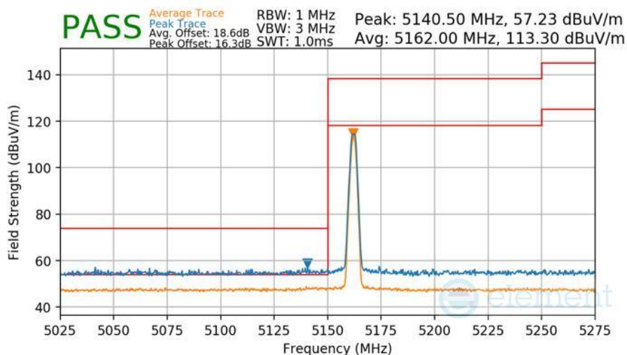
Plot 7-568 Radiated Lower Band Edge Measurement Antenna 3b
