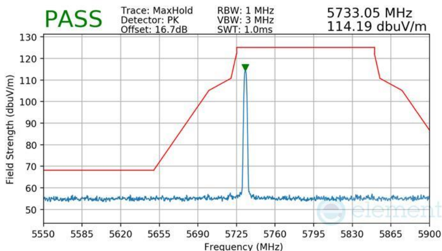
Plot 7-579 Radiated Lower Band Edge Measurement Antenna 3b
