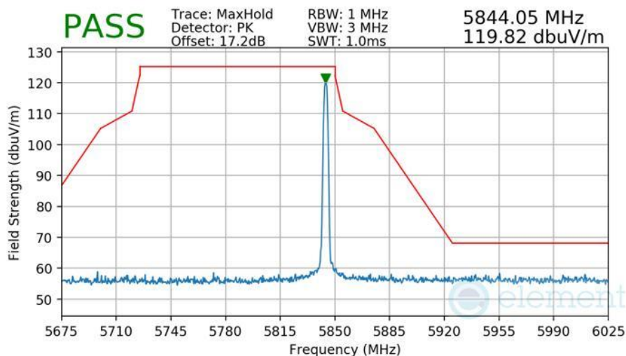
Plot 7-554 Radiated Upper Band Edge Measurement Antenna 5T
