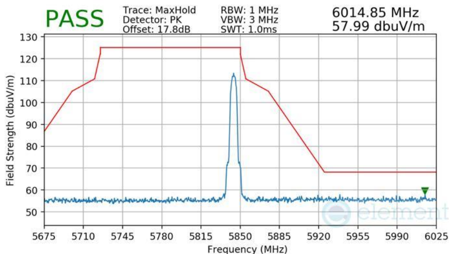
Plot 7-597 Radiated Upper Band Edge Measurement Antenna 3b
