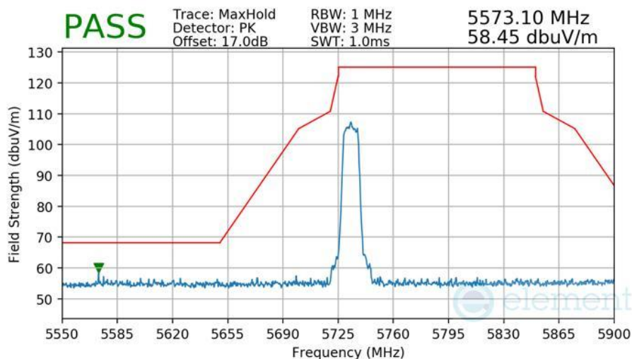
Plot 7-586 Radiated Lower Band Edge Measurement Antenna 3b
