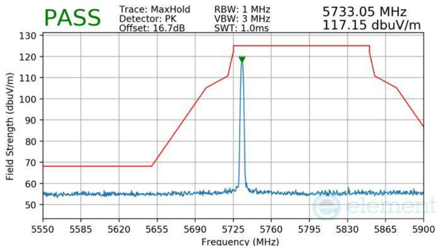
Plot 7-615 Radiated Lower Band Edge Measurement Antenna 1b
