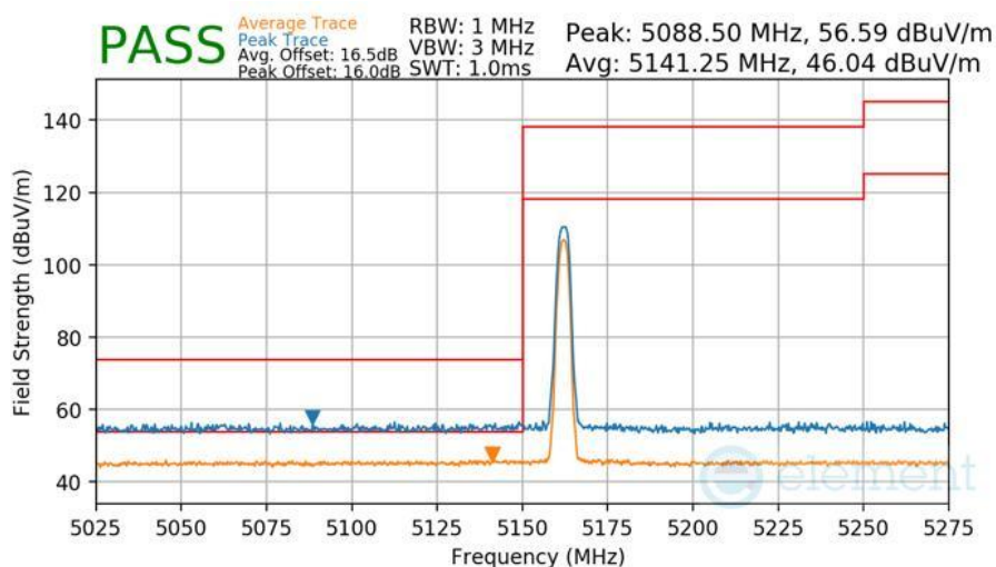
Plot 7-576 Radiated Lower Band Edge Measurement Antenna 3b
