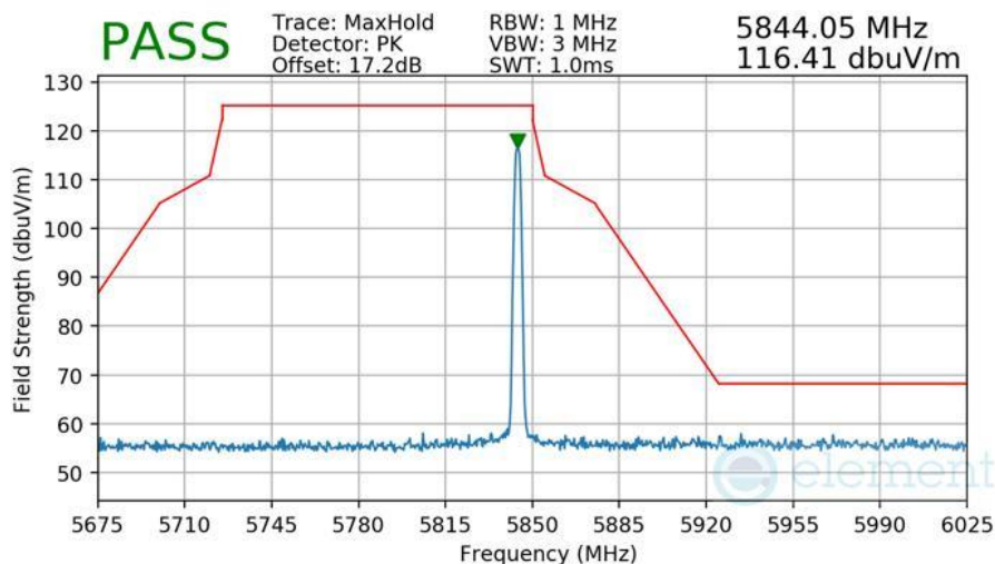
Plot 7-591 Radiated Upper Band Edge Measurement Antenna 3b
