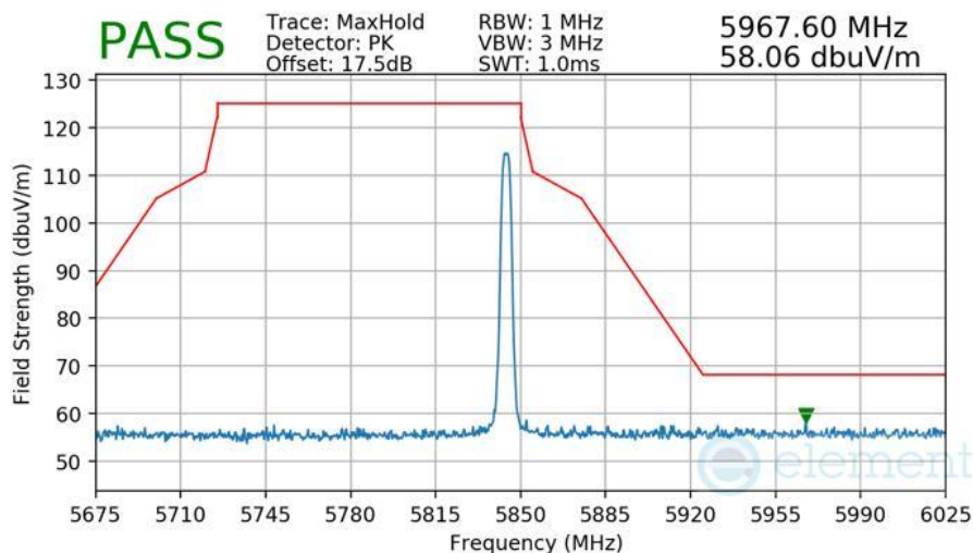
Plot 7-564 Radiated Upper Band Edge Measurement Antenna 5T
