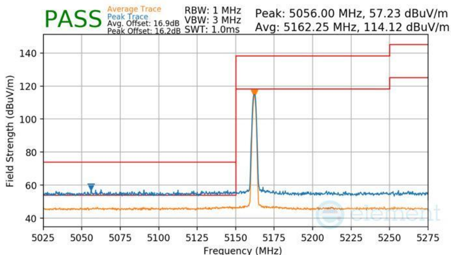
Plot 7-567 Radiated Lower Band Edge Measurement Antenna 3b
