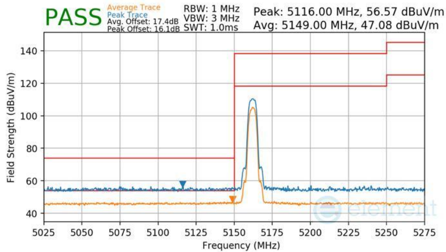
Plot 7-570 Radiated Lower Band Edge Measurement Antenna 3b
