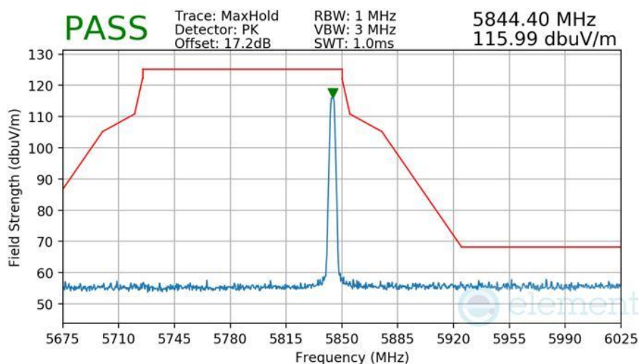
Plot 7-592 Radiated Upper Band Edge Measurement Antenna 3b
