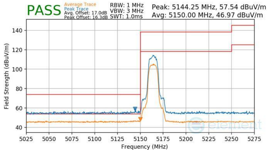
Plot 7-647 Radiated Lower Band Edge Measurement TxBF Primary
