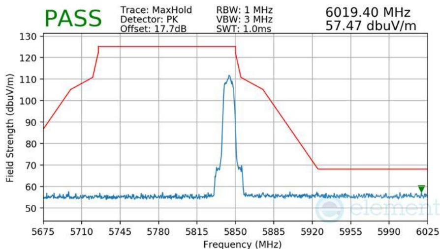
Plot 7-599 Radiated Upper Band Edge Measurement Antenna 3b
