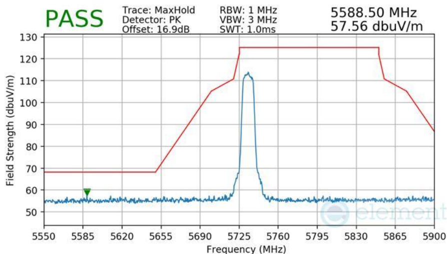
Plot 7-550 Radiated Lower Band Edge Measurement Antenna 5T
