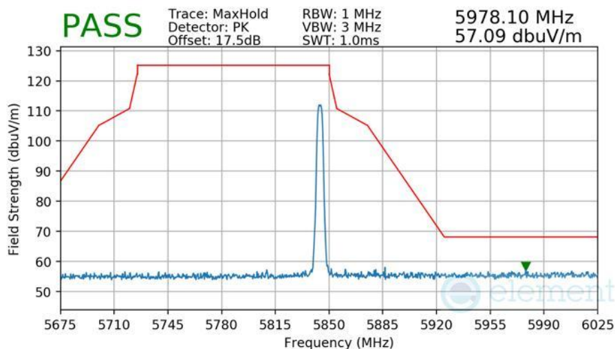
Plot 7-593 Radiated Upper Band Edge Measurement Antenna 3b
