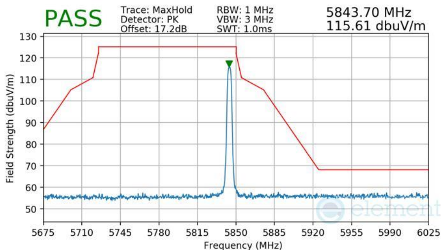
Plot 7-557 Radiated Upper Band Edge Measurement Antenna 5T
