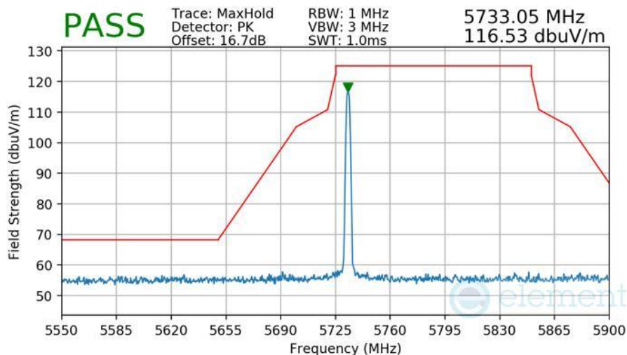
Plot 7-614 Radiated Lower Band Edge Measurement Antenna 1b
