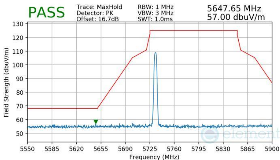
Plot 7-588 Radiated Lower Band Edge Measurement Antenna 3b
