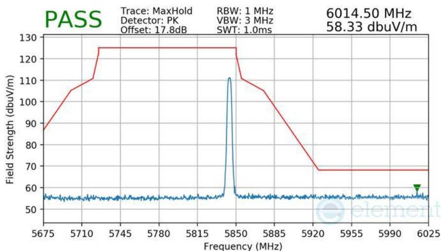
Plot 7-600 Radiated Upper Band Edge Measurement Antenna 3b
