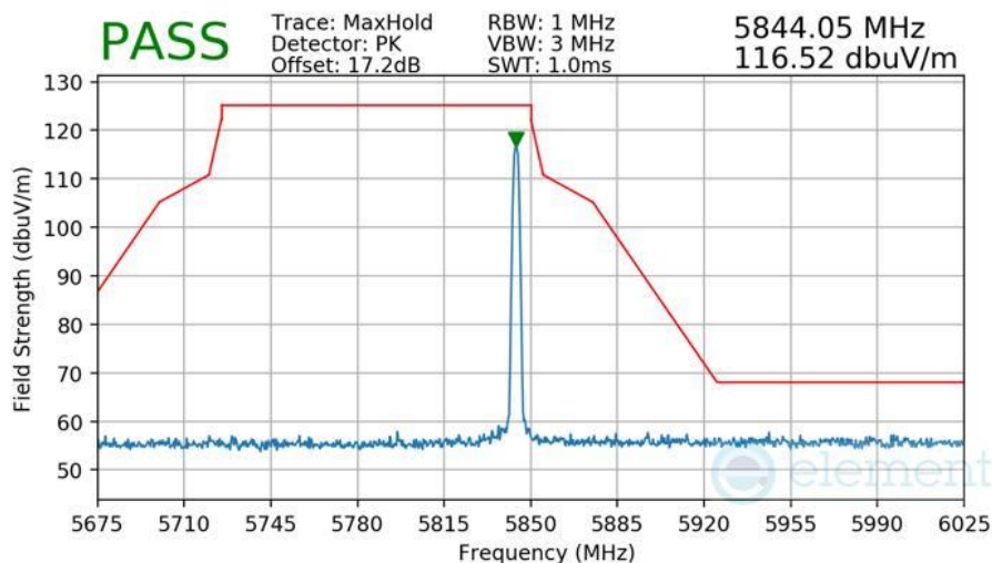
Plot 7-590 Radiated Upper Band Edge Measurement Antenna 3b
