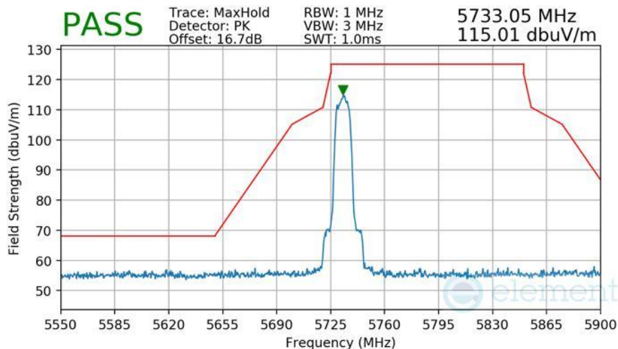
Plot 7-551 Radiated Lower Band Edge Measurement Antenna 5T
