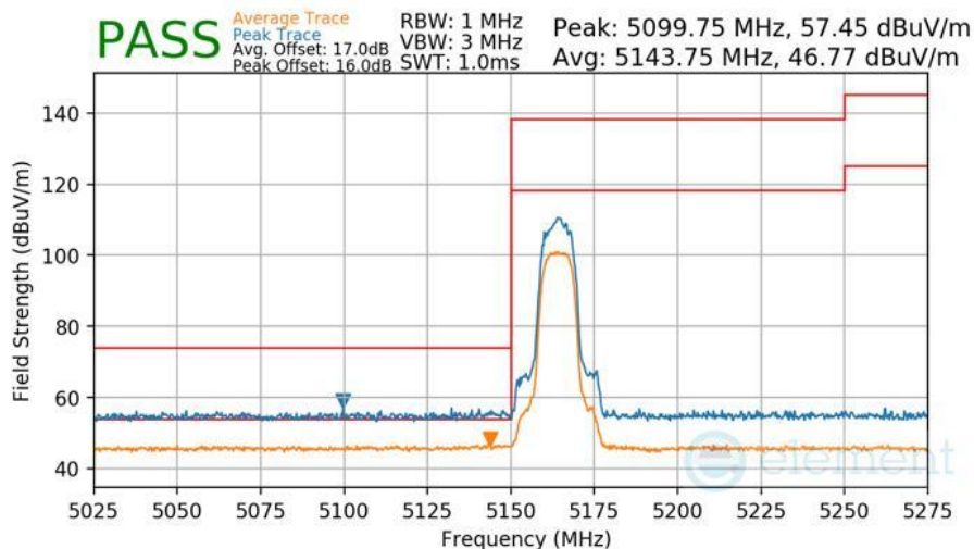
Plot 7-575 Radiated Lower Band Edge Measurement Antenna 3b
