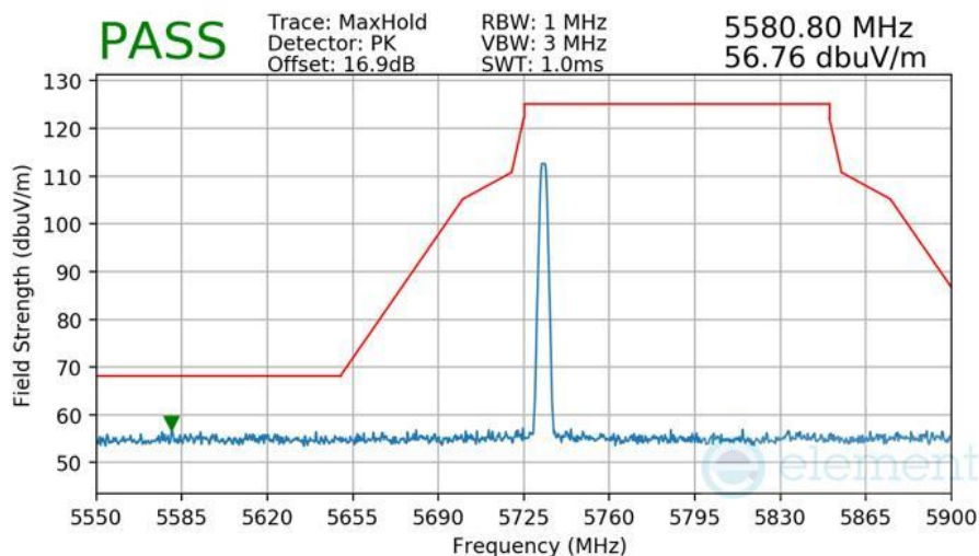
Plot 7-580 Radiated Lower Band Edge Measurement Antenna 3b
