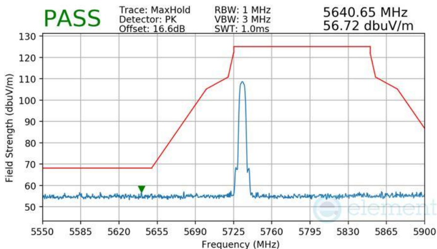
Plot 7-582 Radiated Lower Band Edge Measurement Antenna 3b
