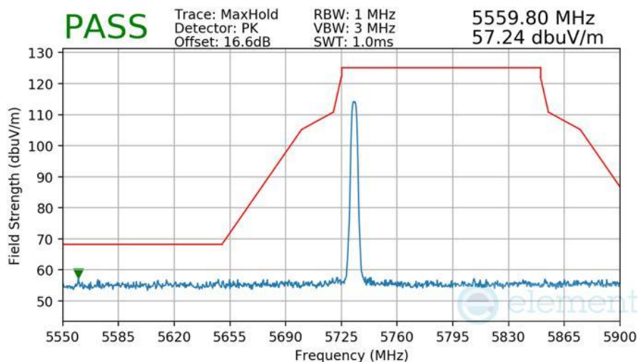
Plot 7-552 Radiated Lower Band Edge Measurement Antenna 5T
