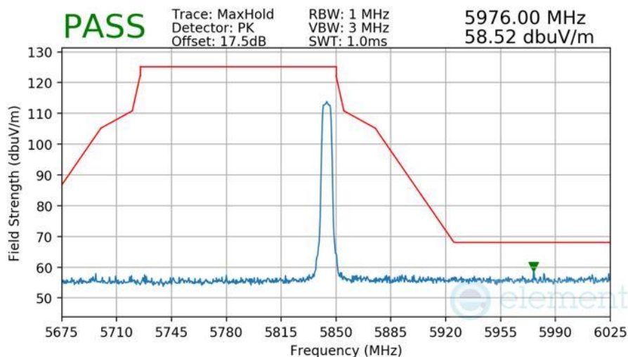
Plot 7-560 Radiated Upper Band Edge Measurement Antenna 5T
