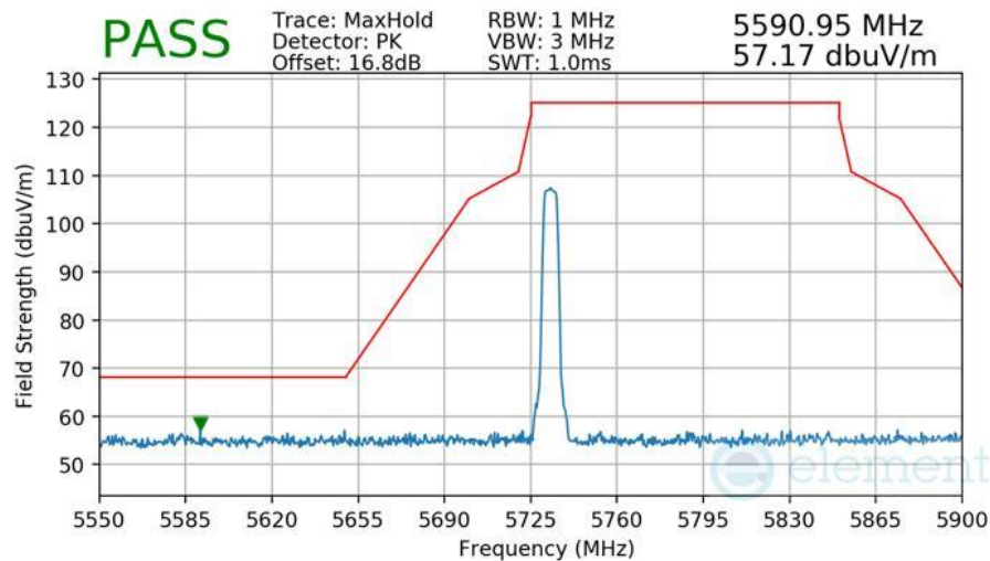
Plot 7-584 Radiated Lower Band Edge Measurement Antenna 3b
