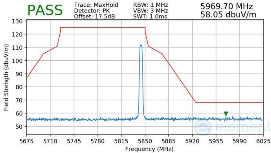
Plot 7-595 Radiated Upper Band Edge Measurement Antenna 3b
