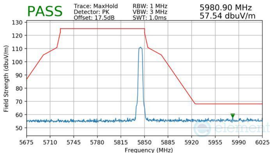
Plot 7-596 Radiated Upper Band Edge Measurement Antenna 3b
