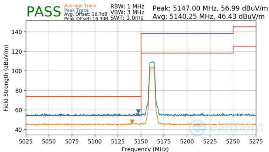
Plot 7-572 Radiated Lower Band Edge Measurement Antenna 3b
