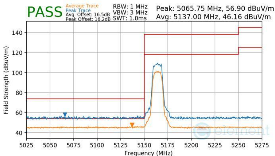
Plot 7-574 Radiated Lower Band Edge Measurement Antenna 3b
