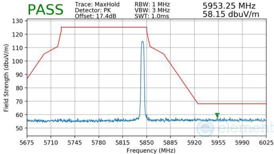
Plot 7-559 Radiated Upper Band Edge Measurement Antenna 5T
