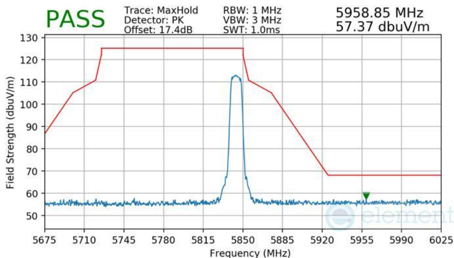
Plot 7-562 Radiated Upper Band Edge Measurement Antenna 5T
