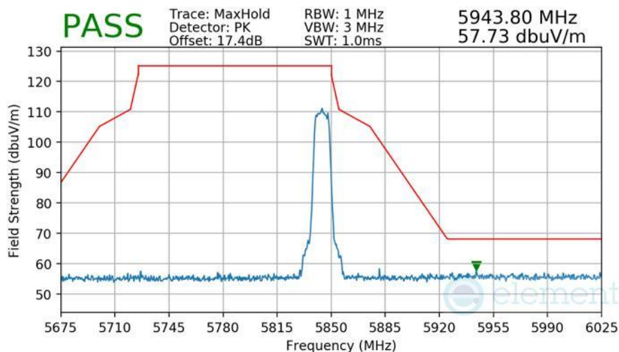
Plot 7-598 Radiated Upper Band Edge Measurement Antenna 3b
