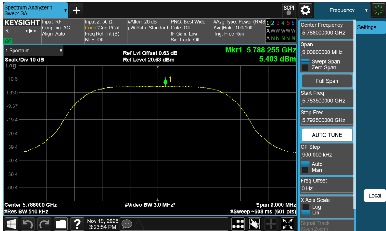
Plot 7-454. PSD TxBF Diversity Antenna 5T (NB UNII XHDRPM6, ePA – 5788MHz)
