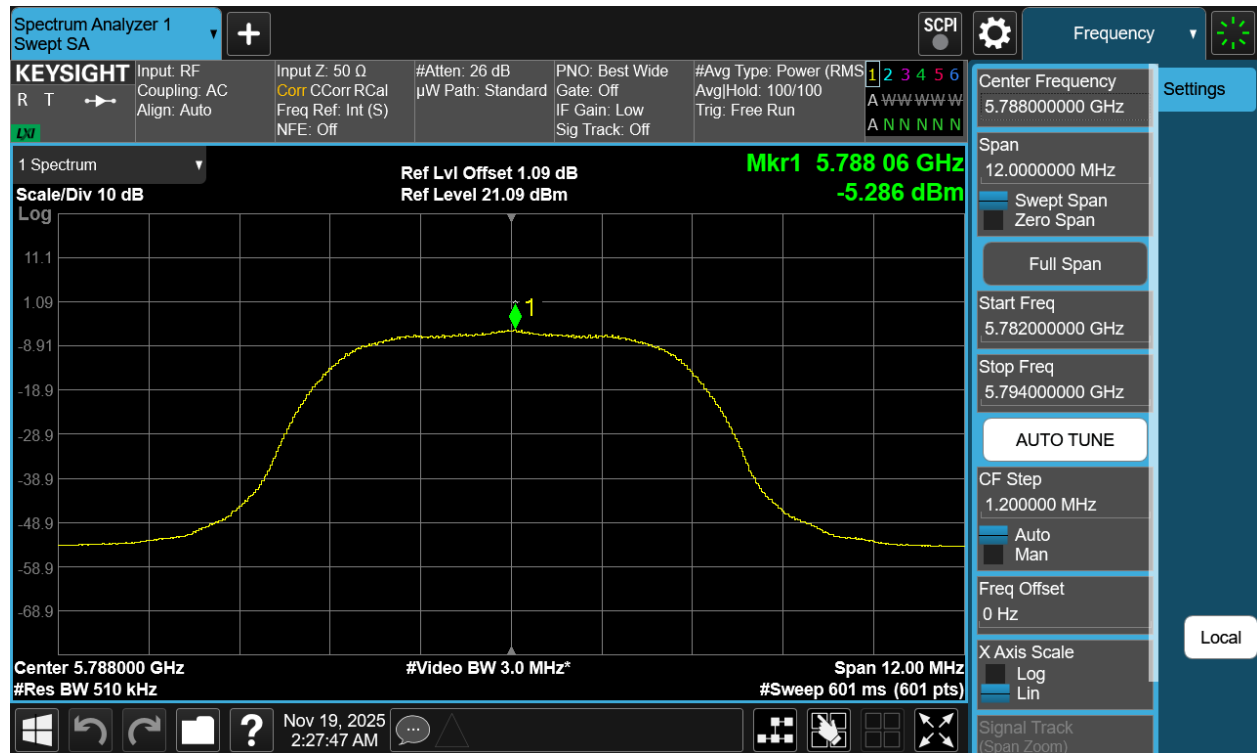
Plot 7-448. PSD Tx BF Diversity Antenna 5T (NB UNII HDR8, iPA - 5788MHz)
