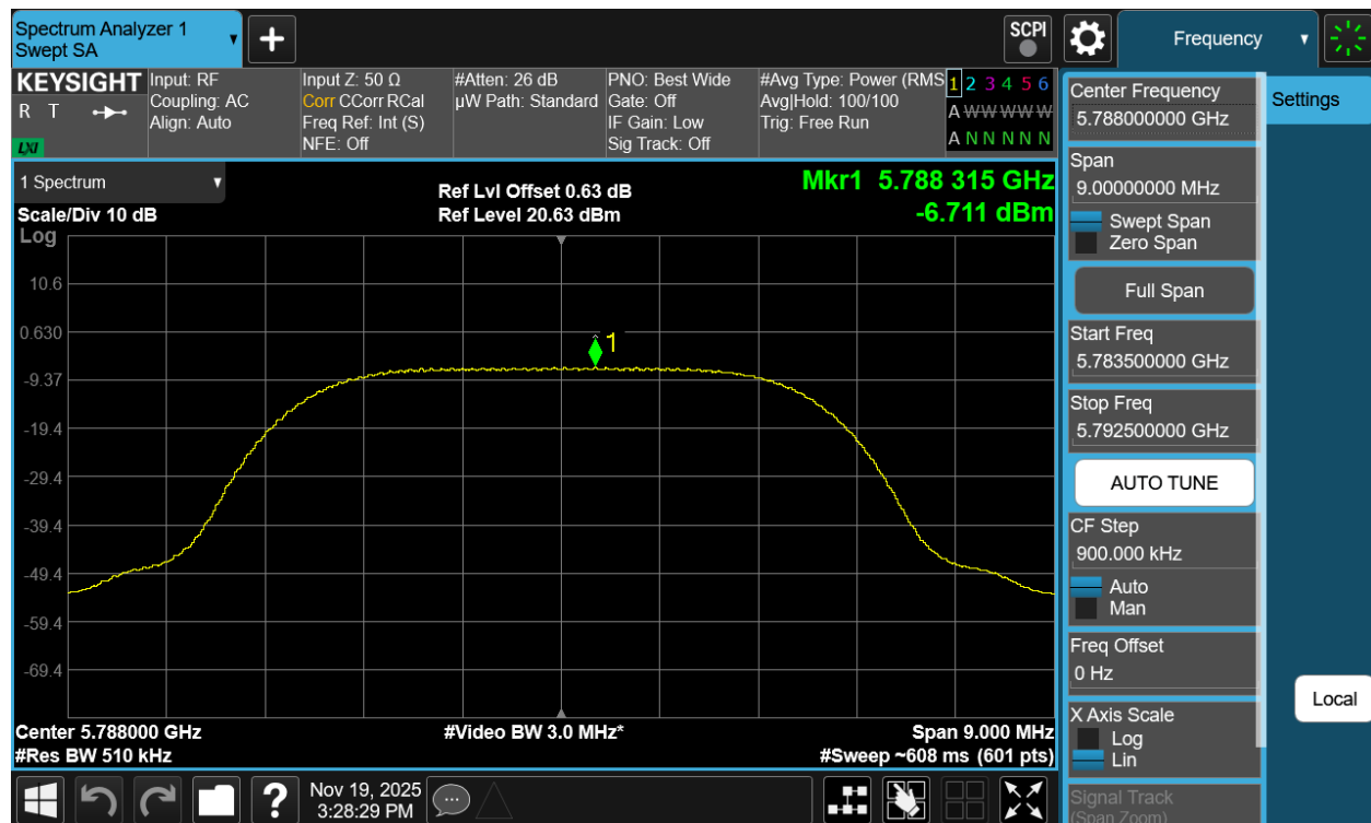
Plot 7-456. PSD TxBF Diversity Antenna 5T (NB UNII XHDRPM6, iPA - 5788MHz)
