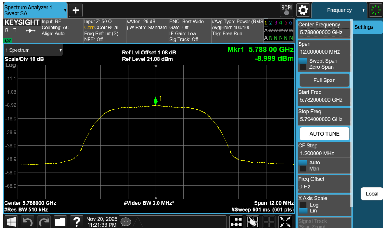
Plot 7-449. PSD Tx BF Diversity Antenna 1b (NB UNII HDR8, iPA - 5788MHz)
