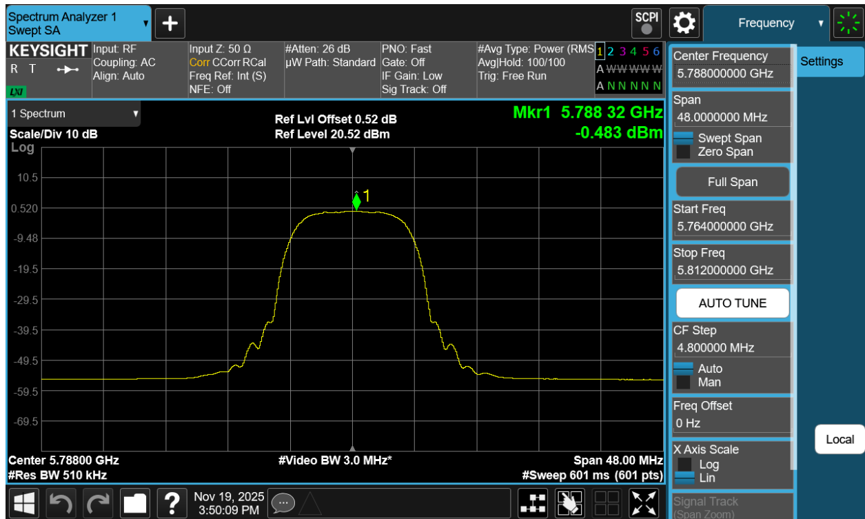
Plot 7-466. PSD Tx BF Diversity Antenna 5T (NB UNII HDRPL32, ePA – 5788MHz)
