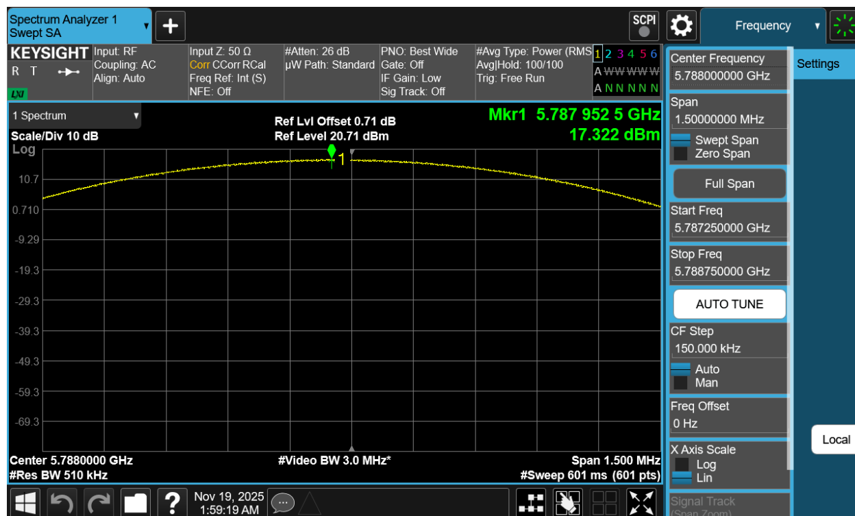
Plot 7-434. PSD Tx BF Diversity Antenna 5T (NB UNII LE1M, ePA – 5788MHz)
