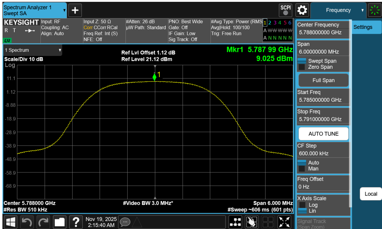
Plot 7-442. PSD Tx BF Diversity Antenna 5T (NB UNII HDR4, ePA – 5788MHz)
