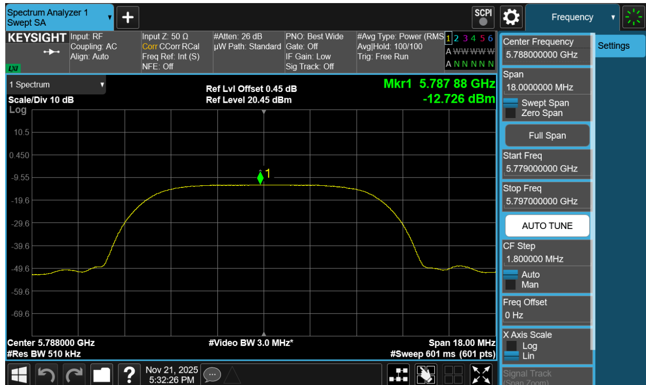
Plot 7-465. PSD TxBF Diversity Antenna 1b (NB UNII HDRPL12, iPA - 5788MHz)
