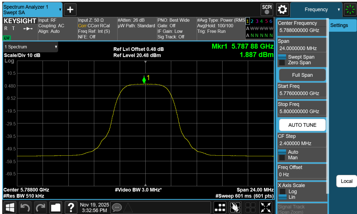
Plot 7-458. PSD TxBF Diversity Antenna 5T (NB UNII HDRPM16, ePA – 5788MHz)
