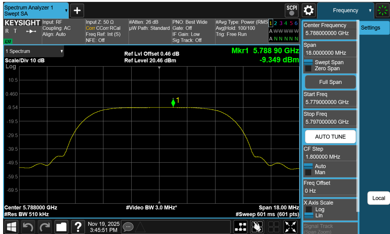
Plot 7-464. PSD TxBF Diversity Antenna 5T (NB UNII HDRPL12, iPA - 5788MHz)
