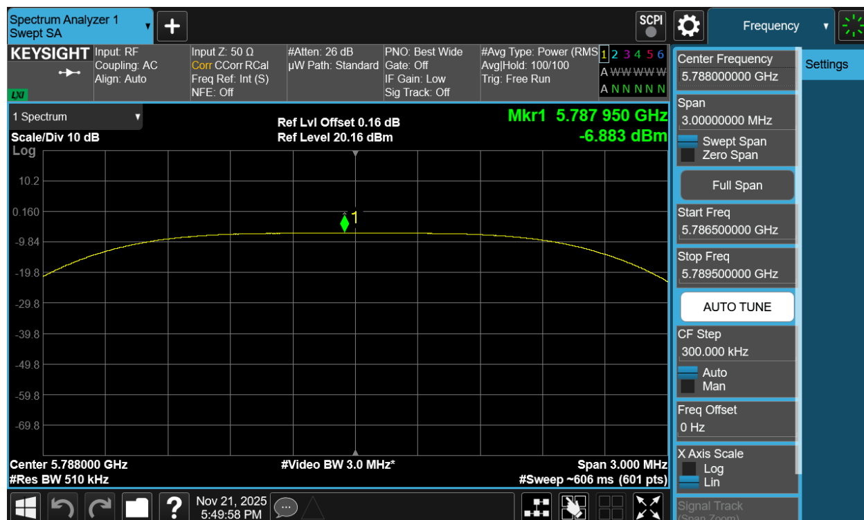
Plot 7-473. PSD Tx BF Diversity Antenna 1b (NB UNII HDT2, iPA - 5788MHz)
