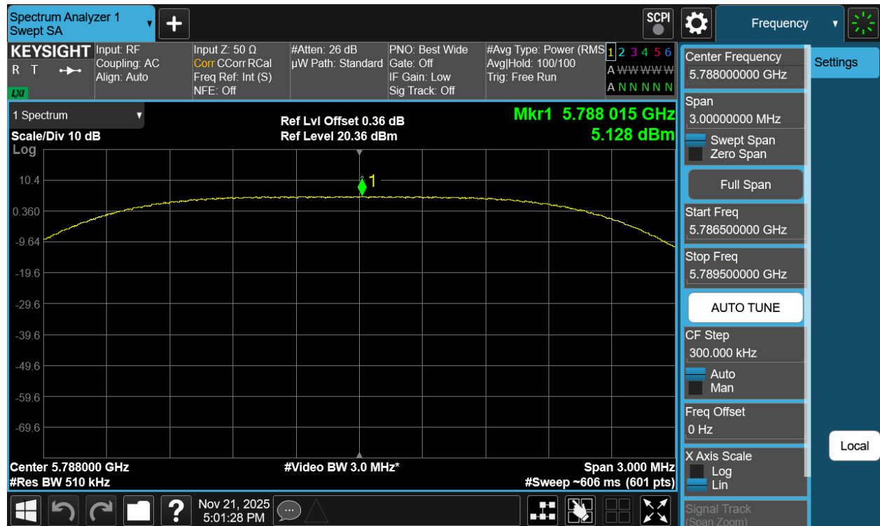
Plot 7-451. PSD Tx BF Diversity Antenna 1b (NB UNII HDRPS2, ePA – 5788MHz)
