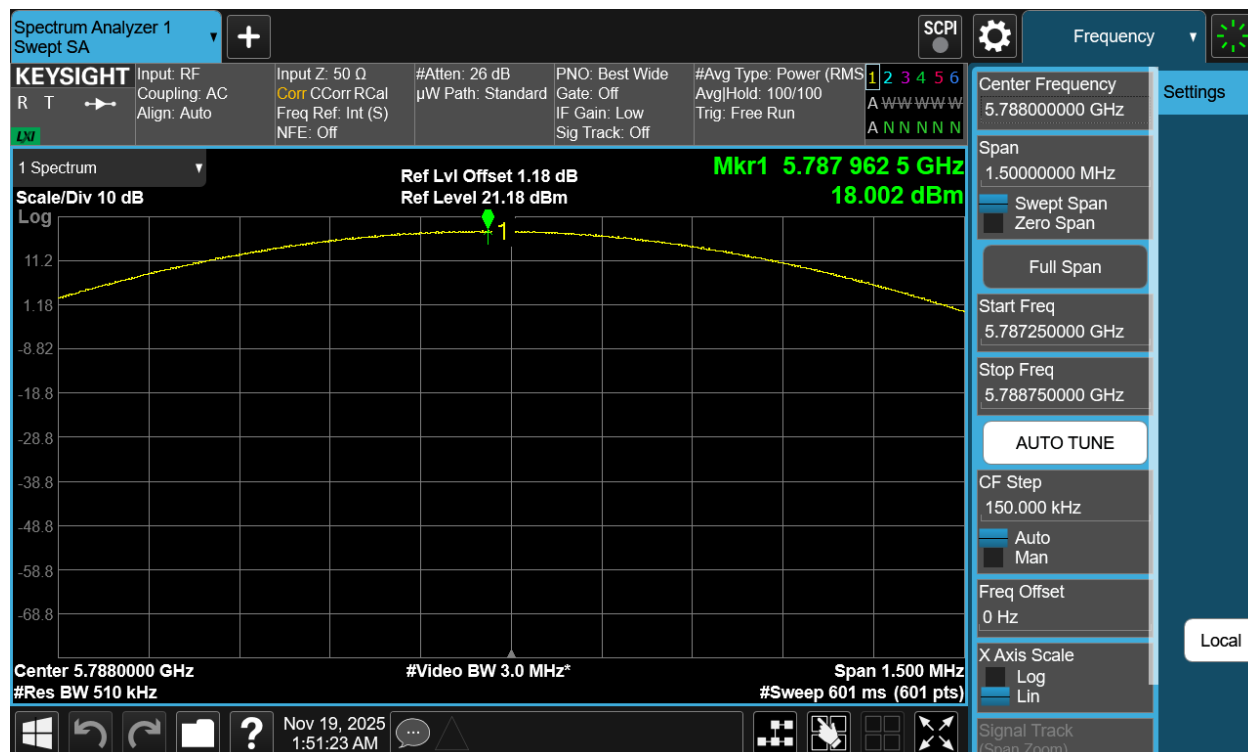
Plot 7-430. PSD Tx BF Diversity Antenna 5T (NB UNII BDR, ePA – 5788MHz)
