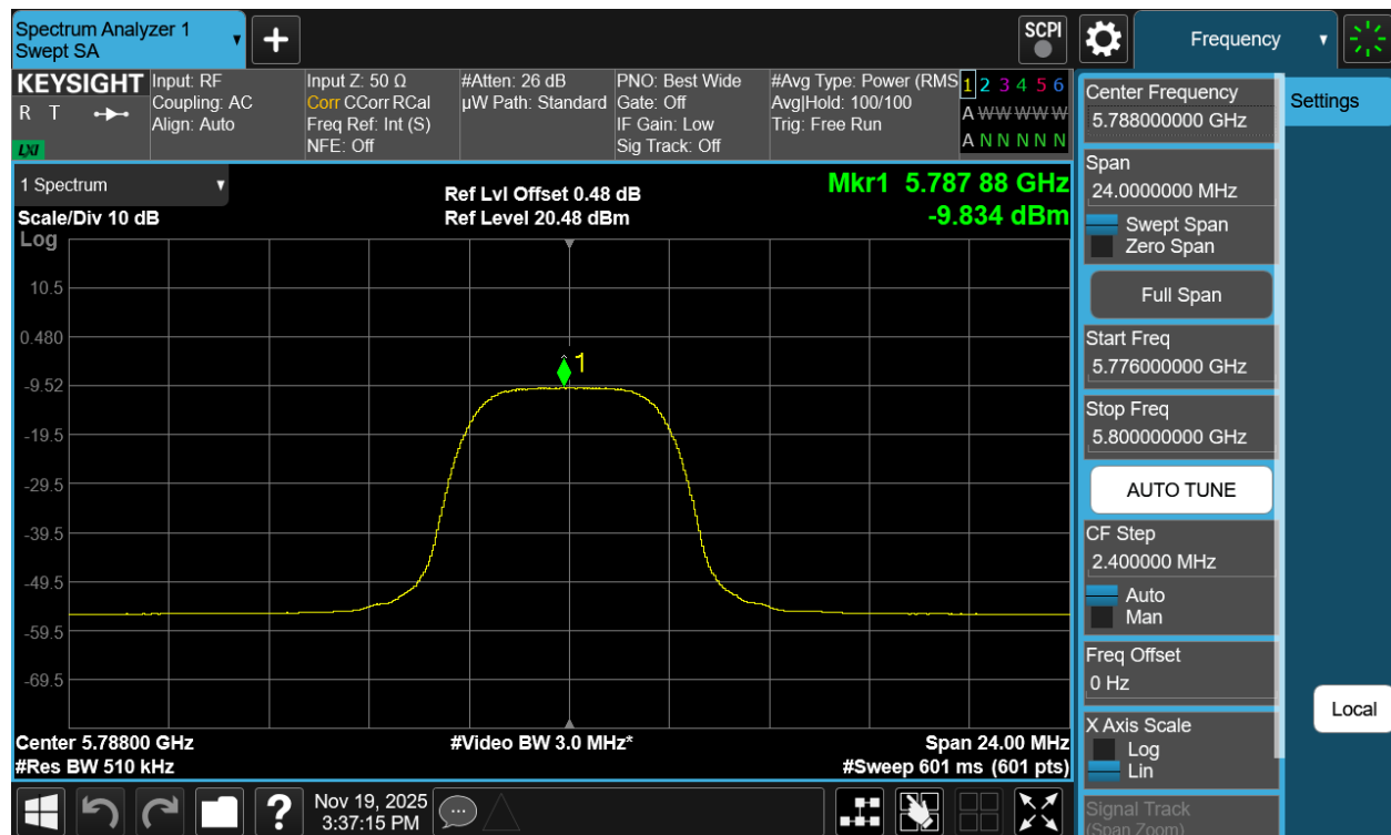
Plot 7-460. PSD TxBF Diversity Antenna 5T (NB UNII HDRPM16, iPA – 5788MHz)
