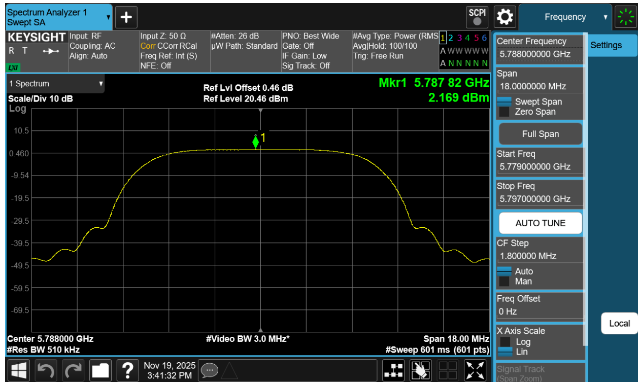
Plot 7-462. PSD TxBF Diversity Antenna 5T (NB UNII HDRPL12, ePA – 5788MHz)
