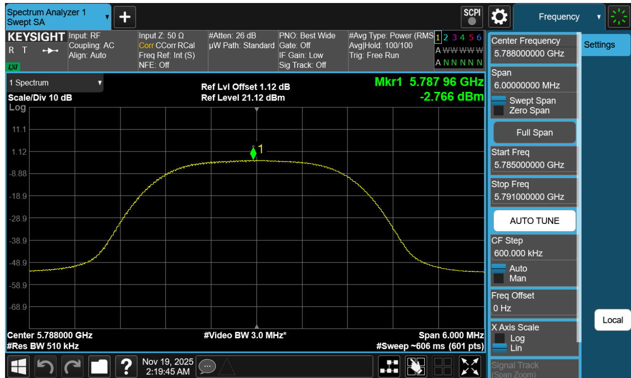
Plot 7-444. PSD TxBF Diversity Antenna 5T (NB UNII HDR4, iPA – 5788MHz)
