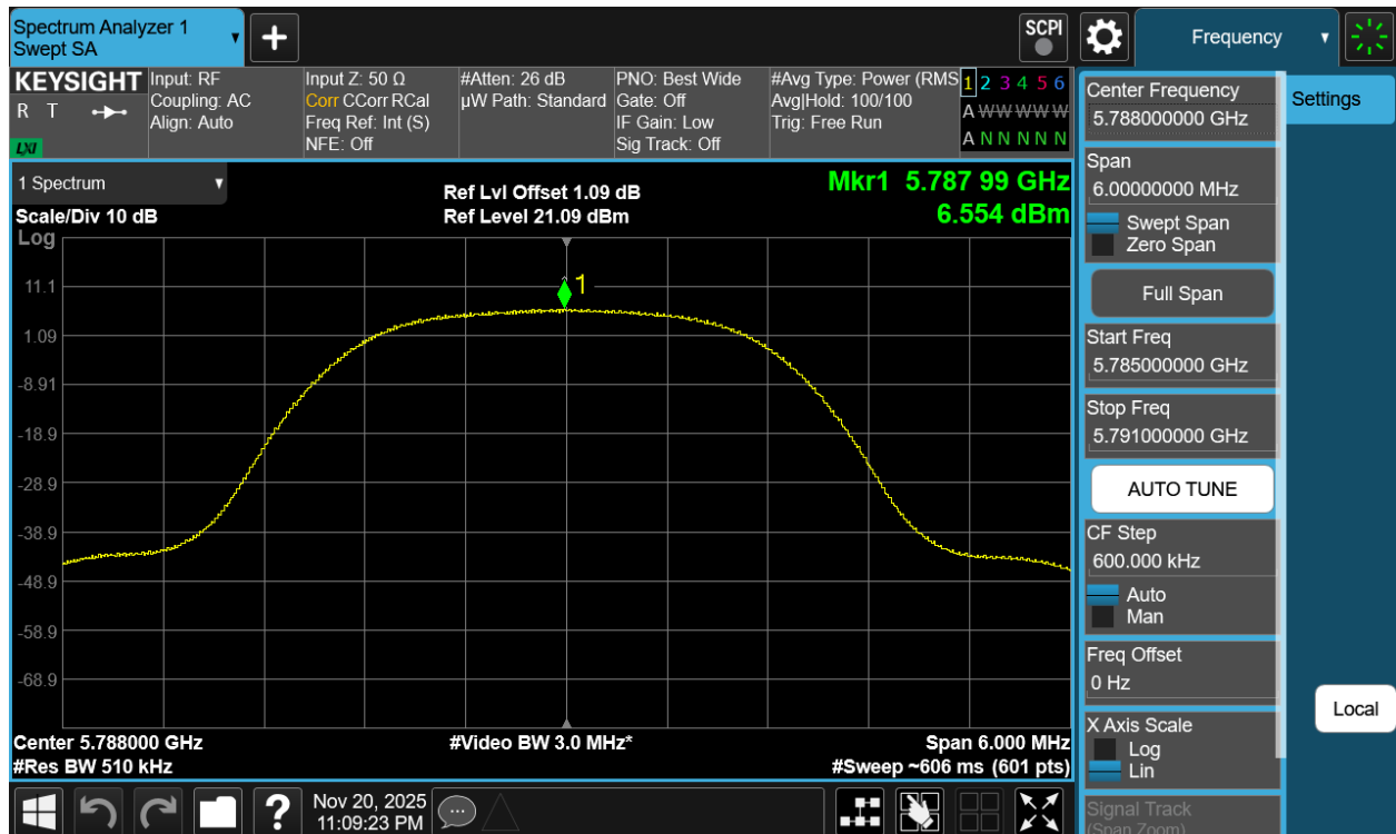
Plot 7-443. PSD Tx BF Diversity Antenna 1b (NB UNII HDR4, ePA – 5788MHz)
