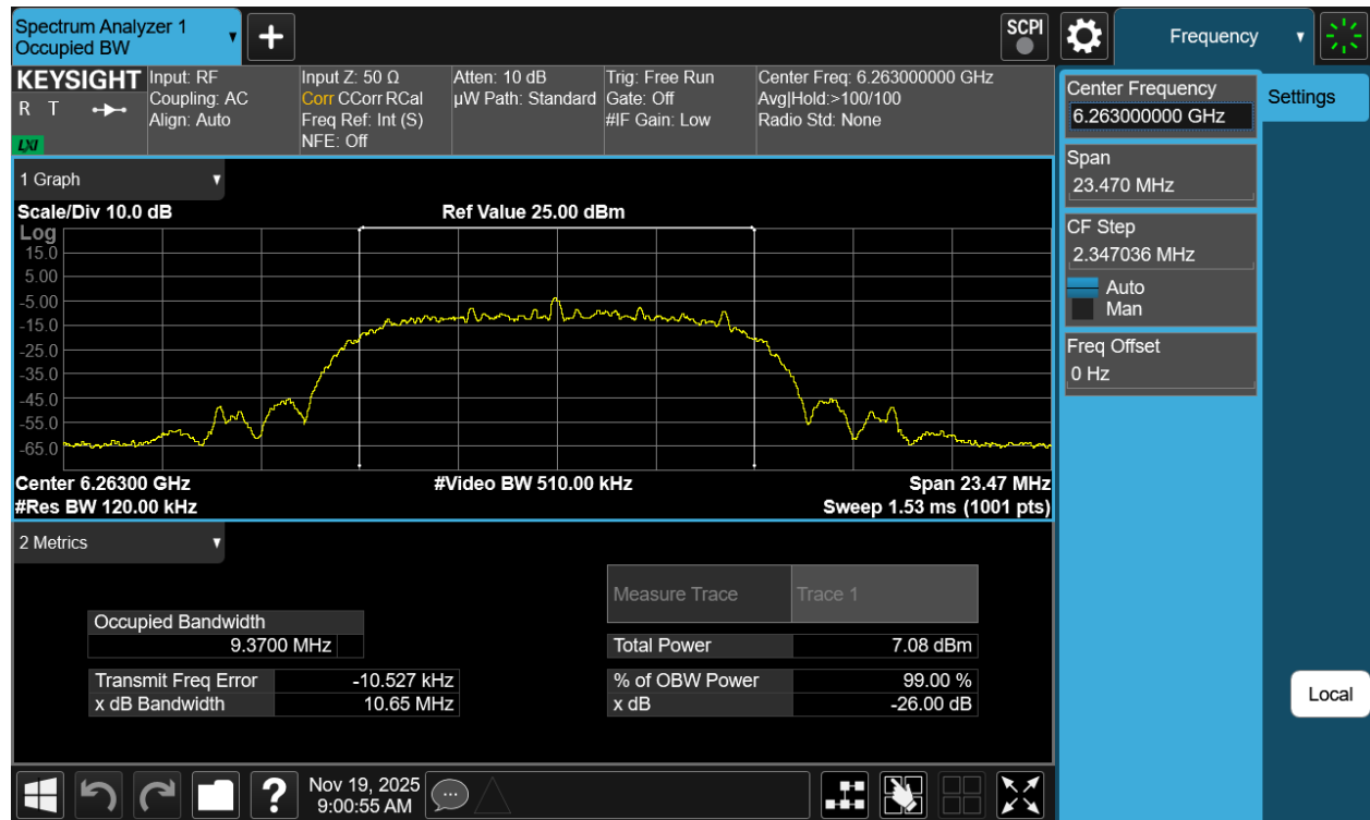
Plot 7-9. 26dB BW & 99% OBW Antenna 5T (NB UNII HDRPL12, ePA- 6263MHz)
