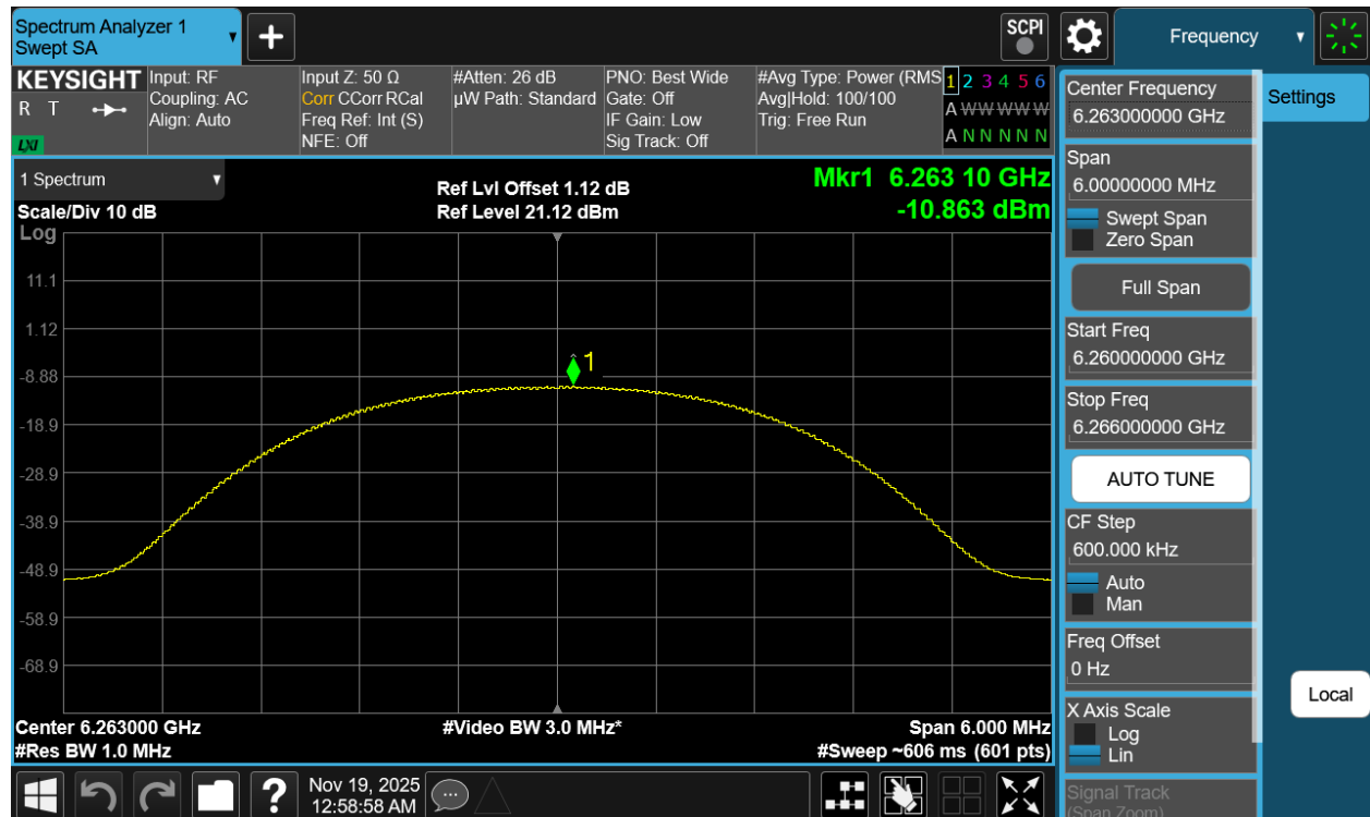
Plot 7-47. PSD Antenna 5T (NB UNII HDR4, iPA – 6263MHz)
