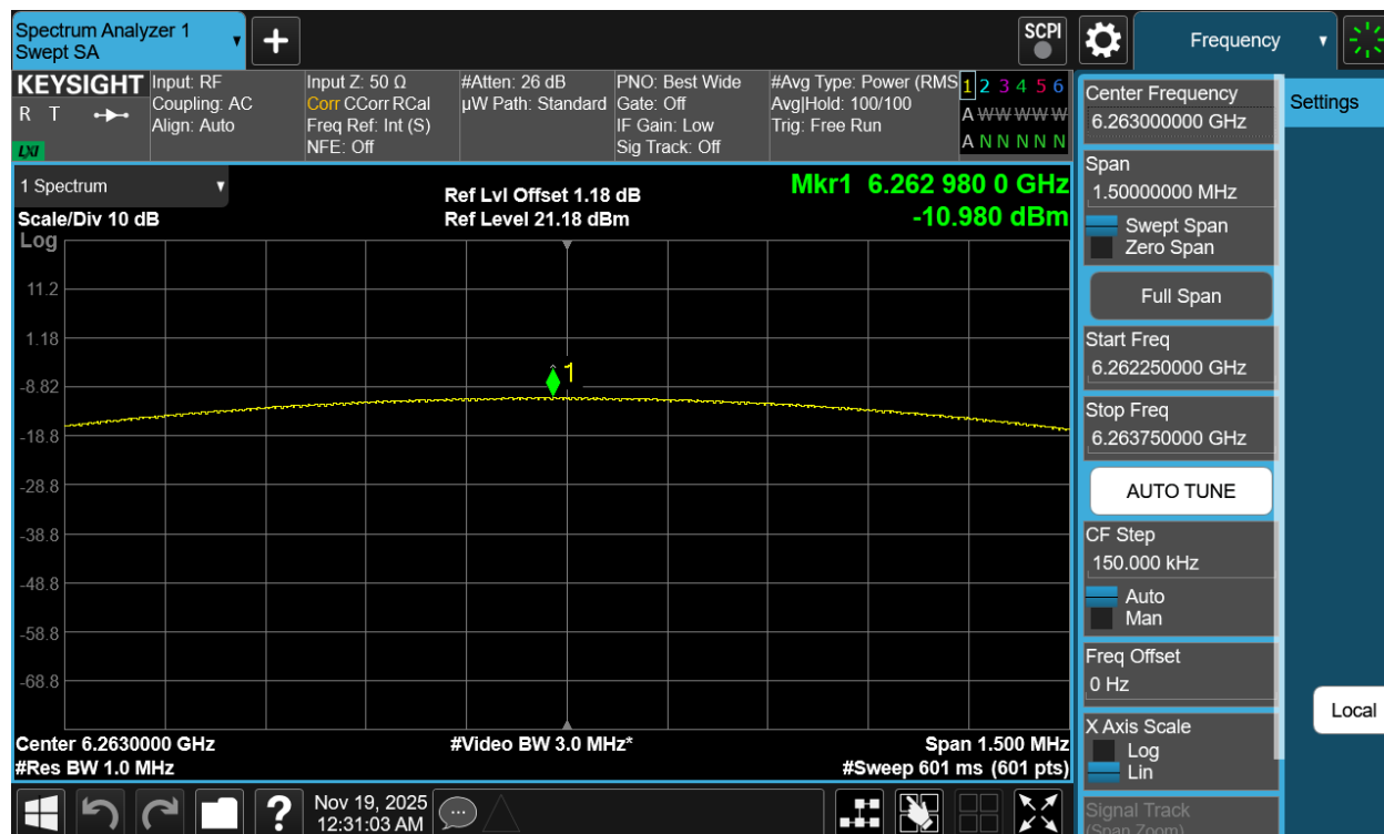
Plot 7-40. PSD Antenna 5T (NB UNII BDR, ePA – 6263MHz)
