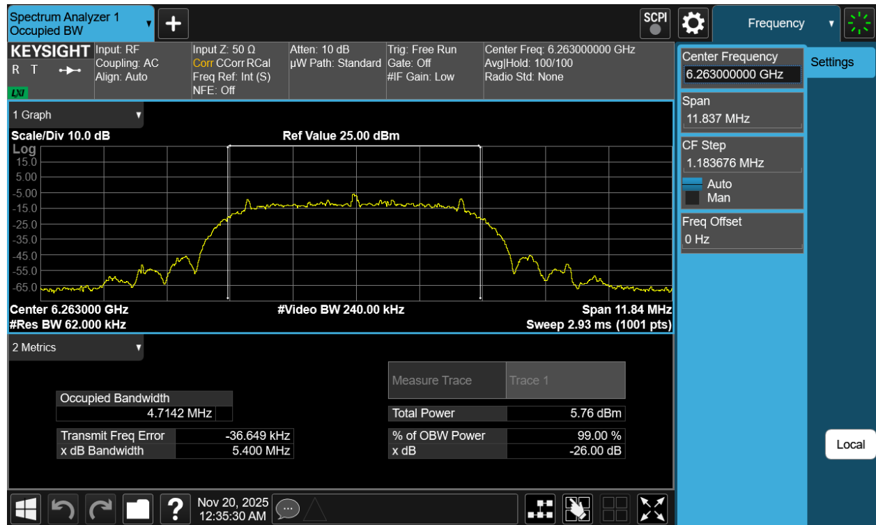
Plot 7-20. 26dB BW & 99% OBW Antenna 3b (NB UNII XHDRPM6, ePA- 6263MHz)
