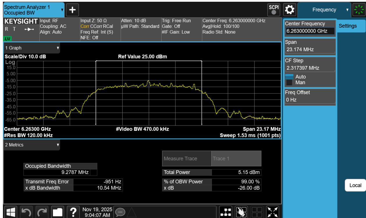
Plot 7-10. 26dB BW & 99% OBW Antenna 5T (NB UNII HDRPL32, ePA- 6263MHz)
