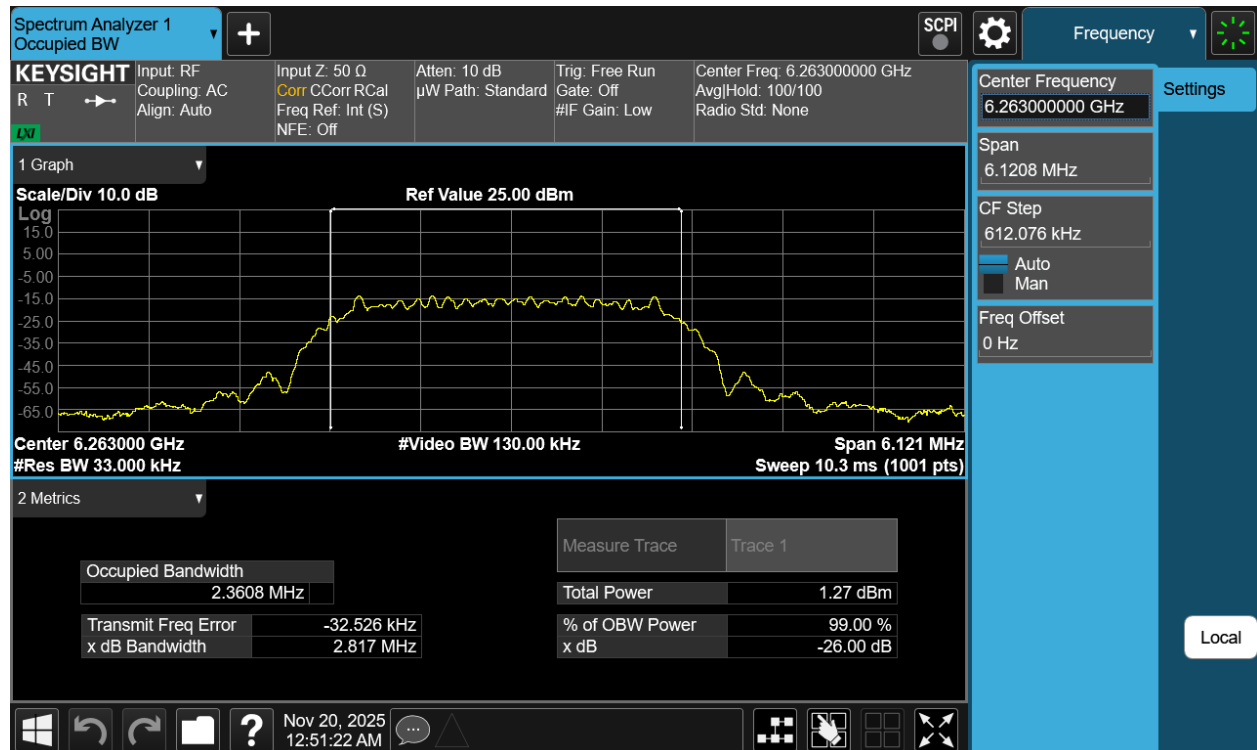
Plot 7-25. 26dB BW & 99% OBW Antenna 3b (NB UNII HDT4, ePA- 6263MHz)
