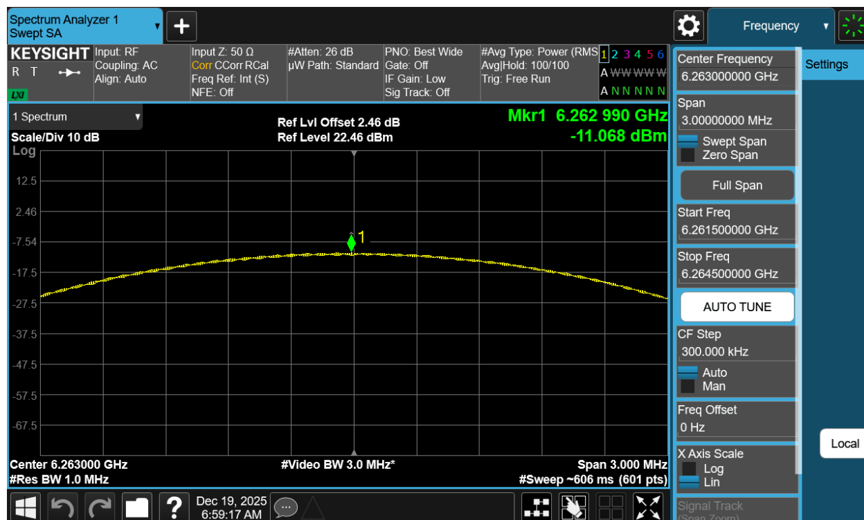
Plot 7-45. PSD Antenna 5T (NB UNII LE2M, iPA – 6263MHz)
