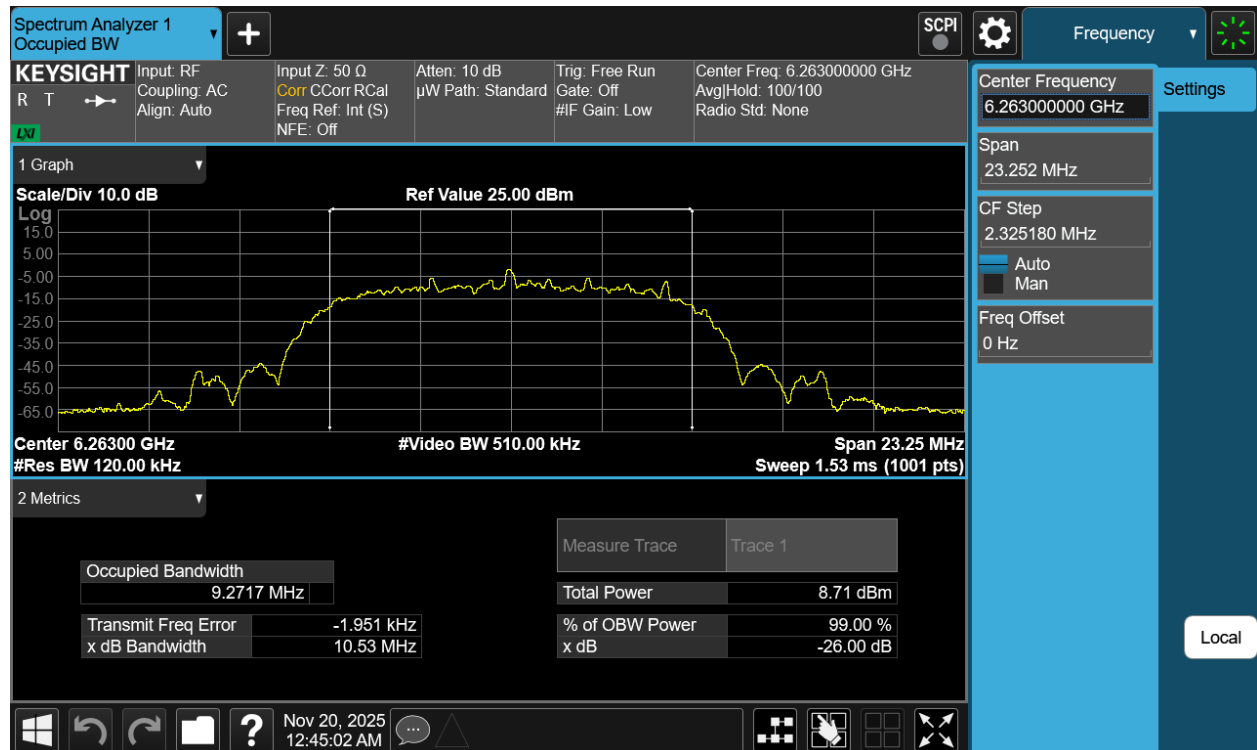
Plot 7-23. 26dB BW & 99% OBW Antenna 3b (NB UNII HDRPL32, ePA- 6263MHz)
