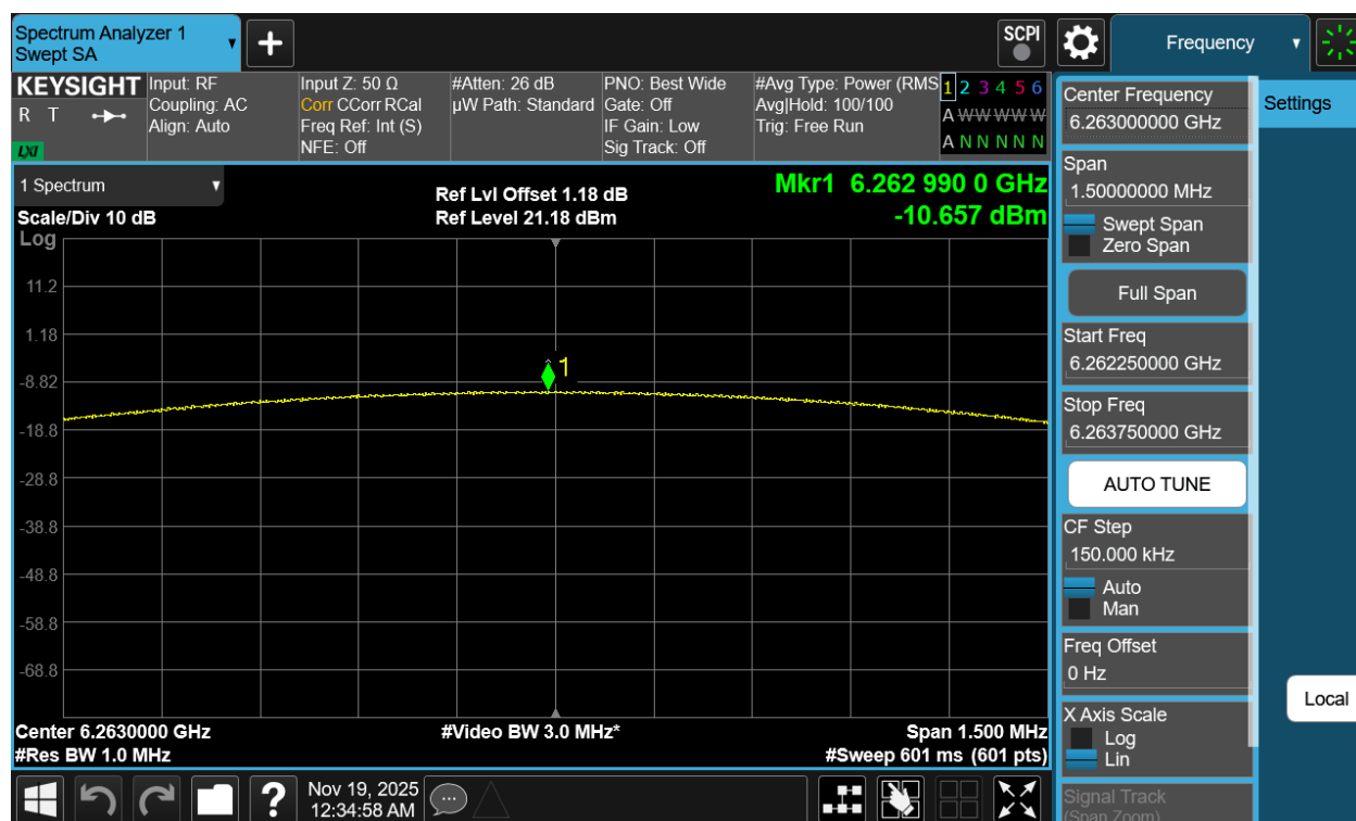
Plot 7-41. PSD Antenna 5T (NB UNII BDR, iPA – 6263MHz)
