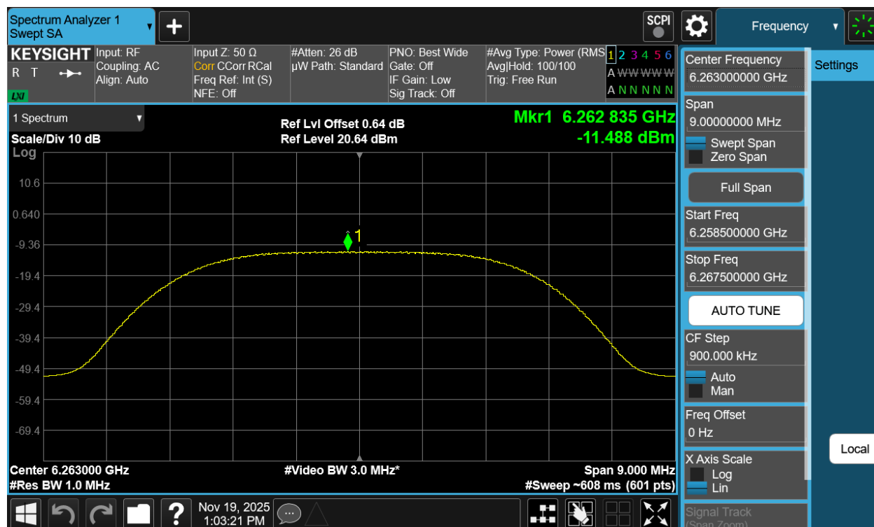
Plot 7-52. PSD Antenna 5T (NB UNII XHDRPM6, ePA – 6263MHz)
