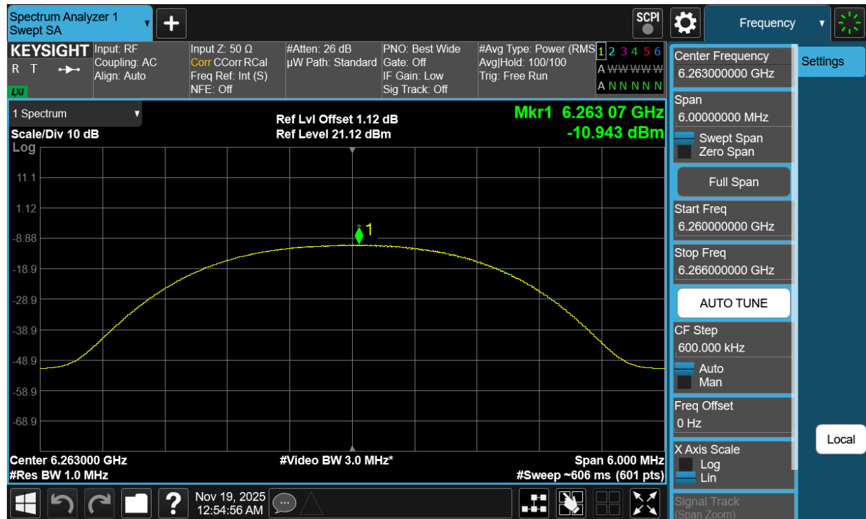
Plot 7-46. PSD Antenna 5T (NB UNII HDR4, ePA – 6263MHz)
