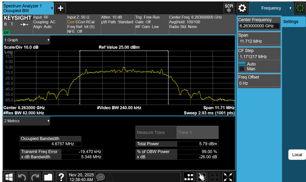
Plot 7-21. 26dB BW & 99% OBW Antenna 3b (NB UNII HDRPM16, ePA- 6263MHz)
