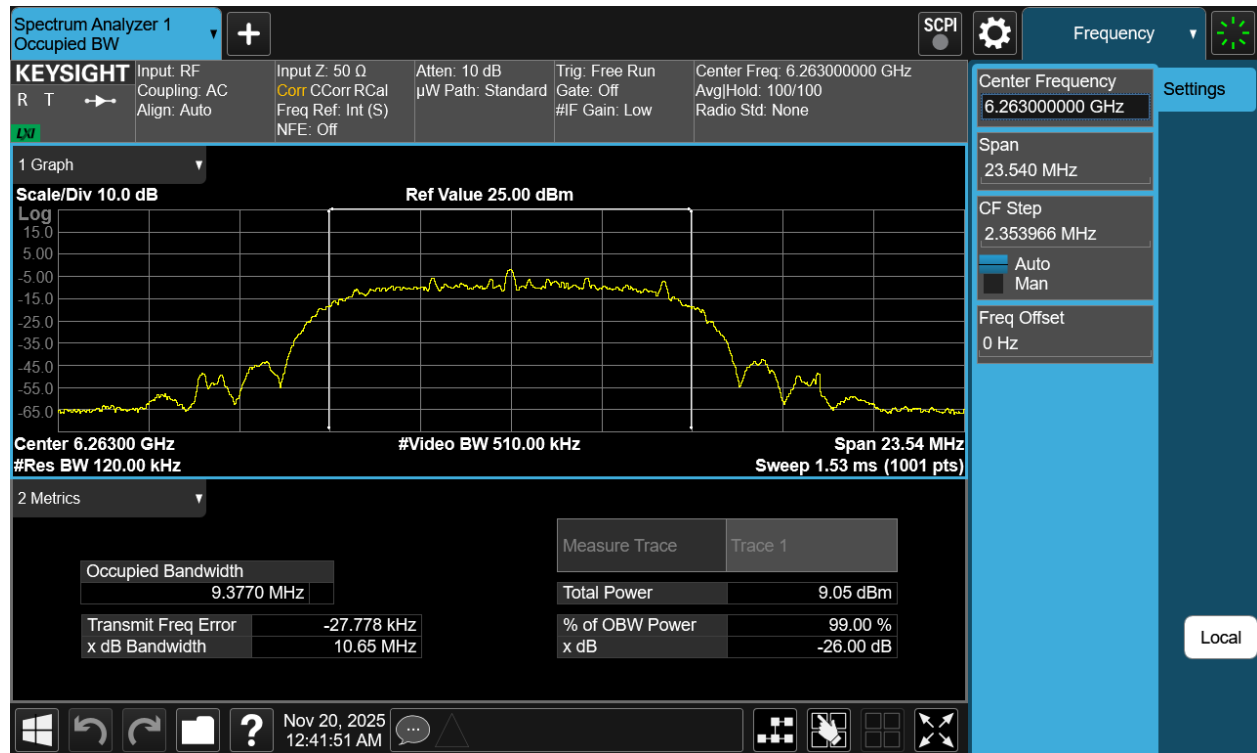
Plot 7-22. 26dB BW & 99% OBW Antenna 3b (NB UNII HDRPL12, ePA- 6263MHz)
