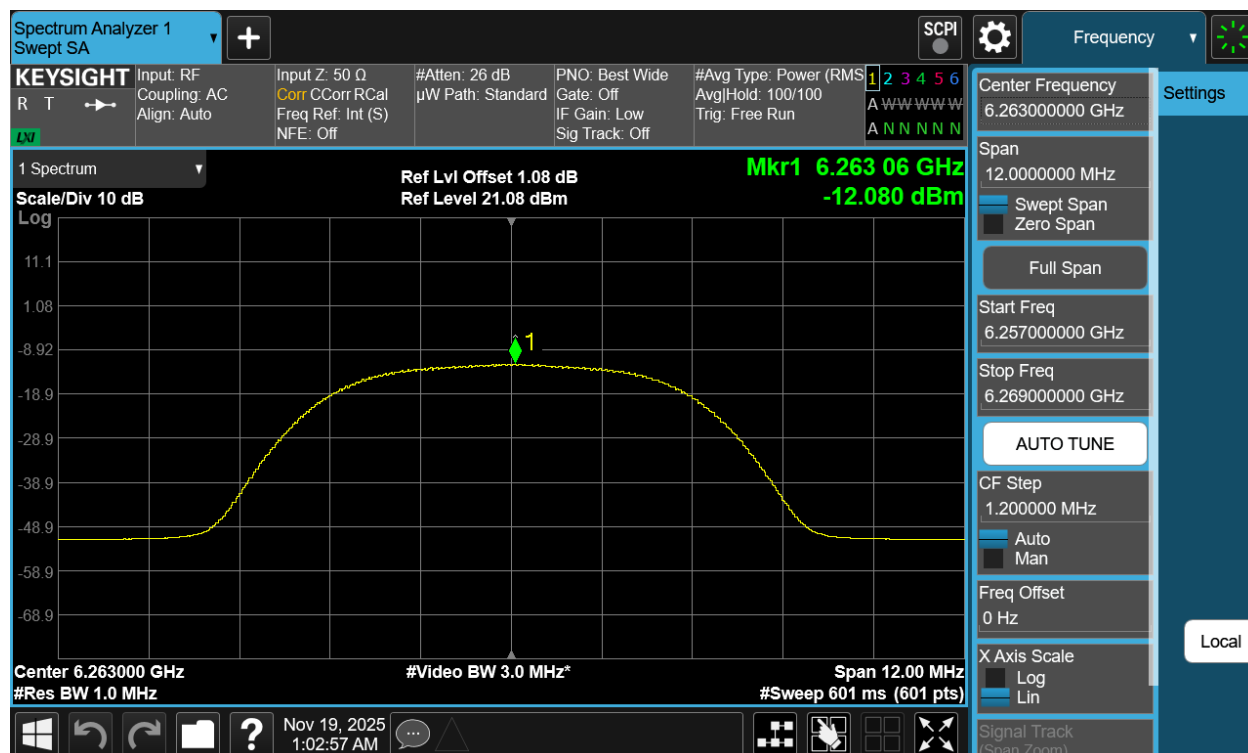
Plot 7-48. PSD Antenna 5T (NB UNII HDR8, ePA – 6263MHz)
