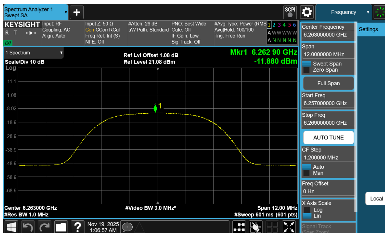
Plot 7-49. PSD Antenna 5T (NB UNII HDR8, iPA – 6263MHz)
