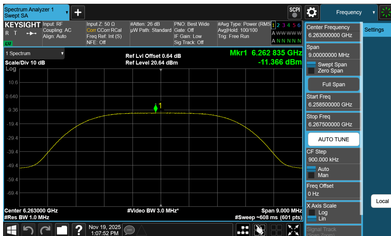
Plot 7-53. PSD Antenna 5T (NB UNII XHDRPM6, iPA – 6263MHz)
