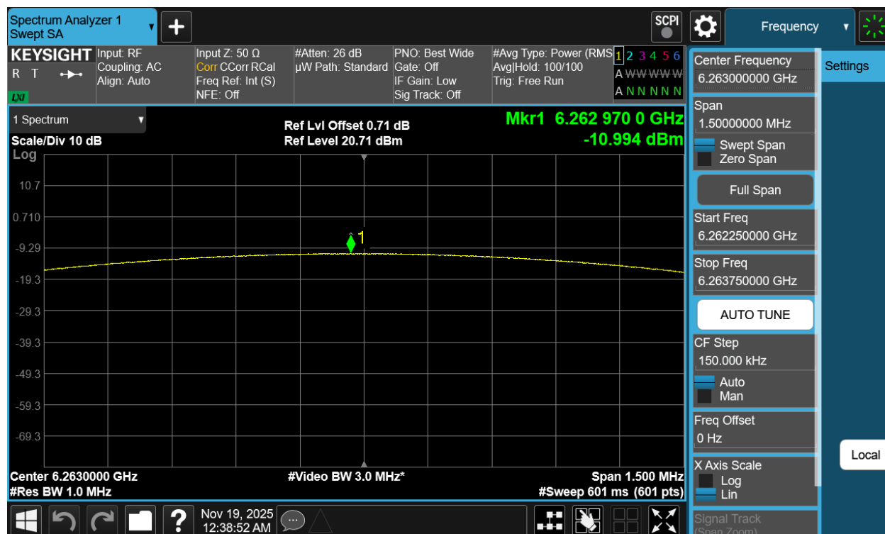
Plot 7-42. PSD Antenna 5T (NB UNII LE1M, ePA – 6263MHz)
