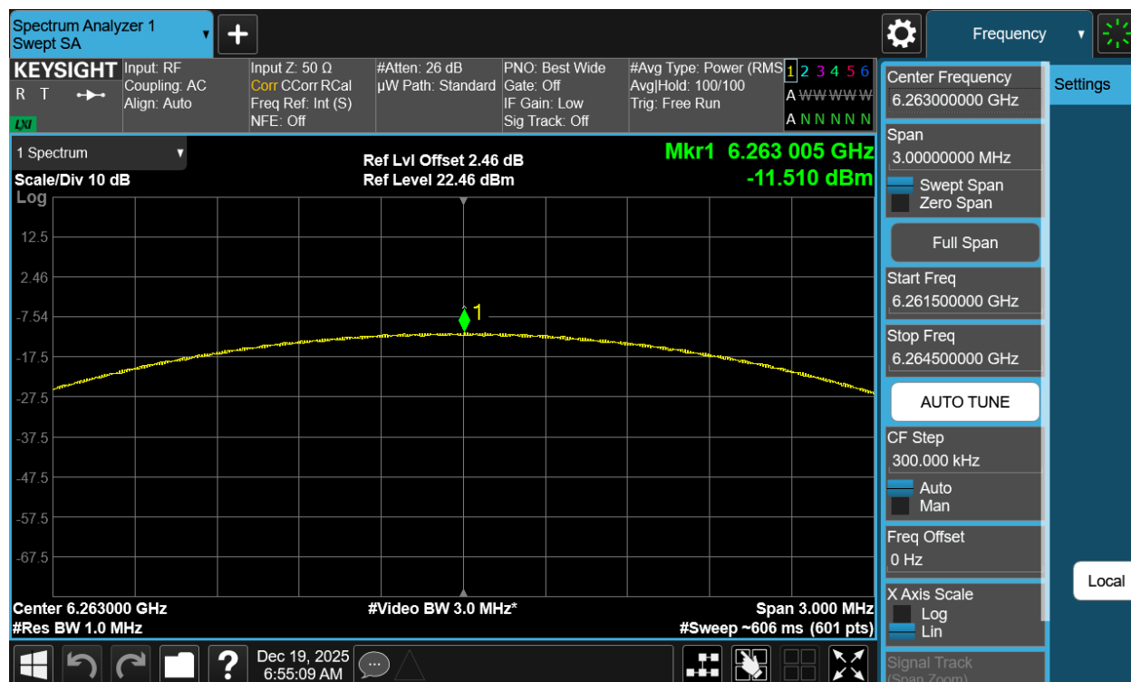
Plot 7-44. PSD Antenna 5T (NB UNII LE2M, ePA – 6263MHz)
