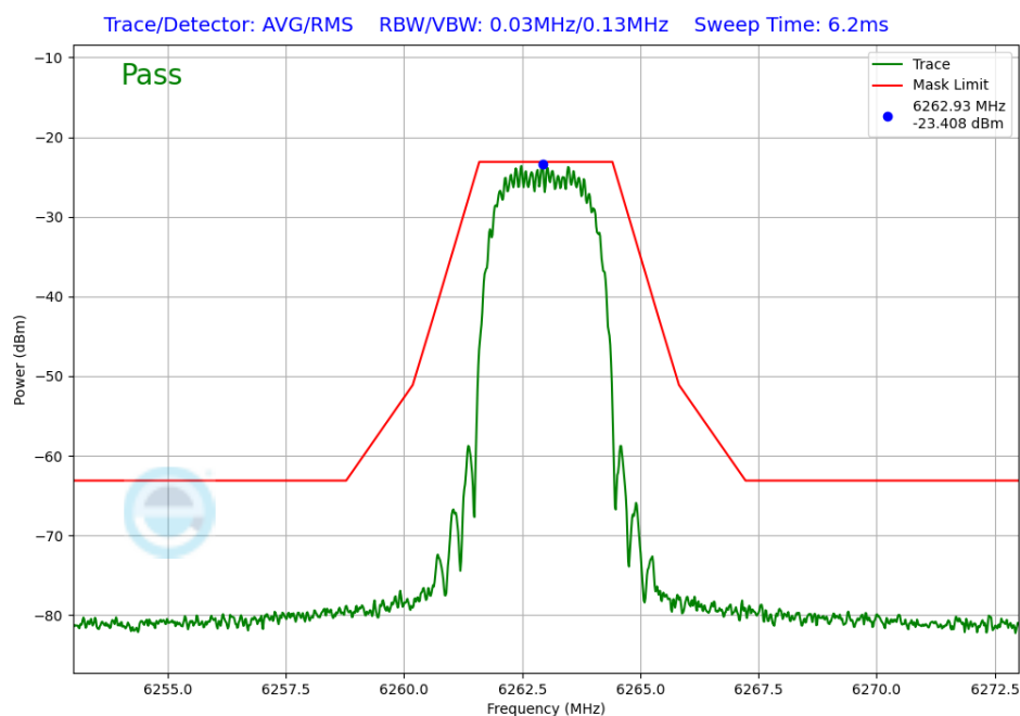
Plot 7-244. In-Band Emission Antenna 5T (NB UNII HDT4, ePA – 6263MHz)
