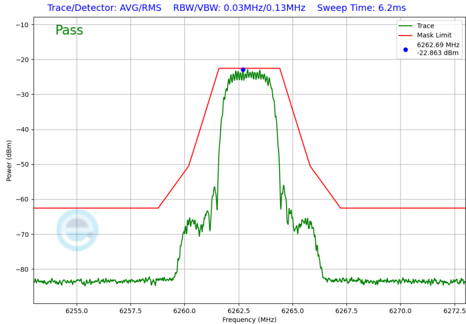
Plot 7-245. In-Band Emission Antenna 5T (NB UNII HDT4, iPA – 6263MHz)
