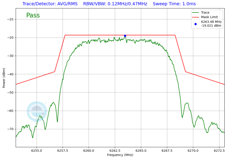
Plot 7-241. In-Band Emission Antenna 5T (NB UNII HDRPL32, iPA – 6263MHz)
