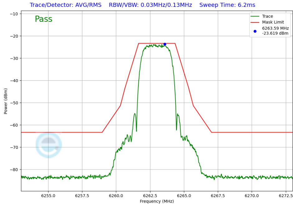
Plot 7-233. In-Band Emission Antenna 5T (NB UNII HDRPS2, iPA – 6263MHz)
