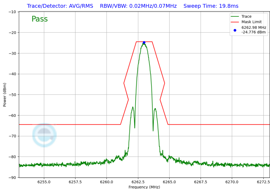
Plot 7-224. In-Band Emission Antenna 5T (NB UNII LE1M, ePA – 6263MHz)
