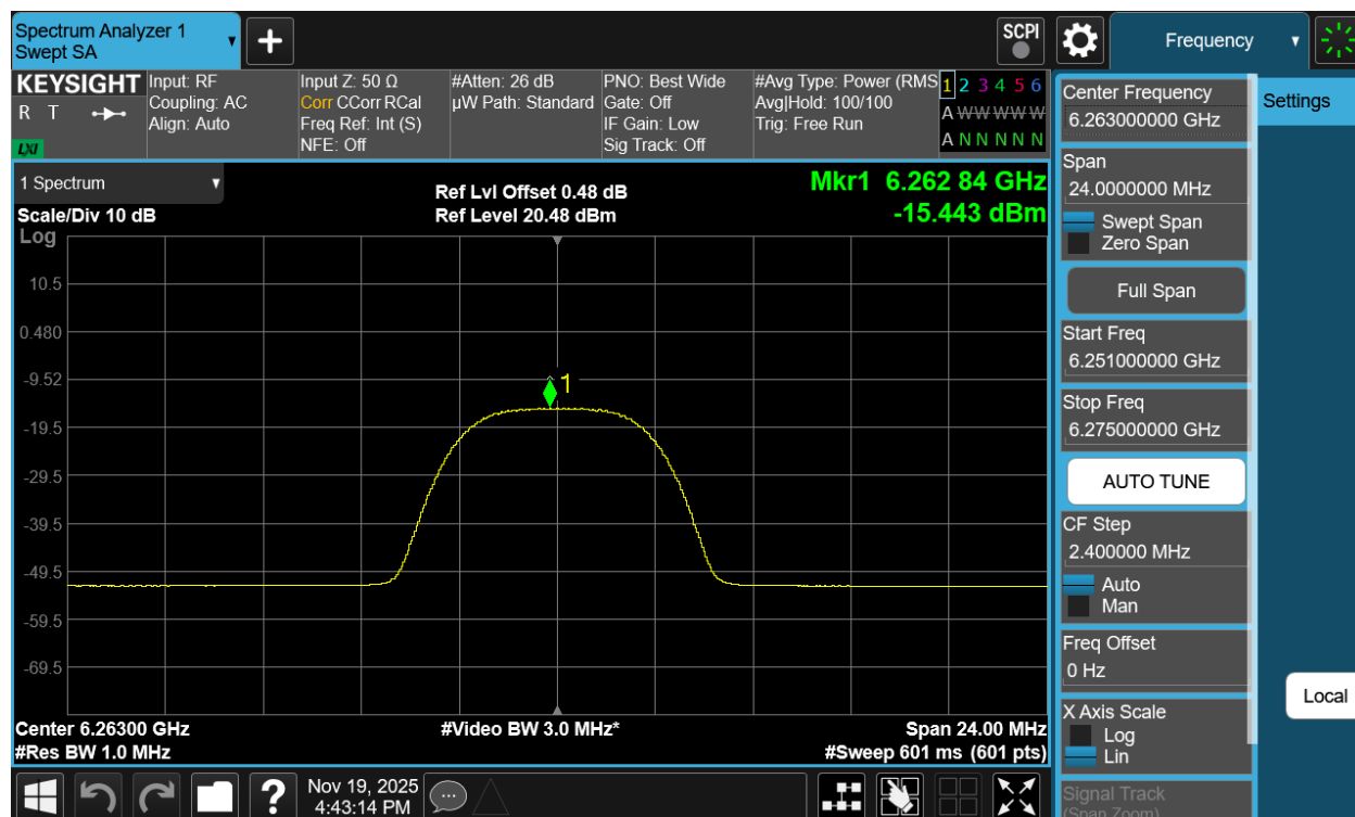
Plot 7-198. PSD TxBF Diversity Antenna 5T (NB UNII HDRPM16, ePA – 6263MHz)
