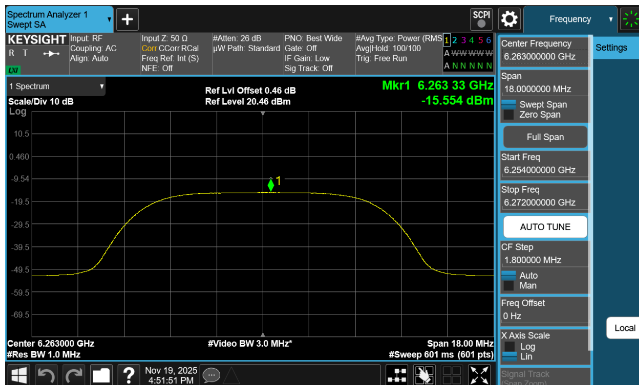
Plot 7-202. PSD TxBF Diversity Antenna 5T (NB UNII HDRPL12, ePA - 6263MHz)
