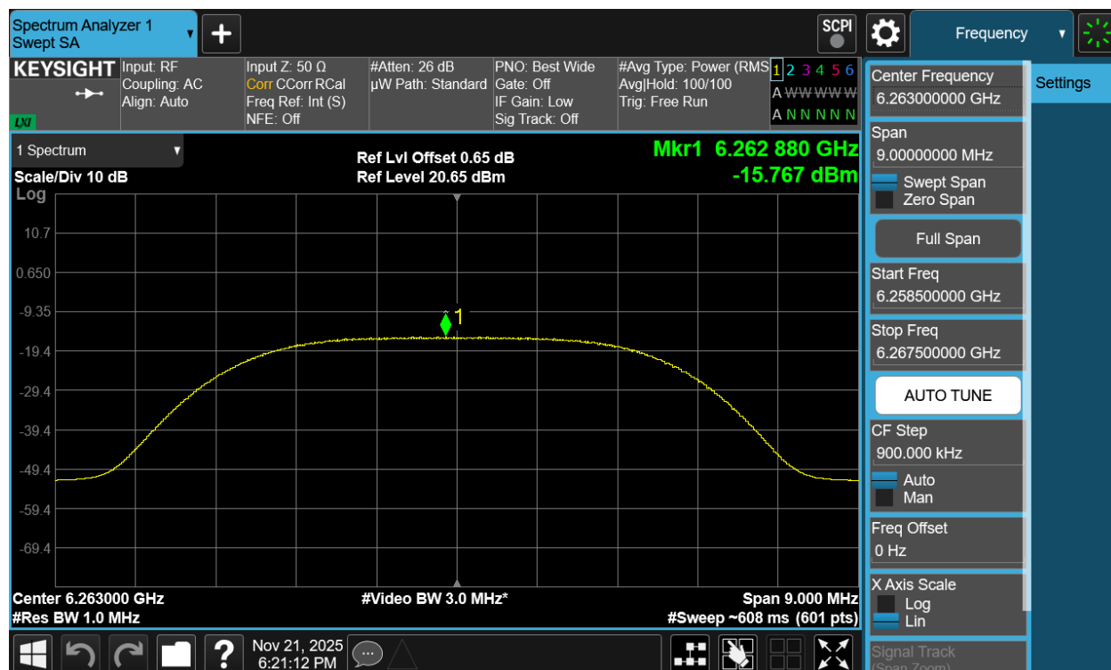
Plot 7-195. PSD TxBF Diversity Antenna 1b (NB UNII XHDRPM6, ePA – 6263MHz)
