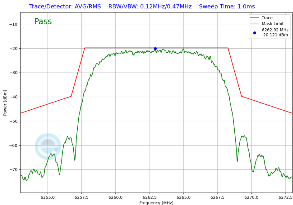
Plot 7-240. In-Band Emission Antenna 5T (NB UNII HDRPL32, ePA – 6263MHz)
