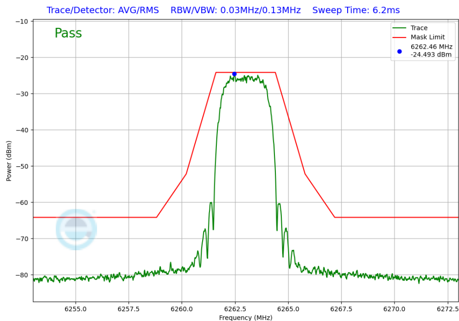
Plot 7-246. In-Band Emission Antenna 5T (NB UNII HDT6, ePA – 6263MHz)
