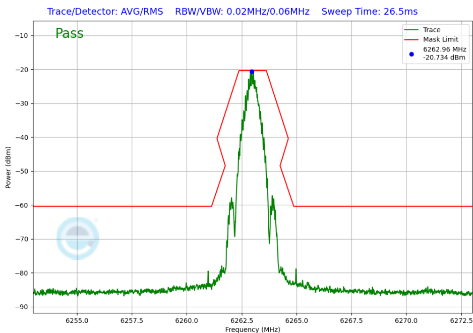
Plot 7-248. In-Band Emission Antenna 3b (NB UNII BDR, ePA – 6263MHz)
