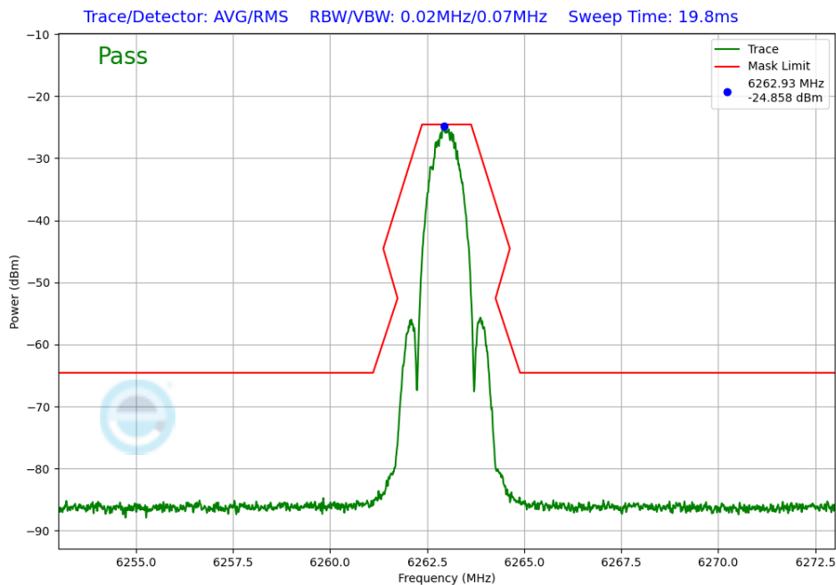
Plot 7-225. In-Band Emission Antenna 5T (NB UNII LE1M, iPA – 6263MHz)
