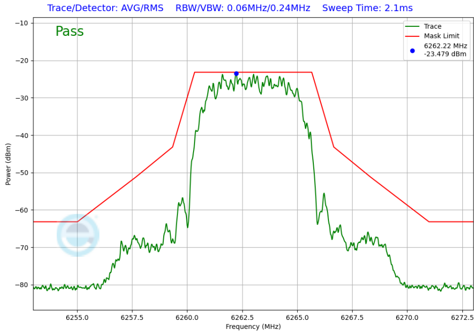
Plot 7-231. In-Band Emission Antenna 5T (NB UNII HDR8, iPA – 6263MHz)
