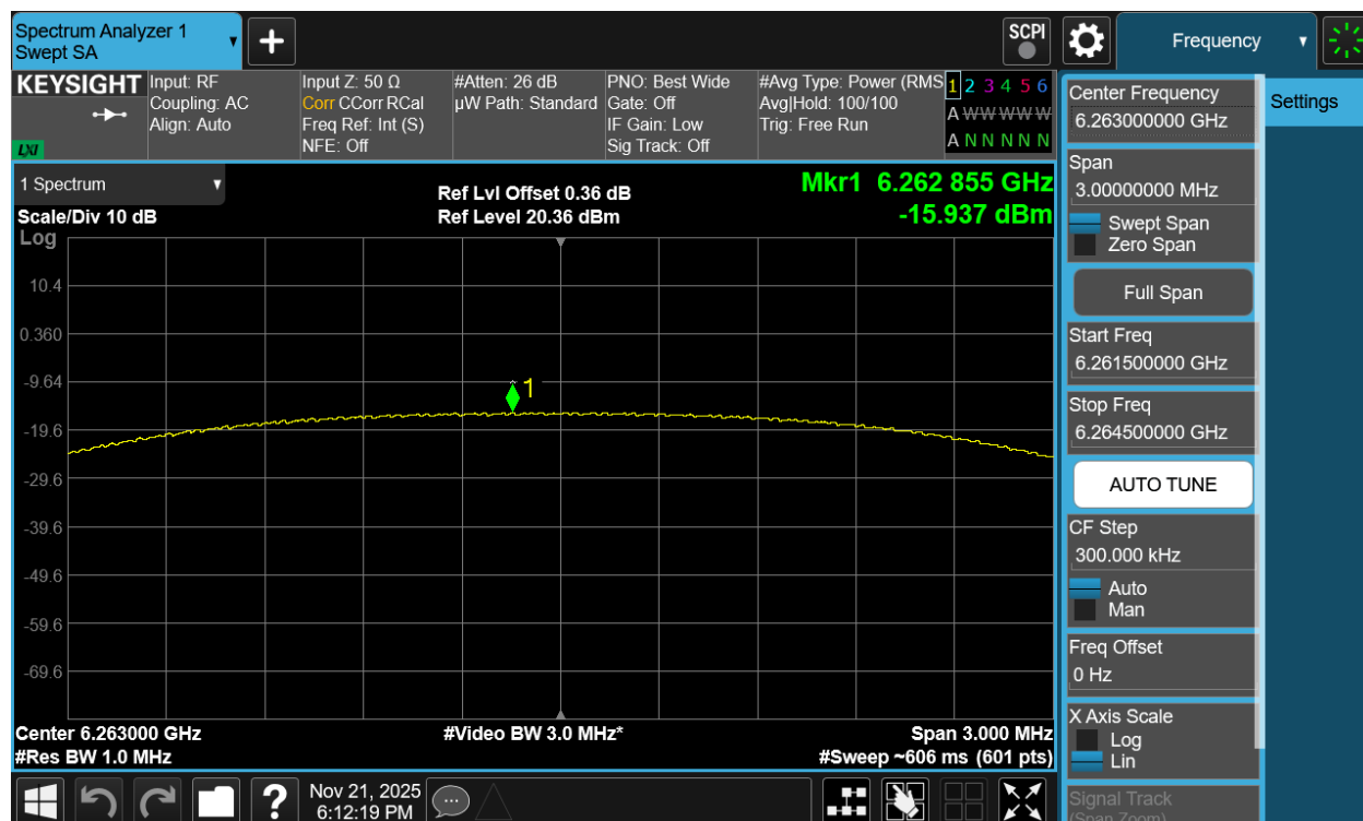
Plot 7-191. PSD TxBF Diversity Antenna 1b (NB UNII HDRPS2, ePA – 6263MHz)
