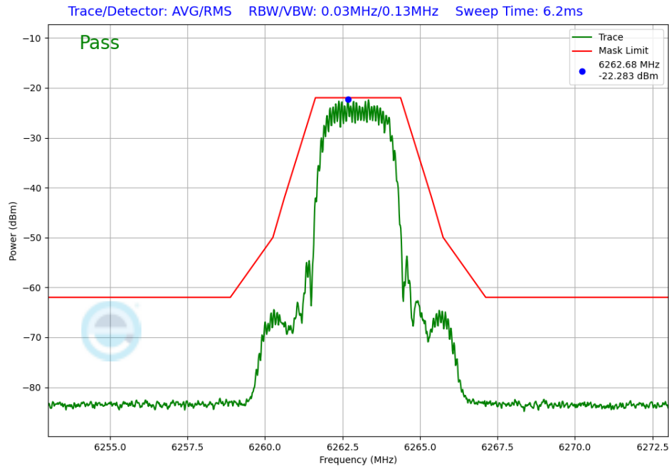
Plot 7-243. In-Band Emission Antenna 5T (NB UNII HDT2, iPA – 6263MHz)
