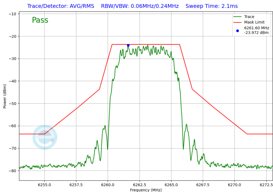
Plot 7-230. In-Band Emission Antenna 5T (NB UNII HDR8, ePA – 6263MHz)
