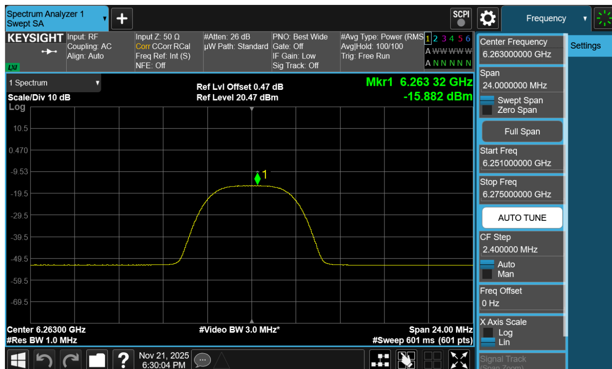
Plot 7-199. PSD TxBF Diversity Antenna 1b (NB UNII HDRPM16, ePA – 6263MHz)
