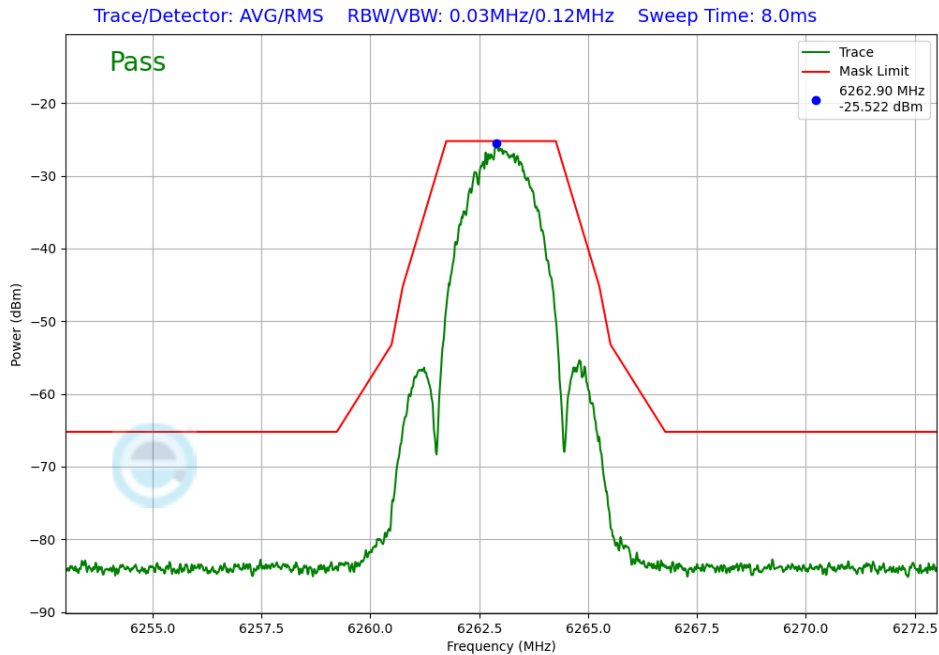
Plot 7-227. In-Band Emission Antenna 5T (NB UNII LE2M, iPA – 6263MHz)
