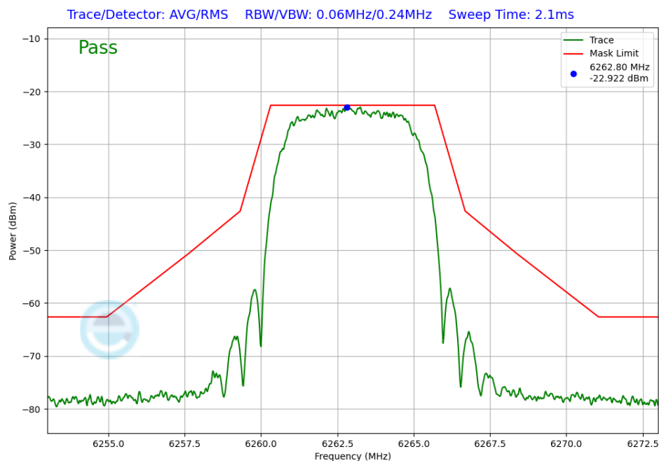
Plot 7-234. In-Band Emission Antenna 5T (NB UNII XHDRPM6, ePA – 6263MHz)
