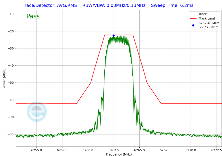
Plot 7-242. In-Band Emission Antenna 5T (NB UNII HDT2, ePA – 6263MHz)
