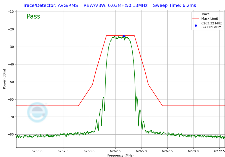
Plot 7-232. In-Band Emission Antenna 5T (NB UNII HDRPS2, ePA – 6263MHz)
