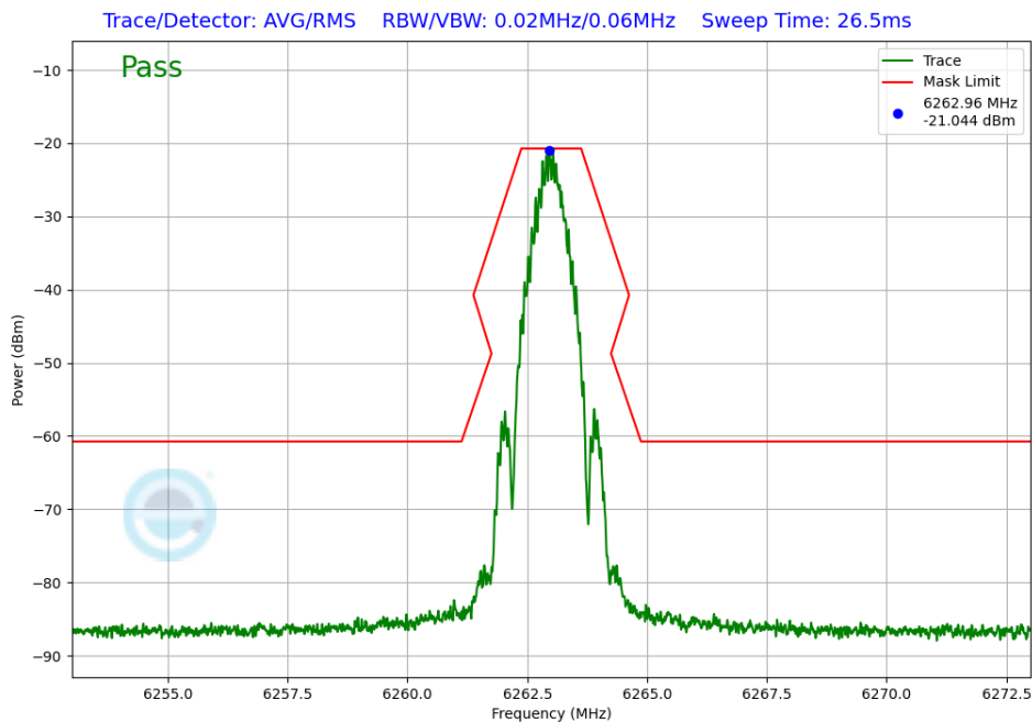
Plot 7-249. In-Band Emission Antenna 3b (NB UNII BDR, iPA – 6263MHz)
