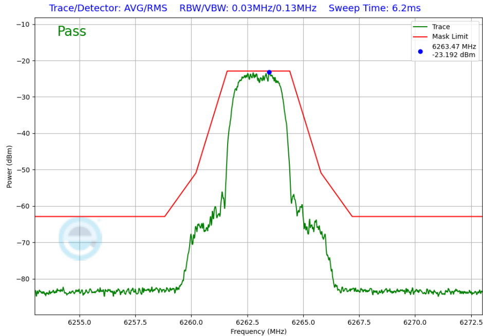
Plot 7-247. In-Band Emission Antenna 5T (NB UNII HDT6, iPA – 6263MHz)
