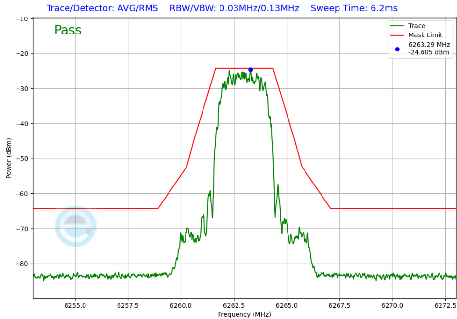
Plot 7-229. In-Band Emission Antenna 5T (NB UNII HDR4, iPA – 6263MHz)
