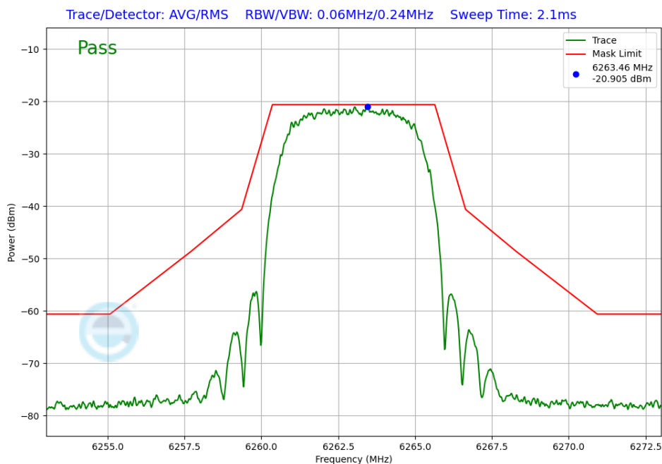
Plot 7-236. In-Band Emission Antenna 5T (NB UNII HDRPM16, ePA – 6263MHz)
