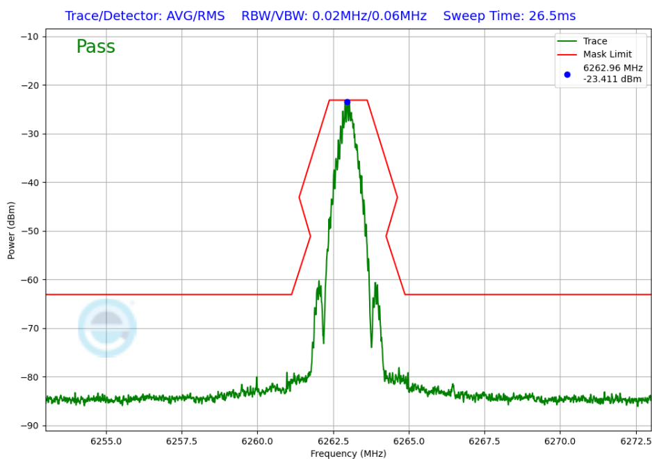
Plot 7-222. In-Band Emission Antenna 5T (NB UNII BDR, ePA – 6263MHz)
