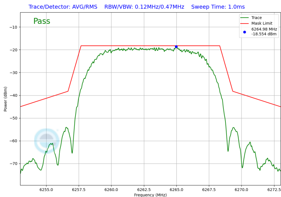
Plot 7-238. In-Band Emission Antenna 5T (NB UNII HDRPL12, ePA – 6263MHz)
