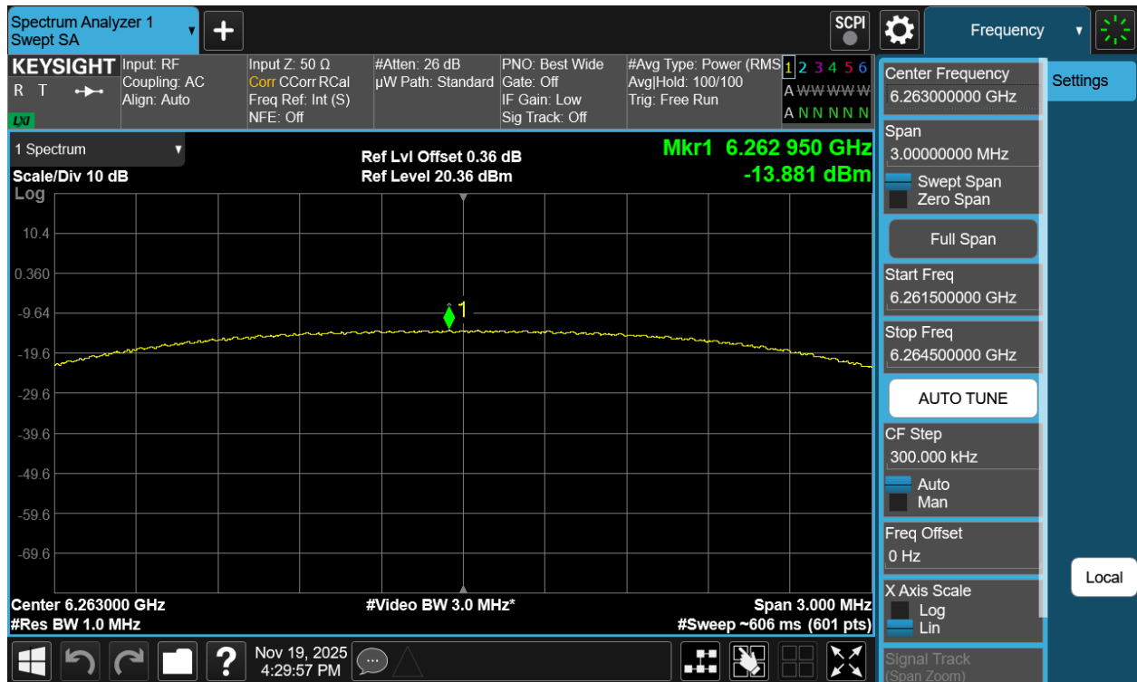
Plot 7-192. PSD TxBF Diversity Antenna 5T (NB UNII HDRPS2, iPA – 6263MHz)
