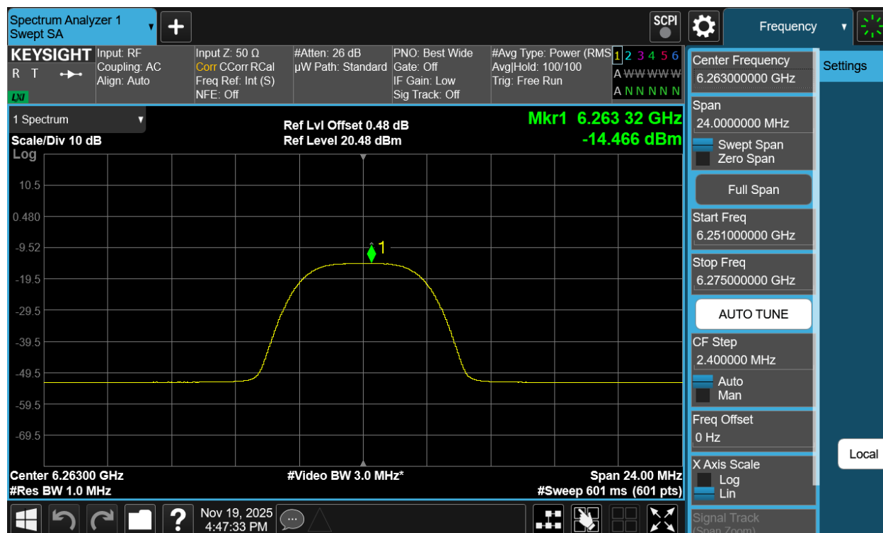
Plot 7-200. PSD TxBF Diversity Antenna 5T (NB UNII HDRPM16, iPA – 6263MHz)
