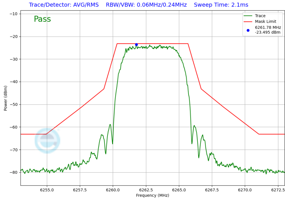
Plot 7-235. In-Band Emission Antenna 5T (NB UNII XHDRPM6, iPA – 6263MHz)
