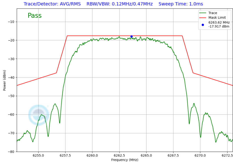
Plot 7-239. In-Band Emission Antenna 5T (NB UNII HDRPL12, iPA – 6263MHz)
