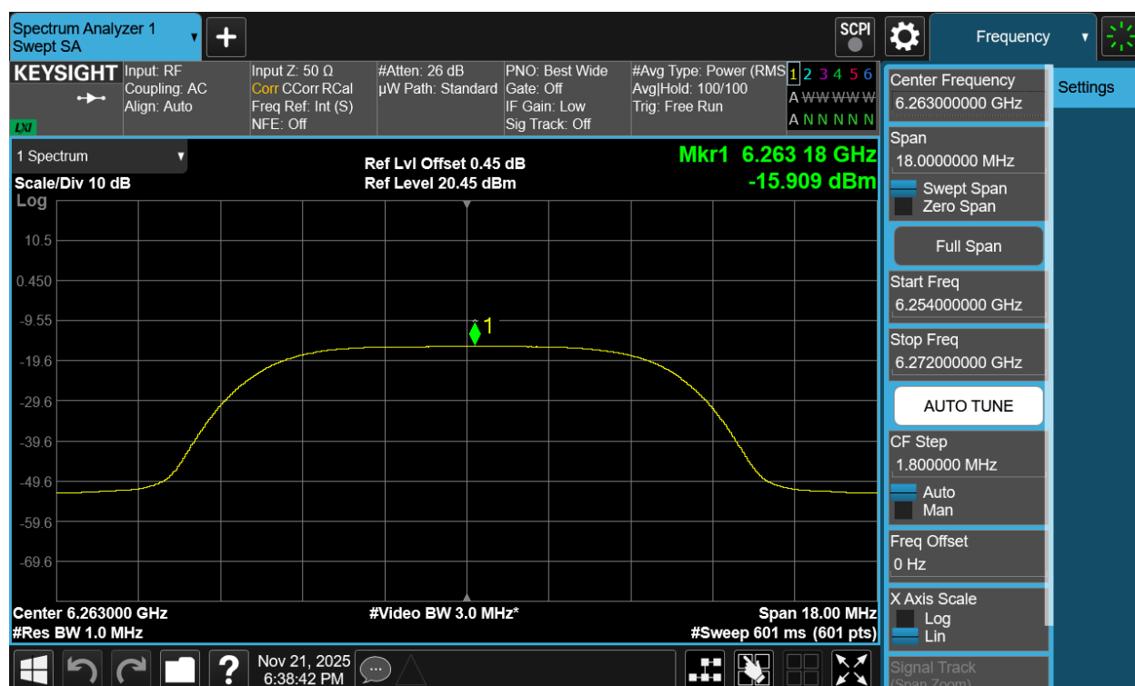
Plot 7-203. PSD TxBF Diversity Antenna 1b (NB UNII HDRPL12, ePA - 6263MHz)
