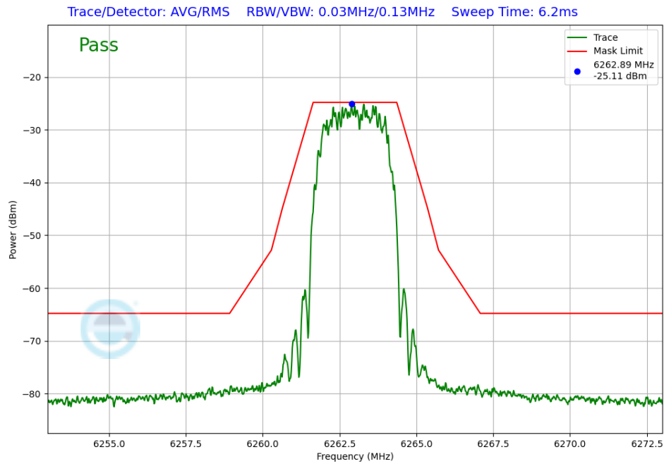
Plot 7-228. In-Band Emission Antenna 5T (NB UNII HDR4, ePA – 6263MHz)
