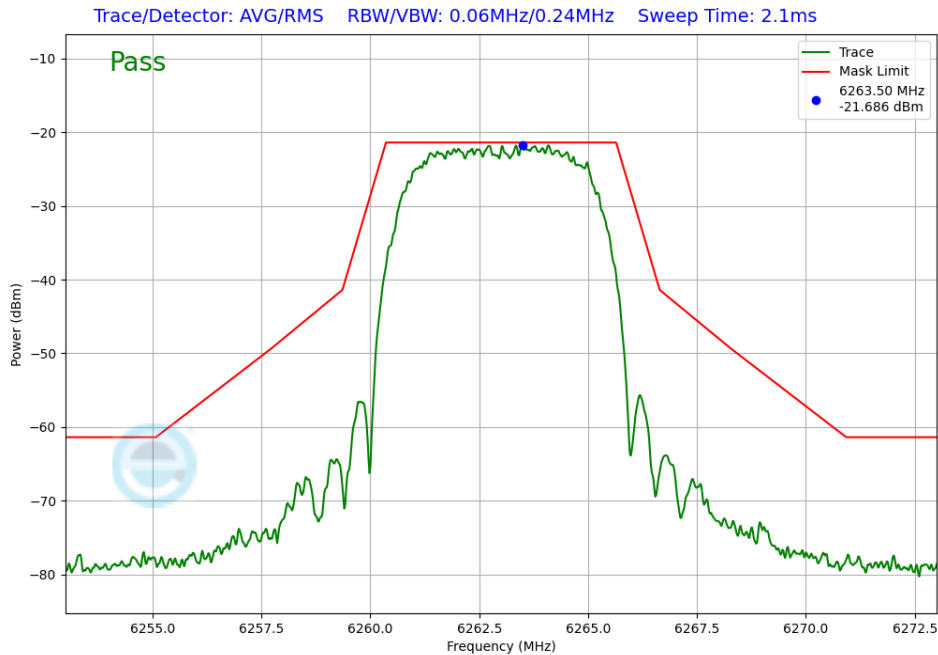
Plot 7-237. In-Band Emission Antenna 5T (NB UNII HDRPM16, iPA – 6263MHz)
