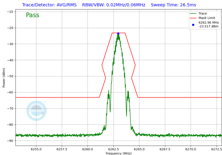
Plot 7-223. In-Band Emission Antenna 5T (NB UNII BDR, iPA – 6263MHz)
