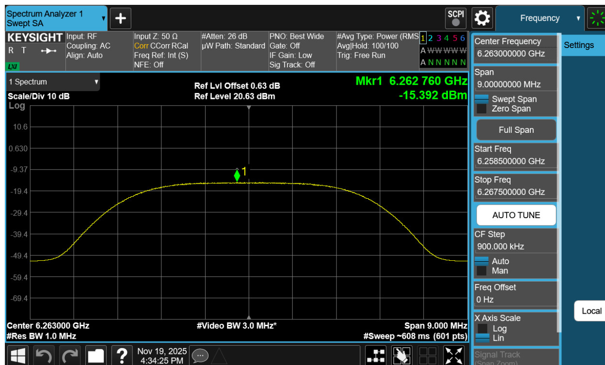
Plot 7-194. PSD TxBF Diversity Antenna 5T (NB UNII XHDRPM6, ePA – 6263MHz)
