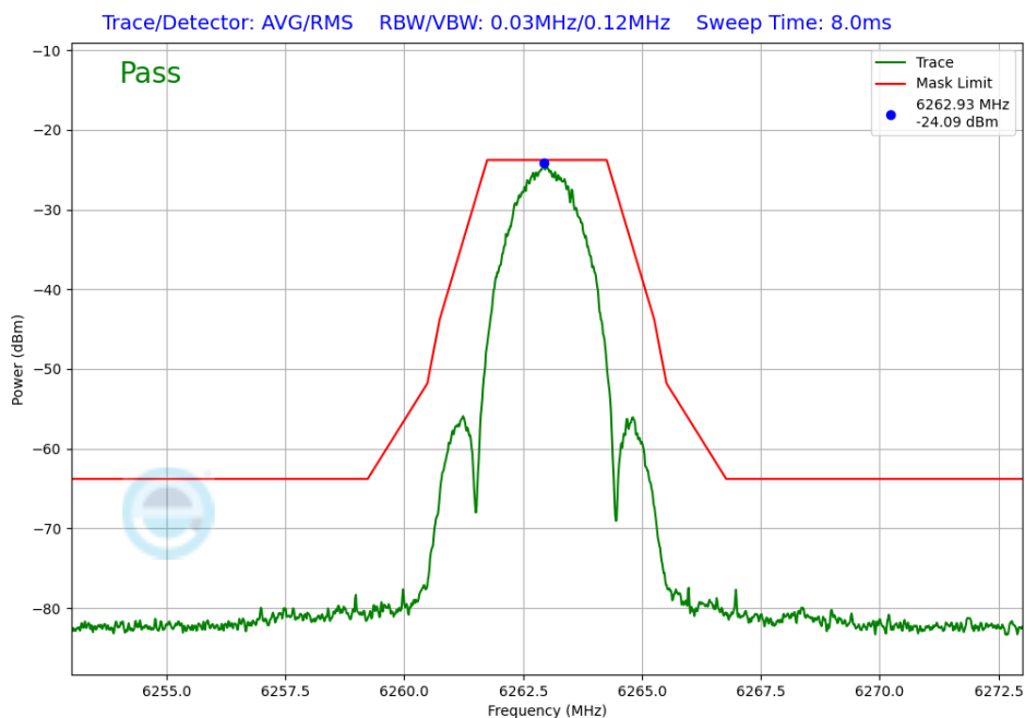
Plot 7-226. In-Band Emission Antenna 5T (NB UNII LE2M, ePA – 6263MHz)
