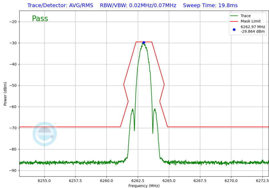
Plot 7-307. In-Band Emission TxBF Primary Antenna 3b (NB UNII LE1M, iPA – 6263MHz)
