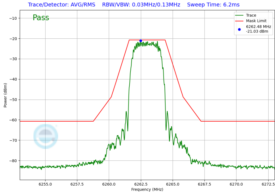
Plot 7-271. In-Band Emission Antenna 3b (NB UNII HDT4, iPA – 6263MHz)
