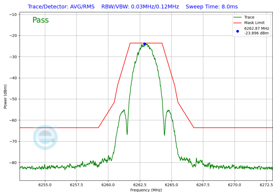
Plot 7-252. In-Band Emission Antenna 3b (NB UNII LE2M, ePA – 6263MHz)
