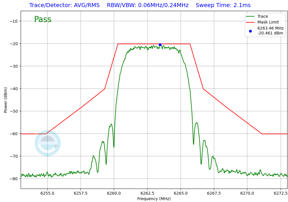
Plot 7-260. In-Band Emission Antenna 3b (NB UNII XHDRPM6, ePA – 6263MHz)
