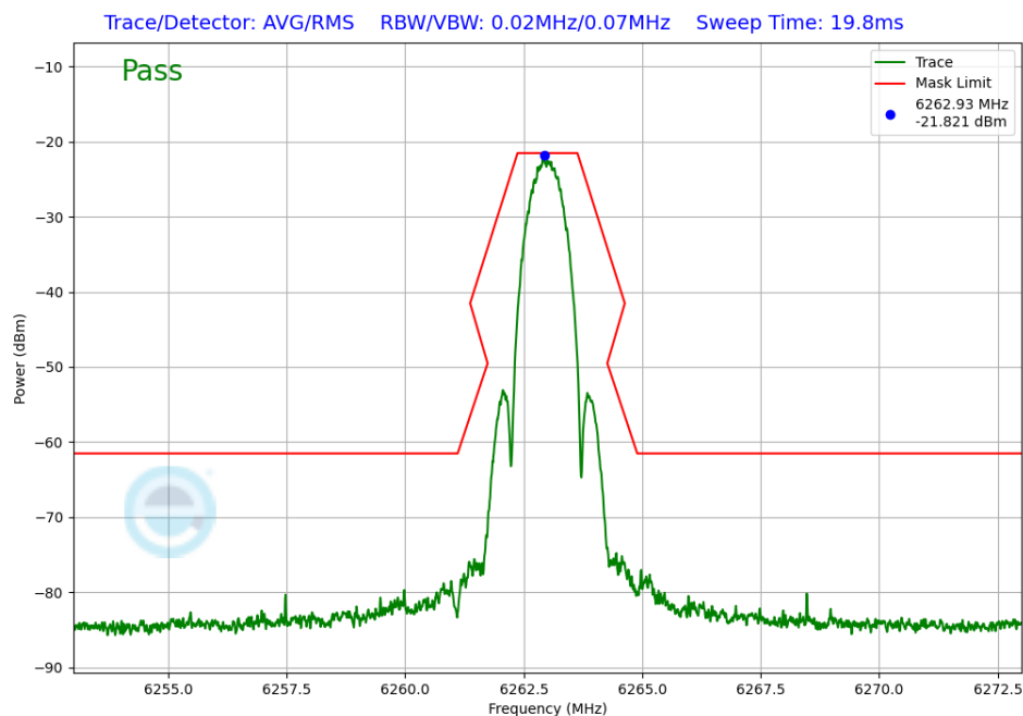
Plot 7-250. In-Band Emission Antenna 3b (NB UNII LE1M, ePA – 6263MHz)
