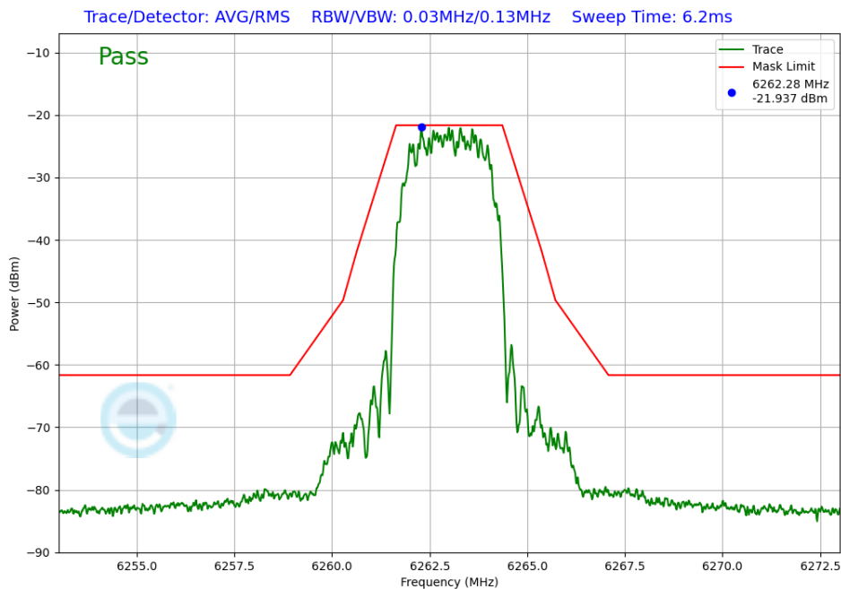
Plot 7-255. In-Band Emission Antenna 3b (NB UNII HDR4, iPA – 6263MHz)
