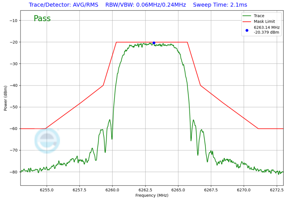
Plot 7-261. In-Band Emission Antenna 3b (NB UNII XHDRPM6, iPA – 6263MHz)
