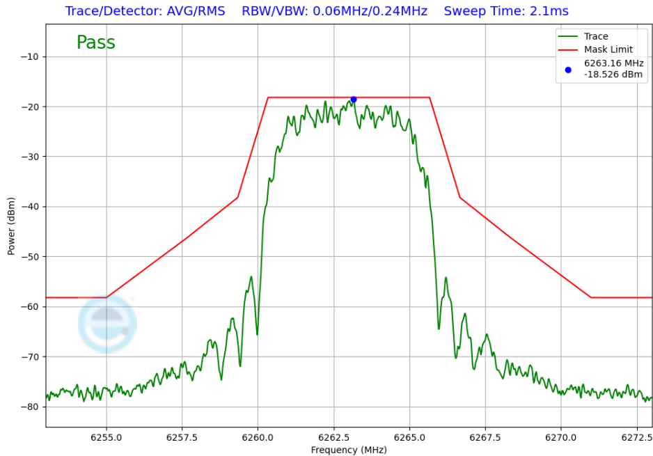
Plot 7-257. In-Band Emission Antenna 3b (NB UNII HDR8, iPA – 6263MHz)
