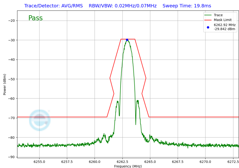
Plot 7-304. In-Band Emission TxBF Primary Antenna 5T (NB UNII LE1M, ePA – 6263MHz)
