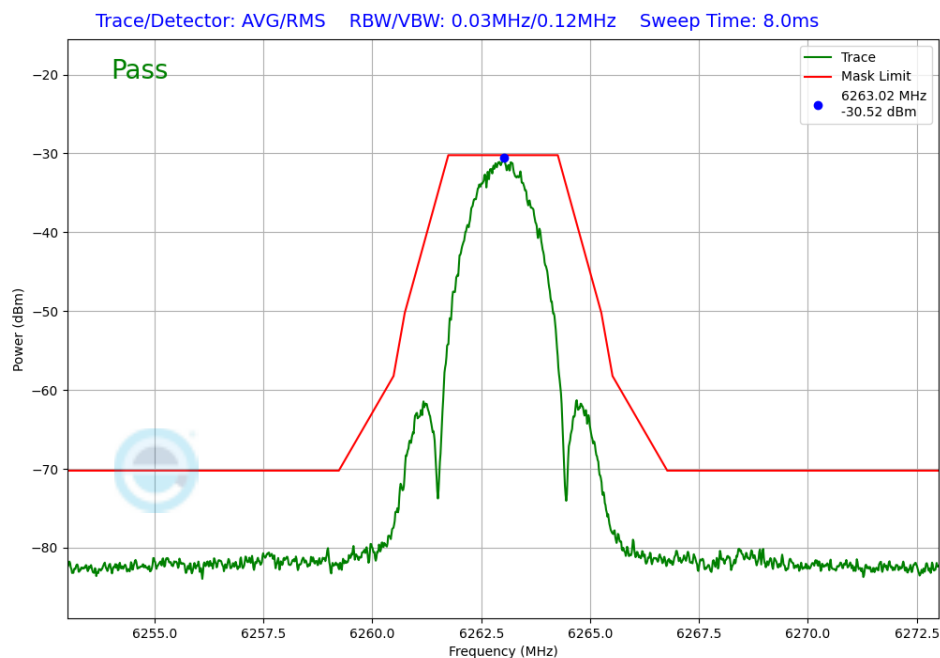
Plot 7-308. In-Band Emission TxBF Primary Antenna 5T (NB UNII LE2M, ePA – 6263MHz)
