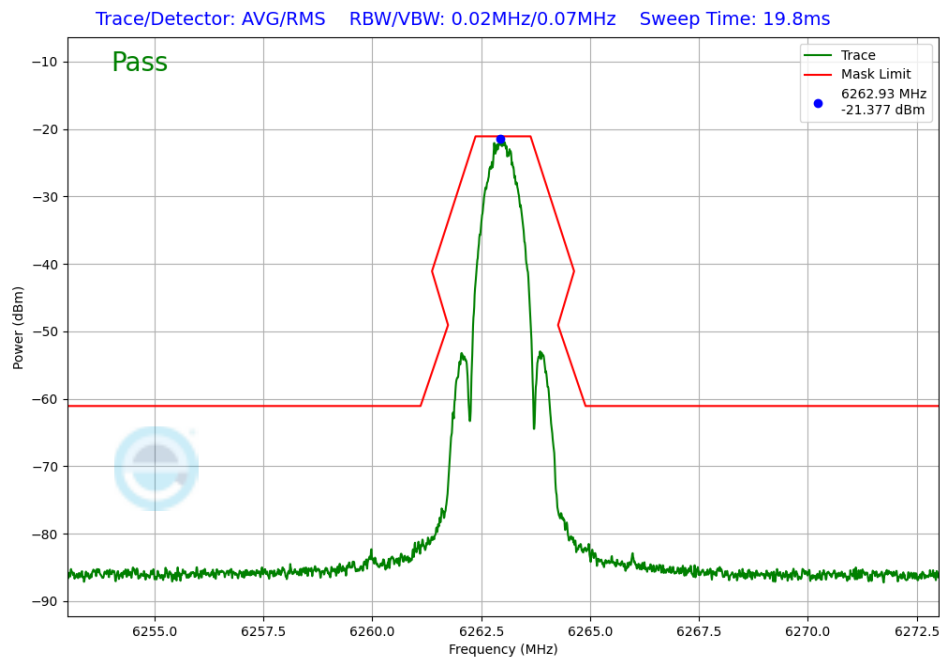
Plot 7-251. In-Band Emission Antenna 3b (NB UNII LE1M, iPA – 6263MHz)
