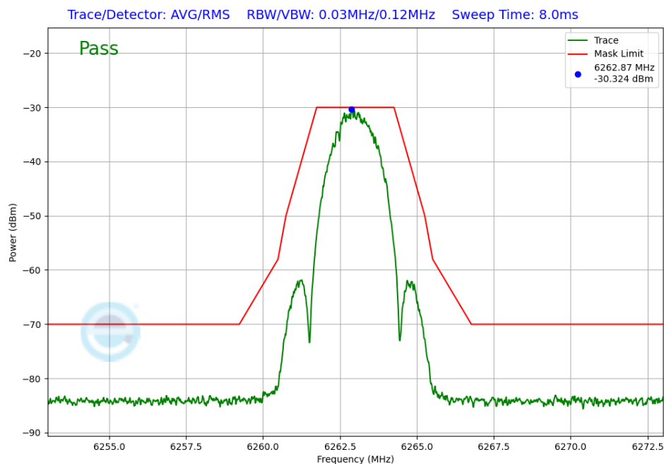
Plot 7-310. In-Band Emission TxBF Primary Antenna 5T (NB UNII LE2M, iPA – 6263MHz)
