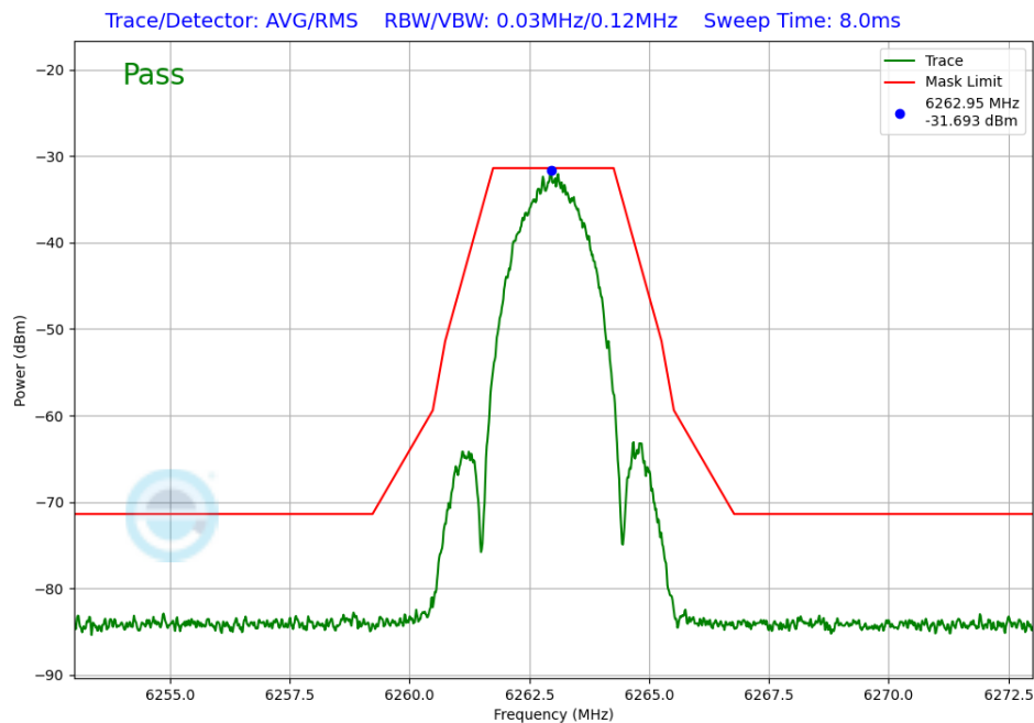
Plot 7-311. In-Band Emission TxBF Primary Antenna 3b (NB UNII LE2M, iPA – 6263MHz)
