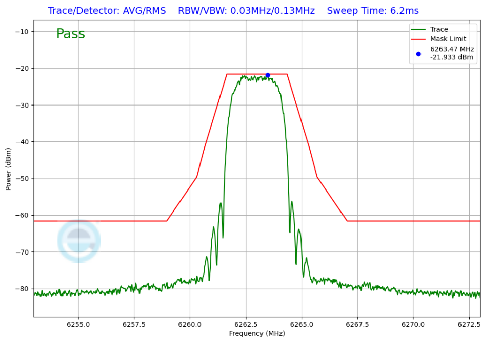
Plot 7-258. In-Band Emission Antenna 3b (NB UNII HDRPS2, ePA – 6263MHz)
