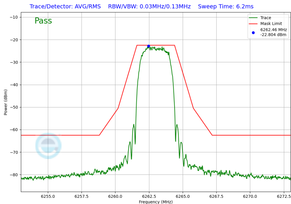
Plot 7-272. In-Band Emission Antenna 3b (NB UNII HDT6, ePA – 6263MHz)
