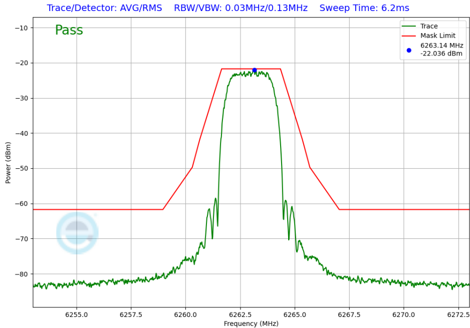
Plot 7-259. In-Band Emission Antenna 3b (NB UNII HDRPS2, iPA – 6263MHz)
