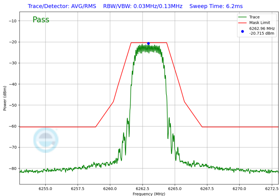
Plot 7-268. In-Band Emission Antenna 3b (NB UNII HDT2, ePA – 6263MHz)
