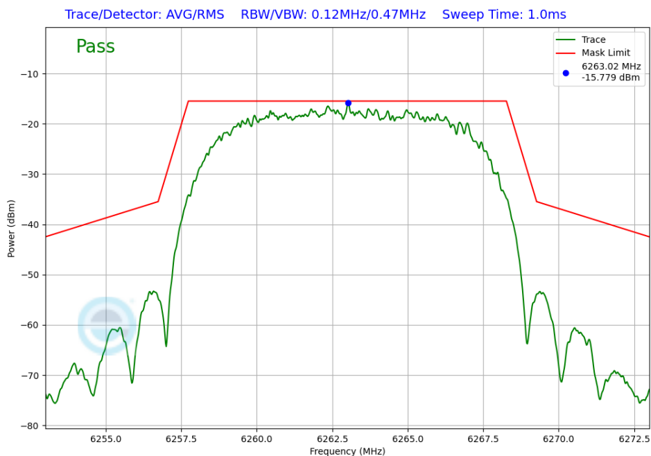
Plot 7-266. In-Band Emission Antenna 3b (NB UNII HDRPL32, ePA – 6263MHz)
