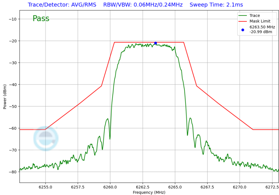
Plot 7-263. In-Band Emission Antenna 3b (NB UNII HDRPM16, iPA – 6263MHz)
