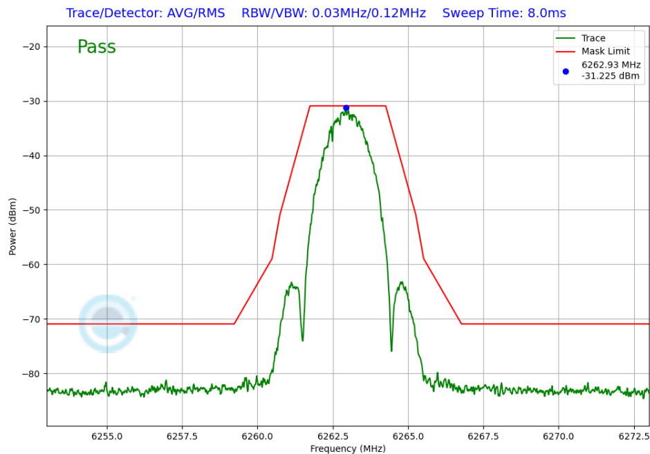
Plot 7-309. In-Band Emission TxBF Primary Antenna 3b (NB UNII LE2M, ePA – 6263MHz)
