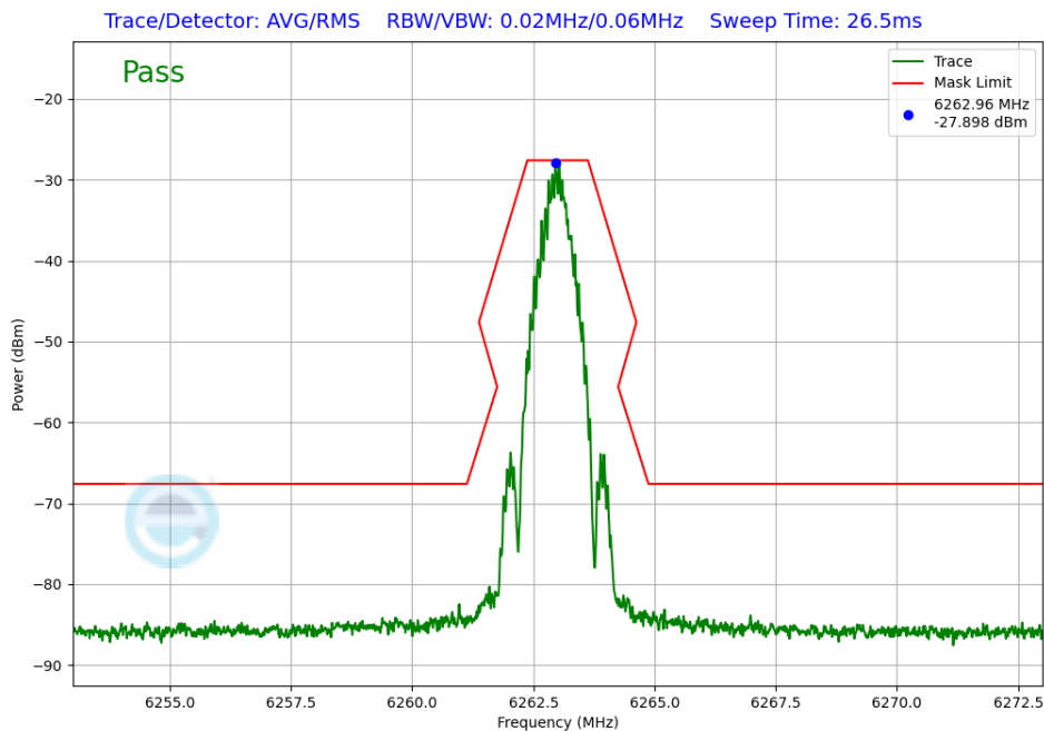
Plot 7-301. In-Band Emission TxBF Primary Antenna 3b (NB UNII BDR, ePA – 6263MHz)
