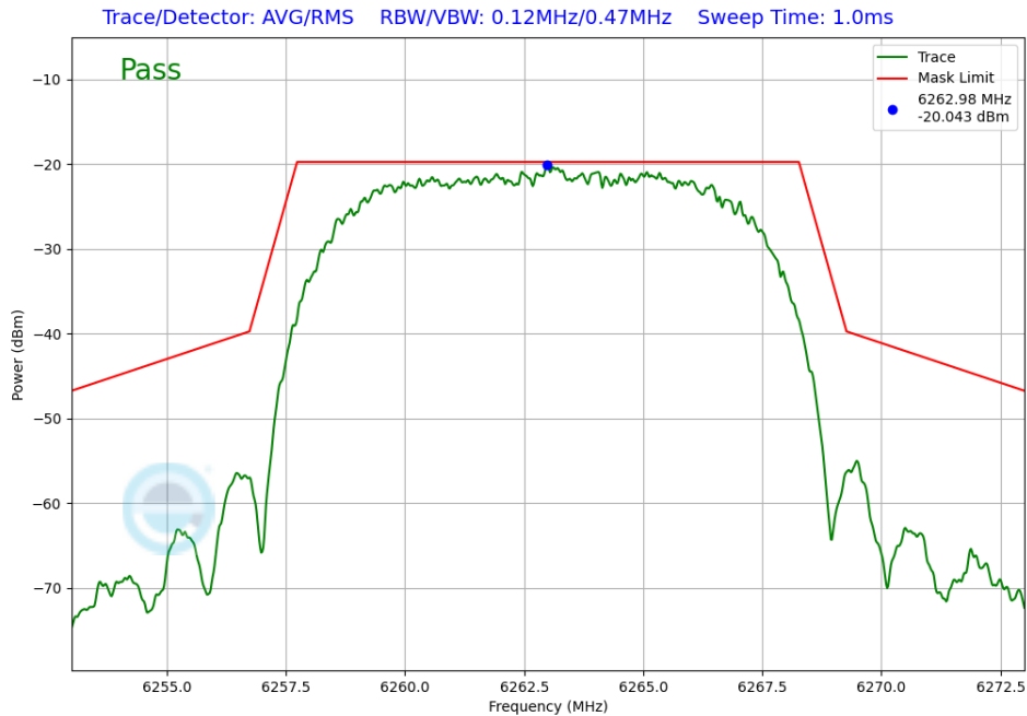
Plot 7-267. In-Band Emission Antenna 3b (NB UNII HDRPL32, iPA – 6263MHz)
