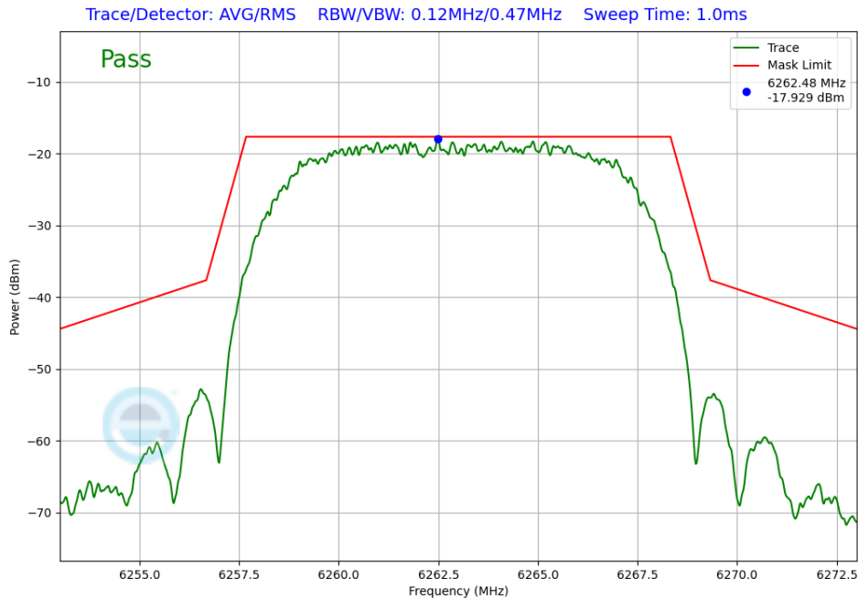
Plot 7-265. In-Band Emission Antenna 3b (NB UNII HDRPL12, iPA – 6263MHz)
