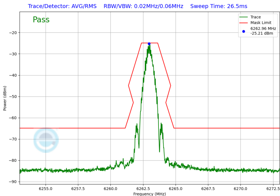
Plot 7-300. In-Band Emission TxBF Primary Antenna 5T (NB UNII BDR, ePA – 6263MHz)
