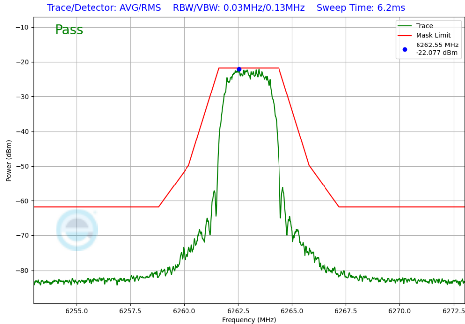
Plot 7-273. In-Band Emission Antenna 3b (NB UNII HDT6, iPA – 6263MHz)
