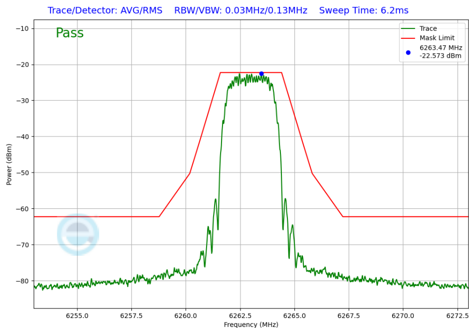
Plot 7-270. In-Band Emission Antenna 3b (NB UNII HDT4, ePA – 6263MHz)
