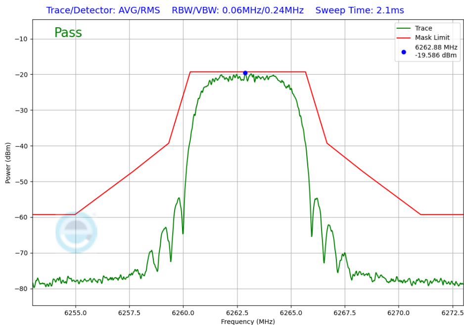
Plot 7-262. In-Band Emission Antenna 3b (NB UNII HDRPM16, ePA – 6263MHz)
