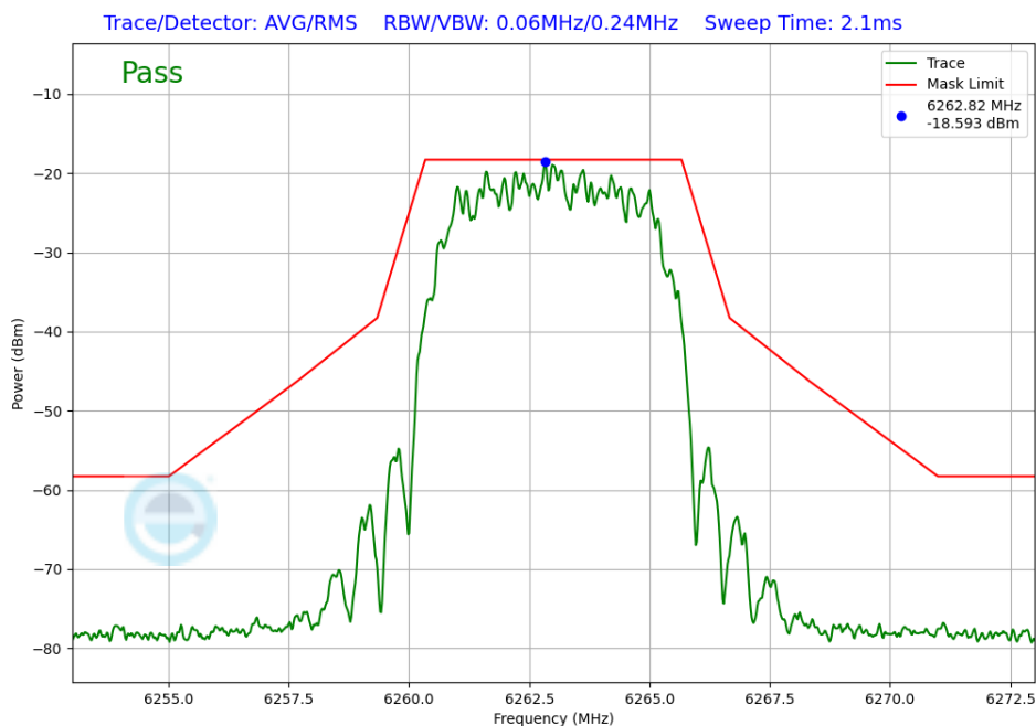
Plot 7-256. In-Band Emission Antenna 3b (NB UNII HDR8, ePA – 6263MHz)
