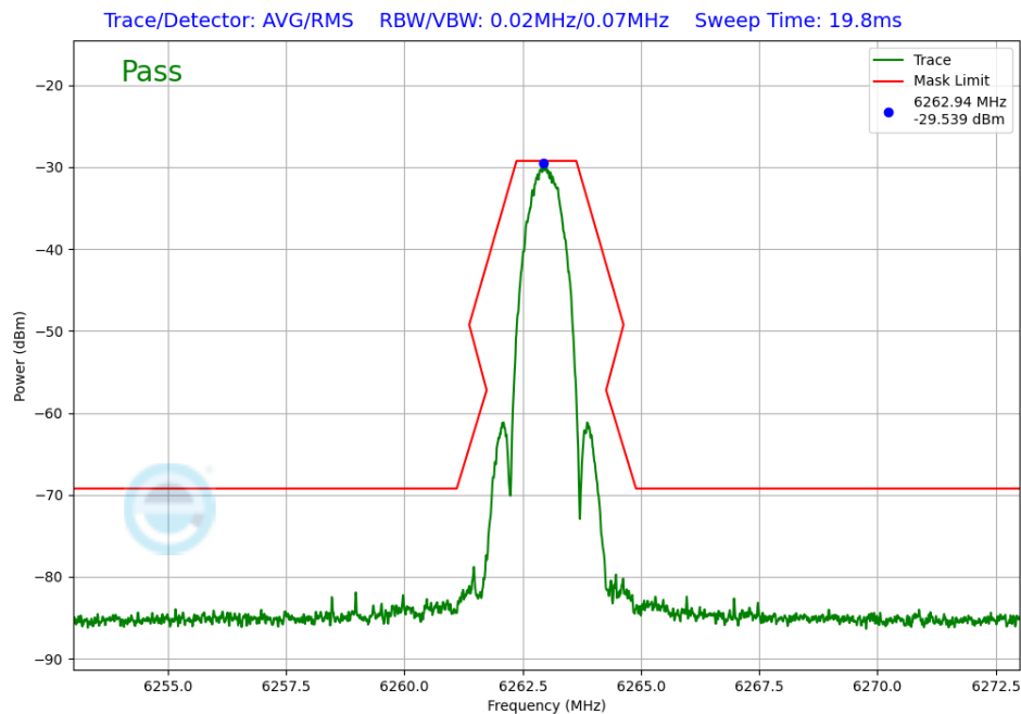
Plot 7-305. In-Band Emission TxBF Primary Antenna 3b (NB UNII LE1M, ePA – 6263MHz)
