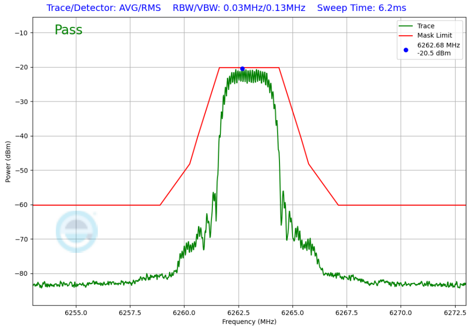
Plot 7-269. In-Band Emission Antenna 3b (NB UNII HDT2, iPA – 6263MHz)
