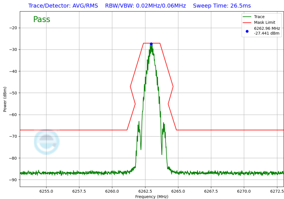
Plot 7-303. In-Band Emission TxBF Primary Antenna 3b (NB UNII BDR, iPA – 6263MHz)
