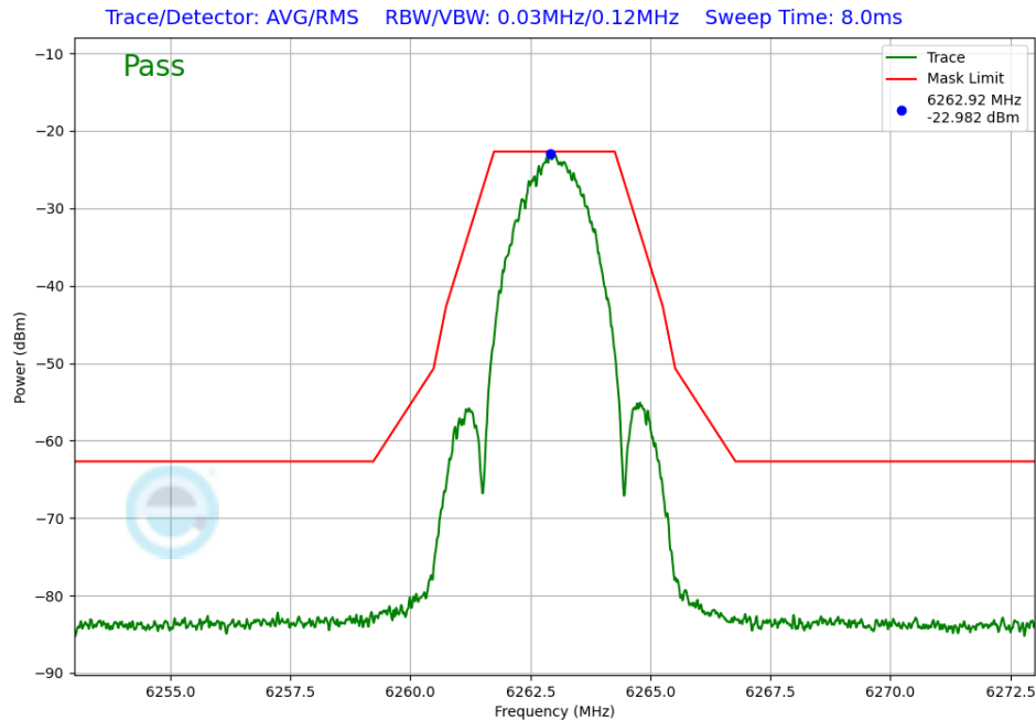
Plot 7-253. In-Band Emission Antenna 3b (NB UNII LE2M, iPA – 6263MHz)
