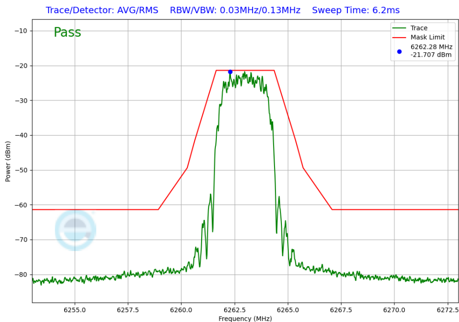
Plot 7-254. In-Band Emission Antenna 3b (NB UNII HDR4, ePA – 6263MHz)
