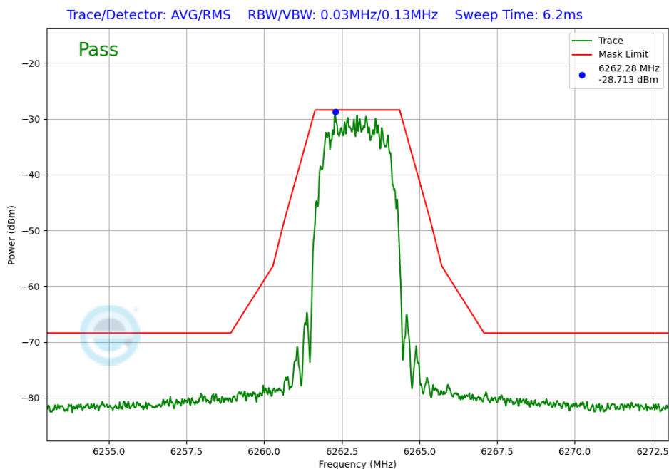
Plot 7-364. In-Band Emission TxBF Diversity Antenna 5T (NB UNII HDR4, ePA – 6263MHz)
