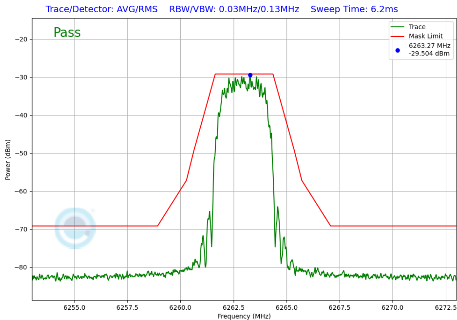
Plot 7-313. In-Band Emission TxBF Primary Antenna 3b (NB UNII HDR4, ePA – 6263MHz)
