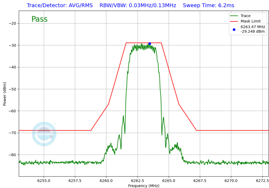
Plot 7-347. In-Band Emission TxBF Primary Antenna 3b (NB UNII HDT4, iPA – 6263MHz)
