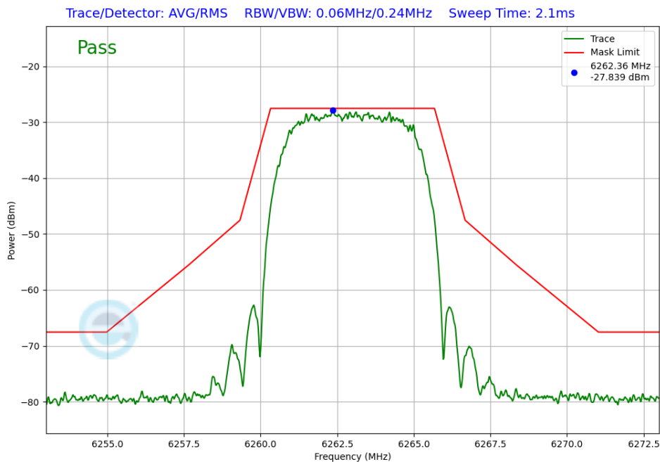
Plot 7-329. In-Band Emission TxBF Primary Antenna 3b (NB UNII HDRPM16, ePA – 6263MHz)
