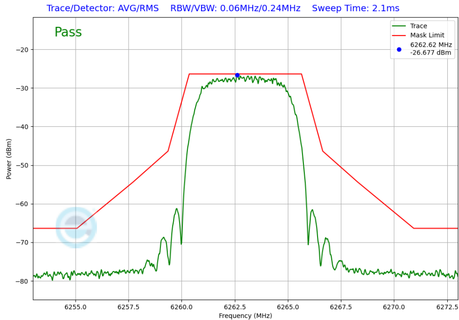
Plot 7-380. In-Band Emission Tx BF Diversity Antenna 5T (NB UNII HDRPM16, ePA – 6263MHz)
