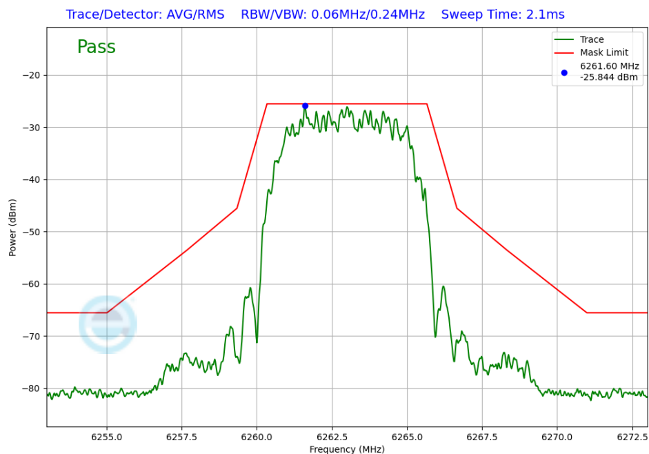
Plot 7-318. In-Band Emission TxBF Primary Antenna 5T (NB UNII HDR8, iPA – 6263MHz)
