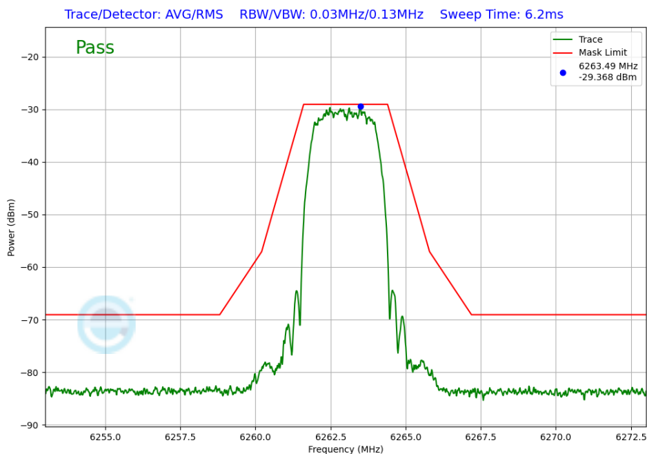
Plot 7-350. In-Band Emission TxBF Primary Antenna 5T (NB UNII HDT6, iPA – 6263MHz)
