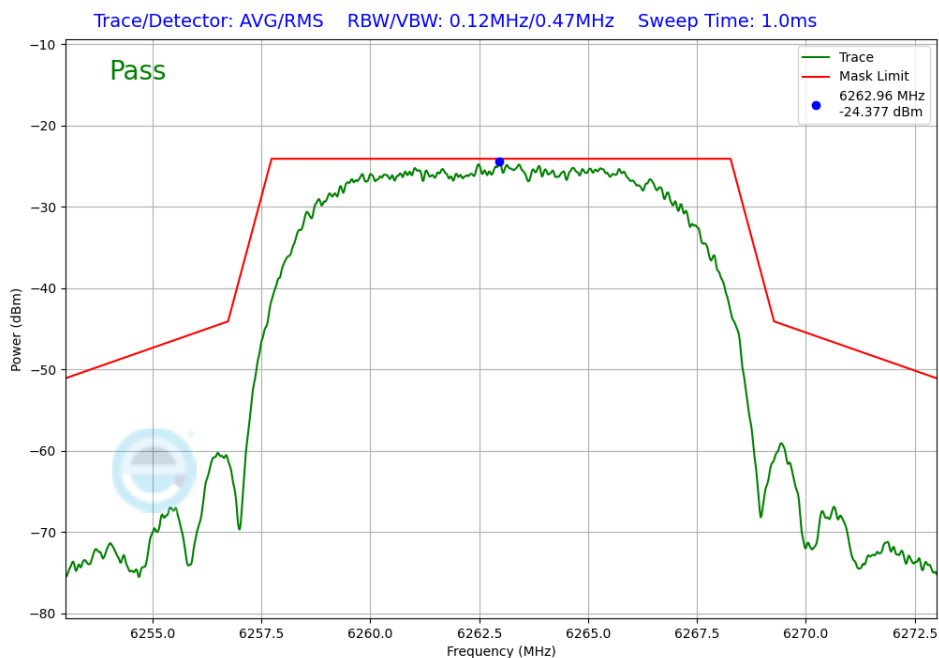
Plot 7-338. In-Band Emission TxBF Primary Antenna 5T (NB UNII HDRPL32, iPA – 6263MHz)
