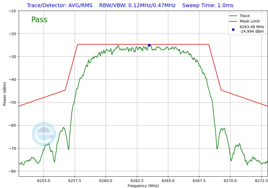
Plot 7-337. In-Band Emission TxBF Primary Antenna 3b (NB UNII HDRPL32, ePA – 6263MHz)
