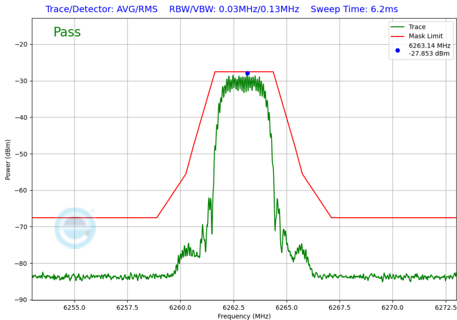
Plot 7-343. In-Band Emission TxBF Primary Antenna 3b (NB UNII HDT2, iPA – 6263MHz)
