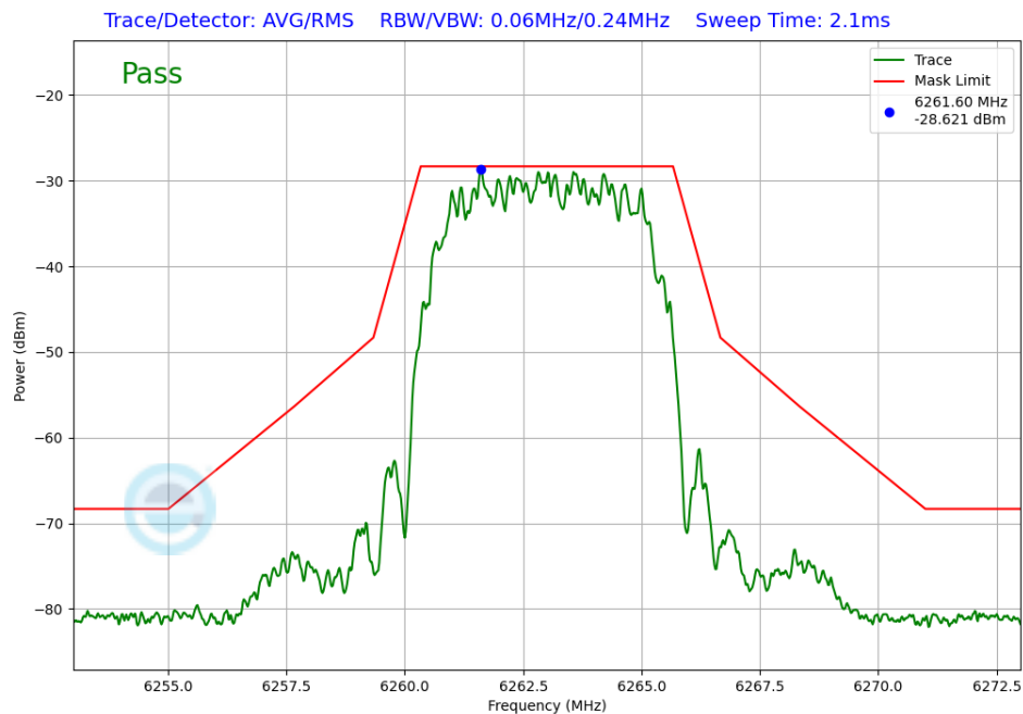
Plot 7-319. In-Band Emission TxBF Primary Antenna 3b (NB UNII HDR8, iPA – 6263MHz)
