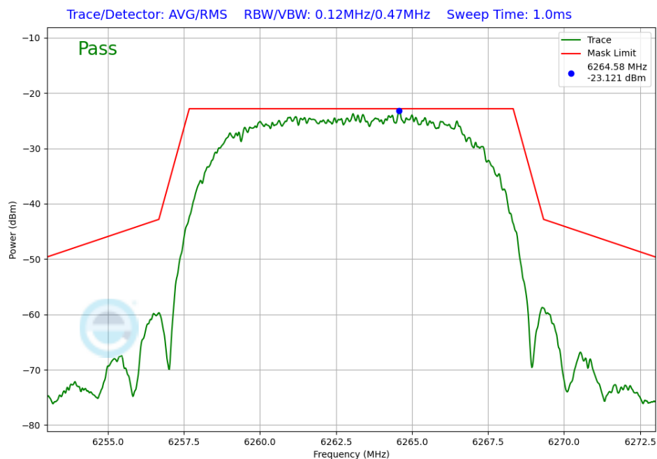
Plot 7-332. In-Band Emission TxBF Primary Antenna 5T (NB UNII HDRPL12, ePA – 6263MHz)
