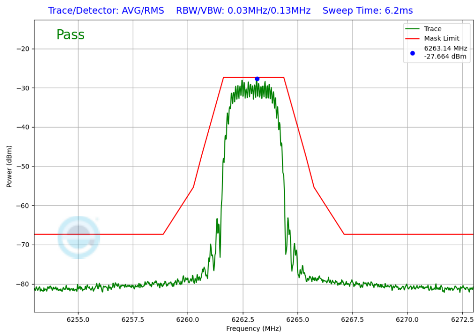
Plot 7-340. In-Band Emission TxBF Primary Antenna 5T (NB UNII HDT2, ePA – 6263MHz)
