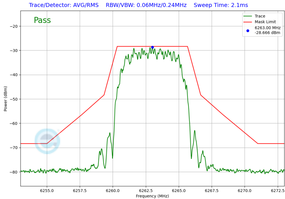
Plot 7-317. In-Band Emission TxBF Primary Antenna 3b (NB UNII HDR8, ePA – 6263MHz)
