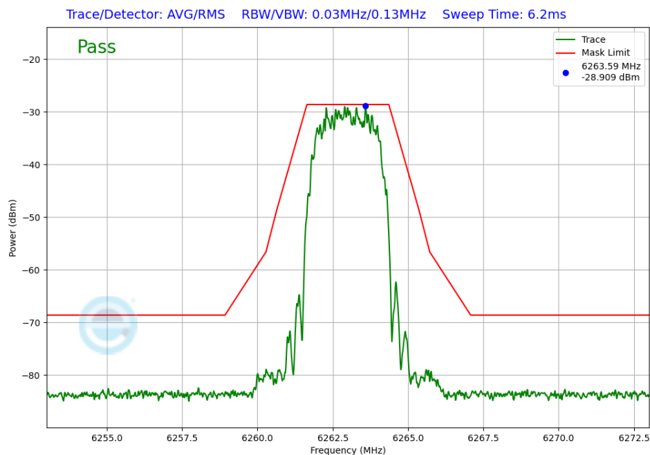
Plot 7-366. In-Band Emission Tx BF Diversity Antenna 5T (NB UNII HDR4, iPA – 6263MHz)
