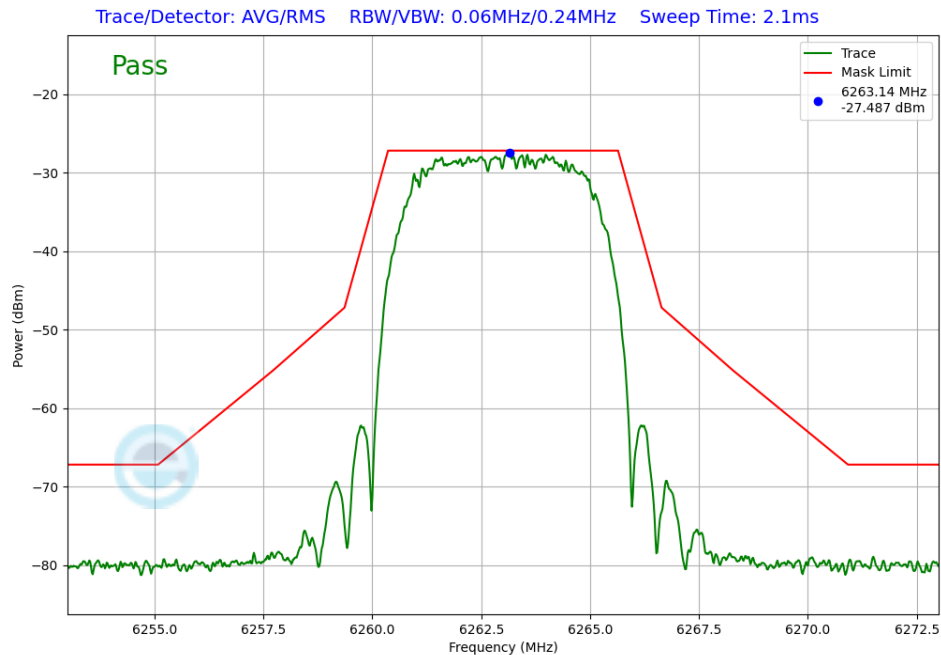
Plot 7-381. In-Band Emission Tx BF Diversity Antenna 1b (NB UNII HDRPM16, ePA – 6263MHz)
