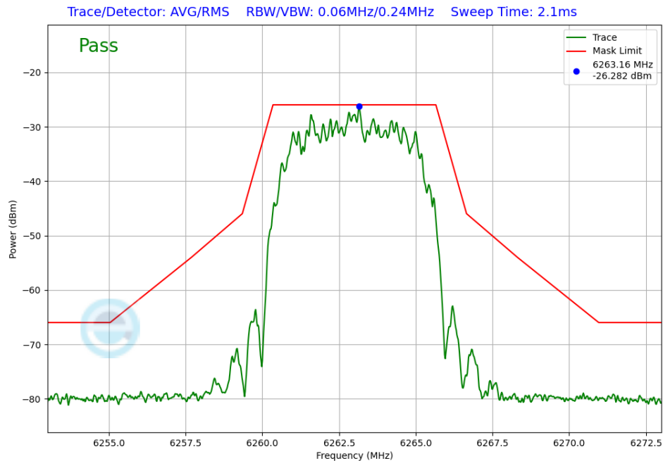
Plot 7-369. In-Band Emission TxBF Diversity Antenna 1b (NB UNII HDR8, ePA – 6263MHz)
