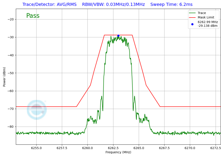
Plot 7-367. In-Band Emission Tx BF Diversity Antenna 1b (NB UNII HDR4, iPA – 6263MHz)
