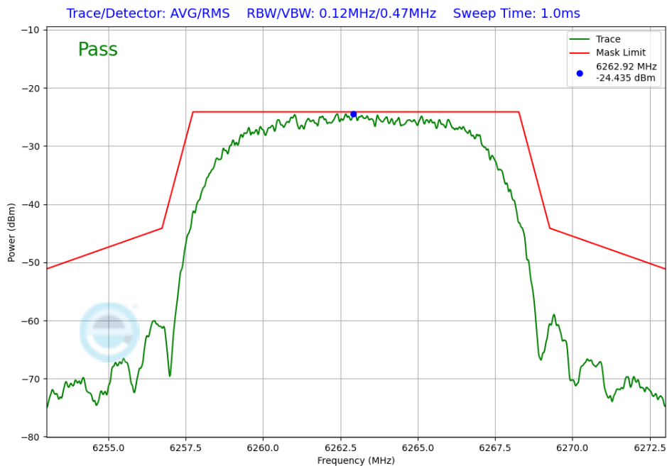
Plot 7-339. In-Band Emission TxBF Primary Antenna 3b (NB UNII HDRPL32, iPA – 6263MHz)
