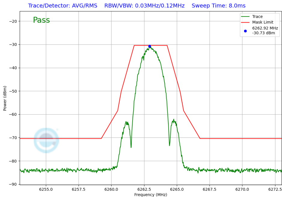
Plot 7-363. In-Band Emission TxBF Diversity Antenna 1b (NB UNII LE2M, iPA – 6263MHz)
