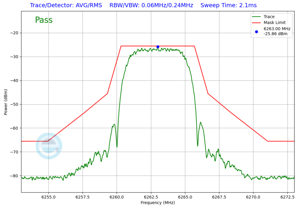
Plot 7-326. In-Band Emission Tx BF Primary Antenna 5T (NB UNII XHDRPM6, iPA – 6263MHz)
