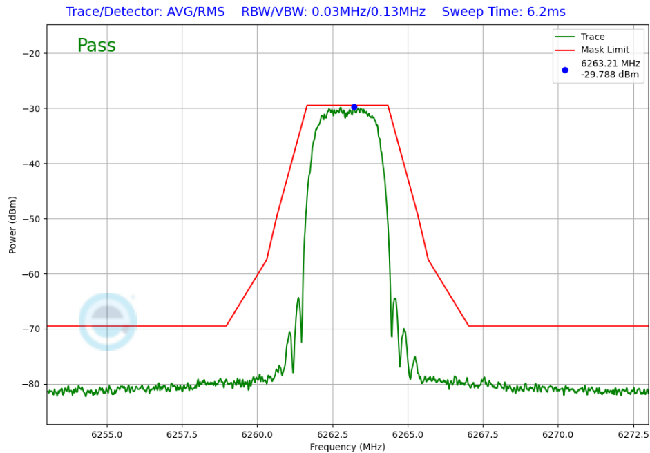
Plot 7-320. In-Band Emission TxBF Primary Antenna 5T (NB UNII HDRPS2, ePA – 6263MHz)
