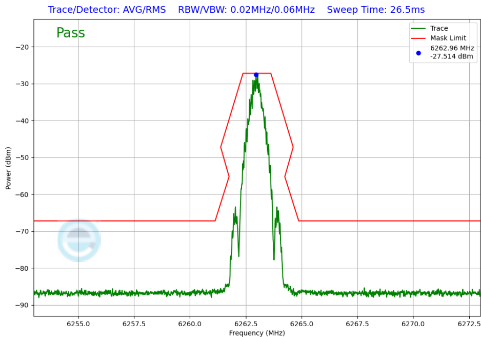
Plot 7-355. In-Band Emission Tx BF Diversity Antenna 1b (NB UNII BDR, iPA – 6263MHz)
