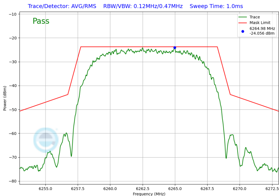
Plot 7-336. In-Band Emission TxBF Primary Antenna 5T (NB UNII HDRPL32, ePA – 6263MHz)
