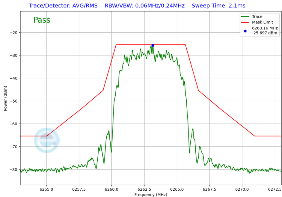
Plot 7-371. In-Band Emission TxBF Diversity Antenna 1b (NB UNII HDR8, iPA – 6263MHz)
