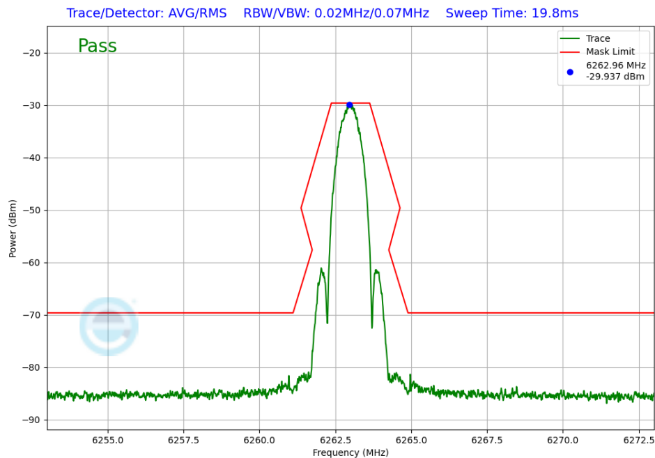
Plot 7-357. In-Band Emission TxBF Diversity Antenna 1b (NB UNII LE1M, ePA – 6263MHz)
