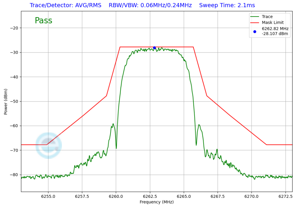
Plot 7-327. In-Band Emission Tx BF Primary Antenna 3b (NB UNII XHDRPM6, iPA – 6263MHz)
