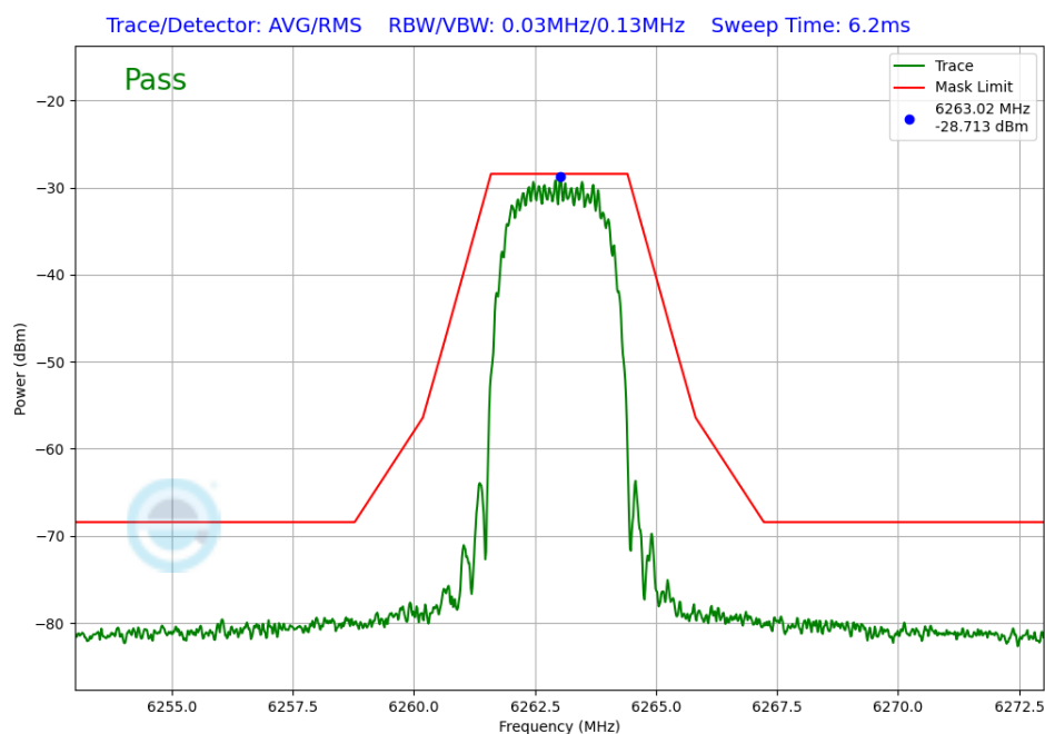
Plot 7-344. In-Band Emission TxBF Primary Antenna 5T (NB UNII HDT4, ePA – 6263MHz)
