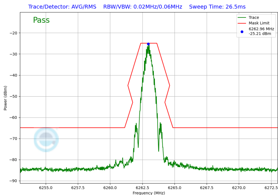
Plot 7-352. In-Band Emission TxBF Diversity Antenna 5T (NB UNII BDR, ePA – 6263MHz)
