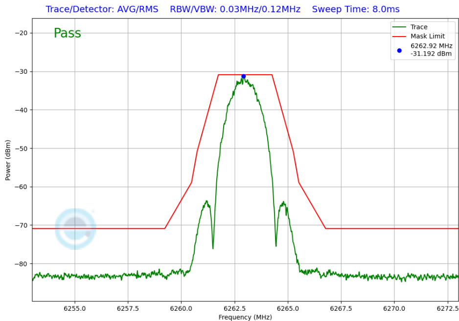
Plot 7-361. In-Band Emission TxBF Diversity Antenna 1b (NB UNII LE2M, ePA – 6263MHz)
