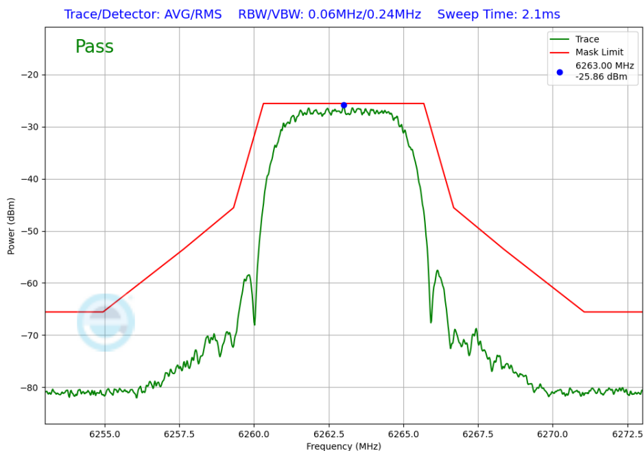
Plot 7-378. In-Band Emission TxBF Diversity Antenna 5T (NB UNII XHDRPM6, iPA – 6263MHz)
