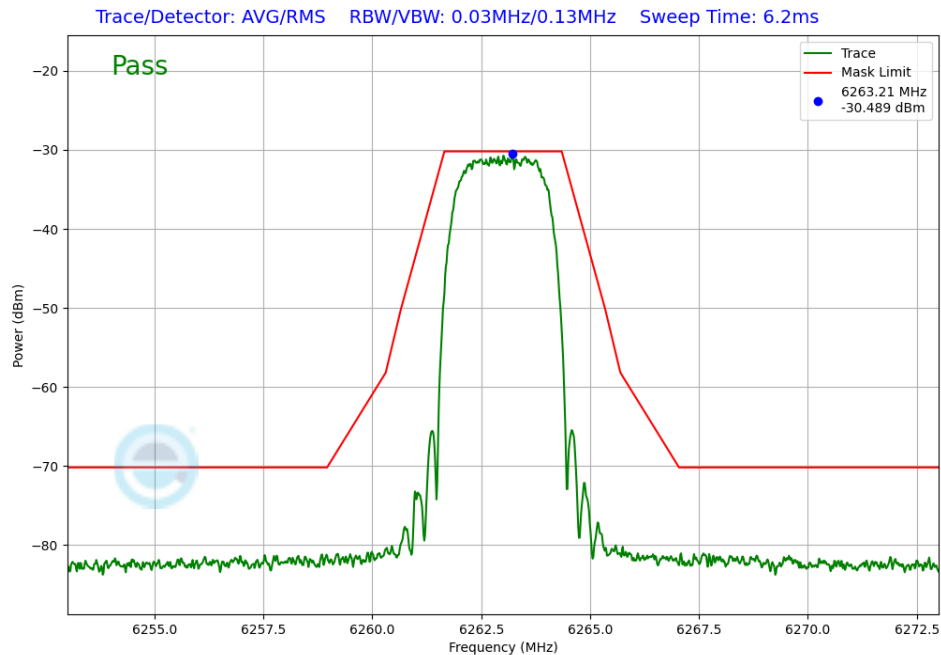
Plot 7-321. In-Band Emission TxBF Primary Antenna 3b (NB UNII HDRPS2, ePA – 6263MHz)
