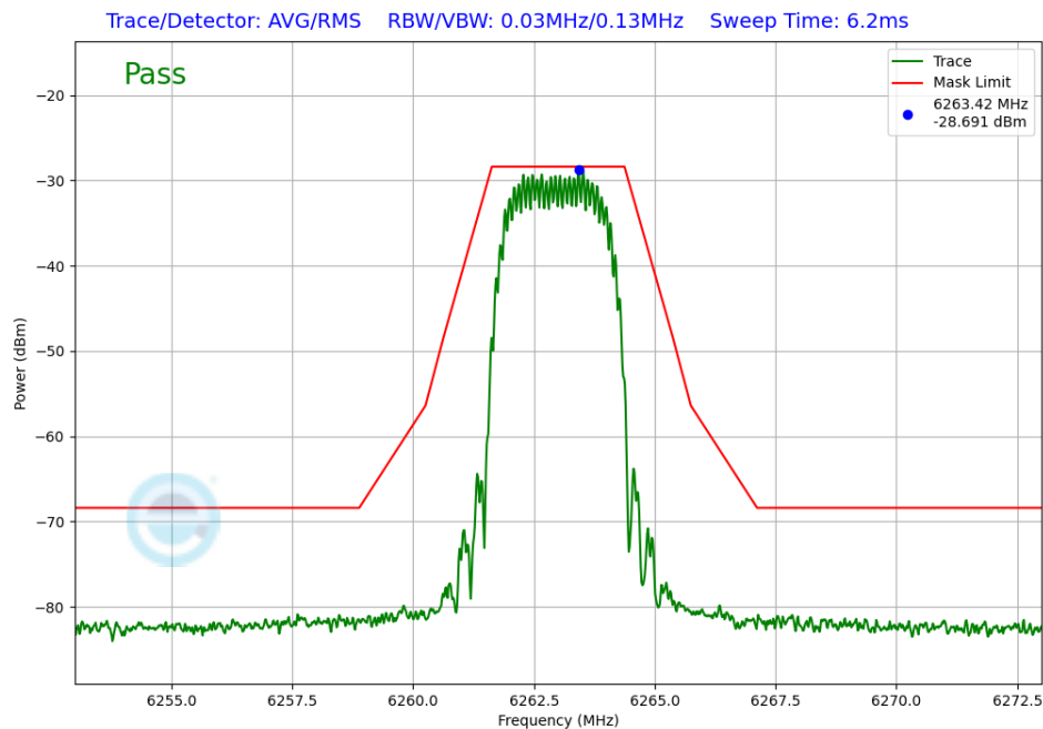
Plot 7-341. In-Band Emission TxBF Primary Antenna 3b (NB UNII HDT2, ePA – 6263MHz)
