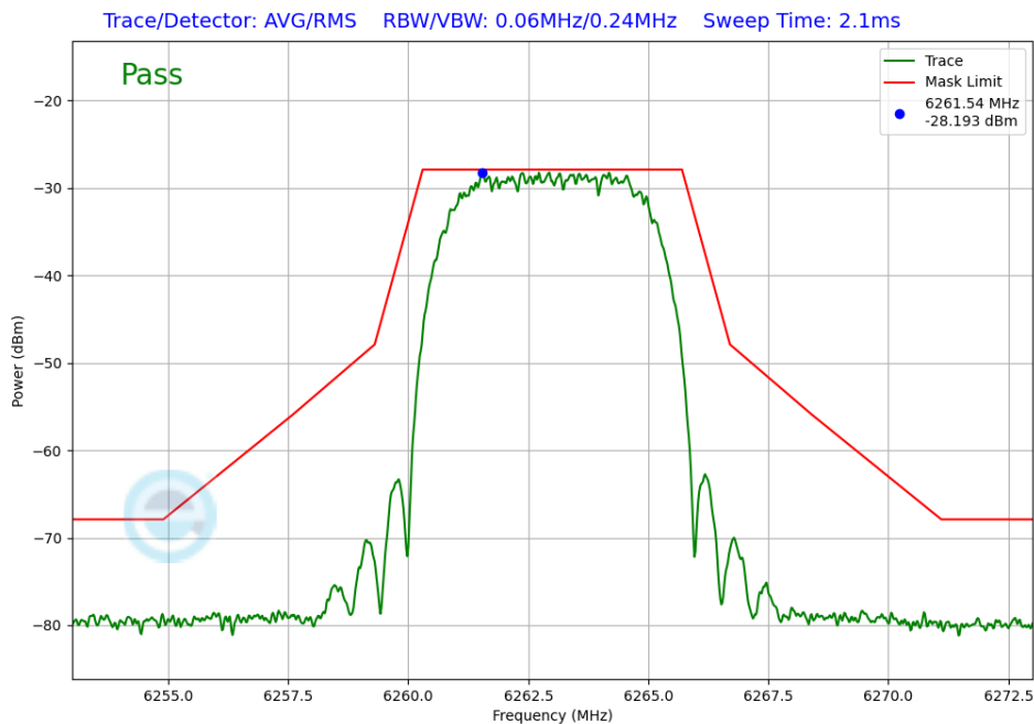
Plot 7-325. In-Band Emission TxBF Primary Antenna 3b (NB UNII XHDRPM6, ePA – 6263MHz)
