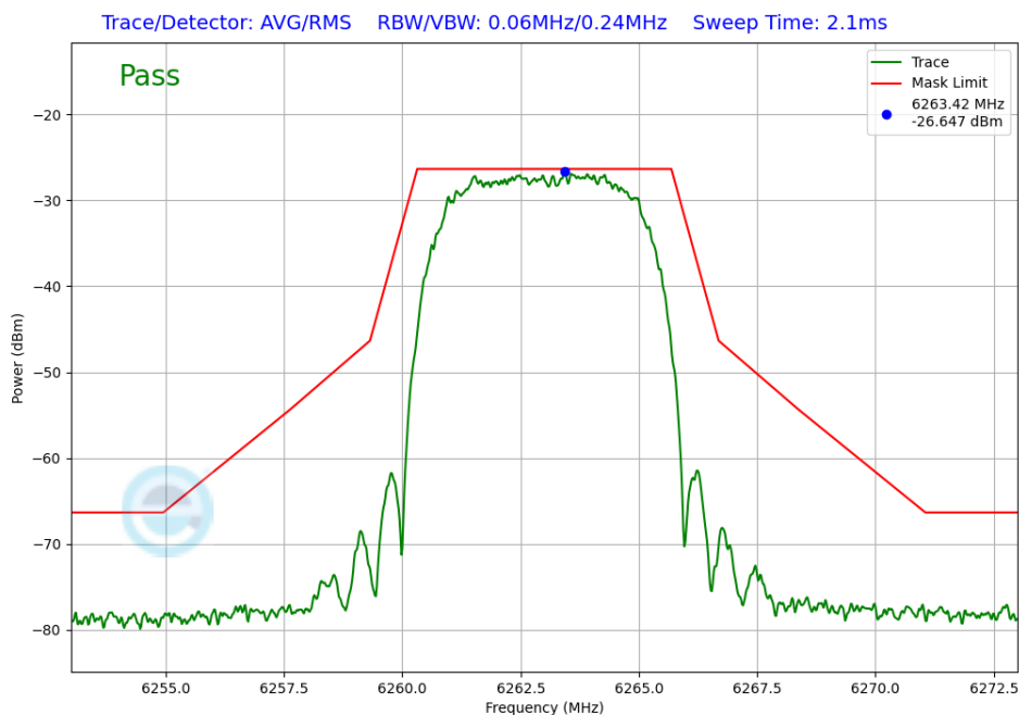
Plot 7-324. In-Band Emission TxBF Primary Antenna 5T (NB UNII XHDRPM6, ePA – 6263MHz)
