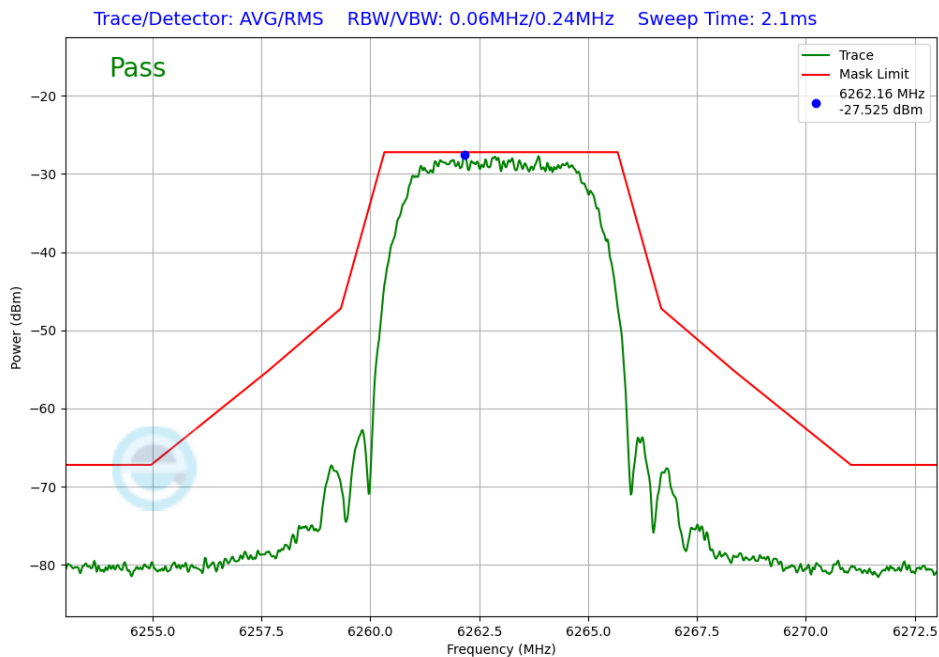
Plot 7-379. In-Band Emission TxBF Diversity Antenna 1b (NB UNII XHDRPM6, iPA – 6263MHz)
