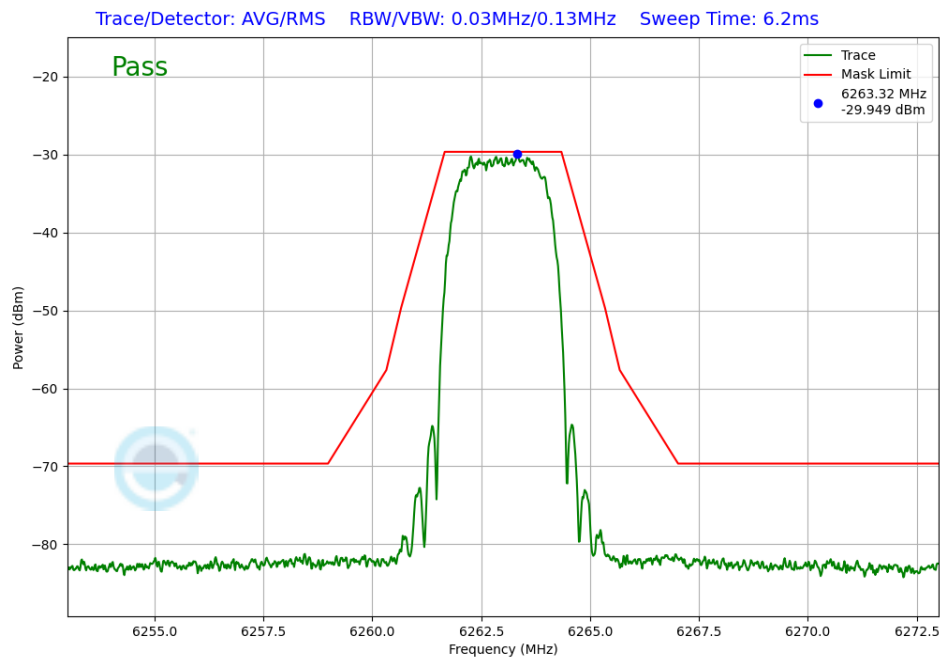
Plot 7-373. In-Band Emission Tx BF Diversity Antenna 1b (NB UNII HDRPS2, ePA – 6263MHz)
