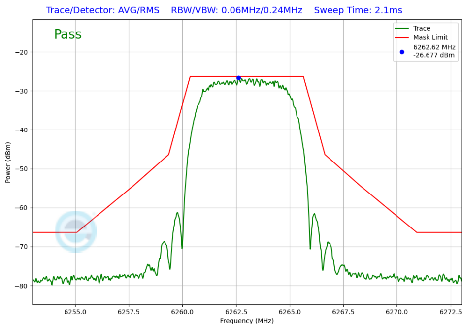
Plot 7-328. In-Band Emission TxBF Primary Antenna 5T (NB UNII HDRPM16, ePA – 6263MHz)
