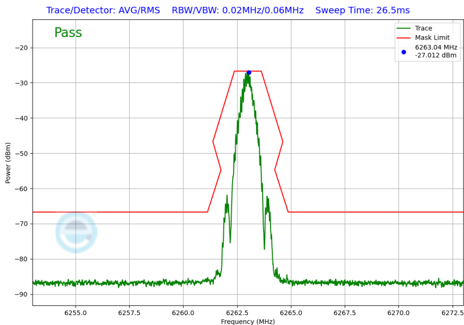
Plot 7-354. In-Band Emission Tx BF Diversity Antenna 5T (NB UNII BDR, iPA – 6263MHz)
