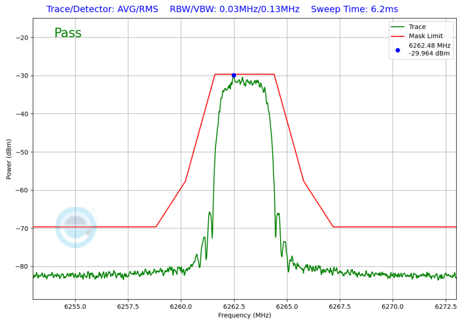
Plot 7-349. In-Band Emission TxBF Primary Antenna 3b (NB UNII HDT6, ePA – 6263MHz)
