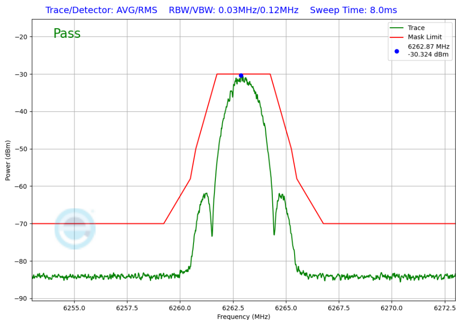
Plot 7-362. In-Band Emission TxBF Diversity Antenna 5T (NB UNII LE2M, iPA – 6263MHz)
