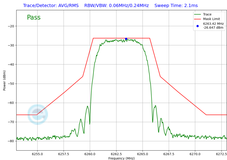
Plot 7-376. In-Band Emission TxBF Diversity Antenna 5T (NB UNII XHDRPM6, ePA – 6263MHz)
