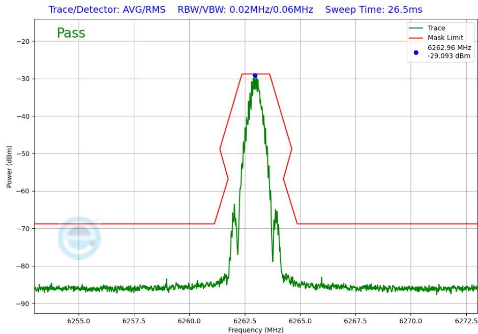
Plot 7-353. In-Band Emission TxBF Diversity Antenna 1b (NB UNII BDR, ePA – 6263MHz)
