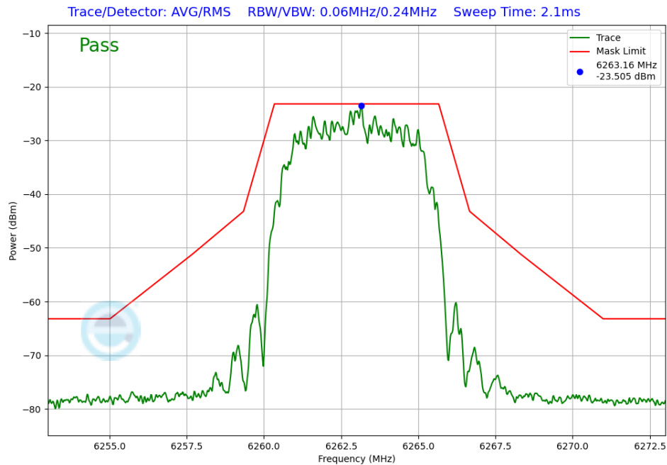
Plot 7-368. In-Band Emission TxBF Diversity Antenna 5T (NB UNII HDR8, ePA – 6263MHz)
