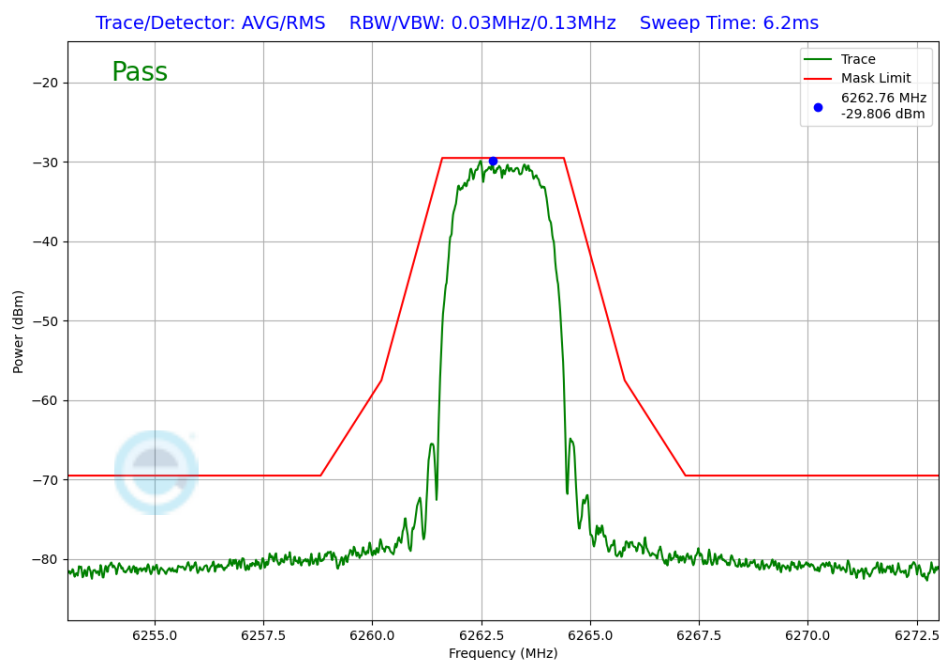
Plot 7-348. In-Band Emission TxBF Primary Antenna 5T (NB UNII HDT6, ePA – 6263MHz)
