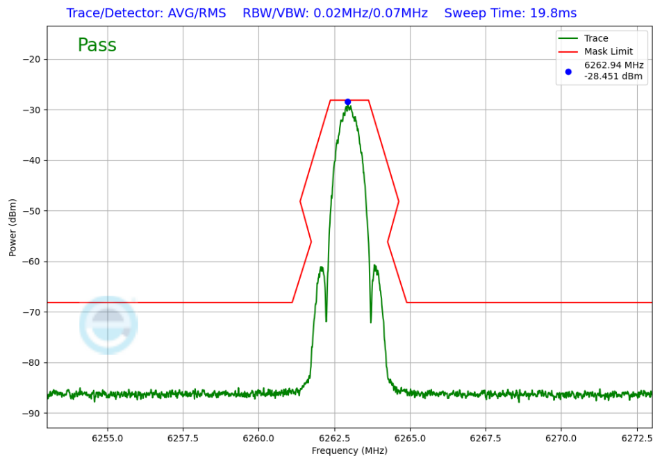
Plot 7-359. In-Band Emission TxBF Diversity Antenna 1b (NB UNII LE1M, iPA – 6263MHz)
