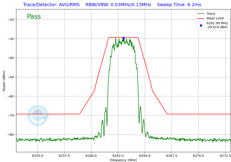
Plot 7-365. In-Band Emission TxBF Diversity Antenna 1b (NB UNII HDR4, ePA – 6263MHz)
