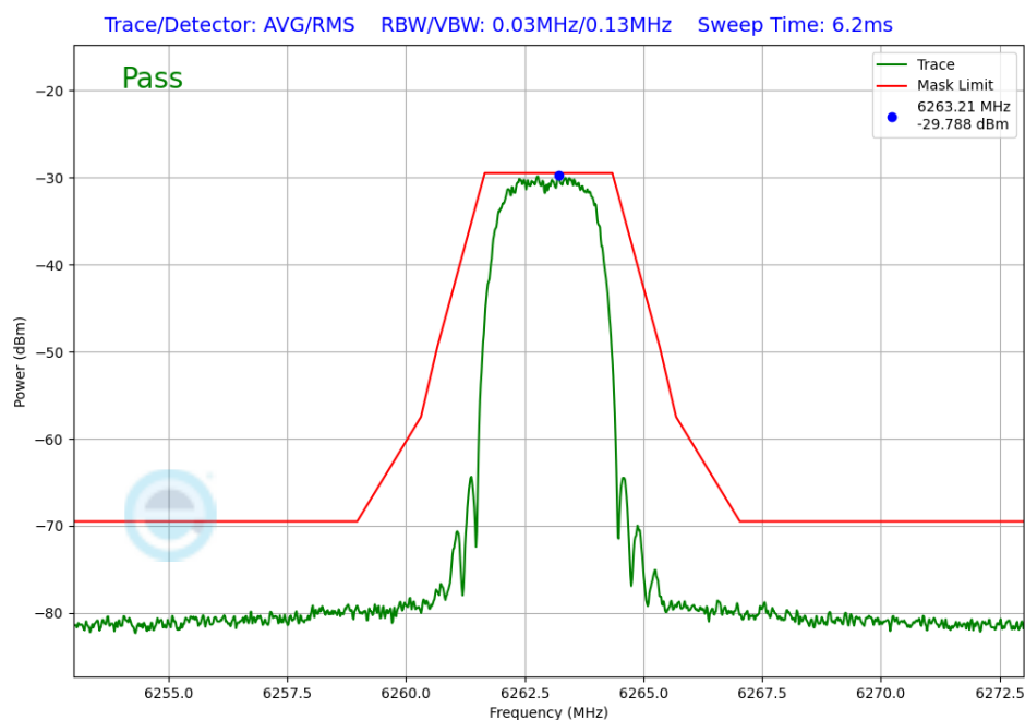
Plot 7-372. In-Band Emission Tx BF Diversity Antenna 5T (NB UNII HDRPS2, ePA – 6263MHz)
