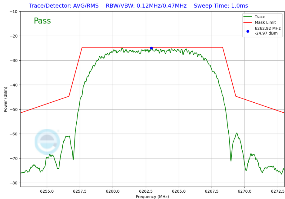
Plot 7-333. In-Band Emission TxBF Primary Antenna 3b (NB UNII HDRPL12, ePA – 6263MHz)
