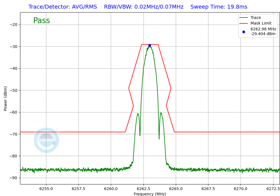
Plot 7-358. In-Band Emission TxBF Diversity Antenna 5T (NB UNII LE1M, iPA – 6263MHz)
