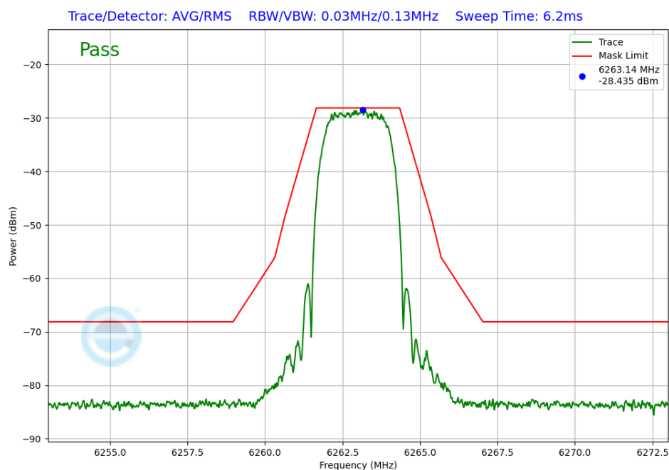
Plot 7-322. In-Band Emission TxBF Primary Antenna 5T (NB UNII HDRPS2, iPA – 6263MHz)
