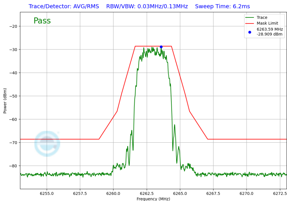
Plot 7-314. In-Band Emission TxBF Primary Antenna 5T (NB UNII HDR4, iPA – 6263MHz)
