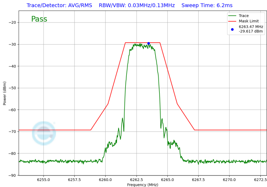
Plot 7-351. In-Band Emission TxBF Primary Antenna 3b (NB UNII HDT6, iPA – 6263MHz)
