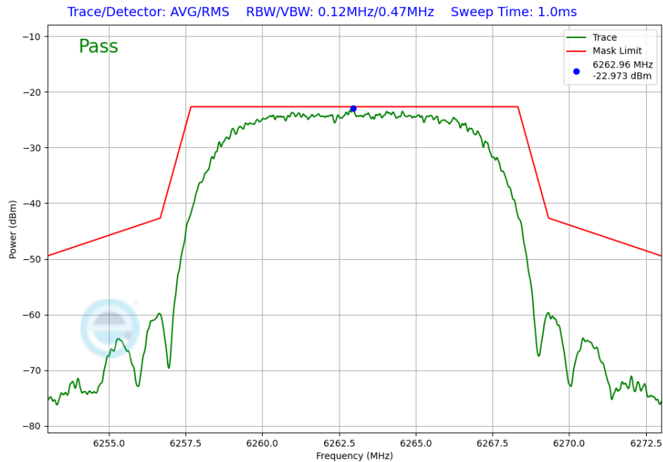
Plot 7-334. In-Band Emission TxBF Primary Antenna 5T (NB UNII HDRPL12, iPA – 6263MHz)
