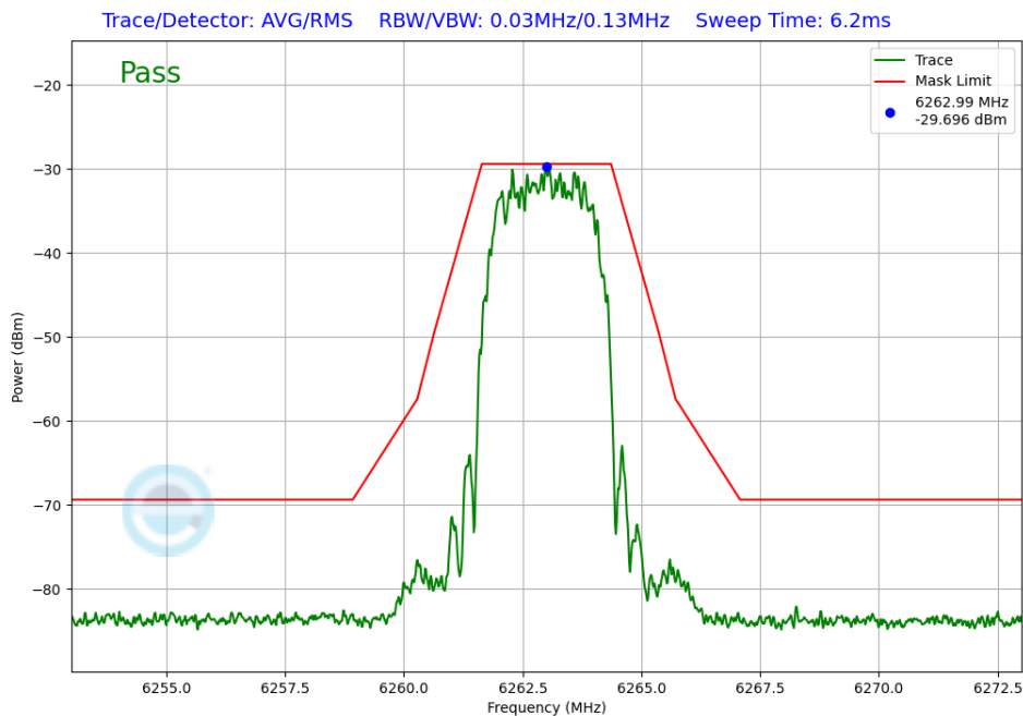
Plot 7-315. In-Band Emission TxBF Primary Antenna 3b (NB UNII HDR4, iPA – 6263MHz)
