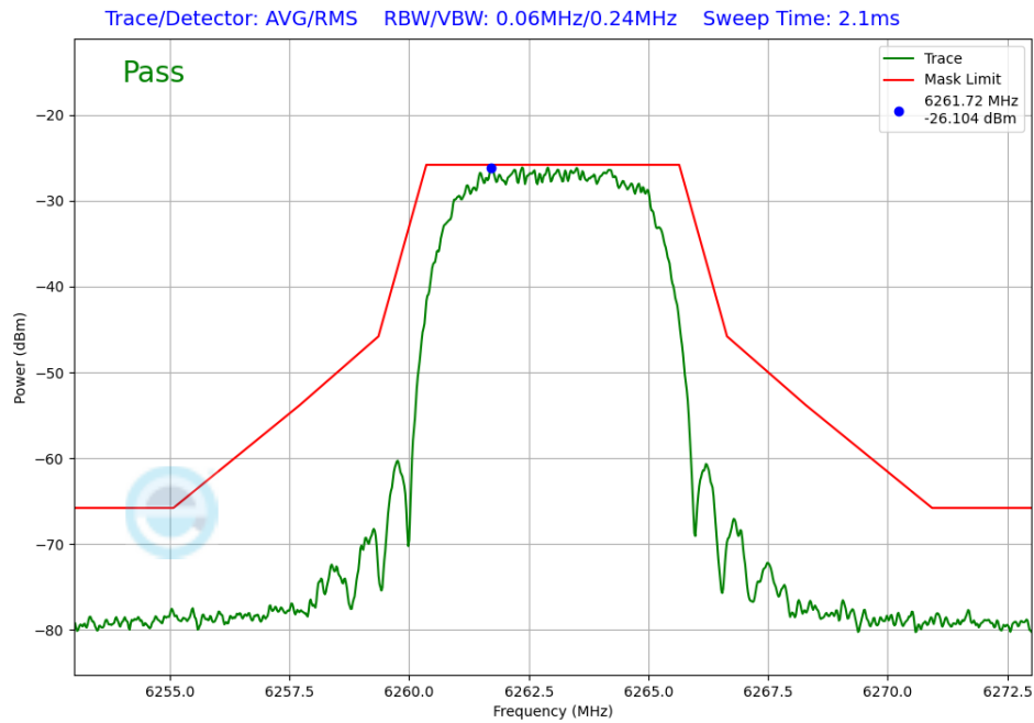
Plot 7-330. In-Band Emission TxBF Primary Antenna 5T (NB UNII HDRPM16, iPA – 6263MHz)
