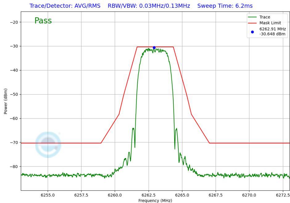
Plot 7-323. In-Band Emission TxBF Primary Antenna 3b (NB UNII HDRPS2, iPA – 6263MHz)
