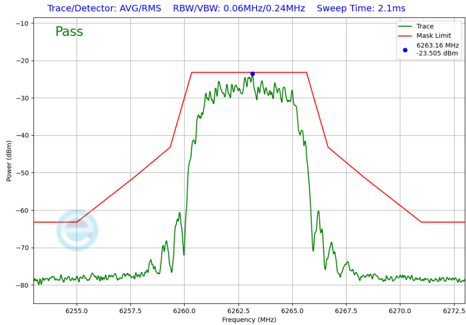
Plot 7-316. In-Band Emission TxBF Primary Antenna 5T (NB UNII HDR8, ePA – 6263MHz)
