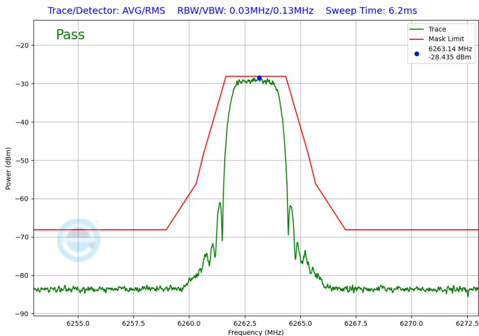
Plot 7-374. In-Band Emission TxBF Diversity Antenna 5T (NB UNII HDRPS2, iPA – 6263MHz)
