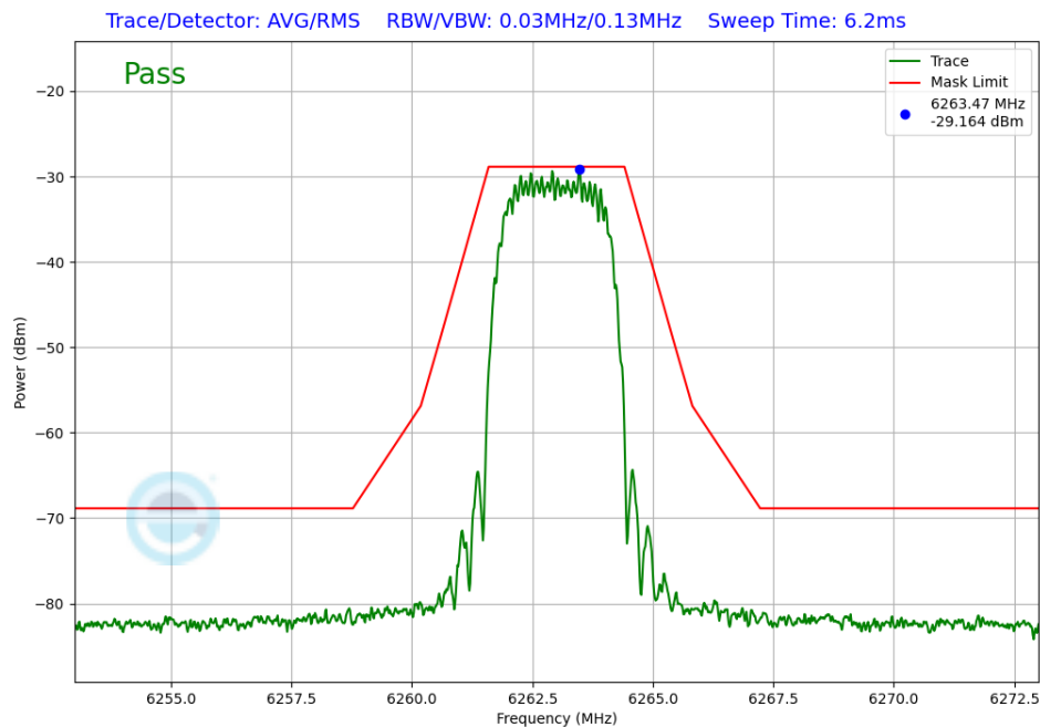
Plot 7-345. In-Band Emission TxBF Primary Antenna 3b (NB UNII HDT4, ePA – 6263MHz)
