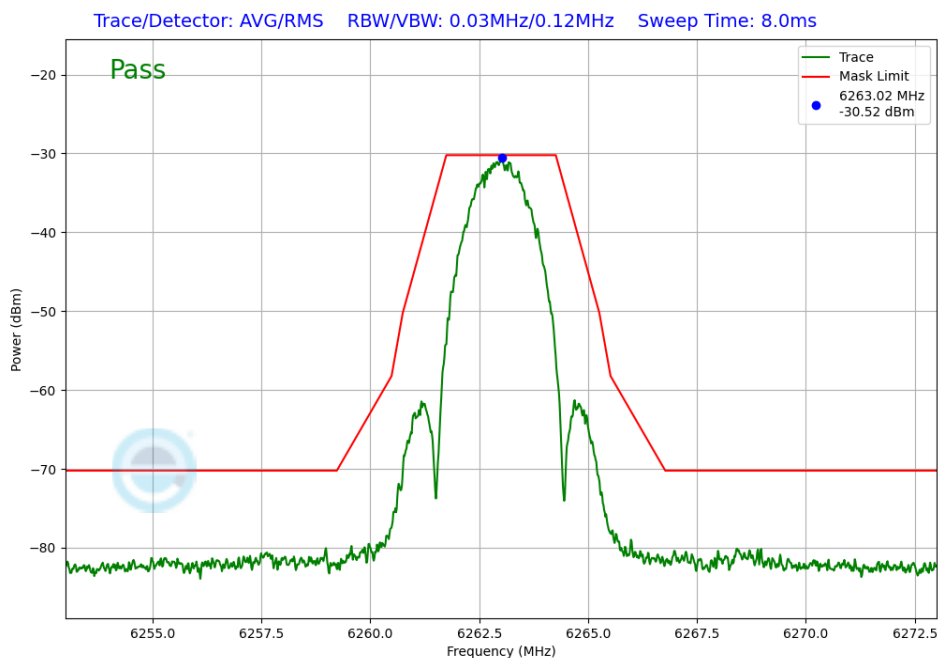
Plot 7-360. In-Band Emission TxBF Diversity Antenna 5T (NB UNII LE2M, ePA – 6263MHz)
