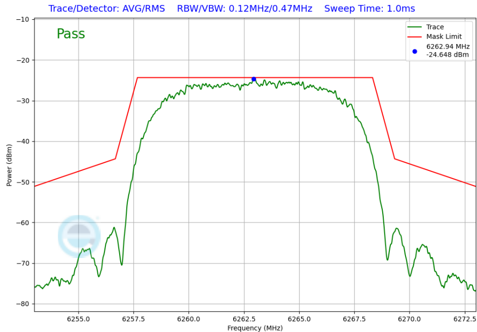
Plot 7-335. In-Band Emission TxBF Primary Antenna 3b (NB UNII HDRPL12, iPA – 6263MHz)
