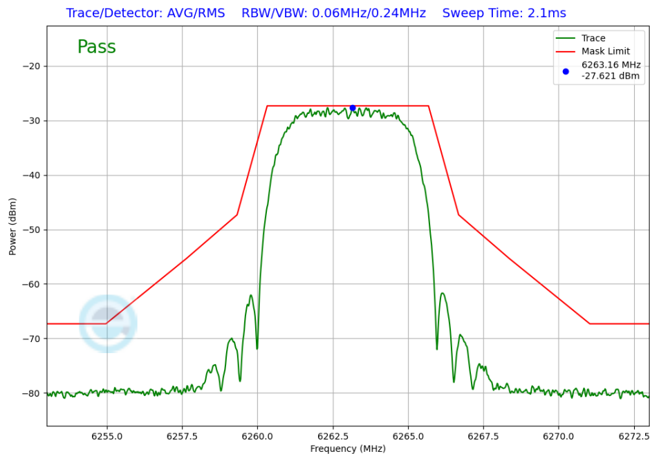
Plot 7-377. In-Band Emission TxBF Diversity Antenna 1b (NB UNII XHDRPM6, ePA – 6263MHz)
