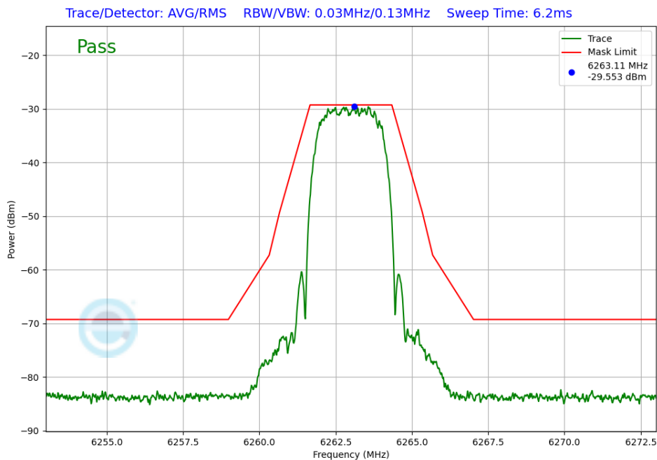
Plot 7-375. In-Band Emission TxBF Diversity Antenna 1b (NB UNII HDRPS2, iPA – 6263MHz)
