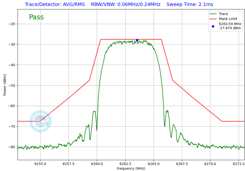
Plot 7-331. In-Band Emission TxBF Primary Antenna 3b (NB UNII HDRPM16, iPA – 6263MHz)
