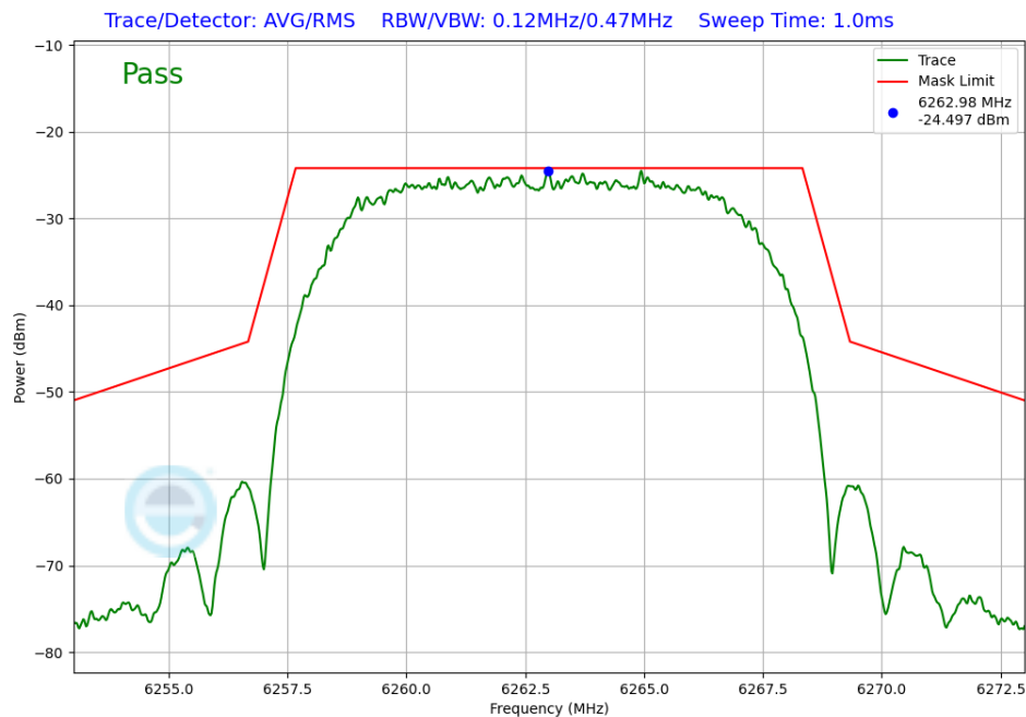
Plot 7-385. In-Band Emission TxBF Diversity Antenna 1b (NB UNII HDRPL12, ePA – 6263MHz)
