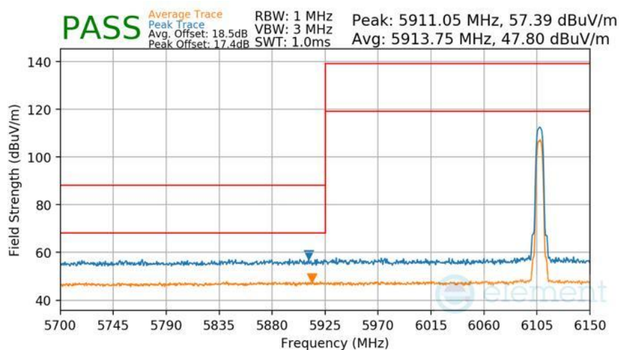
Plot 7-439 Radiated Lower Band Edge Measurement Antenna 5T
