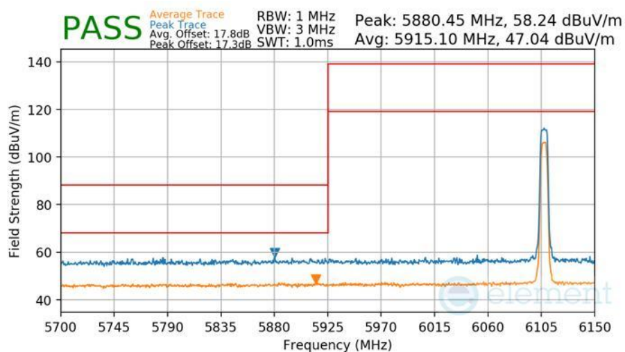
Plot 7-441 Radiated Lower Band Edge Measurement Antenna 5T
