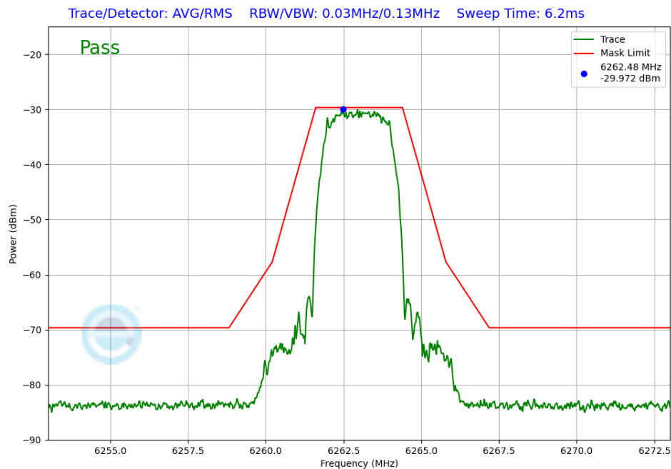
Plot 7-403. In-Band Emission TxBF Diversity Antenna 1b (NB UNII HDT6, iPA – 6263MHz)
