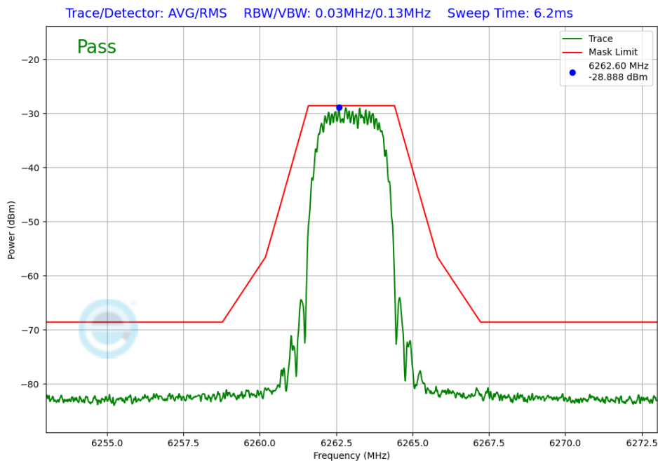
Plot 7-397. In-Band Emission TxBF Diversity Antenna 1b (NB UNII HDT4, ePA – 6263MHz)
