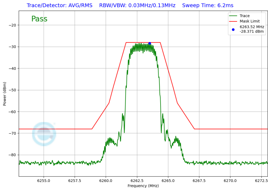
Plot 7-395. In-Band Emission TxBF Diversity Antenna 1b (NB UNII HDT2, iPA – 6263MHz)
