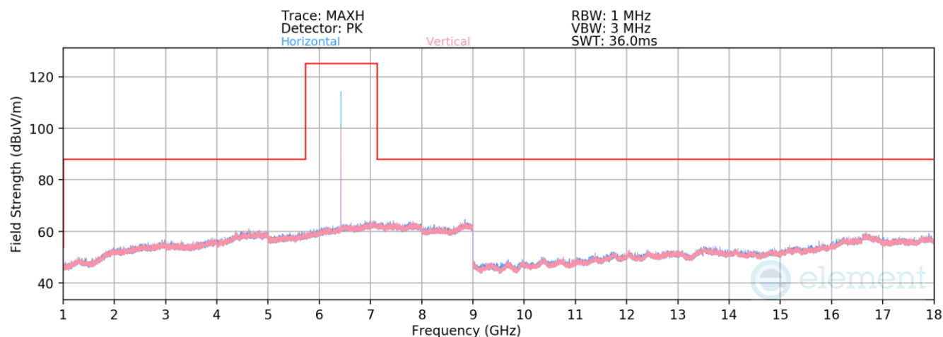
Plot 7-430. Radiated Spurious Emissions 1-18GHz TxBF Diversity (HDR4 ePA – 6420MHz)
