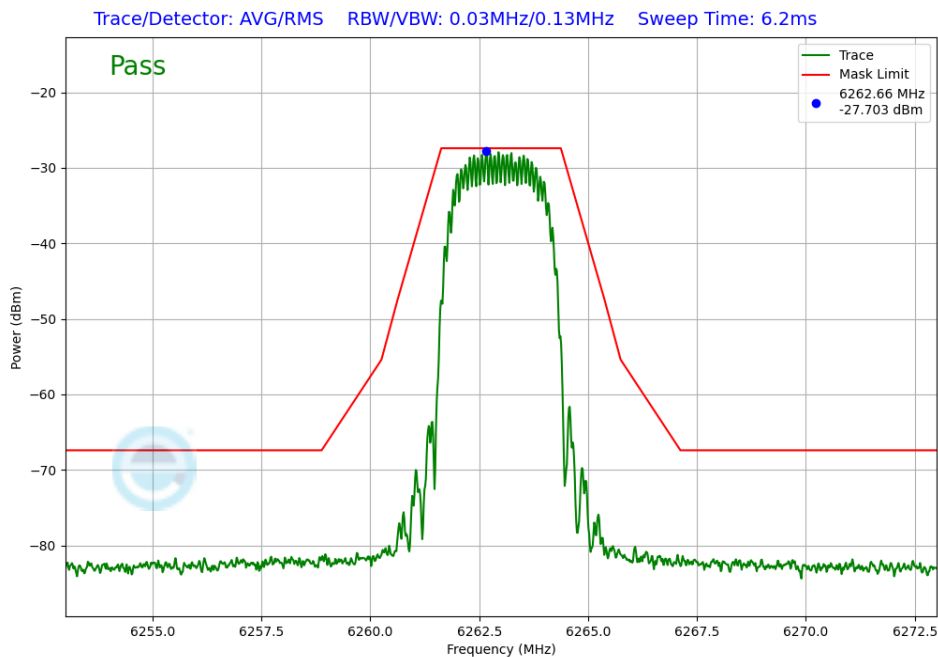
Plot 7-393. In-Band Emission TxBF Diversity Antenna 1b (NB UNII HDT2, ePA – 6263MHz)
