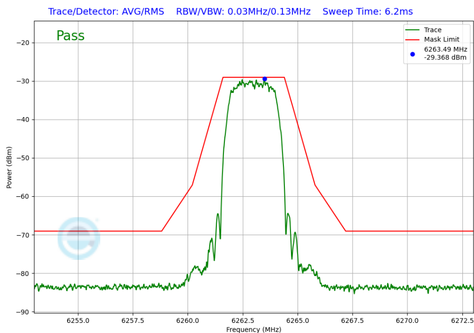
Plot 7-402. In-Band Emission TxBF Diversity Antenna 5T (NB UNII HDT6, iPA – 6263MHz)
