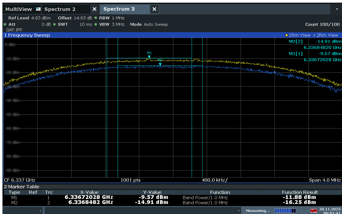
Plot 7-410. Power Density Plot – 6337MHz Antenna 5T
