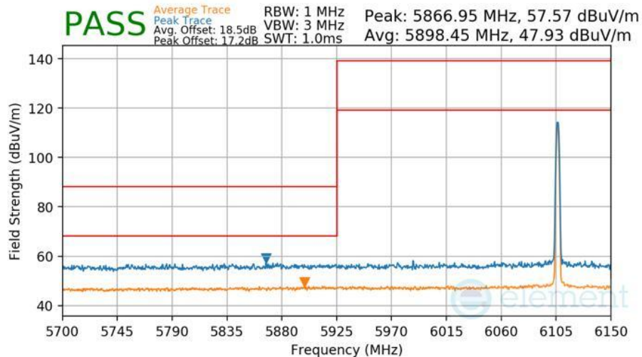
Plot 7-447 Radiated Lower Band Edge Measurement Antenna 3b
