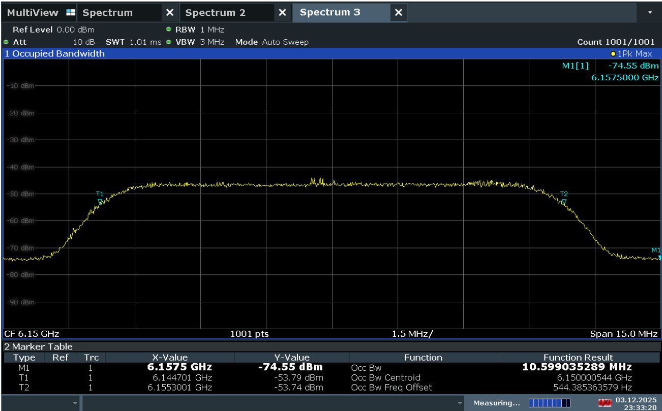
Plot 7-404. AWGN Signal
