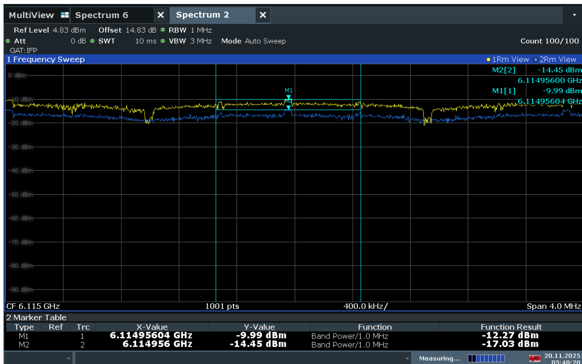
Plot 7-408. Power Density Plot 6115MHz Antenna 5T
