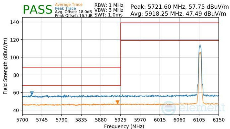
Plot 7-442 Radiated Lower Band Edge Measurement Antenna 5T
