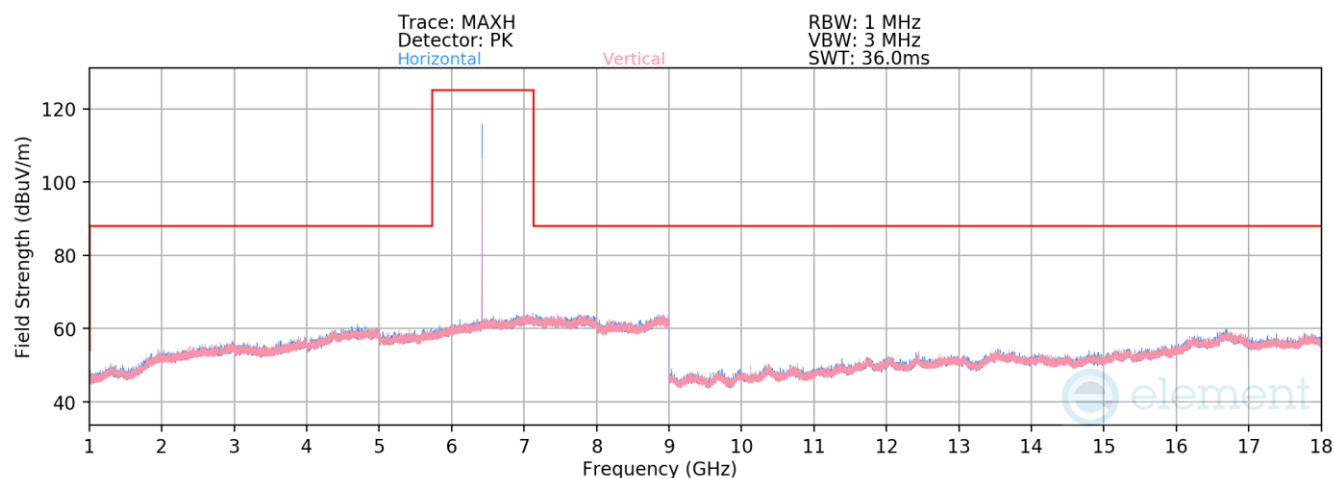
Plot 7-418. Radiated Spurious Emissions 1-18GHz TxBF Primary (HDR4 GFSK ePA – 6420MHz)
