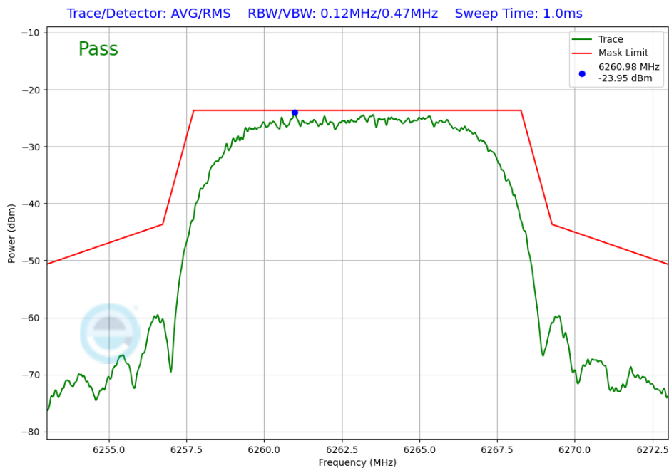
Plot 7-391. In-Band Emission Tx BF Diversity Antenna 1b (NB UNII HDRPL32, iPA – 6263MHz)
