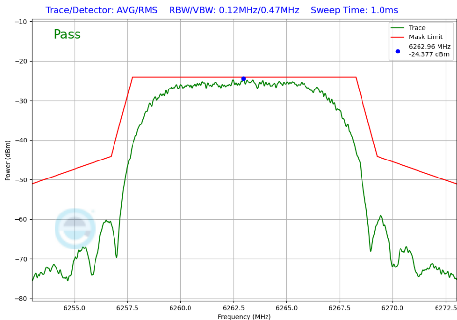
Plot 7-390. In-Band Emission Tx BF Diversity Antenna 5T (NB UNII HDRPL32, iPA – 6263MHz)
