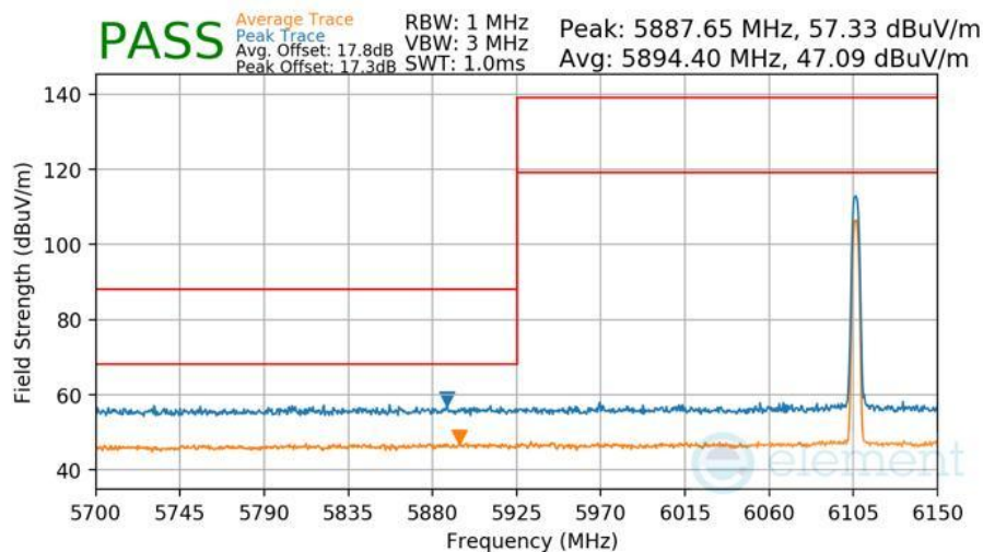
Plot 7-446 Radiated Lower Band Edge Measurement Antenna 5T
