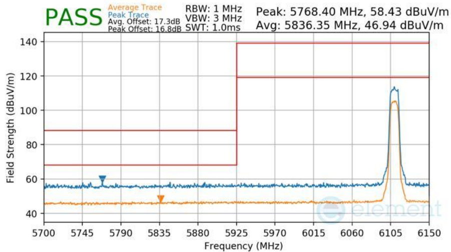
Plot 7-443 Radiated Lower Band Edge Measurement Antenna 5T
