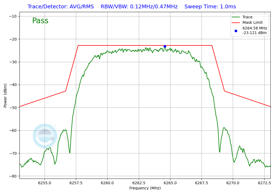
Plot 7-384. In-Band Emission TxBF Diversity Antenna 5T (NB UNII HDRPL12, ePA – 6263MHz)
