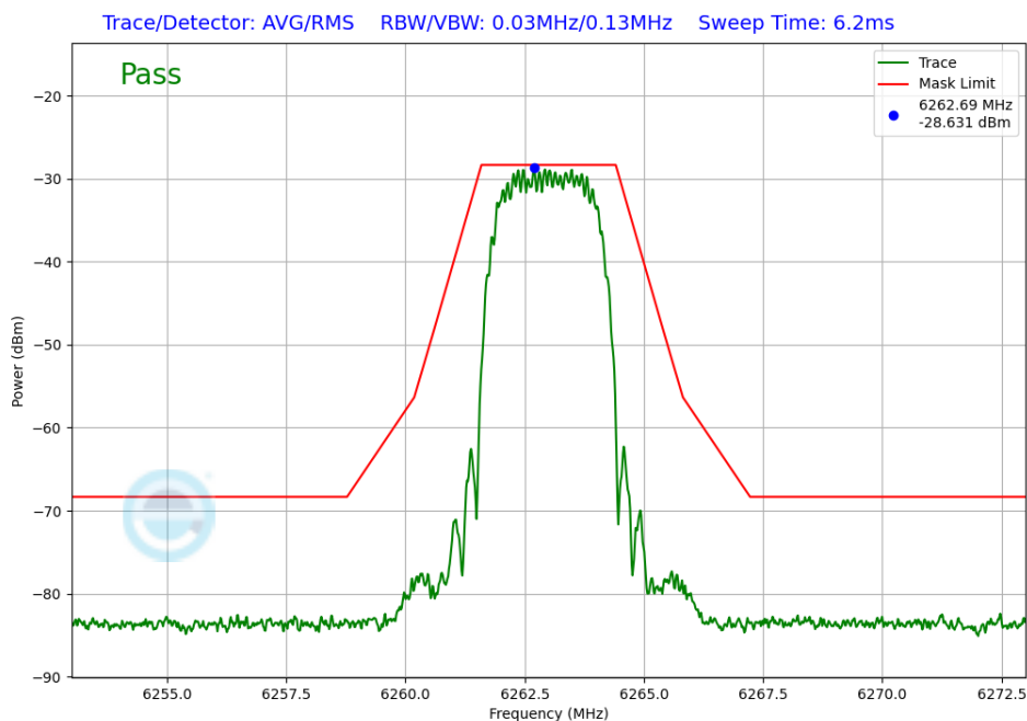
Plot 7-398. In-Band Emission TxBF Diversity Antenna 5T (NB UNII HDT4, iPA – 6263MHz)
