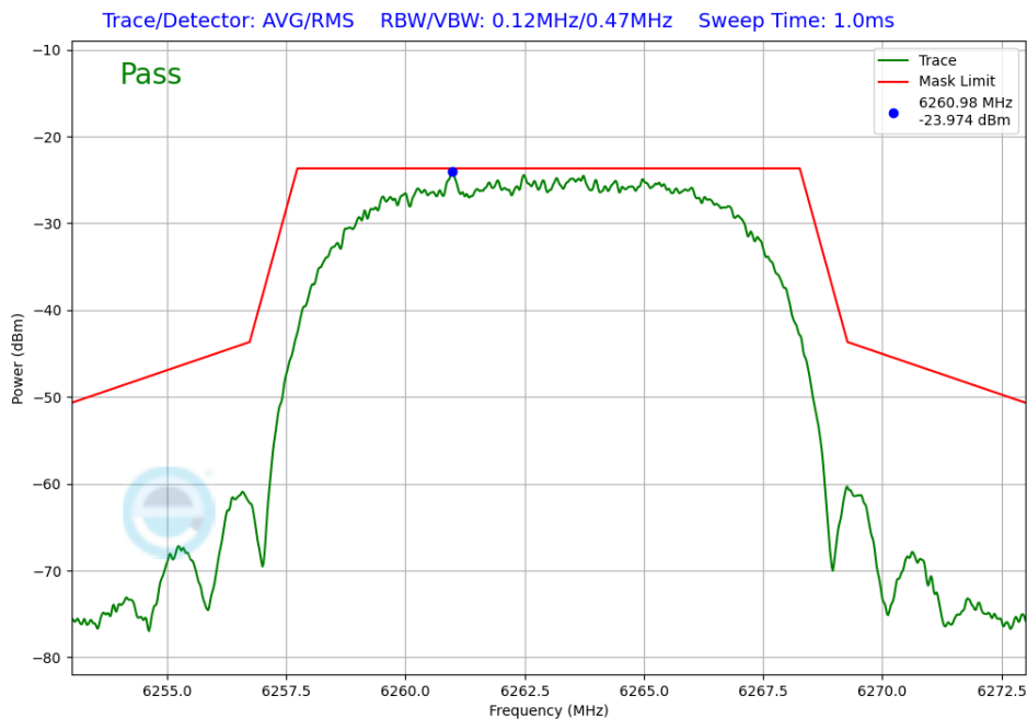
Plot 7-389. In-Band Emission TxBF Diversity Antenna 1b (NB UNII HDRPL32, ePA – 6263MHz)
