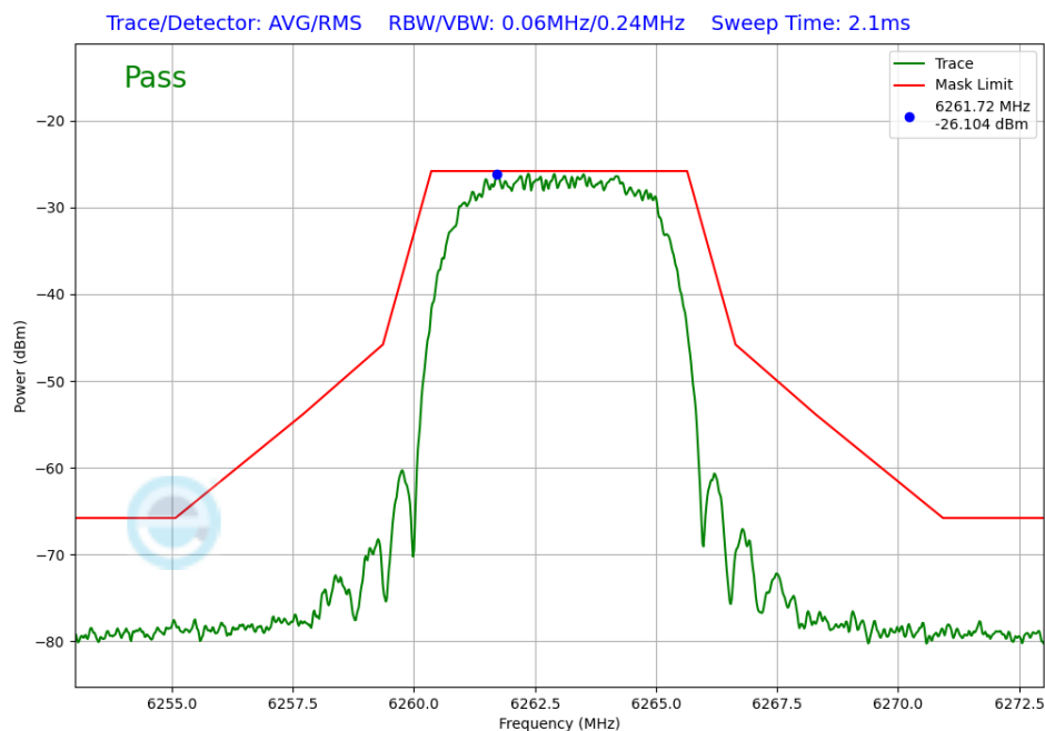
Plot 7-382. In-Band Emission TxBF Diversity Antenna 5T (NB UNII HDRPM16, iPA – 6263MHz)
