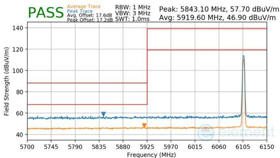
Plot 7-445 Radiated Lower Band Edge Measurement Antenna 5T
