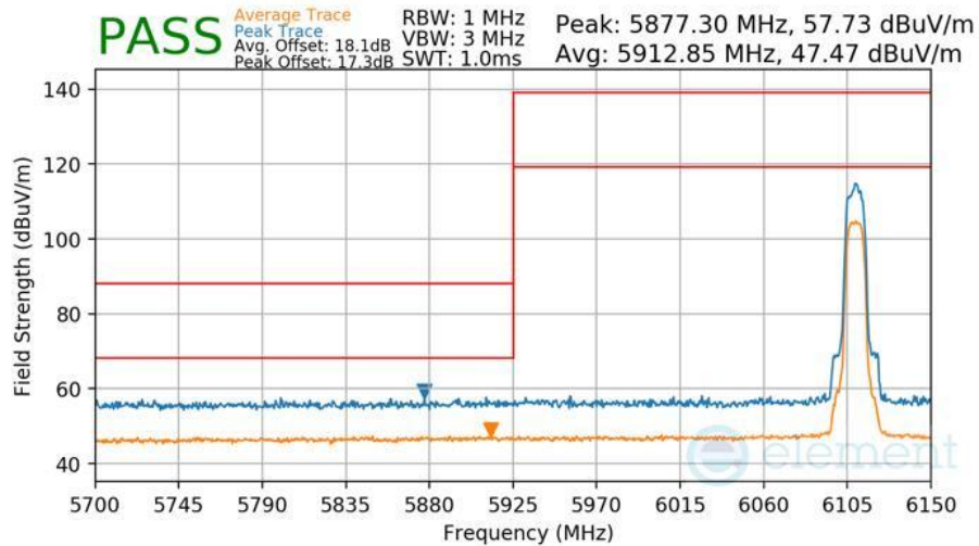
Plot 7-444 Radiated Lower Band Edge Measurement Antenna 5T
