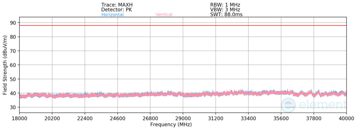
Plot 7-413. Radiated Spurious Emissions Above 18GHz (BDR GFSK ePA – 6263MHz)
