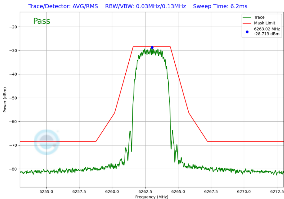
Plot 7-396. In-Band Emission TxBF Diversity Antenna 5T (NB UNII HDT4, ePA – 6263MHz)
