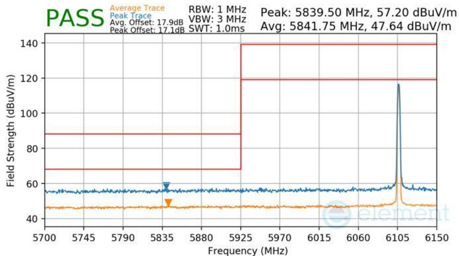
Plot 7-436 Radiated Lower Band Edge Measurement Antenna 5T
