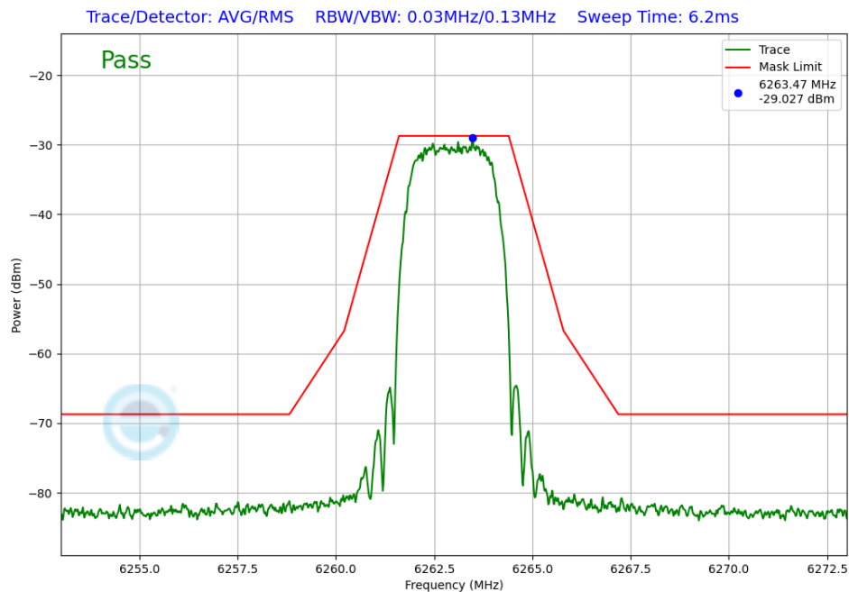
Plot 7-401. In-Band Emission TxBF Diversity Antenna 1b (NB UNII HDT6, ePA – 6263MHz)
