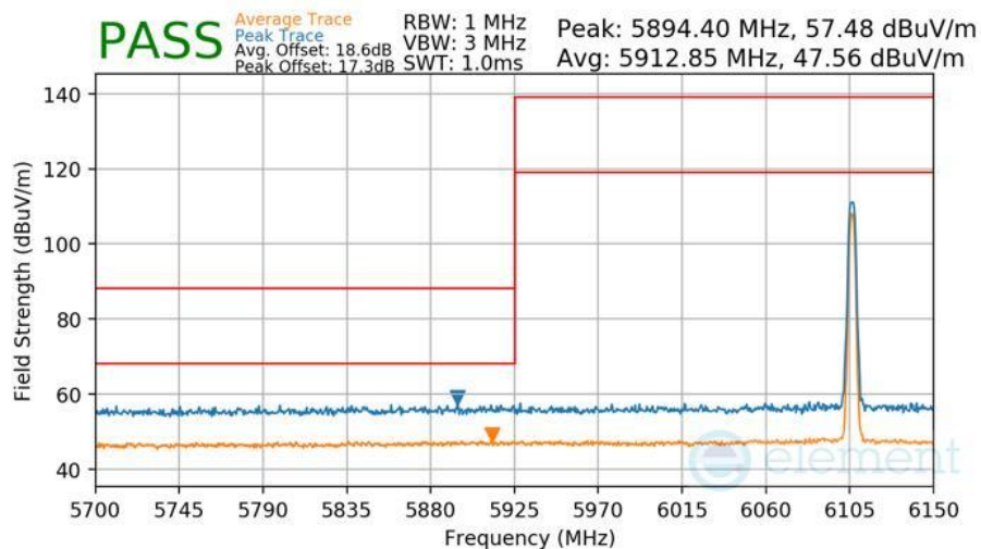
Plot 7-450 Radiated Lower Band Edge Measurement Antenna 3b
