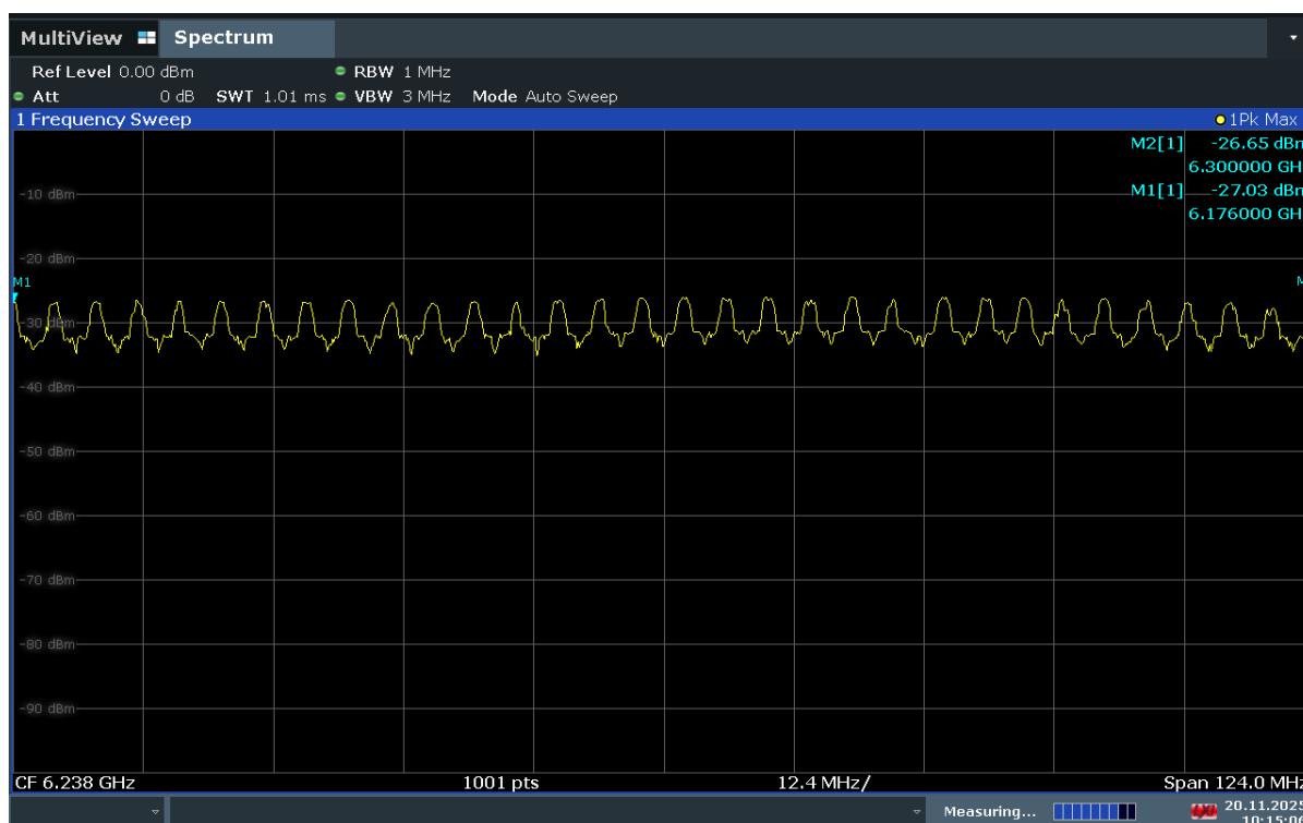
Plot 7-406. Before AWGN Signal Injected
