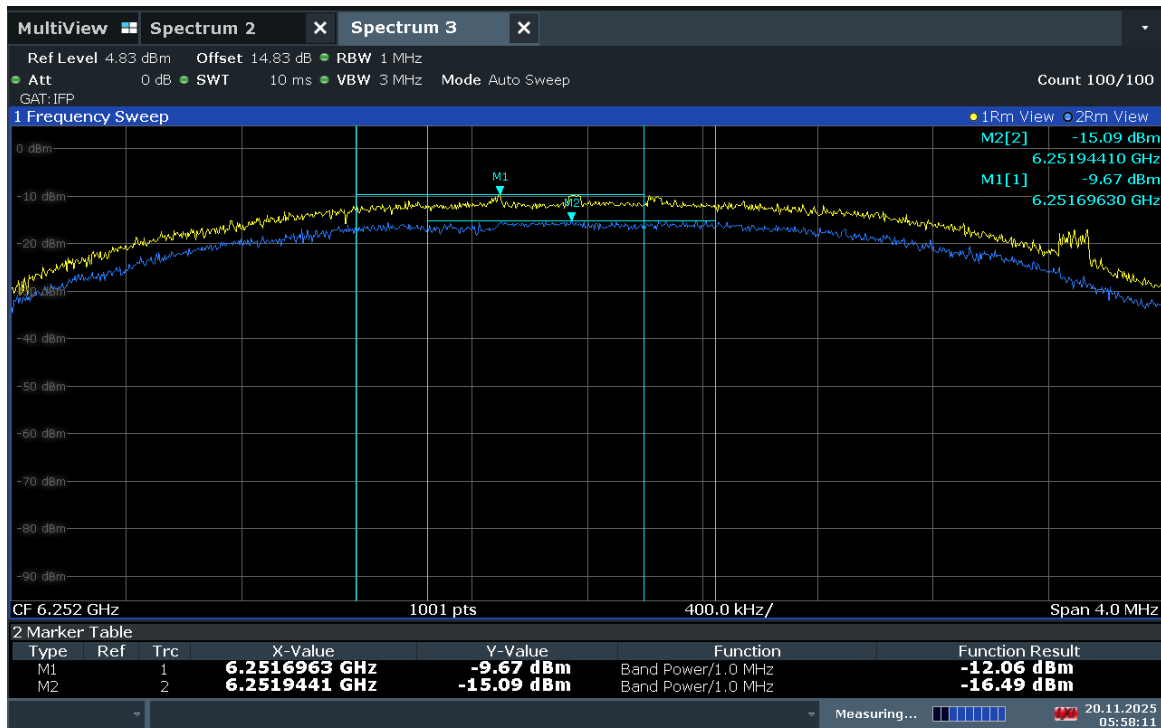
Plot 7-409. Power Density Plot – 6252MHz Antenna 5T
