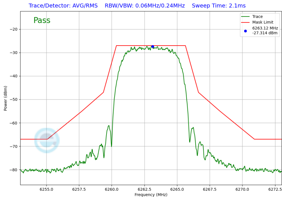
Plot 7-383. In-Band Emission TxBF Diversity Antenna 1b (NB UNII HDRPM16, iPA – 6263MHz)
