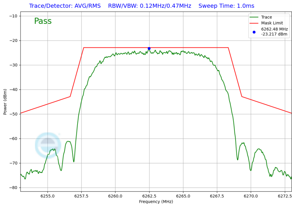
Plot 7-387. In-Band Emission Tx BF Diversity Antenna 1b (NB UNII HDRPL12, iPA – 6263MHz)
