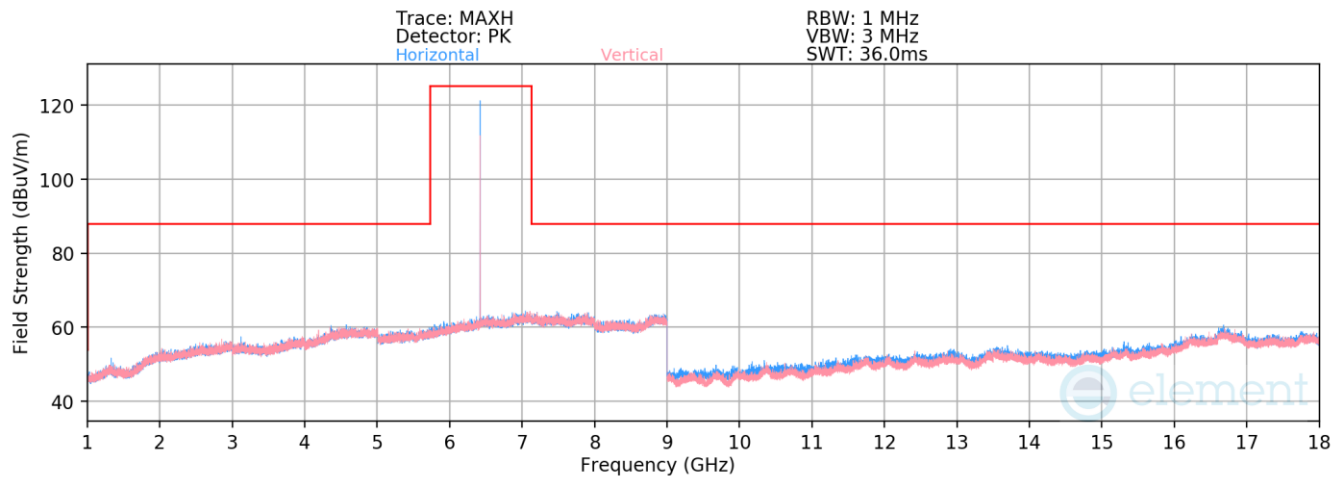
Plot 7-414. Radiated Spurious Emissions 1-18GHz TxBF Primary (BDR GFSK ePA – 6420MHz)
