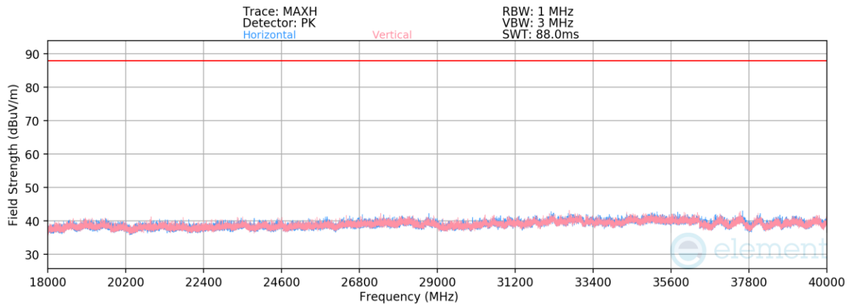
Plot 7-417. Radiated Spurious Emissions Above 18GHz (HDR4 GFSK ePA – 6263MHz)
