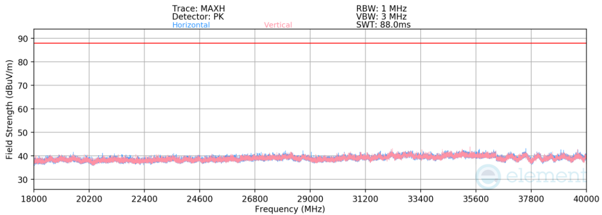
Plot 7-429. Radiated Spurious Emissions Above 18GHz TxBF Diversity (HDR4 ePA – 6263MHz)
