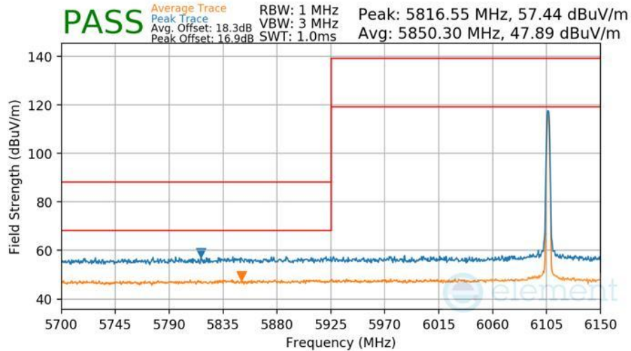
Plot 7-435 Radiated Lower Band Edge Measurement Antenna 5T
