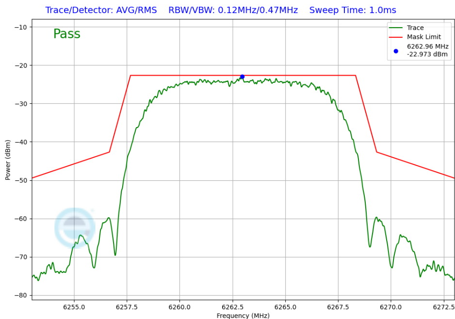
Plot 7-386. In-Band Emission Tx BF Diversity Antenna 5T (NB UNII HDRPL12, iPA – 6263MHz)
