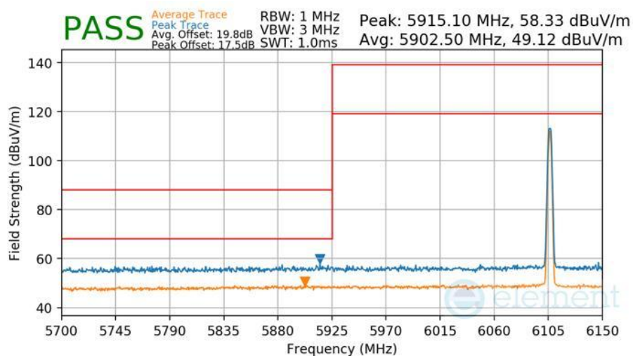
Plot 7-449 Radiated Lower Band Edge Measurement Antenna 3b
