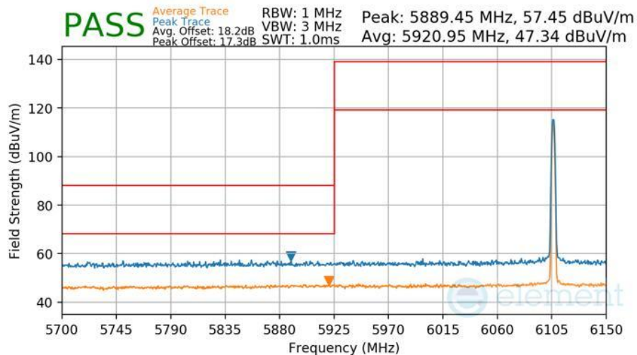
Plot 7-448 Radiated Lower Band Edge Measurement Antenna 3b
