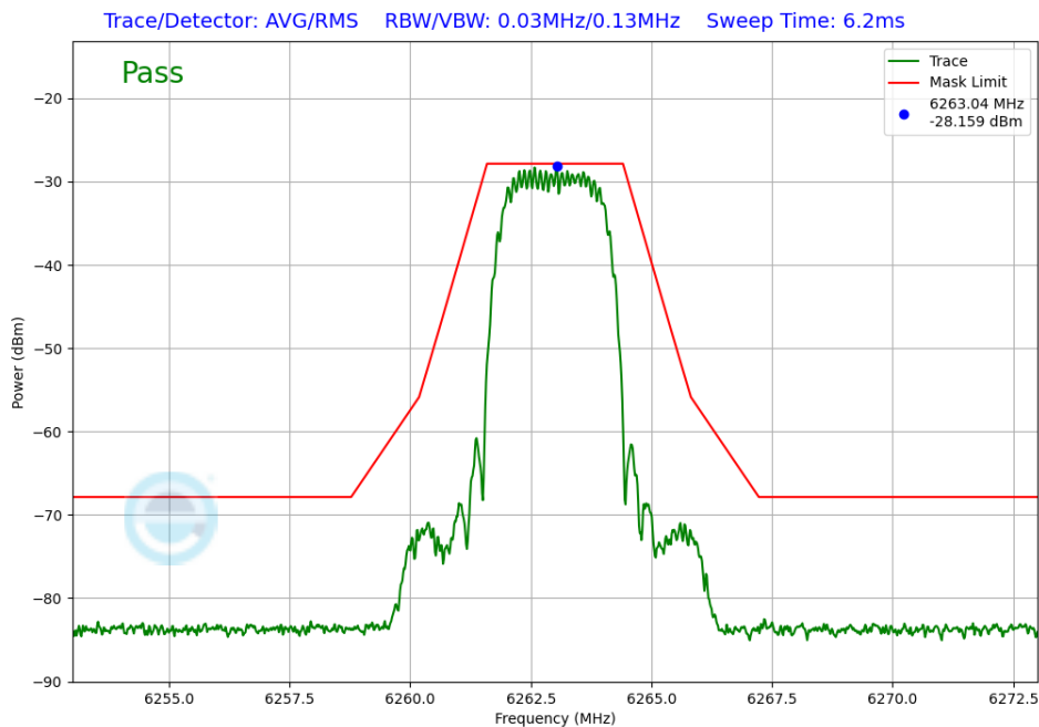
Plot 7-399. In-Band Emission TxBF Diversity Antenna 1b (NB UNII HDT4, iPA – 6263MHz)
