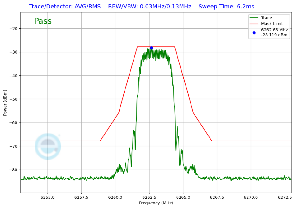
Plot 7-394. In-Band Emission TxBF Diversity Antenna 5T (NB UNII HDT2, iPA – 6263MHz)
