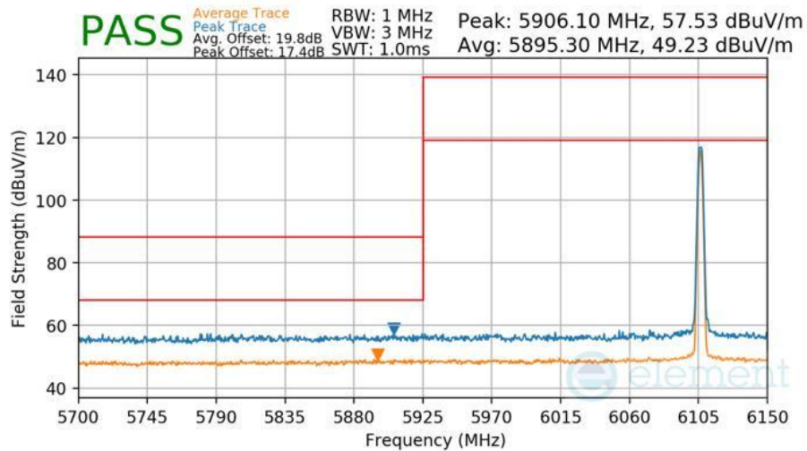
Plot 7-437 Radiated Lower Band Edge Measurement Antenna 5T
