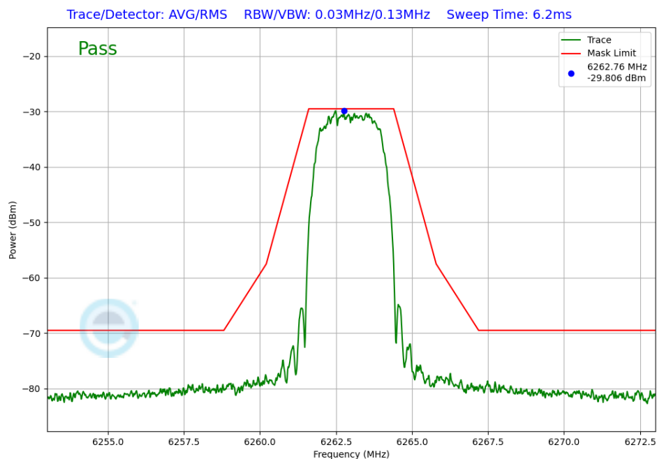
Plot 7-400. In-Band Emission TxBF Diversity Antenna 5T (NB UNII HDT6, ePA – 6263MHz)
