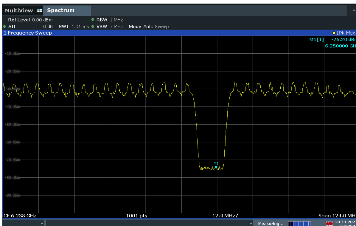
Plot 7-407. After AWGN Signal Injected
