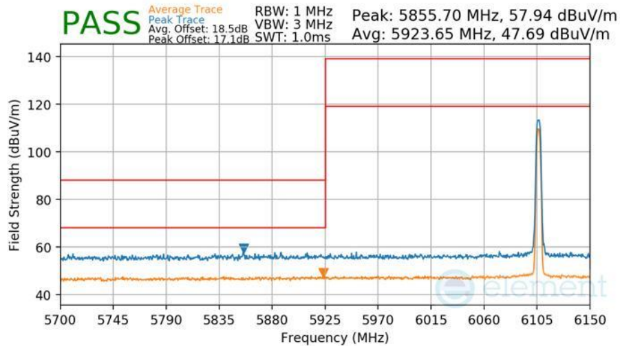
Plot 7-438 Radiated Lower Band Edge Measurement Antenna 5T
