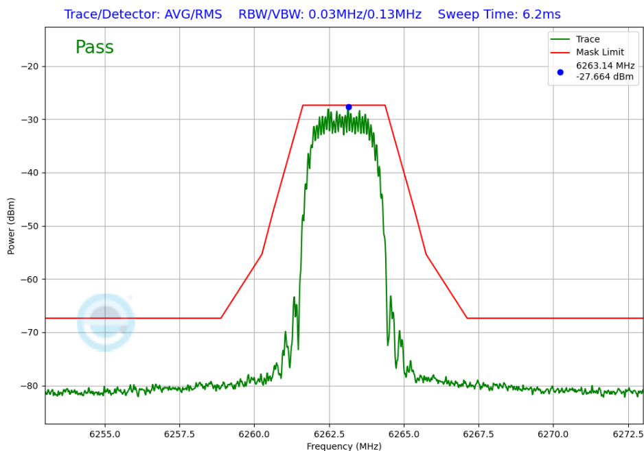
Plot 7-392. In-Band Emission TxBF Diversity Antenna 5T (NB UNII HDT2, ePA – 6263MHz)
