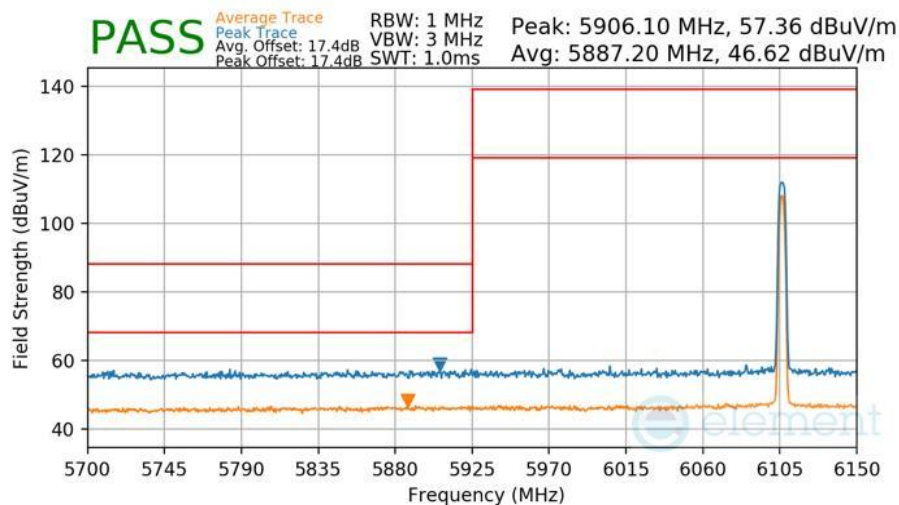
Plot 7-440 Radiated Lower Band Edge Measurement Antenna 5T
