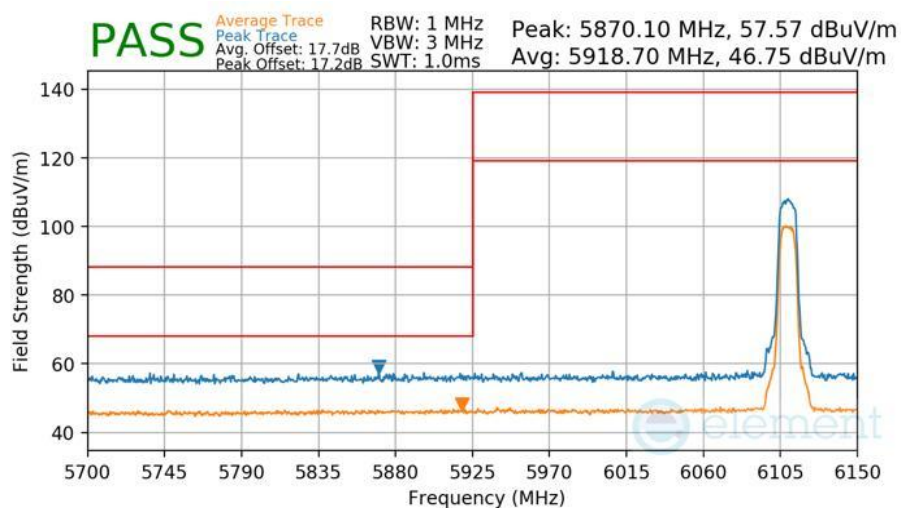
Plot 7-455 Radiated Lower Band Edge Measurement Antenna 3b
