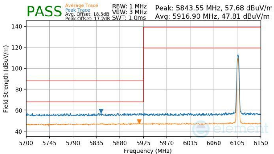
Plot 7-462 Radiated Lower Band Edge Measurement Antenna 1b
