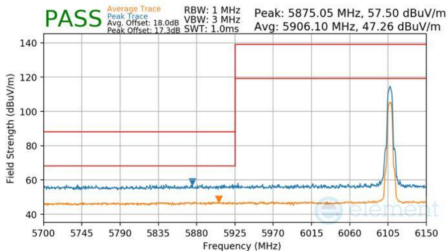
Plot 7-466 Radiated Lower Band Edge Measurement Antenna 1b
