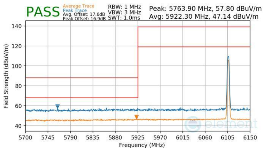
Plot 7-457 Radiated Lower Band Edge Measurement Antenna 3b
