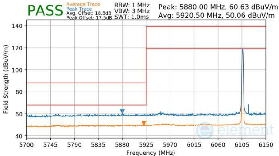
Plot 7-483 Radiated Lower Band Edge Measurement TxBF Diversity
