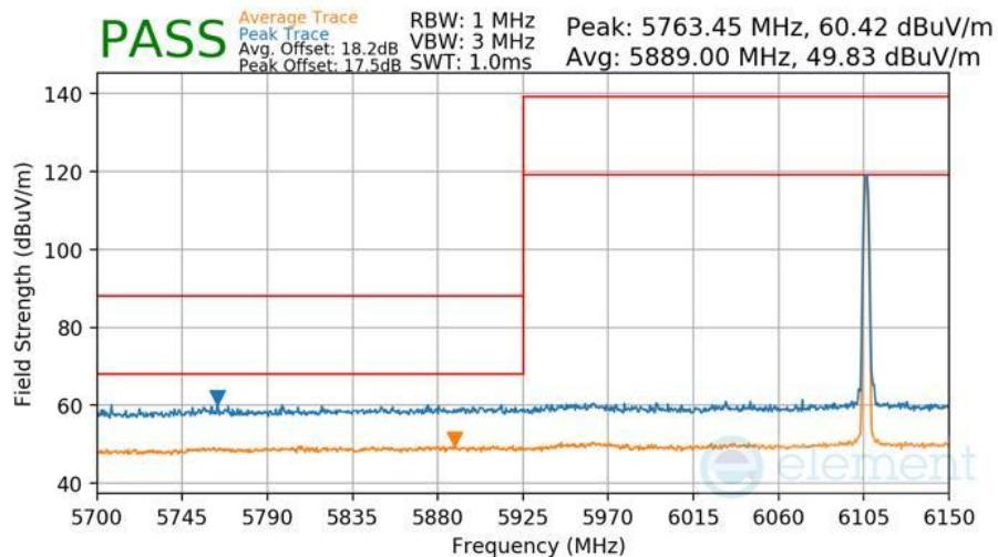
Plot 7-472 Radiated Lower Band Edge Measurement TxBF Primary
