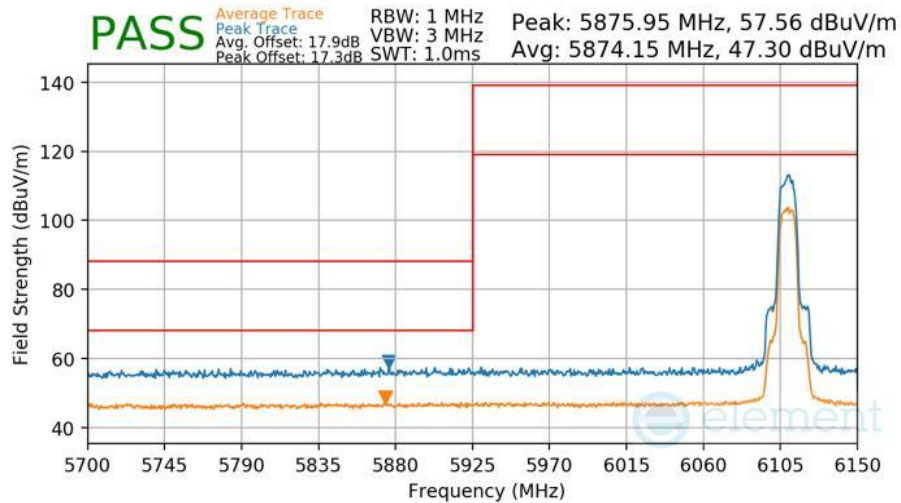
Plot 7-468 Radiated Lower Band Edge Measurement Antenna 1b
