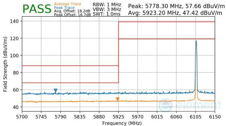
Plot 7-460 Radiated Lower Band Edge Measurement Antenna 1b
