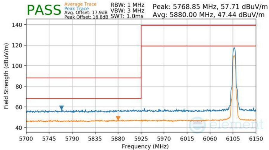
Plot 7-490 Radiated Lower Band Edge Measurement TxBF Diversity
