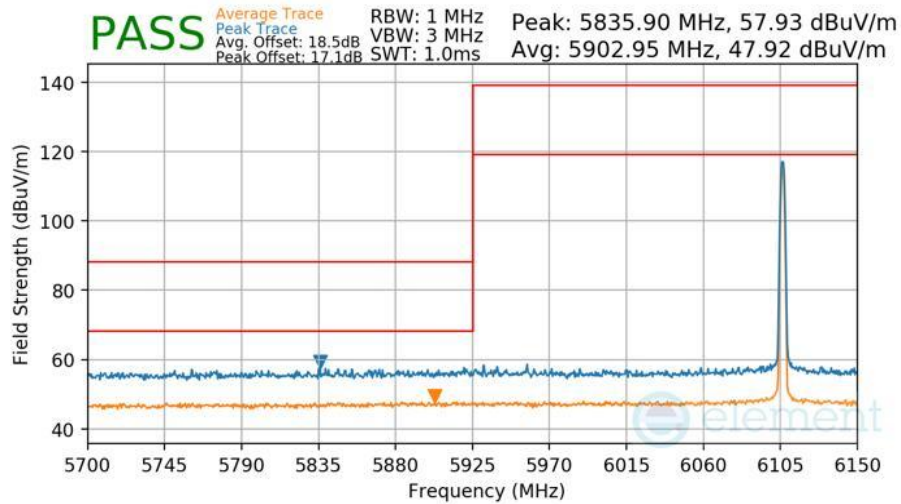
Plot 7-459 Radiated Lower Band Edge Measurement Antenna 1b
