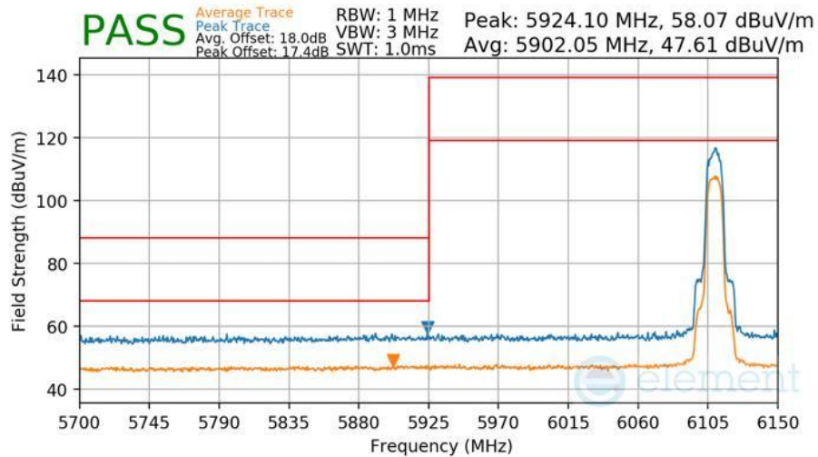
Plot 7-492 Radiated Lower Band Edge Measurement TxBF Diversity
