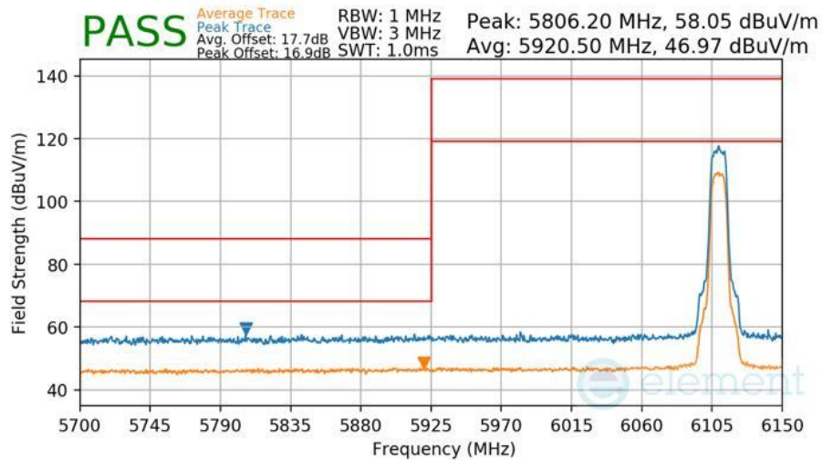
Plot 7-491 Radiated Lower Band Edge Measurement TxBF Diversity
