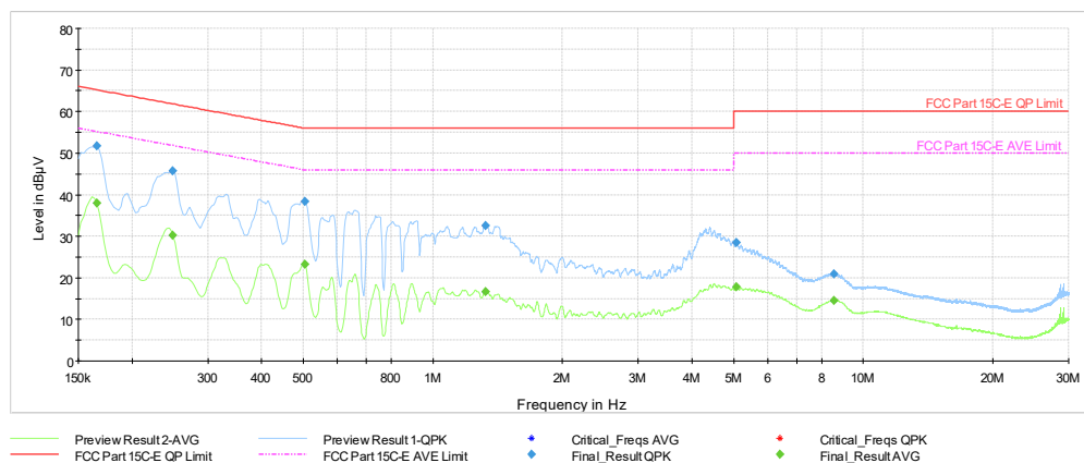
Plot 7-510. AC Line Conducted Plot TxBF Diversity (NB UNII HDR4 ePA – 6263MHz) (N) with AC/DC adaptor
