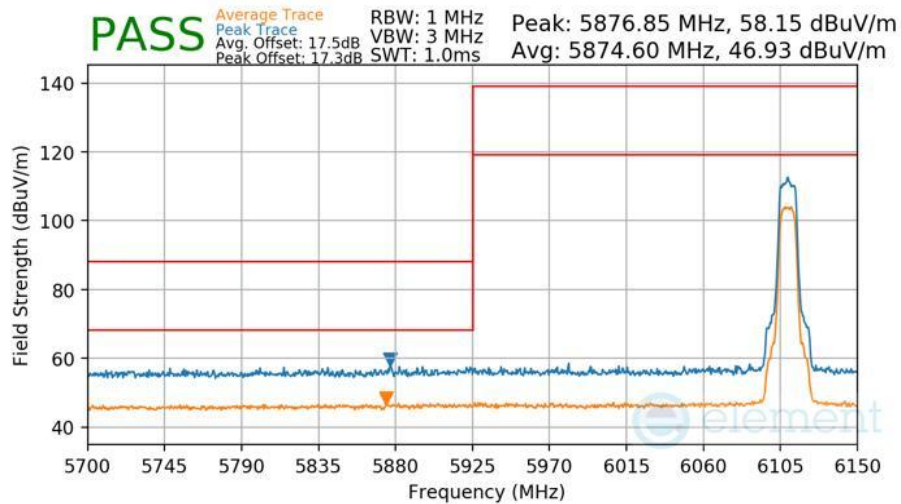
Plot 7-467 Radiated Lower Band Edge Measurement Antenna 1b
