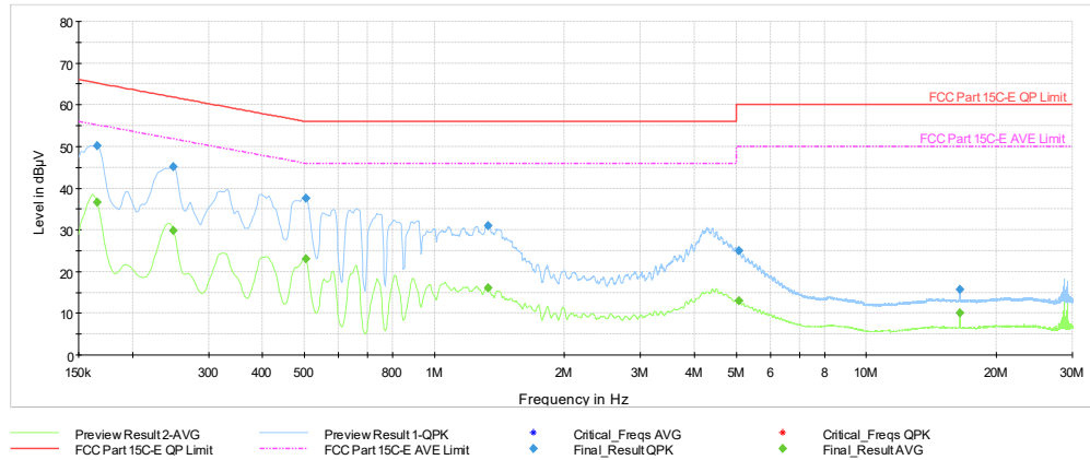
Plot 7-509. AC Line Conducted Plot TxBF Diversity (NB UNII HDR4 ePA – 6263MHz) (L1) with AC/DC adaptor
