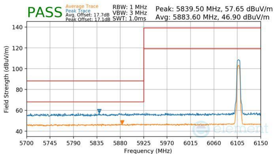
Plot 7-453 Radiated Lower Band Edge Measurement Antenna 3b
