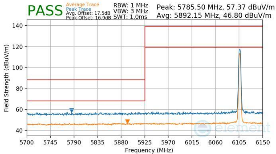
Plot 7-481 Radiated Lower Band Edge Measurement TxBF Primary
