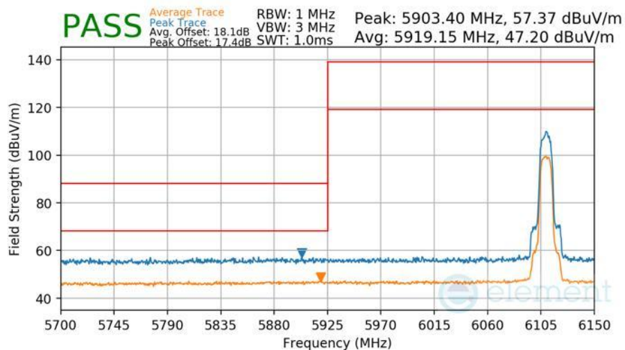
Plot 7-456 Radiated Lower Band Edge Measurement Antenna 3b
