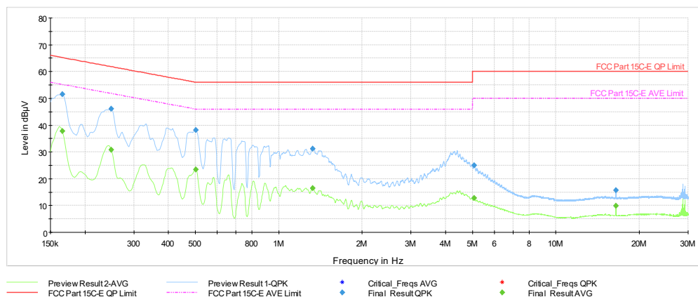
Plot 7-507. AC Line Conducted Plot TxBF Diversity (NB UNII BDR ePA – 6263MHz) (L1) with AC/DC adaptor
