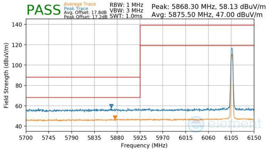
Plot 7-482 Radiated Lower Band Edge Measurement TxBF Primary
