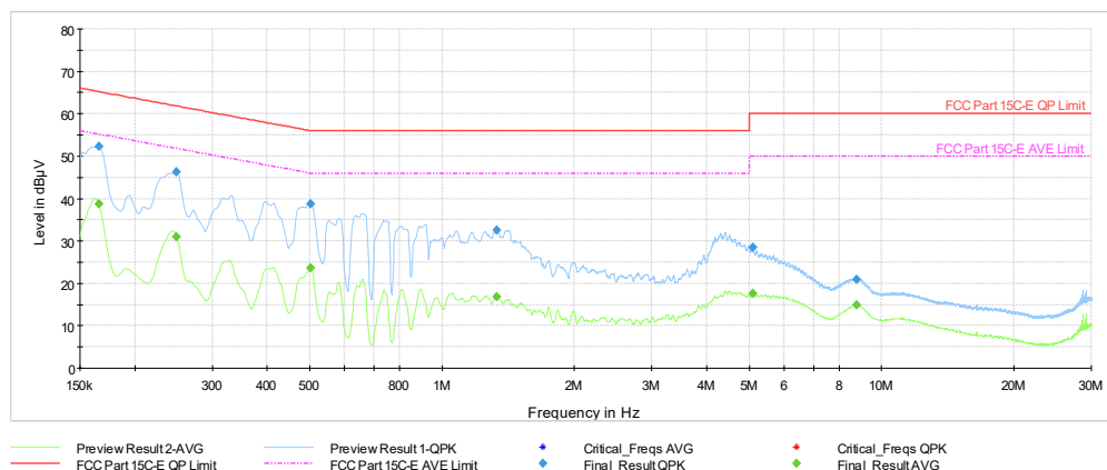
Plot 7-512. AC Line Conducted Plot TxBF Diversity (NB UNII LE1M ePA – 6263MHz) (N) with AC/DC adaptor
