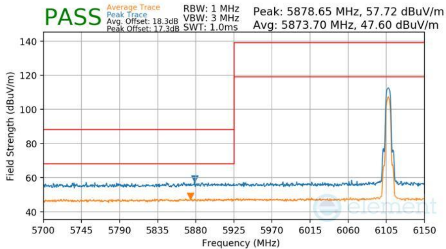
Plot 7-463 Radiated Lower Band Edge Measurement Antenna 1b
