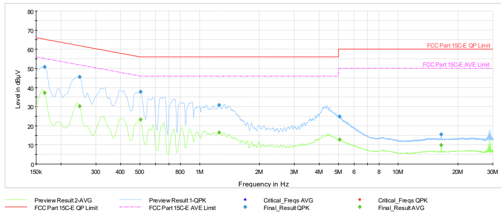
Plot 7-511. AC Line Conducted Plot TxBF Diversity (NB UNII LE1M ePA – 6263MHz) (L1) with AC/DC adaptor
