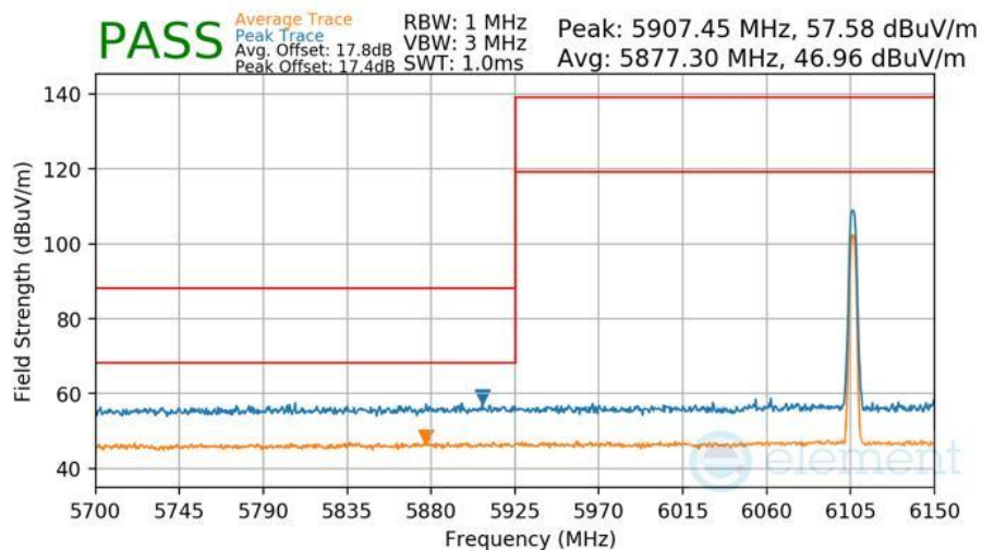
Plot 7-458 Radiated Lower Band Edge Measurement Antenna 3b
