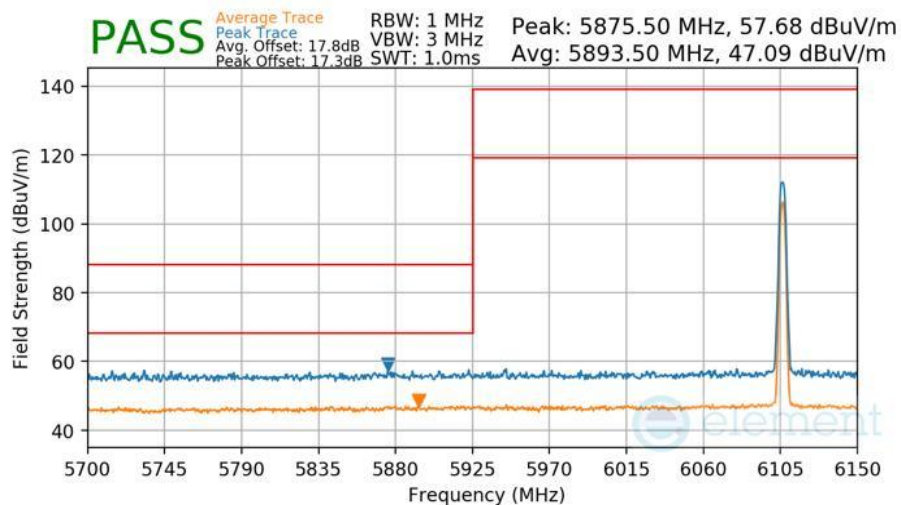
Plot 7-470 Radiated Lower Band Edge Measurement Antenna 1b
