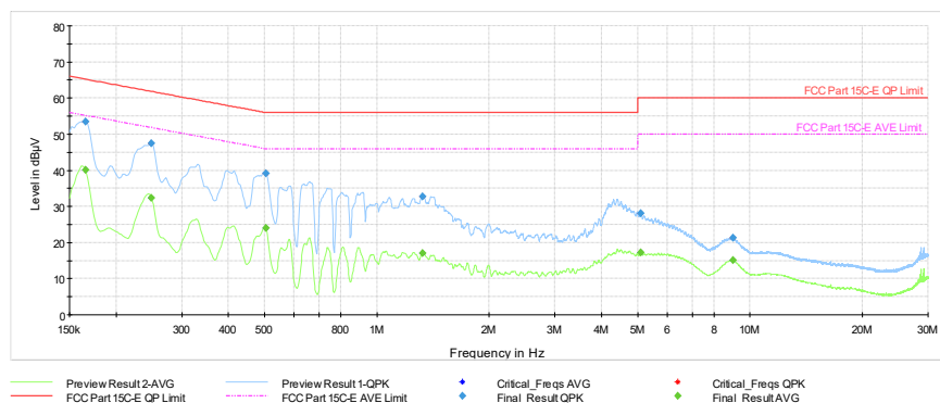
Plot 7-508. AC Line Conducted Plot TxBF Diversity (NB UNII BDR ePA – 6263MHz) (N) with AC/DC adaptor
