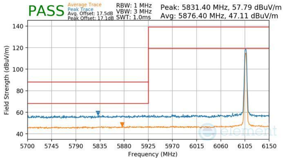
Plot 7-493 Radiated Lower Band Edge Measurement TxBF Diversity
