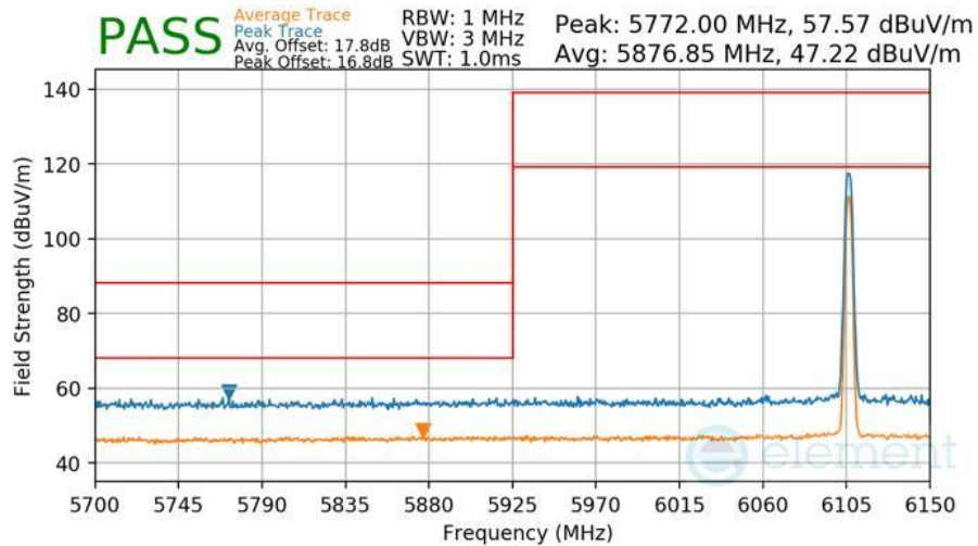
Plot 7-494 Radiated Lower Band Edge Measurement TxBF Diversity
