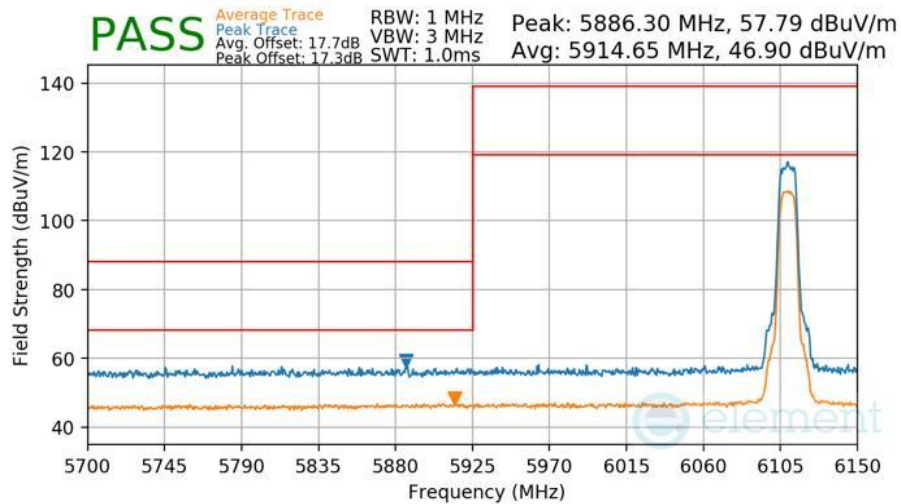
Plot 7-479 Radiated Lower Band Edge Measurement TxBF Primary
