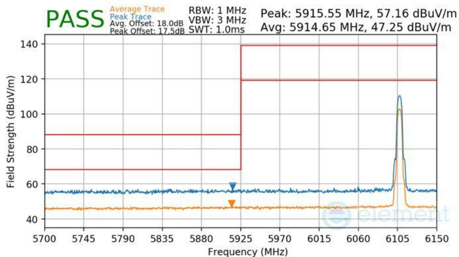
Plot 7-454 Radiated Lower Band Edge Measurement Antenna 3b
