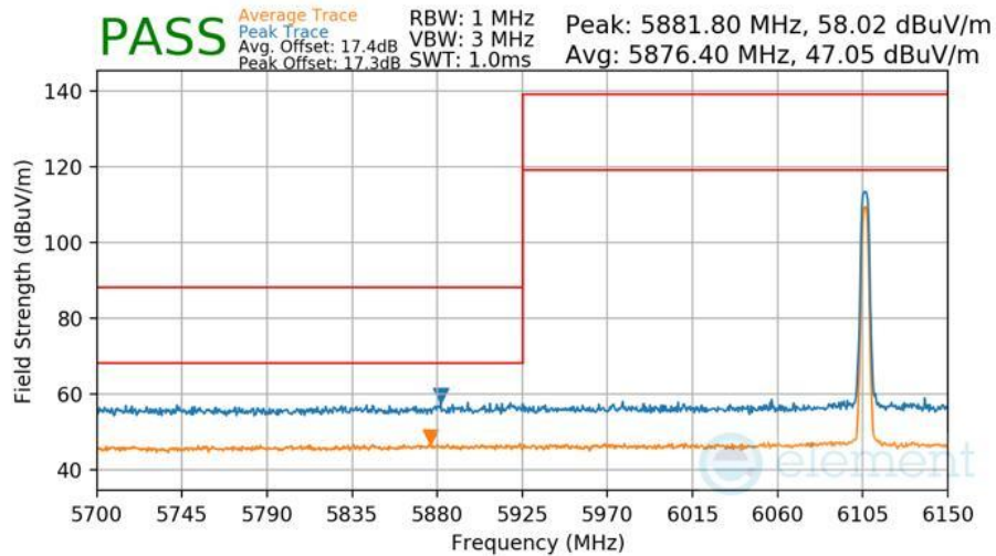
Plot 7-464 Radiated Lower Band Edge Measurement Antenna 1b
