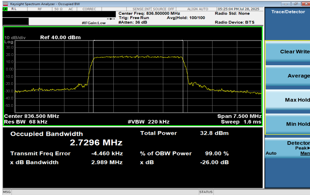
Plot 7-7. Occupied Bandwidth Plot (LTE Band 26/5 - 3MHz 64-QAM - Full RB Configuration)
