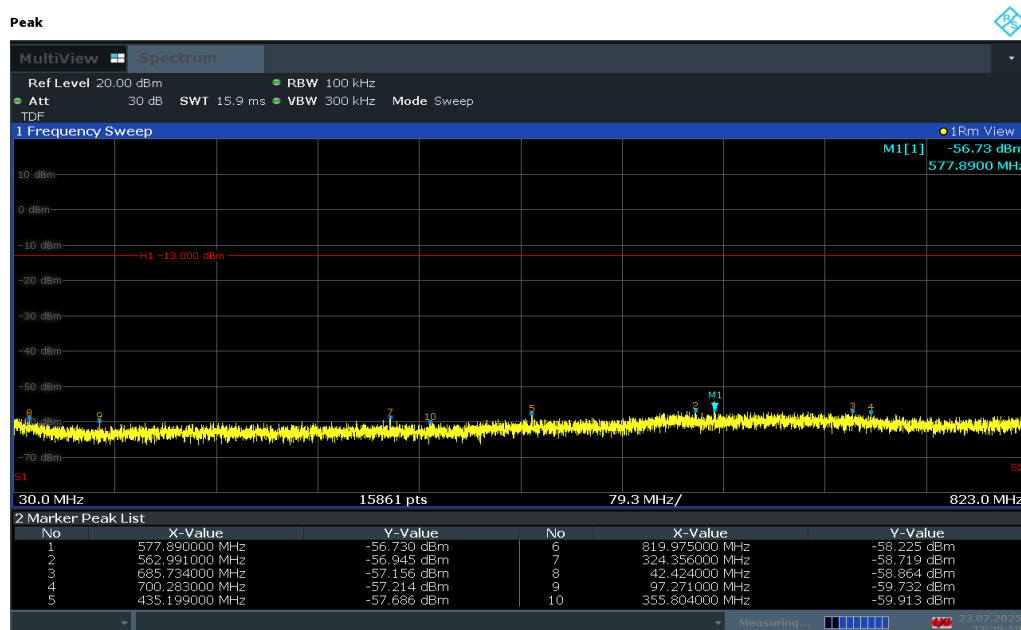
Plot 7-45. Conducted Spurious Plot (LTE Band 26/5 - 10MHz QPSK - RB Size 1, RB Offset 0 - Mid Channel)
