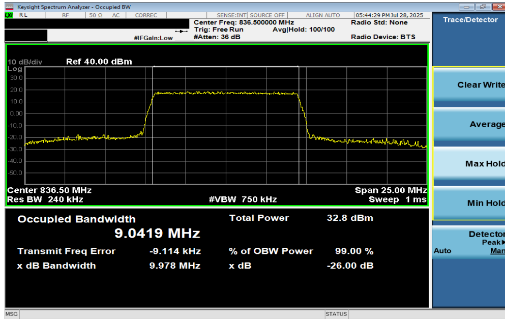
Plot 7-15. Occupied Bandwidth Plot (LTE Band 26/5 - 10MHz 64-QAM - Full RB Configuration)
