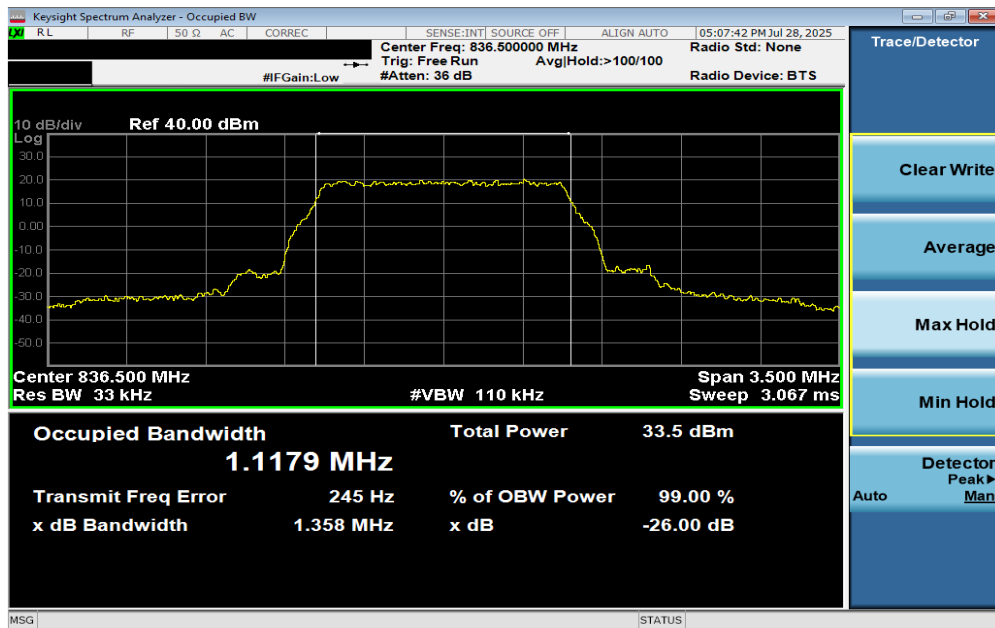
Plot 7-2. Occupied Bandwidth Plot (LTE Band 26/5 - 1.4MHz 16-QAM - Full RB Configuration)
