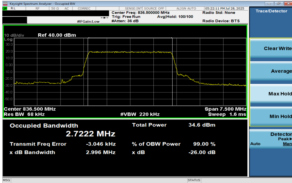
Plot 7-5. Occupied Bandwidth Plot (LTE Band 26/5 - 3MHz QPSK - Full RB Configuration)
