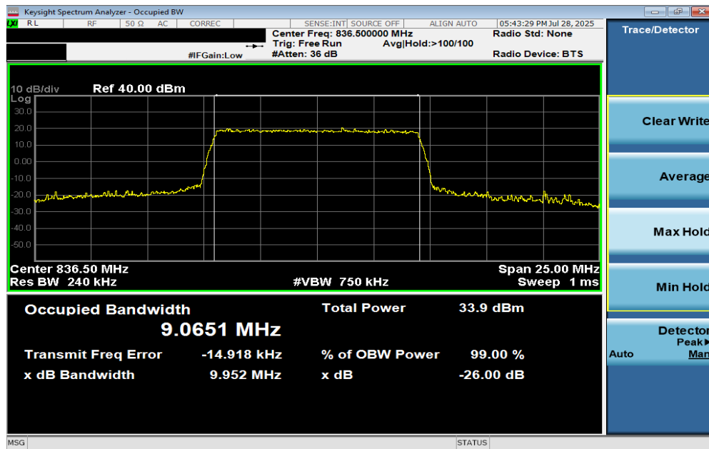
Plot 7-14. Occupied Bandwidth Plot (LTE Band 26/5 - 10MHz 16-QAM - Full RB Configuration)
