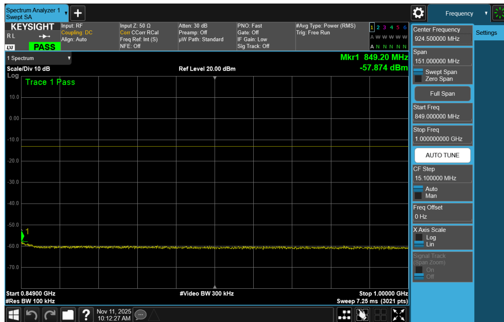
Plot 7-52. Conducted Spurious Plot (ULCA LTE Band 5 – (10 + 10)MHz QPSK – PCC 1/49 SCC 1/0 - Low Channel)
