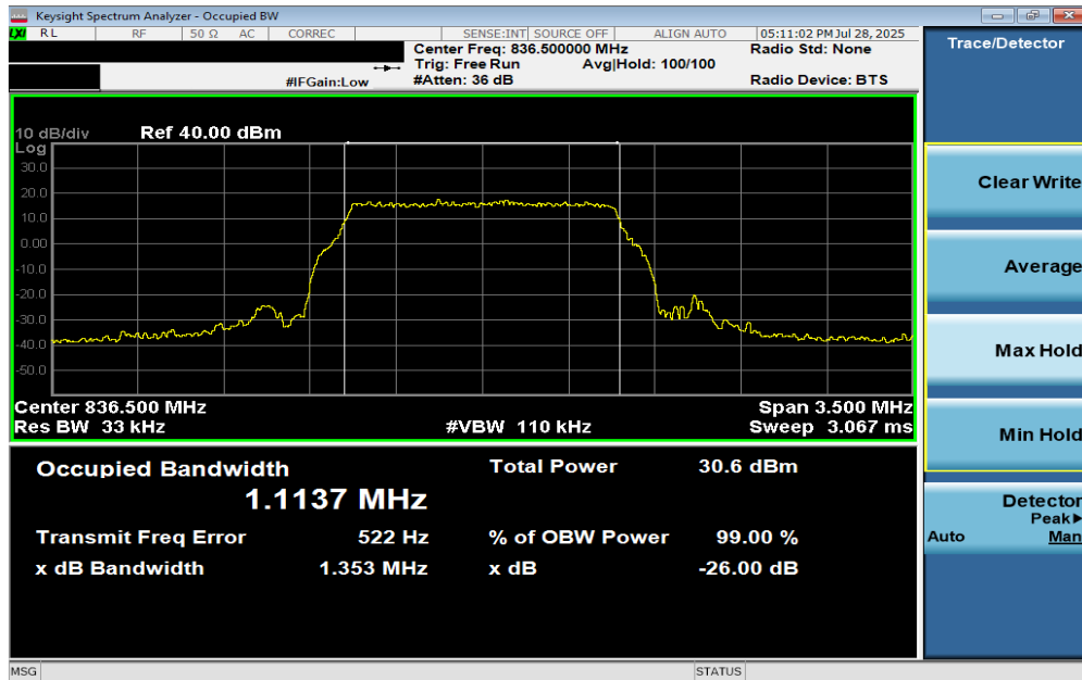
Plot 7-4. Occupied Bandwidth Plot (LTE Band 26/5 - 1.4MHz 256-QAM - Full RB Configuration)
