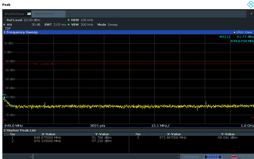
Plot 7-49. Conducted Spurious Plot (LTE Band 26/5 - 10MHz QPSK - RB Size 1, RB Offset 0 - High Channel)
