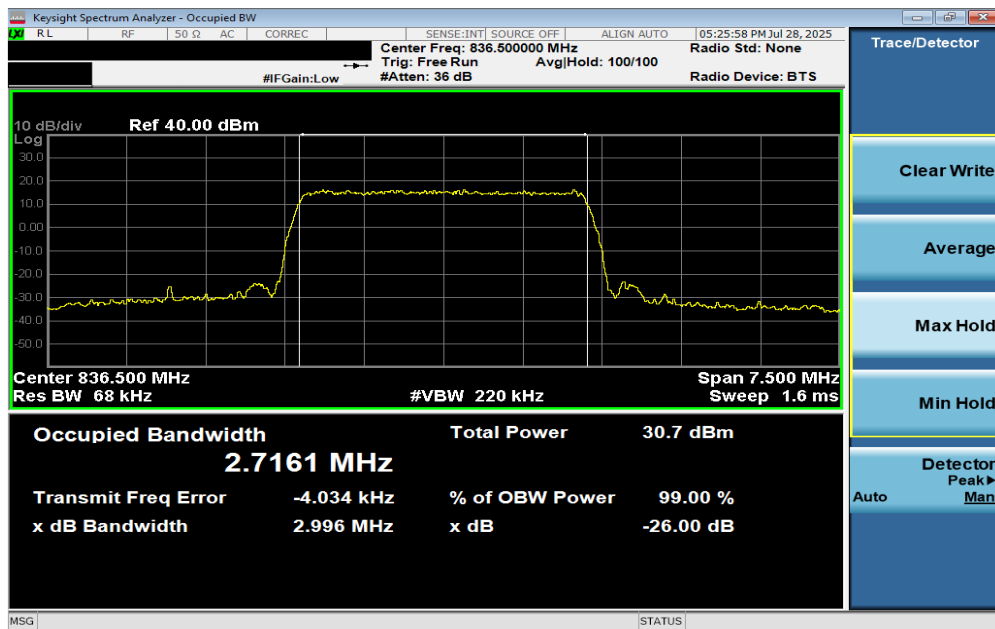
Plot 7-8. Occupied Bandwidth Plot (LTE Band 26/5 - 3MHz 256-QAM - Full RB Configuration)
