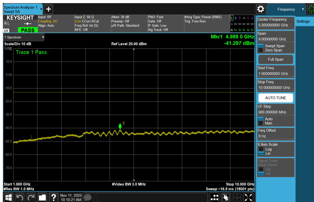
Plot 7-59. Conducted Spurious Plot (ULCA LTE Band 5 – (10 + 10)MHz QPSK – PCC 1/0 SCC 1/49 - High Channel)
