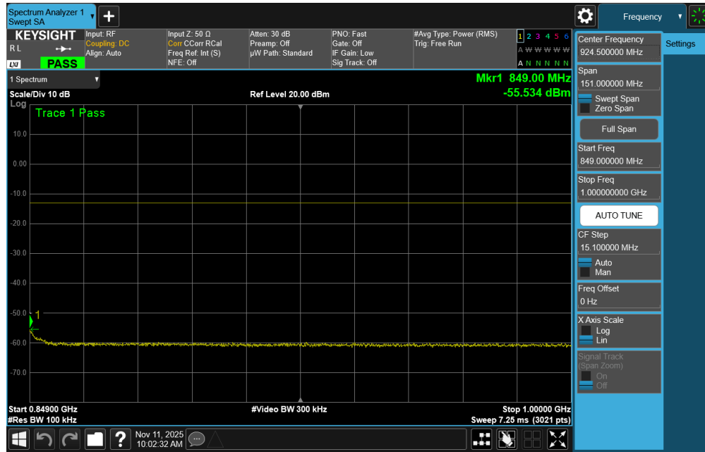
Plot 7-55. Conducted Spurious Plot (ULCA LTE Band 5 – (10 + 10)MHz QPSK – PCC 1/49 SCC 1/0 - Mid Channel)
