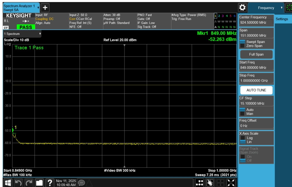
Plot 7-58. Conducted Spurious Plot (ULCA LTE Band 5 – (10 + 10)MHz QPSK – PCC 1/0 SCC 1/49 - High Channel)
