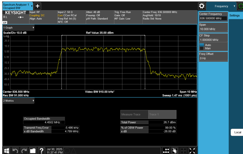
Plot 7-21. Occupied Bandwidth Plot (NR Band n26/n5 - 5MHz n5 DFT-s-OFDM \pi/2 BPSK - Full RB Configuration)
