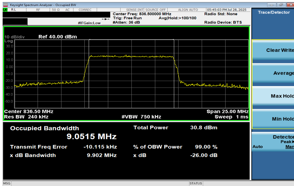
Plot 7-16. Occupied Bandwidth Plot (LTE Band 26/5 - 10MHz 256-QAM - Full RB Configuration)
