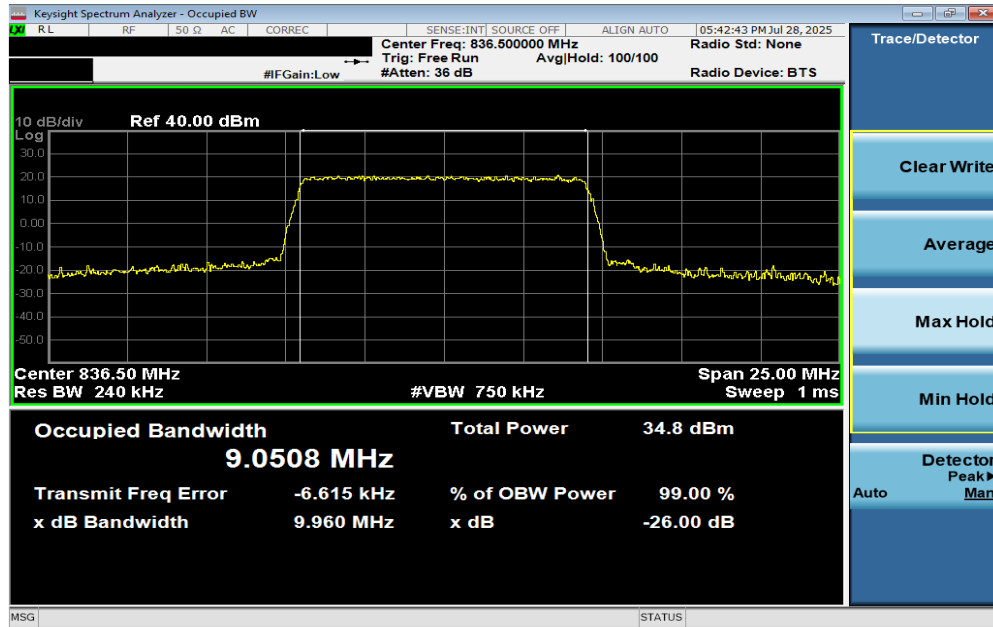
Plot 7-13. Occupied Bandwidth Plot (LTE Band 26/5 - 10MHz QPSK - Full RB Configuration)
