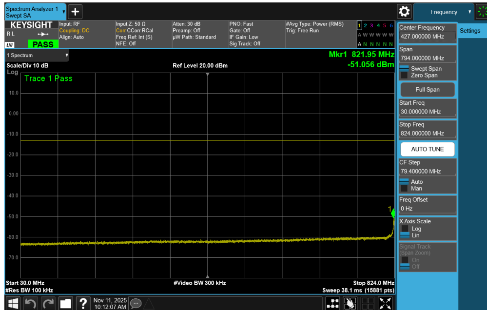
Plot 7-51. Conducted Spurious Plot (ULCA LTE Band 5 – (10 + 10)MHz QPSK – PCC 1/49 SCC 1/0 - Low Channel)
