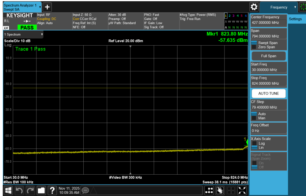
Plot 7-57. Conducted Spurious Plot (ULCA LTE Band 5 – (10 + 10)MHz QPSK – PCC 1/0 SCC 1/49 - High Channel)
