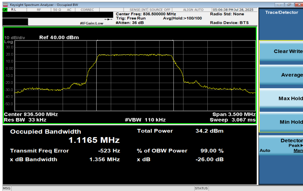
Plot 7-1. Occupied Bandwidth Plot (LTE Band 26/5 - 1.4MHz QPSK - Full RB Configuration)
