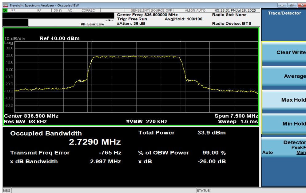
Plot 7-6. Occupied Bandwidth Plot (LTE Band 26/5 - 3MHz 16-QAM - Full RB Configuration)
