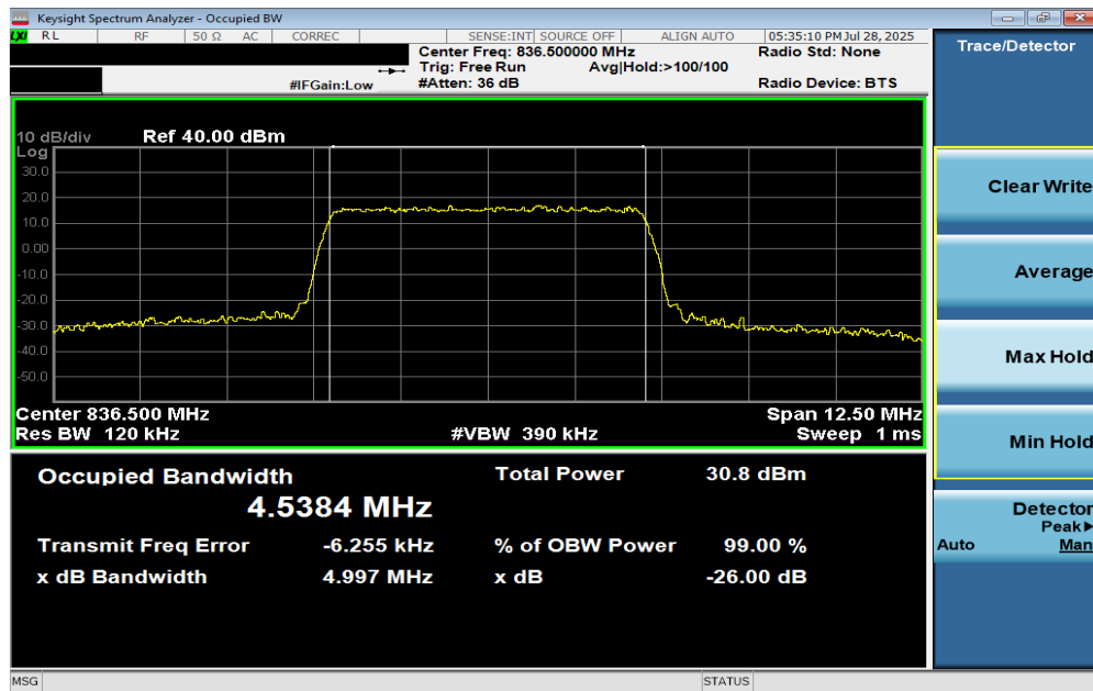
Plot 7-12. Occupied Bandwidth Plot (LTE Band 26/5 - 5MHz 256-QAM - Full RB Configuration)
