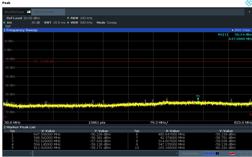
Plot 7-48. Conducted Spurious Plot (LTE Band 26/5 - 10MHz QPSK - RB Size 1, RB Offset 0 - High Channel)
