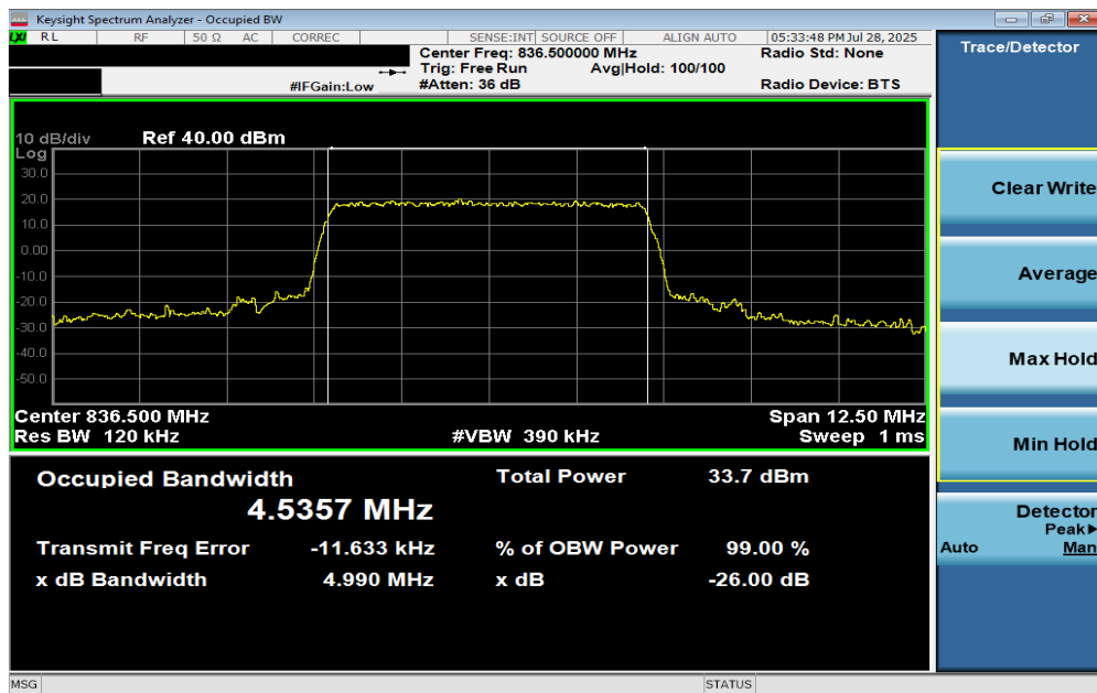
Plot 7-10. Occupied Bandwidth Plot (LTE Band 26/5 - 5MHz 16-QAM - Full RB Configuration)
