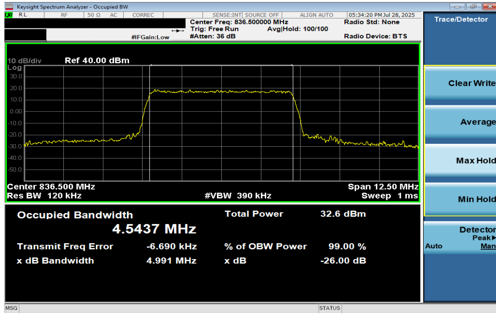
Plot 7-11. Occupied Bandwidth Plot (LTE Band 26/5 - 5MHz 64-QAM - Full RB Configuration)
