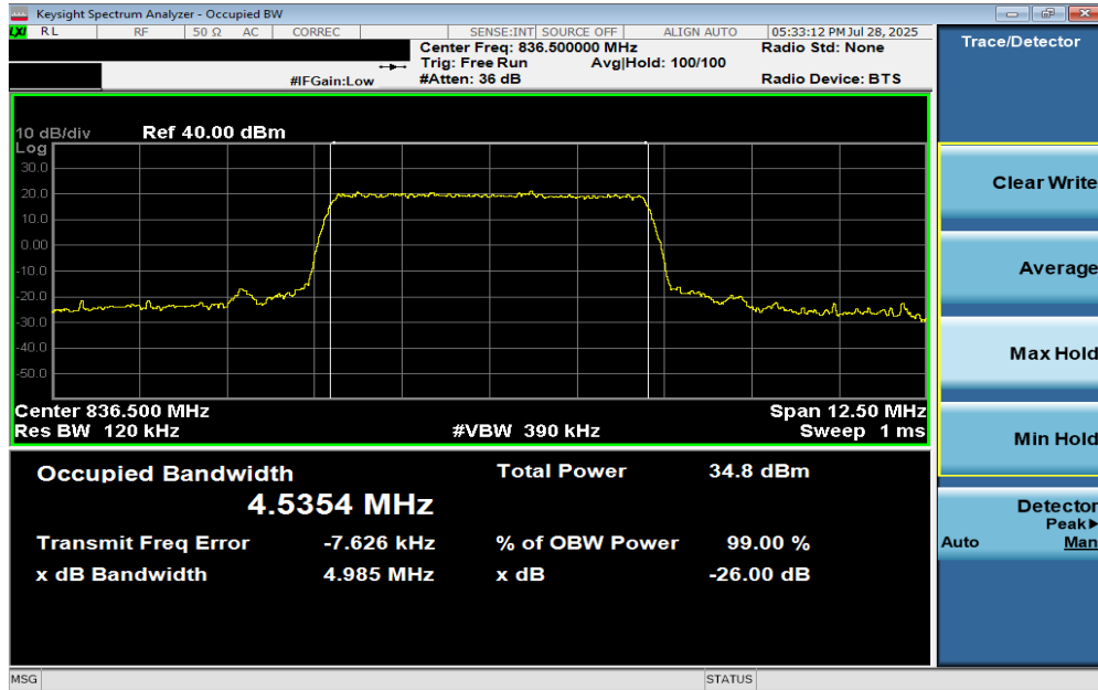
Plot 7-9. Occupied Bandwidth Plot (LTE Band 26/5 - 5MHz QPSK - Full RB Configuration)
