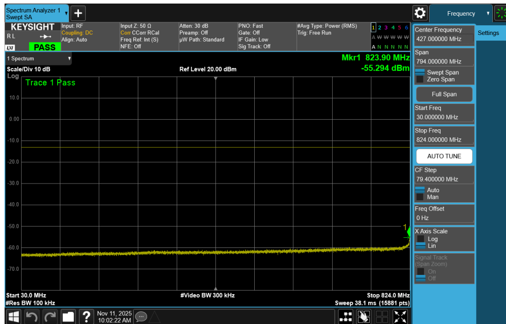
Plot 7-54. Conducted Spurious Plot (ULCA LTE Band 5 – (10 + 10)MHz QPSK – PCC 1/49 SCC 1/0 - Mid Channel)
