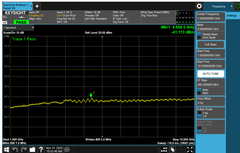
Plot 7-56. Conducted Spurious Plot (ULCA LTE Band 5 – (10 + 10)MHz QPSK – PCC 1/49 SCC 1/0 - Mid Channel)
