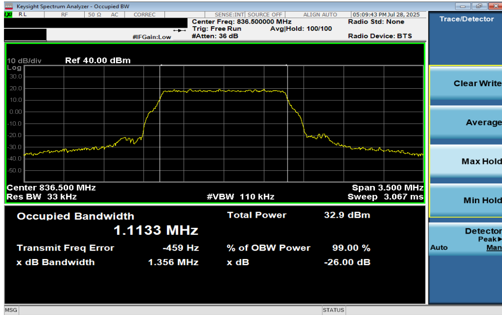
Plot 7-3. Occupied Bandwidth Plot (LTE Band 26/5 - 1.4MHz 64-QAM - Full RB Configuration)
