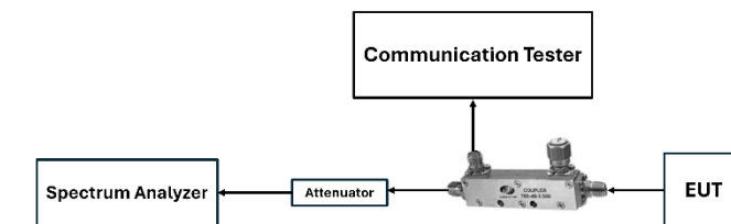
Figure 7-3. LTE Test Instrument & Measurement Setup
