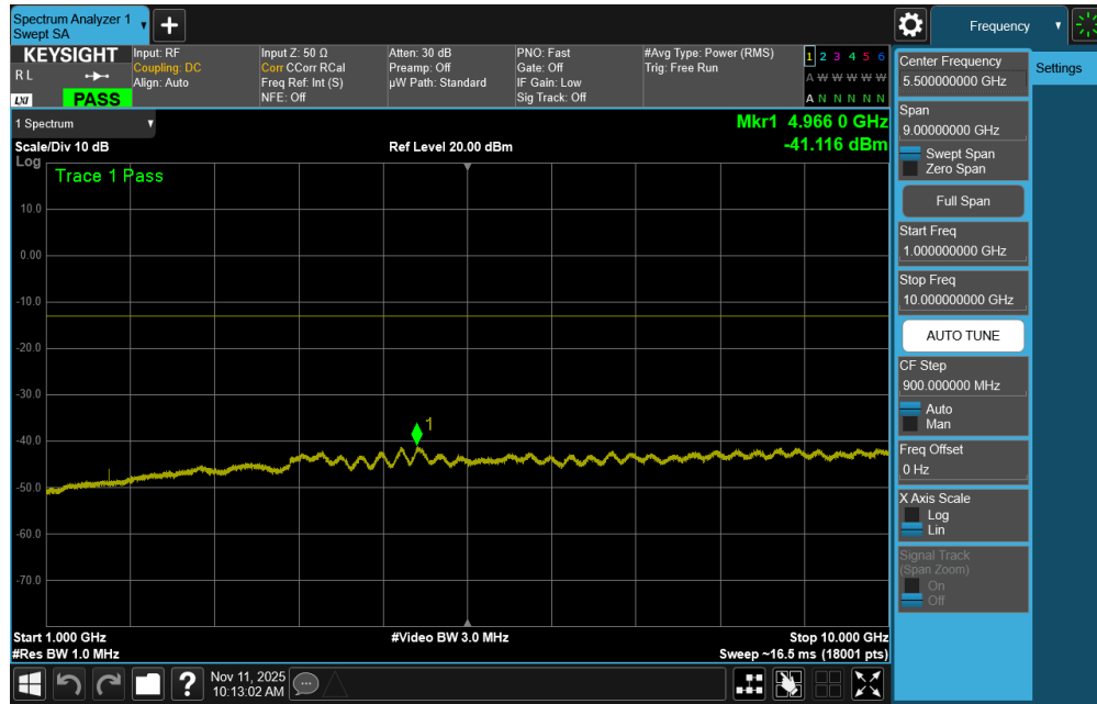
Plot 7-53. Conducted Spurious Plot (ULCA LTE Band 5 – (10 + 10)MHz QPSK – PCC 1/49 SCC 1/0 - Low Channel)
