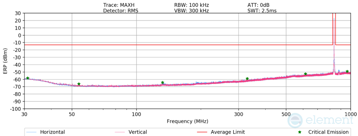
Plot 7-114. Antenna 2 Radiated Spurious Plot below 1GHz (LTE Band 26/5)
