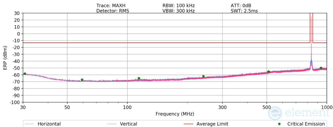
Plot 7-118. Antenna 2 Radiated Spurious Plot below 1GHz (NR Band n26/n5)
