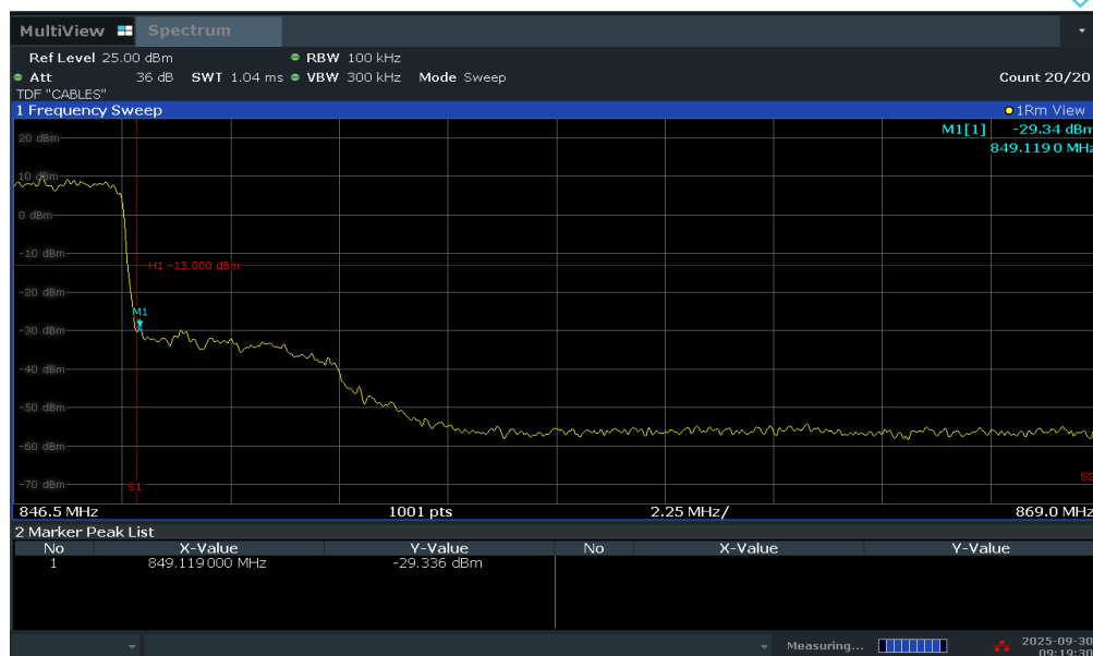
Plot 7-83. Upper BE Plot (LTE Band 26 - 5MHz QPSK – Full RB Configuration)
