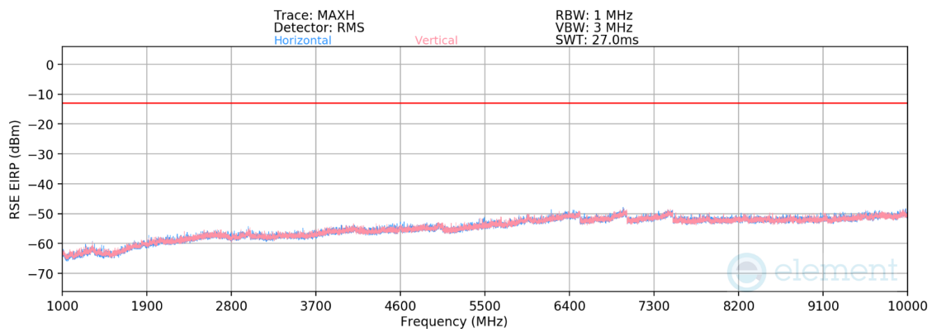
Plot 7-117. Antenna 2 Radiated Spurious Plot above 1GHz (ULCA LTE Band 5)
