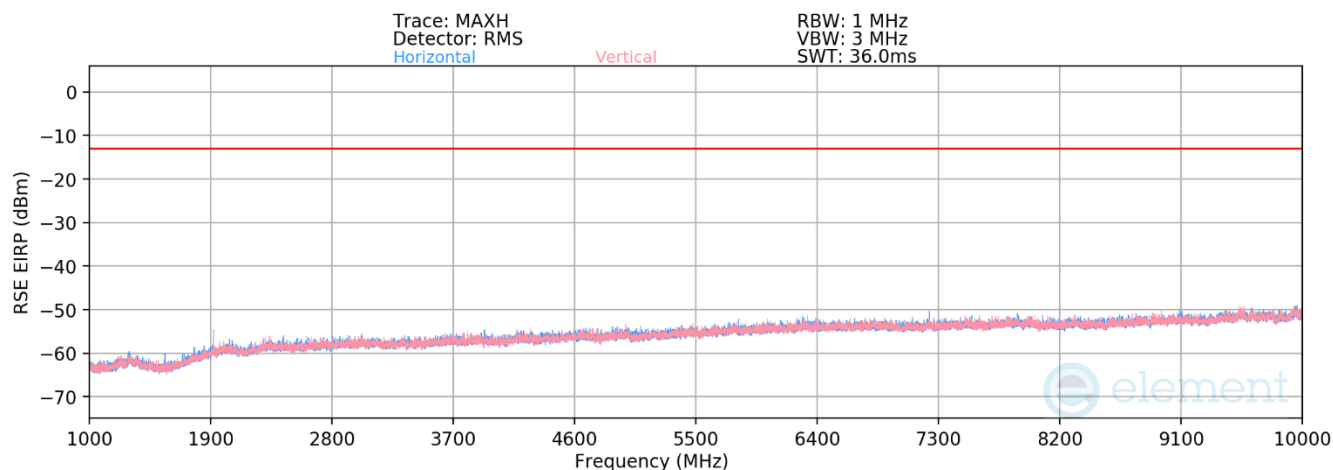
Plot 7-119. Antenna 2 Radiated Spurious Plot above 1GHz (NR Band n26/n5)
