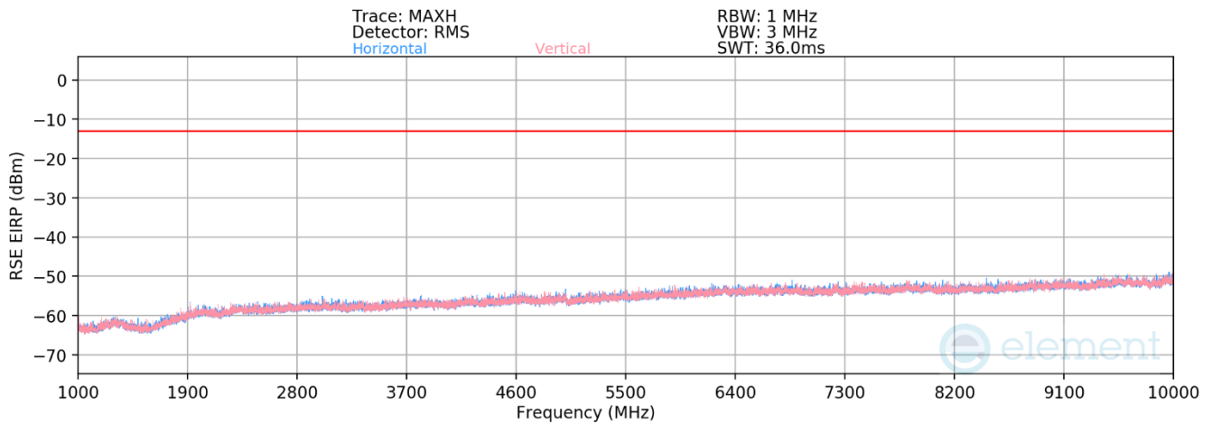
Plot 7-115. Antenna 2 Radiated Spurious Plot above 1GHz (LTE Band 26/5)
