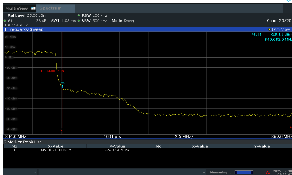
Plot 7-85. Upper BE Plot (LTE Band 26 - 10MHz QPSK – Full RB Configuration)
