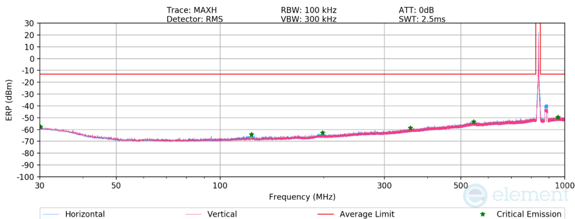
Plot 7-116. Antenna 2 Radiated Spurious Plot below 1GHz (ULCA LTE Band 5)
