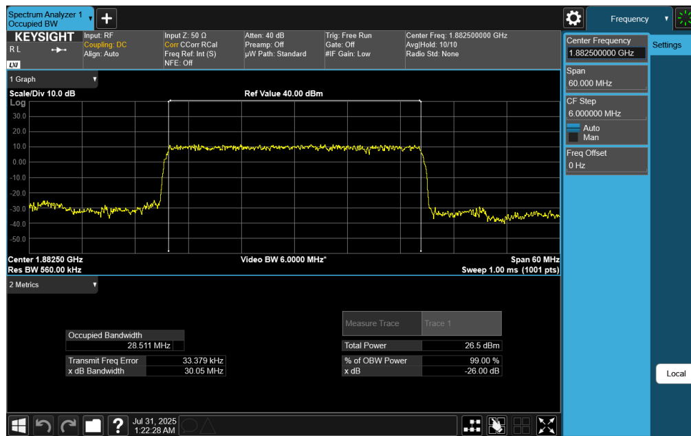
Plot 7-50. Occupied Bandwidth Plot (NR Band n25/n2 - 30MHz DFT-s-OFDM \pi/2 BPSK - Full RB)
