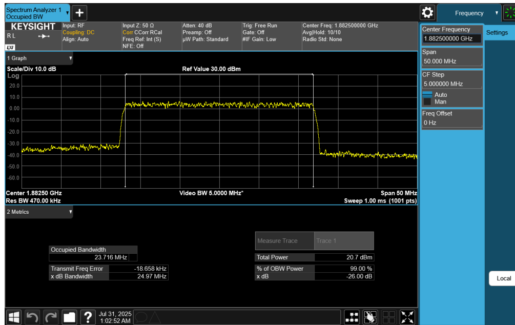
Plot 7-49. Occupied Bandwidth Plot (NR Band n25/n2 - 25MHz CP-OFDM 256QAM - Full RB)
