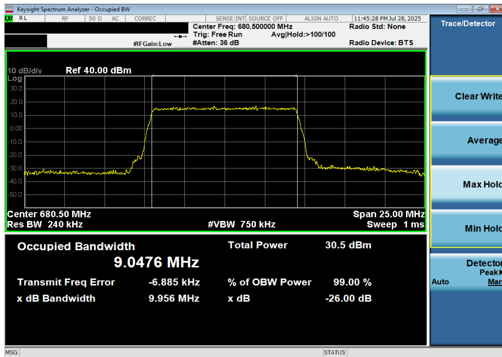
Plot 7-32. Occupied Bandwidth Plot (LTE Band 71 - 10MHz 256-QAM - Full RB)
