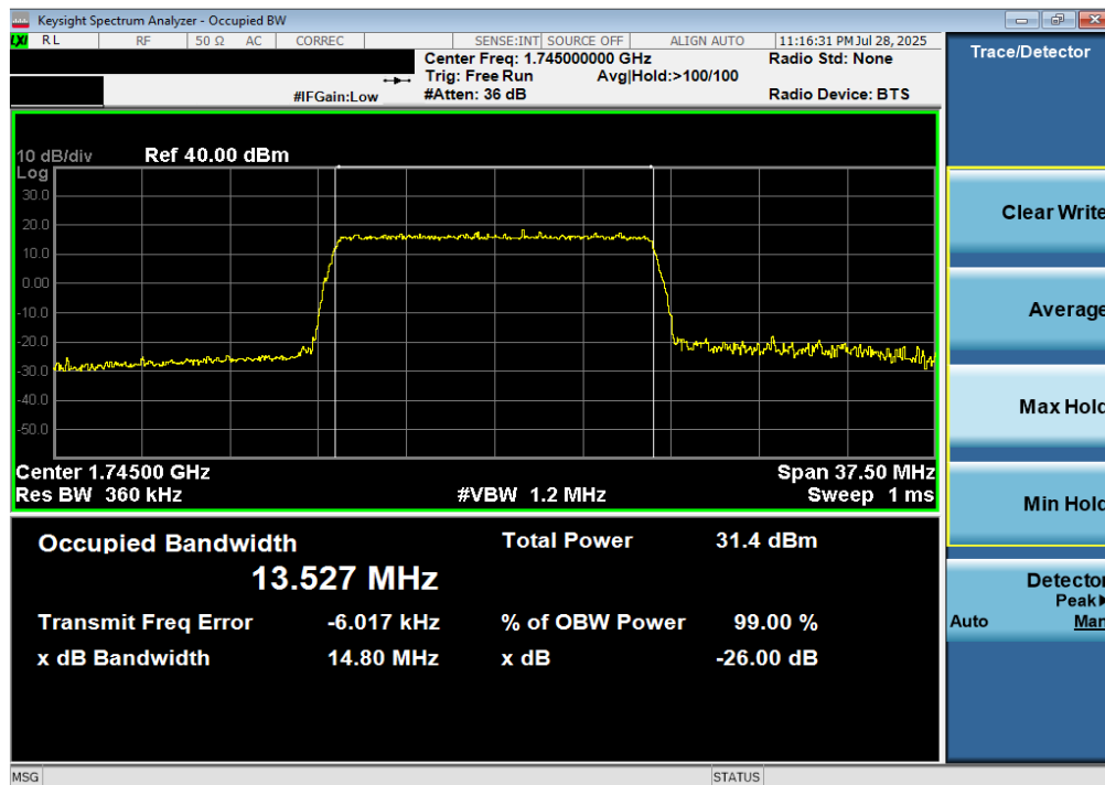
Plot 7-20. Occupied Bandwidth Plot (LTE Band 66/4 - 15MHz 256-QAM - Full RB)
