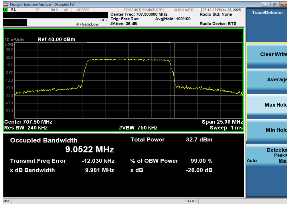
Plot 7-55. Occupied Bandwidth Plot (LTE Band 12/17 - 10MHz 64-QAM - Full RB)
