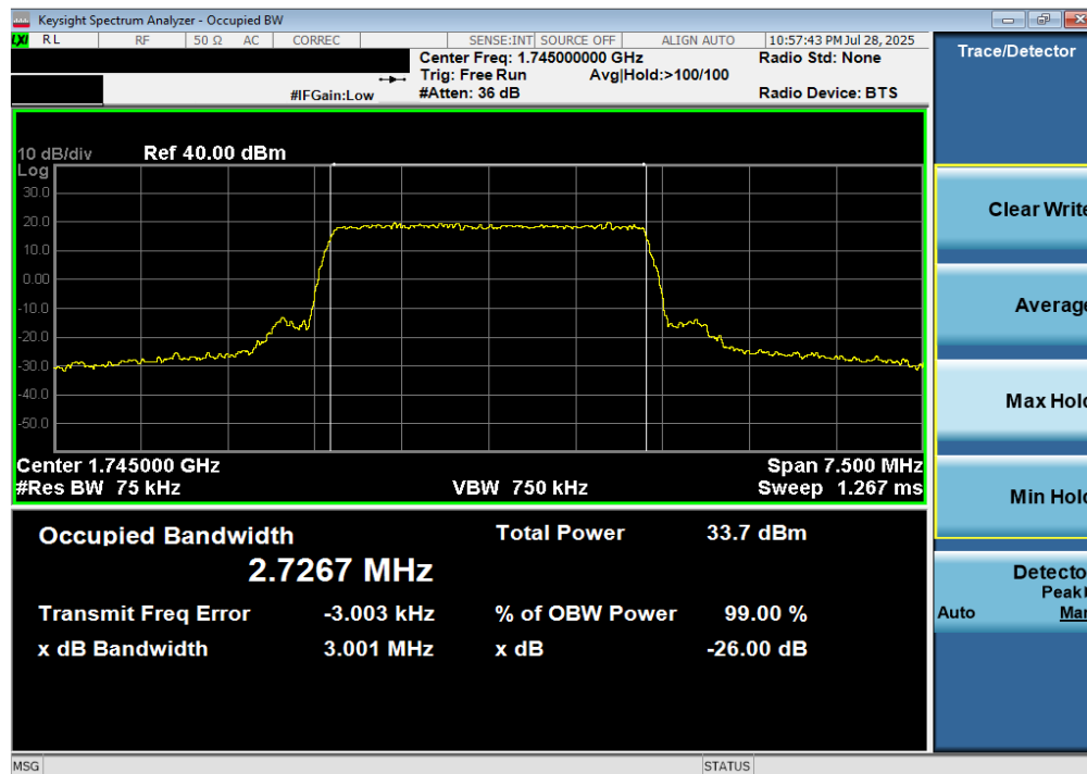
Plot 7-6. Occupied Bandwidth Plot (LTE Band 66/4 - 3MHz 16-QAM - Full RB)
