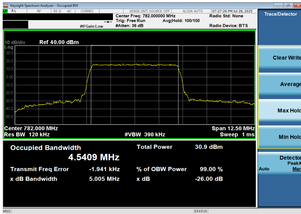
Plot 7-60. Occupied Bandwidth Plot (LTE Band 13 - 5MHz 256-QAM - Full RB)
