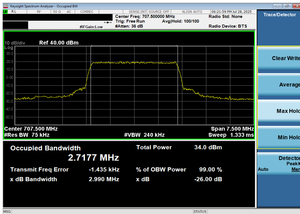
Plot 7-45. Occupied Bandwidth Plot (LTE Band 12 - 3MHz QPSK - Full RB)
