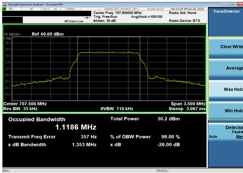
Plot 7-44. Occupied Bandwidth Plot (LTE Band 12 – 1.4MHz 256-QAM - Full RB)
