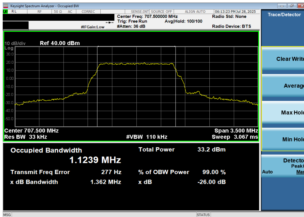
Plot 7-42. Occupied Bandwidth Plot (LTE Band 12 – 1.4MHz 16-QAM - Full RB)
