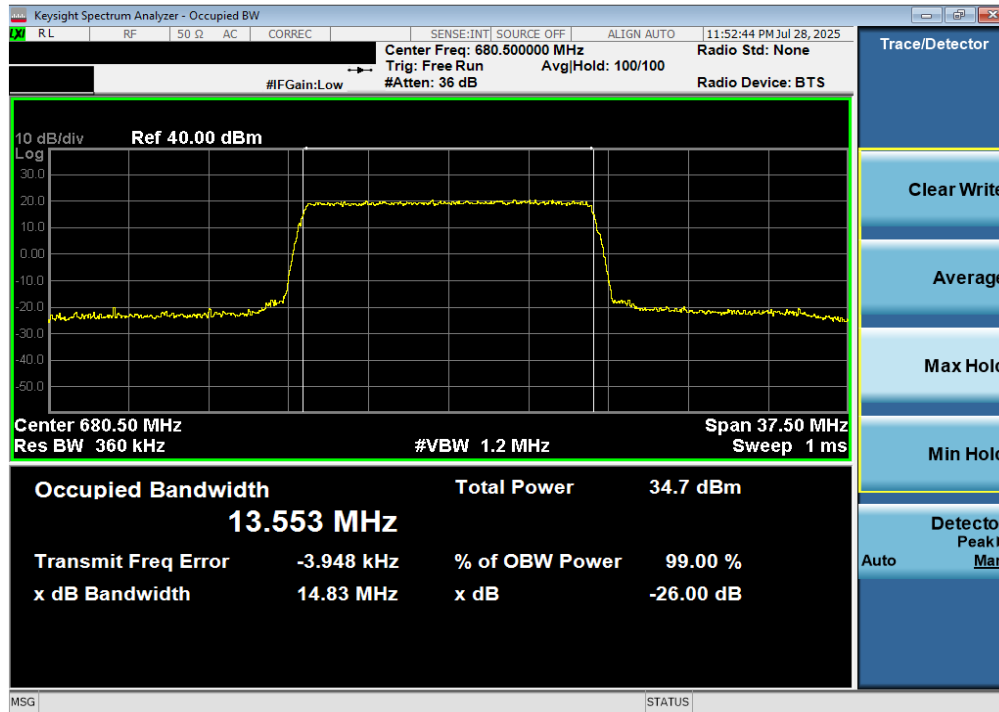
Plot 7-33. Occupied Bandwidth Plot (LTE Band 71 - 15MHz QPSK - Full RB)
