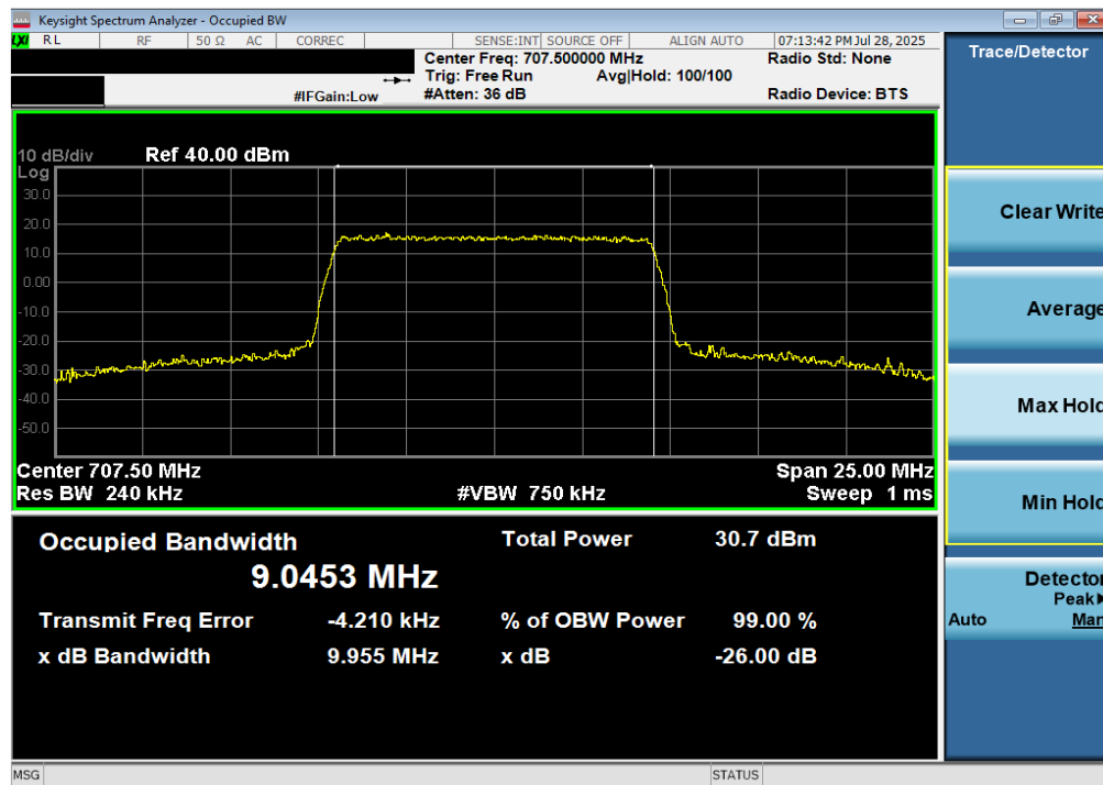
Plot 7-56. Occupied Bandwidth Plot (LTE Band 12/17 - 10MHz 256-QAM - Full RB)
