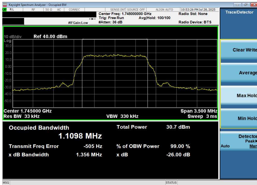
Plot 7-4. Occupied Bandwidth Plot (LTE Band 66/4 - 1.4MHz 256-QAM - Full RB)
