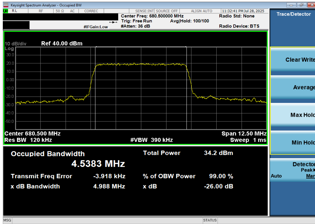
Plot 7-25. Occupied Bandwidth Plot (LTE Band 71 - 5MHz QPSK - Full RB)
