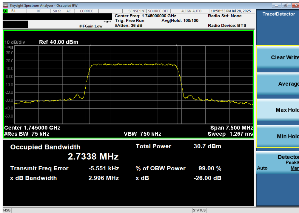
Plot 7-8. Occupied Bandwidth Plot (LTE Band 66/4 - 3MHz 256-QAM - Full RB)
