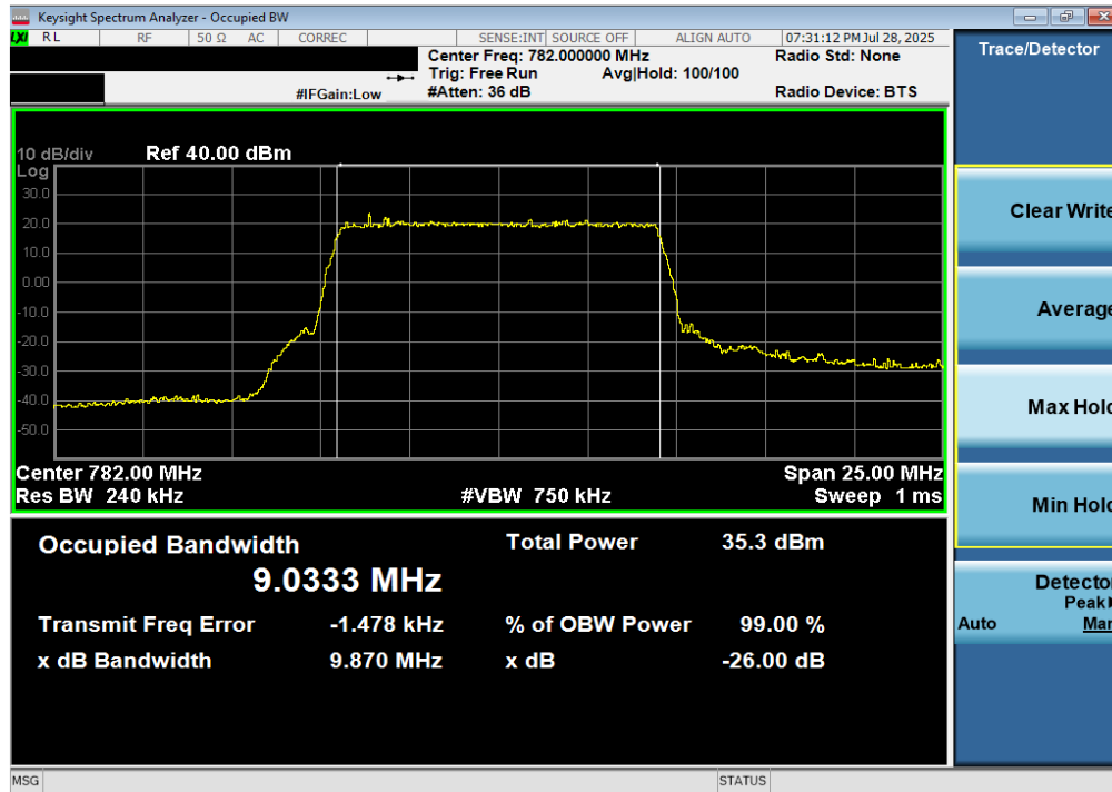
Plot 7-61. Occupied Bandwidth Plot (LTE Band 13 - 10MHz QPSK - Full RB)
