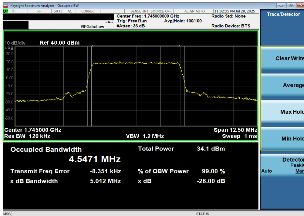
Plot 7-10. Occupied Bandwidth Plot (LTE Band 66/4 - 5MHz 16-QAM - Full RB)
