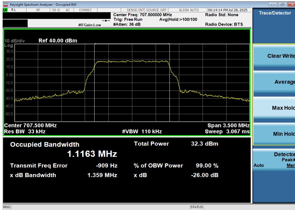
Plot 7-43. Occupied Bandwidth Plot (LTE Band 12 – 1.4MHz 64-QAM - Full RB)
