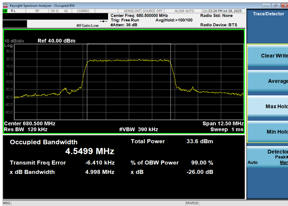
Plot 7-26. Occupied Bandwidth Plot (LTE Band 71 - 5MHz 16-QAM - Full RB)
