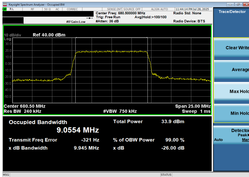
Plot 7-30. Occupied Bandwidth Plot (LTE Band 71 - 10MHz 16-QAM - Full RB)
