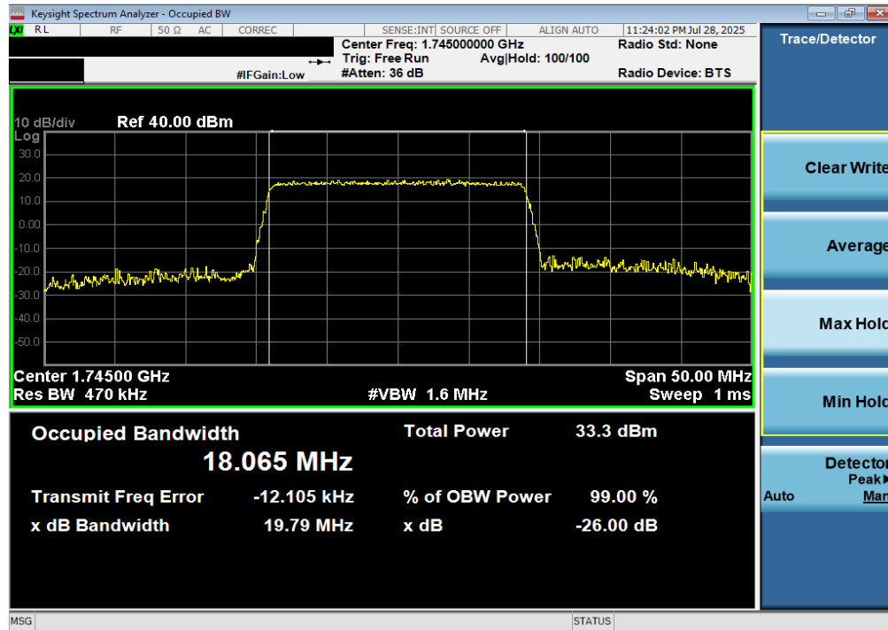
Plot 7-23. Occupied Bandwidth Plot (LTE Band 66/4 - 20MHz 64-QAM - Full RB)
