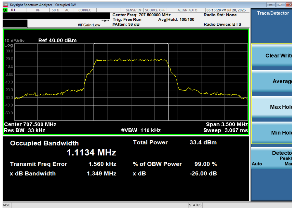
Plot 7-41. Occupied Bandwidth Plot (LTE Band 12 – 1.4MHz QPSK - Full RB)
