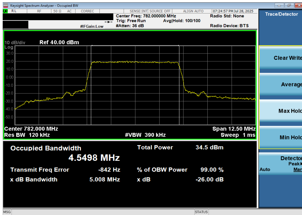
Plot 7-58. Occupied Bandwidth Plot (LTE Band 13 - 5MHz 16-QAM - Full RB)
