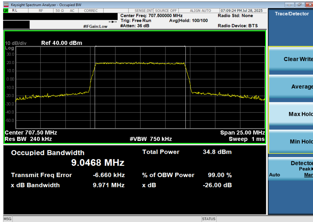
Plot 7-53. Occupied Bandwidth Plot (LTE Band 12/17 - 10MHz QPSK - Full RB)
