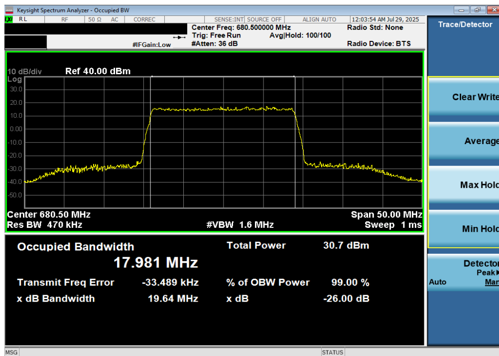
Plot 7-40. Occupied Bandwidth Plot (LTE Band 71 - 20MHz 256-QAM - Full RB)
