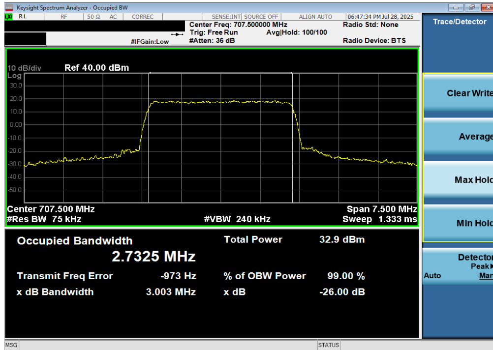
Plot 7-47. Occupied Bandwidth Plot (LTE Band 12 - 3MHz 64-QAM - Full RB)
