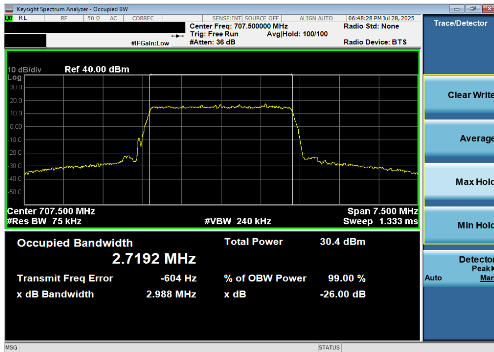
Plot 7-48. Occupied Bandwidth Plot (LTE Band 12 - 3MHz 256-QAM - Full RB)
