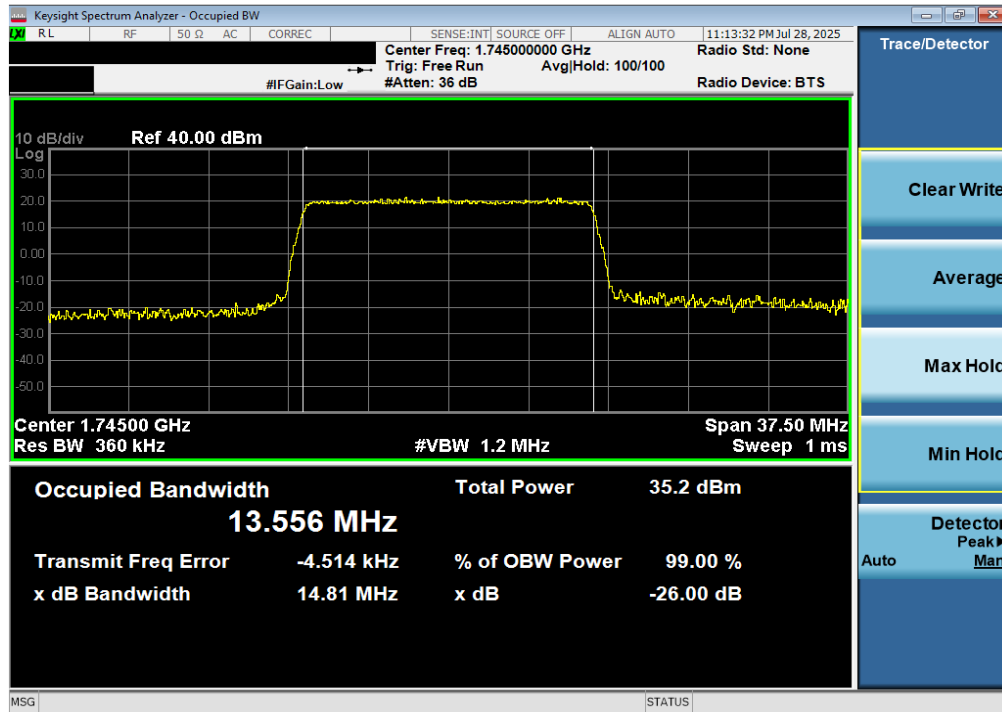
Plot 7-17. Occupied Bandwidth Plot (LTE Band 66/4 - 15MHz QPSK - Full RB)
