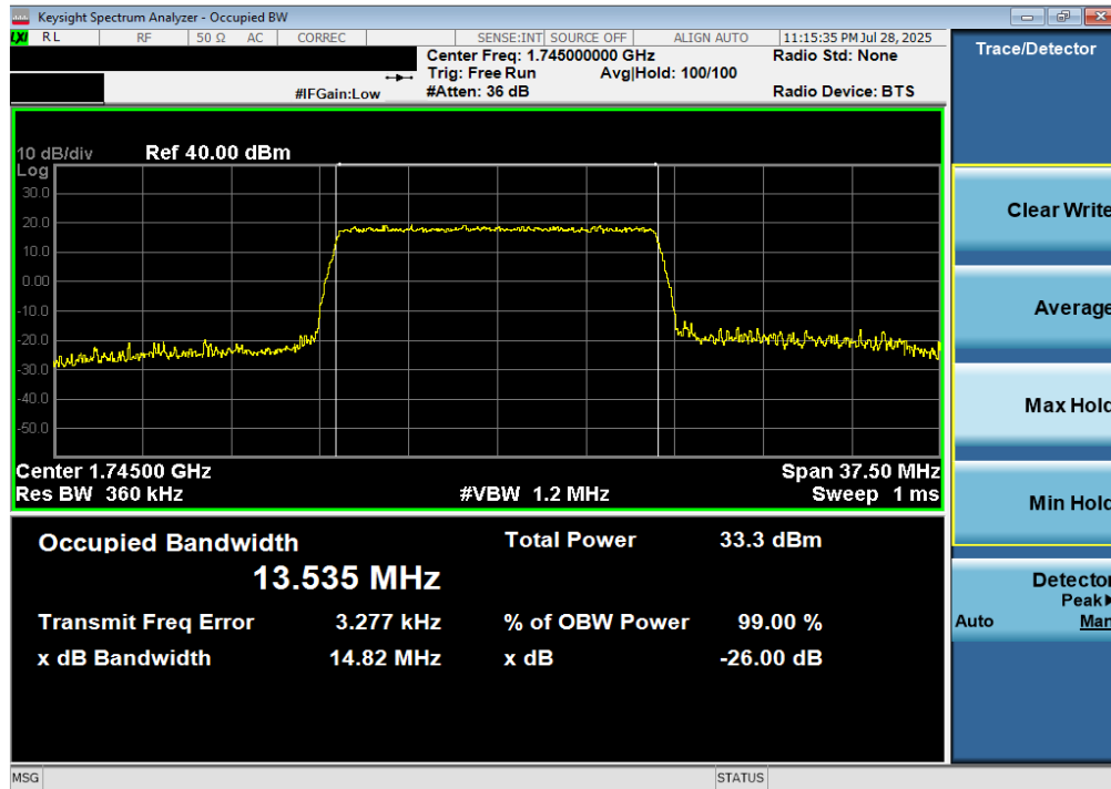
Plot 7-19. Occupied Bandwidth Plot (LTE Band 66/4 - 15MHz 64-QAM - Full RB)
