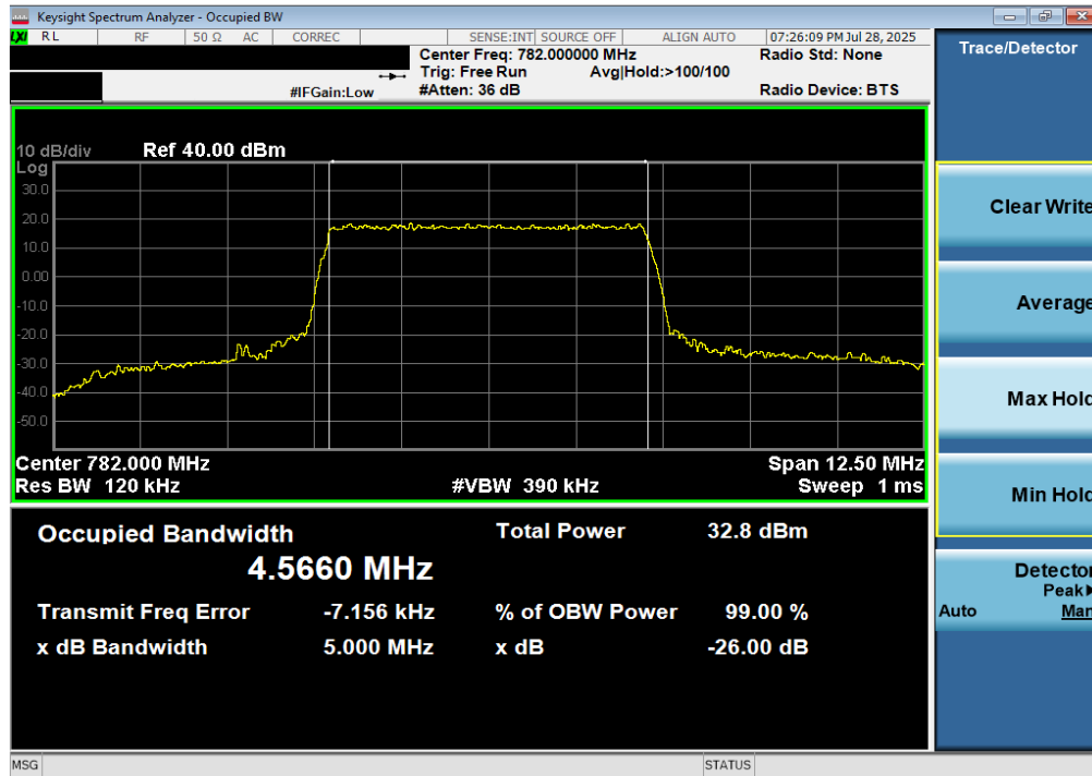
Plot 7-59. Occupied Bandwidth Plot (LTE Band 13 - 5MHz 64-QAM - Full RB)
