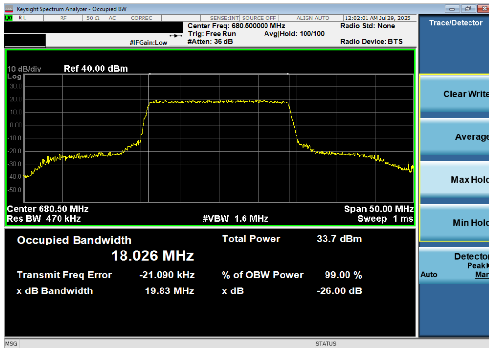
Plot 7-38. Occupied Bandwidth Plot (LTE Band 71 - 20MHz 16-QAM - Full RB)
