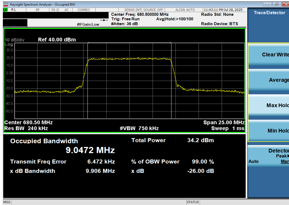
Plot 7-29. Occupied Bandwidth Plot (LTE Band 71 - 10MHz QPSK - Full RB)
