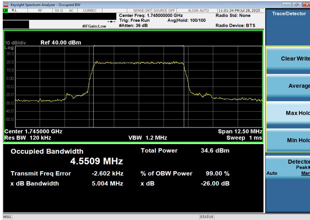
Plot 7-9. Occupied Bandwidth Plot (LTE Band 66/4 - 5MHz QPSK - Full RB)
