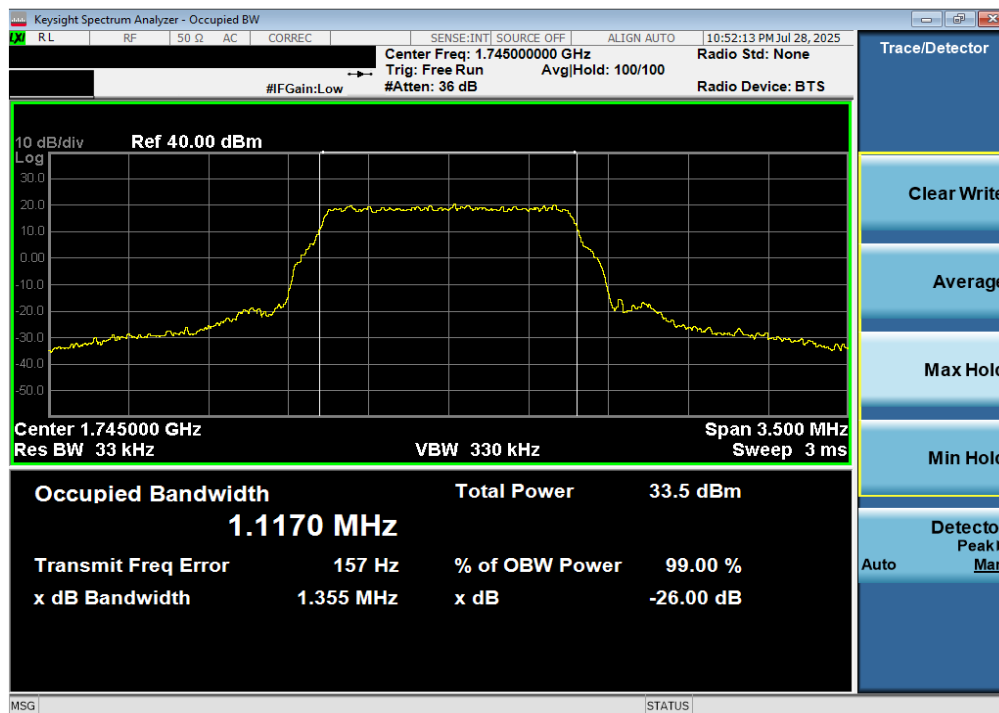
Plot 7-2. Occupied Bandwidth Plot (LTE Band 66/4 - 1.4MHz 16-QAM - Full RB)
