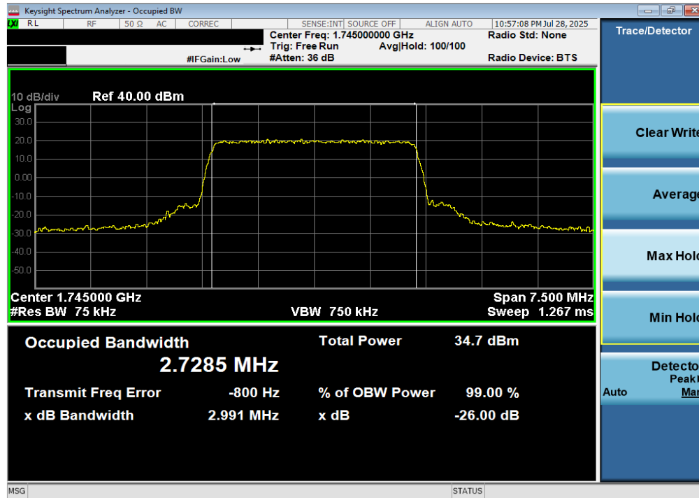
Plot 7-5. Occupied Bandwidth Plot (LTE Band 66/4 - 3MHz QPSK - Full RB)
