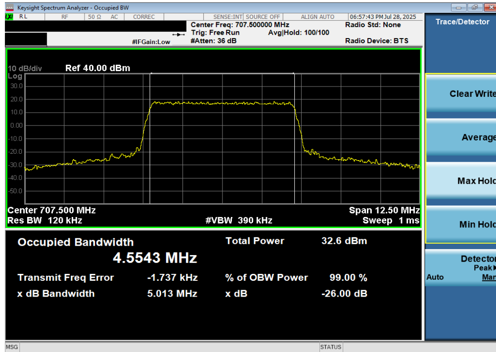
Plot 7-51. Occupied Bandwidth Plot (LTE Band 12/17 - 5MHz 64-QAM - Full RB)
