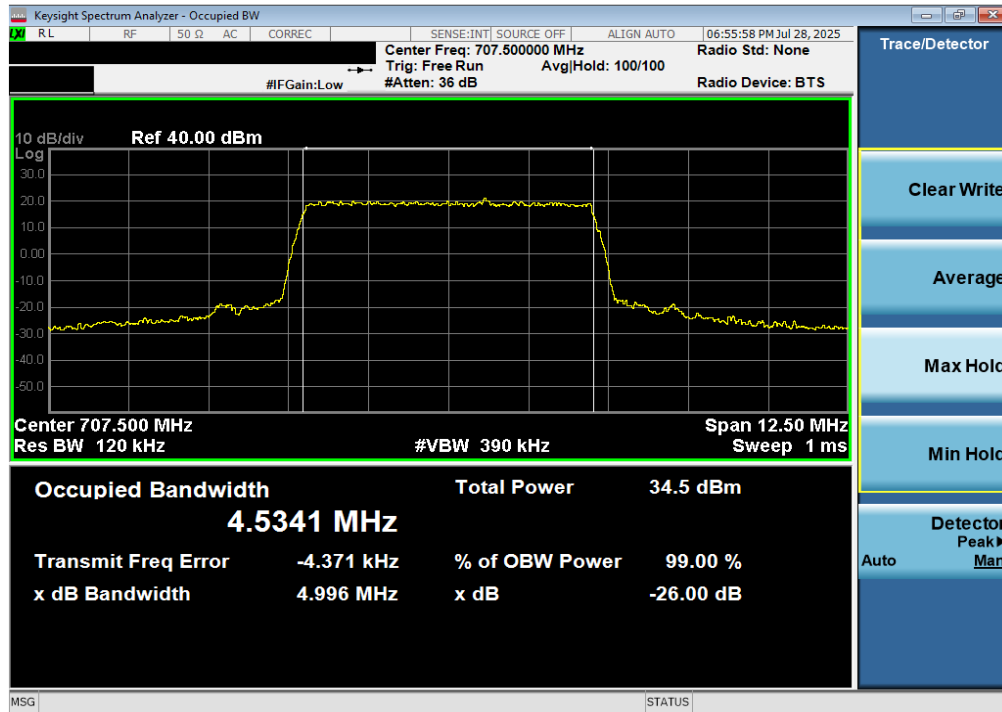
Plot 7-49. Occupied Bandwidth Plot (LTE Band 12/17 - 5MHz QPSK - Full RB)
