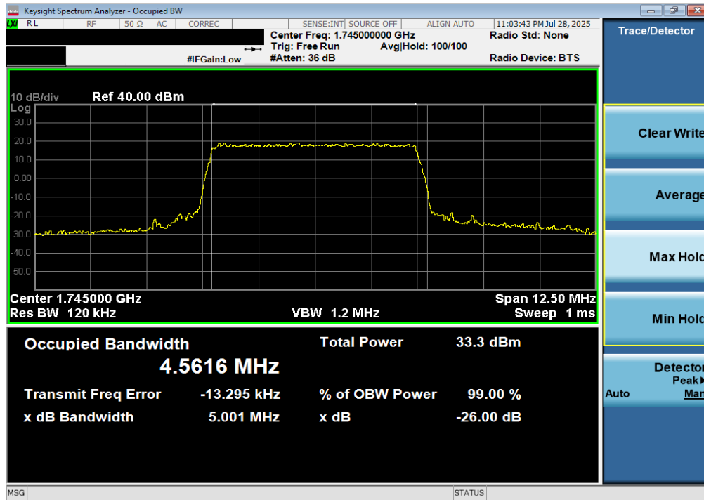
Plot 7-11. Occupied Bandwidth Plot (LTE Band 66/4 - 5MHz 64-QAM - Full RB)
