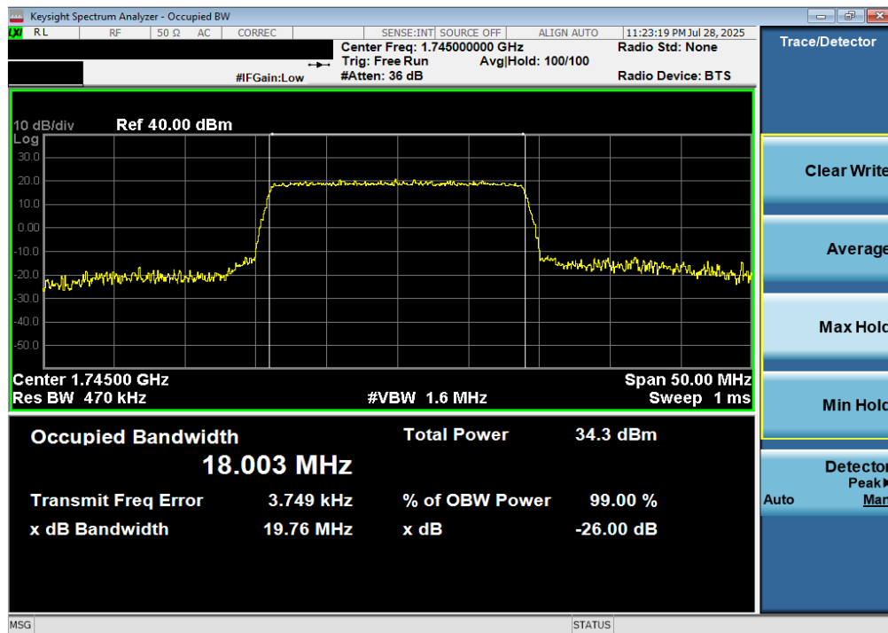
Plot 7-22. Occupied Bandwidth Plot (LTE Band 66/4 - 20MHz 16-QAM - Full RB)
