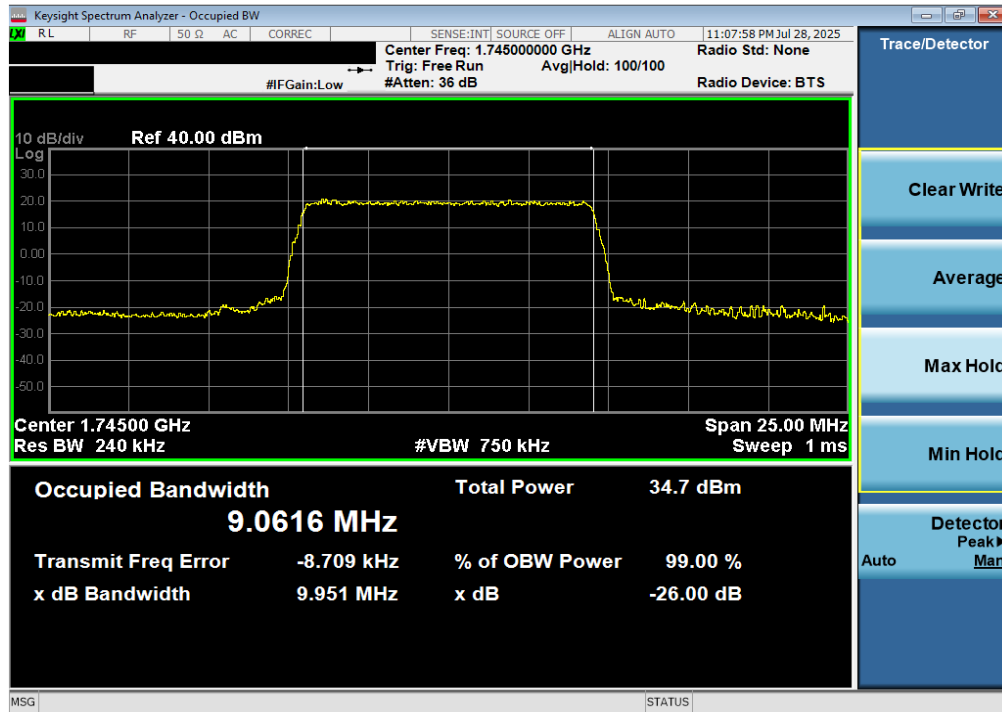
Plot 7-13. Occupied Bandwidth Plot (LTE Band 66/4 - 10MHz QPSK - Full RB)
