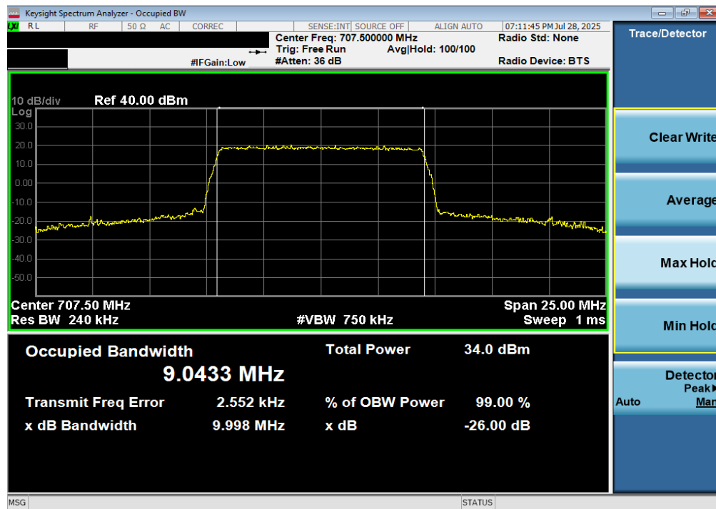
Plot 7-54. Occupied Bandwidth Plot (LTE Band 12/17 - 10MHz 16-QAM - Full RB)
