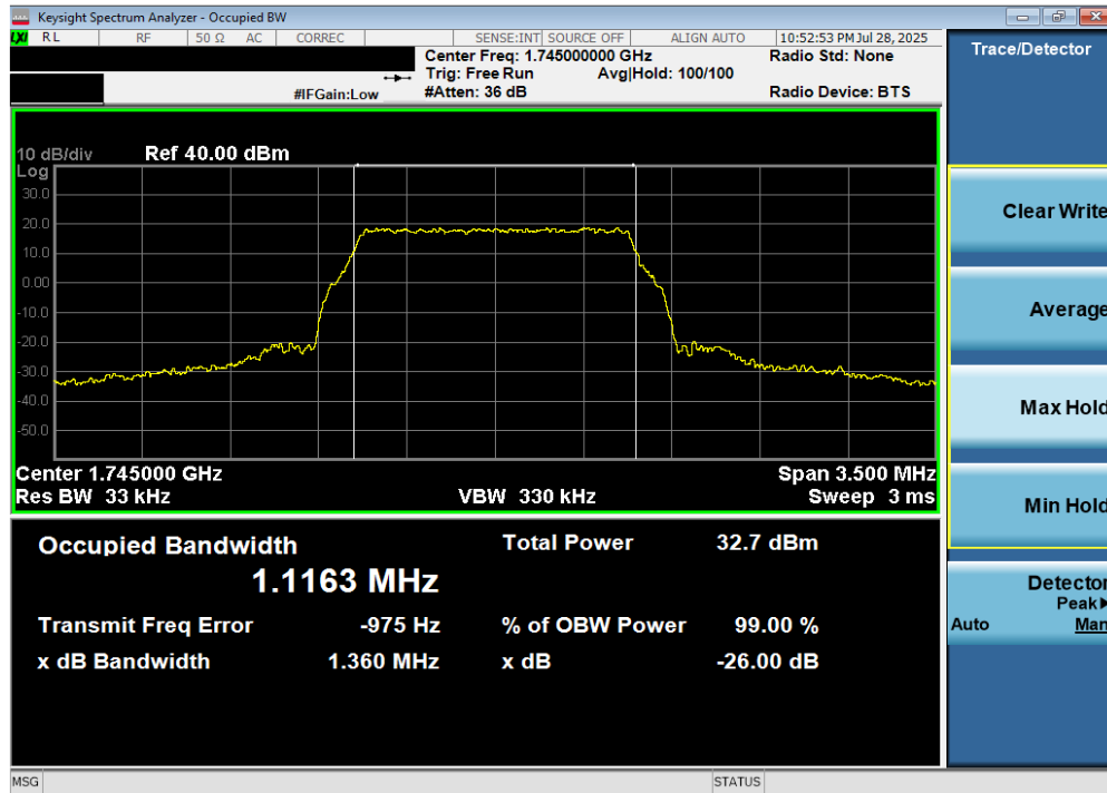
Plot 7-3. Occupied Bandwidth Plot (LTE Band 66/4 - 1.4MHz 64-QAM - Full RB)
