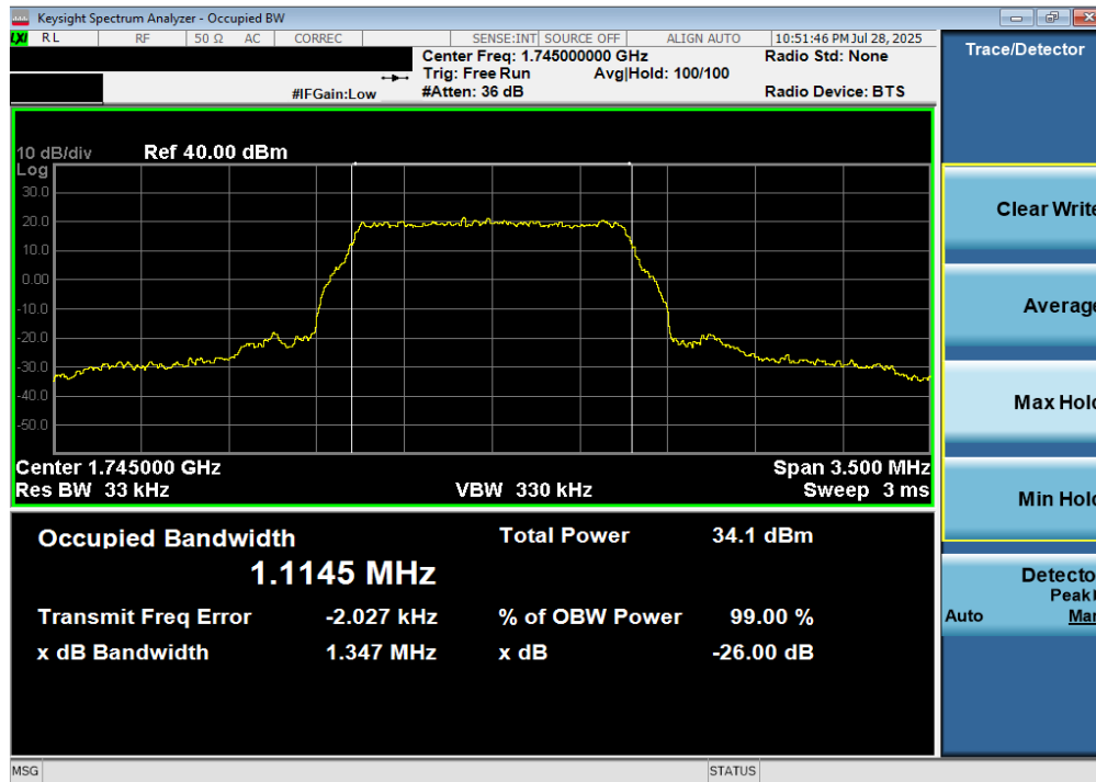
Plot 7-1. Occupied Bandwidth Plot (LTE Band 66/4 - 1.4MHz QPSK - Full RB)
