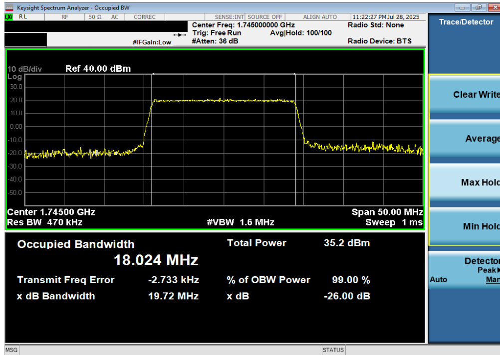
Plot 7-21. Occupied Bandwidth Plot (LTE Band 66/4 - 20MHz QPSK - Full RB)
