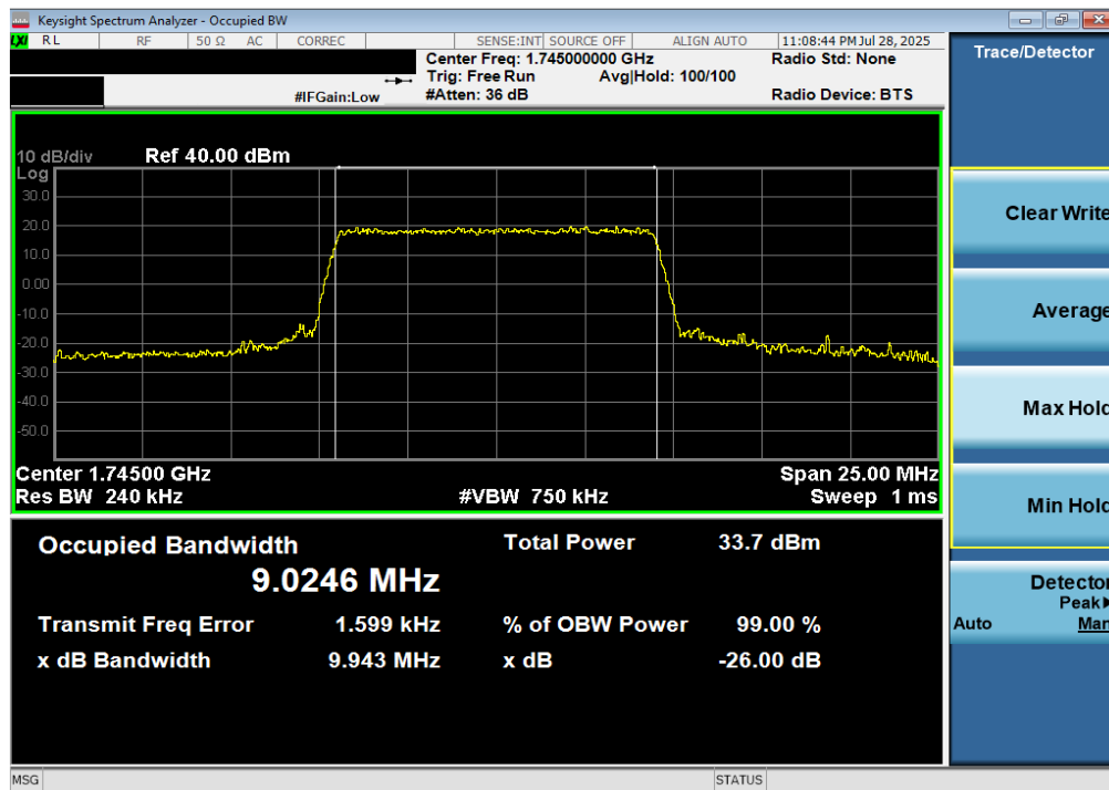
Plot 7-14. Occupied Bandwidth Plot (LTE Band 66/4 - 10MHz 16-QAM - Full RB)
