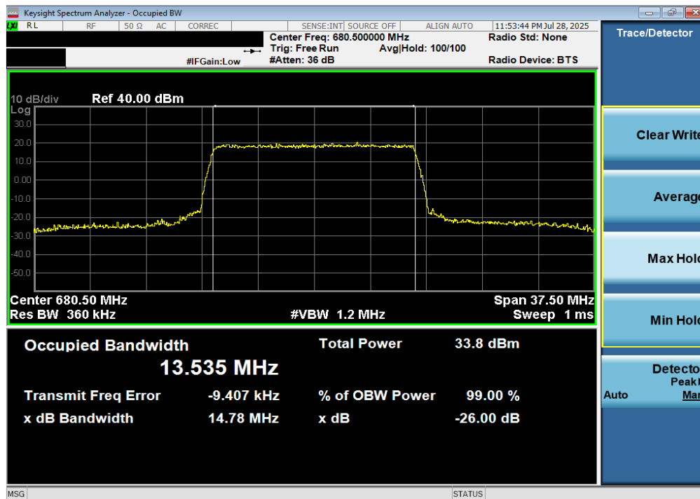
Plot 7-34. Occupied Bandwidth Plot (LTE Band 71 - 15MHz 16-QAM - Full RB)
