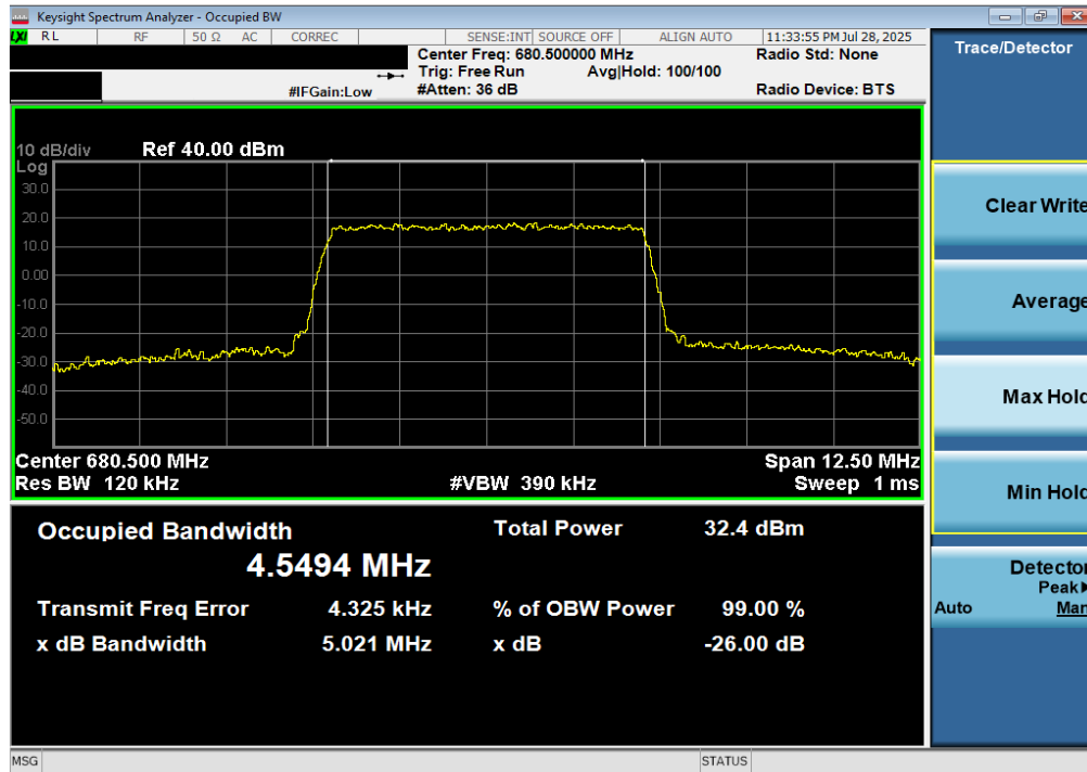
Plot 7-27. Occupied Bandwidth Plot (LTE Band 71 - 5MHz 64-QAM - Full RB)
