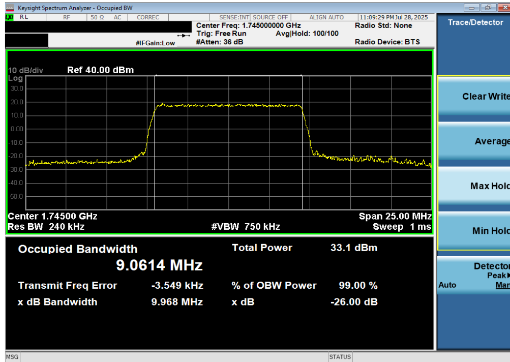
Plot 7-15. Occupied Bandwidth Plot (LTE Band 66/4 - 10MHz 64-QAM - Full RB)
