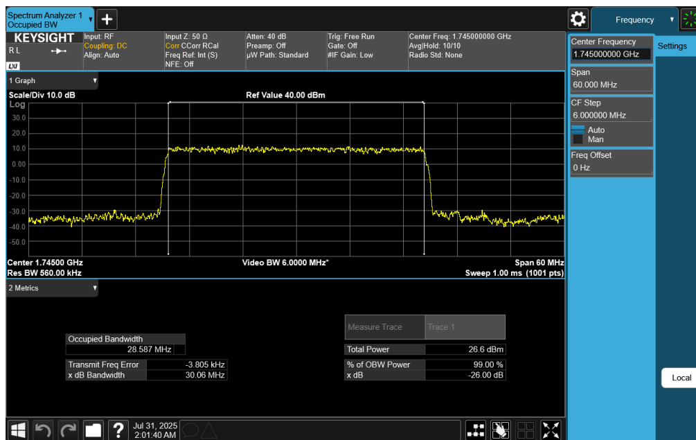
Plot 7-90. Occupied Bandwidth Plot (NR Band n66 - 30MHz DFT-s-OFDM π/2 BPSK - Full RB)
