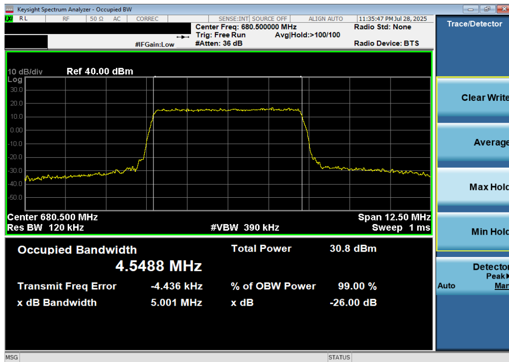
Plot 7-28. Occupied Bandwidth Plot (LTE Band 71 - 5MHz 256-QAM - Full RB)
