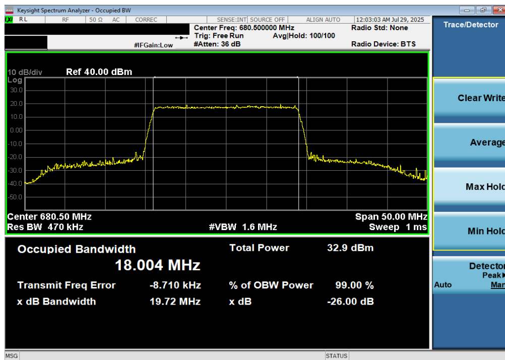
Plot 7-39. Occupied Bandwidth Plot (LTE Band 71 - 20MHz 64-QAM - Full RB)
