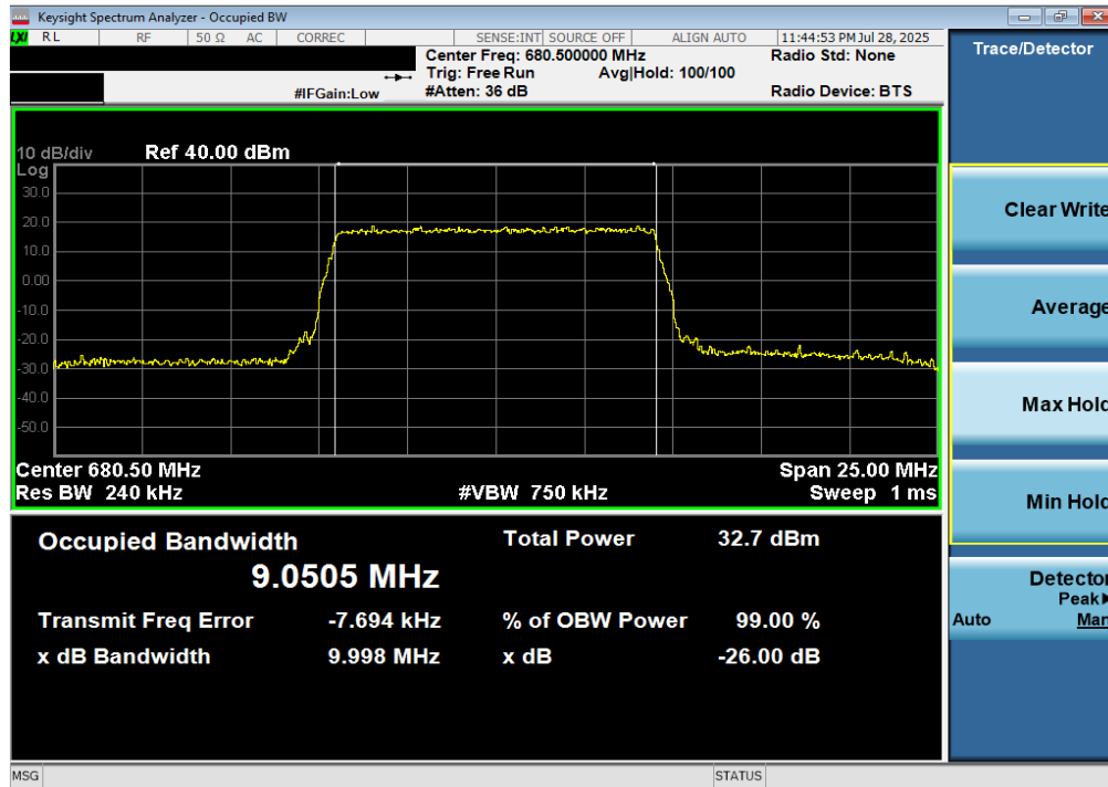
Plot 7-31. Occupied Bandwidth Plot (LTE Band 71 - 10MHz 64-QAM - Full RB)
