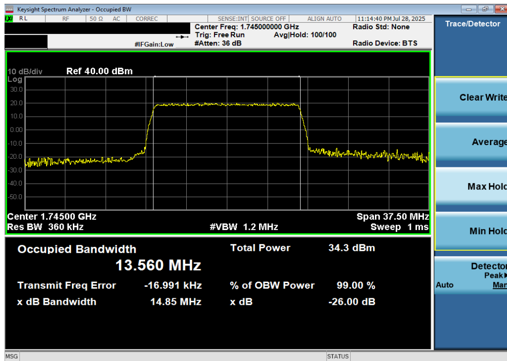
Plot 7-18. Occupied Bandwidth Plot (LTE Band 66/4 - 15MHz 16-QAM - Full RB)
