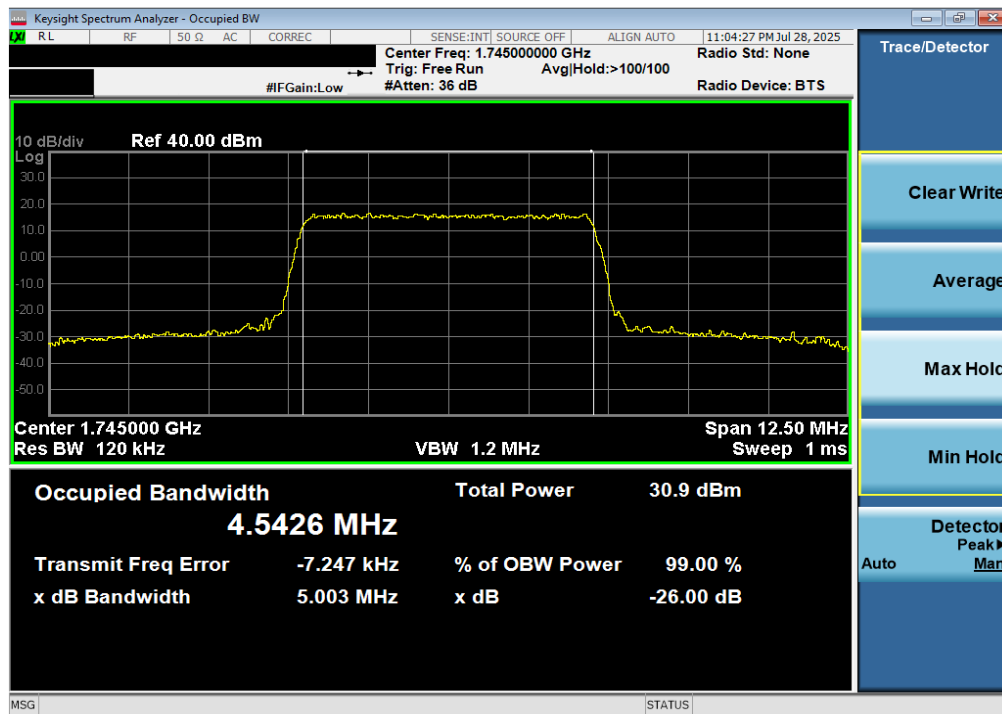
Plot 7-12. Occupied Bandwidth Plot (LTE Band 66/4 - 5MHz 256-QAM - Full RB)
