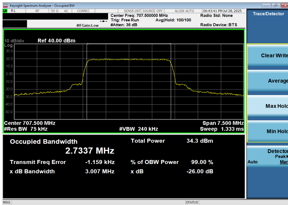
Plot 7-46. Occupied Bandwidth Plot (LTE Band 12 - 3MHz 16-QAM - Full RB)
