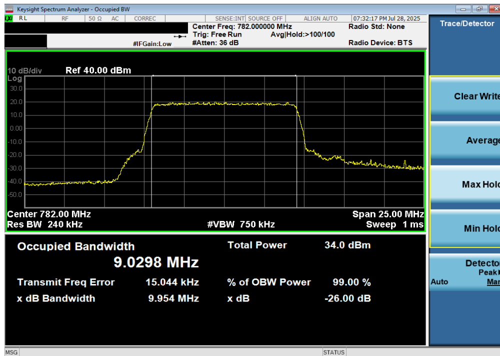
Plot 7-62. Occupied Bandwidth Plot (LTE Band 13 - 10MHz 16-QAM - Full RB)
