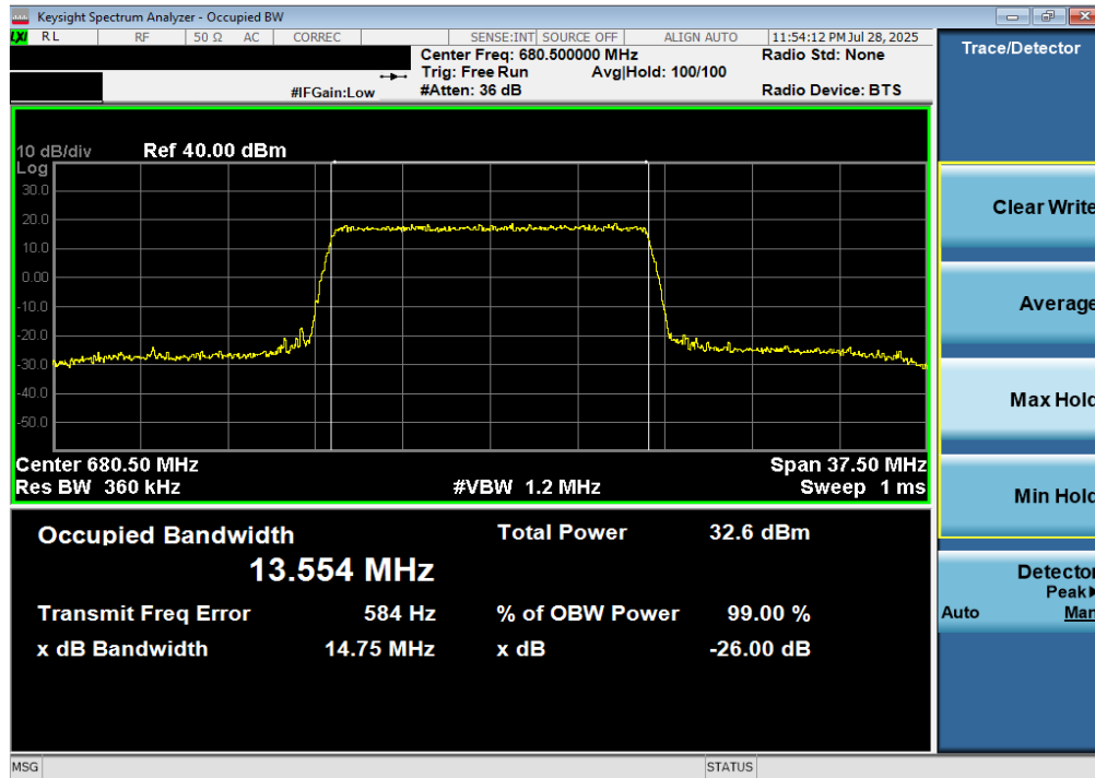
Plot 7-35. Occupied Bandwidth Plot (LTE Band 71 - 15MHz 64-QAM - Full RB)
