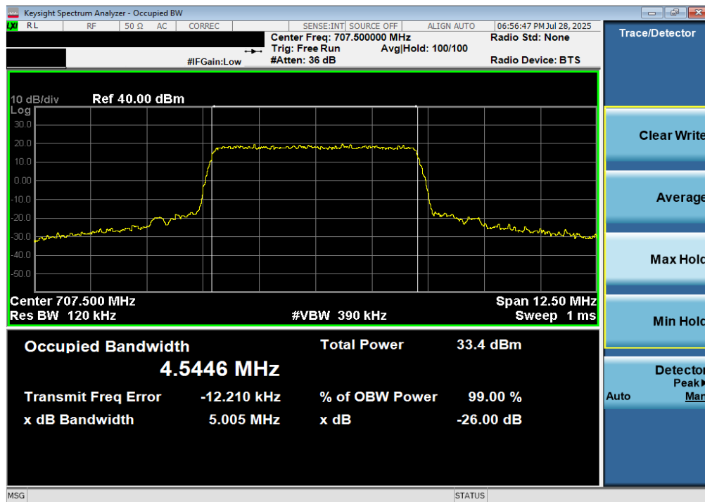
Plot 7-50. Occupied Bandwidth Plot (LTE Band 12/17 - 5MHz 16-QAM - Full RB)
