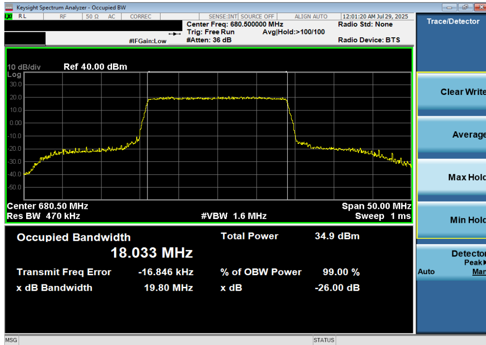
Plot 7-37. Occupied Bandwidth Plot (LTE Band 71 - 20MHz QPSK - Full RB)
