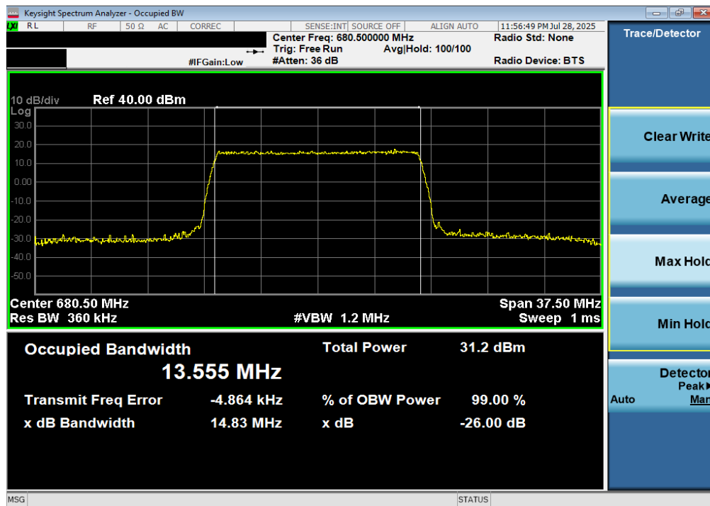
Plot 7-36. Occupied Bandwidth Plot (LTE Band 71 - 15MHz 256-QAM - Full RB)
