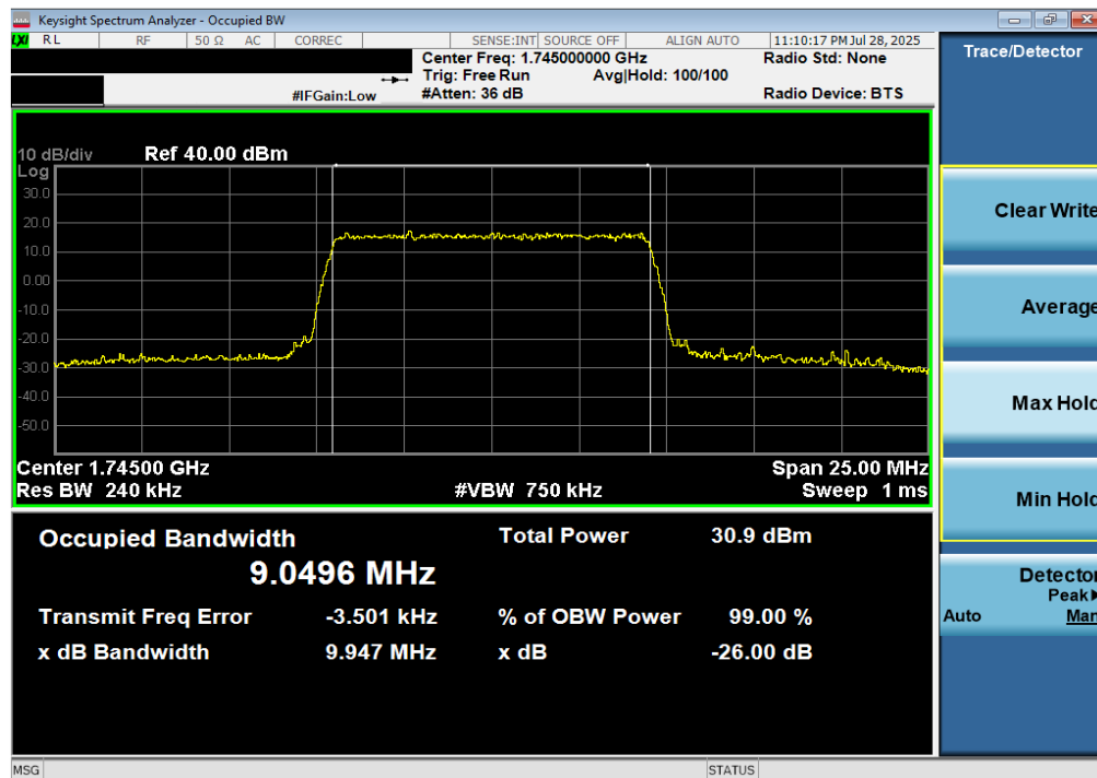
Plot 7-16. Occupied Bandwidth Plot (LTE Band 66/4 - 10MHz 256-QAM - Full RB)
