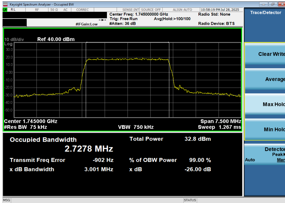
Plot 7-7. Occupied Bandwidth Plot (LTE Band 66/4 - 3MHz 64-QAM - Full RB)
