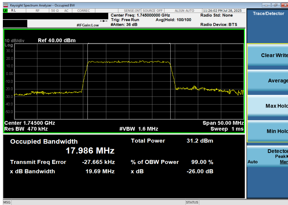
Plot 7-24. Occupied Bandwidth Plot (LTE Band 66/4 - 20MHz 256-QAM - Full RB)
