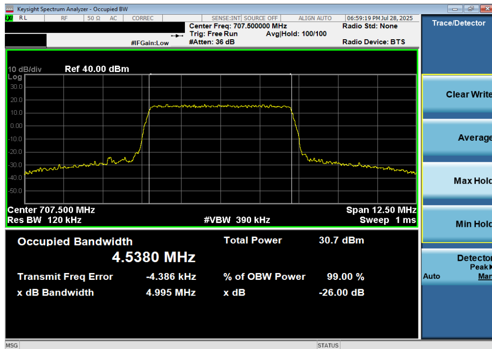
Plot 7-52. Occupied Bandwidth Plot (LTE Band 12/17 - 5MHz 256-QAM - Full RB)
