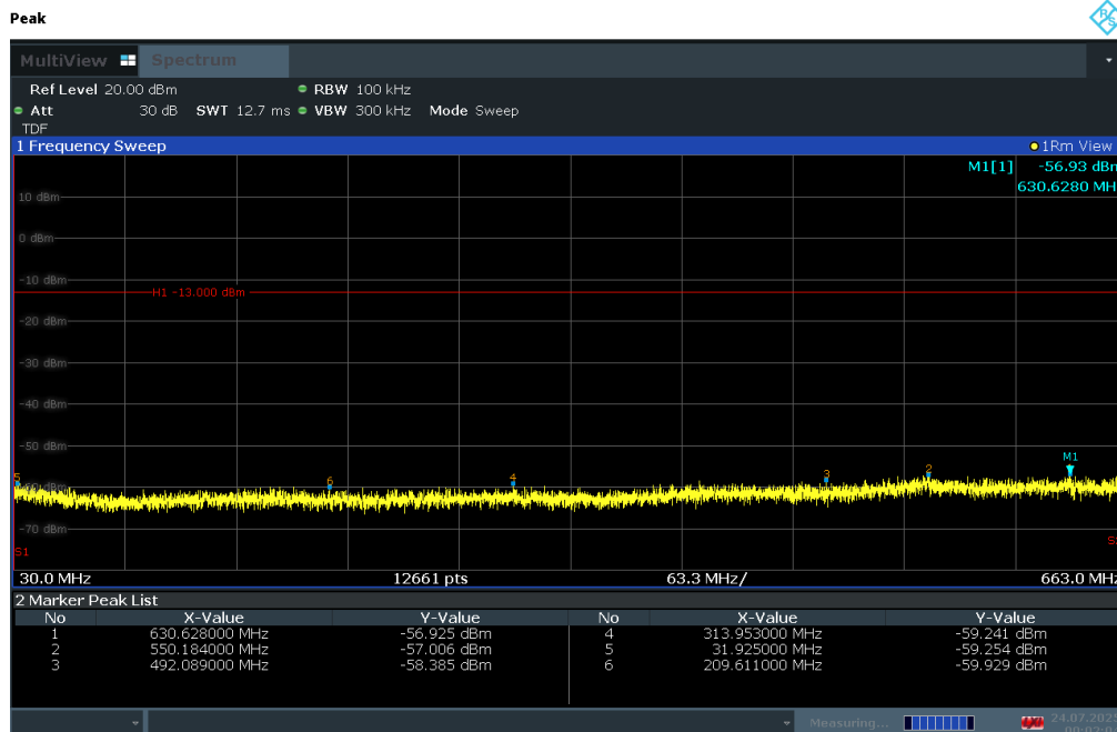
Plot 7-176. Conducted Spurious Plot (LTE Band 71 - 20MHz QPSK - RB Size 1, RB Offset 0 - High Channel)
