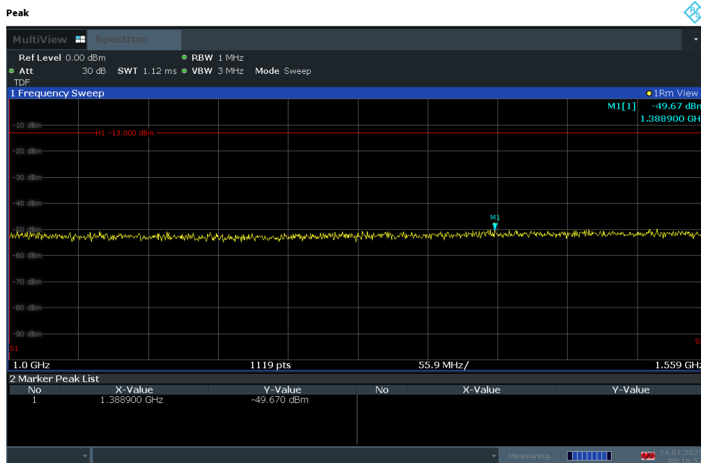
Plot 7-193. Conducted Spurious Plot (LTE Band 13 - 10MHz QPSK - RB Size 1, RB Offset 0)
