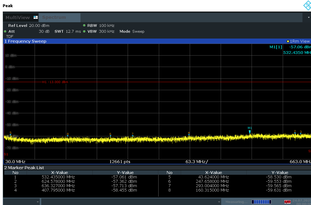
Plot 7-173. Conducted Spurious Plot (LTE Band 71 - 20MHz QPSK - RB Size 1, RB Offset 0 - Mid Channel)
