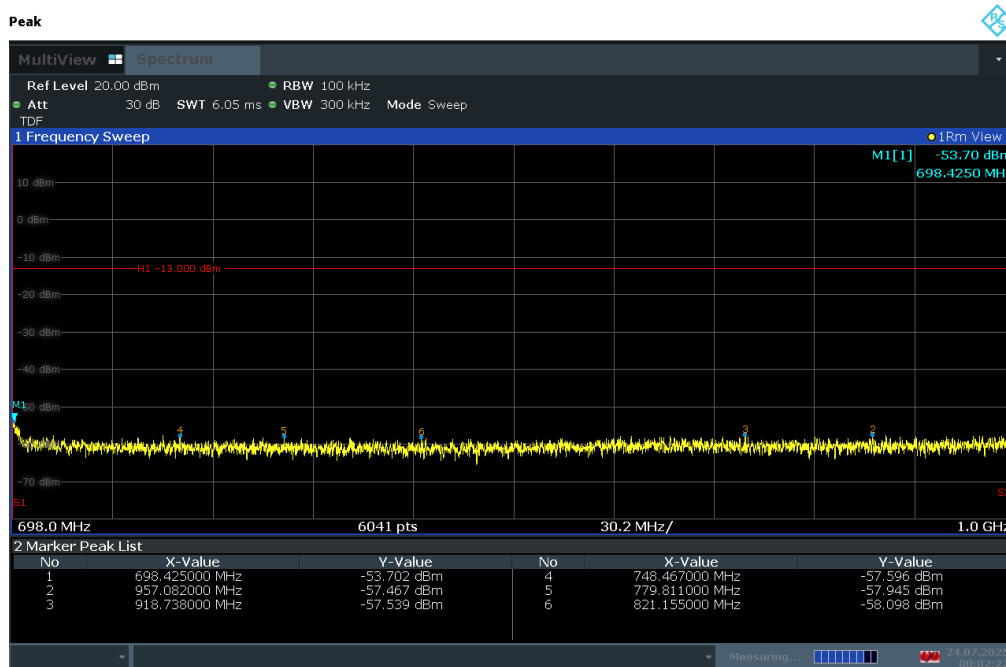
Plot 7-177. Conducted Spurious Plot (LTE Band 71 - 20MHz QPSK - RB Size 1, RB Offset 0 - High Channel)
