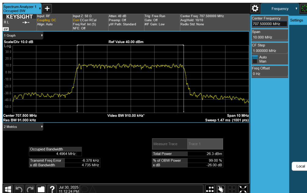
Plot 7-145. Occupied Bandwidth Plot (NR Band n12 - 5MHz DFT-s-OFDM \pi/2 BPSK - Full RB)
