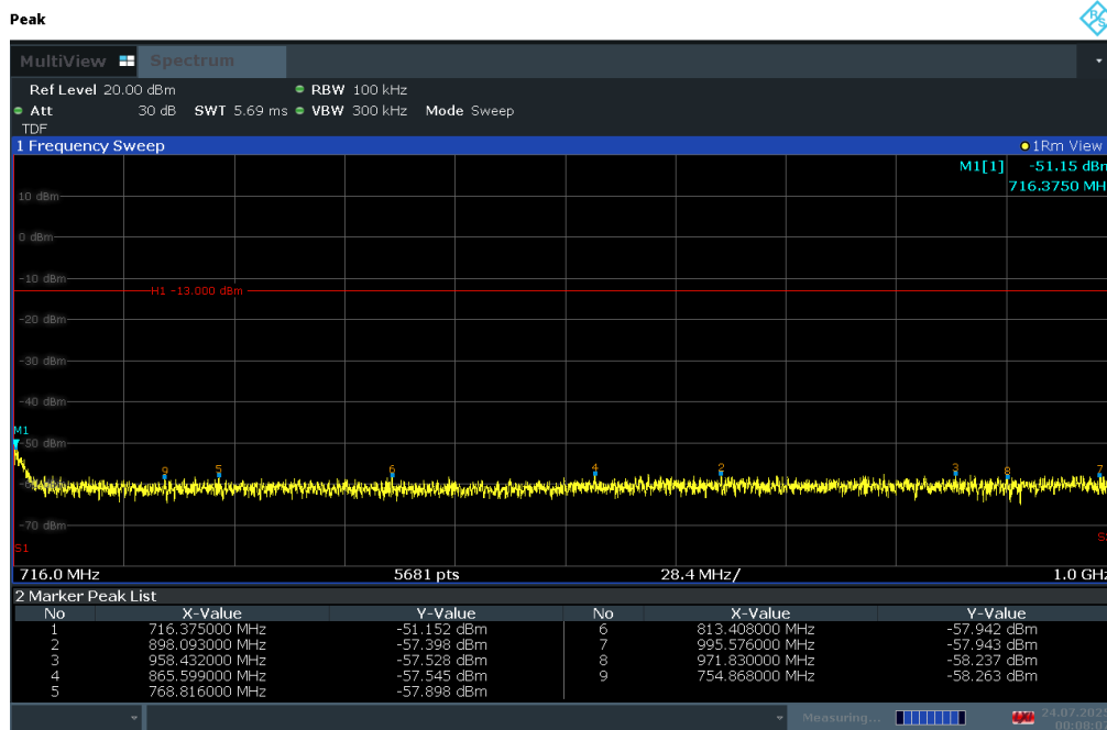
Plot 7-186. Conducted Spurious Plot (LTE Band 12/17 - 10MHz QPSK - RB Size 1, RB Offset 0 - High Channel)
