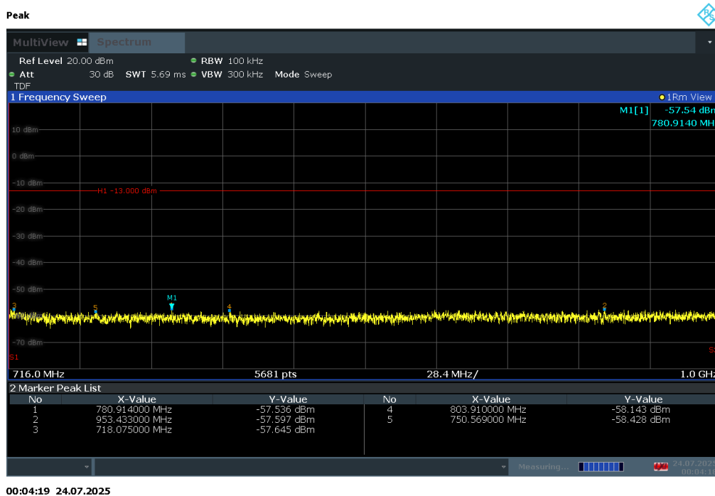
Plot 7-180. Conducted Spurious Plot (LTE Band 12/17 - 10MHz QPSK - RB Size 1, RB Offset 0 - Low Channel)
