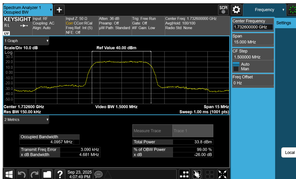
Plot 7-160. Occupied Bandwidth Plot (WCDMA, Ch. 1413)
