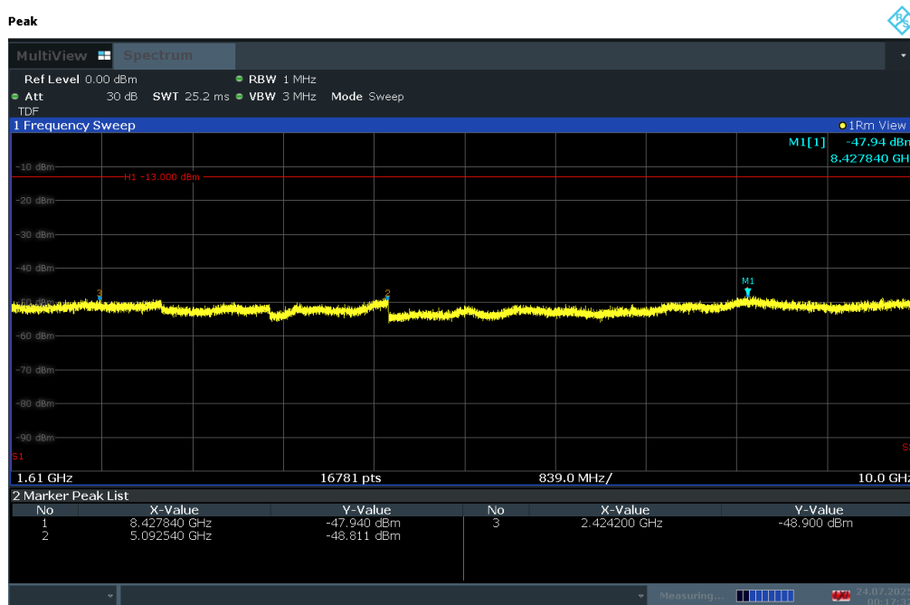
Plot 7-195. Conducted Spurious Plot (LTE Band 13 - 10MHz QPSK - RB Size 1, RB Offset 0)
