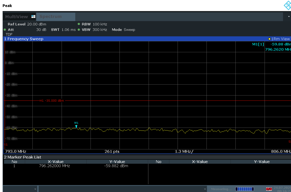
Plot 7-191. Conducted Spurious Plot (LTE Band 13 - 10MHz QPSK - RB Size 1, RB Offset 0)
