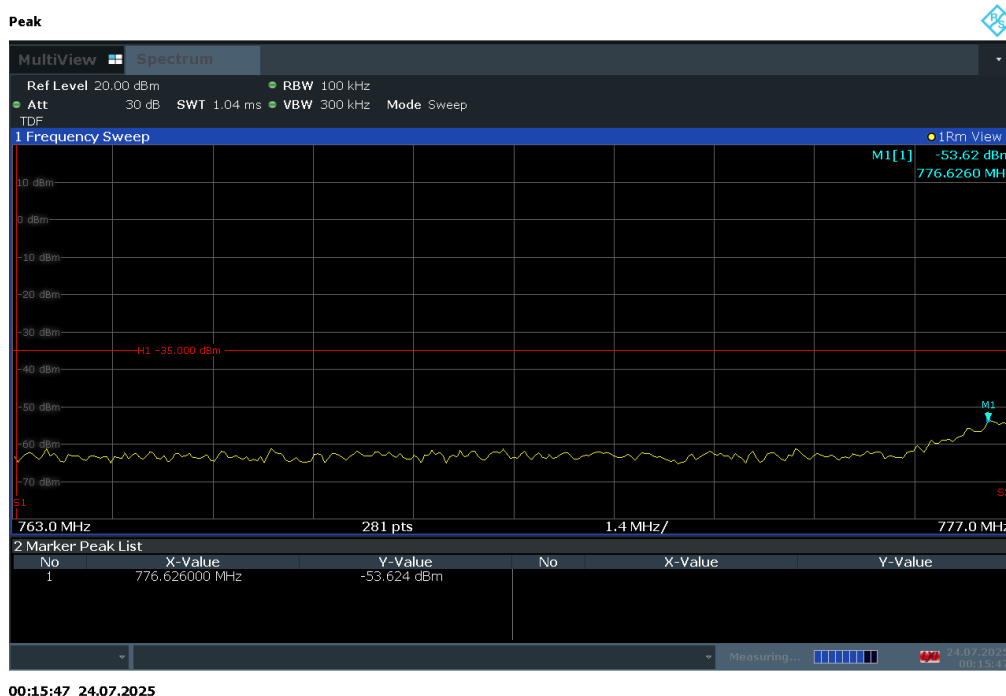
Plot 7-189. Conducted Spurious Plot (LTE Band 13 - 10MHz QPSK - RB Size 1, RB Offset 0)
