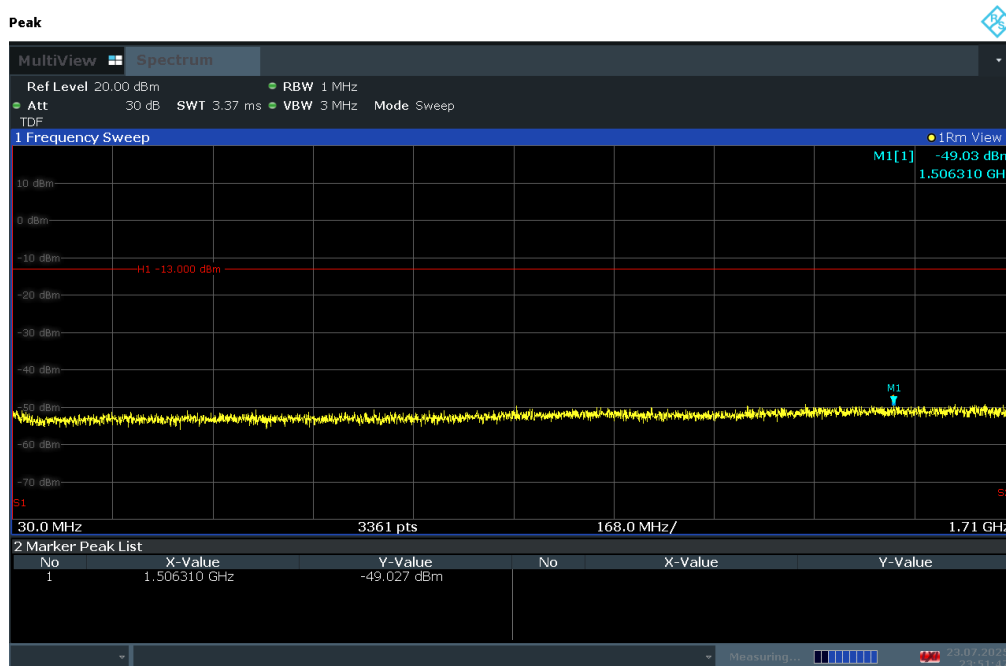
Plot 7-164. Conducted Spurious Plot (LTE Band 66/4 - 20MHz QPSK - RB Size 1, RB Offset 0 - Mid Channel)
