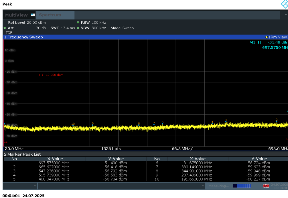
Plot 7-179. Conducted Spurious Plot (LTE Band 12/17 - 10MHz QPSK - RB Size 1, RB Offset 0 - Low Channel)
