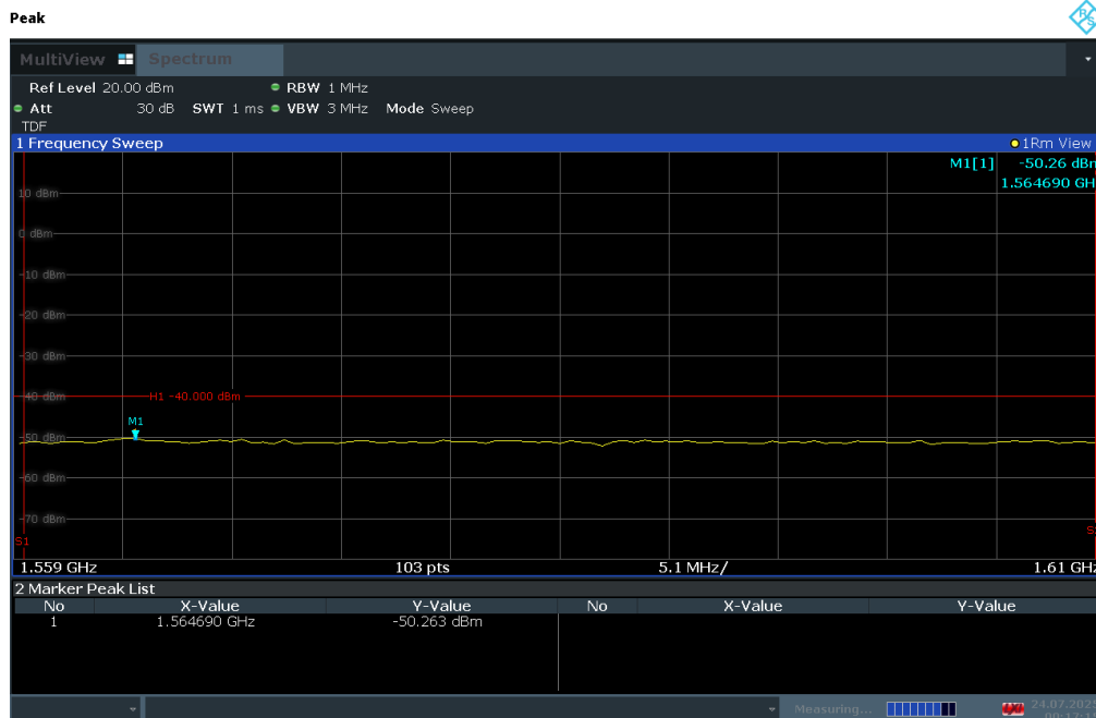
Plot 7-194. Conducted Spurious Plot (LTE Band 13 - 10MHz QPSK - RB Size 1, RB Offset 0)
