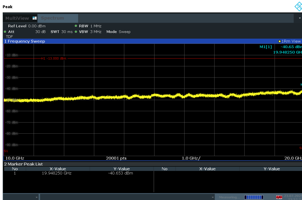
Plot 7-166. Conducted Spurious Plot (LTE Band 66/4 - 20MHz QPSK - RB Size 1, RB Offset 0 - Mid Channel)
