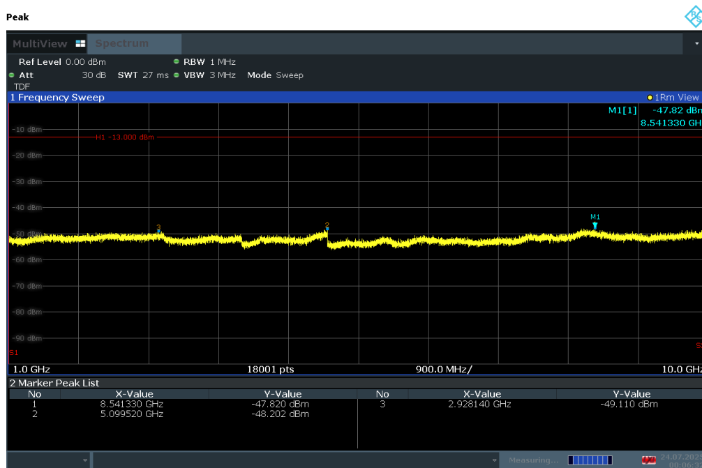
Plot 7-184. Conducted Spurious Plot (LTE Band 12/17 - 10MHz QPSK - RB Size 1, RB Offset 0 - Mid Channel)
