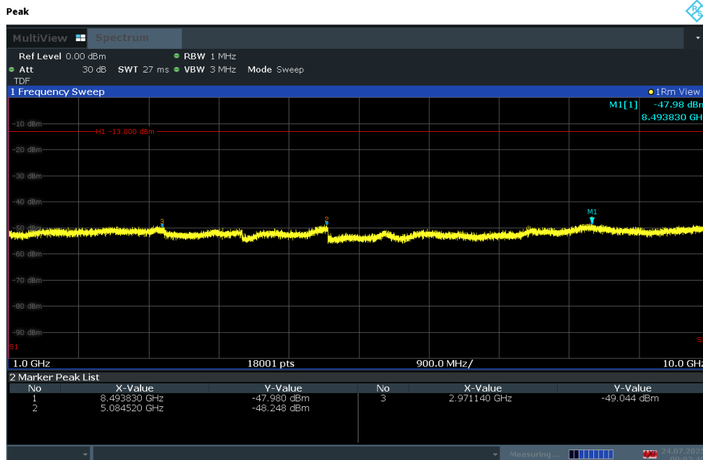
Plot 7-178. Conducted Spurious Plot (LTE Band 71 - 20MHz QPSK - RB Size 1, RB Offset 0 - High Channel)
