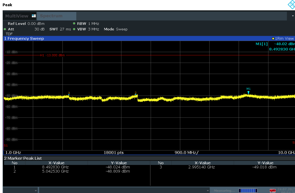
Plot 7-181. Conducted Spurious Plot (LTE Band 12/17 - 10MHz QPSK - RB Size 1, RB Offset 0 - Low Channel)
