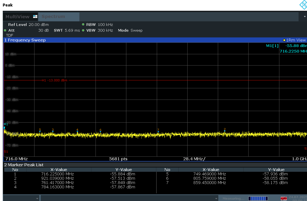
Plot 7-183. Conducted Spurious Plot (LTE Band 12/17 - 10MHz QPSK - RB Size 1, RB Offset 0 - Mid Channel)
