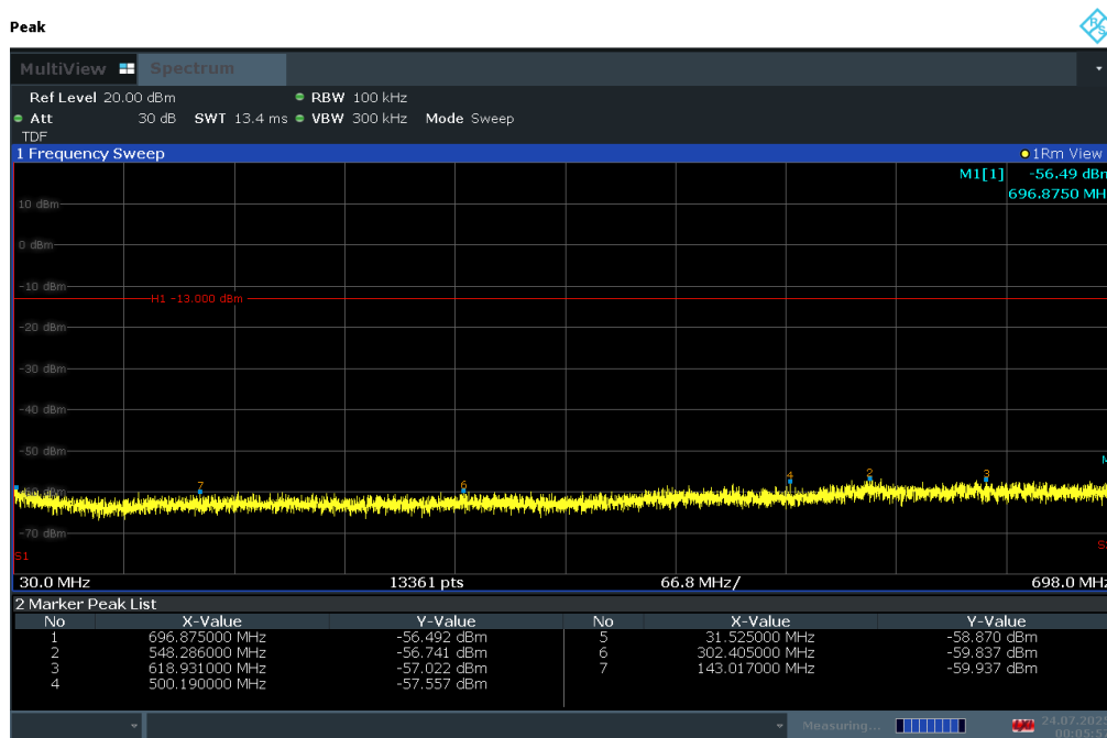
Plot 7-182. Conducted Spurious Plot (LTE Band 12/17 - 10MHz QPSK - RB Size 1, RB Offset 0 - Mid Channel)
