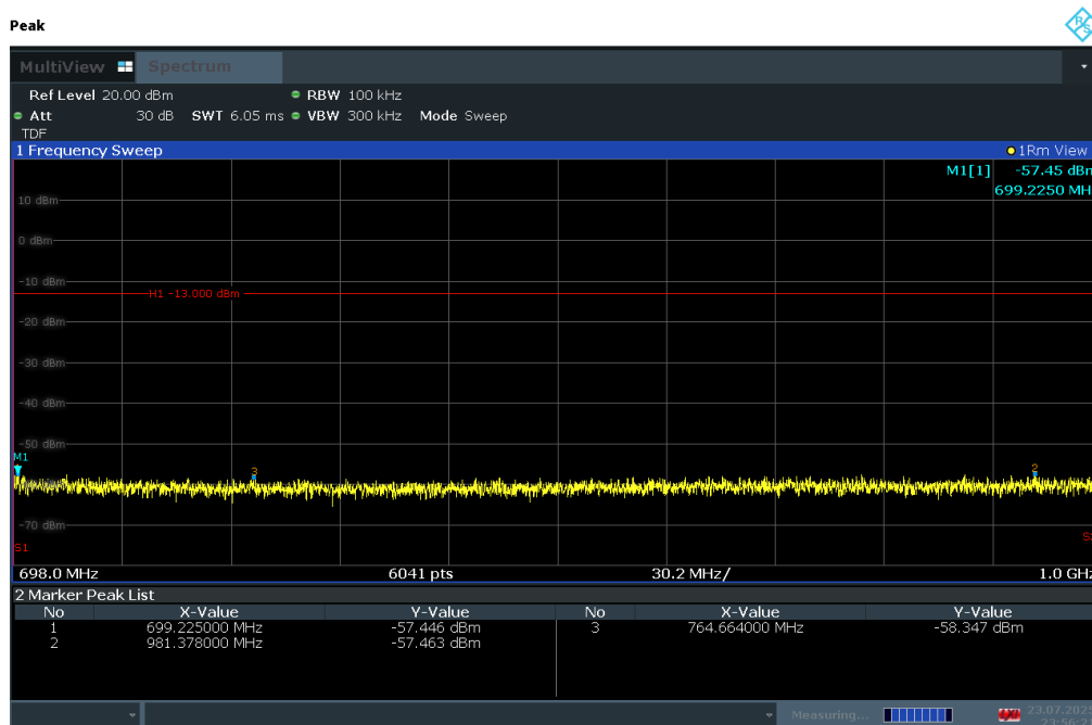
Plot 7-171. Conducted Spurious Plot (LTE Band 71 - 20MHz QPSK - RB Size 1, RB Offset 0 - Low Channel)
