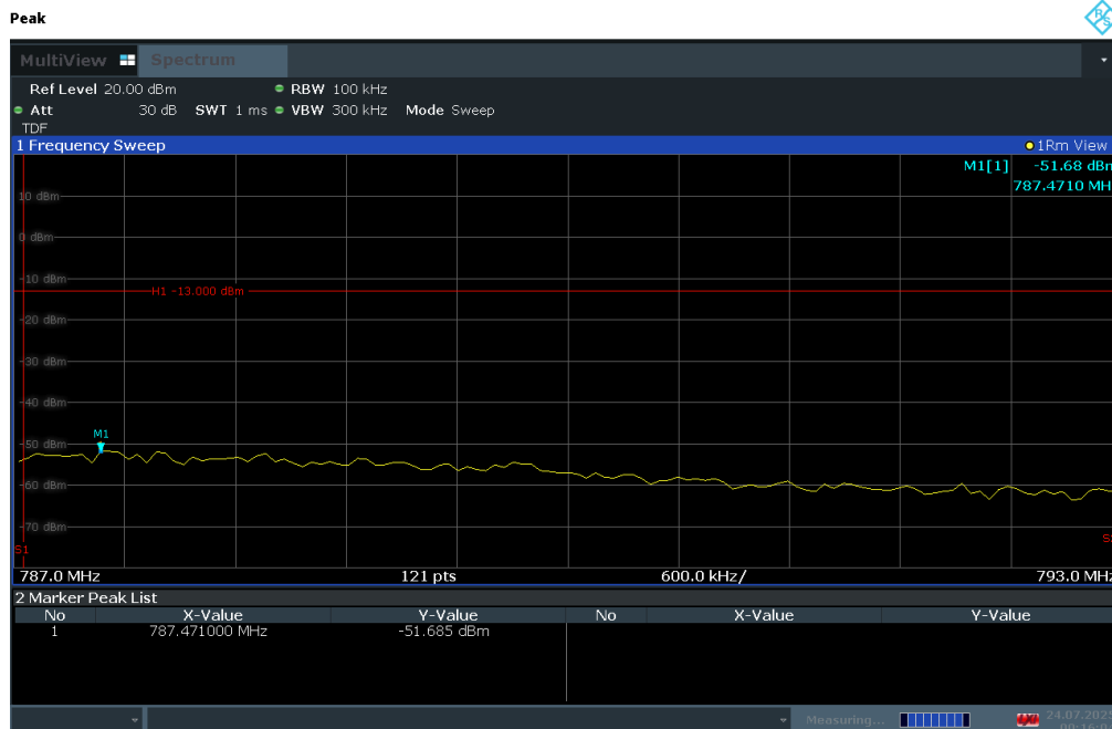
Plot 7-190. Conducted Spurious Plot (LTE Band 13 - 10MHz QPSK - RB Size 1, RB Offset 0)
