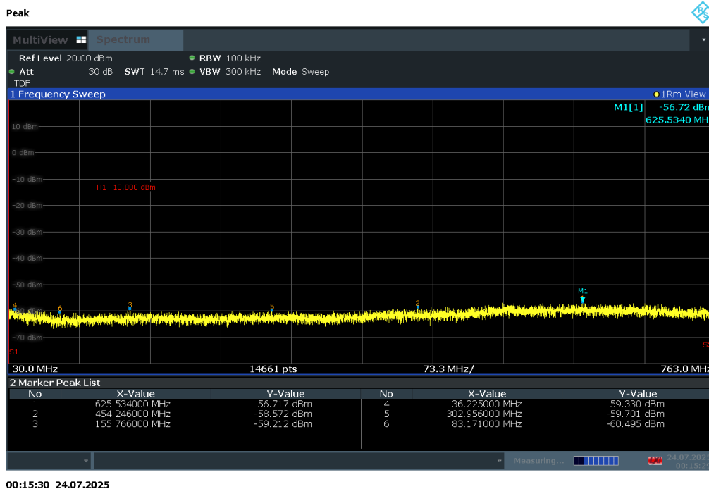
Plot 7-188. Conducted Spurious Plot (LTE Band 13 - 10MHz QPSK - RB Size 1, RB Offset 0)
