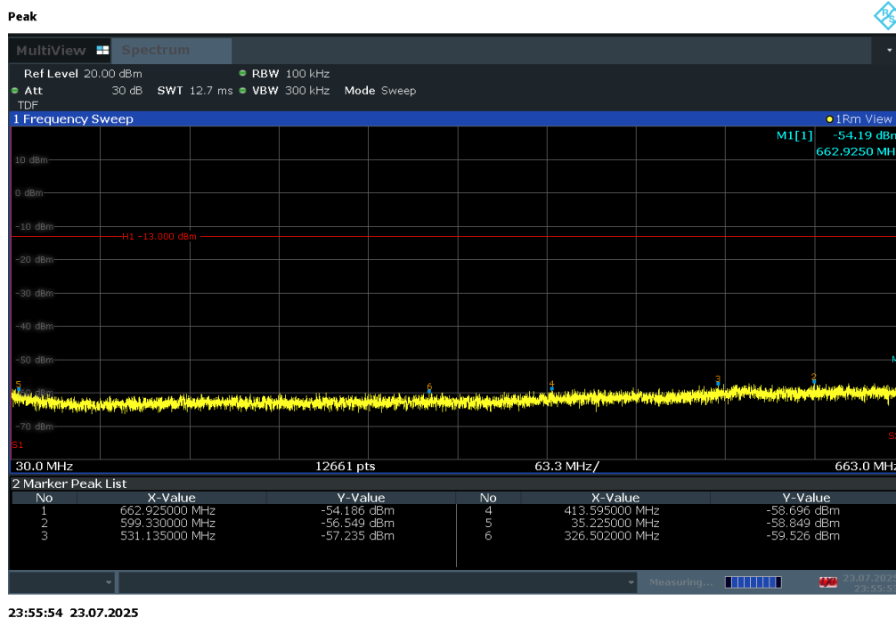
Plot 7-170. Conducted Spurious Plot (LTE Band 71 - 20MHz QPSK - RB Size 1, RB Offset 0 - Low Channel)
