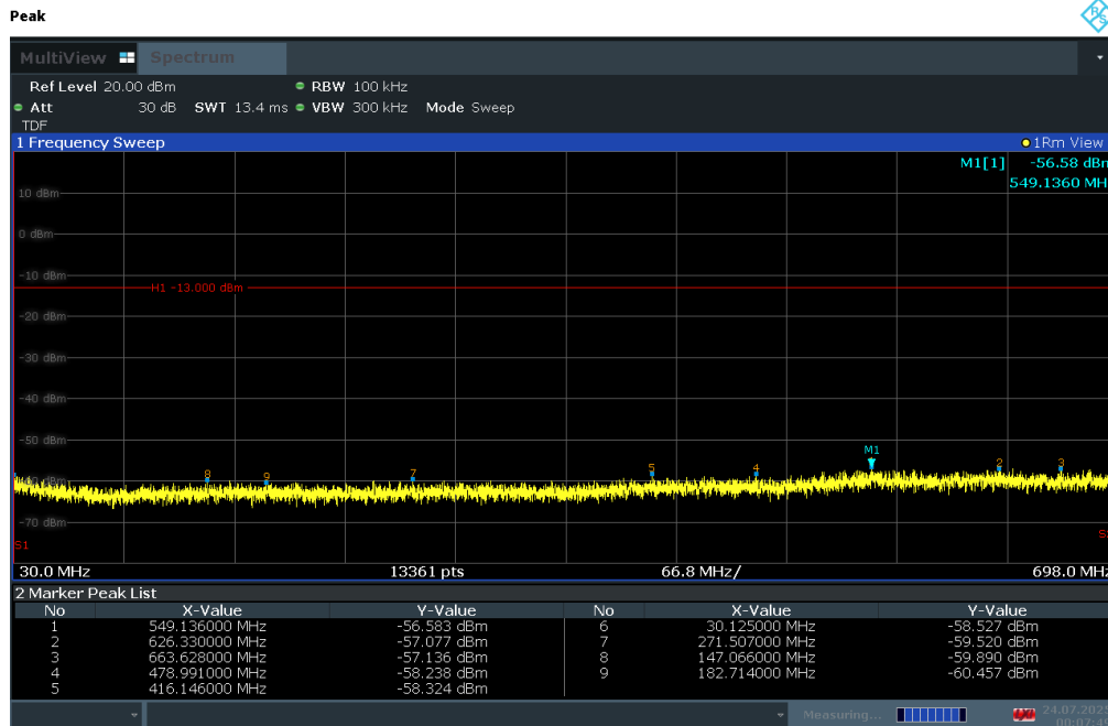
Plot 7-185. Conducted Spurious Plot (LTE Band 12/17 - 10MHz QPSK - RB Size 1, RB Offset 0 - High Channel)
