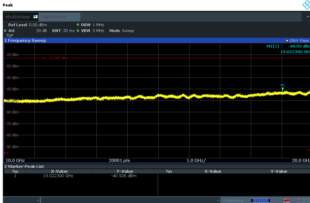
Plot 7-163. Conducted Spurious Plot (LTE Band 66/4 - 20MHz QPSK - RB Size 1, RB Offset 0 - Low Channel)
