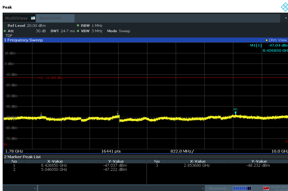
Plot 7-162. Conducted Spurious Plot (LTE Band 66/4 - 20MHz QPSK - RB Size 1, RB Offset 0 - Low Channel)
