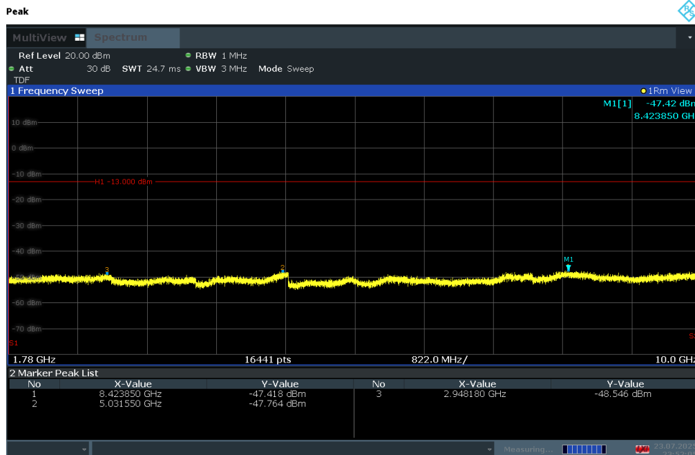
Plot 7-165. Conducted Spurious Plot (LTE Band 66/4 - 20MHz QPSK - RB Size 1, RB Offset 0 - Mid Channel)
