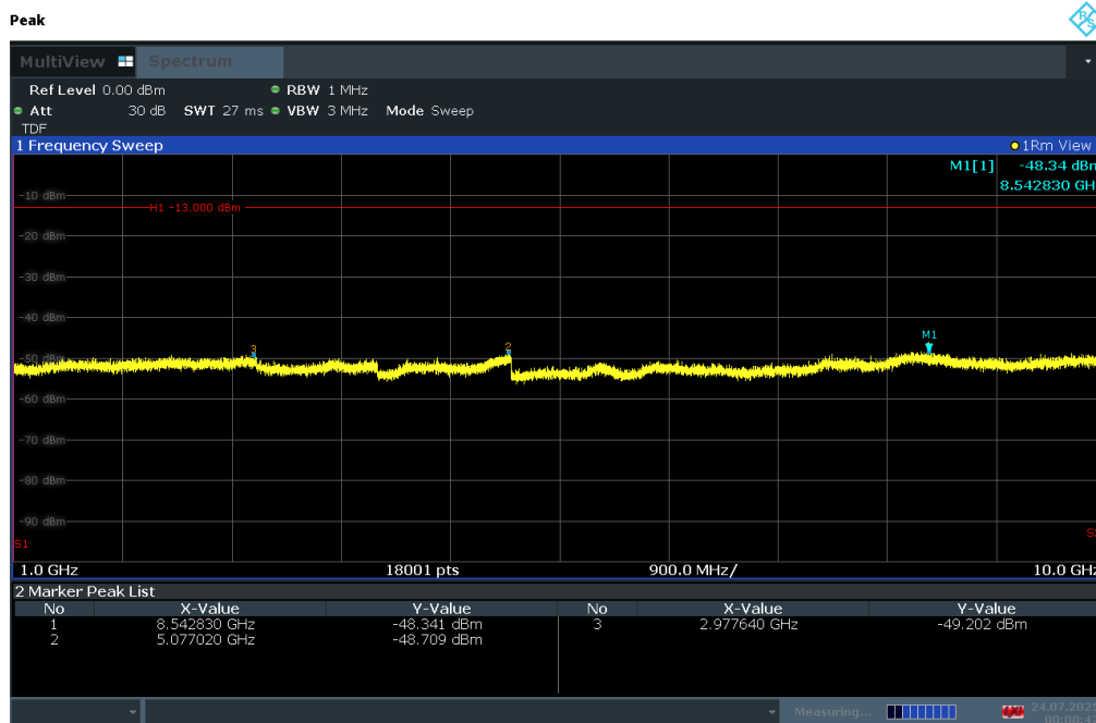
Plot 7-175. Conducted Spurious Plot (LTE Band 71 - 20MHz QPSK - RB Size 1, RB Offset 0 - Mid Channel)
