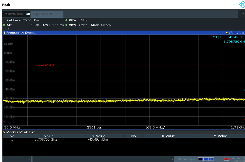
Plot 7-161. Conducted Spurious Plot (LTE Band 66/4 - 20MHz QPSK - RB Size 1, RB Offset 0 - Low Channel)
