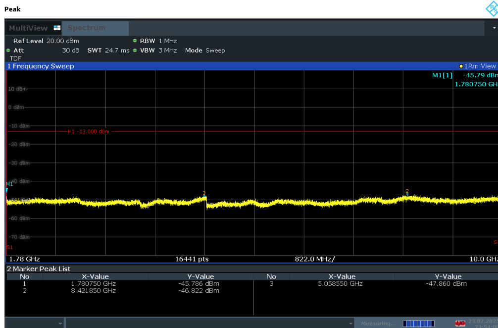
Plot 7-168. Conducted Spurious Plot (LTE Band 66/4 - 20MHz QPSK - RB Size 1, RB Offset 0 - High Channel)
