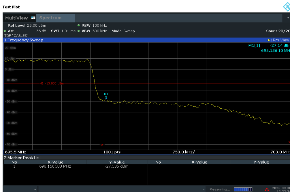
Plot 7-290. Upper Band Edge Plot (LTE Band 71 - 5MHz QPSK – Full RB)
