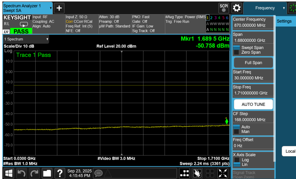
Plot 7-238. Conducted Spurious Plot (WCDMA Ch. 1513- High Channel)
