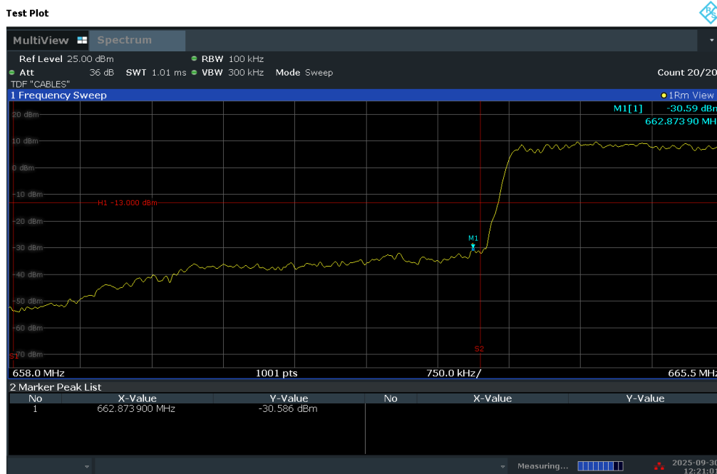
Plot 7-289. Lower Band Edge Plot (LTE Band 71 - 5MHz QPSK – Full RB)
