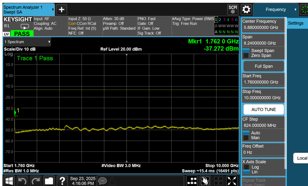
Plot 7-239. Conducted Spurious Plot (WCDMA Ch. 1513- High Channel)
