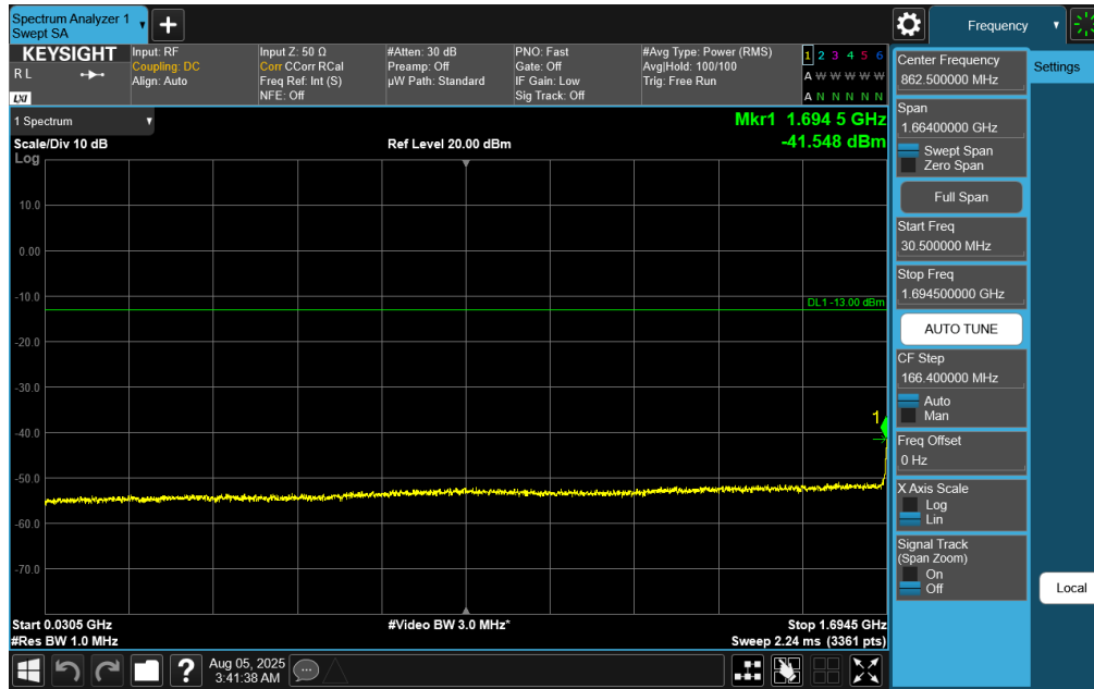
Plot 7-205. Conducted Spurious Plot (NR Band n70 -10.0MHz DFT-s-OFDM QPSK - RB Size 1, RB Offset 0 - Low Channel)
