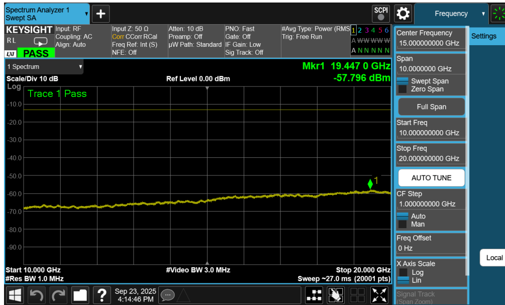
Plot 7-234. Conducted Spurious Plot (WCDMA Ch. 1312- Low Channel)
