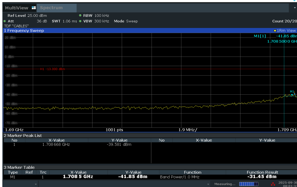
Plot 7-266. Lower Extended Band Edge Plot (LTE Band 4 – 1.4MHz QPSK – Full RB)
