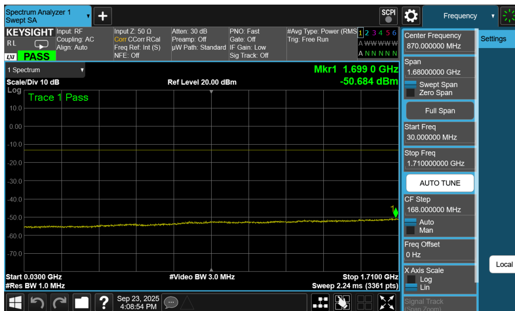
Plot 7-235. Conducted Spurious Plot (WCDMA Ch. 1413- Mid Channel)
