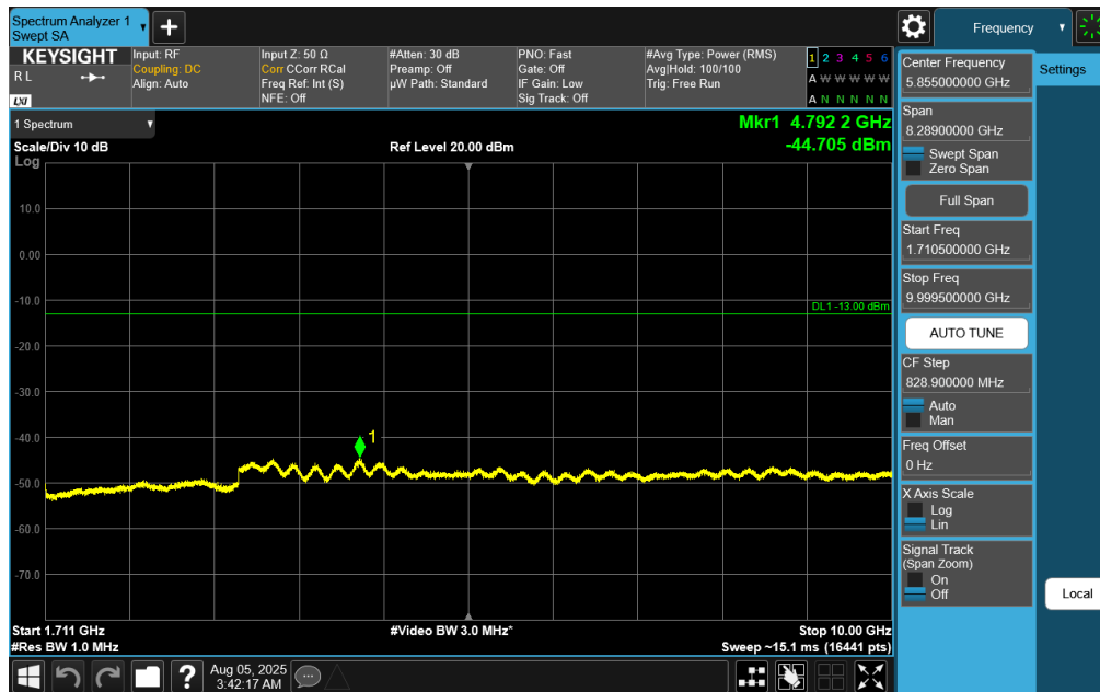
Plot 7-206. Conducted Spurious Plot (NR Band n70 - 10.0MHz DFT-s-OFDM QPSK - RB Size 1, RB Offset 0 - Low Channel)
