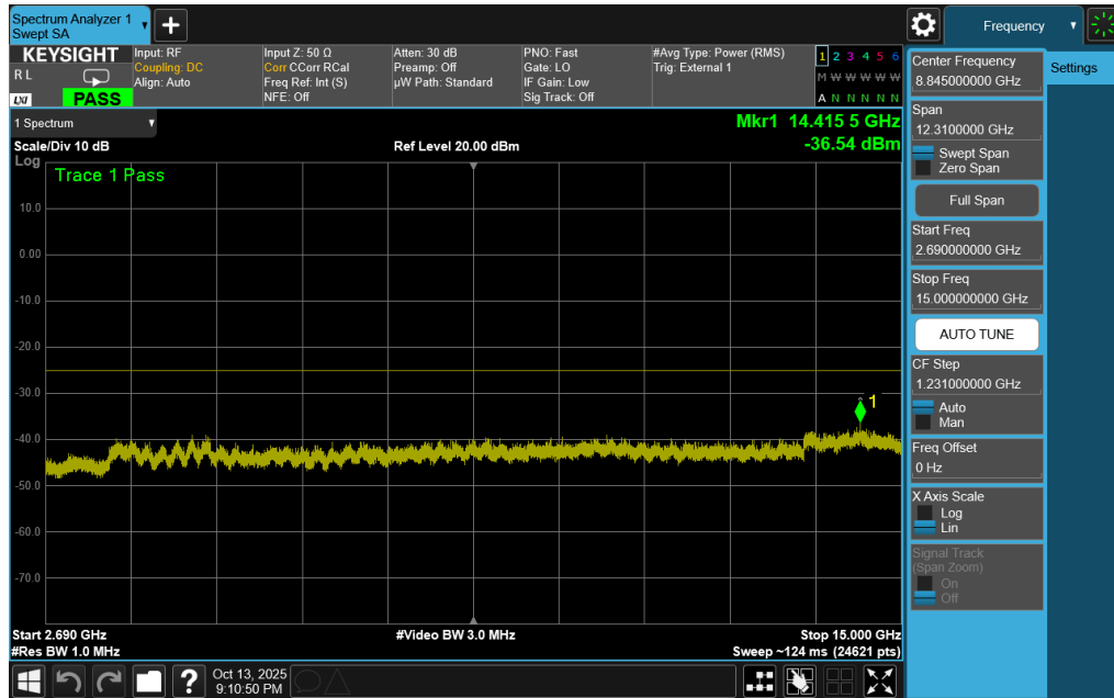
Plot 7-241. Conducted Spurious Plot (ULCA LTE Band 41 – (20+20)MHz QPSK – RB Size 1, RB Offset 0 – Mid Channel)
