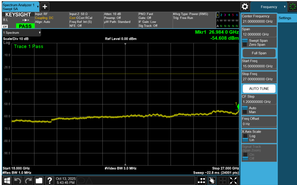
Plot 7-236. Conducted Spurious Plot (ULCA LTE Band 7 – (20+20)MHz QPSK – RB Size 1, RB Offset 0 – High Channel)
