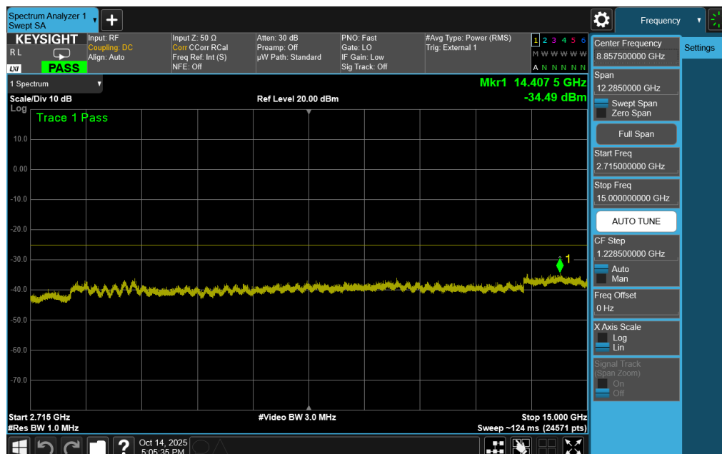
Plot 7-244. Conducted Spurious Plot (ULCA LTE Band 41 – (20+20)MHz QPSK – RB Size 1, RB Offset 0 – High Channel)
