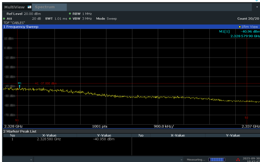
Plot 7-270. Extended Upper Band Edge Plot (LTE Band 30 - 10MHz QPSK – Full RB)
