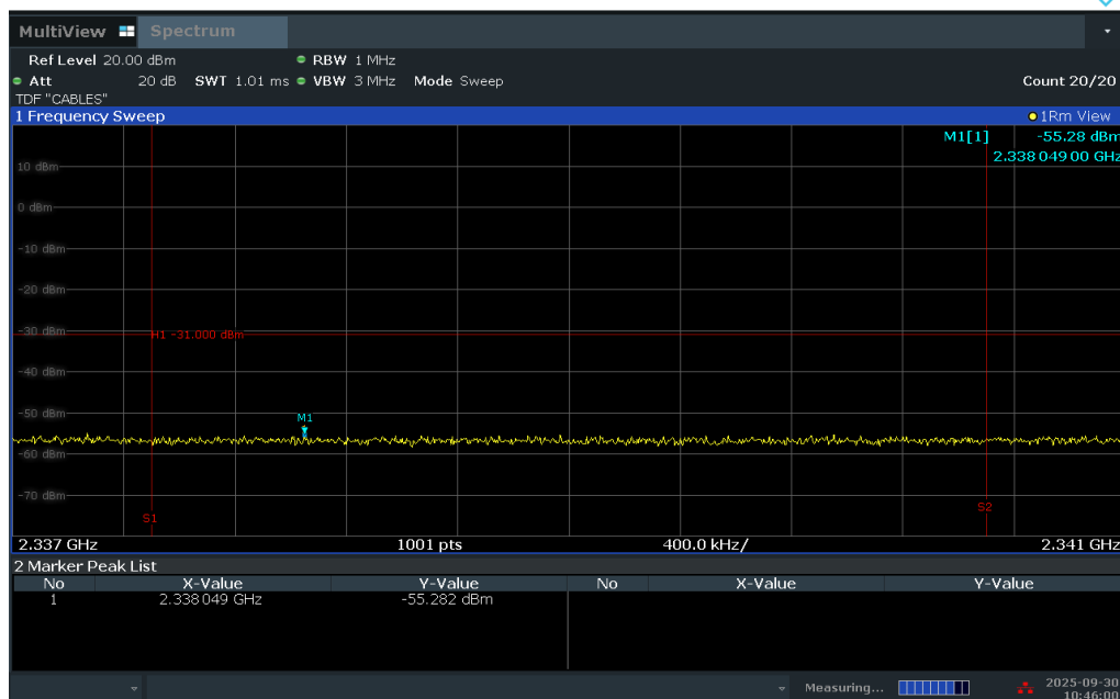
Plot 7-271. Extended Upper Band Edge Plot (LTE Band 30 - 10MHz QPSK – Full RB)
