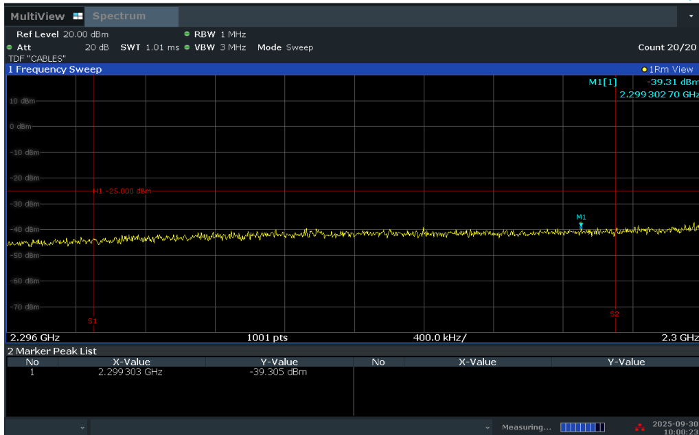
Plot 7-250. Extended Lower Band Edge Plot (LTE Band 30 - 5MHz QPSK – Full RB)
