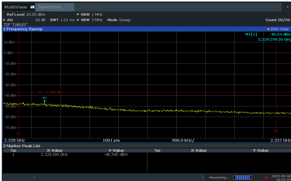
Plot 7-255. Extended Upper Band Edge Plot (LTE Band 30 - 5MHz QPSK – Full RB)
