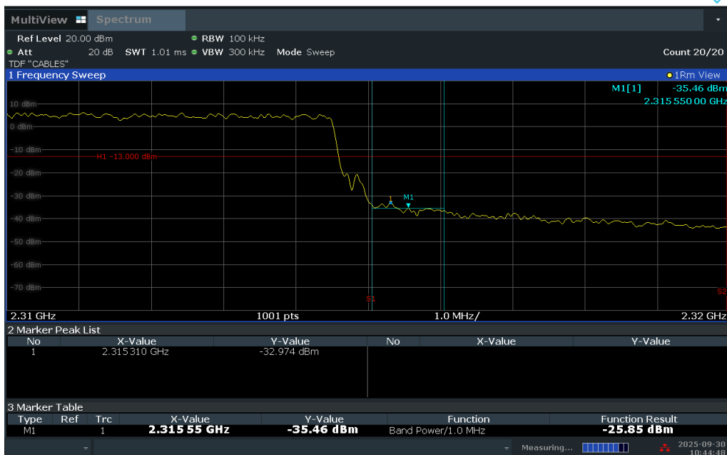
Plot 7-267. Upper Band Edge Plot (LTE Band 30 - 10MHz QPSK – Full RB)
