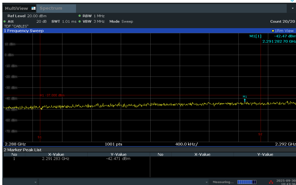
Plot 7-263. Extended Lower Band Edge Plot (LTE Band 30 - 10MHz QPSK – Full RB)
