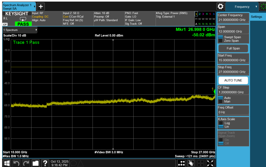
Plot 7-242. Conducted Spurious Plot (ULCA LTE Band 41 – (20+20)MHz QPSK – RB Size 1, RB Offset 0 – Mid Channel)
