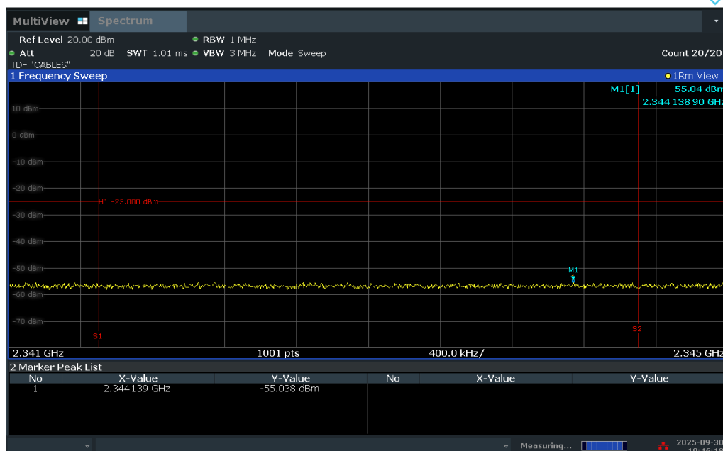
Plot 7-272. Extended Upper Band Edge Plot (LTE Band 30 - 10MHz QPSK – Full RB)
