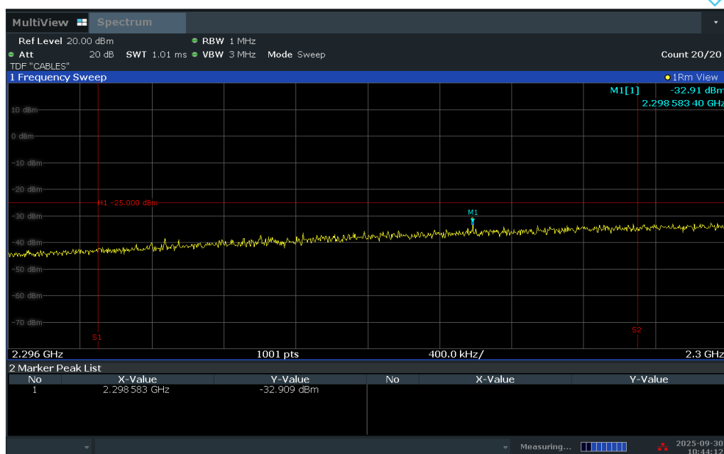
Plot 7-265. Extended Lower Band Edge Plot (LTE Band 30 - 10MHz QPSK – Full RB)
