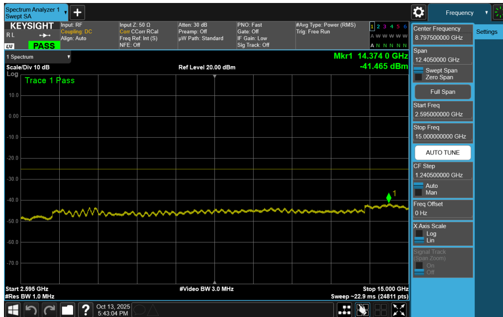
Plot 7-235. Conducted Spurious Plot (ULCA LTE Band 7 – (20+20)MHz QPSK – RB Size 1, RB Offset 0 – High Channel)
