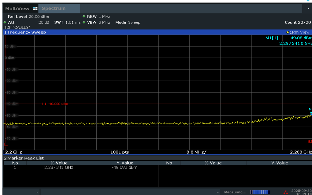
Plot 7-262. Extended Lower Band Edge Plot (LTE Band 30 - 10MHz QPSK – Full RB)
