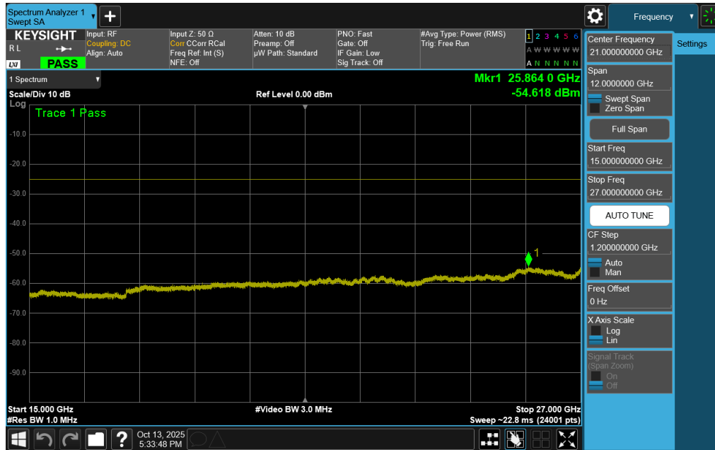
Plot 7-230. Conducted Spurious Plot (ULCA LTE Band 7 – (20+20)MHz QPSK – RB Size 1, RB Offset 0 – Low Channel)
