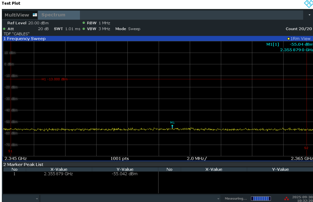
Plot 7-258. Extended Upper Band Edge Plot (LTE Band 30 - 5MHz QPSK – Full RB)
