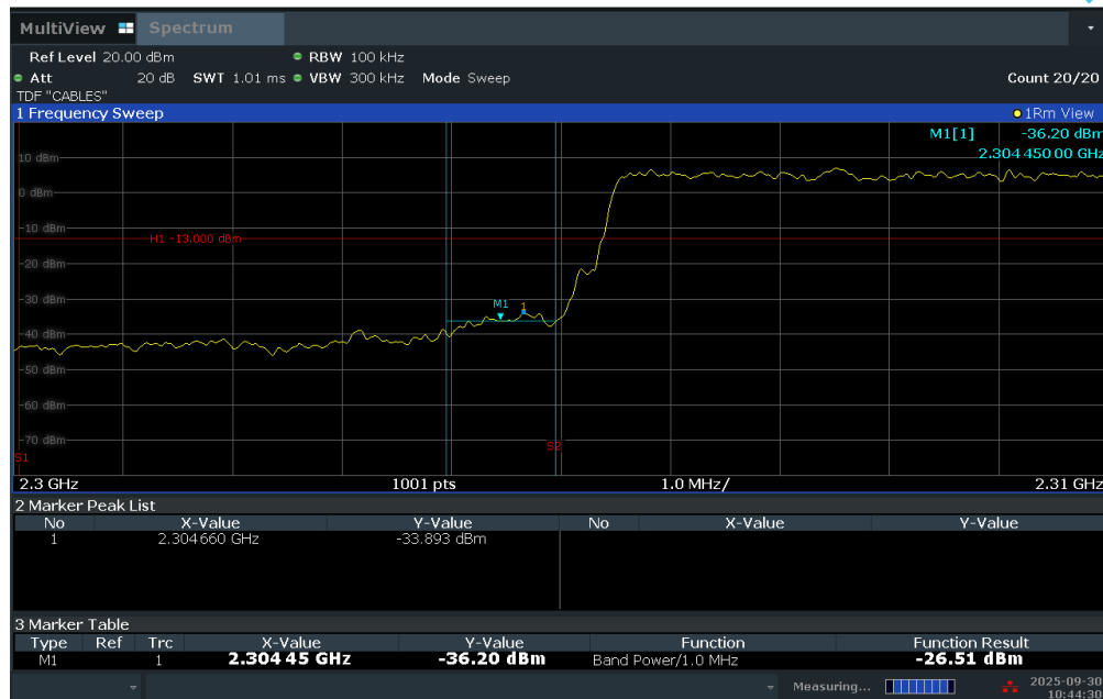
Plot 7-266. Lower Band Edge Plot (LTE Band 30 - 10MHz QPSK – Full RB)
