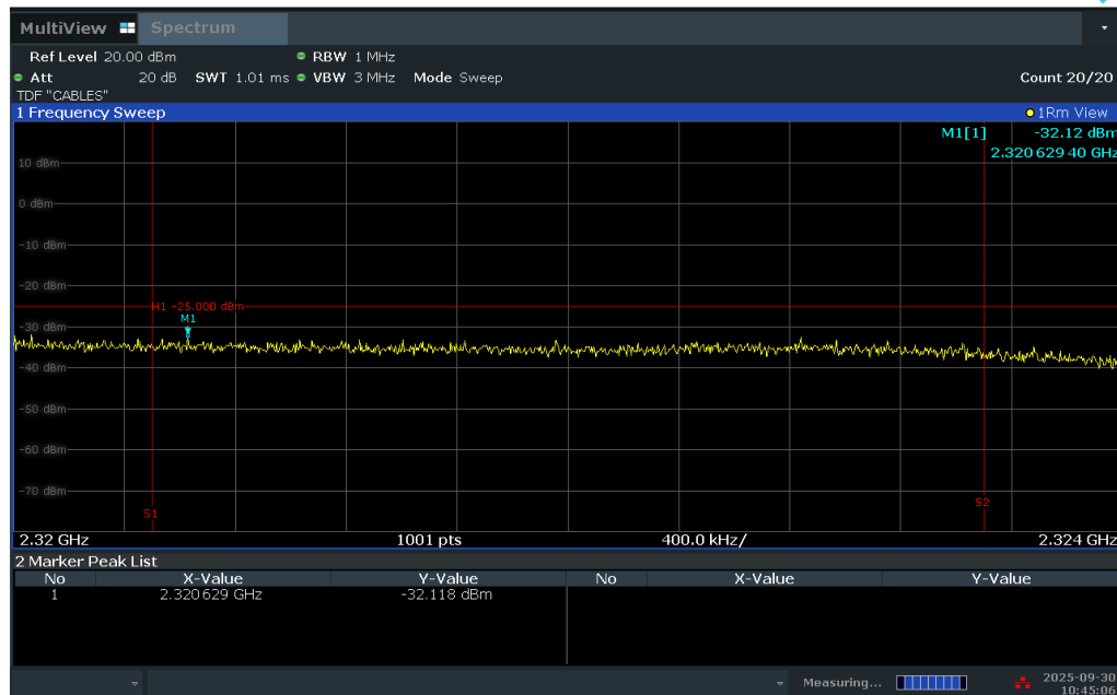
Plot 7-268. Extended Upper Band Edge Plot (LTE Band 30 - 10MHz QPSK – Full RB)
