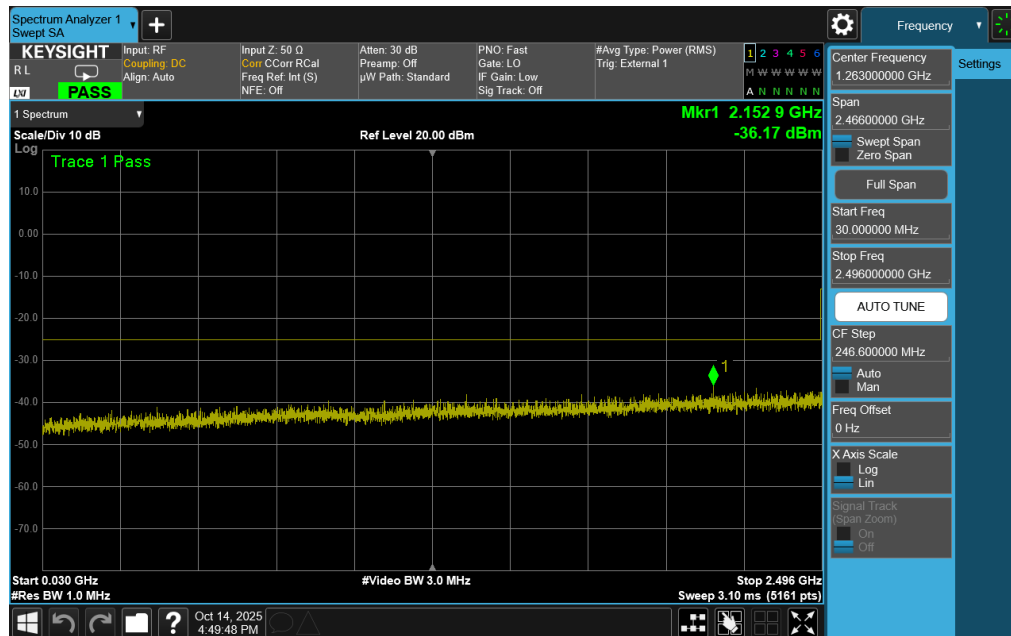
Plot 7-243. Conducted Spurious Plot (ULCA LTE Band 41 – (20+20)MHz QPSK – RB Size 1, RB Offset 0 – High Channel)
