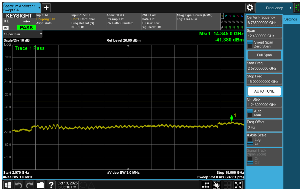
Plot 7-229. Conducted Spurious Plot (ULCA LTE Band 7 – (20+20)MHz QPSK – RB Size 1, RB Offset 0 – Low Channel)
