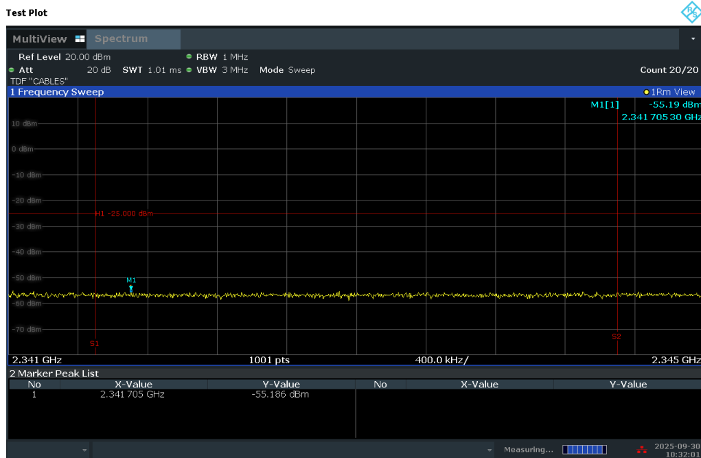
Plot 7-257. Extended Upper Band Edge Plot (LTE Band 30 - 5MHz QPSK – Full RB)
