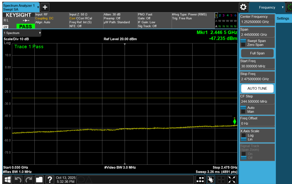
Plot 7-228. Conducted Spurious Plot (ULCA LTE Band 7 – (20+20)MHz QPSK – RB Size 1, RB Offset 0 – Low Channel)
