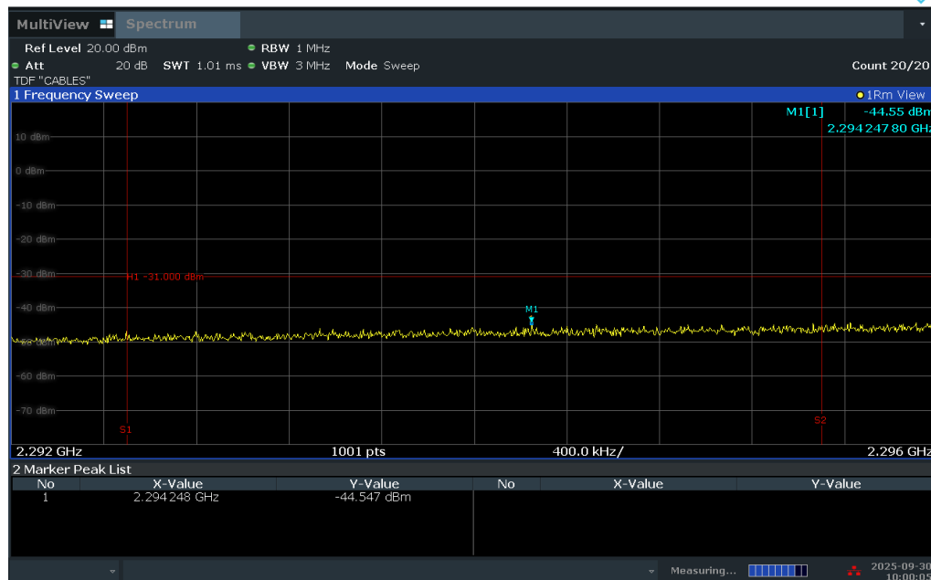
Plot 7-249. Extended Lower Band Edge Plot (LTE Band 30 - 5MHz QPSK – Full RB)
