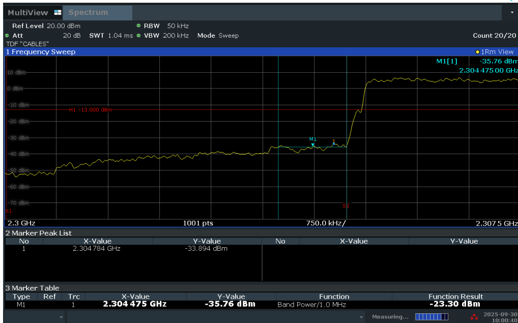
Plot 7-251. Lower Band Edge Plot (LTE Band 30 - 5MHz QPSK – Full RB)
