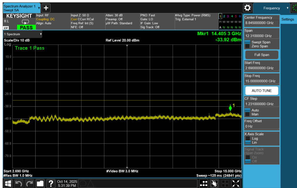
Plot 7-238. Conducted Spurious Plot (ULCA LTE Band 41 – (20+20)MHz QPSK – RB Size 1, RB Offset 0 – Low Channel)
