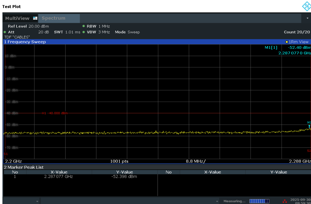
Plot 7-247. Extended Lower Band Edge Plot (LTE Band 30 - 5MHz QPSK – Full RB)
