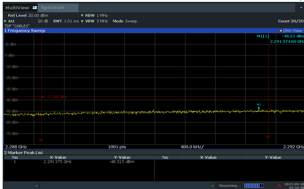
Plot 7-248. Extended Lower Band Edge Plot (LTE Band 30 - 5MHz QPSK – Full RB)
