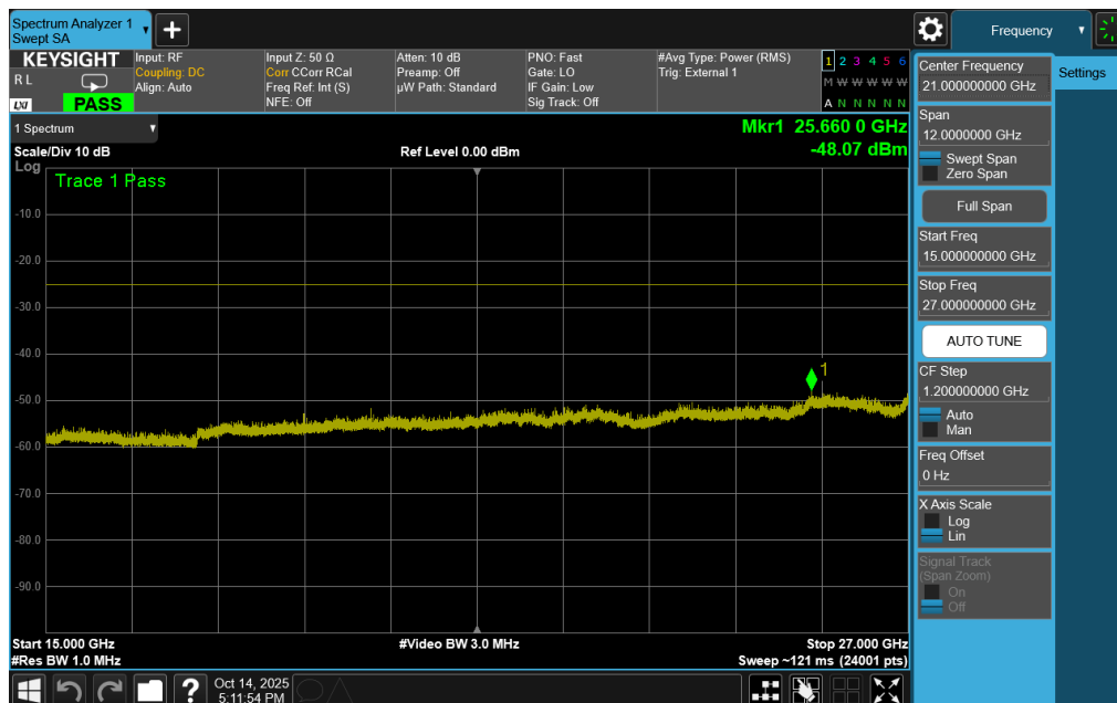
Plot 7-245. Conducted Spurious Plot (ULCA LTE Band 41 – (20+20)MHz QPSK – RB Size 1, RB Offset 0 – High Channel)
