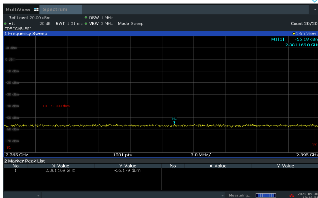
Plot 7-273. Extended Upper Band Edge Plot (LTE Band 30 - 10MHz QPSK – Full RB)
