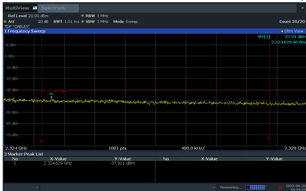
Plot 7-269. Extended Upper Band Edge Plot (LTE Band 30 - 10MHz QPSK – Full RB)
