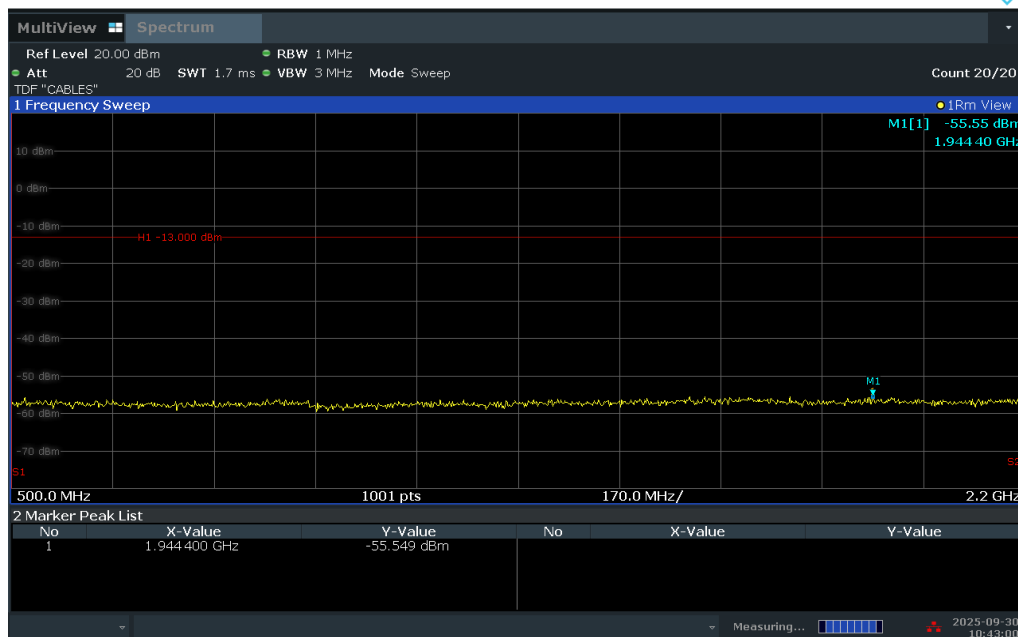
Plot 7-261. Extended Lower Band Edge Plot (LTE Band 30 - 10MHz QPSK – Full RB)
