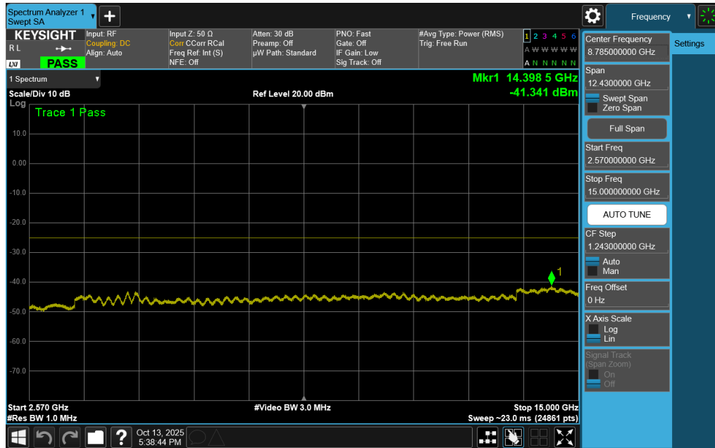
Plot 7-232. Conducted Spurious Plot (ULCA LTE Band 7 – (20+20)MHz QPSK – RB Size 1, RB Offset 0 – Mid Channel)
