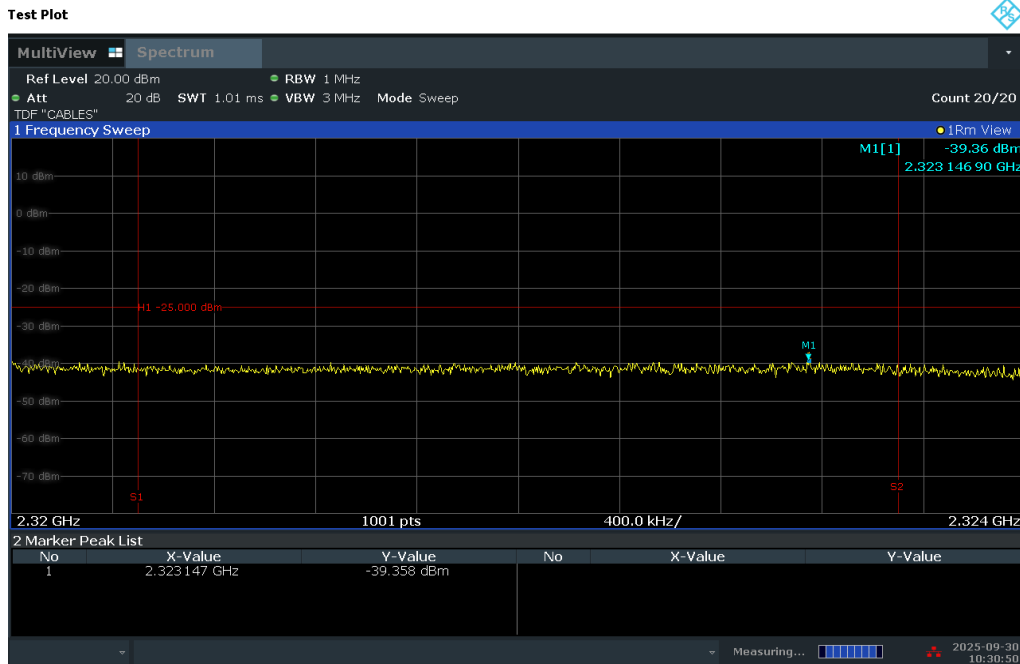
Plot 7-253. Extended Upper Band Edge Plot (LTE Band 30 - 5MHz QPSK – Full RB)
