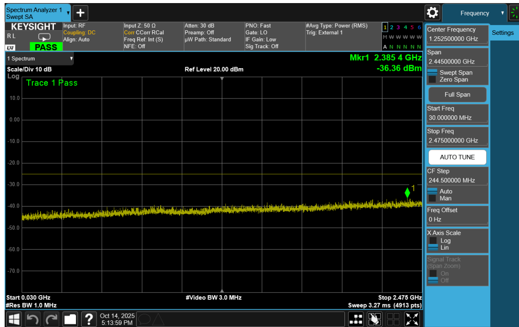
Plot 7-237. Conducted Spurious Plot (ULCA LTE Band 41 – (20+20)MHz QPSK – RB Size 1, RB Offset 0 – Low Channel)
