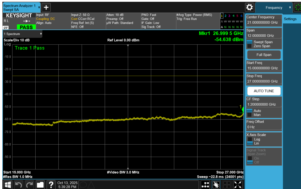
Plot 7-233. Conducted Spurious Plot (ULCA LTE Band 7 – (20+20)MHz QPSK – RB Size 1, RB Offset 0 – Mid Channel)
