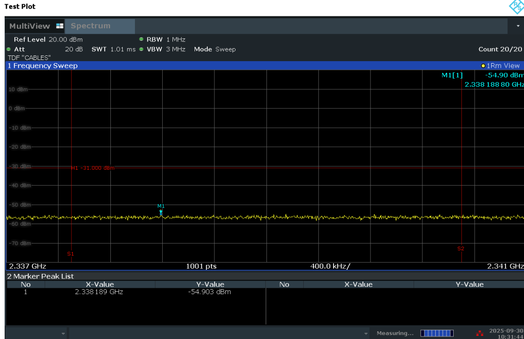
Plot 7-256. Extended Upper Band Edge Plot (LTE Band 30 - 5MHz QPSK – Full RB)
