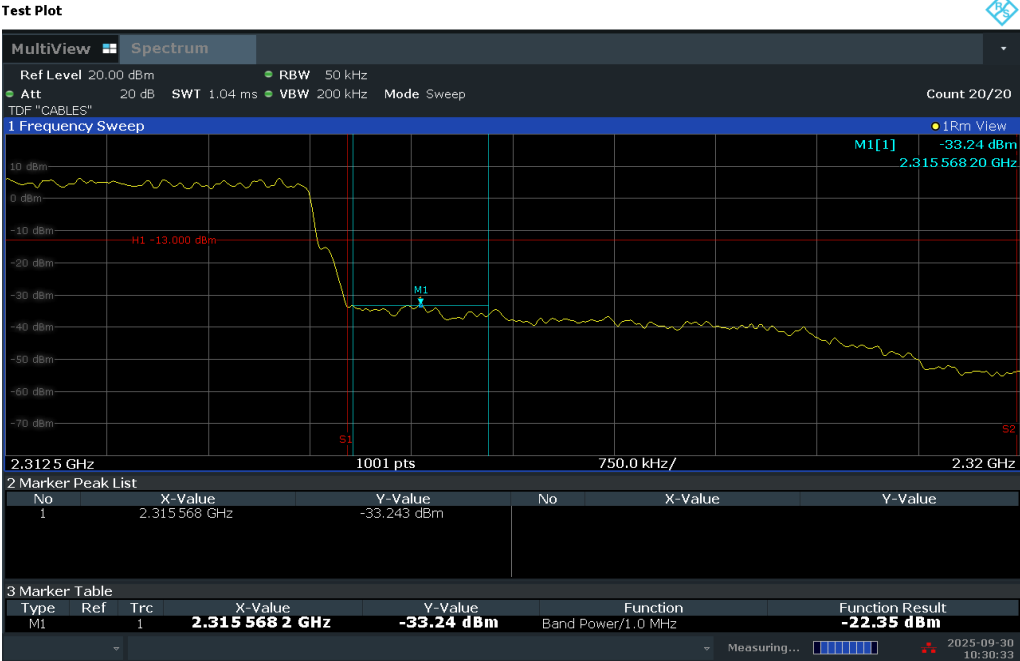
Plot 7-252. Upper Band Edge Plot (LTE Band 30 - 5MHz QPSK – Full RB)
