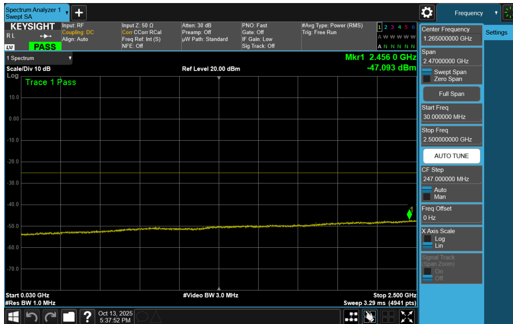
Plot 7-231. Conducted Spurious Plot (ULCA LTE Band 7 – (20+20)MHz QPSK – RB Size 1, RB Offset 0 – Mid Channel)
