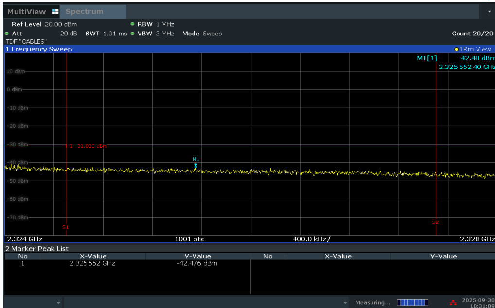
Plot 7-254. Extended Upper Band Edge Plot (LTE Band 30 - 5MHz QPSK – Full RB)
