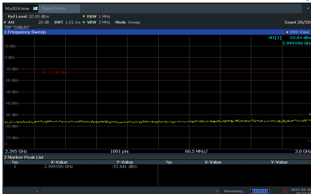
Plot 7-260. Extended Upper Band Edge Plot (LTE Band 30 - 5MHz QPSK – Full RB)
