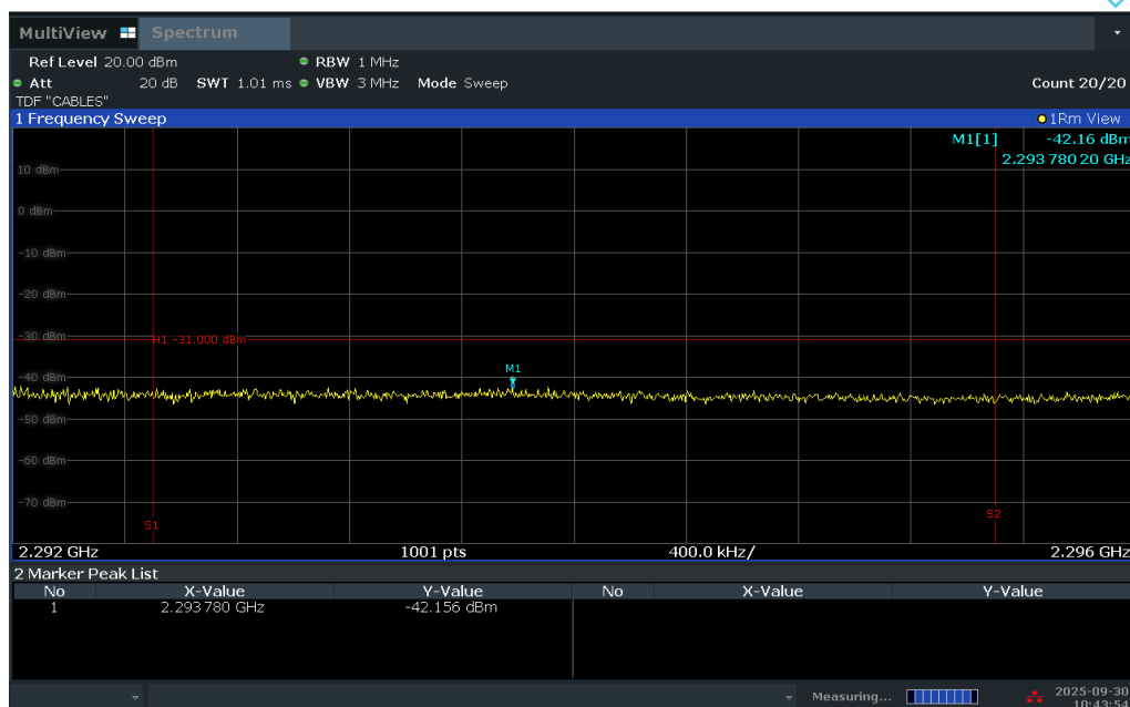
Plot 7-264. Extended Lower Band Edge Plot (LTE Band 30 - 10MHz QPSK – Full RB)
