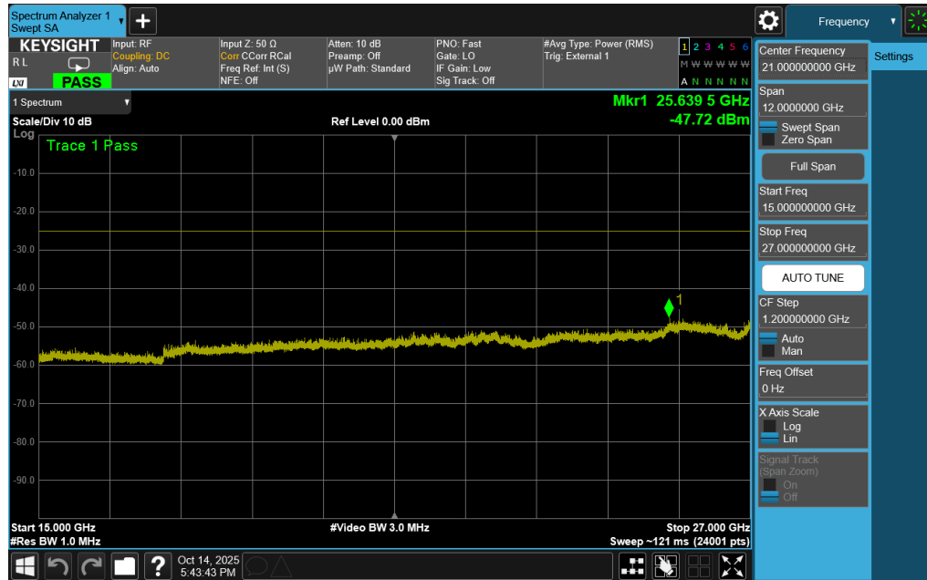
Plot 7-239. Conducted Spurious Plot (ULCA LTE Band 41 – (20+20)MHz QPSK – RB Size 1, RB Offset 0 – Low Channel)
