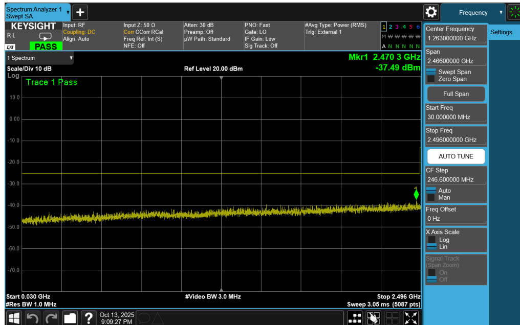
Plot 7-240. Conducted Spurious Plot (ULCA LTE Band 41 – (20+20)MHz QPSK – RB Size 1, RB Offset 0 – Mid Channel)
