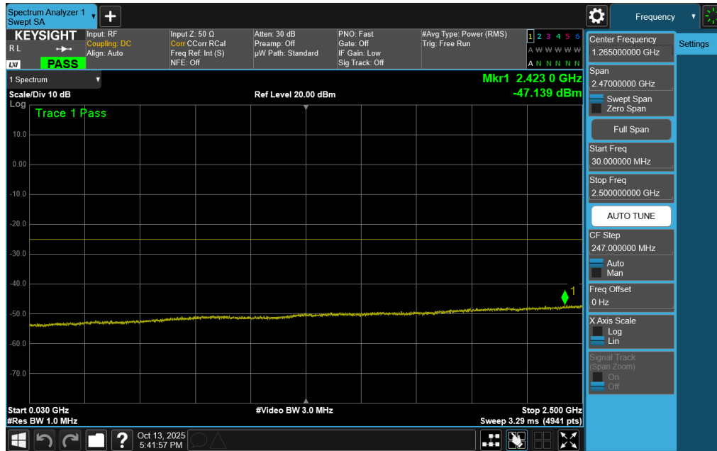
Plot 7-234. Conducted Spurious Plot (ULCA LTE Band 7 – (20+20)MHz QPSK – RB Size 1, RB Offset 0 – High Channel)
