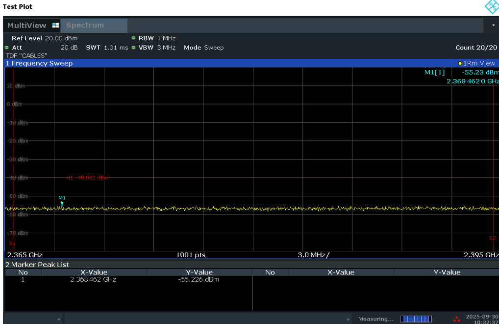
Plot 7-259. Extended Upper Band Edge Plot (LTE Band 30 - 5MHz QPSK – Full RB)
