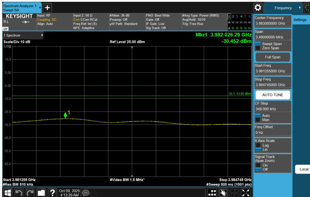
Plot 7-221. Extended Upper Band Edge Plot (NR Band n77 C-Band - 15MHz DFT-s-OFDM QPSK – Full RB)
