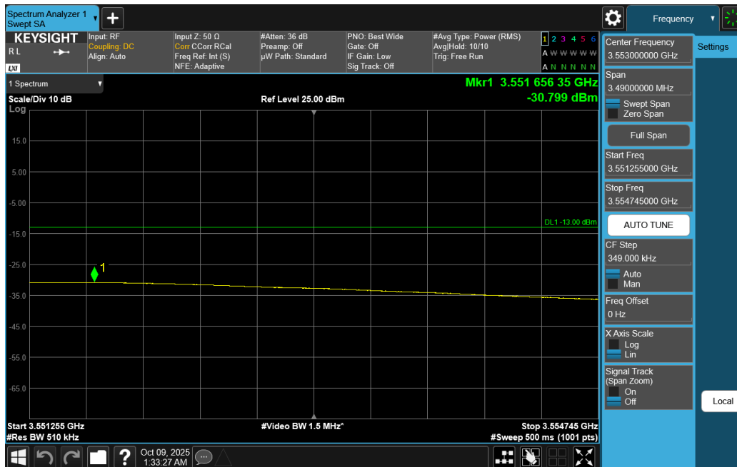
Plot 7-185. Extended Upper Band Edge Plot (NR Band n77 DoD-Band - 60MHz DFT-s-OFDM QPSK – Full RB)
