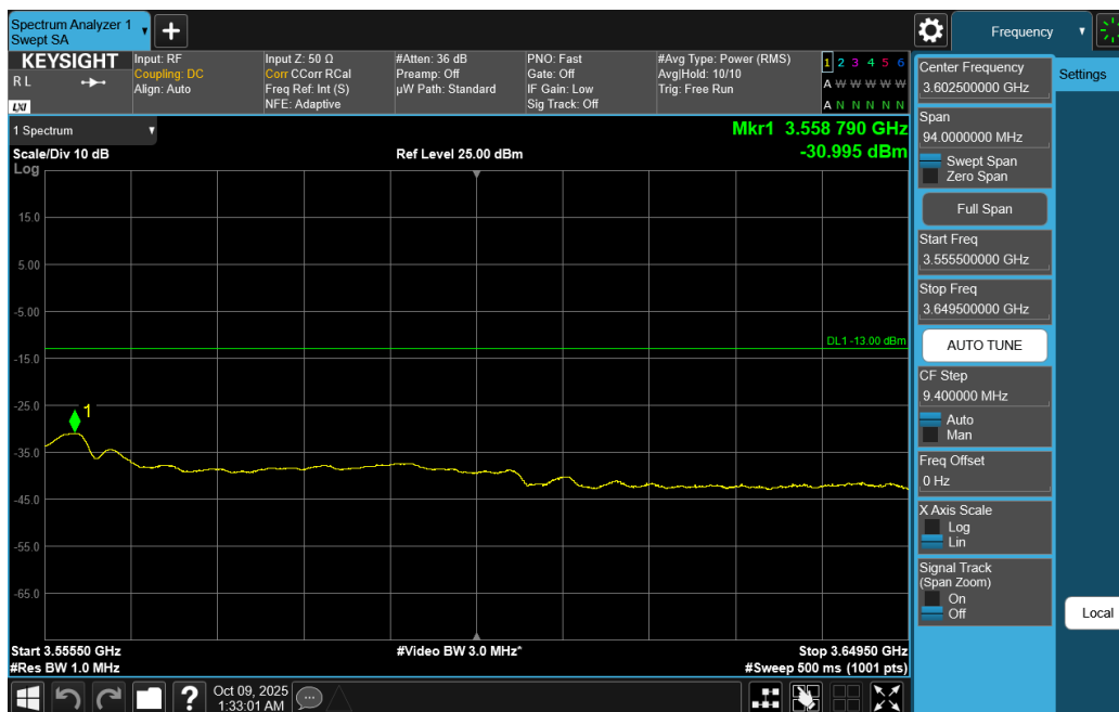
Plot 7-186. Extended Upper Band Edge Plot (NR Band n77 DoD-Band - 60MHz DFT-s-OFDM QPSK – Full RB)
