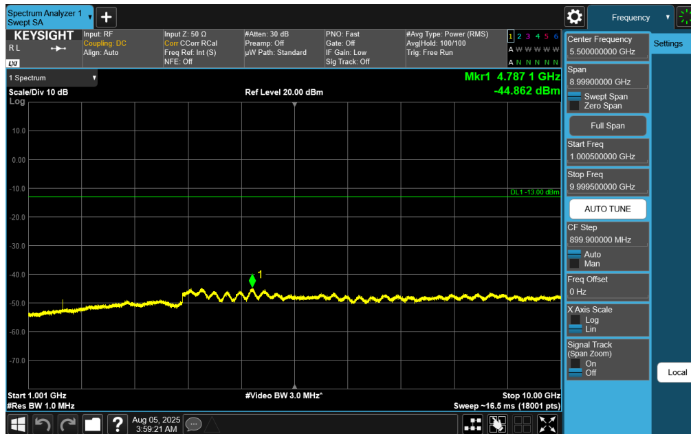
Plot 7-74. Conducted Spurious Plot (NR Band n14 - 5MHz DFT-s-OFDM QPSK - RB Size 1, RB Offset 0 - Low Channel)
