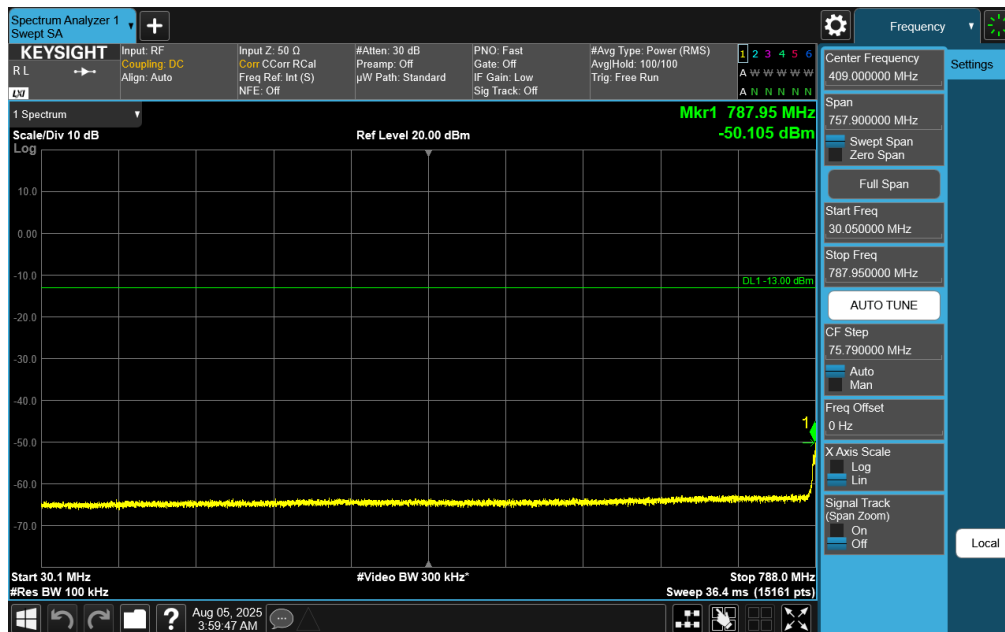
Plot 7-75. Conducted Spurious Plot (NR Band n14 - 10MHz DFT-s-OFDM QPSK - RB Size 1, RB Offset 0 - Mid Channel)
