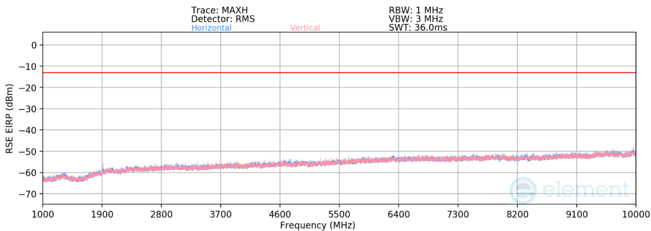
Plot 7-128. Antenna 2 Radiated Spurious Plot Above 1GHz (NR Band n26)
