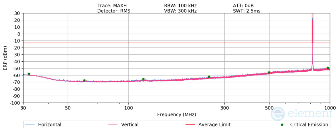
Plot 7-127. Antenna 2 Radiated Spurious Plot Below 1GHz (NR Band n26)
