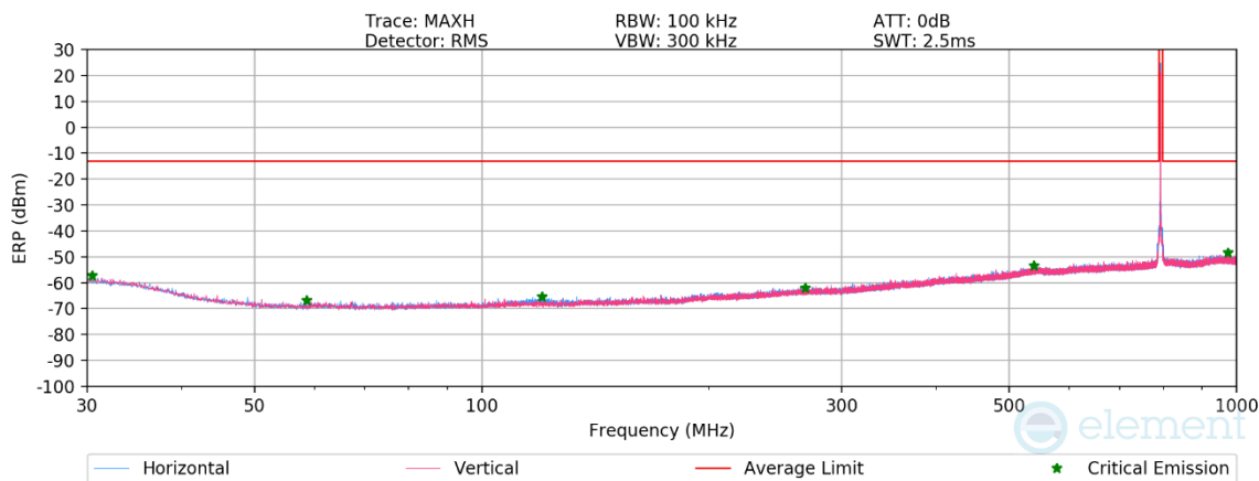
Plot 7-125. Antenna 2 Radiated Spurious Plot Below 1GHz (NR Band n14)
