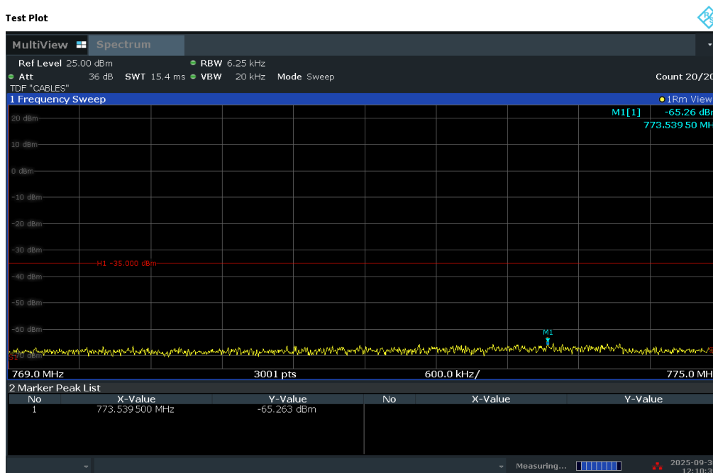
Plot 7-98. Lower Emission Mask Plot (LTE Band 14 - 5MHz QPSK – RB Size 25)
