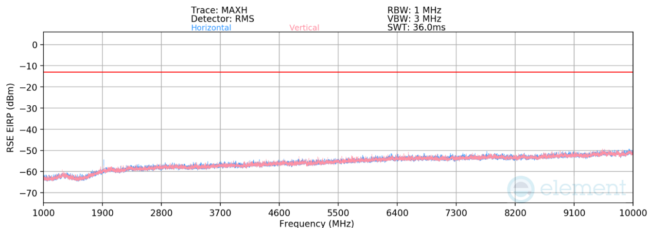
Plot 7-126. Antenna 2 Radiated Spurious Plot Above 1GHz (NR Band n14)
