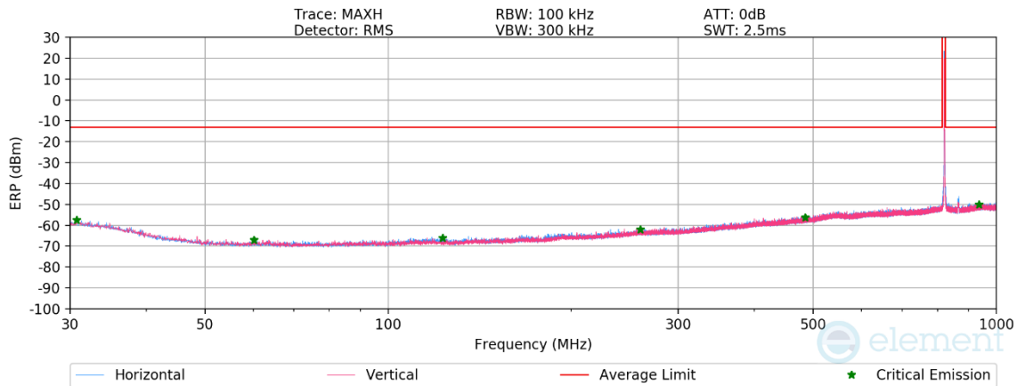
Plot 7-121. Antenna 2 Radiated Spurious Plot Below 1GHz (LTE Band 26)
