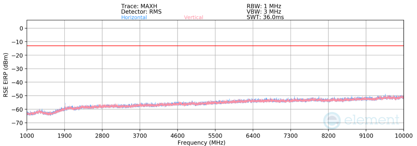
Plot 7-122. Antenna 2 Radiated Spurious Plot Above 1GHz (LTE Band 26)
