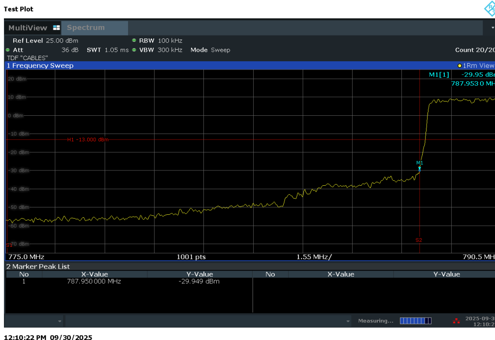
Plot 7-97. Lower Band Edge Plot (LTE Band 14 - 5MHz QPSK – RB Size 25)
