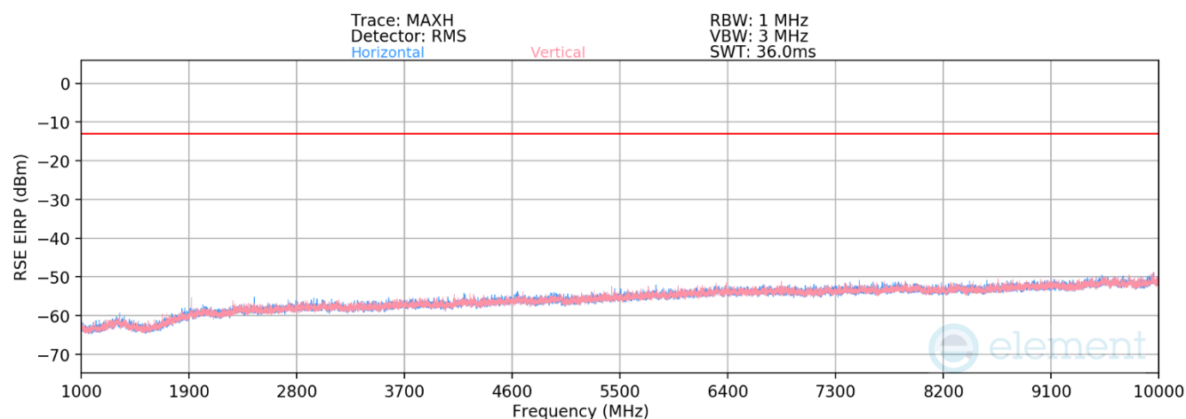
Plot 7-124. Antenna 2 Radiated Spurious Plot Above 1GHz (LTE Band 14)
