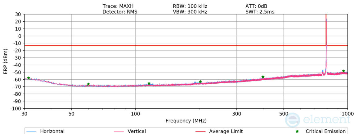
Plot 7-123. Antenna 2 Radiated Spurious Plot Below 1GHz (LTE Band 14)
