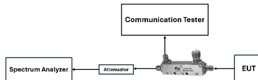
Figure 7-3. LTE Test Instrument & Measurement Setup
