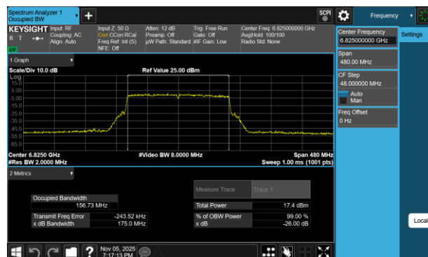
Plot 7-12 26dB BW & 99% OBW Antenna 5T (160MHz BW 802.11be(SU) - Ch.175)
