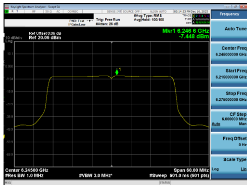
Plot 7-66 PSD Antenna 3b (40MHz BW 802.11be(SU) - Ch.59)
