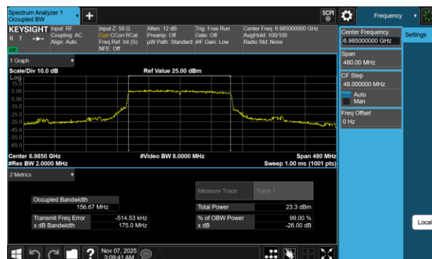
Plot 7-48 26dB BW & 99% OBW Antenna 1b (160MHz BW 802.11be(SU) - Ch.207)
