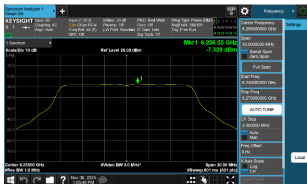
Plot 7-65 PSD Antenna 3b (20MHz BW 802.11a - Ch.61)
