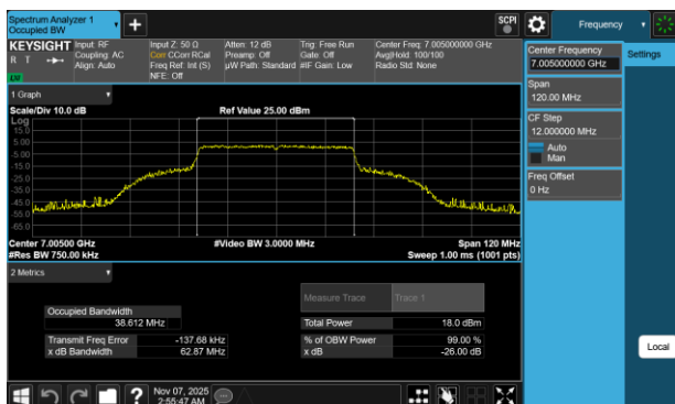
Plot 7-46 26dB BW & 99% OBW Antenna 1b (40MHz BW 802.11be(SU) - Ch.211)
