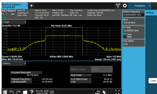
Plot 7-10 26dB BW & 99% OBW Antenna 5T (40MHz BW 802.11be(SU) - Ch.123)
