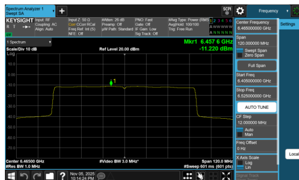
Plot 7-55 PSD Antenna 5T (80MHz BW 802.11be(SU) - Ch.103)
