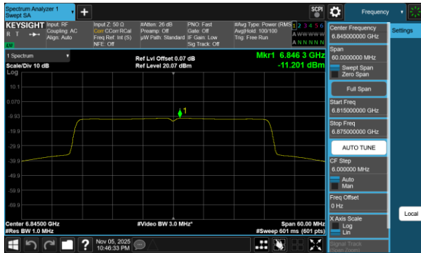
Plot 7-58 PSD Antenna 5T (40MHz BW 802.11be(SU) - Ch.179)
