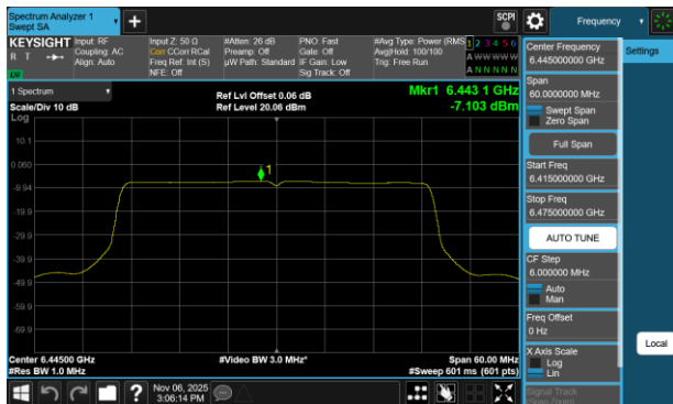
Plot 7-70 PSD Antenna 3b (40MHz BW 802.11be(SU) - Ch.99)
