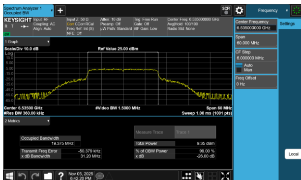
Plot 7-9 26dB BW & 99% OBW Antenna 5T (20MHz BW 802.11be(SU) - Ch.117)
