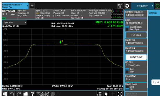
Plot 7-69 PSD Antenna 3b (20MHz BW 802.11a - Ch.97)
