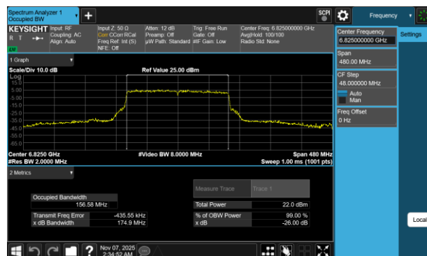
Plot 7-44 26dB BW & 99% OBW Antenna 1b (160MHz BW 802.11be(SU) - Ch.175)
