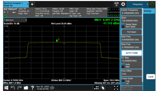
Plot 7-59 PSD Antenna 5T (80MHz BW 802.11be(SU) - Ch.151)
