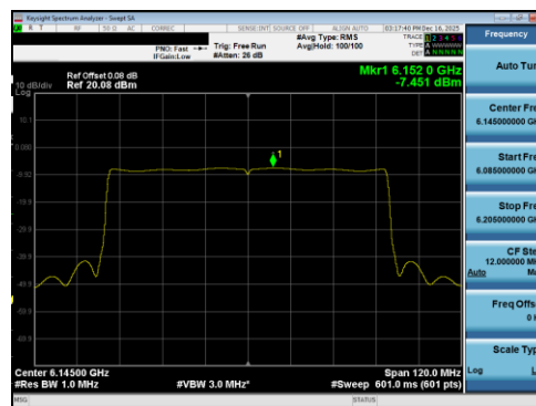
Plot 7-67 PSD Antenna 3b (80MHz BW 802.11be(SU) - Ch.39)
