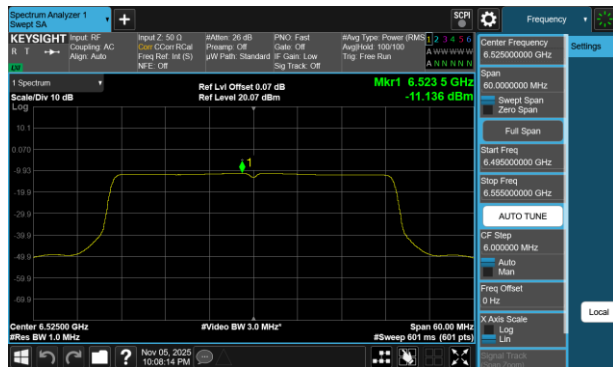
Plot 7-54 PSD Antenna 5T (40MHz BW 802.11be(SU) - Ch.115)
