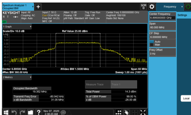
Plot 7-45 26dB BW & 99% OBW Antenna 1b (20MHz BW 802.11be(SU) - Ch.189)
