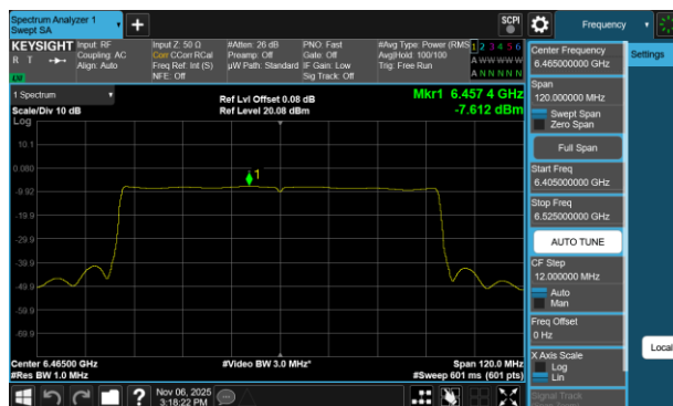
Plot 7-71 PSD Antenna 3b (80MHz BW 802.11be(SU) - Ch.103)
