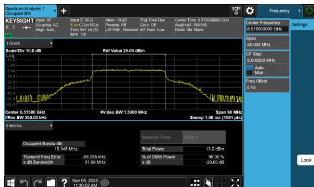
Plot 7-21 26dB BW & 99% OBW Antenna 3b (20MHz BW 802.11be(SU) - Ch.113)
