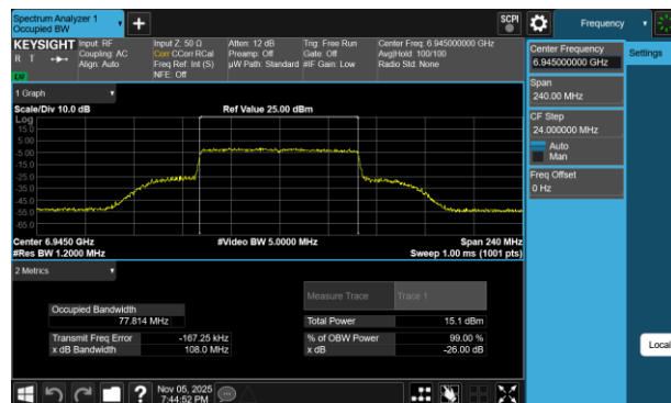
Plot 7-15 26dB BW & 99% OBW Antenna 5T (80MHz BW 802.11be(SU) - Ch.199)
