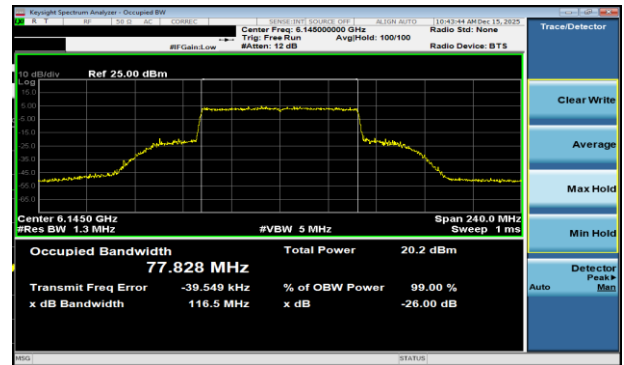
Plot 7-35 26dB BW & 99% OBW Antenna 1b (80MHz BW 802.11be(SU) - Ch.39)
