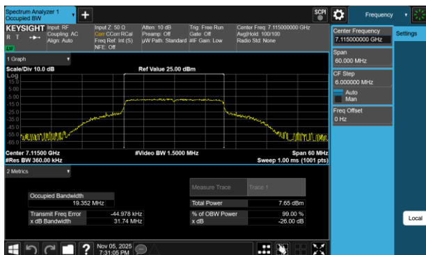
Plot 7-13 26dB BW & 99% OBW Antenna 5T (20MHz BW 802.11be(SU) - Ch.233)
