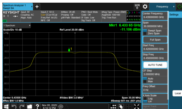
Plot 7-53 PSD Antenna 5T (20MHz BW 802.11a - Ch.97)
