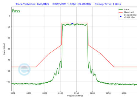
Plot 7-179 In-Band Emission Plot Antenna 3b (80MHz BW 802.11be(SU) (UNII Band 5) - Ch.39)
