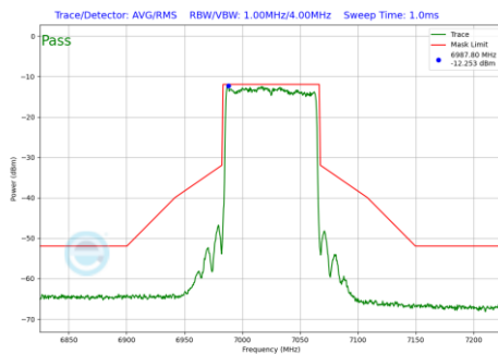
Plot 7-235 In-Band Emission Plot CDD Primary Antenna 5T (80MHz BW 802.11be(SU) (UNII Band 8) - Ch.215)
