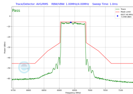
Plot 7-191 In-Band Emission Plot Antenna 3b (80MHz BW 802.11be(SU) (UNII Band 8) - Ch.199)
