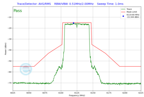
Plot 7-214 In-Band Emission Plot CDD Primary Antenna 3b (40MHz BW 802.11be(SU) (UNII Band 5) - Ch.35)
