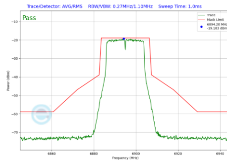
Plot 7-269 In-Band Emission Plot CDD Diversity Antenna 1b (20MHz BW 802.11a (UNII Band 8) - Ch.189)
