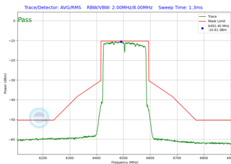
Plot 7-252 In-Band Emission Plot SDM Diversity Antenna 5T (160MHz BW 802.11be(SU) (UNII Band 6) - Ch.111)
