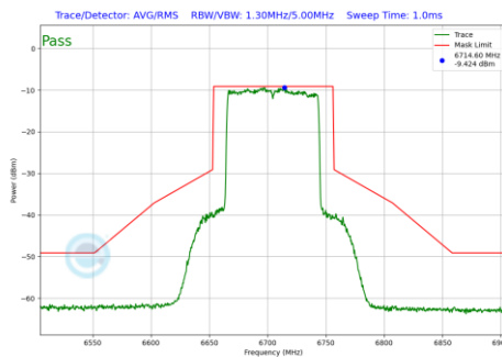
Plot 7-171 In-Band Emission Plot Antenna 5T (80MHz BW 802.11be(SU) (UNII Band 7) - Ch.151)
