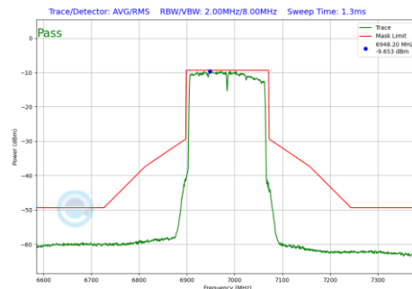
Plot 7-176 In-Band Emission Plot Antenna 5T (160MHz BW 802.11be(SU) (UNII Band 8) - Ch.207)
