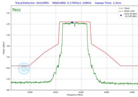
Plot 7-217 In-Band Emission Plot CDD Primary Antenna 5T (20MHz BW 802.11be(SU) (UNII Band 6) - Ch.97)
