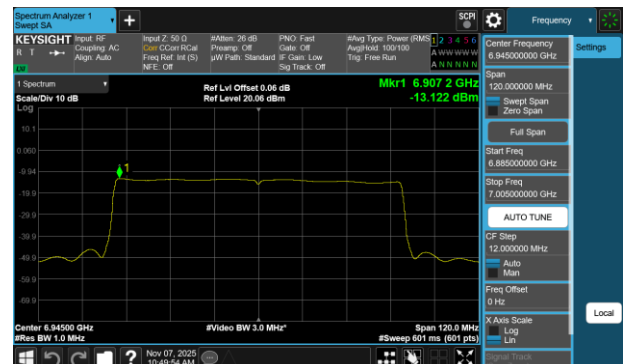
Plot 7-159 PSD SDM Diversity Antenna 1b (80MHz BW 802.11be(SU) - Ch.199)
