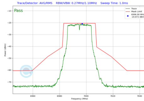
Plot 7-237 In-Band Emission Plot CDD Primary Antenna 3b (20MHz BW 802.11a (UNII Band 8) - Ch.209)
