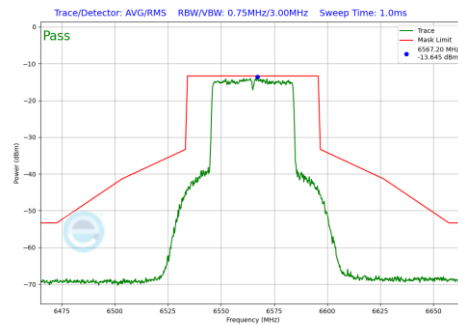
Plot 7-230 In-Band Emission Plot CDD Primary Antenna 3b (40MHz BW 802.11be(SU) (UNII Band 7) - Ch.123)
