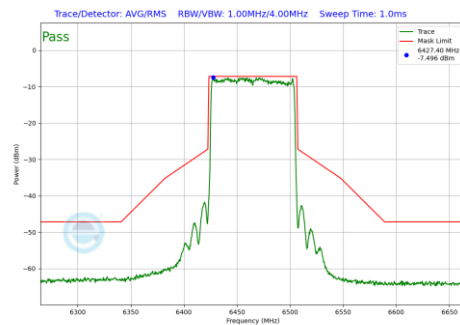
Plot 7-183 In-Band Emission Plot Antenna 3b (80MHz BW 802.11be(SU) (UNII Band 6) - Ch.103)
