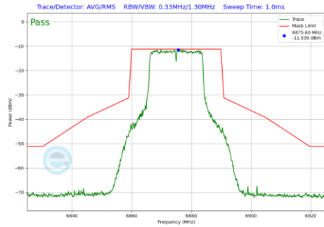
Plot 7-201 In-Band Emission Plot Antenna 1b (20MHz BW 802.11a (UNII Band 7) - Ch.185)
