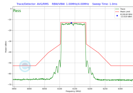
Plot 7-215 In-Band Emission Plot CDD Primary Antenna 3b (80MHz BW 802.11be(SU) (UNII Band 5) - Ch.39)
