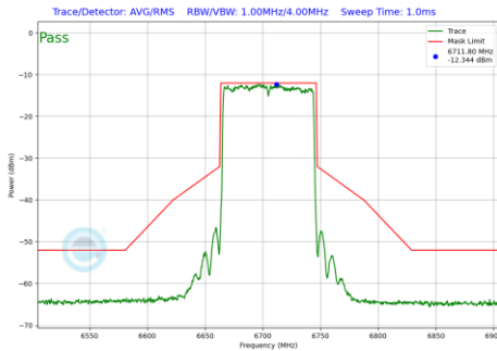
Plot 7-259 In-Band Emission Plot SDM Diversity Antenna 5T (80MHz BW 802.11be(SU) (UNII Band 7) - Ch.151)
