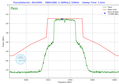
Plot 7-169 In-Band Emission Plot Antenna 5T (20MHz BW 802.11be(SU) (UNII Band 7) - Ch.117)
