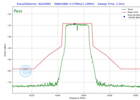
Plot 7-245 In-Band Emission Plot CDD Diversity Antenna 1b (20MHz BW 802.11a (UNII Band 5) - Ch.61)
