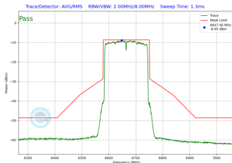
Plot 7-172 In-Band Emission Plot Antenna 5T (160MHz BW 802.11be(SU) (UNII Band 7) - Ch.143)
