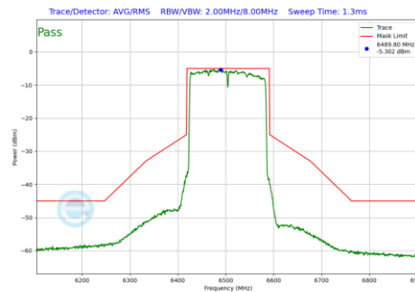
Plot 7-184 In-Band Emission Plot Antenna 3b (160MHz BW 802.11be(SU) (UNII Band 6) - Ch.111)
