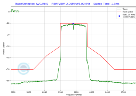
Plot 7-212 In-Band Emission Plot CDD Primary Antenna 5T (160MHz BW 802.11be(SU) (UNII Band 5) - Ch.47)
