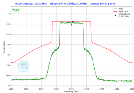
Plot 7-202 In-Band Emission Plot Antenna 1b (40MHz BW 802.11be(SU) (UNII Band 7) - Ch.155)
