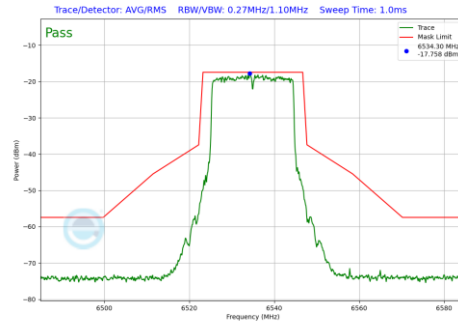
Plot 7-229 In-Band Emission Plot CDD Primary Antenna 3b (20MHz BW 802.11be(SU) (UNII Band 7) - Ch.117)
