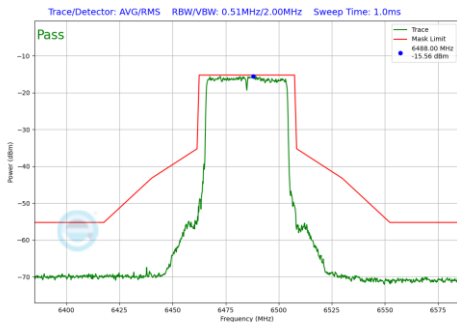
Plot 7-250 In-Band Emission Plot SDM Diversity Antenna 5T (40MHz BW 802.11be(SU) (UNII Band 6) - Ch.107)
