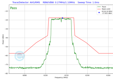
Plot 7-209 In-Band Emission Plot CDD Primary Antenna 5T (20MHz BW 802.11be(SU) (UNII Band 5) - Ch.33)
