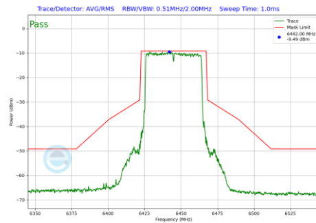
Plot 7-182 In-Band Emission Plot Antenna 3b (40MHz BW 802.11be(SU) (UNII Band 6) - Ch.99)
