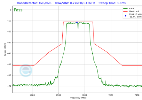
Plot 7-189 In-Band Emission Plot Antenna 3b (20MHz BW 802.11a (UNII Band 8) - Ch.209)
