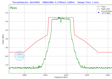
Plot 7-161 In-Band Emission Plot Antenna 5T (20MHz BW 802.11a (UNII Band 5) - Ch.33)
