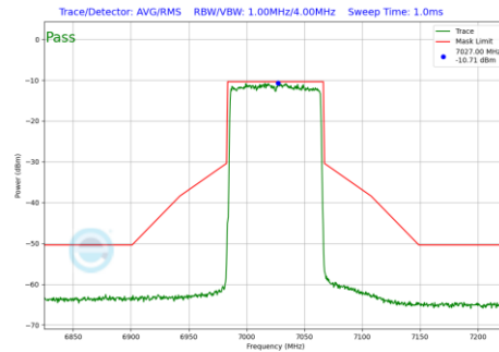
Plot 7-271 In-Band Emission Plot SDM Diversity Antenna 1b (80MHz BW 802.11be(SU) (UNII Band 8) - Ch.215)
