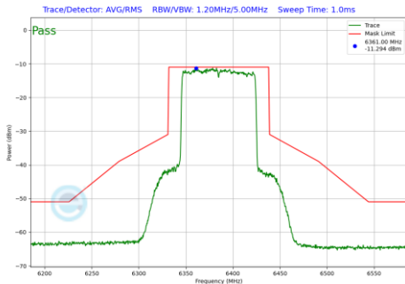
Plot 7-243 In-Band Emission Plot SDM Diversity Antenna 5T (80MHz BW 802.11be(SU) (UNII Band 5) - Ch.87)
