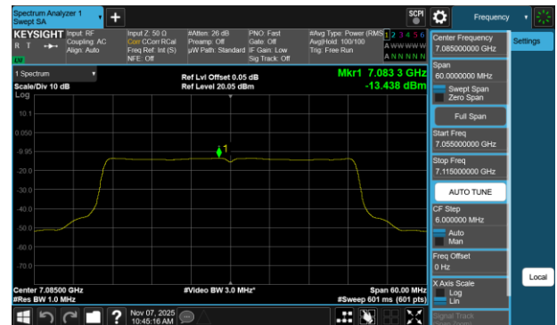
Plot 7-158 PSD SDM Diversity Antenna 1b (40MHz BW 802.11be(SU) - Ch.227)
