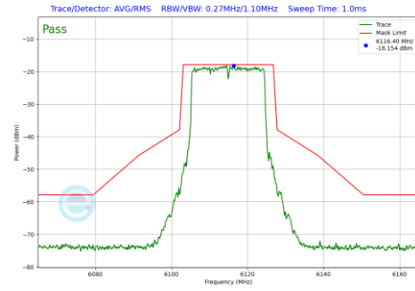
Plot 7-213 In-Band Emission Plot CDD Primary Antenna 3b (20MHz BW 802.11be(SU) (UNII Band 5) - Ch.33)
