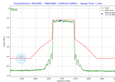
Plot 7-231 In-Band Emission Plot CDD Primary Antenna 3b (80MHz BW 802.11be(SU) (UNII Band 7) - Ch.151)
