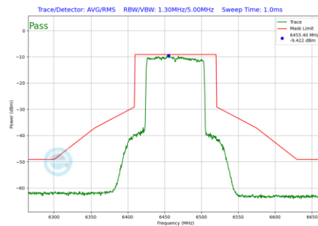
Plot 7-167 In-Band Emission Plot Antenna 5T (80MHz BW 802.11be(SU) (UNII Band 6) - Ch.103)
