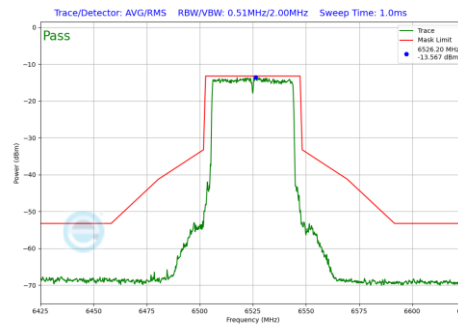
Plot 7-166 In-Band Emission Plot Antenna 5T (40MHz BW 802.11be(SU) (UNII Band 6) - Ch.115)
