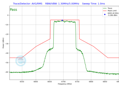
Plot 7-187 In-Band Emission Plot Antenna 3b (80MHz BW 802.11be(SU) (UNII Band 7) - Ch.151)
