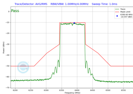
Plot 7-163 In-Band Emission Plot Antenna 5T (80MHz BW 802.11be(SU) (UNII Band 5) - Ch.87)
