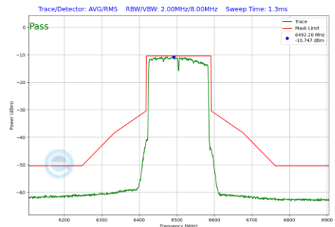
Plot 7-224 In-Band Emission Plot CDD Primary Antenna 3b (160MHz BW 802.11be(SU) (UNII Band 6) - Ch.111)
