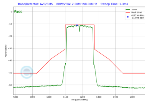
Plot 7-216 In-Band Emission Plot CDD Primary Antenna 3b (160MHz BW 802.11be(SU) (UNII Band 5) - Ch.47)
