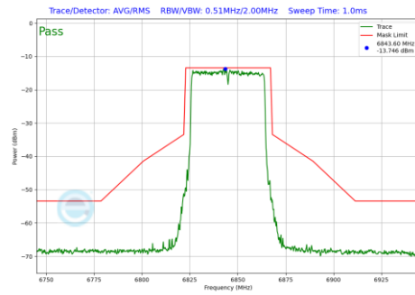
Plot 7-262 In-Band Emission Plot SDM Diversity Antenna 1b (40MHz BW 802.11be(SU) (UNII Band 7) - Ch.179)
