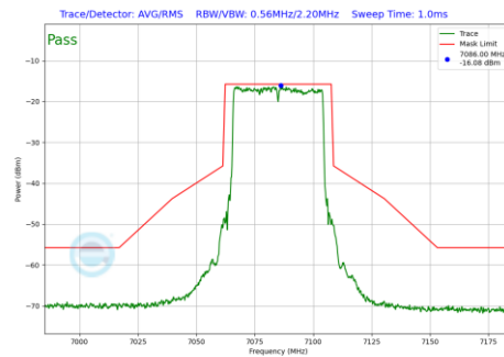
Plot 7-238 In-Band Emission Plot CDD Primary Antenna 3b (40MHz BW 802.11be(SU) (UNII Band 8) - Ch.227)
