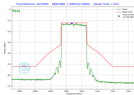
Plot 7-239 In-Band Emission Plot CDD Primary Antenna 3b (80MHz BW 802.11be(SU) (UNII Band 8) - Ch.215)
