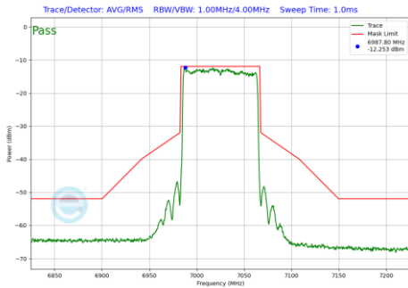
Plot 7-267 In-Band Emission Plot SDM Diversity Antenna 5T (80MHz BW 802.11be(SU) (UNII Band 8) - Ch.215)
