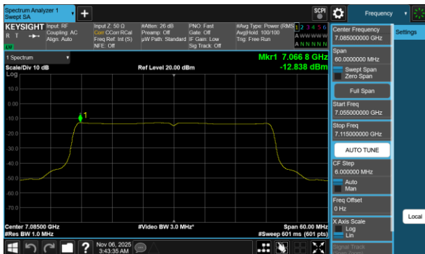
Plot 7-154 PSD SDM Diversity Antenna 5T (40MHz BW 802.11be(SU) - Ch.227)
