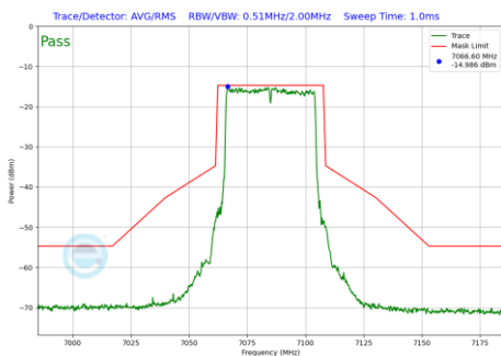
Plot 7-266 In-Band Emission Plot SDM Diversity Antenna 5T (40MHz BW 802.11be(SU) (UNII Band 8) - Ch.227)
