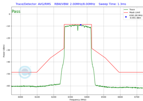
Plot 7-164 In-Band Emission Plot Antenna 5T (160MHz BW 802.11be(SU) (UNII Band 5) - Ch.79)
