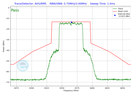
Plot 7-226 In-Band Emission Plot CDD Primary Antenna 5T (40MHz BW 802.11be(SU) (UNII Band 7) - Ch.123)
