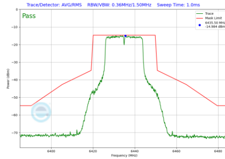
Plot 7-165 In-Band Emission Plot Antenna 5T (20MHz BW 802.11a (UNII Band 6) - Ch.97)
