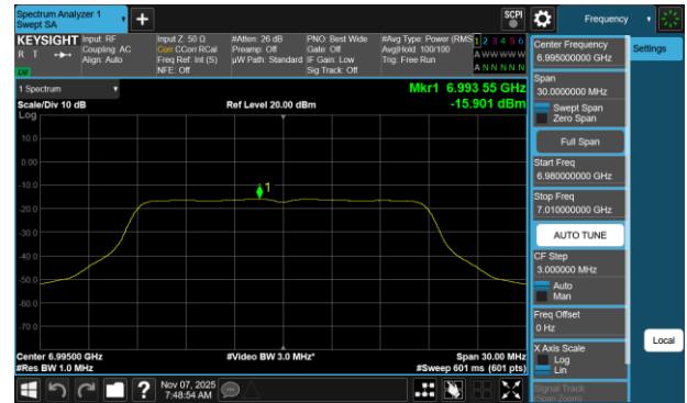
Plot 7-157 PSD CDD Diversity Antenna 1b (20MHz BW 802.11a - Ch.209)
