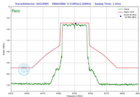
Plot 7-218 In-Band Emission Plot CDD Primary Antenna 5T (40MHz BW 802.11be(SU) (UNII Band 6) - Ch.115)
