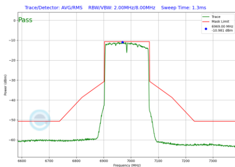
Plot 7-268 In-Band Emission Plot SDM Diversity Antenna 5T (160MHz BW 802.11be(SU) (UNII Band 8) - Ch.207)
