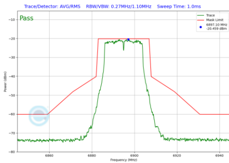
Plot 7-265 In-Band Emission Plot CDD Diversity Antenna 5T (20MHz BW 802.11a (UNII Band 8) - Ch.189)
