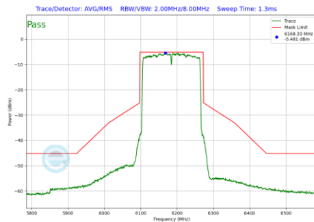
Plot 7-180 In-Band Emission Plot Antenna 3b (160MHz BW 802.11be(SU) (UNII Band 5) - Ch.47)
