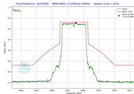
Plot 7-174 In-Band Emission Plot Antenna 5T (40MHz BW 802.11be(SU) (UNII Band 8) - Ch.187)
