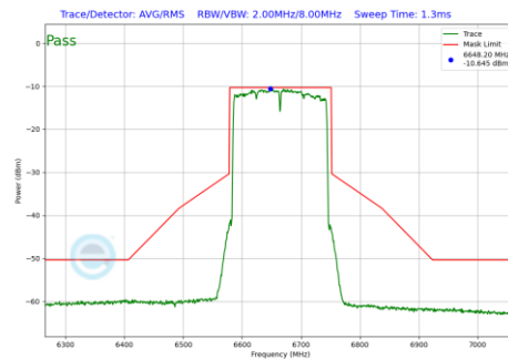
Plot 7-232 In-Band Emission Plot CDD Primary Antenna 3b (160MHz BW 802.11be(SU) (UNII Band 7) - Ch.143)
