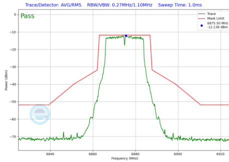
Plot 7-185 In-Band Emission Plot Antenna 3b (20MHz BW 802.11a (UNII Band 7) - Ch.185)
