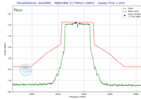
Plot 7-221 In-Band Emission Plot CDD Primary Antenna 3b (20MHz BW 802.11be(SU) (UNII Band 6) - Ch.97)
