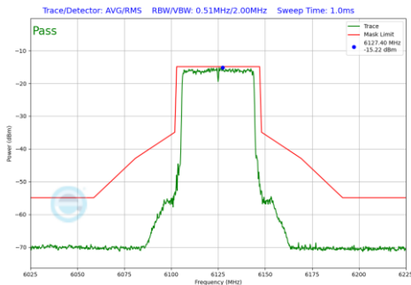
Plot 7-242 In-Band Emission Plot SDM Diversity Antenna 5T (40MHz BW 802.11be(SU) (UNII Band 5) - Ch.35)
