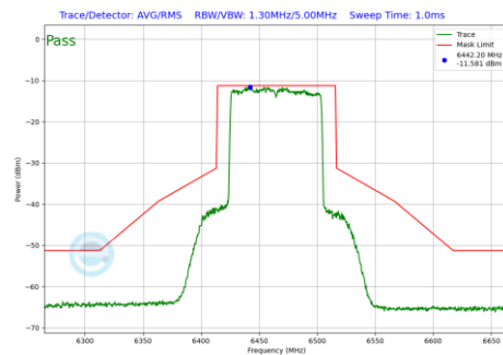
Plot 7-223 In-Band Emission Plot CDD Primary Antenna 3b (80MHz BW 802.11be(SU) (UNII Band 6) - Ch.103)
