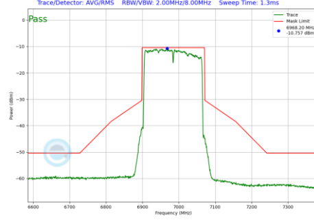
Plot 7-240 In-Band Emission Plot CDD Primary Antenna 3b (160MHz BW 802.11be(SU) (UNII Band 8) - Ch.207)
