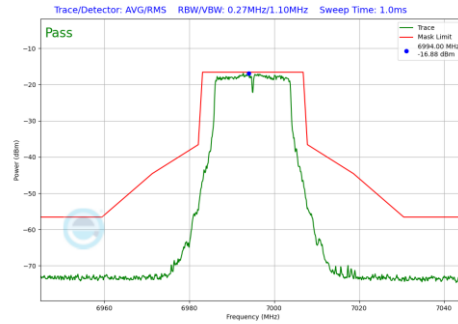
Plot 7-173 In-Band Emission Plot Antenna 5T (20MHz BW 802.11a (UNII Band 8) - Ch.209)
