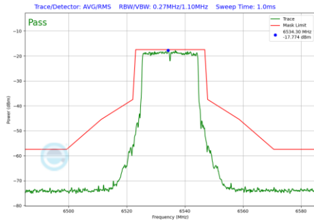
Plot 7-225 In-Band Emission Plot CDD Primary Antenna 5T (20MHz BW 802.11be(SU) (UNII Band 7) - Ch.117)
