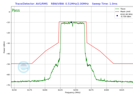
Plot 7-178 In-Band Emission Plot Antenna 3b (40MHz BW 802.11be(SU) (UNII Band 5) - Ch.59)
