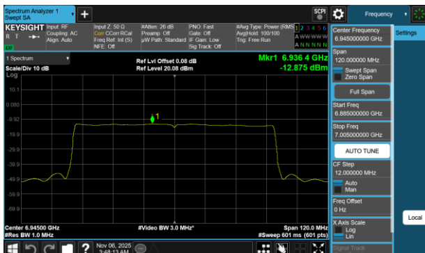
Plot 7-155 PSD SDM Diversity Antenna 5T (80MHz BW 802.11be(SU) - Ch.199)
