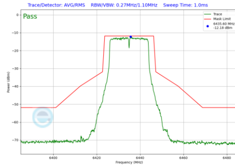
Plot 7-181 In-Band Emission Plot Antenna 3b (20MHz BW 802.11a (UNII Band 6) - Ch.97)
