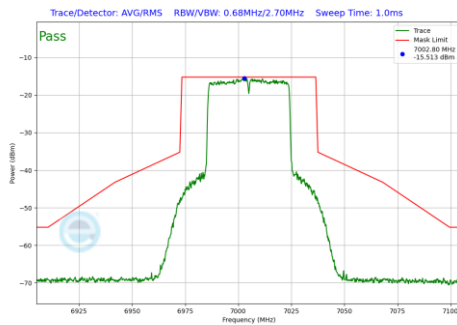
Plot 7-234 In-Band Emission Plot SDM Primary Antenna 5T (40MHz BW 802.11be(SU) (UNII Band 8) - Ch.211)
