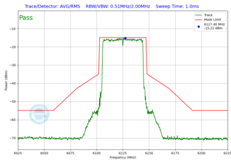
Plot 7-210 In-Band Emission Plot CDD Primary Antenna 5T (40MHz BW 802.11be(SU) (UNII Band 5) - Ch.35)
