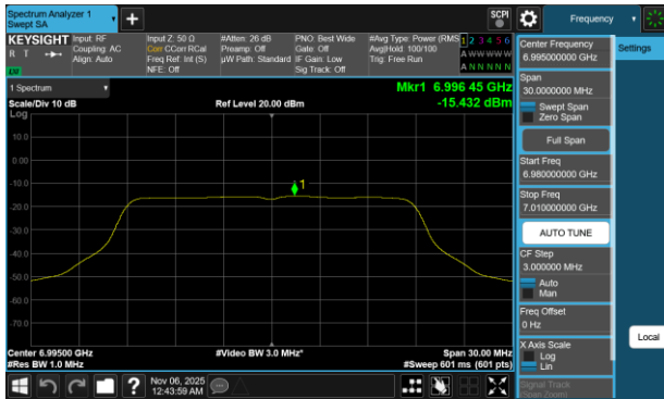
Plot 7-153 PSD CDD Diversity Antenna 5T (20MHz BW 802.11a - Ch.209)
