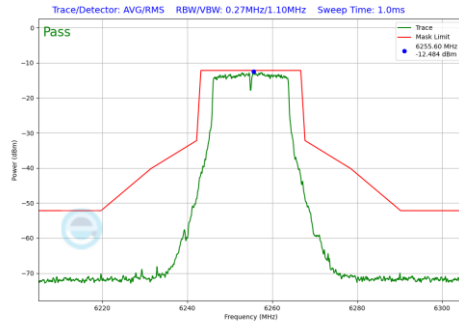
Plot 7-177 In-Band Emission Plot Antenna 3b (20MHz BW 802.11a (UNII Band 5) - Ch.61)
