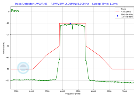
Plot 7-228 In-Band Emission Plot CDD Primary Antenna 5T (160MHz BW 802.11be(SU) (UNII Band 7) - Ch.143)
