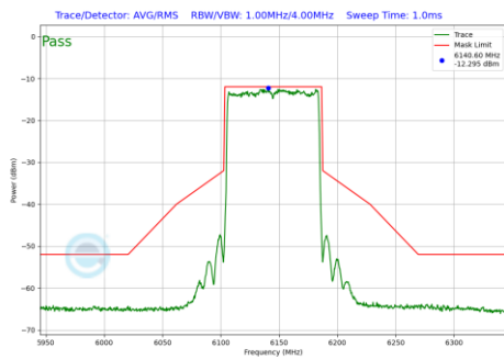
Plot 7-211 In-Band Emission Plot CDD Primary Antenna 5T (80MHz BW 802.11be(SU) (UNII Band 5) - Ch.39)
