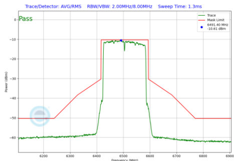
Plot 7-220 In-Band Emission Plot CDD Primary Antenna 5T (160MHz BW 802.11be(SU) (UNII Band 6) - Ch.111)
