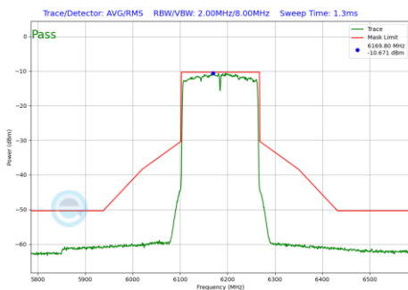
Plot 7-244 In-Band Emission Plot SDM Diversity Antenna 5T (160MHz BW 802.11be(SU) (UNII Band 5) - Ch.47)
