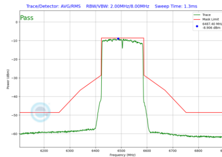
Plot 7-168 In-Band Emission Plot Antenna 5T (160MHz BW 802.11be(SU) (UNII Band 6) - Ch.111)
