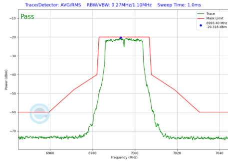
Plot 7-233 In-Band Emission Plot CDD Primary Antenna 5T (20MHz BW 802.11a (UNII Band 8) - Ch.209)
