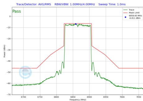
Plot 7-203 In-Band Emission Plot Antenna 1b (80MHz BW 802.11be(SU) (UNII Band 7) - Ch.183)
