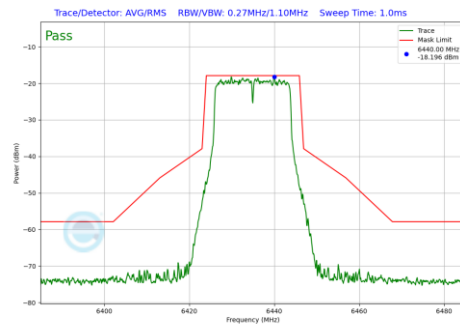
Plot 7-253 In-Band Emission Plot CDD Diversity Antenna 1b (20MHz BW 802.11a (UNII Band 6) - Ch.97)
