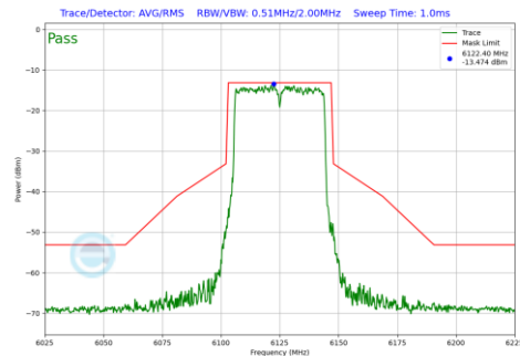
Plot 7-246 In-Band Emission Plot SDM Diversity Antenna 1b (40MHz BW 802.11be(SU) (UNII Band 5) - Ch.35)
