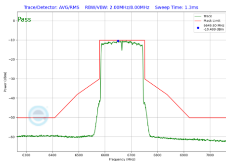
Plot 7-260 In-Band Emission Plot SDM Diversity Antenna 5T (160MHz BW 802.11be(SU) (UNII Band 7) - Ch.143)
