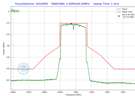
Plot 7-236 In-Band Emission Plot CDD Primary Antenna 5T (160MHz BW 802.11be(SU) (UNII Band 8) - Ch.207)
