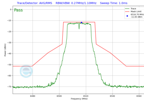
Plot 7-197 In-Band Emission Plot Antenna 1b (20MHz BW 802.11a (UNII Band 6) - Ch.113)
