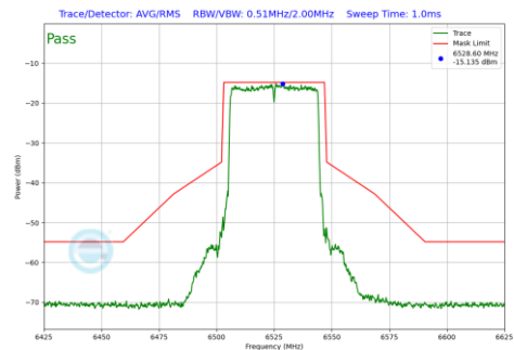
Plot 7-222 In-Band Emission Plot CDD Primary Antenna 3b (40MHz BW 802.11be(SU) (UNII Band 6) - Ch.115)
