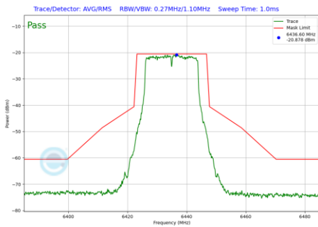
Plot 7-249 In-Band Emission Plot CDD Diversity Antenna 5T (20MHz BW 802.11a (UNII Band 6) - Ch.97)
