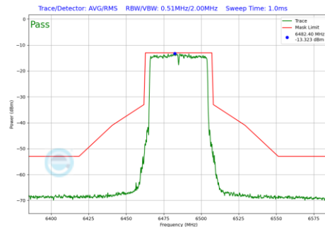
Plot 7-254 In-Band Emission Plot SDM Diversity Antenna 1b (40MHz BW 802.11be(SU) (UNII Band 6) - Ch.107)
