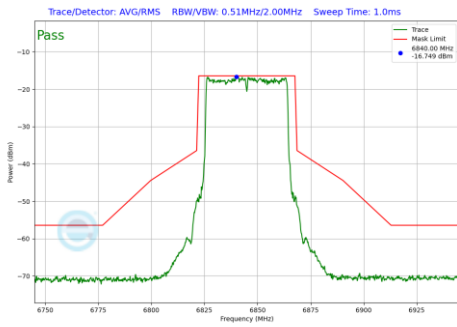
Plot 7-258 In-Band Emission Plot SDM Diversity Antenna 5T (40MHz BW 802.11be(SU) (UNII Band 7) - Ch.179)
