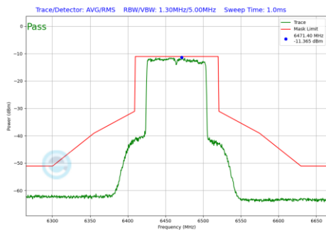
Plot 7-219 In-Band Emission Plot CDD Primary Antenna 5T (80MHz BW 802.11be(SU) (UNII Band 6) - Ch.103)
