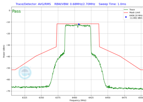
Plot 7-162 In-Band Emission Plot Antenna 5T (40MHz BW 802.11be(SU) (UNII Band 5) - Ch.91)
