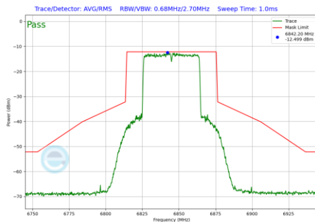
Plot 7-170 In-Band Emission Plot Antenna 5T (40MHz BW 802.11be(SU) (UNII Band 7) - Ch.179)
