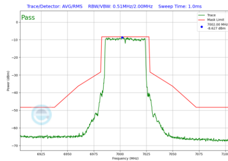
Plot 7-190 In-Band Emission Plot Antenna 3b (40MHz BW 802.11be(SU) (UNII Band 8) - Ch.211)
