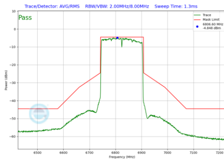
Plot 7-188 In-Band Emission Plot Antenna 3b (160MHz BW 802.11be(SU) (UNII Band 7) - Ch.175)
