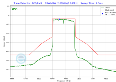
Plot 7-192 In-Band Emission Plot Antenna 3b (160MHz BW 802.11be(SU) (UNII Band 8) - Ch.207)
