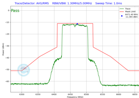
Plot 7-251 In-Band Emission Plot SDM Diversity Antenna 5T (80MHz BW 802.11be(SU) (UNII Band 6) - Ch.103)
