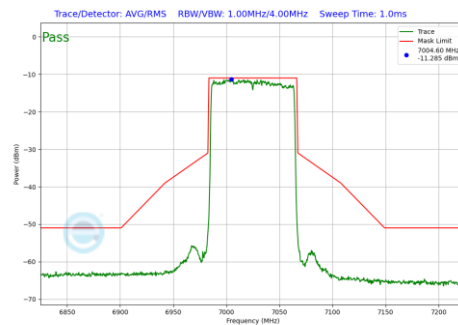
Plot 7-175 In-Band Emission Plot Antenna 5T (80MHz BW 802.11be(SU) (UNII Band 8) - Ch.215)
