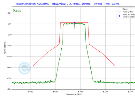
Plot 7-261 In-Band Emission Plot CDD Diversity Antenna 1b (20MHz BW 802.11a (UNII Band 7) - Ch.149)
