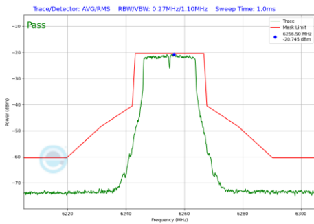
Plot 7-241 In-Band Emission Plot CDD Diversity Antenna 5T (20MHz BW 802.11a (UNII Band 5) - Ch.61)
