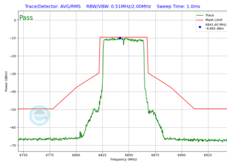
Plot 7-186 In-Band Emission Plot Antenna 3b (40MHz BW 802.11be(SU) (UNII Band 7) - Ch.179)
