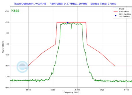
Plot 7-257 In-Band Emission Plot CDD Diversity Antenna 5T (20MHz BW 802.11a (UNII Band 7) - Ch.149)
