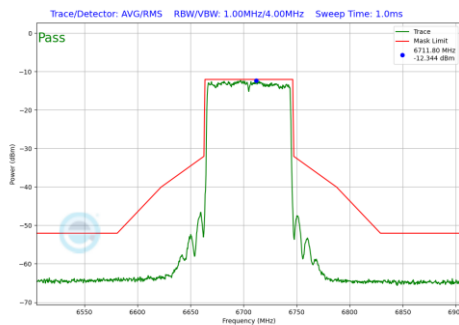
Plot 7-227 In-Band Emission Plot CDD Primary Antenna 5T (80MHz BW 802.11be(SU) (UNII Band 7) - Ch.151)
