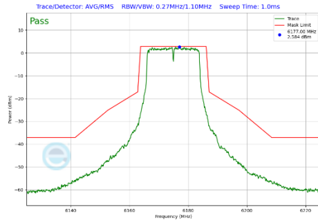
Plot 7-281 In-Band Emission Plot Antenna 5T (20MHz BW 802.11a (UNII Band 5) - Ch.45)
