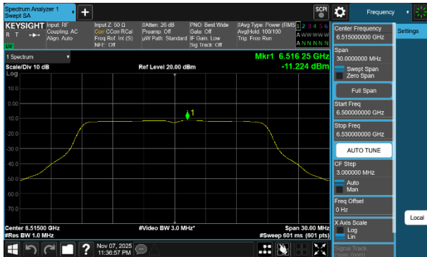
Plot 7-257 PSD Diversity Antenna 5T (20MHz BW 802.11a - Ch.113)
