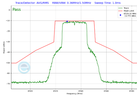
Plot 7-301 In-Band Emission Plot Antenna 5T (20MHz BW 802.11be(SU) (UNII Band 7) - Ch.117)
