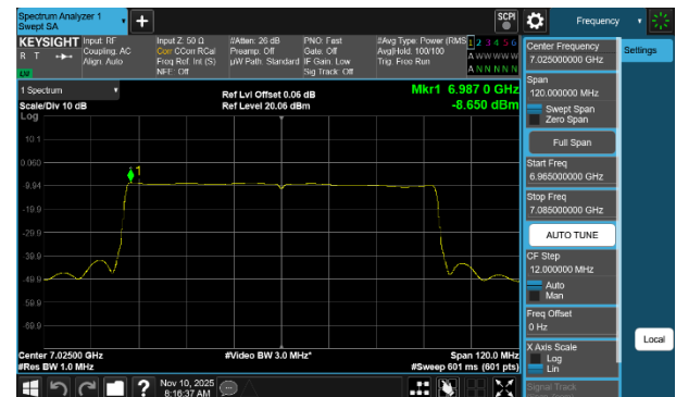
Plot 7-279 PSD SDM Diversity Antenna 1b (80MHz BW 802.11be(SU) - Ch.215)
