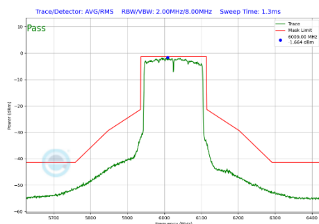
Plot 7-340 In-Band Emission Plot Antenna 1b (160MHz BW 802.11be(SU) (UNII Band 5) - Ch.15)
