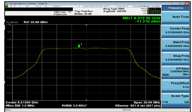
Plot 7-261 PSD CDD Diversity Antenna 1b (20MHz BW 802.11a - Ch.113)
