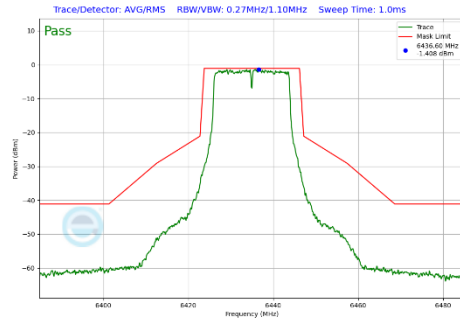
Plot 7-313 In-Band Emission Plot Antenna 3b (20MHz BW 802.11a (UNII Band 6) - Ch.97)
