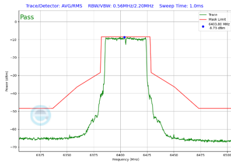
Plot 7-294 In-Band Emission Plot Antenna 5T (40MHz BW 802.11be(SU) (UNII Band 5) - Ch.91)
