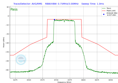
Plot 7-330 In-Band Emission Plot Antenna 3b (40MHz BW 802.11be(SU) (UNII Band 7) - Ch.123)
