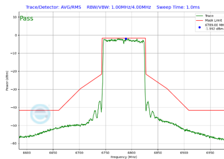
Plot 7-347 In-Band Emission Plot Antenna 1b (80MHz BW 802.11be(SU) (UNII Band 7) - Ch.167)
