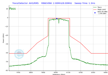
Plot 7-324 In-Band Emission Plot Antenna 3b (160MHz BW 802.11be(SU) (UNII Band 5) - Ch.15)
