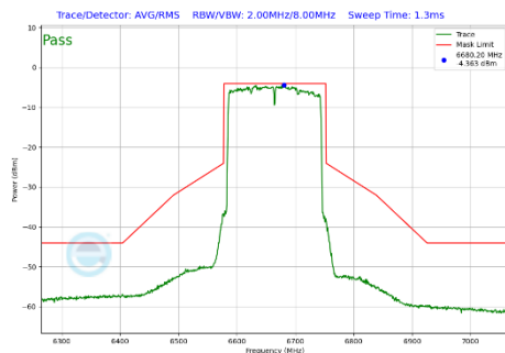
Plot 7-304 In-Band Emission Plot Antenna 5T (160MHz BW 802.11be(SU) (UNII Band 7) - Ch.143)
