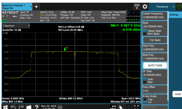
Plot 7-276 PSD SDM Diversity Antenna 5T (160MHz BW 802.11be(SU) - Ch.207)
