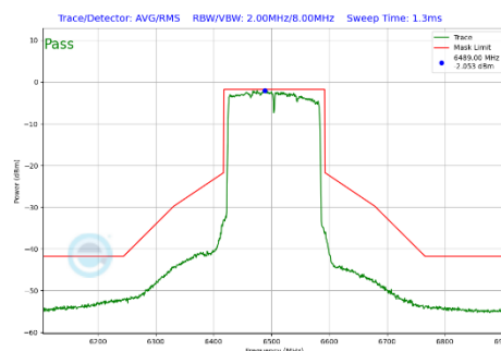
Plot 7-316 In-Band Emission Plot Antenna 3b (160MHz BW 802.11be(SU) (UNII Band 6) - Ch.111)
