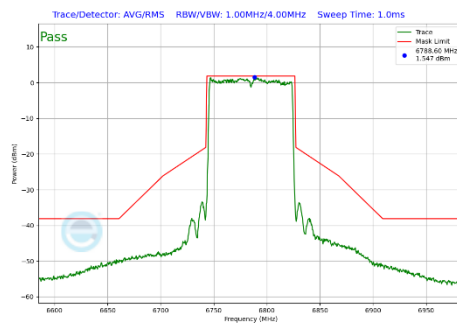
Plot 7-291 In-Band Emission Plot Antenna 5T (80MHz BW 802.11be(SU) (UNII Band 7) - Ch.167)
