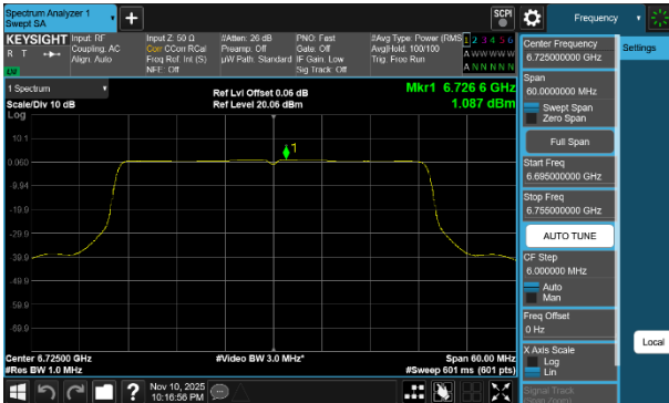
Plot 7-242 PSD CDD Diversity Antenna 5T (40MHz BW 802.11be(SU) - Ch.155)
