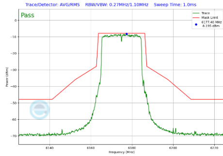
Plot 7-321 In-Band Emission Plot Antenna 3b (20MHz BW 802.11be(SU) (UNII Band 5) - Ch.45)
