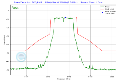
Plot 7-325 In-Band Emission Plot Antenna 3b (20MHz BW 802.11a (UNII Band 6) - Ch.97)
