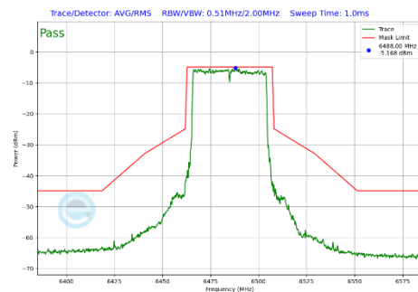
Plot 7-326 In-Band Emission Plot Antenna 3b (40MHz BW 802.11be(SU) (UNII Band 6) - Ch.107)
