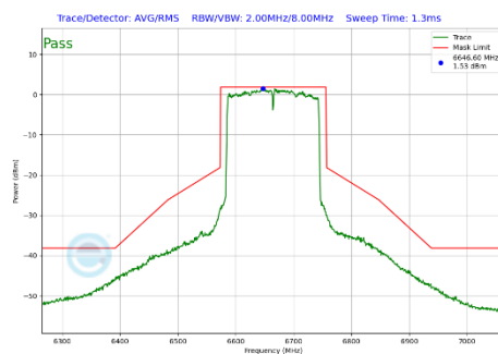
Plot 7-292 In-Band Emission Plot Antenna 5T (160MHz BW 802.11be(SU) (UNII Band 7) - Ch.143)
