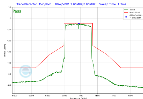
Plot 7-308 In-Band Emission Plot Antenna 5T (160MHz BW 802.11be(SU) (UNII Band 8) - Ch.207)
