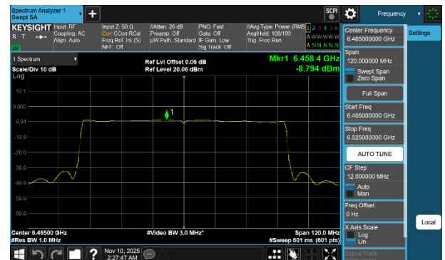
Plot 7-263 PSD SDM Diversity Antenna 1b (80MHz BW 802.11be(SU) - Ch.103)
