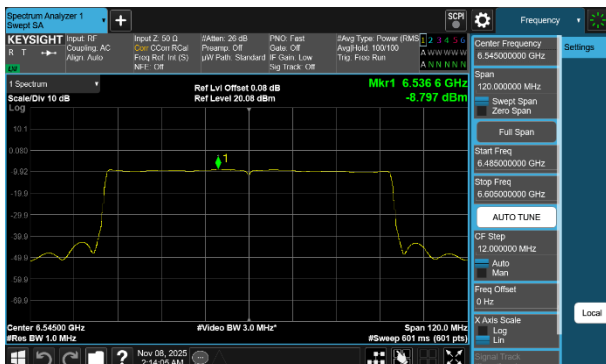
Plot 7-267 PSD SDM Diversity Antenna 5T (80MHz BW 802.11be(SU) - Ch.119)
