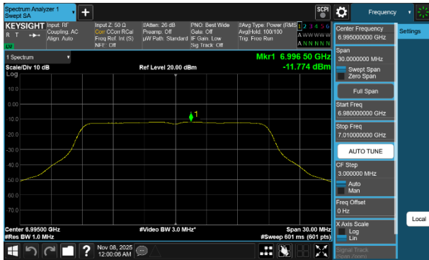
Plot 7-273 PSD CDD Diversity Antenna 5T (20MHz BW 802.11a - Ch.209)
