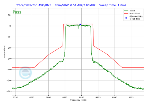
Plot 7-290 In-Band Emission Plot Antenna 5T (40MHz BW 802.11be(SU) (UNII Band 7) - Ch.179)
