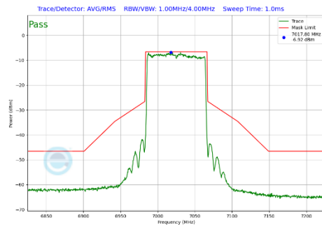
Plot 7-307 In-Band Emission Plot Antenna 5T (80MHz BW 802.11be(SU) (UNII Band 8) - Ch.215)
