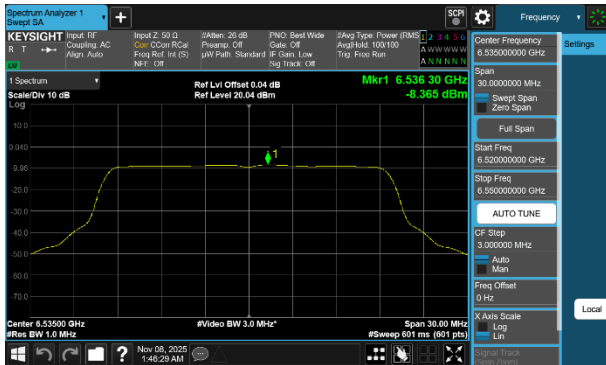
Plot 7-265 PSD SDM Diversity Antenna 5T (20MHz BW 802.11be(SU) - Ch.117)
