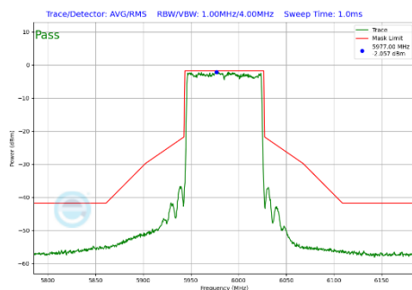
Plot 7-339 In-Band Emission Plot Antenna 1b (80MHz BW 802.11be(SU) (UNII Band 5) - Ch.7)
