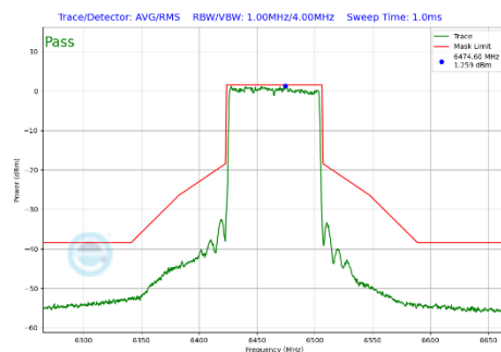
Plot 7-287 In-Band Emission Plot Antenna 5T (80MHz BW 802.11be(SU) (UNII Band 6) - Ch.103)
