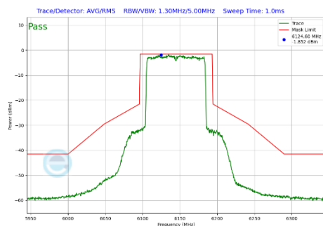
Plot 7-323 In-Band Emission Plot Antenna 3b (80MHz BW 802.11be(SU) (UNII Band 5) - Ch.39)
