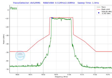
Plot 7-306 In-Band Emission Plot Antenna 5T (40MHz BW 802.11be(SU) (UNII Band 8) - Ch.227)
