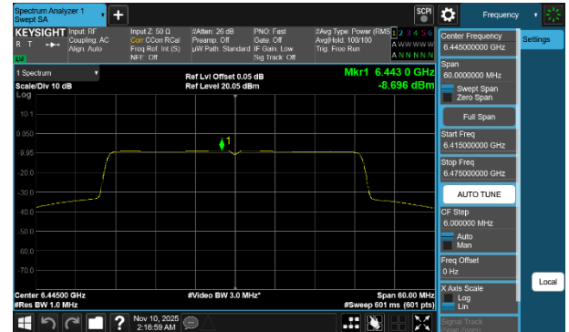
Plot 7-262 PSD SDM Diversity Antenna 1b (40MHz BW 802.11be(SU) - Ch.99)
