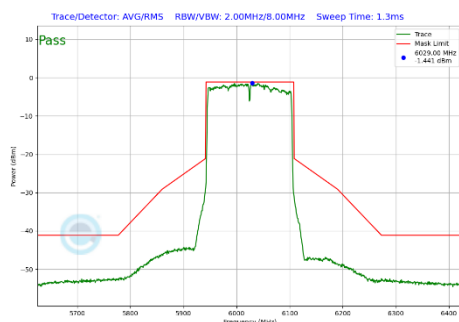
Plot 7-312 In-Band Emission Plot Antenna 3b (160MHz BW 802.11be(SU) (UNII Band 5) - Ch.15)
