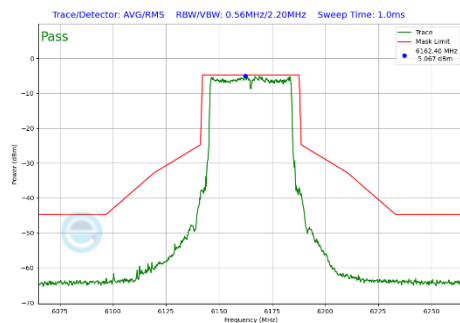
Plot 7-322 In-Band Emission Plot Antenna 3b (40MHz BW 802.11be(SU) (UNII Band 5) - Ch.43)
