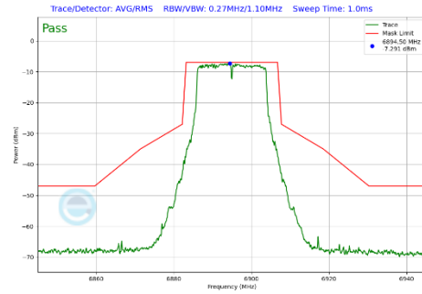
Plot 7-333 In-Band Emission Plot Antenna 3b (20MHz BW 802.11a (UNII Band 8) - Ch.189)
