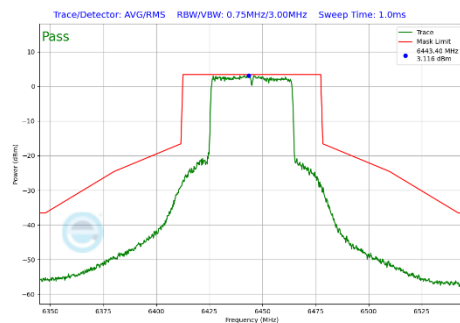
Plot 7-286 In-Band Emission Plot Antenna 5T (40MHz BW 802.11be(SU) (UNII Band 6) - Ch.99)
