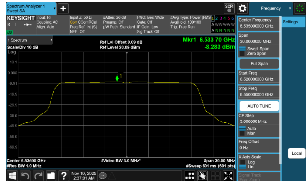
Plot 7-269 PSD SDM Diversity Antenna 1b (20MHz BW 802.11be(SU) - Ch.117)
