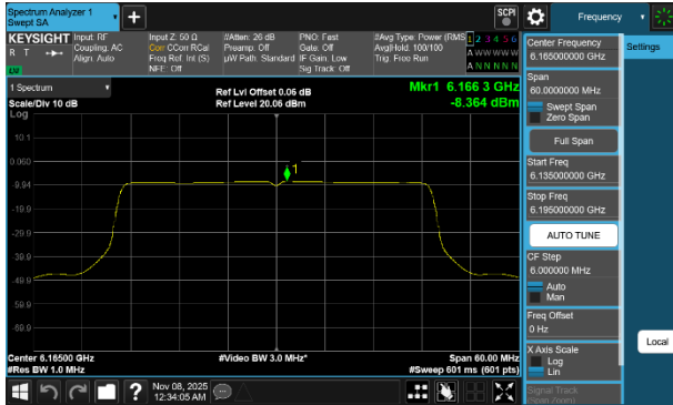
Plot 7-250 PSD SDM Diversity Antenna 5T (40MHz BW 802.11be(SU) - Ch.43)
