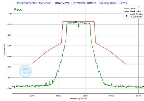
Plot 7-329 In-Band Emission Plot Antenna 3b (20MHz BW 802.11a (UNII Band 7) - Ch.185)
