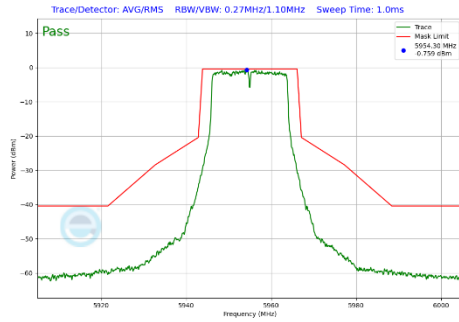
Plot 7-309 In-Band Emission Plot Antenna 3b (20MHz BW 802.11a (UNII Band 5) - Ch.1)
