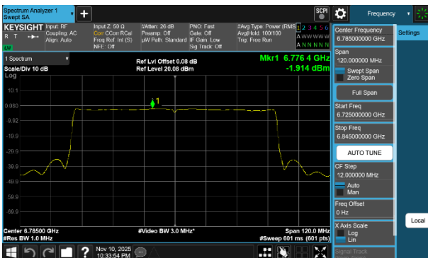
Plot 7-243 PSD CDD Diversity Antenna 5T (80MHz BW 802.11be(SU) - Ch.167)
