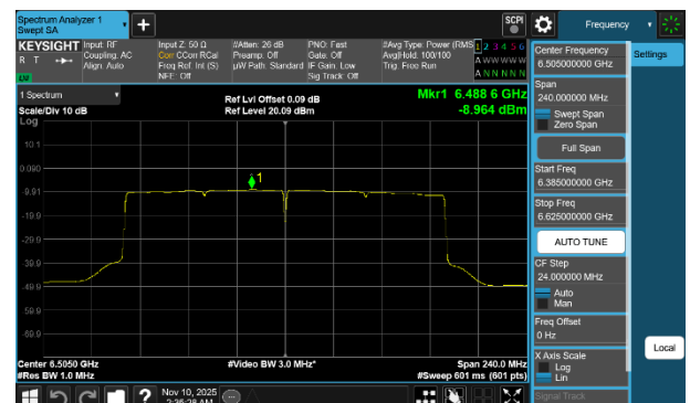
Plot 7-264 PSD SDM Diversity Antenna 1b (160MHz BW 802.11be(SU) - Ch.111)
