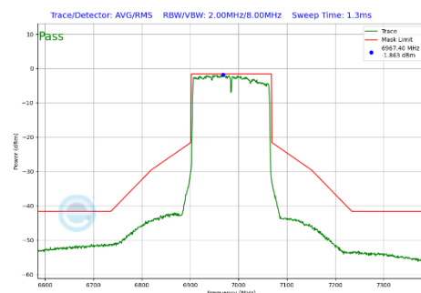
Plot 7-336 In-Band Emission Plot Antenna 3b (160MHz BW 802.11be(SU) (UNII Band 8) - Ch.207)
