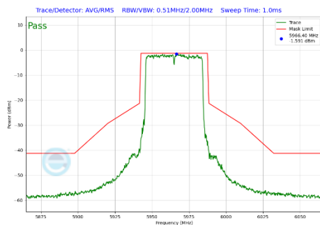
Plot 7-310 In-Band Emission Plot Antenna 3b (40MHz BW 802.11be(SU) (UNII Band 5) - Ch.3)
