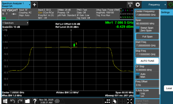
Plot 7-274 PSD SDM Diversity Antenna 5T (40MHz BW 802.11be(SU) - Ch.227)
