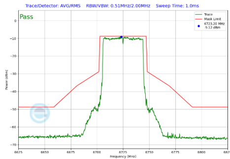
Plot 7-302 In-Band Emission Plot Antenna 5T (40MHz BW 802.11be(SU) (UNII Band 7) - Ch.155)
