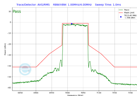
Plot 7-335 In-Band Emission Plot Antenna 3b (80MHz BW 802.11be(SU) (UNII Band 8) - Ch.215)
