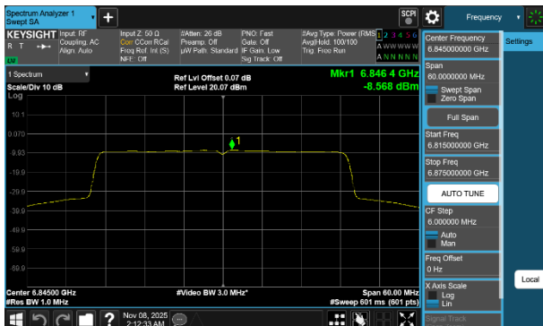
Plot 7-266 PSD SDM Diversity Antenna 5T (40MHz BW 802.11be(SU) - Ch.179)
