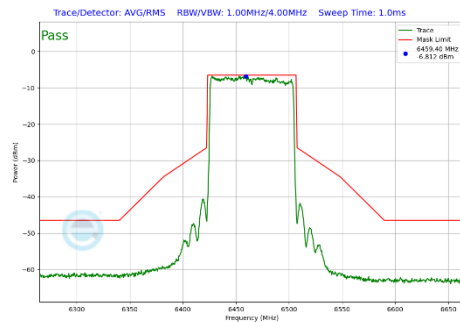
Plot 7-299 In-Band Emission Plot Antenna 5T (80MHz BW 802.11be(SU) (UNII Band 6) - Ch.103)
