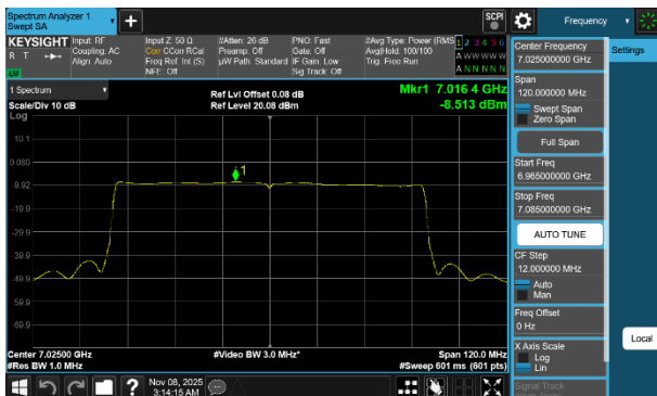
Plot 7-275 PSD SDM Diversity Antenna 5T (80MHz BW 802.11be(SU) - Ch.215)
