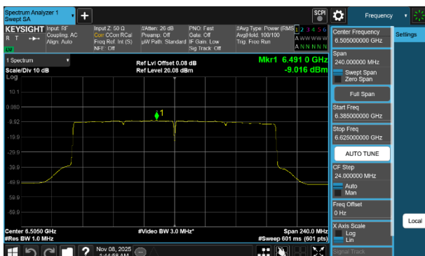
Plot 7-260 PSD SDM Diversity Antenna 5T (160MHz BW 802.11be(SU) - Ch.111)
