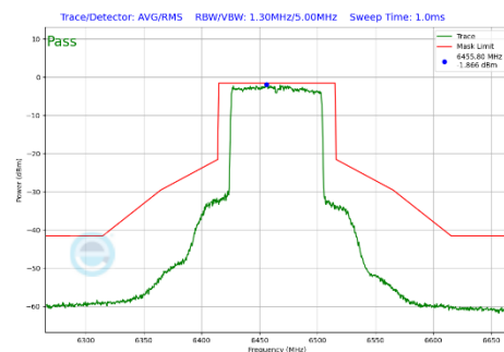
Plot 7-327 In-Band Emission Plot Antenna 3b (80MHz BW 802.11be(SU) (UNII Band 6) - Ch.103)
