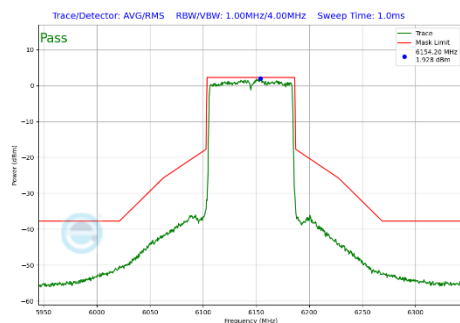
Plot 7-283 In-Band Emission Plot Antenna 5T (80MHz BW 802.11be(SU) (UNII Band 5) - Ch.39)
