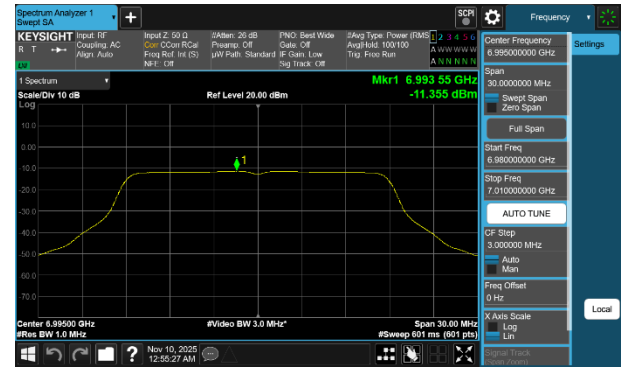
Plot 7-277 PSD CDD Diversity Antenna 1b (20MHz BW 802.11a - Ch.209)
