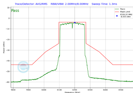
Plot 7-296 In-Band Emission Plot Antenna 5T (160MHz BW 802.11be(SU) (UNII Band 5) - Ch.47)
