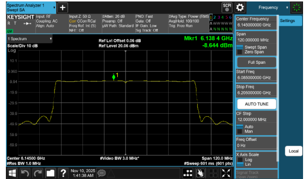
Plot 7-255 PSD SDM Diversity Antenna 1b (80MHz BW 802.11be(SU) - Ch.39)
