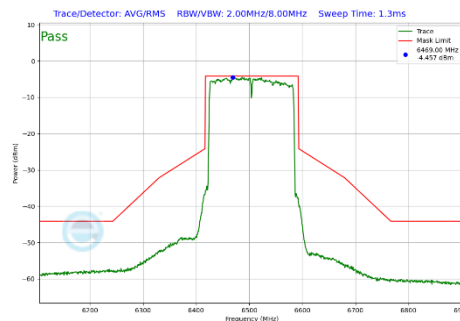
Plot 7-300 In-Band Emission Plot Antenna 5T (160MHz BW 802.11be(SU) (UNII Band 6) - Ch.111)
