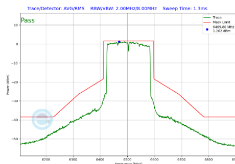
Plot 7-288 In-Band Emission Plot Antenna 5T (160MHz BW 802.11be(SU) (UNII Band 6) - Ch.111)
