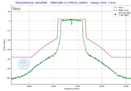
Plot 7-285 In-Band Emission Plot Antenna 5T (20MHz BW 802.11a (UNII Band 6) - Ch.113)
