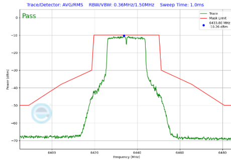
Plot 7-297 In-Band Emission Plot Antenna 5T (20MHz BW 802.11a (UNII Band 6) - Ch.97)
