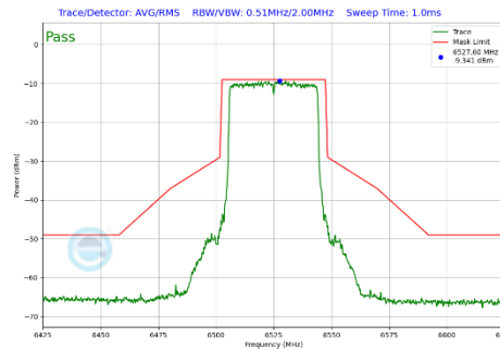
Plot 7-298 In-Band Emission Plot Antenna 5T (40MHz BW 802.11be(SU) (UNII Band 6) - Ch.115)
