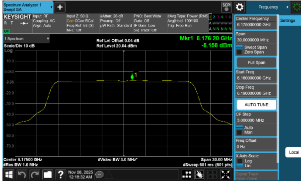
Plot 7-249 PSD SDM Diversity Antenna 5T (20MHz BW 802.11be(SU) - Ch.45)
