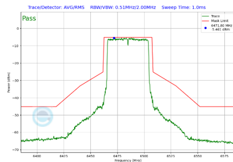
Plot 7-354 In-Band Emission Plot Antenna 1b (40MHz BW 802.11be(SU) (UNII Band 6) - Ch.107)
