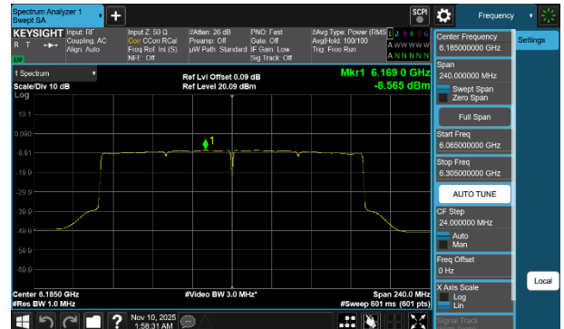
Plot 7-256 PSD SDM Diversity Antenna 1b (160MHz BW 802.11be(SU) - Ch.47)
