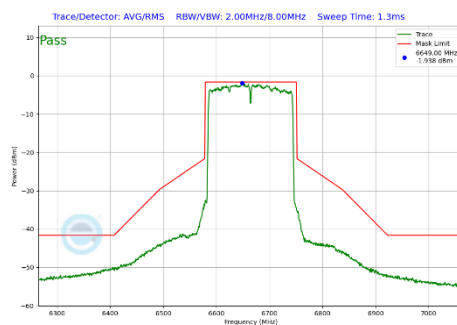
Plot 7-320 In-Band Emission Plot Antenna 3b (160MHz BW 802.11be(SU) (UNII Band 7) - Ch.143)
