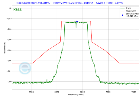
Plot 7-305 In-Band Emission Plot Antenna 5T (20MHz BW 802.11a (UNII Band 8) - Ch.209)
