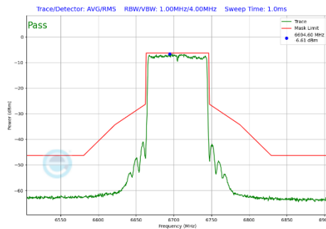
Plot 7-303 In-Band Emission Plot Antenna 5T (80MHz BW 802.11be(SU) (UNII Band 7) - Ch.151)
