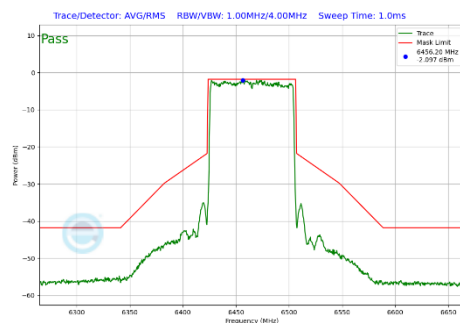
Plot 7-315 In-Band Emission Plot Antenna 3b (80MHz BW 802.11be(SU) (UNII Band 6) - Ch.103)
