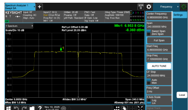
Plot 7-280 PSD SDM Diversity Antenna 1b (160MHz BW 802.11be(SU) - Ch.207)
