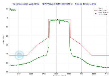
Plot 7-332 In-Band Emission Plot Antenna 3b (160MHz BW 802.11be(SU) (UNII Band 7) - Ch.175)
