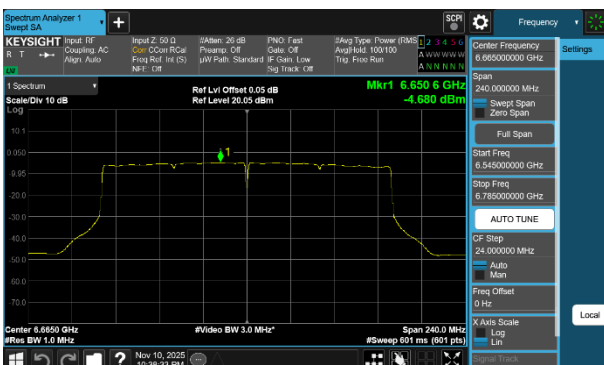
Plot 7-244 PSD CDD Diversity Antenna 5T (160MHz BW 802.11be(SU) - Ch.143)
