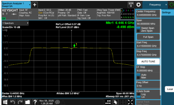
Plot 7-258 PSD SDM Diversity Antenna 5T (40MHz BW 802.11be(SU) - Ch.99)
