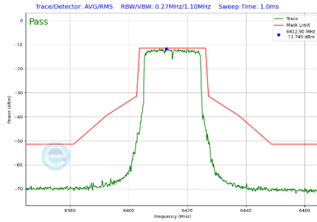
Plot 7-293 In-Band Emission Plot Antenna 5T (20MHz BW 802.11be(SU) (UNII Band 5) - Ch.93)
