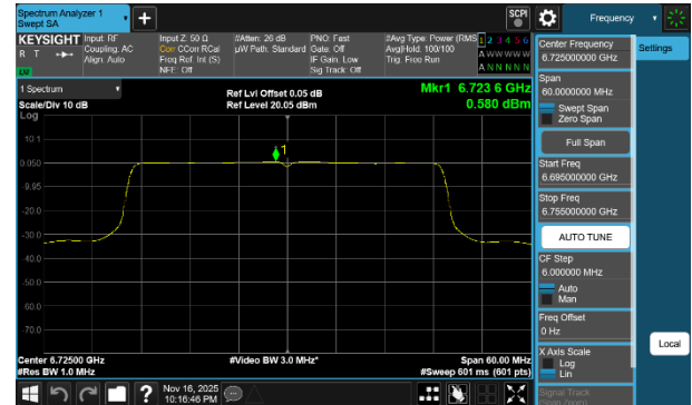
Plot 7-246 PSD CDD Diversity Antenna 1b (40MHz BW 802.11be(SU) - Ch.155)
