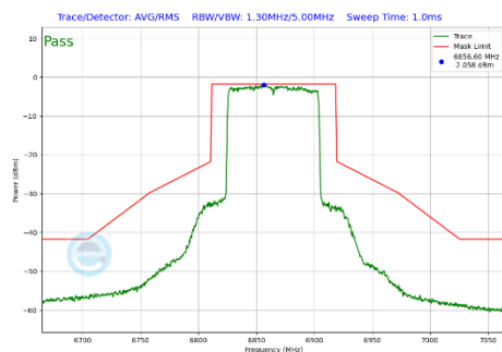
Plot 7-331 In-Band Emission Plot Antenna 3b (80MHz BW 802.11be(SU) (UNII Band 7) - Ch.183)
