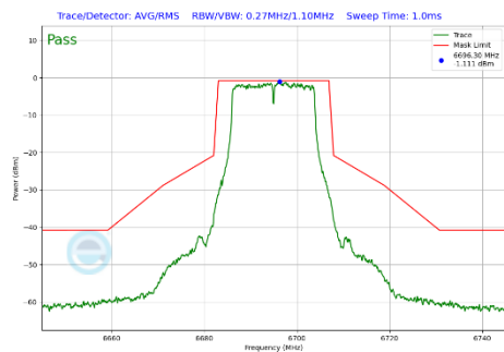
Plot 7-317 In-Band Emission Plot Antenna 3b (20MHz BW 802.11a (UNII Band 7) - Ch.149)
