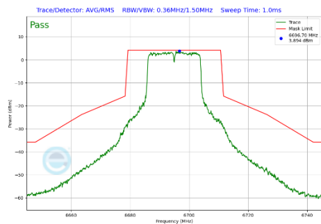
Plot 7-289 In-Band Emission Plot Antenna 5T (20MHz BW 802.11a (UNII Band 7) - Ch.149)
