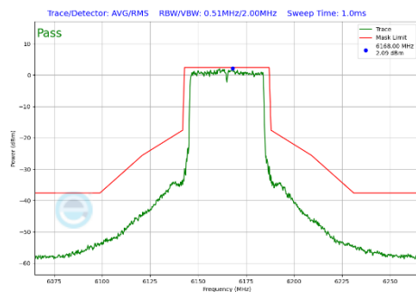
Plot 7-282 In-Band Emission Plot Antenna 5T (40MHz BW 802.11be(SU) (UNII Band 5) - Ch.43)
