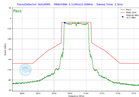
Plot 7-334 In-Band Emission Plot Antenna 3b (40MHz BW 802.11be(SU) (UNII Band 8) - Ch.227)
