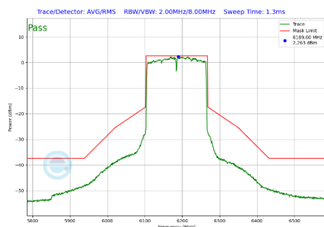
Plot 7-284 In-Band Emission Plot Antenna 5T (160MHz BW 802.11be(SU) (UNII Band 5) - Ch.47)
