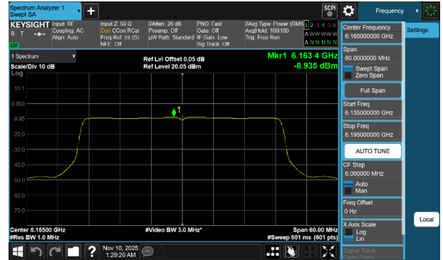
Plot 7-254 PSD SDM Diversity Antenna 1b (40MHz BW 802.11be(SU) - Ch.43)
