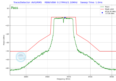
Plot 7-341 In-Band Emission Plot Antenna 1b (20MHz BW 802.11a (UNII Band 6) - Ch.113)
