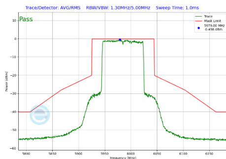
Plot 7-311 In-Band Emission Plot Antenna 3b (80MHz BW 802.11be(SU) (UNII Band 5) - Ch.7)
