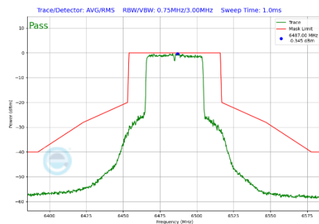
Plot 7-314 In-Band Emission Plot Antenna 3b (40MHz BW 802.11be(SU) (UNII Band 6) - Ch.107)
