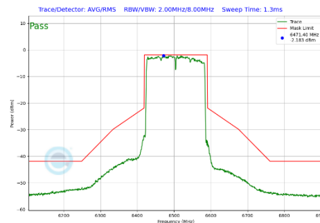
Plot 7-328 In-Band Emission Plot Antenna 3b (160MHz BW 802.11be(SU) (UNII Band 6) - Ch.111)
