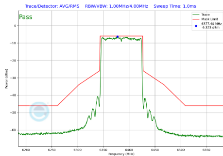
Plot 7-295 In-Band Emission Plot Antenna 5T (80MHz BW 802.11be(SU) (UNII Band 5) - Ch.87)
