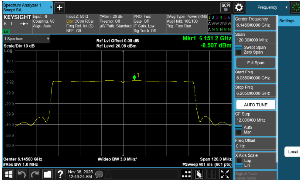
Plot 7-251 PSD SDM Diversity Antenna 5T (80MHz BW 802.11be(SU) - Ch.39)
