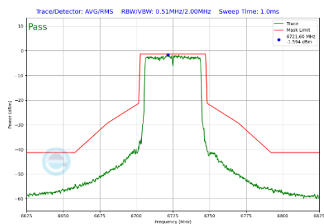
Plot 7-318 In-Band Emission Plot Antenna 3b (40MHz BW 802.11be(SU) (UNII Band 7) - Ch.155)
