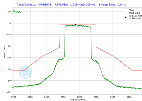
Plot 7-319 In-Band Emission Plot Antenna 3b (80MHz BW 802.11be(SU) (UNII Band 7) - Ch.119)
