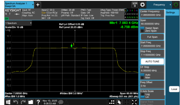
Plot 7-278 PSD SDM Diversity Antenna 1b (40MHz BW 802.11be(SU) - Ch.227)
